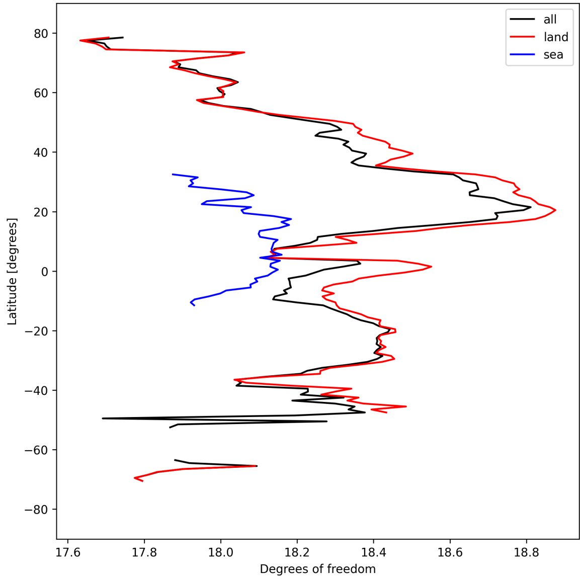
Figure 19: Zonal average of “Degrees of freedom” for 2025-09-13 to 2025-09-15.
