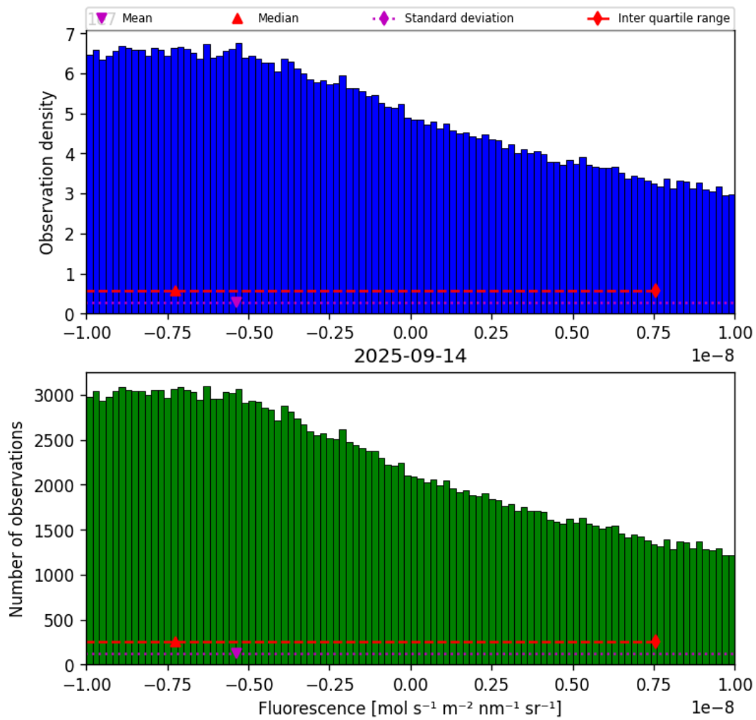
Figure 32: Histogram of “Fluorescence” for 2025-09-13 to 2025-09-15
