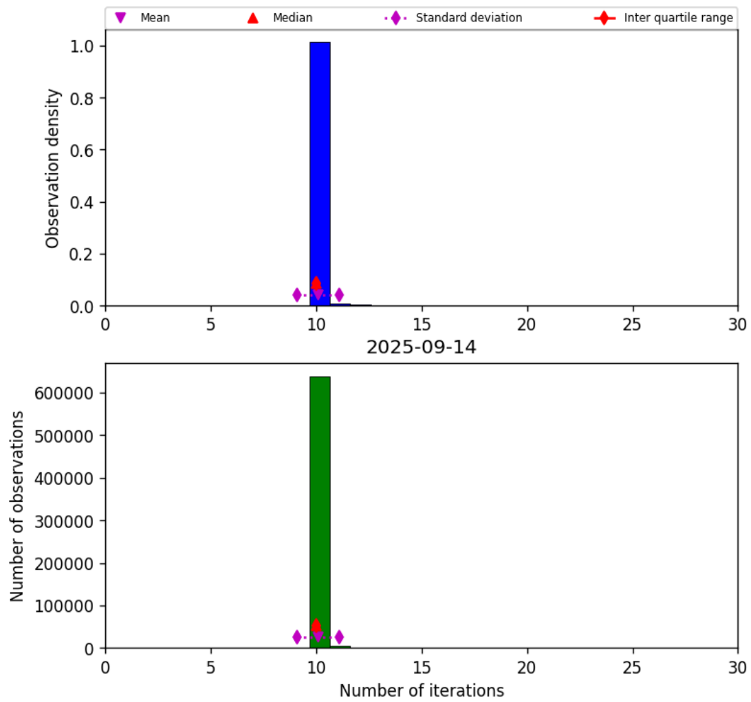
Figure 31: Histogram of “Number of iterations” for 2025-09-13 to 2025-09-15
