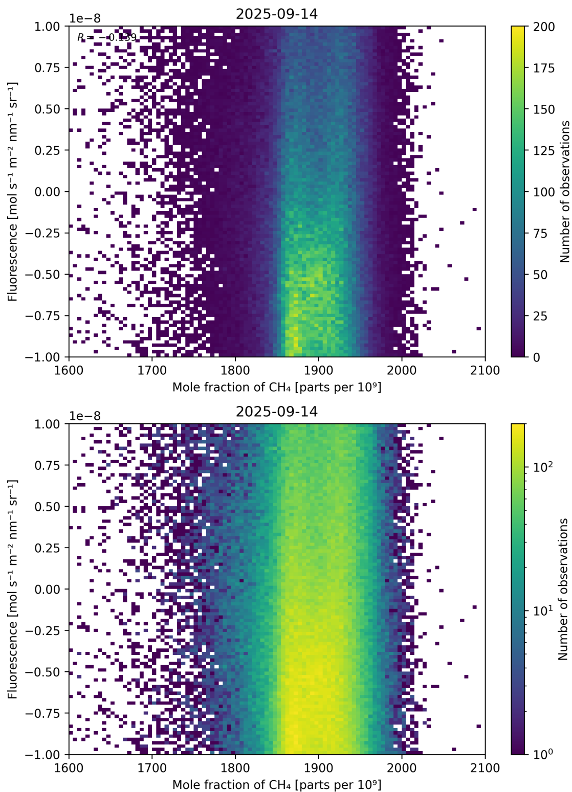
Figure 73: Scatter density plot of “Mole fraction of \text{CH}_4 ” against “Fluorescence” for 2025-09-13 to 2025-09-15.
