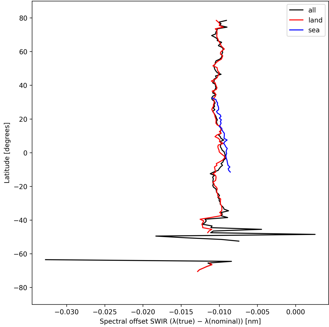
Figure 16: Zonal average of “Spectral offset SWIR ( \lambda_{\text{true}} - \lambda_{\text{nominal}} )” for 2025-09-13 to 2025-09-15.
