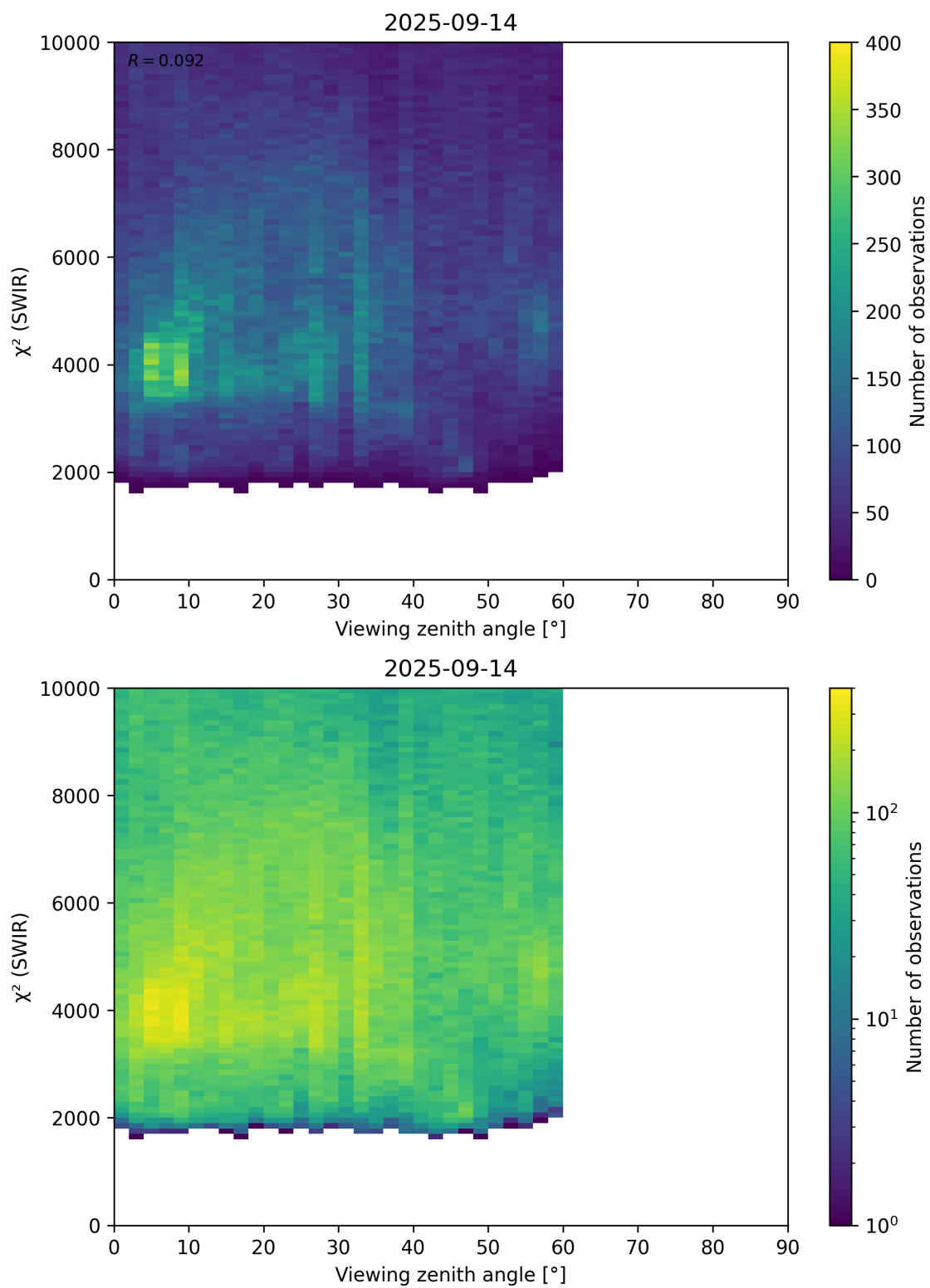
Figure 106: Scatter density plot of “Viewing zenith angle” against “ \chi^2 (SWIR)” for 2025-09-13 to 2025-09-15.
