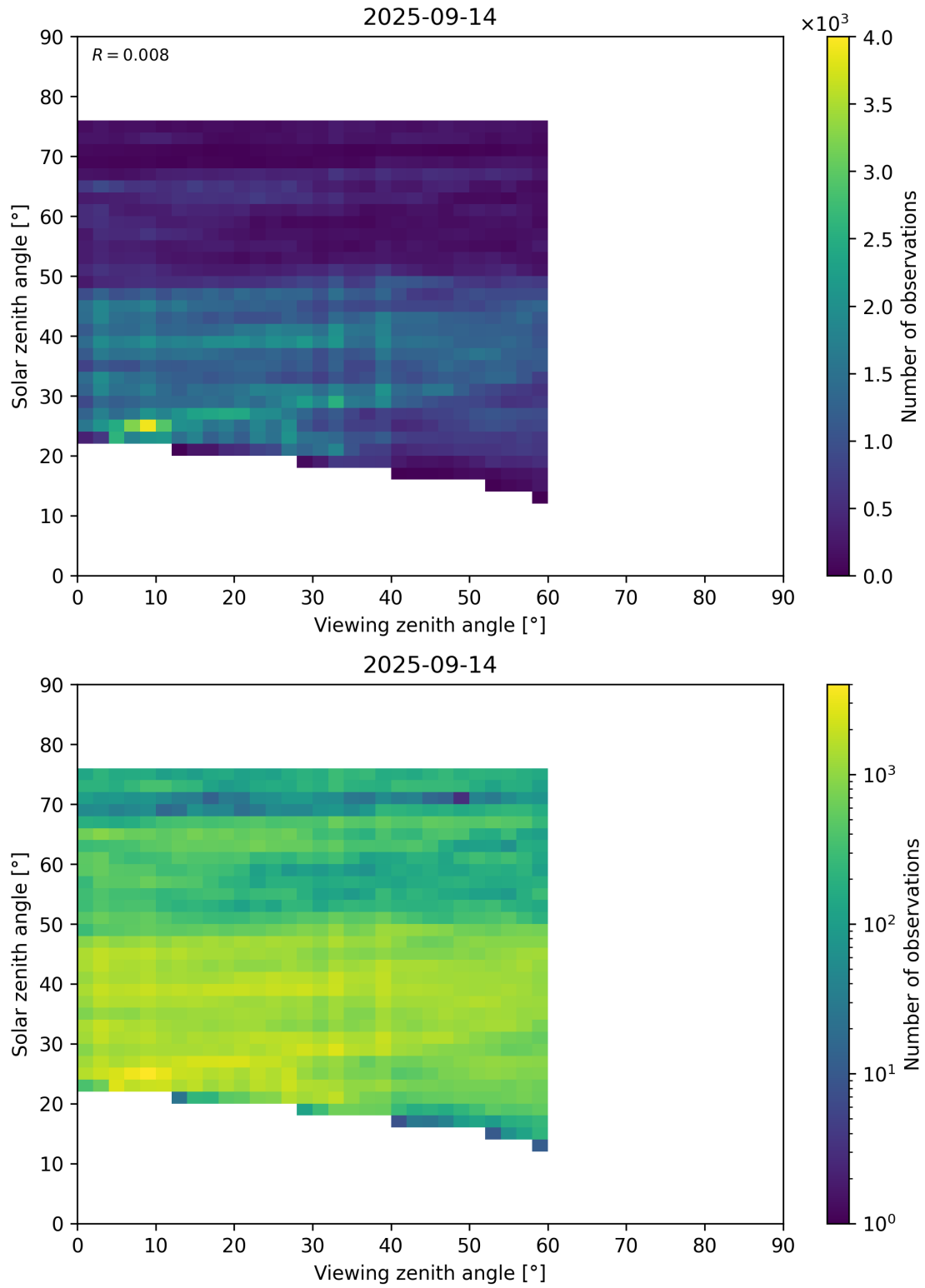
Figure 115: Scatter density plot of “Viewing zenith angle” against “Solar zenith angle” for 2025-09-13 to 2025-09-15.
