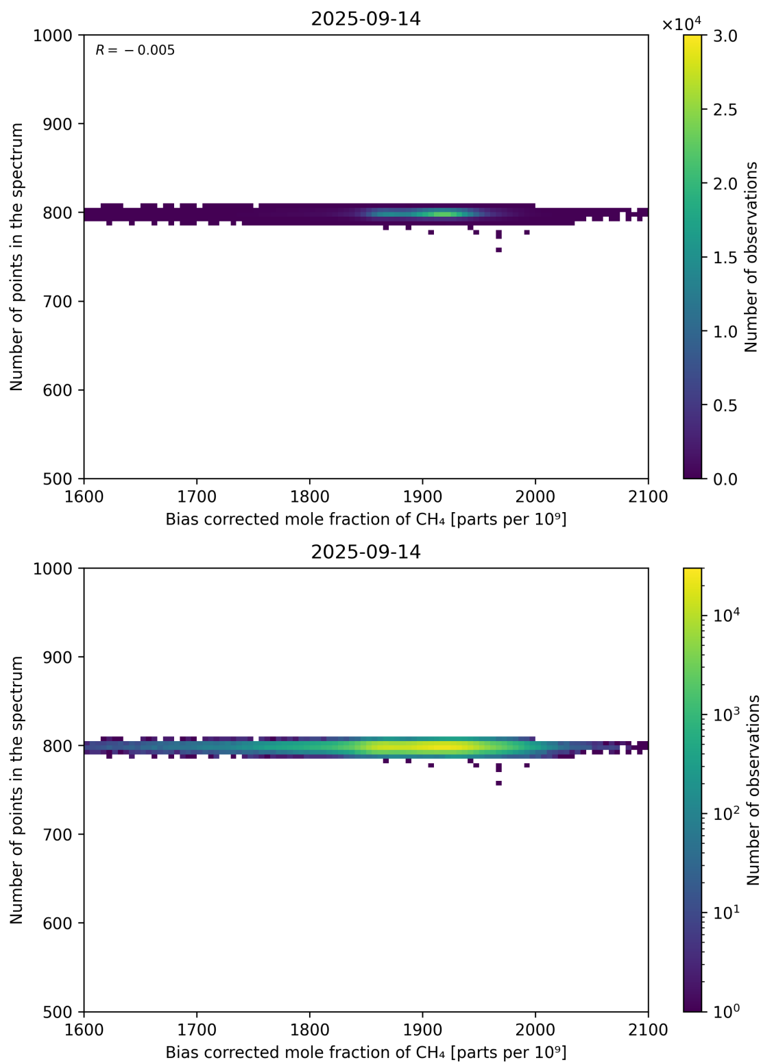
Figure 68: Scatter density plot of “Bias corrected mole fraction of CH 4 ” against “Number of points in the spectrum” for 2025-09-13 to 2025-09-15.
