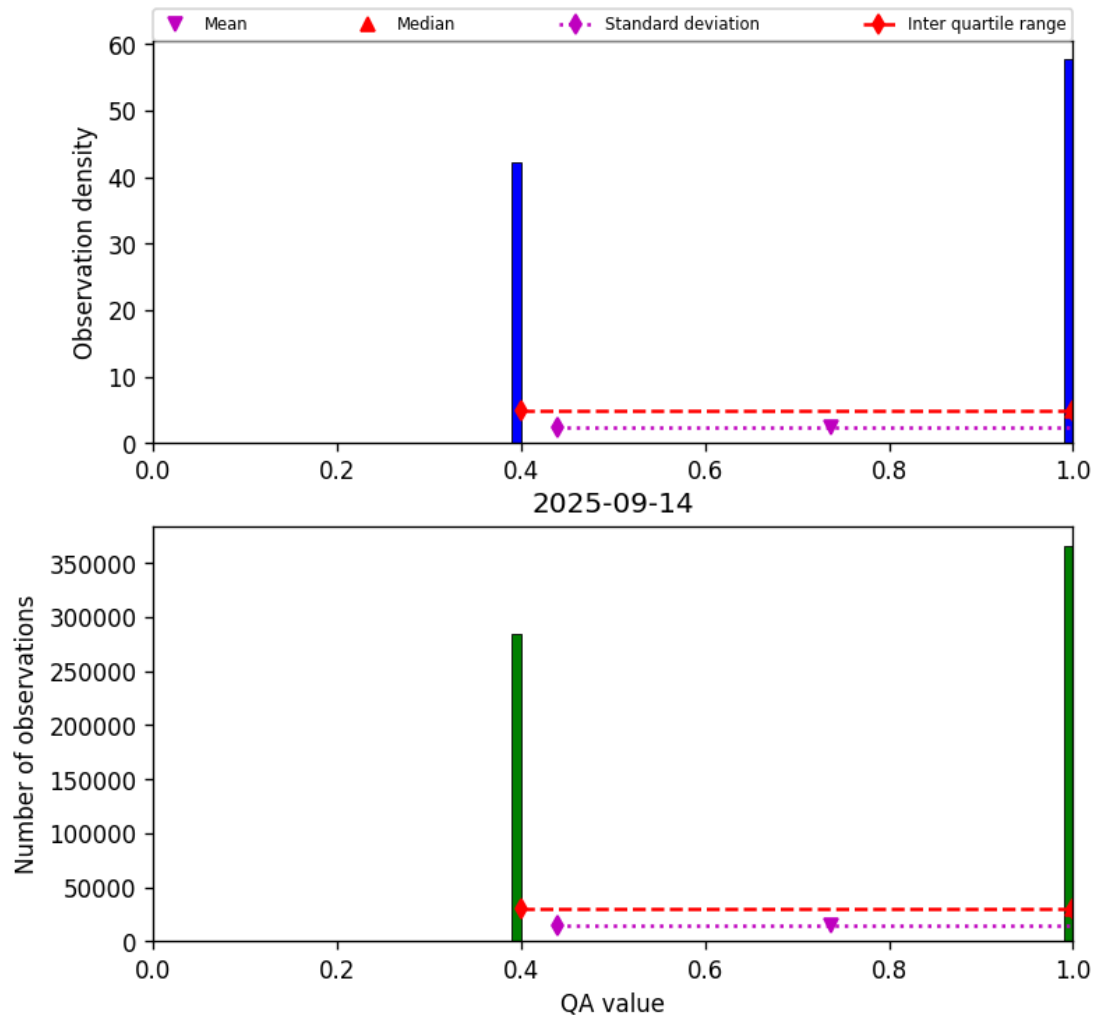
Figure 22: Histogram of “QA value” for 2025-09-13 to 2025-09-15
