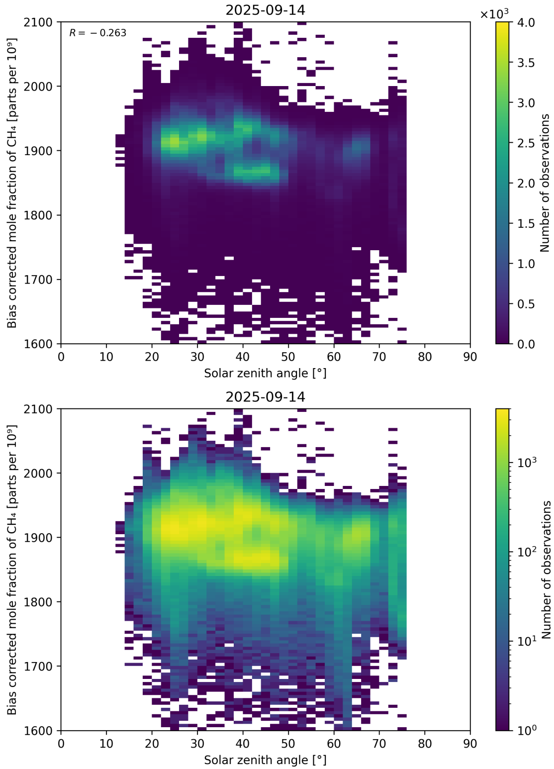
Figure 100: Scatter density plot of “Solar zenith angle” against “Bias corrected mole fraction of \text{CH}_4 ” for 2025-09-13 to 2025-09-15.
