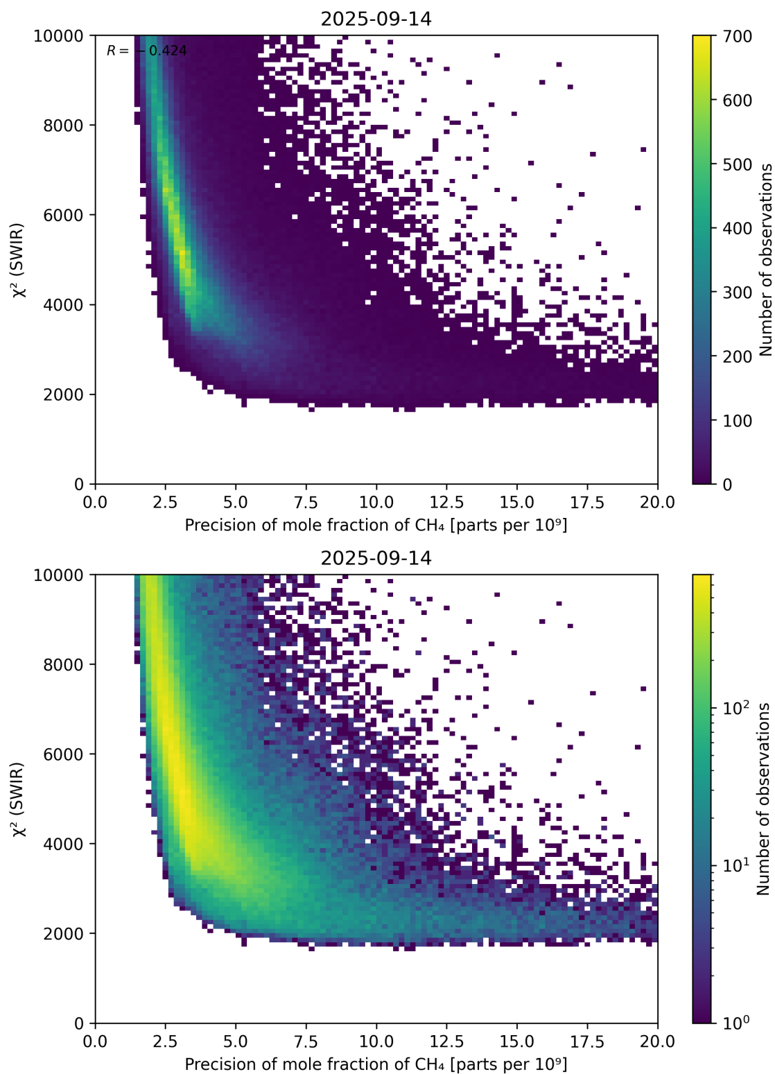
Figure 79: Scatter density plot of “Precision of mole fraction of \text{CH}_4 ” against “ \chi^2 (SWIR)” for 2025-09-13 to 2025-09-15.
