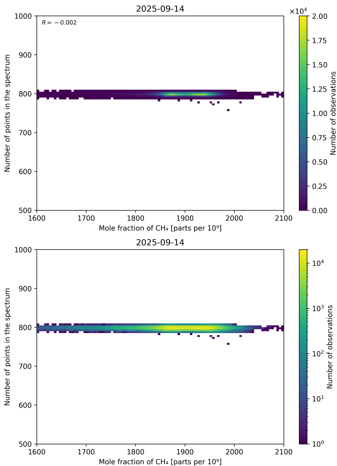
Figure 77: Scatter density plot of “Mole fraction of CH 4 ” against “Number of points in the spectrum” for 2025-09-13 to 2025-09-15.
