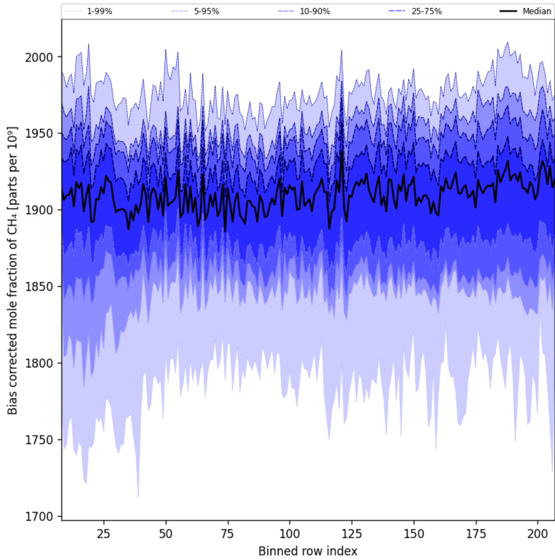
Figure 36: Along track statistics of “Bias corrected mole fraction of CH 4 ” for 2025-09-13 to 2025-09-15
