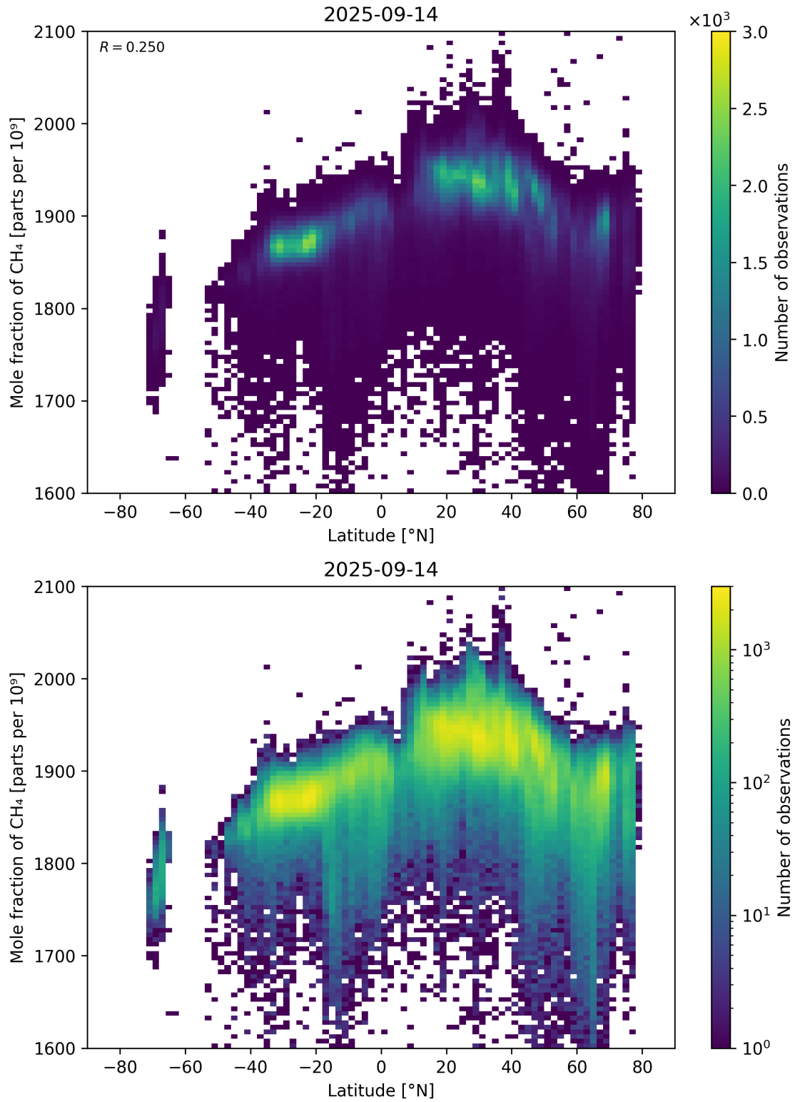
Figure 57: Scatter density plot of “Latitude” against “Mole fraction of CH 4 ” for 2025-09-13 to 2025-09-15.
