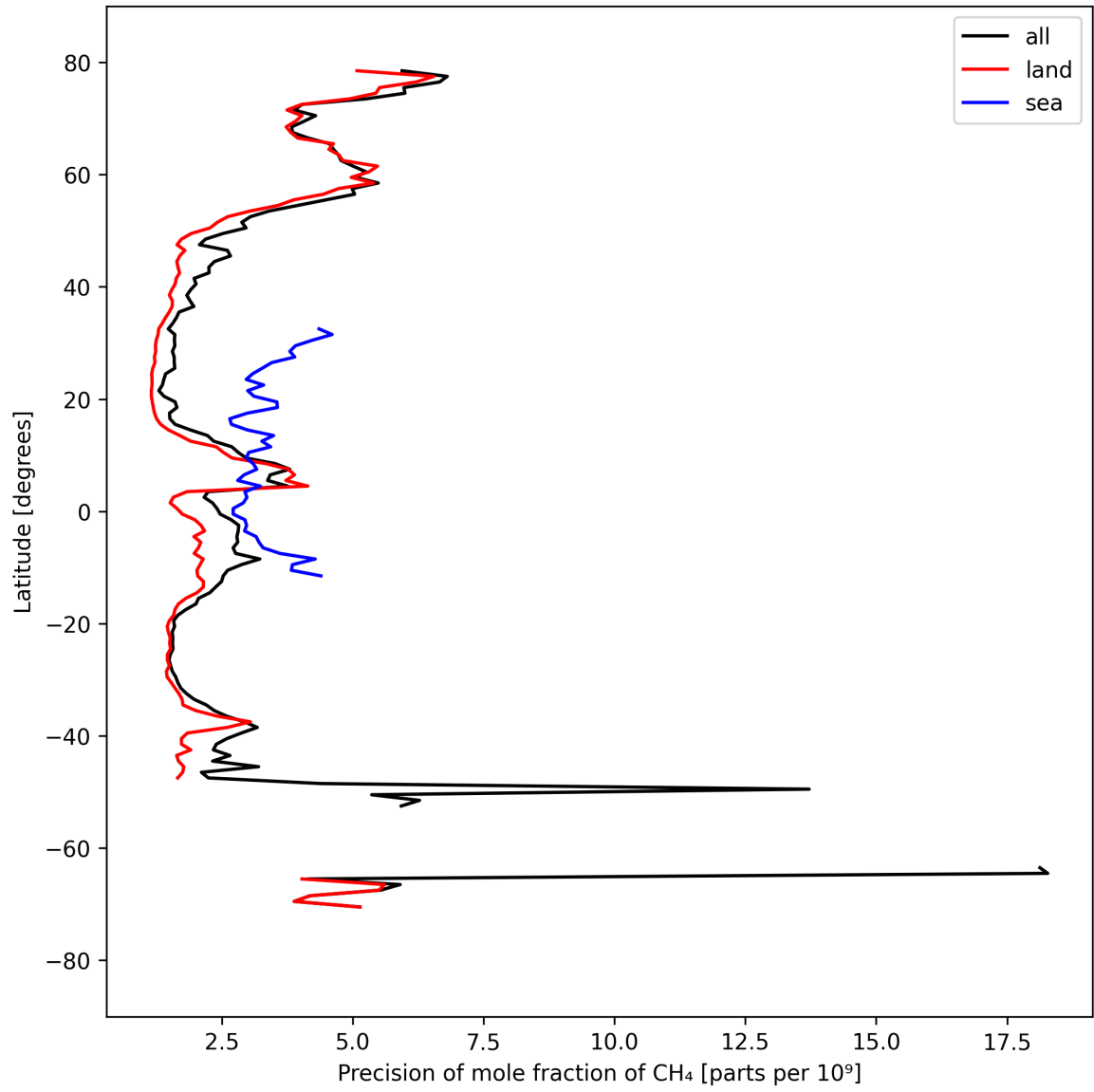
Figure 13: Zonal average of “Precision of mole fraction of CH 4 ” for 2025-09-13 to 2025-09-15.
