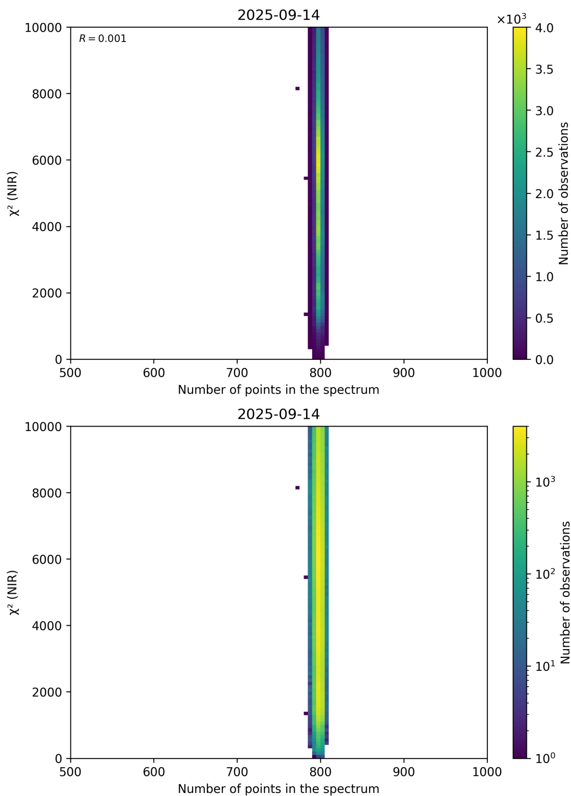
Figure 88: Scatter density plot of “Number of points in the spectrum” against “ \chi^2 (NIR)” for 2025-09-13 to 2025-09-15.
