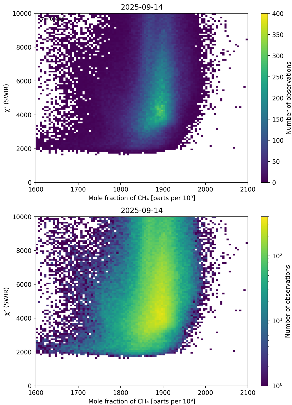
Figure 71: Scatter density plot of “Mole fraction of CH 4 ” against “ \chi^2 (SWIR)” for 2025-09-13 to 2025-09-15.
