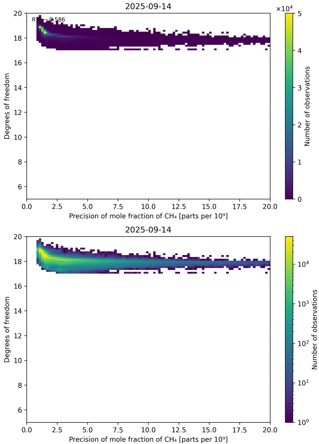
Figure 80: Scatter density plot of “Precision of mole fraction of CH 4 ” against “Degrees of freedom” for 2025-09-13 to 2025-09-15.
