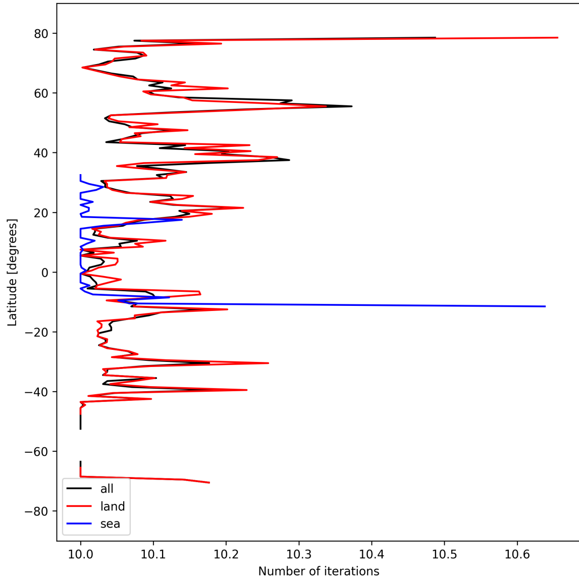
Figure 20: Zonal average of “Number of iterations” for 2025-09-13 to 2025-09-15.
