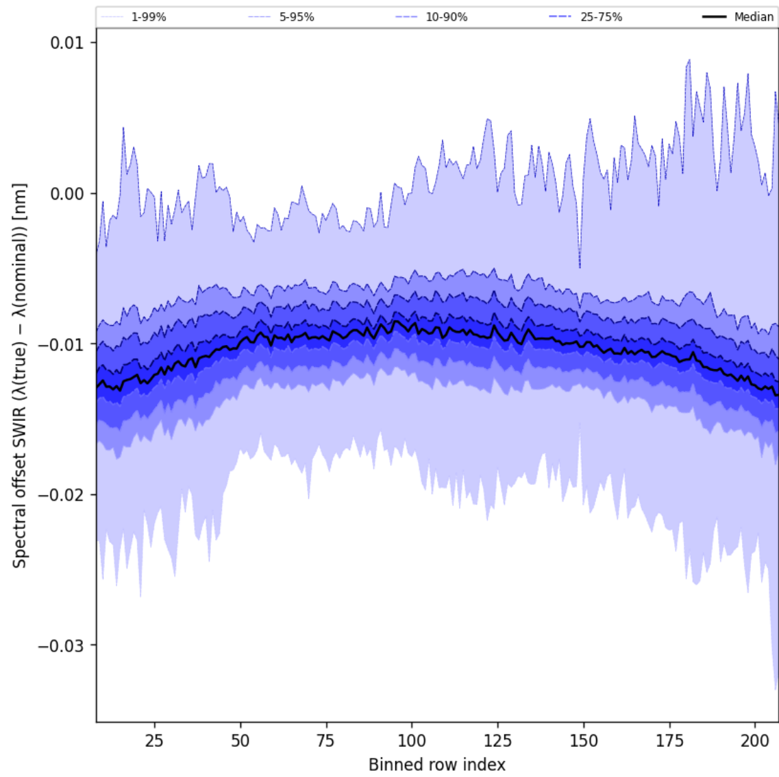
Figure 38: Along track statistics of “Spectral offset SWIR ( \lambda_{\text{true}} - \lambda_{\text{nominal}} )” for 2025-09-13 to 2025-09-15
