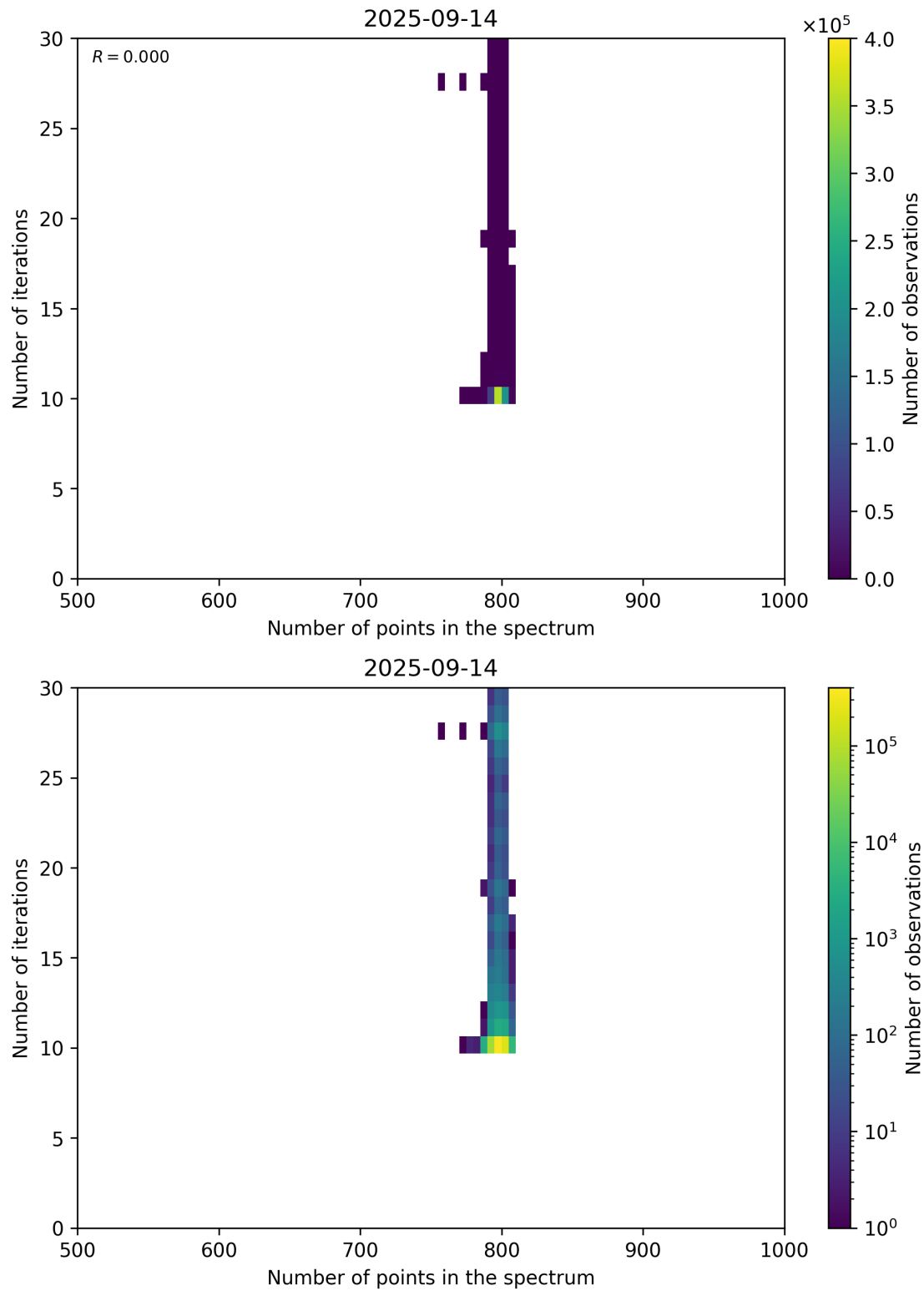
Figure 92: Scatter density plot of “Number of points in the spectrum” against “Number of iterations” for 2025-09-13 to 2025-09-15.
