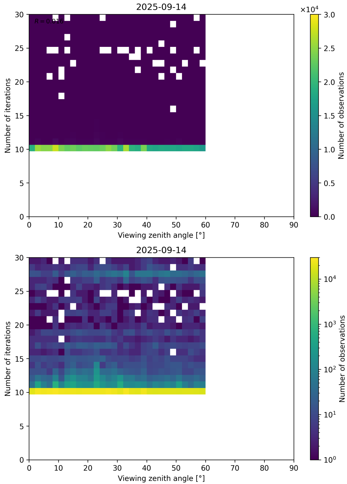
Figure 113: Scatter density plot of “Viewing zenith angle” against “Number of iterations” for 2025-09-13 to 2025-09-15.
