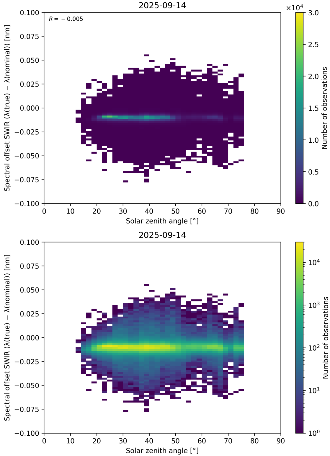
Figure 104: Scatter density plot of “Solar zenith angle” against “Spectral offset SWIR ( \lambda_{\text{true}} - \lambda_{\text{nominal}} )” for 2025-09-13 to 2025-09-15.
