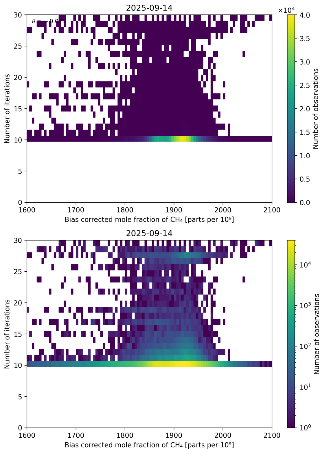
Figure 67: Scatter density plot of “Bias corrected mole fraction of CH 4 ” against “Number of iterations” for 2025-09-13 to 2025-09-15.
