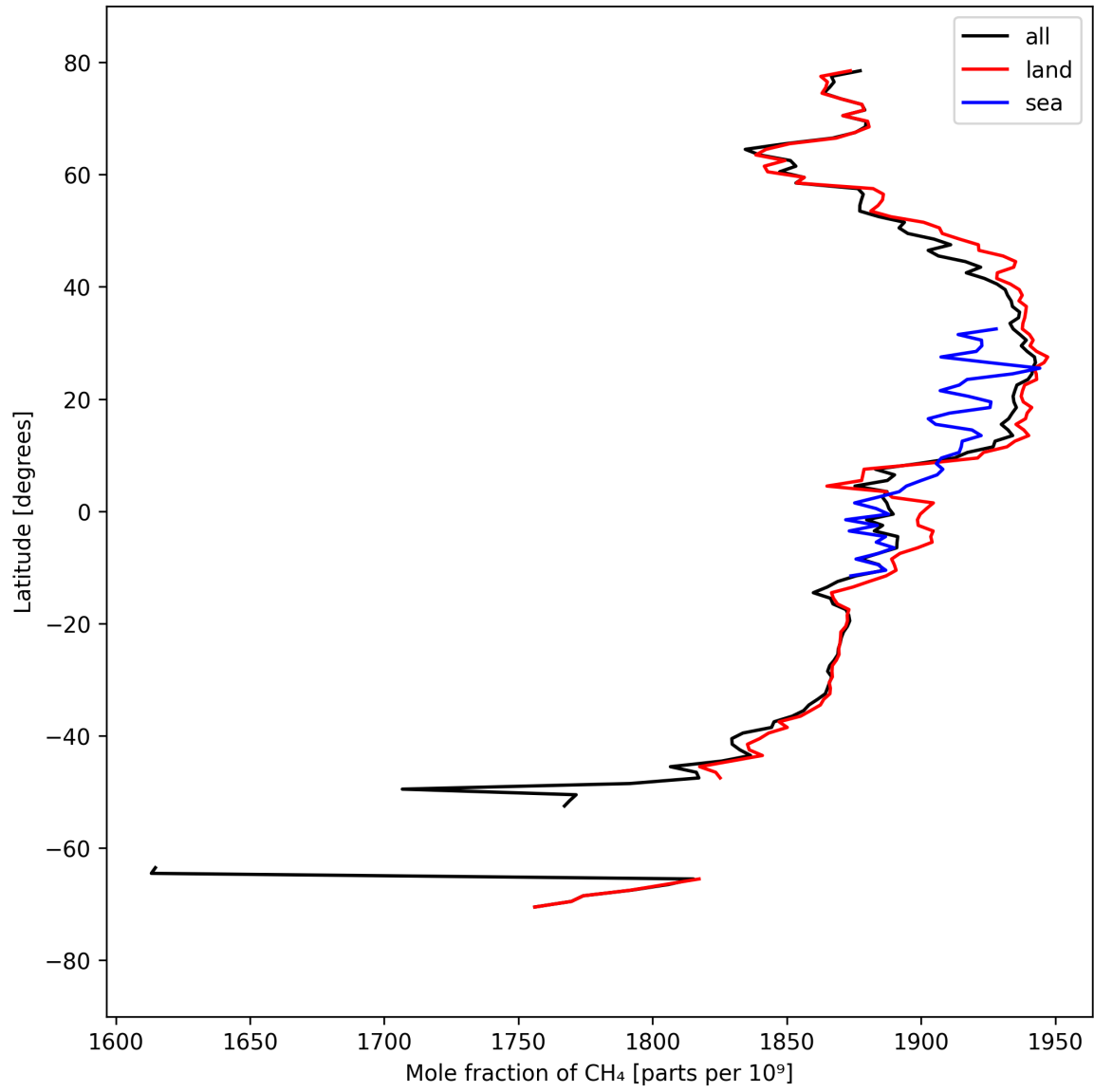
Figure 12: Zonal average of “Mole fraction of \text{CH}_4 ” for 2025-09-13 to 2025-09-15.
