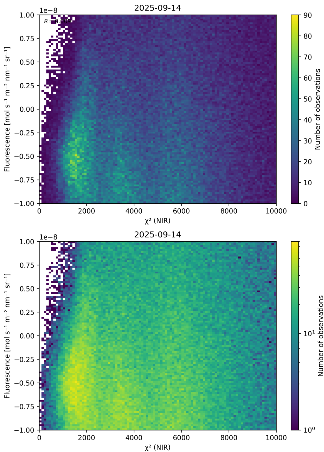
Figure 45: Scatter density plot of “ \chi^2 (NIR)” against “Fluorescence” for 2025-09-13 to 2025-09-15.
