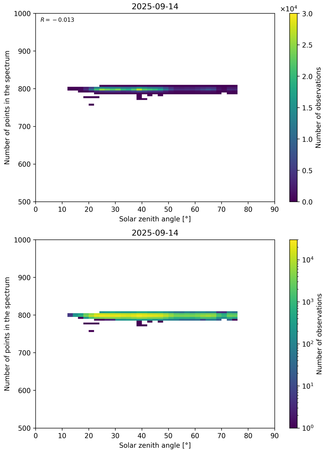
Figure 103: Scatter density plot of “Solar zenith angle” against “Number of points in the spectrum” for 2025-09-13 to 2025-09-15.
