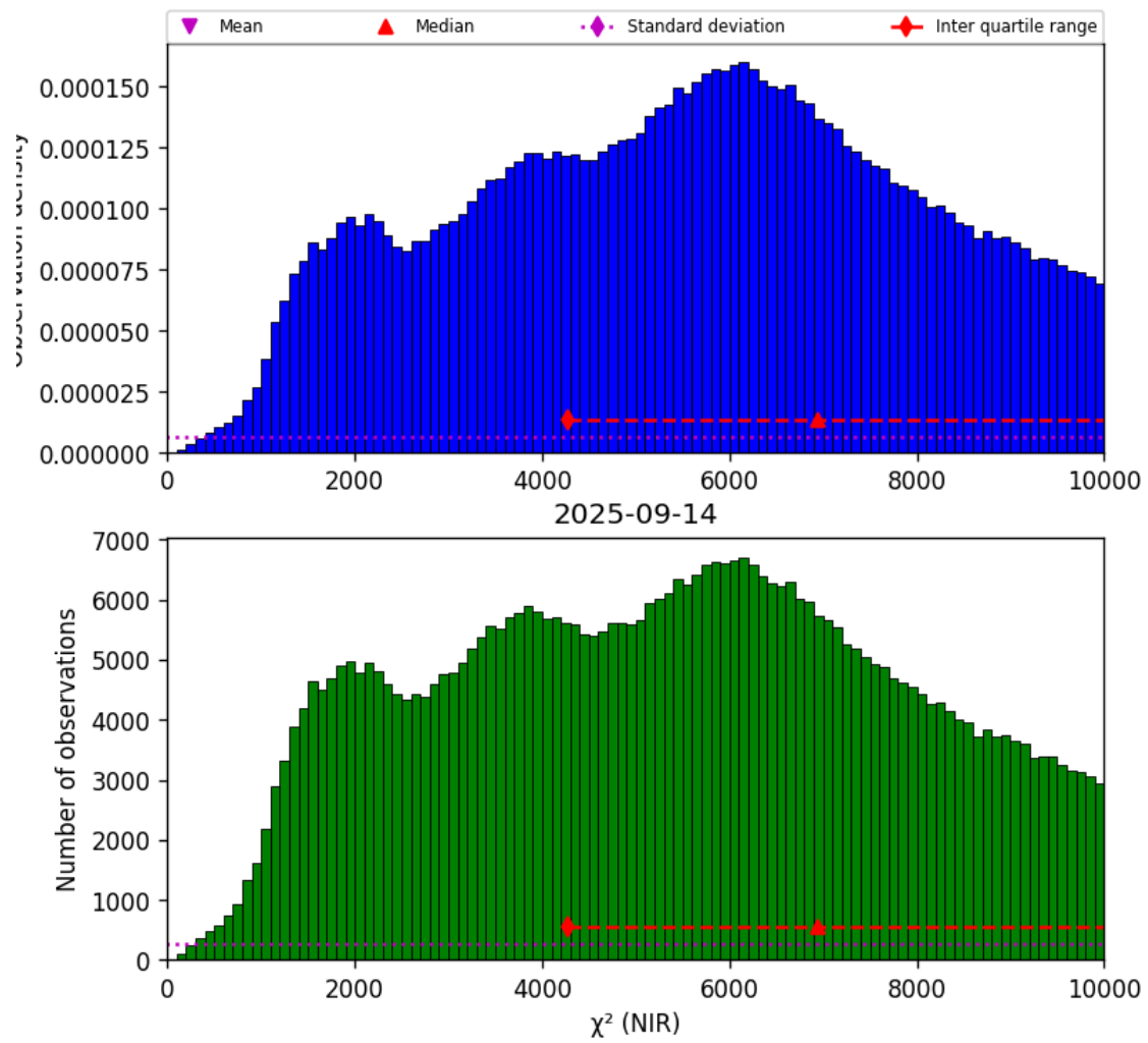
Figure 29: Histogram of “ \chi^2 (NIR)” for 2025-09-13 to 2025-09-15
