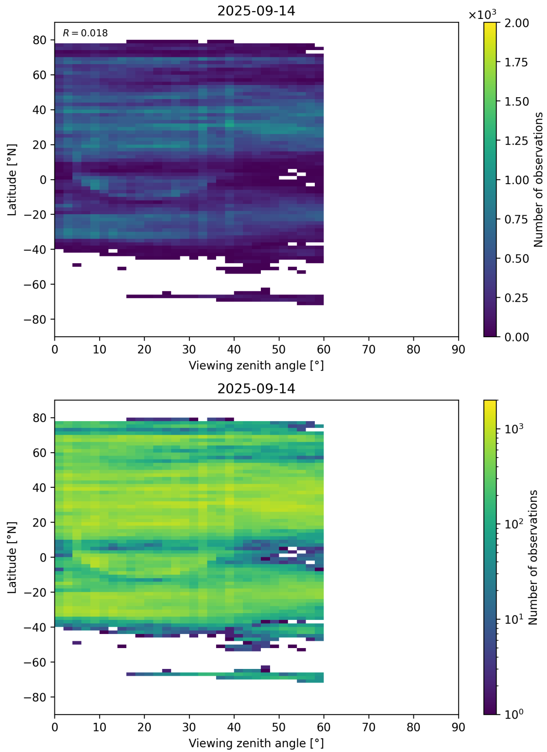
Figure 109: Scatter density plot of “Viewing zenith angle” against “Latitude” for 2025-09-13 to 2025-09-15.
