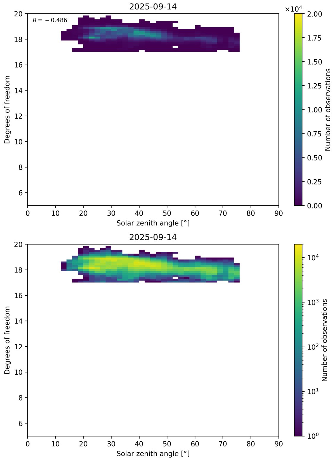
Figure 96: Scatter density plot of “Solar zenith angle” against “Degrees of freedom” for 2025-09-13 to 2025-09-15.
