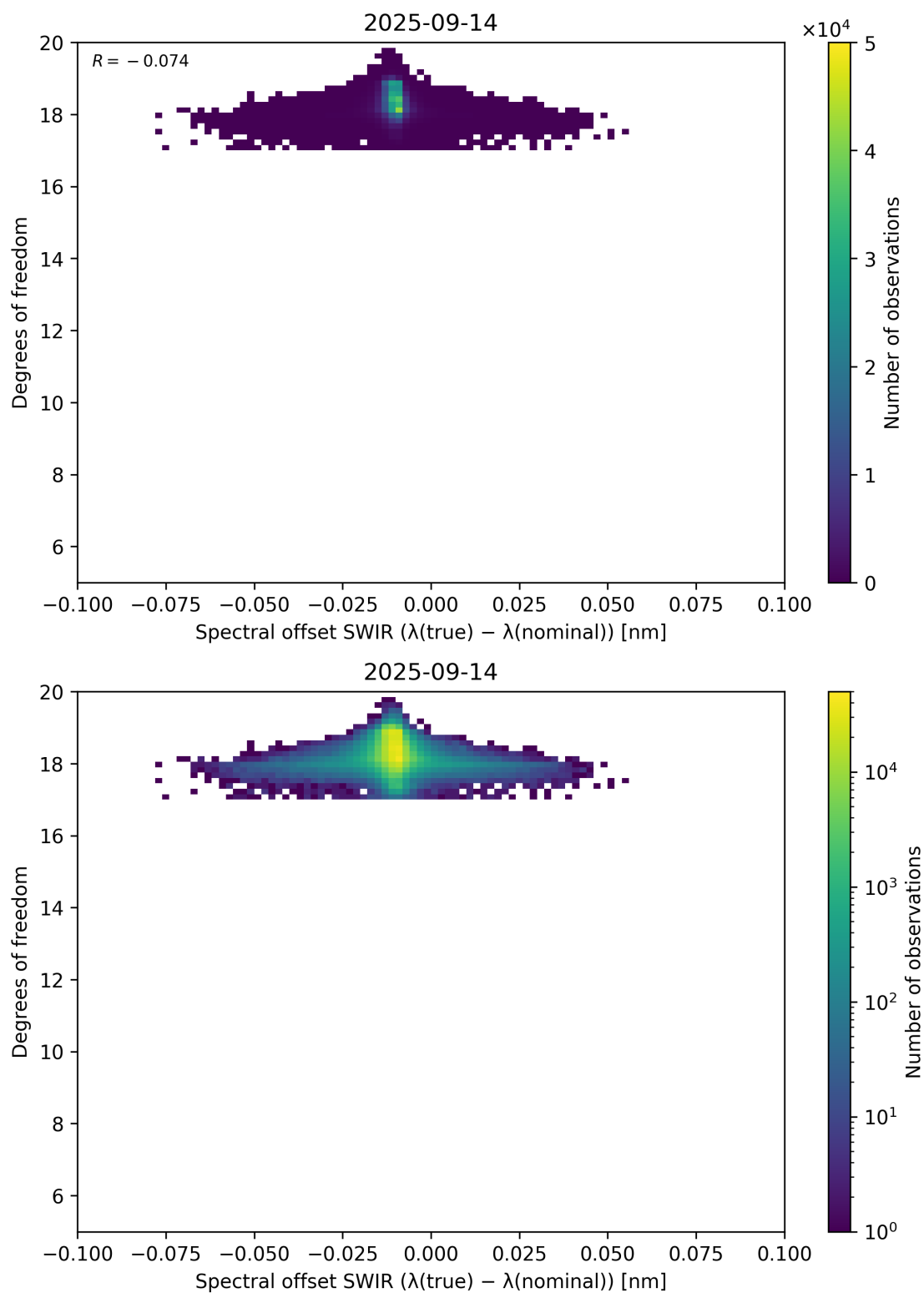
Figure 119: Scatter density plot of “Spectral offset SWIR ( \lambda_{\text{true}} - \lambda_{\text{nominal}} )” against “Degrees of freedom” for 2025-09-13 to 2025-09-15.
