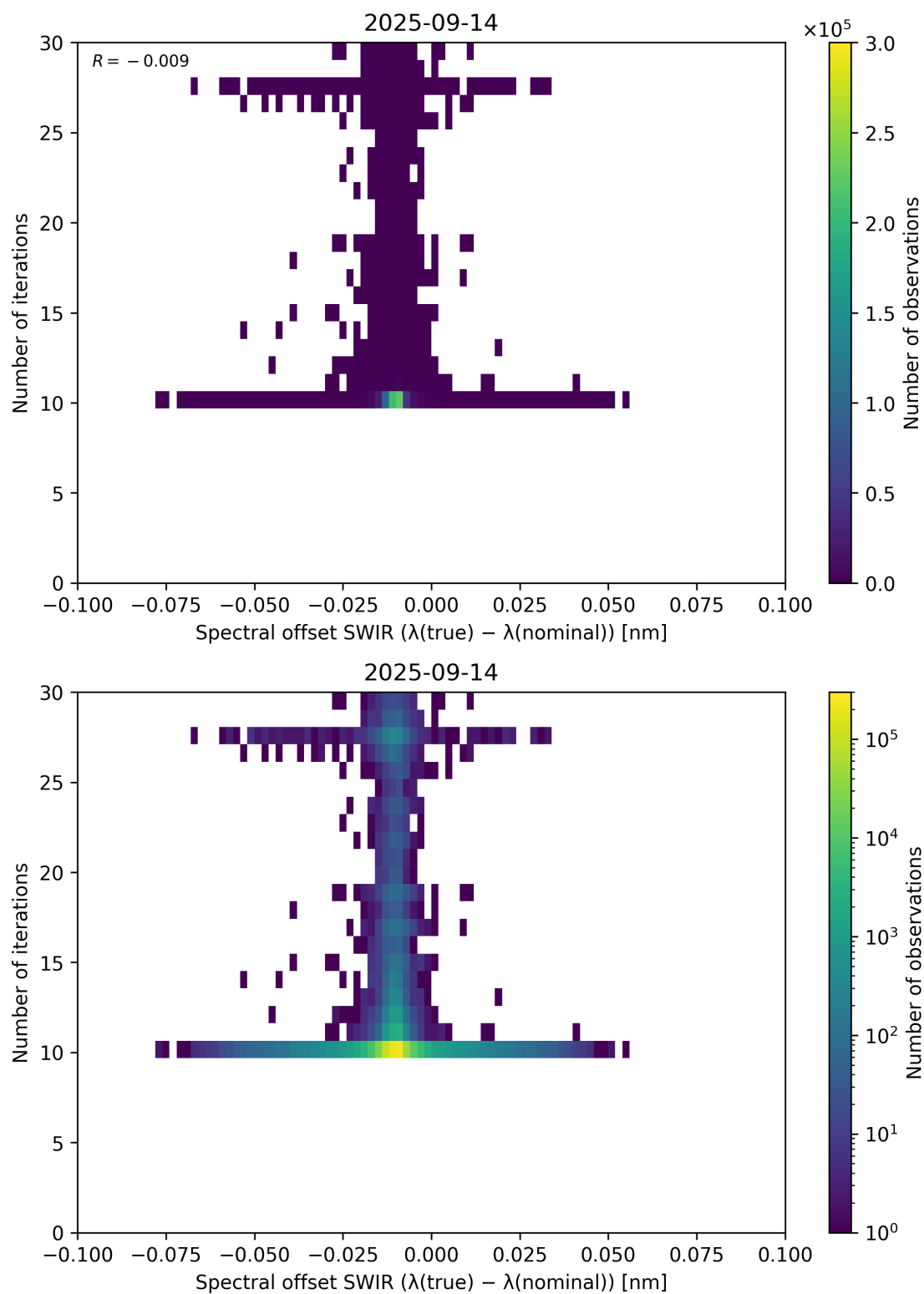
Figure 121: Scatter density plot of “Spectral offset SWIR ( \lambda_{\text{true}} - \lambda_{\text{nominal}} )” against “Number of iterations” for 2025-09-13 to 2025-09-15.
