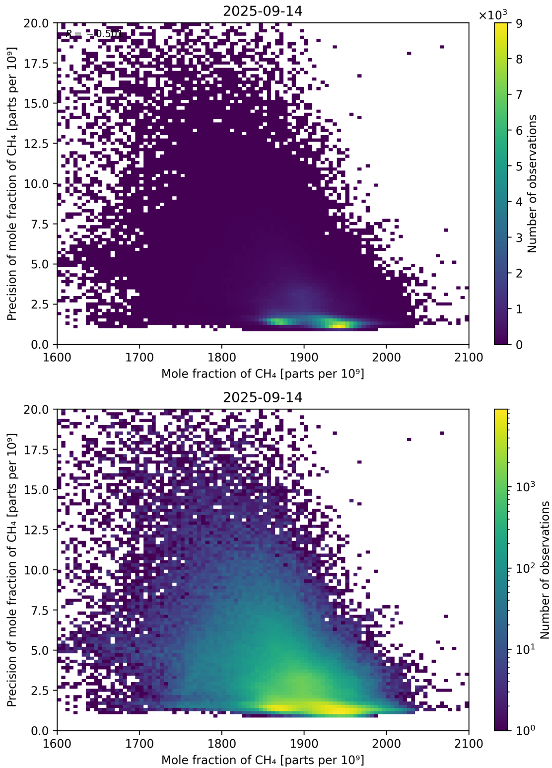
Figure 75: Scatter density plot of “Mole fraction of CH 4 ” against “Precision of mole fraction of CH 4 ” for 2025-09-13 to 2025-09-15.
