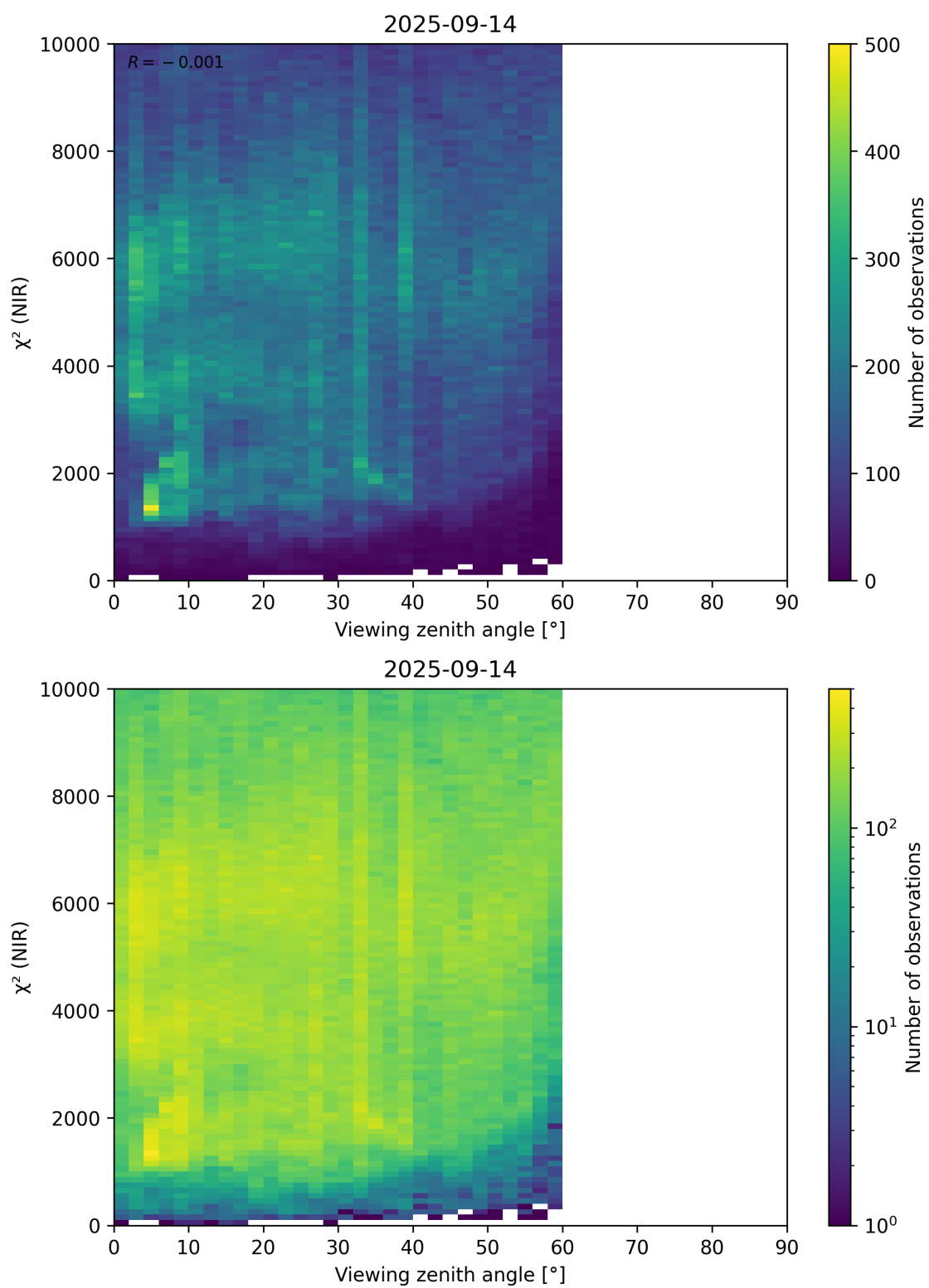
Figure 105: Scatter density plot of “Viewing zenith angle” against “ \chi^2 (NIR)” for 2025-09-13 to 2025-09-15.
