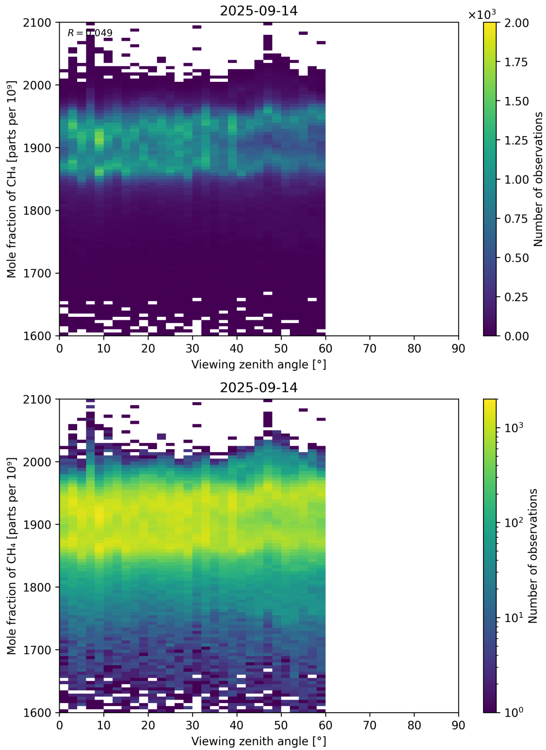
Figure 110: Scatter density plot of “Viewing zenith angle” against “Mole fraction of CH 4 ” for 2025-09-13 to 2025-09-15.
