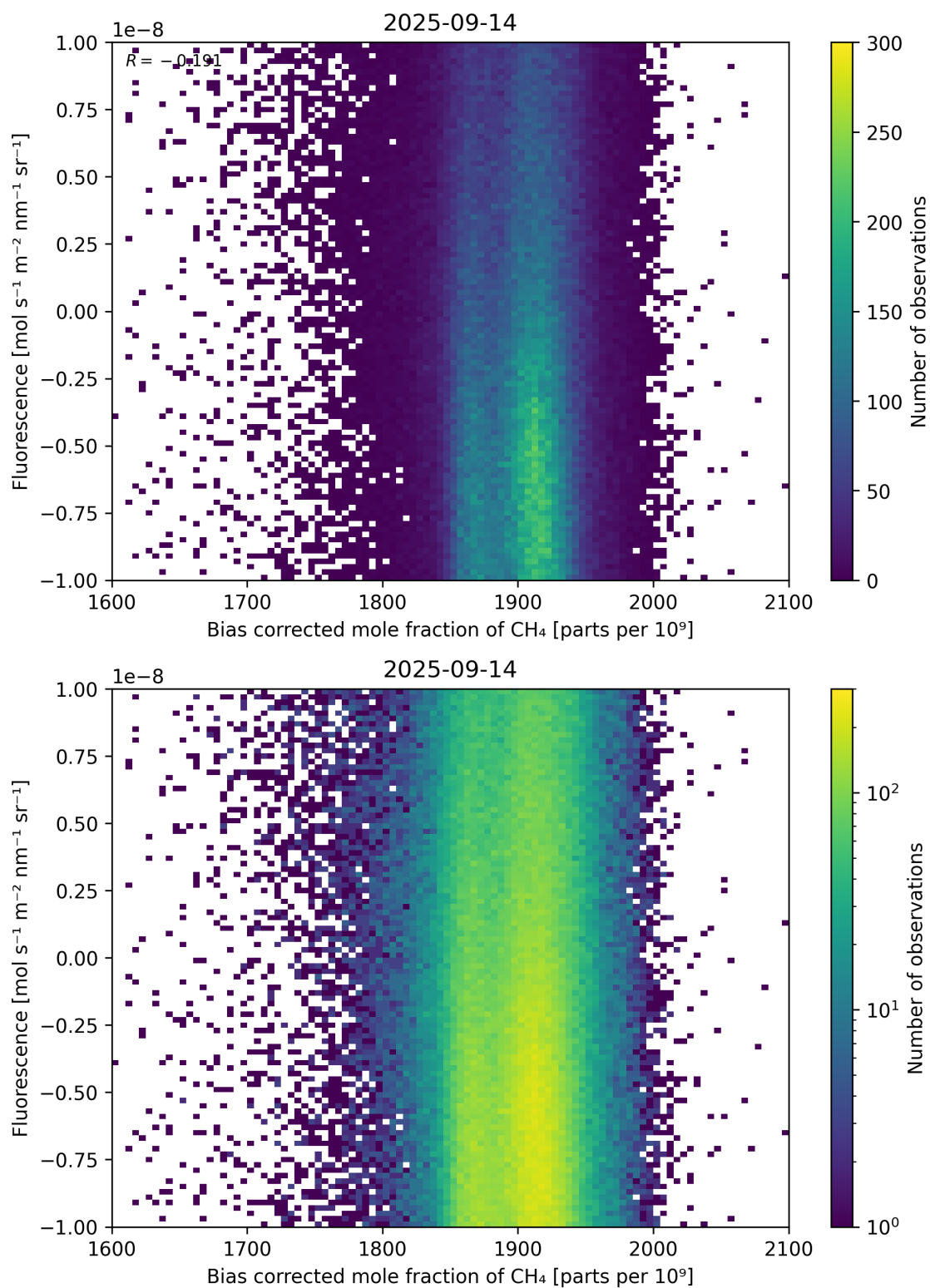
Figure 66: Scatter density plot of “Bias corrected mole fraction of \text{CH}_4 ” against “Fluorescence” for 2025-09-13 to 2025-09-15.
