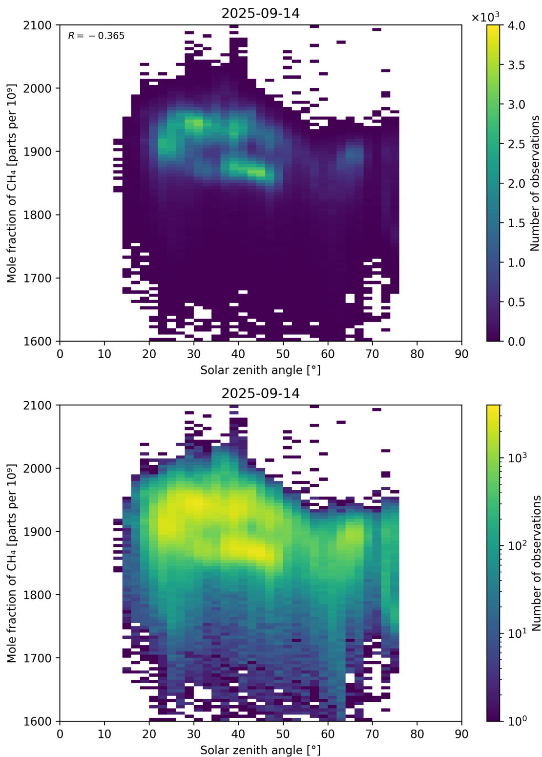
Figure 99: Scatter density plot of “Solar zenith angle” against “Mole fraction of CH 4 ” for 2025-09-13 to 2025-09-15.
