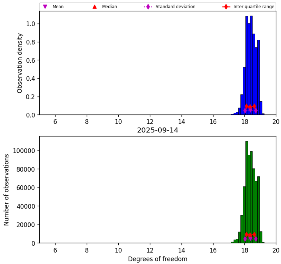
Figure 30: Histogram of “Degrees of freedom” for 2025-09-13 to 2025-09-15
