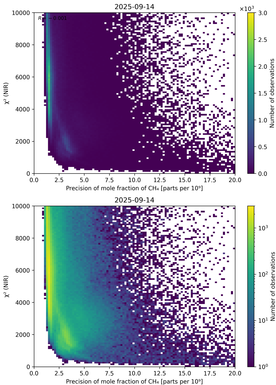
Figure 78: Scatter density plot of “Precision of mole fraction of CH 4 ” against “ \chi^2 (NIR)” for 2025-09-13 to 2025-09-15.
