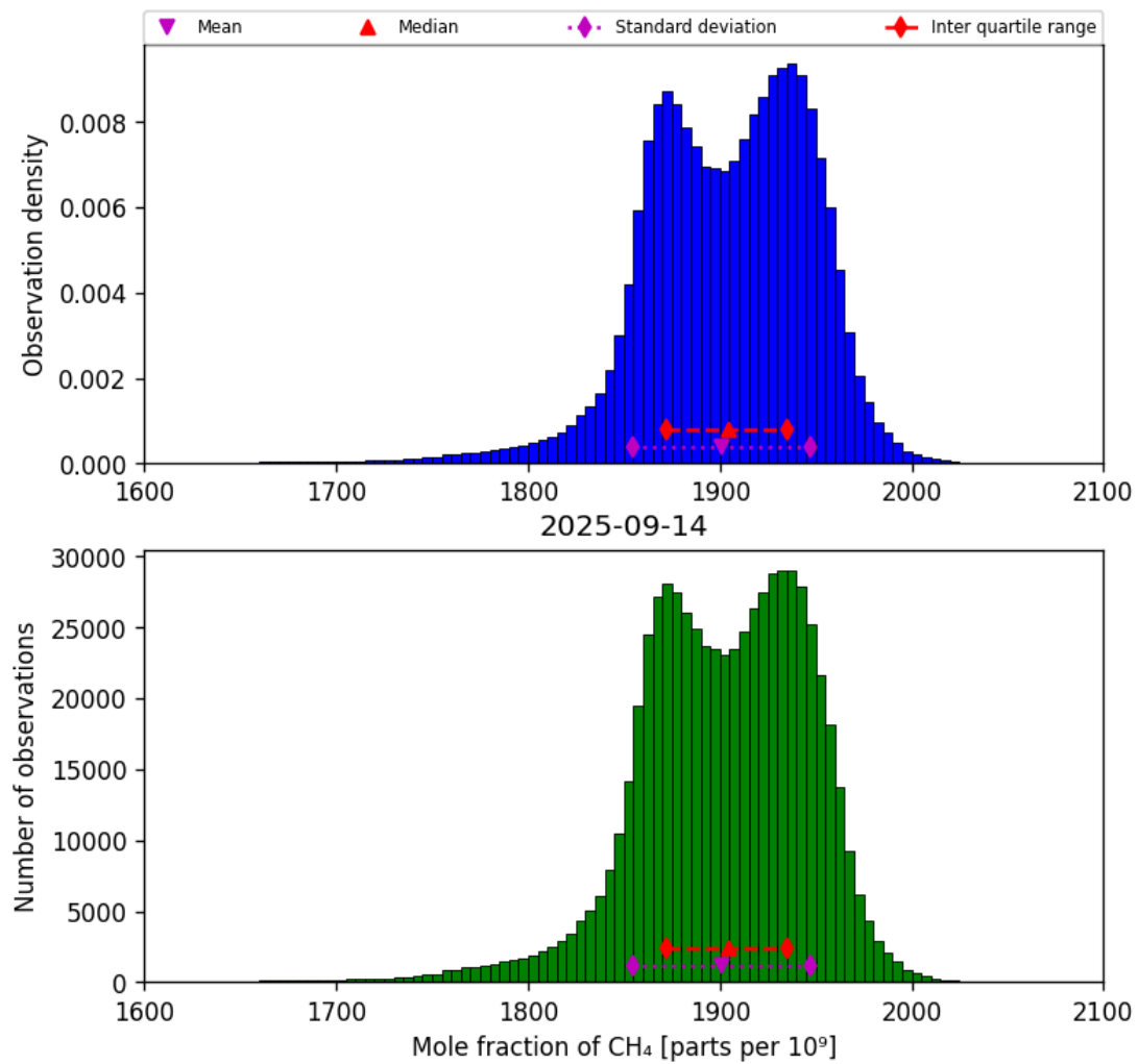
Figure 23: Histogram of “Mole fraction of CH 4 ” for 2025-09-13 to 2025-09-15
