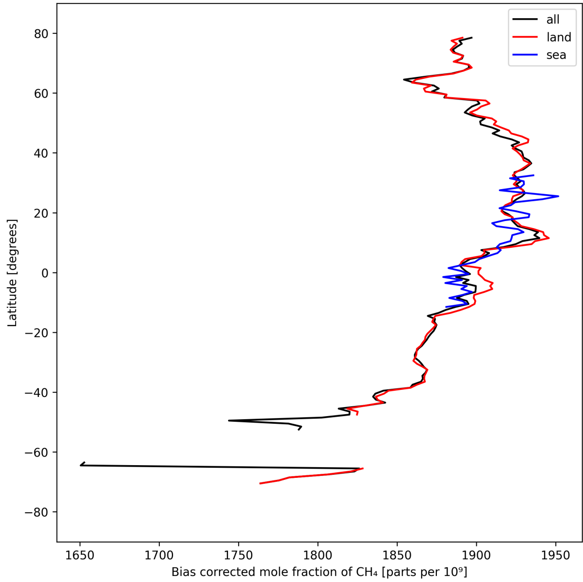
Figure 14: Zonal average of “Bias corrected mole fraction of CH 4 ” for 2025-09-13 to 2025-09-15.
