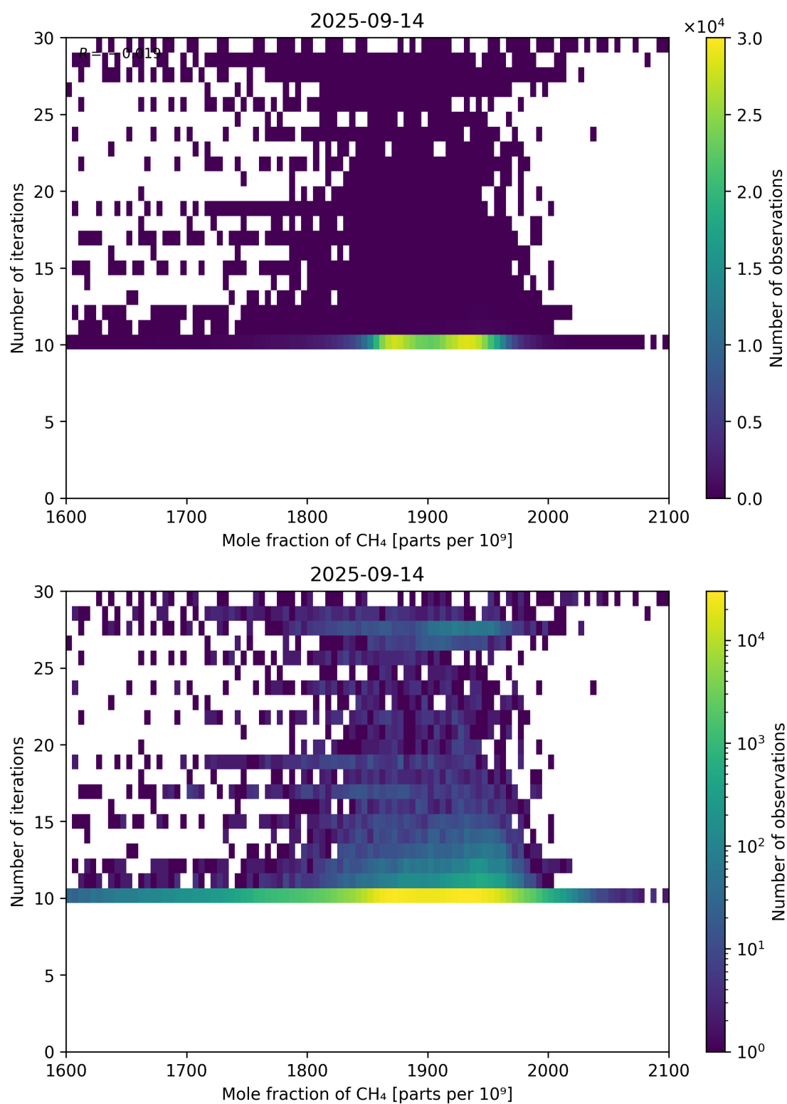
Figure 76: Scatter density plot of “Mole fraction of CH 4 ” against “Number of iterations” for 2025-09-13 to 2025-09-15.
