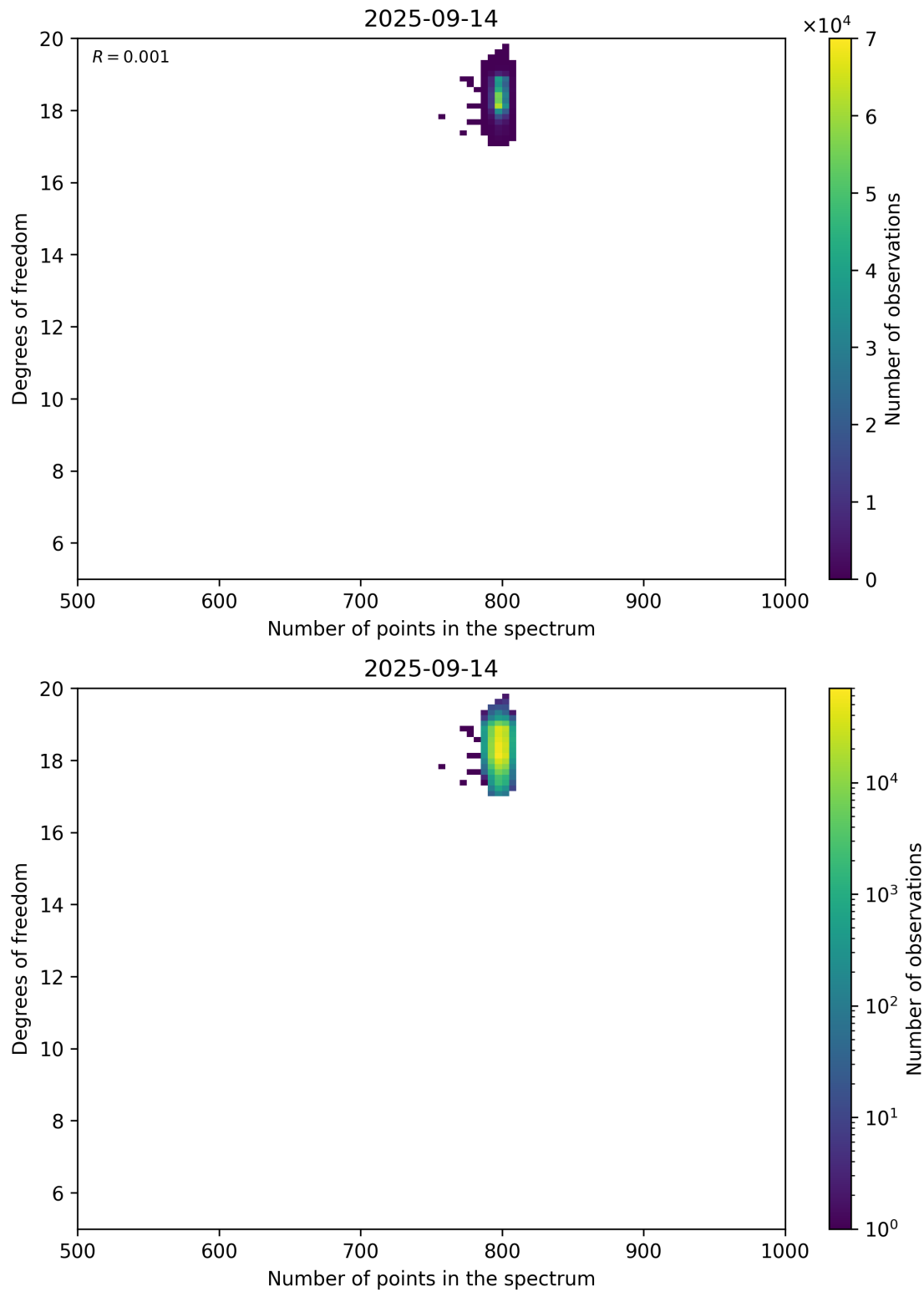
Figure 90: Scatter density plot of “Number of points in the spectrum” against “Degrees of freedom” for 2025-09-13 to 2025-09-15.
