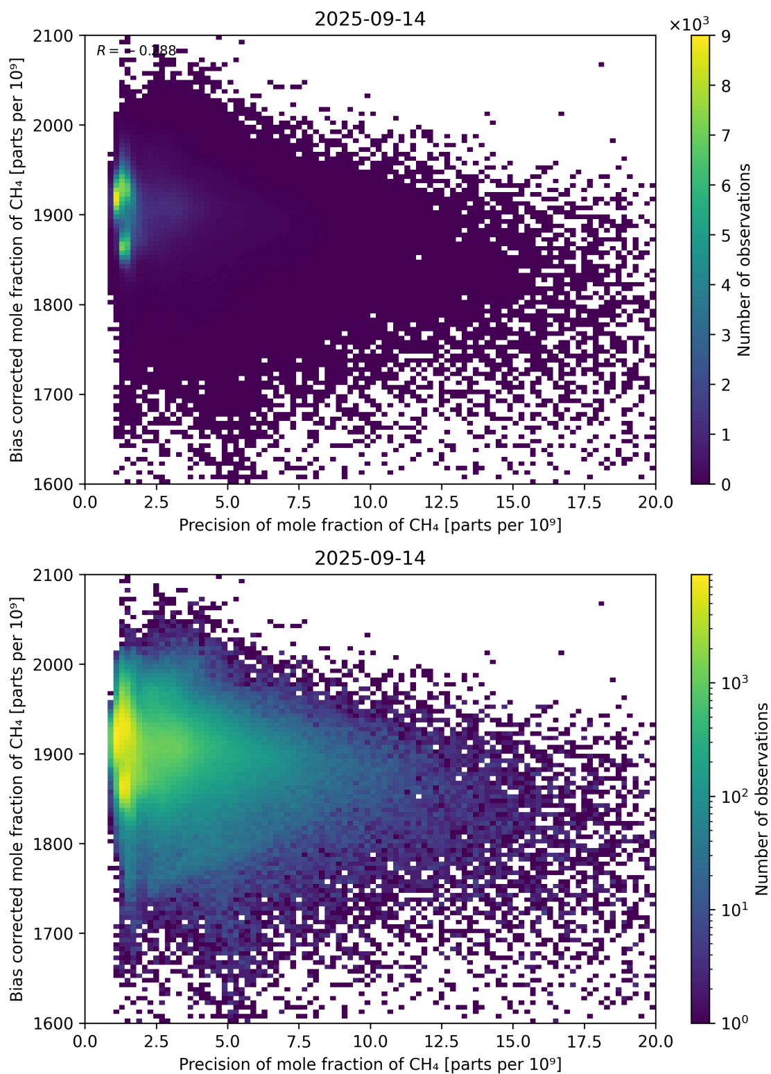
Figure 82: Scatter density plot of “Precision of mole fraction of CH 4 ” against “Bias corrected mole fraction of CH 4 ” for 2025-09-13 to 2025-09-15.
