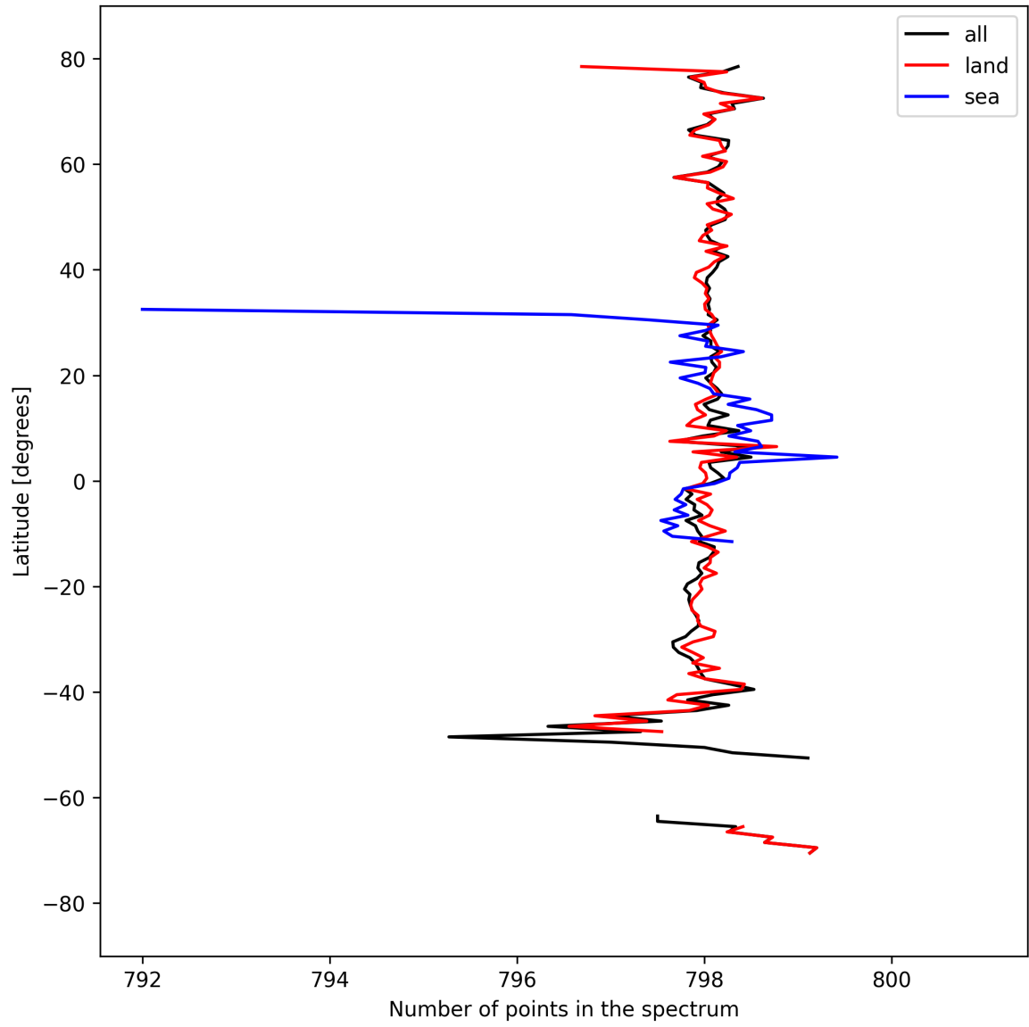
Figure 15: Zonal average of “Number of points in the spectrum” for 2025-09-13 to 2025-09-15.
