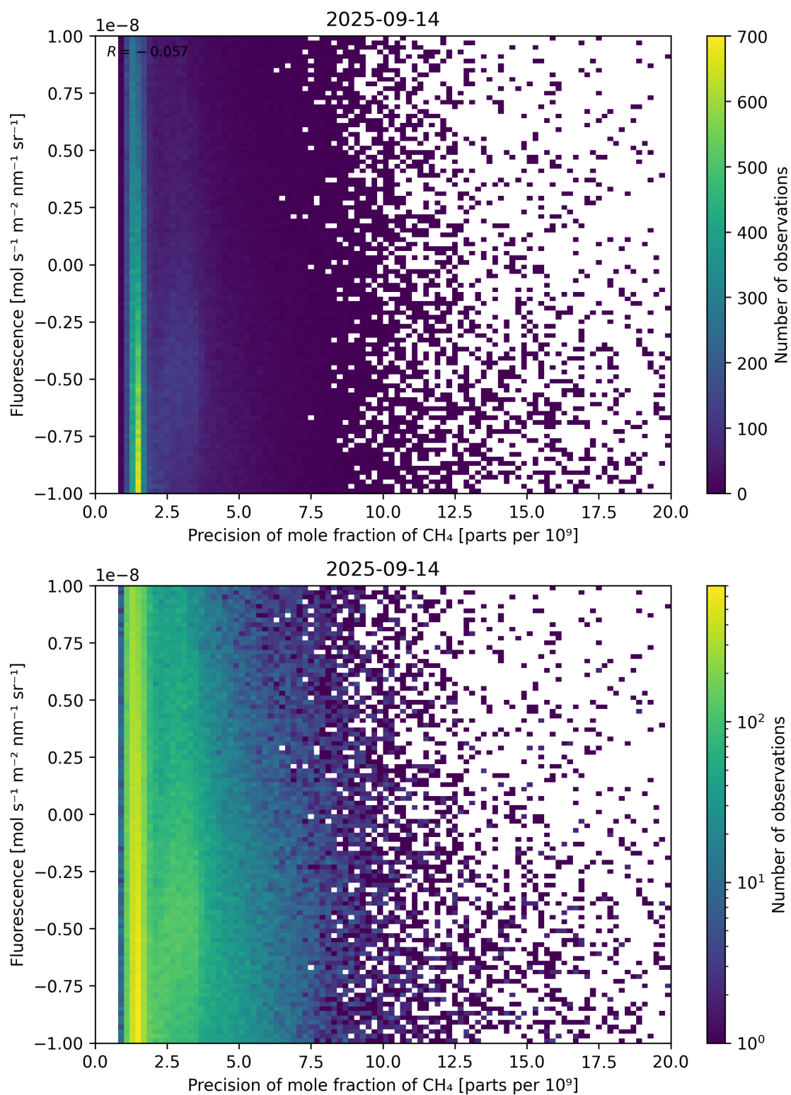
Figure 81: Scatter density plot of “Precision of mole fraction of CH 4 ” against “Fluorescence” for 2025-09-13 to 2025-09-15.
