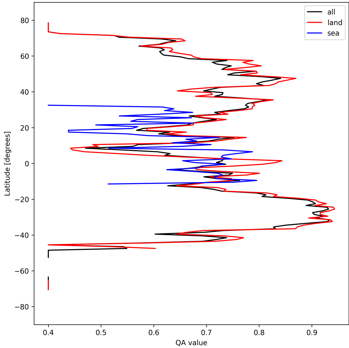
Figure 11: Zonal average of “QA value” for 2025-09-13 to 2025-09-15.
