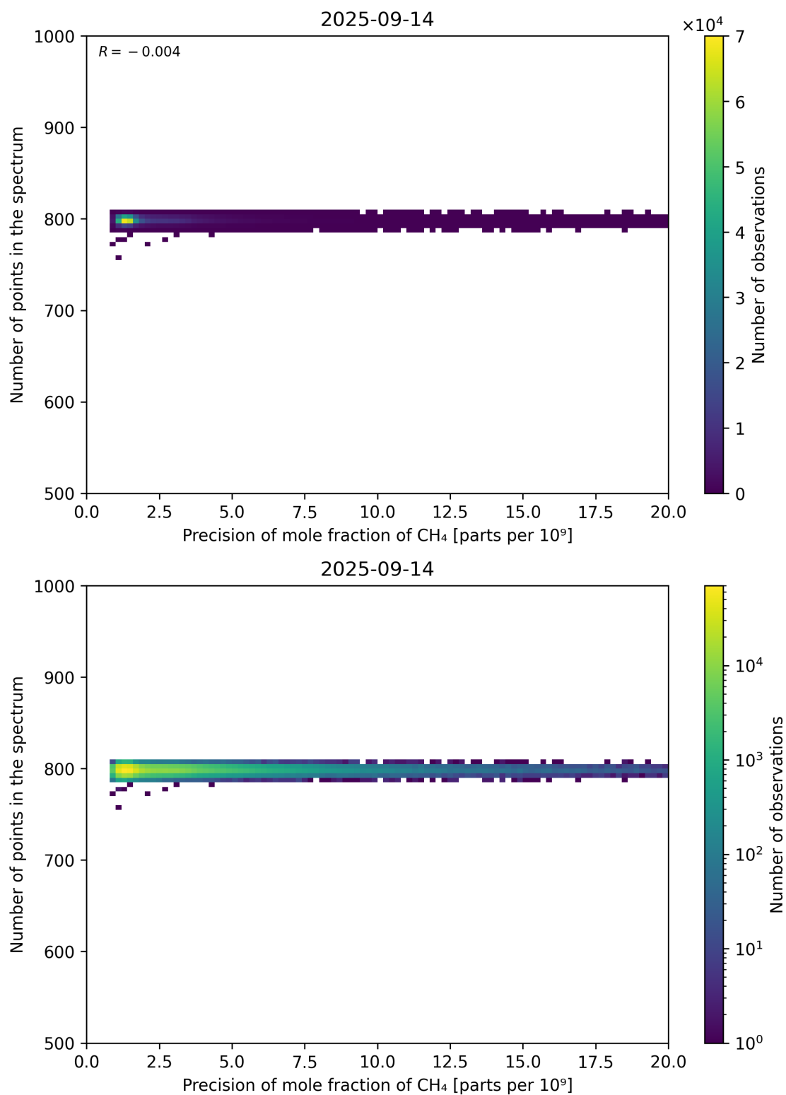
Figure 84: Scatter density plot of “Precision of mole fraction of CH 4 ” against “Number of points in the spectrum” for 2025-09-13 to 2025-09-15.
