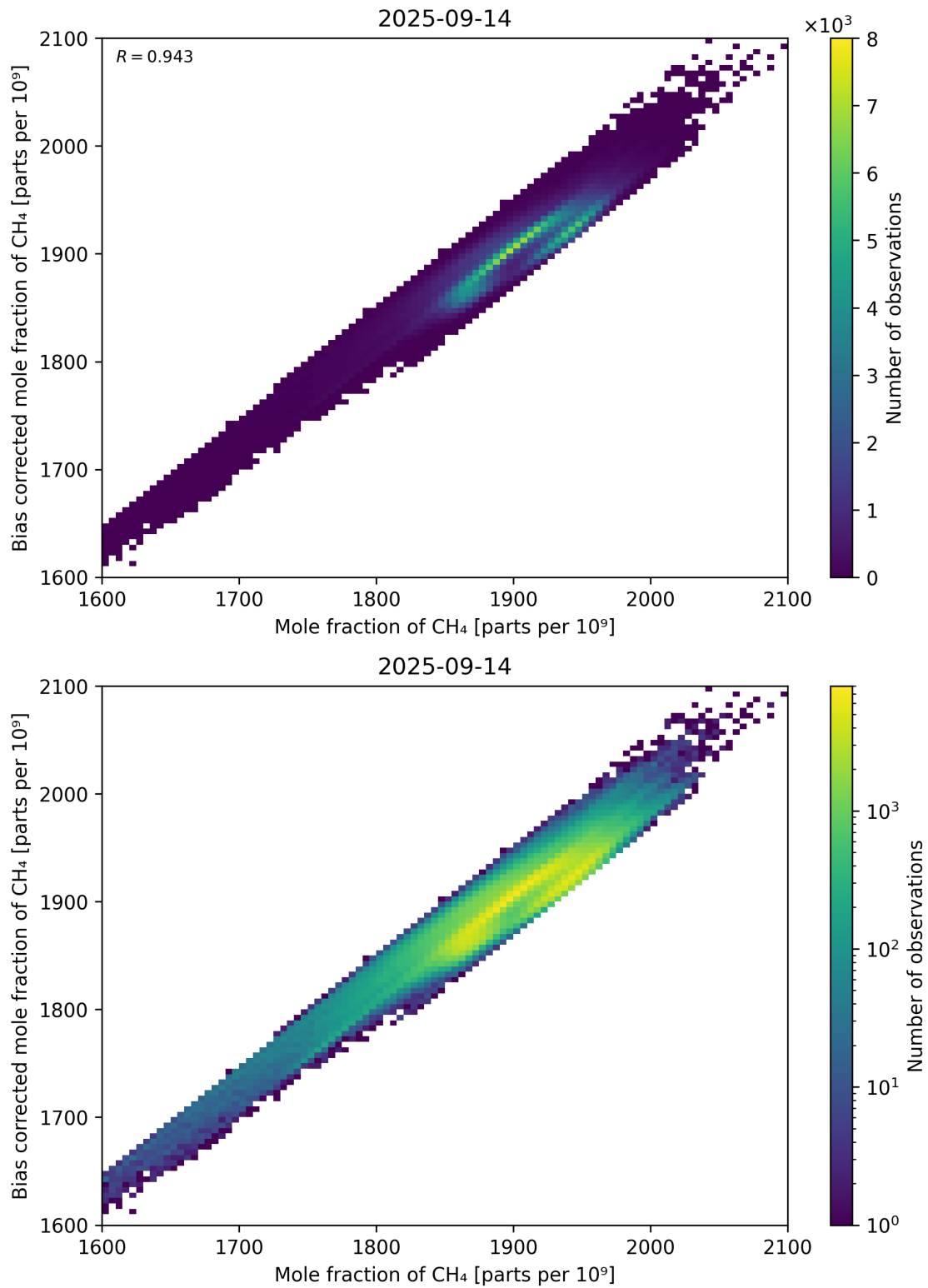
Figure 74: Scatter density plot of “Mole fraction of CH 4 ” against “Bias corrected mole fraction of CH 4 ” for 2025-09-13 to 2025-09-15.
