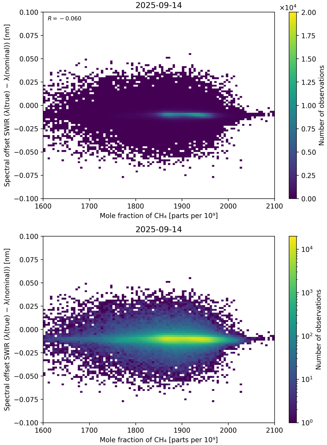
Figure 86: Scatter density plot of “Mole fraction of CH 4 ” against “Spectral offset SWIR ( \lambda_{\text{true}} - \lambda_{\text{nominal}} )” for 2025-09-13 to 2025-09-15.
