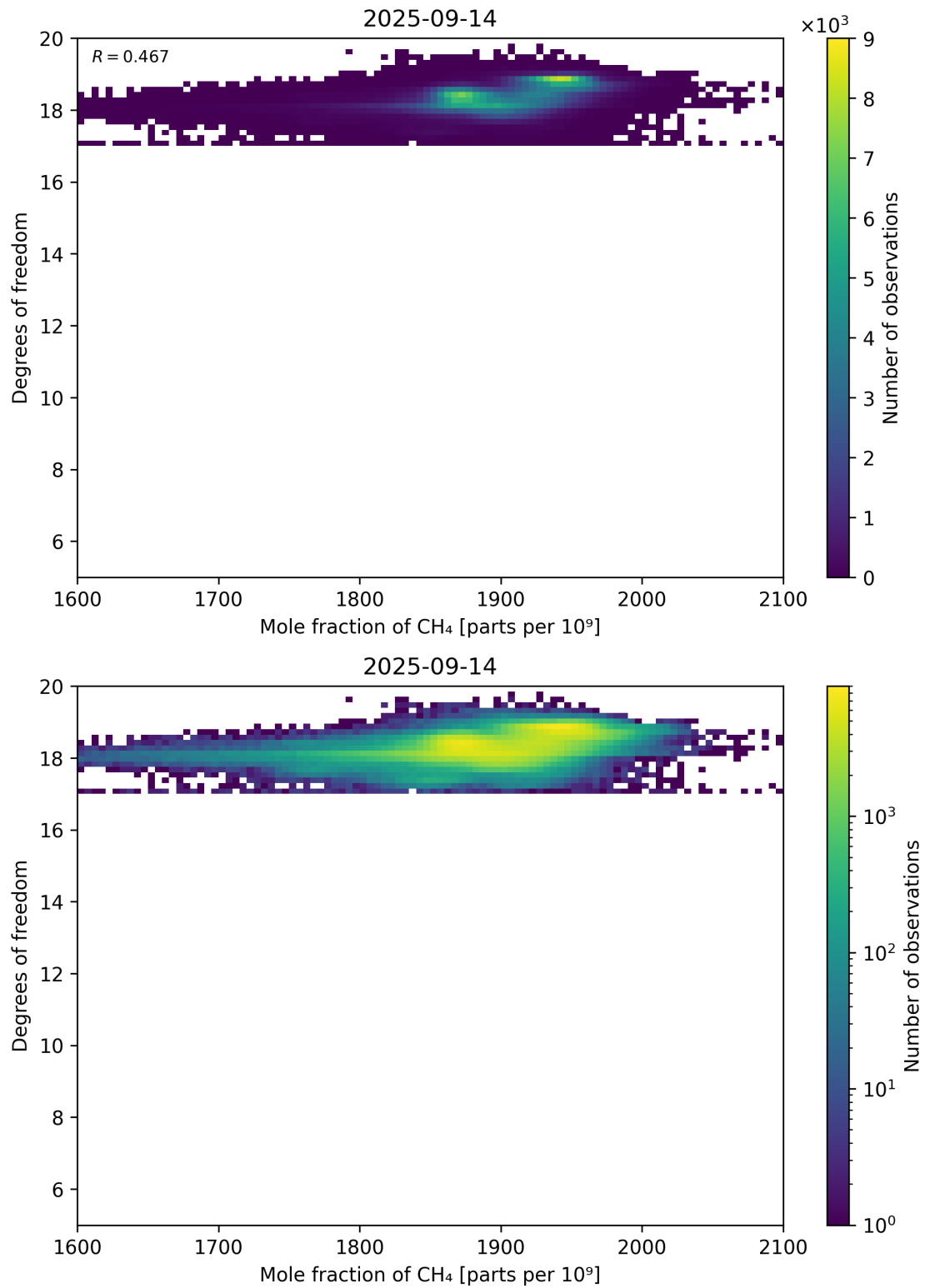
Figure 72: Scatter density plot of “Mole fraction of CH 4 ” against “Degrees of freedom” for 2025-09-13 to 2025-09-15.
