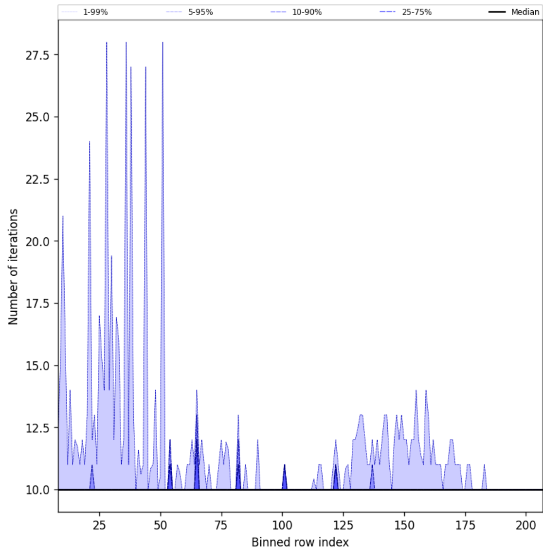
Figure 42: Along track statistics of “Number of iterations” for 2025-09-13 to 2025-09-15
