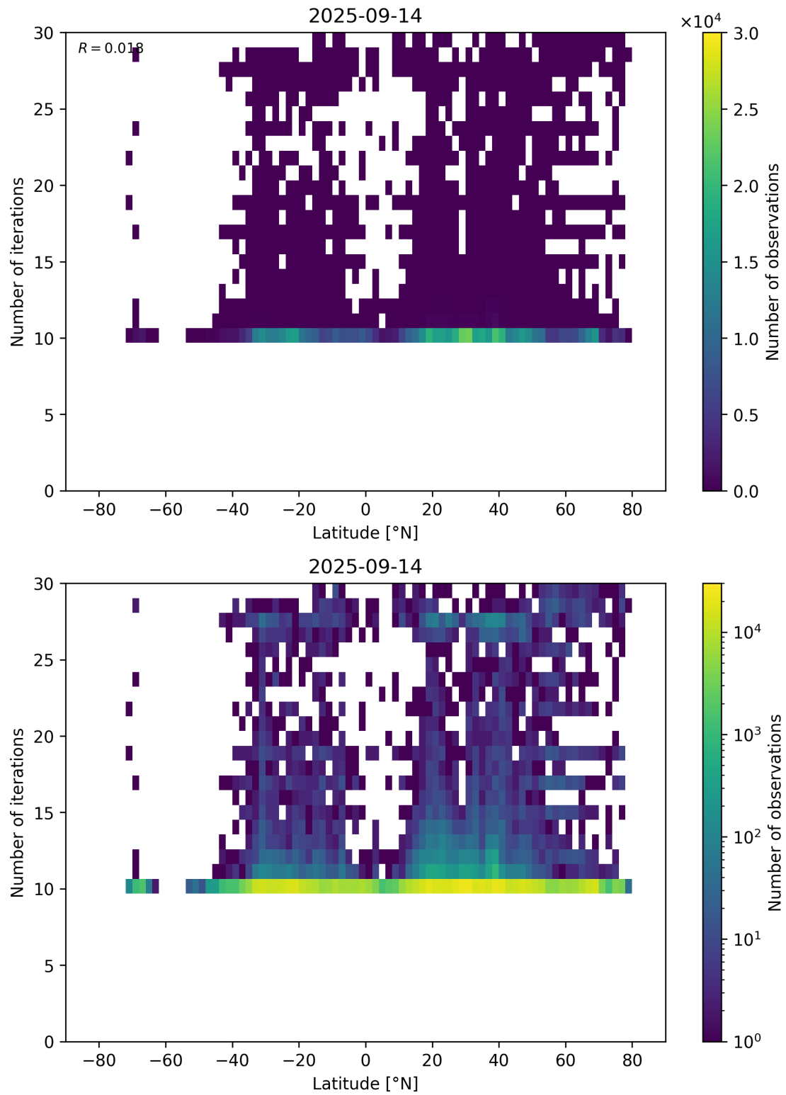
Figure 60: Scatter density plot of “Latitude” against “Number of iterations” for 2025-09-13 to 2025-09-15.
