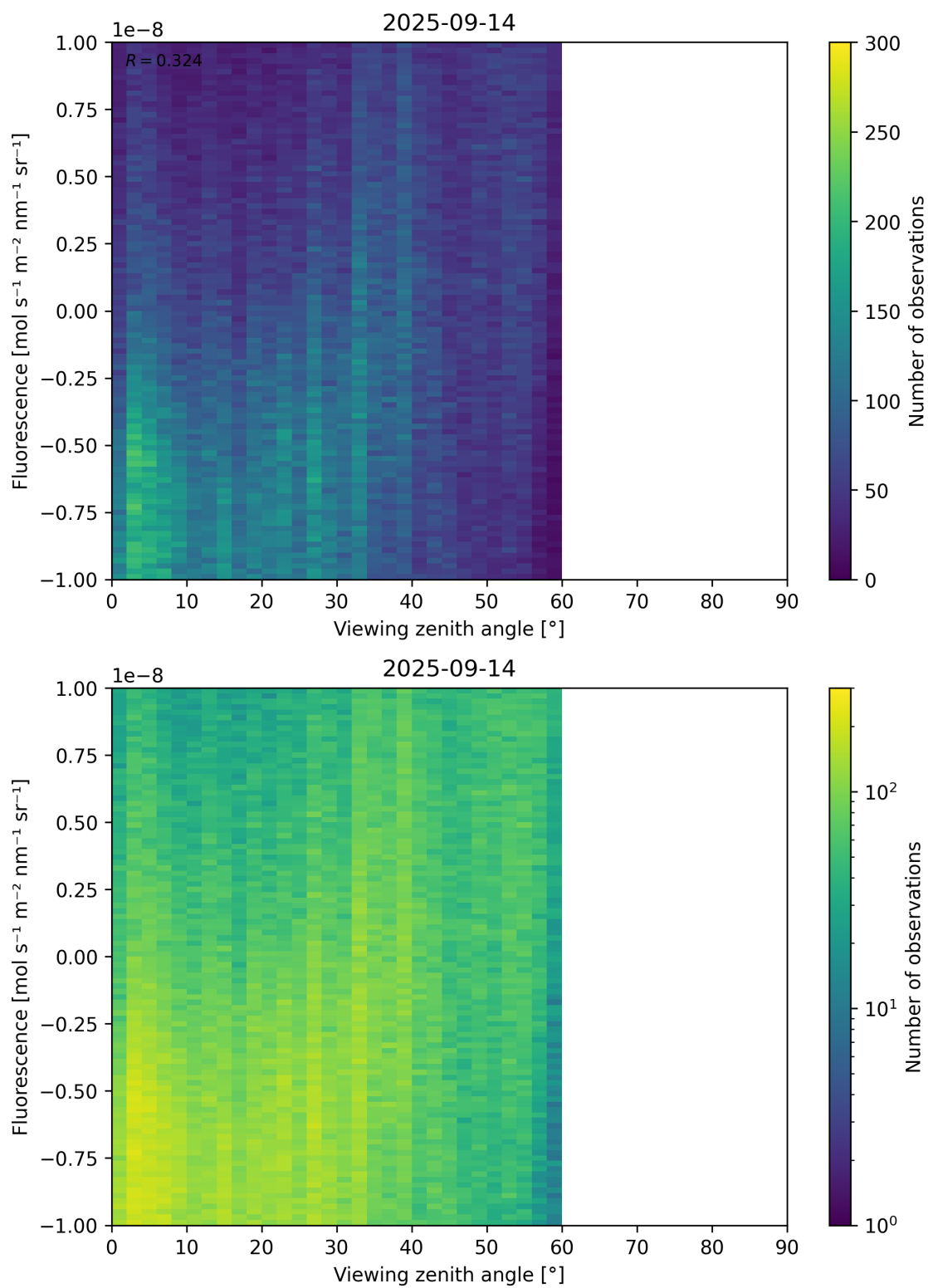
Figure 108: Scatter density plot of “Viewing zenith angle” against “Fluorescence” for 2025-09-13 to 2025-09-15.
