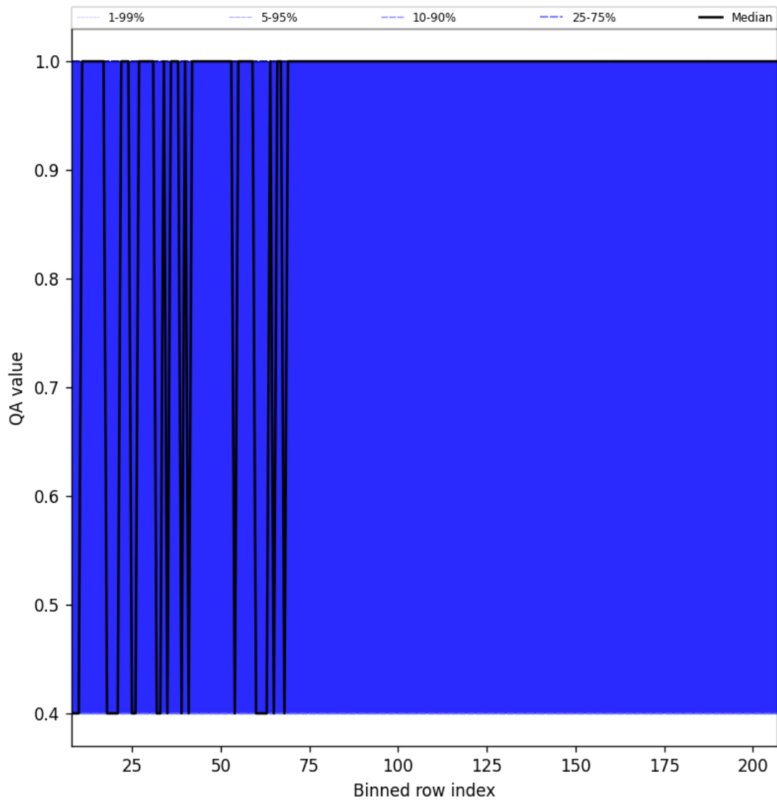
Figure 33: Along track statistics of “QA value” for 2025-09-13 to 2025-09-15
