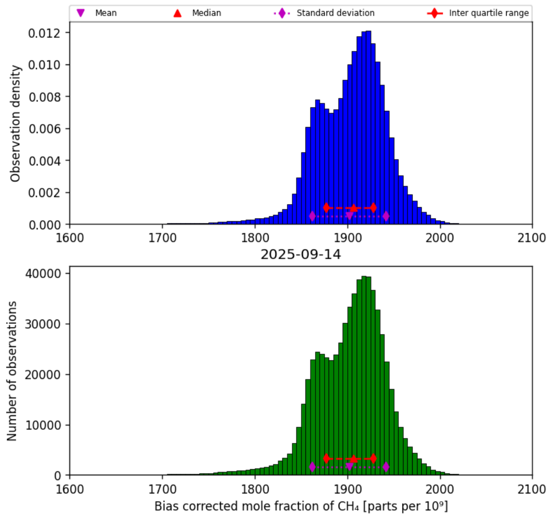
Figure 25: Histogram of “Bias corrected mole fraction of CH 4 ” for 2025-09-13 to 2025-09-15
