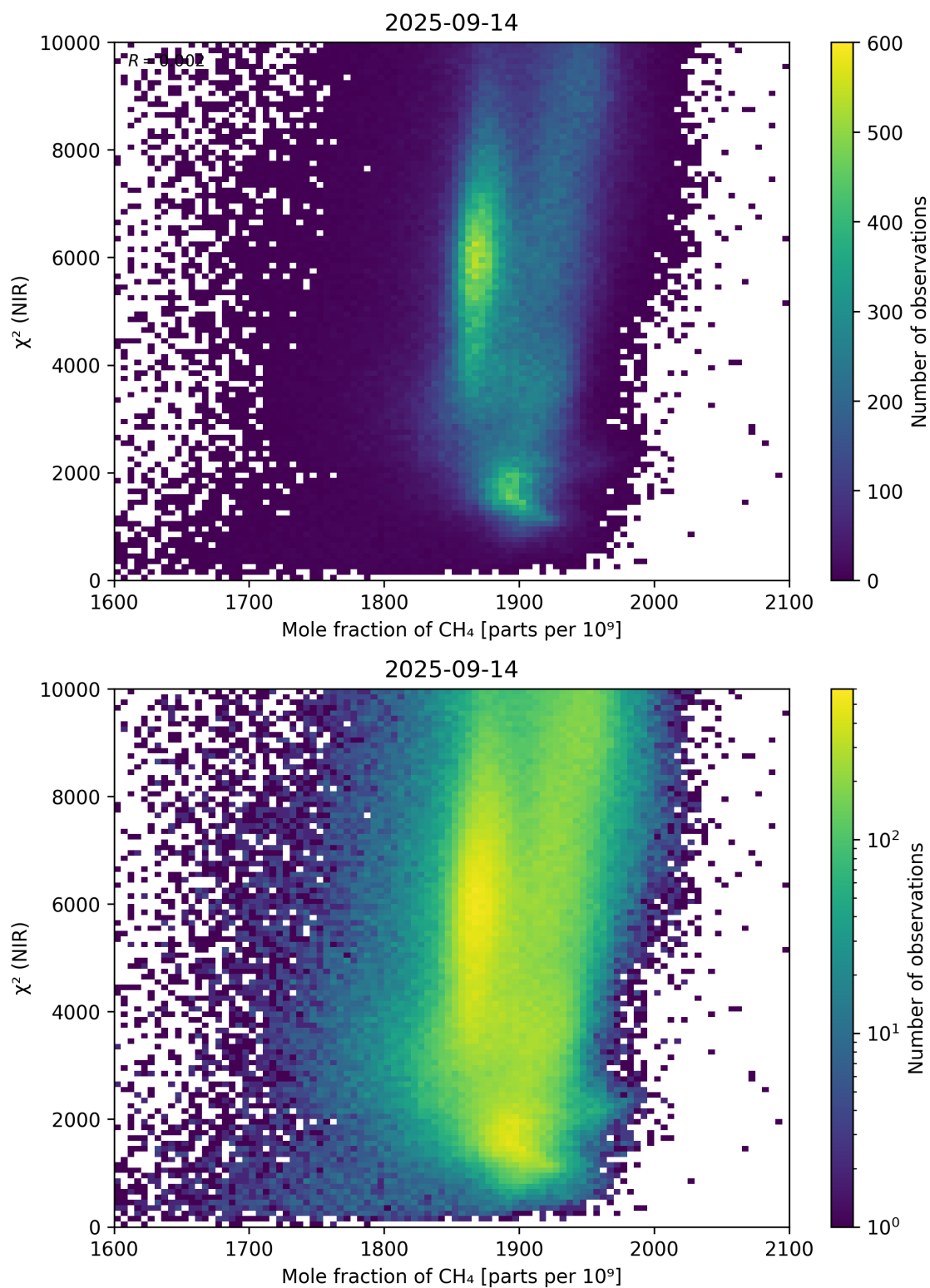
Figure 70: Scatter density plot of “Mole fraction of \text{CH}_4 ” against “ \chi^2 (NIR)” for 2025-09-13 to 2025-09-15.
