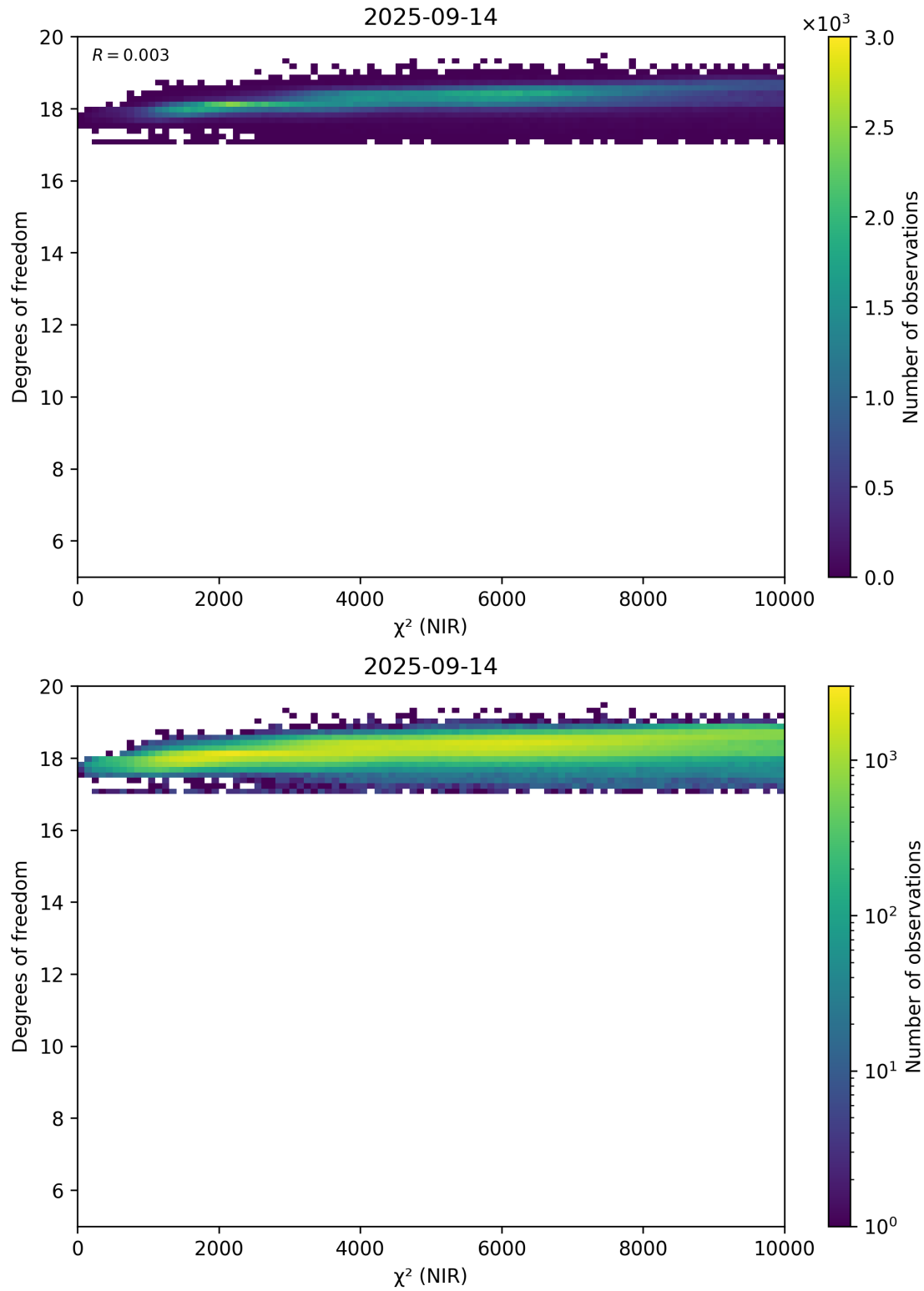
Figure 44: Scatter density plot of “ \chi^2 (NIR)” against “Degrees of freedom” for 2025-09-13 to 2025-09-15.
