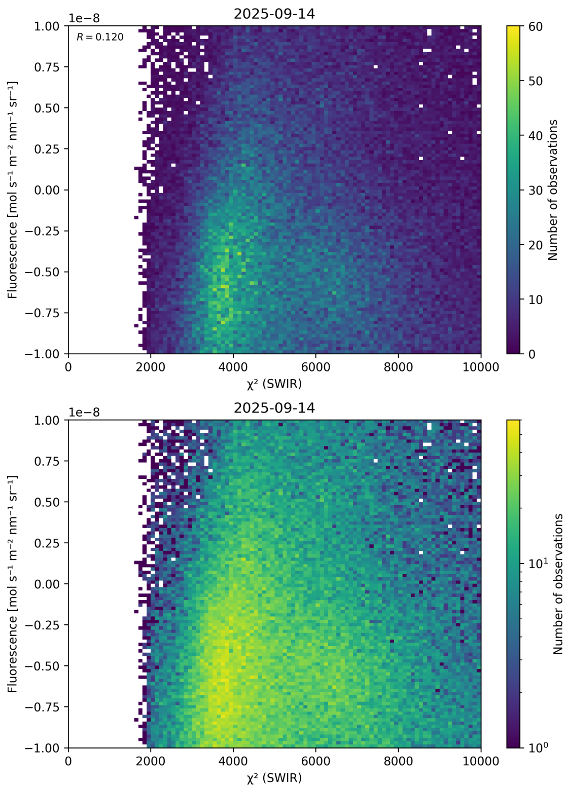
Figure 49: Scatter density plot of “ \chi^2 (SWIR)” against “Fluorescence” for 2025-09-13 to 2025-09-15.
