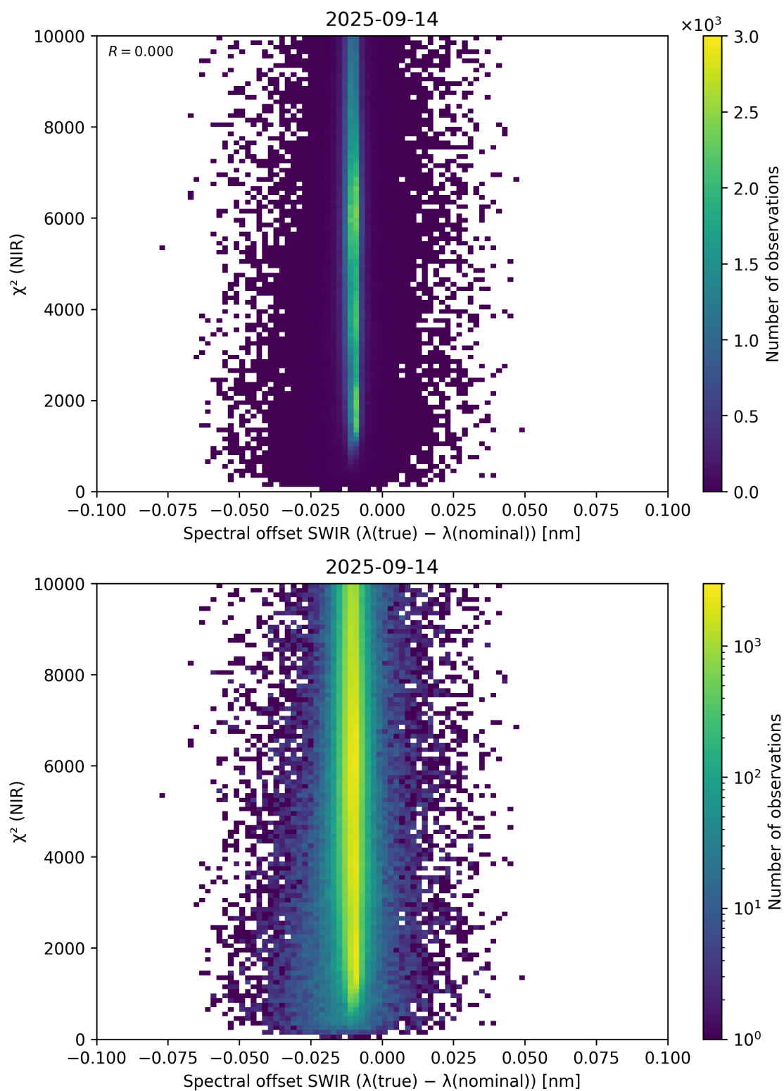
Figure 117: Scatter density plot of “Spectral offset SWIR ( \lambda_{\text{true}} - \lambda_{\text{nominal}} )” against “ \chi^2 (NIR)” for 2025-09-13 to 2025-09-15.
