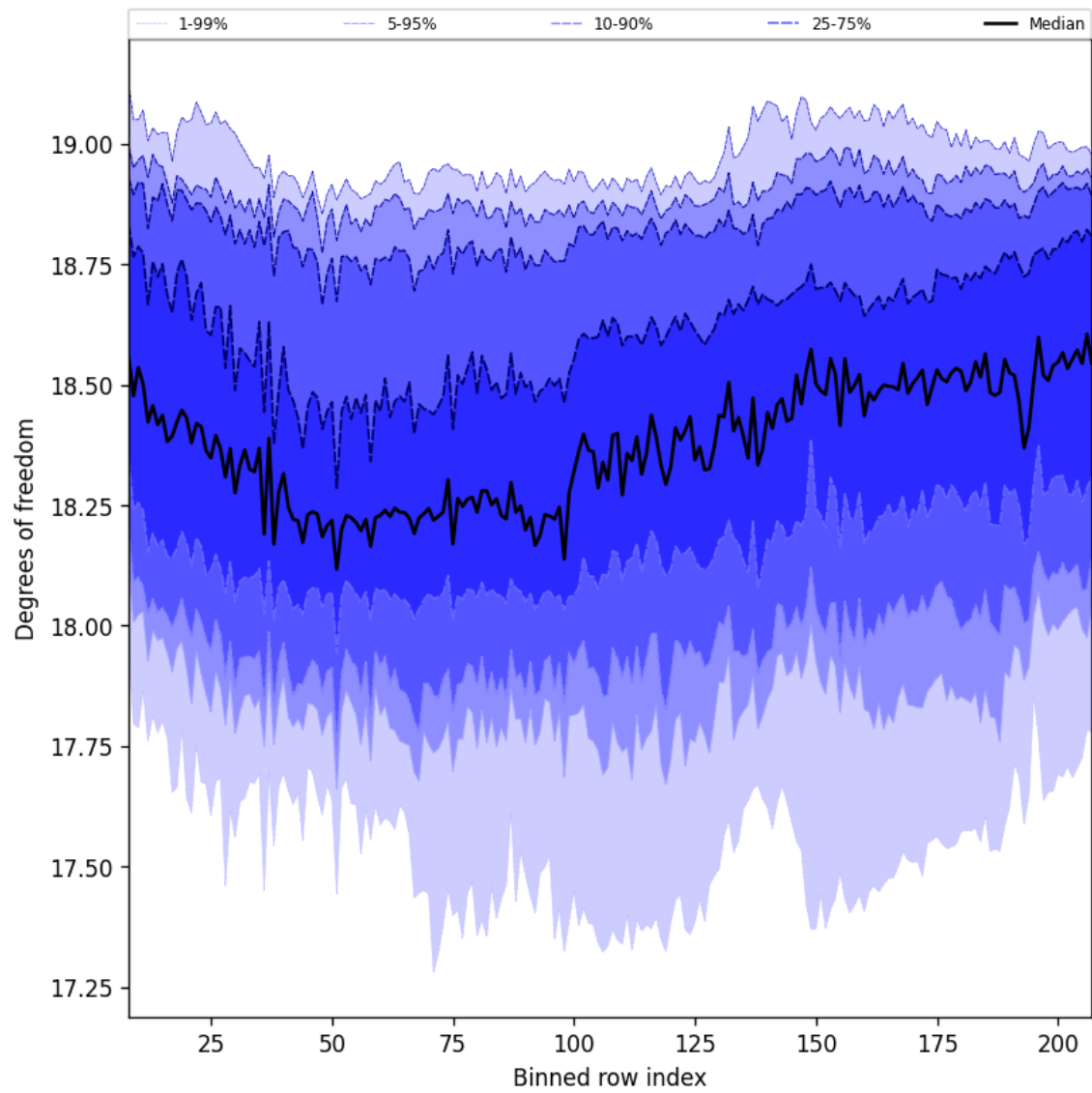
Figure 41: Along track statistics of “Degrees of freedom” for 2025-09-13 to 2025-09-15
