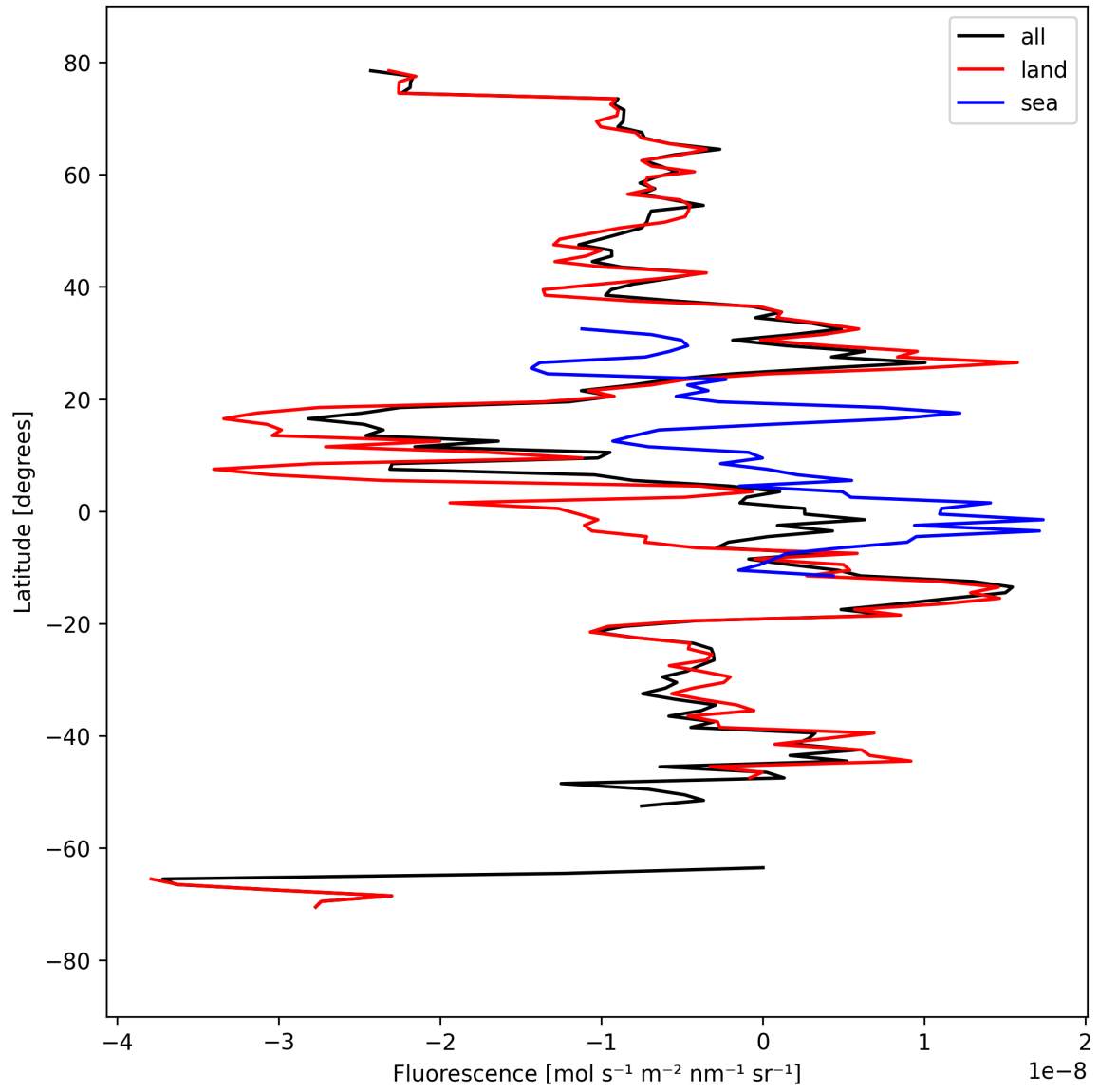
Figure 21: Zonal average of “Fluorescence” for 2025-09-13 to 2025-09-15.
