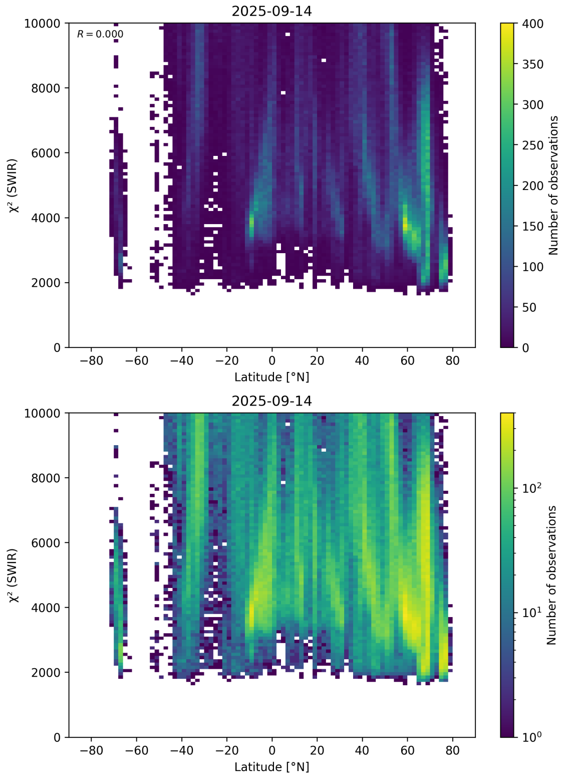
Figure 54: Scatter density plot of “Latitude” against “ \chi^2 (SWIR)” for 2025-09-13 to 2025-09-15.
