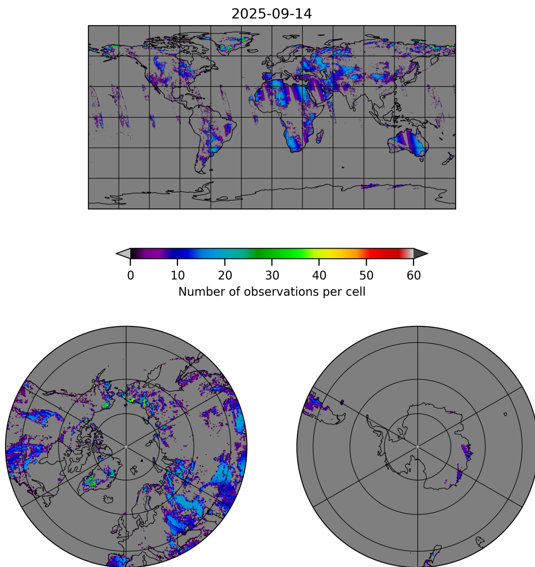
Figure 10: Map of the number of observations for 2025-09-13 to 2025-09-15
