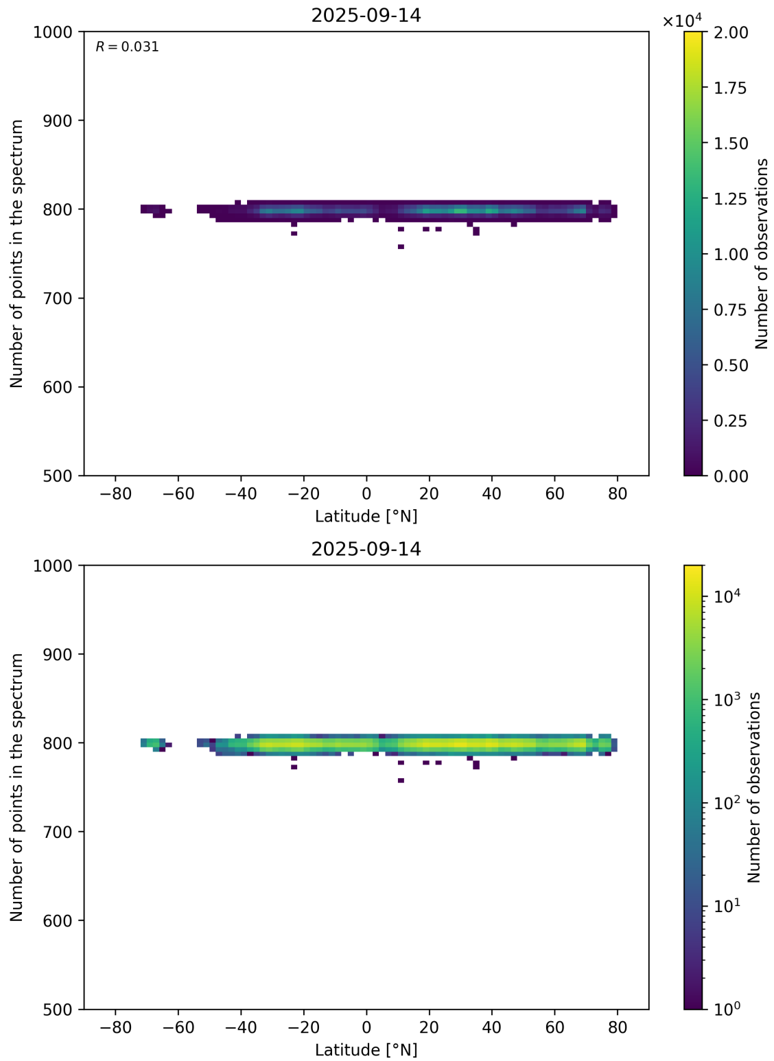
Figure 61: Scatter density plot of “Latitude” against “Number of points in the spectrum” for 2025-09-13 to 2025-09-15.
