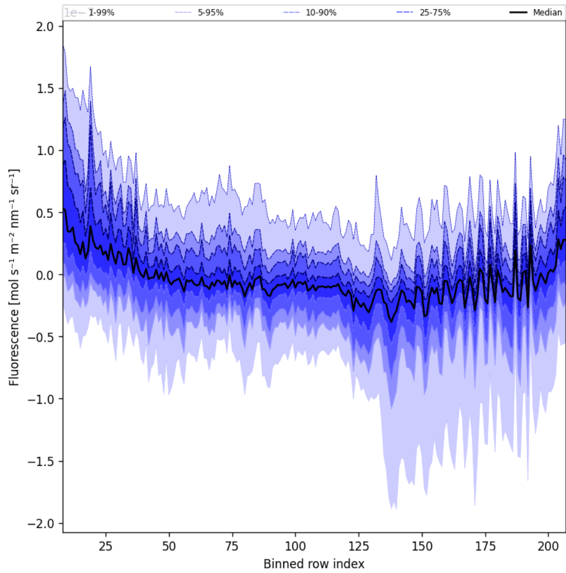
Figure 43: Along track statistics of “Fluorescence” for 2025-09-13 to 2025-09-15
