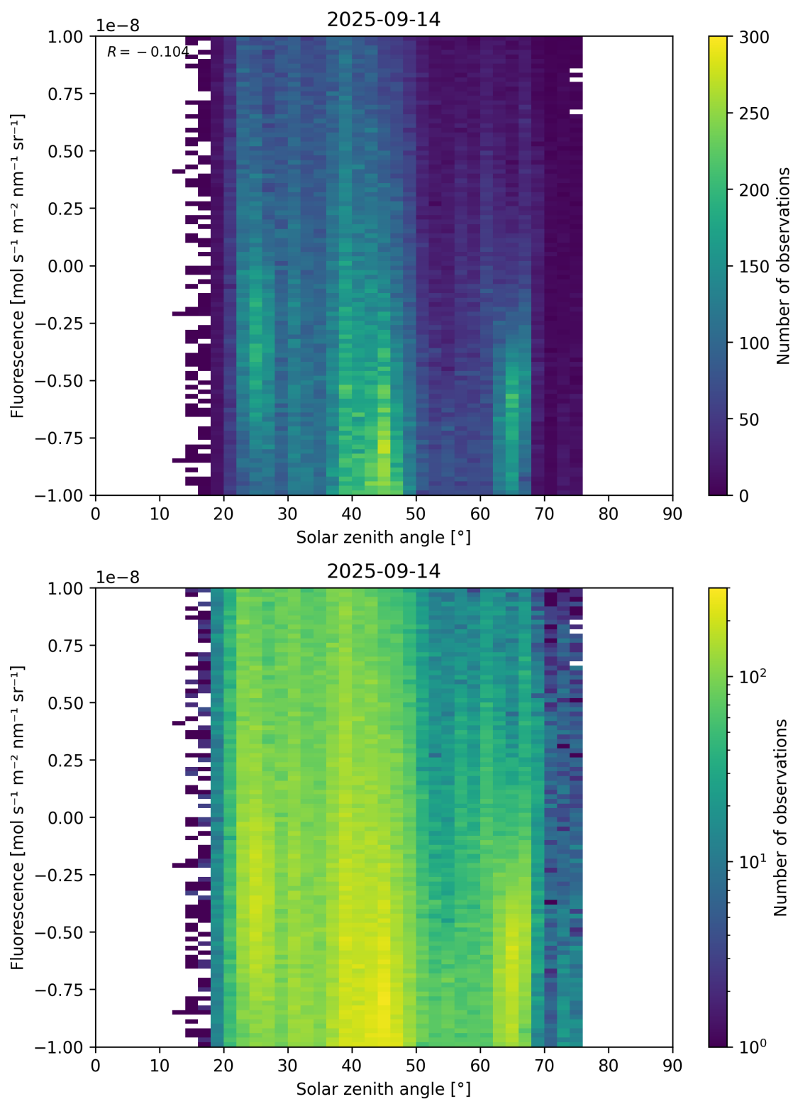
Figure 97: Scatter density plot of “Solar zenith angle” against “Fluorescence” for 2025-09-13 to 2025-09-15.
