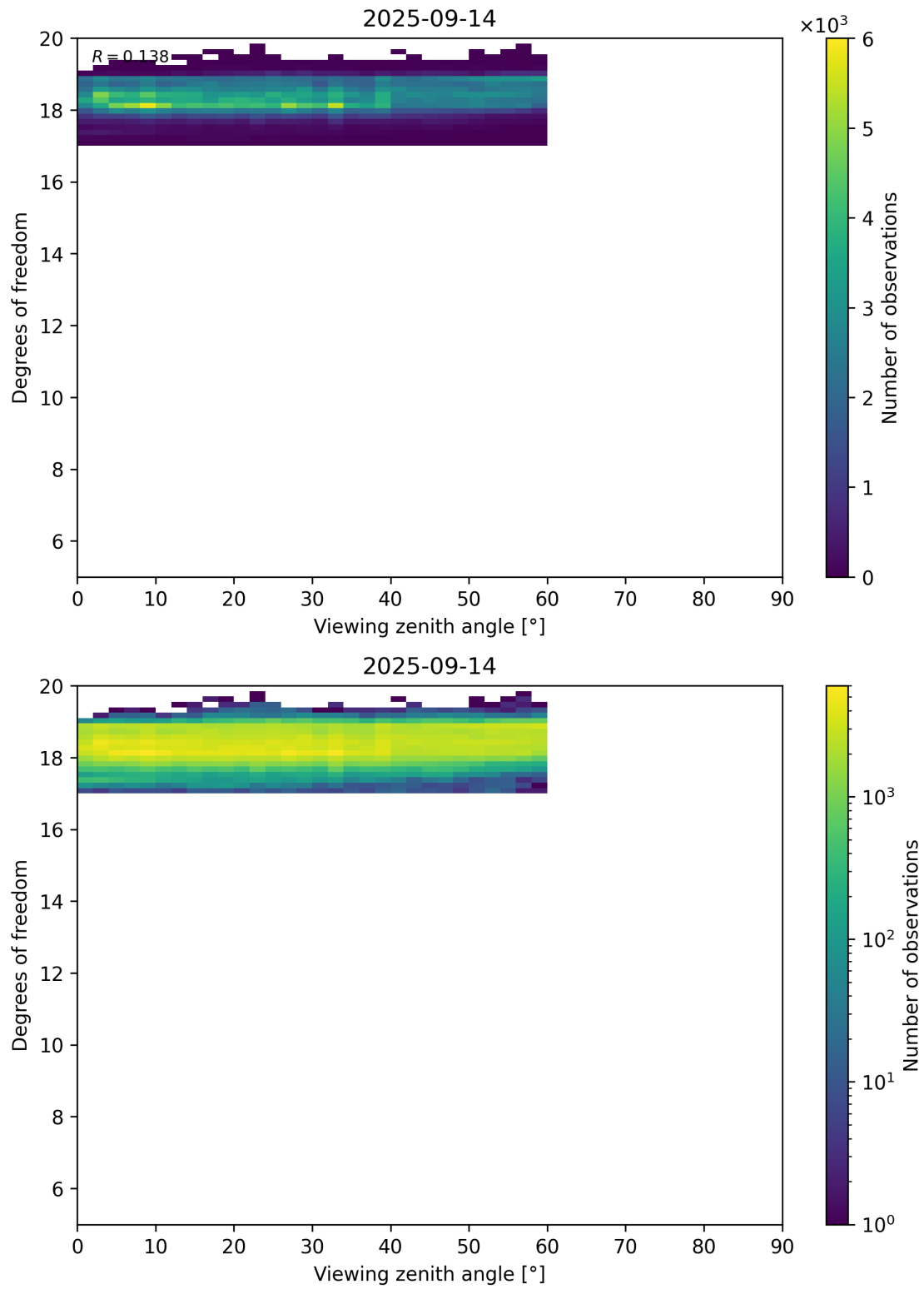
Figure 107: Scatter density plot of “Viewing zenith angle” against “Degrees of freedom” for 2025-09-13 to 2025-09-15.
