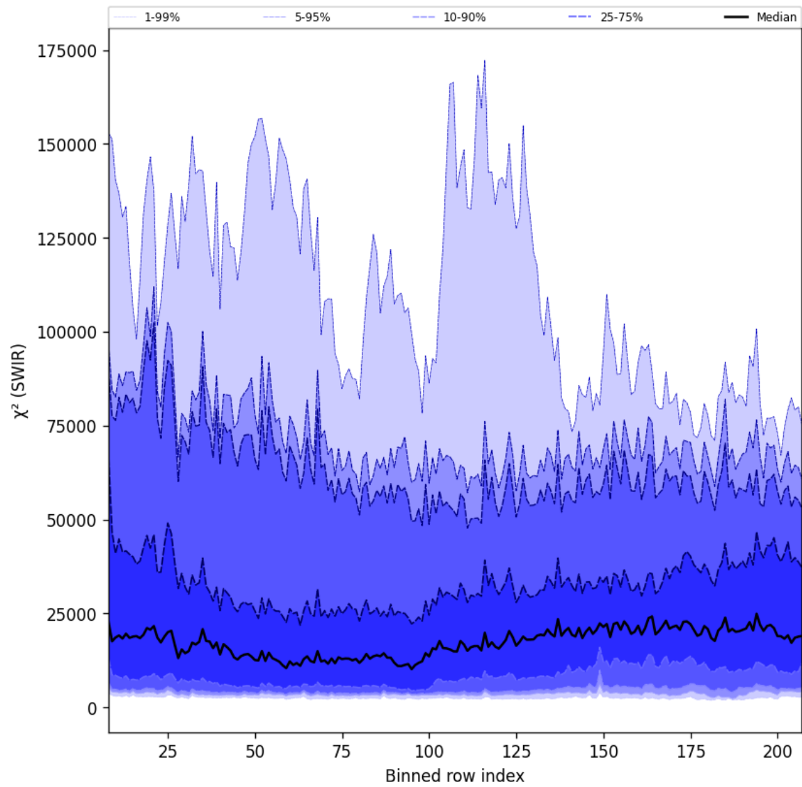
Figure 39: Along track statistics of “ \chi^2 (SWIR)” for 2025-09-13 to 2025-09-15
