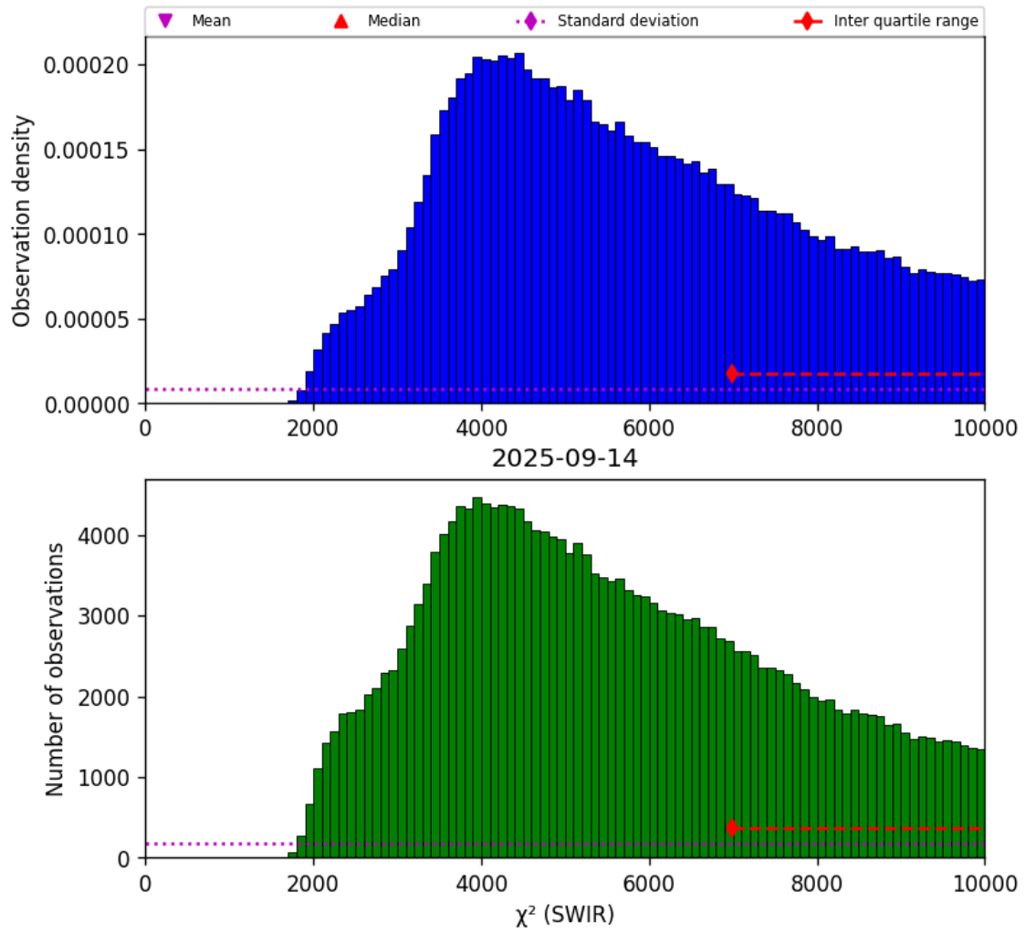
Figure 28: Histogram of “ \chi^2 (SWIR)” for 2025-09-13 to 2025-09-15
