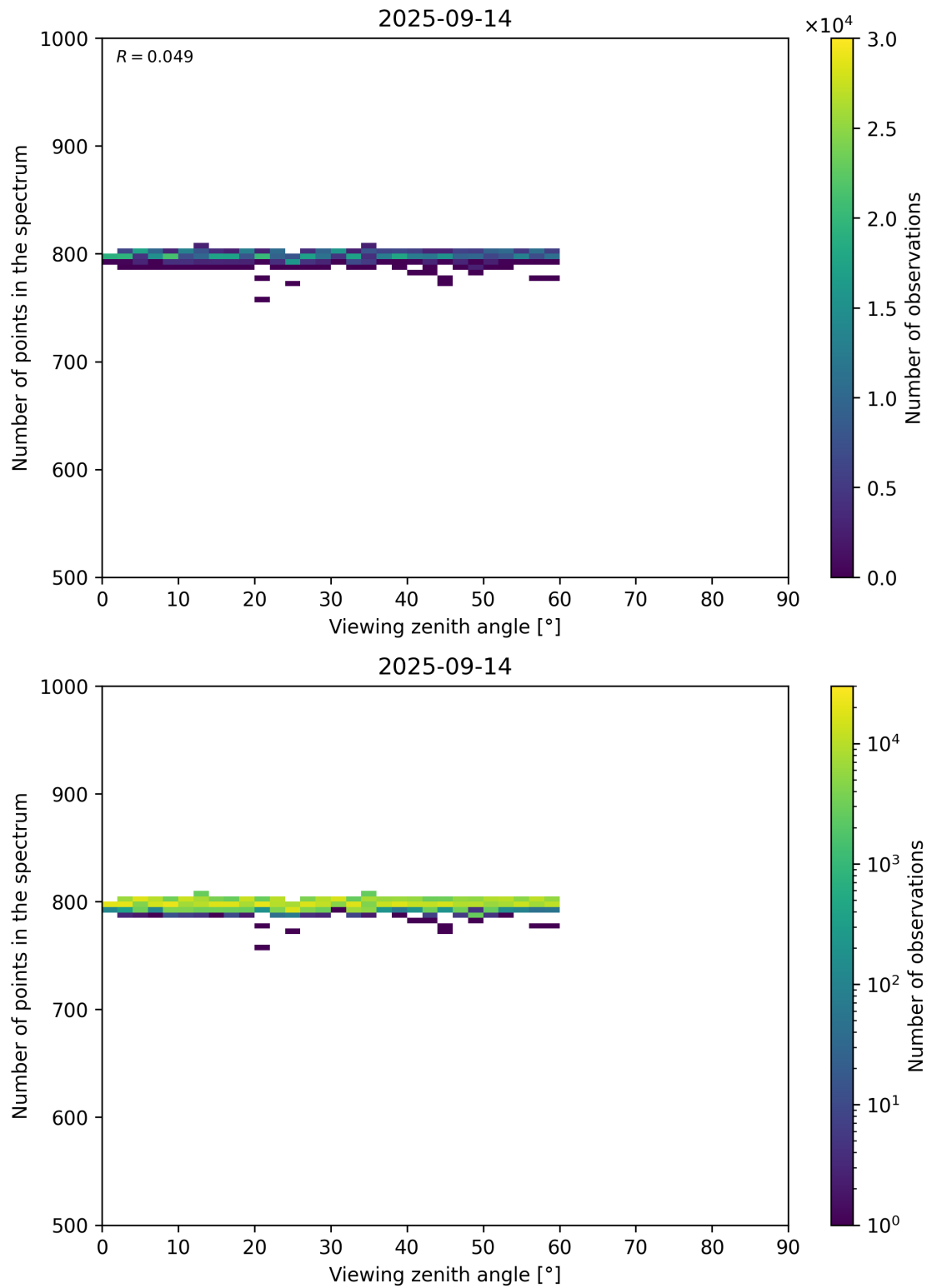
Figure 114: Scatter density plot of “Viewing zenith angle” against “Number of points in the spectrum” for 2025-09-13 to 2025-09-15.
