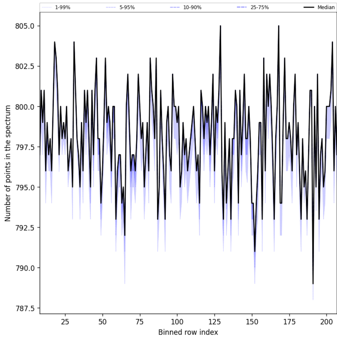
Figure 37: Along track statistics of “Number of points in the spectrum” for 2025-09-13 to 2025-09-15
