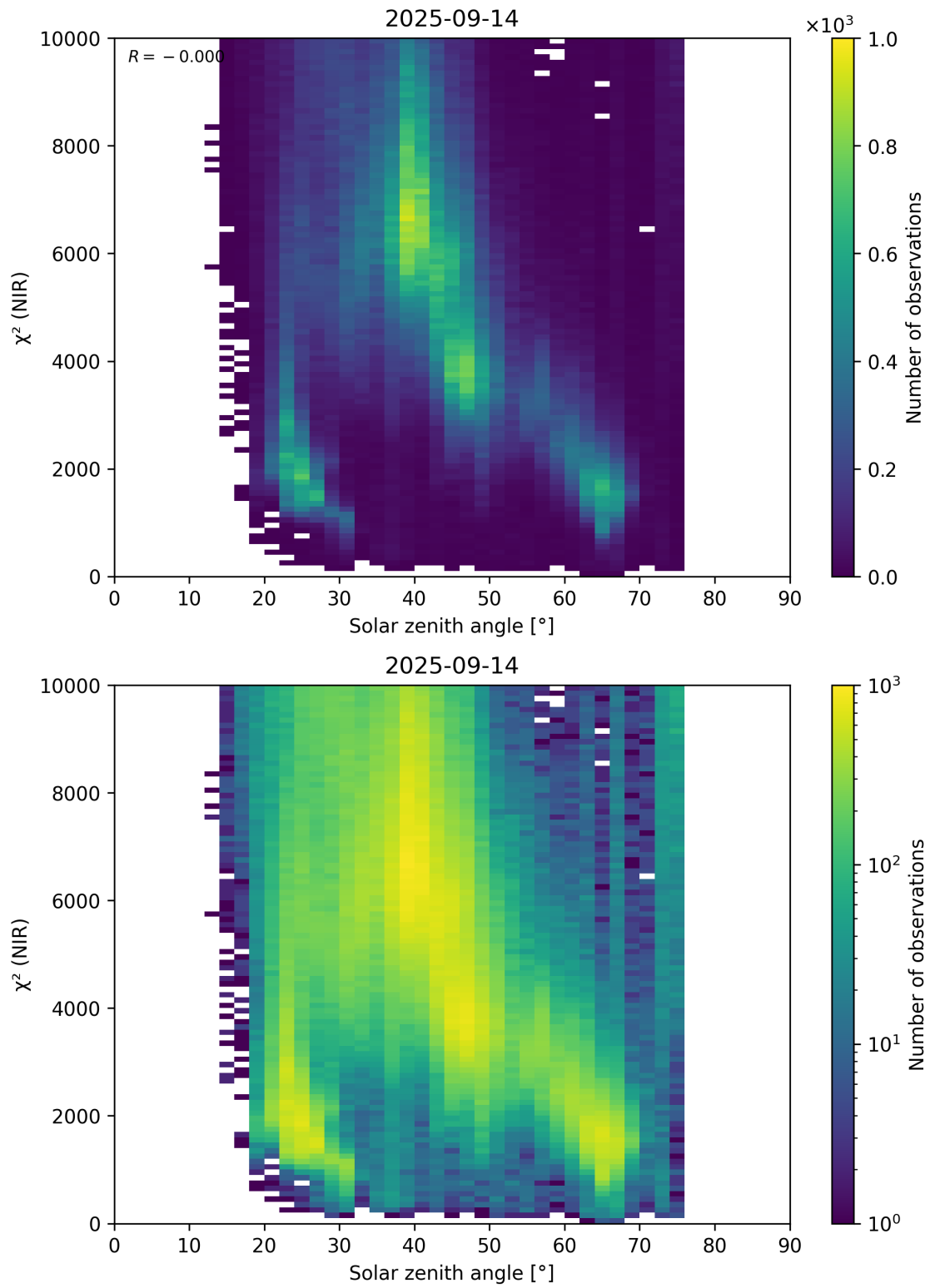
Figure 94: Scatter density plot of “Solar zenith angle” against “ \chi^2 (NIR)” for 2025-09-13 to 2025-09-15.
