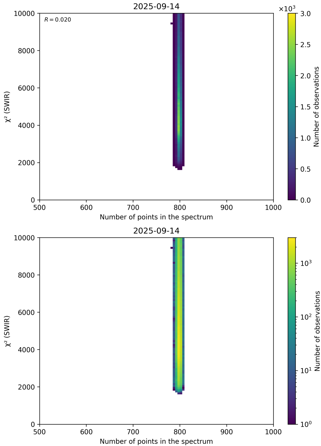
Figure 89: Scatter density plot of “Number of points in the spectrum” against “ \chi^2 (SWIR)” for 2025-09-13 to 2025-09-15.
