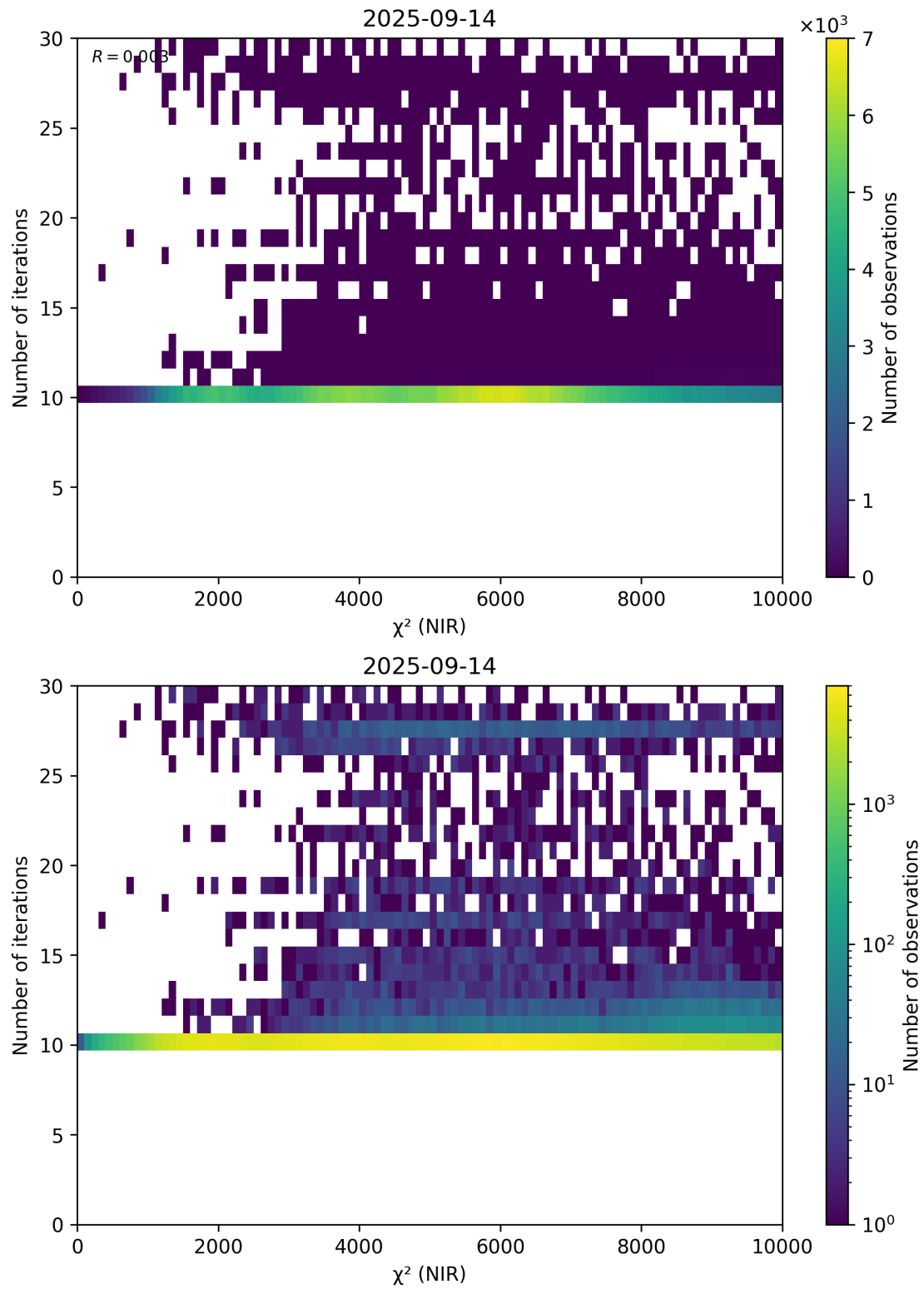
Figure 46: Scatter density plot of “ \chi^2 (NIR)” against “Number of iterations” for 2025-09-13 to 2025-09-15.
