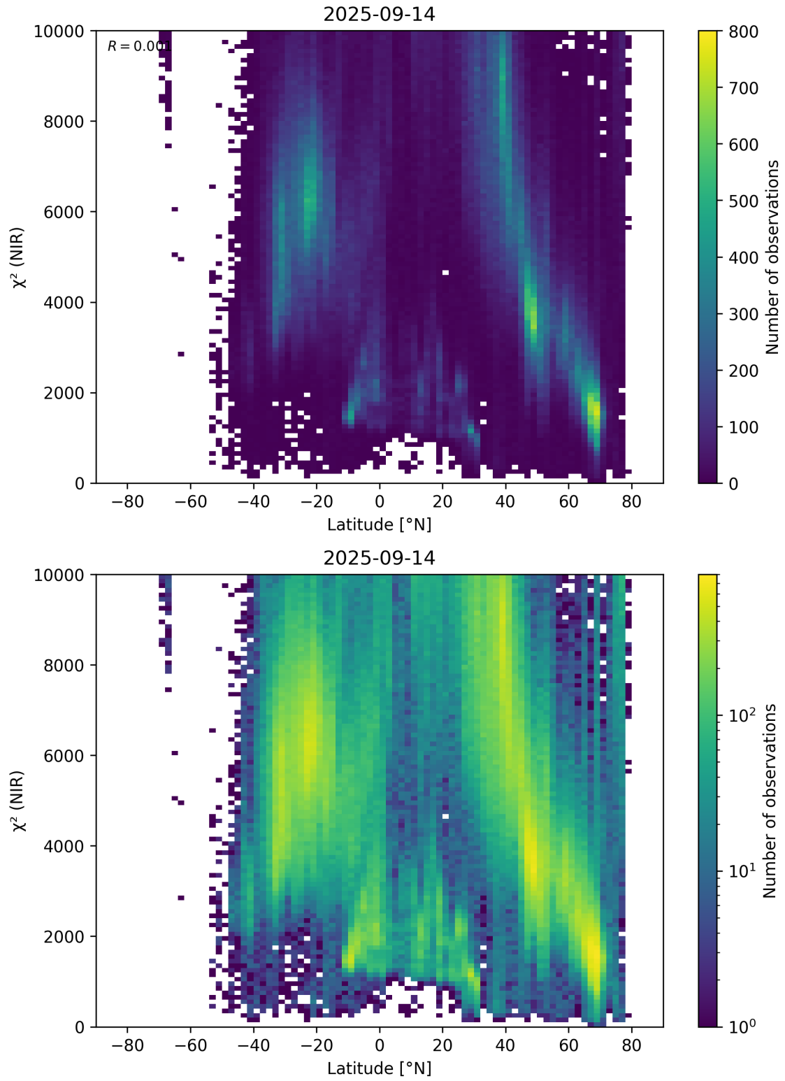
Figure 53: Scatter density plot of “Latitude” against “ \chi^2 (NIR)” for 2025-09-13 to 2025-09-15.
