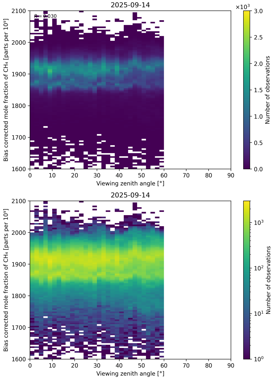
Figure 111: Scatter density plot of “Viewing zenith angle” against “Bias corrected mole fraction of CH 4 ” for 2025-09-13 to 2025-09-15.
