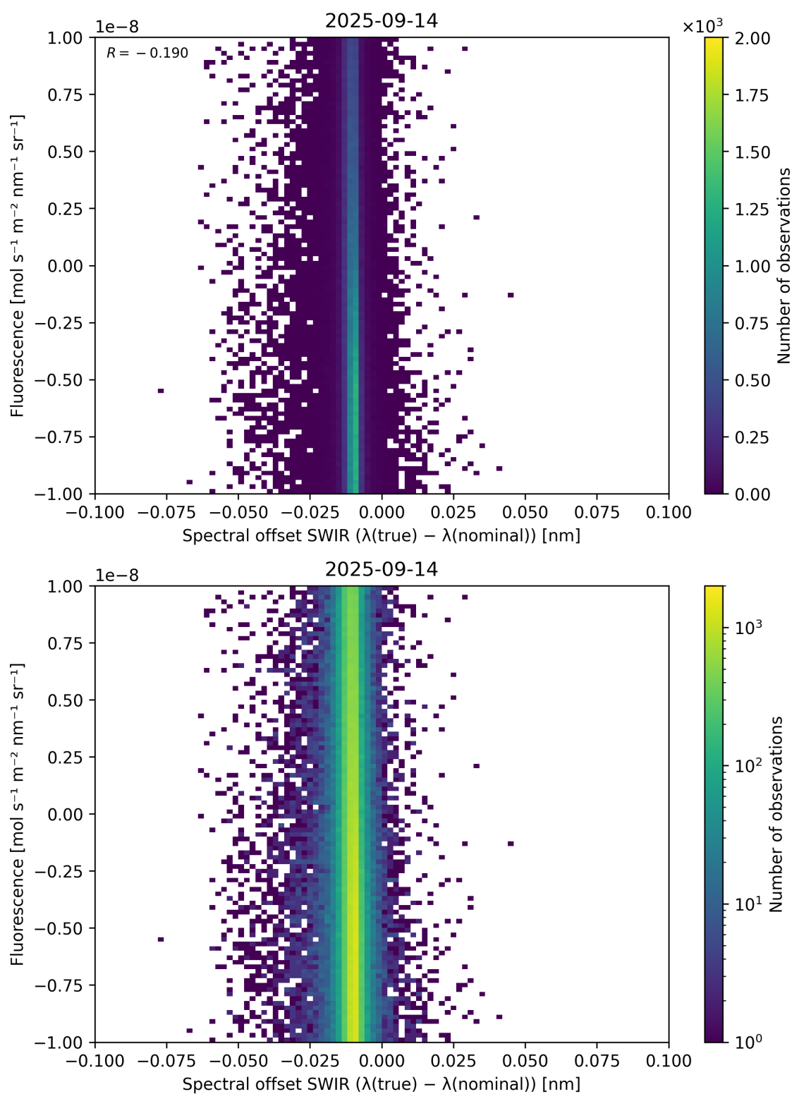
Figure 120: Scatter density plot of “Spectral offset SWIR ( \lambda_{\text{true}} - \lambda_{\text{nominal}} )” against “Fluorescence” for 2025-09-13 to 2025-09-15.
