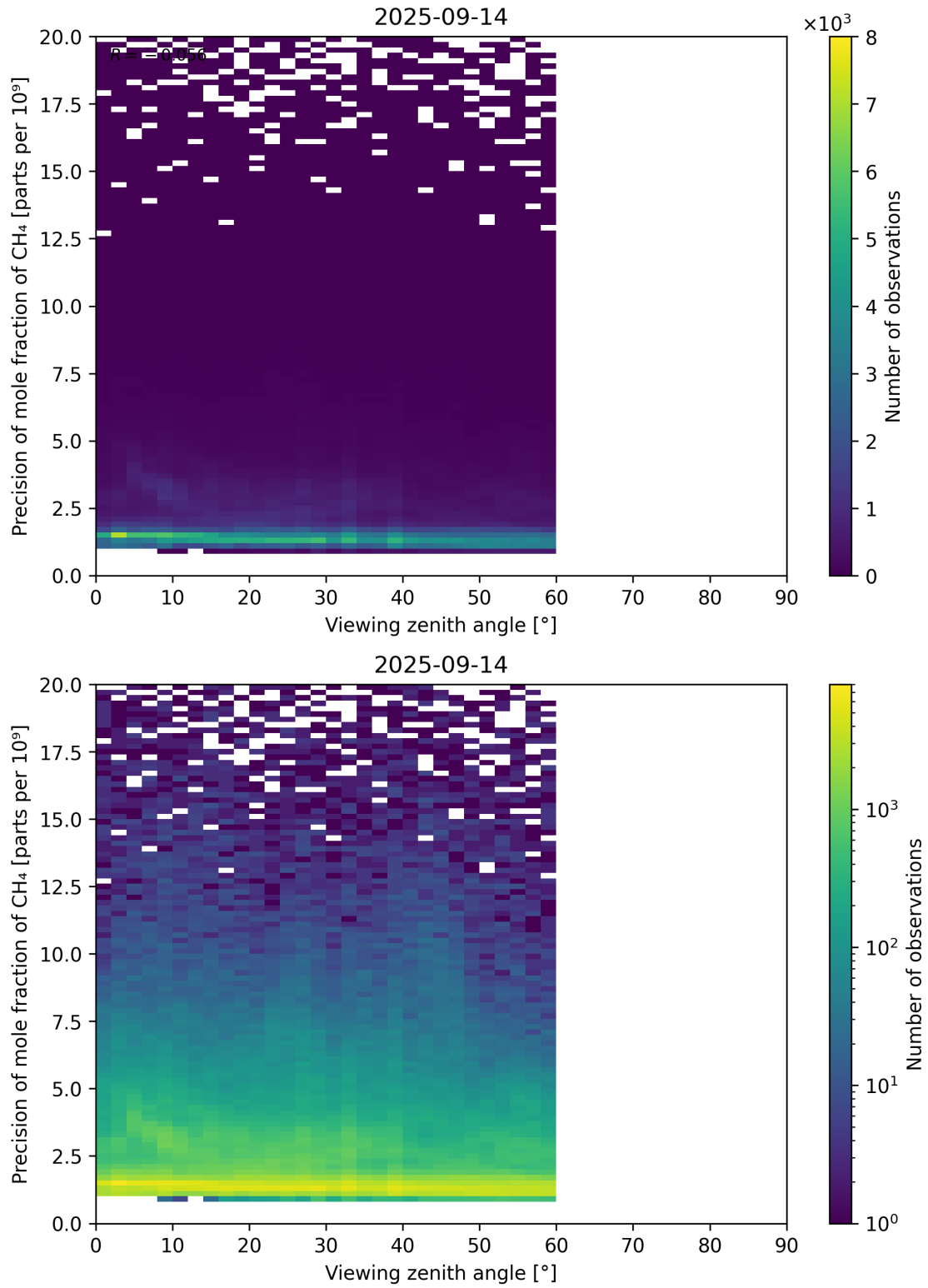
Figure 112: Scatter density plot of “Viewing zenith angle” against “Precision of mole fraction of CH 4 ” for 2025-09-13 to 2025-09-15.
