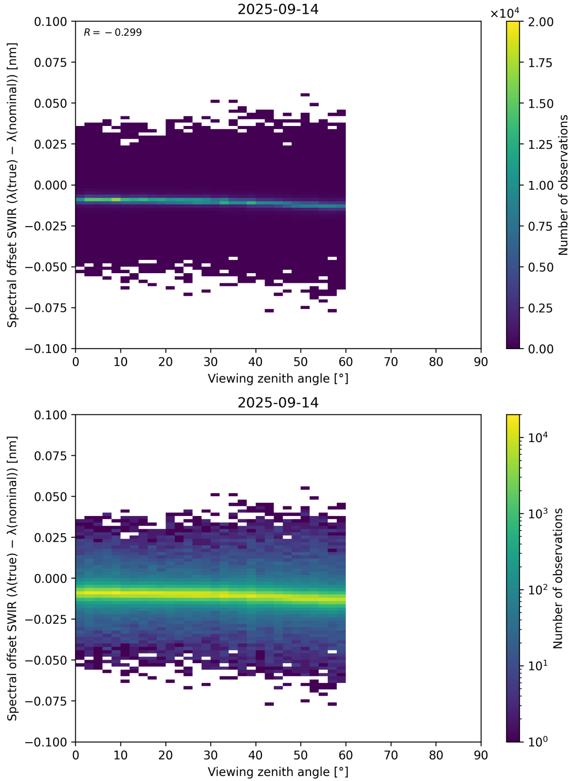
Figure 116: Scatter density plot of “Viewing zenith angle” against “Spectral offset SWIR ( \lambda_{\text{true}} - \lambda_{\text{nominal}} )” for 2025-09-13 to 2025-09-15.
