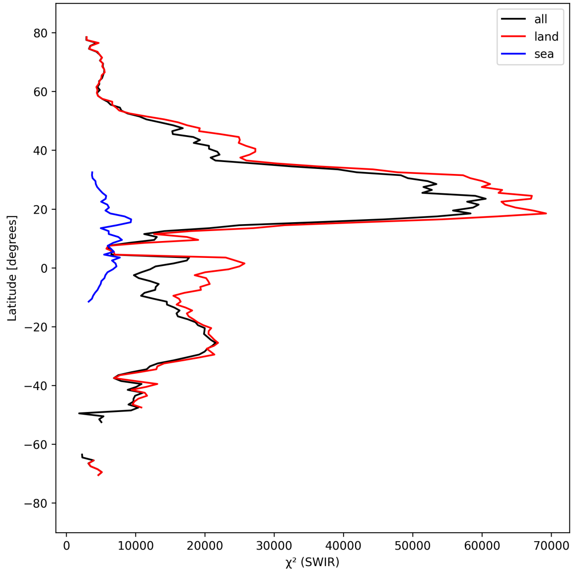
Figure 17: Zonal average of “ \chi^2 (SWIR)” for 2025-09-13 to 2025-09-15.
