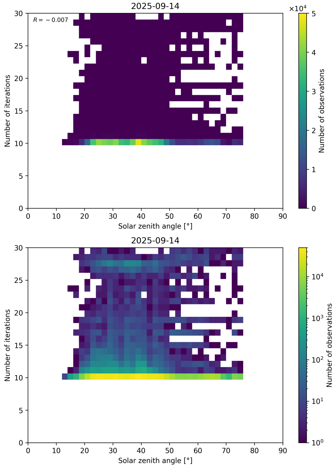
Figure 102: Scatter density plot of “Solar zenith angle” against “Number of iterations” for 2025-09-13 to 2025-09-15.
