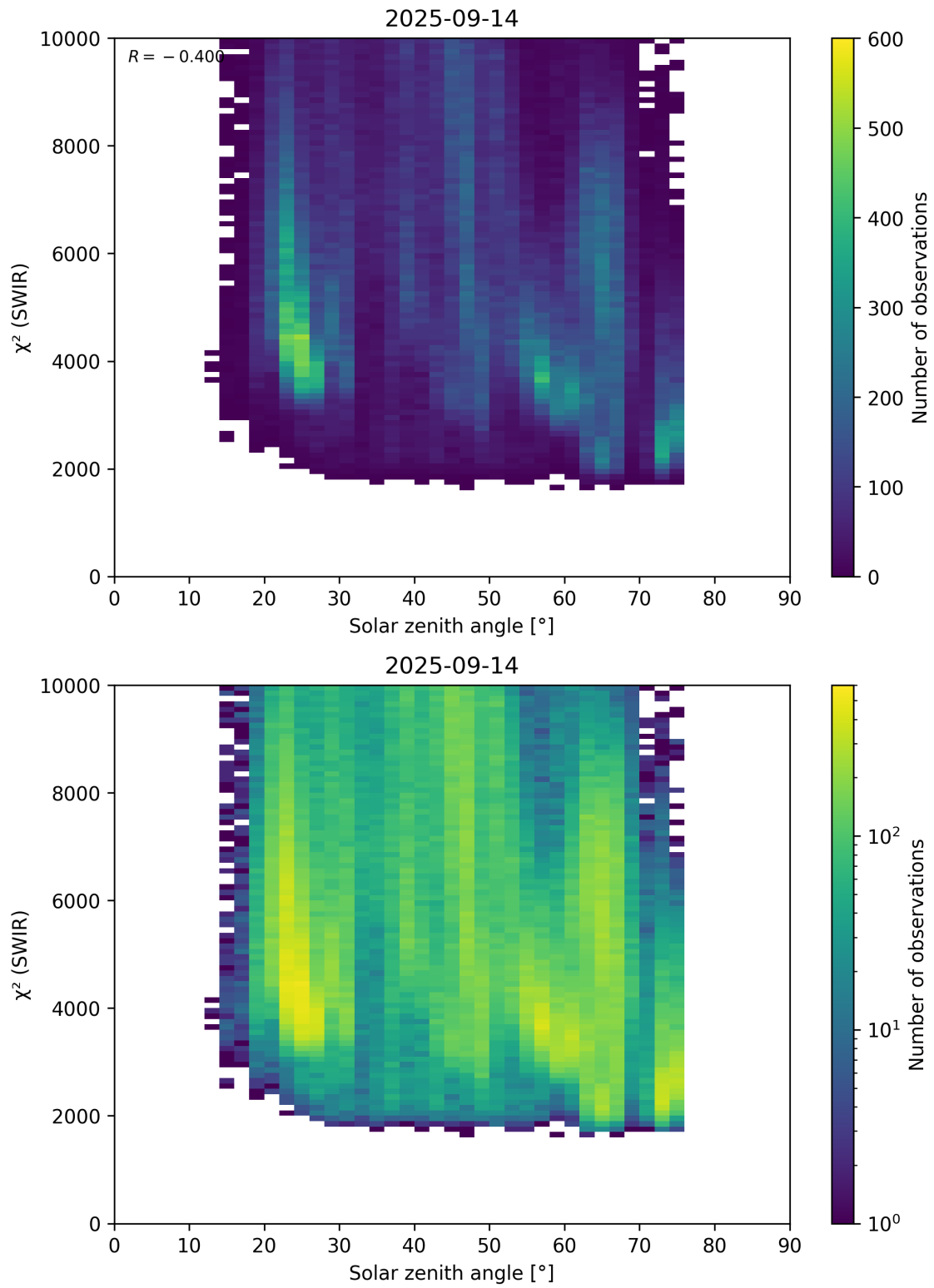
Figure 95: Scatter density plot of “Solar zenith angle” against “ \chi^2 (SWIR)” for 2025-09-13 to 2025-09-15.
