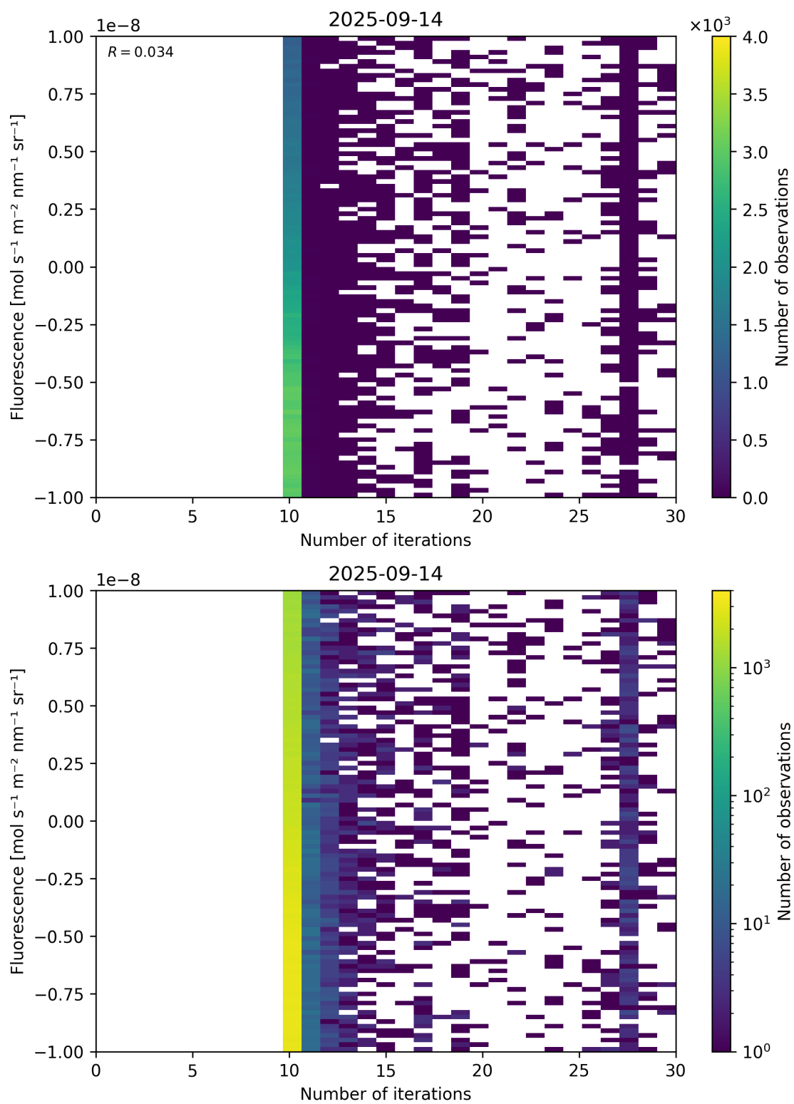
Figure 87: Scatter density plot of “Number of iterations” against “Fluorescence” for 2025-09-13 to 2025-09-15.
