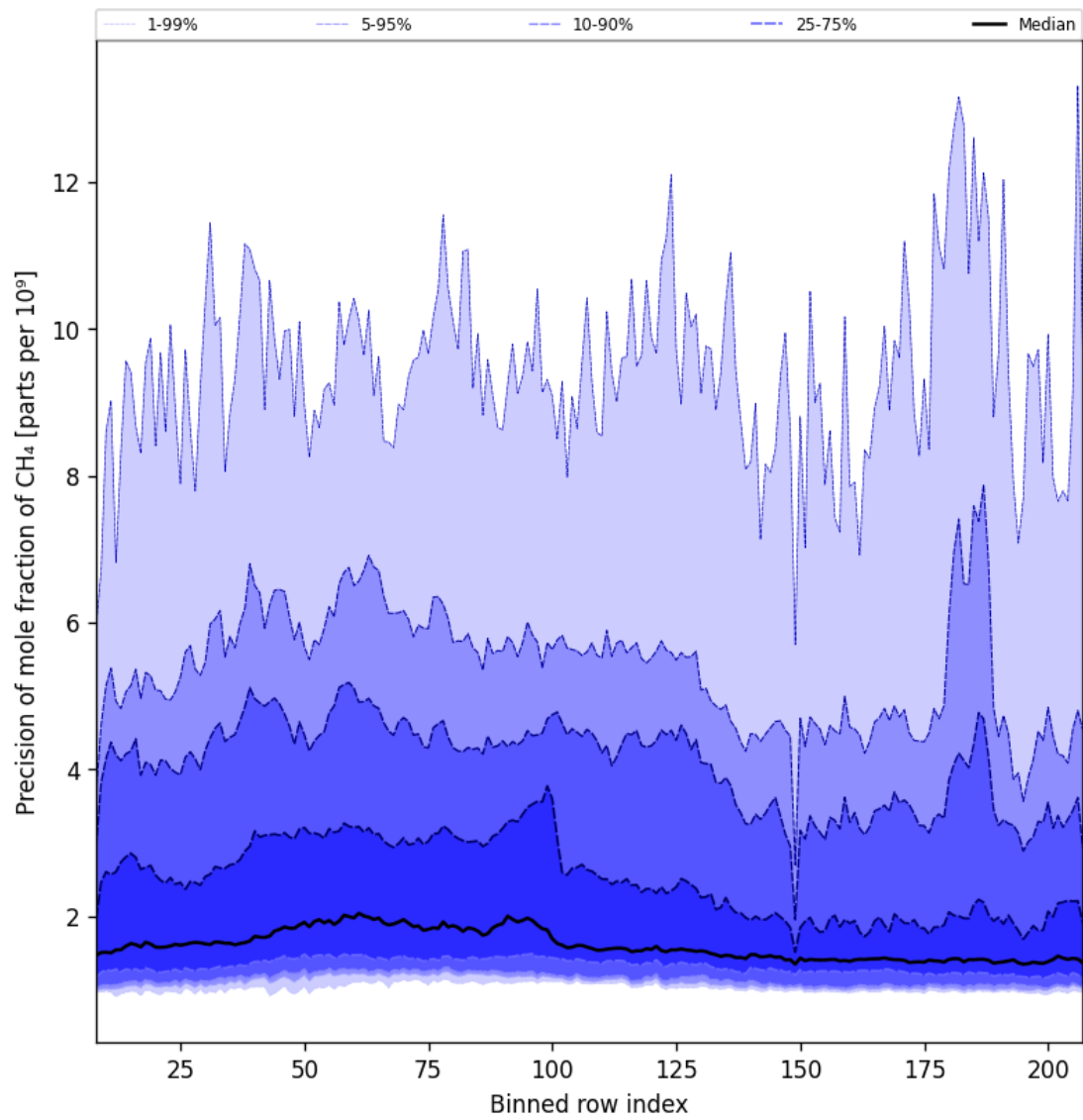
Figure 35: Along track statistics of “Precision of mole fraction of CH 4 ” for 2025-09-13 to 2025-09-15
