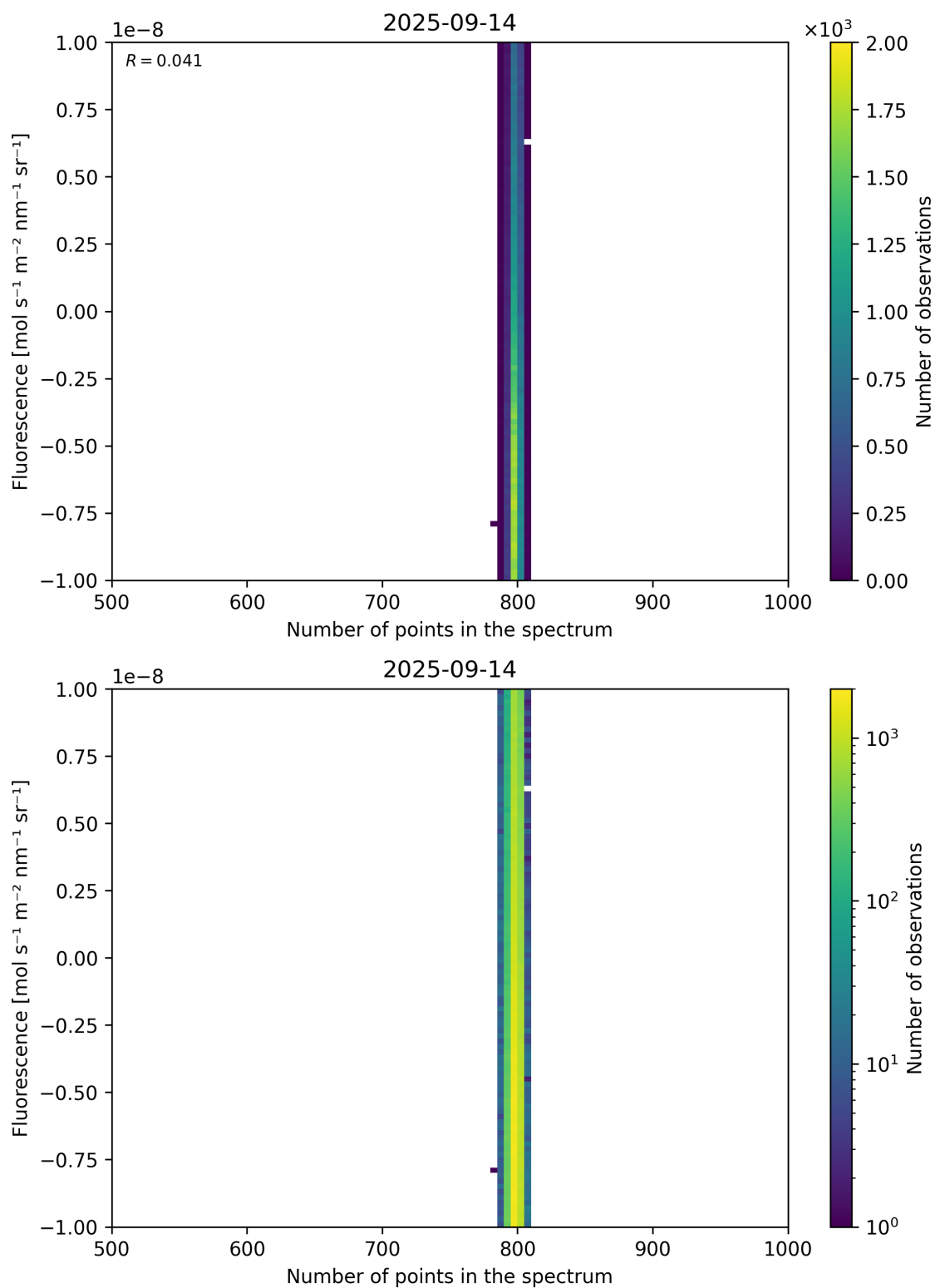
Figure 91: Scatter density plot of “Number of points in the spectrum” against “Fluorescence” for 2025-09-13 to 2025-09-15.
