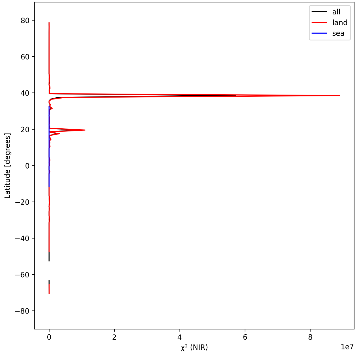
Figure 18: Zonal average of “ \chi^2 (NIR)” for 2025-09-13 to 2025-09-15.
