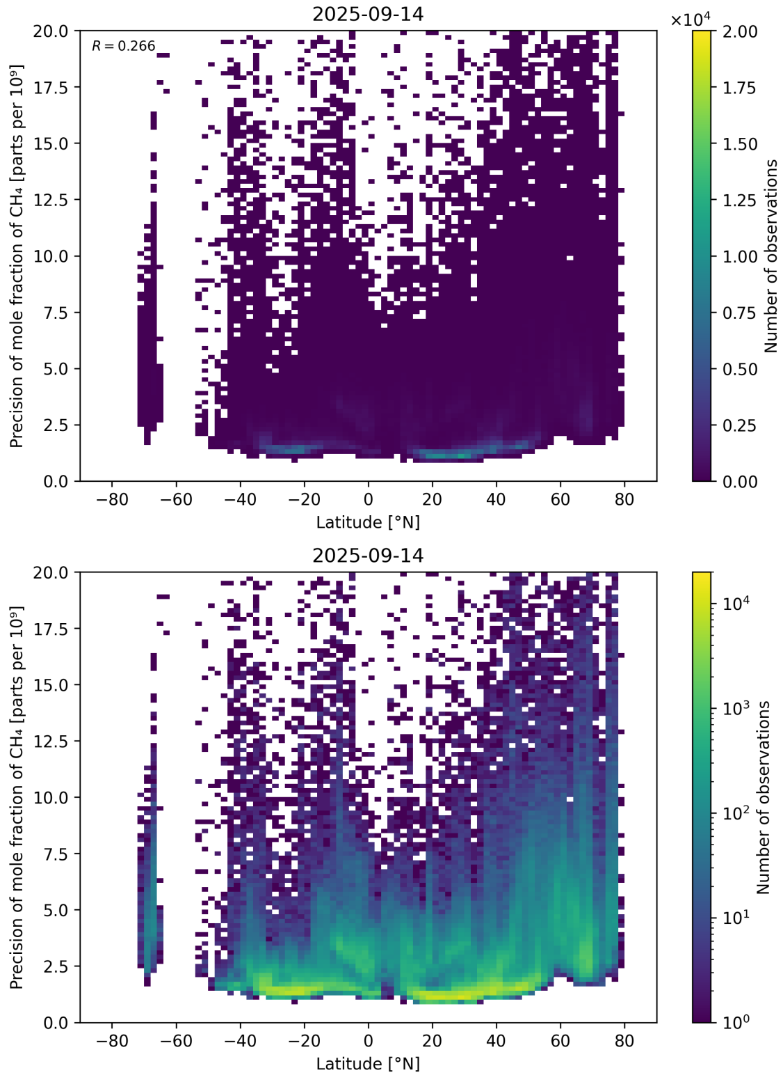
Figure 59: Scatter density plot of “Latitude” against “Precision of mole fraction of CH 4 ” for 2025-09-13 to 2025-09-15.
