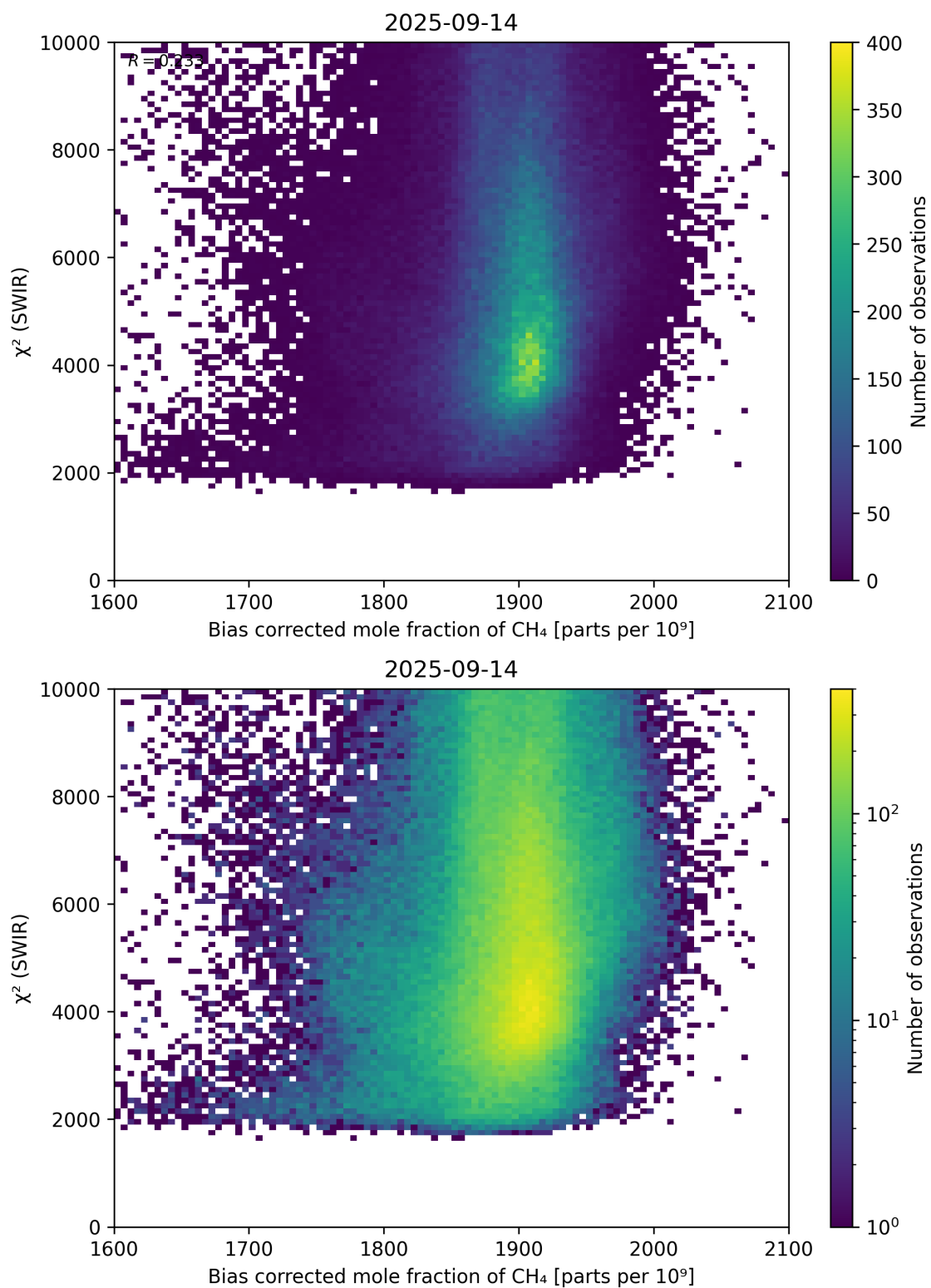
Figure 64: Scatter density plot of “Bias corrected mole fraction of \text{CH}_4 ” against “ \chi^2 (SWIR)” for 2025-09-13 to 2025-09-15.
