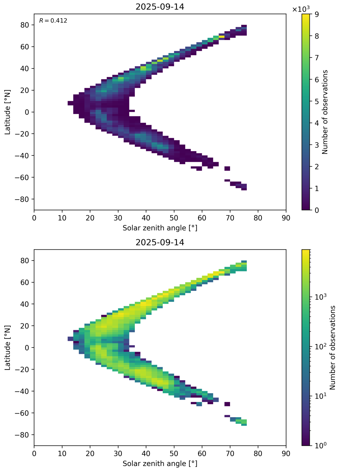
Figure 98: Scatter density plot of “Solar zenith angle” against “Latitude” for 2025-09-13 to 2025-09-15.
