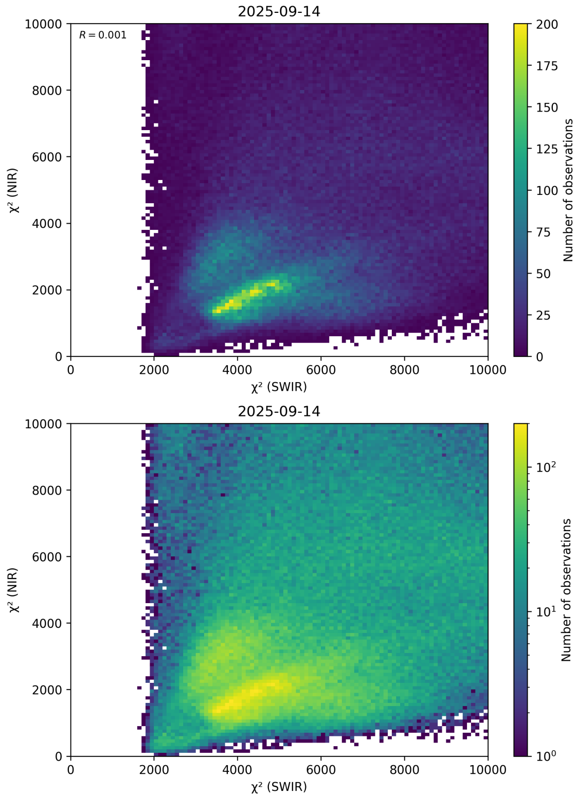
Figure 47: Scatter density plot of “ \chi^2 (SWIR)” against “ \chi^2 (NIR)” for 2025-09-13 to 2025-09-15.
