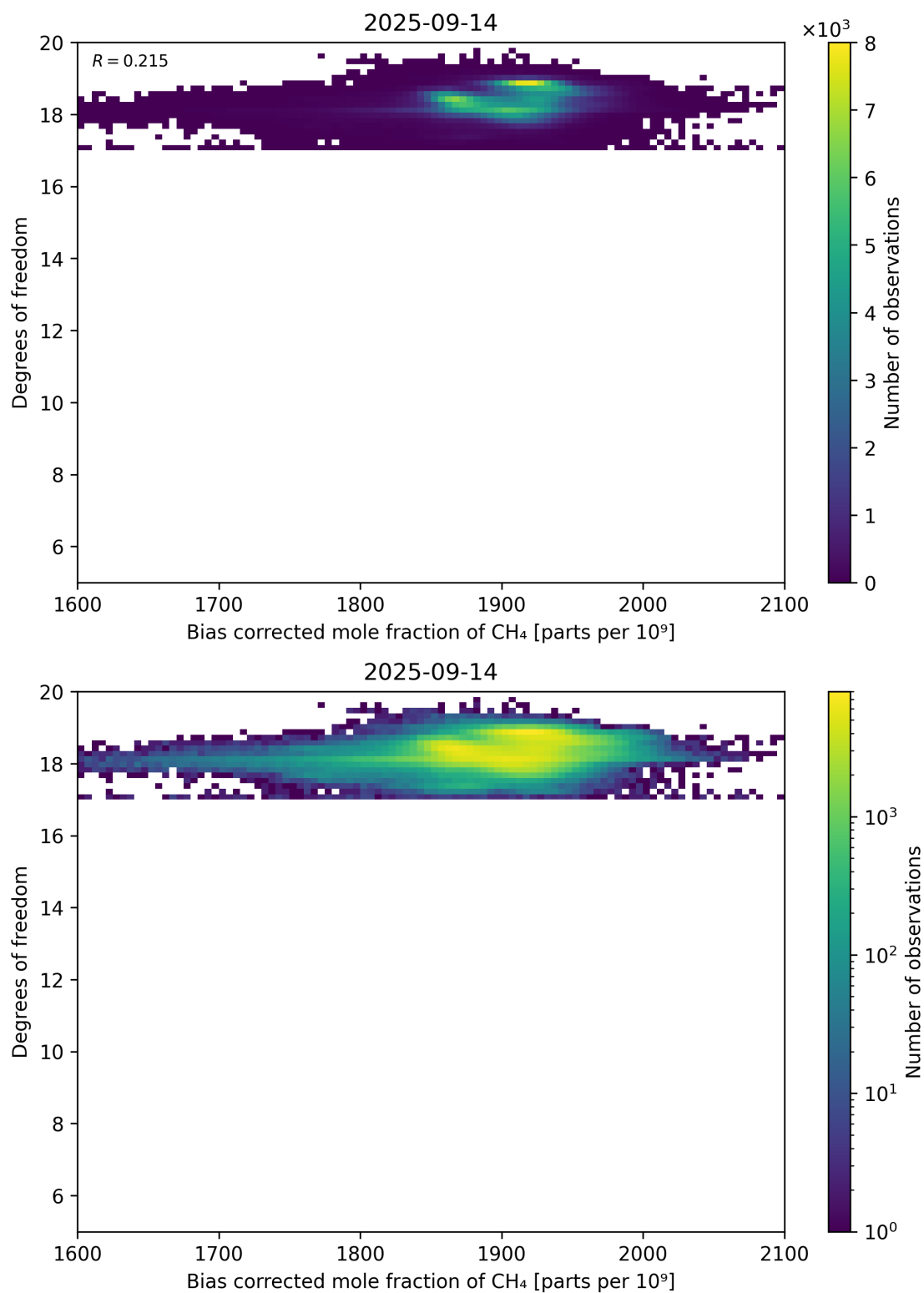
Figure 65: Scatter density plot of “Bias corrected mole fraction of CH 4 ” against “Degrees of freedom” for 2025-09-13 to 2025-09-15.
