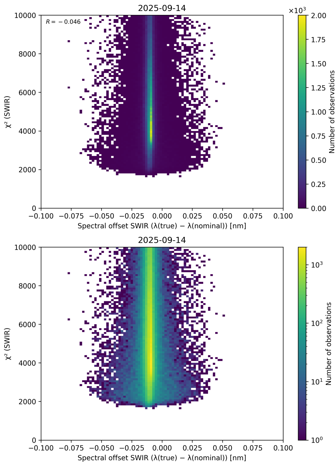
Figure 118: Scatter density plot of “Spectral offset SWIR ( \lambda_{\text{true}} - \lambda_{\text{nominal}} )” against “ \chi^2 (SWIR)” for 2025-09-13 to 2025-09-15.
