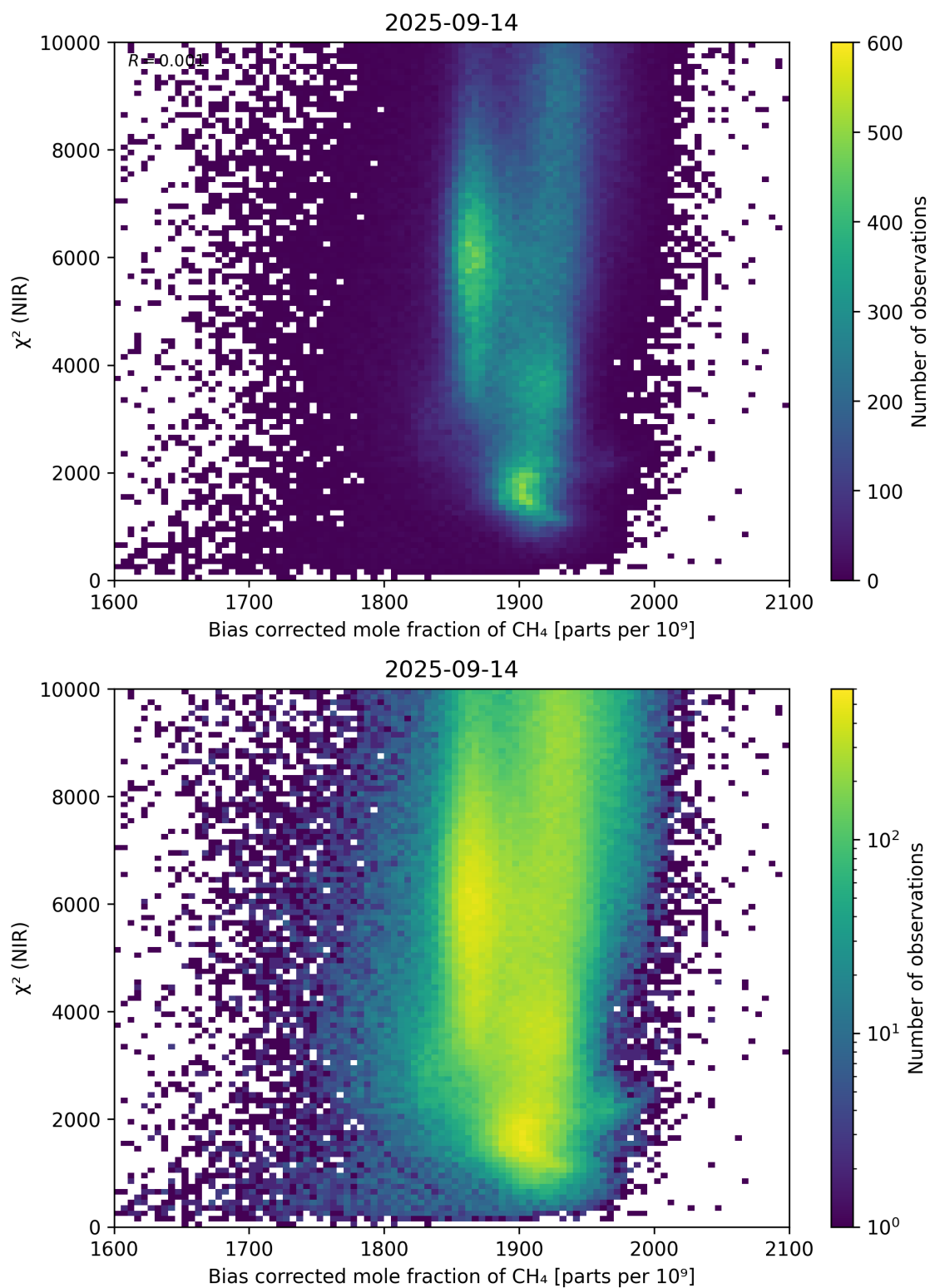
Figure 63: Scatter density plot of “Bias corrected mole fraction of \text{CH}_4 ” against “ \chi^2 (NIR)” for 2025-09-13 to 2025-09-15.
