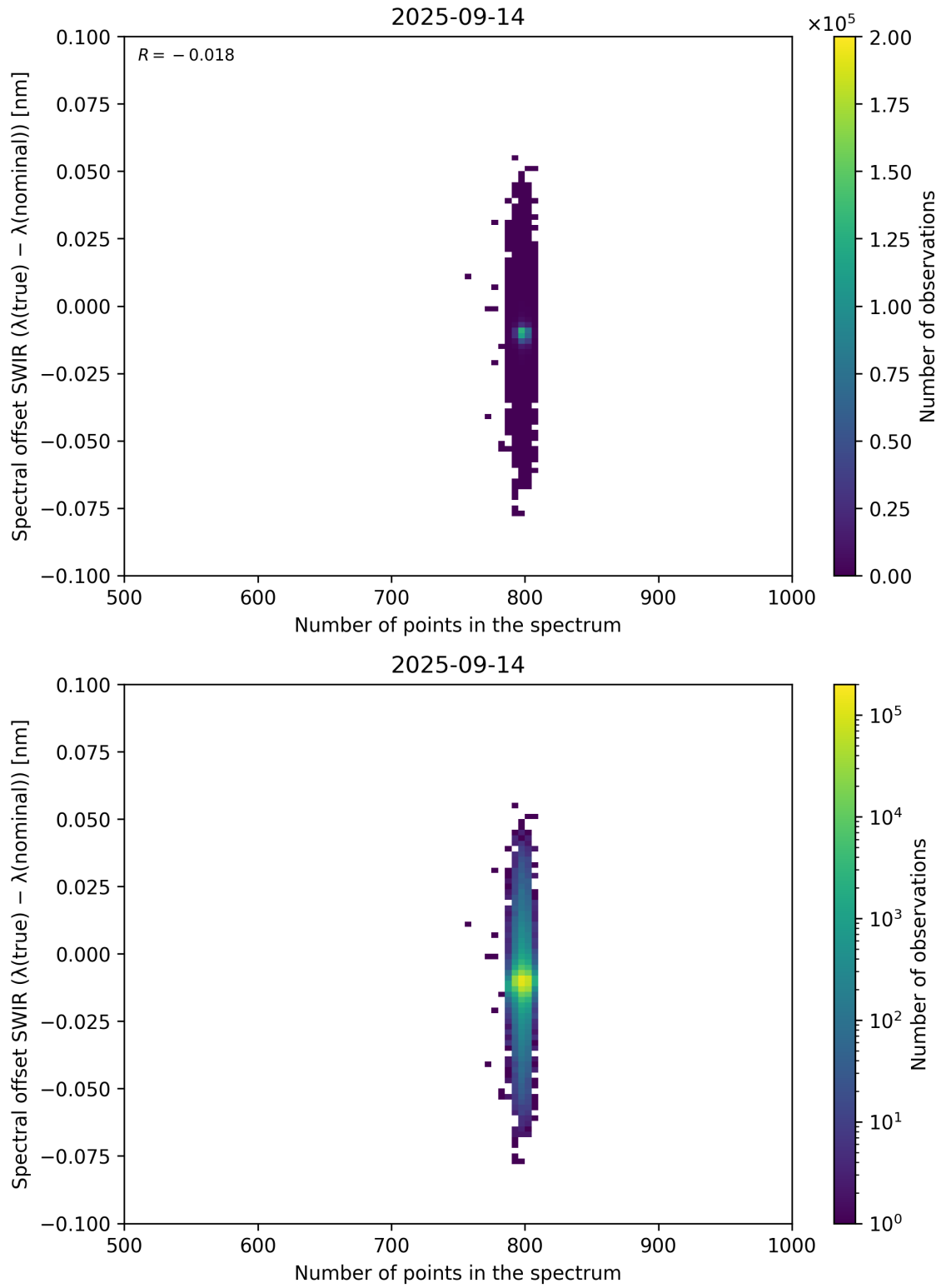
Figure 93: Scatter density plot of “Number of points in the spectrum” against “Spectral offset SWIR ( \lambda_{\text{true}} - \lambda_{\text{nominal}} )” for 2025-09-13 to 2025-09-15.
