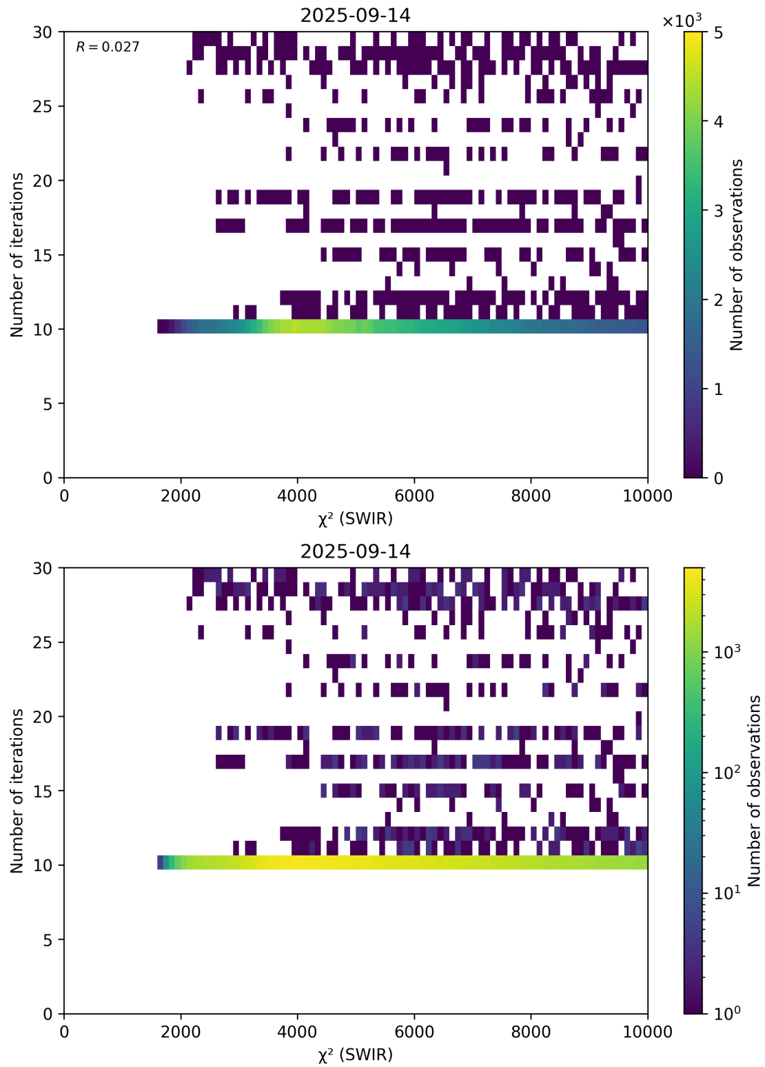
Figure 50: Scatter density plot of “ \chi^2 (SWIR)” against “Number of iterations” for 2025-09-13 to 2025-09-15.
