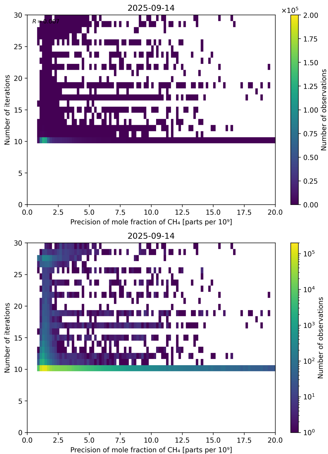
Figure 83: Scatter density plot of “Precision of mole fraction of CH 4 ” against “Number of iterations” for 2025-09-13 to 2025-09-15.
