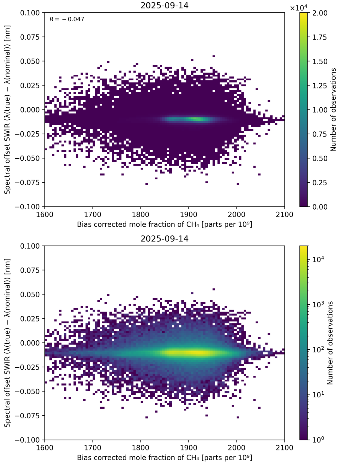
Figure 69: Scatter density plot of “Bias corrected mole fraction of \text{CH}_4 ” against “Spectral offset SWIR ( \lambda_{\text{true}} - \lambda_{\text{nominal}} )” for 2025-09-13 to 2025-09-15.
