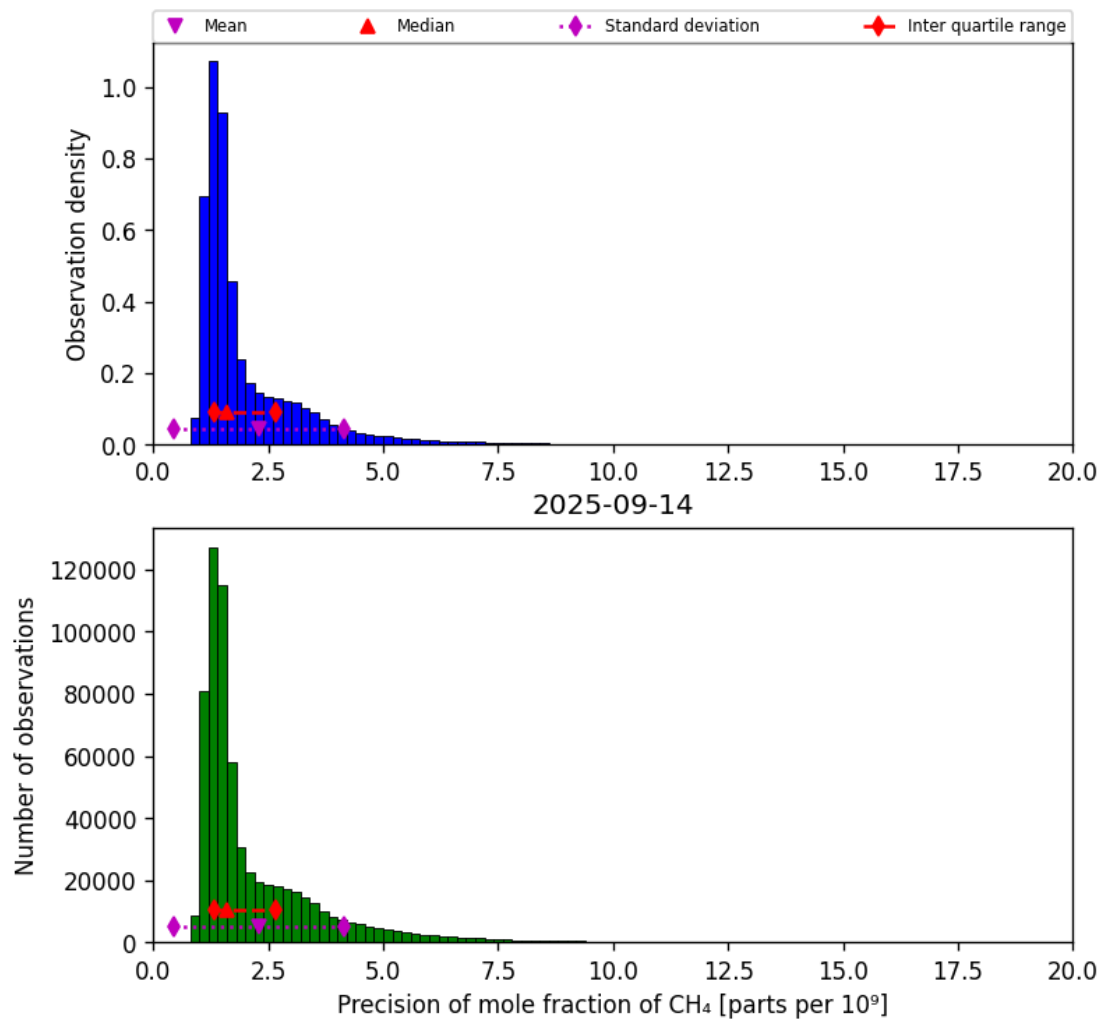
Figure 24: Histogram of “Precision of mole fraction of CH 4 ” for 2025-09-13 to 2025-09-15
