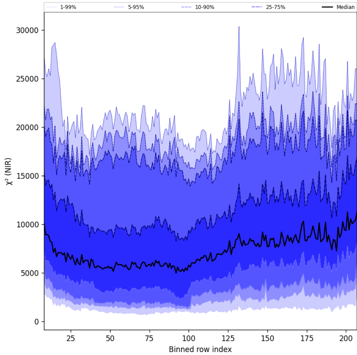
Figure 40: Along track statistics of “ \chi^2 (NIR)” for 2025-09-13 to 2025-09-15
