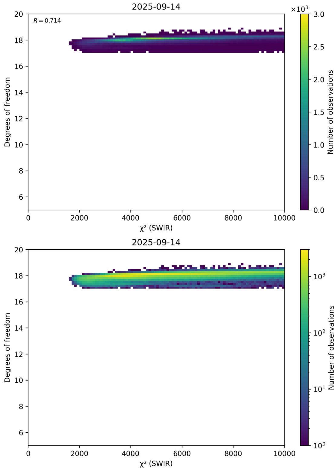
Figure 48: Scatter density plot of “ \chi^2 (SWIR)” against “Degrees of freedom” for 2025-09-13 to 2025-09-15.
