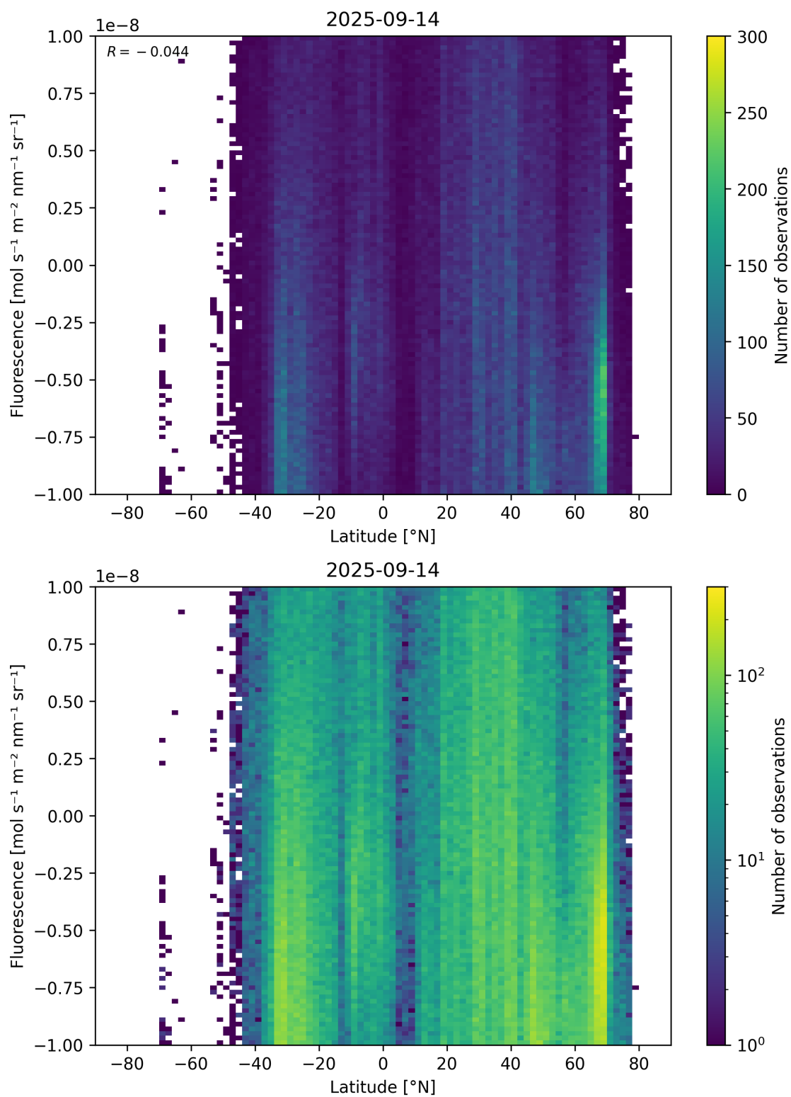
Figure 56: Scatter density plot of “Latitude” against “Fluorescence” for 2025-09-13 to 2025-09-15.
