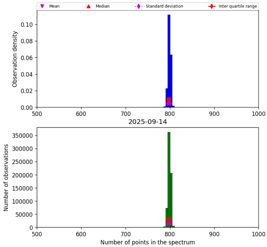
Figure 26: Histogram of “Number of points in the spectrum” for 2025-09-13 to 2025-09-15
