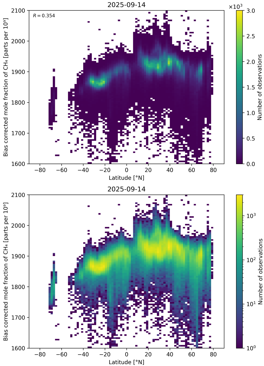
Figure 58: Scatter density plot of “Latitude” against “Bias corrected mole fraction of \text{CH}_4 ” for 2025-09-13 to 2025-09-15.
