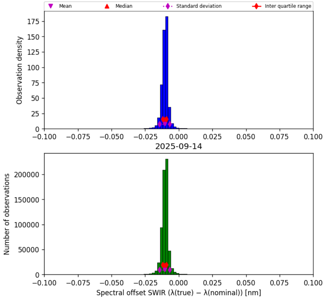
Figure 27: Histogram of “Spectral offset SWIR ( \lambda_{\text{true}} - \lambda_{\text{nominal}} )” for 2025-09-13 to 2025-09-15
