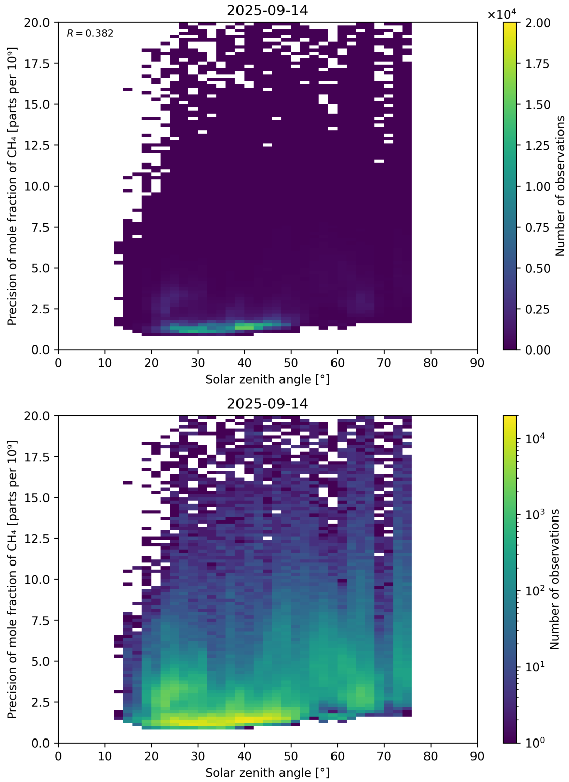
Figure 101: Scatter density plot of “Solar zenith angle” against “Precision of mole fraction of \text{CH}_4 ” for 2025-09-13 to 2025-09-15.
