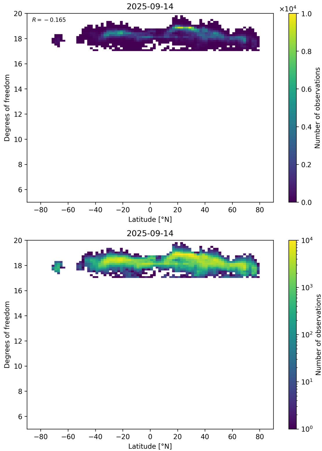
Figure 55: Scatter density plot of “Latitude” against “Degrees of freedom” for 2025-09-13 to 2025-09-15.
