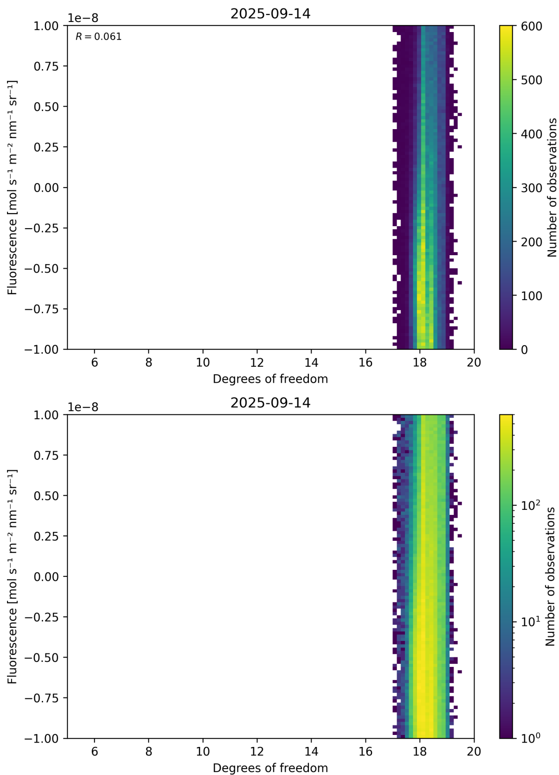
Figure 51: Scatter density plot of “Degrees of freedom” against “Fluorescence” for 2025-09-13 to 2025-09-15.
