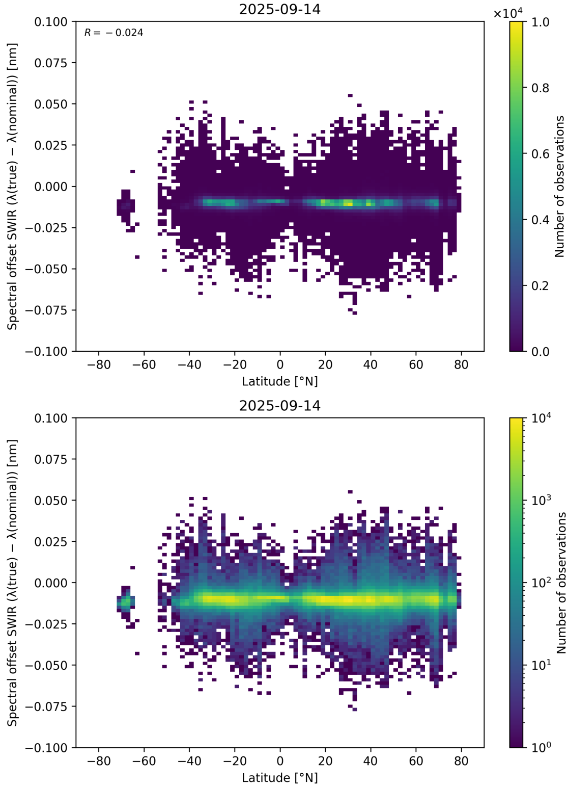
Figure 62: Scatter density plot of “Latitude” against “Spectral offset SWIR ( \lambda_{\text{true}} - \lambda_{\text{nominal}} )” for 2025-09-13 to 2025-09-15.
