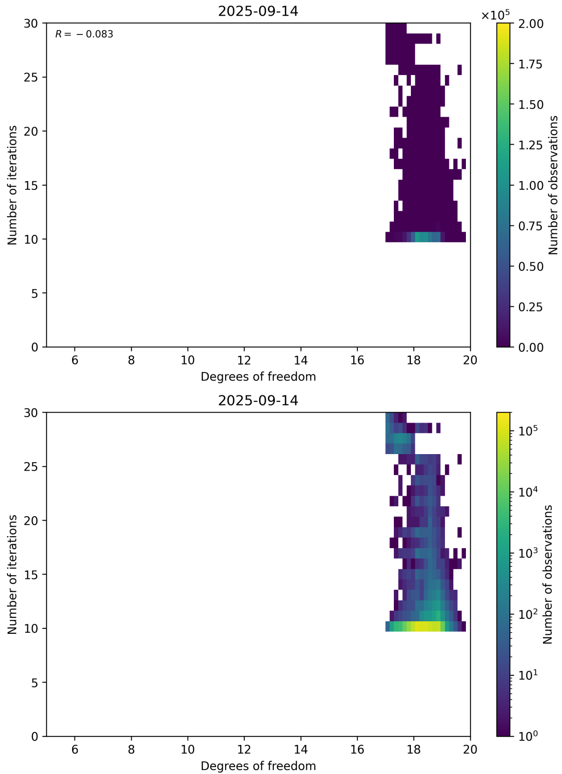
Figure 52: Scatter density plot of “Degrees of freedom” against “Number of iterations” for 2025-09-13 to 2025-09-15.
