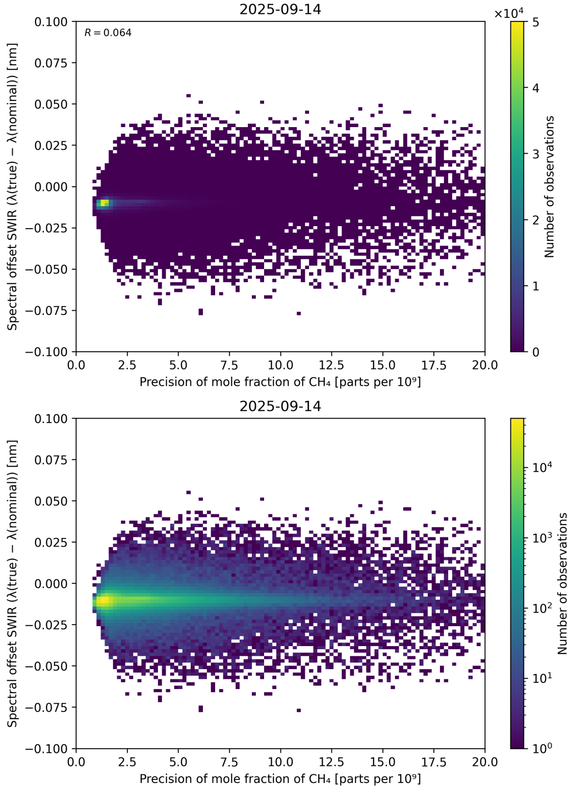
Figure 85: Scatter density plot of “Precision of mole fraction of CH 4 ” against “Spectral offset SWIR ( \lambda_{\text{true}} - \lambda_{\text{nominal}} )” for 2025-09-13 to 2025-09-15.
