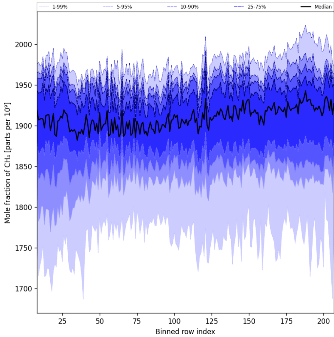
Figure 34: Along track statistics of “Mole fraction of CH 4 ” for 2025-09-13 to 2025-09-15
