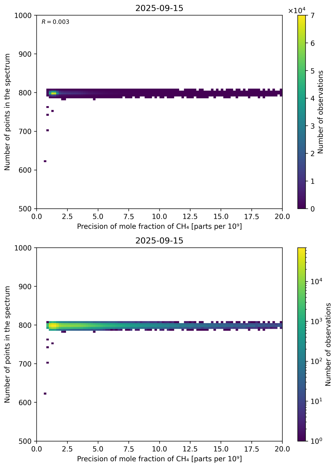
Figure 84: Scatter density plot of “Precision of mole fraction of CH 4 ” against “Number of points in the spectrum” for 2025-09-15 to 2025-09-16.
