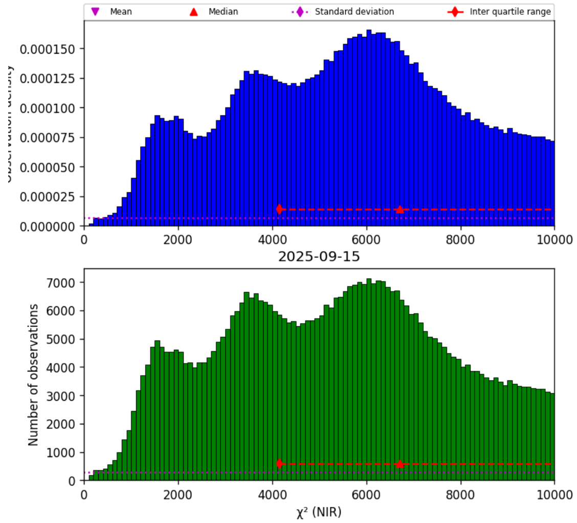
Figure 29: Histogram of “ \chi^2 (NIR)” for 2025-09-15 to 2025-09-16
