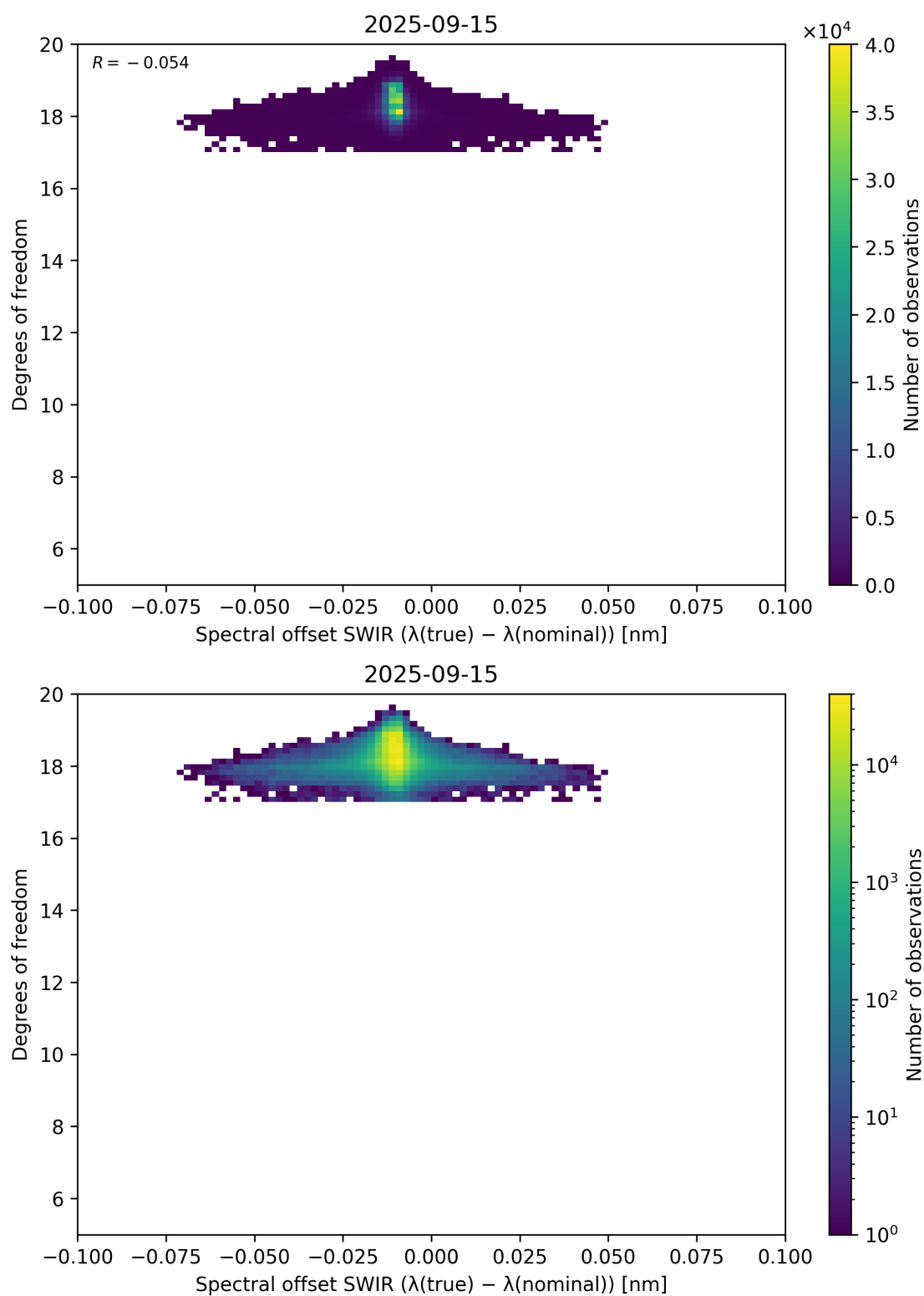
Figure 119: Scatter density plot of “Spectral offset SWIR ( \lambda_{\text{true}} - \lambda_{\text{nominal}} )” against “Degrees of freedom” for 2025-09-15 to 2025-09-16.
