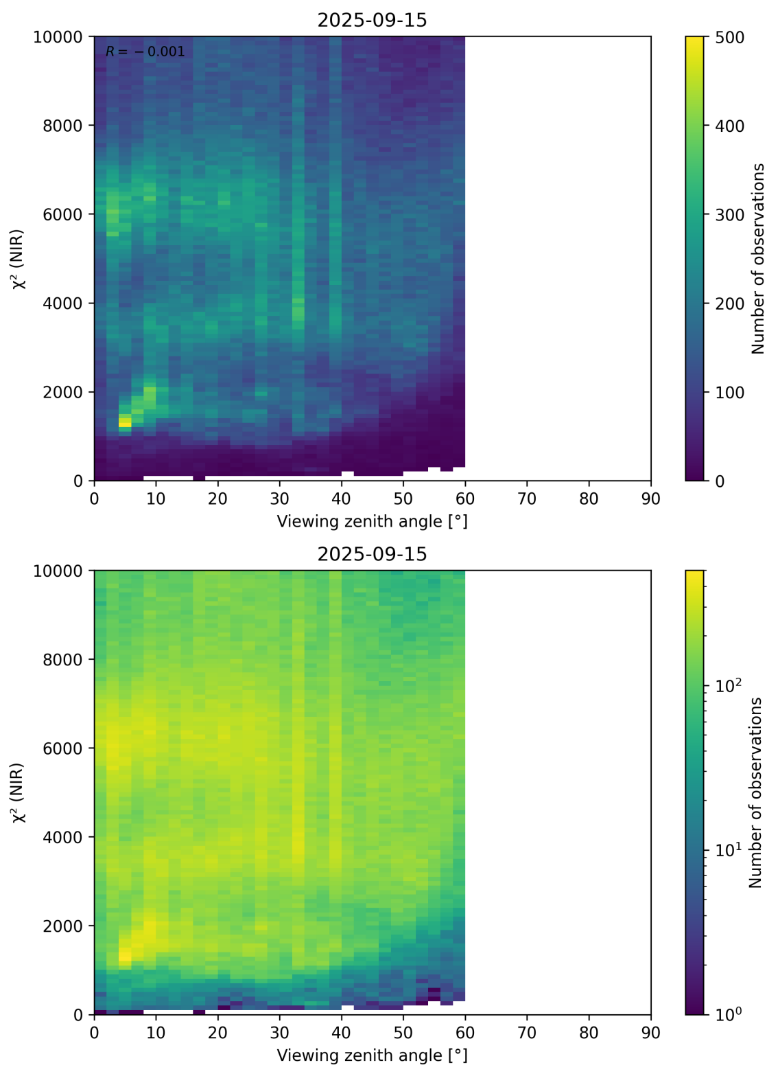
Figure 105: Scatter density plot of “Viewing zenith angle” against “ \chi^2 (NIR)” for 2025-09-15 to 2025-09-16.
