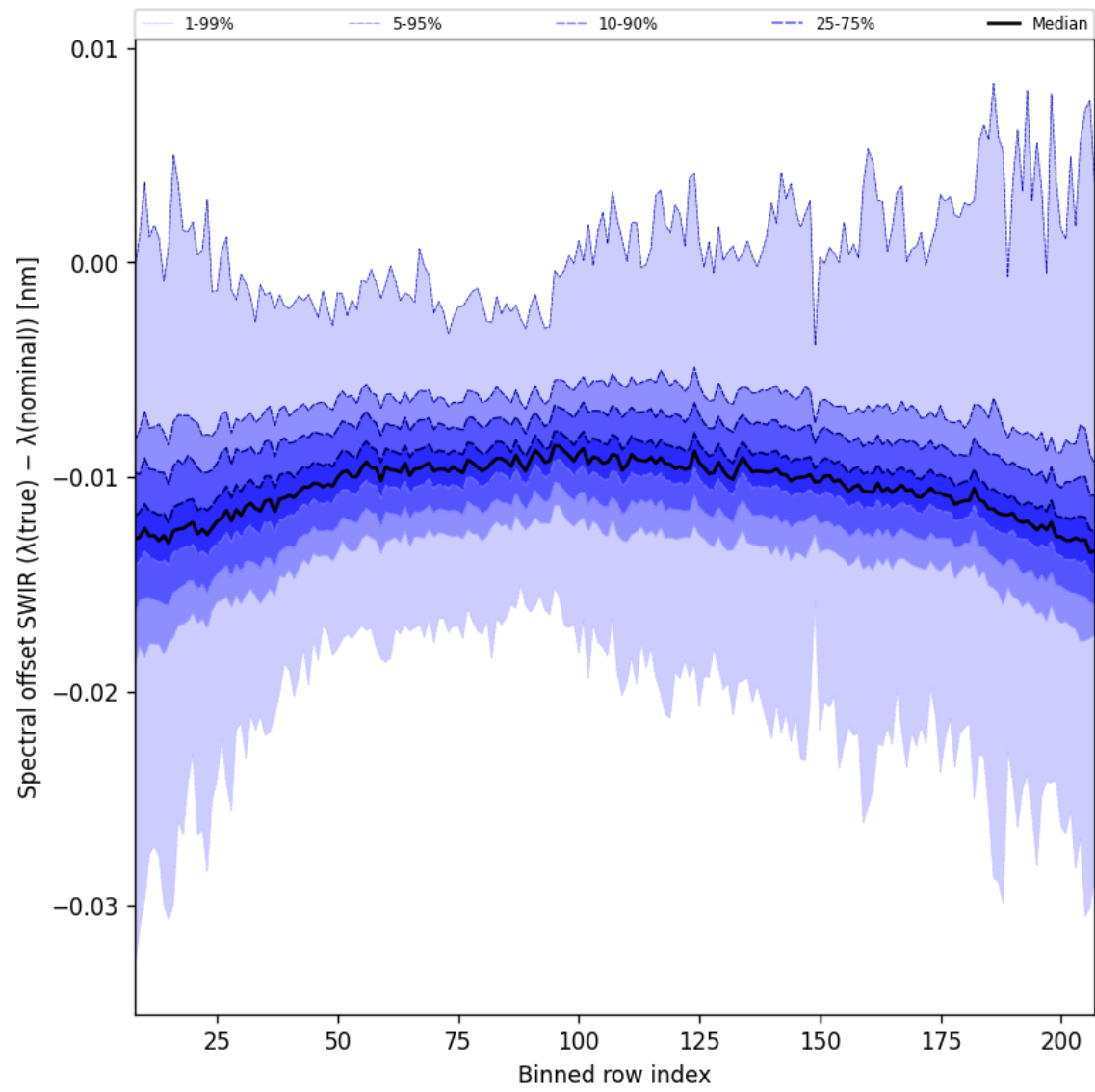
Figure 38: Along track statistics of “Spectral offset SWIR ( \lambda_{\text{true}} - \lambda_{\text{nominal}} )” for 2025-09-15 to 2025-09-16
