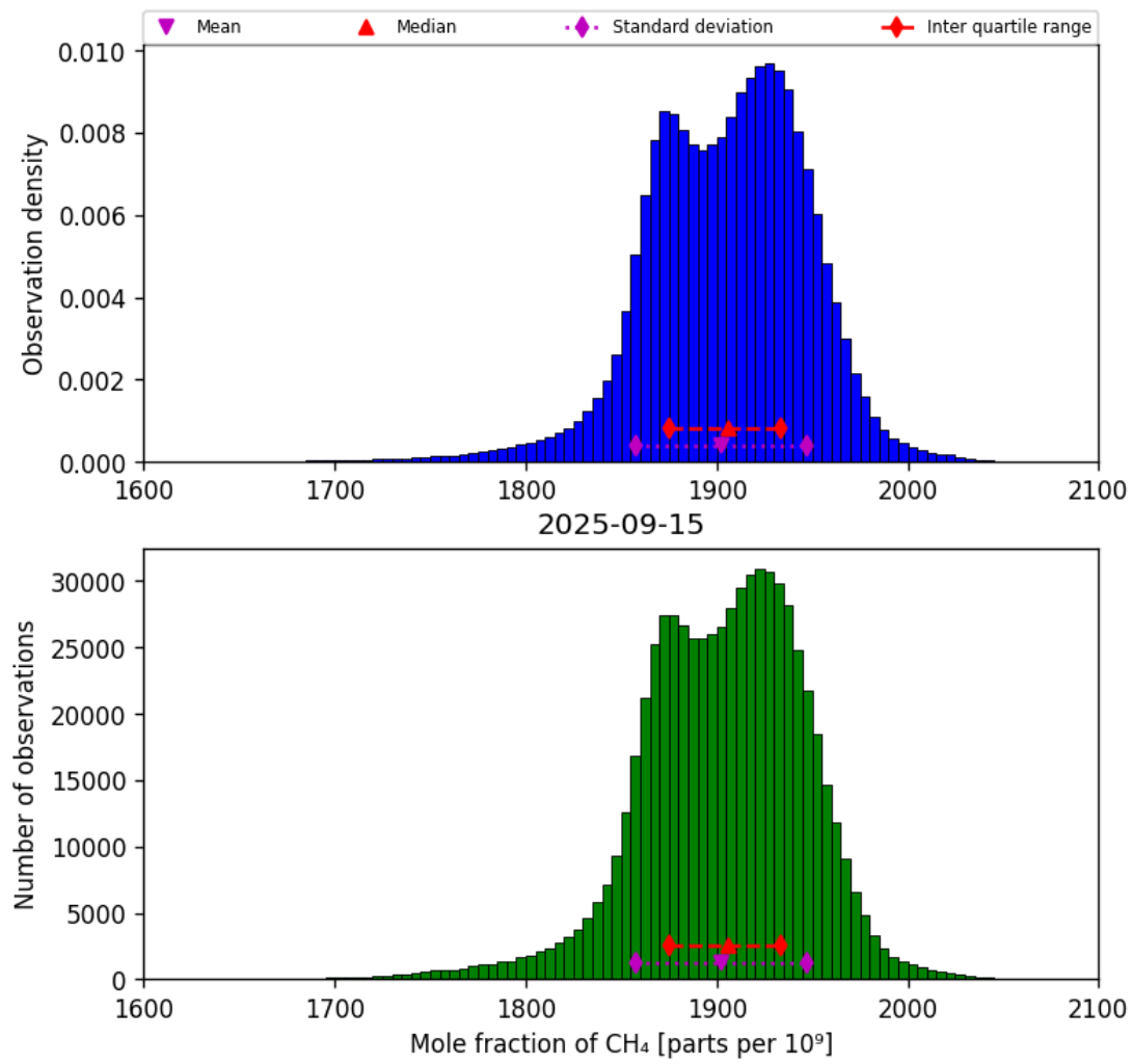
Figure 23: Histogram of “Mole fraction of CH 4 ” for 2025-09-15 to 2025-09-16
