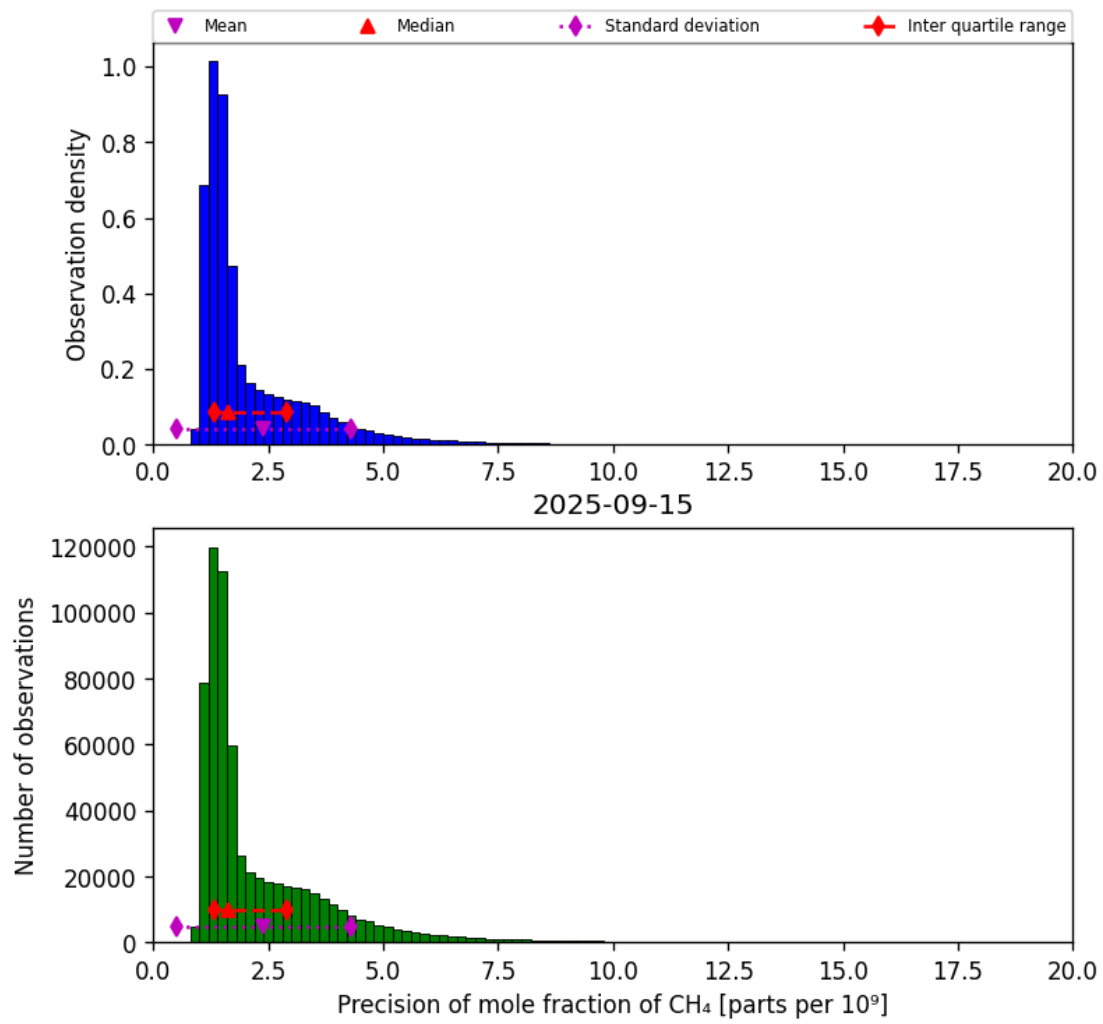
Figure 24: Histogram of “Precision of mole fraction of CH 4 ” for 2025-09-15 to 2025-09-16
