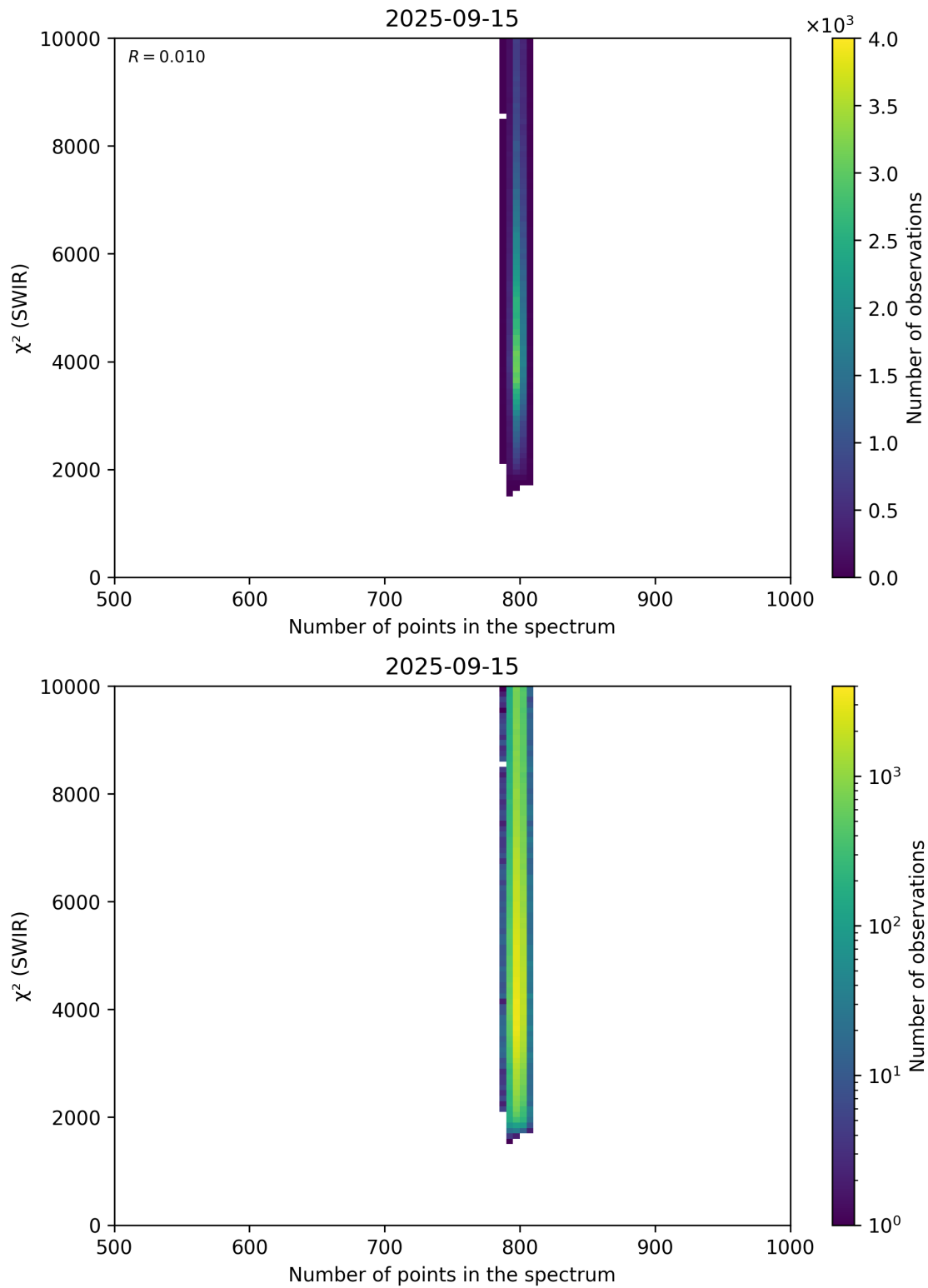
Figure 89: Scatter density plot of “Number of points in the spectrum” against “ \chi^2 (SWIR)” for 2025-09-15 to 2025-09-16.
