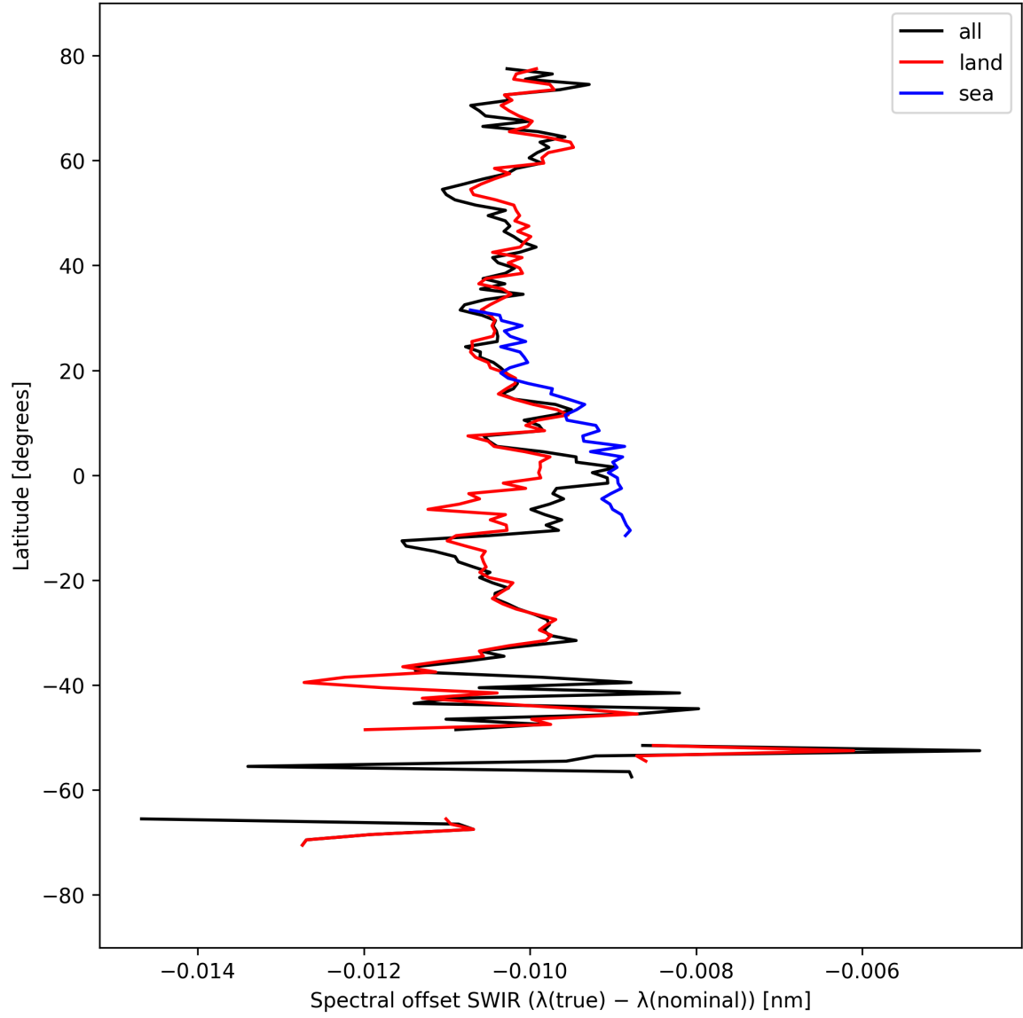
Figure 16: Zonal average of “Spectral offset SWIR ( \lambda_{\text{true}} - \lambda_{\text{nominal}} )” for 2025-09-15 to 2025-09-16.
