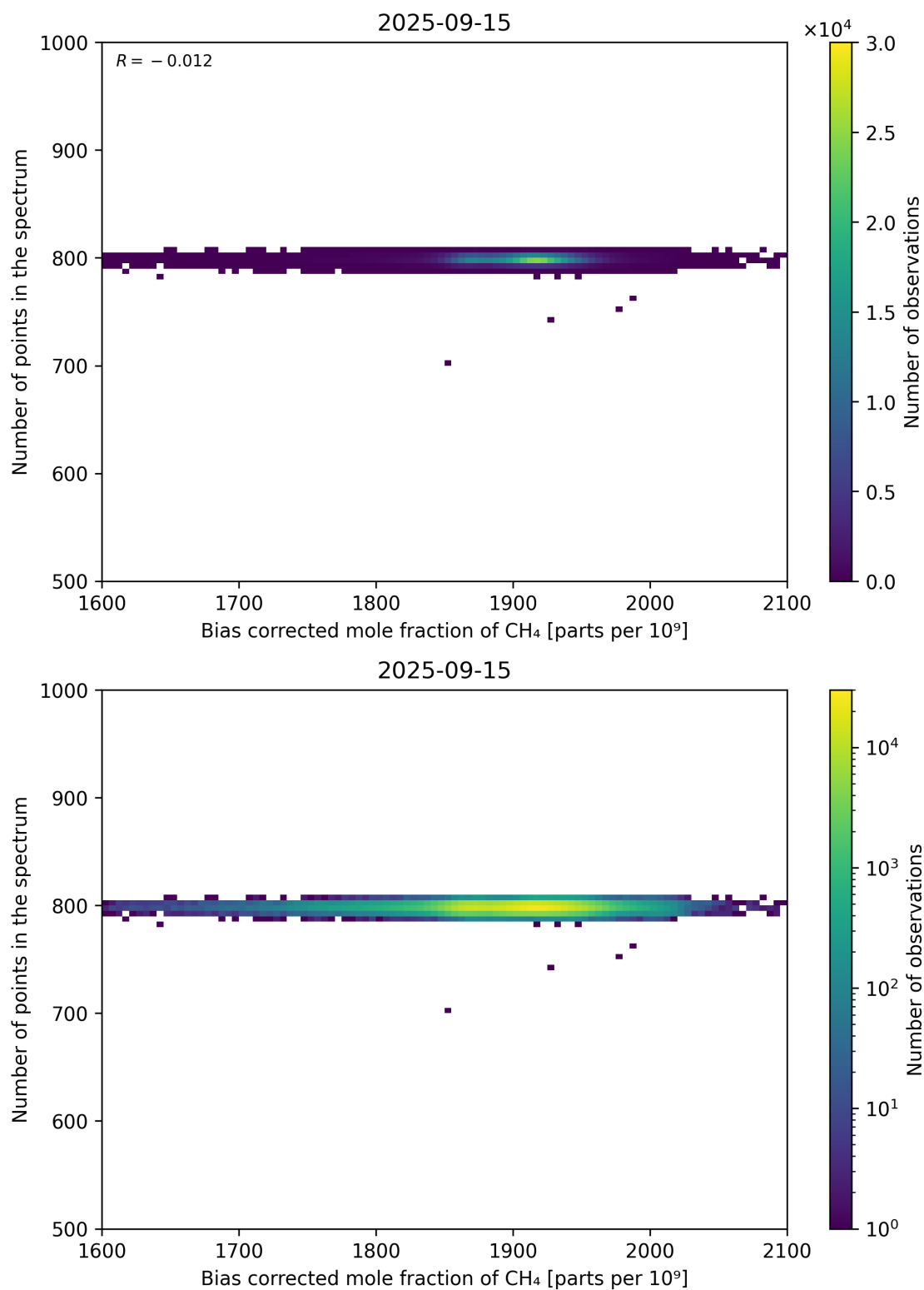
Figure 68: Scatter density plot of “Bias corrected mole fraction of CH 4 ” against “Number of points in the spectrum” for 2025-09-15 to 2025-09-16.
