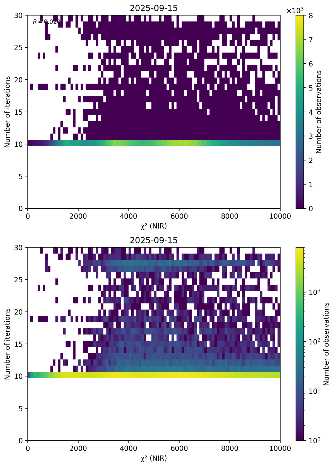
Figure 46: Scatter density plot of “ \chi^2 (NIR)” against “Number of iterations” for 2025-09-15 to 2025-09-16.
