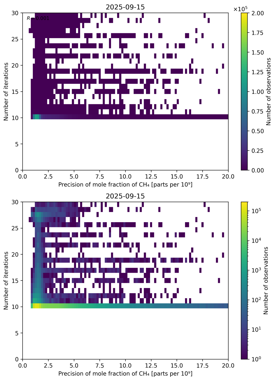
Figure 83: Scatter density plot of “Precision of mole fraction of CH 4 ” against “Number of iterations” for 2025-09-15 to 2025-09-16.
