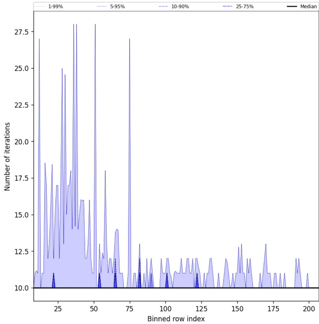
Figure 42: Along track statistics of “Number of iterations” for 2025-09-15 to 2025-09-16
