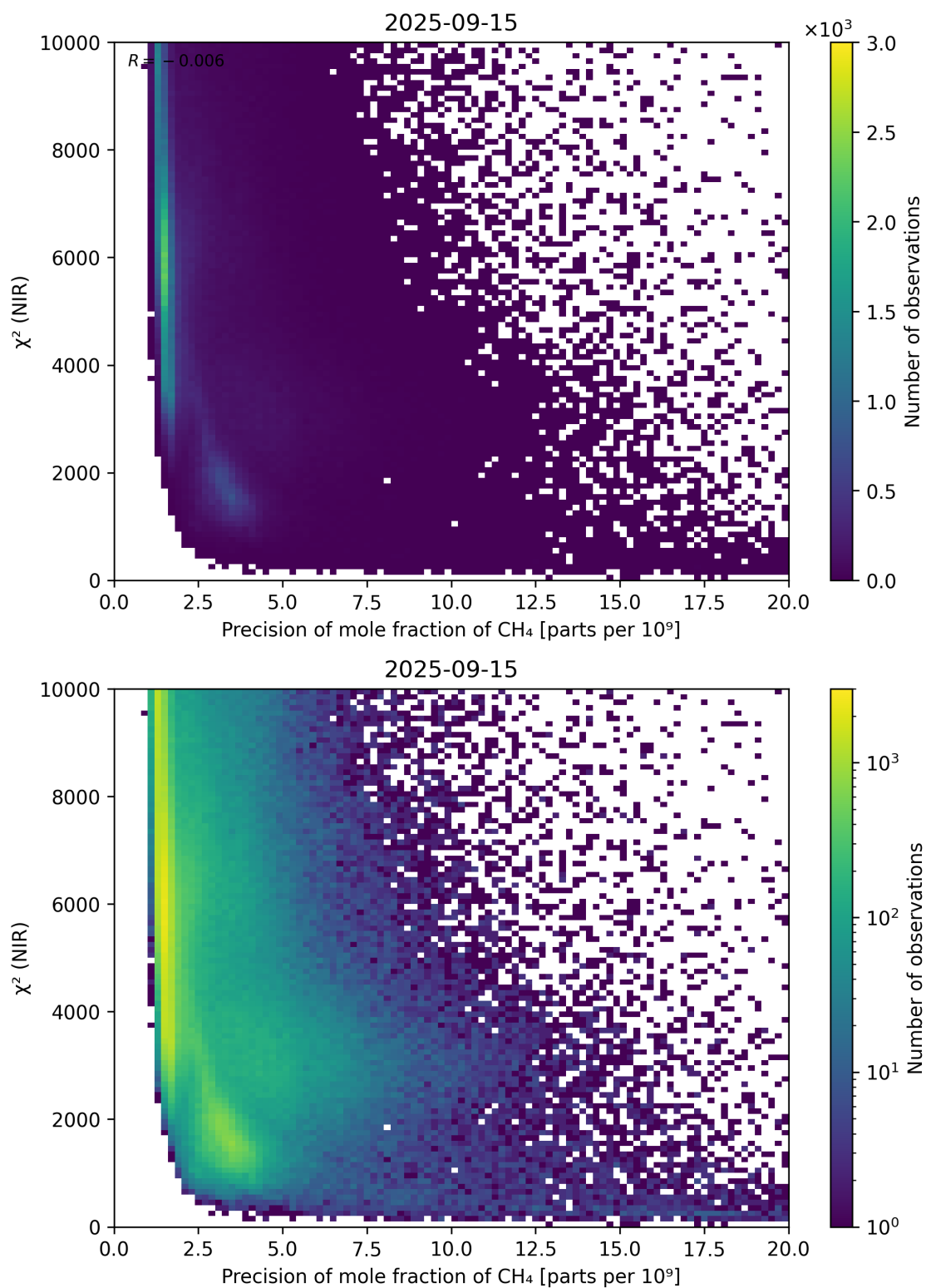
Figure 78: Scatter density plot of “Precision of mole fraction of CH 4 ” against “ \chi^2 (NIR)” for 2025-09-15 to 2025-09-16.
