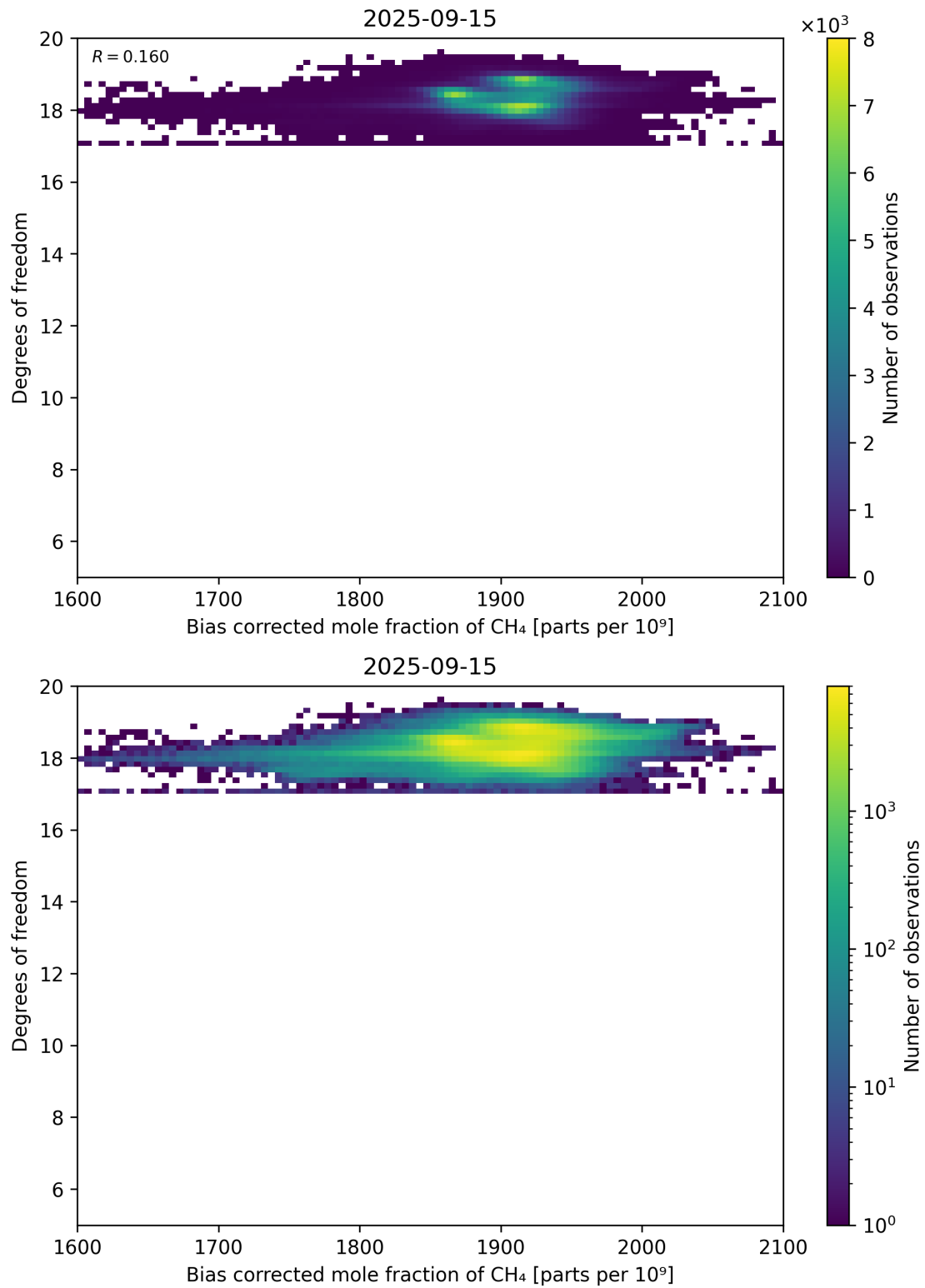
Figure 65: Scatter density plot of “Bias corrected mole fraction of CH 4 ” against “Degrees of freedom” for 2025-09-15 to 2025-09-16.
