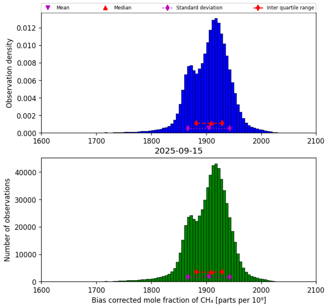
Figure 25: Histogram of “Bias corrected mole fraction of CH 4 ” for 2025-09-15 to 2025-09-16
