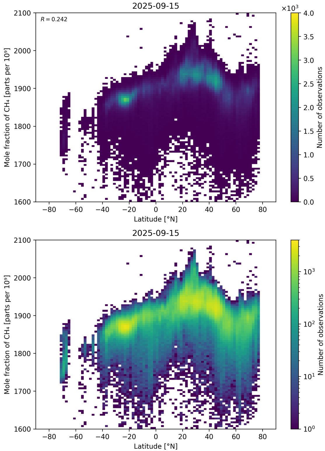
Figure 57: Scatter density plot of “Latitude” against “Mole fraction of \text{CH}_4 ” for 2025-09-15 to 2025-09-16.
