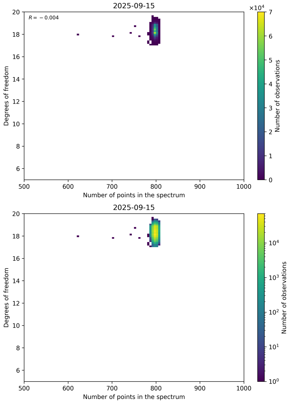
Figure 90: Scatter density plot of “Number of points in the spectrum” against “Degrees of freedom” for 2025-09-15 to 2025-09-16.
