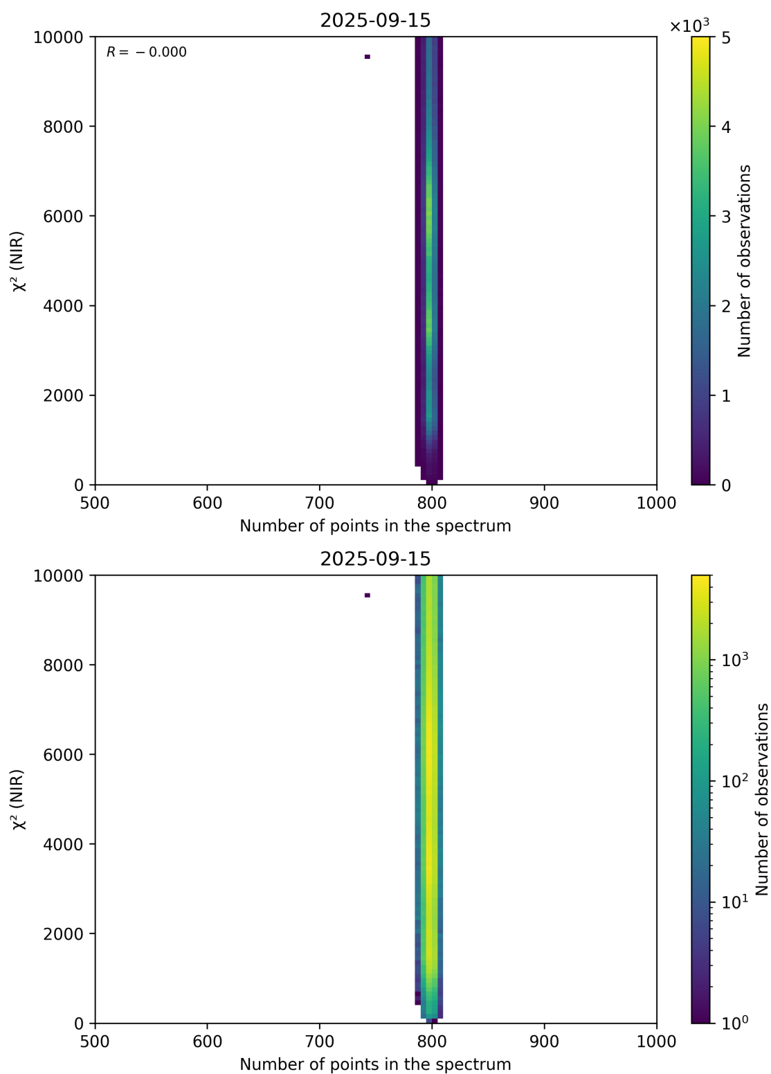
Figure 88: Scatter density plot of “Number of points in the spectrum” against “ \chi^2 (NIR)” for 2025-09-15 to 2025-09-16.
