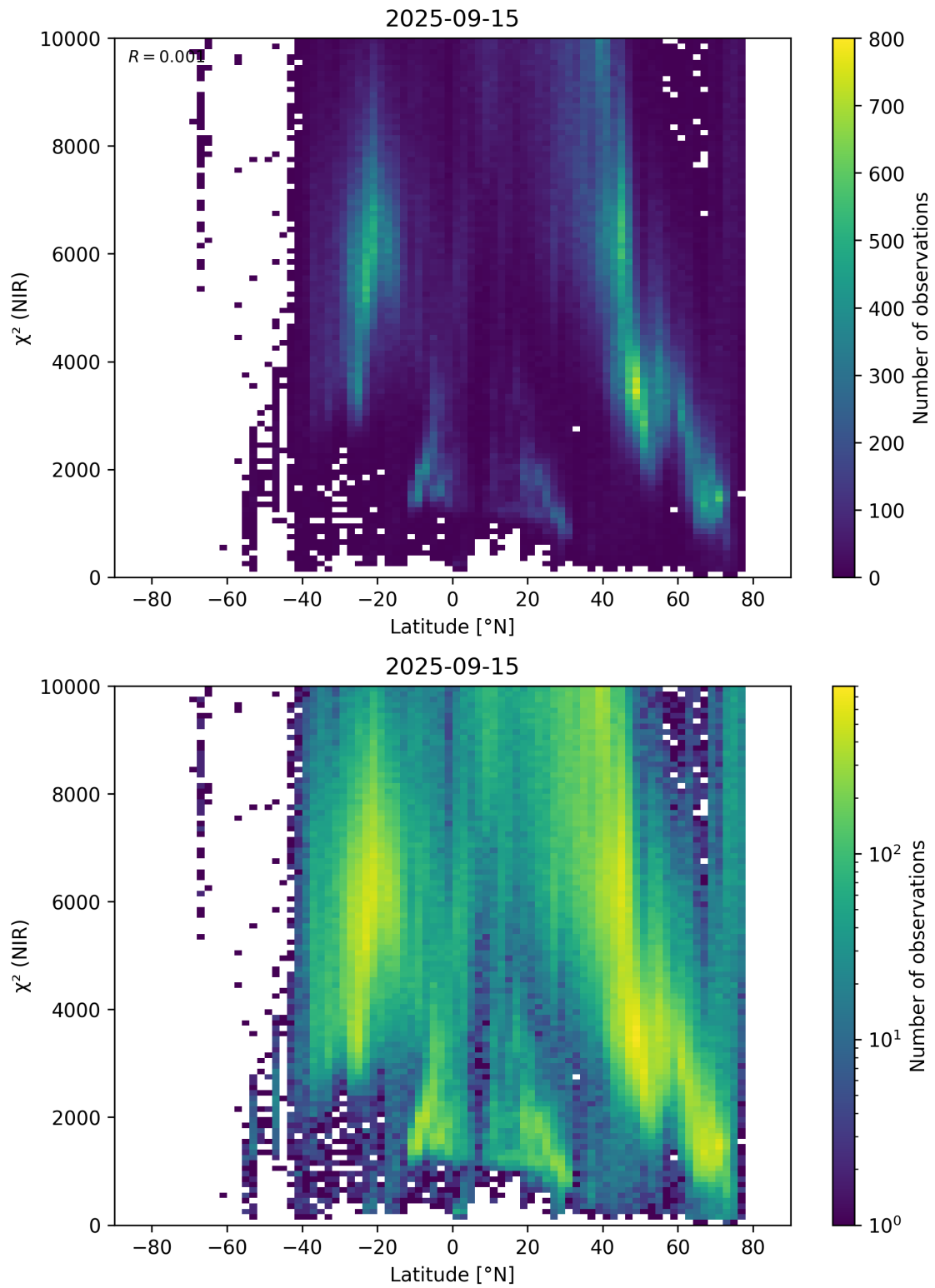
Figure 53: Scatter density plot of “Latitude” against “ \chi^2 (NIR)” for 2025-09-15 to 2025-09-16.
