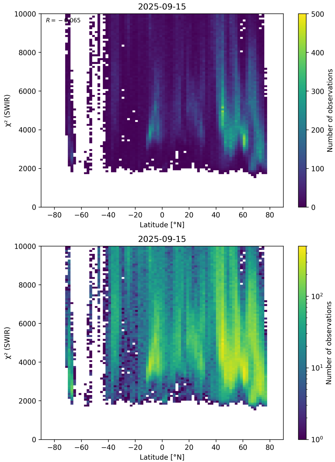
Figure 54: Scatter density plot of “Latitude” against “ \chi^2 (SWIR)” for 2025-09-15 to 2025-09-16.
