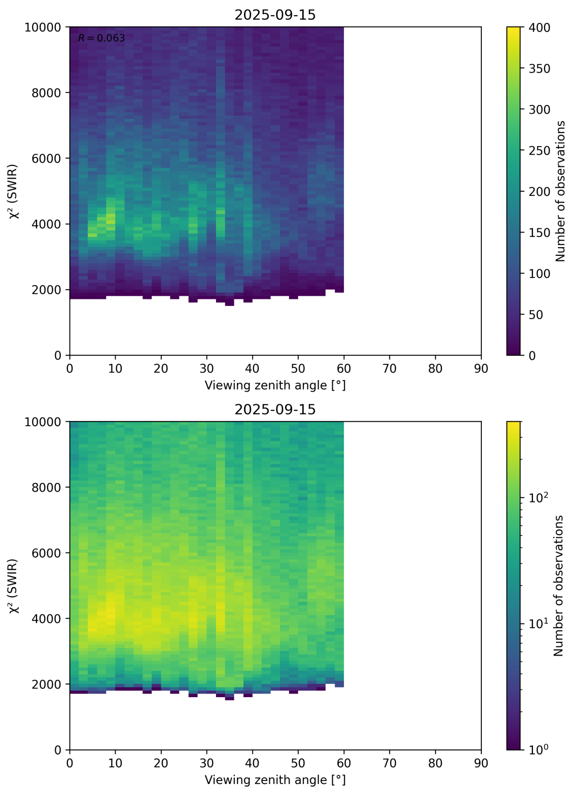
Figure 106: Scatter density plot of “Viewing zenith angle” against “ \chi^2 (SWIR)” for 2025-09-15 to 2025-09-16.
