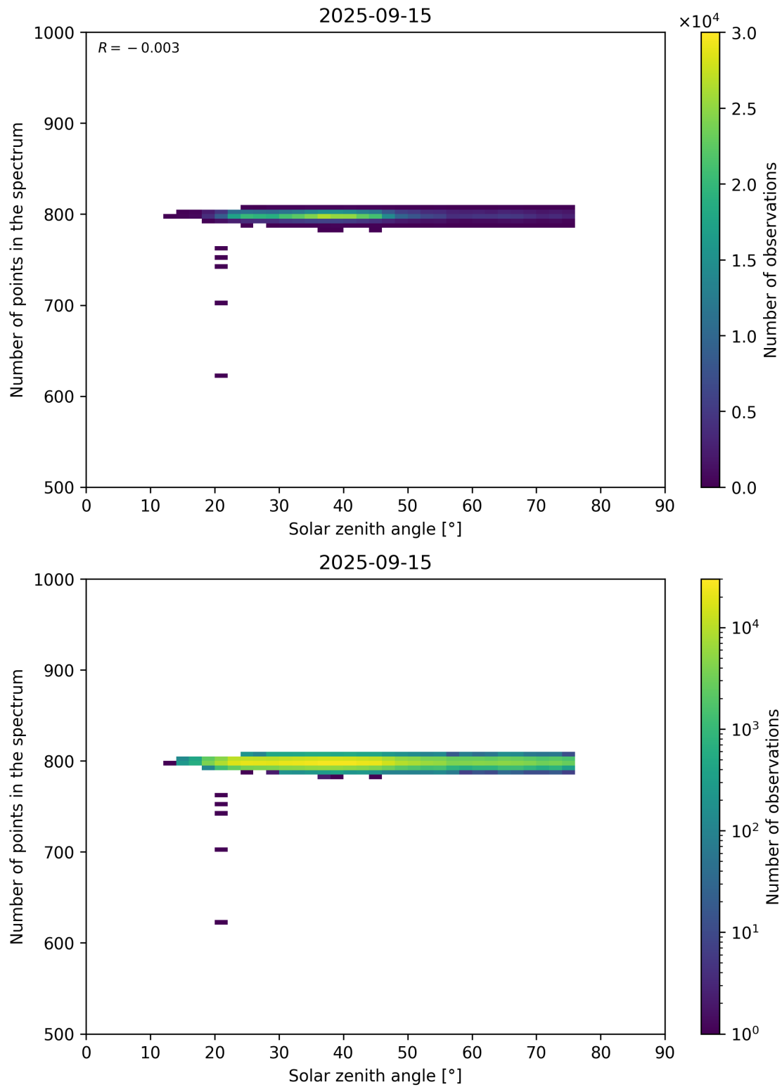
Figure 103: Scatter density plot of “Solar zenith angle” against “Number of points in the spectrum” for 2025-09-15 to 2025-09-16.
