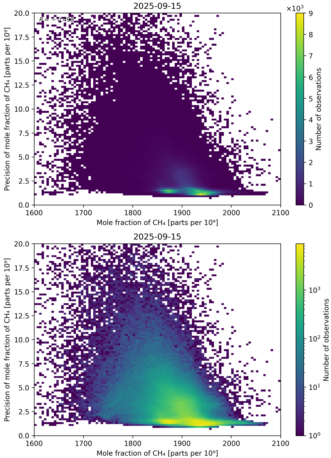
Figure 75: Scatter density plot of “Mole fraction of CH 4 ” against “Precision of mole fraction of CH 4 ” for 2025-09-15 to 2025-09-16.
