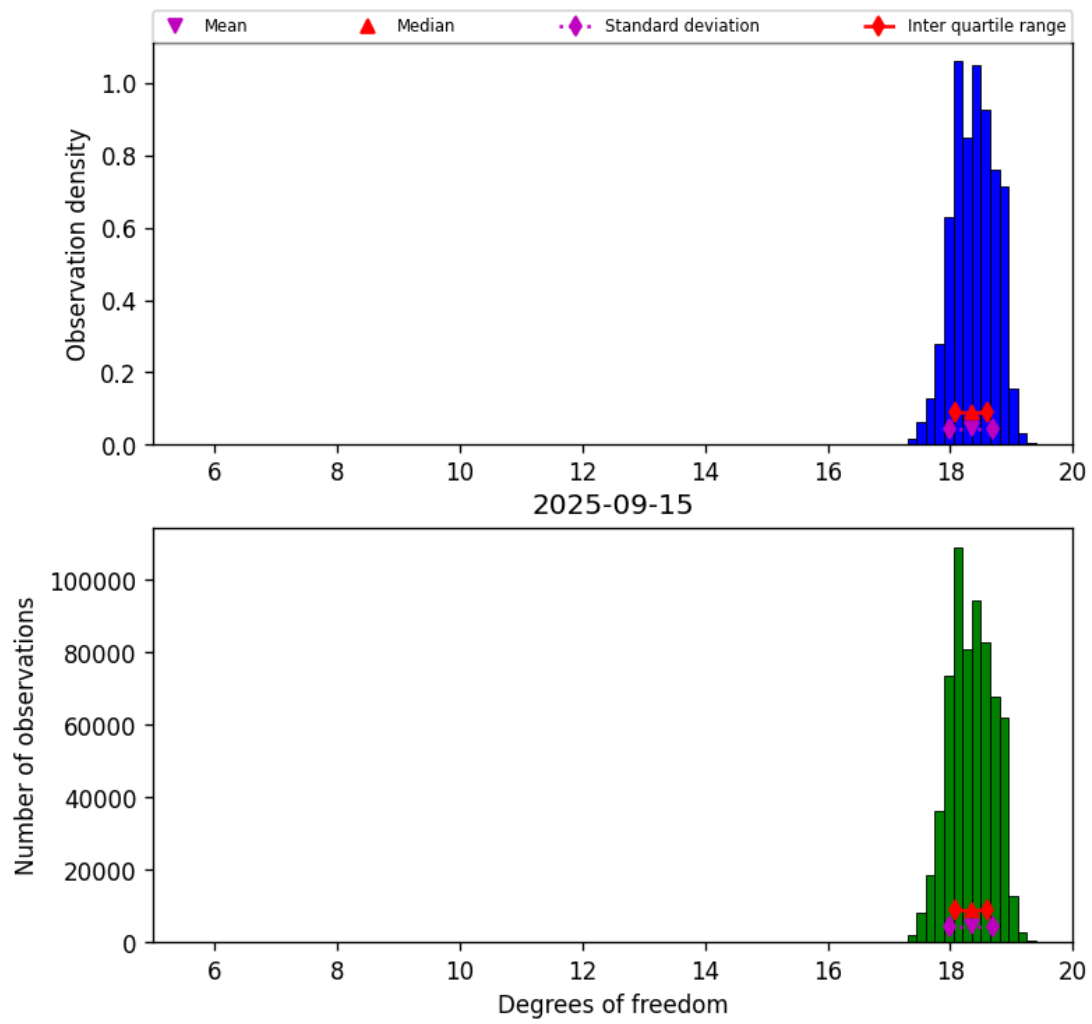
Figure 30: Histogram of “Degrees of freedom” for 2025-09-15 to 2025-09-16
