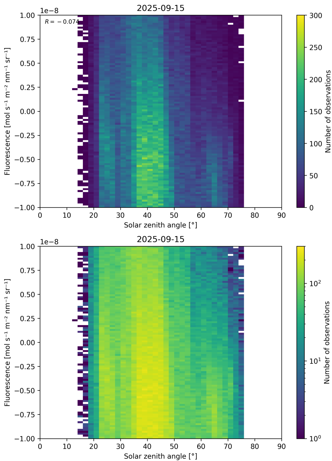
Figure 97: Scatter density plot of “Solar zenith angle” against “Fluorescence” for 2025-09-15 to 2025-09-16.
