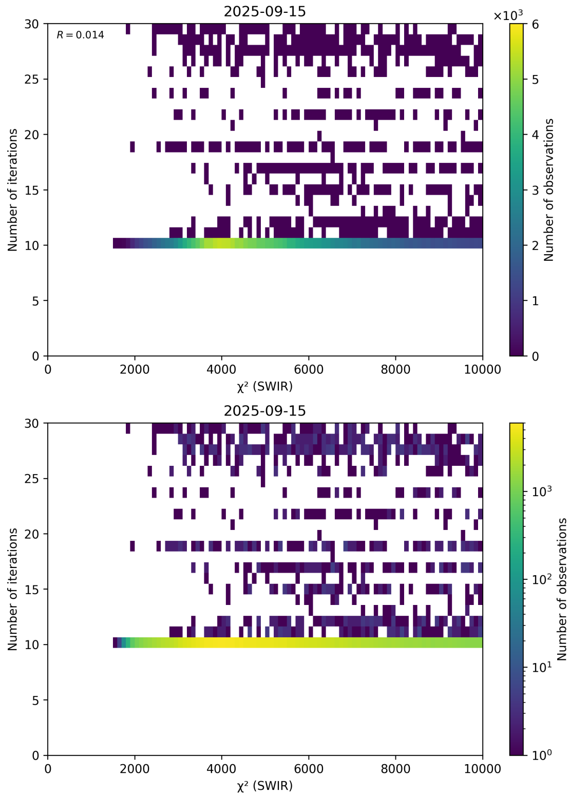
Figure 50: Scatter density plot of “ \chi^2 (SWIR)” against “Number of iterations” for 2025-09-15 to 2025-09-16.
