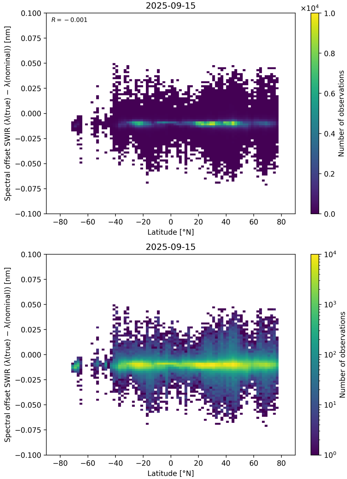
Figure 62: Scatter density plot of “Latitude” against “Spectral offset SWIR ( \lambda_{\text{true}} - \lambda_{\text{nominal}} )” for 2025-09-15 to 2025-09-16.
