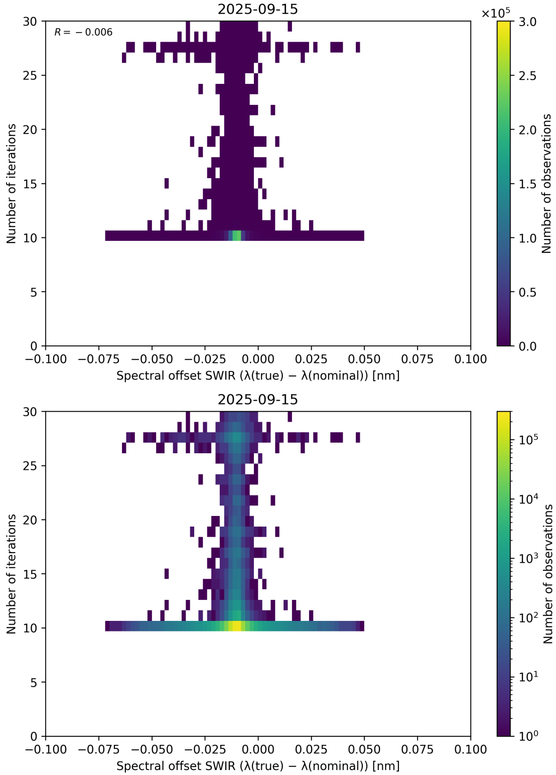
Figure 121: Scatter density plot of “Spectral offset SWIR ( \lambda_{\text{true}} - \lambda_{\text{nominal}} )” against “Number of iterations” for 2025-09-15 to 2025-09-16.
