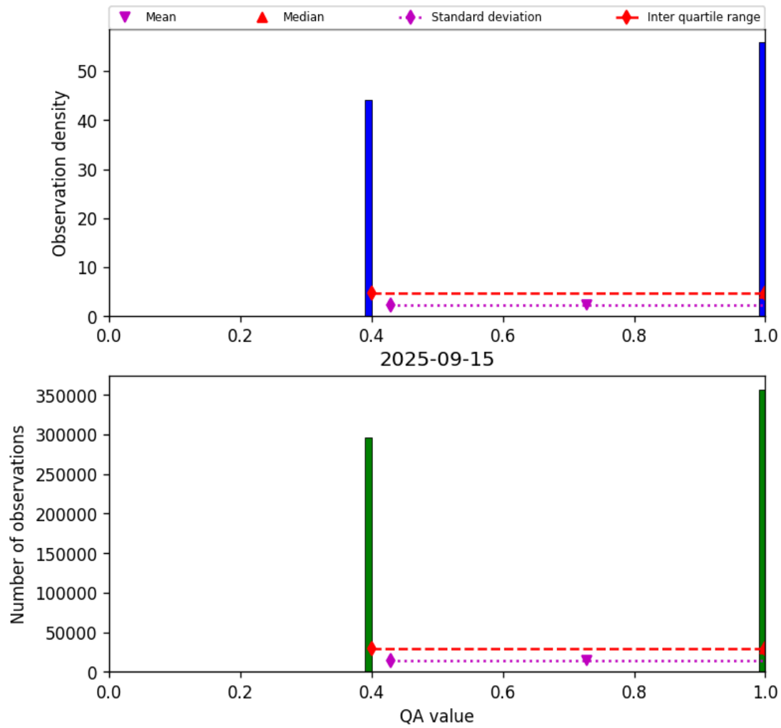
Figure 22: Histogram of “QA value” for 2025-09-15 to 2025-09-16
