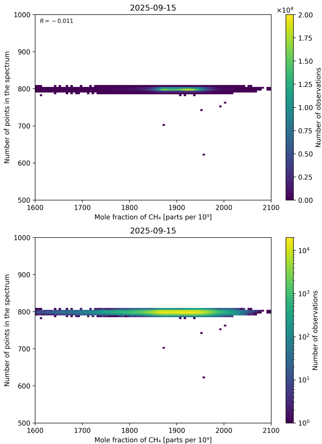
Figure 77: Scatter density plot of “Mole fraction of CH 4 ” against “Number of points in the spectrum” for 2025-09-15 to 2025-09-16.
