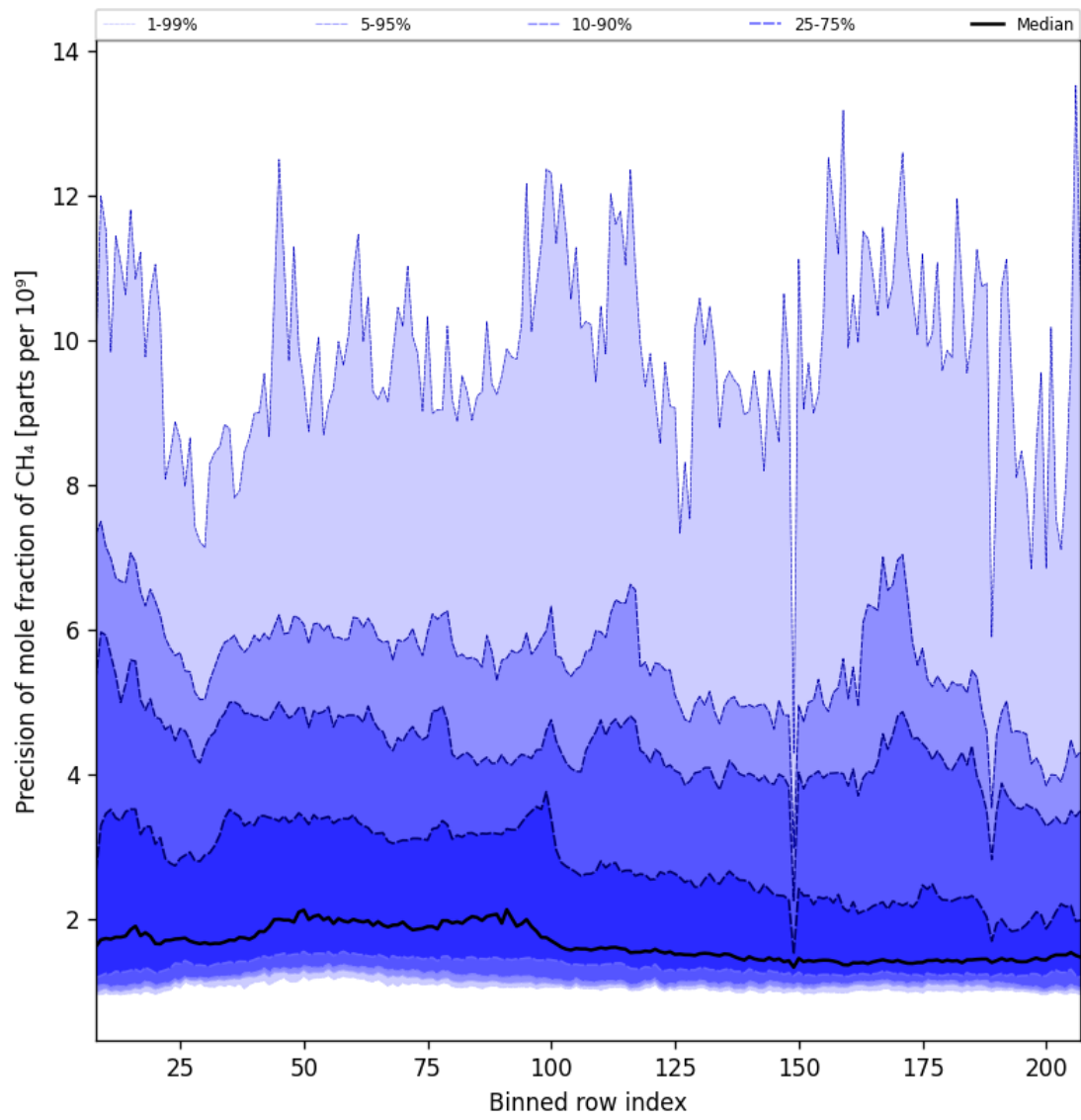
Figure 35: Along track statistics of “Precision of mole fraction of CH 4 ” for 2025-09-15 to 2025-09-16
