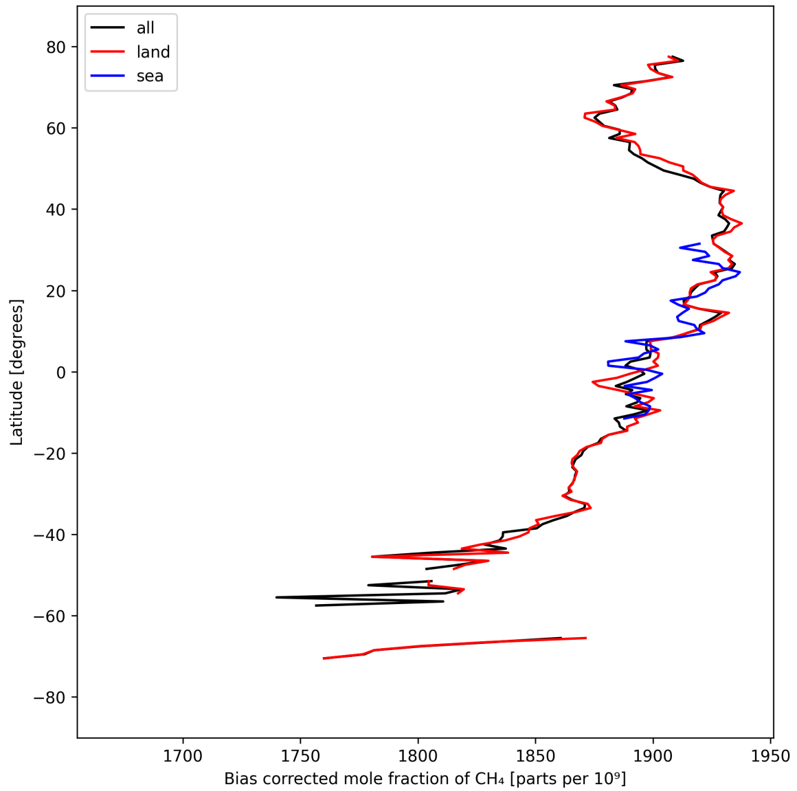
Figure 14: Zonal average of “Bias corrected mole fraction of CH 4 ” for 2025-09-15 to 2025-09-16.
