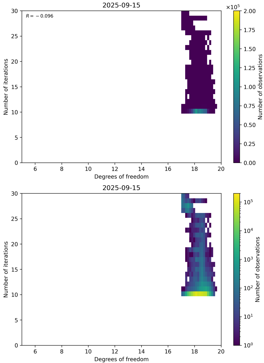
Figure 52: Scatter density plot of “Degrees of freedom” against “Number of iterations” for 2025-09-15 to 2025-09-16.
