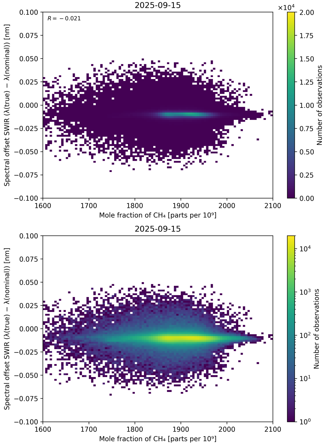
Figure 86: Scatter density plot of “Mole fraction of CH 4 ” against “Spectral offset SWIR ( \lambda_{\text{true}} - \lambda_{\text{nominal}} )” for 2025-09-15 to 2025-09-16.
