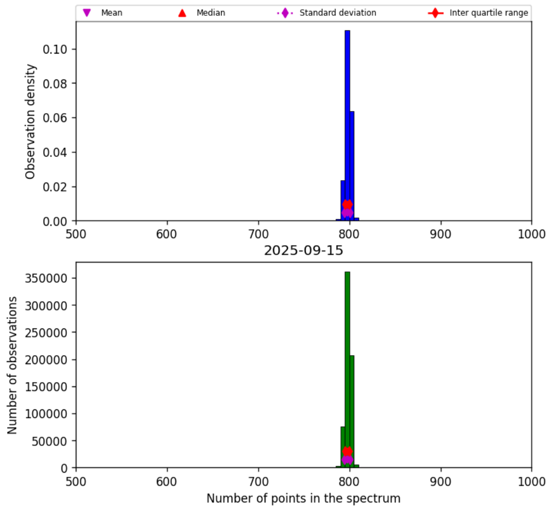
Figure 26: Histogram of “Number of points in the spectrum” for 2025-09-15 to 2025-09-16
