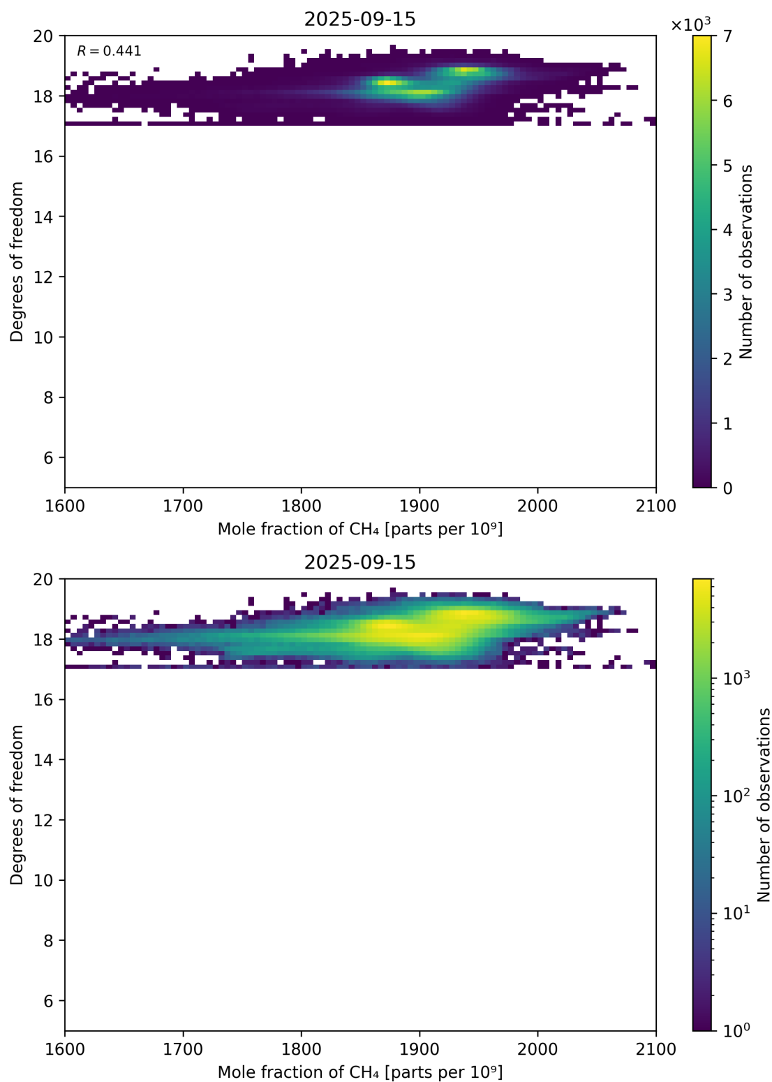
Figure 72: Scatter density plot of “Mole fraction of CH 4 ” against “Degrees of freedom” for 2025-09-15 to 2025-09-16.
