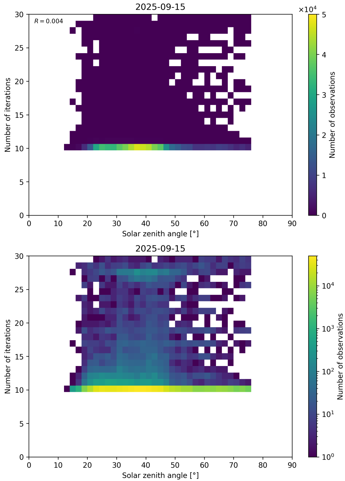
Figure 102: Scatter density plot of “Solar zenith angle” against “Number of iterations” for 2025-09-15 to 2025-09-16.
