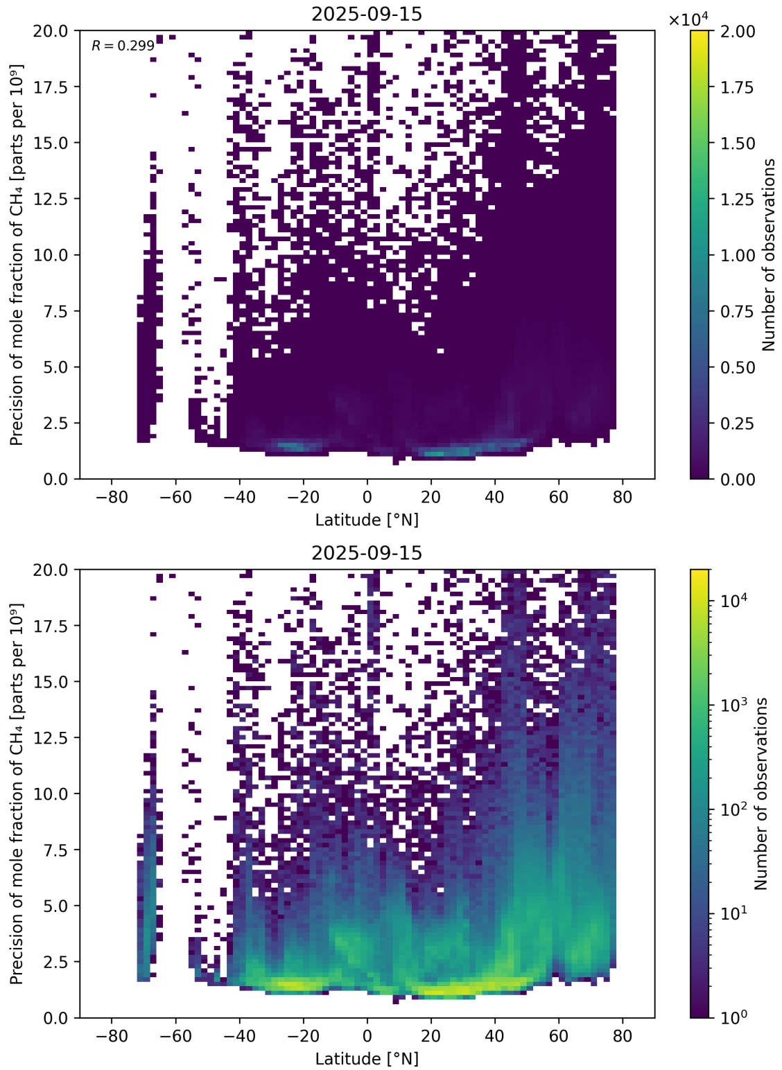
Figure 59: Scatter density plot of “Latitude” against “Precision of mole fraction of \text{CH}_4 ” for 2025-09-15 to 2025-09-16.
