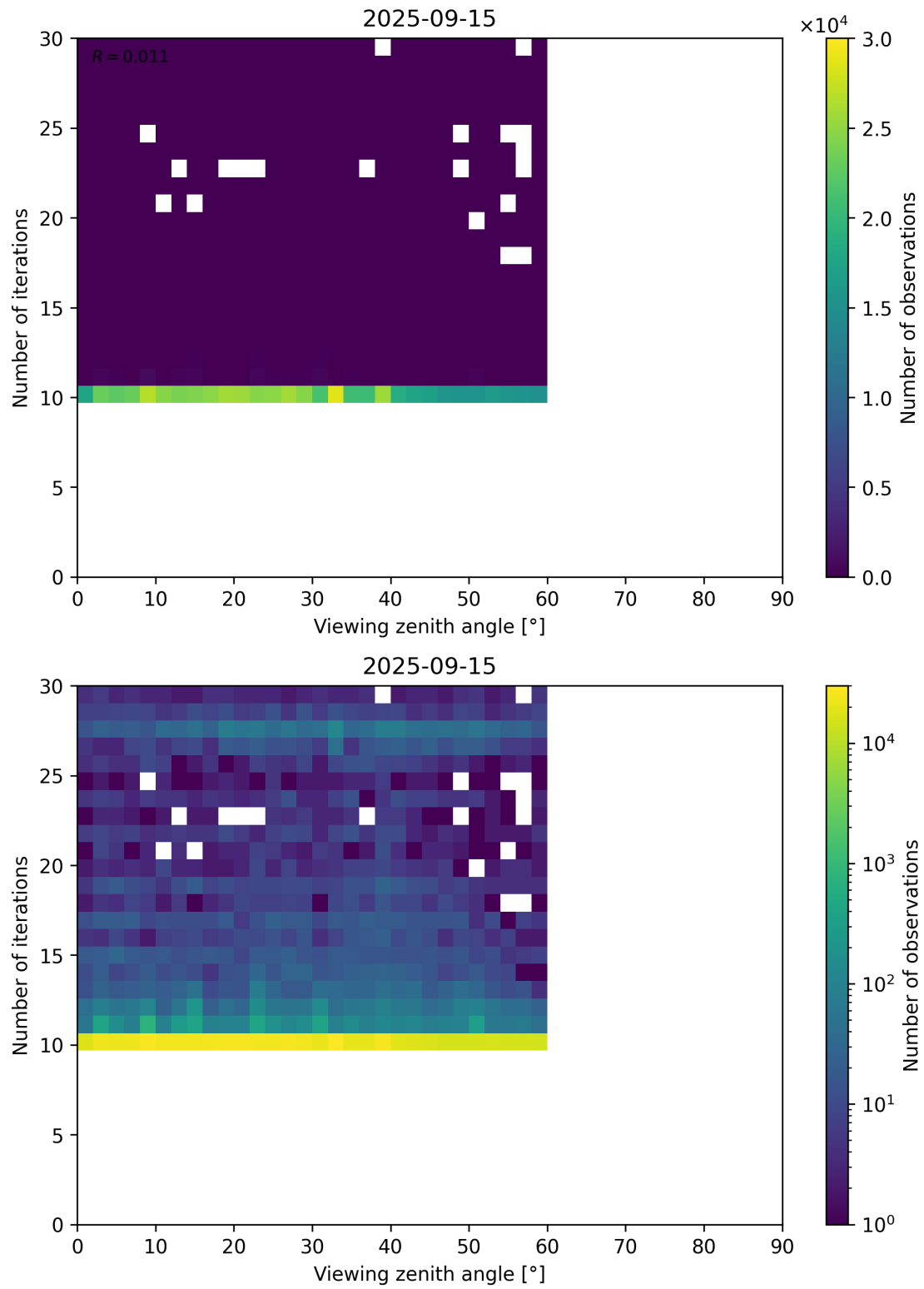
Figure 113: Scatter density plot of “Viewing zenith angle” against “Number of iterations” for 2025-09-15 to 2025-09-16.
