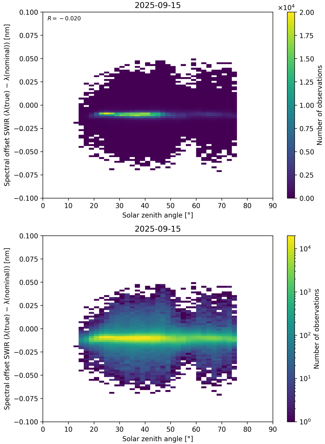
Figure 104: Scatter density plot of “Solar zenith angle” against “Spectral offset SWIR ( \lambda_{\text{true}} - \lambda_{\text{nominal}} )” for 2025-09-15 to 2025-09-16.
