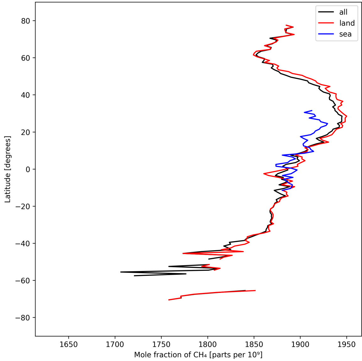
Figure 12: Zonal average of “Mole fraction of CH 4 ” for 2025-09-15 to 2025-09-16.
