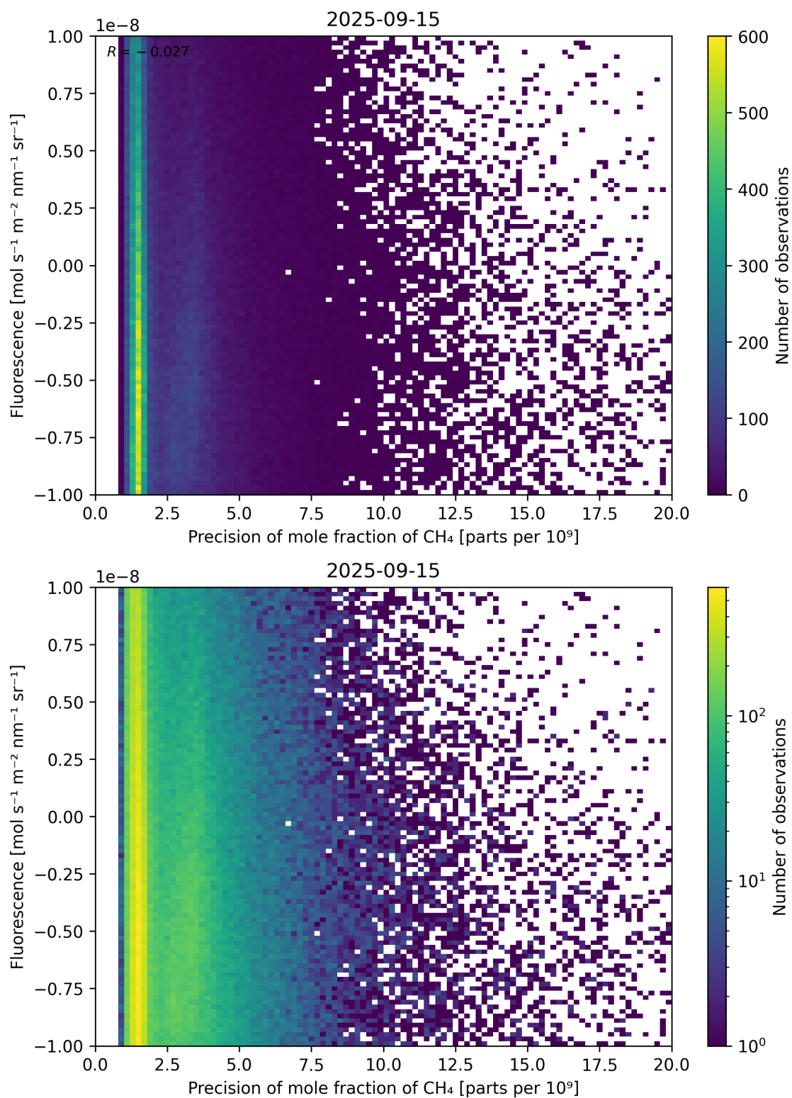
Figure 81: Scatter density plot of “Precision of mole fraction of CH 4 ” against “Fluorescence” for 2025-09-15 to 2025-09-16.
