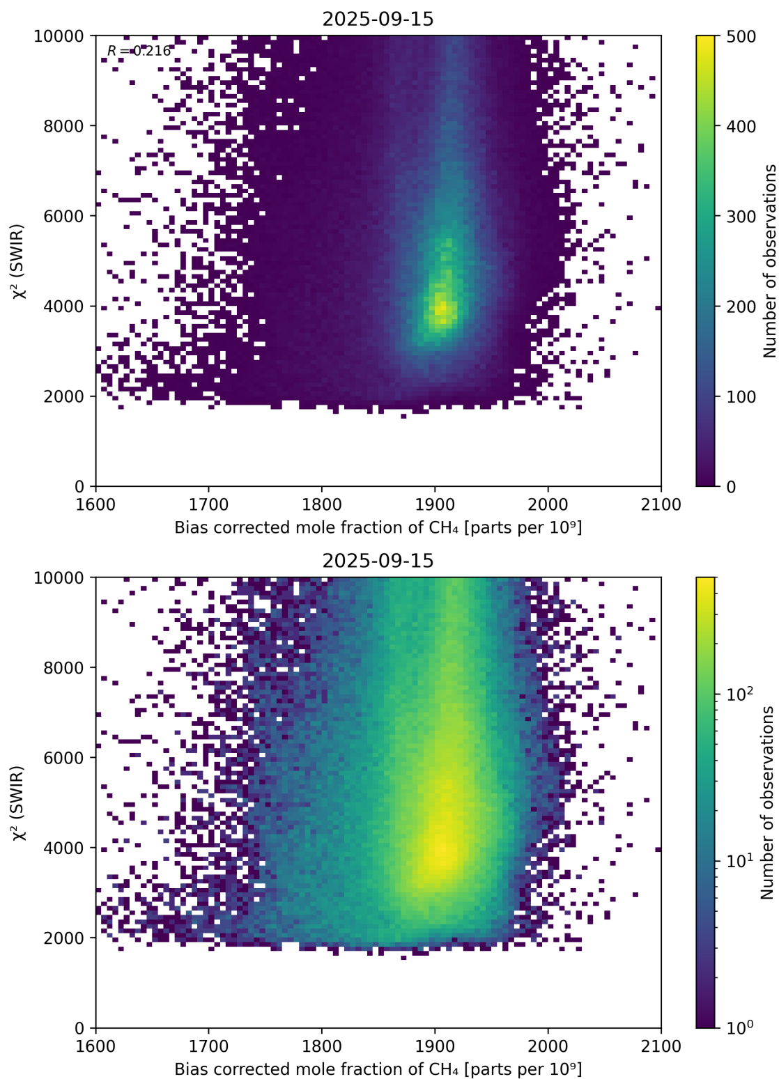
Figure 64: Scatter density plot of “Bias corrected mole fraction of \text{CH}_4 ” against “ \chi^2 (SWIR)” for 2025-09-15 to 2025-09-16.
