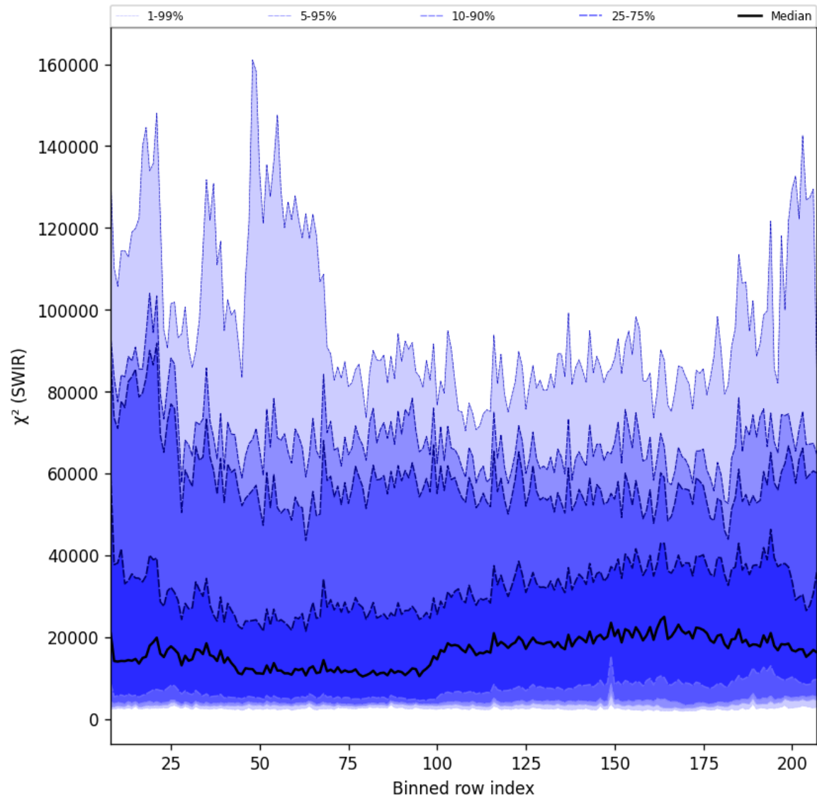
Figure 39: Along track statistics of " \chi^2 (SWIR)" for 2025-09-15 to 2025-09-16
