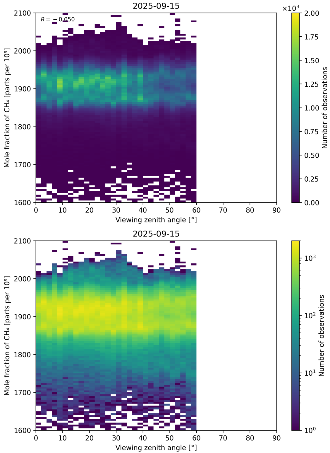
Figure 110: Scatter density plot of “Viewing zenith angle” against “Mole fraction of CH 4 ” for 2025-09-15 to 2025-09-16.
