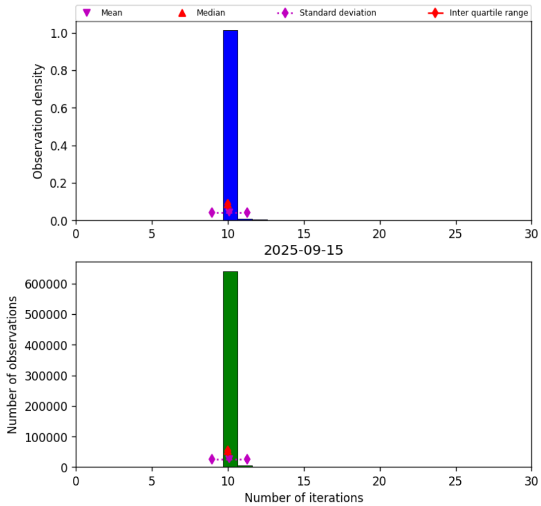
Figure 31: Histogram of “Number of iterations” for 2025-09-15 to 2025-09-16
