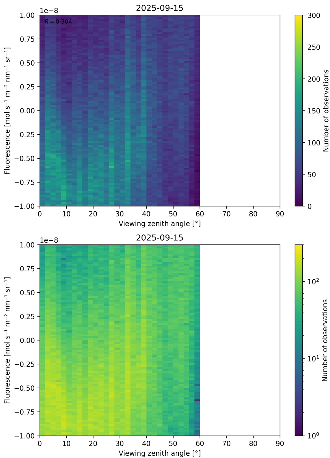
Figure 108: Scatter density plot of “Viewing zenith angle” against “Fluorescence” for 2025-09-15 to 2025-09-16.
