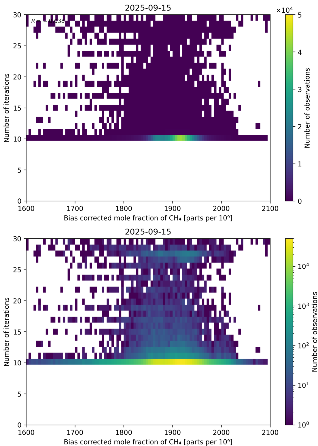
Figure 67: Scatter density plot of “Bias corrected mole fraction of CH 4 ” against “Number of iterations” for 2025-09-15 to 2025-09-16.
