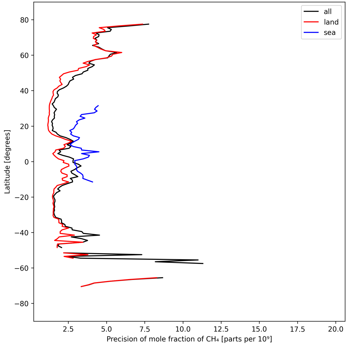
Figure 13: Zonal average of “Precision of mole fraction of \text{CH}_4 ” for 2025-09-15 to 2025-09-16.
