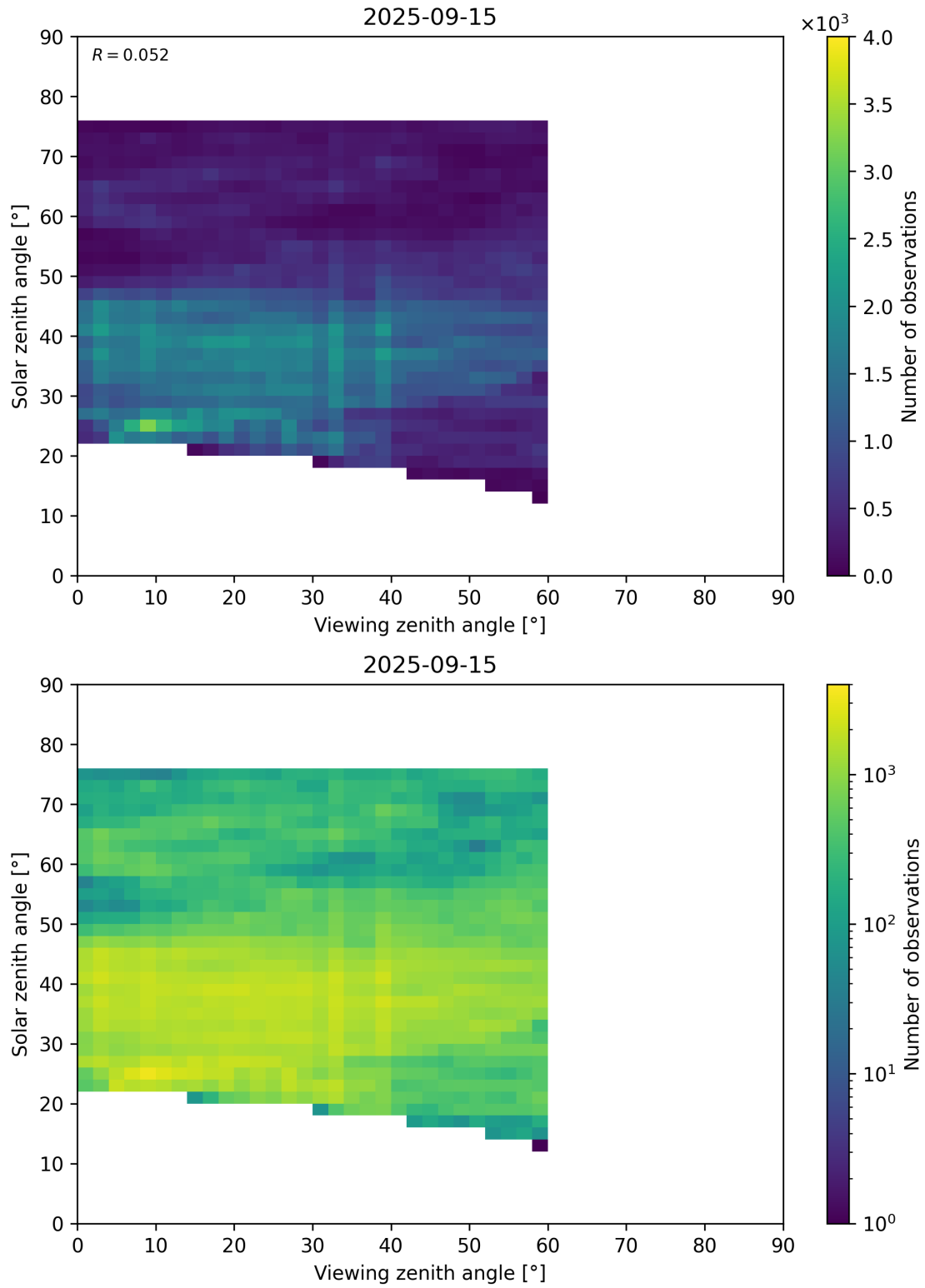
Figure 115: Scatter density plot of “Viewing zenith angle” against “Solar zenith angle” for 2025-09-15 to 2025-09-16.
