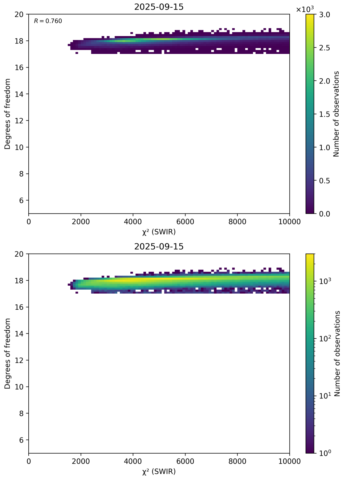
Figure 48: Scatter density plot of “ \chi^2 (SWIR)” against “Degrees of freedom” for 2025-09-15 to 2025-09-16.
