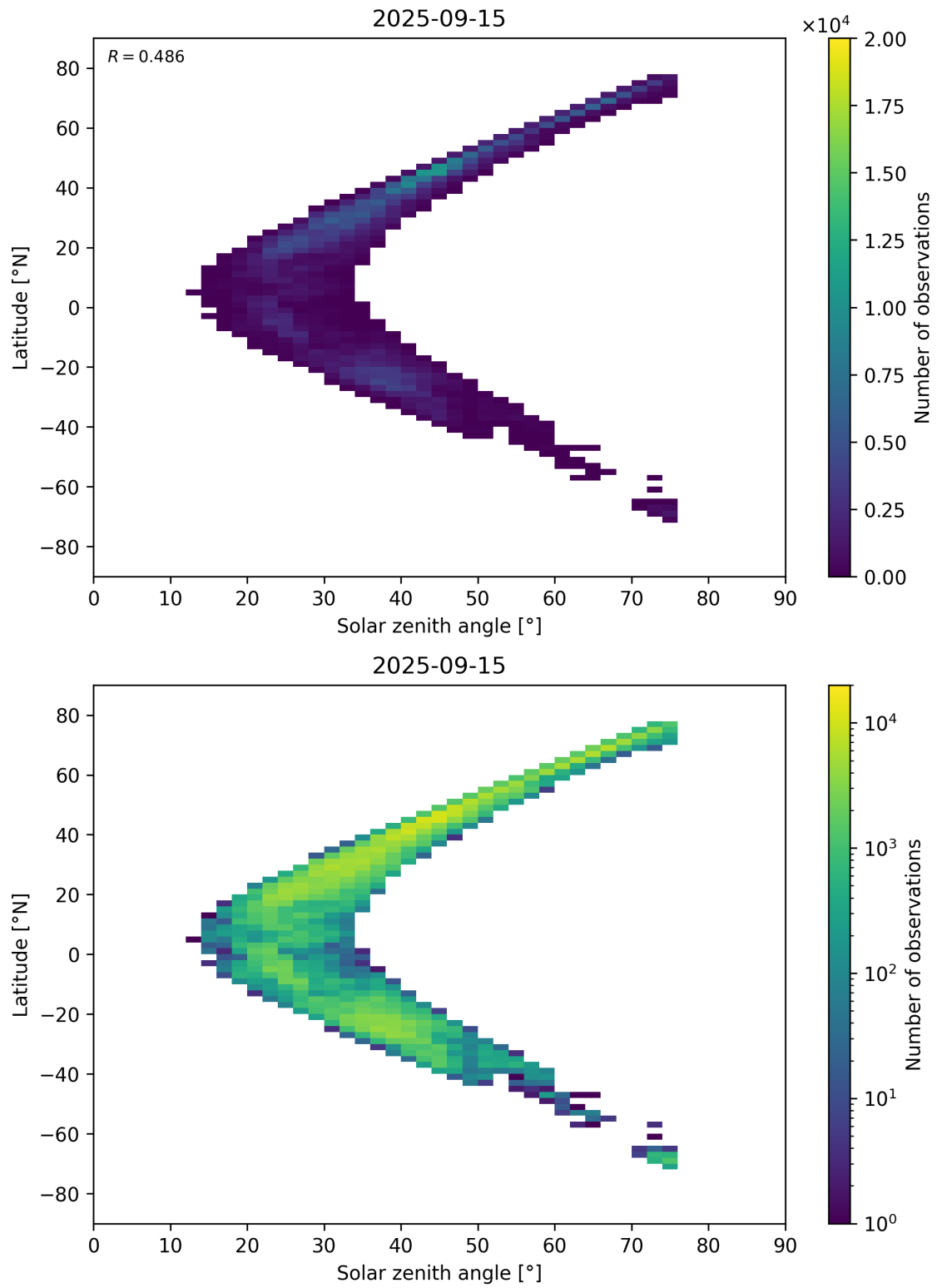
Figure 98: Scatter density plot of “Solar zenith angle” against “Latitude” for 2025-09-15 to 2025-09-16.
