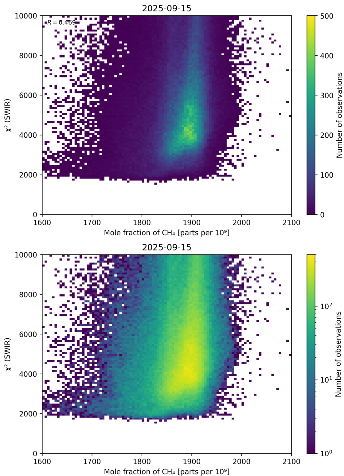
Figure 71: Scatter density plot of “Mole fraction of \text{CH}_4 ” against “ \chi^2 (SWIR)” for 2025-09-15 to 2025-09-16.
