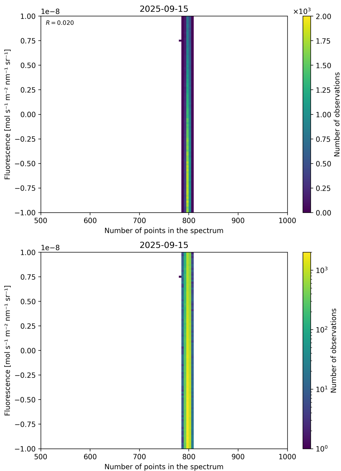
Figure 91: Scatter density plot of “Number of points in the spectrum” against “Fluorescence” for 2025-09-15 to 2025-09-16.
