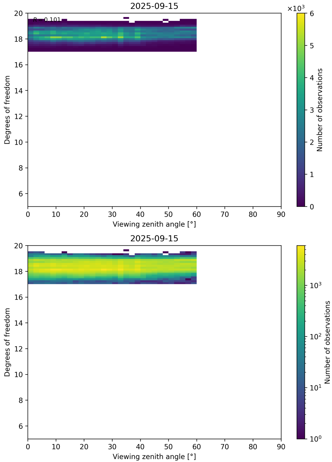
Figure 107: Scatter density plot of “Viewing zenith angle” against “Degrees of freedom” for 2025-09-15 to 2025-09-16.
