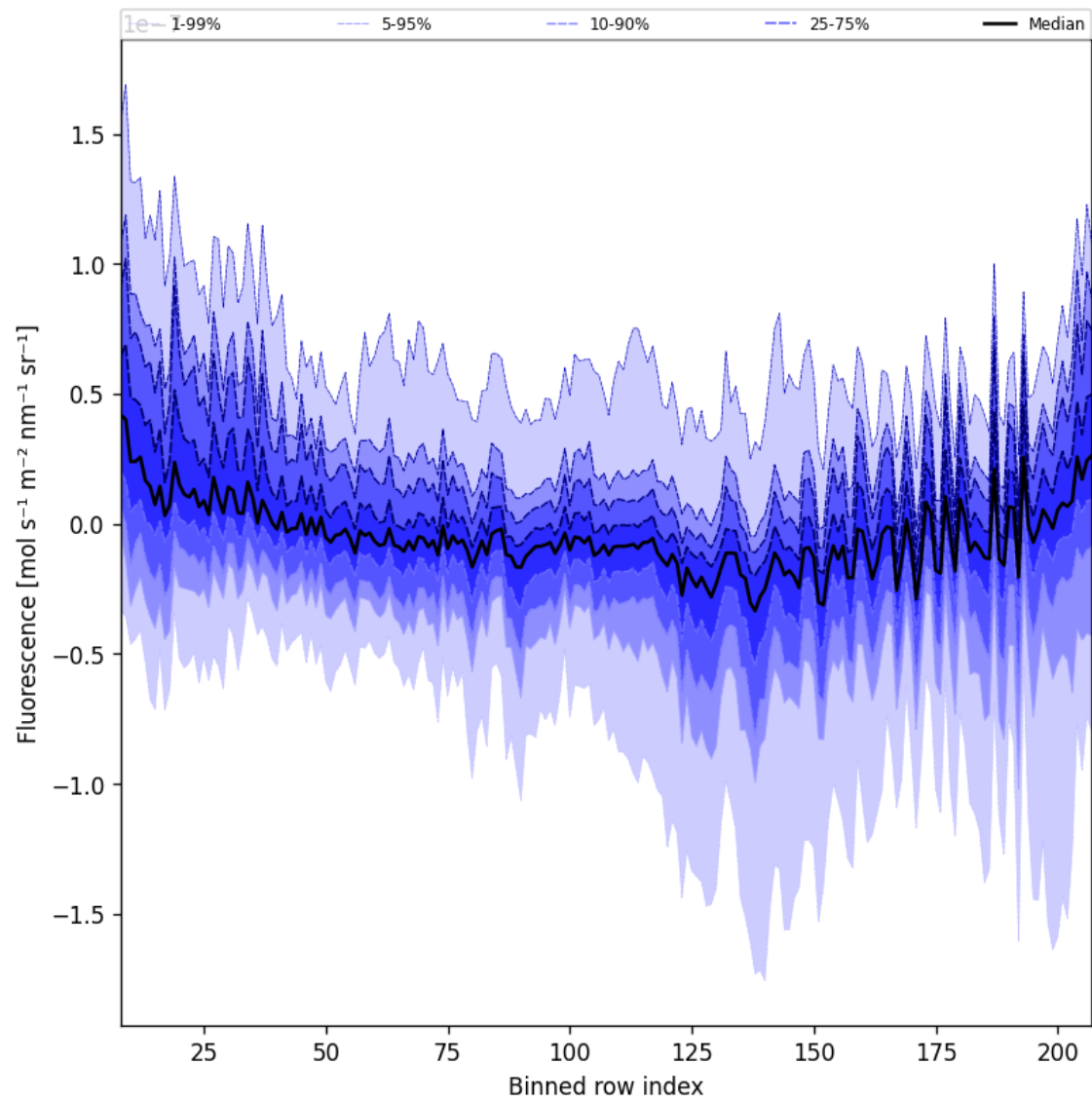
Figure 43: Along track statistics of “Fluorescence” for 2025-09-15 to 2025-09-16
