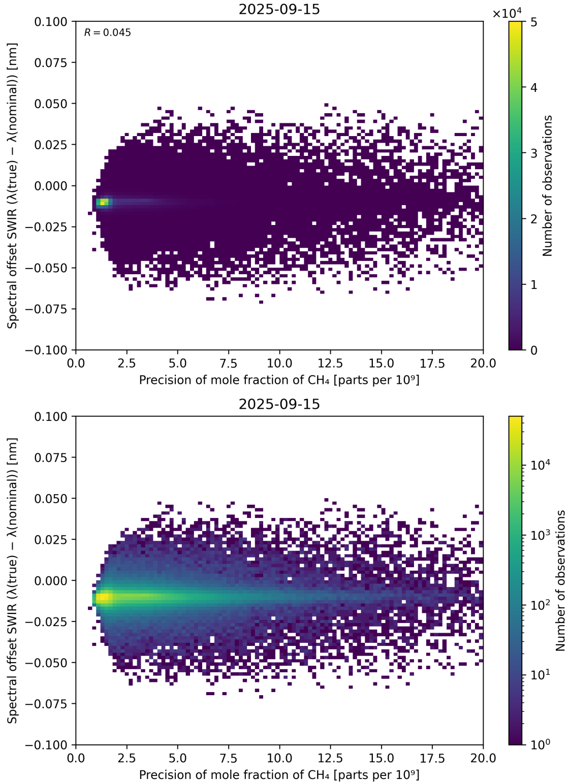
Figure 85: Scatter density plot of “Precision of mole fraction of CH 4 ” against “Spectral offset SWIR ( \lambda_{\text{true}} - \lambda_{\text{nominal}} )” for 2025-09-15 to 2025-09-16.
