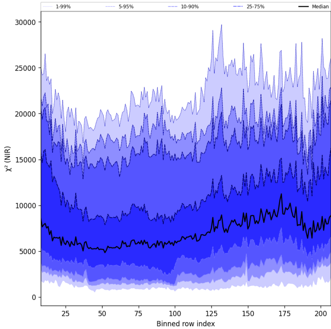
Figure 40: Along track statistics of “ \chi^2 (NIR)” for 2025-09-15 to 2025-09-16
