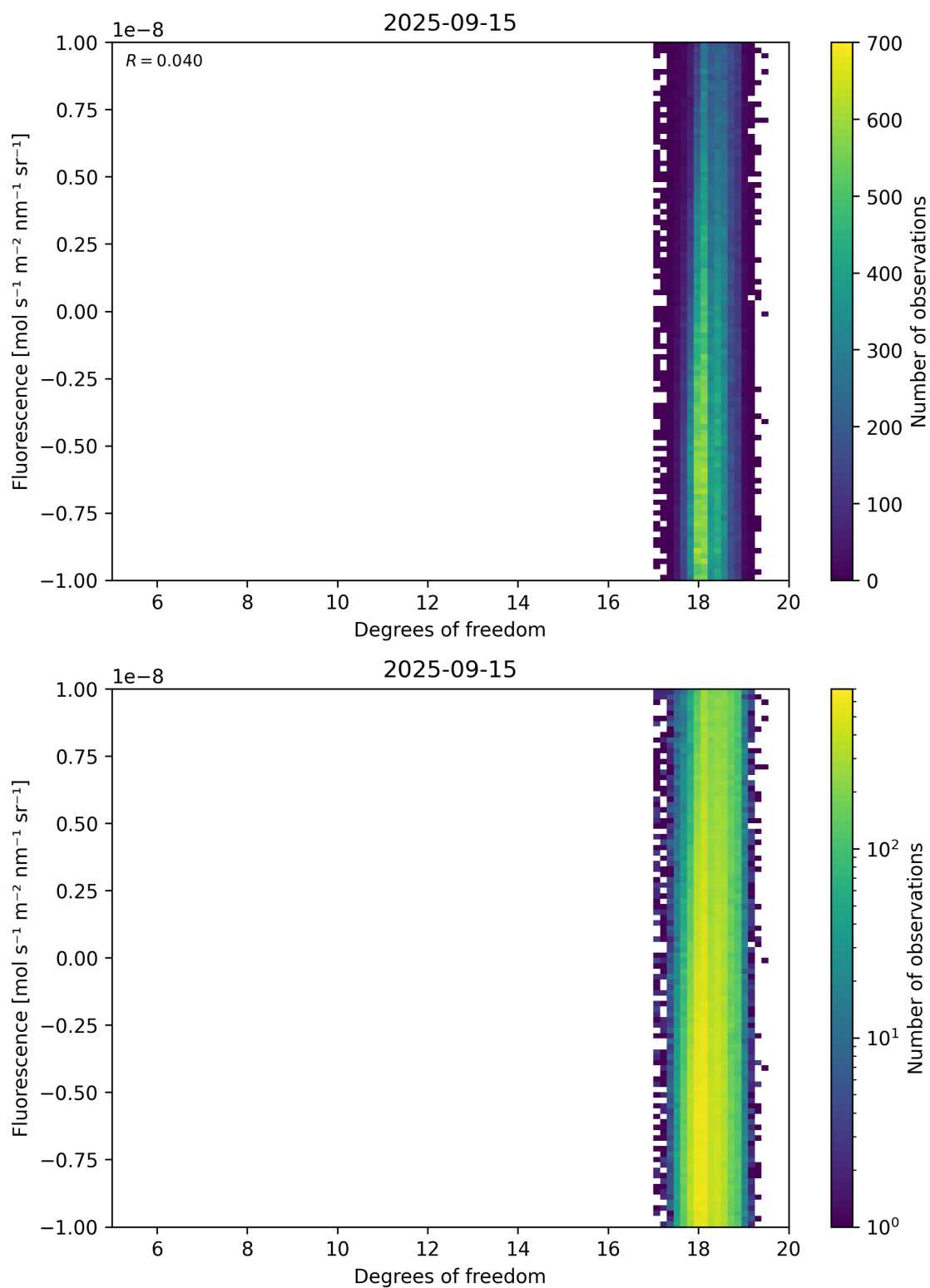
Figure 51: Scatter density plot of “Degrees of freedom” against “Fluorescence” for 2025-09-15 to 2025-09-16.
