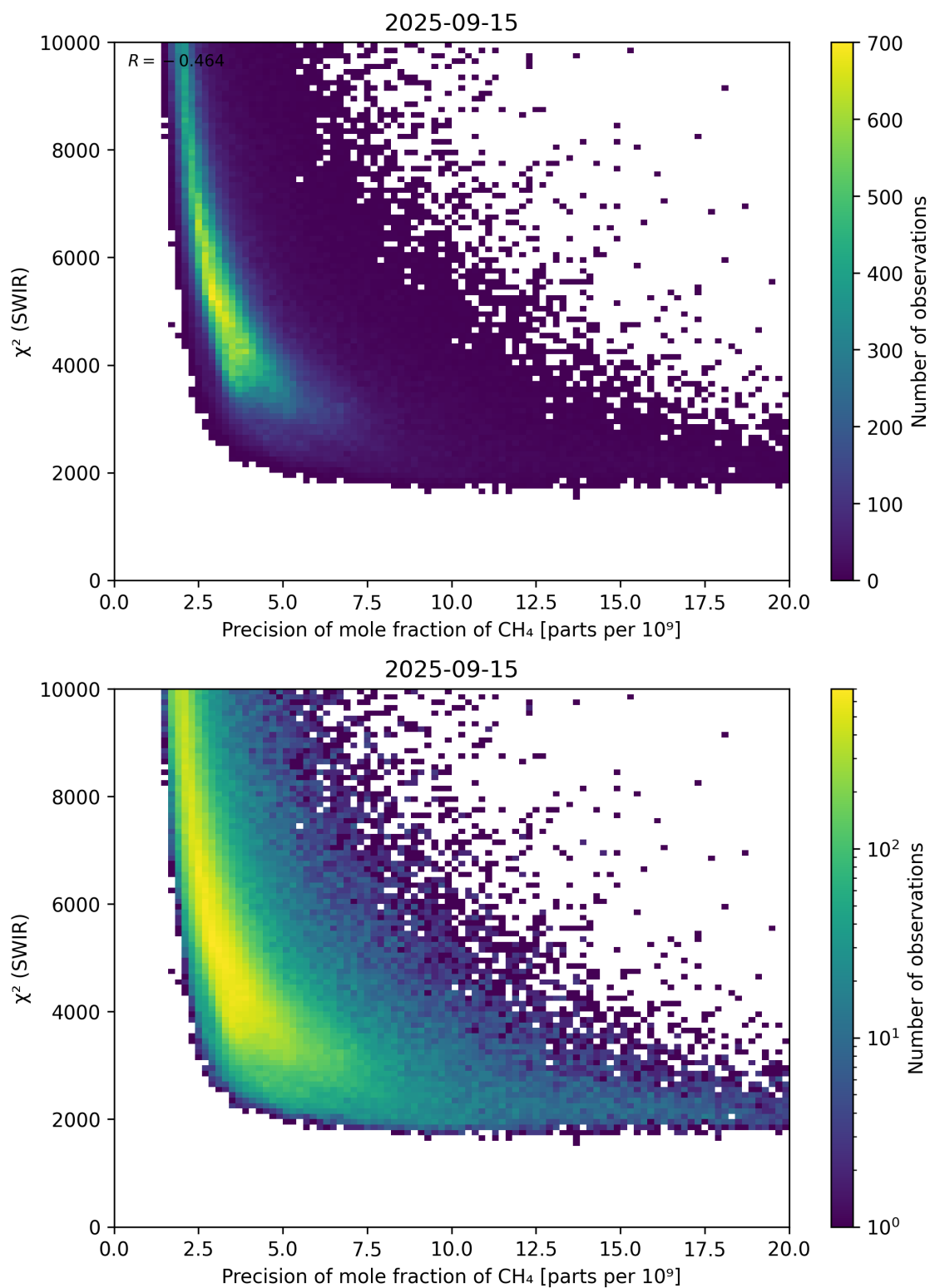
Figure 79: Scatter density plot of “Precision of mole fraction of \text{CH}_4 ” against “ \chi^2 (SWIR)” for 2025-09-15 to 2025-09-16.
