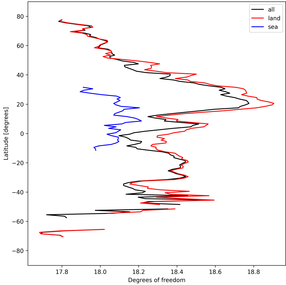
Figure 19: Zonal average of “Degrees of freedom” for 2025-09-15 to 2025-09-16.
