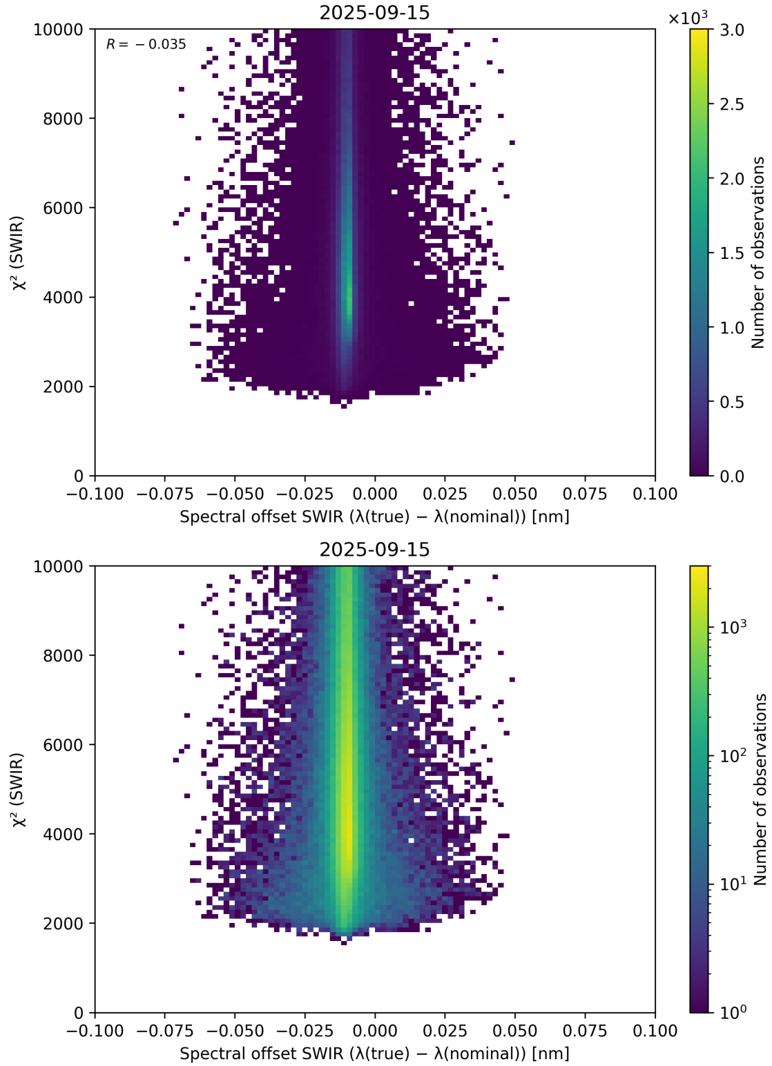
Figure 118: Scatter density plot of “Spectral offset SWIR ( \lambda_{\text{true}} - \lambda_{\text{nominal}} )” against “ \chi^2 (SWIR)” for 2025-09-15 to 2025-09-16.
