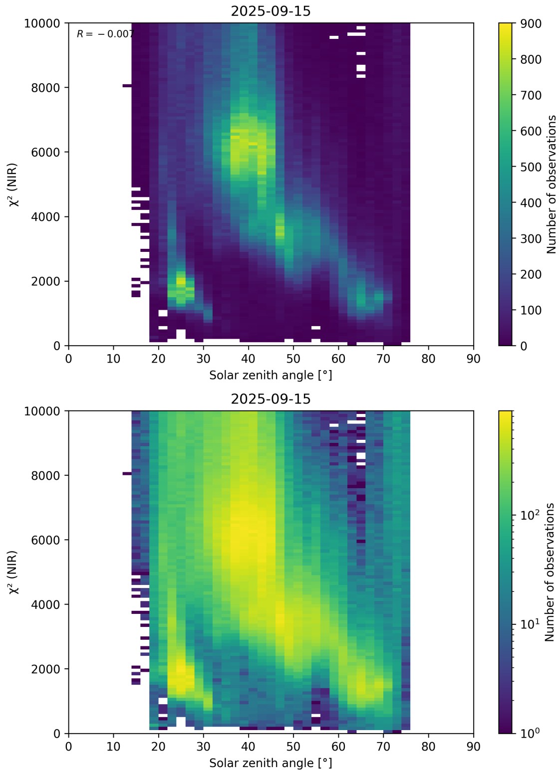
Figure 94: Scatter density plot of “Solar zenith angle” against “ \chi^2 (NIR)” for 2025-09-15 to 2025-09-16.
