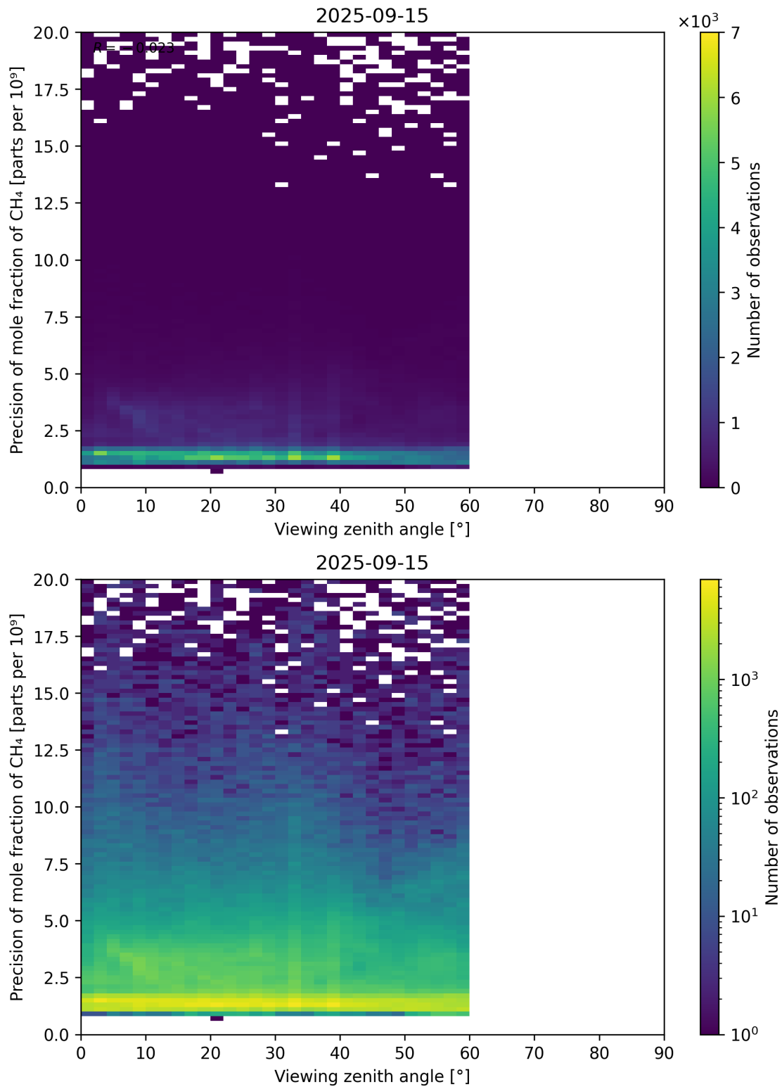
Figure 112: Scatter density plot of “Viewing zenith angle” against “Precision of mole fraction of CH 4 ” for 2025-09-15 to 2025-09-16.
