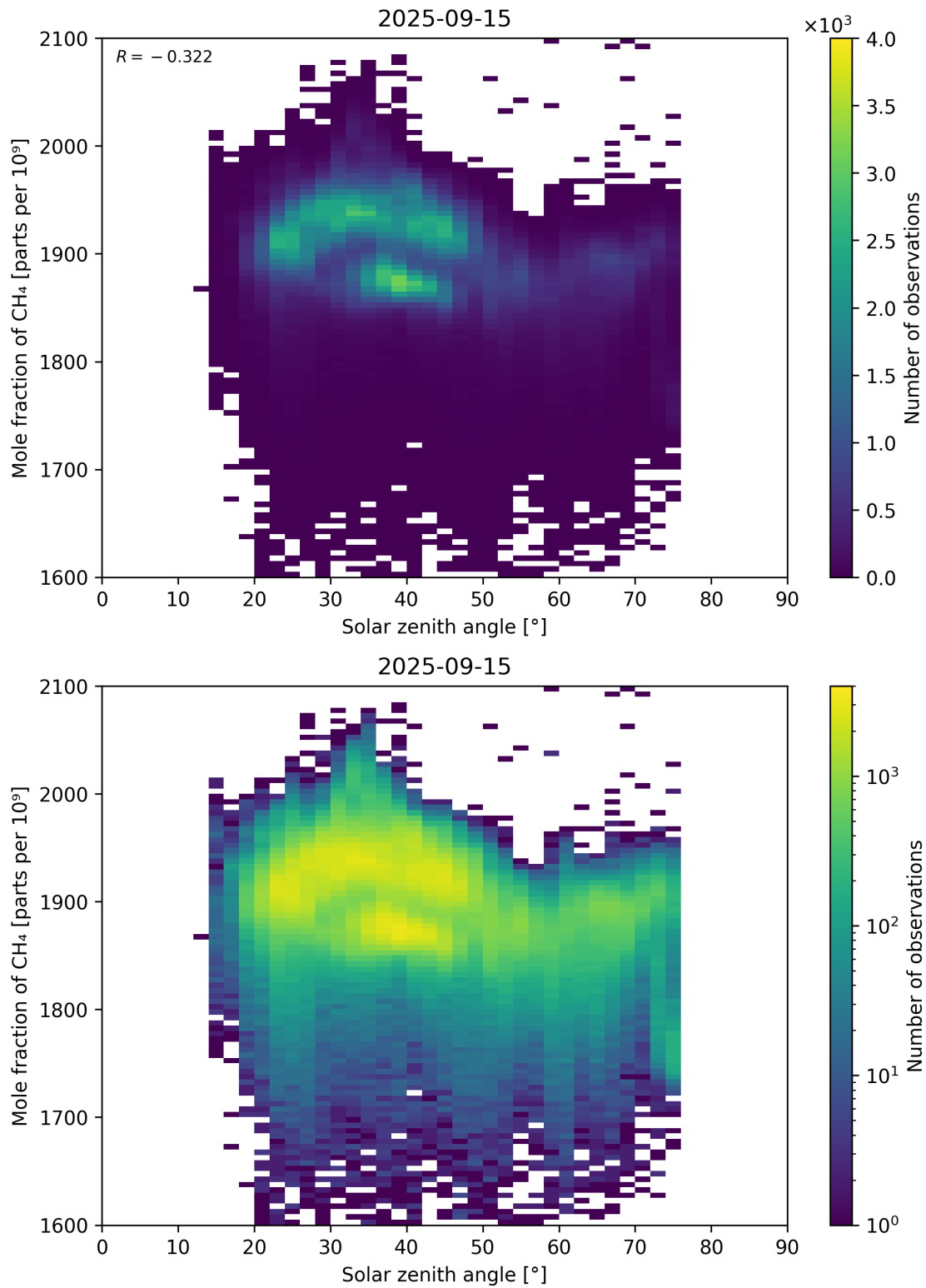
Figure 99: Scatter density plot of “Solar zenith angle” against “Mole fraction of CH 4 ” for 2025-09-15 to 2025-09-16.
