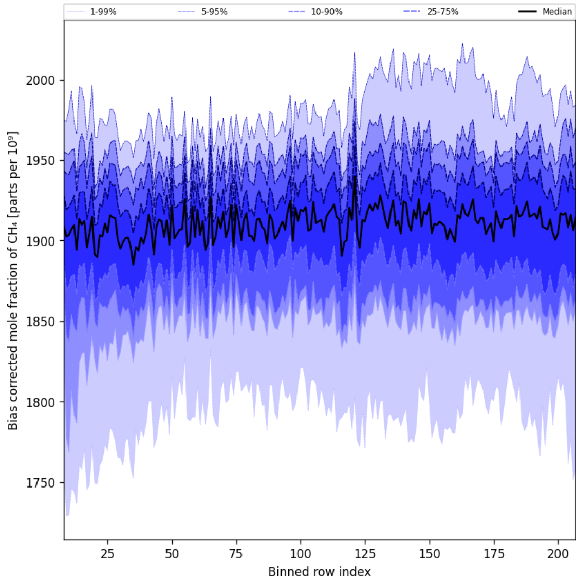
Figure 36: Along track statistics of “Bias corrected mole fraction of \text{CH}_4 ” for 2025-09-15 to 2025-09-16
