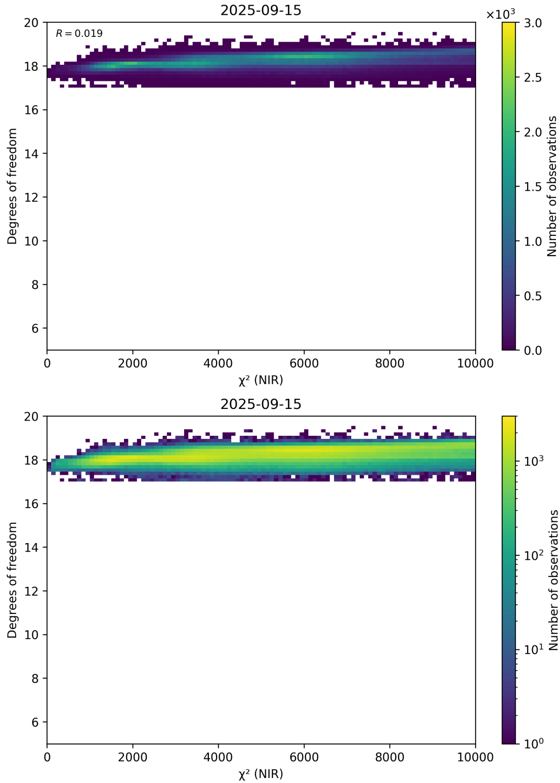
Figure 44: Scatter density plot of “ \chi^2 (NIR)” against “Degrees of freedom” for 2025-09-15 to 2025-09-16.
