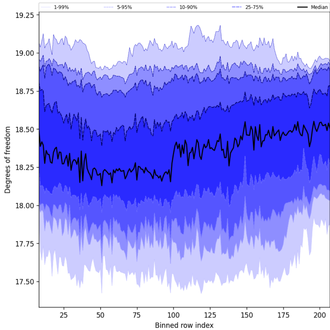
Figure 41: Along track statistics of “Degrees of freedom” for 2025-09-15 to 2025-09-16
