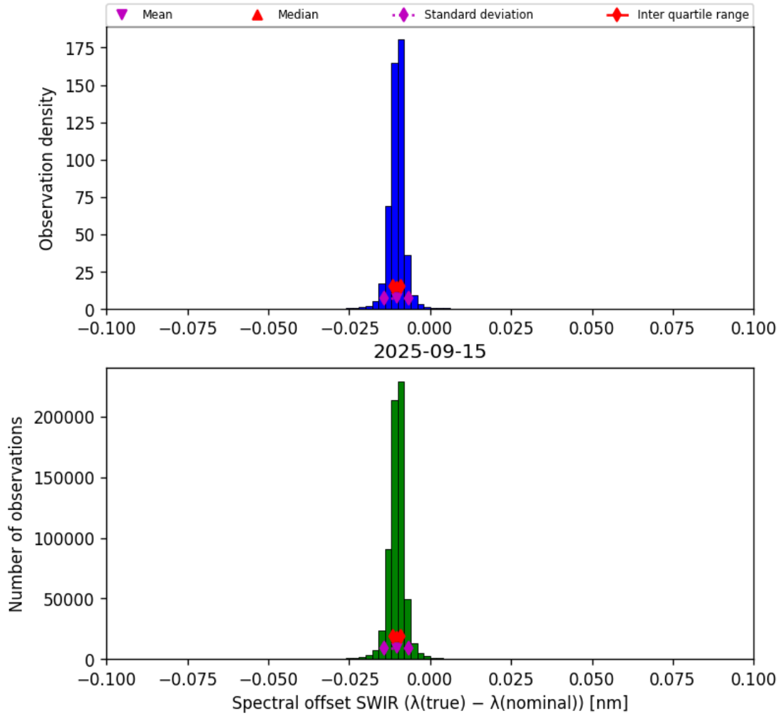
Figure 27: Histogram of “Spectral offset SWIR ( \lambda_{\text{true}} - \lambda_{\text{nominal}} )” for 2025-09-15 to 2025-09-16
