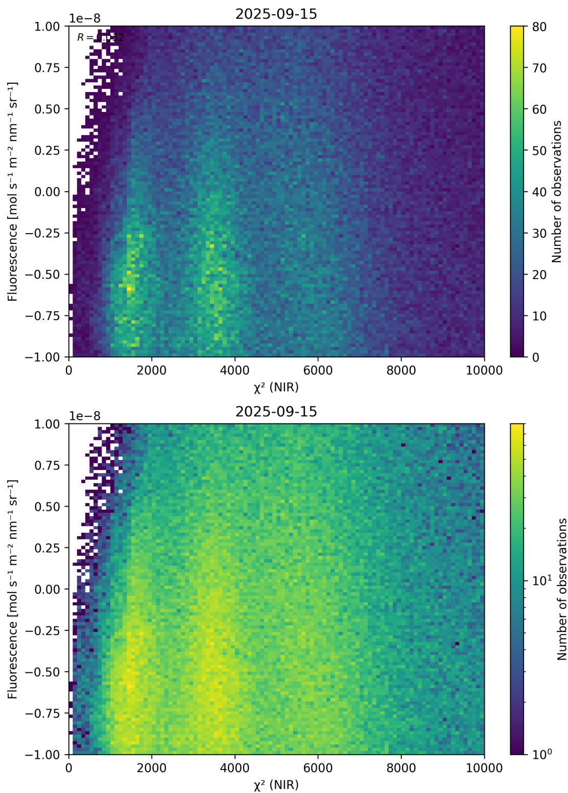
Figure 45: Scatter density plot of “ \chi^2 (NIR)” against “Fluorescence” for 2025-09-15 to 2025-09-16.
