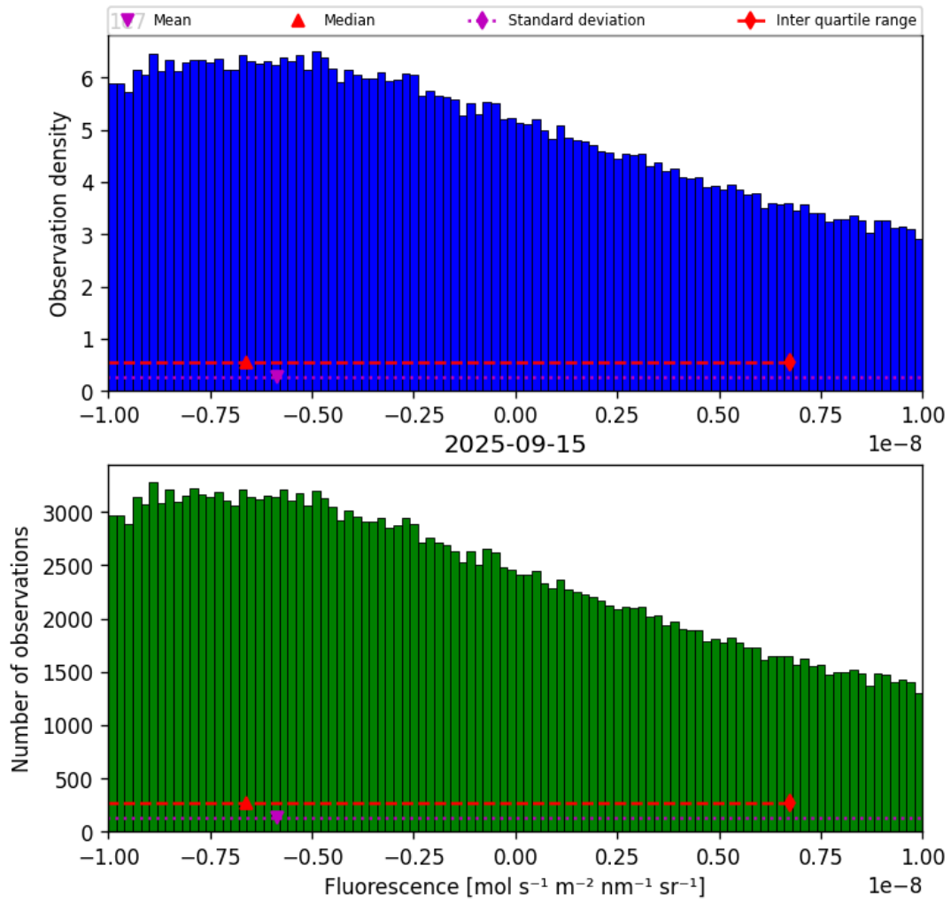
Figure 32: Histogram of “Fluorescence” for 2025-09-15 to 2025-09-16
