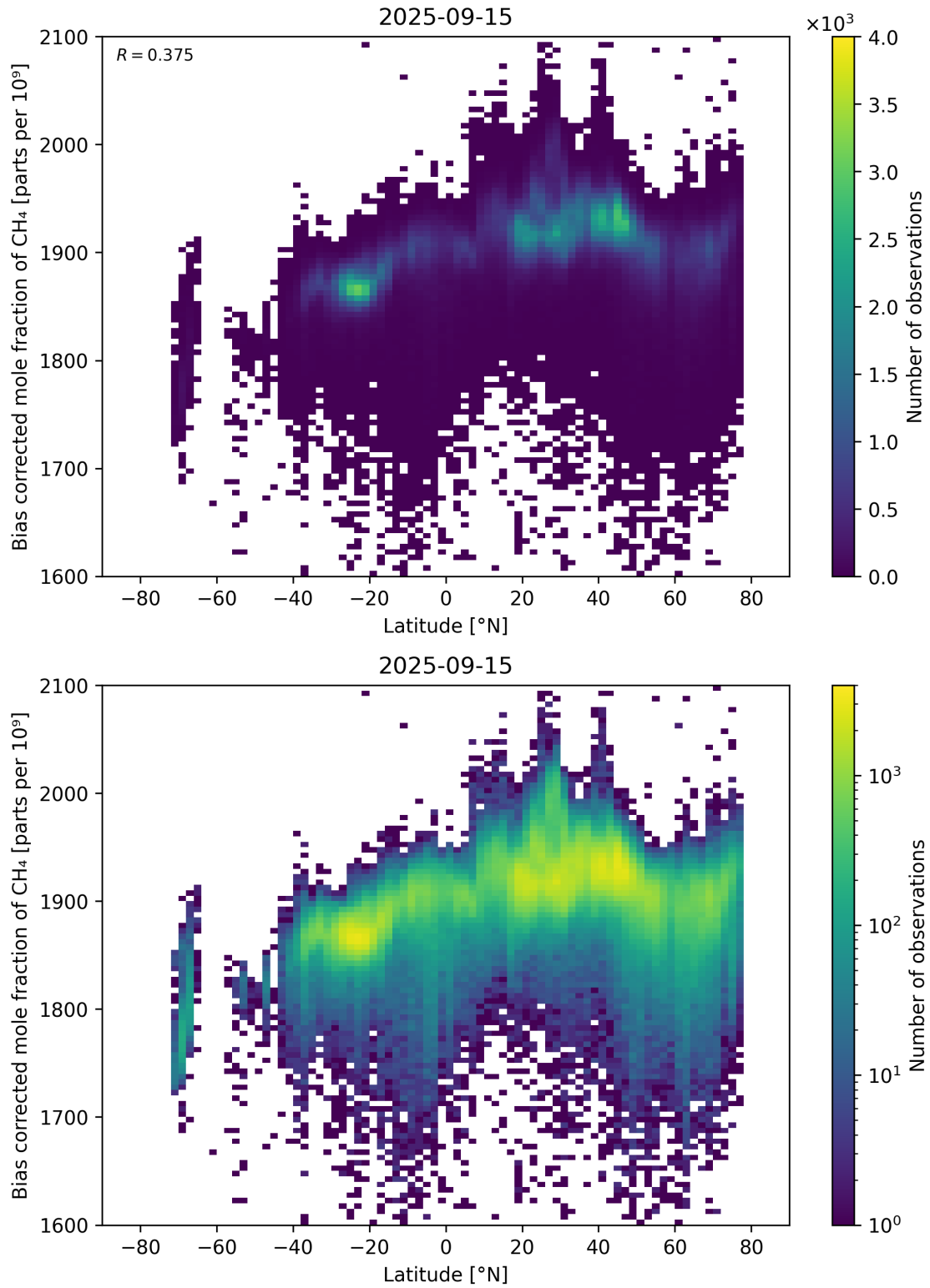
Figure 58: Scatter density plot of “Latitude” against “Bias corrected mole fraction of CH 4 ” for 2025-09-15 to 2025-09-16.
