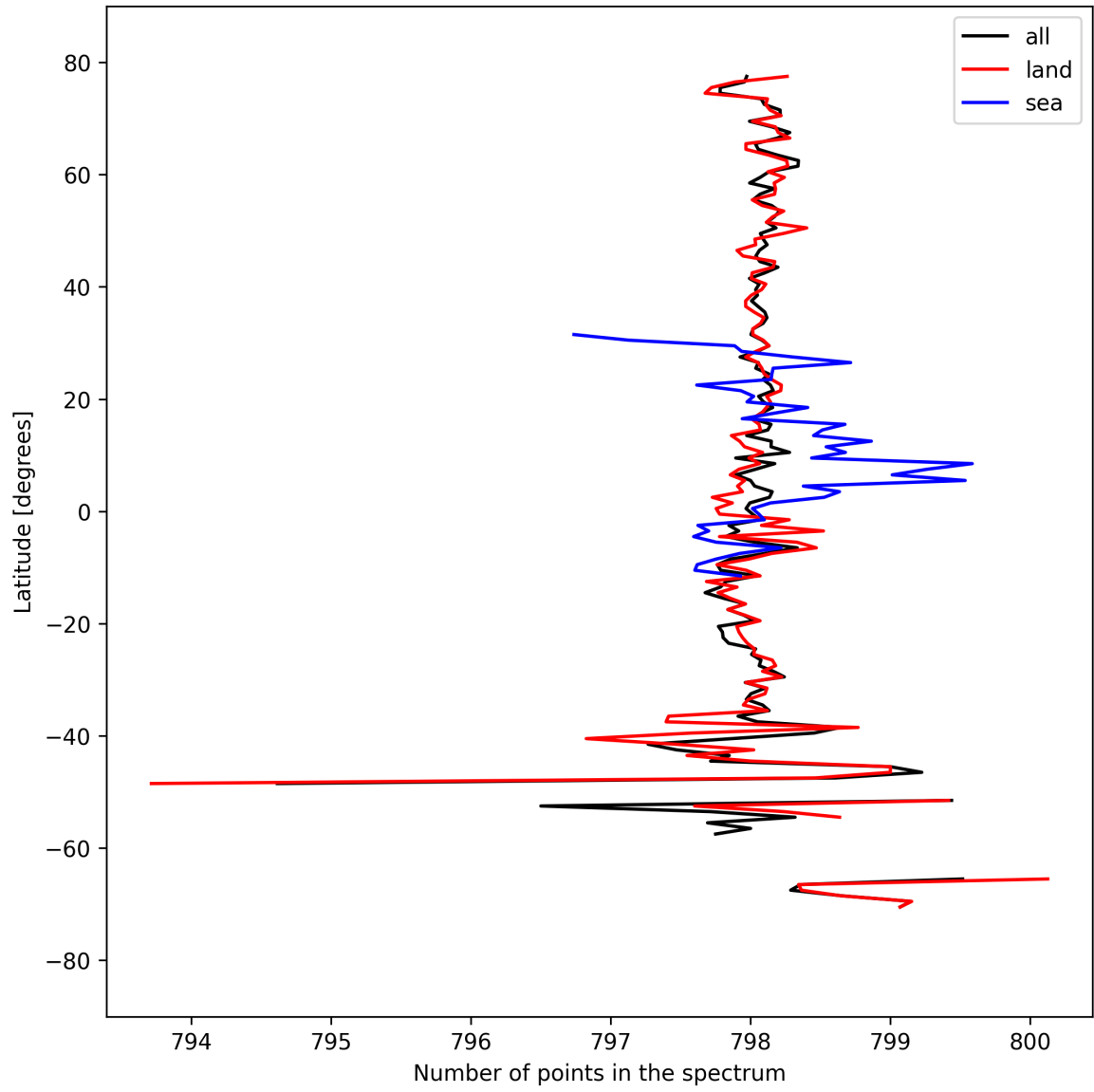
Figure 15: Zonal average of “Number of points in the spectrum” for 2025-09-15 to 2025-09-16.
