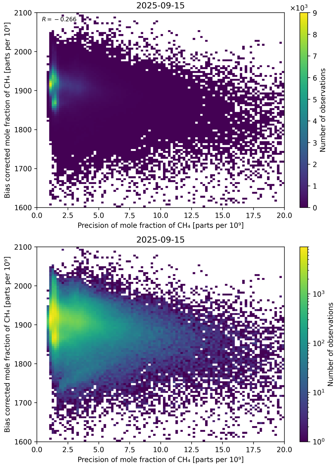
Figure 82: Scatter density plot of “Precision of mole fraction of CH 4 ” against “Bias corrected mole fraction of CH 4 ” for 2025-09-15 to 2025-09-16.
