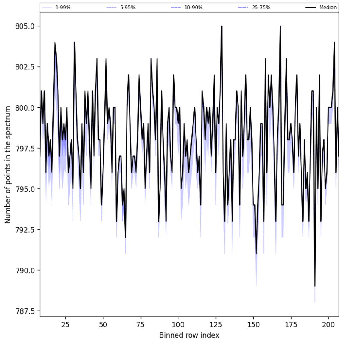
Figure 37: Along track statistics of “Number of points in the spectrum” for 2025-09-15 to 2025-09-16
