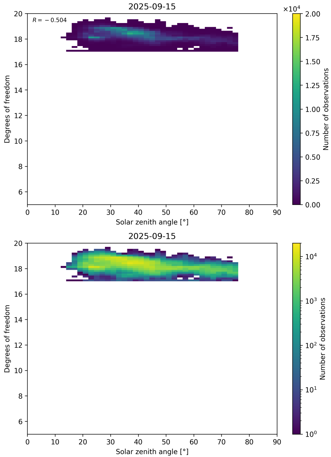
Figure 96: Scatter density plot of “Solar zenith angle” against “Degrees of freedom” for 2025-09-15 to 2025-09-16.
