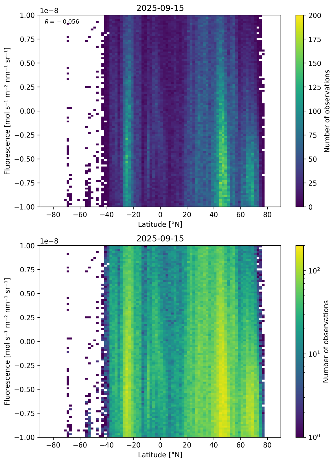
Figure 56: Scatter density plot of “Latitude” against “Fluorescence” for 2025-09-15 to 2025-09-16.
