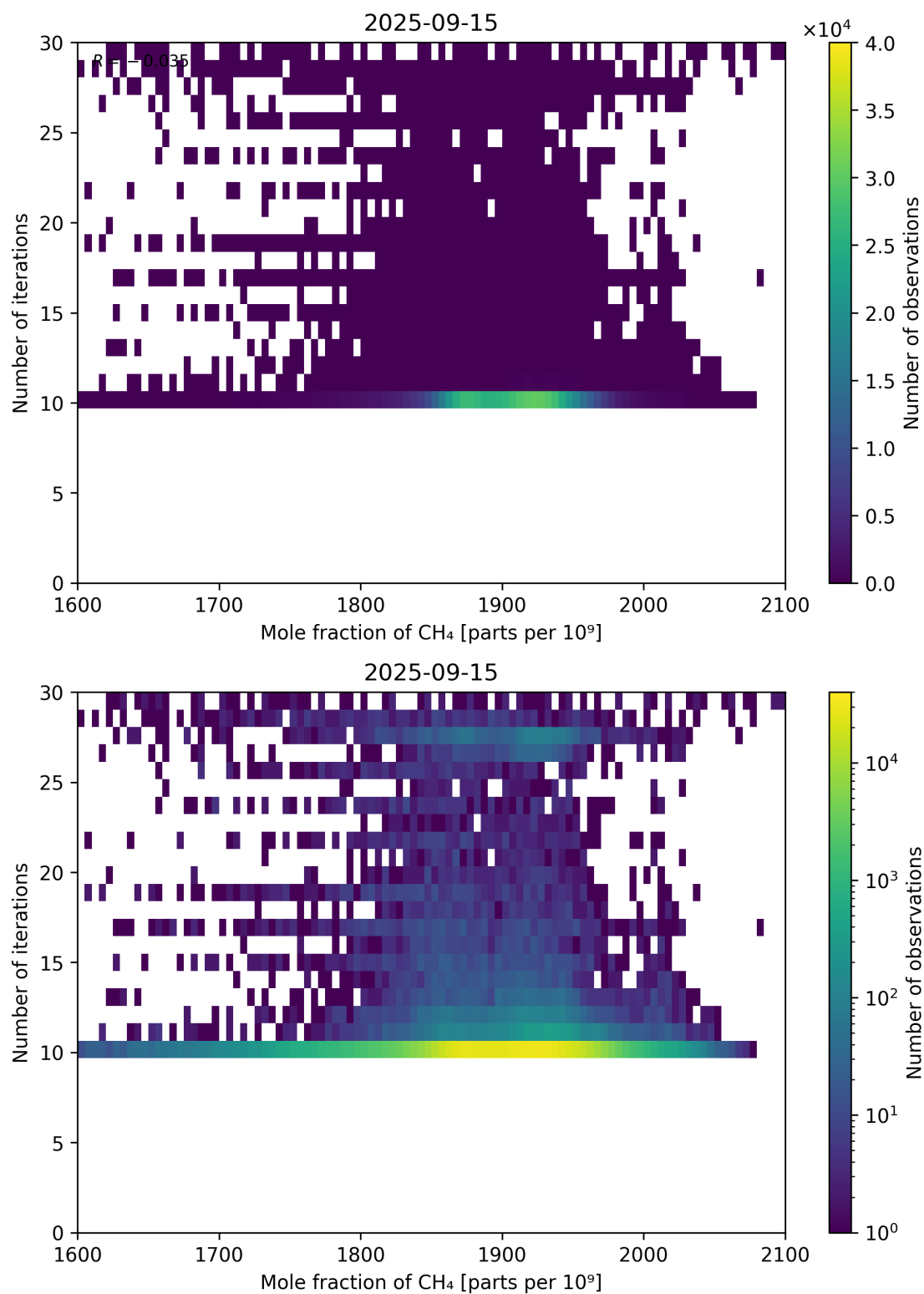
Figure 76: Scatter density plot of “Mole fraction of CH 4 ” against “Number of iterations” for 2025-09-15 to 2025-09-16.
