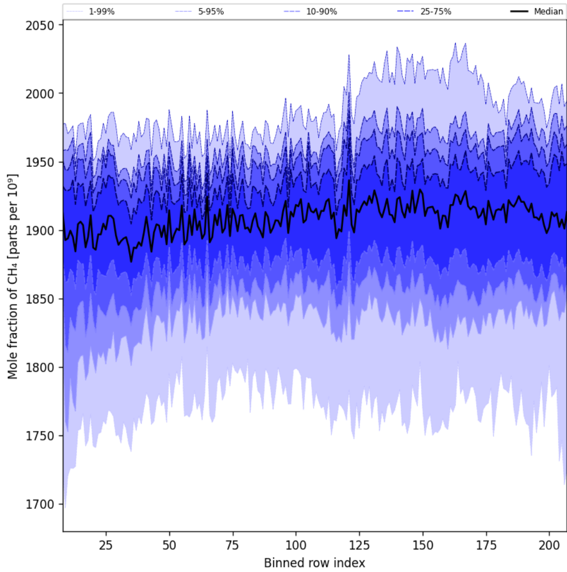
Figure 34: Along track statistics of “Mole fraction of CH 4 ” for 2025-09-15 to 2025-09-16
