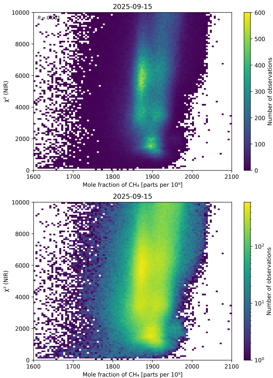
Figure 70: Scatter density plot of “Mole fraction of CH 4 ” against “ \chi^2 (NIR)” for 2025-09-15 to 2025-09-16.
