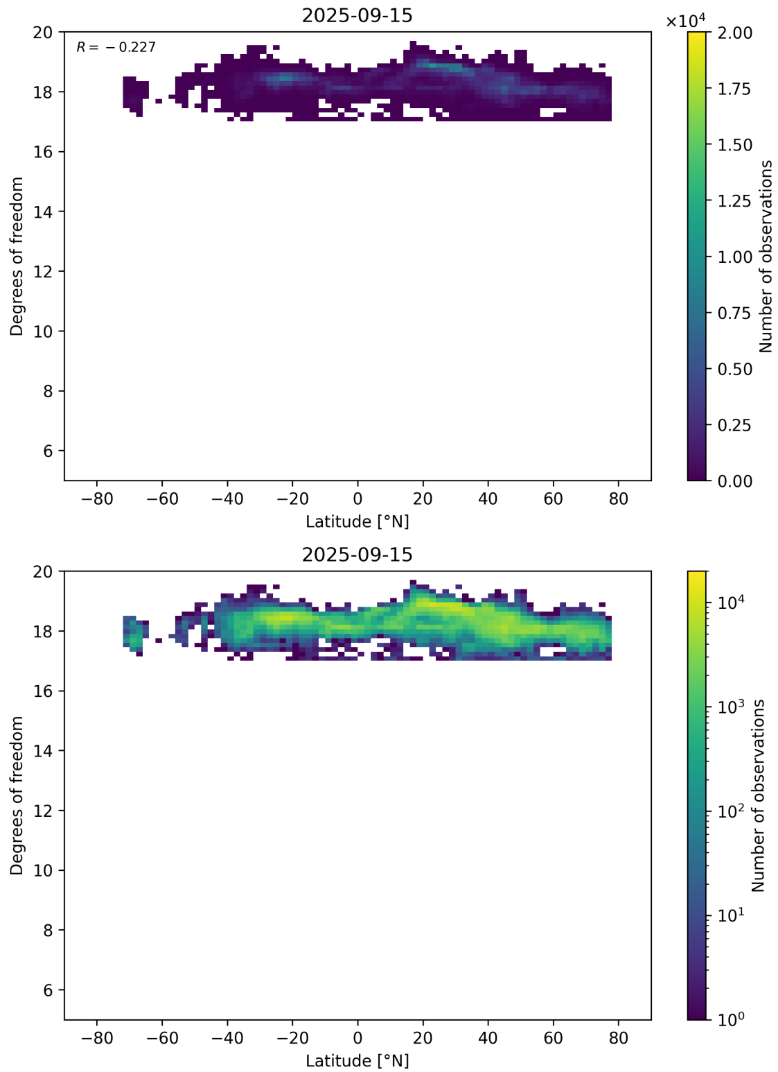
Figure 55: Scatter density plot of “Latitude” against “Degrees of freedom” for 2025-09-15 to 2025-09-16.
