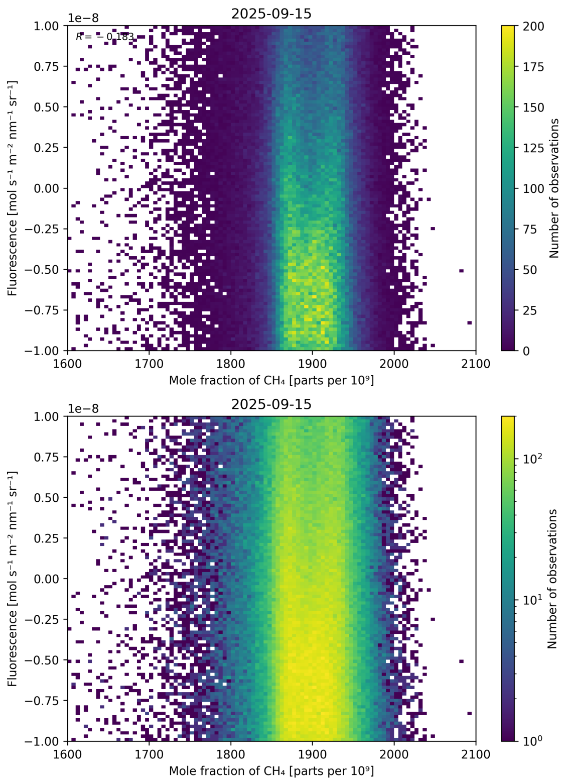
Figure 73: Scatter density plot of “Mole fraction of \text{CH}_4 ” against “Fluorescence” for 2025-09-15 to 2025-09-16.
