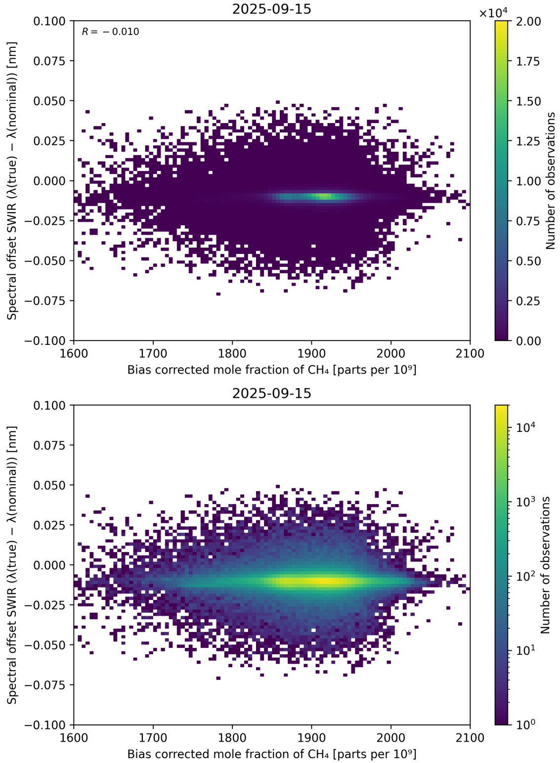
Figure 69: Scatter density plot of “Bias corrected mole fraction of \text{CH}_4 ” against “Spectral offset SWIR ( \lambda_{\text{true}} - \lambda_{\text{nominal}} )” for 2025-09-15 to 2025-09-16.
