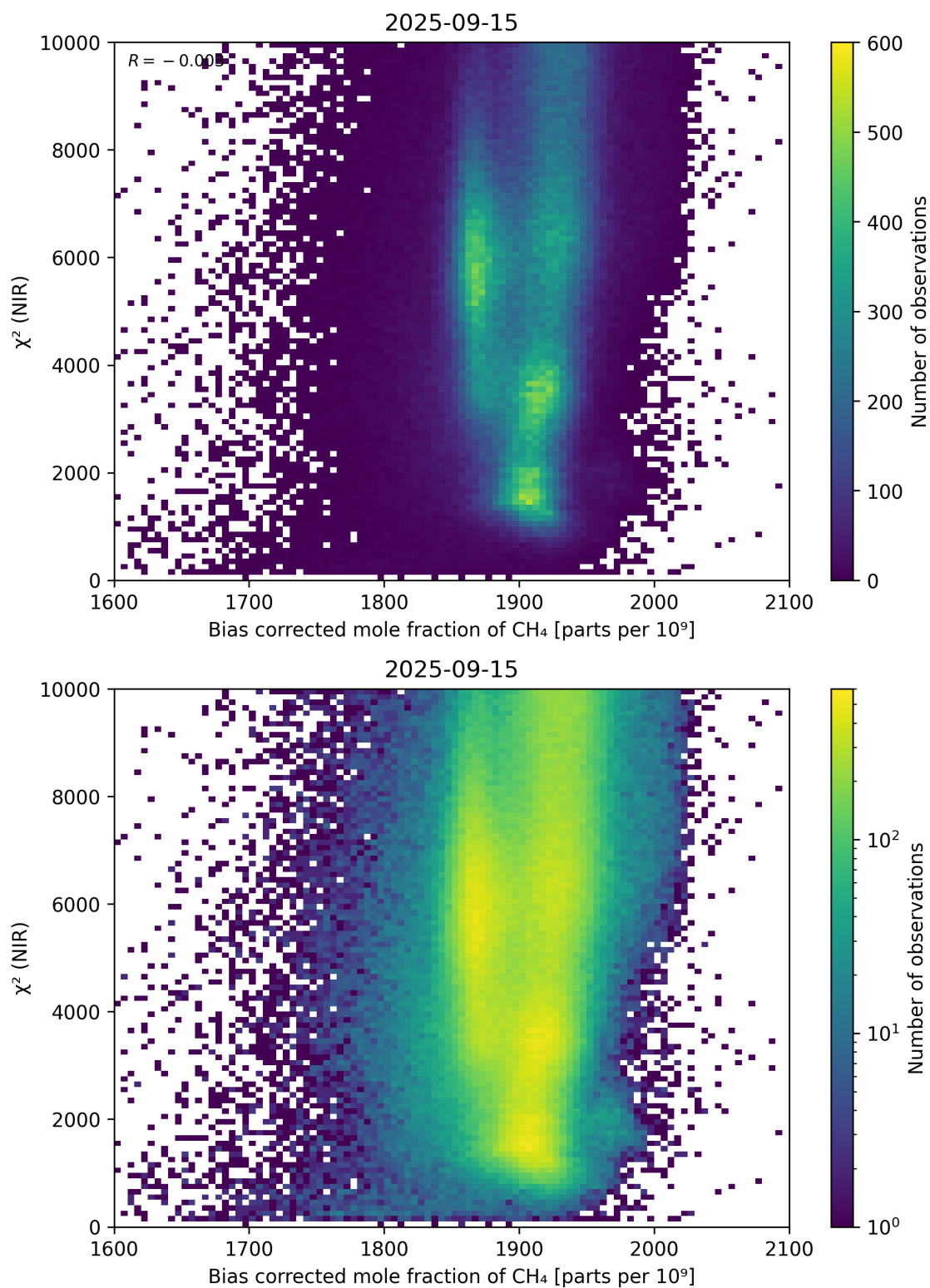
Figure 63: Scatter density plot of “Bias corrected mole fraction of CH 4 ” against “ \chi^2 (NIR)” for 2025-09-15 to 2025-09-16.
