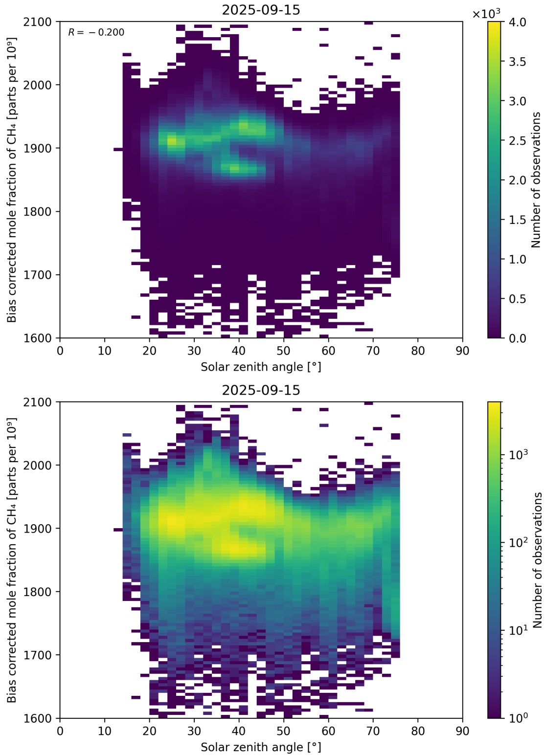
Figure 100: Scatter density plot of “Solar zenith angle” against “Bias corrected mole fraction of CH 4 ” for 2025-09-15 to 2025-09-16.
