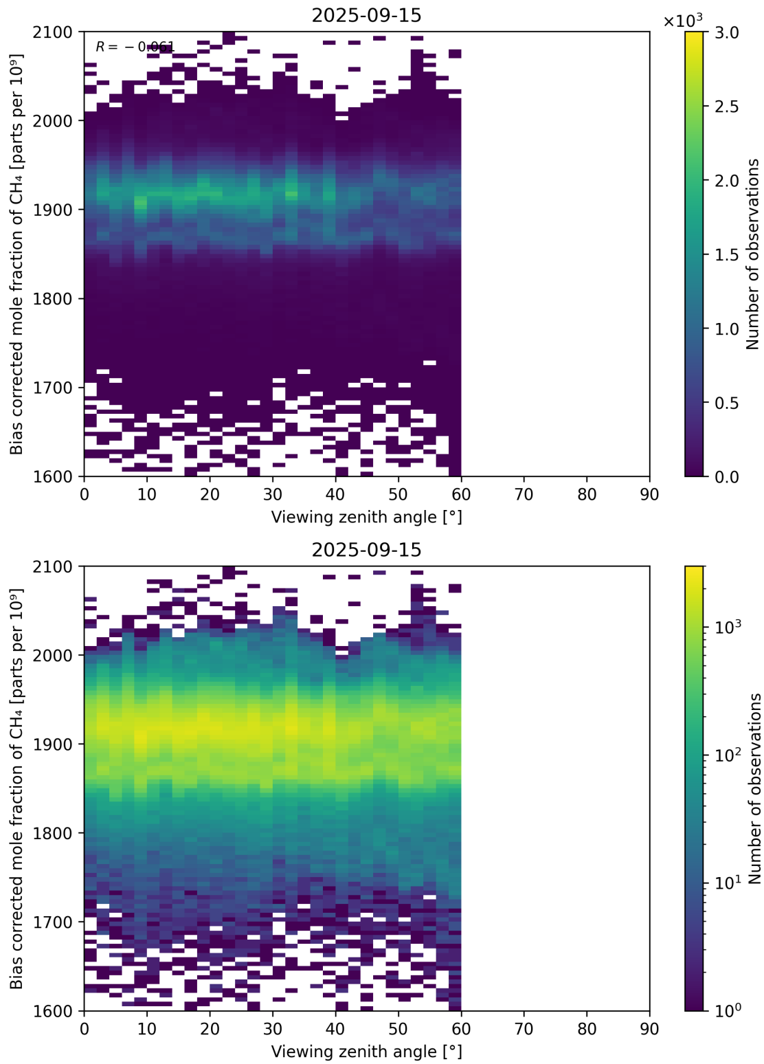
Figure 111: Scatter density plot of “Viewing zenith angle” against “Bias corrected mole fraction of CH 4 ” for 2025-09-15 to 2025-09-16.
