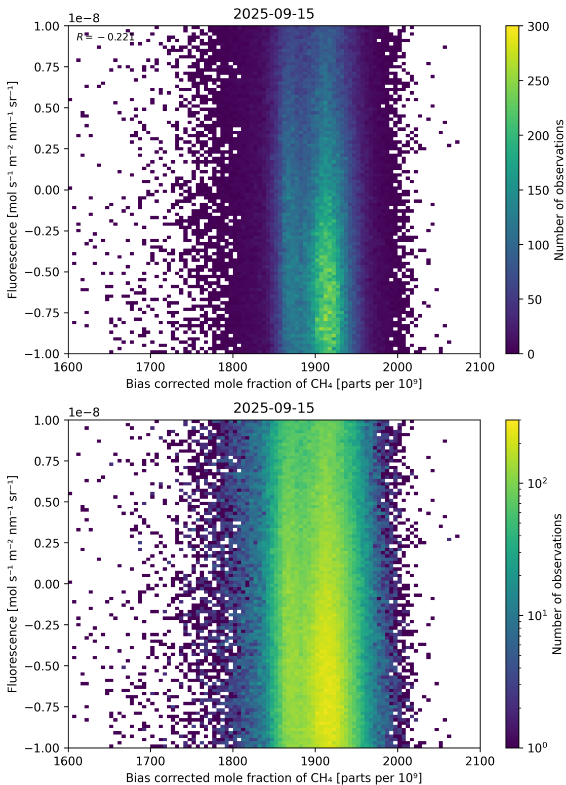
Figure 66: Scatter density plot of “Bias corrected mole fraction of CH 4 ” against “Fluorescence” for 2025-09-15 to 2025-09-16.
