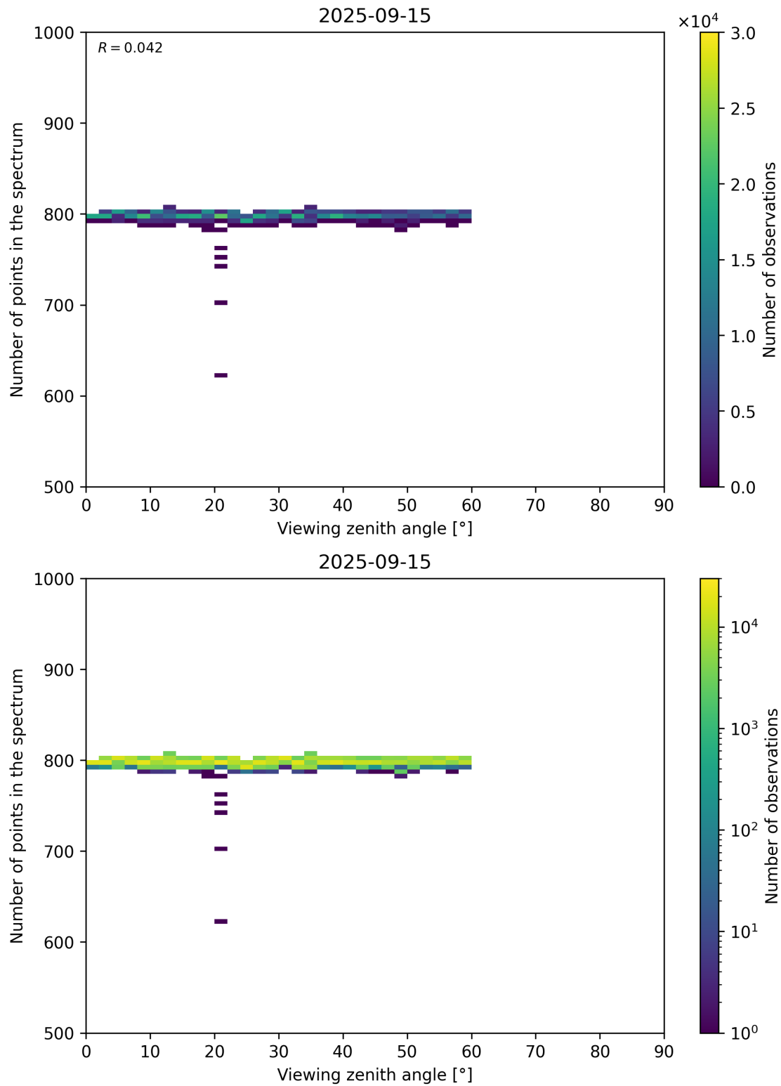
Figure 114: Scatter density plot of “Viewing zenith angle” against “Number of points in the spectrum” for 2025-09-15 to 2025-09-16.
