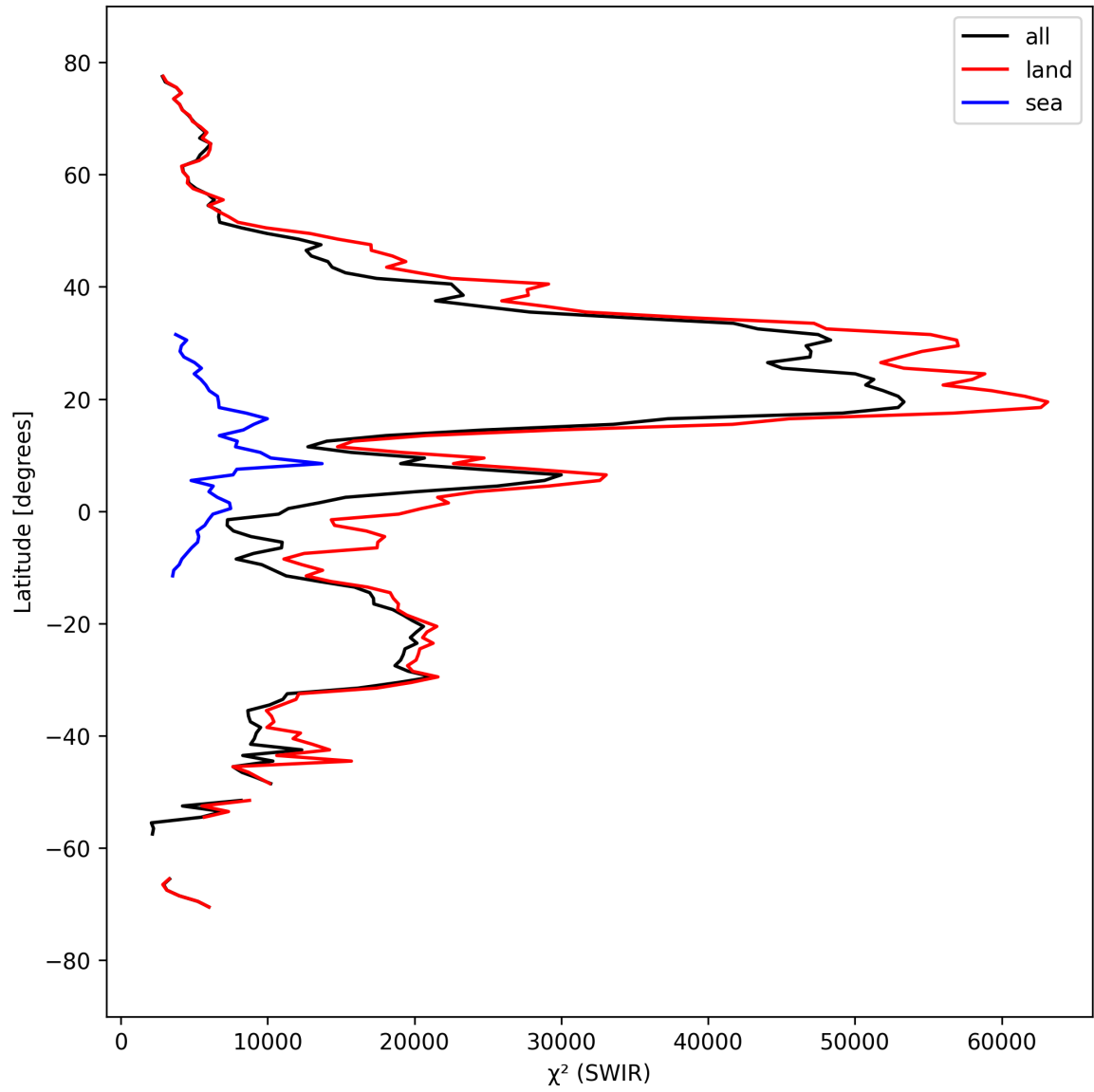
Figure 17: Zonal average of “ \chi^2 (SWIR)” for 2025-09-15 to 2025-09-16.
