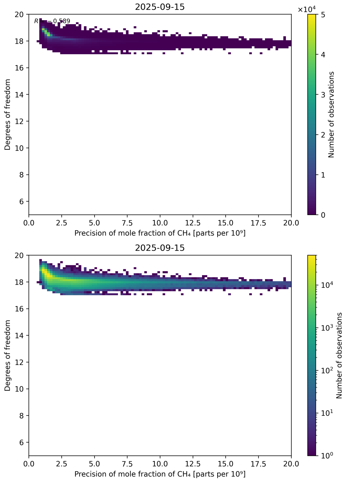
Figure 80: Scatter density plot of “Precision of mole fraction of CH 4 ” against “Degrees of freedom” for 2025-09-15 to 2025-09-16.
