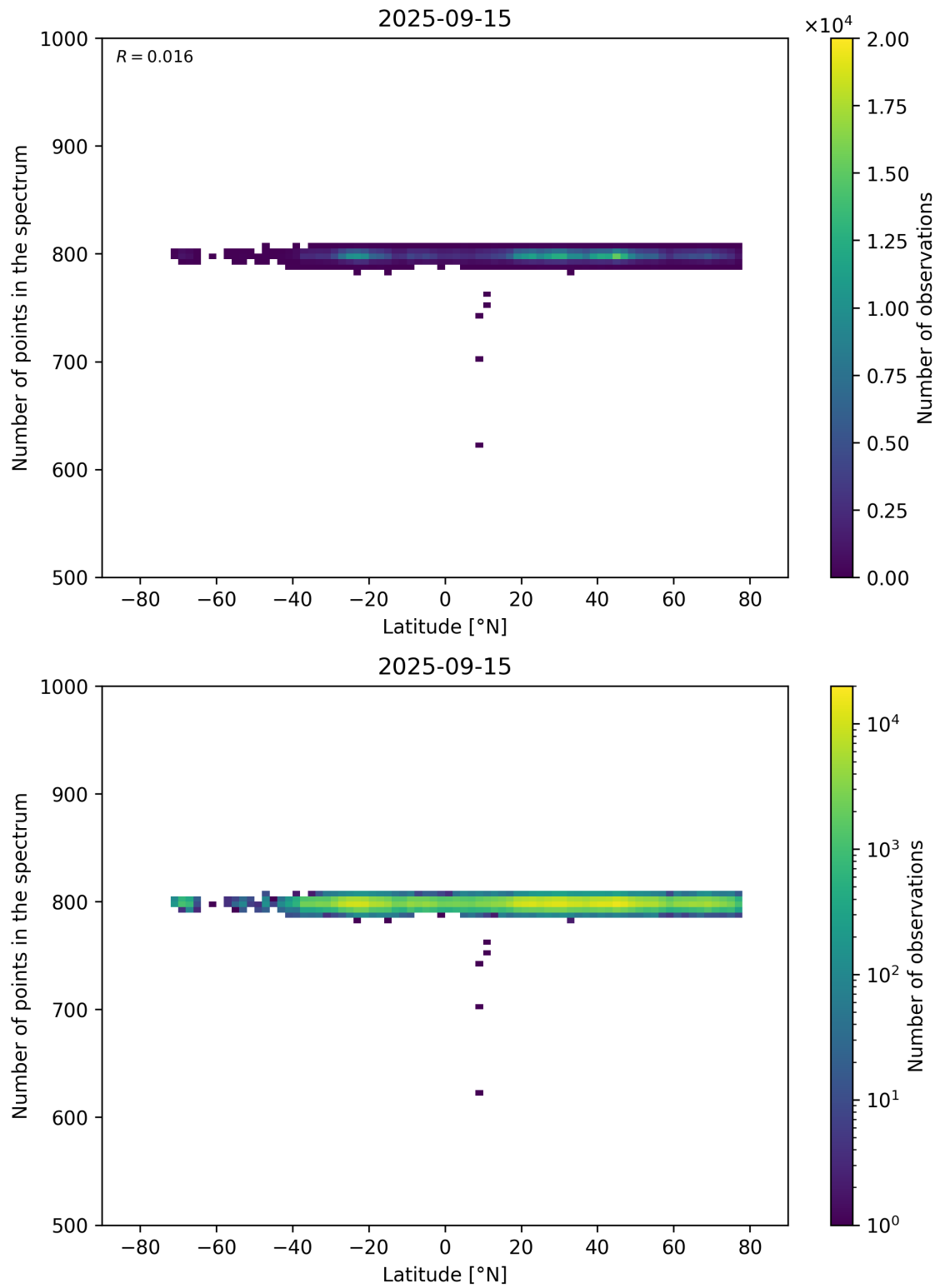
Figure 61: Scatter density plot of “Latitude” against “Number of points in the spectrum” for 2025-09-15 to 2025-09-16.
