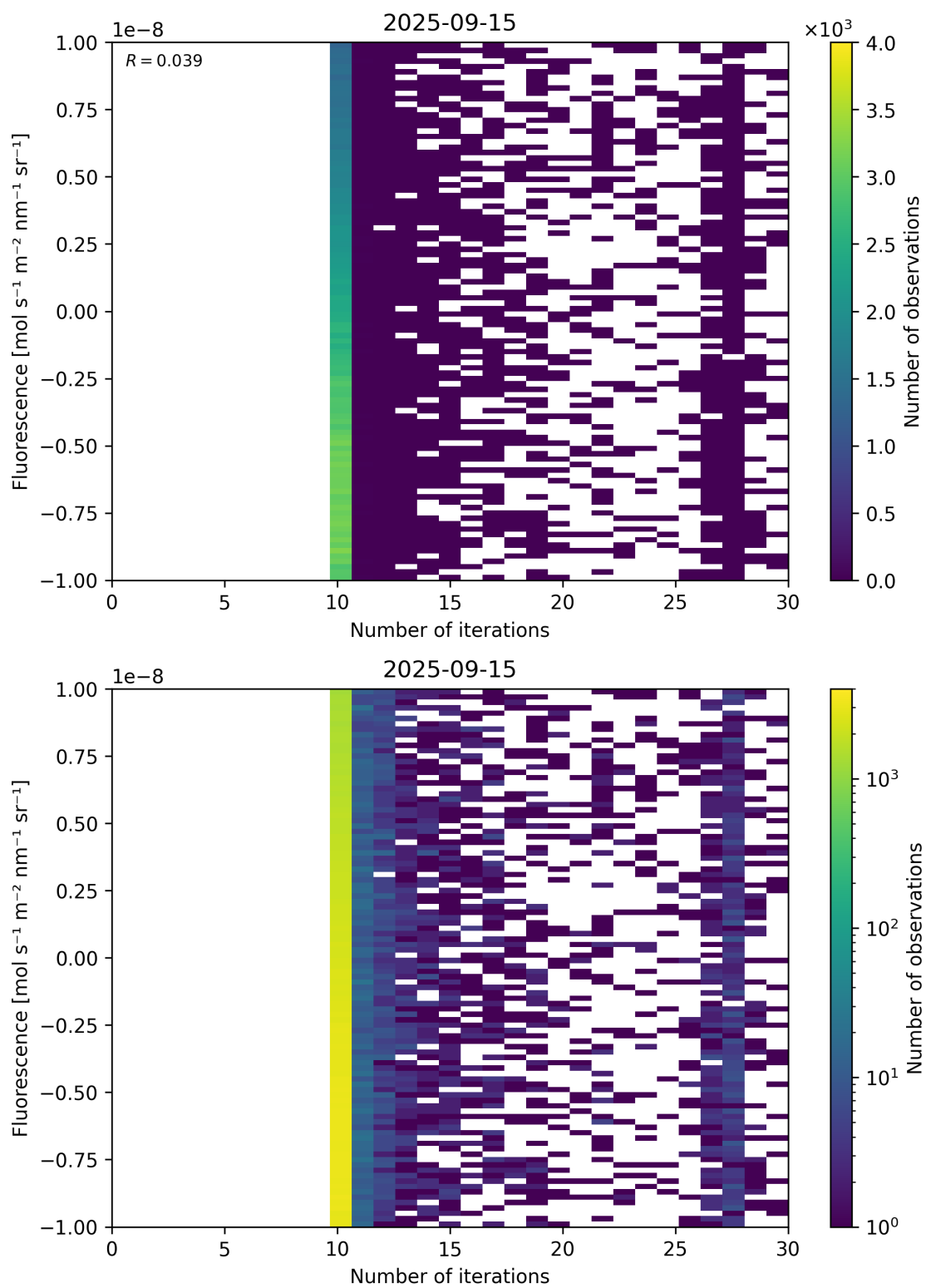
Figure 87: Scatter density plot of “Number of iterations” against “Fluorescence” for 2025-09-15 to 2025-09-16.
