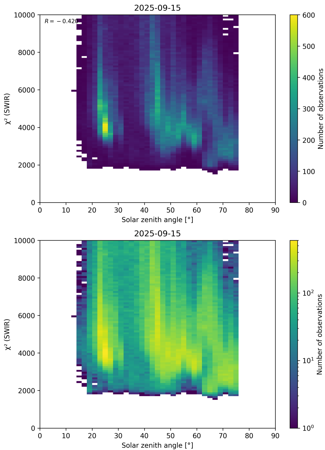
Figure 95: Scatter density plot of “Solar zenith angle” against “ \chi^2 (SWIR)” for 2025-09-15 to 2025-09-16.
