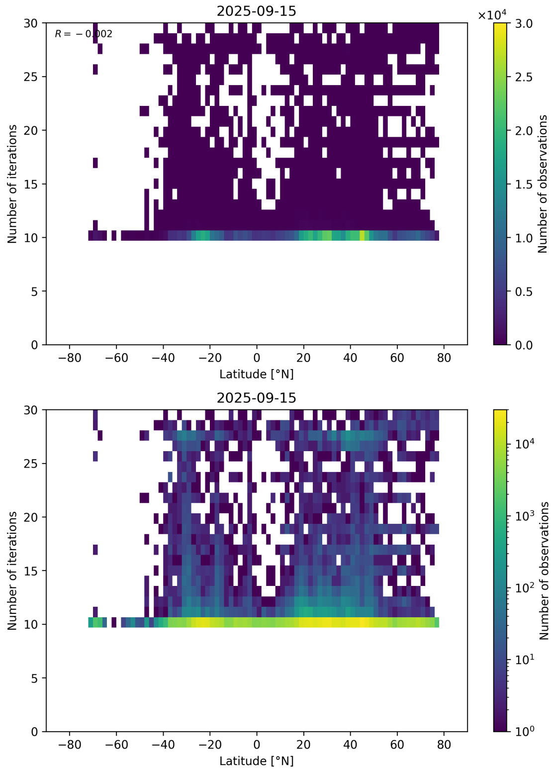
Figure 60: Scatter density plot of “Latitude” against “Number of iterations” for 2025-09-15 to 2025-09-16.
