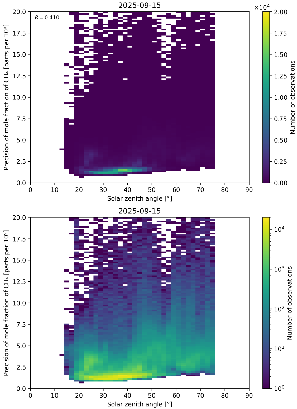
Figure 101: Scatter density plot of “Solar zenith angle” against “Precision of mole fraction of \text{CH}_4 ” for 2025-09-15 to 2025-09-16.
