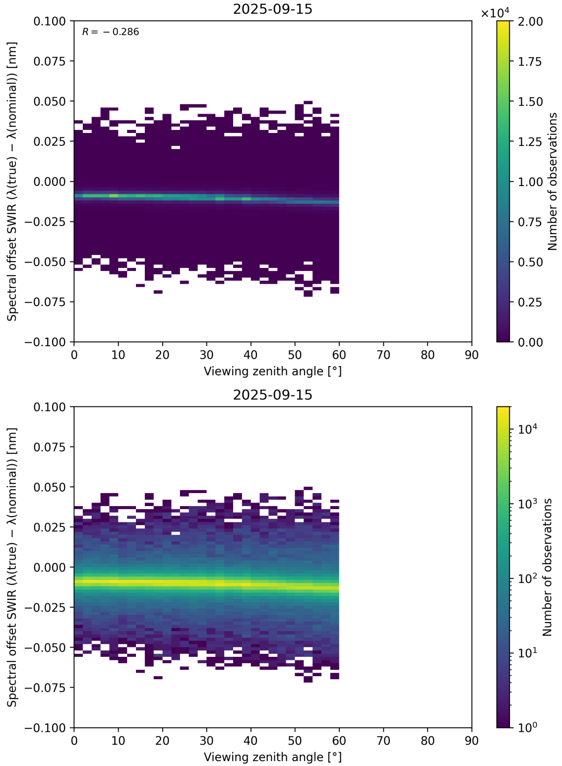
Figure 116: Scatter density plot of “Viewing zenith angle” against “Spectral offset SWIR ( \lambda_{\text{true}} - \lambda_{\text{nominal}} )” for 2025-09-15 to 2025-09-16.
