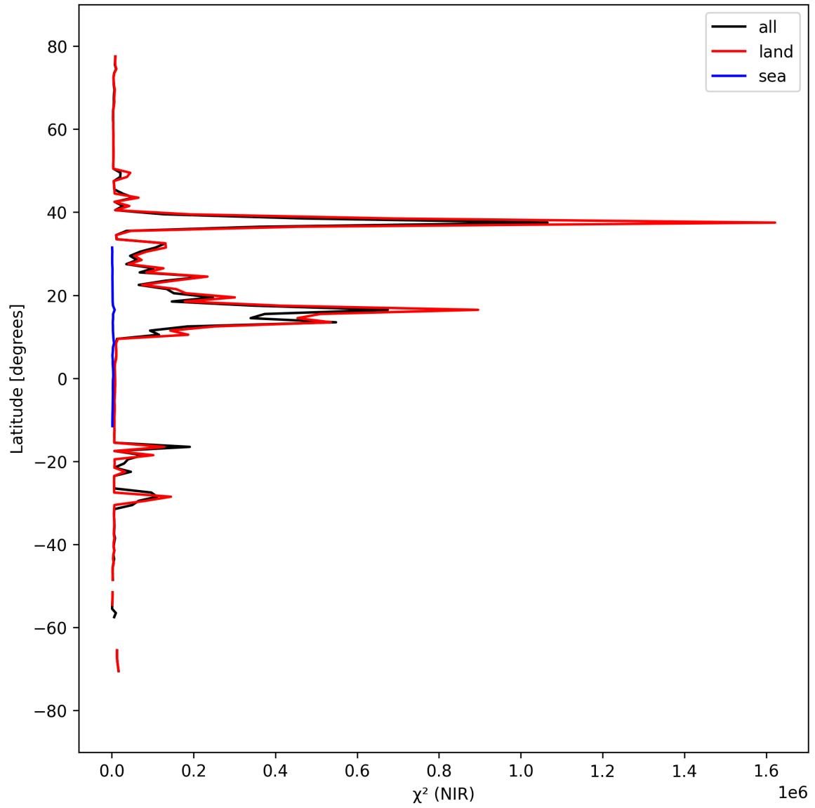
Figure 18: Zonal average of “ \chi^2 (NIR)” for 2025-09-15 to 2025-09-16.
