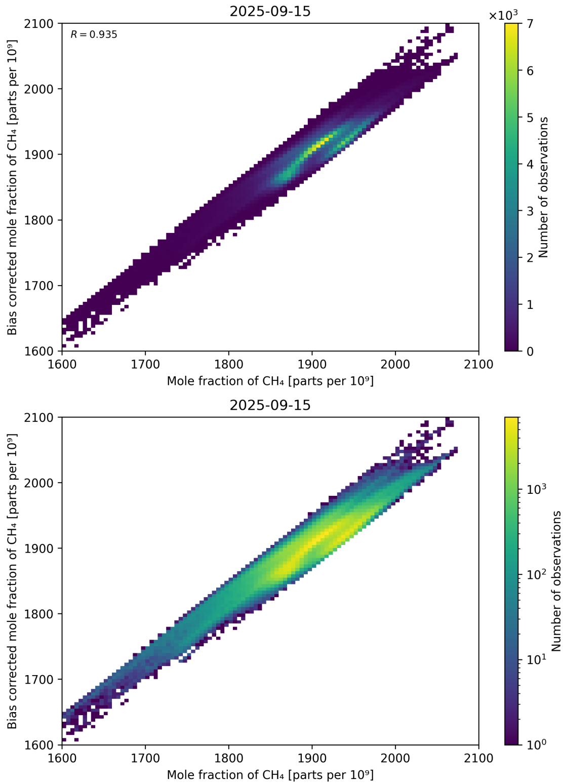
Figure 74: Scatter density plot of “Mole fraction of CH 4 ” against “Bias corrected mole fraction of CH 4 ” for 2025-09-15 to 2025-09-16.
