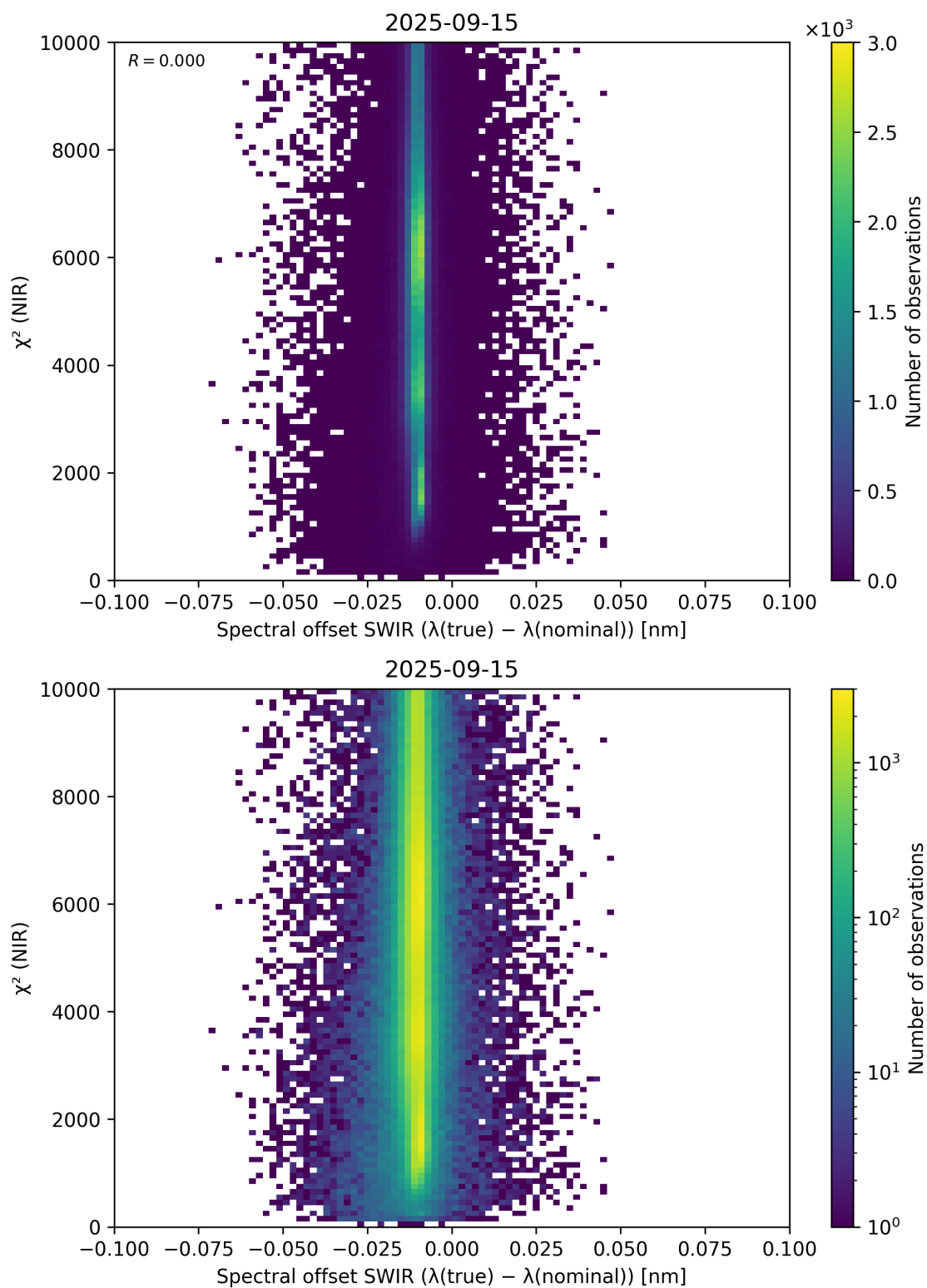
Figure 117: Scatter density plot of “Spectral offset SWIR ( \lambda_{\text{true}} - \lambda_{\text{nominal}} )” against “ \chi^2 (NIR)” for 2025-09-15 to 2025-09-16.
