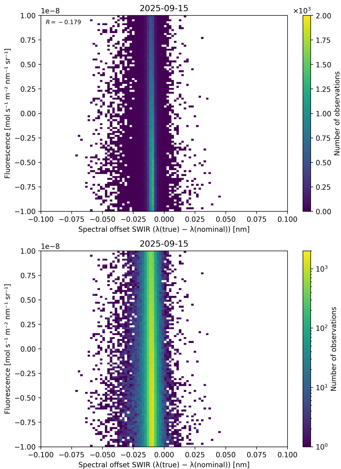
Figure 120: Scatter density plot of “Spectral offset SWIR ( \lambda_{\text{true}} - \lambda_{\text{nominal}} )” against “Fluorescence” for 2025-09-15 to 2025-09-16.
