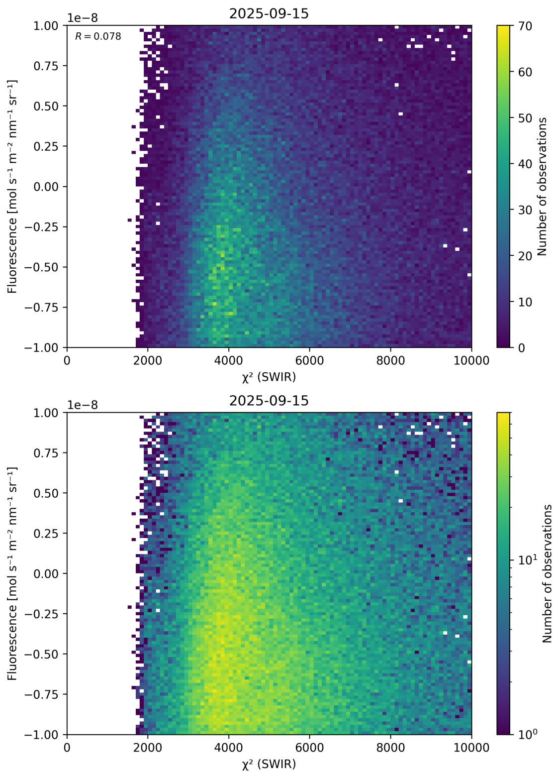
Figure 49: Scatter density plot of “ \chi^2 (SWIR)” against “Fluorescence” for 2025-09-15 to 2025-09-16.
