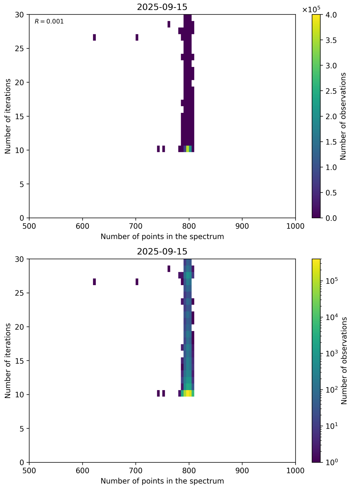
Figure 92: Scatter density plot of “Number of points in the spectrum” against “Number of iterations” for 2025-09-15 to 2025-09-16.
