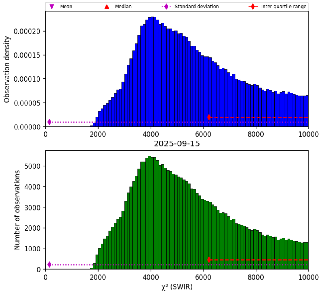
Figure 28: Histogram of “ \chi^2 (SWIR)” for 2025-09-15 to 2025-09-16
