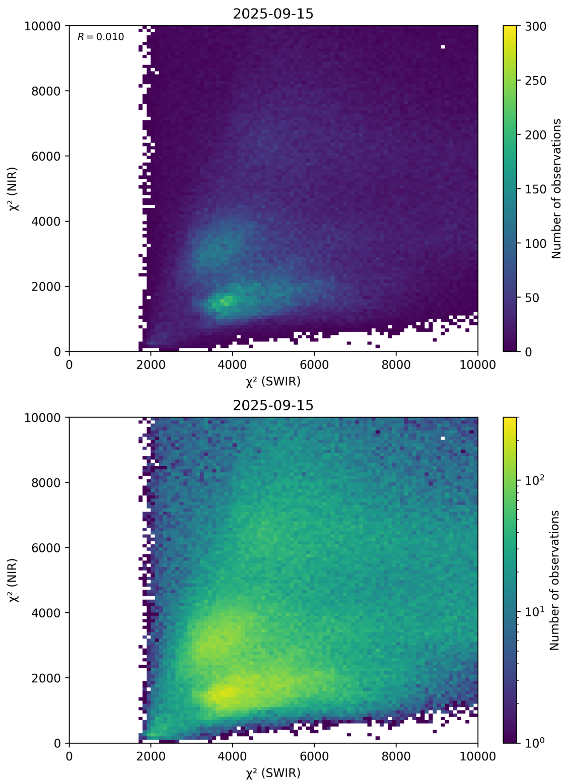
Figure 47: Scatter density plot of “ \chi^2 (SWIR)” against “ \chi^2 (NIR)” for 2025-09-15 to 2025-09-16.
