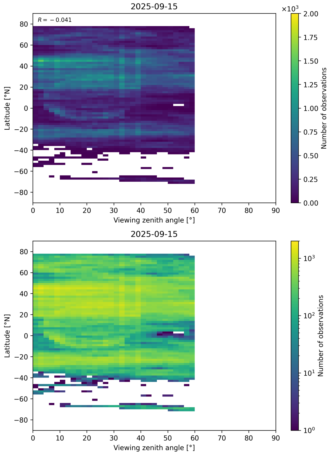
Figure 109: Scatter density plot of “Viewing zenith angle” against “Latitude” for 2025-09-15 to 2025-09-16.
