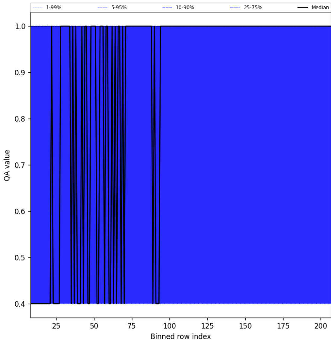
Figure 33: Along track statistics of “QA value” for 2025-09-15 to 2025-09-16
