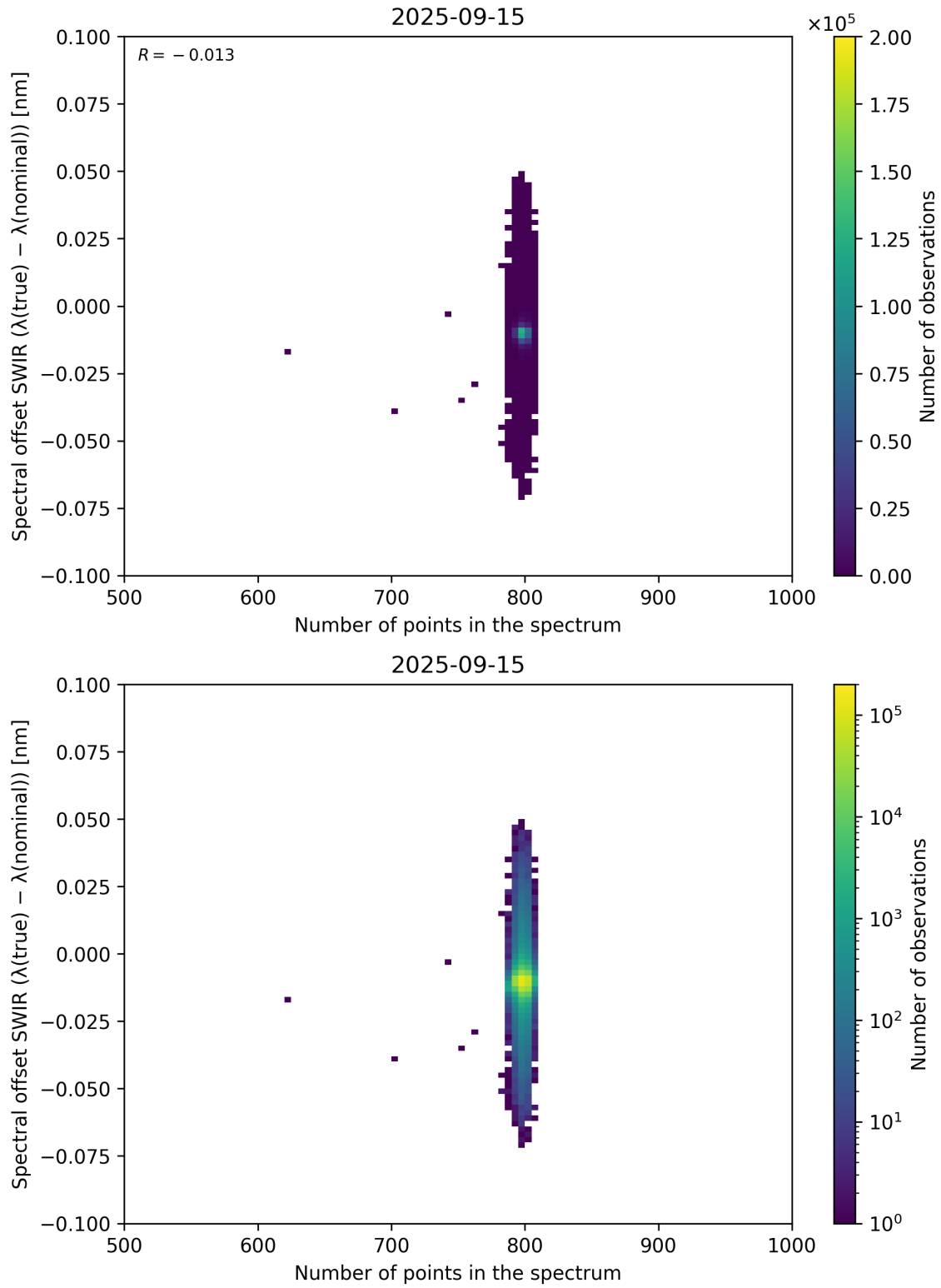
Figure 93: Scatter density plot of “Number of points in the spectrum” against “Spectral offset SWIR ( \lambda_{\text{true}} - \lambda_{\text{nominal}} )” for 2025-09-15 to 2025-09-16.
