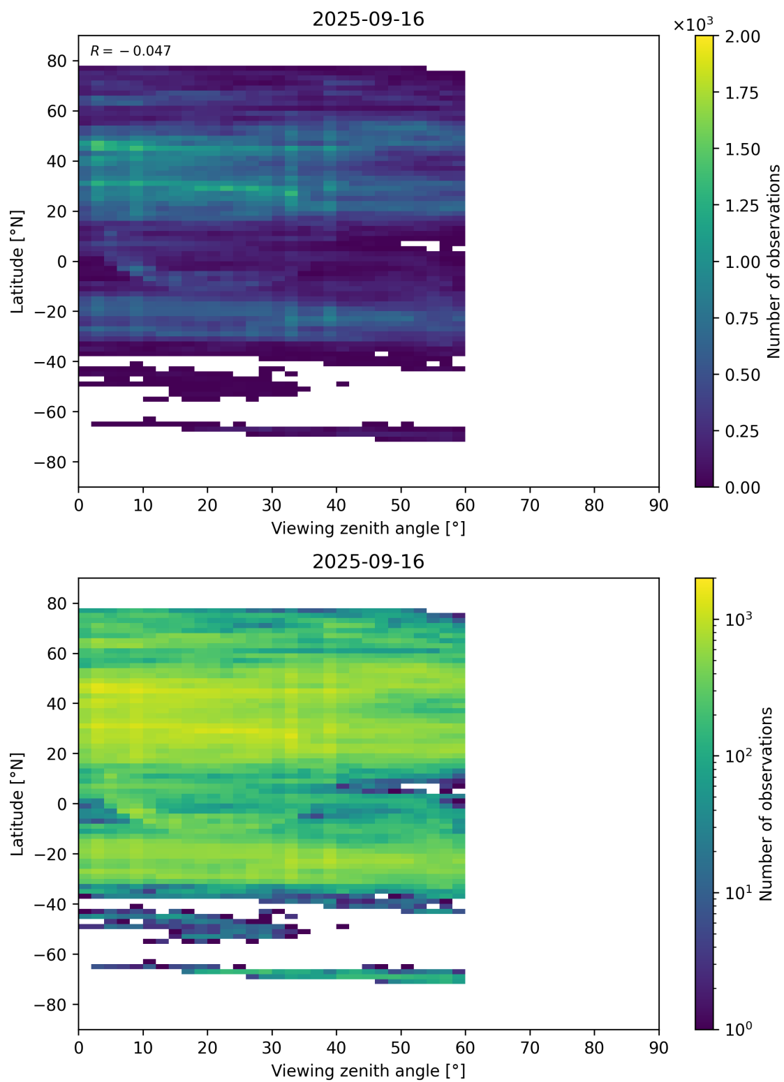
Figure 109: Scatter density plot of “Viewing zenith angle” against “Latitude” for 2025-09-15 to 2025-09-17.
