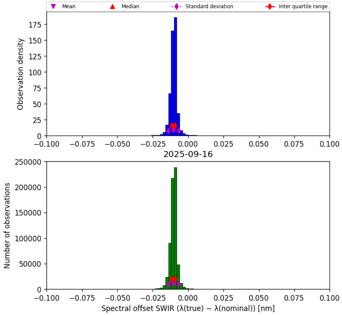
Figure 27: Histogram of “Spectral offset SWIR ( \lambda_{\text{true}} - \lambda_{\text{nominal}} )” for 2025-09-15 to 2025-09-17
