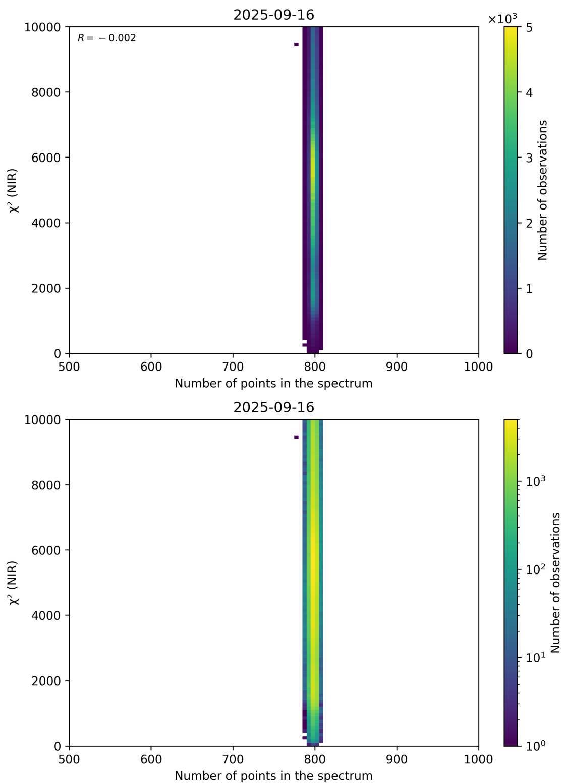
Figure 88: Scatter density plot of “Number of points in the spectrum” against “ \chi^2 (NIR)” for 2025-09-15 to 2025-09-17.
