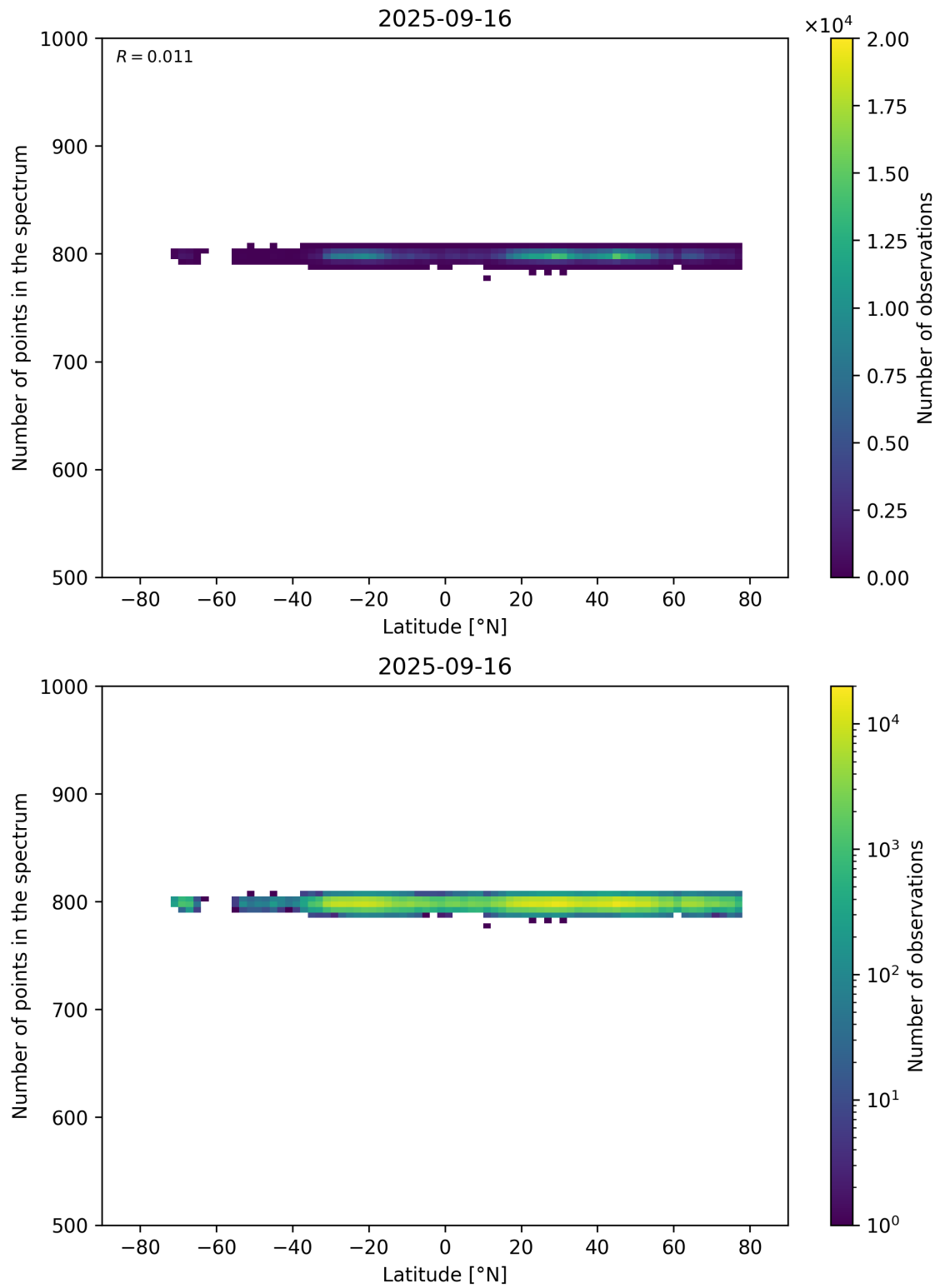
Figure 61: Scatter density plot of “Latitude” against “Number of points in the spectrum” for 2025-09-15 to 2025-09-17.
