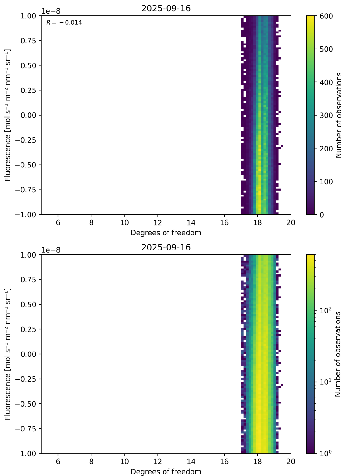
Figure 51: Scatter density plot of “Degrees of freedom” against “Fluorescence” for 2025-09-15 to 2025-09-17.
