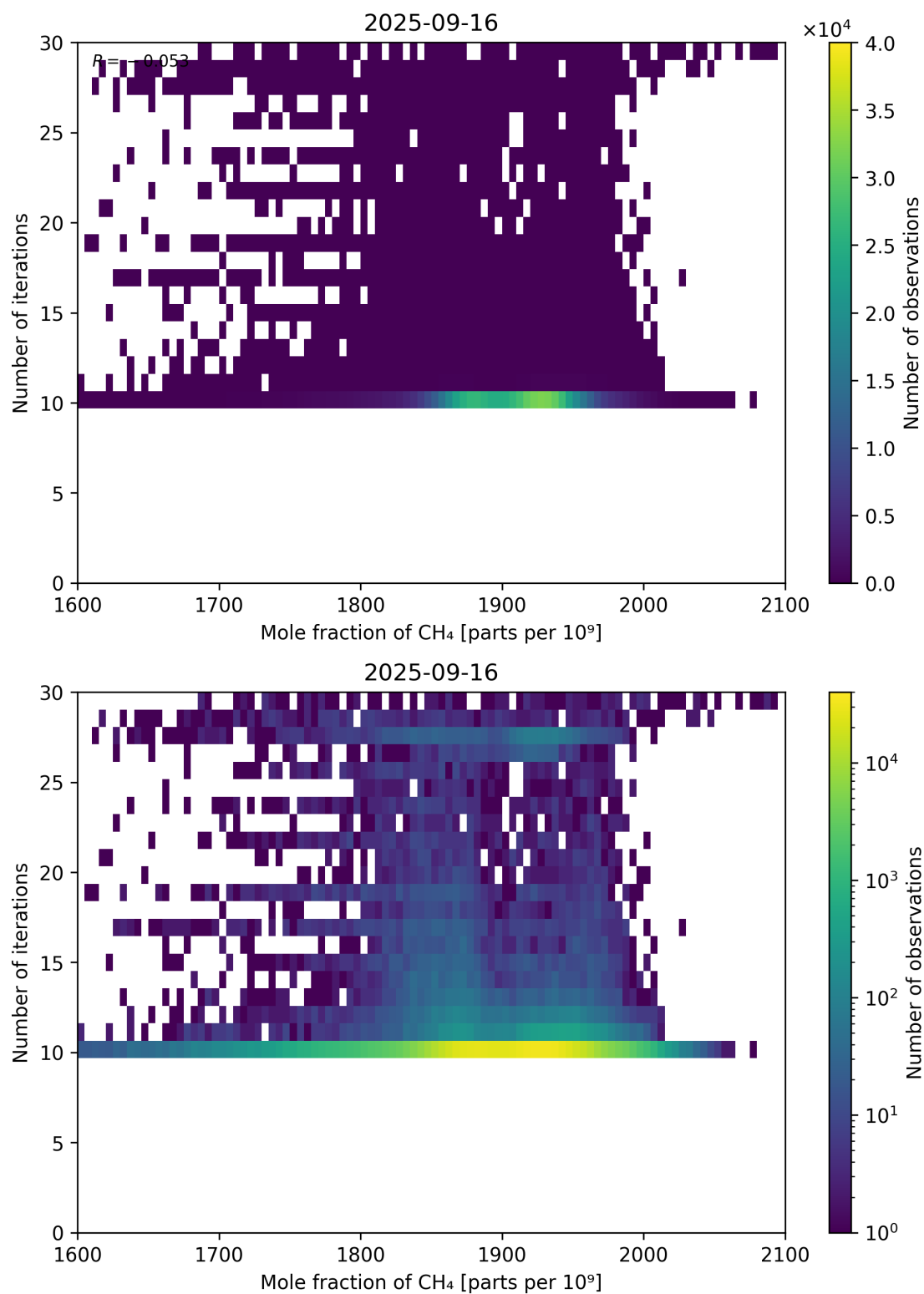
Figure 76: Scatter density plot of “Mole fraction of CH 4 ” against “Number of iterations” for 2025-09-15 to 2025-09-17.
