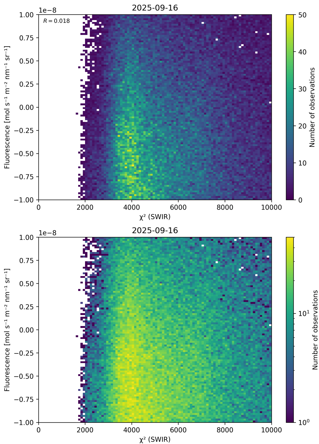
Figure 49: Scatter density plot of “ \chi^2 (SWIR)” against “Fluorescence” for 2025-09-15 to 2025-09-17.
