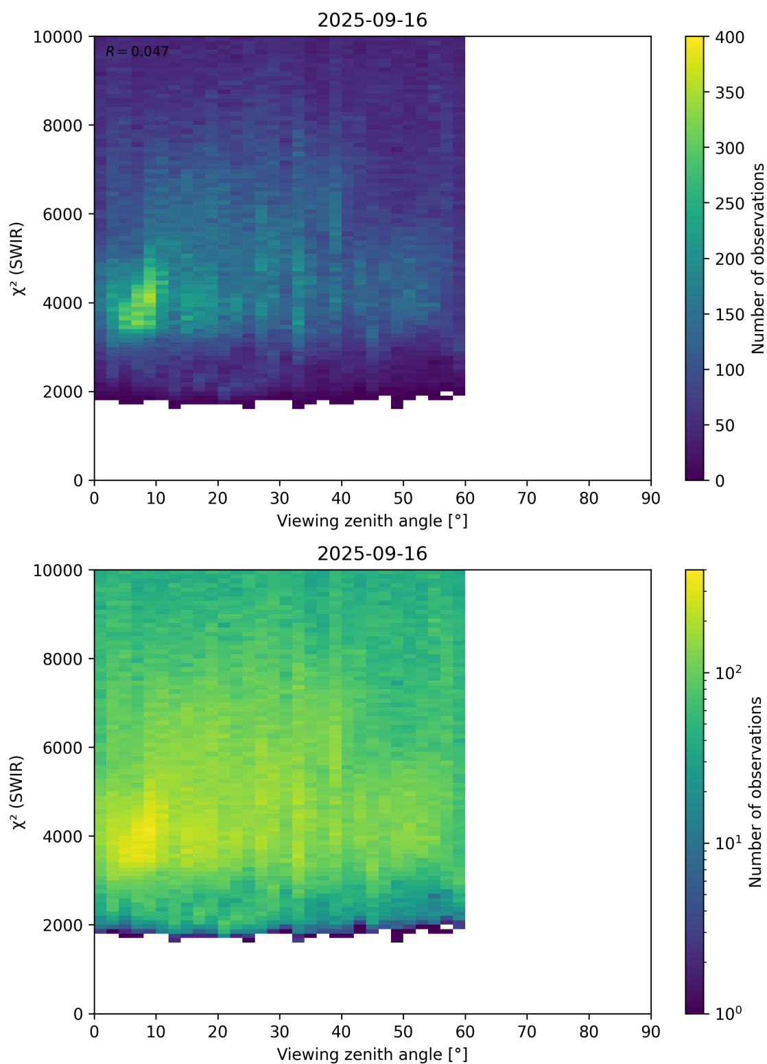
Figure 106: Scatter density plot of “Viewing zenith angle” against “ \chi^2 (SWIR)” for 2025-09-15 to 2025-09-17.
