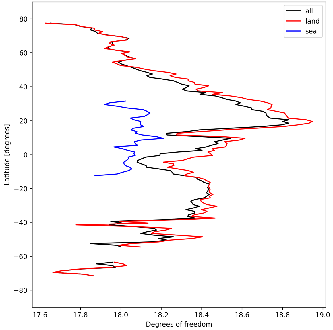
Figure 19: Zonal average of “Degrees of freedom” for 2025-09-15 to 2025-09-17.
