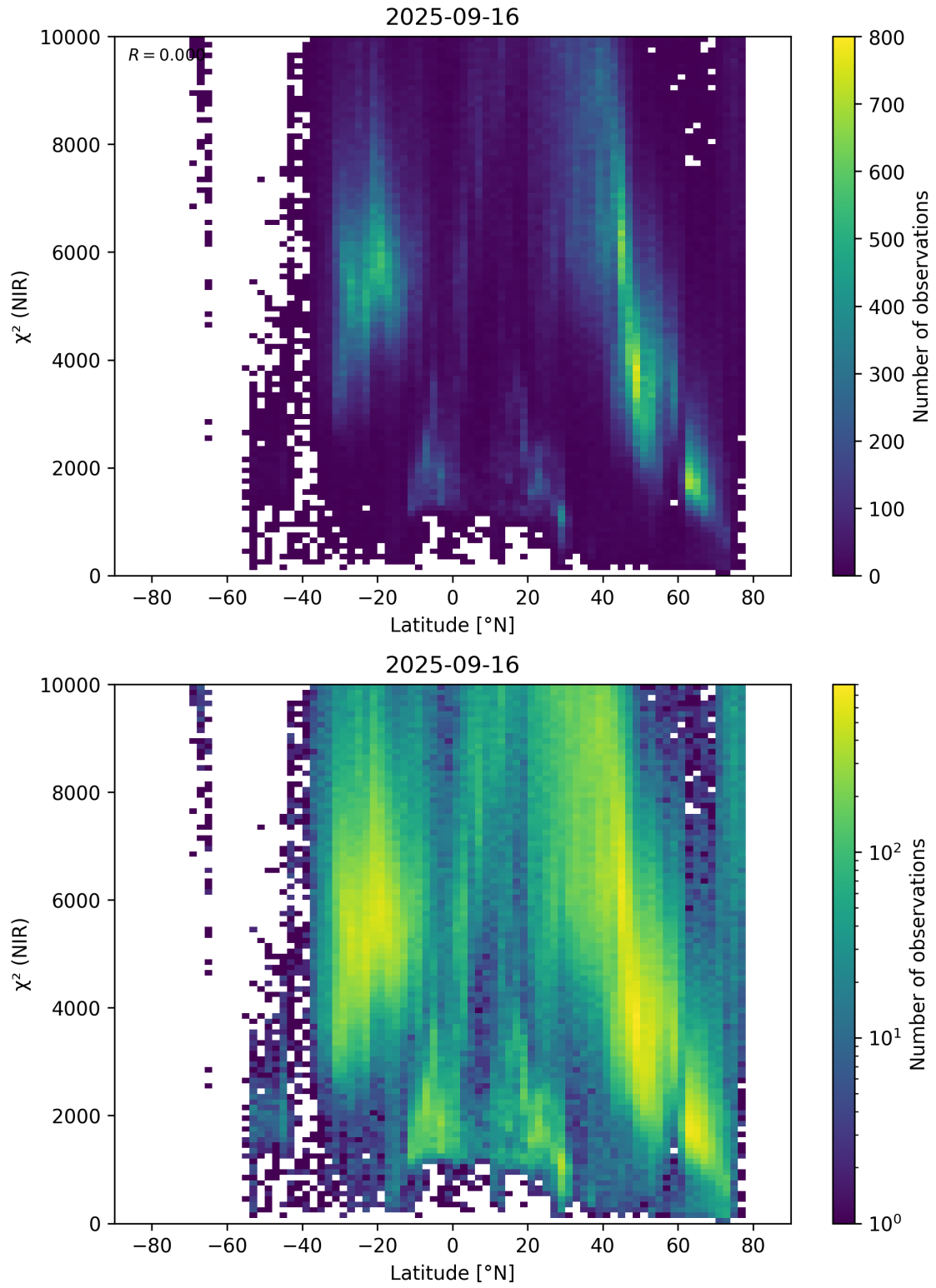
Figure 53: Scatter density plot of “Latitude” against “ \chi^2 (NIR)” for 2025-09-15 to 2025-09-17.
