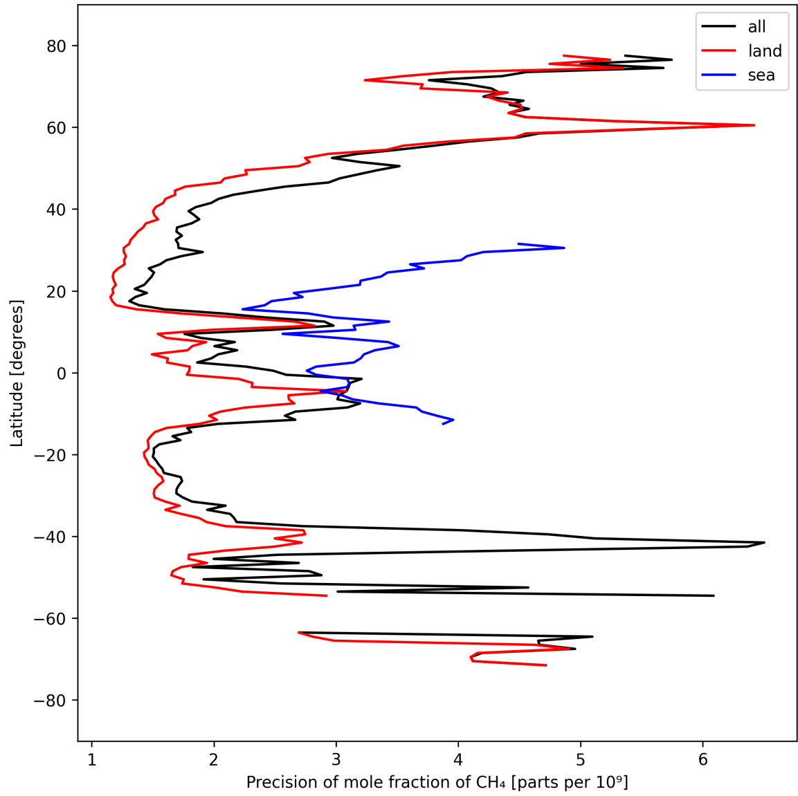
Figure 13: Zonal average of “Precision of mole fraction of CH 4 ” for 2025-09-15 to 2025-09-17.
