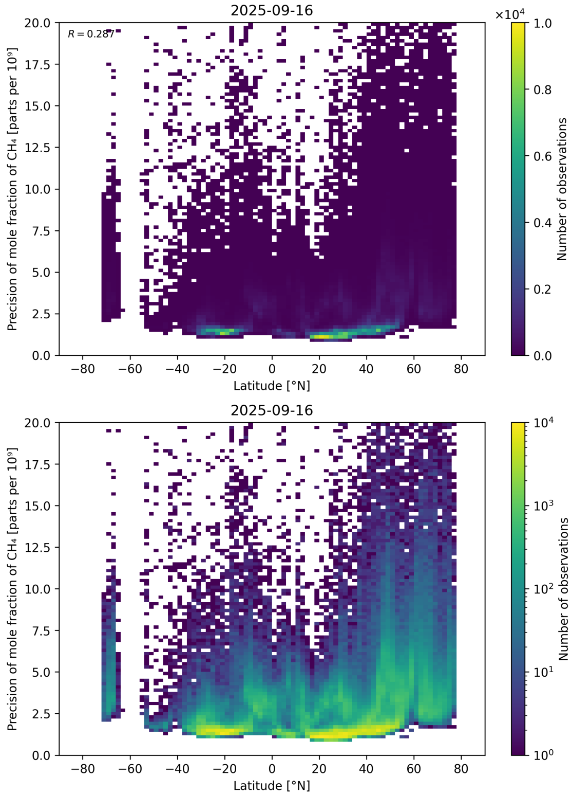
Figure 59: Scatter density plot of “Latitude” against “Precision of mole fraction of \text{CH}_4 ” for 2025-09-15 to 2025-09-17.
