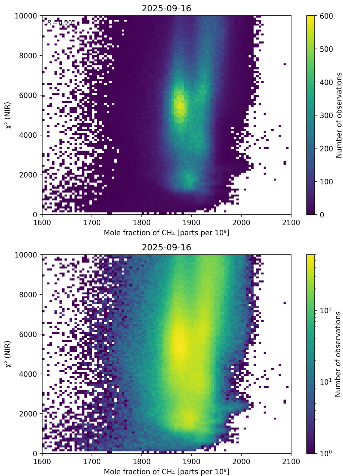
Figure 70: Scatter density plot of “Mole fraction of \text{CH}_4 ” against “ \chi^2 (NIR)” for 2025-09-15 to 2025-09-17.
