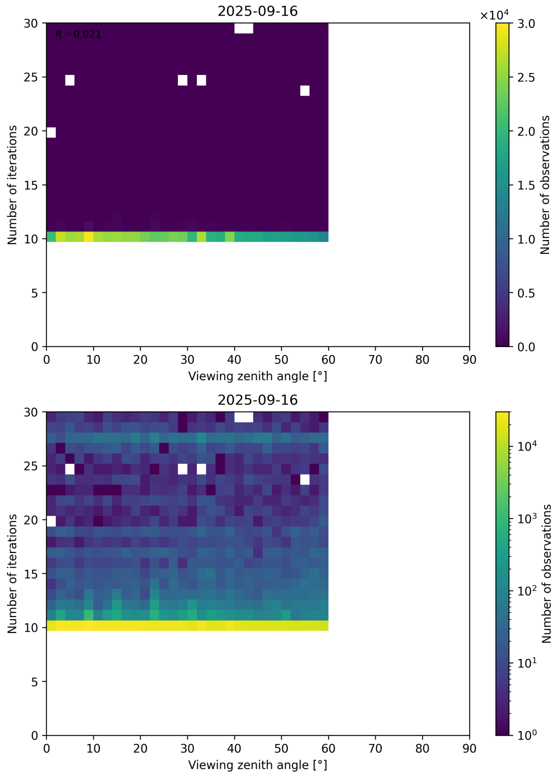
Figure 113: Scatter density plot of “Viewing zenith angle” against “Number of iterations” for 2025-09-15 to 2025-09-17.
