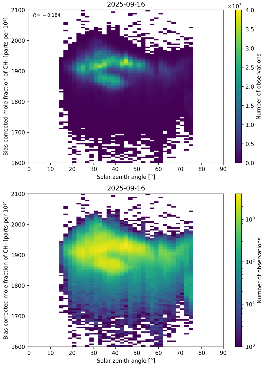
Figure 100: Scatter density plot of “Solar zenith angle” against “Bias corrected mole fraction of CH 4 ” for 2025-09-15 to 2025-09-17.
