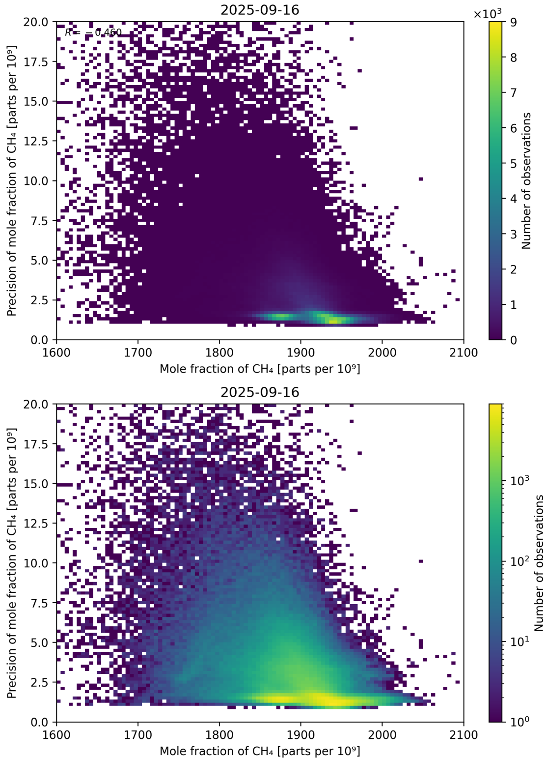
Figure 75: Scatter density plot of “Mole fraction of CH 4 ” against “Precision of mole fraction of CH 4 ” for 2025-09-15 to 2025-09-17.
