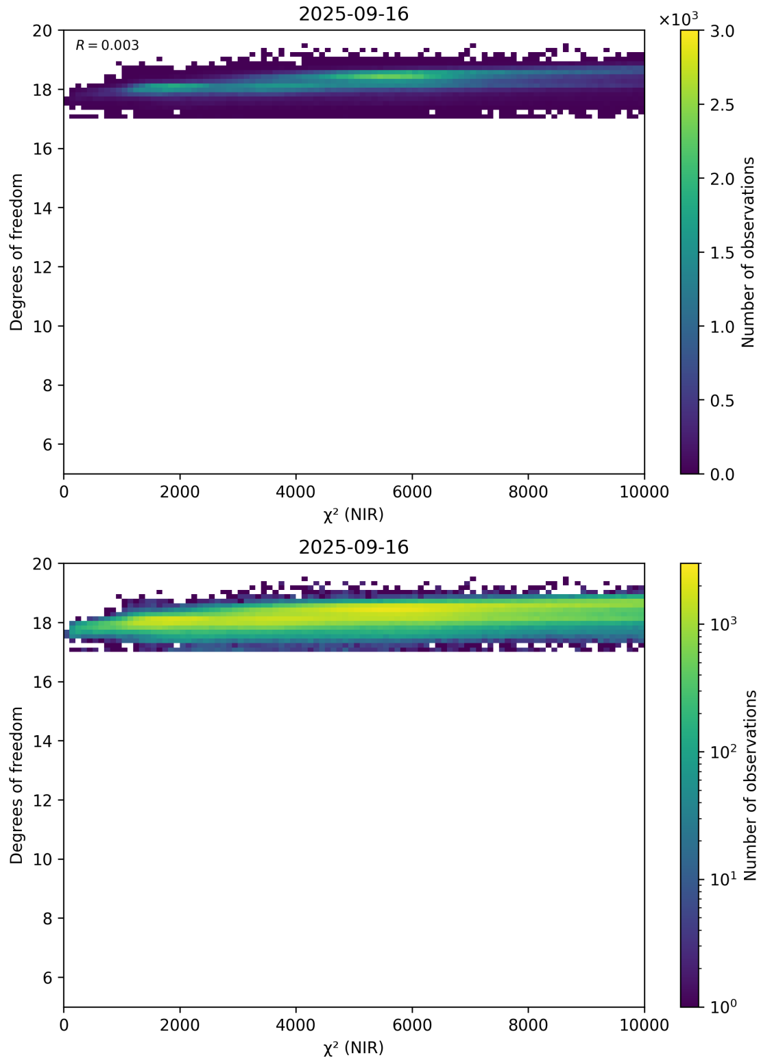
Figure 44: Scatter density plot of “ \chi^2 (NIR)” against “Degrees of freedom” for 2025-09-15 to 2025-09-17.
