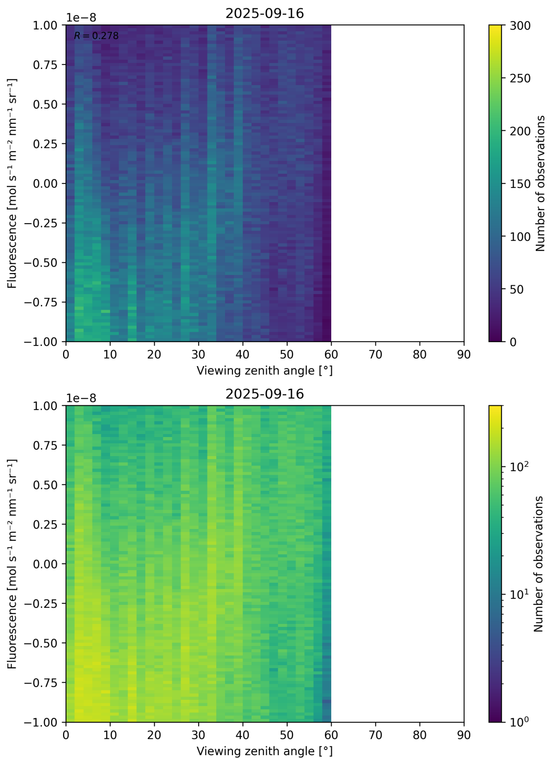
Figure 108: Scatter density plot of “Viewing zenith angle” against “Fluorescence” for 2025-09-15 to 2025-09-17.
