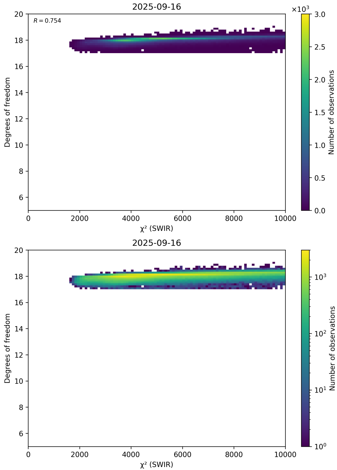
Figure 48: Scatter density plot of “ \chi^2 (SWIR)” against “Degrees of freedom” for 2025-09-15 to 2025-09-17.
