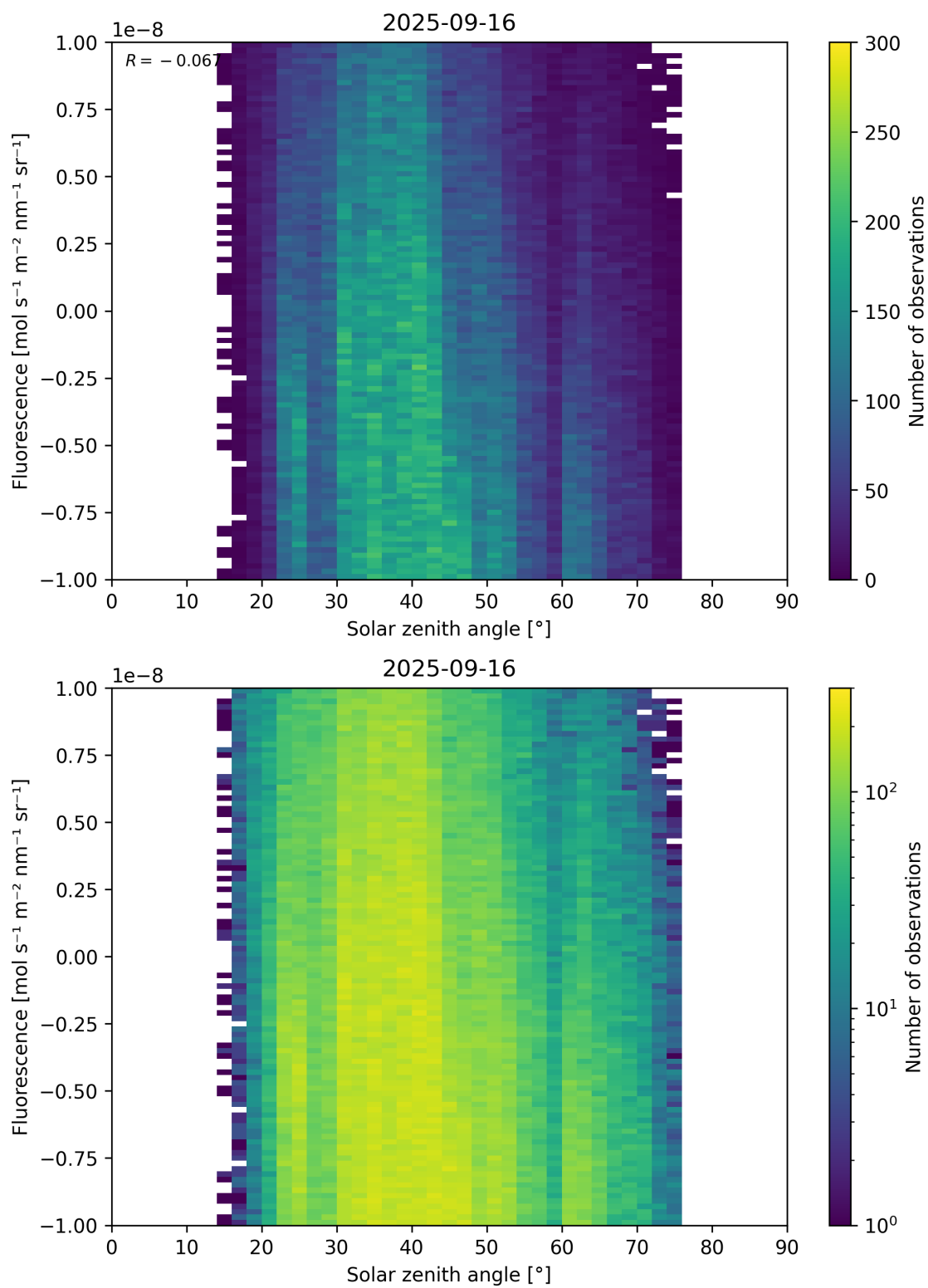
Figure 97: Scatter density plot of “Solar zenith angle” against “Fluorescence” for 2025-09-15 to 2025-09-17.
