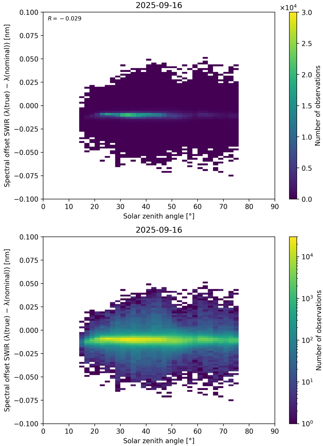
Figure 104: Scatter density plot of “Solar zenith angle” against “Spectral offset SWIR ( \lambda_{\text{true}} - \lambda_{\text{nominal}} )” for 2025-09-15 to 2025-09-17.
