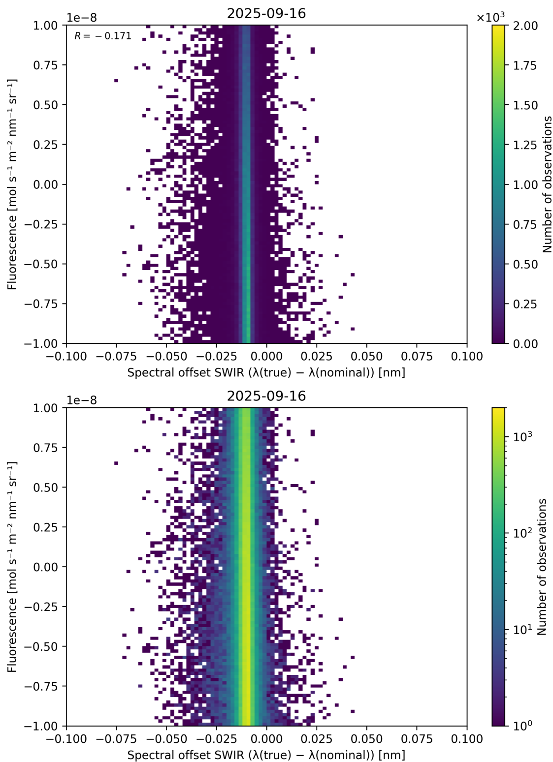
Figure 120: Scatter density plot of “Spectral offset SWIR ( \lambda_{\text{true}} - \lambda_{\text{nominal}} )” against “Fluorescence” for 2025-09-15 to 2025-09-17.
