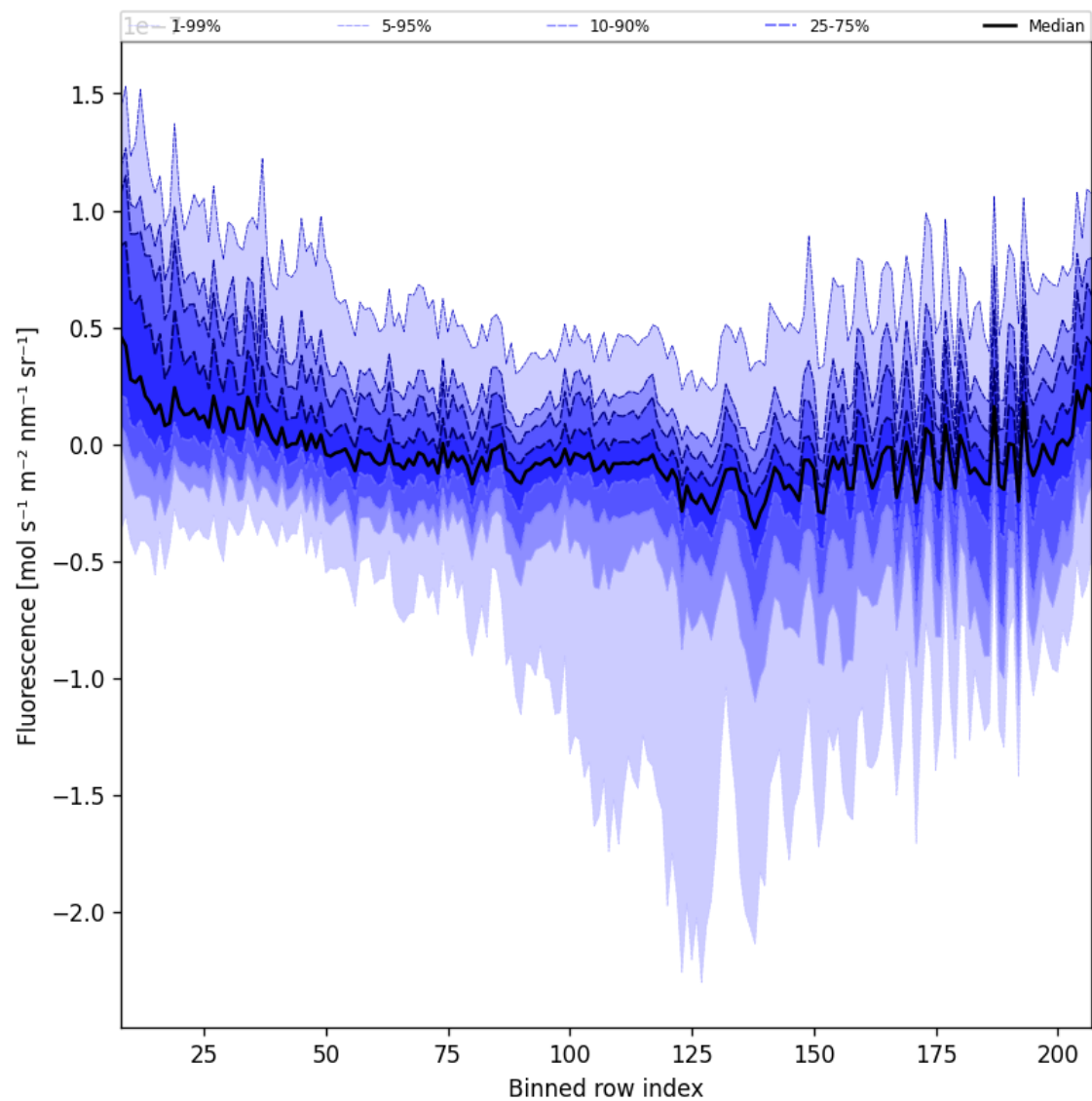
Figure 43: Along track statistics of “Fluorescence” for 2025-09-15 to 2025-09-17
