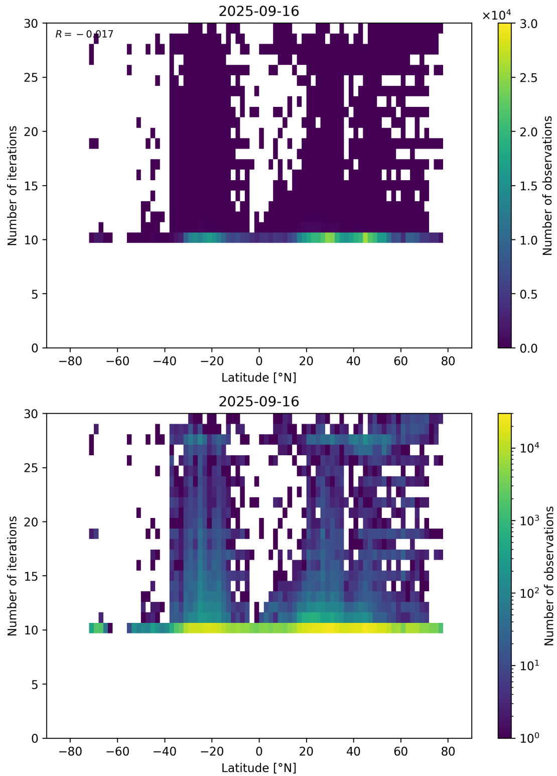
Figure 60: Scatter density plot of “Latitude” against “Number of iterations” for 2025-09-15 to 2025-09-17.
