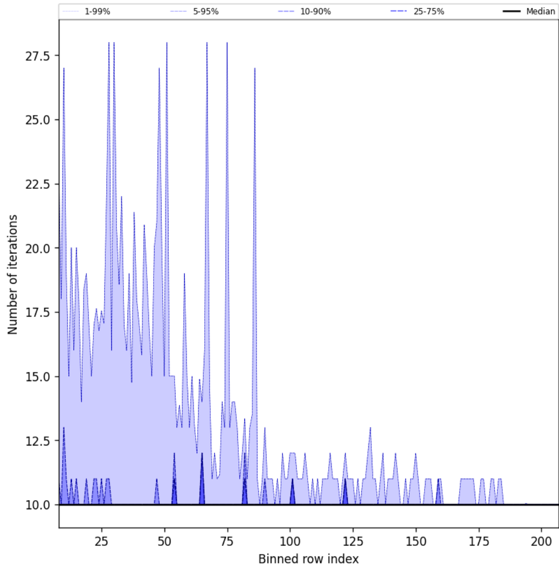
Figure 42: Along track statistics of “Number of iterations” for 2025-09-15 to 2025-09-17
