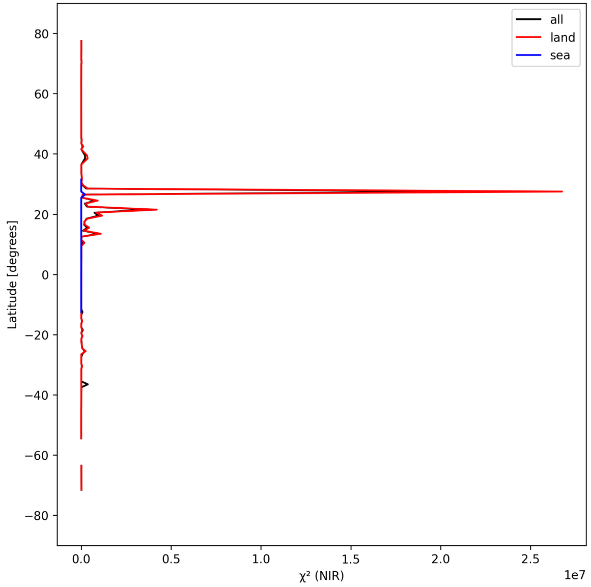
Figure 18: Zonal average of “ \chi^2 (NIR)” for 2025-09-15 to 2025-09-17.
