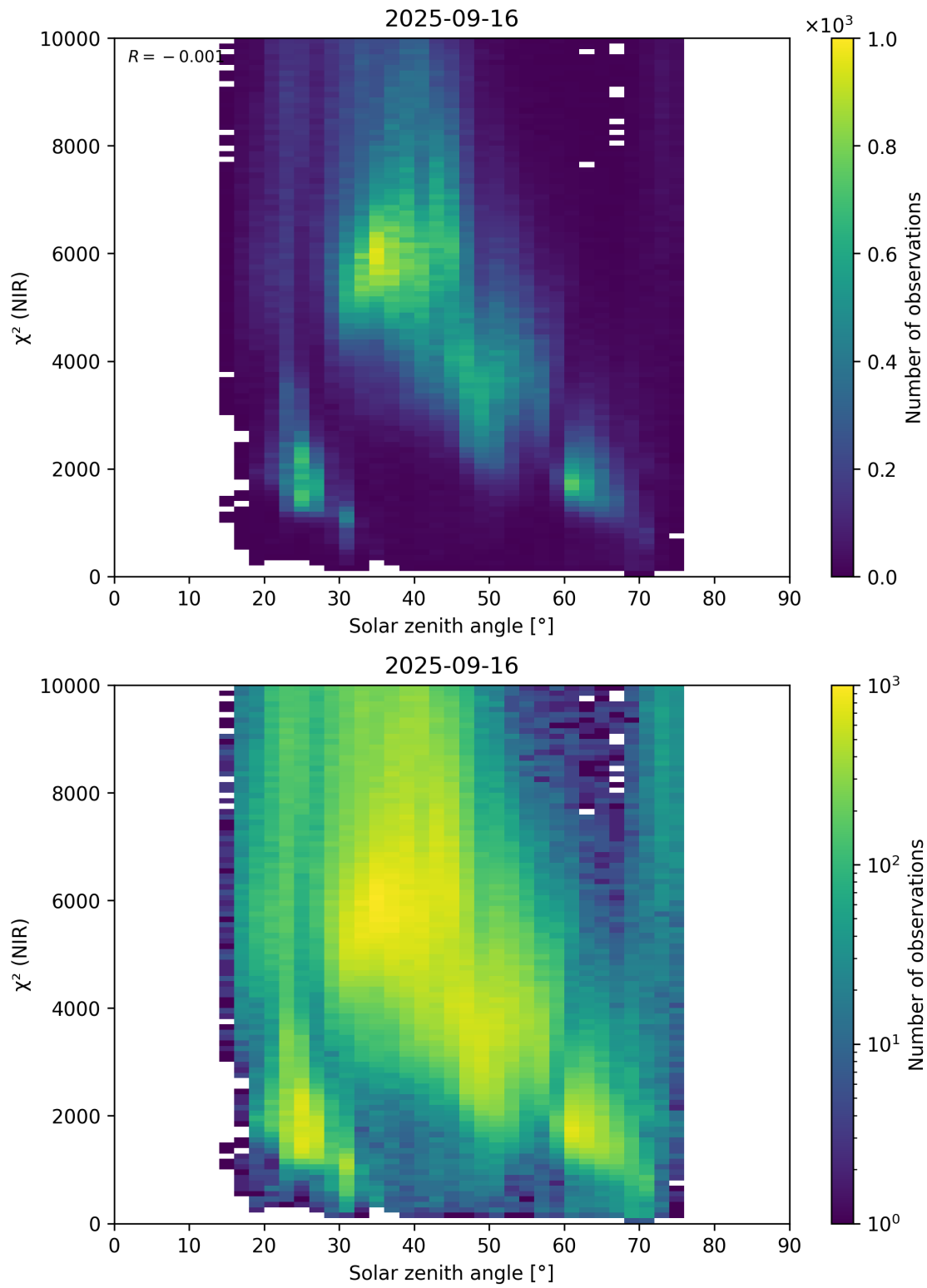
Figure 94: Scatter density plot of “Solar zenith angle” against “ \chi^2 (NIR)” for 2025-09-15 to 2025-09-17.
