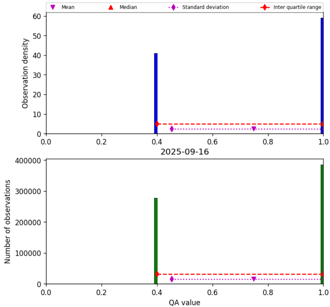
Figure 22: Histogram of “QA value” for 2025-09-15 to 2025-09-17
