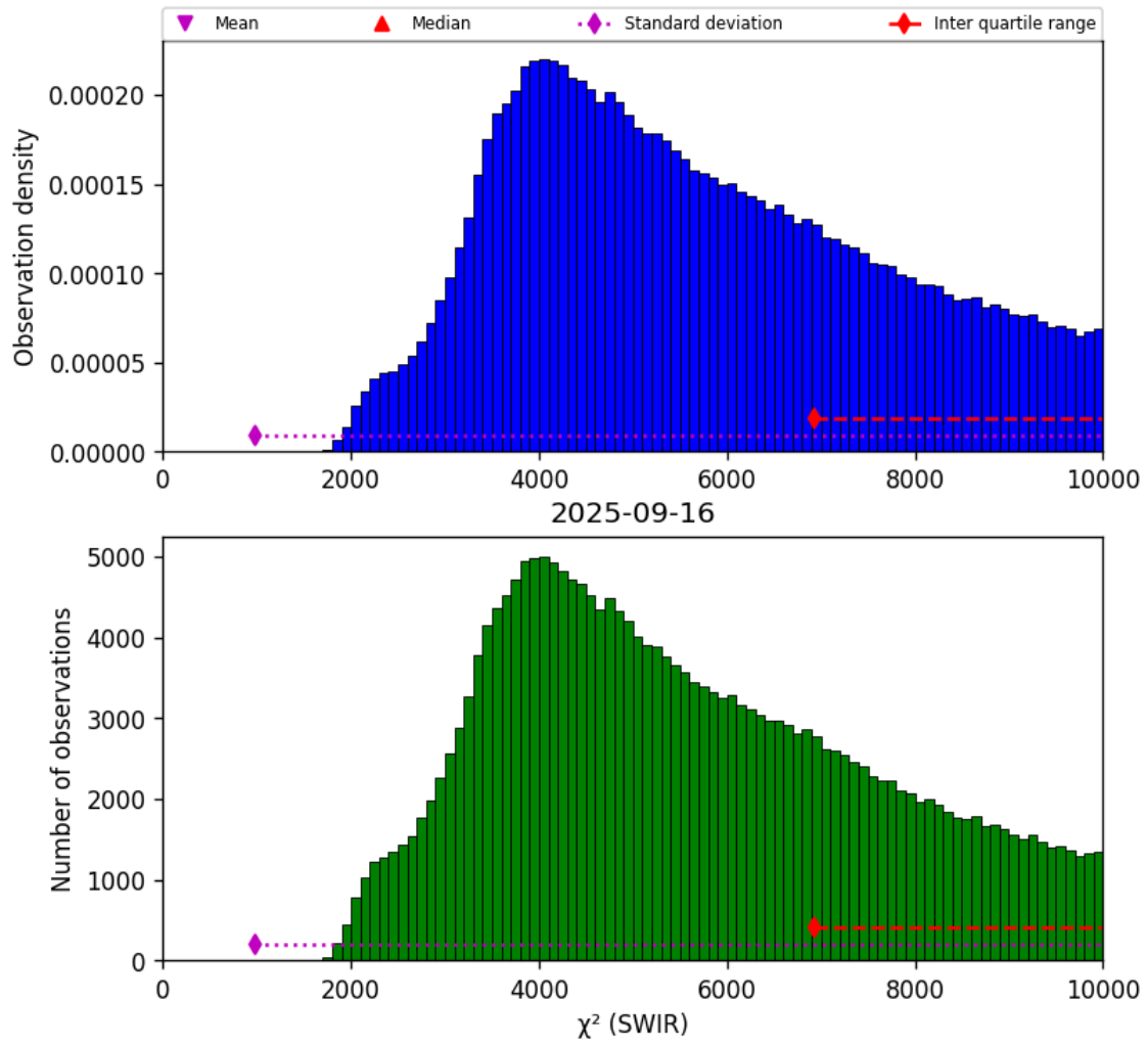
Figure 28: Histogram of “ \chi^2 (SWIR)” for 2025-09-15 to 2025-09-17
