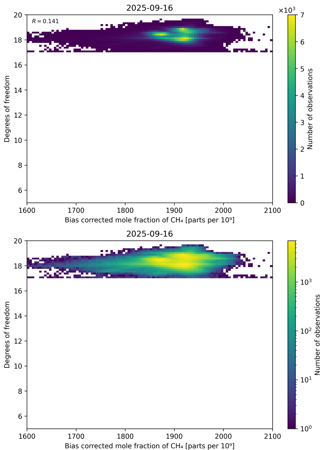
Figure 65: Scatter density plot of “Bias corrected mole fraction of CH 4 ” against “Degrees of freedom” for 2025-09-15 to 2025-09-17.
