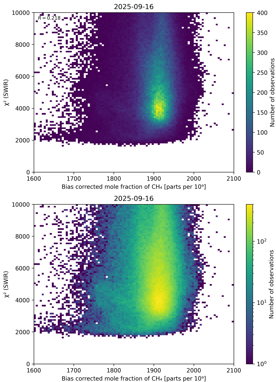
Figure 64: Scatter density plot of “Bias corrected mole fraction of CH 4 ” against “ \chi^2 (SWIR)” for 2025-09-15 to 2025-09-17.
