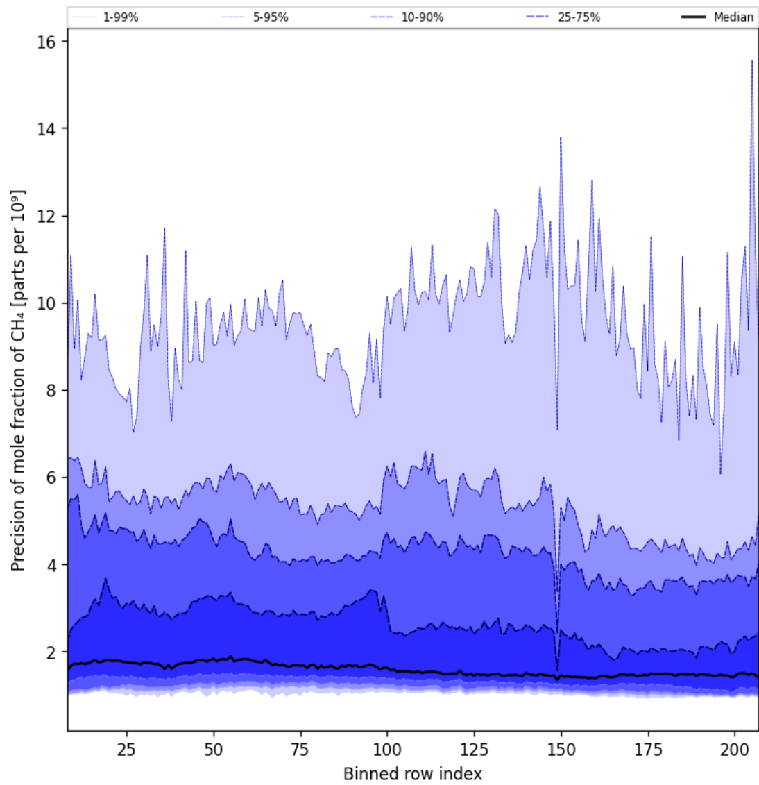
Figure 35: Along track statistics of “Precision of mole fraction of CH 4 ” for 2025-09-15 to 2025-09-17
