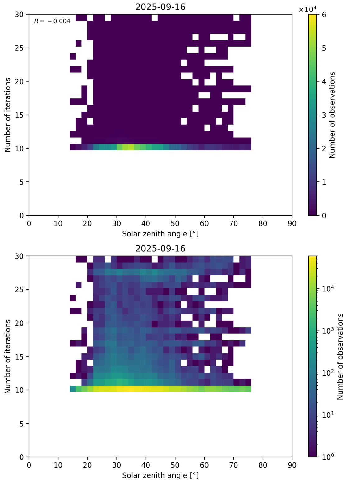
Figure 102: Scatter density plot of “Solar zenith angle” against “Number of iterations” for 2025-09-15 to 2025-09-17.
