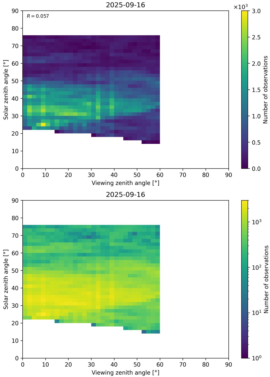
Figure 115: Scatter density plot of “Viewing zenith angle” against “Solar zenith angle” for 2025-09-15 to 2025-09-17.
