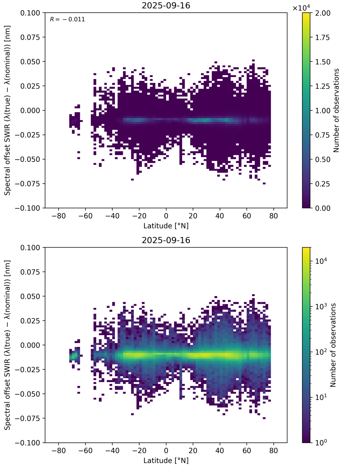
Figure 62: Scatter density plot of “Latitude” against “Spectral offset SWIR ( \lambda_{\text{true}} - \lambda_{\text{nominal}} )” for 2025-09-15 to 2025-09-17.
