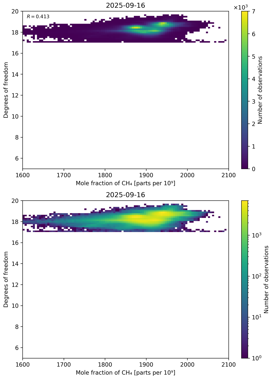
Figure 72: Scatter density plot of “Mole fraction of CH 4 ” against “Degrees of freedom” for 2025-09-15 to 2025-09-17.
