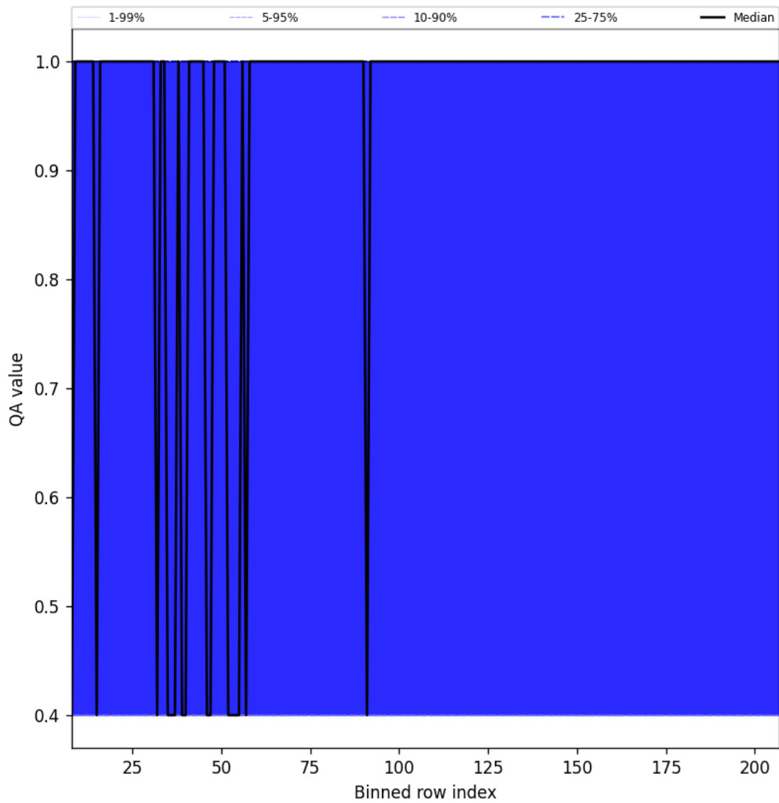
Figure 33: Along track statistics of “QA value” for 2025-09-15 to 2025-09-17
