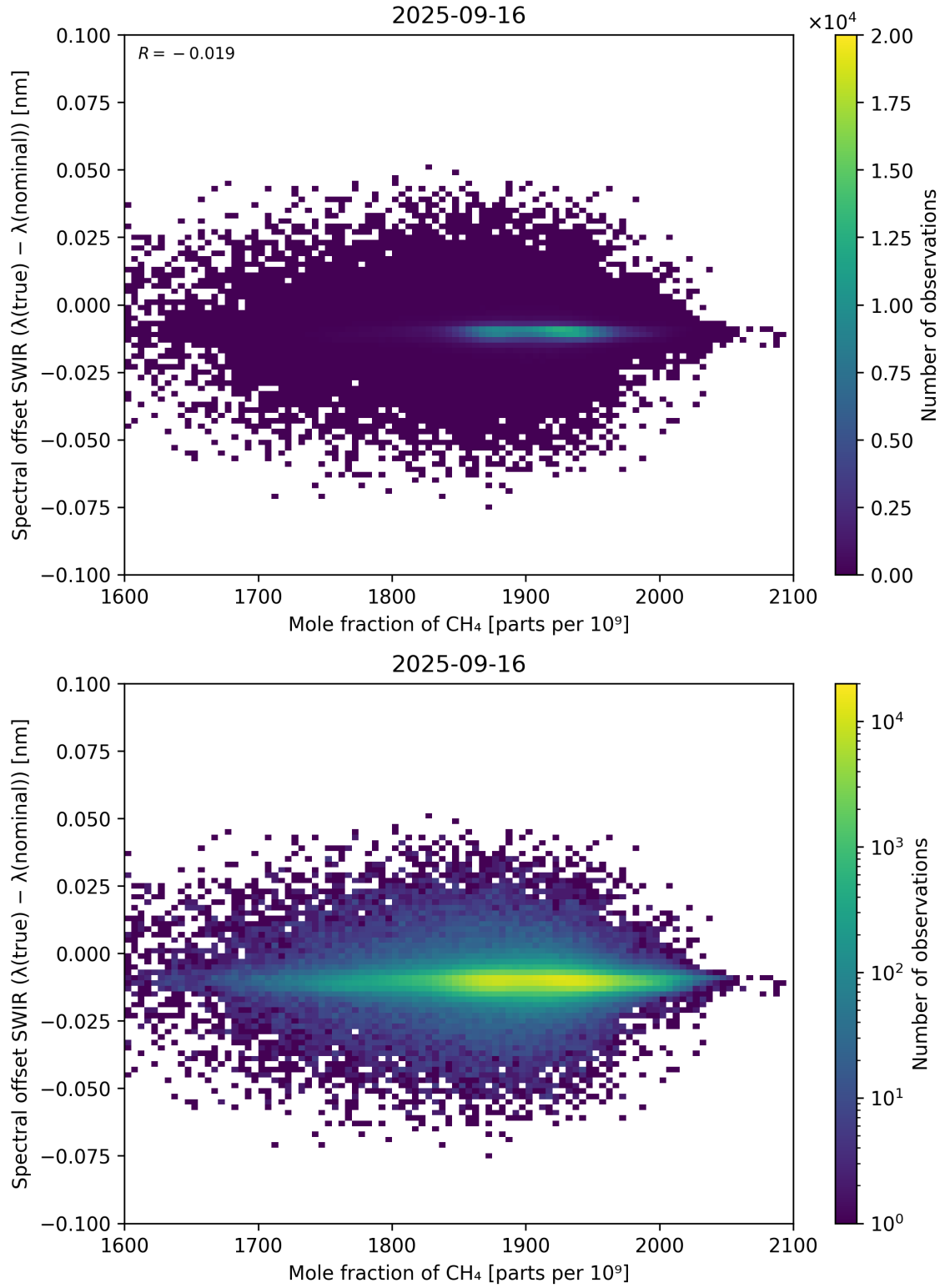
Figure 86: Scatter density plot of “Mole fraction of CH 4 ” against “Spectral offset SWIR ( \lambda_{\text{true}} - \lambda_{\text{nominal}} )” for 2025-09-15 to 2025-09-17.
