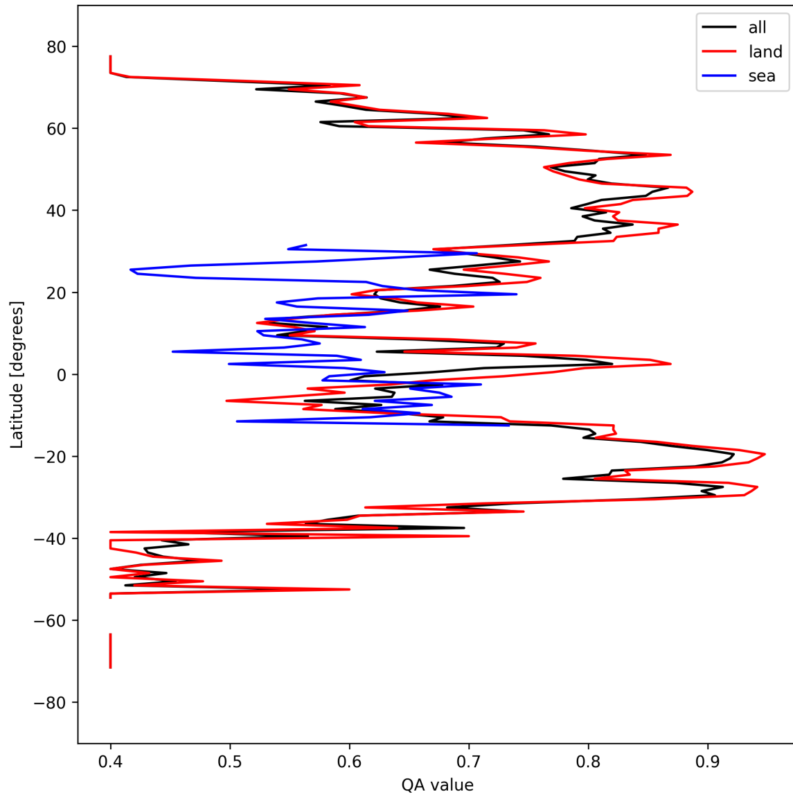
Figure 11: Zonal average of “QA value” for 2025-09-15 to 2025-09-17.
