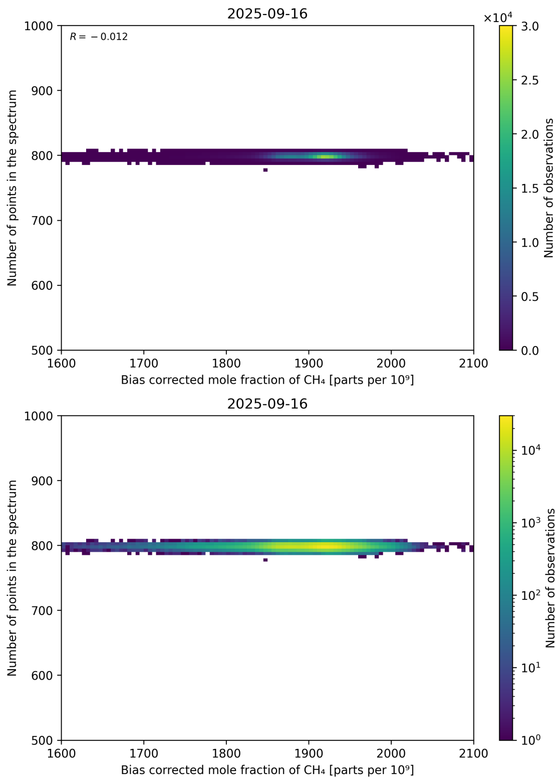
Figure 68: Scatter density plot of “Bias corrected mole fraction of CH 4 ” against “Number of points in the spectrum” for 2025-09-15 to 2025-09-17.
