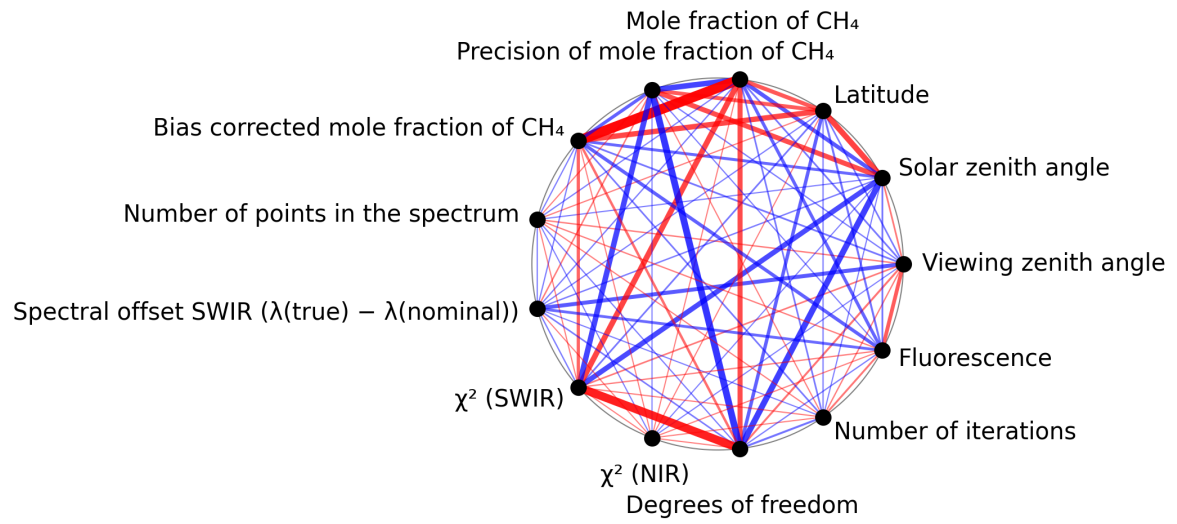
Figure 1: Map of correlation graph for 2025-09-15 to 2025-09-17.
