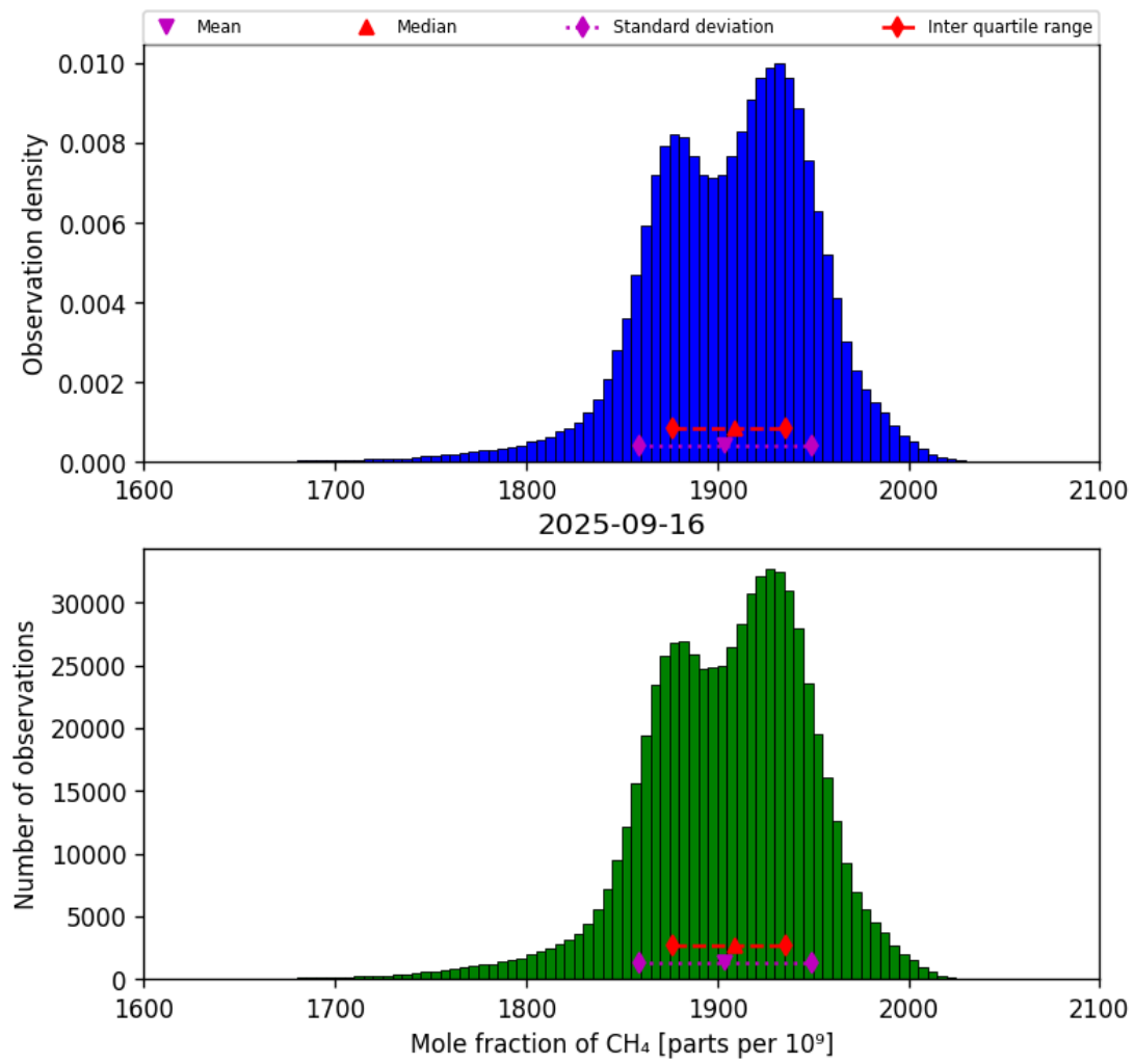
Figure 23: Histogram of “Mole fraction of CH 4 ” for 2025-09-15 to 2025-09-17
