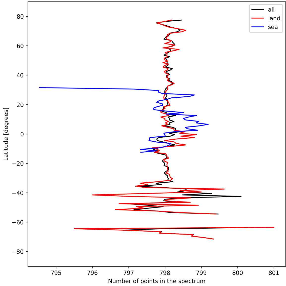
Figure 15: Zonal average of “Number of points in the spectrum” for 2025-09-15 to 2025-09-17.
