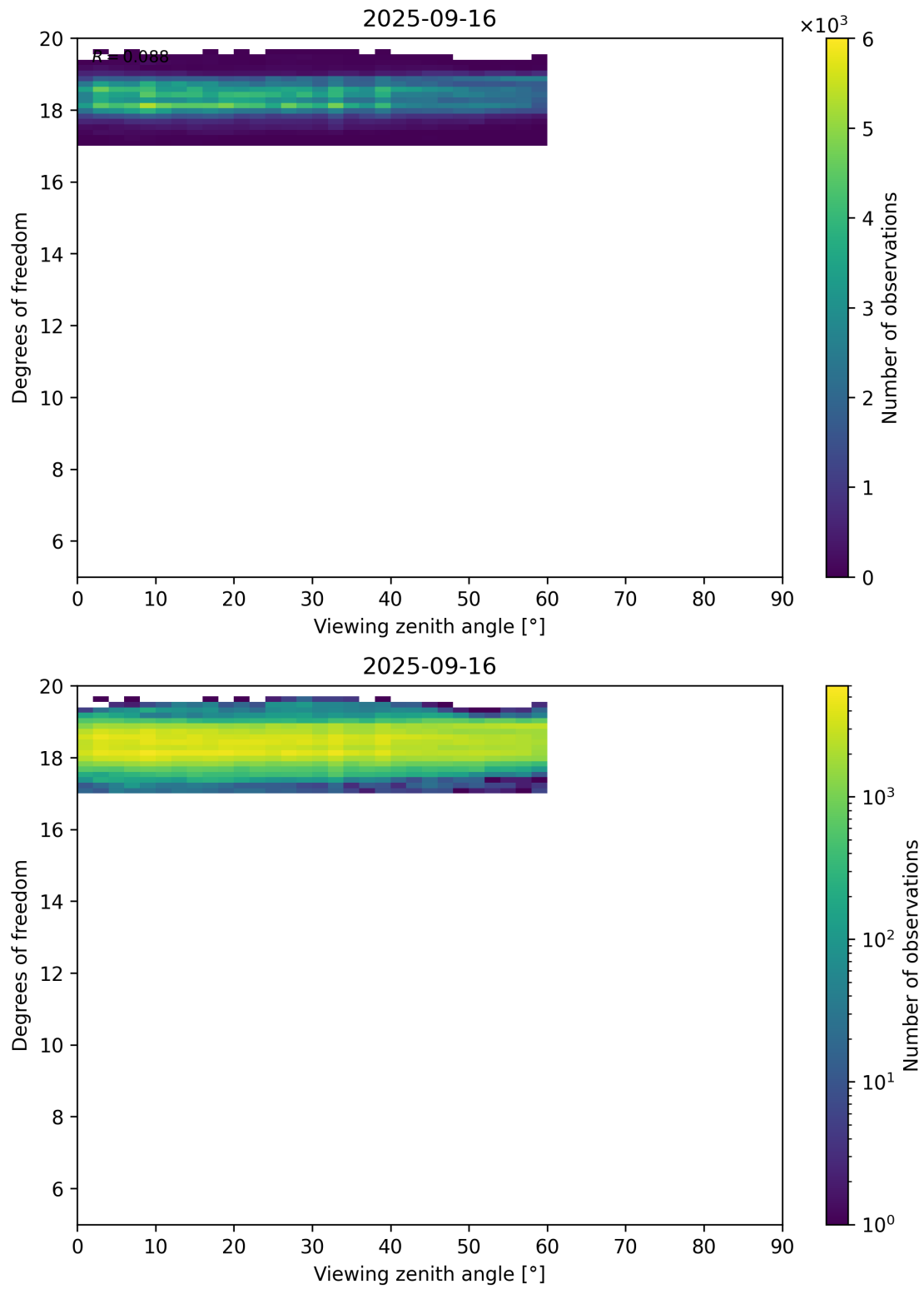
Figure 107: Scatter density plot of “Viewing zenith angle” against “Degrees of freedom” for 2025-09-15 to 2025-09-17.
