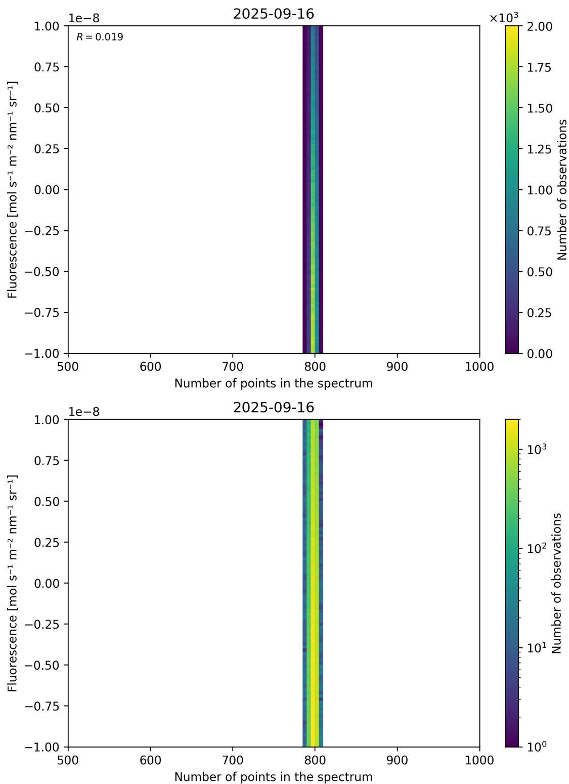
Figure 91: Scatter density plot of “Number of points in the spectrum” against “Fluorescence” for 2025-09-15 to 2025-09-17.
