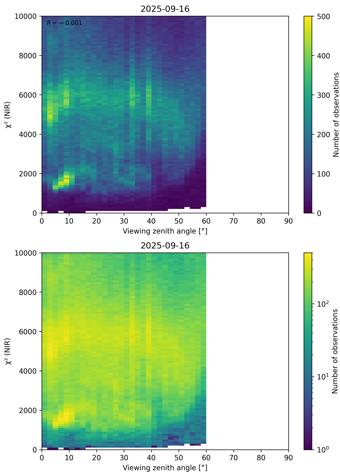
Figure 105: Scatter density plot of “Viewing zenith angle” against “ \chi^2 (NIR)” for 2025-09-15 to 2025-09-17.
