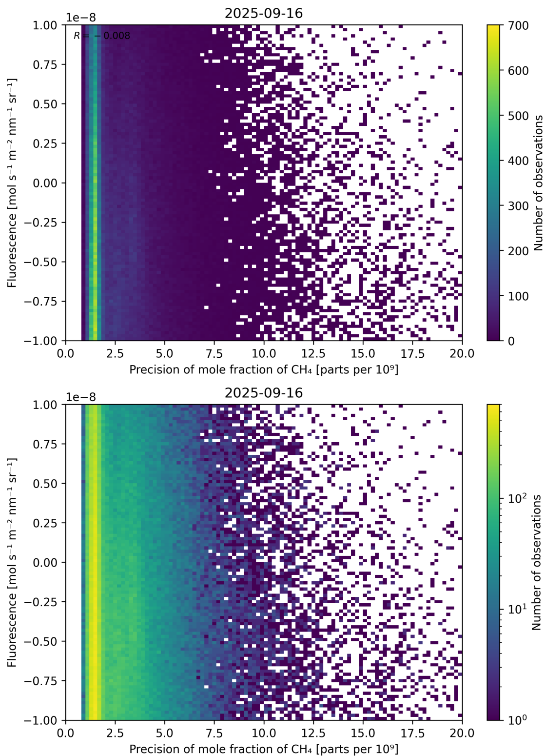
Figure 81: Scatter density plot of “Precision of mole fraction of \text{CH}_4 ” against “Fluorescence” for 2025-09-15 to 2025-09-17.
