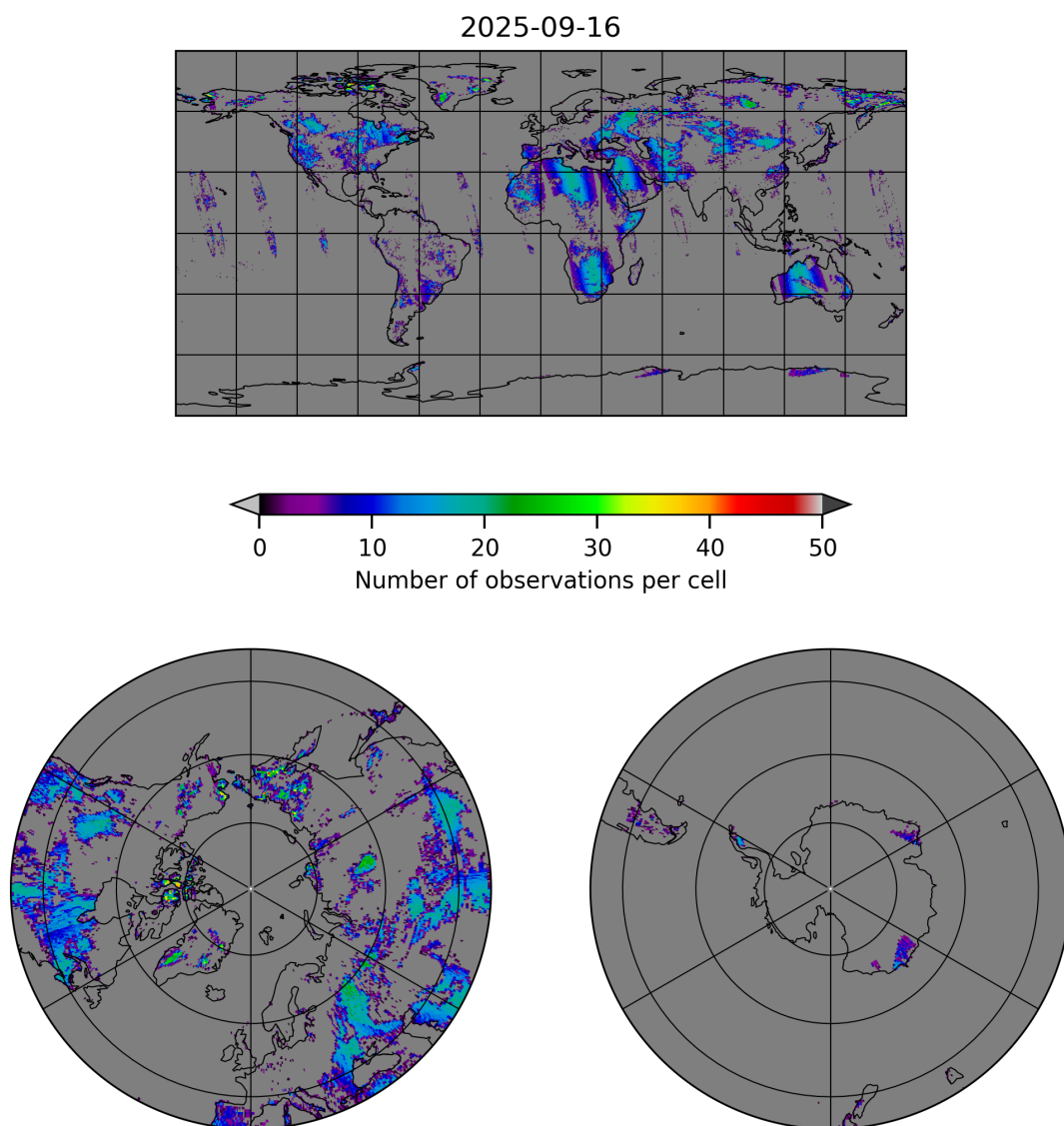
Figure 10: Map of the number of observations for 2025-09-15 to 2025-09-17
