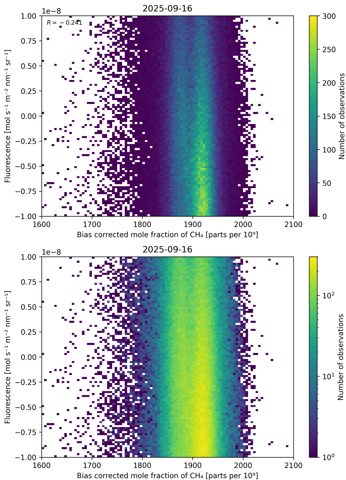
Figure 66: Scatter density plot of “Bias corrected mole fraction of \text{CH}_4 ” against “Fluorescence” for 2025-09-15 to 2025-09-17.
