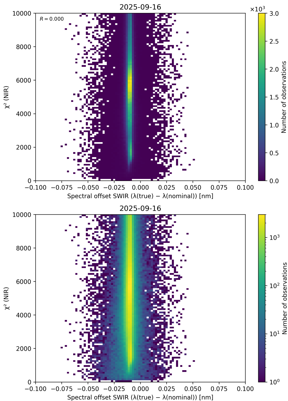
Figure 117: Scatter density plot of “Spectral offset SWIR ( \lambda_{\text{true}} - \lambda_{\text{nominal}} )” against “ \chi^2 (NIR)” for 2025-09-15 to 2025-09-17.
