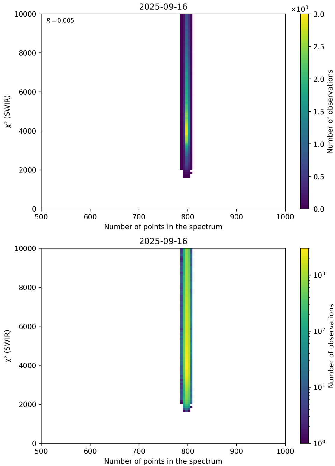
Figure 89: Scatter density plot of “Number of points in the spectrum” against “ \chi^2 (SWIR)” for 2025-09-15 to 2025-09-17.
