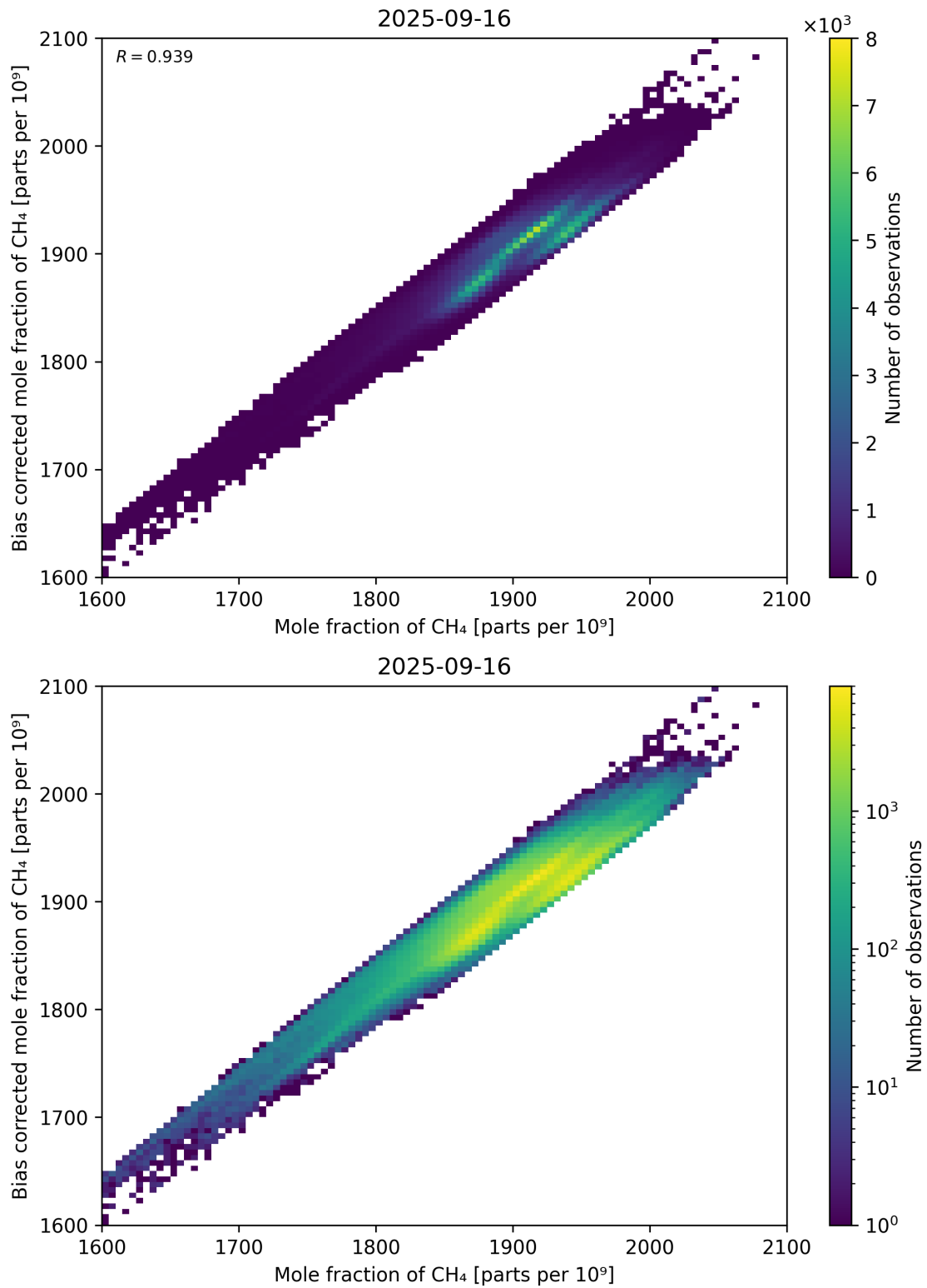
Figure 74: Scatter density plot of “Mole fraction of CH 4 ” against “Bias corrected mole fraction of CH 4 ” for 2025-09-15 to 2025-09-17.
