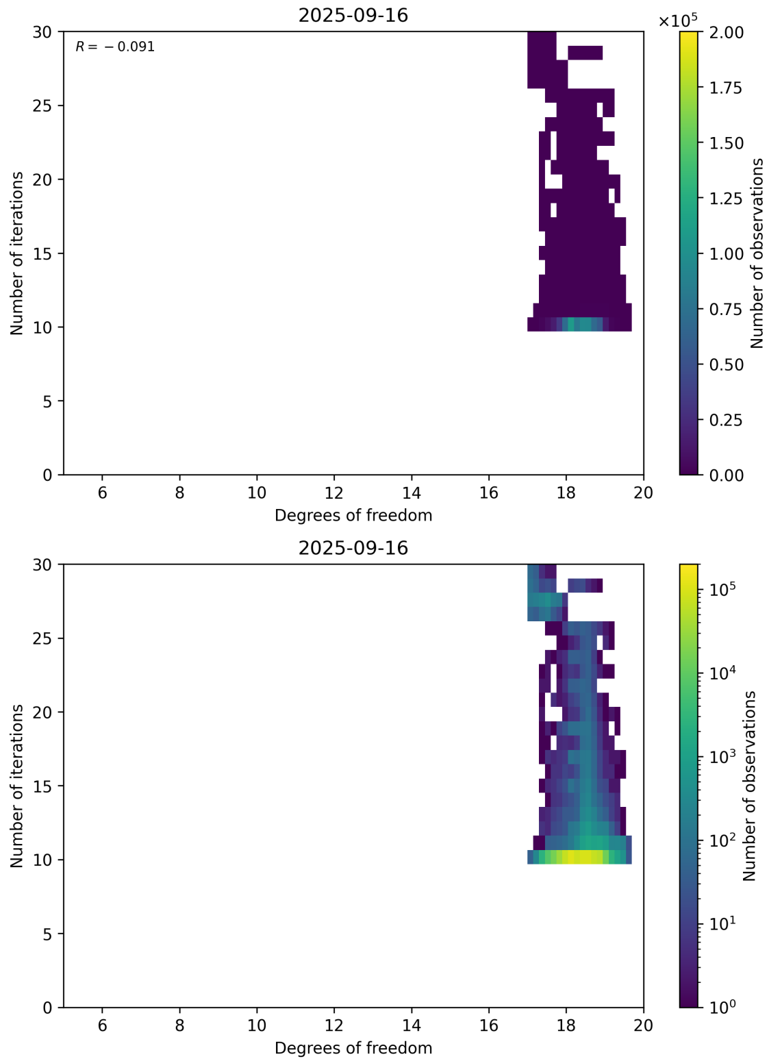
Figure 52: Scatter density plot of “Degrees of freedom” against “Number of iterations” for 2025-09-15 to 2025-09-17.
