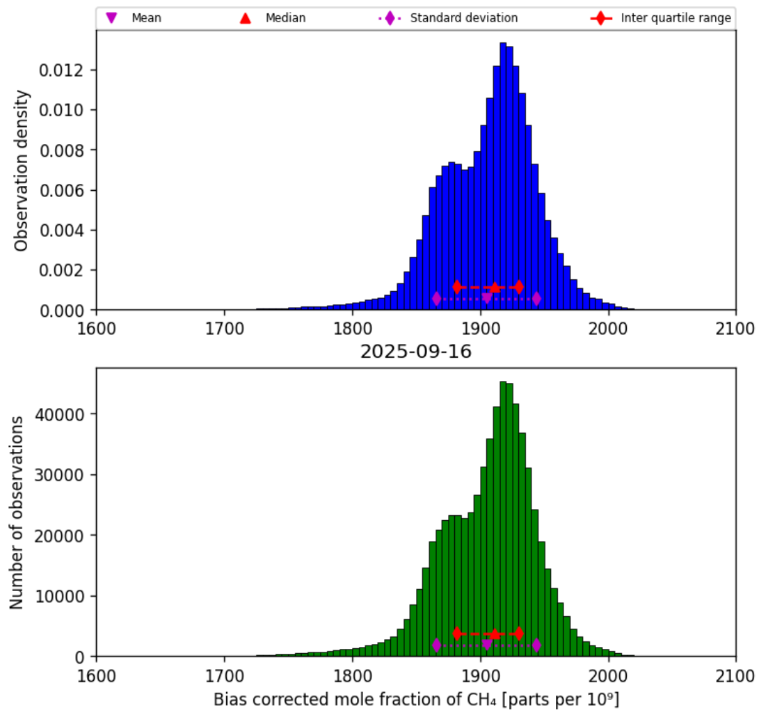
Figure 25: Histogram of “Bias corrected mole fraction of CH 4 ” for 2025-09-15 to 2025-09-17
