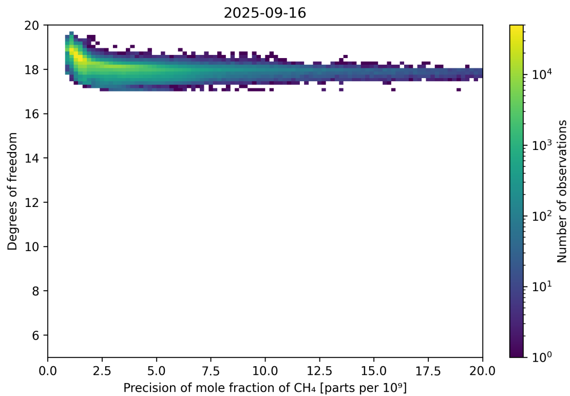
Figure 80: Scatter density plot of “Precision of mole fraction of CH 4 ” against “Degrees of freedom” for 2025-09-15 to 2025-09-17.
