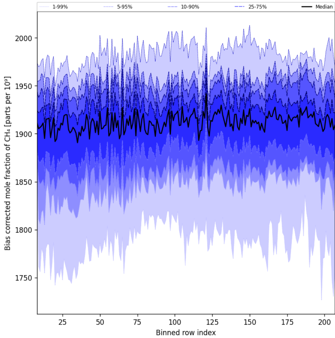
Figure 36: Along track statistics of “Bias corrected mole fraction of CH 4 ” for 2025-09-15 to 2025-09-17
