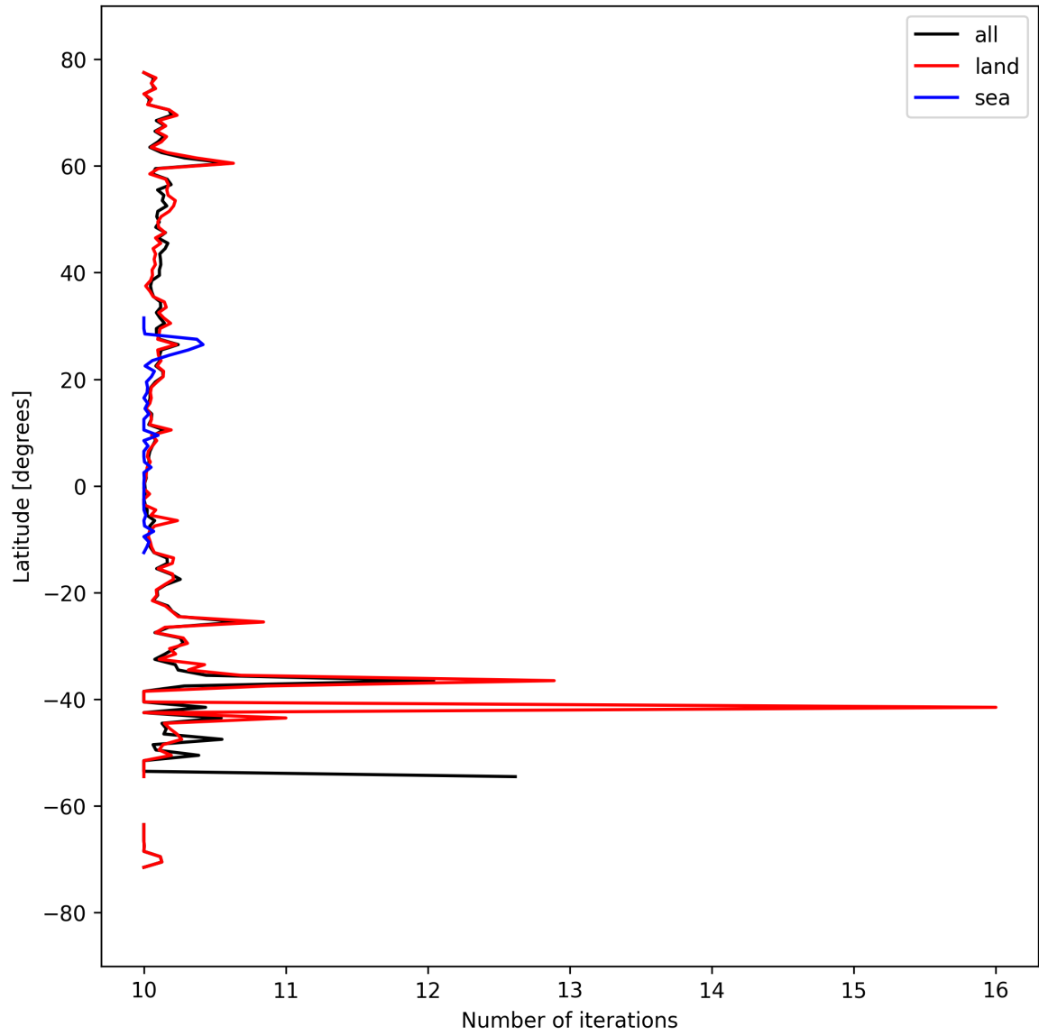
Figure 20: Zonal average of “Number of iterations” for 2025-09-15 to 2025-09-17.
