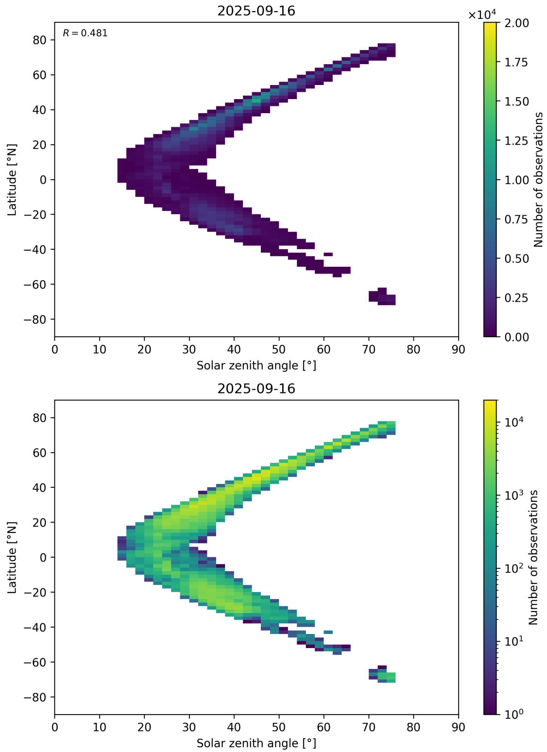
Figure 98: Scatter density plot of “Solar zenith angle” against “Latitude” for 2025-09-15 to 2025-09-17.
