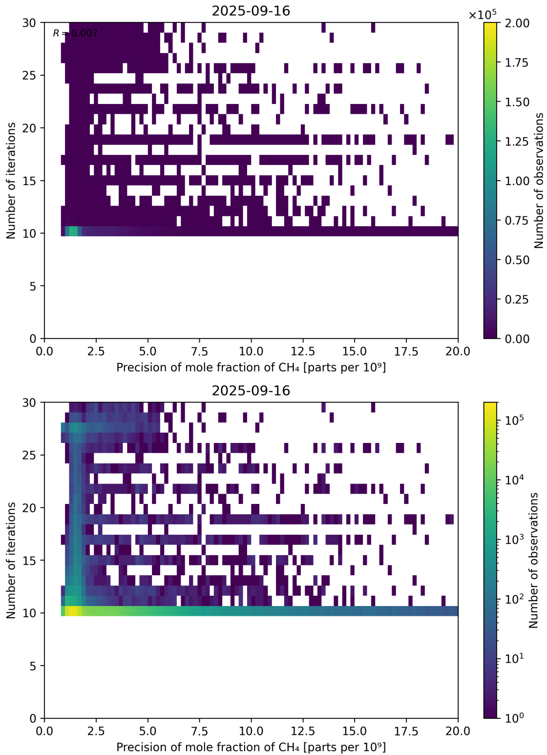
Figure 83: Scatter density plot of “Precision of mole fraction of CH 4 ” against “Number of iterations” for 2025-09-15 to 2025-09-17.
