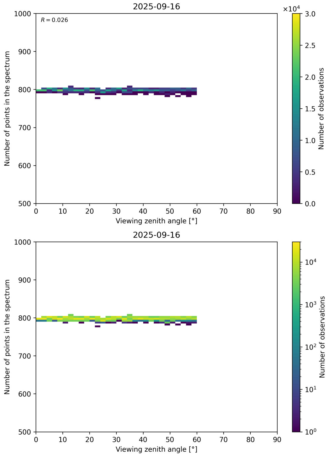
Figure 114: Scatter density plot of “Viewing zenith angle” against “Number of points in the spectrum” for 2025-09-15 to 2025-09-17.
