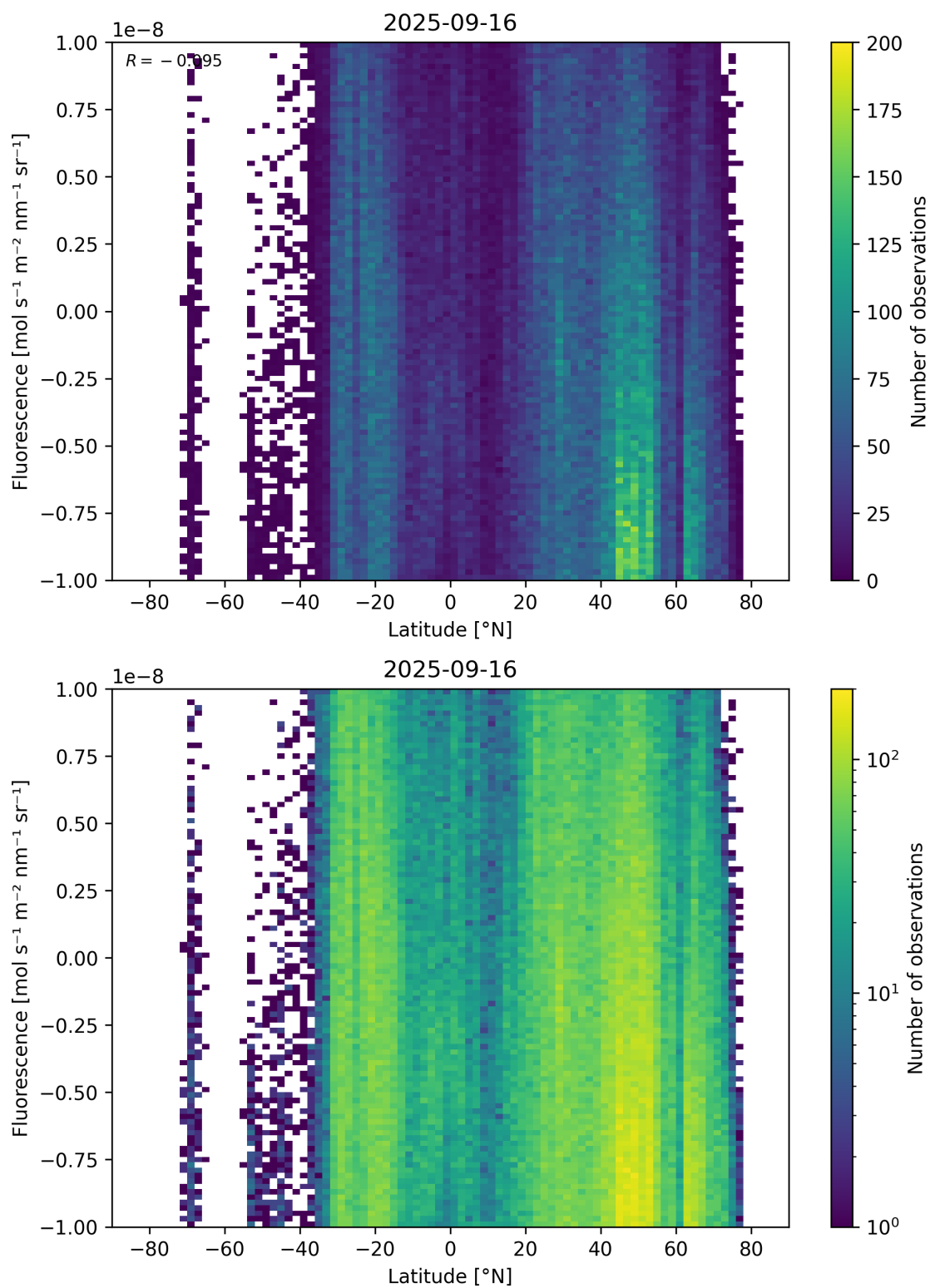
Figure 56: Scatter density plot of “Latitude” against “Fluorescence” for 2025-09-15 to 2025-09-17.
