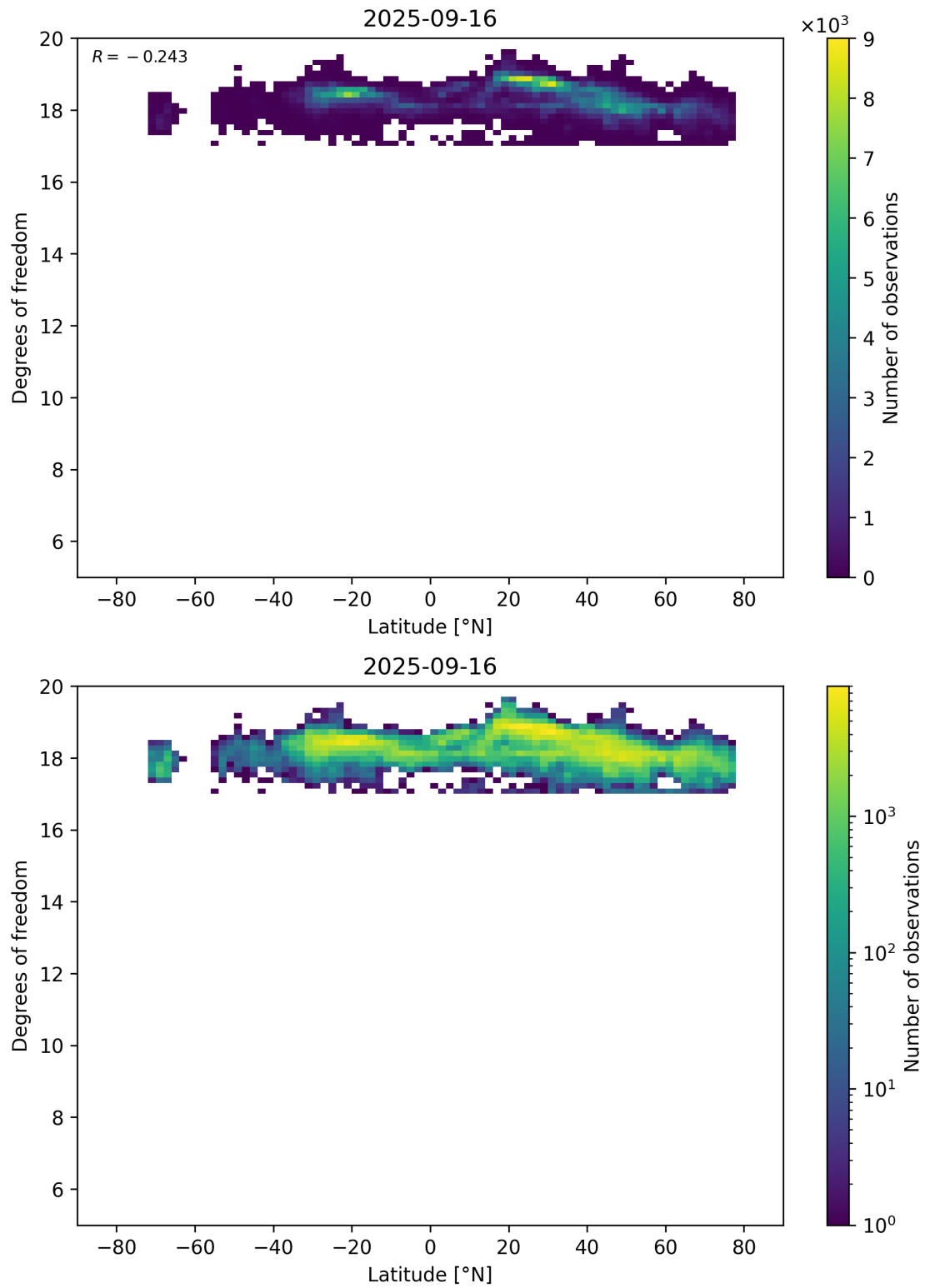
Figure 55: Scatter density plot of “Latitude” against “Degrees of freedom” for 2025-09-15 to 2025-09-17.
