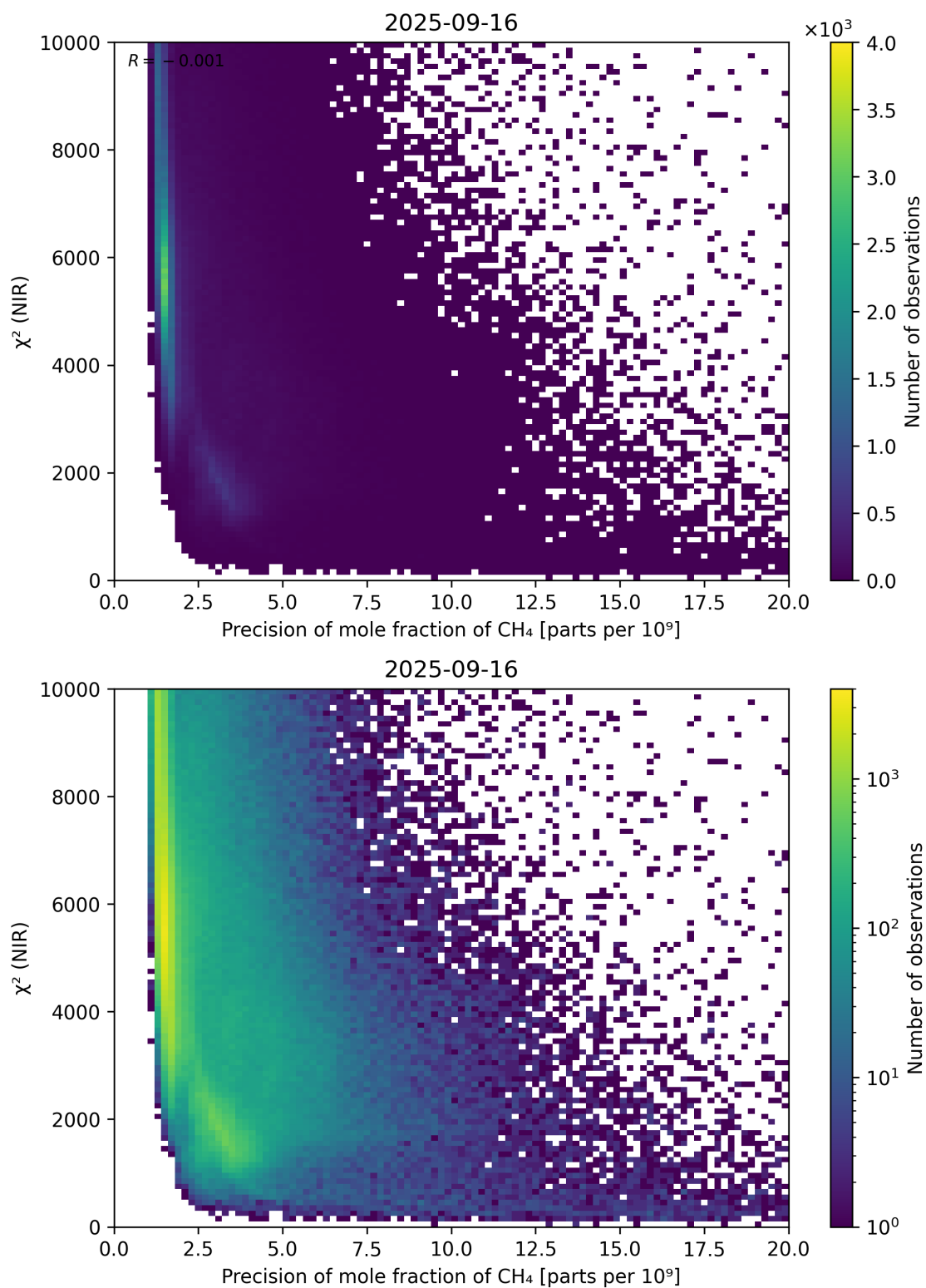
Figure 78: Scatter density plot of “Precision of mole fraction of CH 4 ” against “ \chi^2 (NIR)” for 2025-09-15 to 2025-09-17.
