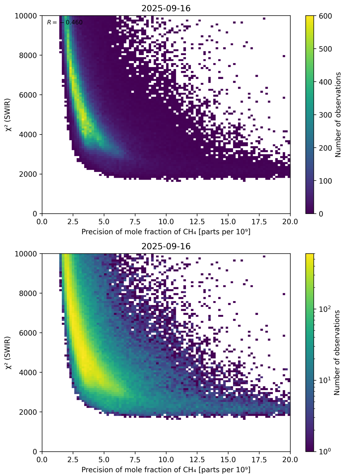
Figure 79: Scatter density plot of “Precision of mole fraction of CH 4 ” against “ \chi^2 (SWIR)” for 2025-09-15 to 2025-09-17.
