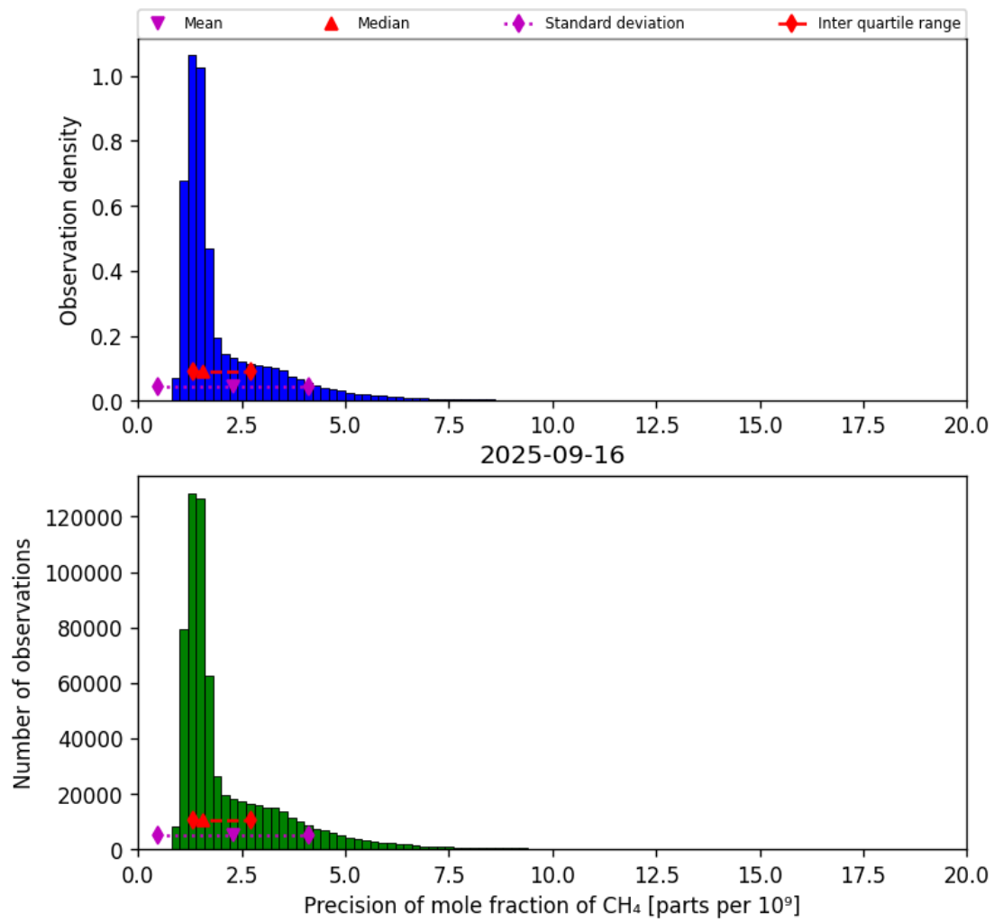
Figure 24: Histogram of “Precision of mole fraction of CH 4 ” for 2025-09-15 to 2025-09-17
