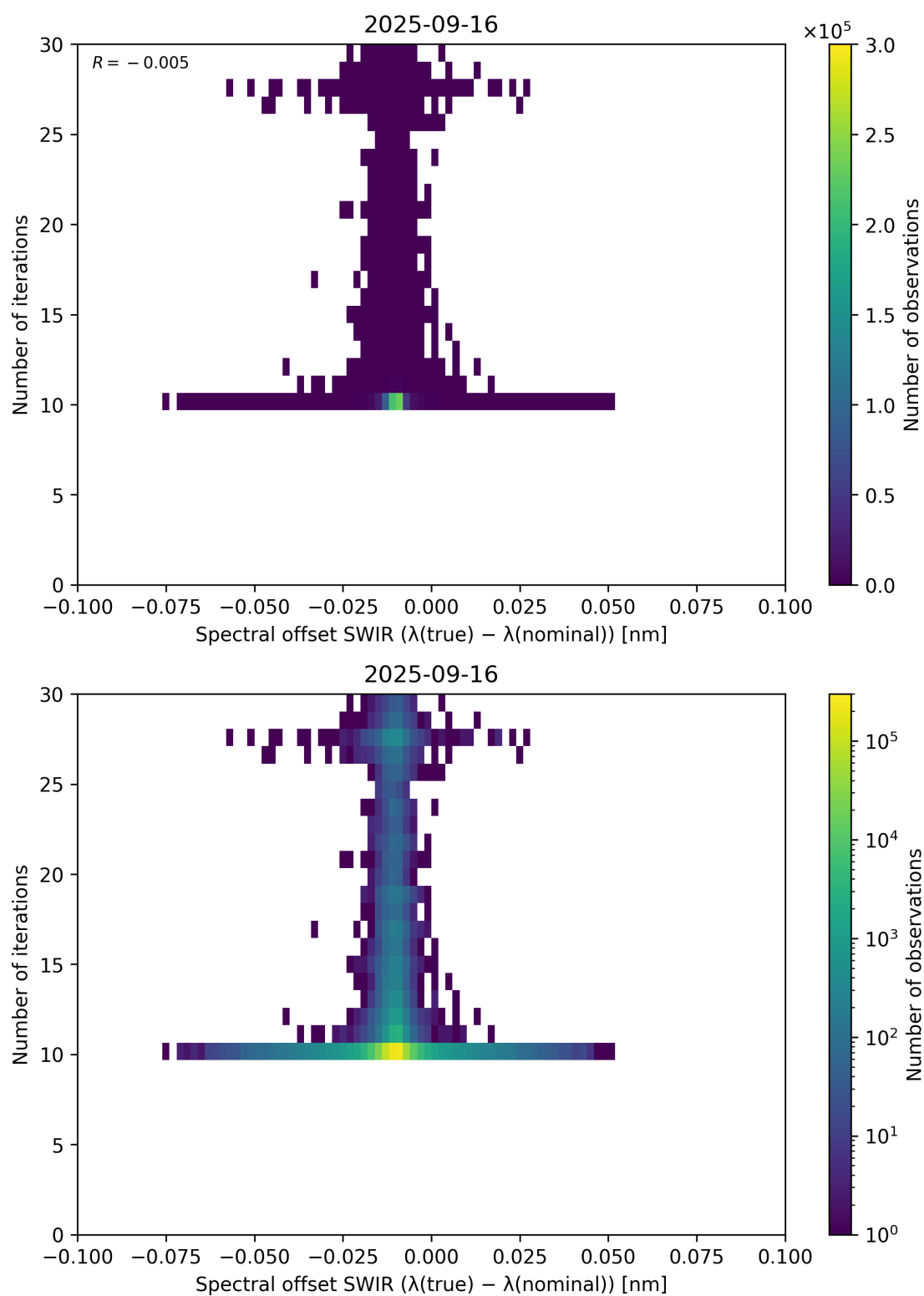
Figure 121: Scatter density plot of “Spectral offset SWIR ( \lambda_{\text{true}} - \lambda_{\text{nominal}} )” against “Number of iterations” for 2025-09-15 to 2025-09-17.
