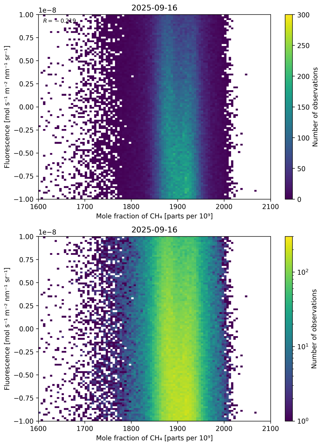
Figure 73: Scatter density plot of “Mole fraction of \text{CH}_4 ” against “Fluorescence” for 2025-09-15 to 2025-09-17.
