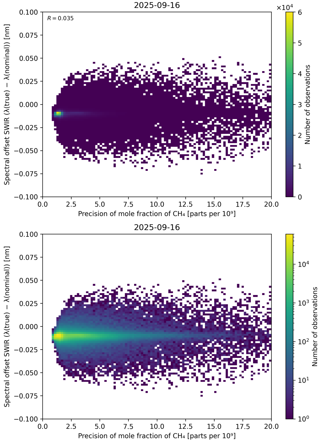
Figure 85: Scatter density plot of “Precision of mole fraction of CH 4 ” against “Spectral offset SWIR ( \lambda_{\text{true}} - \lambda_{\text{nominal}} )” for 2025-09-15 to 2025-09-17.
