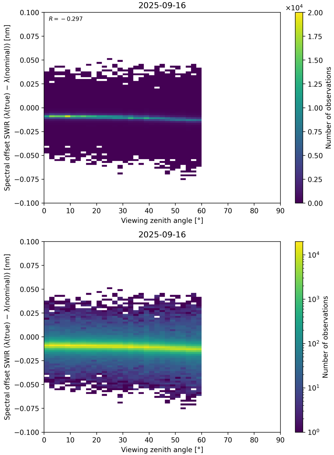
Figure 116: Scatter density plot of “Viewing zenith angle” against “Spectral offset SWIR ( \lambda_{\text{true}} - \lambda_{\text{nominal}} )” for 2025-09-15 to 2025-09-17.
