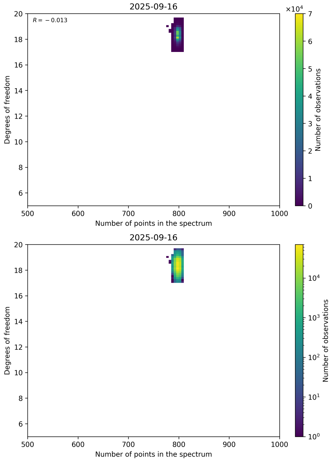
Figure 90: Scatter density plot of “Number of points in the spectrum” against “Degrees of freedom” for 2025-09-15 to 2025-09-17.
