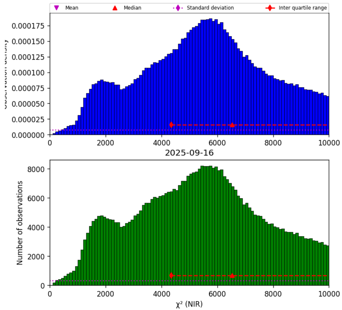
Figure 29: Histogram of “ \chi^2 (NIR)” for 2025-09-15 to 2025-09-17
