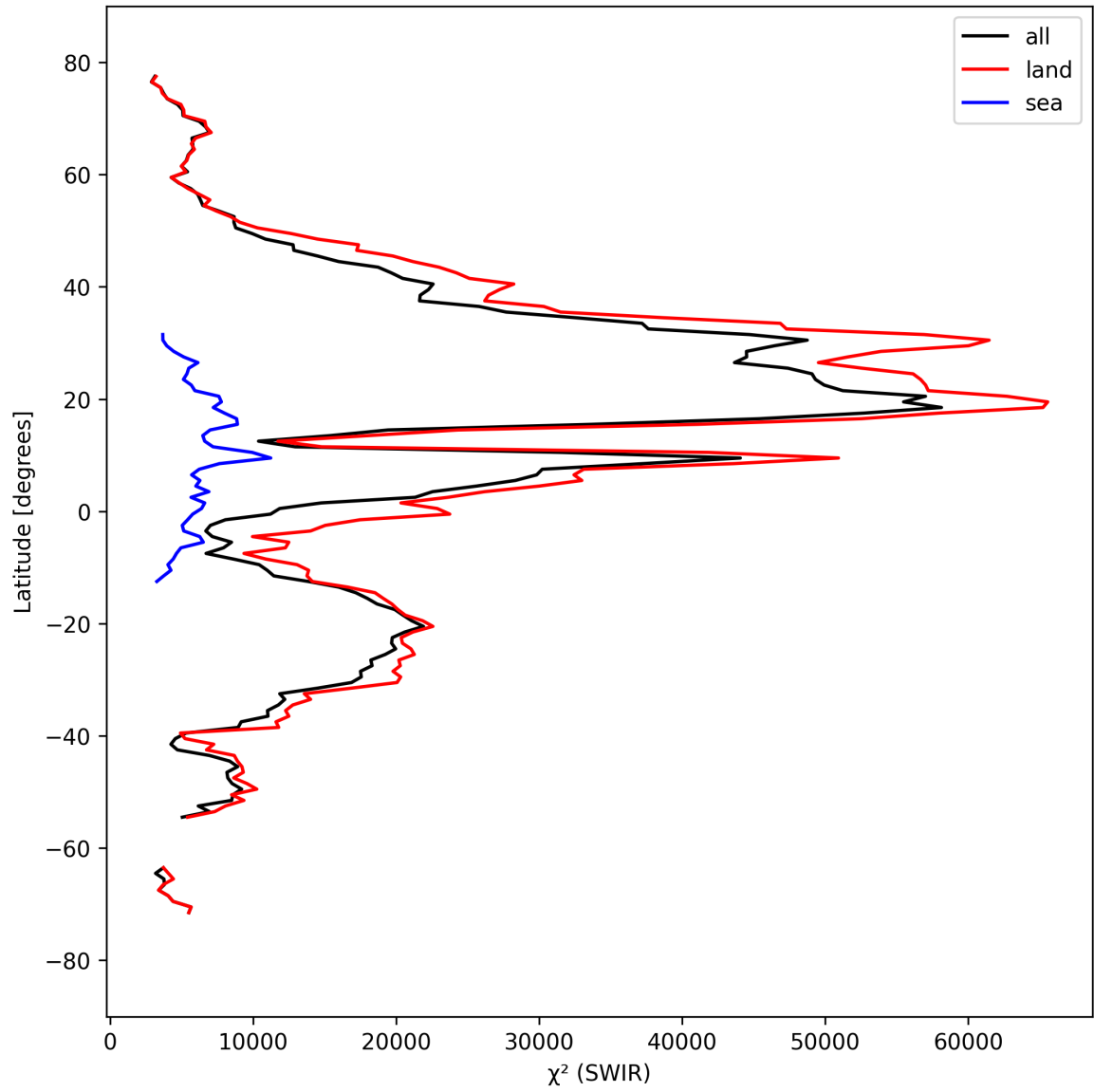
Figure 17: Zonal average of “ \chi^2 (SWIR)” for 2025-09-15 to 2025-09-17.
