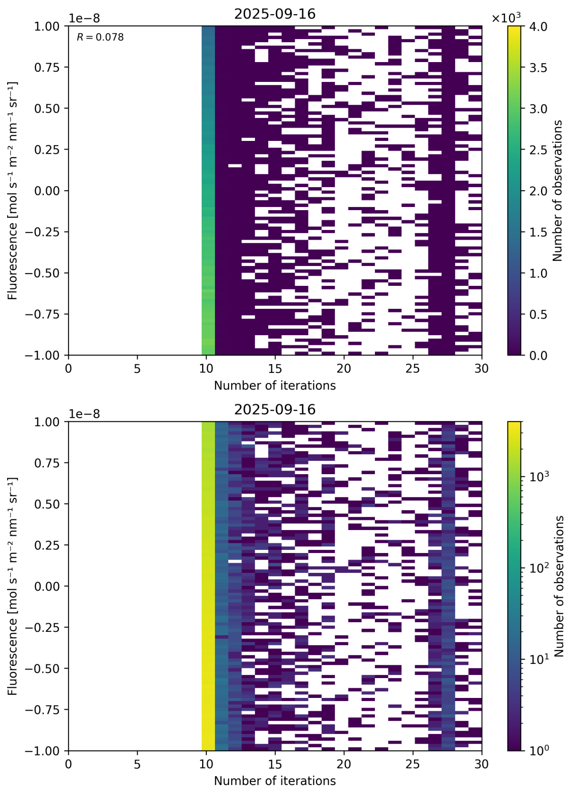
Figure 87: Scatter density plot of “Number of iterations” against “Fluorescence” for 2025-09-15 to 2025-09-17.
