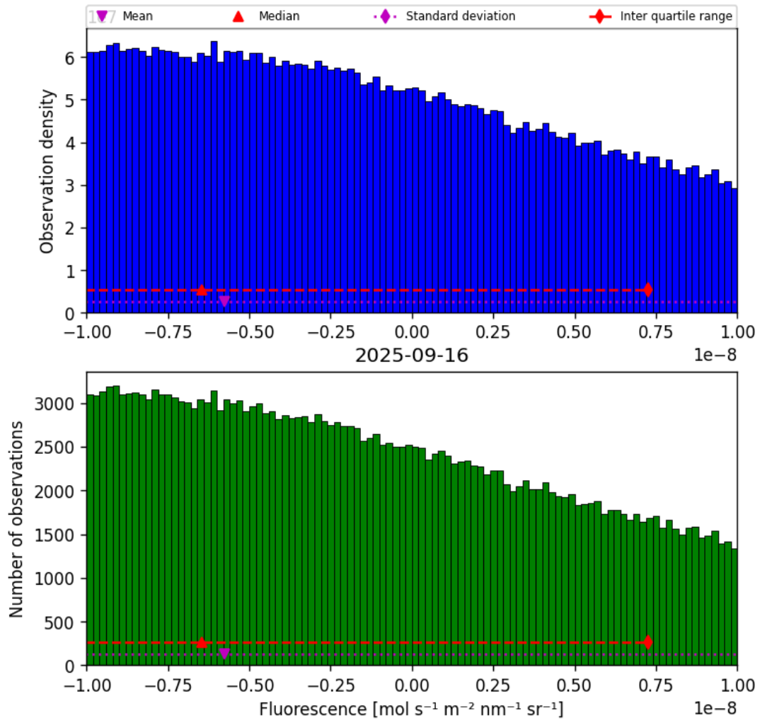
Figure 32: Histogram of “Fluorescence” for 2025-09-15 to 2025-09-17
