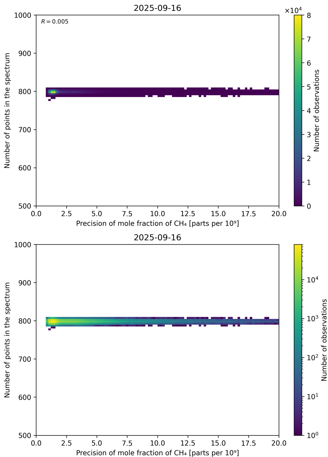
Figure 84: Scatter density plot of “Precision of mole fraction of CH 4 ” against “Number of points in the spectrum” for 2025-09-15 to 2025-09-17.
