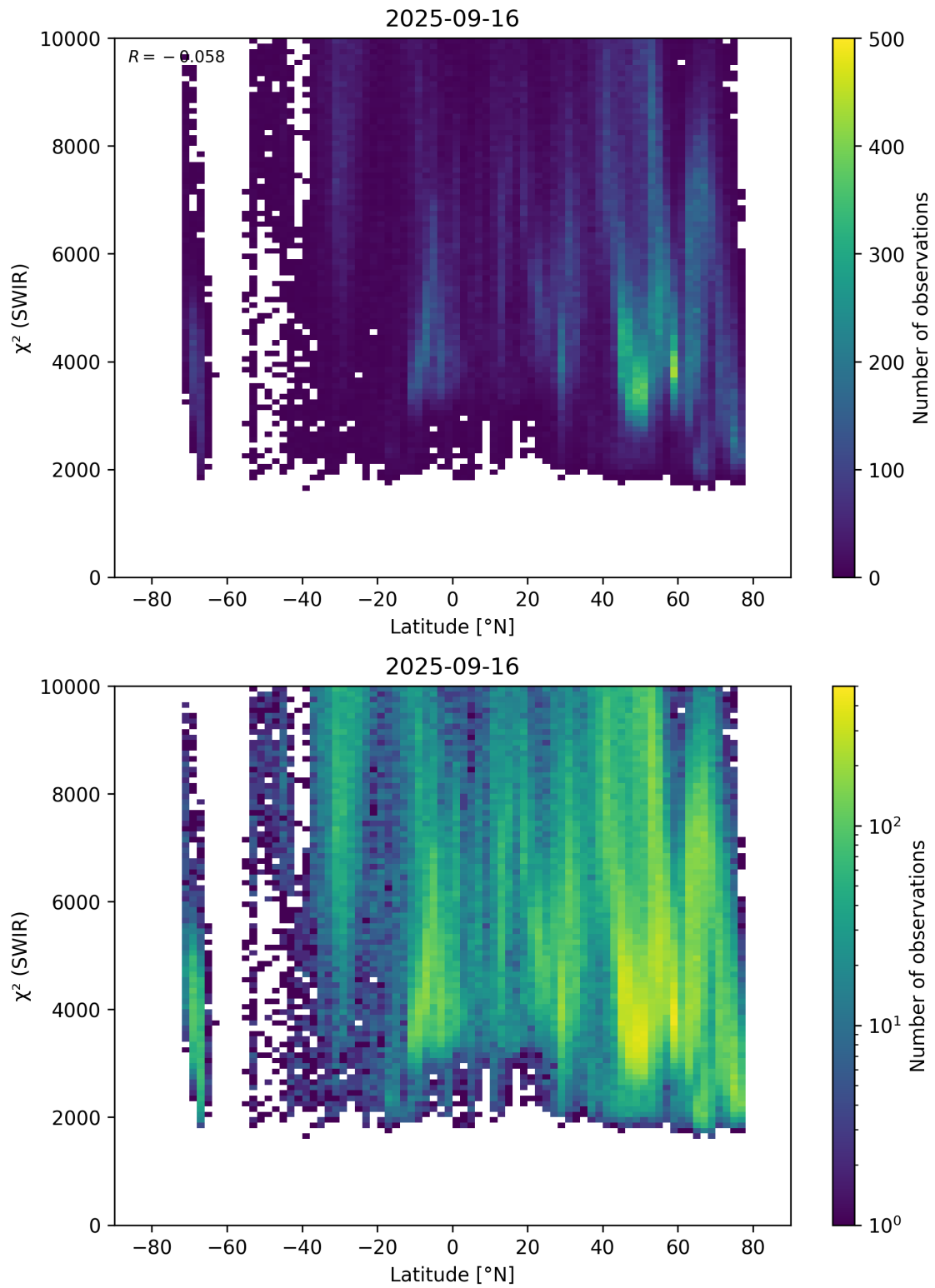
Figure 54: Scatter density plot of “Latitude” against “ \chi^2 (SWIR)” for 2025-09-15 to 2025-09-17.
