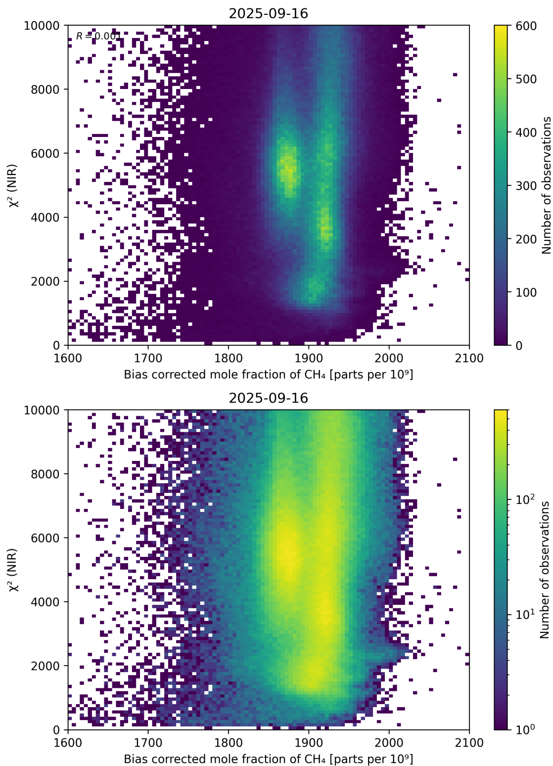
Figure 63: Scatter density plot of “Bias corrected mole fraction of CH 4 ” against “ \chi^2 (NIR)” for 2025-09-15 to 2025-09-17.
