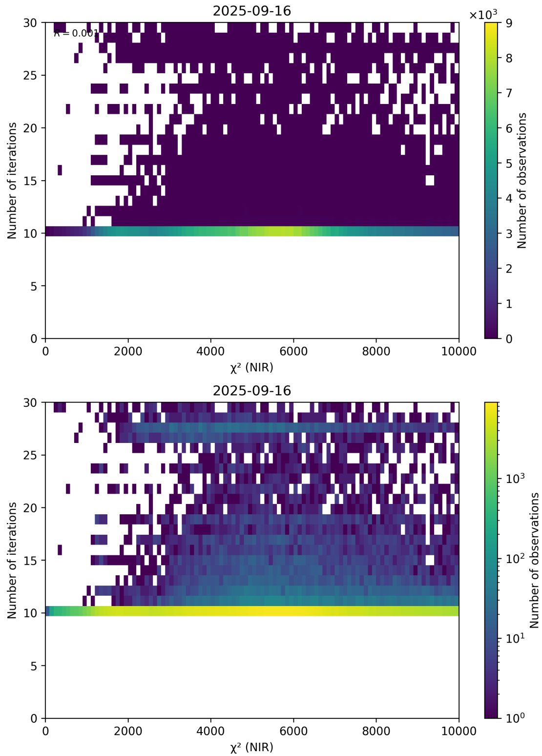
Figure 46: Scatter density plot of “ \chi^2 (NIR)” against “Number of iterations” for 2025-09-15 to 2025-09-17.
