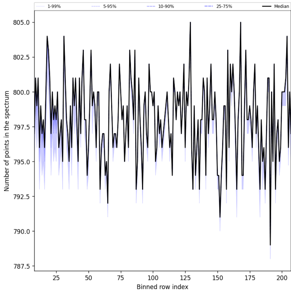
Figure 37: Along track statistics of “Number of points in the spectrum” for 2025-09-15 to 2025-09-17
