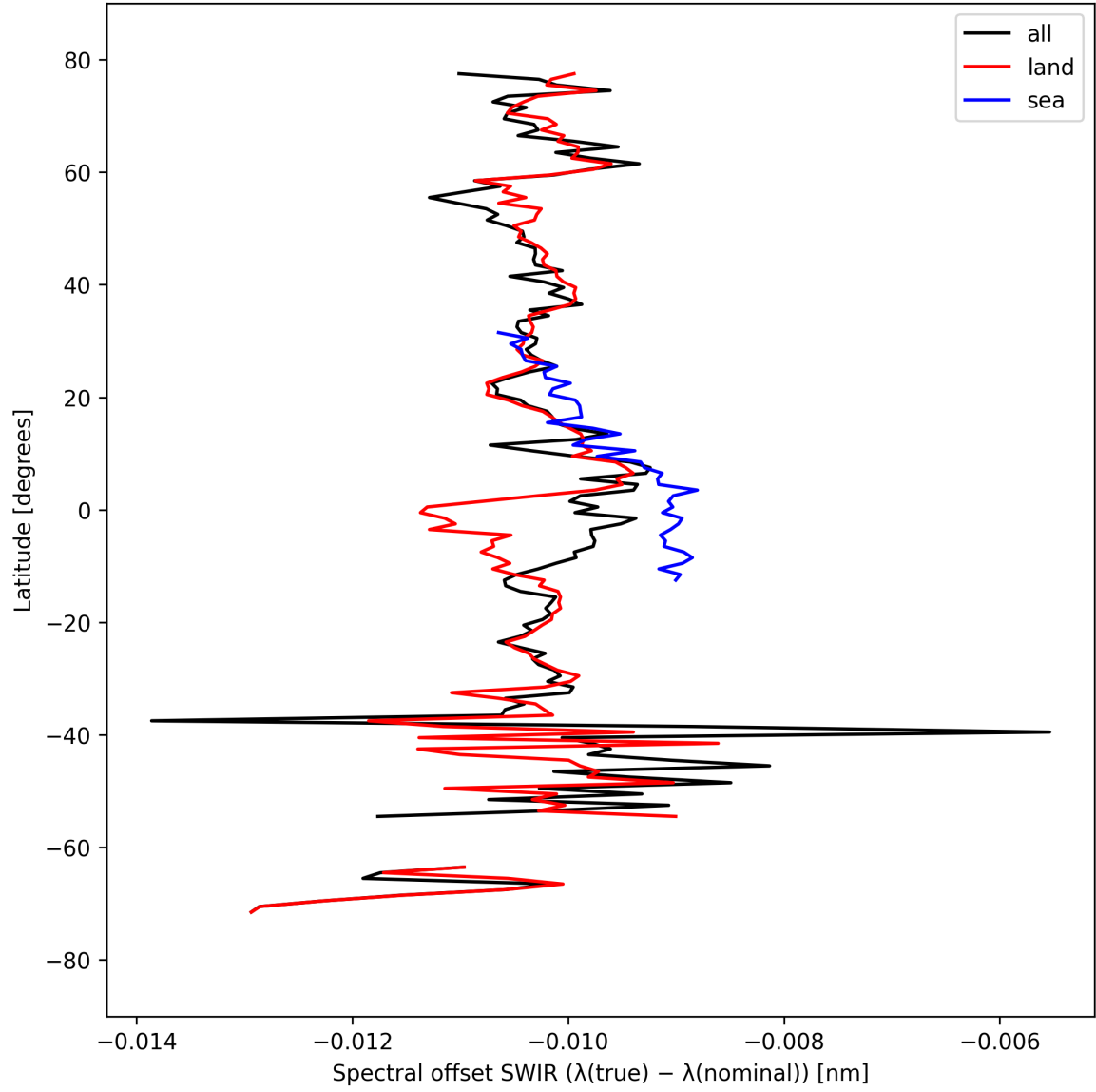
Figure 16: Zonal average of “Spectral offset SWIR ( \lambda_{\text{true}} - \lambda_{\text{nominal}} )” for 2025-09-15 to 2025-09-17.
