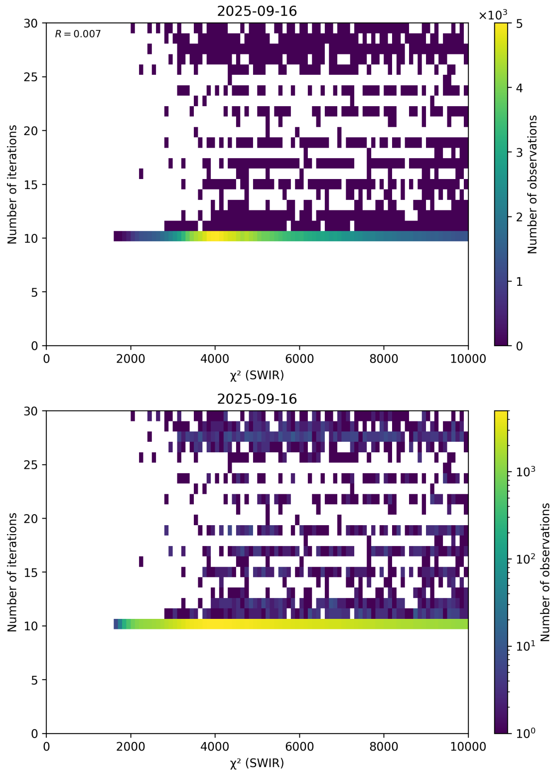
Figure 50: Scatter density plot of “ \chi^2 (SWIR)” against “Number of iterations” for 2025-09-15 to 2025-09-17.
