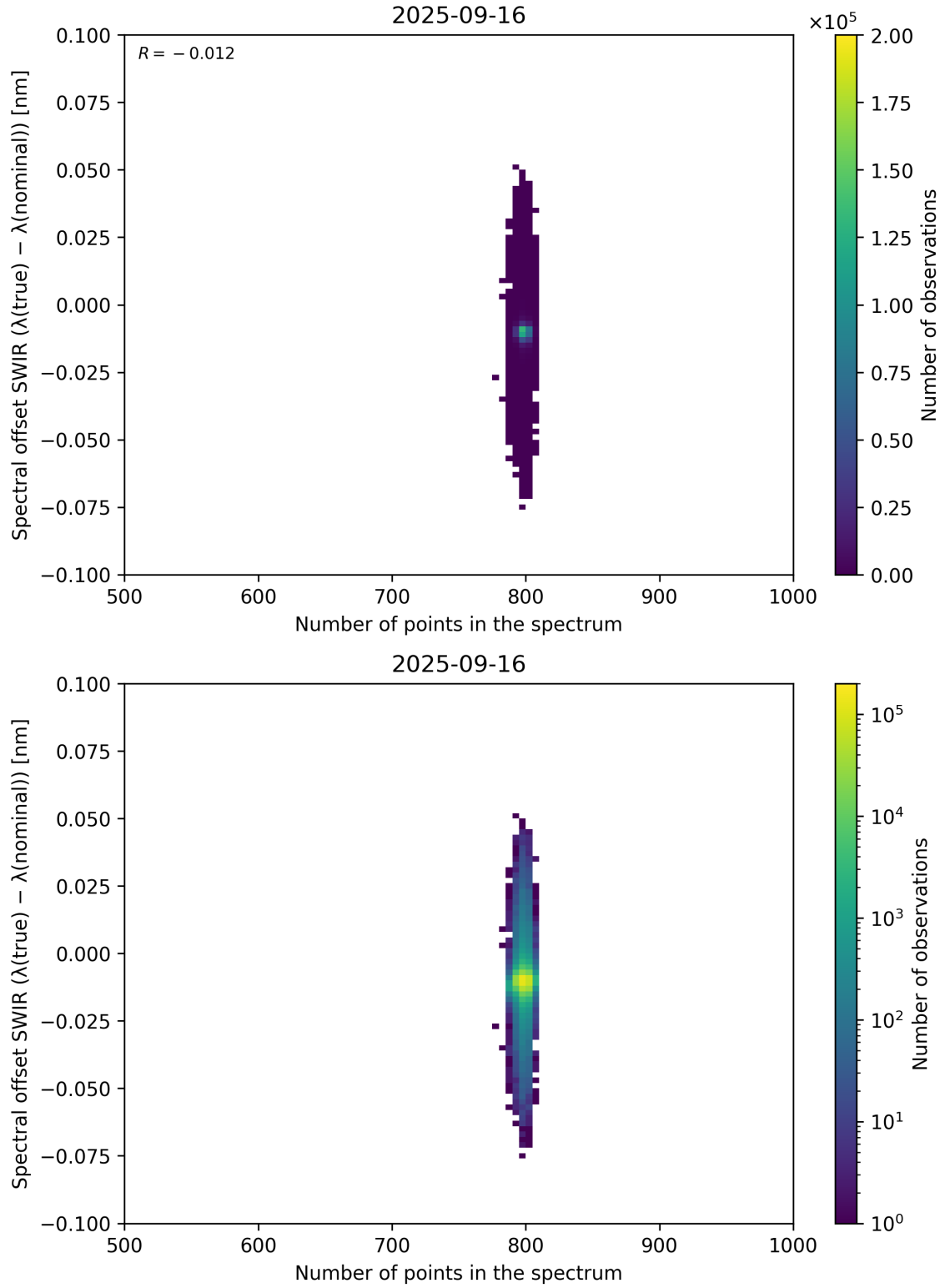
Figure 93: Scatter density plot of “Number of points in the spectrum” against “Spectral offset SWIR ( \lambda_{\text{true}} - \lambda_{\text{nominal}} )” for 2025-09-15 to 2025-09-17.
