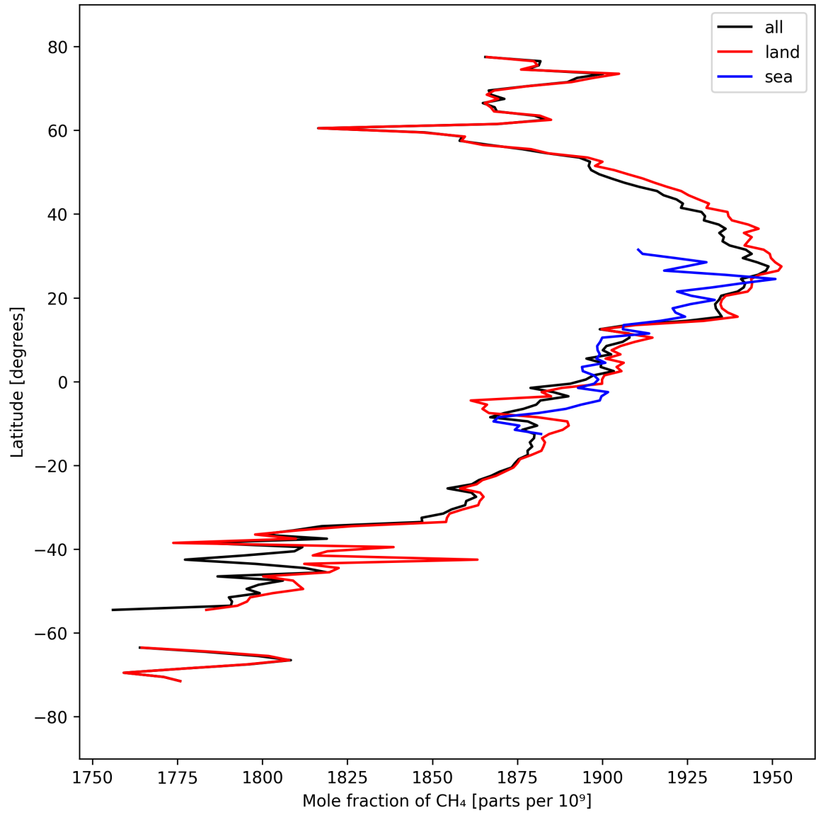
Figure 12: Zonal average of “Mole fraction of CH 4 ” for 2025-09-15 to 2025-09-17.
