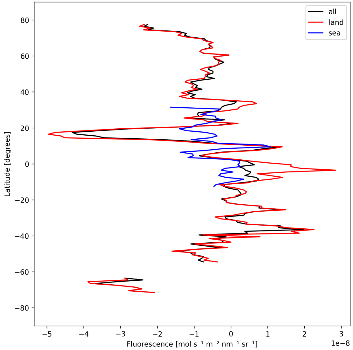
Figure 21: Zonal average of “Fluorescence” for 2025-09-15 to 2025-09-17.
