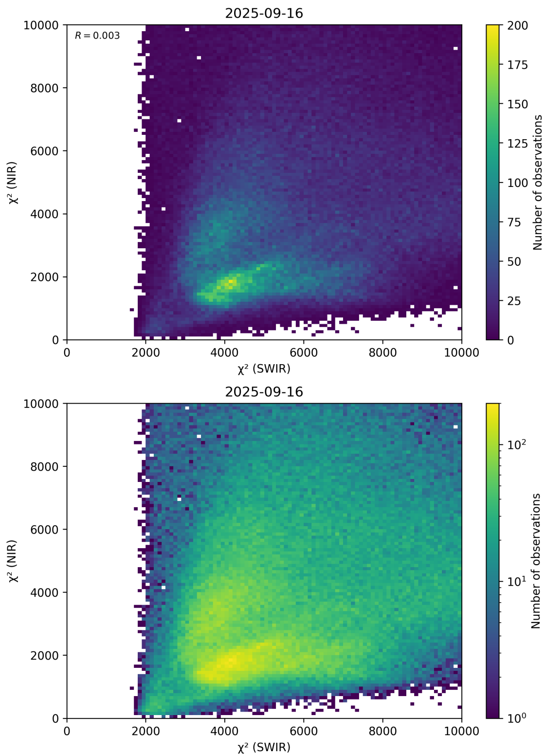
Figure 47: Scatter density plot of “ \chi^2 (SWIR)” against “ \chi^2 (NIR)” for 2025-09-15 to 2025-09-17.
