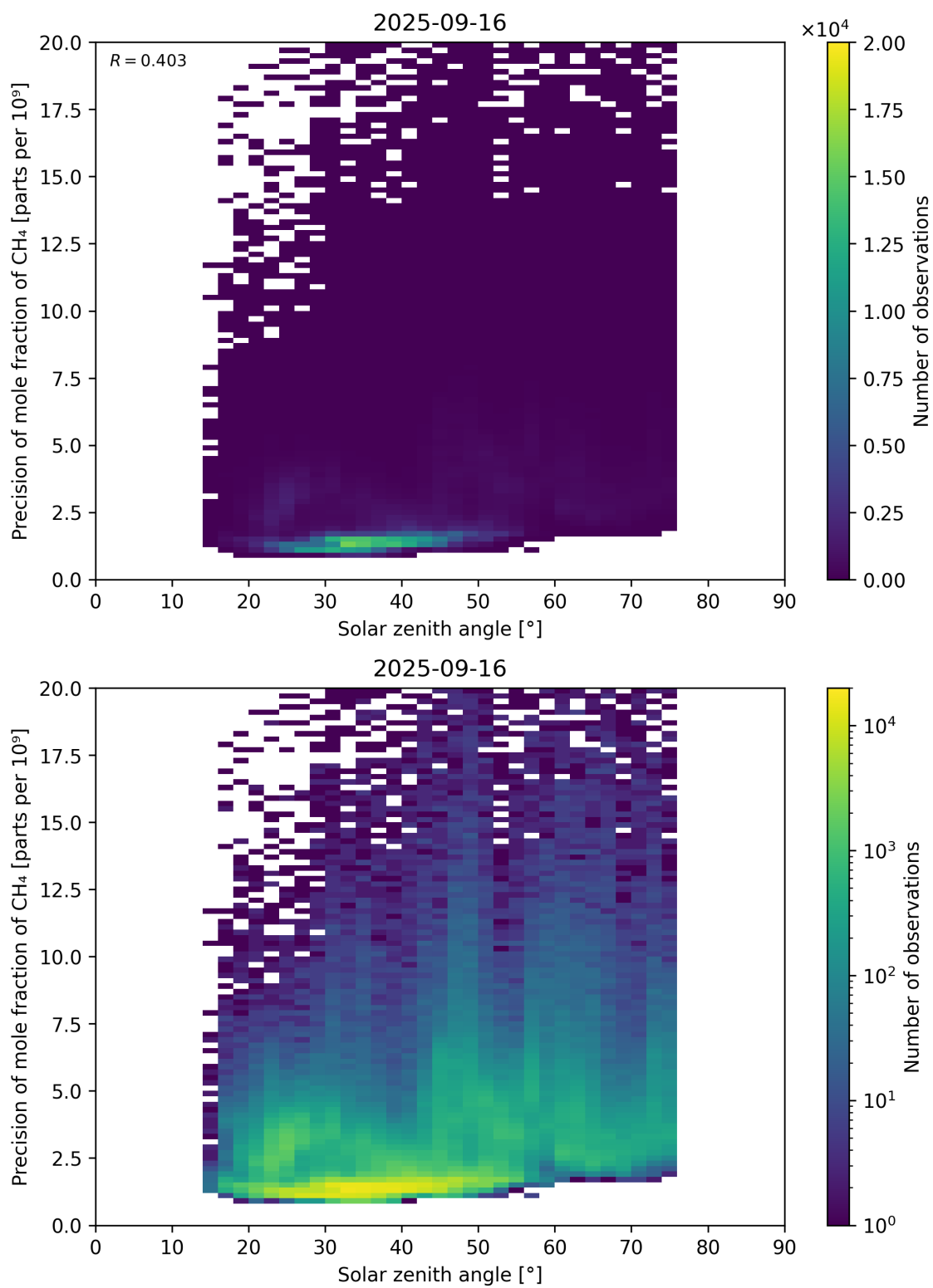
Figure 101: Scatter density plot of “Solar zenith angle” against “Precision of mole fraction of CH 4 ” for 2025-09-15 to 2025-09-17.
