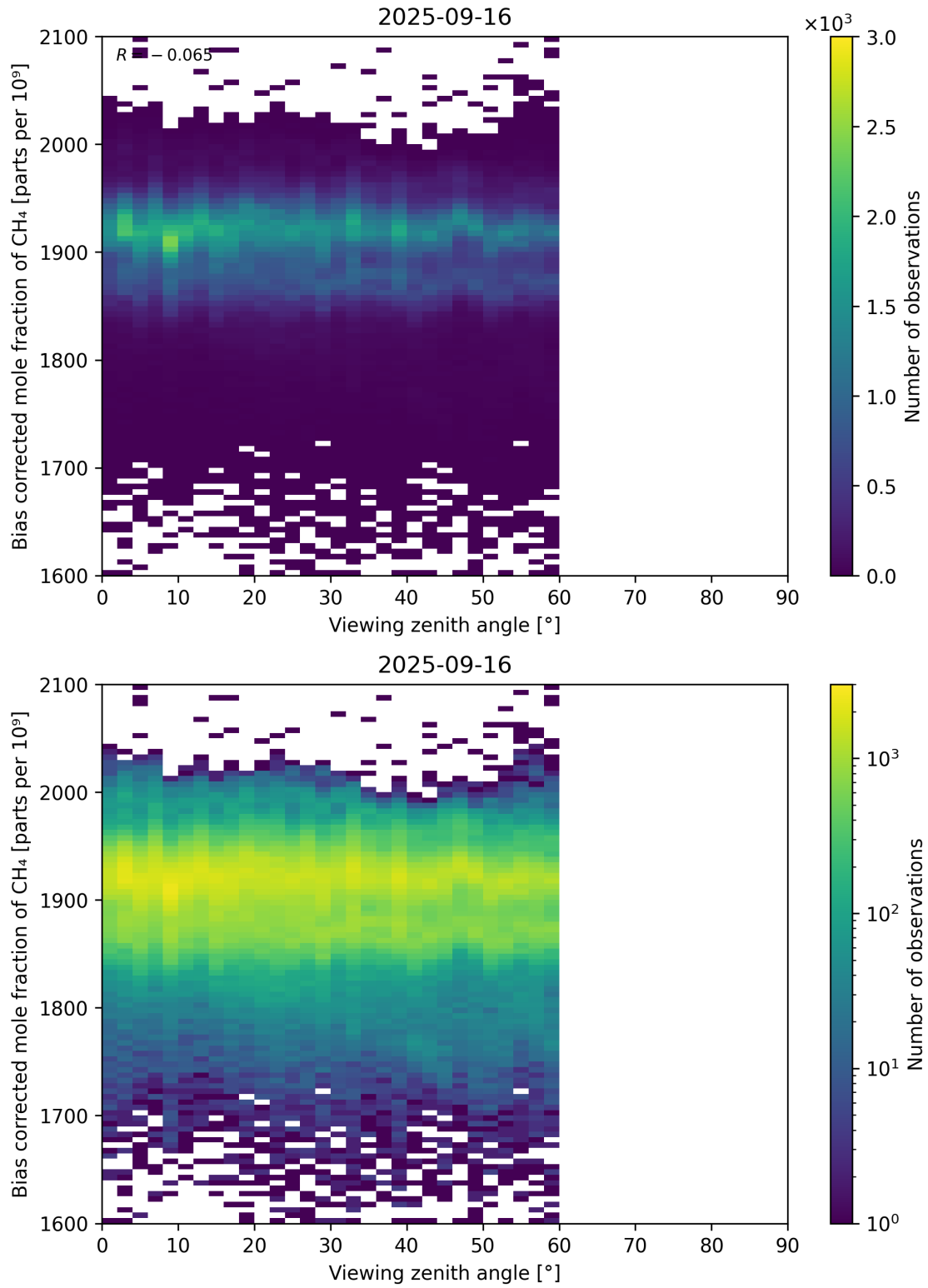
Figure 111: Scatter density plot of “Viewing zenith angle” against “Bias corrected mole fraction of CH 4 ” for 2025-09-15 to 2025-09-17.
