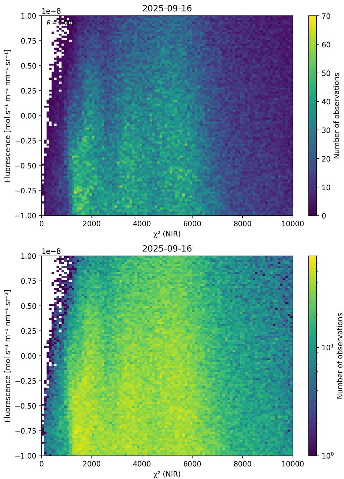
Figure 45: Scatter density plot of “ \chi^2 (NIR)” against “Fluorescence” for 2025-09-15 to 2025-09-17.
