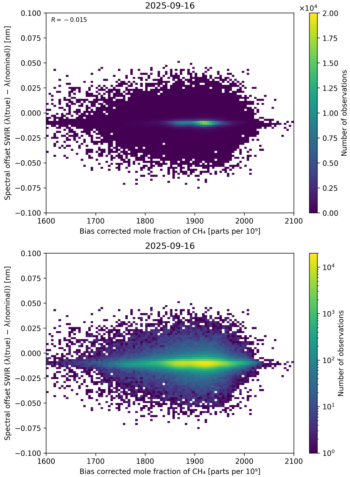
Figure 69: Scatter density plot of “Bias corrected mole fraction of \text{CH}_4 ” against “Spectral offset SWIR ( \lambda_{\text{true}} - \lambda_{\text{nominal}} )” for 2025-09-15 to 2025-09-17.
