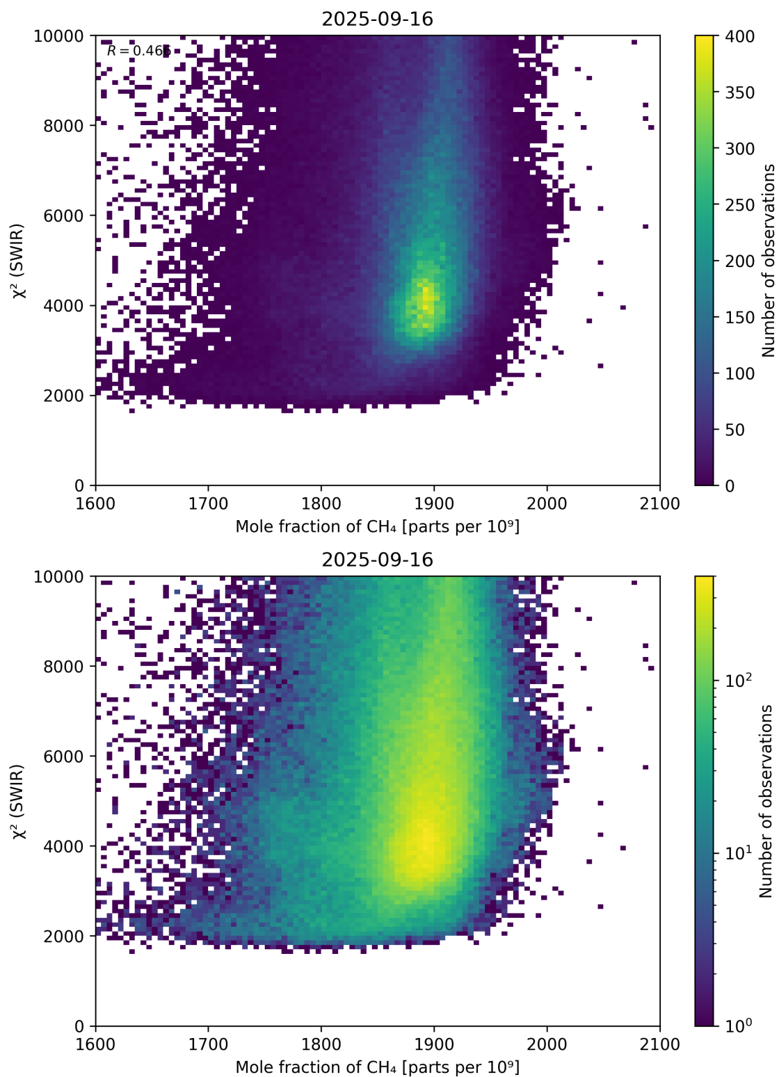
Figure 71: Scatter density plot of “Mole fraction of \text{CH}_4 ” against “ \chi^2 (SWIR)” for 2025-09-15 to 2025-09-17.
