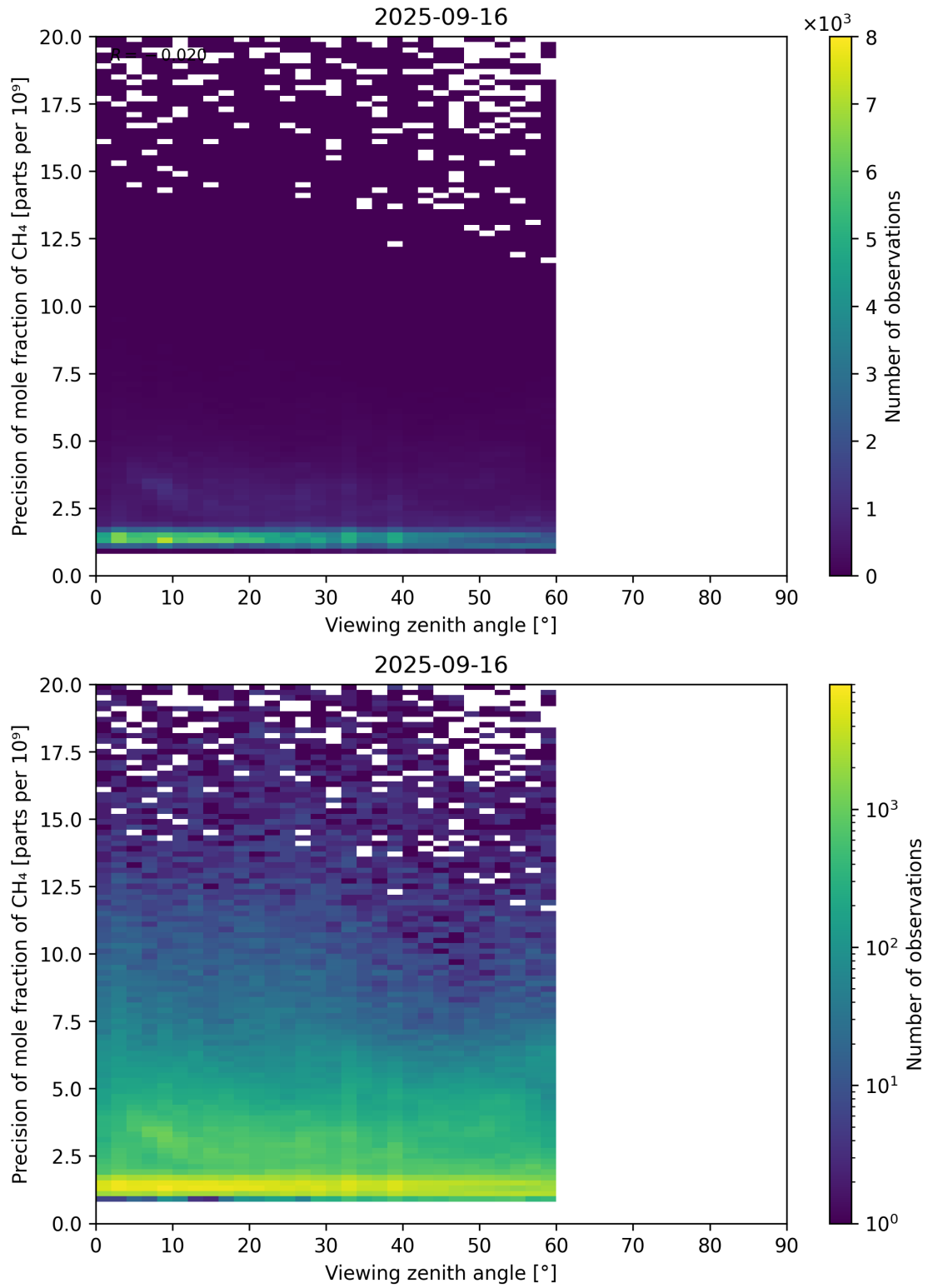
Figure 112: Scatter density plot of “Viewing zenith angle” against “Precision of mole fraction of CH 4 ” for 2025-09-15 to 2025-09-17.
