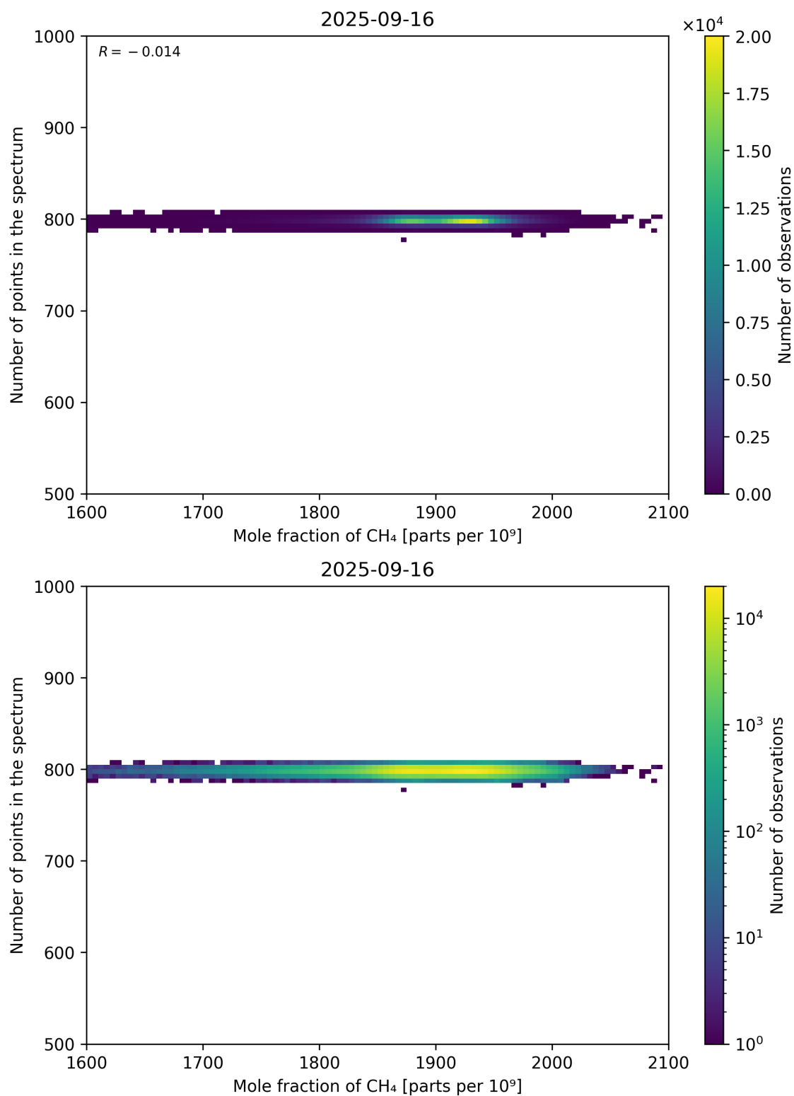
Figure 77: Scatter density plot of “Mole fraction of CH 4 ” against “Number of points in the spectrum” for 2025-09-15 to 2025-09-17.
