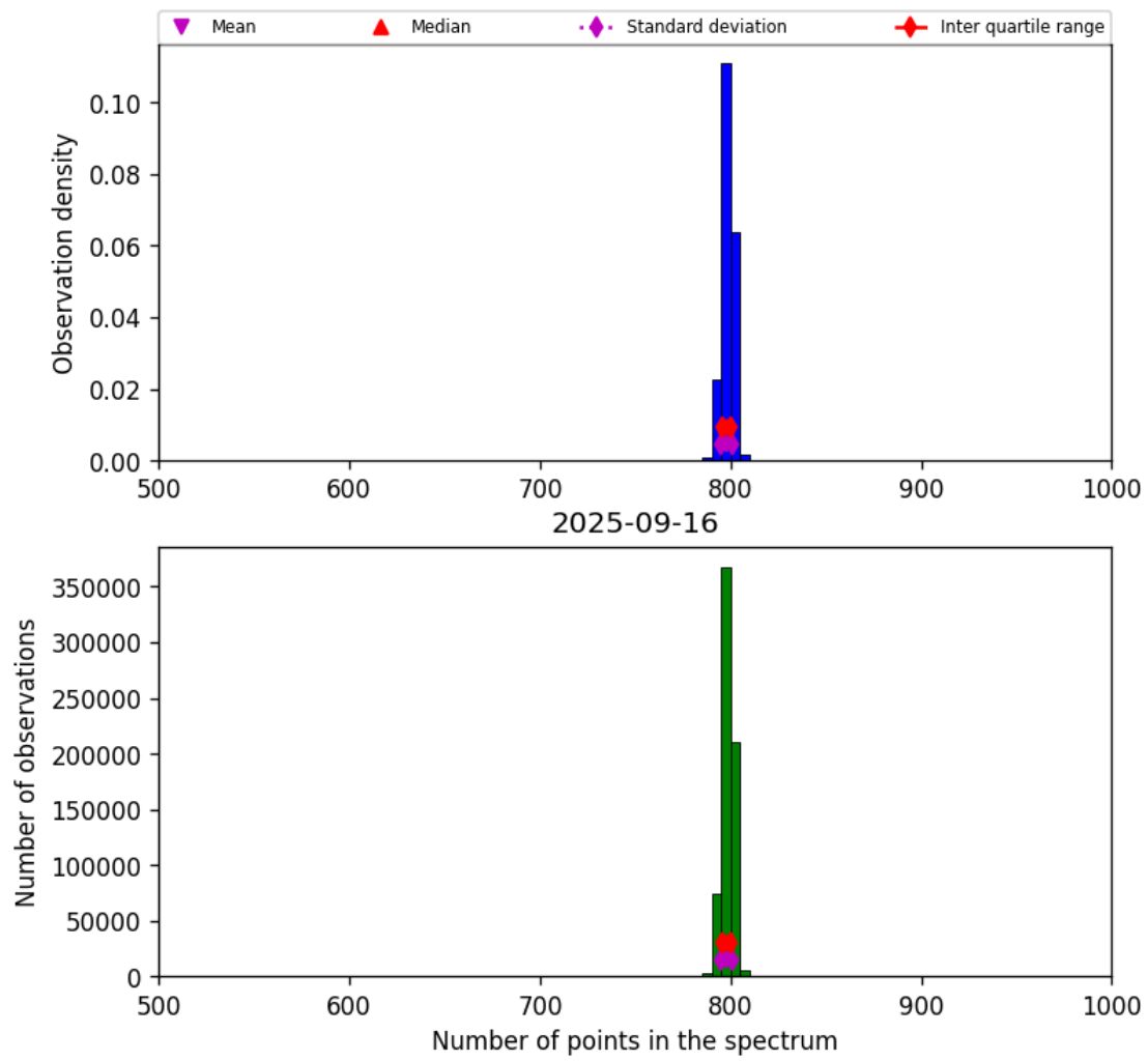
Figure 26: Histogram of “Number of points in the spectrum” for 2025-09-15 to 2025-09-17
