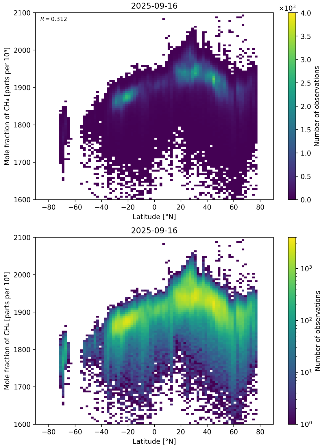
Figure 57: Scatter density plot of “Latitude” against “Mole fraction of CH 4 ” for 2025-09-15 to 2025-09-17.
