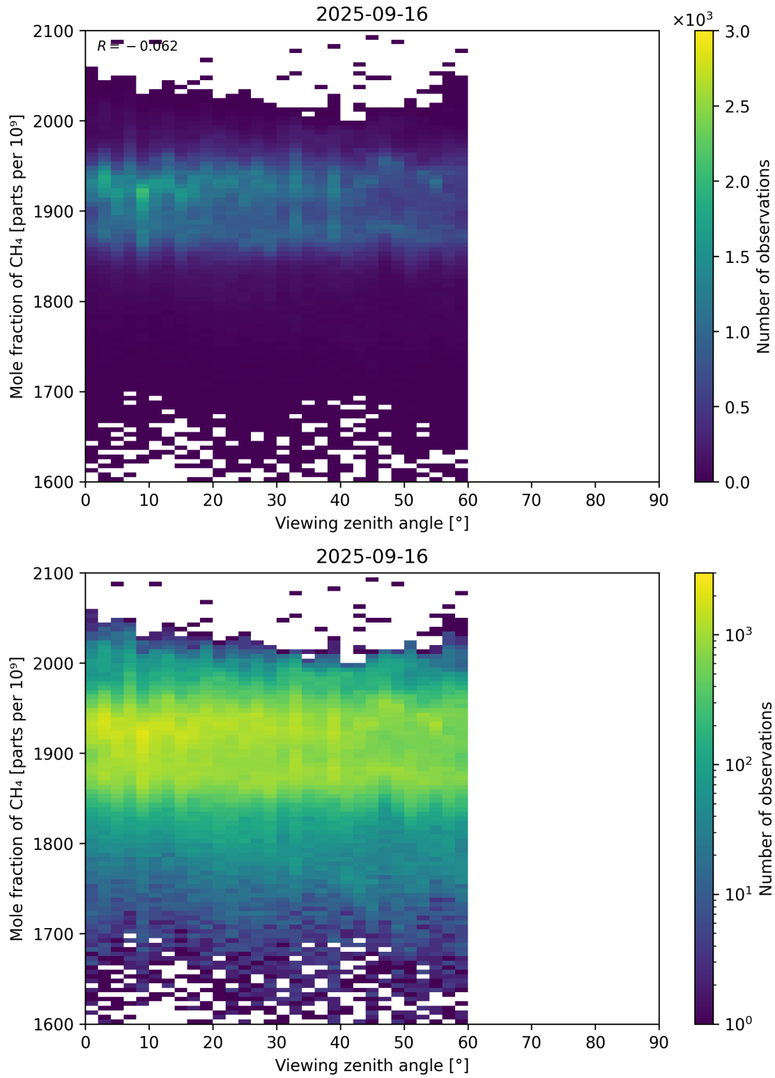
Figure 110: Scatter density plot of “Viewing zenith angle” against “Mole fraction of CH 4 ” for 2025-09-15 to 2025-09-17.
