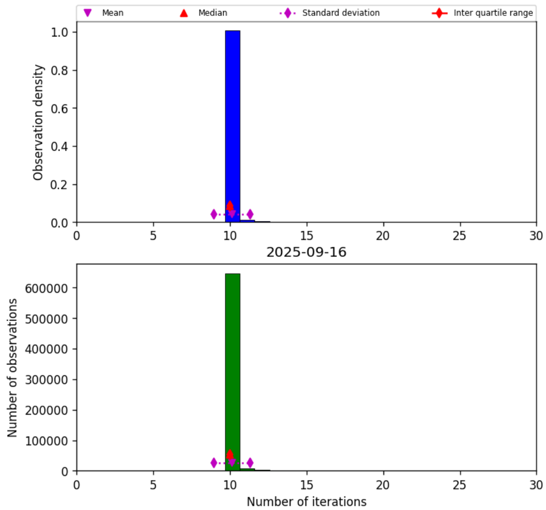
Figure 31: Histogram of “Number of iterations” for 2025-09-15 to 2025-09-17
