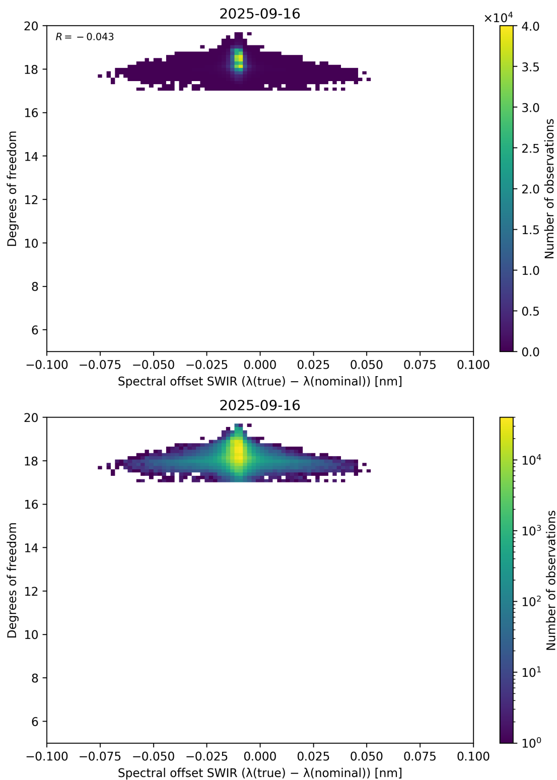
Figure 119: Scatter density plot of “Spectral offset SWIR ( \lambda_{\text{true}} - \lambda_{\text{nominal}} )” against “Degrees of freedom” for 2025-09-15 to 2025-09-17.
