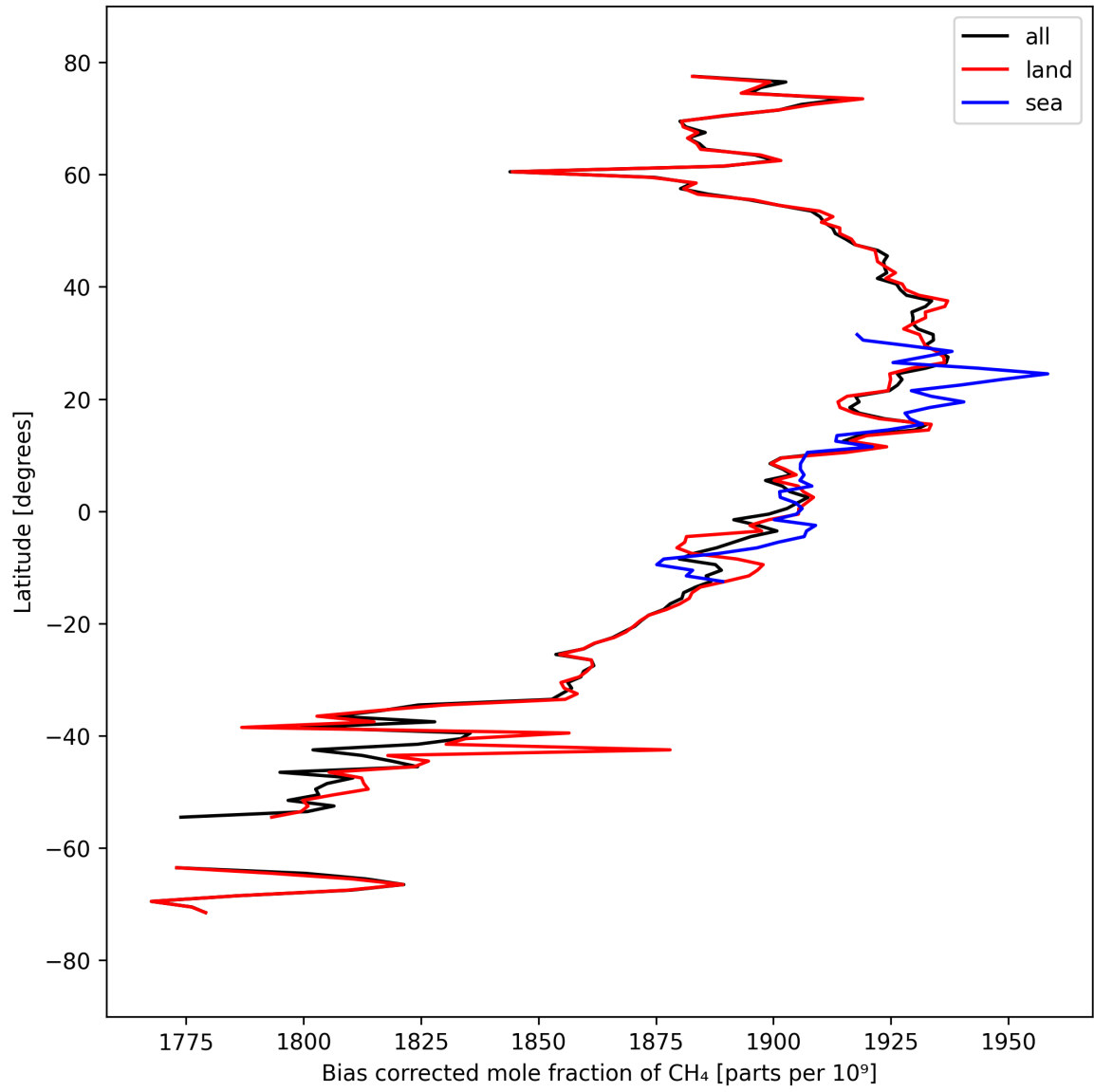
Figure 14: Zonal average of “Bias corrected mole fraction of CH 4 ” for 2025-09-15 to 2025-09-17.
