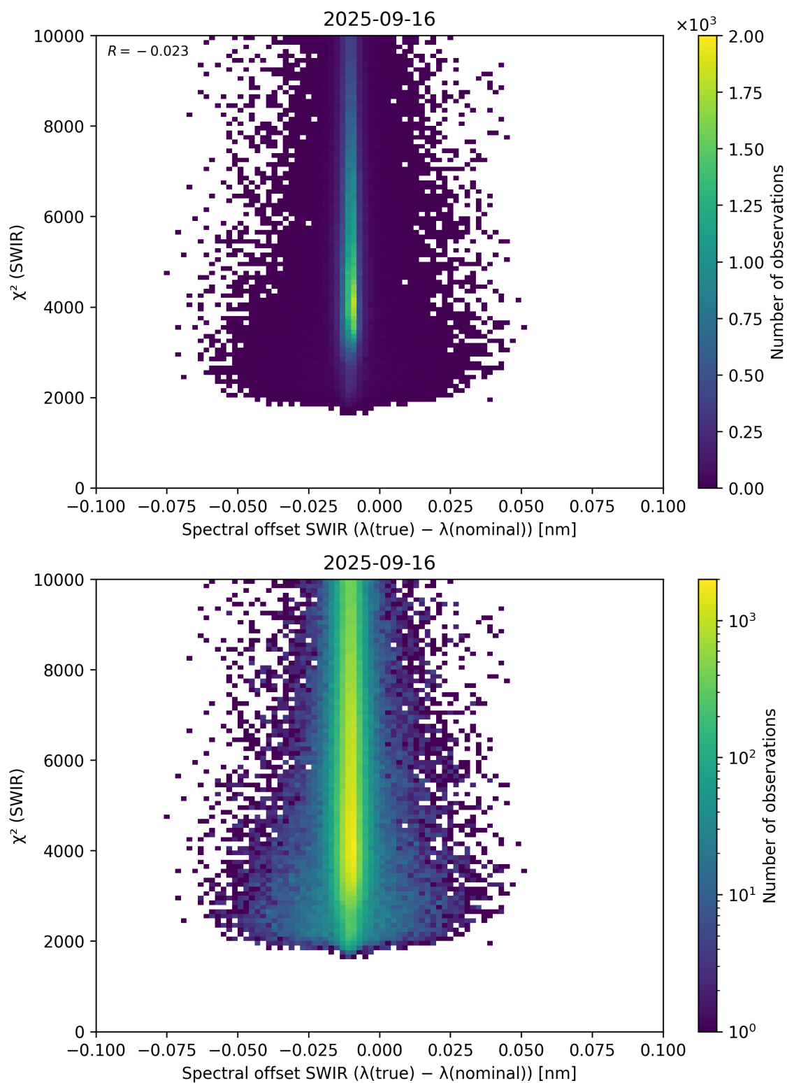
Figure 118: Scatter density plot of “Spectral offset SWIR ( \lambda_{\text{true}} - \lambda_{\text{nominal}} )” against “ \chi^2 (SWIR)” for 2025-09-15 to 2025-09-17.
