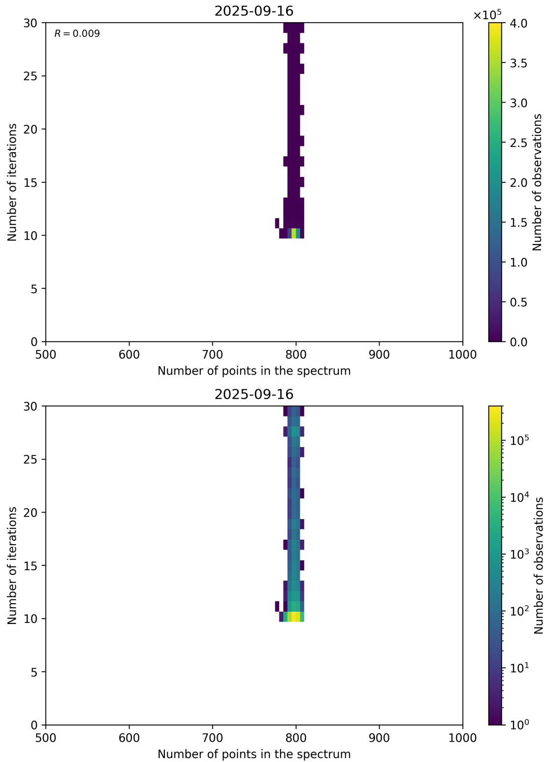
Figure 92: Scatter density plot of “Number of points in the spectrum” against “Number of iterations” for 2025-09-15 to 2025-09-17.
