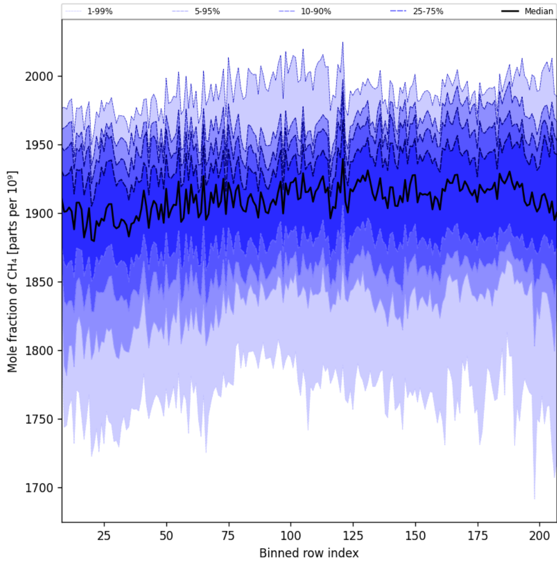
Figure 34: Along track statistics of “Mole fraction of CH 4 ” for 2025-09-15 to 2025-09-17
