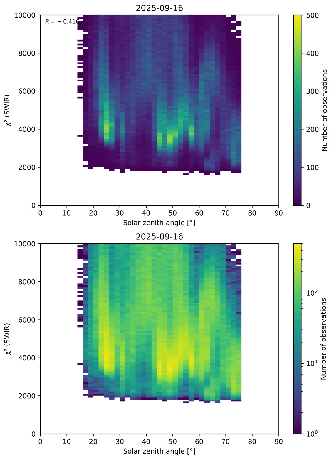
Figure 95: Scatter density plot of “Solar zenith angle” against “ \chi^2 (SWIR)” for 2025-09-15 to 2025-09-17.
