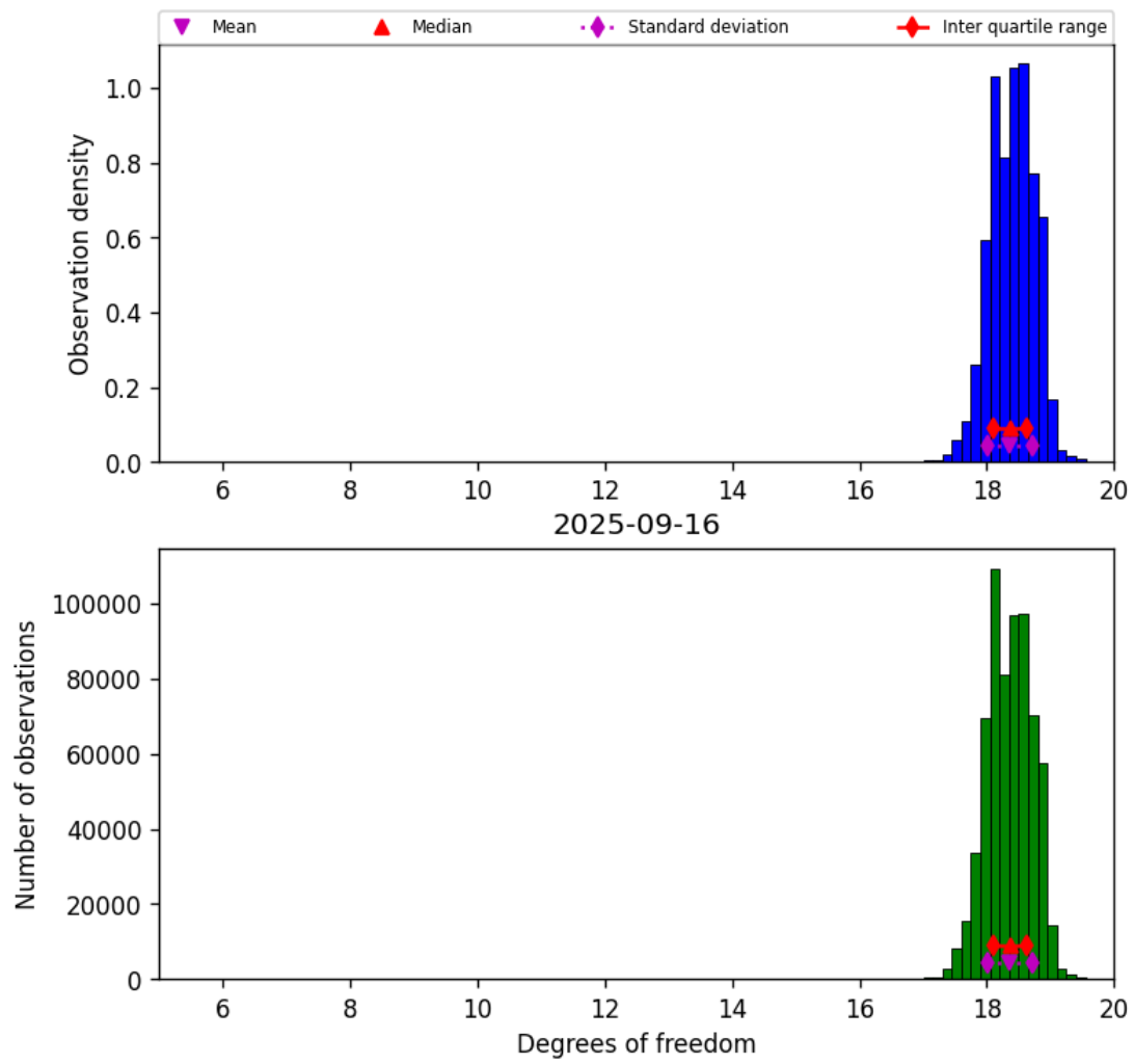
Figure 30: Histogram of “Degrees of freedom” for 2025-09-15 to 2025-09-17
