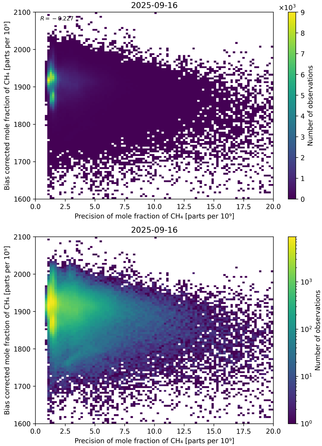
Figure 82: Scatter density plot of “Precision of mole fraction of CH 4 ” against “Bias corrected mole fraction of CH 4 ” for 2025-09-15 to 2025-09-17.
