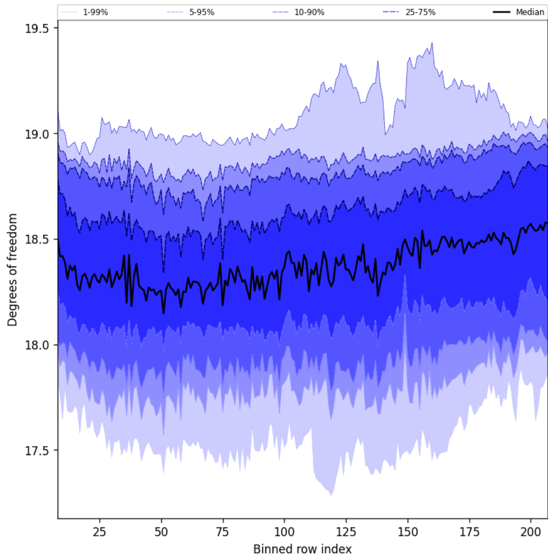
Figure 41: Along track statistics of “Degrees of freedom” for 2025-09-15 to 2025-09-17
