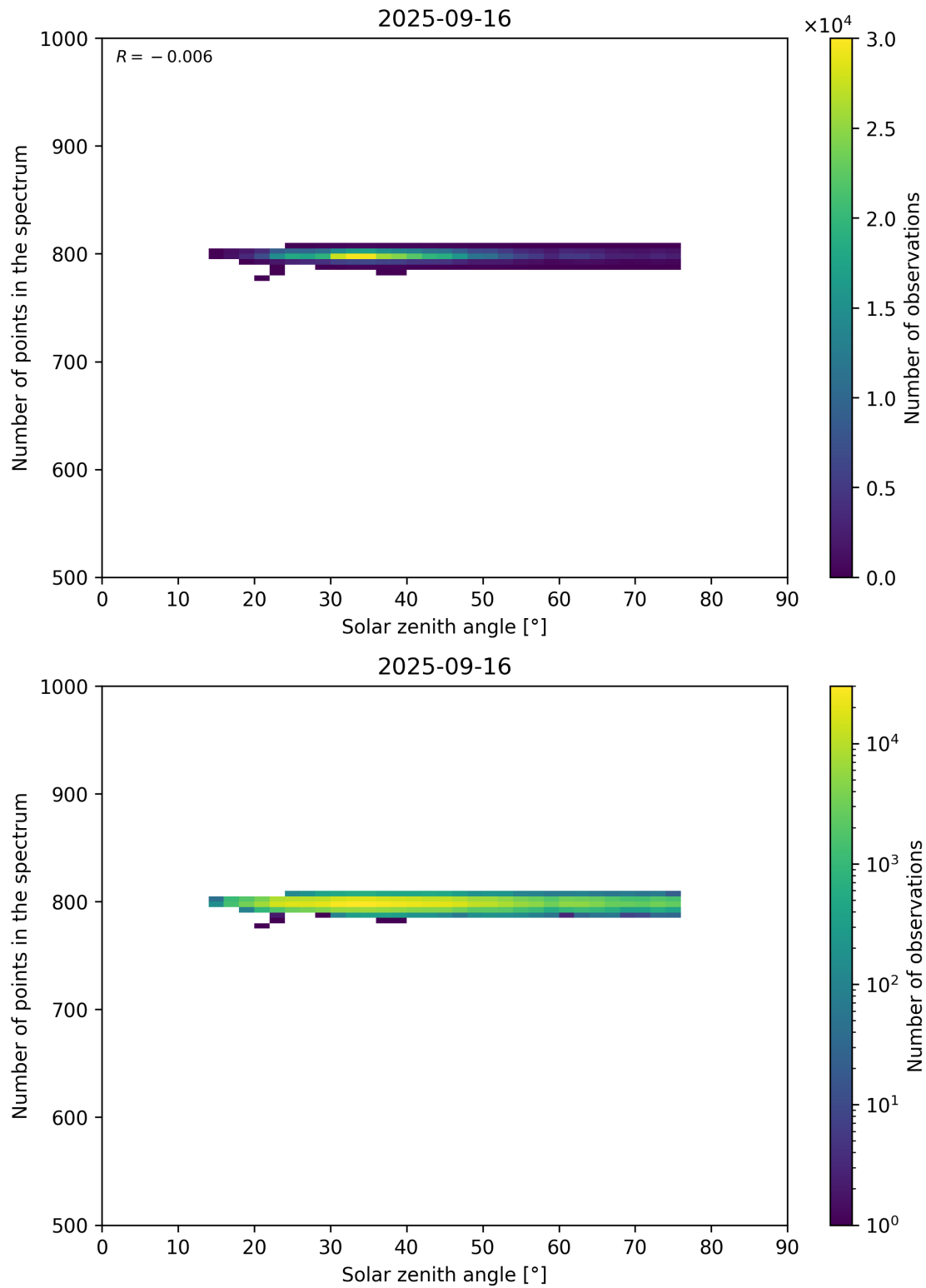
Figure 103: Scatter density plot of “Solar zenith angle” against “Number of points in the spectrum” for 2025-09-15 to 2025-09-17.
