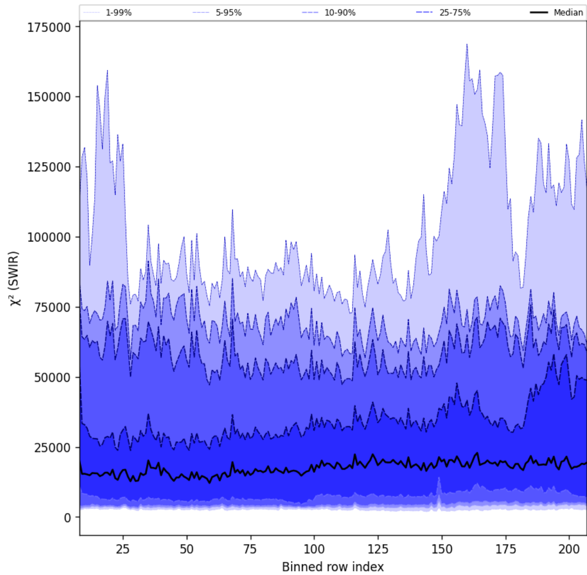
Figure 39: Along track statistics of " \chi^2 (SWIR)" for 2025-09-15 to 2025-09-17
