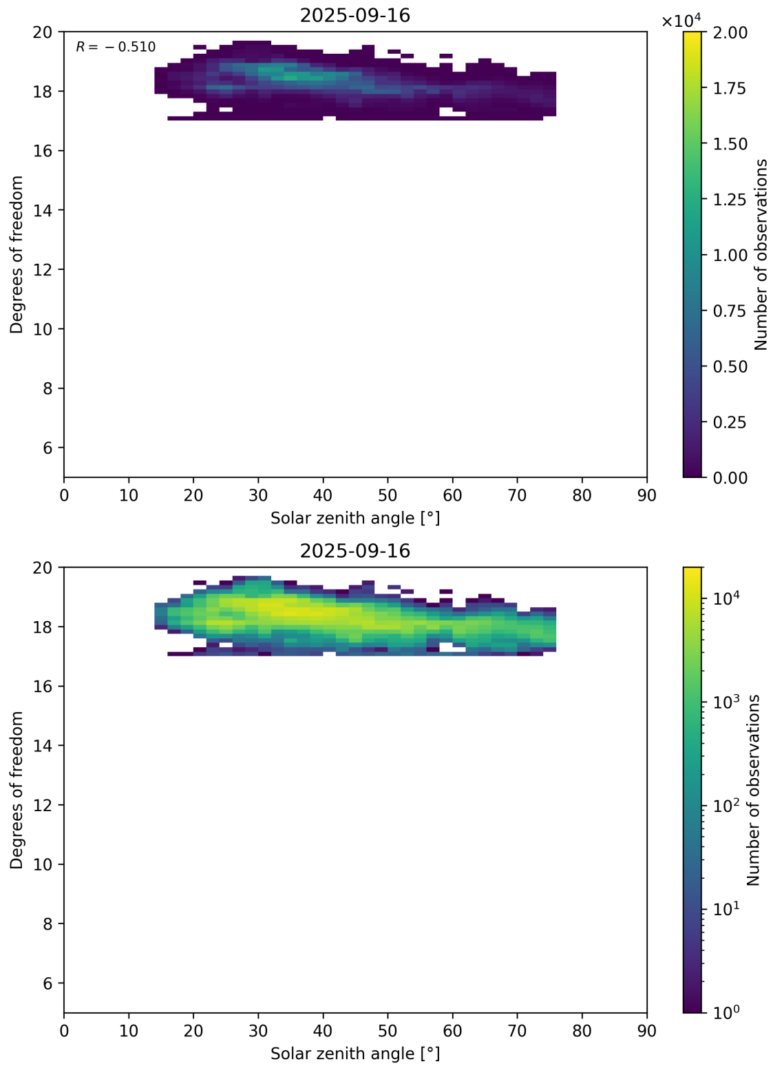
Figure 96: Scatter density plot of “Solar zenith angle” against “Degrees of freedom” for 2025-09-15 to 2025-09-17.
