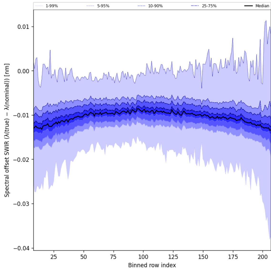
Figure 38: Along track statistics of “Spectral offset SWIR ( \lambda_{\text{true}} - \lambda_{\text{nominal}} )” for 2025-09-15 to 2025-09-17
