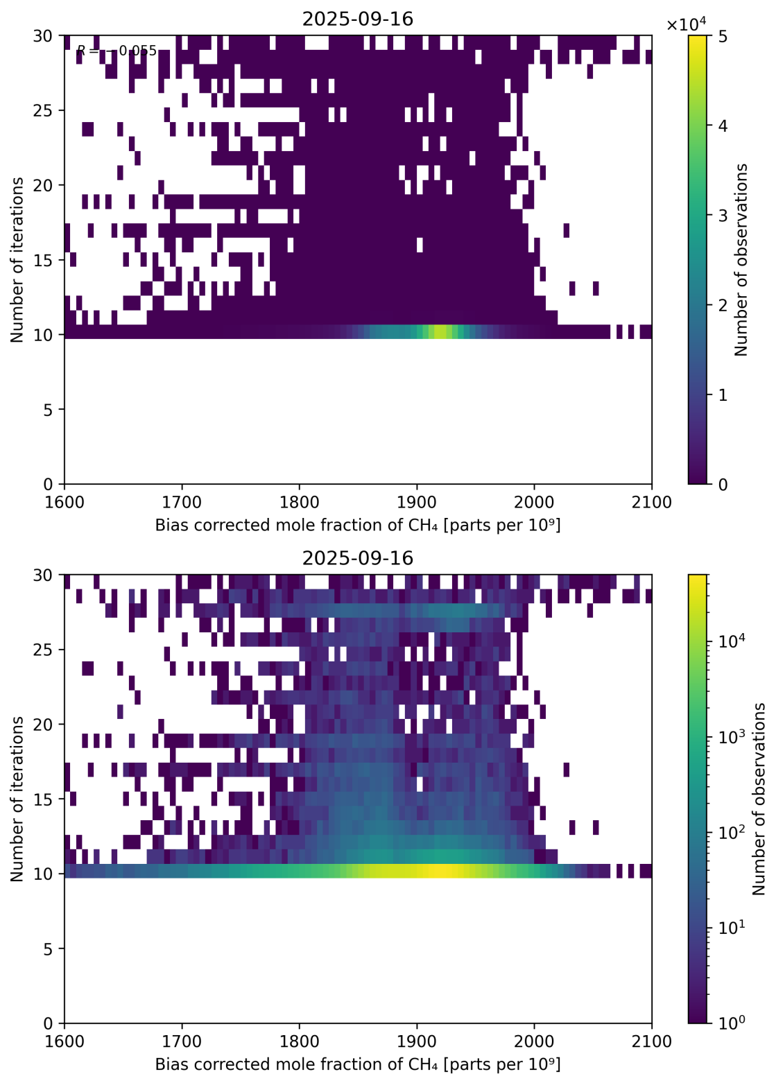
Figure 67: Scatter density plot of “Bias corrected mole fraction of CH 4 ” against “Number of iterations” for 2025-09-15 to 2025-09-17.
