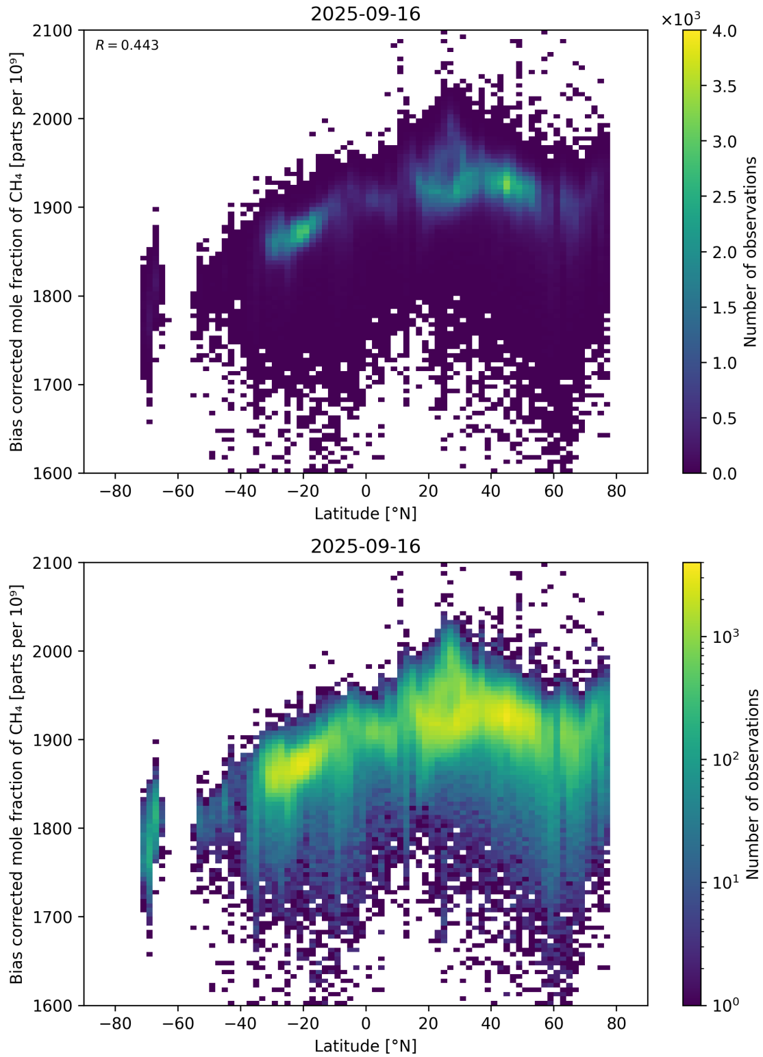
Figure 58: Scatter density plot of “Latitude” against “Bias corrected mole fraction of \text{CH}_4 ” for 2025-09-15 to 2025-09-17.
