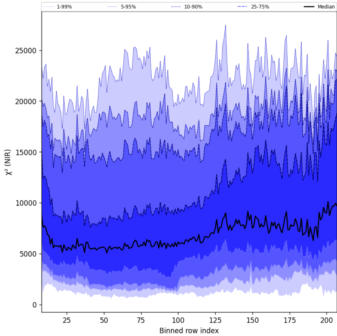
Figure 40: Along track statistics of “ \chi^2 (NIR)” for 2025-09-15 to 2025-09-17
