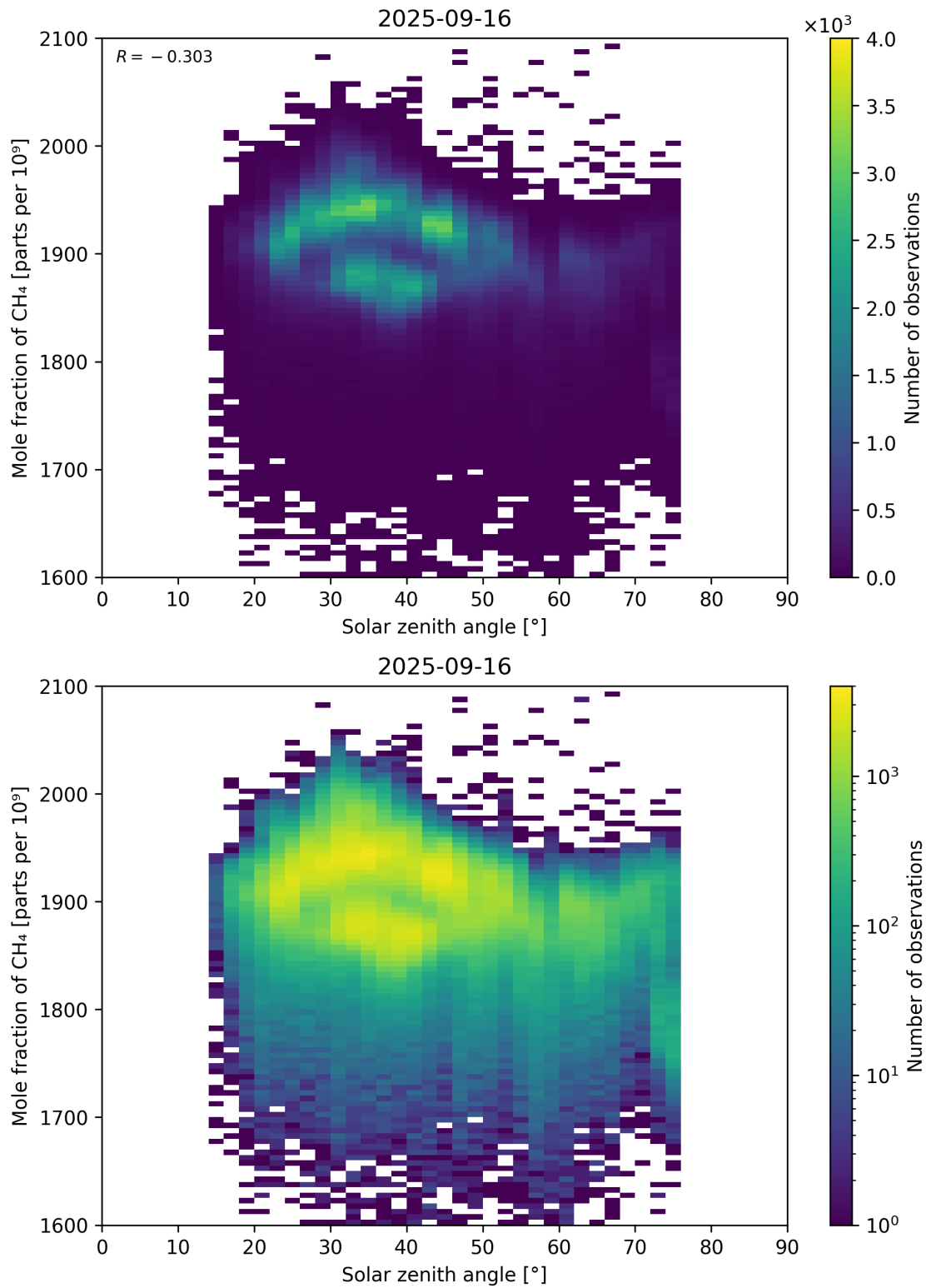
Figure 99: Scatter density plot of “Solar zenith angle” against “Mole fraction of CH 4 ” for 2025-09-15 to 2025-09-17.
