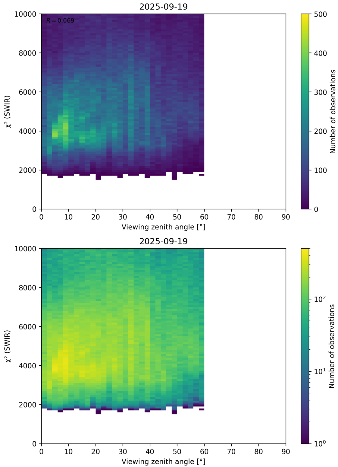
Figure 106: Scatter density plot of “Viewing zenith angle” against “ \chi^2 (SWIR)” for 2025-09-18 to 2025-09-20.
