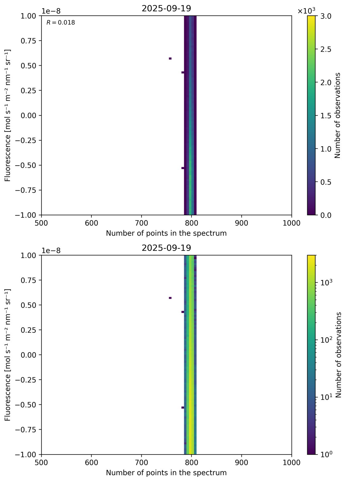
Figure 91: Scatter density plot of “Number of points in the spectrum” against “Fluorescence” for 2025-09-18 to 2025-09-20.
