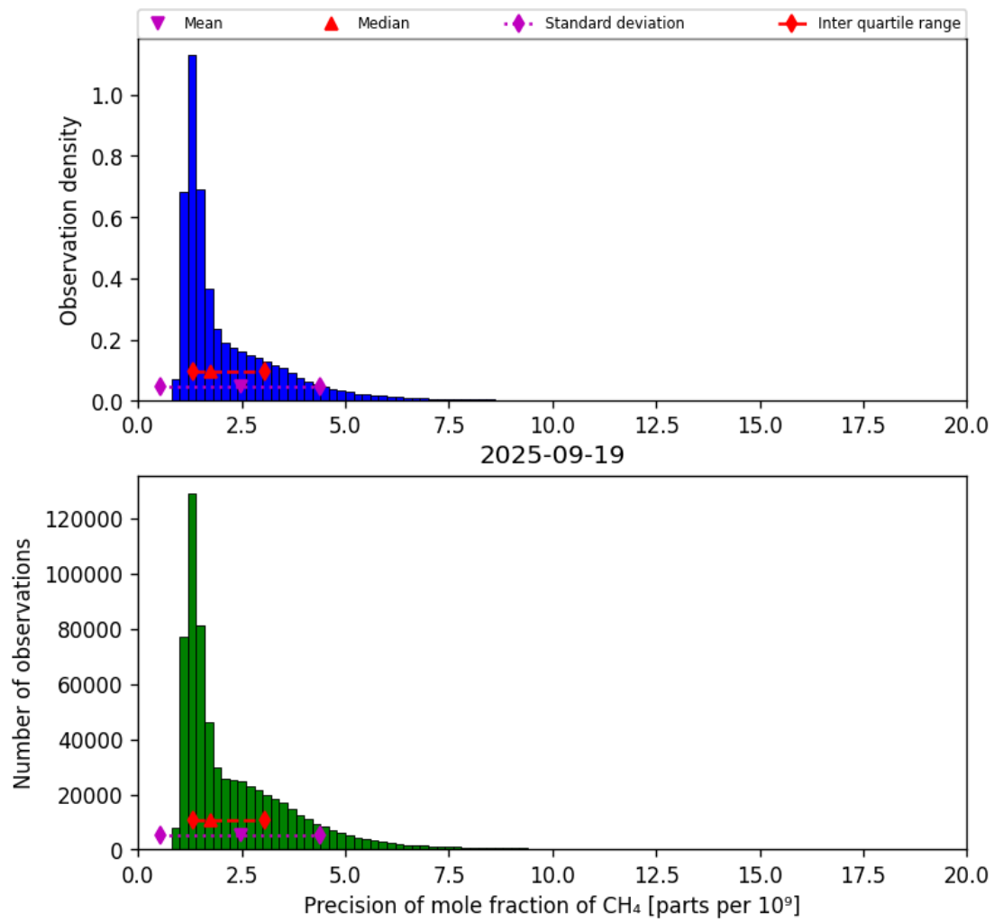
Figure 24: Histogram of “Precision of mole fraction of CH 4 ” for 2025-09-18 to 2025-09-20
