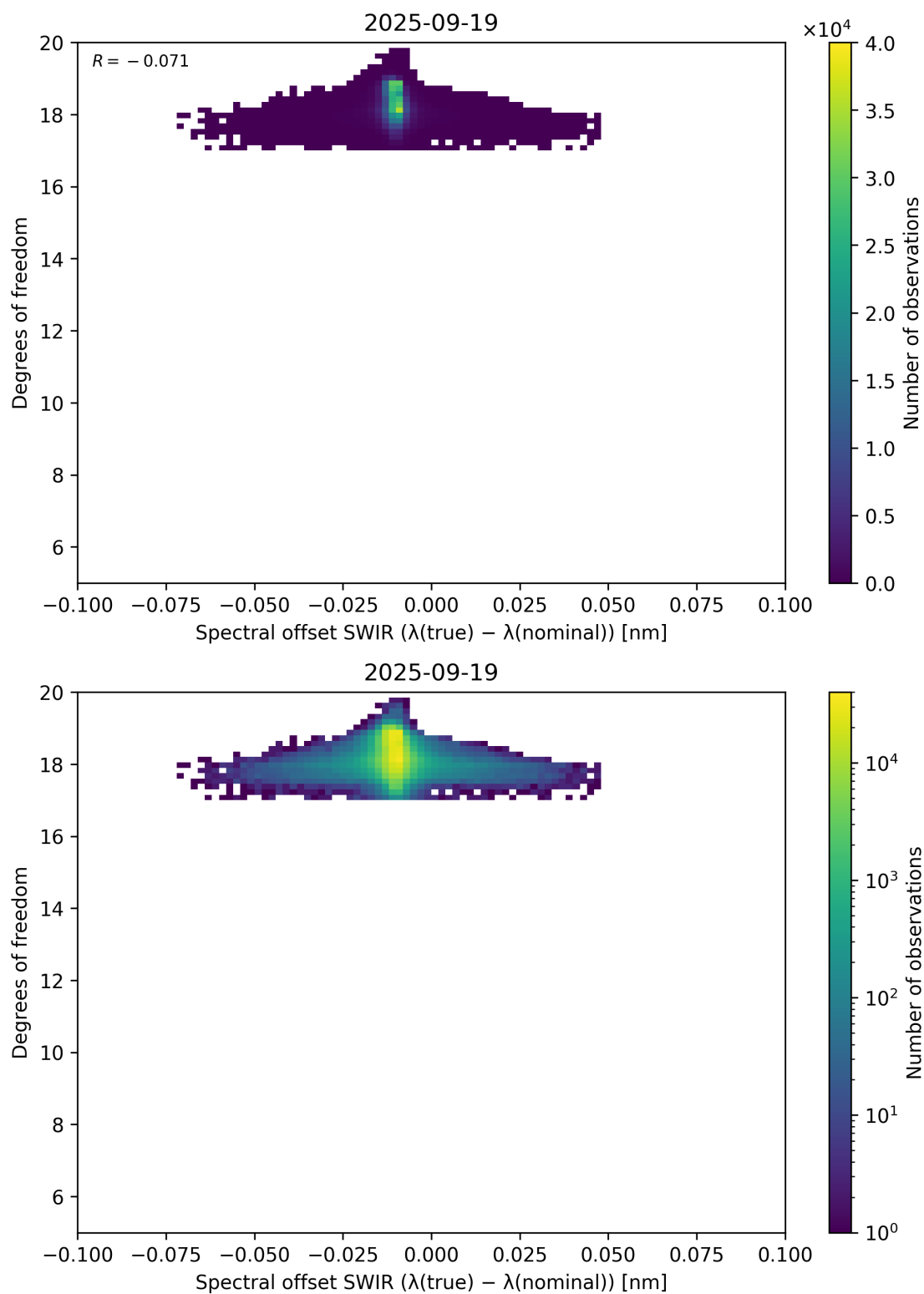
Figure 119: Scatter density plot of “Spectral offset SWIR ( \lambda_{\text{true}} - \lambda_{\text{nominal}} )” against “Degrees of freedom” for 2025-09-18 to 2025-09-20.
