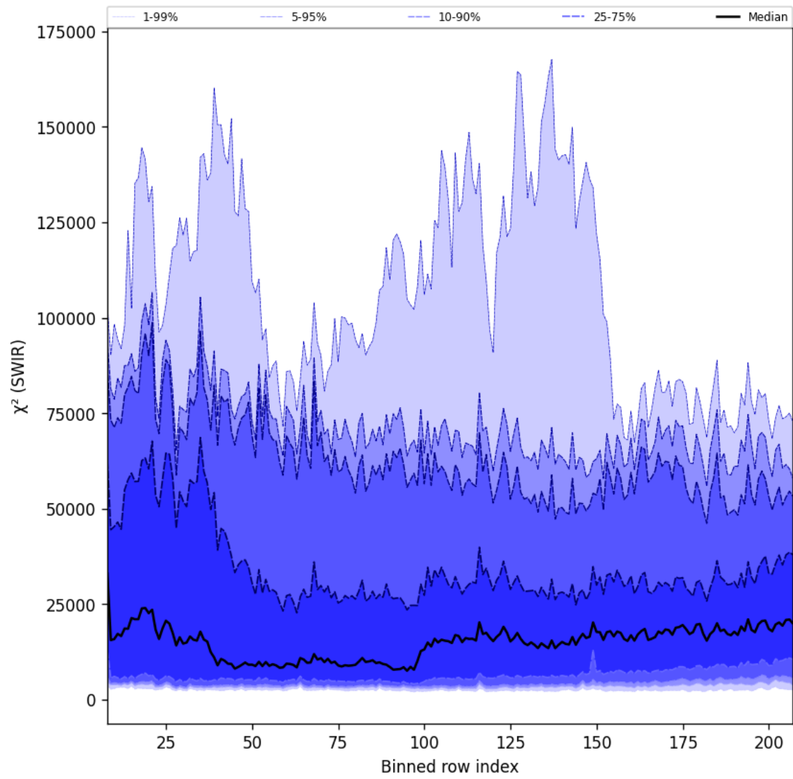
Figure 39: Along track statistics of “ \chi^2 (SWIR)” for 2025-09-18 to 2025-09-20
