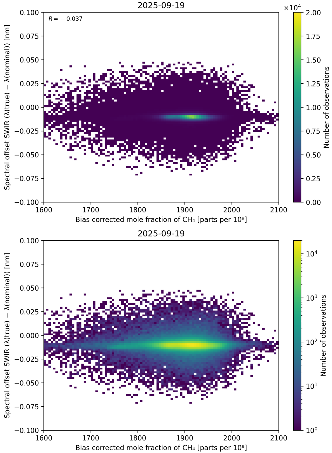
Figure 69: Scatter density plot of “Bias corrected mole fraction of \text{CH}_4 ” against “Spectral offset SWIR ( \lambda_{\text{true}} - \lambda_{\text{nominal}} )” for 2025-09-18 to 2025-09-20.
