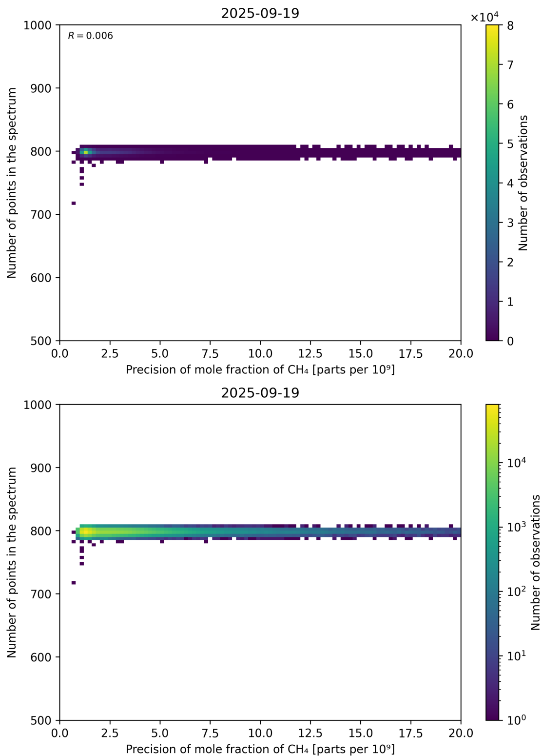
Figure 84: Scatter density plot of “Precision of mole fraction of CH 4 ” against “Number of points in the spectrum” for 2025-09-18 to 2025-09-20.
