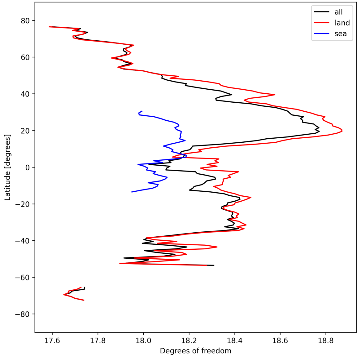
Figure 19: Zonal average of “Degrees of freedom” for 2025-09-18 to 2025-09-20.
