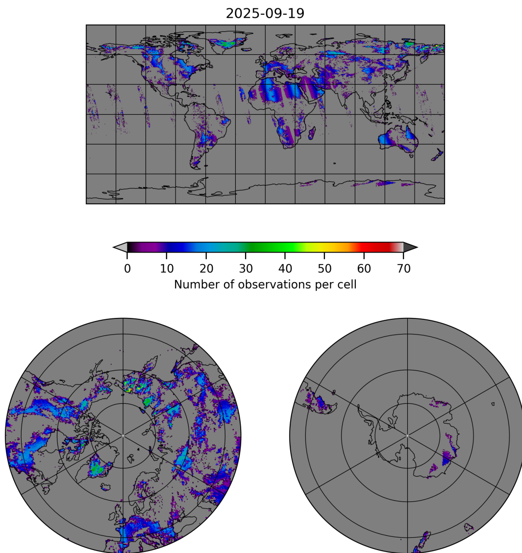
Figure 10: Map of the number of observations for 2025-09-18 to 2025-09-20
