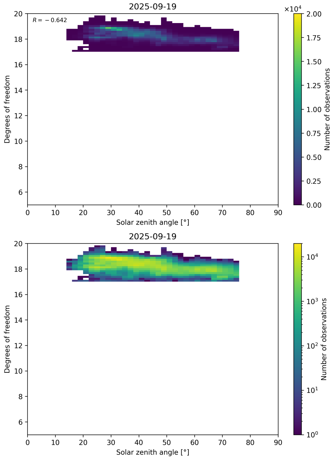
Figure 96: Scatter density plot of “Solar zenith angle” against “Degrees of freedom” for 2025-09-18 to 2025-09-20.
