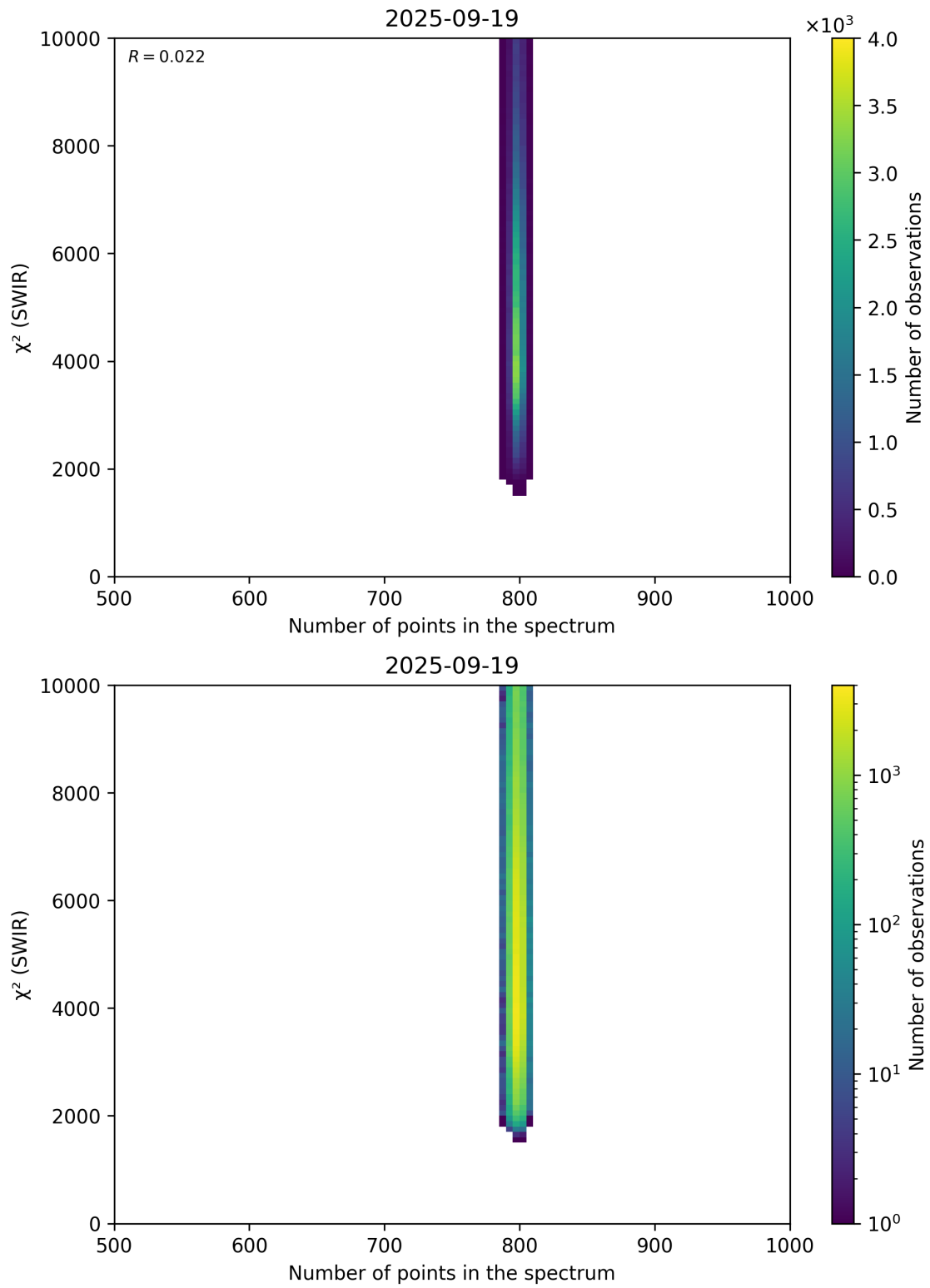
Figure 89: Scatter density plot of “Number of points in the spectrum” against “ \chi^2 (SWIR)” for 2025-09-18 to 2025-09-20.
