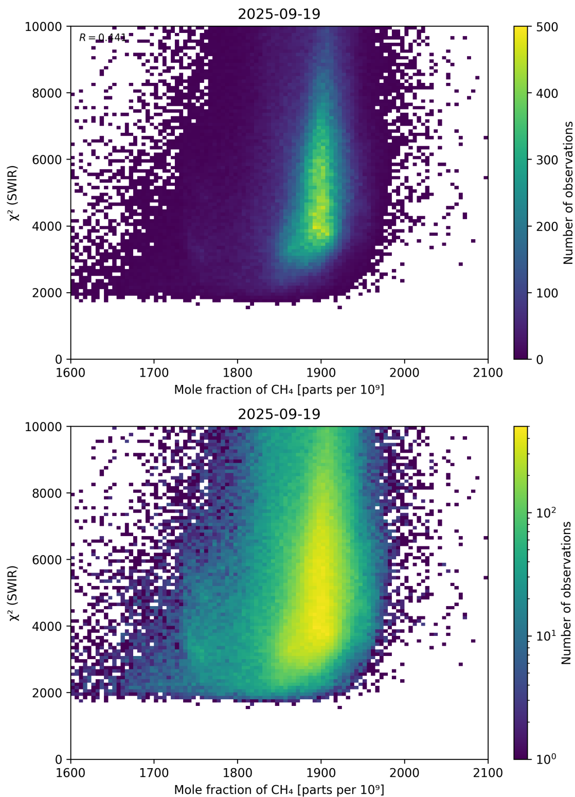
Figure 71: Scatter density plot of “Mole fraction of \text{CH}_4 ” against “ \chi^2 (SWIR)” for 2025-09-18 to 2025-09-20.
