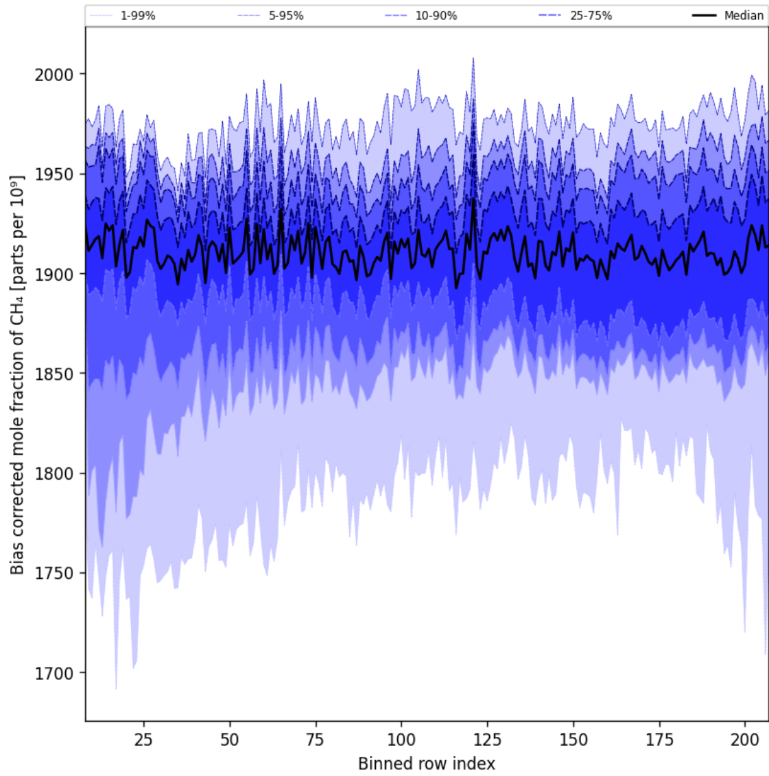
Figure 36: Along track statistics of “Bias corrected mole fraction of \text{CH}_4 ” for 2025-09-18 to 2025-09-20
