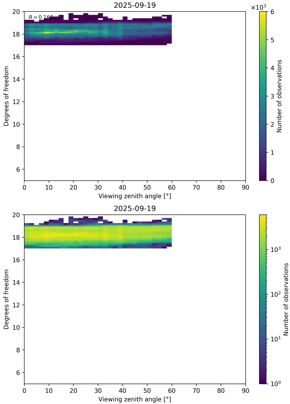
Figure 107: Scatter density plot of “Viewing zenith angle” against “Degrees of freedom” for 2025-09-18 to 2025-09-20.
