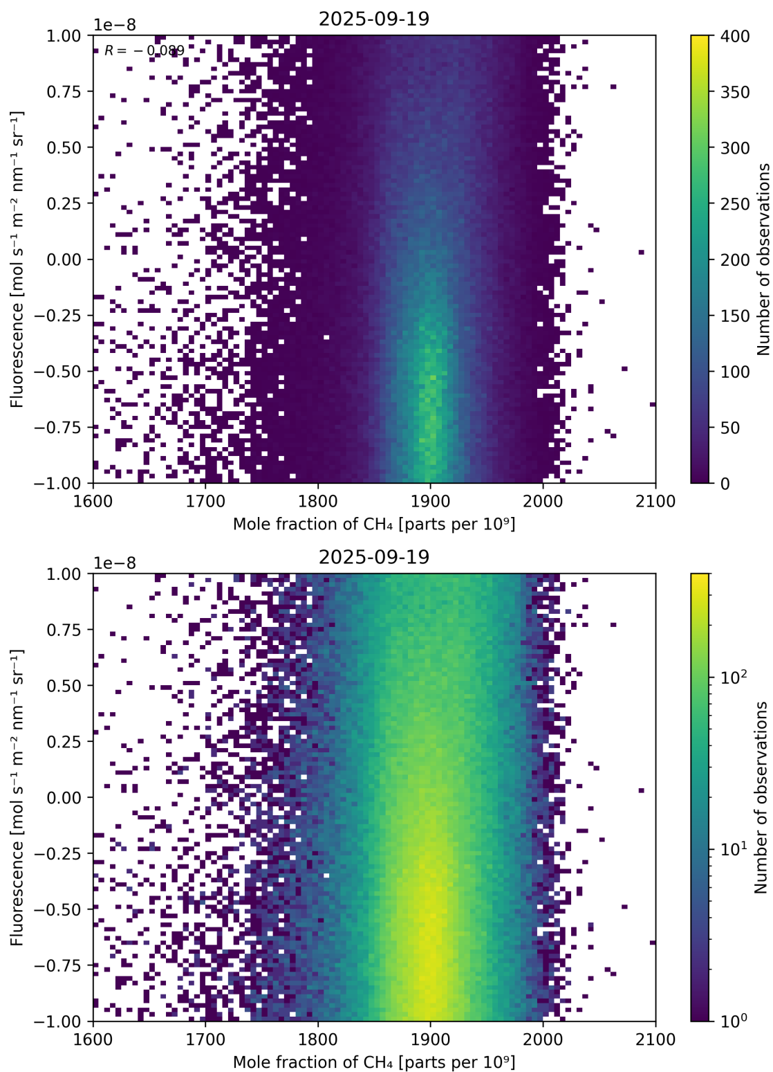
Figure 73: Scatter density plot of “Mole fraction of \text{CH}_4 ” against “Fluorescence” for 2025-09-18 to 2025-09-20.
