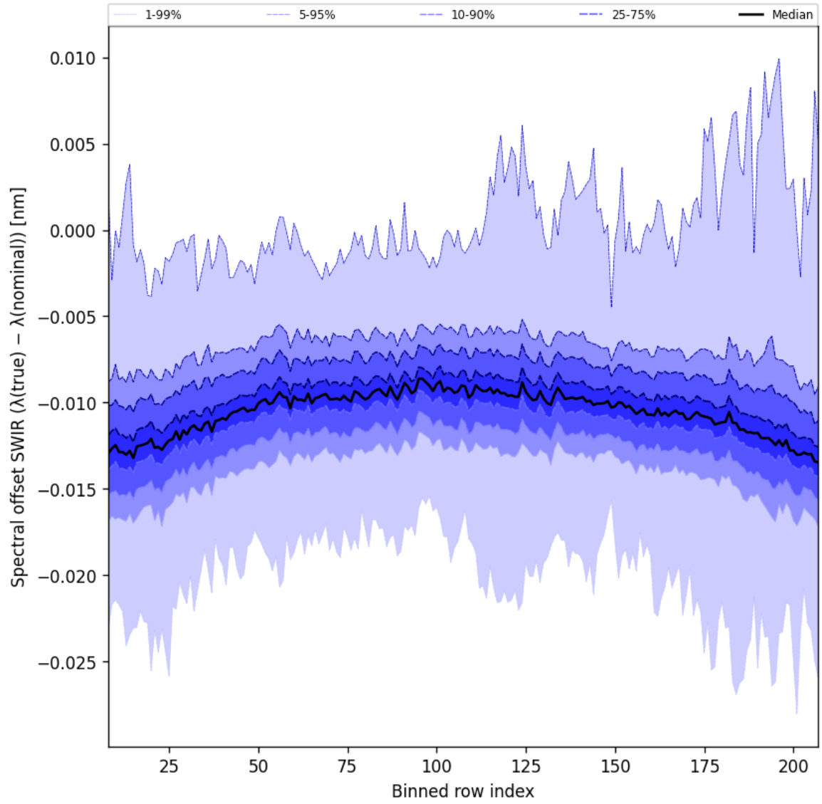
Figure 38: Along track statistics of “Spectral offset SWIR ( \lambda_{\text{true}} - \lambda_{\text{nominal}} )” for 2025-09-18 to 2025-09-20
