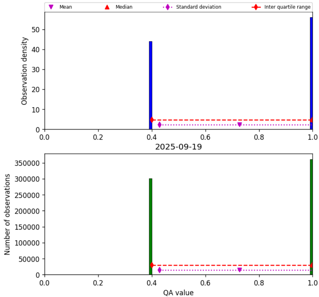
Figure 22: Histogram of “QA value” for 2025-09-18 to 2025-09-20
