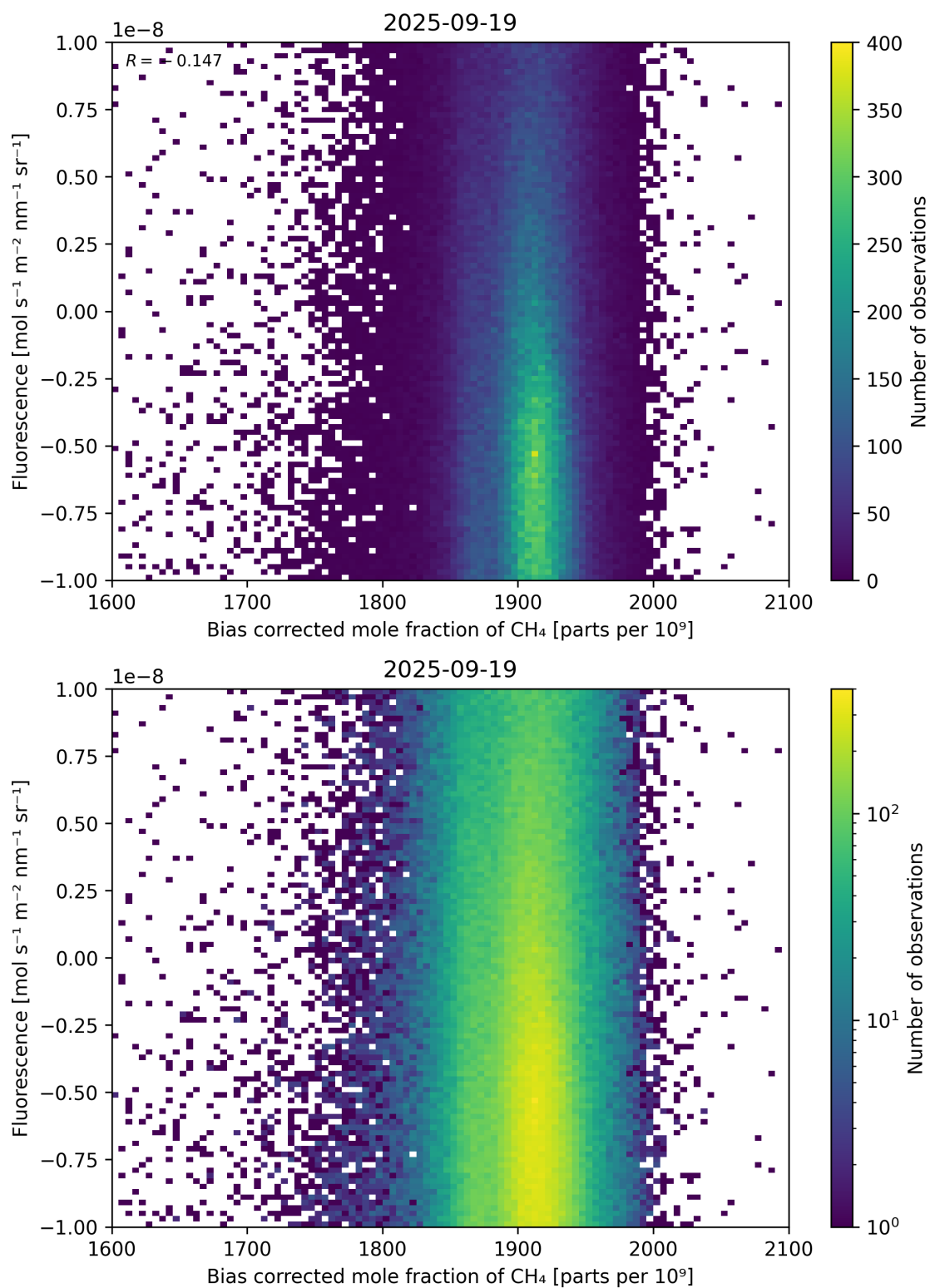
Figure 66: Scatter density plot of “Bias corrected mole fraction of \text{CH}_4 ” against “Fluorescence” for 2025-09-18 to 2025-09-20.
