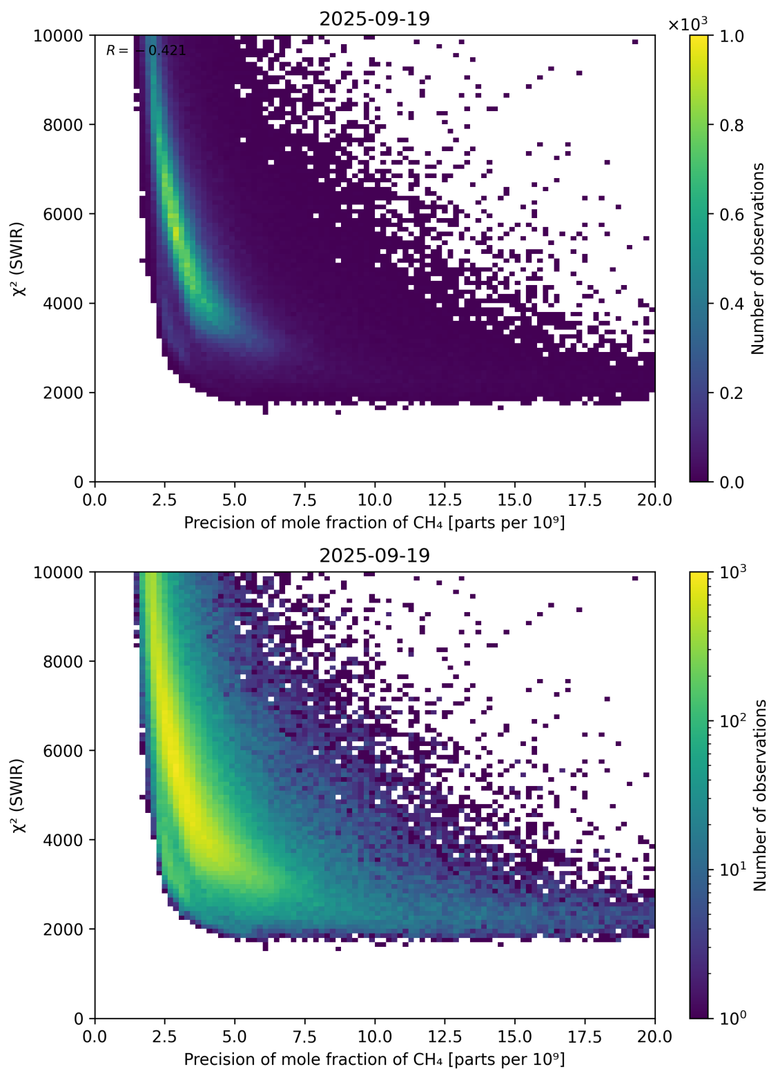
Figure 79: Scatter density plot of “Precision of mole fraction of CH 4 ” against “ \chi^2 (SWIR)” for 2025-09-18 to 2025-09-20.
