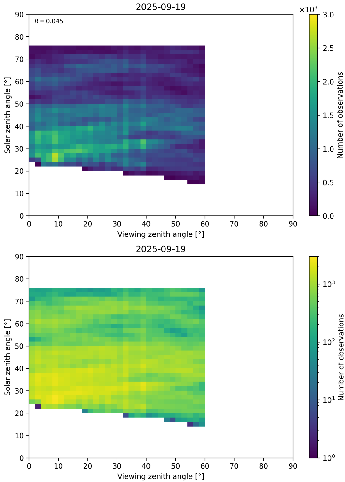
Figure 115: Scatter density plot of “Viewing zenith angle” against “Solar zenith angle” for 2025-09-18 to 2025-09-20.
