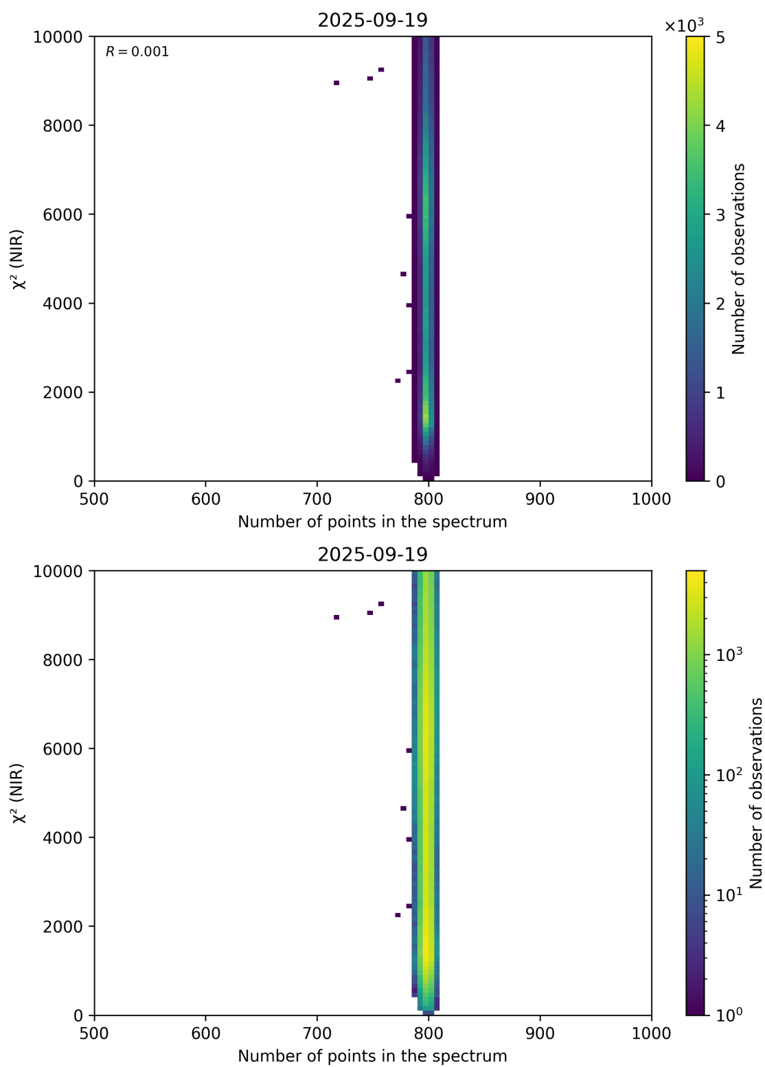
Figure 88: Scatter density plot of “Number of points in the spectrum” against “ \chi^2 (NIR)” for 2025-09-18 to 2025-09-20.
