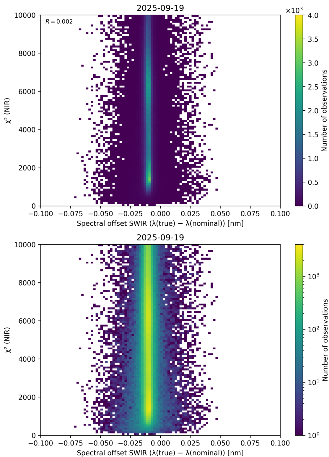
Figure 117: Scatter density plot of “Spectral offset SWIR ( \lambda_{\text{true}} - \lambda_{\text{nominal}} )” against “ \chi^2 (NIR)” for 2025-09-18 to 2025-09-20.
