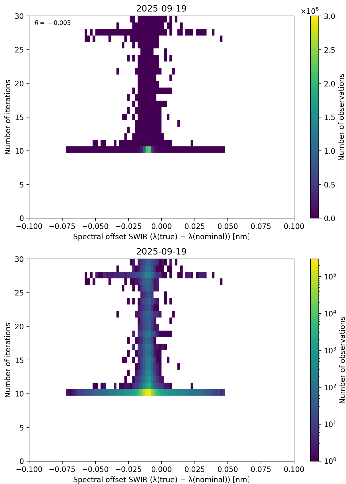
Figure 121: Scatter density plot of “Spectral offset SWIR ( \lambda_{\text{true}} - \lambda_{\text{nominal}} )” against “Number of iterations” for 2025-09-18 to 2025-09-20.
