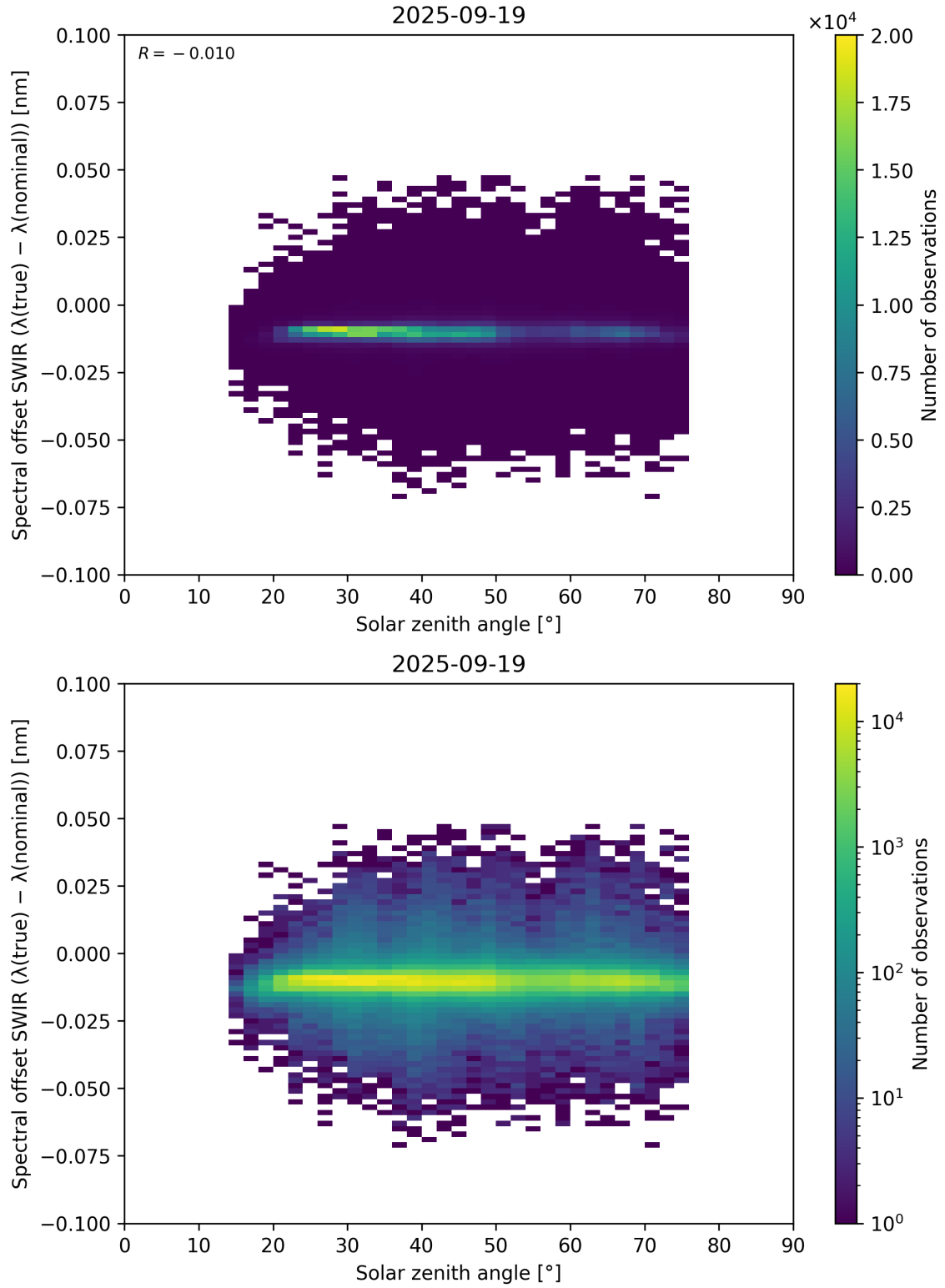
Figure 104: Scatter density plot of “Solar zenith angle” against “Spectral offset SWIR ( \lambda_{\text{true}} - \lambda_{\text{nominal}} )” for 2025-09-18 to 2025-09-20.
