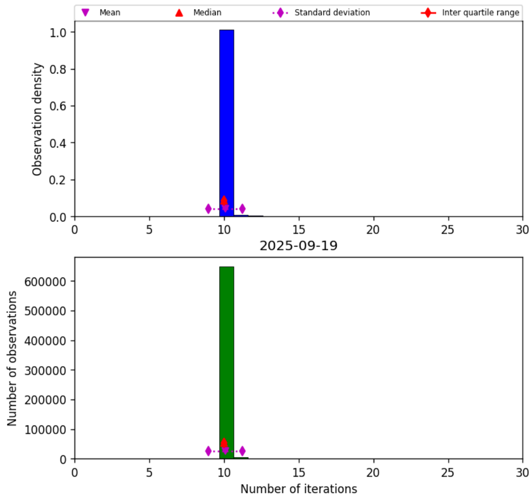
Figure 31: Histogram of “Number of iterations” for 2025-09-18 to 2025-09-20
