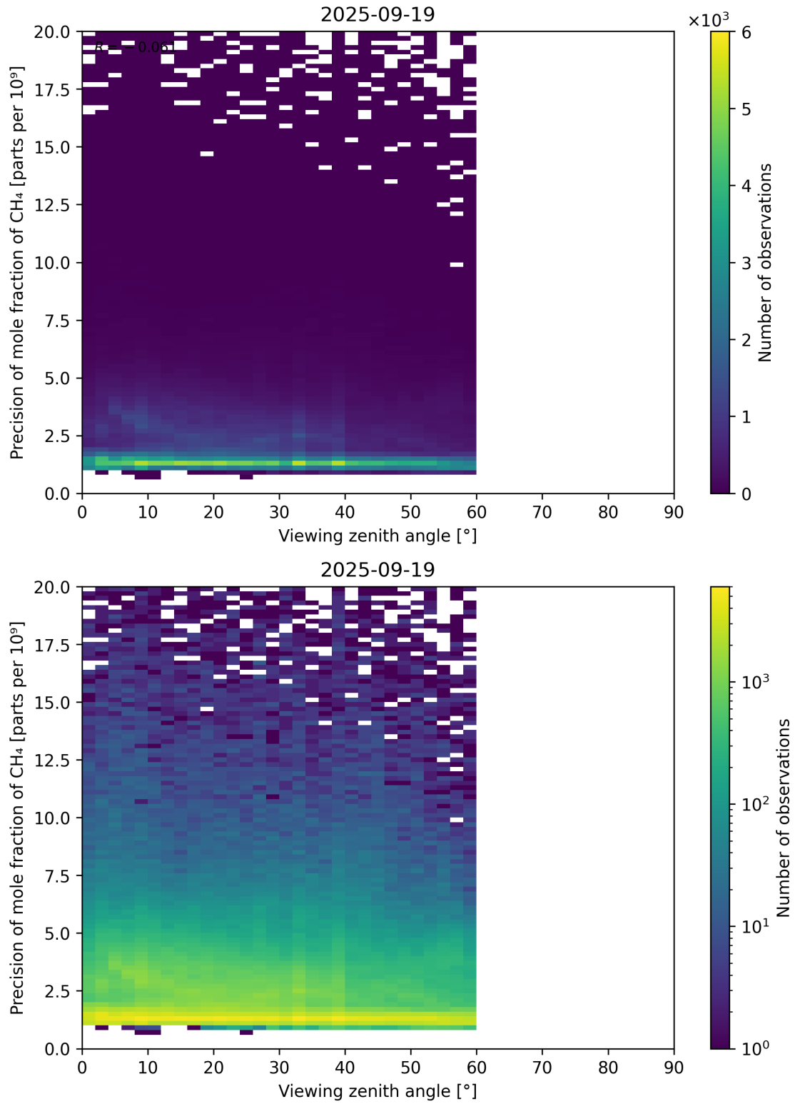
Figure 112: Scatter density plot of “Viewing zenith angle” against “Precision of mole fraction of CH 4 ” for 2025-09-18 to 2025-09-20.
