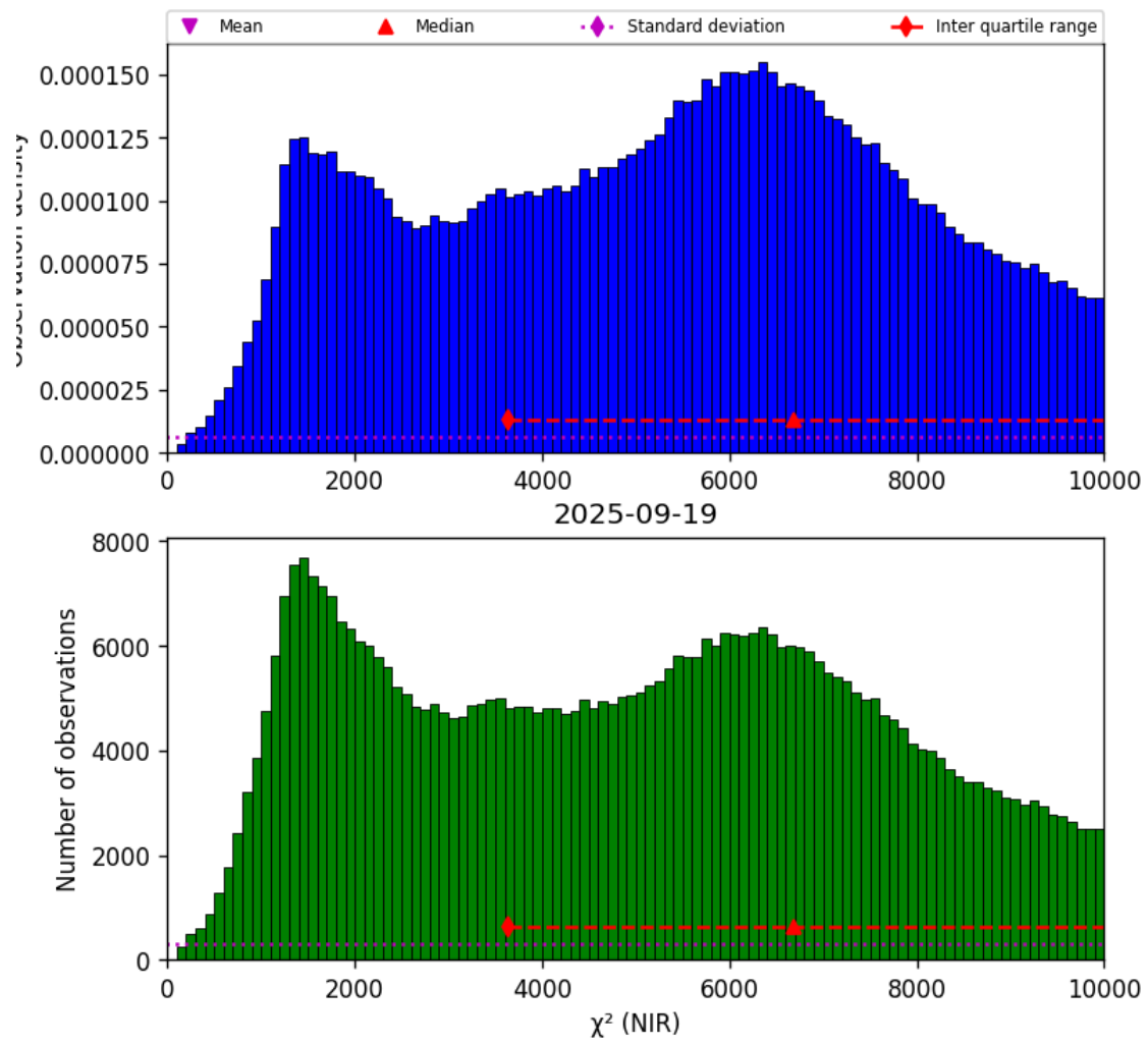
Figure 29: Histogram of “ \chi^2 (NIR)” for 2025-09-18 to 2025-09-20
