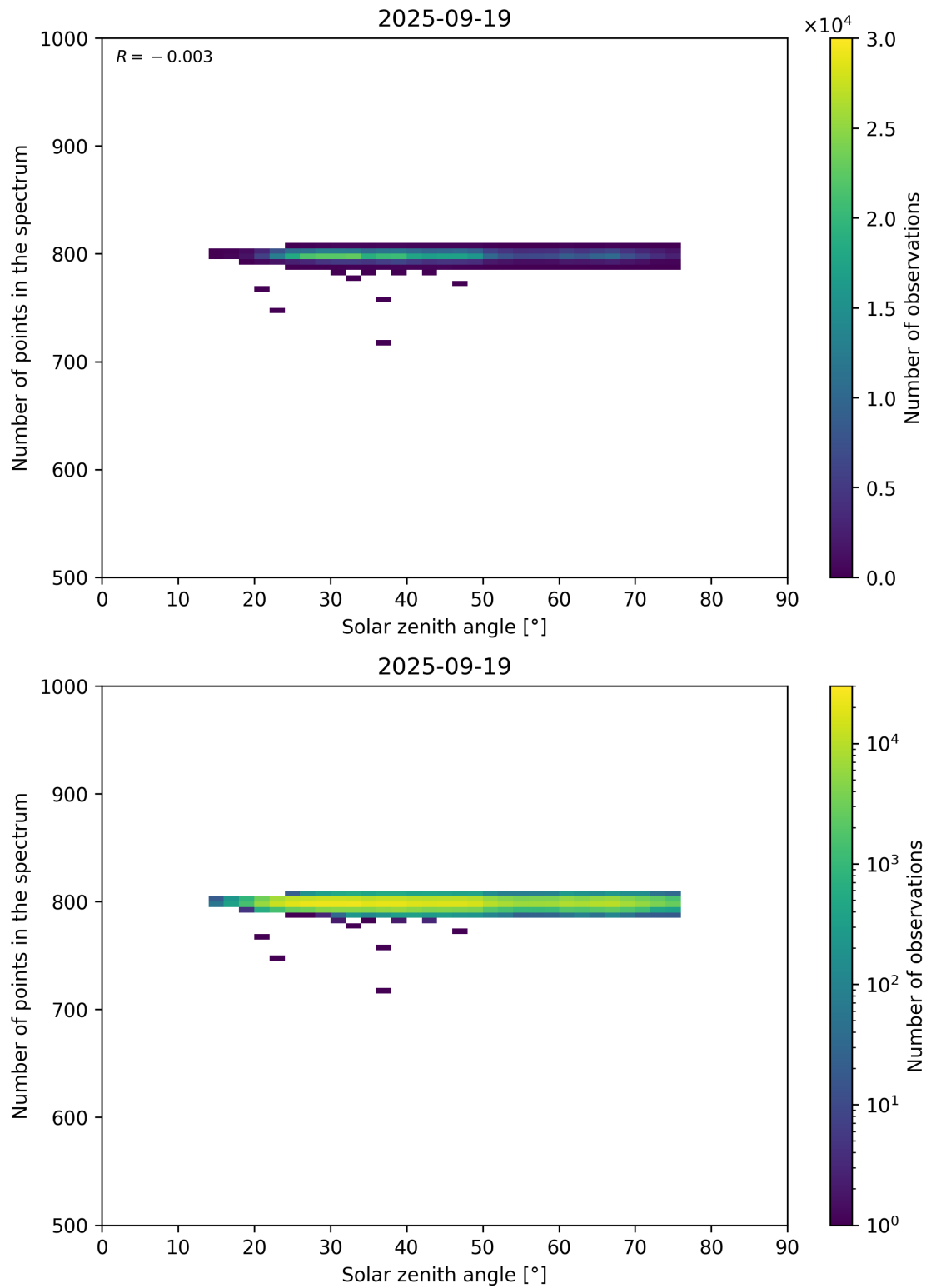
Figure 103: Scatter density plot of “Solar zenith angle” against “Number of points in the spectrum” for 2025-09-18 to 2025-09-20.
