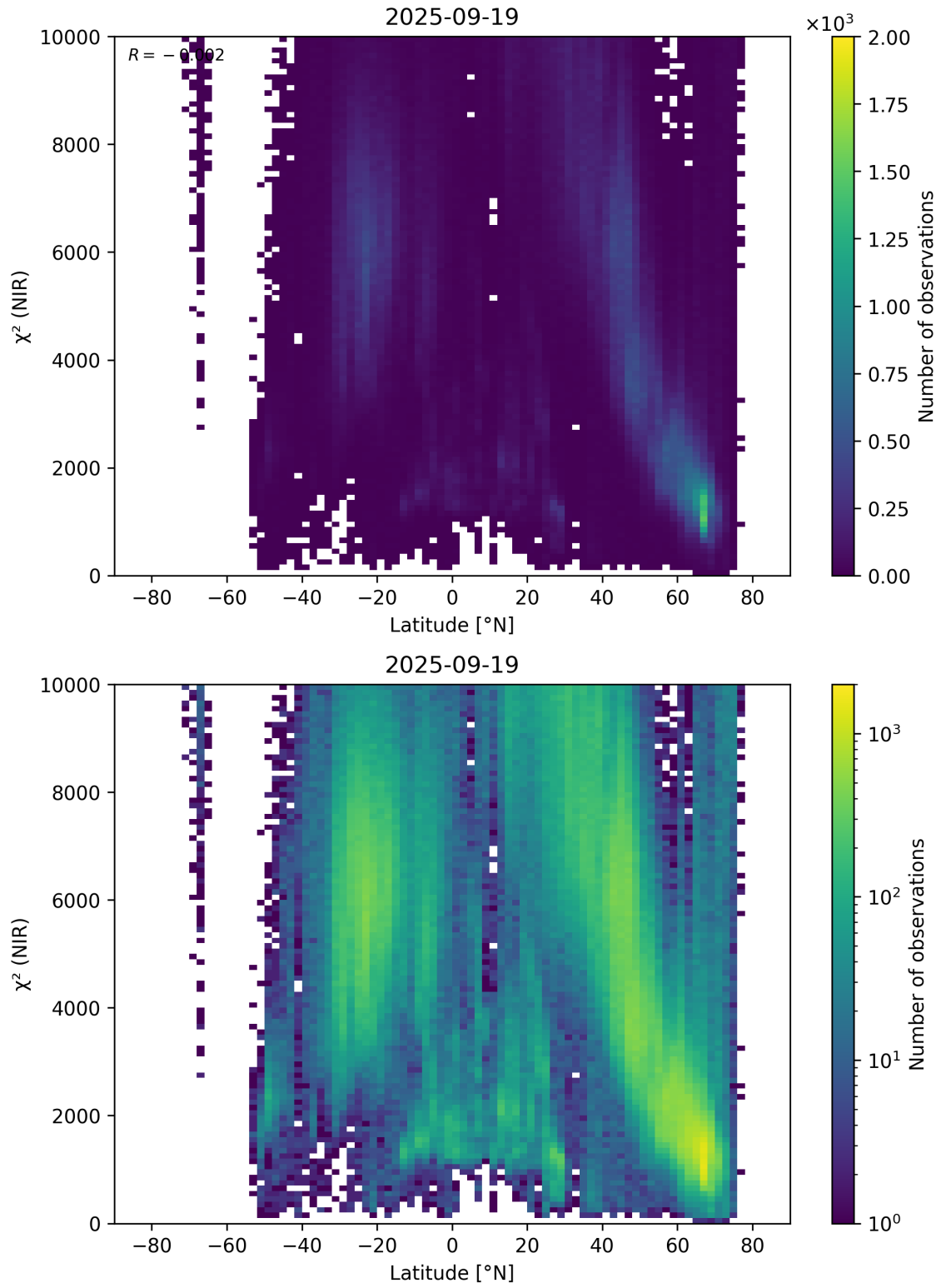
Figure 53: Scatter density plot of “Latitude” against “ \chi^2 (NIR)” for 2025-09-18 to 2025-09-20.
