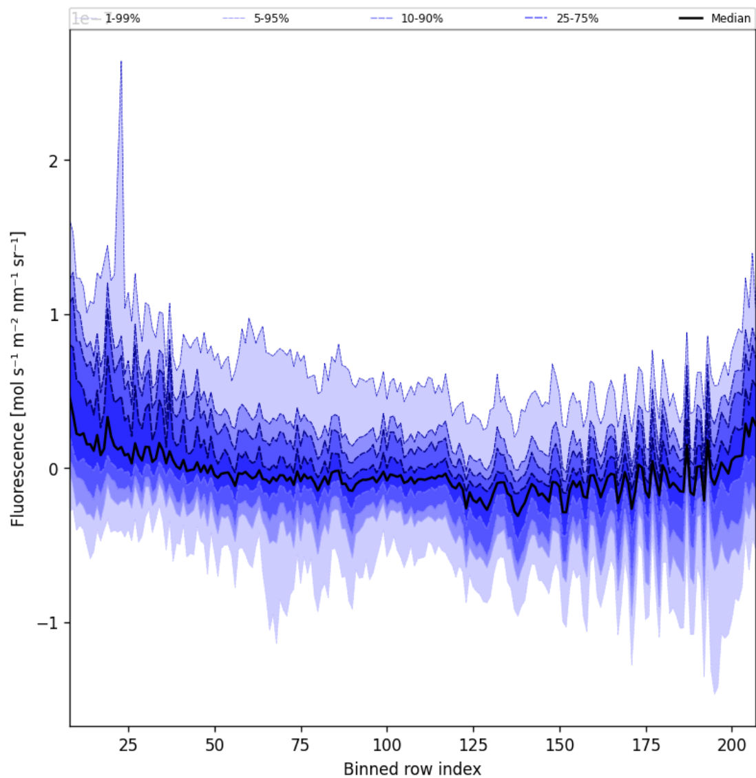
Figure 43: Along track statistics of “Fluorescence” for 2025-09-18 to 2025-09-20
