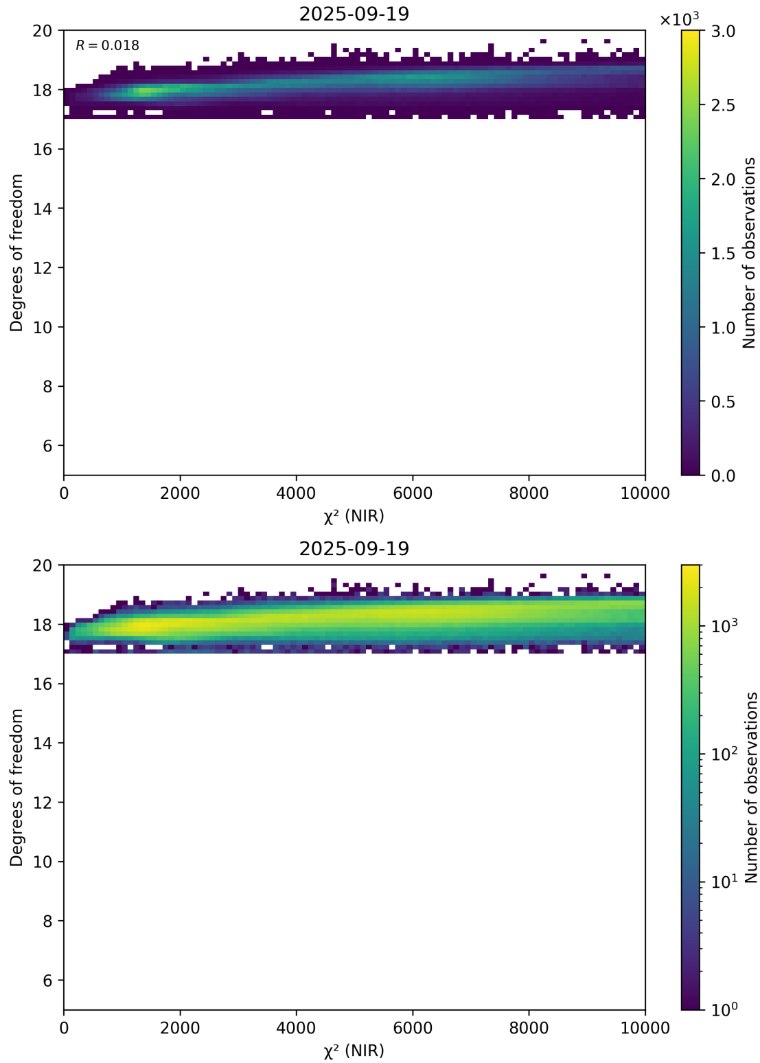
Figure 44: Scatter density plot of “ \chi^2 (NIR)” against “Degrees of freedom” for 2025-09-18 to 2025-09-20.
