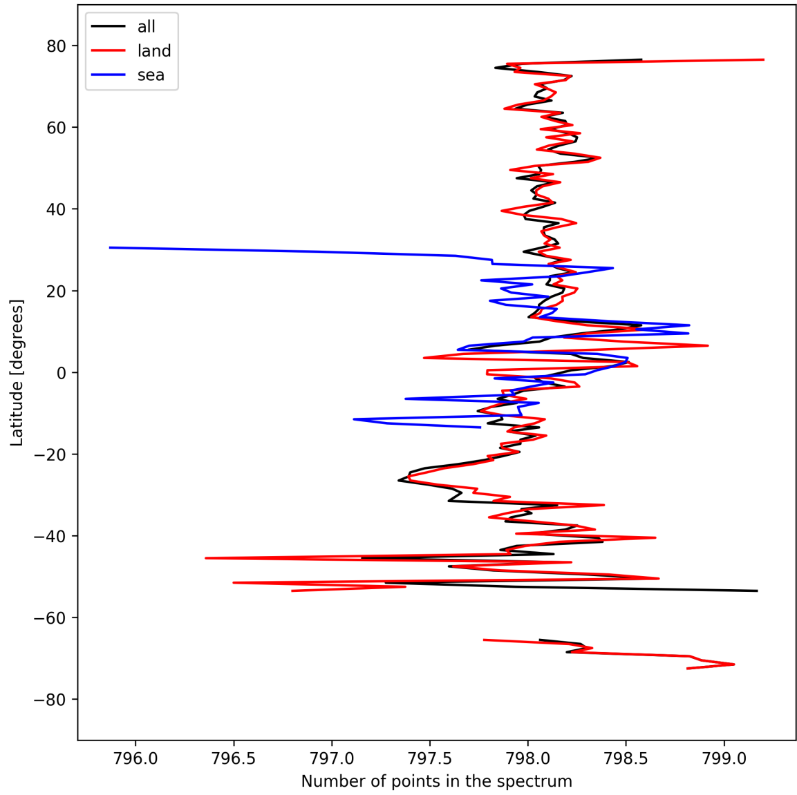
Figure 15: Zonal average of “Number of points in the spectrum” for 2025-09-18 to 2025-09-20.
