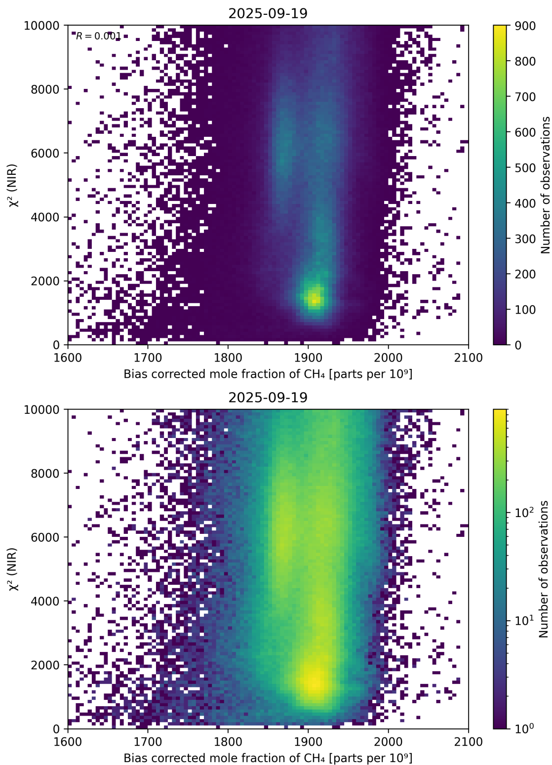
Figure 63: Scatter density plot of “Bias corrected mole fraction of CH 4 ” against “ \chi^2 (NIR)” for 2025-09-18 to 2025-09-20.
