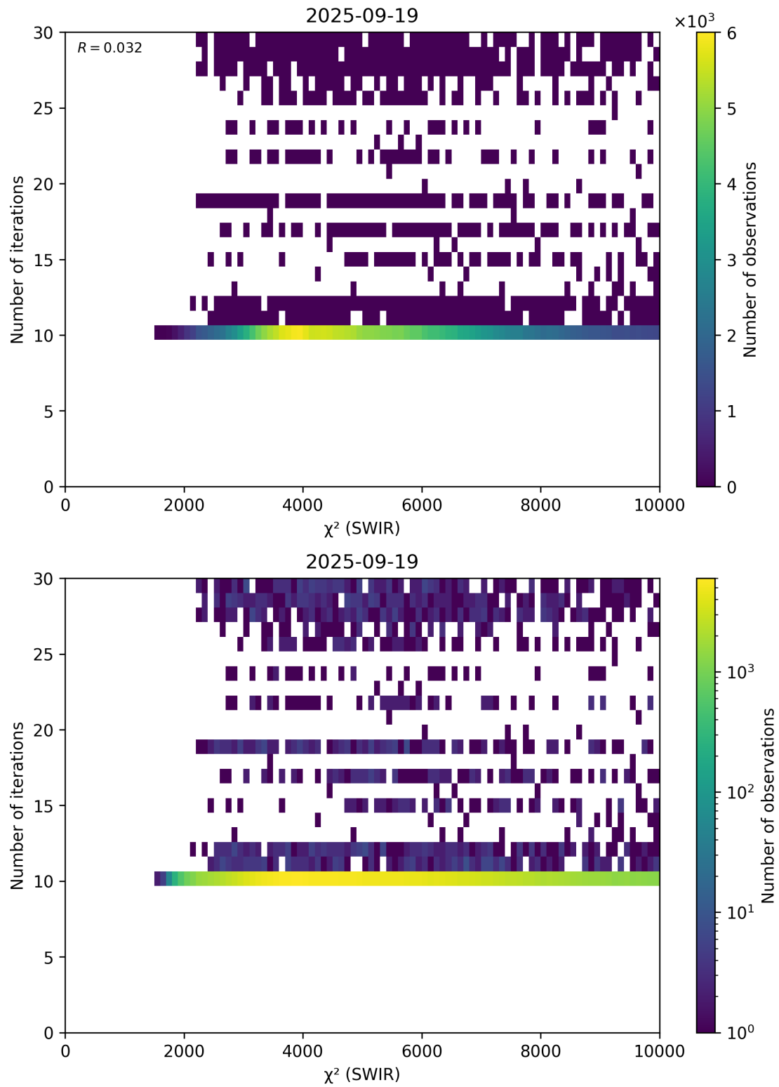
Figure 50: Scatter density plot of “ \chi^2 (SWIR)” against “Number of iterations” for 2025-09-18 to 2025-09-20.
