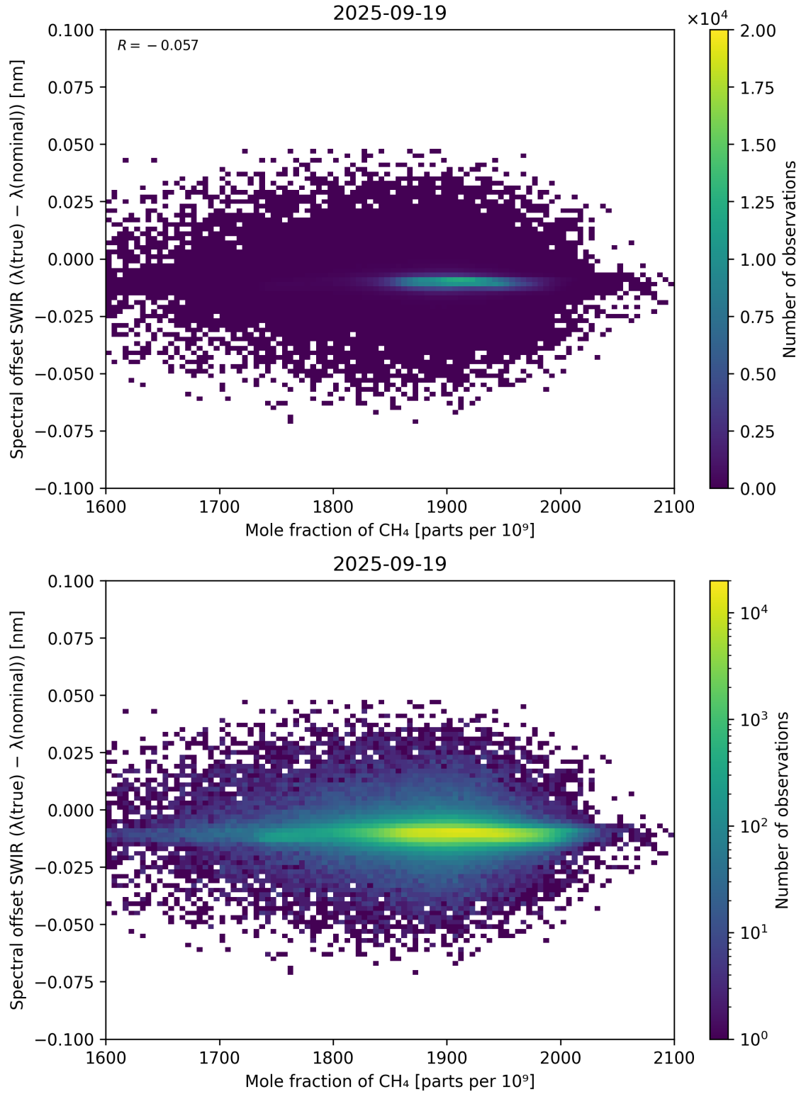
Figure 86: Scatter density plot of “Mole fraction of CH 4 ” against “Spectral offset SWIR ( \lambda_{\text{true}} - \lambda_{\text{nominal}} )” for 2025-09-18 to 2025-09-20.
