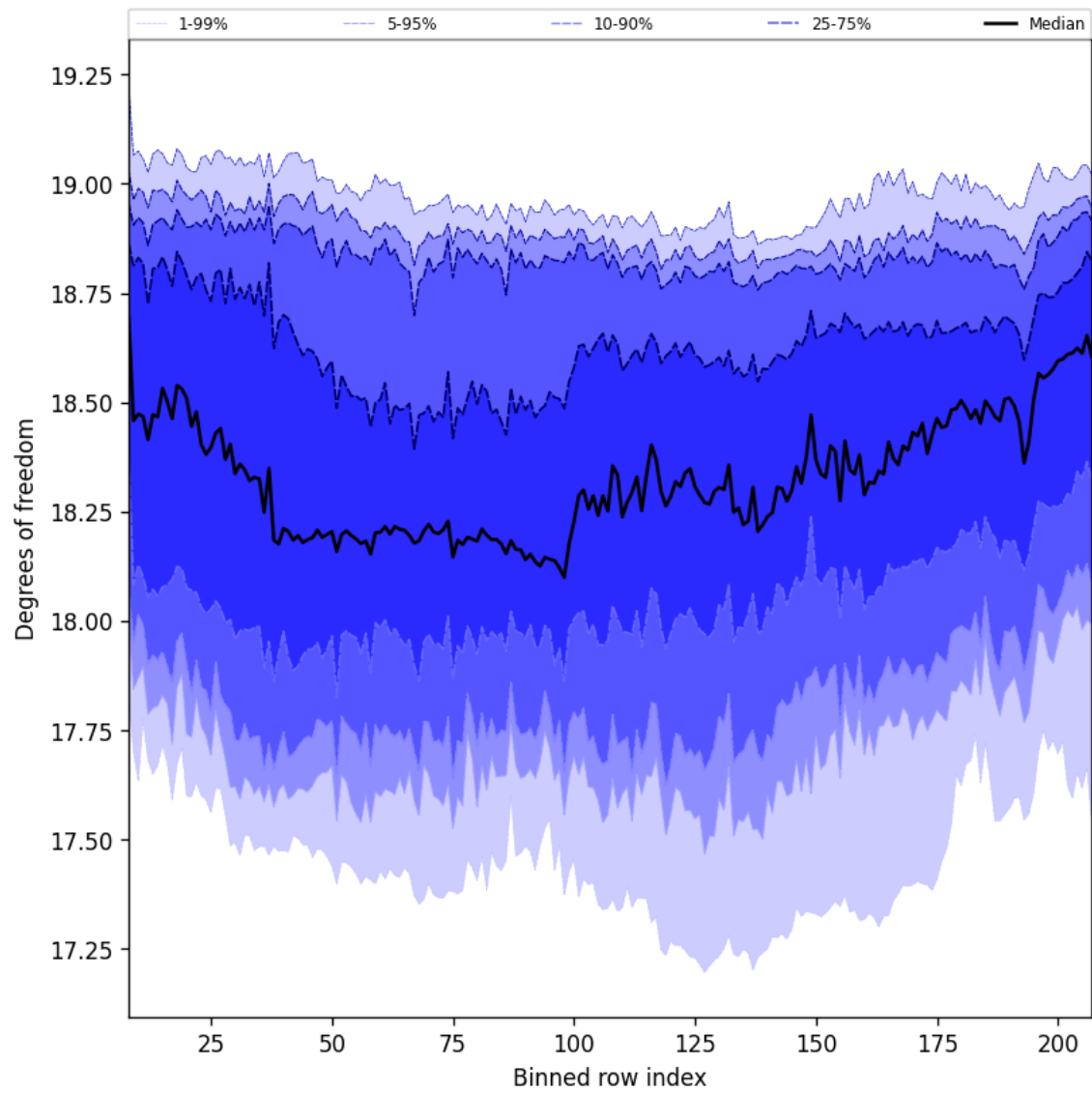
Figure 41: Along track statistics of “Degrees of freedom” for 2025-09-18 to 2025-09-20
