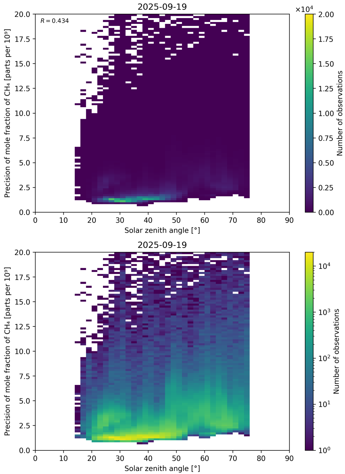
Figure 101: Scatter density plot of “Solar zenith angle” against “Precision of mole fraction of \text{CH}_4 ” for 2025-09-18 to 2025-09-20.
