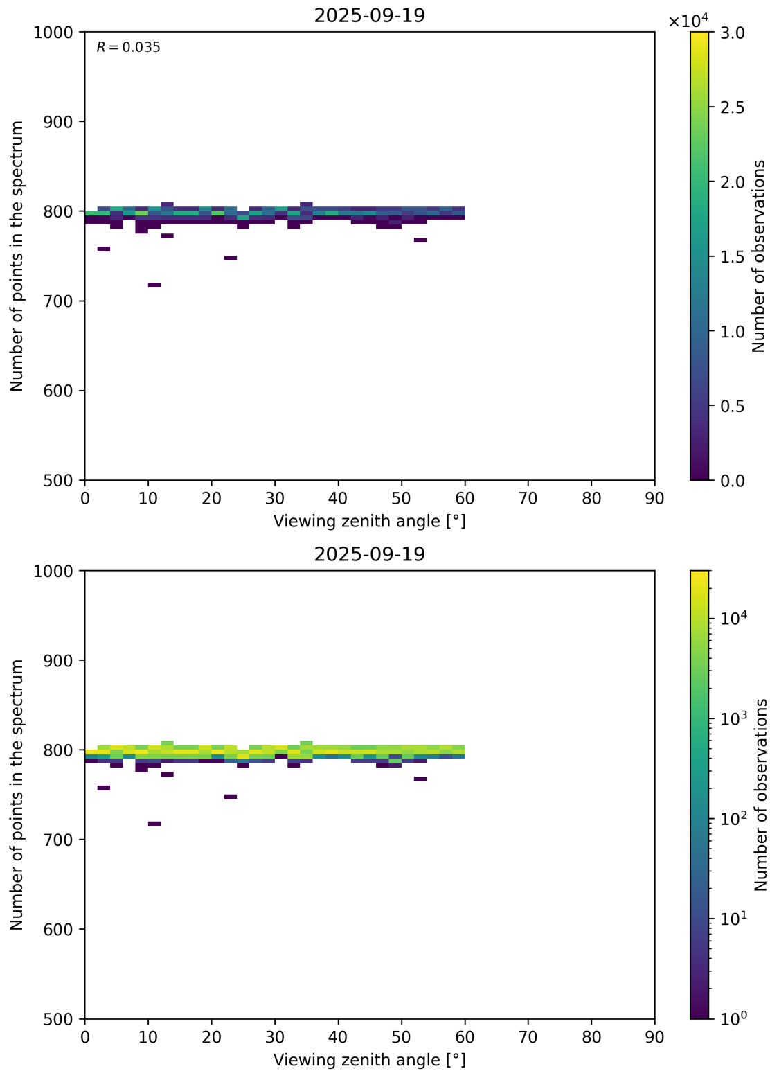
Figure 114: Scatter density plot of “Viewing zenith angle” against “Number of points in the spectrum” for 2025-09-18 to 2025-09-20.
