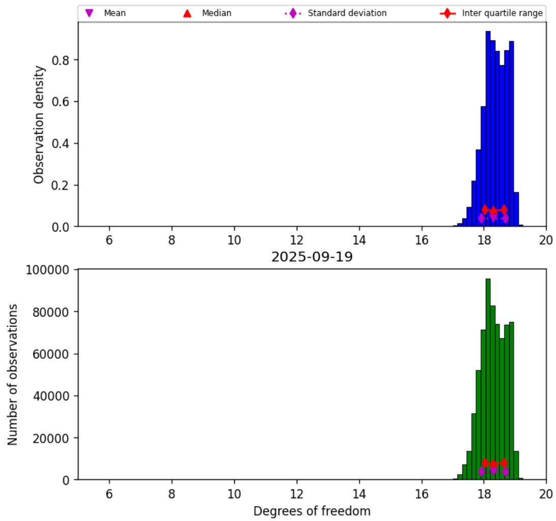
Figure 30: Histogram of “Degrees of freedom” for 2025-09-18 to 2025-09-20
