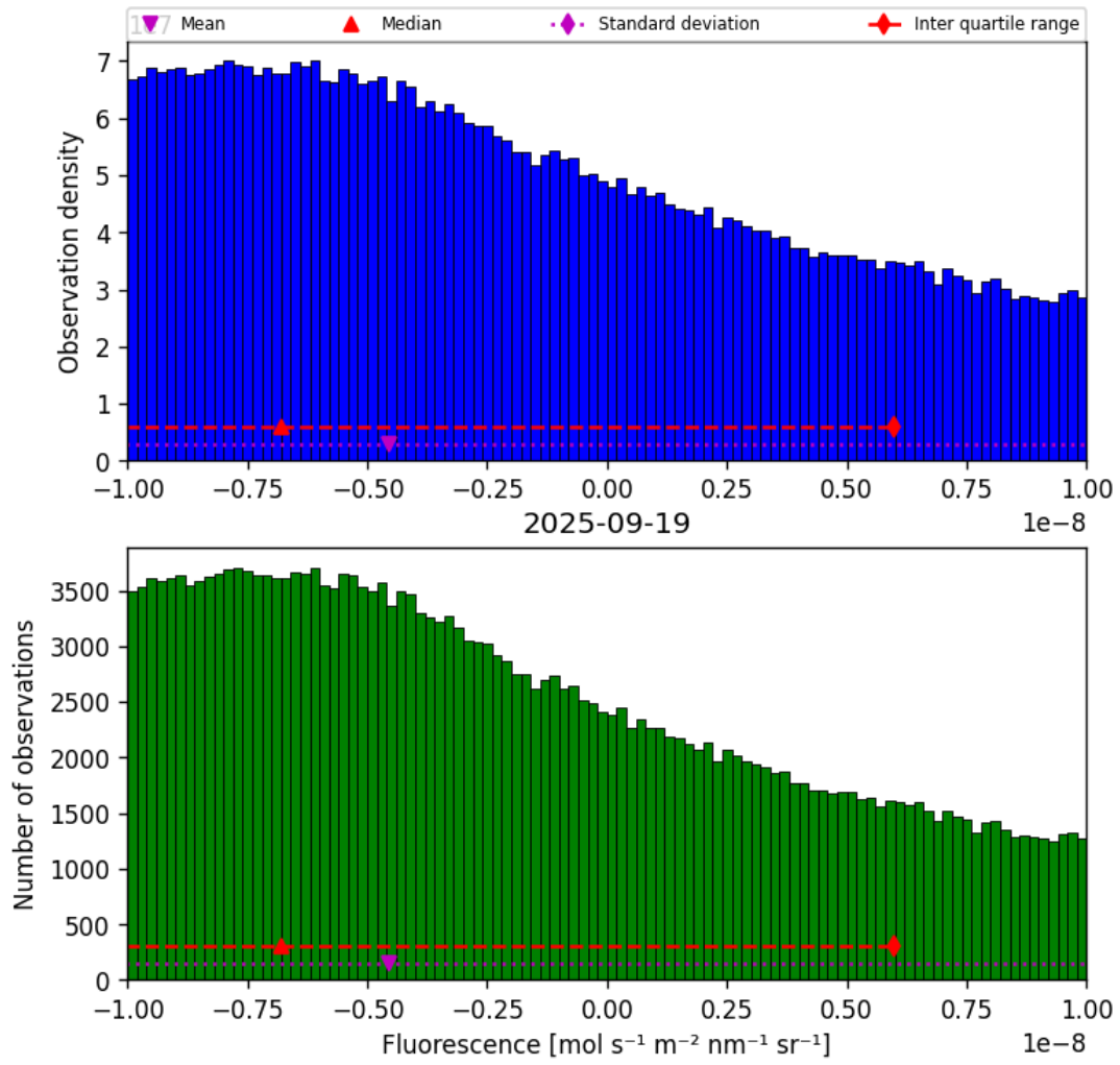
Figure 32: Histogram of “Fluorescence” for 2025-09-18 to 2025-09-20
