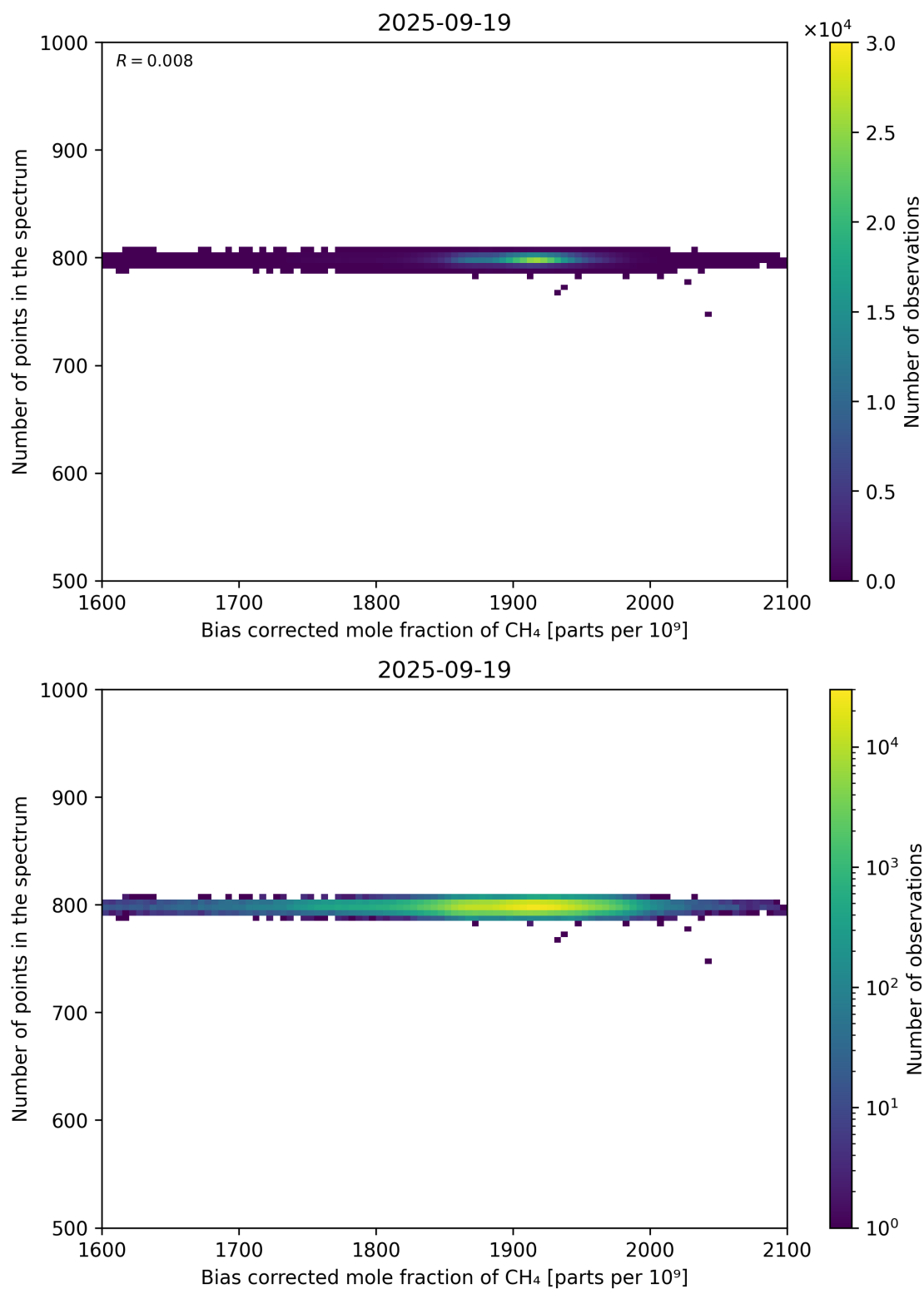
Figure 68: Scatter density plot of “Bias corrected mole fraction of CH 4 ” against “Number of points in the spectrum” for 2025-09-18 to 2025-09-20.
