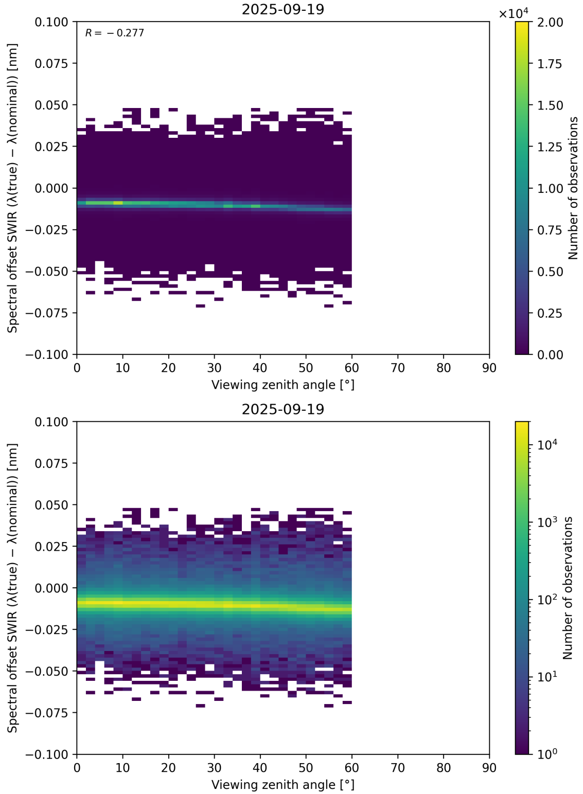
Figure 116: Scatter density plot of “Viewing zenith angle” against “Spectral offset SWIR ( \lambda_{\text{true}} - \lambda_{\text{nominal}} )” for 2025-09-18 to 2025-09-20.
