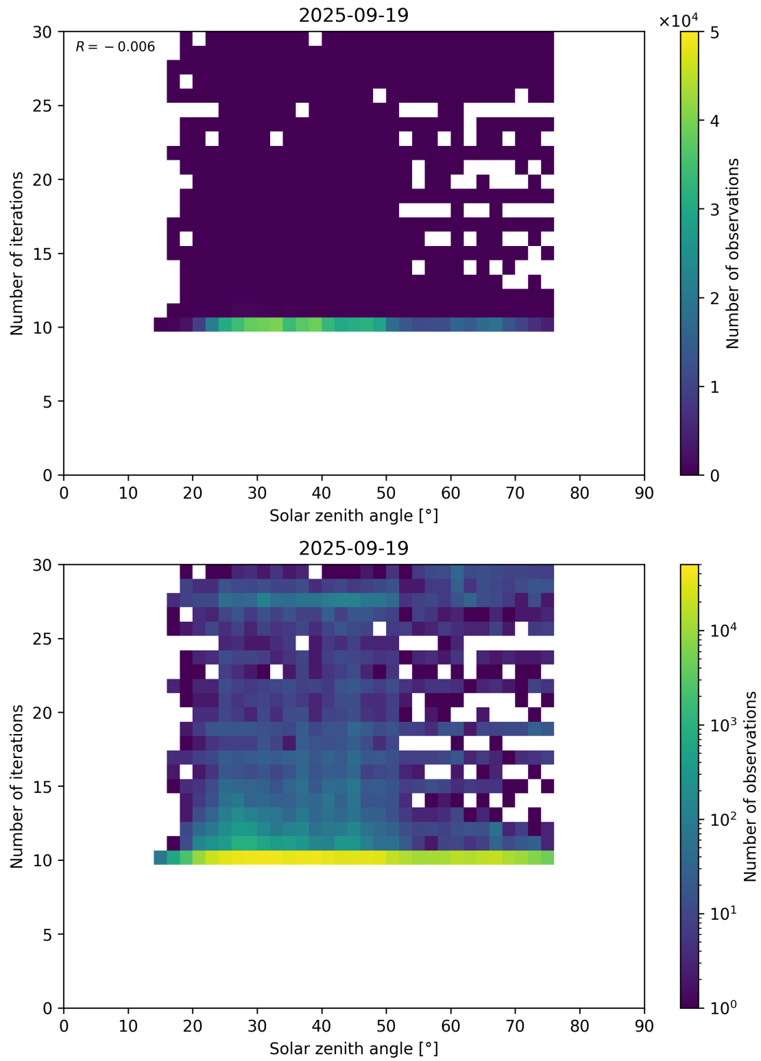
Figure 102: Scatter density plot of “Solar zenith angle” against “Number of iterations” for 2025-09-18 to 2025-09-20.
