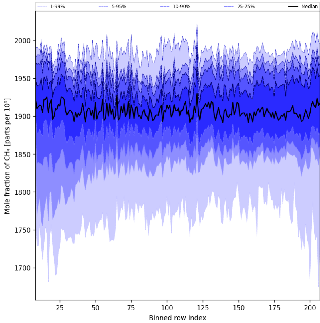
Figure 34: Along track statistics of “Mole fraction of CH 4 ” for 2025-09-18 to 2025-09-20
