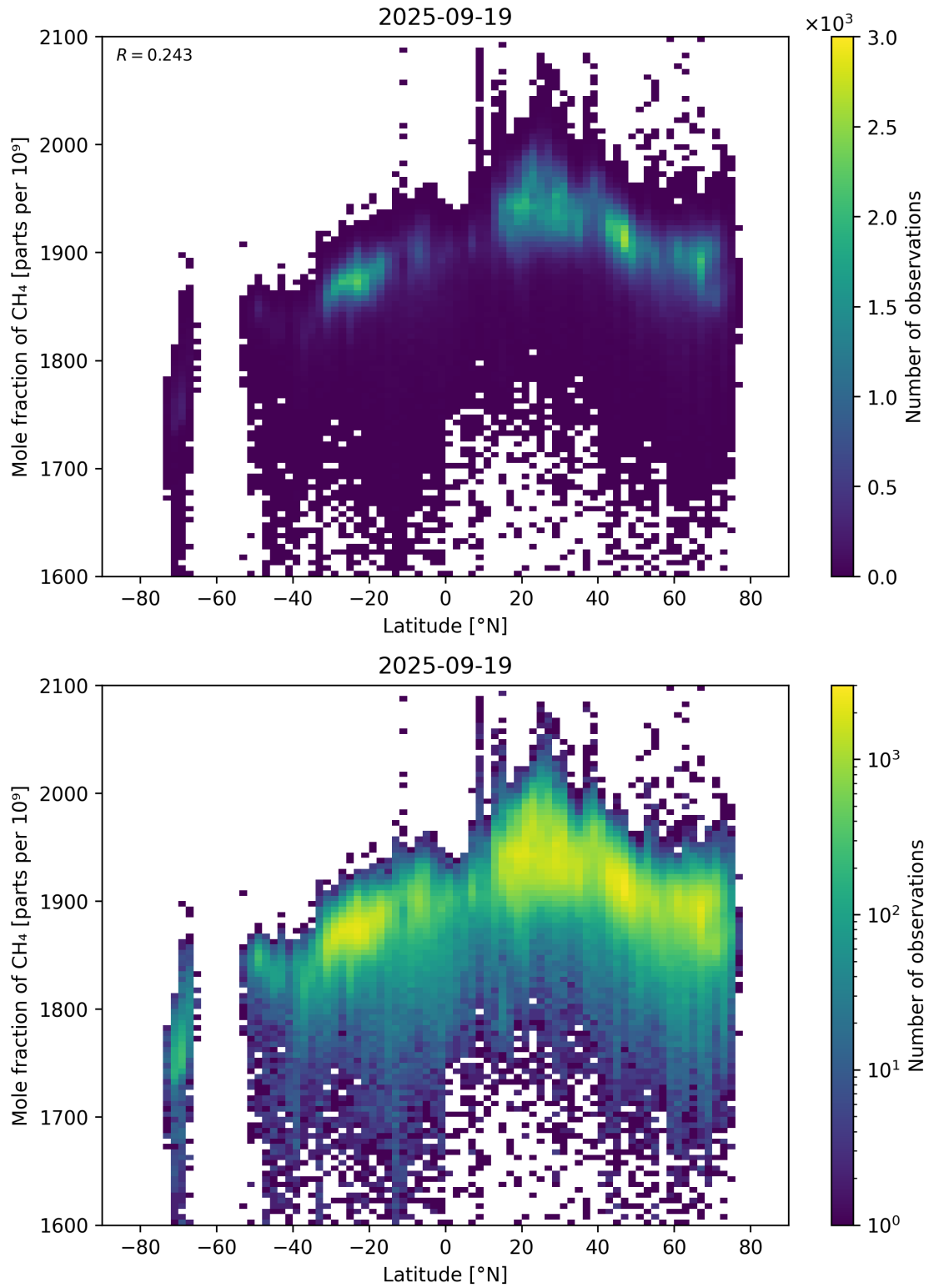
Figure 57: Scatter density plot of “Latitude” against “Mole fraction of CH 4 ” for 2025-09-18 to 2025-09-20.
