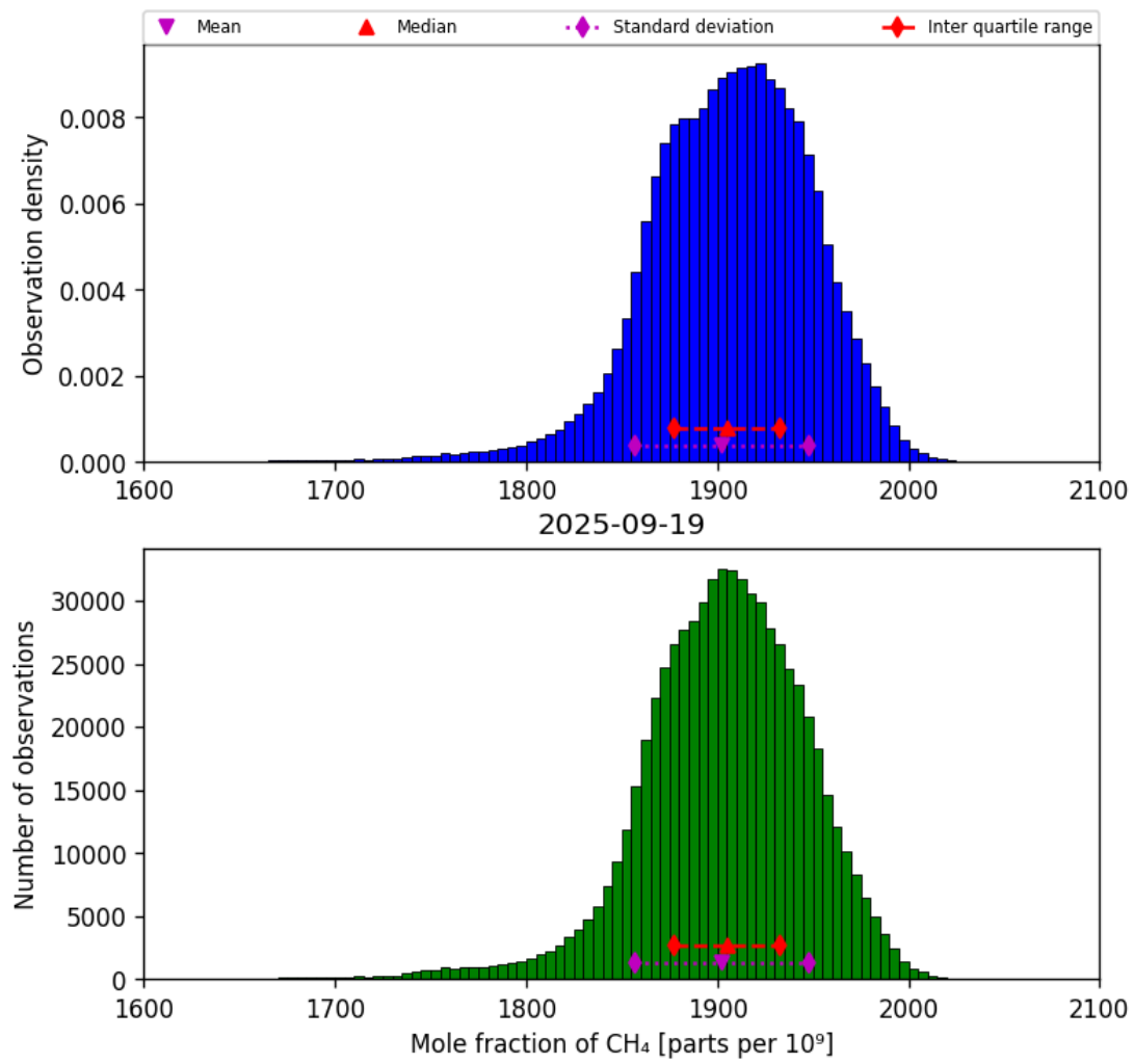
Figure 23: Histogram of “Mole fraction of CH 4 ” for 2025-09-18 to 2025-09-20
