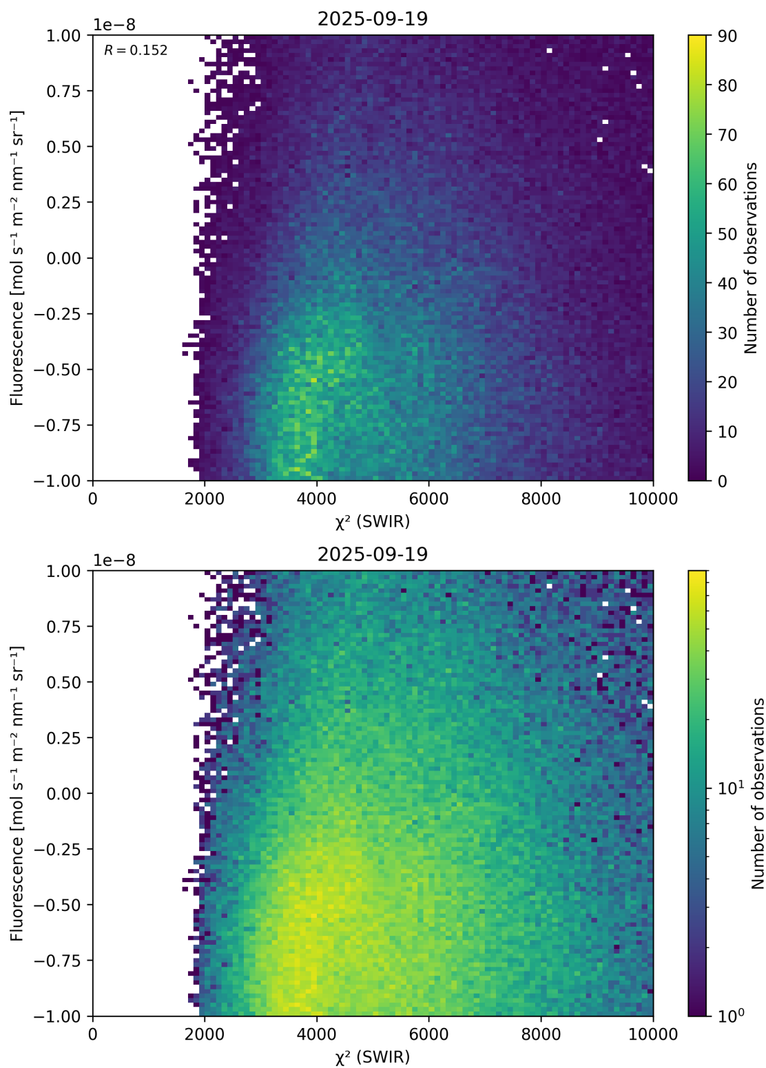
Figure 49: Scatter density plot of “ \chi^2 (SWIR)” against “Fluorescence” for 2025-09-18 to 2025-09-20.
