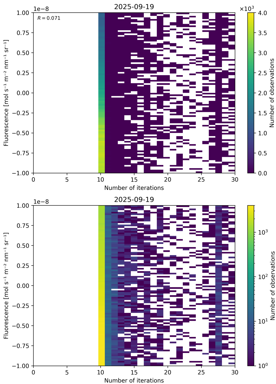
Figure 87: Scatter density plot of “Number of iterations” against “Fluorescence” for 2025-09-18 to 2025-09-20.
