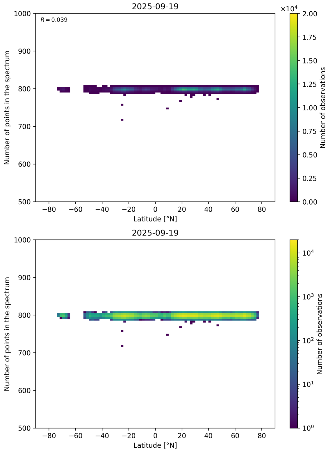
Figure 61: Scatter density plot of “Latitude” against “Number of points in the spectrum” for 2025-09-18 to 2025-09-20.
