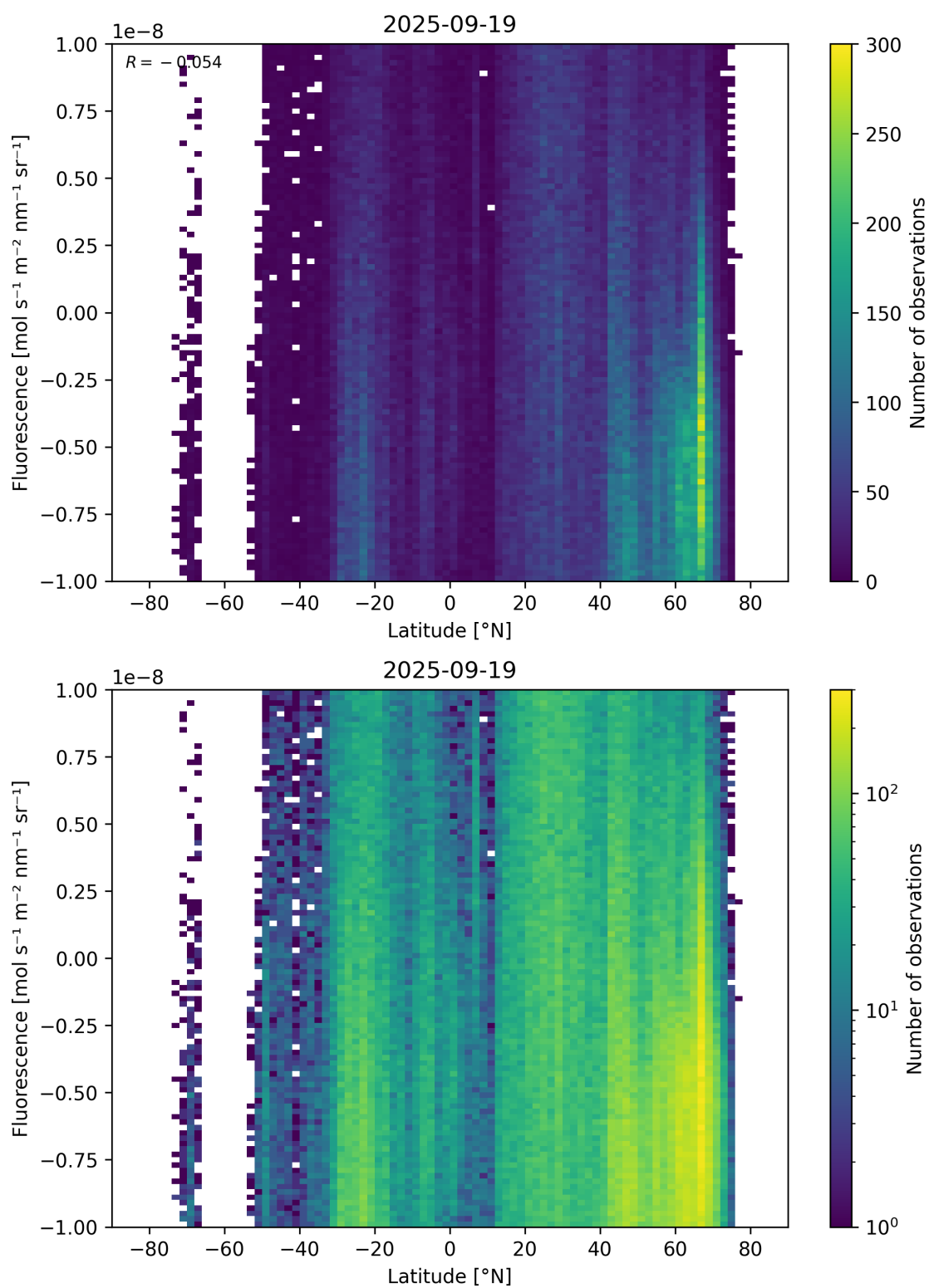
Figure 56: Scatter density plot of “Latitude” against “Fluorescence” for 2025-09-18 to 2025-09-20.
