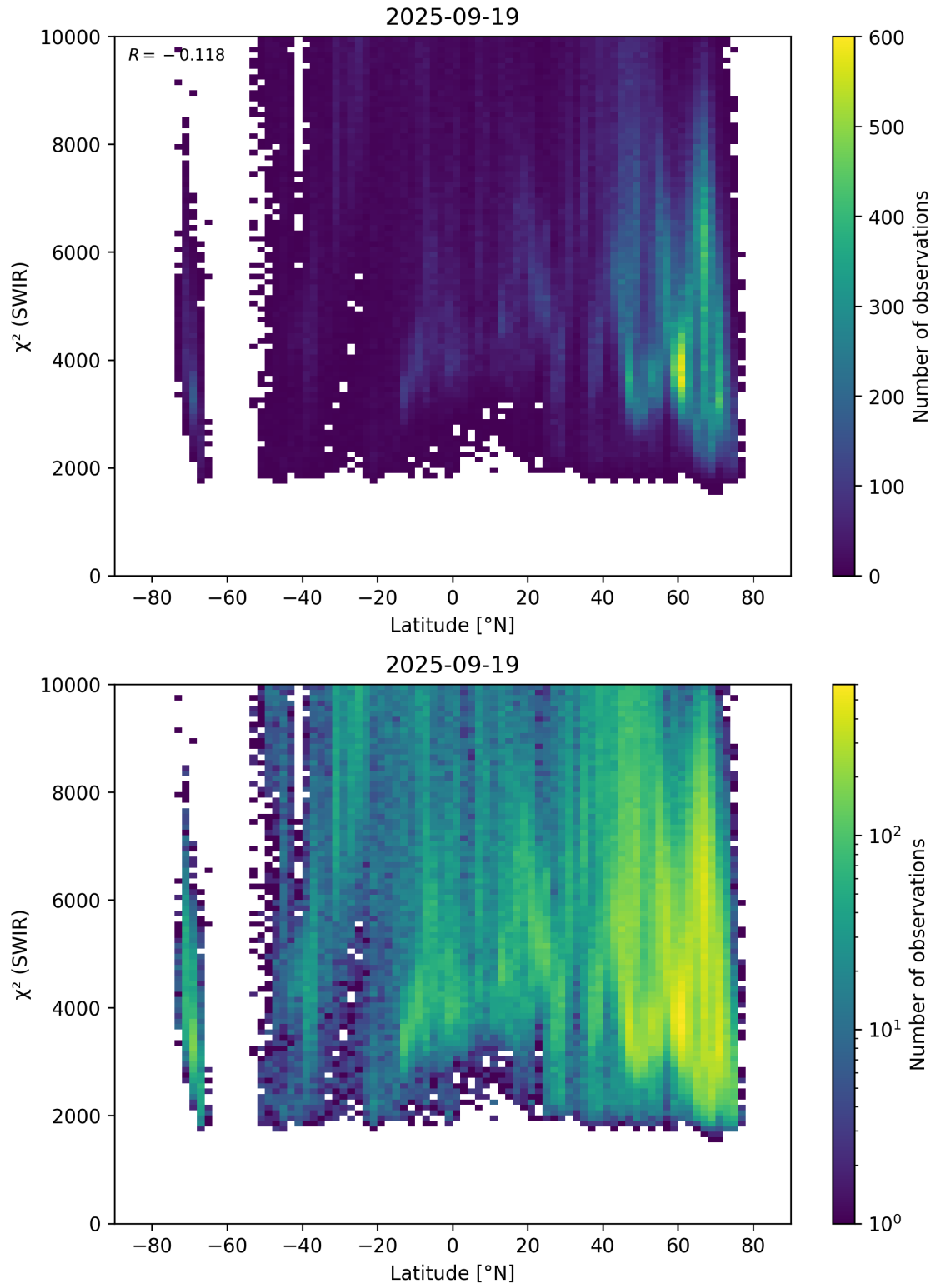
Figure 54: Scatter density plot of “Latitude” against “ \chi^2 (SWIR)” for 2025-09-18 to 2025-09-20.
