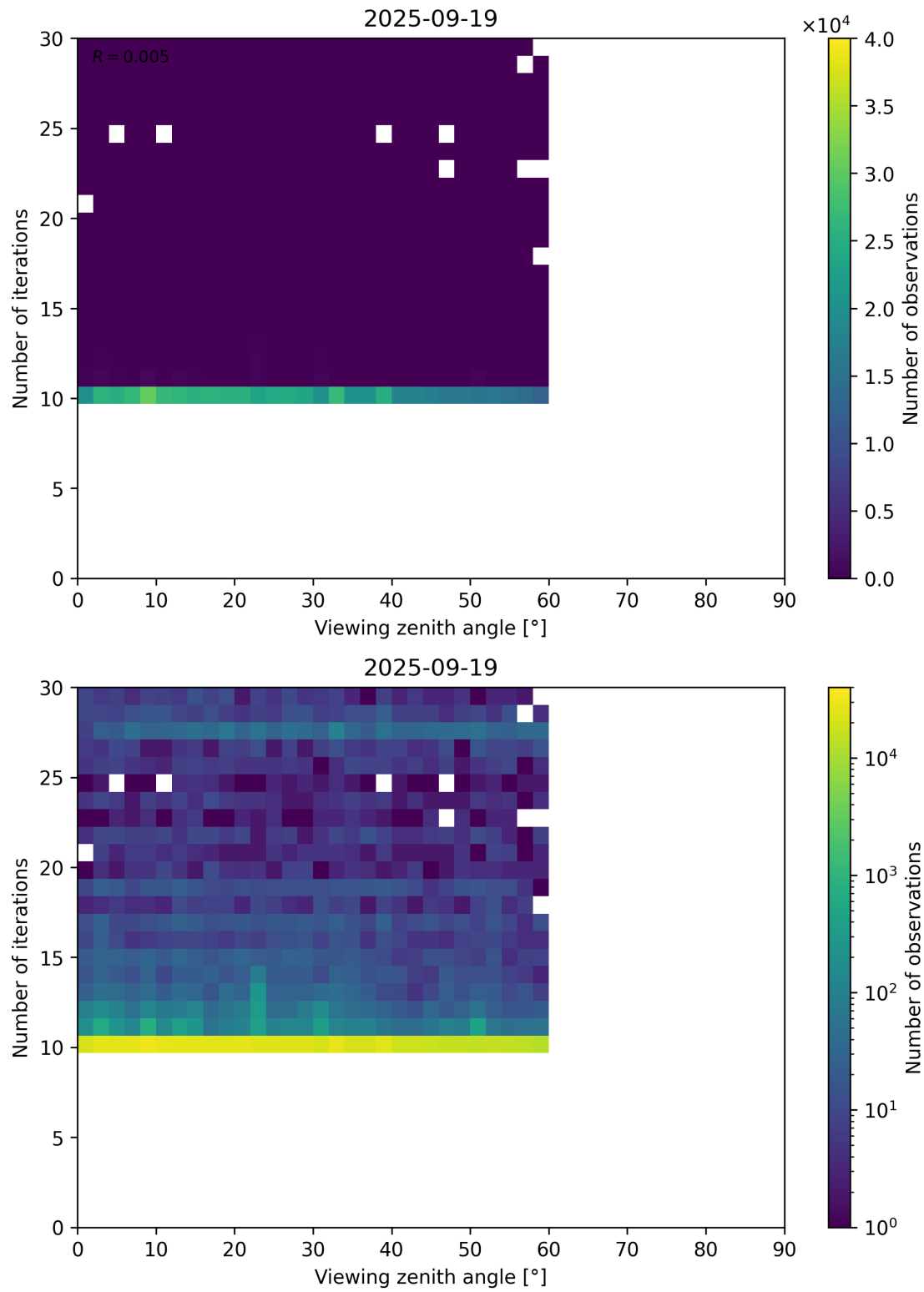
Figure 113: Scatter density plot of “Viewing zenith angle” against “Number of iterations” for 2025-09-18 to 2025-09-20.
