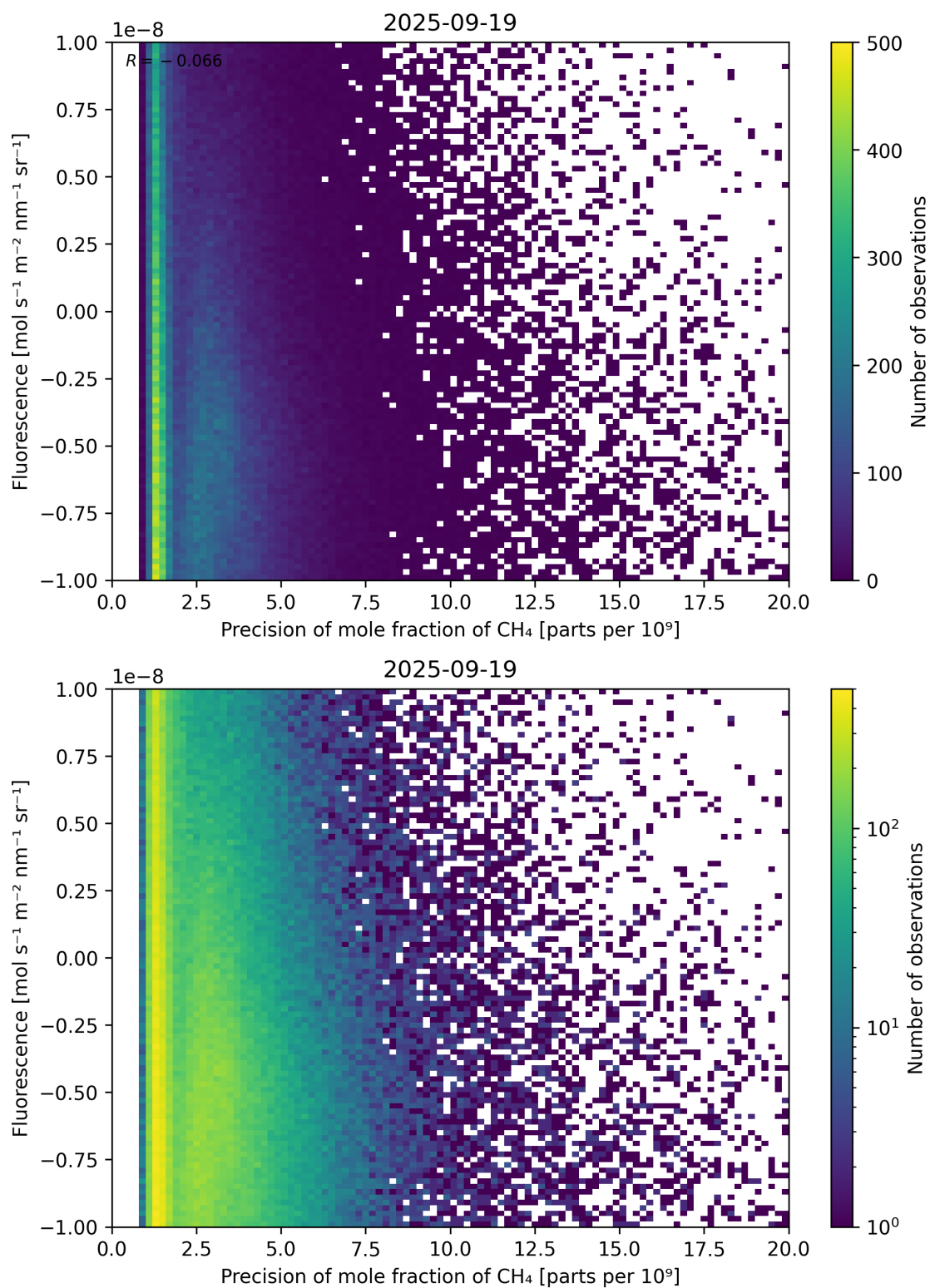
Figure 81: Scatter density plot of “Precision of mole fraction of \text{CH}_4 ” against “Fluorescence” for 2025-09-18 to 2025-09-20.
