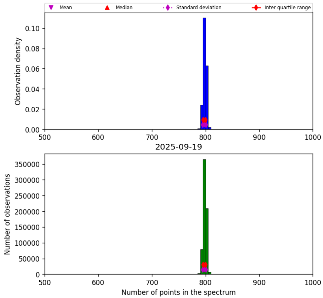
Figure 26: Histogram of “Number of points in the spectrum” for 2025-09-18 to 2025-09-20
