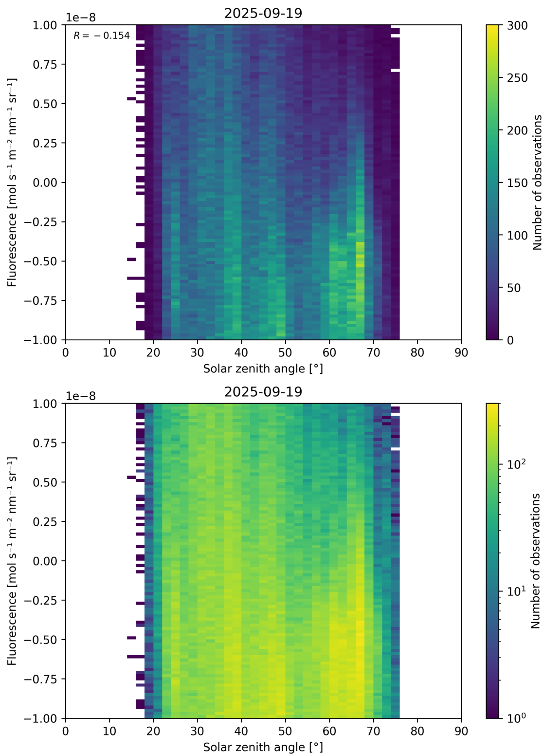
Figure 97: Scatter density plot of “Solar zenith angle” against “Fluorescence” for 2025-09-18 to 2025-09-20.
