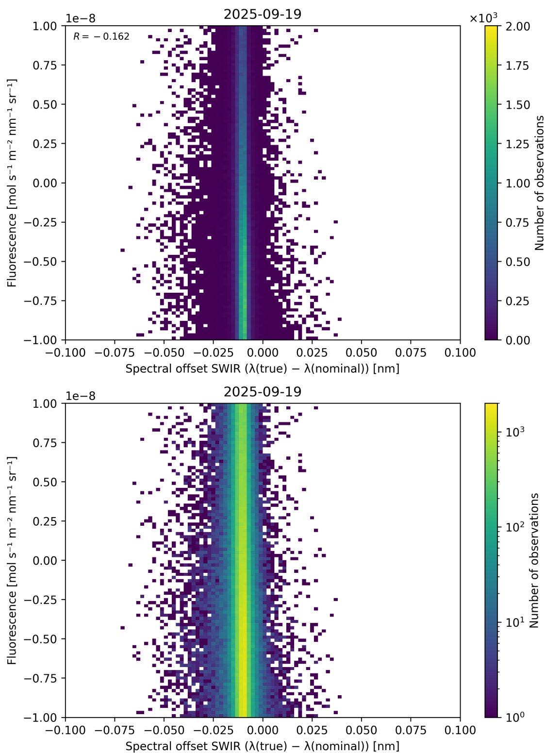
Figure 120: Scatter density plot of “Spectral offset SWIR ( \lambda_{\text{true}} - \lambda_{\text{nominal}} )” against “Fluorescence” for 2025-09-18 to 2025-09-20.
