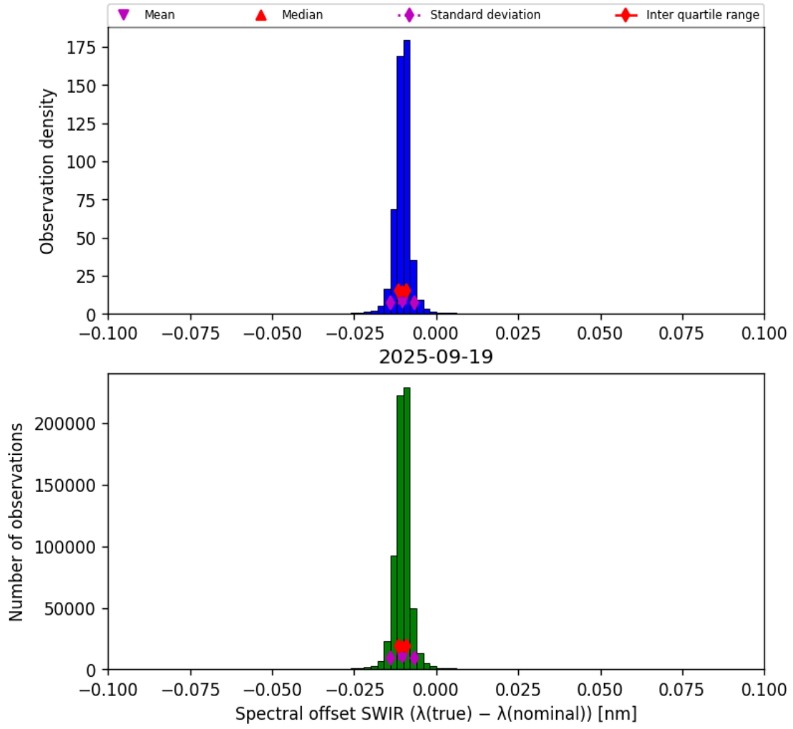
Figure 27: Histogram of “Spectral offset SWIR ( \lambda_{\text{true}} - \lambda_{\text{nominal}} )” for 2025-09-18 to 2025-09-20
