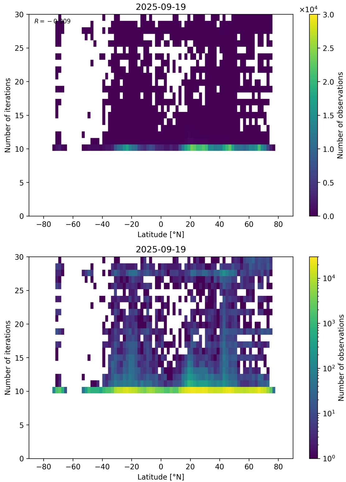
Figure 60: Scatter density plot of “Latitude” against “Number of iterations” for 2025-09-18 to 2025-09-20.
