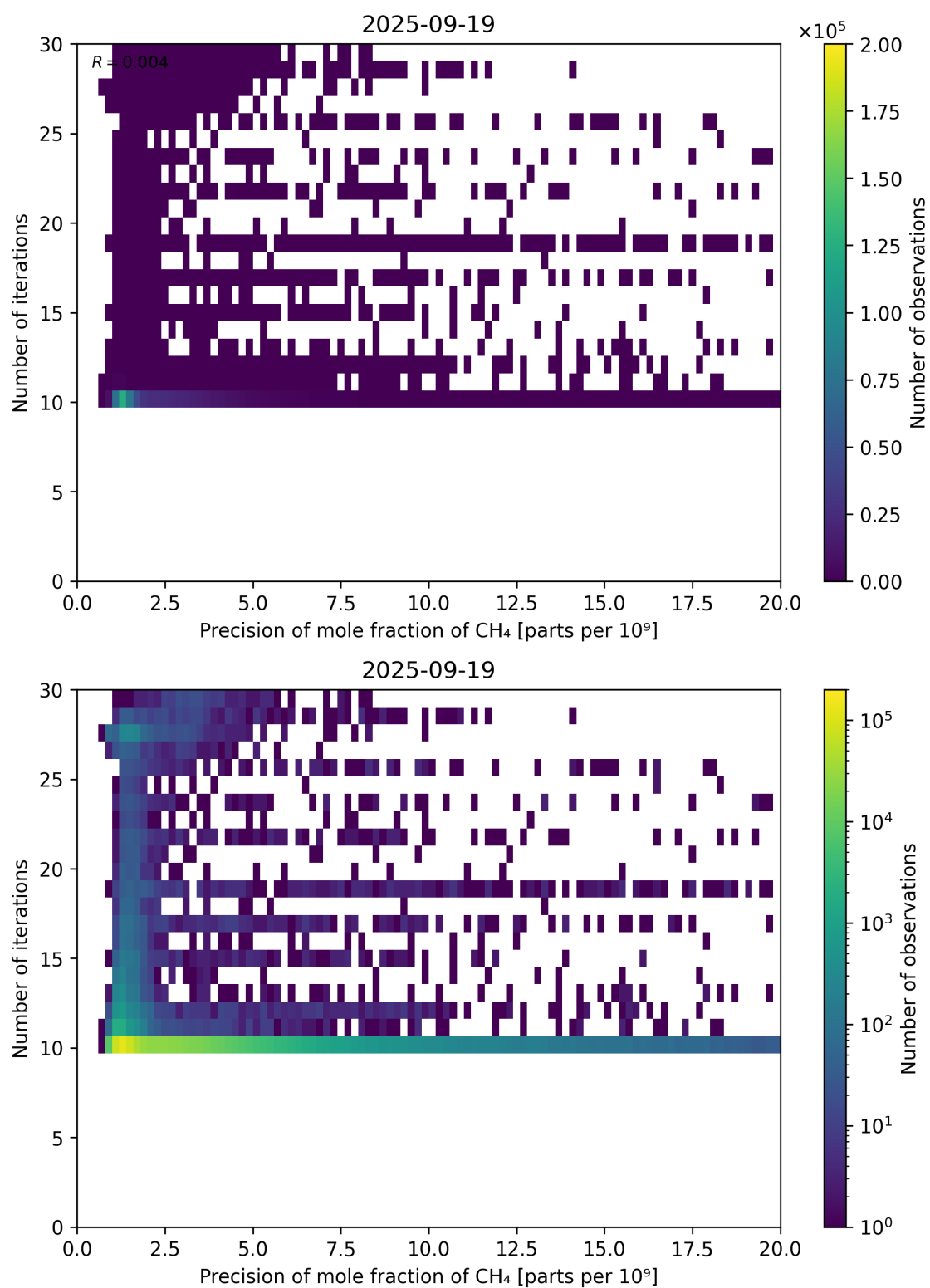
Figure 83: Scatter density plot of “Precision of mole fraction of CH 4 ” against “Number of iterations” for 2025-09-18 to 2025-09-20.
