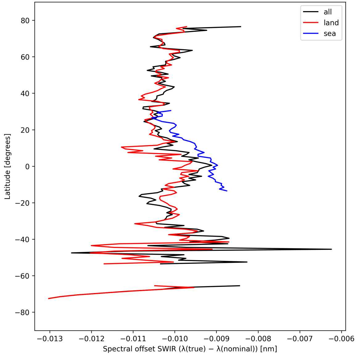
Figure 16: Zonal average of “Spectral offset SWIR ( \lambda_{\text{true}} - \lambda_{\text{nominal}} )” for 2025-09-18 to 2025-09-20.
