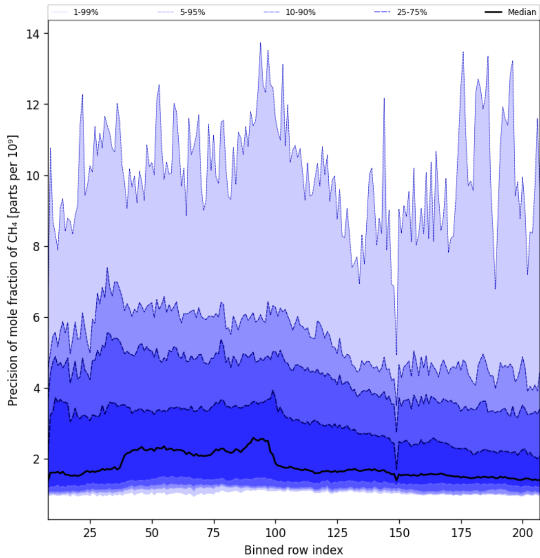
Figure 35: Along track statistics of “Precision of mole fraction of CH 4 ” for 2025-09-18 to 2025-09-20
