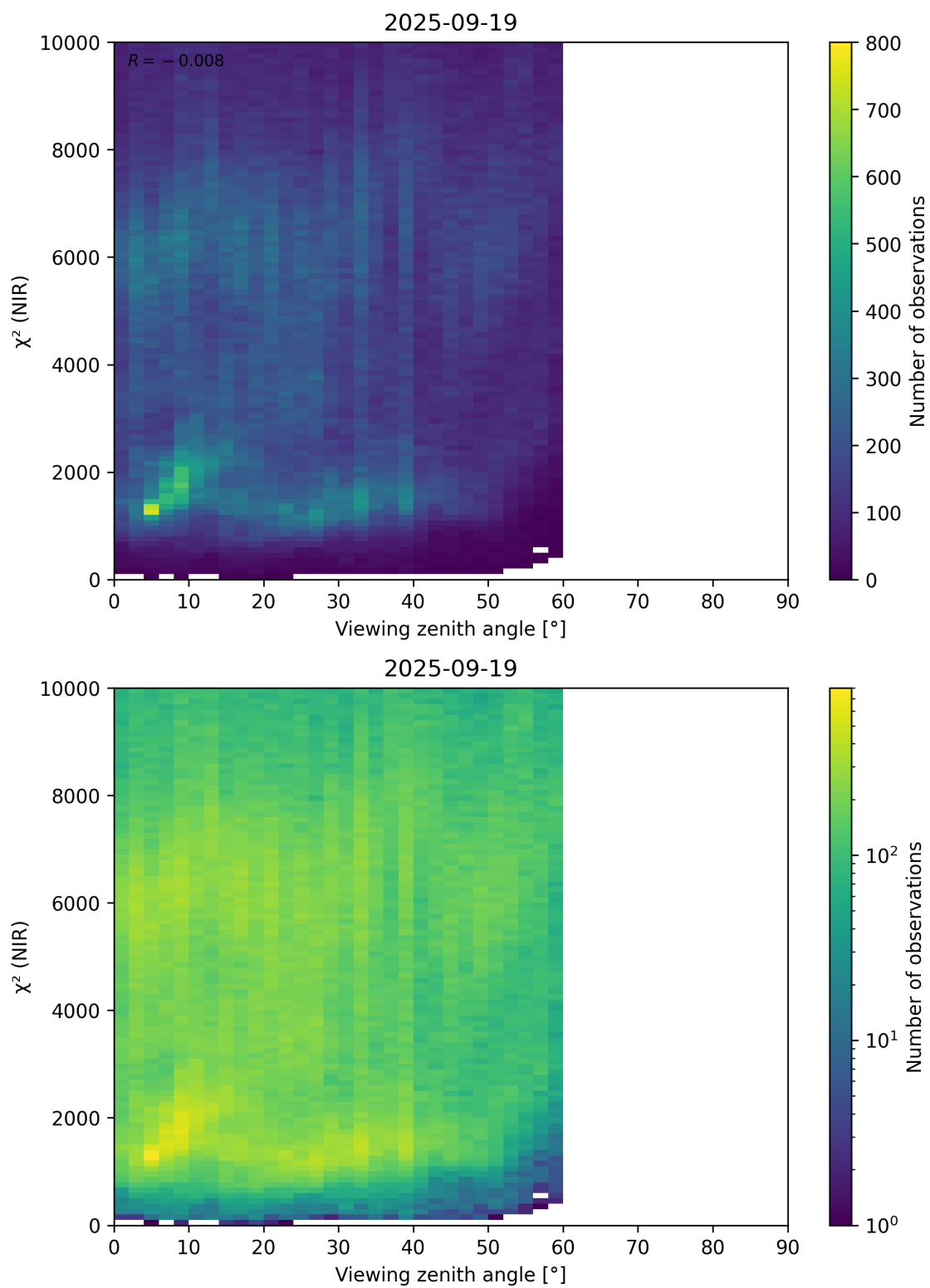
Figure 105: Scatter density plot of “Viewing zenith angle” against “ \chi^2 (NIR)” for 2025-09-18 to 2025-09-20.
