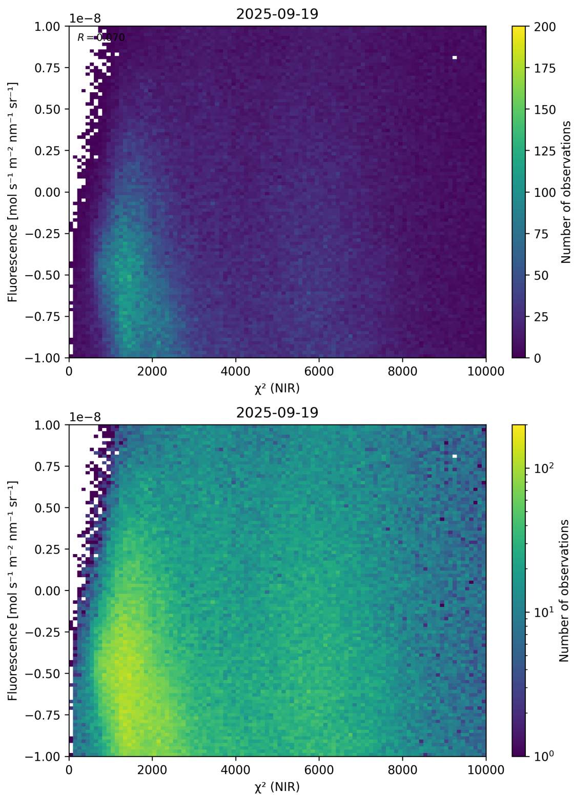
Figure 45: Scatter density plot of “ \chi^2 (NIR)” against “Fluorescence” for 2025-09-18 to 2025-09-20.
