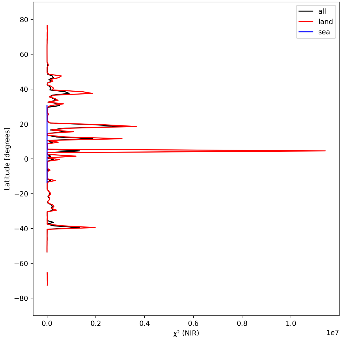
Figure 18: Zonal average of “ \chi^2 (NIR)” for 2025-09-18 to 2025-09-20.
