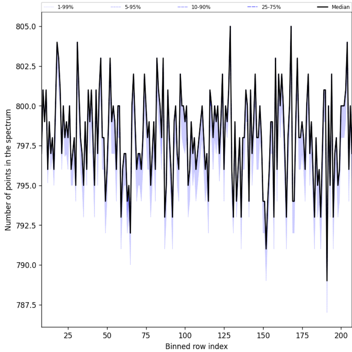
Figure 37: Along track statistics of “Number of points in the spectrum” for 2025-09-18 to 2025-09-20
