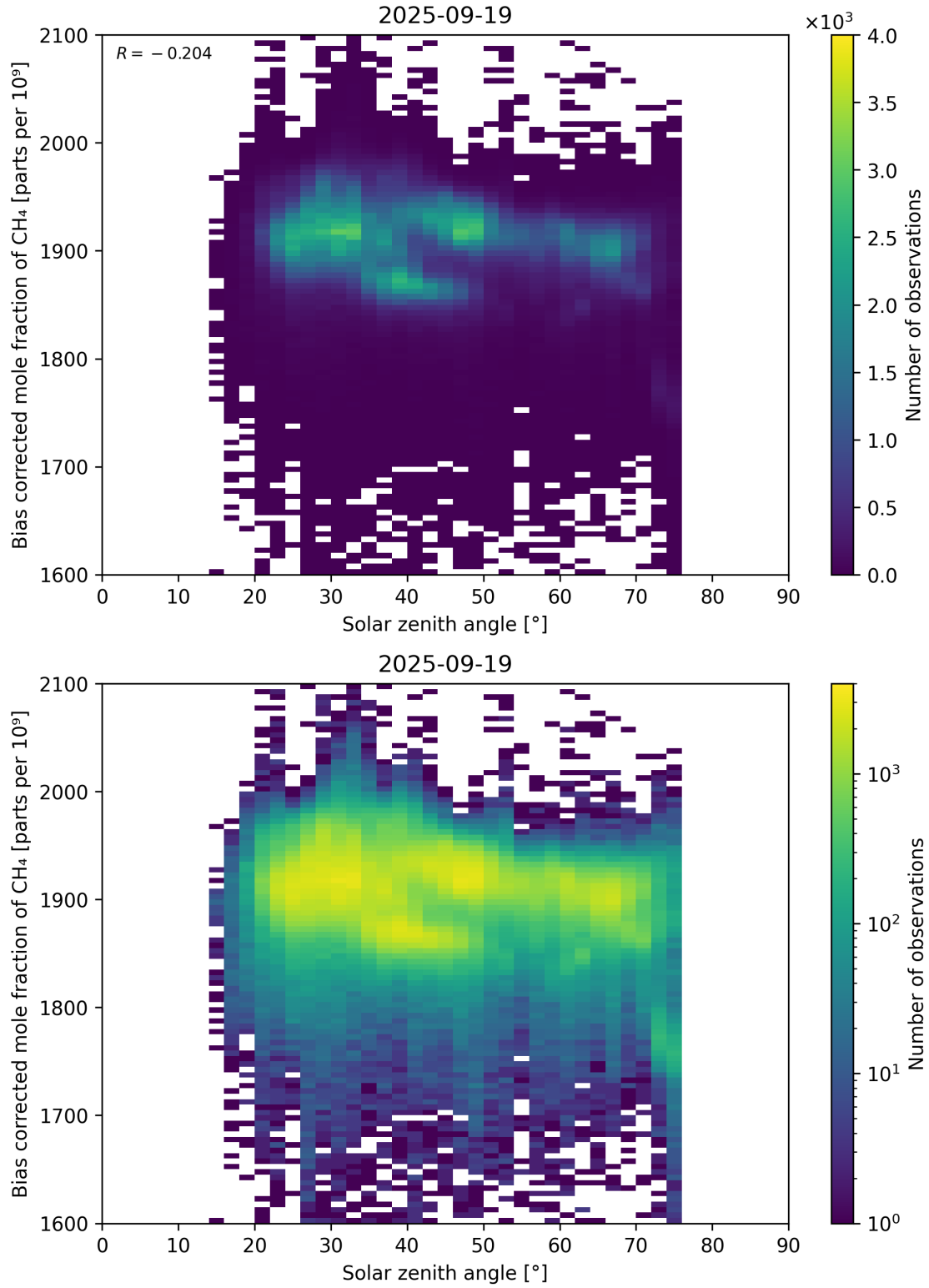
Figure 100: Scatter density plot of “Solar zenith angle” against “Bias corrected mole fraction of CH 4 ” for 2025-09-18 to 2025-09-20.
