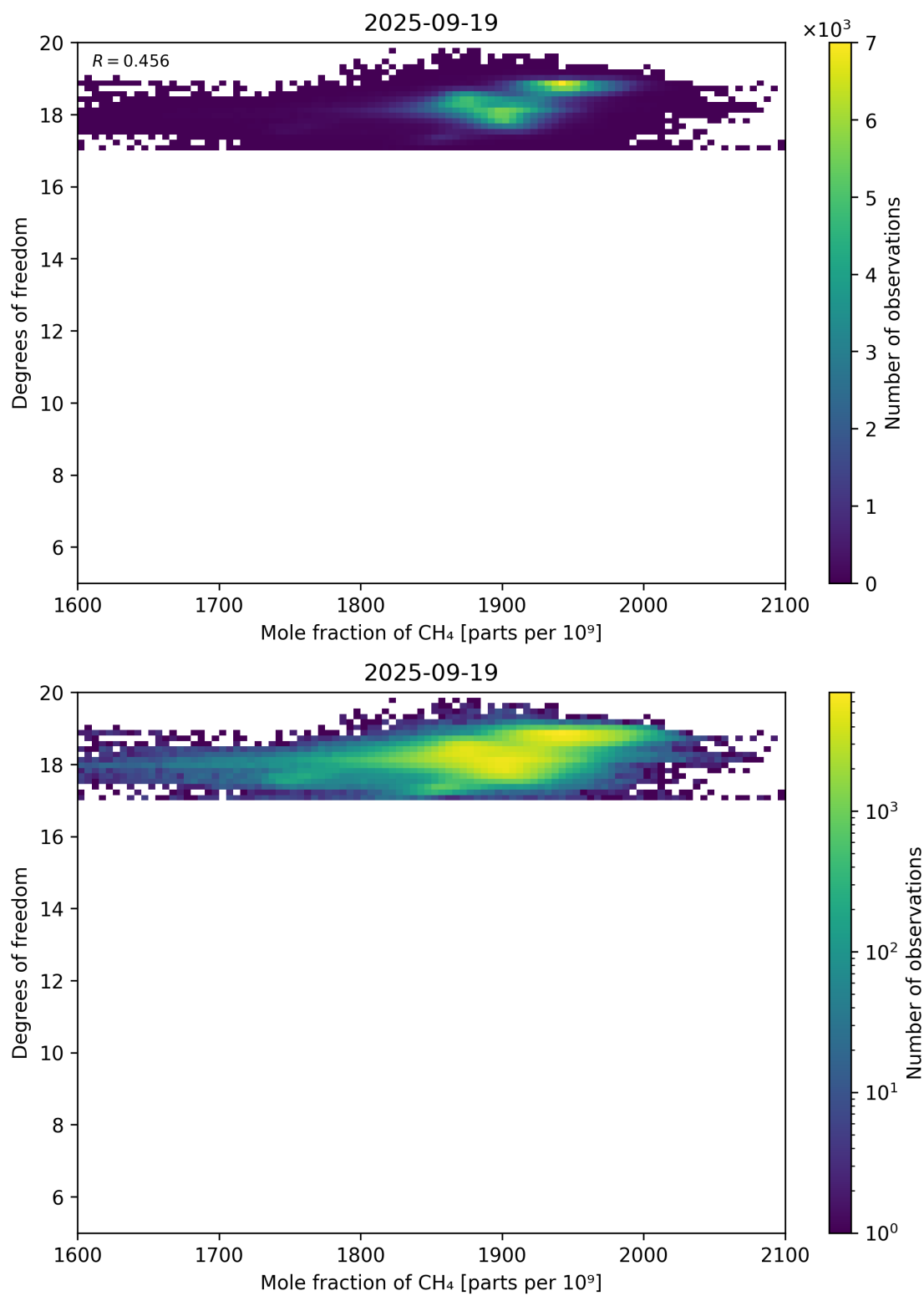
Figure 72: Scatter density plot of “Mole fraction of CH 4 ” against “Degrees of freedom” for 2025-09-18 to 2025-09-20.
