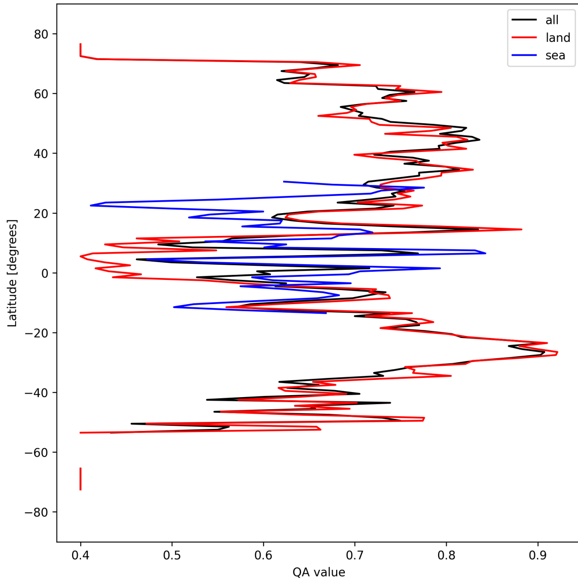
Figure 11: Zonal average of “QA value” for 2025-09-18 to 2025-09-20.
