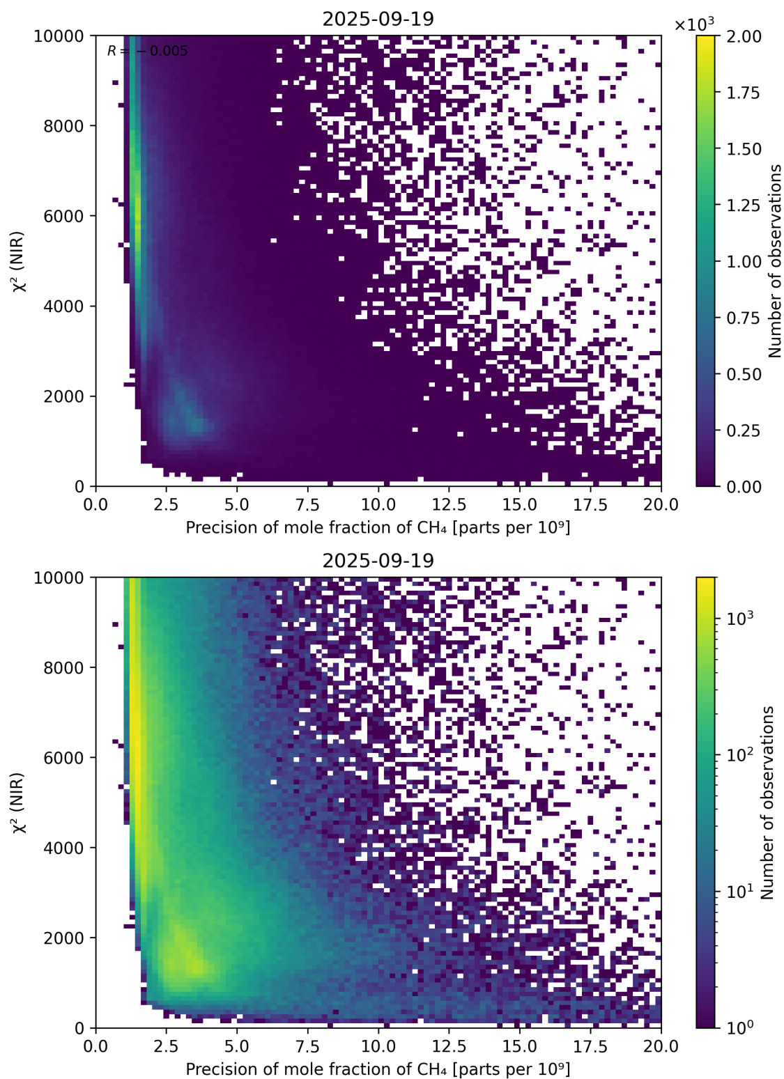
Figure 78: Scatter density plot of “Precision of mole fraction of \text{CH}_4 ” against “ \chi^2 (NIR)” for 2025-09-18 to 2025-09-20.
