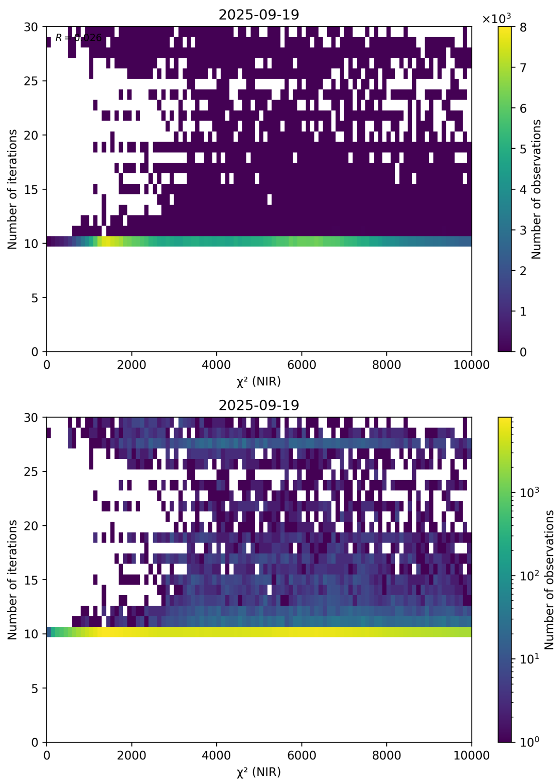
Figure 46: Scatter density plot of “ \chi^2 (NIR)” against “Number of iterations” for 2025-09-18 to 2025-09-20.
