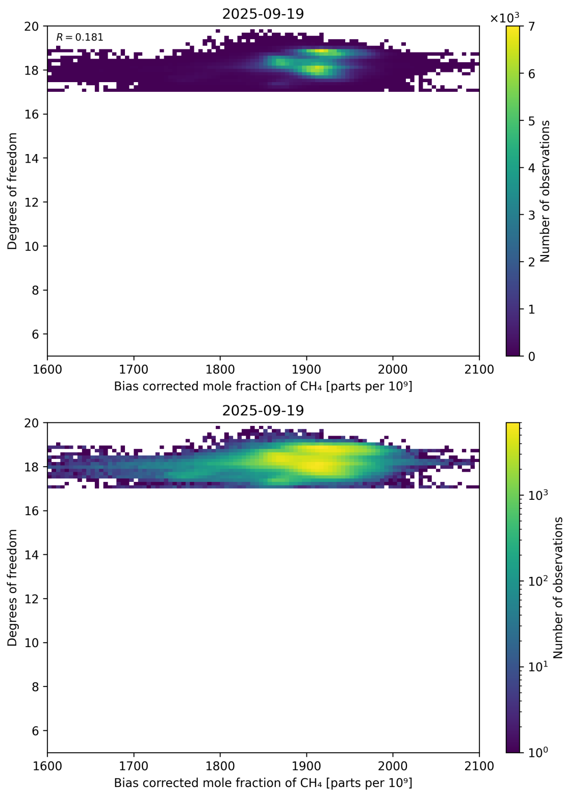
Figure 65: Scatter density plot of “Bias corrected mole fraction of CH 4 ” against “Degrees of freedom” for 2025-09-18 to 2025-09-20.
