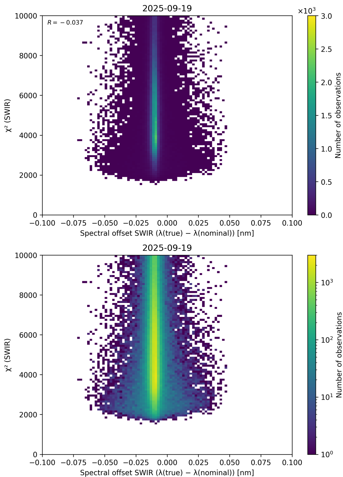
Figure 118: Scatter density plot of “Spectral offset SWIR ( \lambda_{\text{true}} - \lambda_{\text{nominal}} )” against “ \chi^2 (SWIR)” for 2025-09-18 to 2025-09-20.
