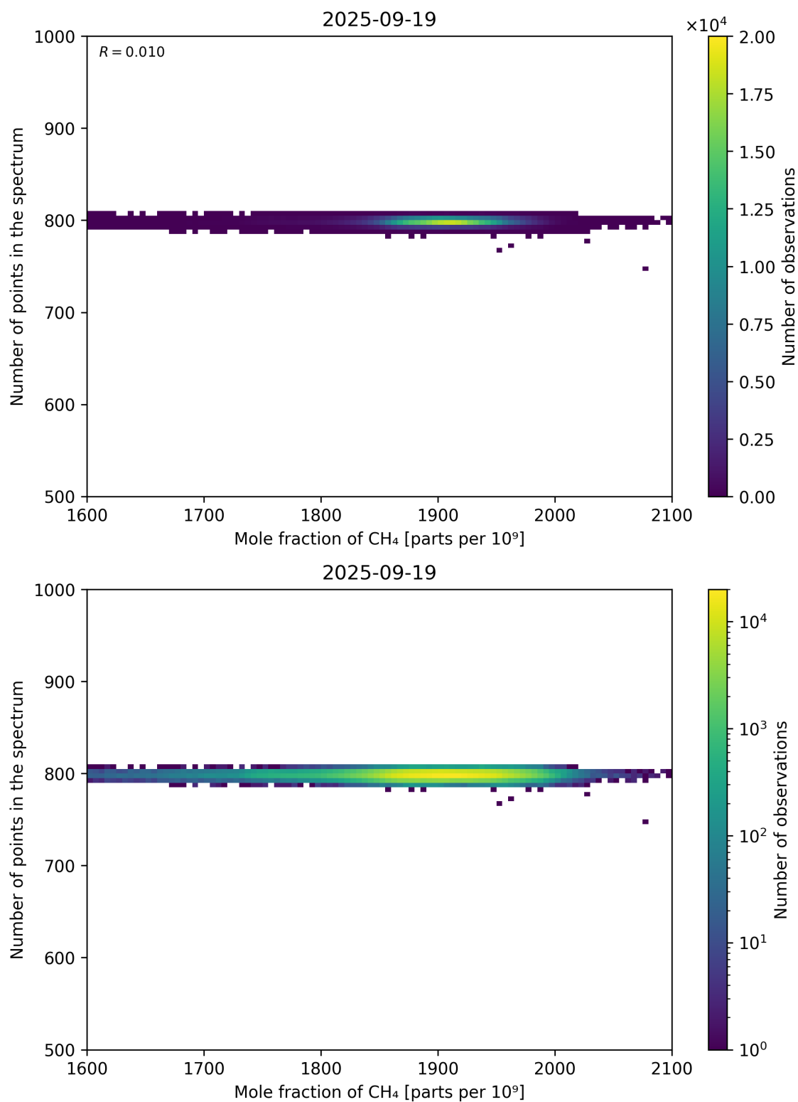
Figure 77: Scatter density plot of “Mole fraction of CH 4 ” against “Number of points in the spectrum” for 2025-09-18 to 2025-09-20.
