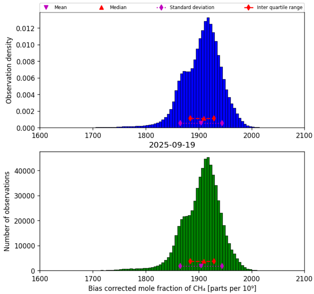
Figure 25: Histogram of “Bias corrected mole fraction of CH 4 ” for 2025-09-18 to 2025-09-20
