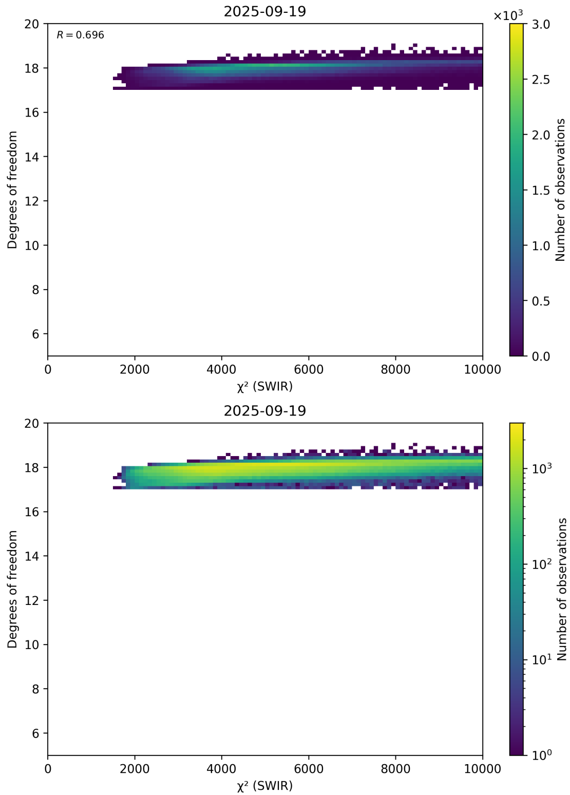
Figure 48: Scatter density plot of “ \chi^2 (SWIR)” against “Degrees of freedom” for 2025-09-18 to 2025-09-20.
