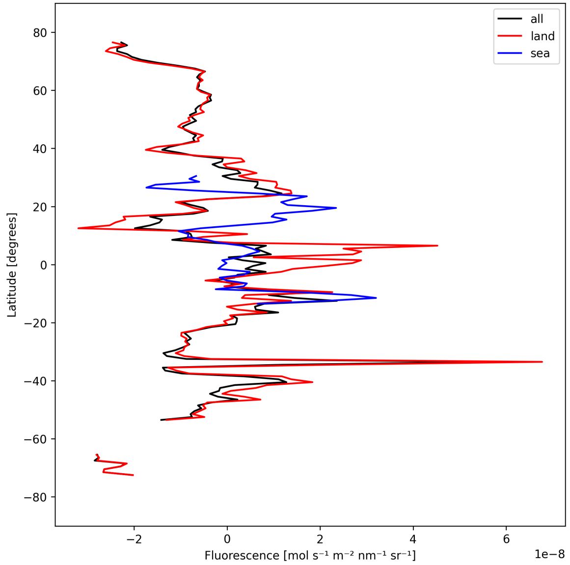
Figure 21: Zonal average of “Fluorescence” for 2025-09-18 to 2025-09-20.
