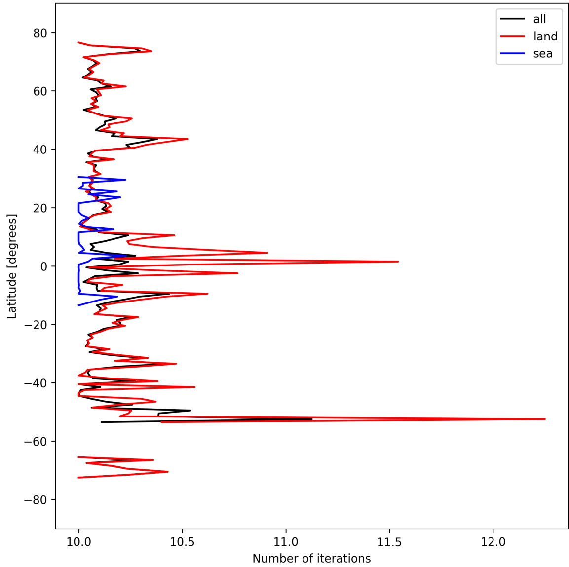
Figure 20: Zonal average of “Number of iterations” for 2025-09-18 to 2025-09-20.
