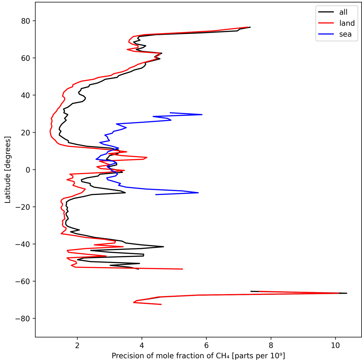
Figure 13: Zonal average of “Precision of mole fraction of CH 4 ” for 2025-09-18 to 2025-09-20.
