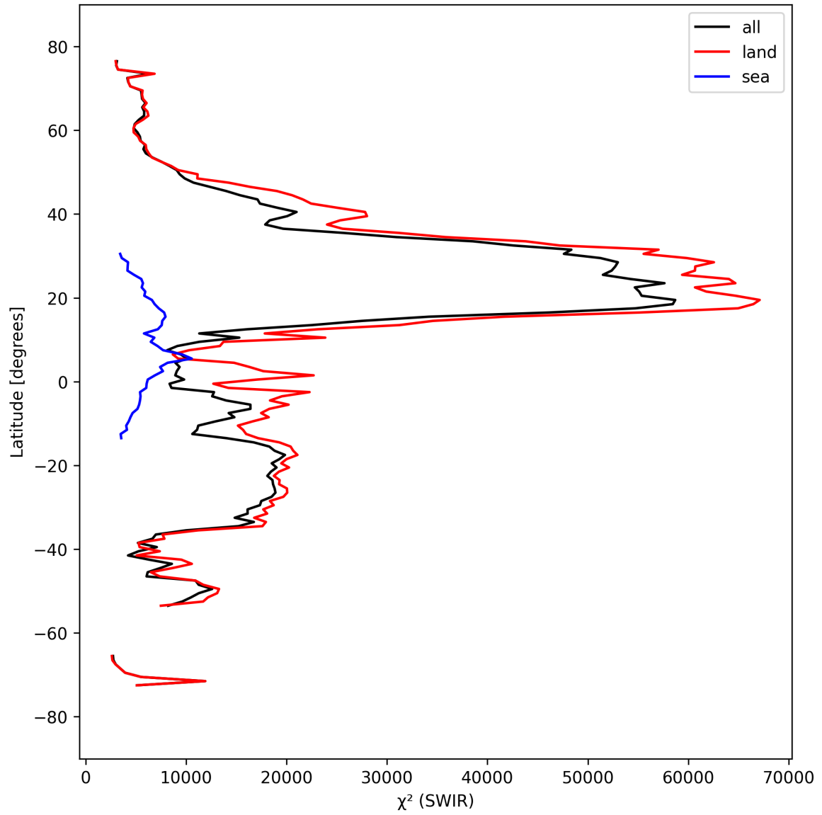
Figure 17: Zonal average of “ \chi^2 (SWIR)” for 2025-09-18 to 2025-09-20.
