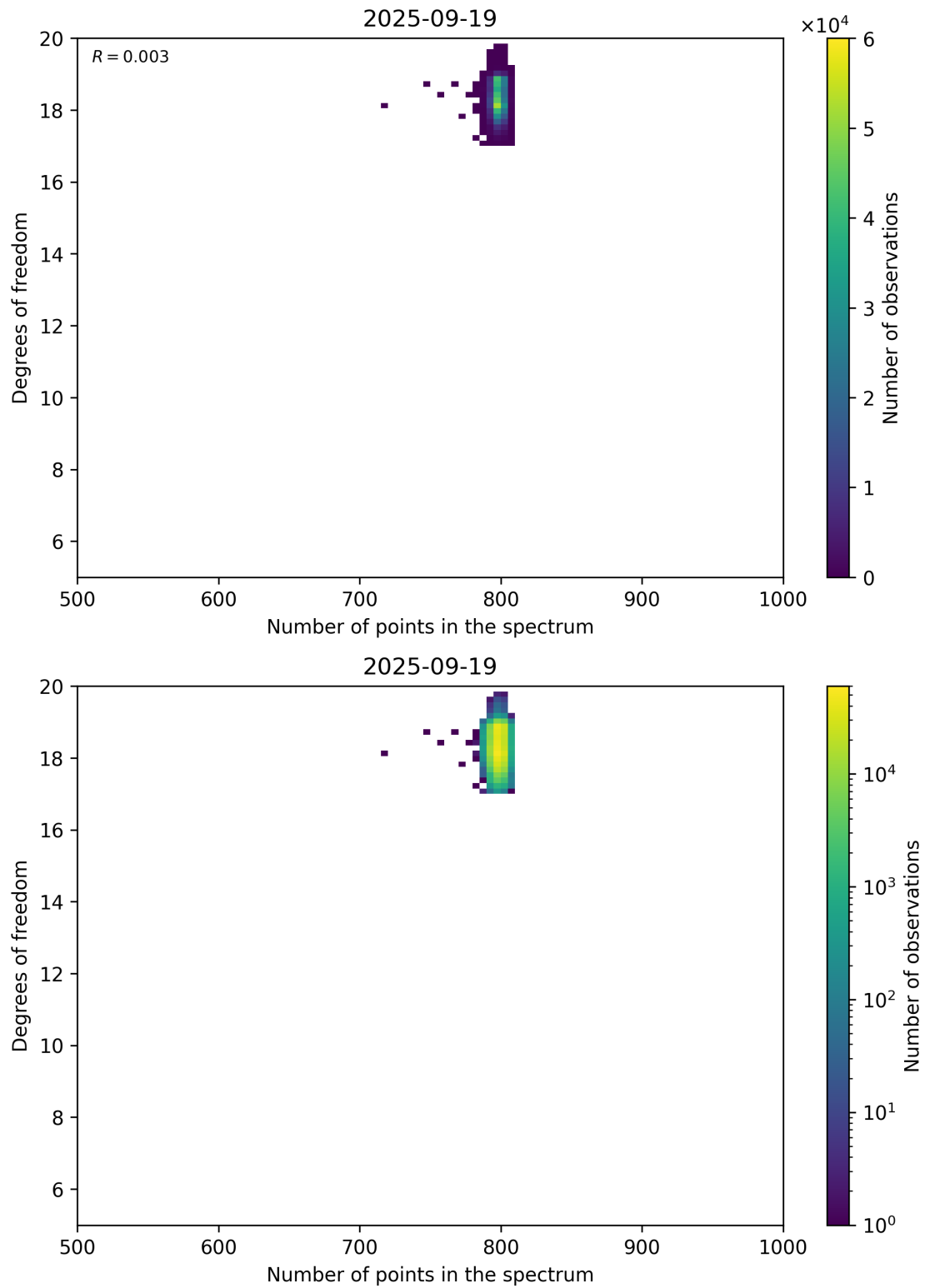
Figure 90: Scatter density plot of “Number of points in the spectrum” against “Degrees of freedom” for 2025-09-18 to 2025-09-20.
