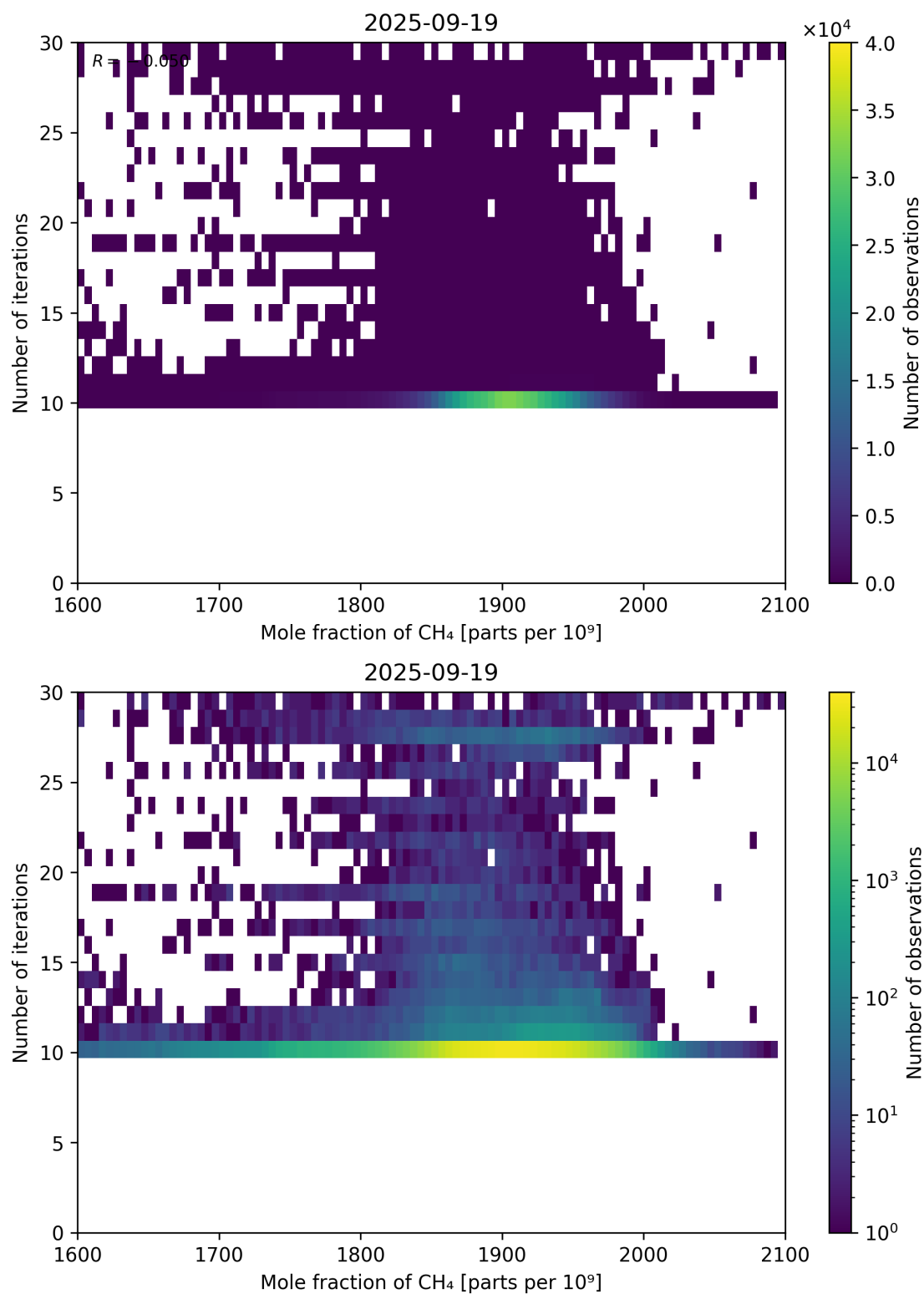
Figure 76: Scatter density plot of “Mole fraction of CH 4 ” against “Number of iterations” for 2025-09-18 to 2025-09-20.
