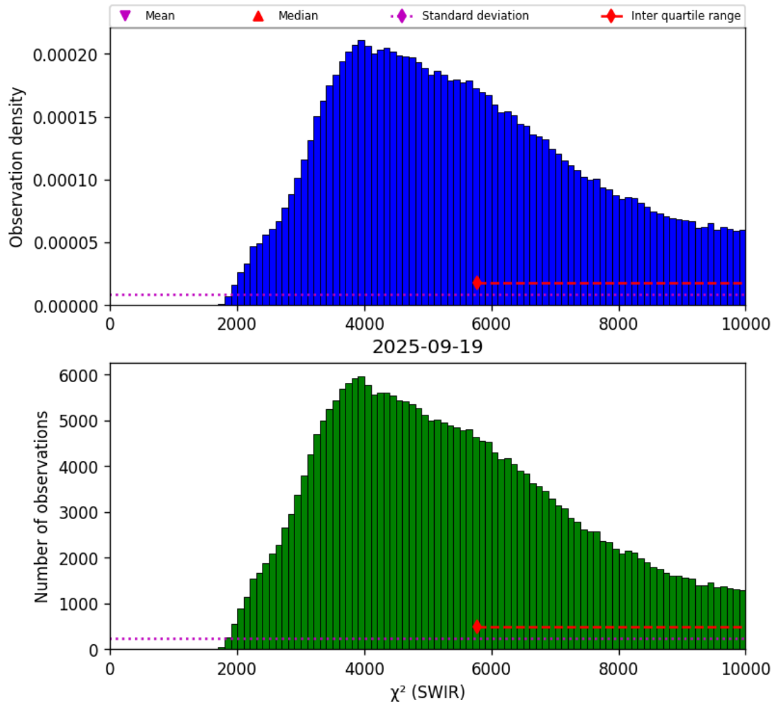
Figure 28: Histogram of " \chi^2 (SWIR)" for 2025-09-18 to 2025-09-20
