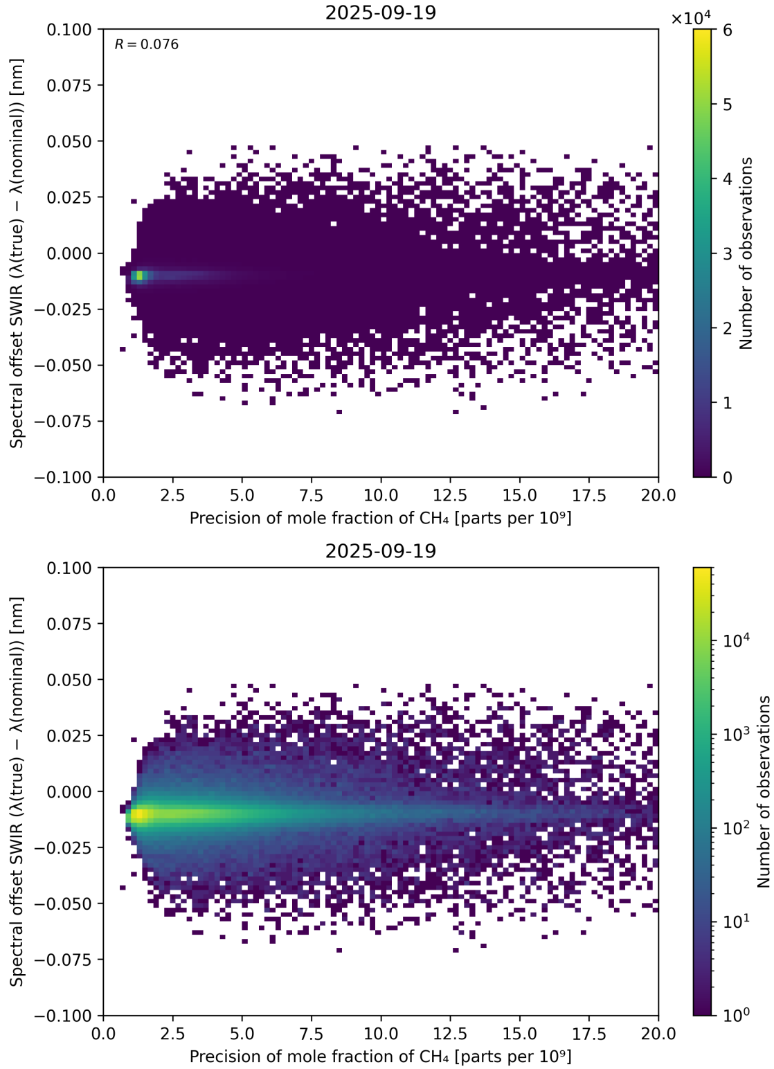
Figure 85: Scatter density plot of “Precision of mole fraction of CH 4 ” against “Spectral offset SWIR ( \lambda_{\text{true}} - \lambda_{\text{nominal}} )” for 2025-09-18 to 2025-09-20.
