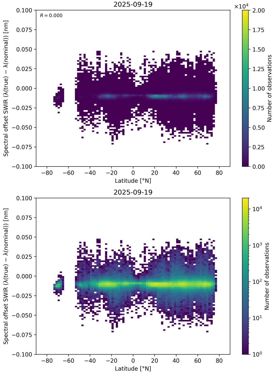
Figure 62: Scatter density plot of “Latitude” against “Spectral offset SWIR ( \lambda_{\text{true}} - \lambda_{\text{nominal}} )” for 2025-09-18 to 2025-09-20.
