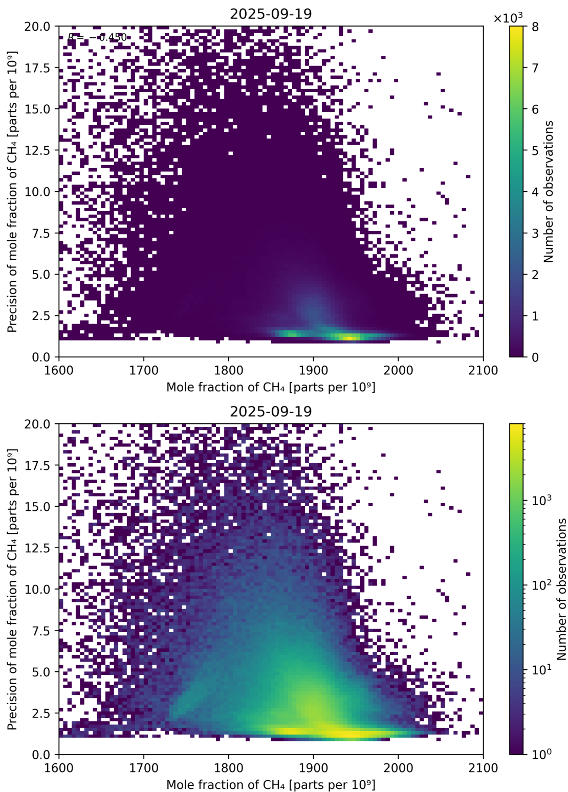
Figure 75: Scatter density plot of “Mole fraction of CH 4 ” against “Precision of mole fraction of CH 4 ” for 2025-09-18 to 2025-09-20.
