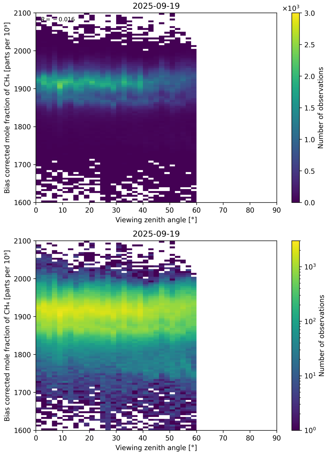
Figure 111: Scatter density plot of “Viewing zenith angle” against “Bias corrected mole fraction of CH 4 ” for 2025-09-18 to 2025-09-20.
