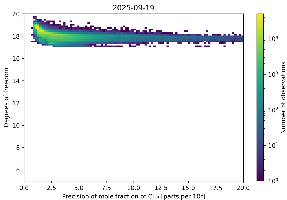
Figure 80: Scatter density plot of “Precision of mole fraction of CH 4 ” against “Degrees of freedom” for 2025-09-18 to 2025-09-20.
