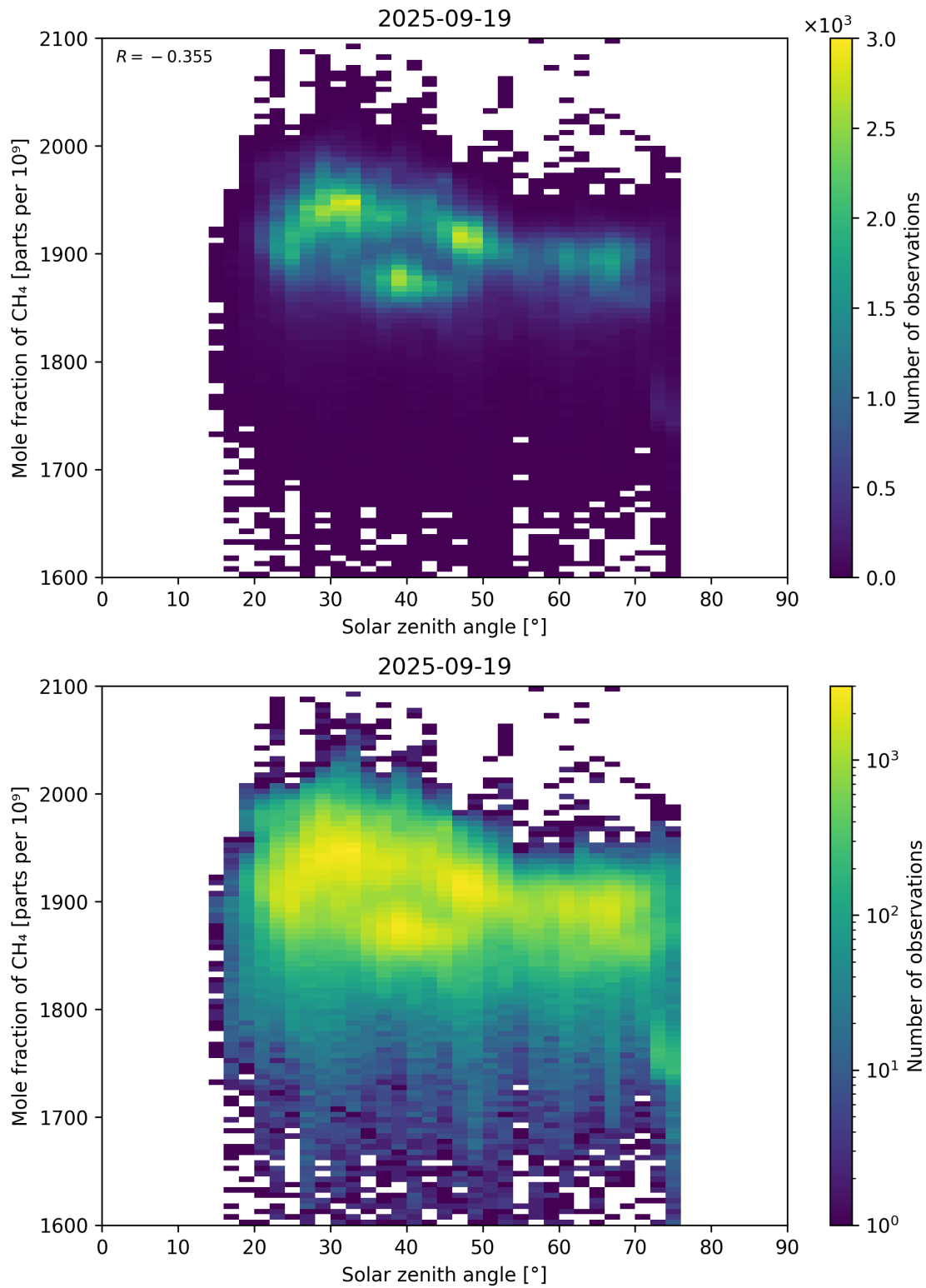
Figure 99: Scatter density plot of “Solar zenith angle” against “Mole fraction of CH 4 ” for 2025-09-18 to 2025-09-20.
