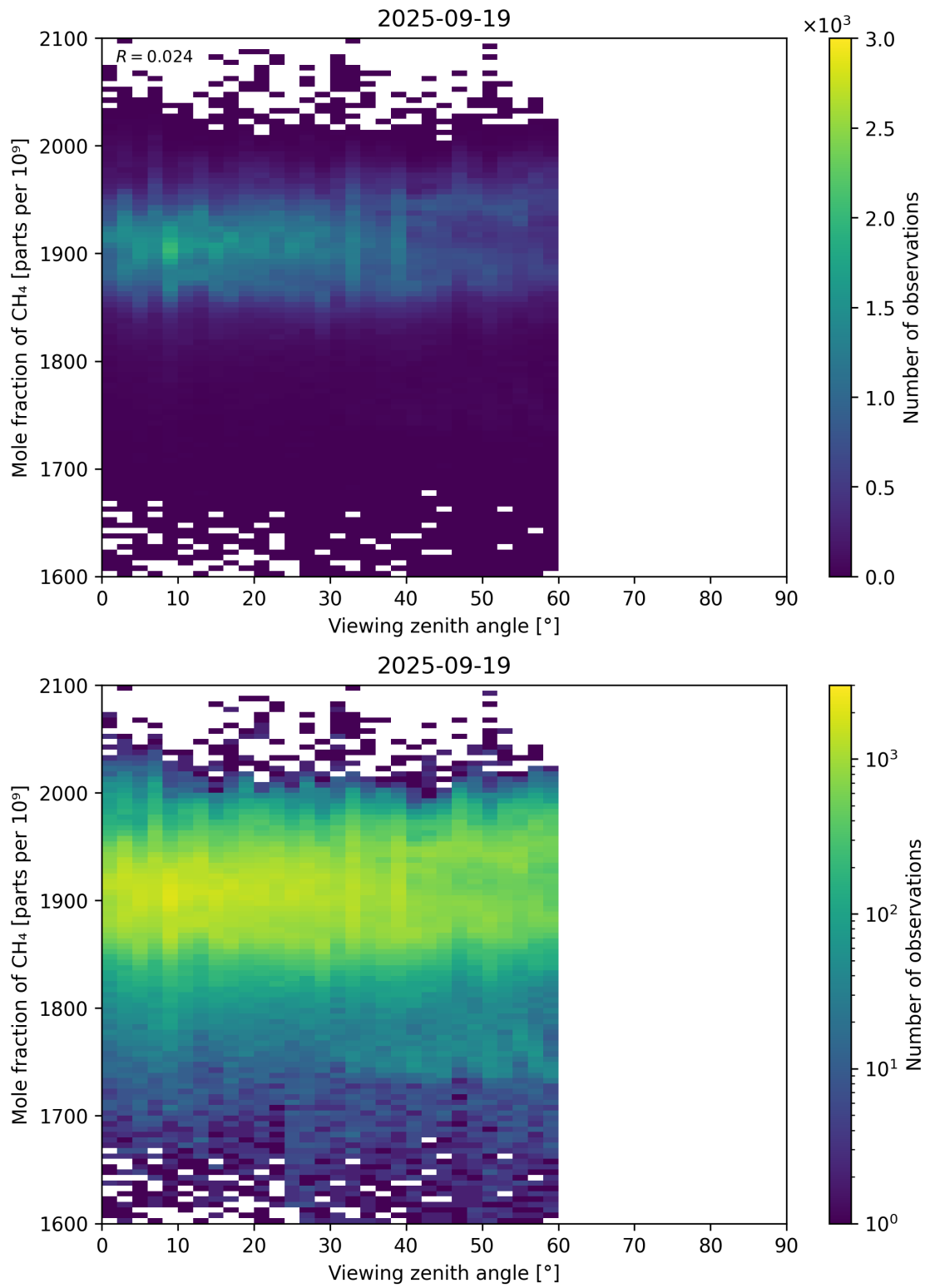
Figure 110: Scatter density plot of “Viewing zenith angle” against “Mole fraction of CH 4 ” for 2025-09-18 to 2025-09-20.
