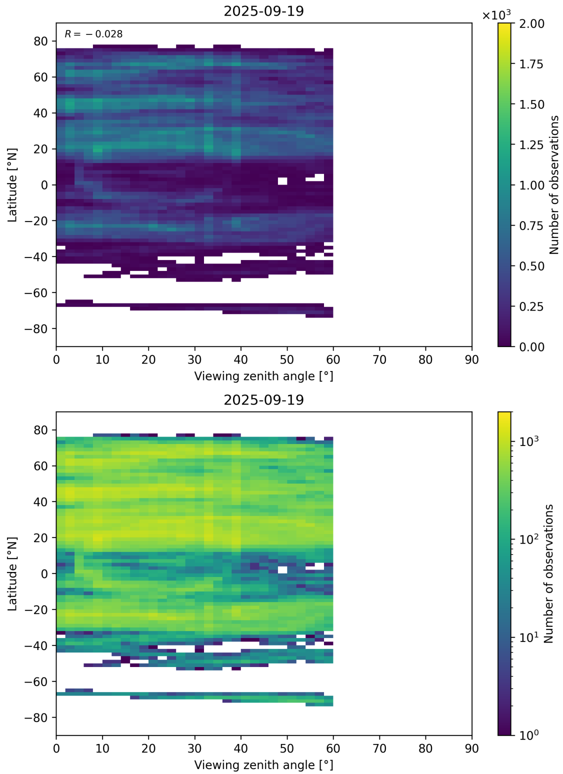
Figure 109: Scatter density plot of “Viewing zenith angle” against “Latitude” for 2025-09-18 to 2025-09-20.
