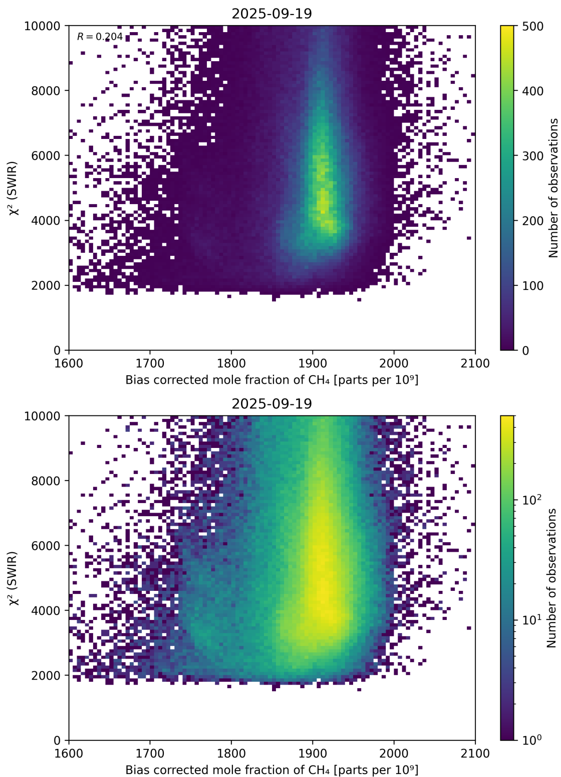
Figure 64: Scatter density plot of “Bias corrected mole fraction of \text{CH}_4 ” against “ \chi^2 (SWIR)” for 2025-09-18 to 2025-09-20.
