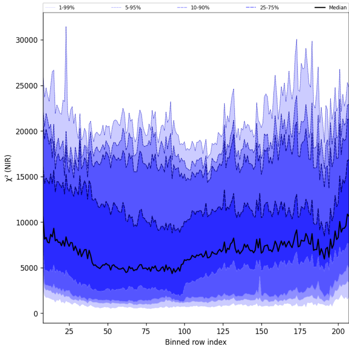
Figure 40: Along track statistics of “ \chi^2 (NIR)” for 2025-09-18 to 2025-09-20
