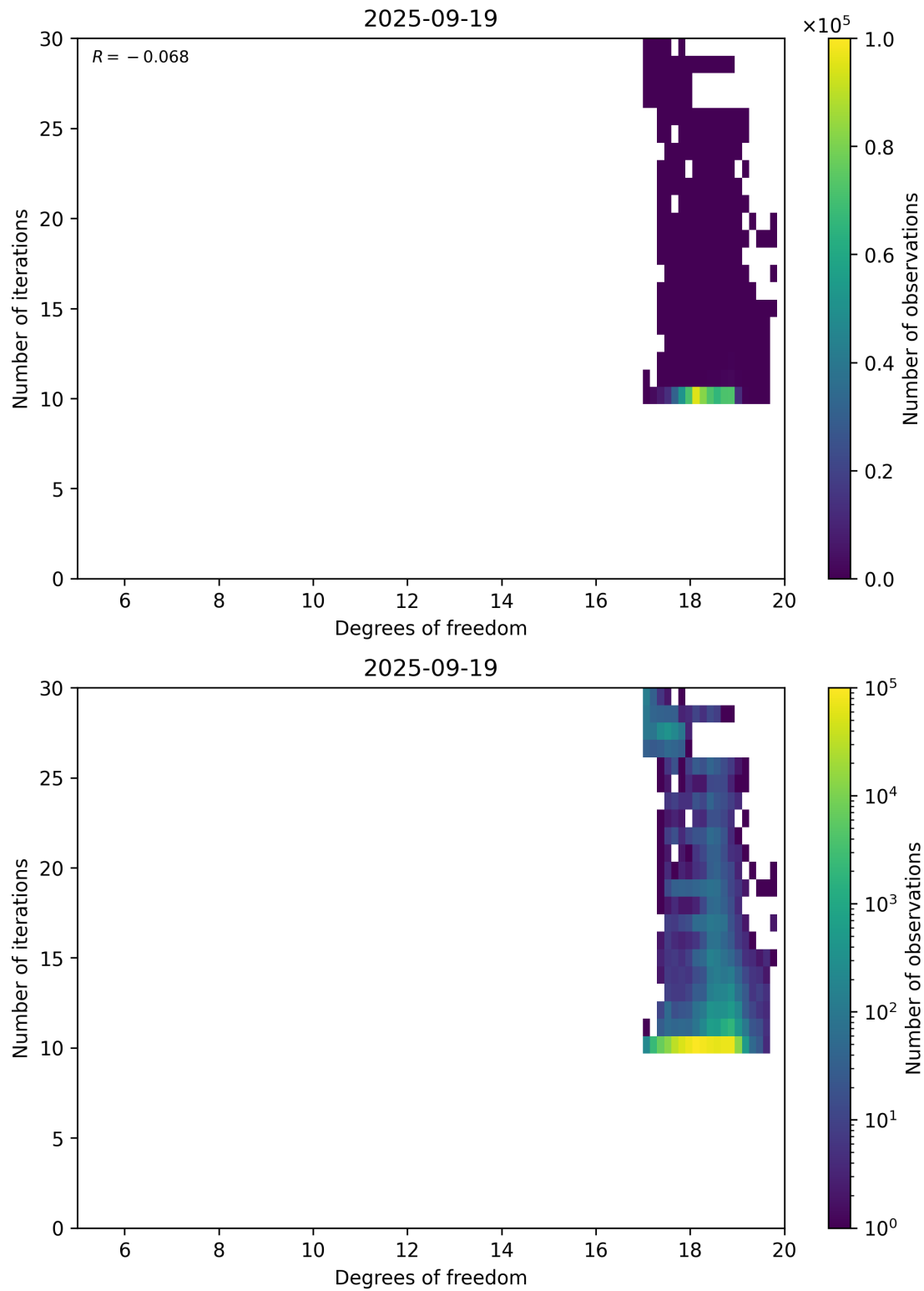
Figure 52: Scatter density plot of “Degrees of freedom” against “Number of iterations” for 2025-09-18 to 2025-09-20.
