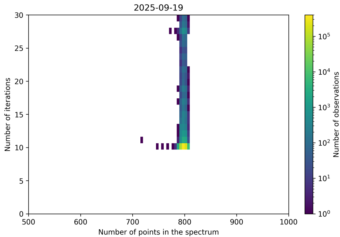
Figure 92: Scatter density plot of “Number of points in the spectrum” against “Number of iterations” for 2025-09-18 to 2025-09-20.
