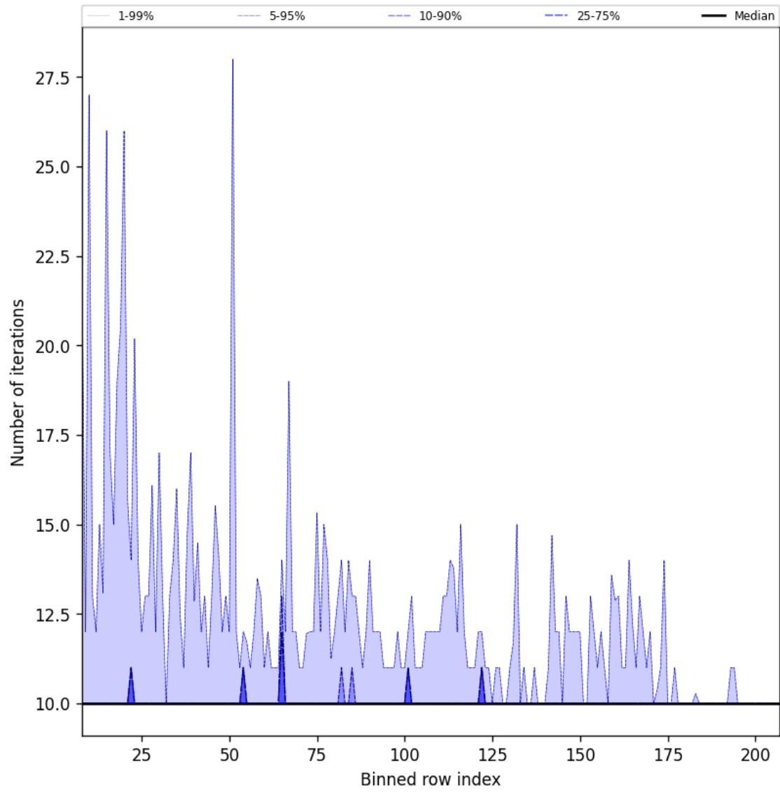
Figure 42: Along track statistics of “Number of iterations” for 2025-09-18 to 2025-09-20
