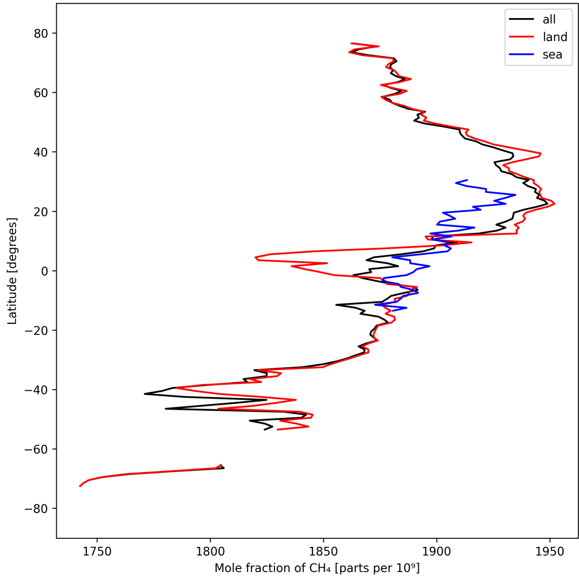
Figure 12: Zonal average of “Mole fraction of CH 4 ” for 2025-09-18 to 2025-09-20.
