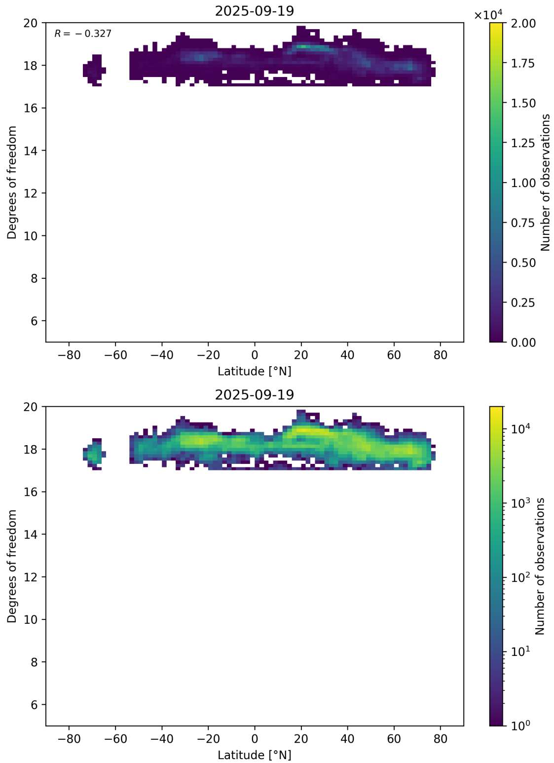
Figure 55: Scatter density plot of “Latitude” against “Degrees of freedom” for 2025-09-18 to 2025-09-20.
