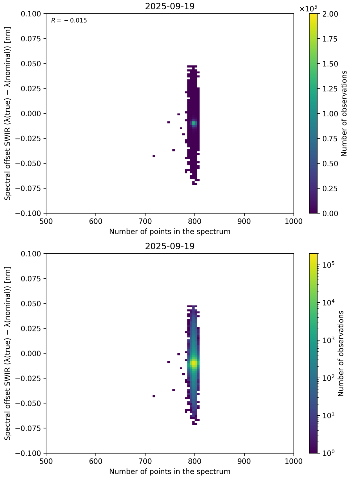
Figure 93: Scatter density plot of “Number of points in the spectrum” against “Spectral offset SWIR ( \lambda_{\text{true}} - \lambda_{\text{nominal}} )” for 2025-09-18 to 2025-09-20.
