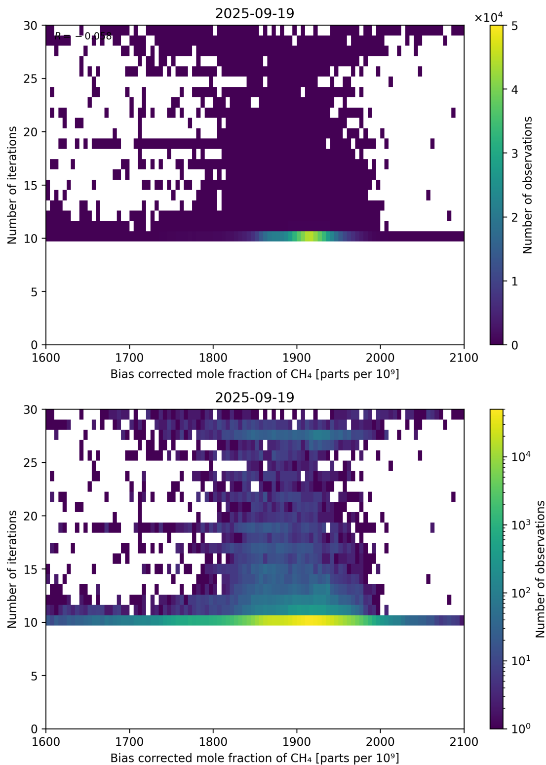
Figure 67: Scatter density plot of “Bias corrected mole fraction of CH 4 ” against “Number of iterations” for 2025-09-18 to 2025-09-20.
