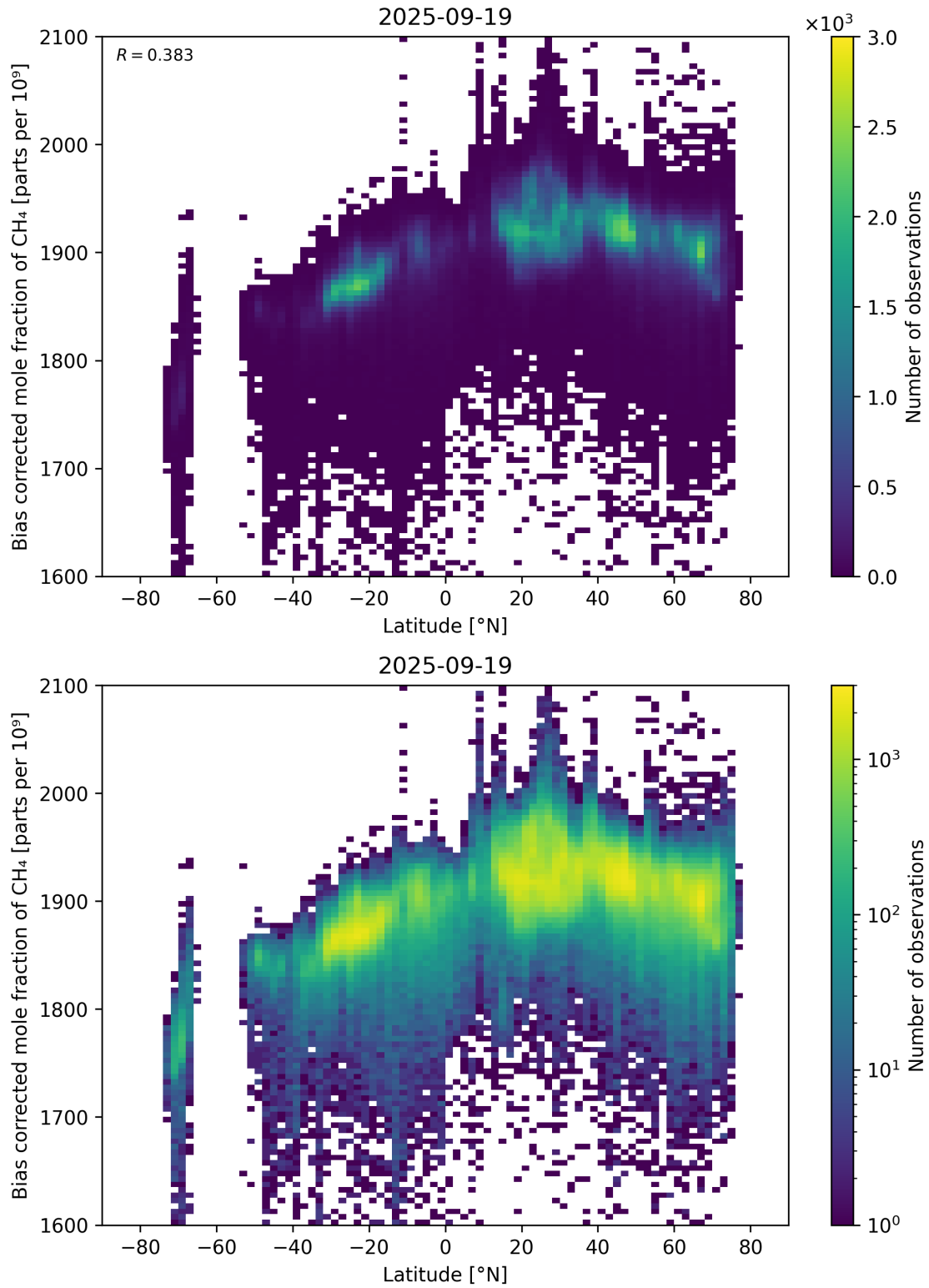
Figure 58: Scatter density plot of “Latitude” against “Bias corrected mole fraction of \text{CH}_4 ” for 2025-09-18 to 2025-09-20.
