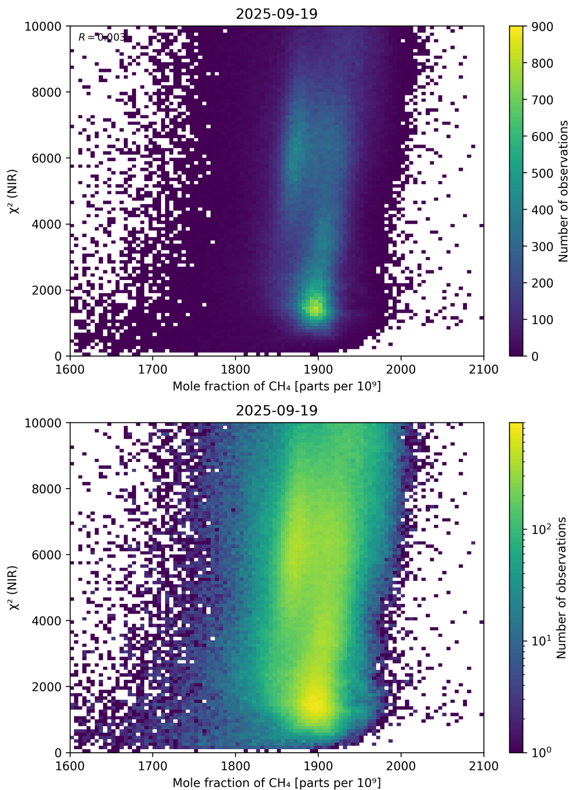
Figure 70: Scatter density plot of “Mole fraction of CH 4 ” against “ \chi^2 (NIR)” for 2025-09-18 to 2025-09-20.
