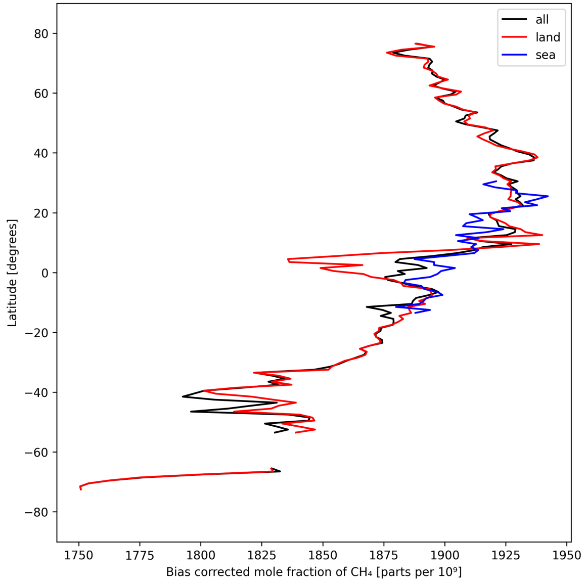
Figure 14: Zonal average of “Bias corrected mole fraction of CH 4 ” for 2025-09-18 to 2025-09-20.
