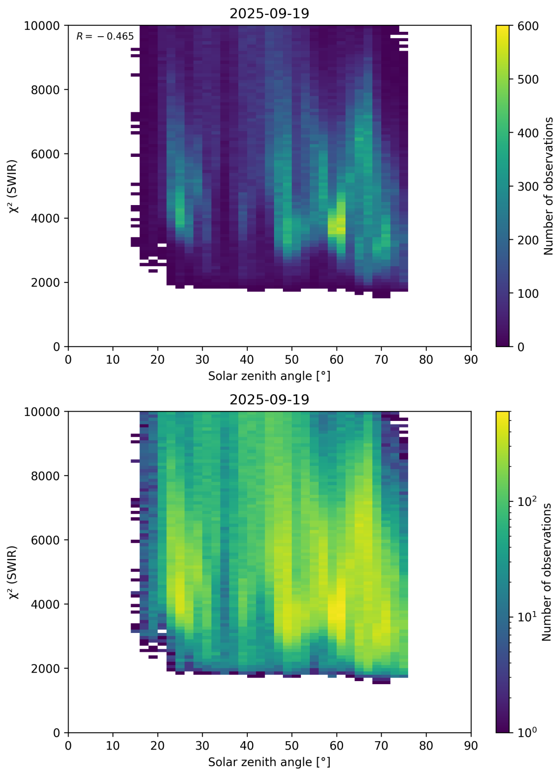
Figure 95: Scatter density plot of “Solar zenith angle” against “ \chi^2 (SWIR)” for 2025-09-18 to 2025-09-20.
