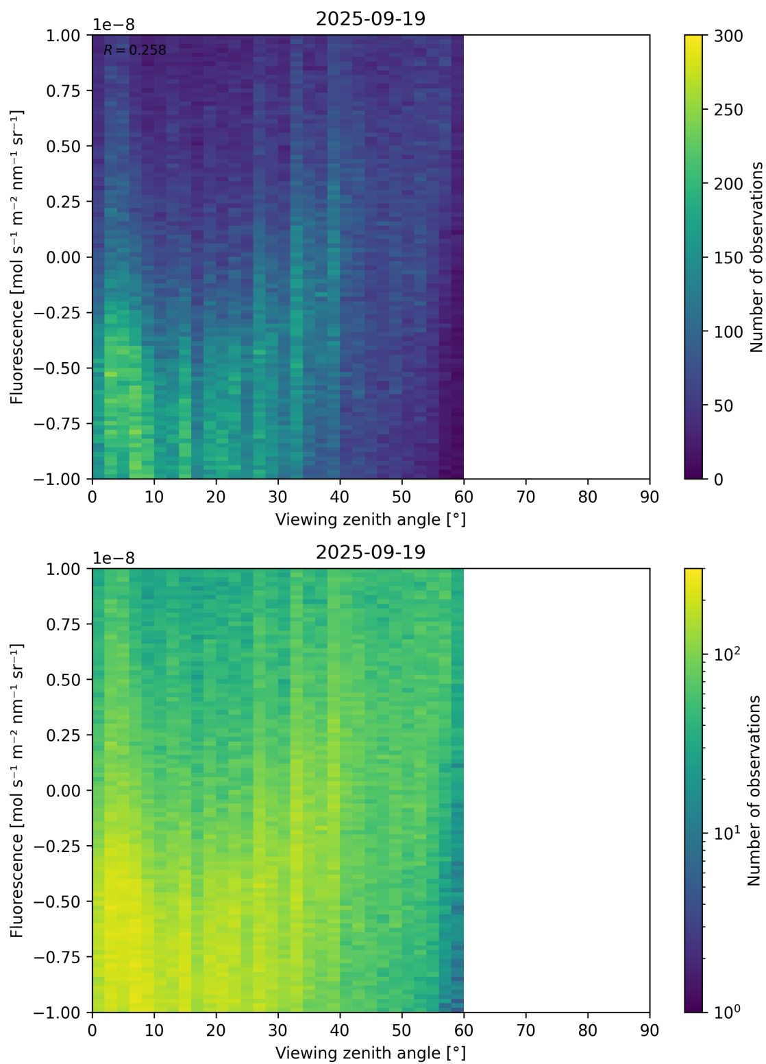
Figure 108: Scatter density plot of “Viewing zenith angle” against “Fluorescence” for 2025-09-18 to 2025-09-20.
