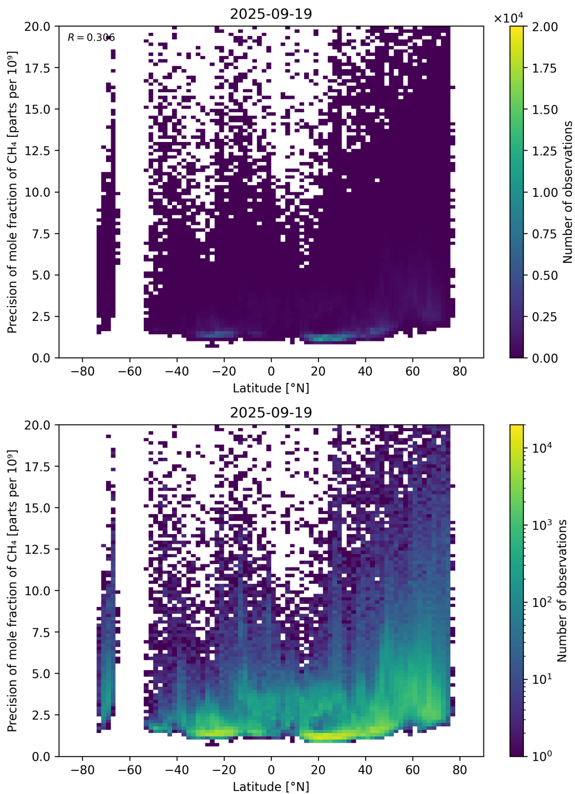
Figure 59: Scatter density plot of “Latitude” against “Precision of mole fraction of \text{CH}_4 ” for 2025-09-18 to 2025-09-20.
