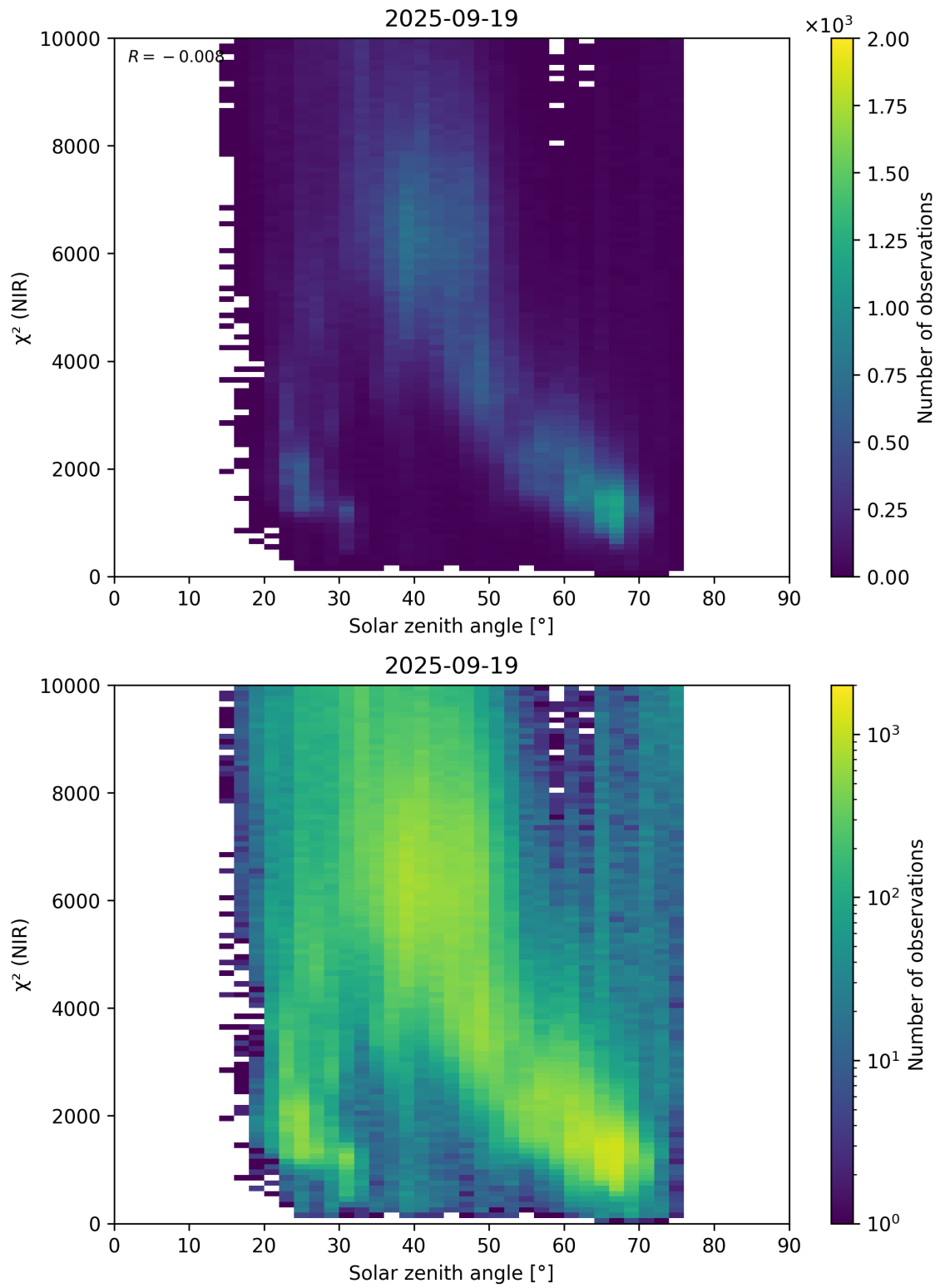
Figure 94: Scatter density plot of “Solar zenith angle” against “ \chi^2 (NIR)” for 2025-09-18 to 2025-09-20.
