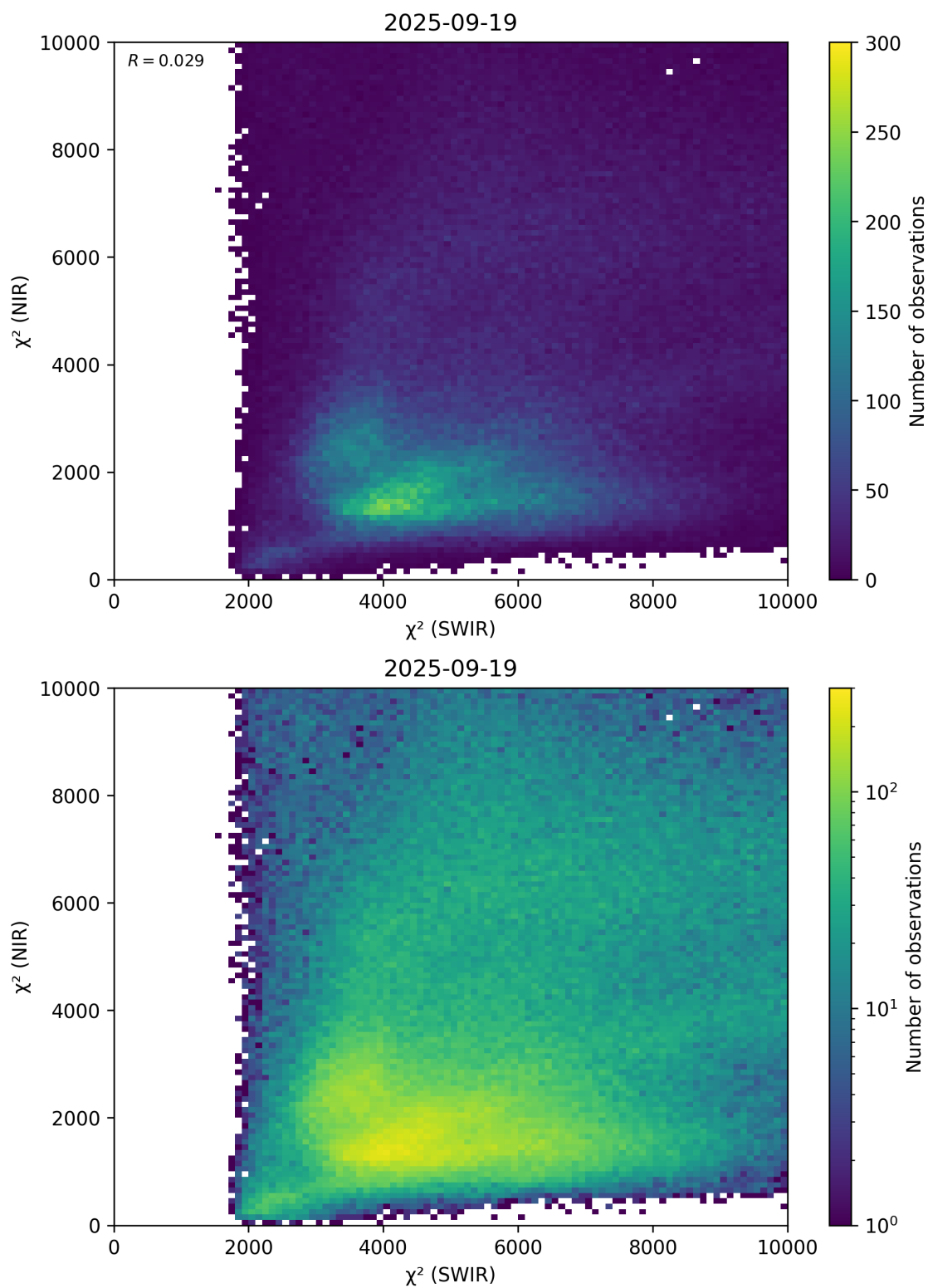
Figure 47: Scatter density plot of “ \chi^2 (SWIR)” against “ \chi^2 (NIR)” for 2025-09-18 to 2025-09-20.
