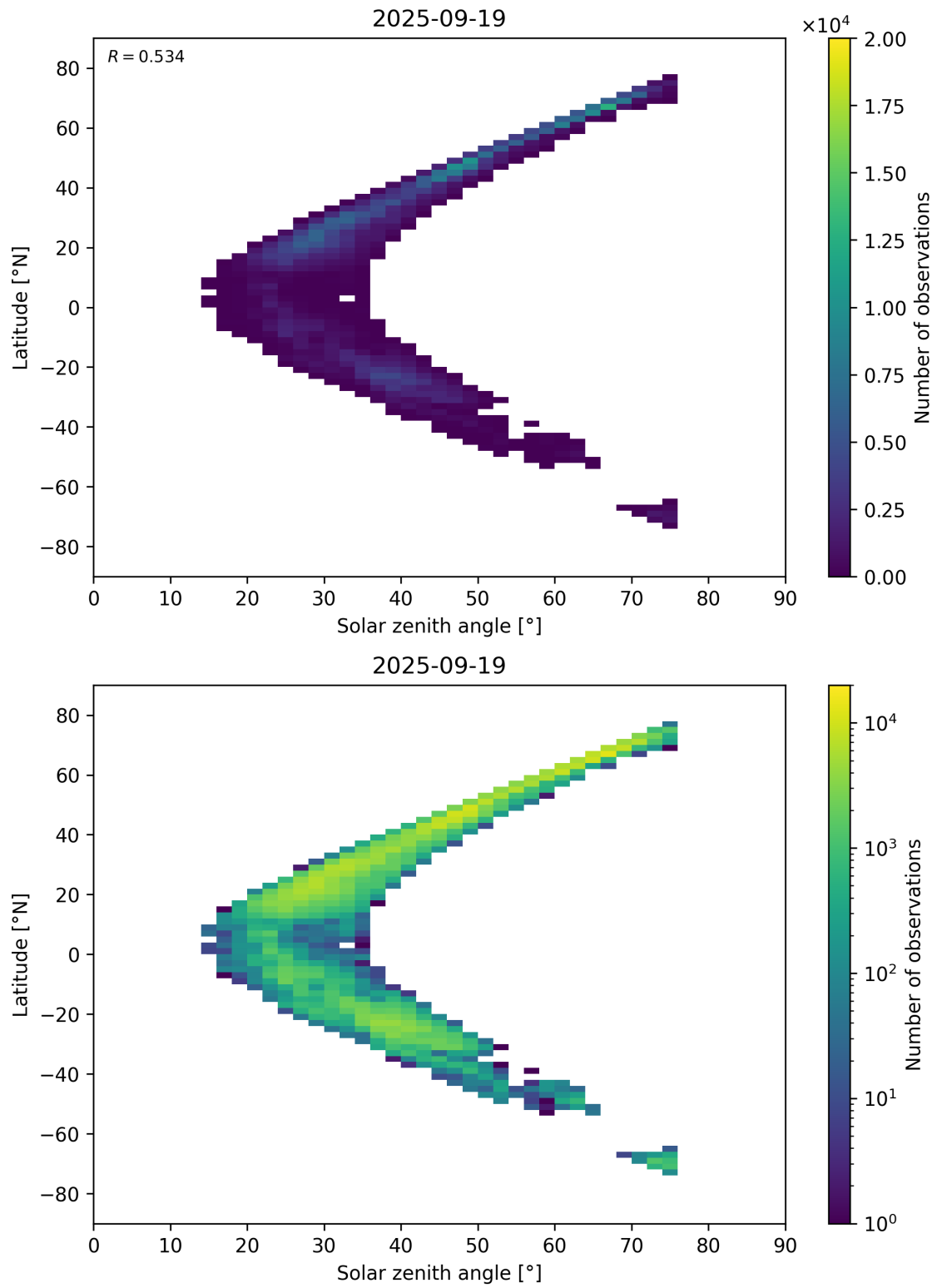
Figure 98: Scatter density plot of “Solar zenith angle” against “Latitude” for 2025-09-18 to 2025-09-20.
