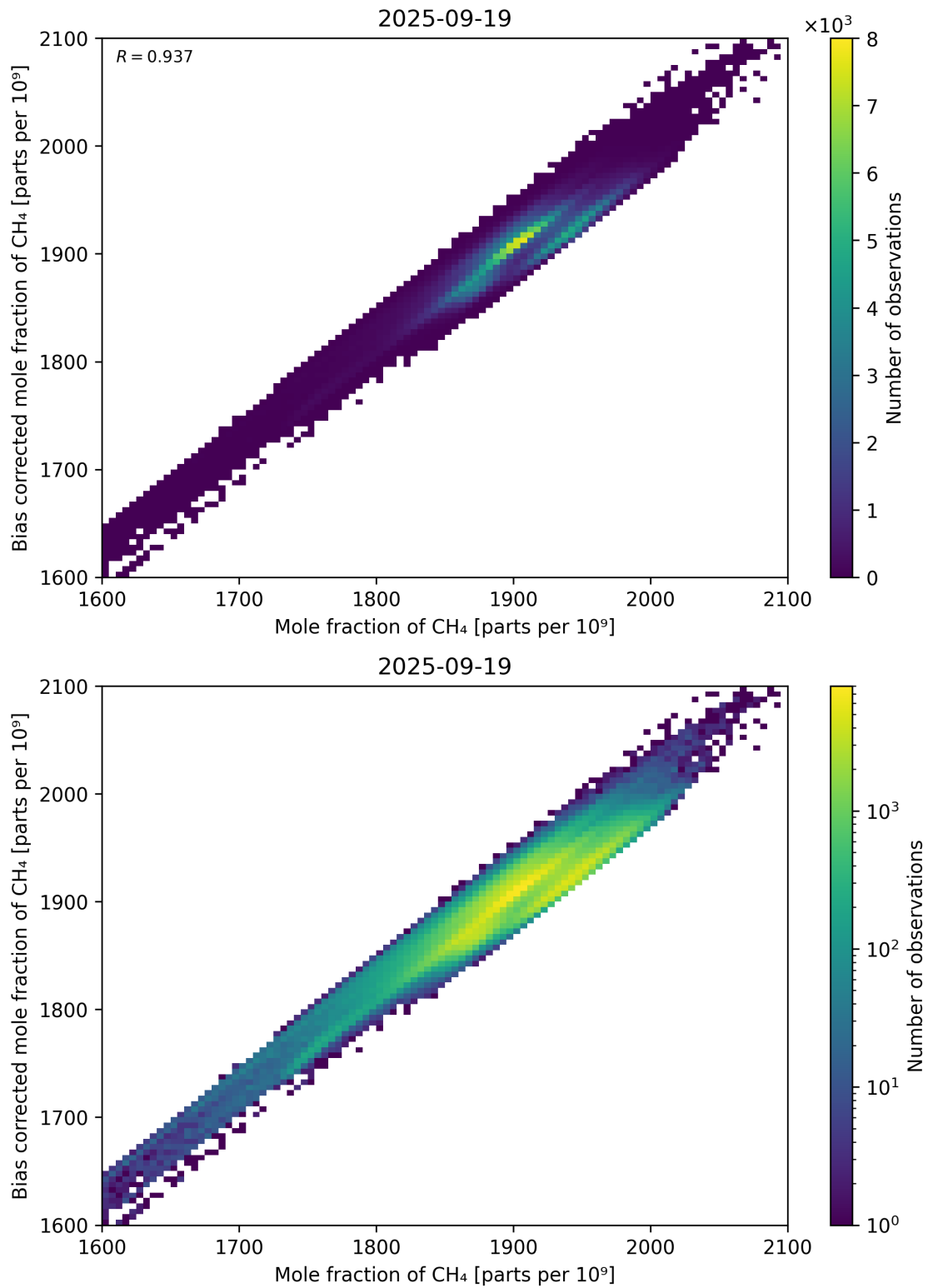
Figure 74: Scatter density plot of “Mole fraction of CH 4 ” against “Bias corrected mole fraction of CH 4 ” for 2025-09-18 to 2025-09-20.
