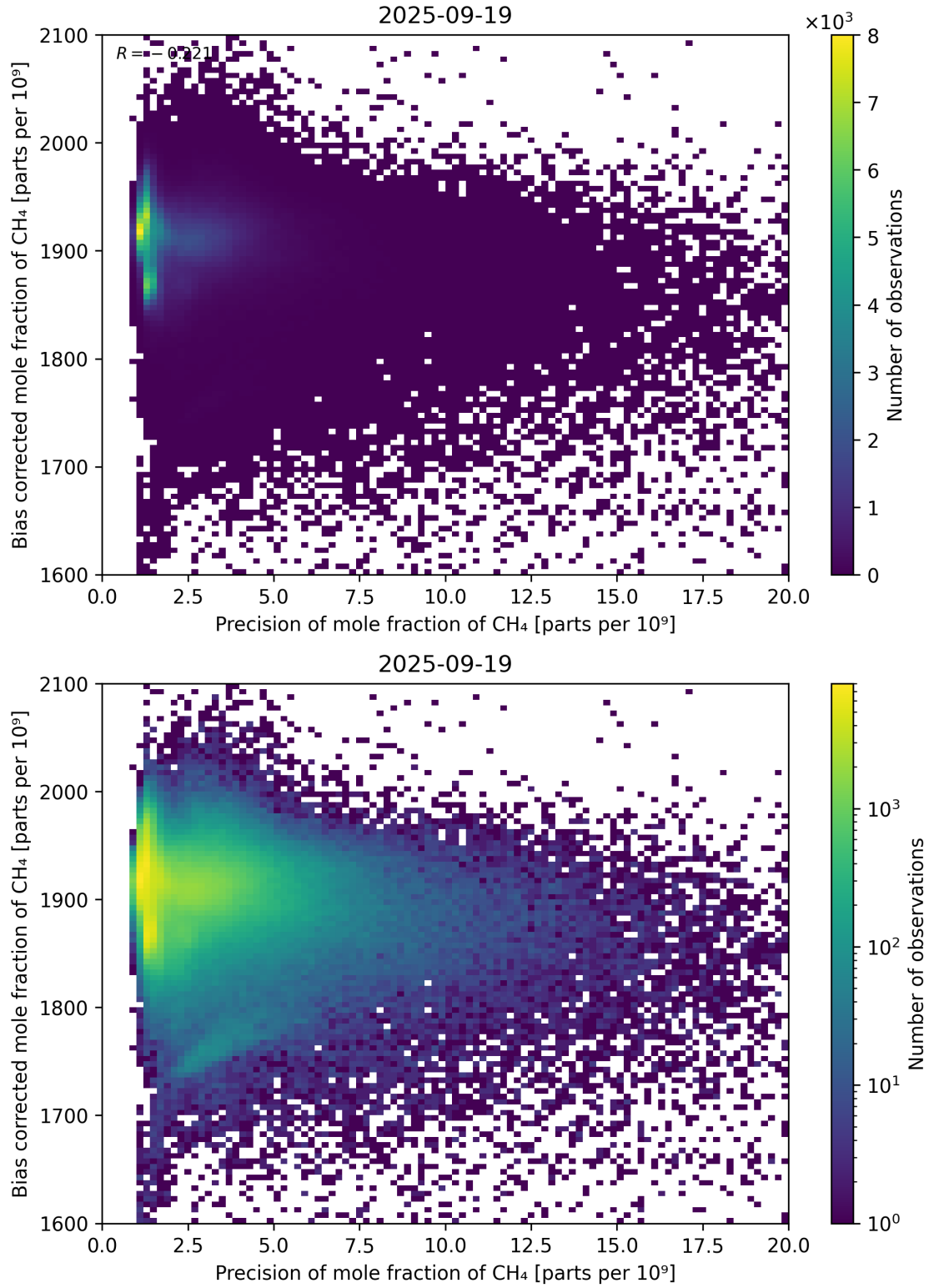
Figure 82: Scatter density plot of “Precision of mole fraction of CH 4 ” against “Bias corrected mole fraction of CH 4 ” for 2025-09-18 to 2025-09-20.
