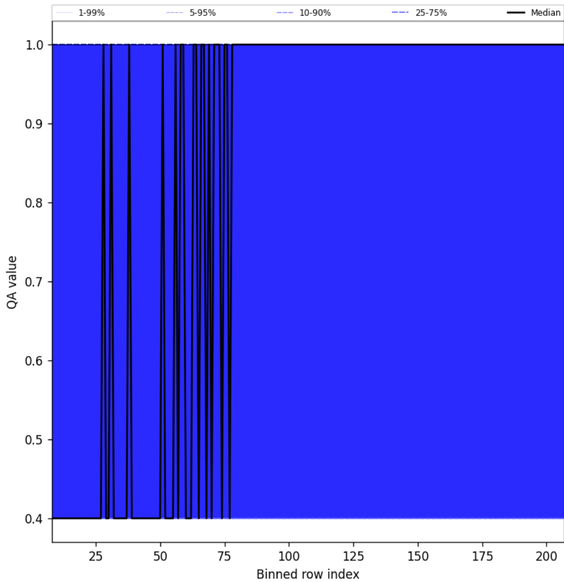
Figure 33: Along track statistics of “QA value” for 2025-09-18 to 2025-09-20
