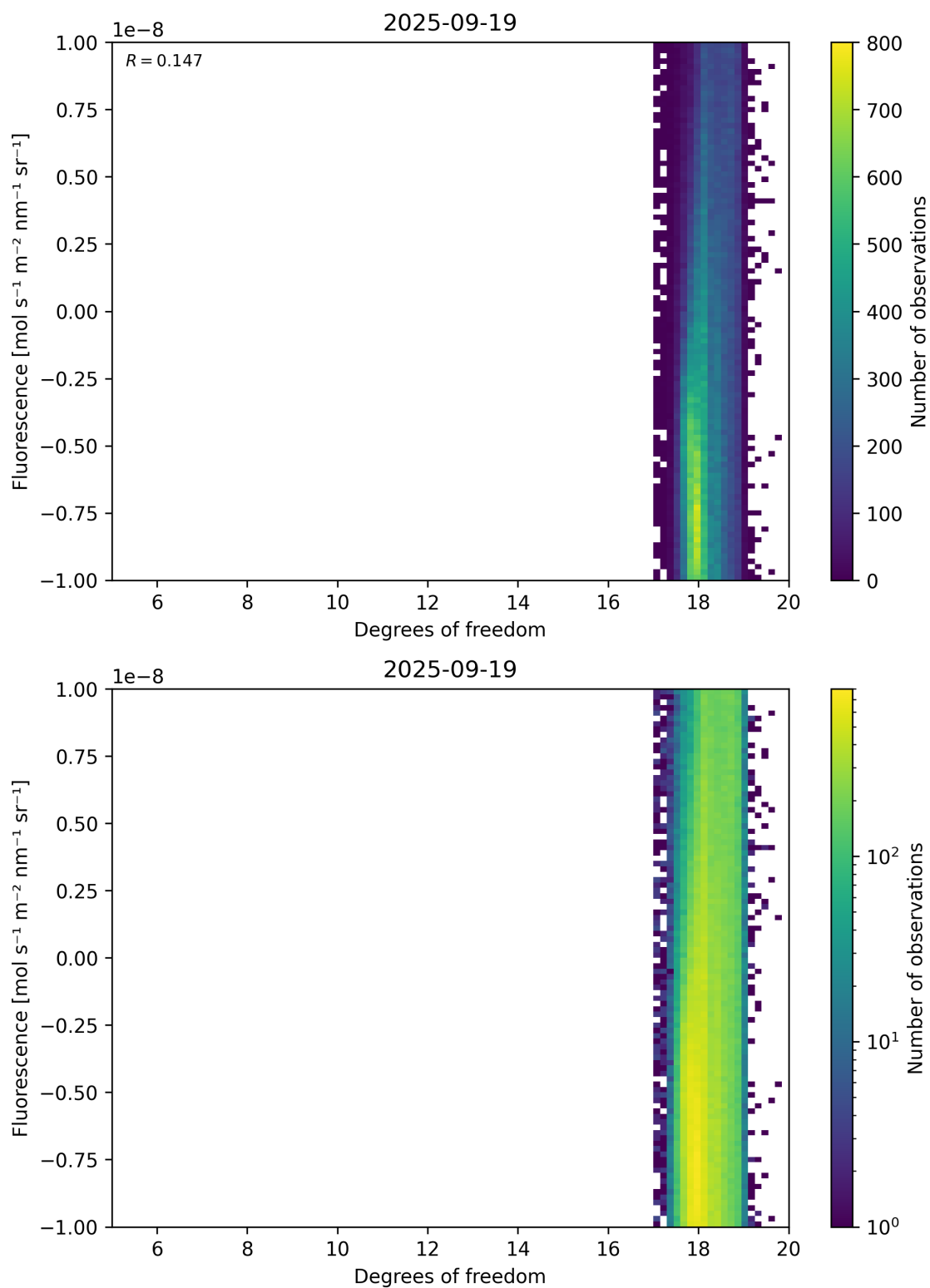
Figure 51: Scatter density plot of “Degrees of freedom” against “Fluorescence” for 2025-09-18 to 2025-09-20.
