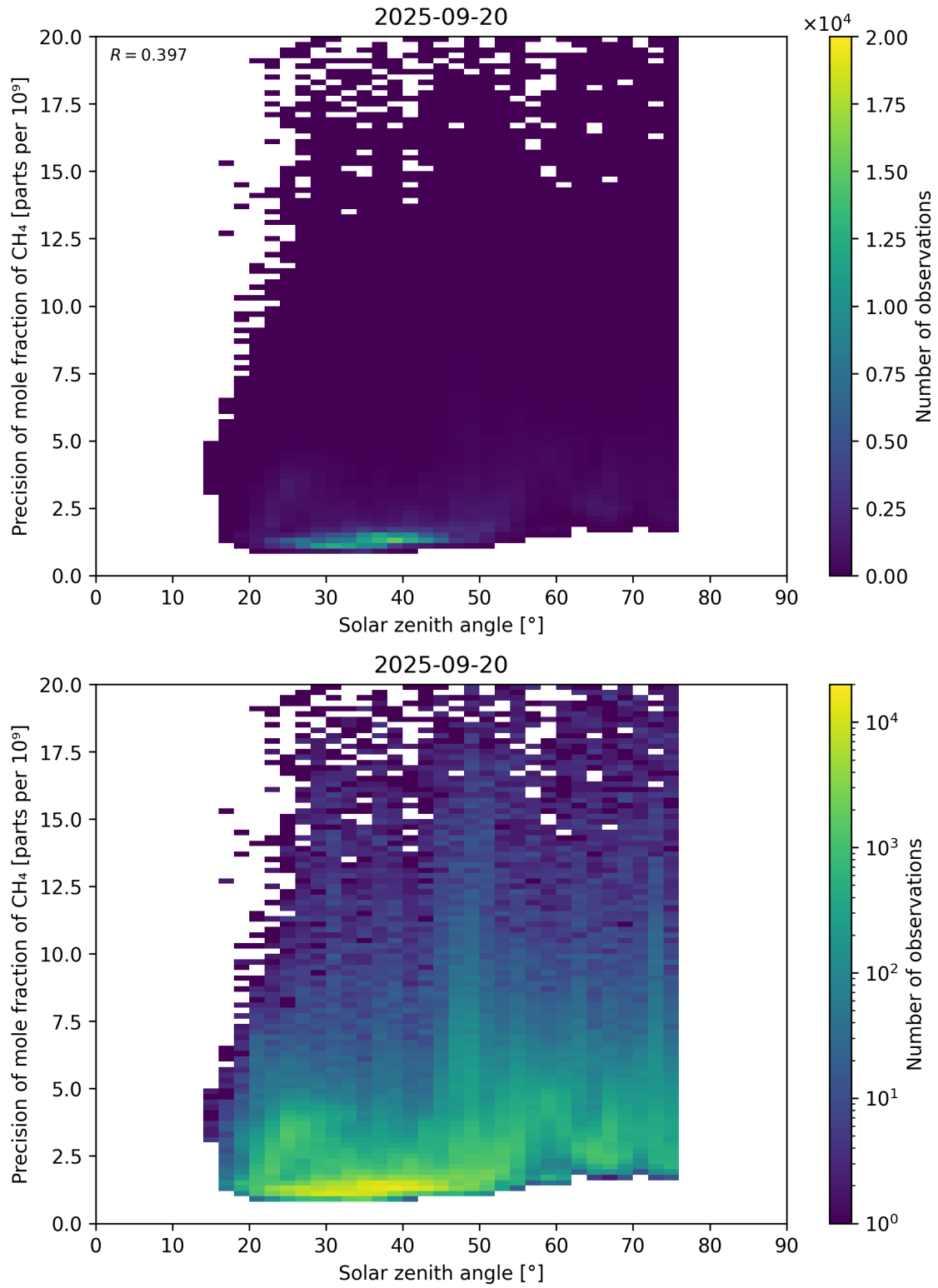
Figure 101: Scatter density plot of “Solar zenith angle” against “Precision of mole fraction of \text{CH}_4 ” for 2025-09-20 to 2025-09-21.
