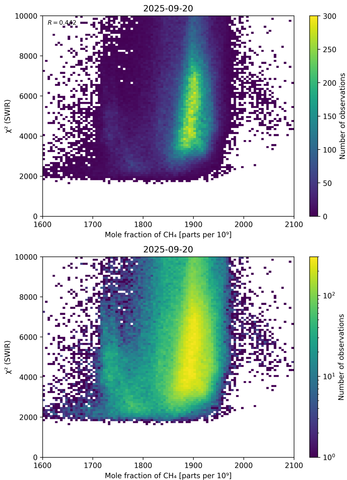
Figure 71: Scatter density plot of “Mole fraction of \text{CH}_4 ” against “ \chi^2 (SWIR)” for 2025-09-20 to 2025-09-21.
