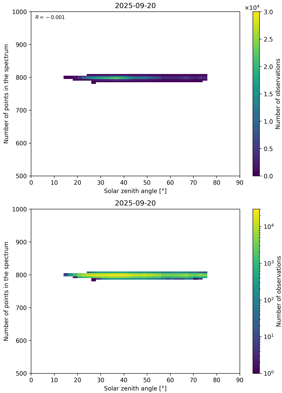
Figure 103: Scatter density plot of “Solar zenith angle” against “Number of points in the spectrum” for 2025-09-20 to 2025-09-21.
