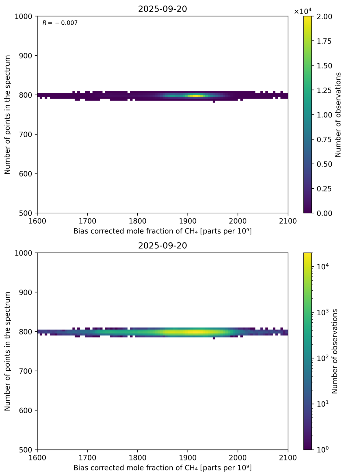
Figure 68: Scatter density plot of “Bias corrected mole fraction of CH 4 ” against “Number of points in the spectrum” for 2025-09-20 to 2025-09-21.
