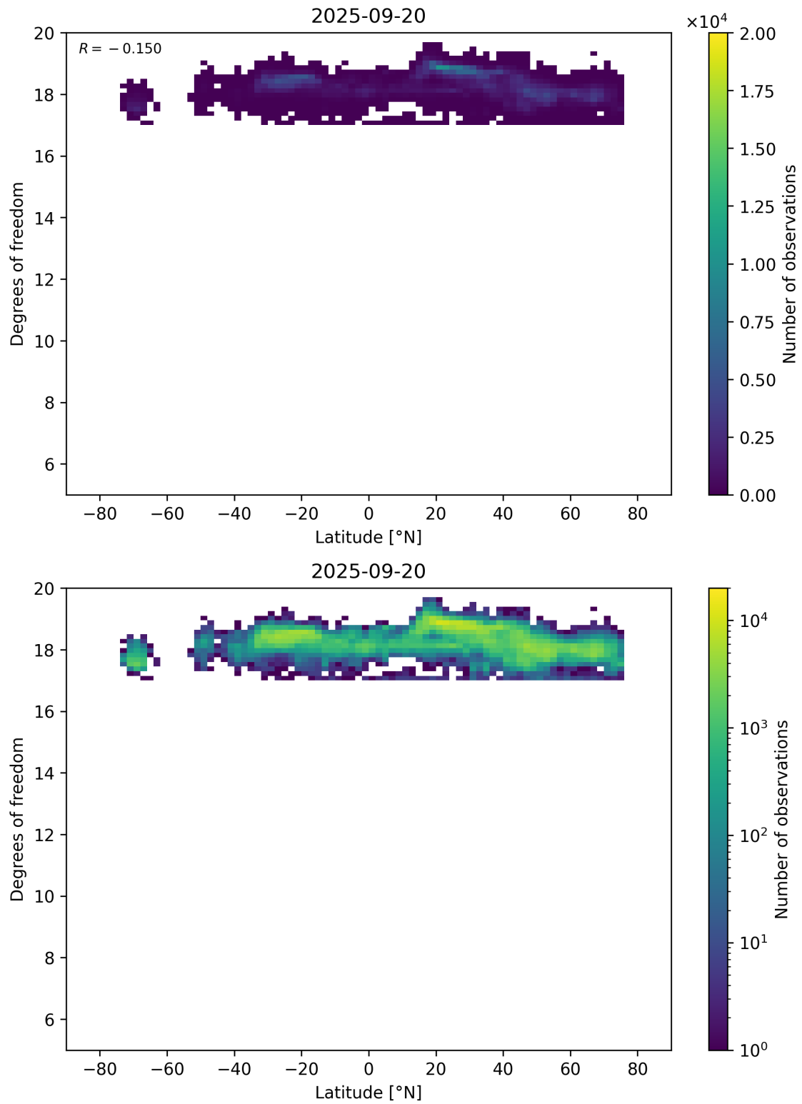
Figure 55: Scatter density plot of “Latitude” against “Degrees of freedom” for 2025-09-20 to 2025-09-21.
