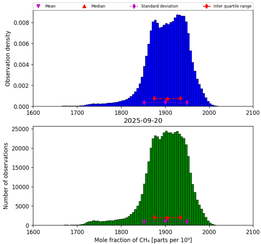
Figure 23: Histogram of “Mole fraction of CH 4 ” for 2025-09-20 to 2025-09-21
