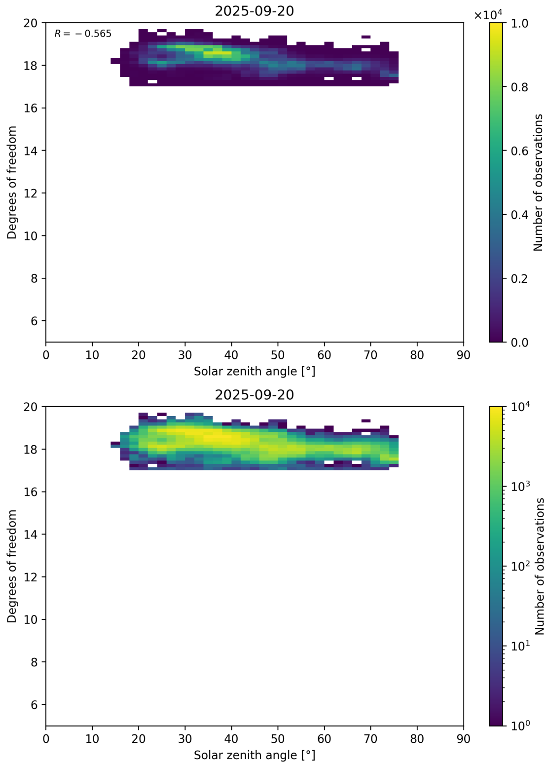
Figure 96: Scatter density plot of “Solar zenith angle” against “Degrees of freedom” for 2025-09-20 to 2025-09-21.
