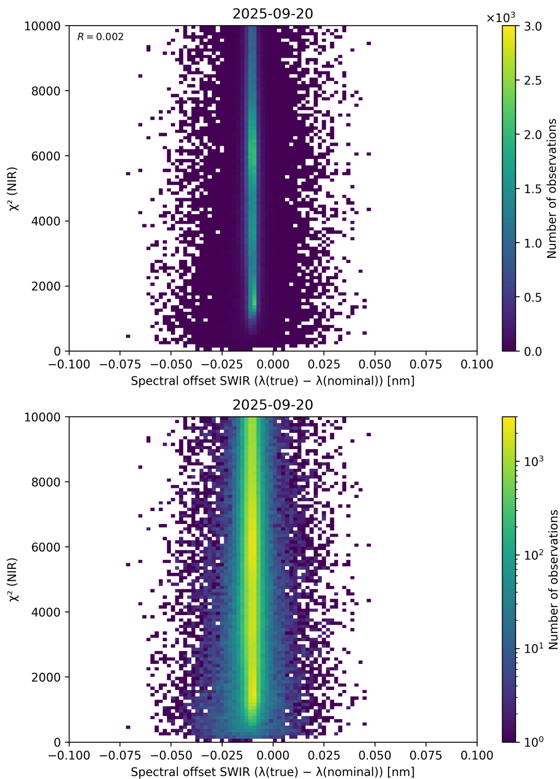
Figure 117: Scatter density plot of “Spectral offset SWIR ( \lambda_{\text{true}} - \lambda_{\text{nominal}} )” against “ \chi^2 (NIR)” for 2025-09-20 to 2025-09-21.
