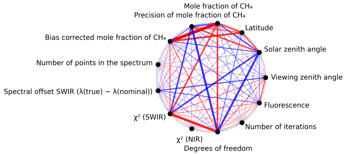
Figure 1: Map of correlation graph for 2025-09-20 to 2025-09-21.
