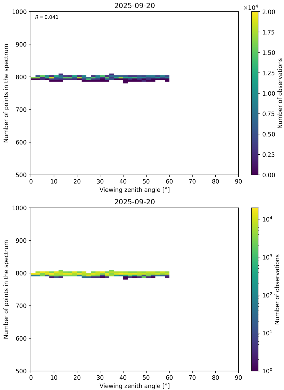
Figure 114: Scatter density plot of “Viewing zenith angle” against “Number of points in the spectrum” for 2025-09-20 to 2025-09-21.
