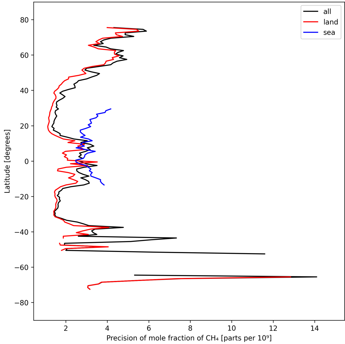
Figure 13: Zonal average of “Precision of mole fraction of CH 4 ” for 2025-09-20 to 2025-09-21.
