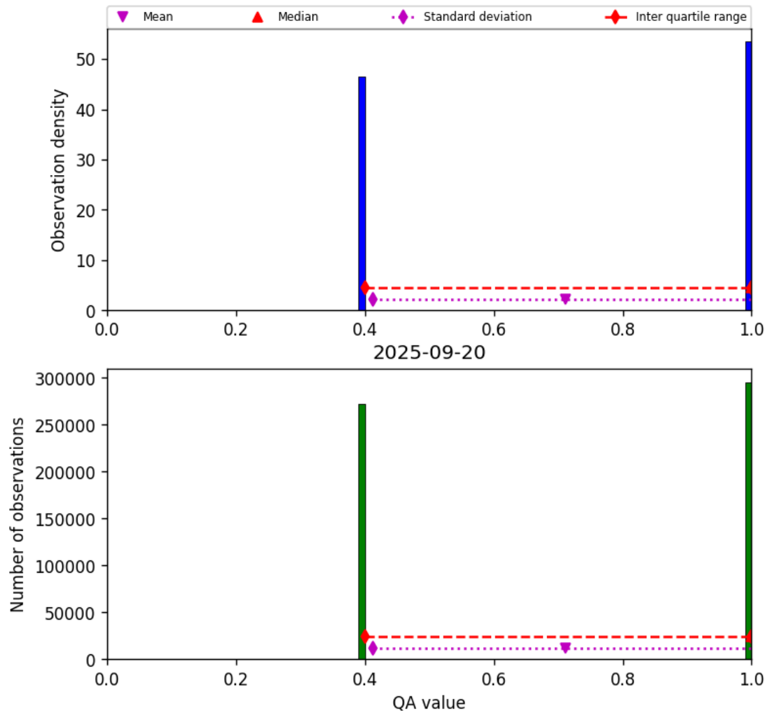
Figure 22: Histogram of “QA value” for 2025-09-20 to 2025-09-21
