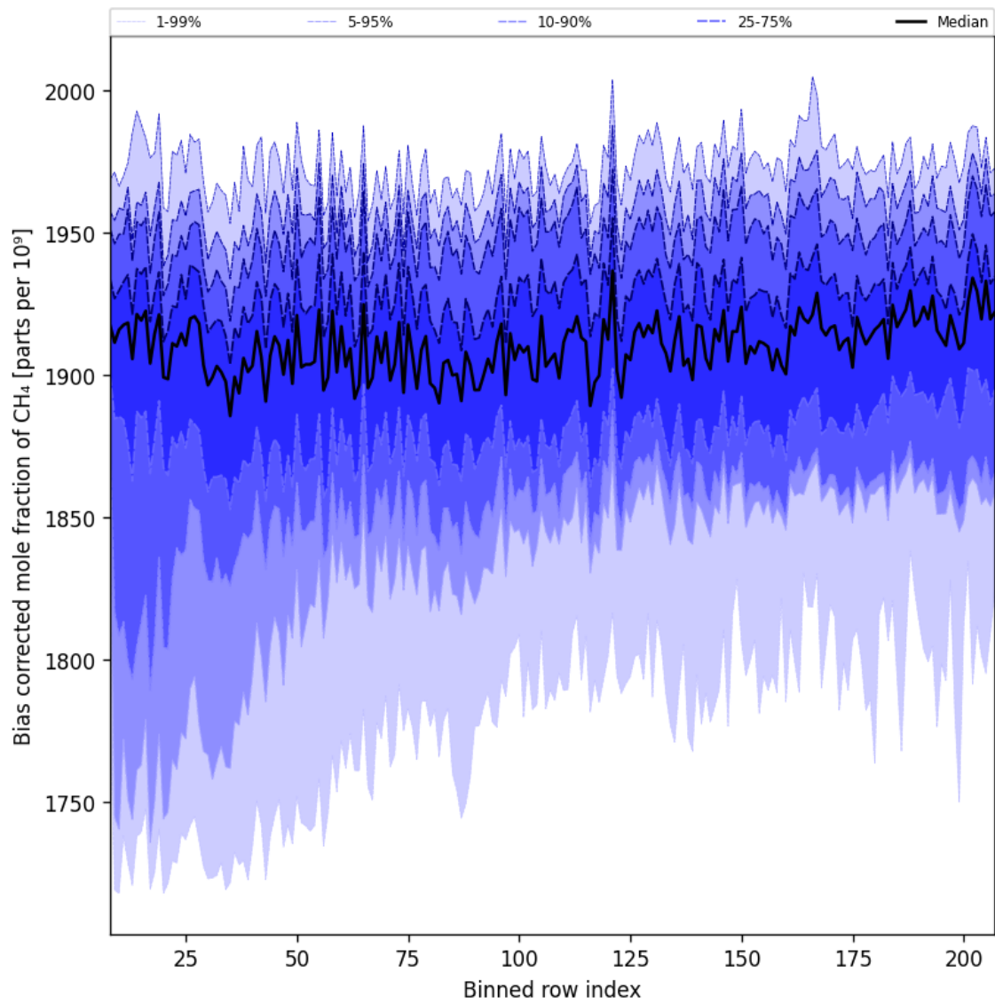
Figure 36: Along track statistics of “Bias corrected mole fraction of CH 4 ” for 2025-09-20 to 2025-09-21
