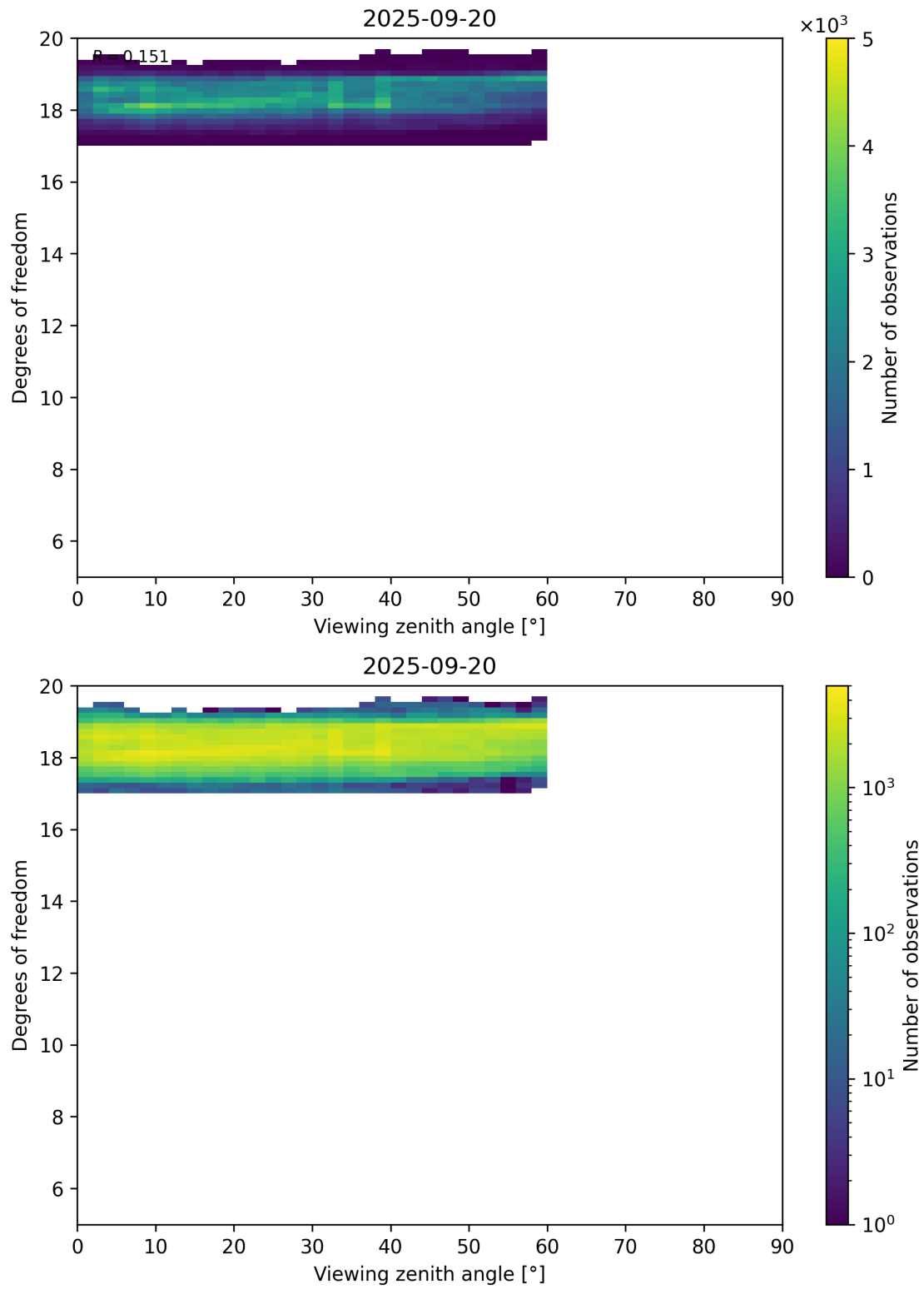
Figure 107: Scatter density plot of “Viewing zenith angle” against “Degrees of freedom” for 2025-09-20 to 2025-09-21.
