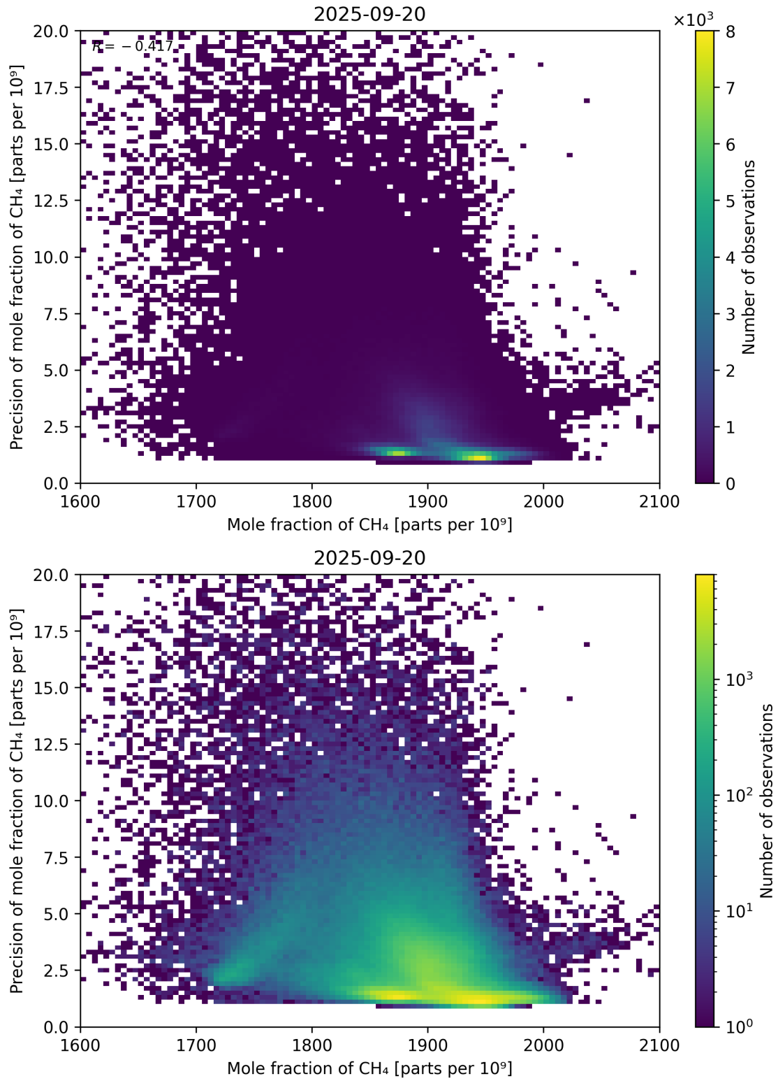
Figure 75: Scatter density plot of “Mole fraction of CH 4 ” against “Precision of mole fraction of CH 4 ” for 2025-09-20 to 2025-09-21.
