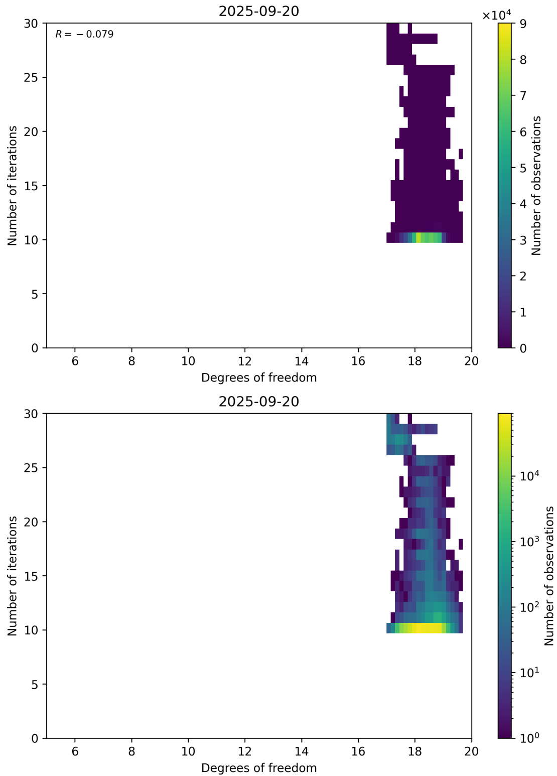
Figure 52: Scatter density plot of “Degrees of freedom” against “Number of iterations” for 2025-09-20 to 2025-09-21.
