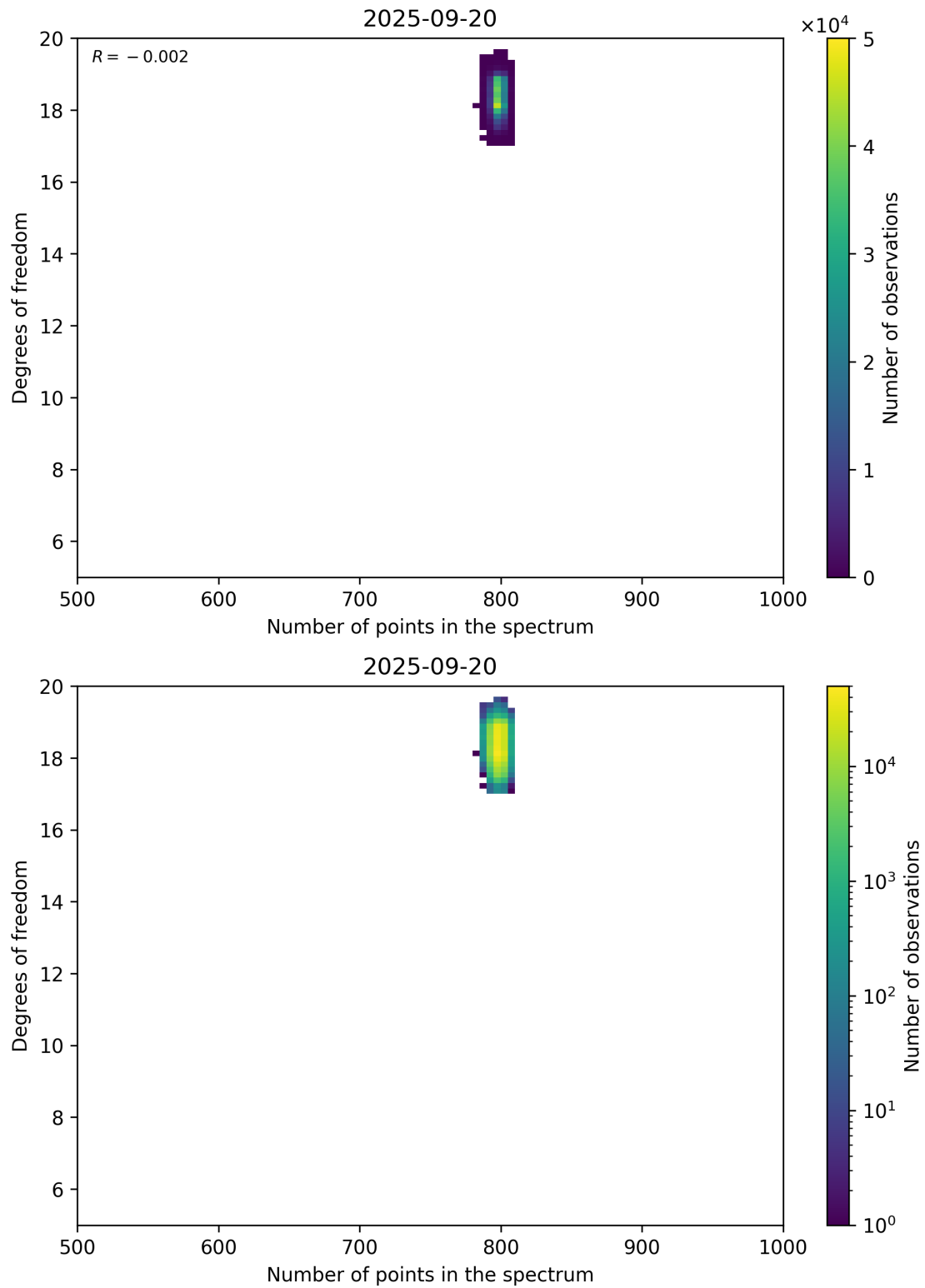
Figure 90: Scatter density plot of “Number of points in the spectrum” against “Degrees of freedom” for 2025-09-20 to 2025-09-21.
