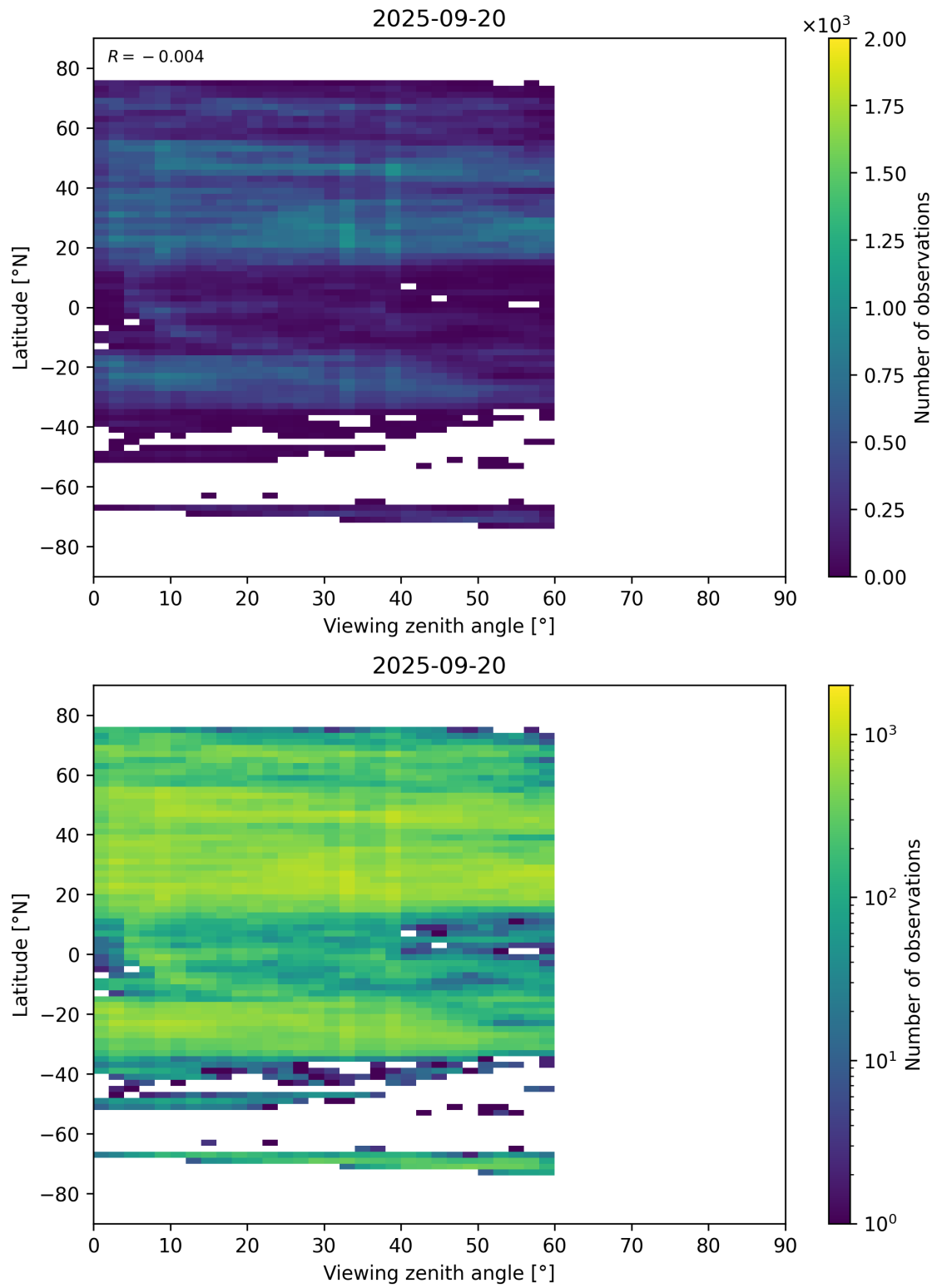
Figure 109: Scatter density plot of “Viewing zenith angle” against “Latitude” for 2025-09-20 to 2025-09-21.
