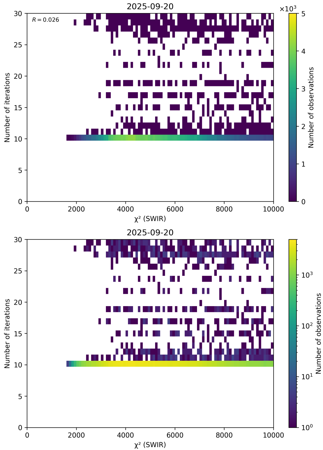
Figure 50: Scatter density plot of “ \chi^2 (SWIR)” against “Number of iterations” for 2025-09-20 to 2025-09-21.
