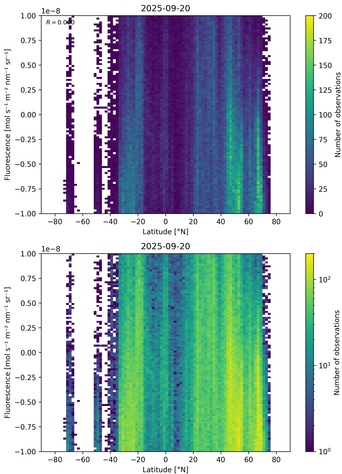
Figure 56: Scatter density plot of “Latitude” against “Fluorescence” for 2025-09-20 to 2025-09-21.
