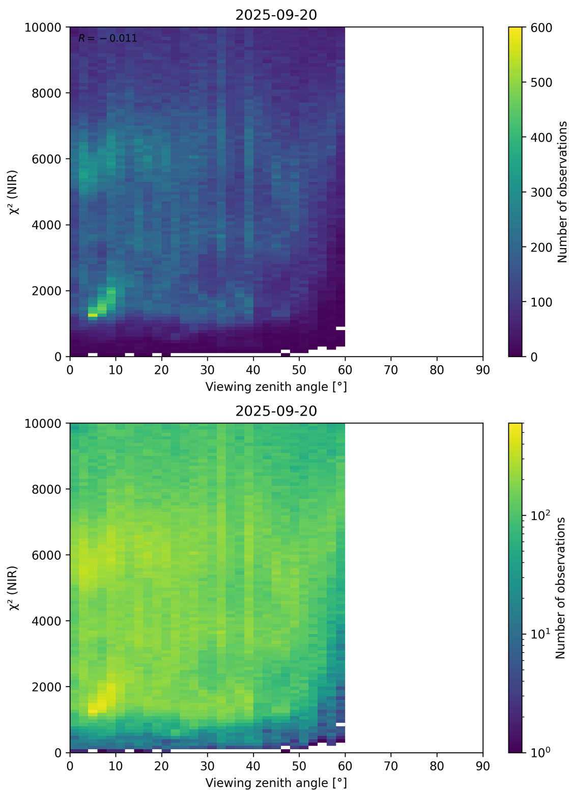
Figure 105: Scatter density plot of “Viewing zenith angle” against “ \chi^2 (NIR)” for 2025-09-20 to 2025-09-21.
