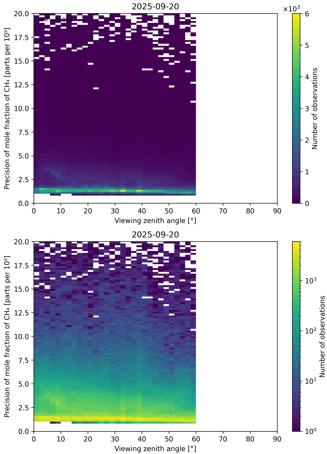
Figure 112: Scatter density plot of “Viewing zenith angle” against “Precision of mole fraction of CH 4 ” for 2025-09-20 to 2025-09-21.
