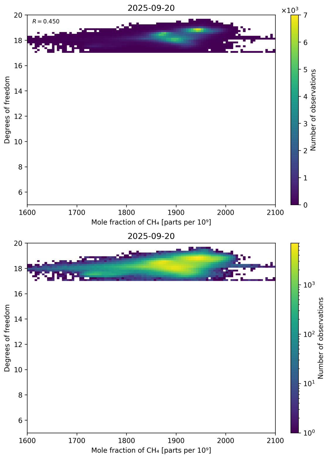
Figure 72: Scatter density plot of “Mole fraction of CH 4 ” against “Degrees of freedom” for 2025-09-20 to 2025-09-21.
