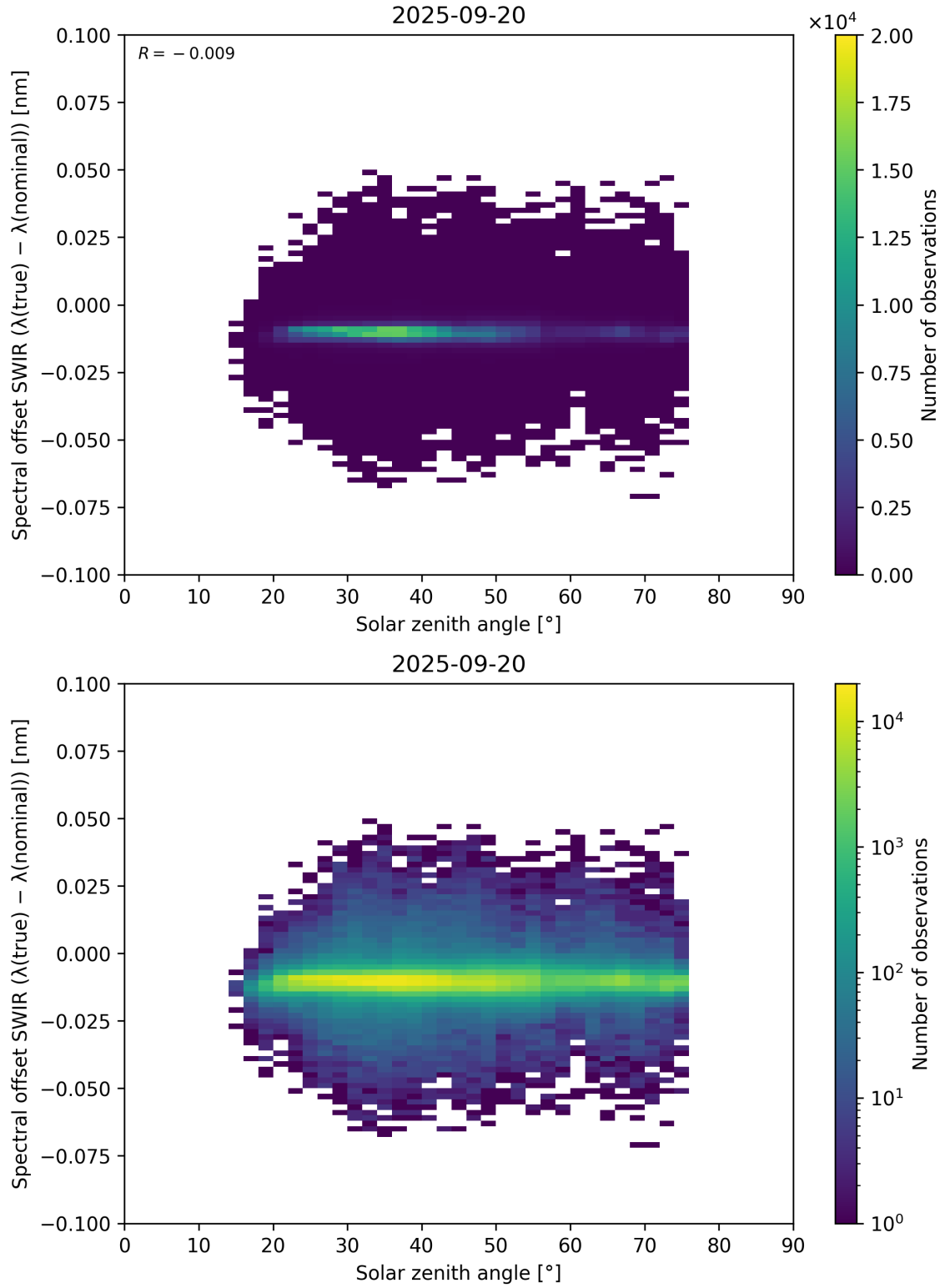
Figure 104: Scatter density plot of “Solar zenith angle” against “Spectral offset SWIR ( \lambda_{\text{true}} - \lambda_{\text{nominal}} )” for 2025-09-20 to 2025-09-21.
