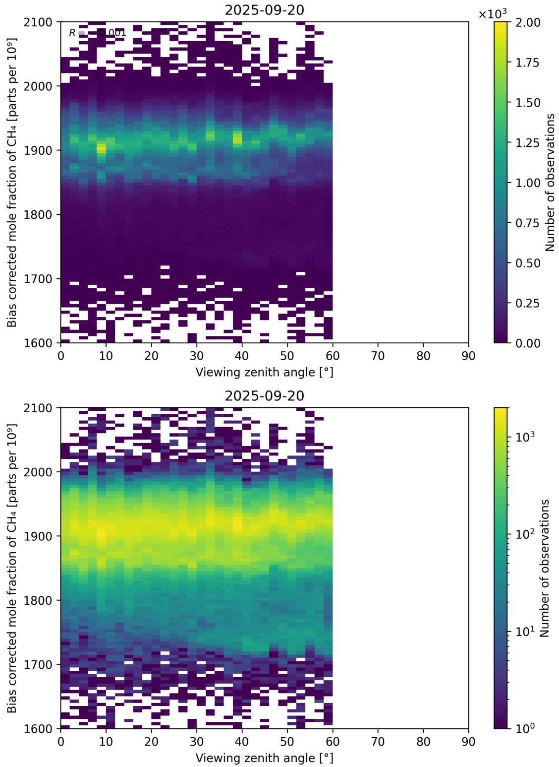
Figure 111: Scatter density plot of “Viewing zenith angle” against “Bias corrected mole fraction of CH 4 ” for 2025-09-20 to 2025-09-21.
