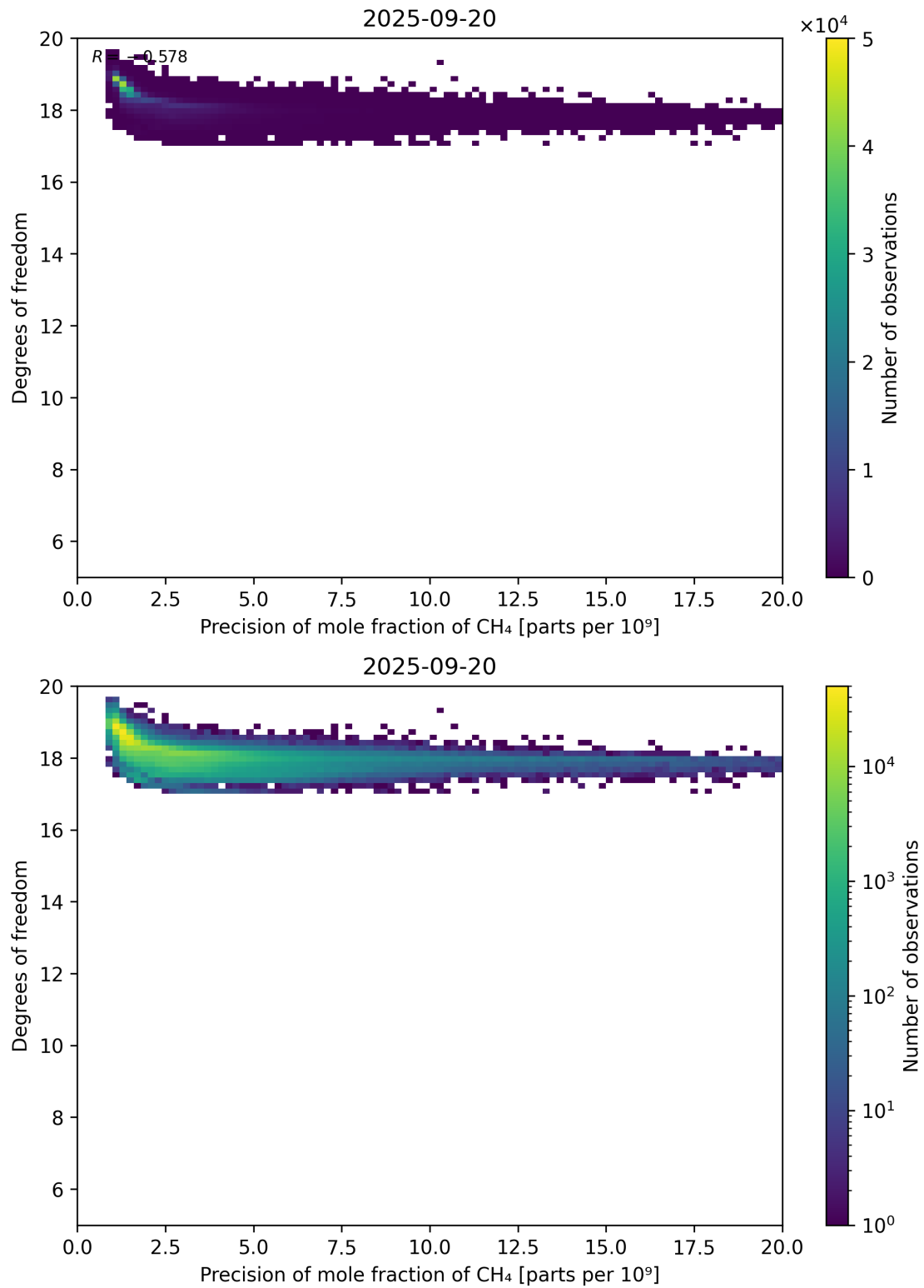
Figure 80: Scatter density plot of “Precision of mole fraction of CH 4 ” against “Degrees of freedom” for 2025-09-20 to 2025-09-21.
