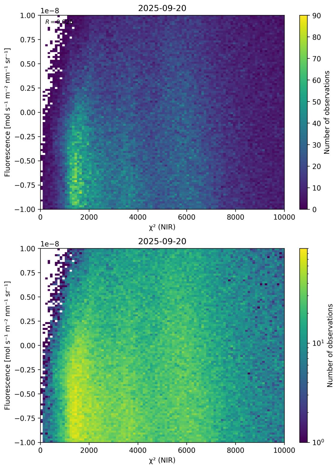
Figure 45: Scatter density plot of “ \chi^2 (NIR)” against “Fluorescence” for 2025-09-20 to 2025-09-21.
