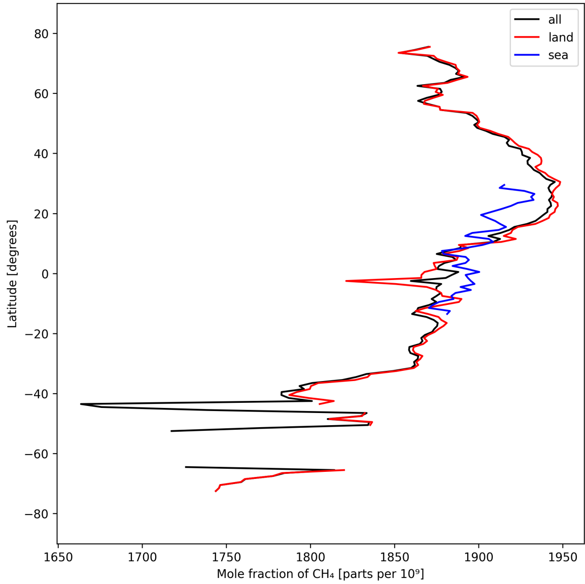
Figure 12: Zonal average of “Mole fraction of \text{CH}_4 ” for 2025-09-20 to 2025-09-21.
