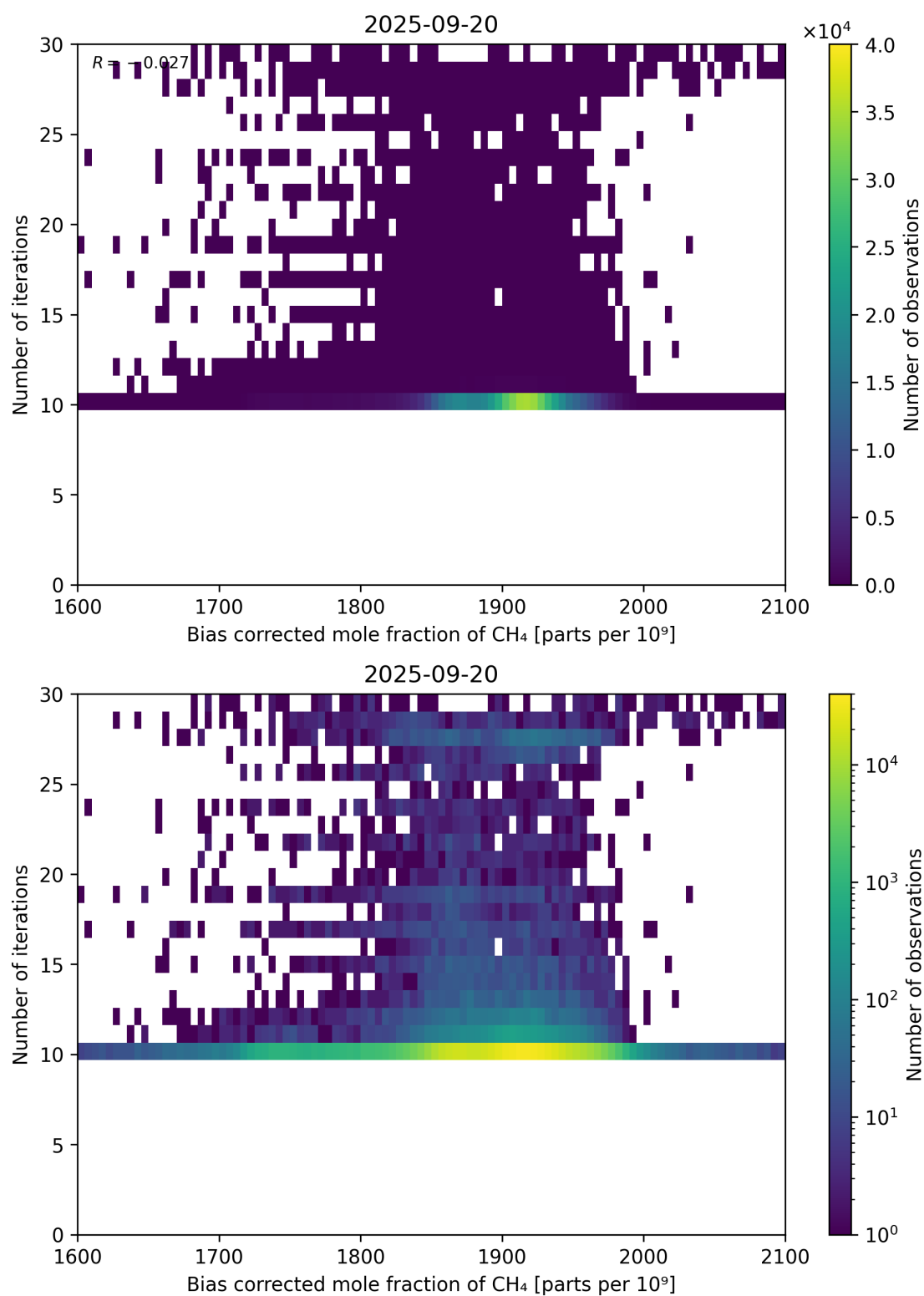
Figure 67: Scatter density plot of “Bias corrected mole fraction of CH 4 ” against “Number of iterations” for 2025-09-20 to 2025-09-21.
