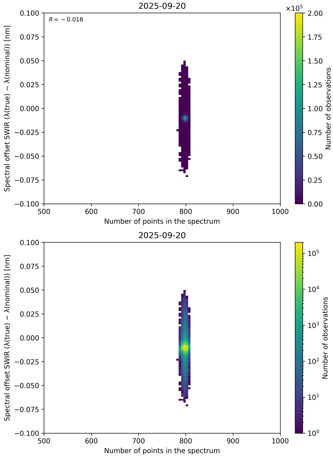
Figure 93: Scatter density plot of “Number of points in the spectrum” against “Spectral offset SWIR ( \lambda_{\text{true}} - \lambda_{\text{nominal}} )” for 2025-09-20 to 2025-09-21.
