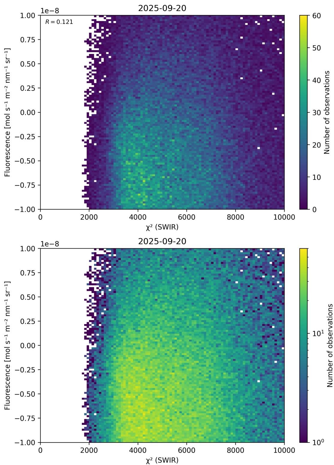
Figure 49: Scatter density plot of “ \chi^2 (SWIR)” against “Fluorescence” for 2025-09-20 to 2025-09-21.
