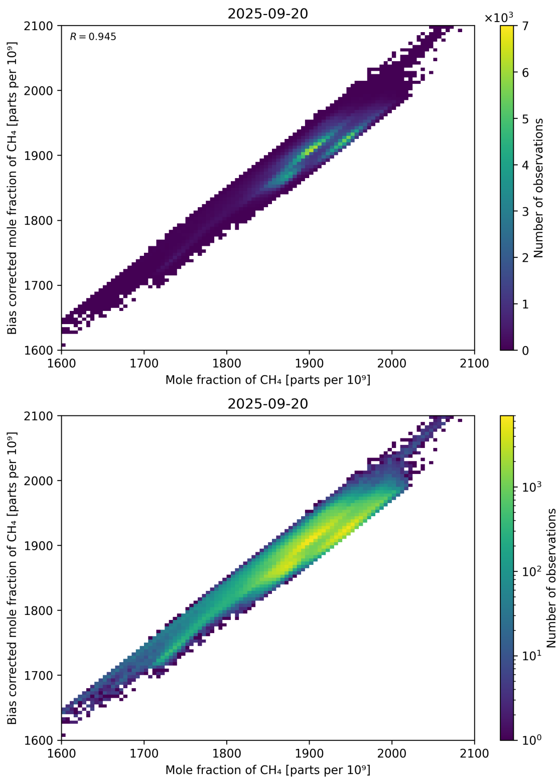
Figure 74: Scatter density plot of “Mole fraction of CH 4 ” against “Bias corrected mole fraction of CH 4 ” for 2025-09-20 to 2025-09-21.
