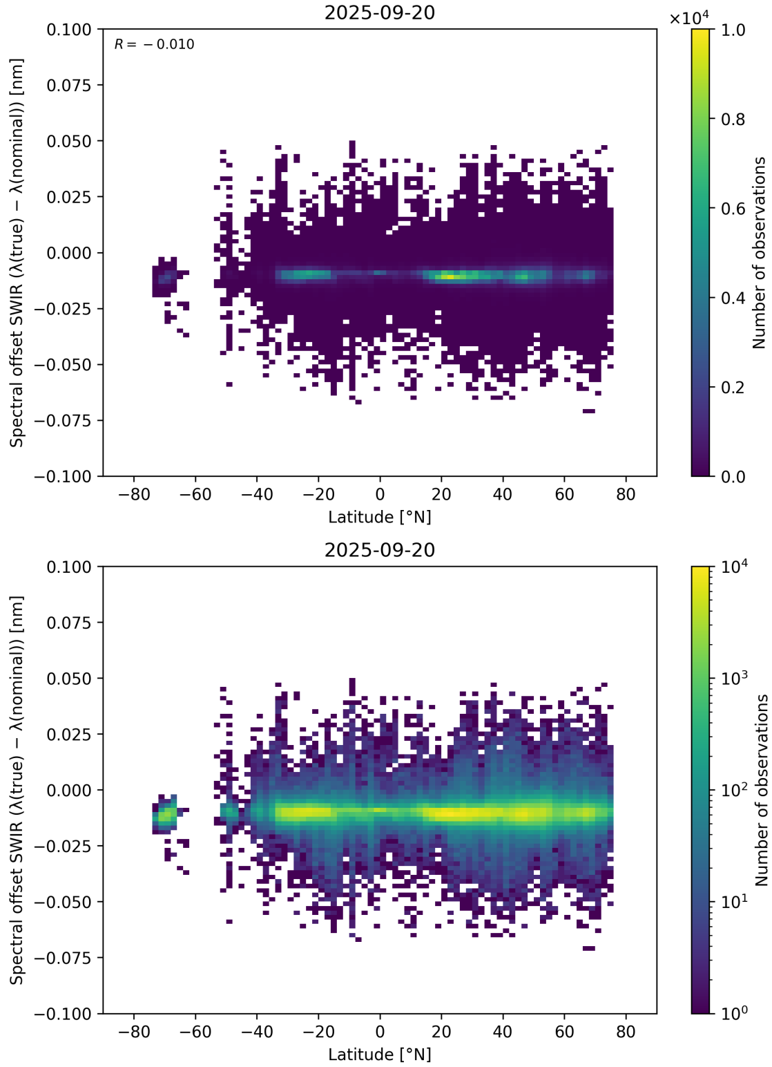
Figure 62: Scatter density plot of “Latitude” against “Spectral offset SWIR ( \lambda_{\text{true}} - \lambda_{\text{nominal}} )” for 2025-09-20 to 2025-09-21.
