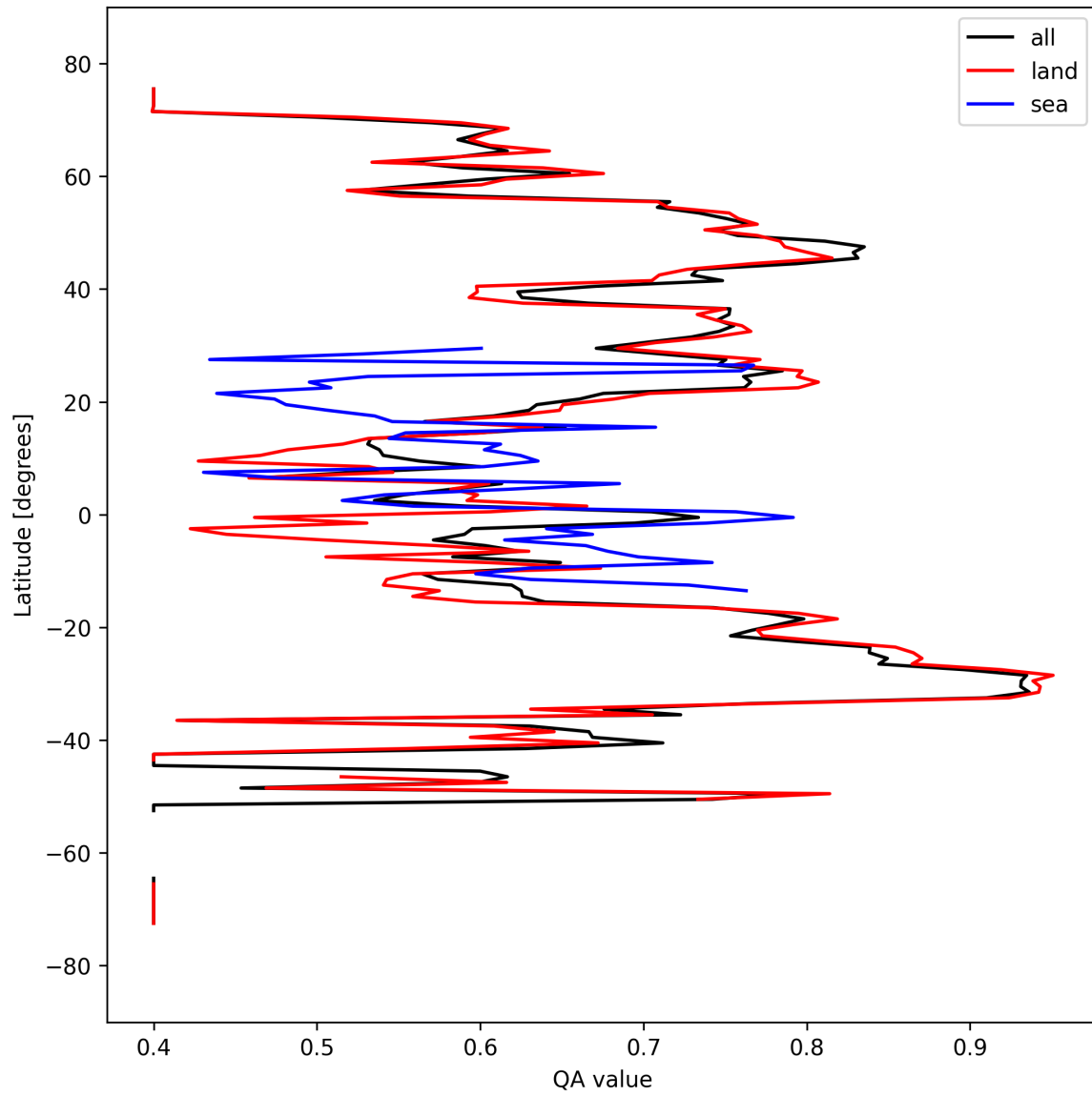
Figure 11: Zonal average of “QA value” for 2025-09-20 to 2025-09-21.
