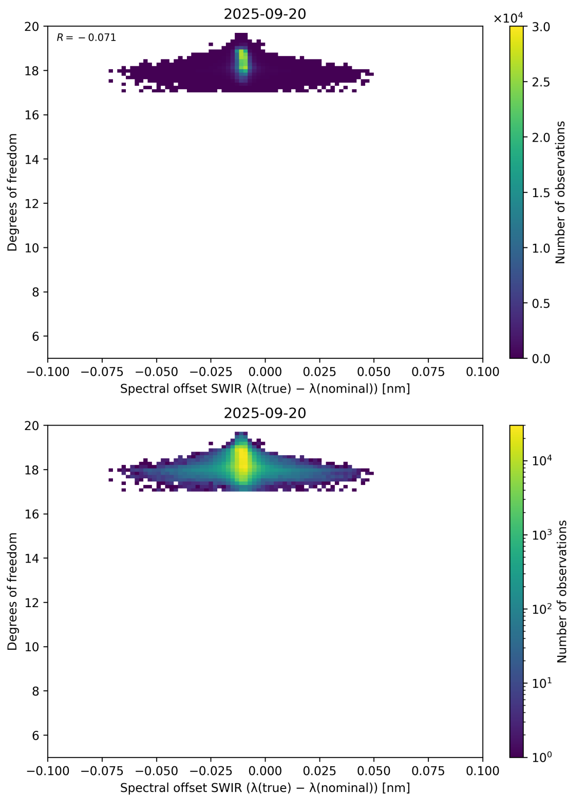
Figure 119: Scatter density plot of “Spectral offset SWIR ( \lambda_{\text{true}} - \lambda_{\text{nominal}} )” against “Degrees of freedom” for 2025-09-20 to 2025-09-21.
