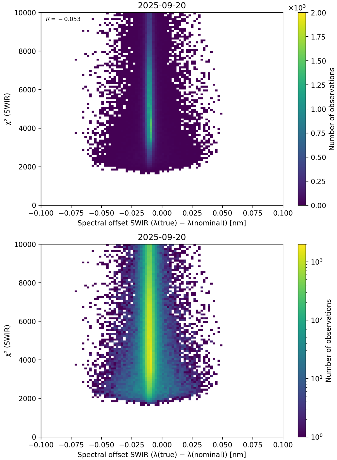
Figure 118: Scatter density plot of “Spectral offset SWIR ( \lambda_{\text{true}} - \lambda_{\text{nominal}} )” against “ \chi^2 (SWIR)” for 2025-09-20 to 2025-09-21.
