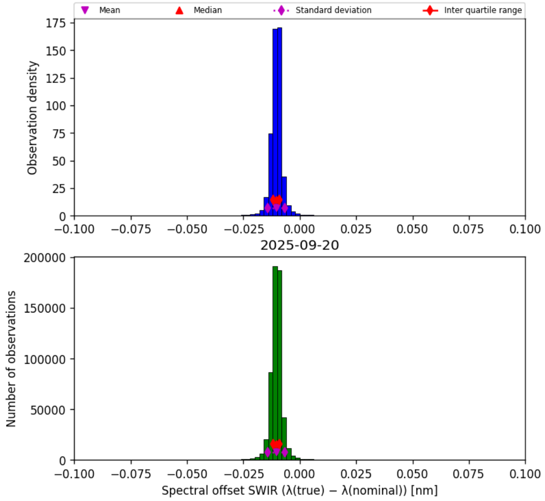
Figure 27: Histogram of “Spectral offset SWIR ( \lambda_{\text{true}} - \lambda_{\text{nominal}} )” for 2025-09-20 to 2025-09-21
