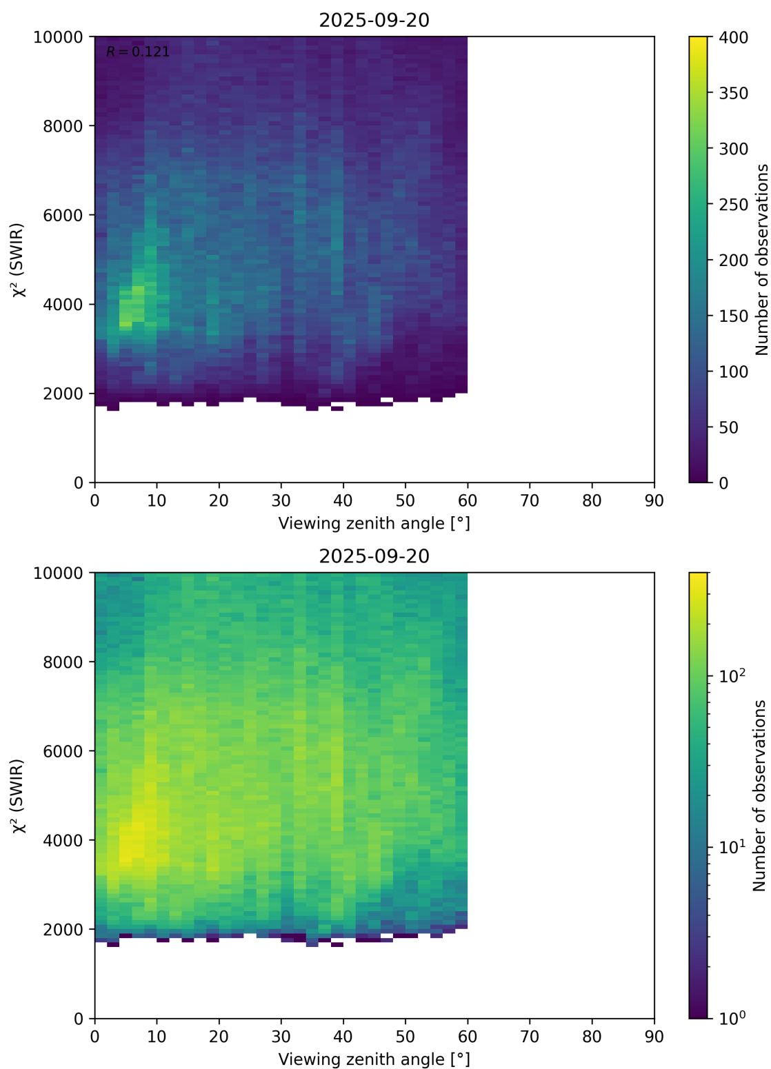
Figure 106: Scatter density plot of “Viewing zenith angle” against “ \chi^2 (SWIR)” for 2025-09-20 to 2025-09-21.
