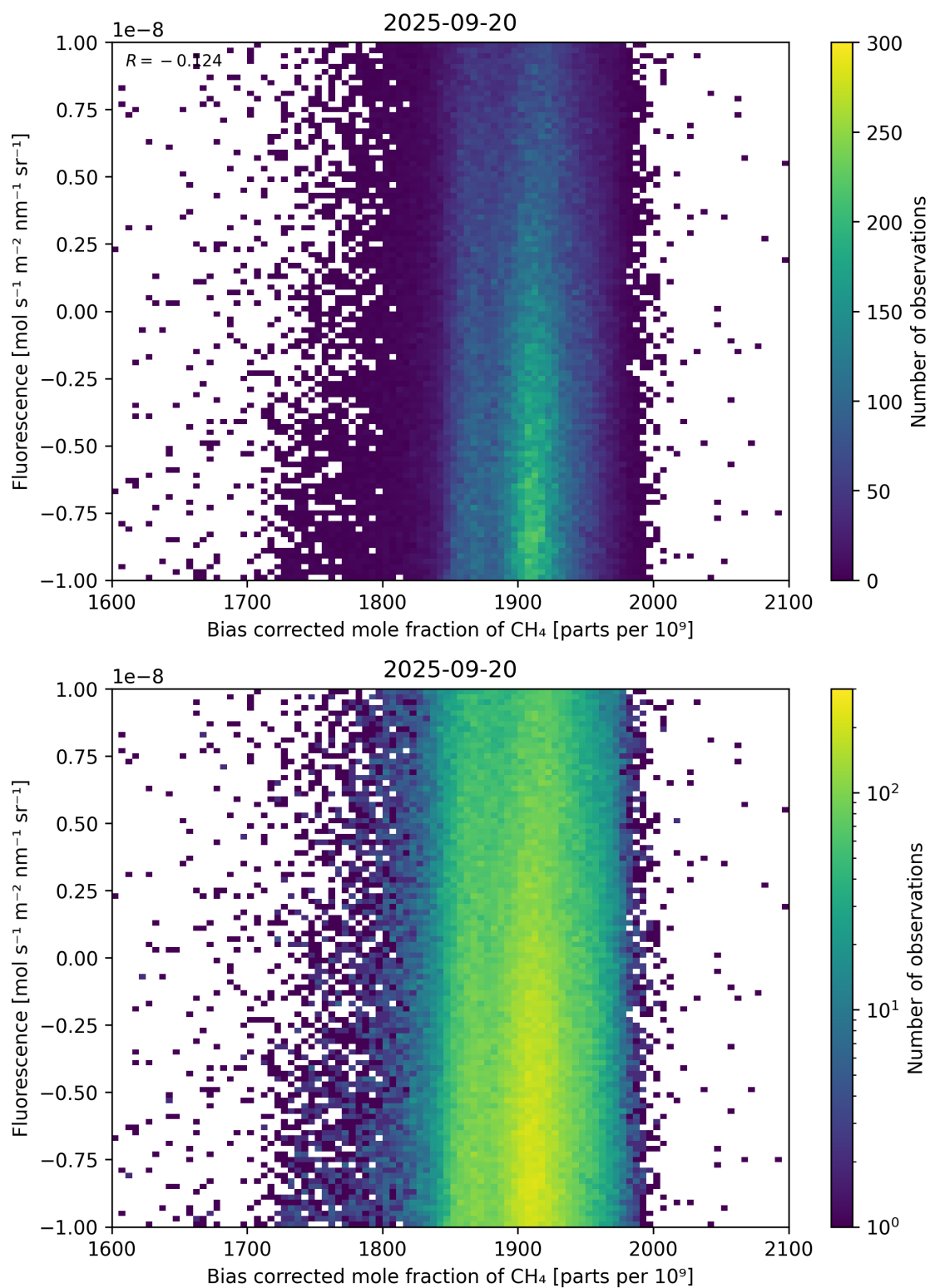
Figure 66: Scatter density plot of “Bias corrected mole fraction of \text{CH}_4 ” against “Fluorescence” for 2025-09-20 to 2025-09-21.
