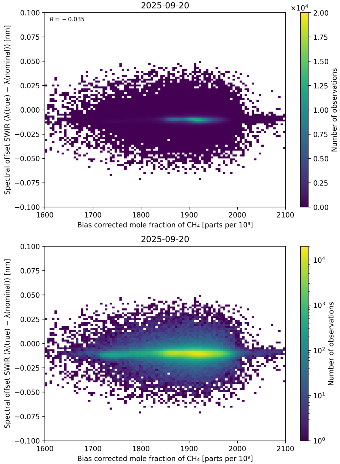
Figure 69: Scatter density plot of “Bias corrected mole fraction of CH 4 ” against “Spectral offset SWIR ( \lambda_{\text{true}} - \lambda_{\text{nominal}} )” for 2025-09-20 to 2025-09-21.
