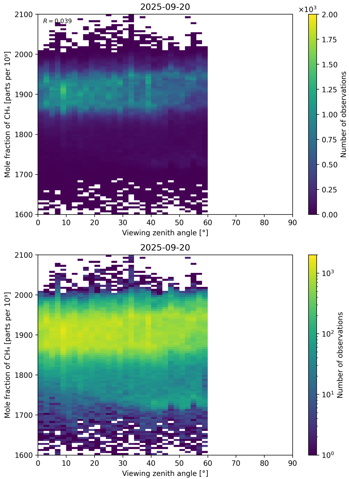
Figure 110: Scatter density plot of “Viewing zenith angle” against “Mole fraction of CH 4 ” for 2025-09-20 to 2025-09-21.
