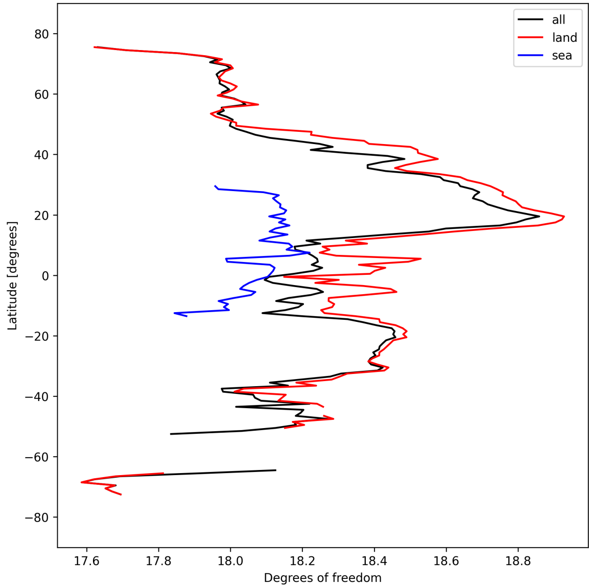
Figure 19: Zonal average of “Degrees of freedom” for 2025-09-20 to 2025-09-21.
