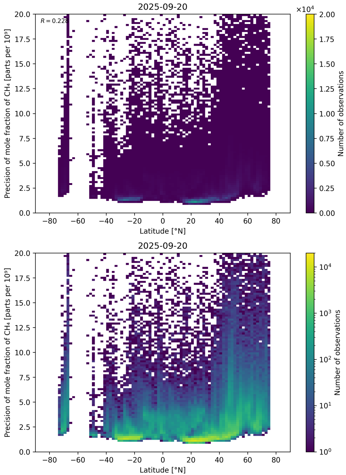
Figure 59: Scatter density plot of “Latitude” against “Precision of mole fraction of CH 4 ” for 2025-09-20 to 2025-09-21.
