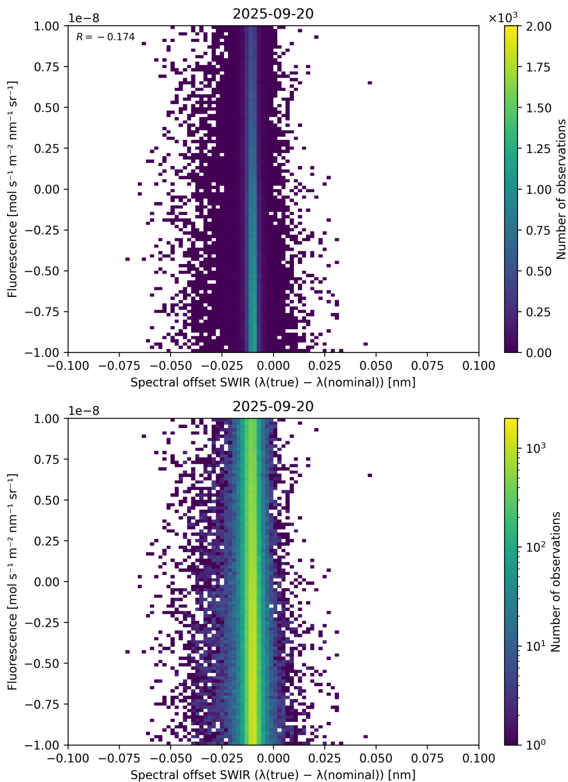
Figure 120: Scatter density plot of “Spectral offset SWIR ( \lambda_{\text{true}} - \lambda_{\text{nominal}} )” against “Fluorescence” for 2025-09-20 to 2025-09-21.
