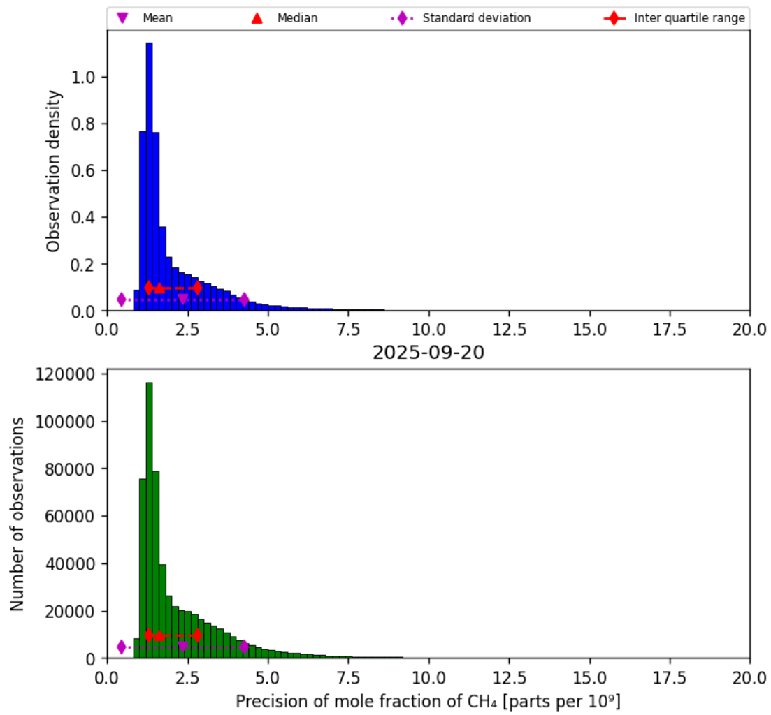
Figure 24: Histogram of “Precision of mole fraction of CH 4 ” for 2025-09-20 to 2025-09-21
