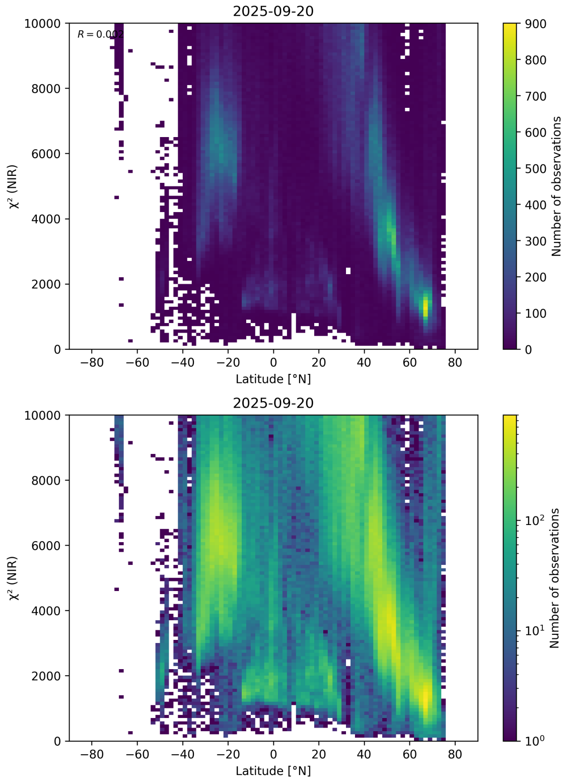
Figure 53: Scatter density plot of “Latitude” against “ \chi^2 (NIR)” for 2025-09-20 to 2025-09-21.
