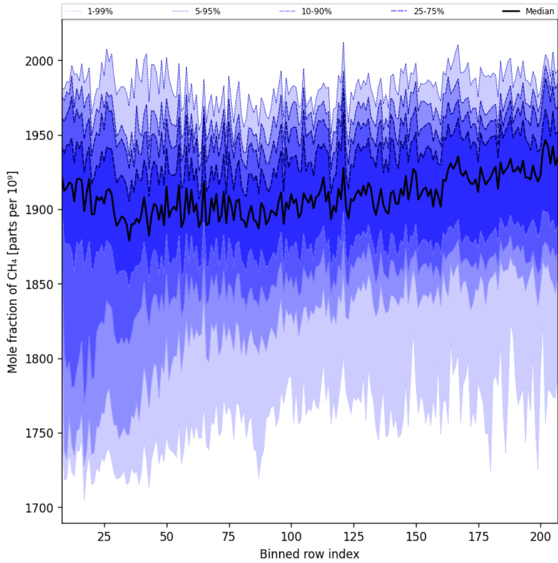
Figure 34: Along track statistics of “Mole fraction of CH 4 ” for 2025-09-20 to 2025-09-21
