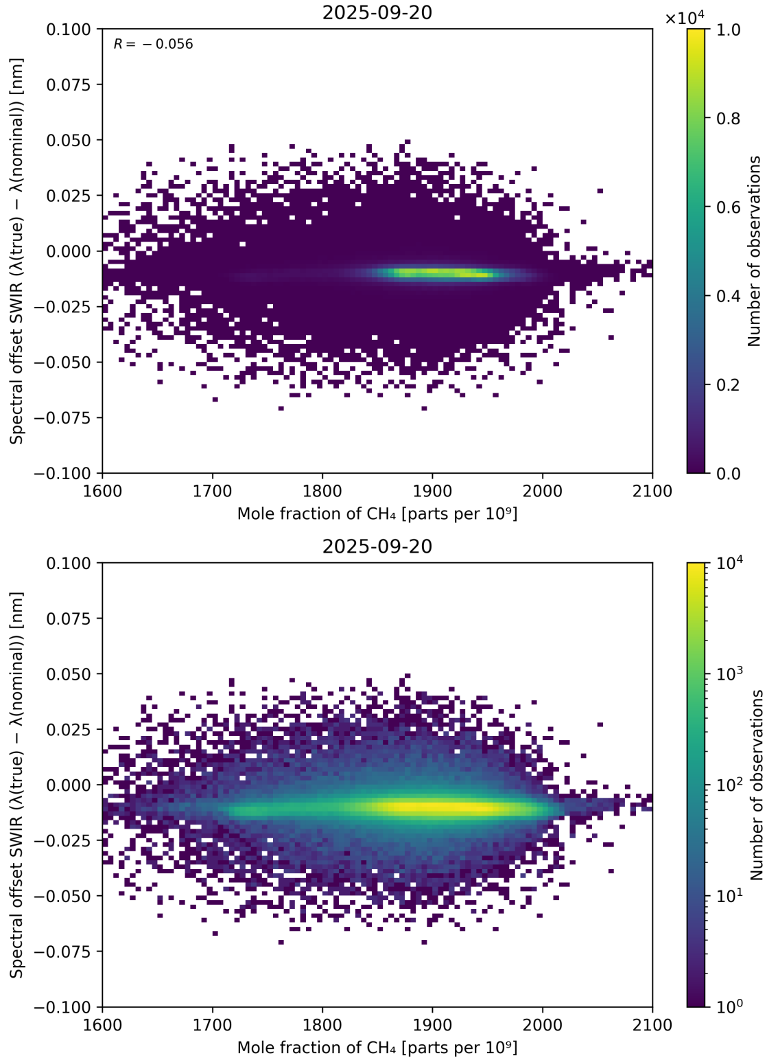
Figure 86: Scatter density plot of “Mole fraction of CH 4 ” against “Spectral offset SWIR ( \lambda_{\text{true}} - \lambda_{\text{nominal}} )” for 2025-09-20 to 2025-09-21.
