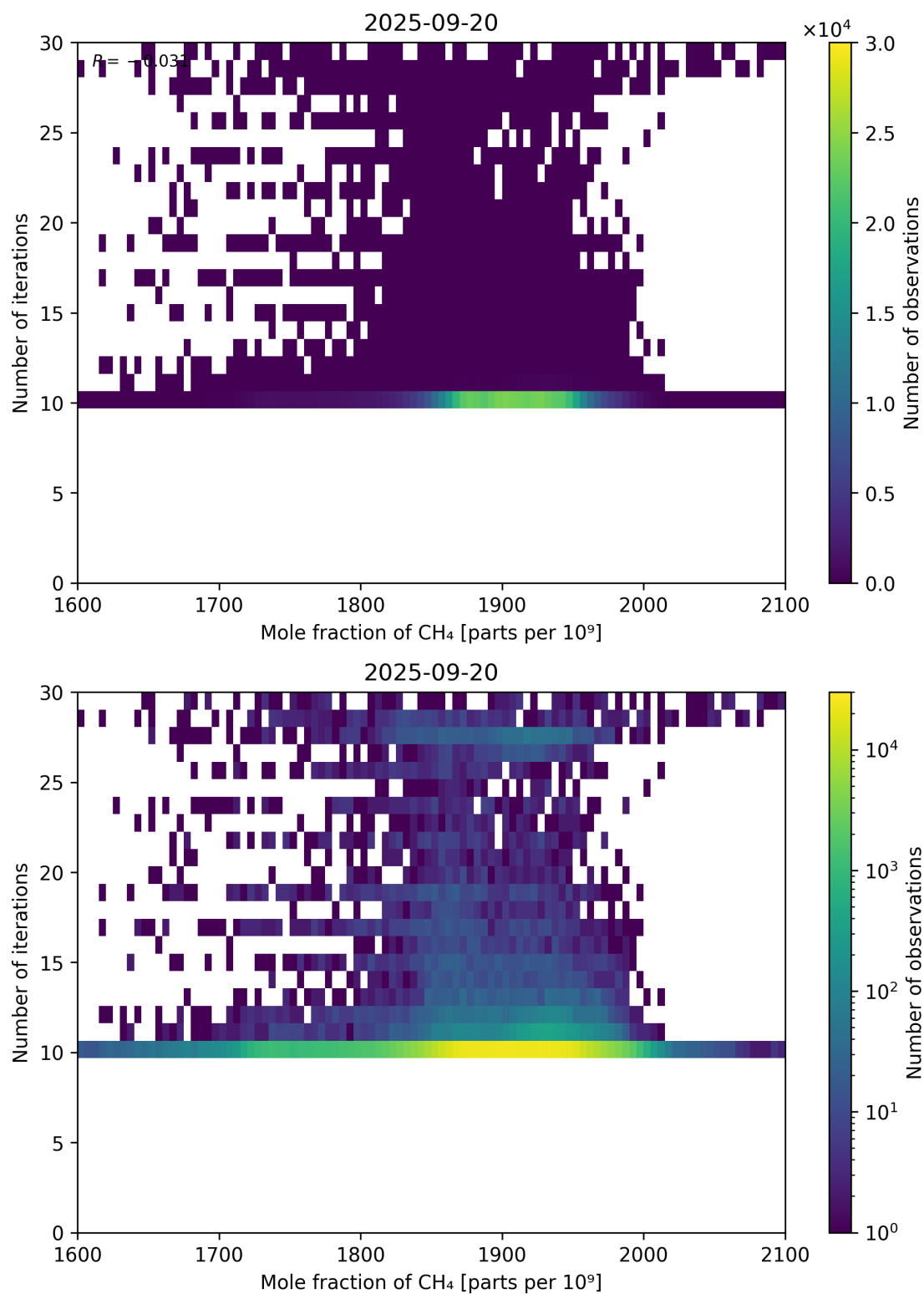
Figure 76: Scatter density plot of “Mole fraction of CH 4 ” against “Number of iterations” for 2025-09-20 to 2025-09-21.
