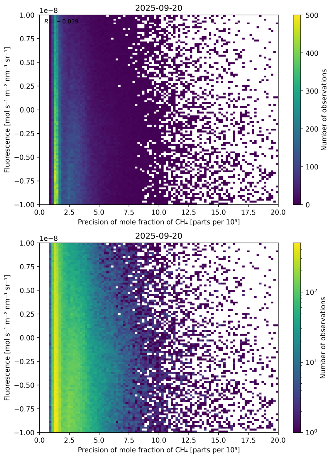
Figure 81: Scatter density plot of “Precision of mole fraction of \text{CH}_4 ” against “Fluorescence” for 2025-09-20 to 2025-09-21.
