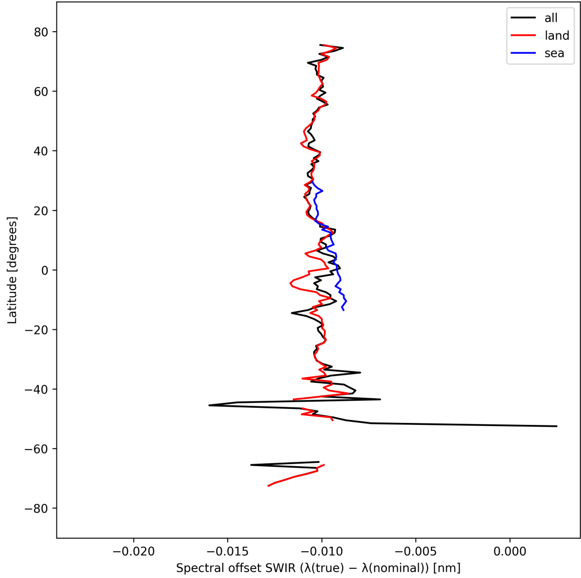
Figure 16: Zonal average of “Spectral offset SWIR ( \lambda_{\text{true}} - \lambda_{\text{nominal}} )” for 2025-09-20 to 2025-09-21.
