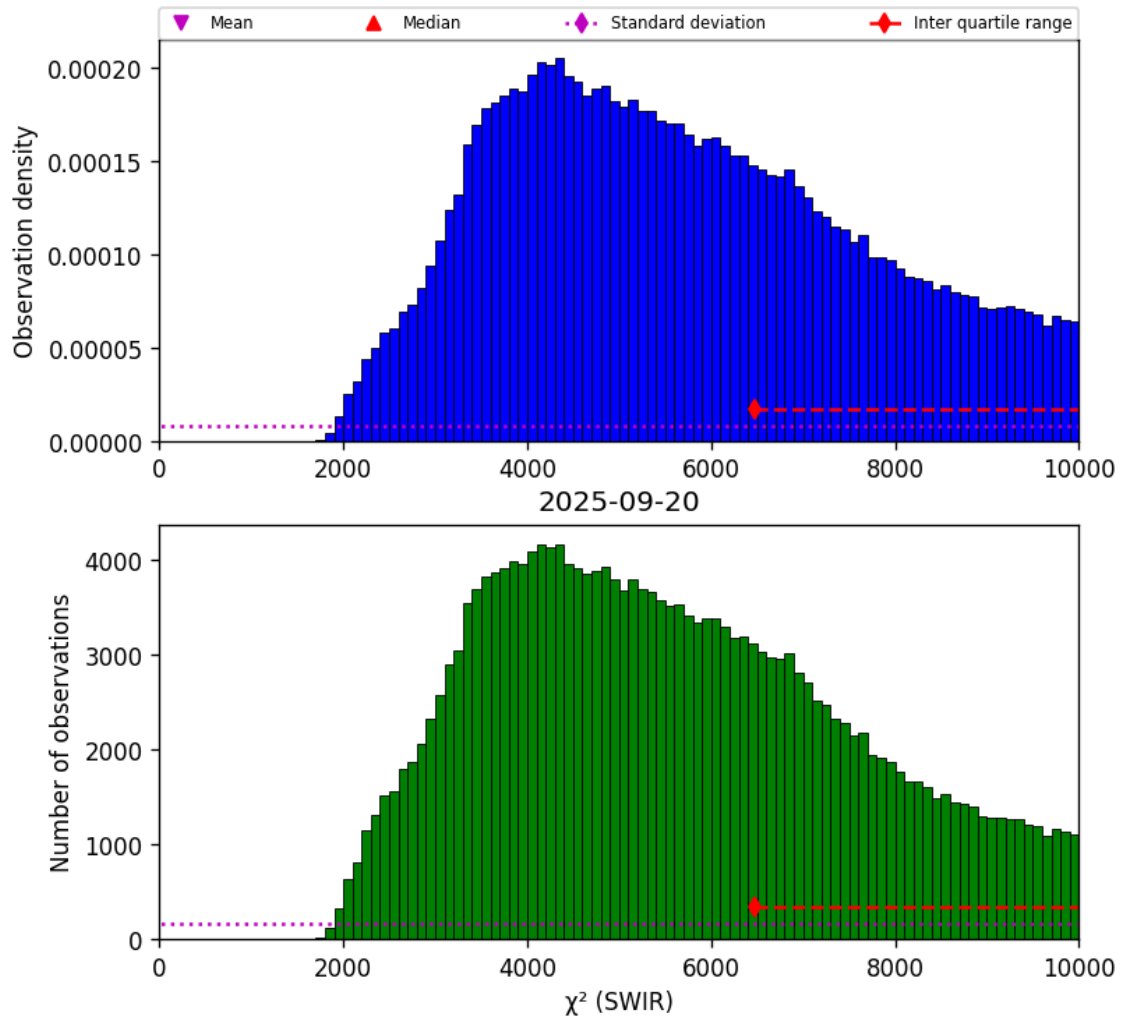
Figure 28: Histogram of " \chi^2 (SWIR)" for 2025-09-20 to 2025-09-21
