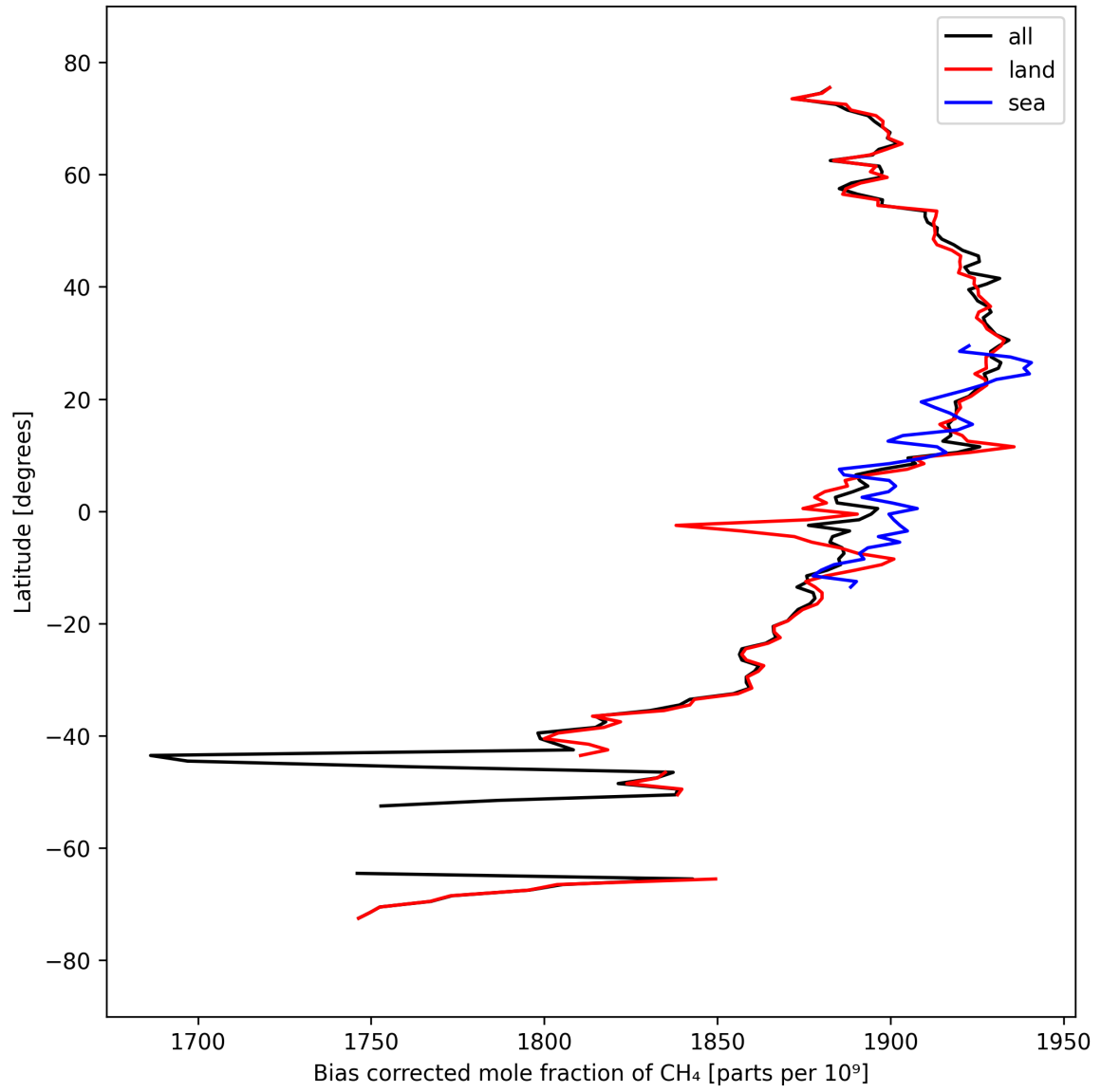
Figure 14: Zonal average of “Bias corrected mole fraction of CH 4 ” for 2025-09-20 to 2025-09-21.
