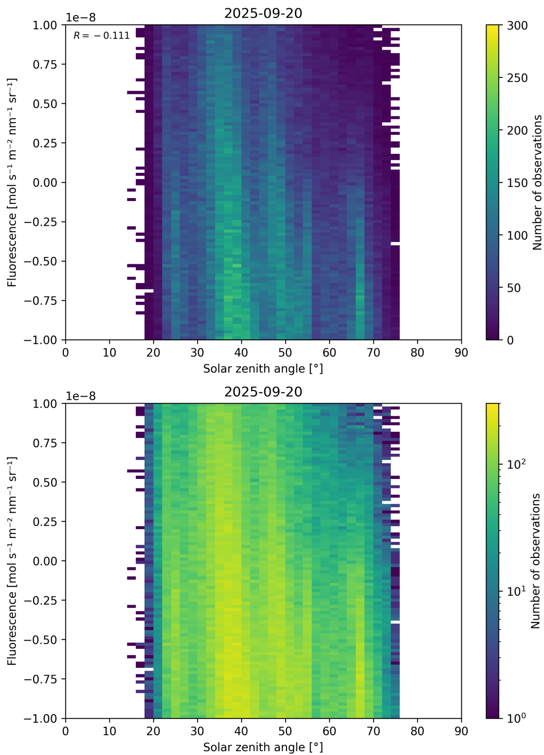
Figure 97: Scatter density plot of “Solar zenith angle” against “Fluorescence” for 2025-09-20 to 2025-09-21.
