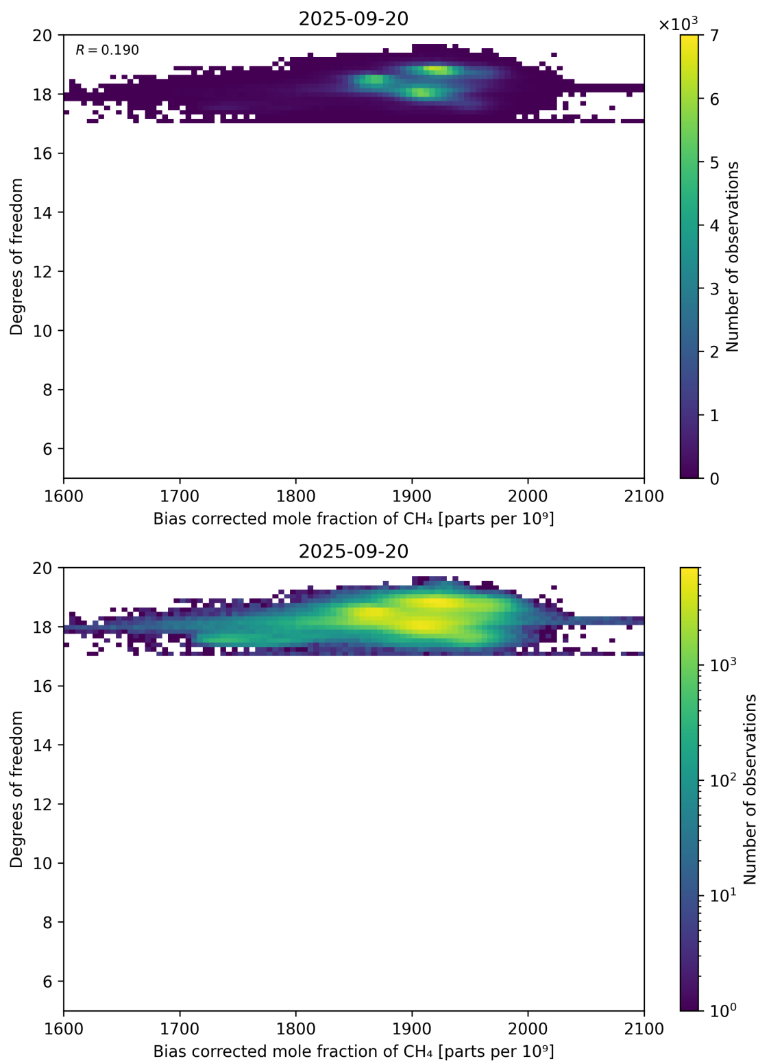
Figure 65: Scatter density plot of “Bias corrected mole fraction of CH 4 ” against “Degrees of freedom” for 2025-09-20 to 2025-09-21.
