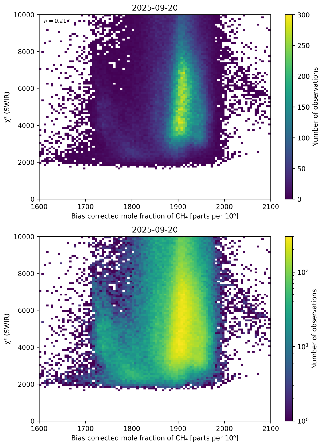
Figure 64: Scatter density plot of “Bias corrected mole fraction of \text{CH}_4 ” against “ \chi^2 (SWIR)” for 2025-09-20 to 2025-09-21.
