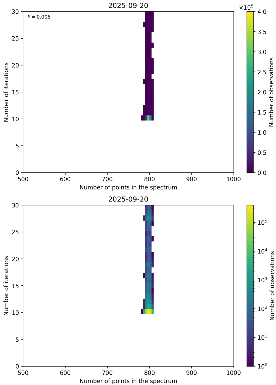
Figure 92: Scatter density plot of “Number of points in the spectrum” against “Number of iterations” for 2025-09-20 to 2025-09-21.
