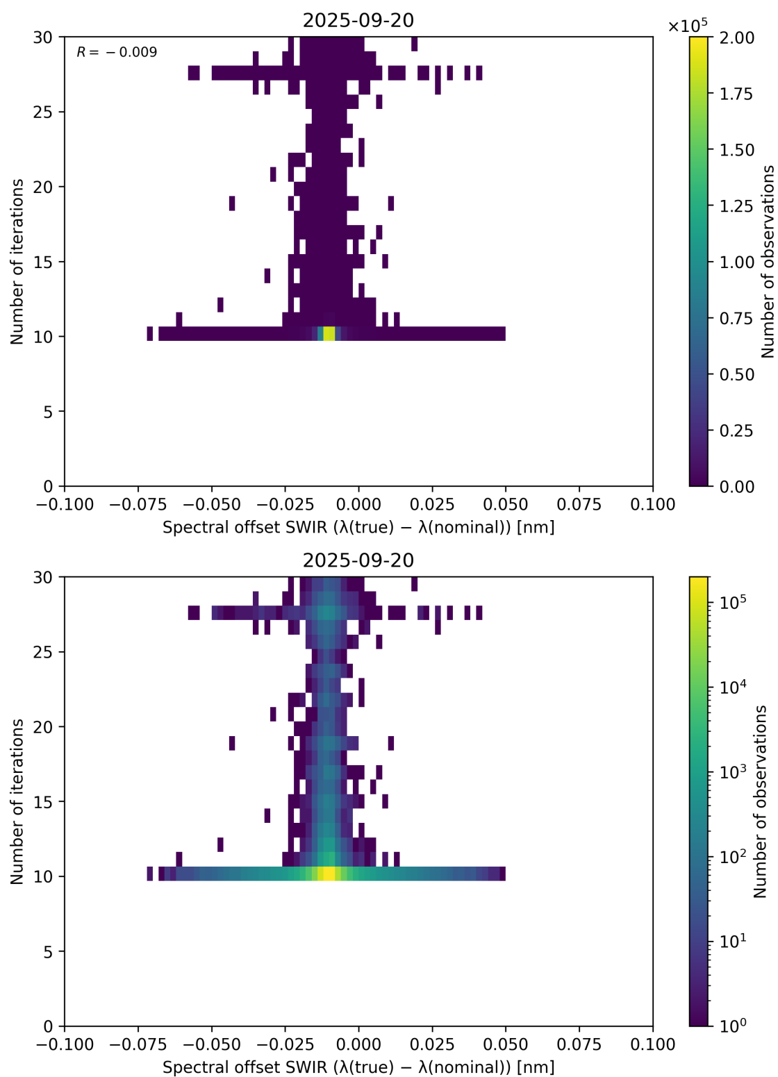
Figure 121: Scatter density plot of “Spectral offset SWIR ( \lambda_{\text{true}} - \lambda_{\text{nominal}} )” against “Number of iterations” for 2025-09-20 to 2025-09-21.
