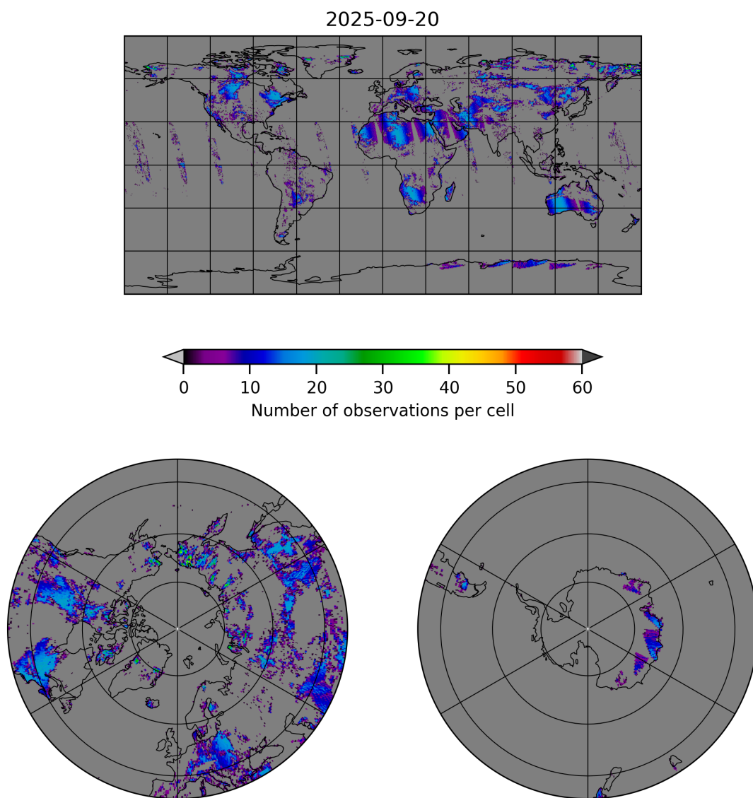
Figure 10: Map of the number of observations for 2025-09-20 to 2025-09-21
