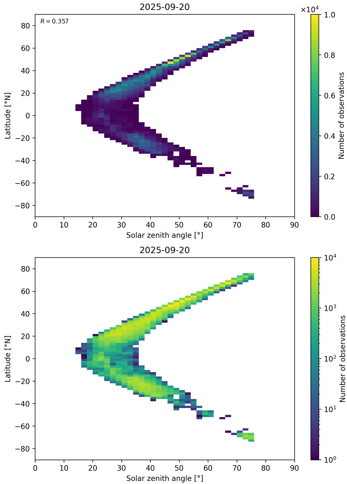
Figure 98: Scatter density plot of “Solar zenith angle” against “Latitude” for 2025-09-20 to 2025-09-21.
