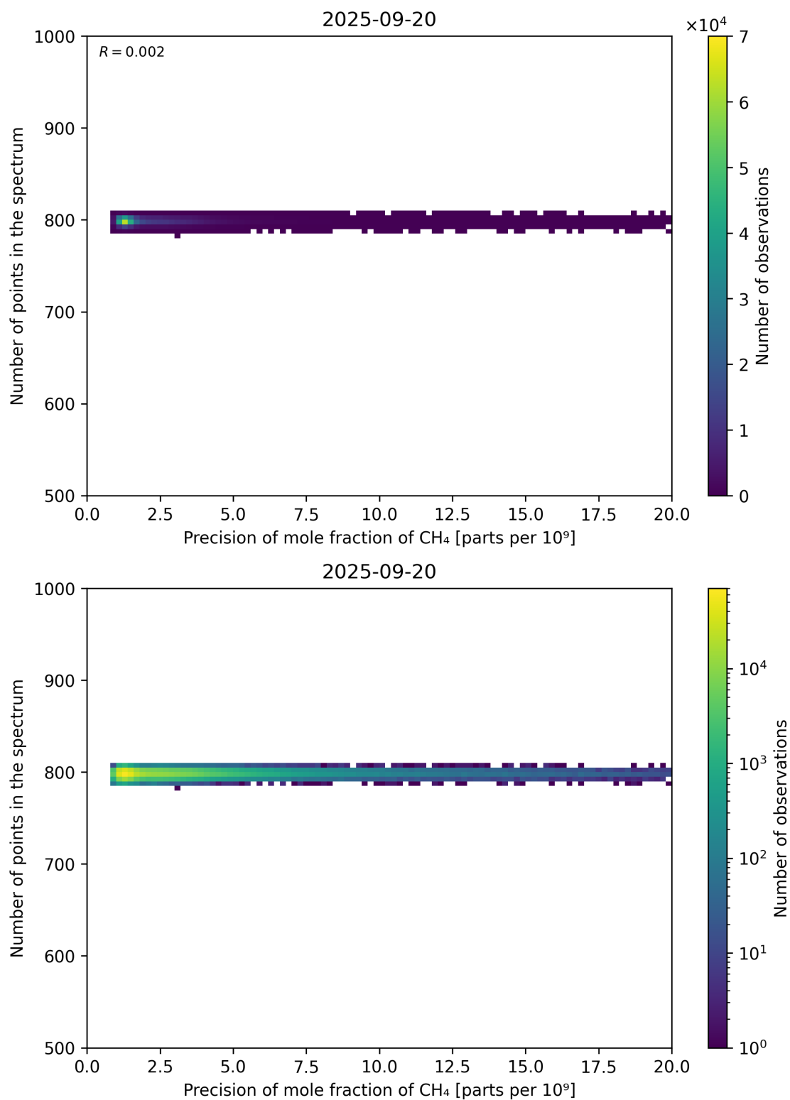
Figure 84: Scatter density plot of “Precision of mole fraction of CH 4 ” against “Number of points in the spectrum” for 2025-09-20 to 2025-09-21.
