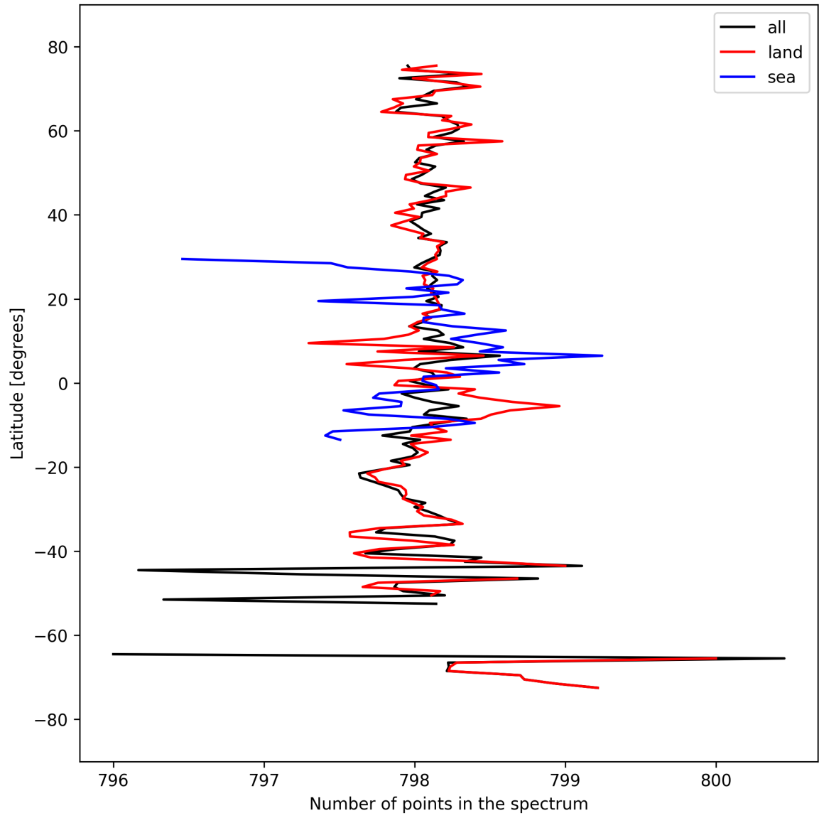
Figure 15: Zonal average of “Number of points in the spectrum” for 2025-09-20 to 2025-09-21.
