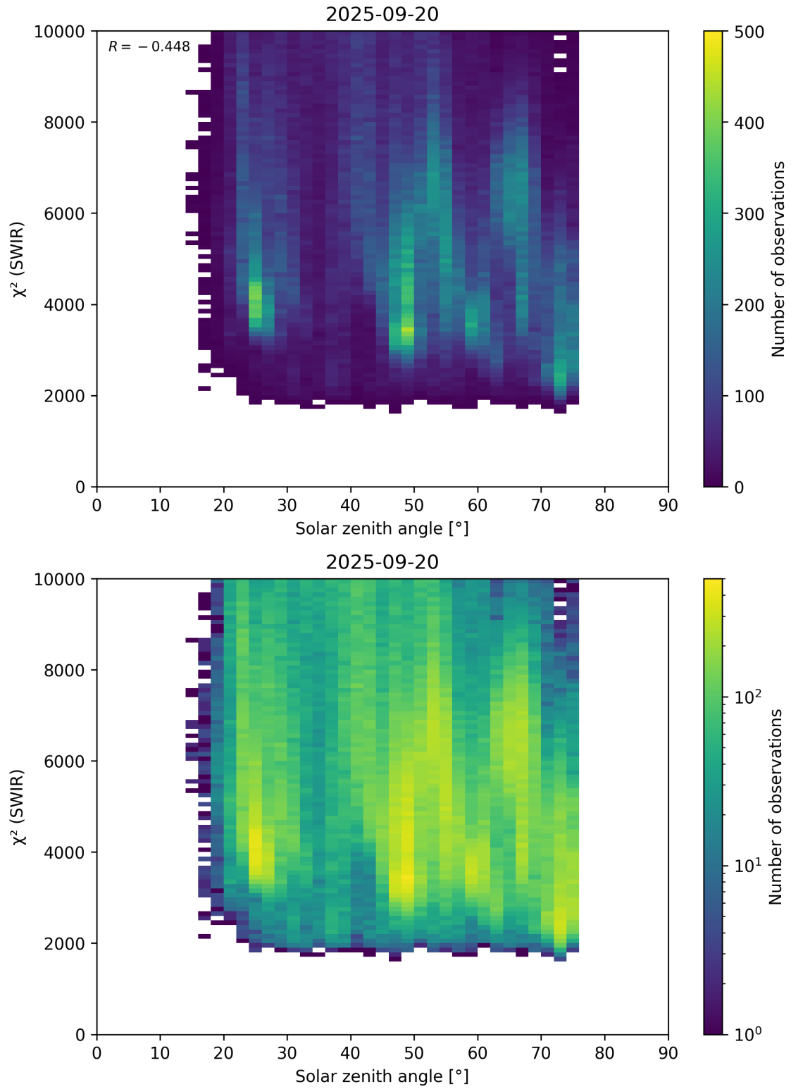
Figure 95: Scatter density plot of “Solar zenith angle” against “ \chi^2 (SWIR)” for 2025-09-20 to 2025-09-21.
