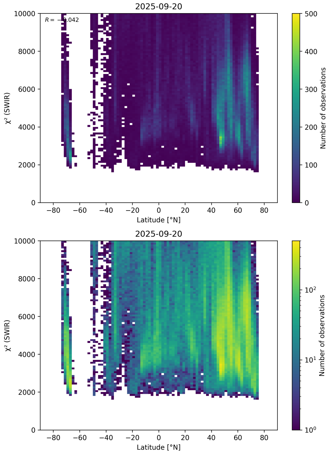
Figure 54: Scatter density plot of “Latitude” against “ \chi^2 (SWIR)” for 2025-09-20 to 2025-09-21.
