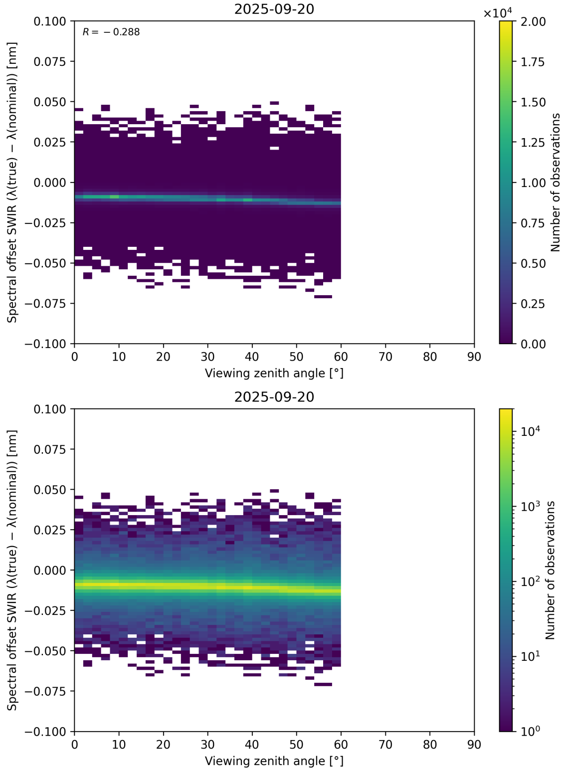
Figure 116: Scatter density plot of “Viewing zenith angle” against “Spectral offset SWIR ( \lambda_{\text{true}} - \lambda_{\text{nominal}} )” for 2025-09-20 to 2025-09-21.
