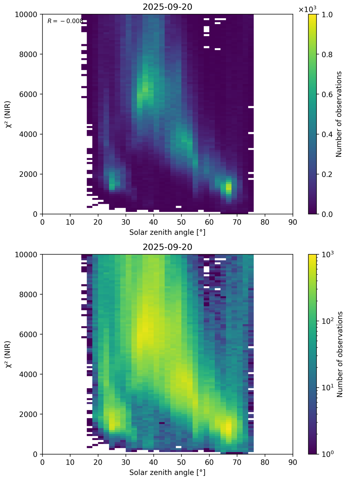
Figure 94: Scatter density plot of “Solar zenith angle” against “ \chi^2 (NIR)” for 2025-09-20 to 2025-09-21.
