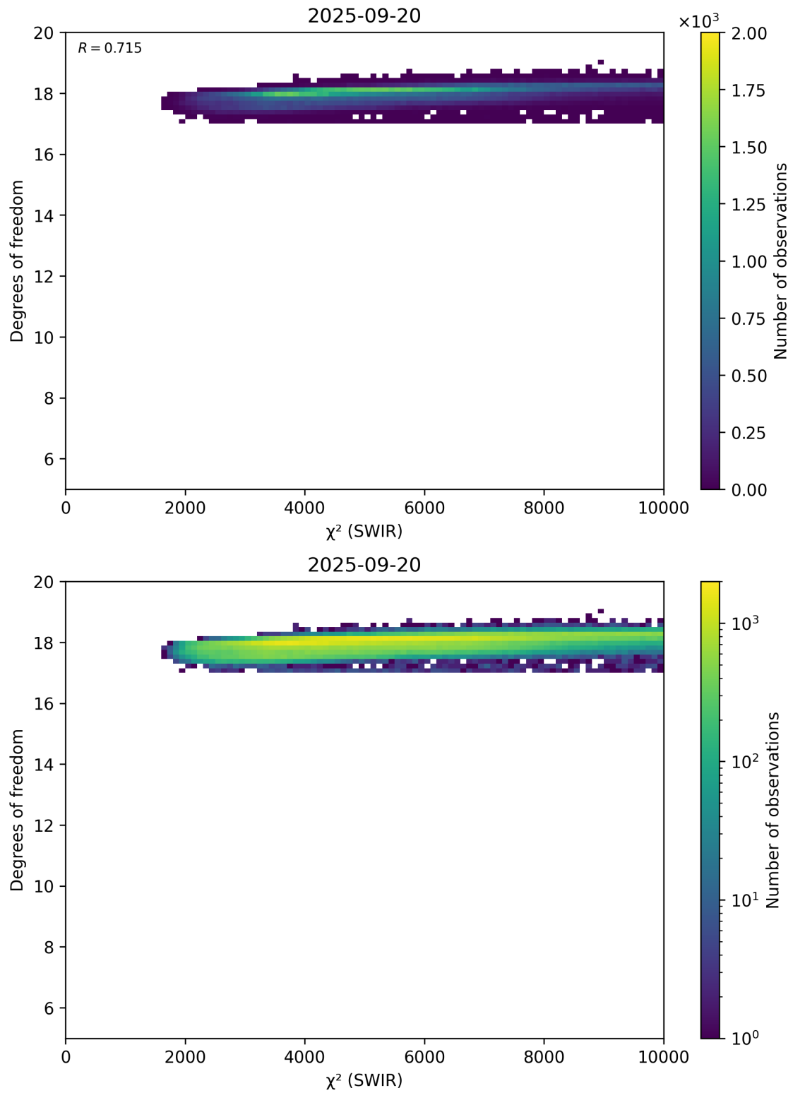
Figure 48: Scatter density plot of “ \chi^2 (SWIR)” against “Degrees of freedom” for 2025-09-20 to 2025-09-21.
