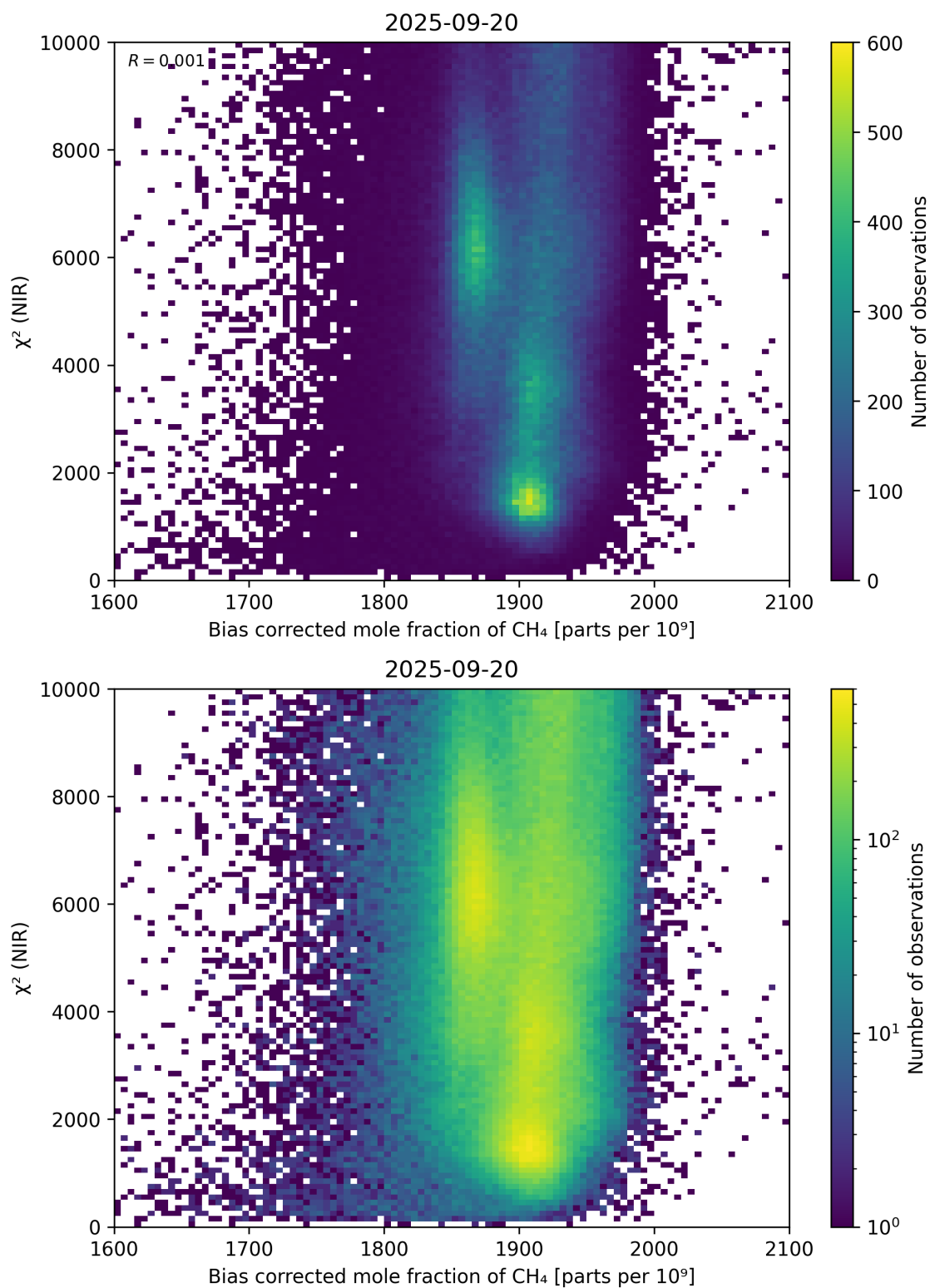
Figure 63: Scatter density plot of “Bias corrected mole fraction of CH 4 ” against “ \chi^2 (NIR)” for 2025-09-20 to 2025-09-21.
