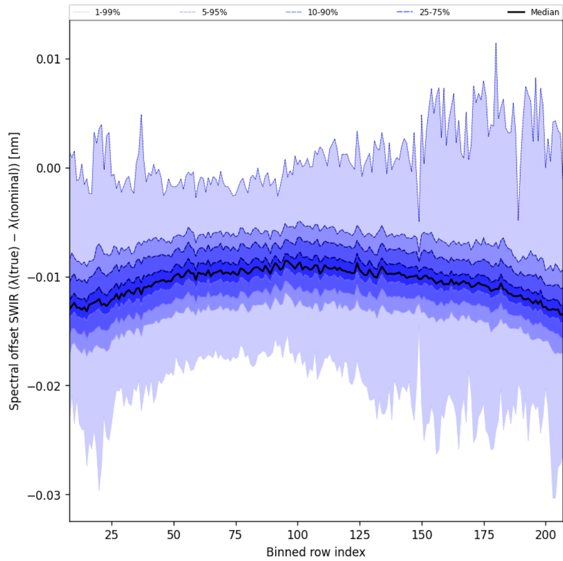
Figure 38: Along track statistics of “Spectral offset SWIR ( \lambda_{\text{true}} - \lambda_{\text{nominal}} )” for 2025-09-20 to 2025-09-21
