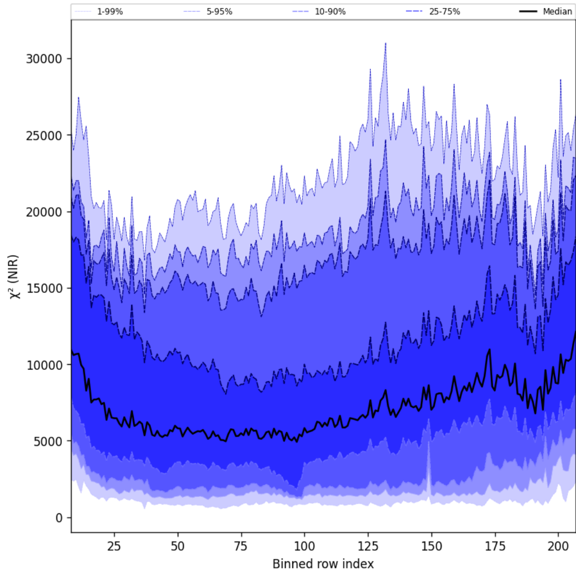
Figure 40: Along track statistics of “ \chi^2 (NIR)” for 2025-09-20 to 2025-09-21
