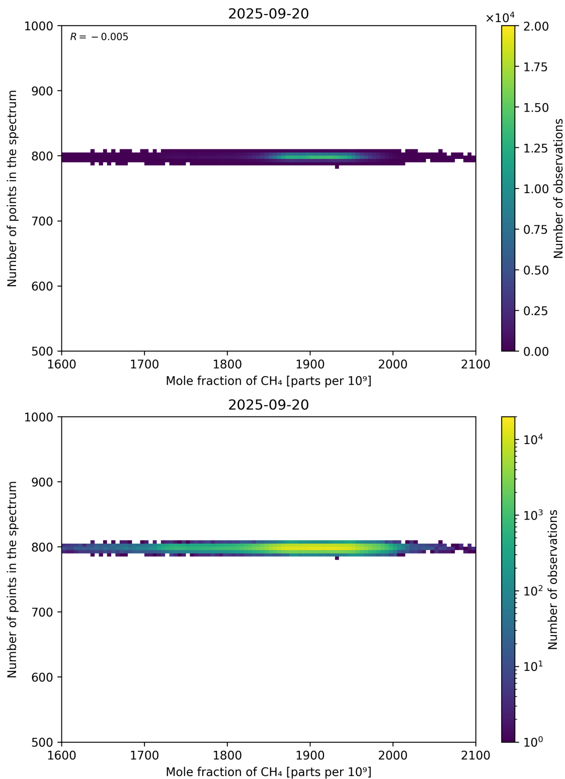
Figure 77: Scatter density plot of “Mole fraction of CH 4 ” against “Number of points in the spectrum” for 2025-09-20 to 2025-09-21.
