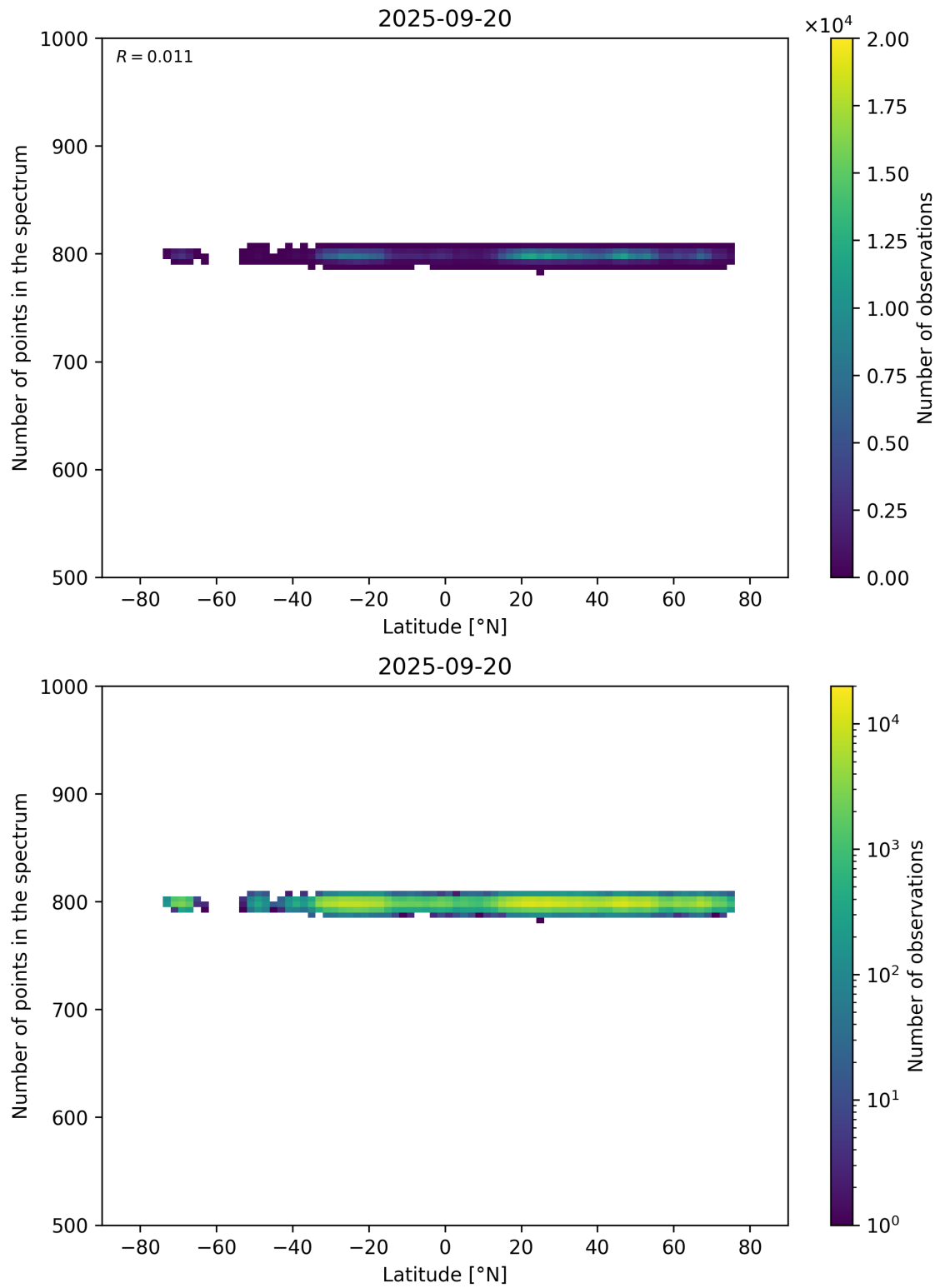
Figure 61: Scatter density plot of “Latitude” against “Number of points in the spectrum” for 2025-09-20 to 2025-09-21.
