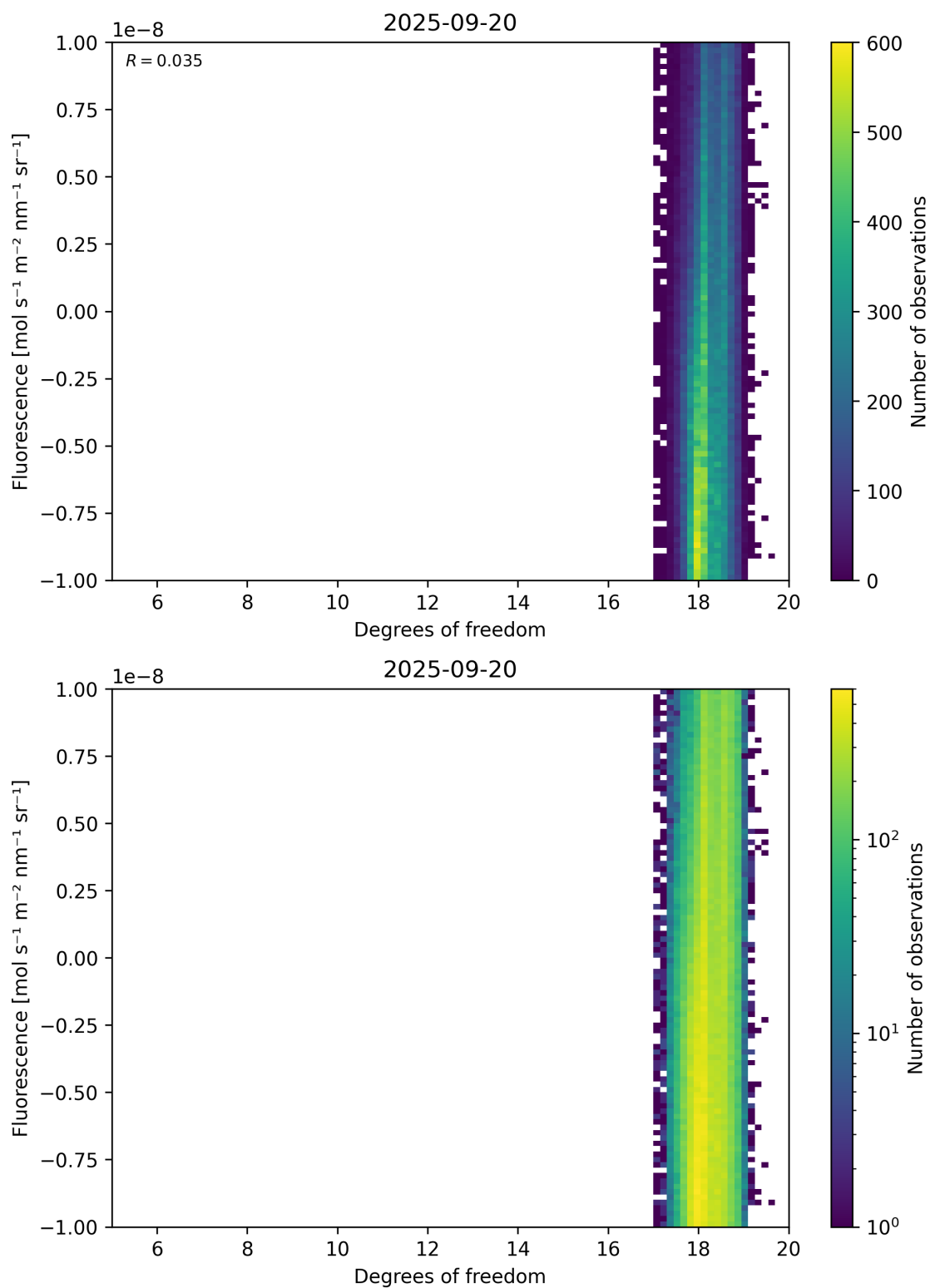
Figure 51: Scatter density plot of “Degrees of freedom” against “Fluorescence” for 2025-09-20 to 2025-09-21.
