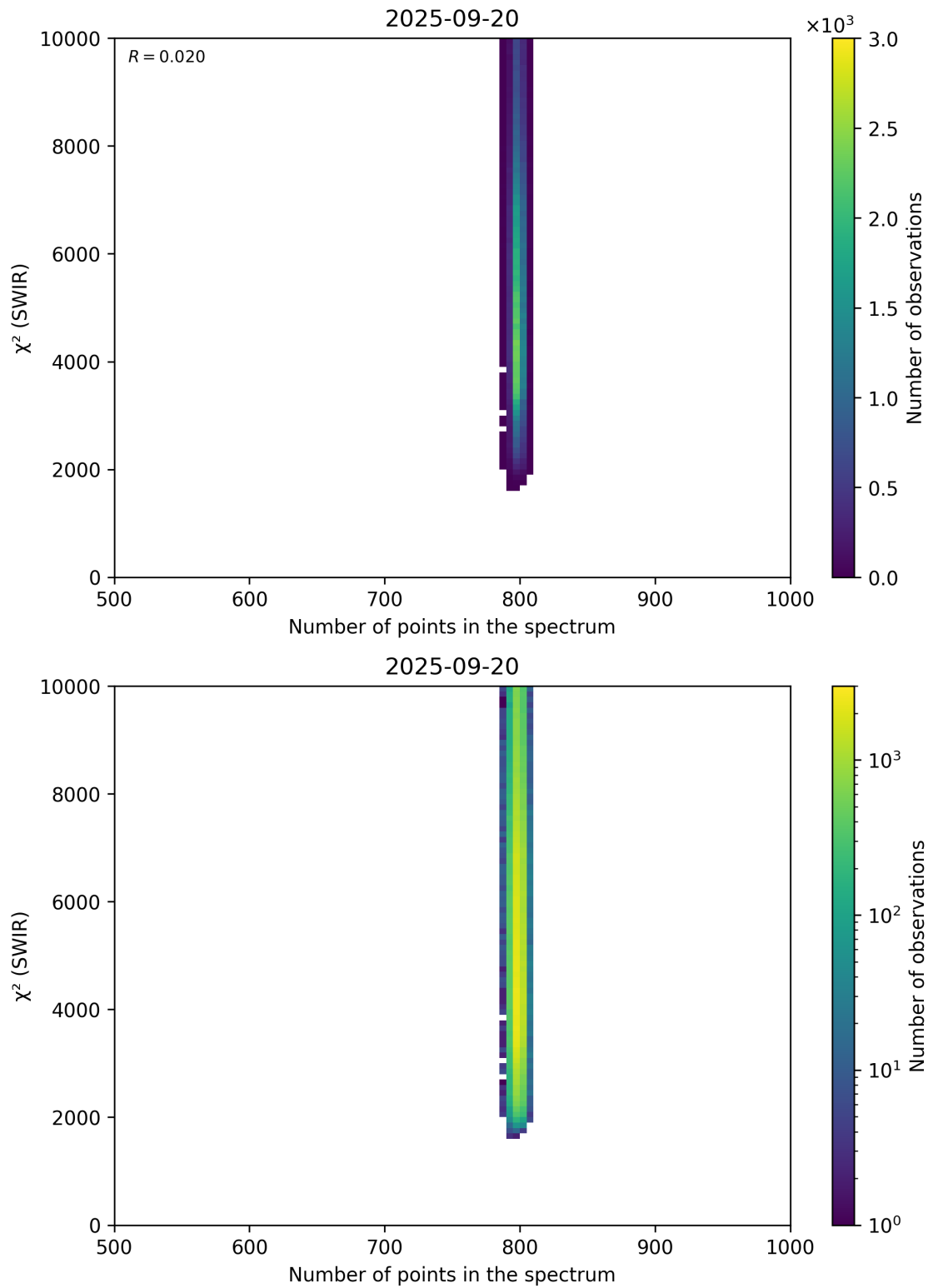
Figure 89: Scatter density plot of “Number of points in the spectrum” against “ \chi^2 (SWIR)” for 2025-09-20 to 2025-09-21.
