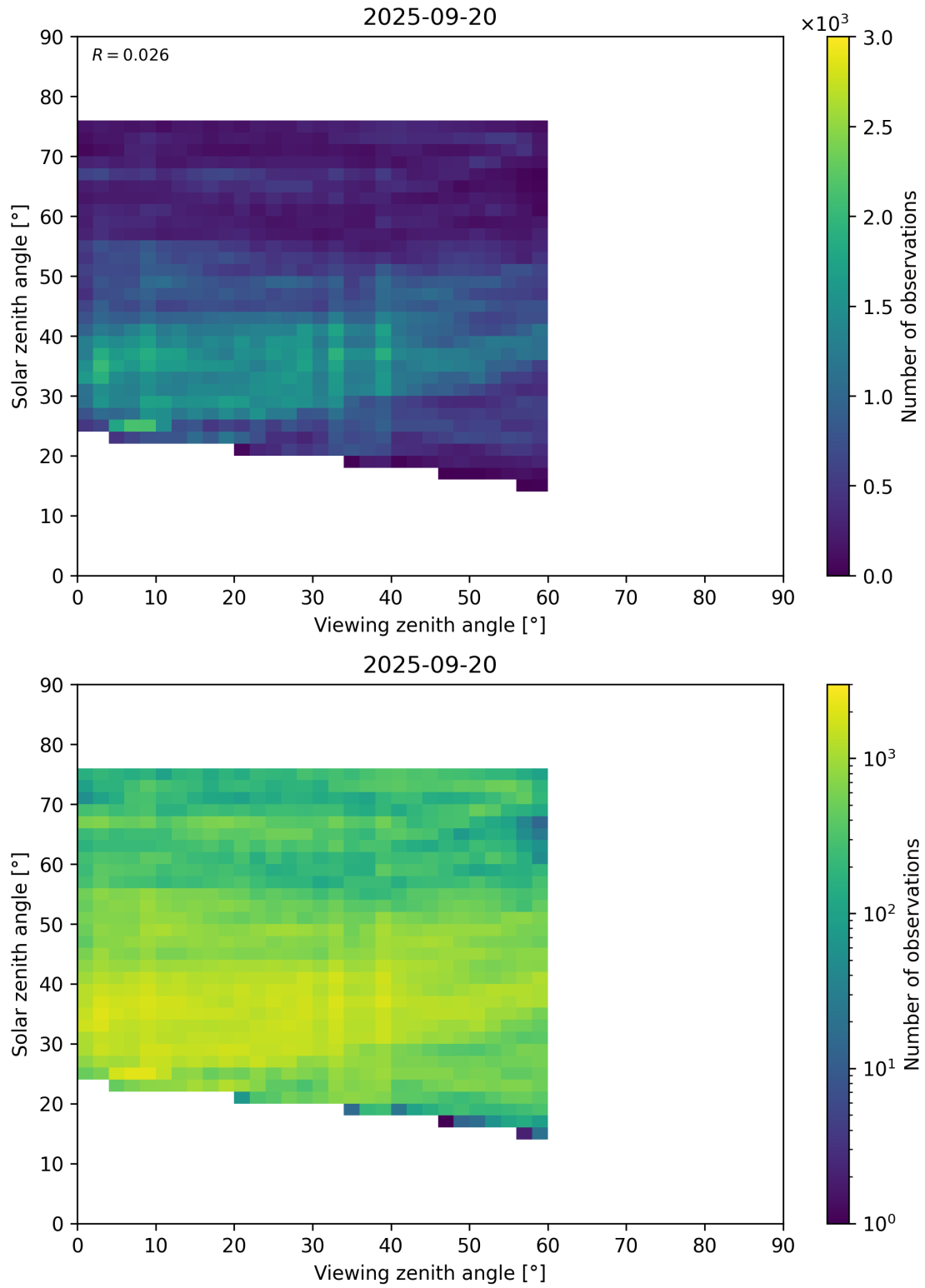
Figure 115: Scatter density plot of “Viewing zenith angle” against “Solar zenith angle” for 2025-09-20 to 2025-09-21.
