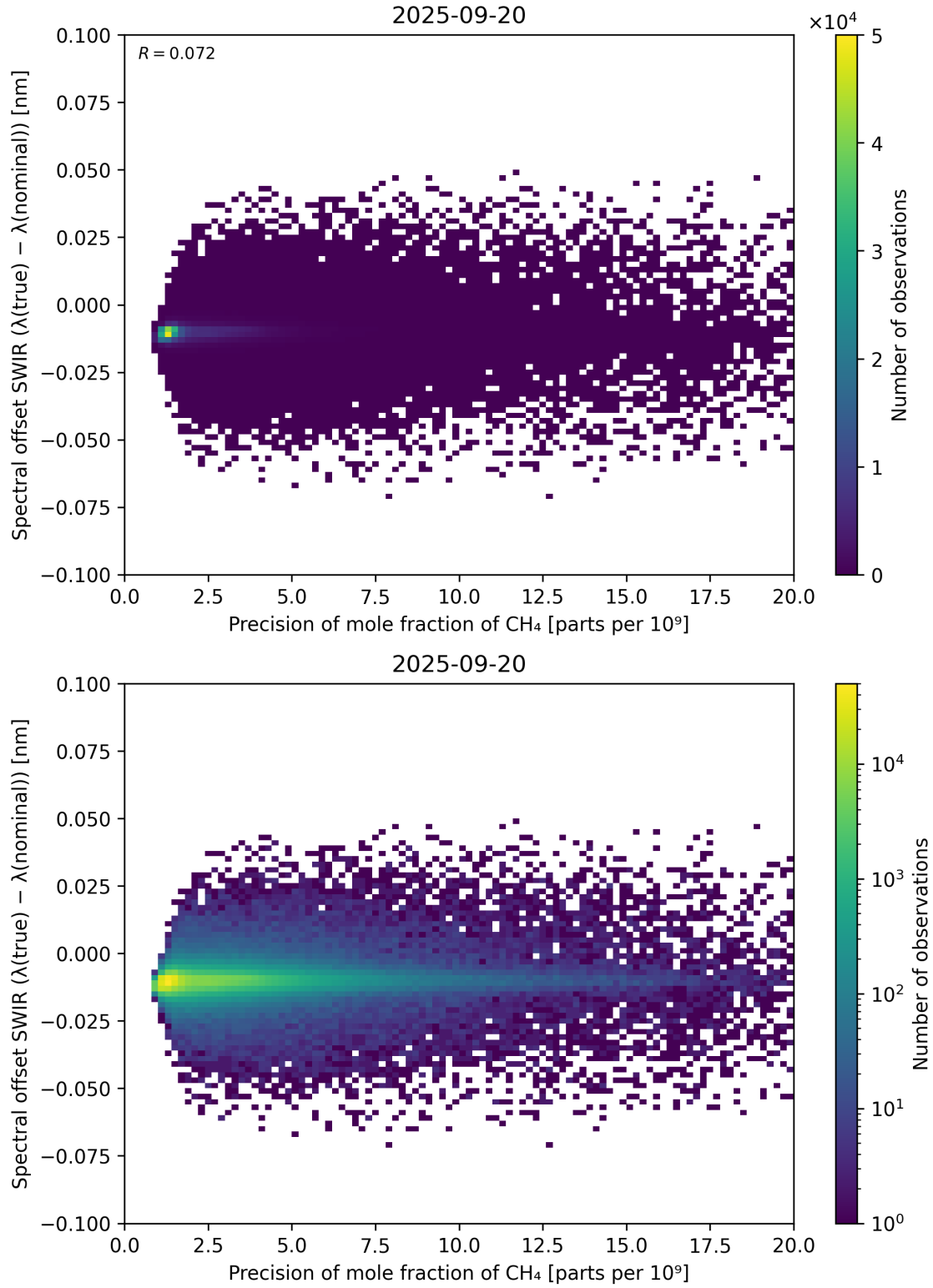
Figure 85: Scatter density plot of “Precision of mole fraction of CH 4 ” against “Spectral offset SWIR ( \lambda_{\text{true}} - \lambda_{\text{nominal}} )” for 2025-09-20 to 2025-09-21.
