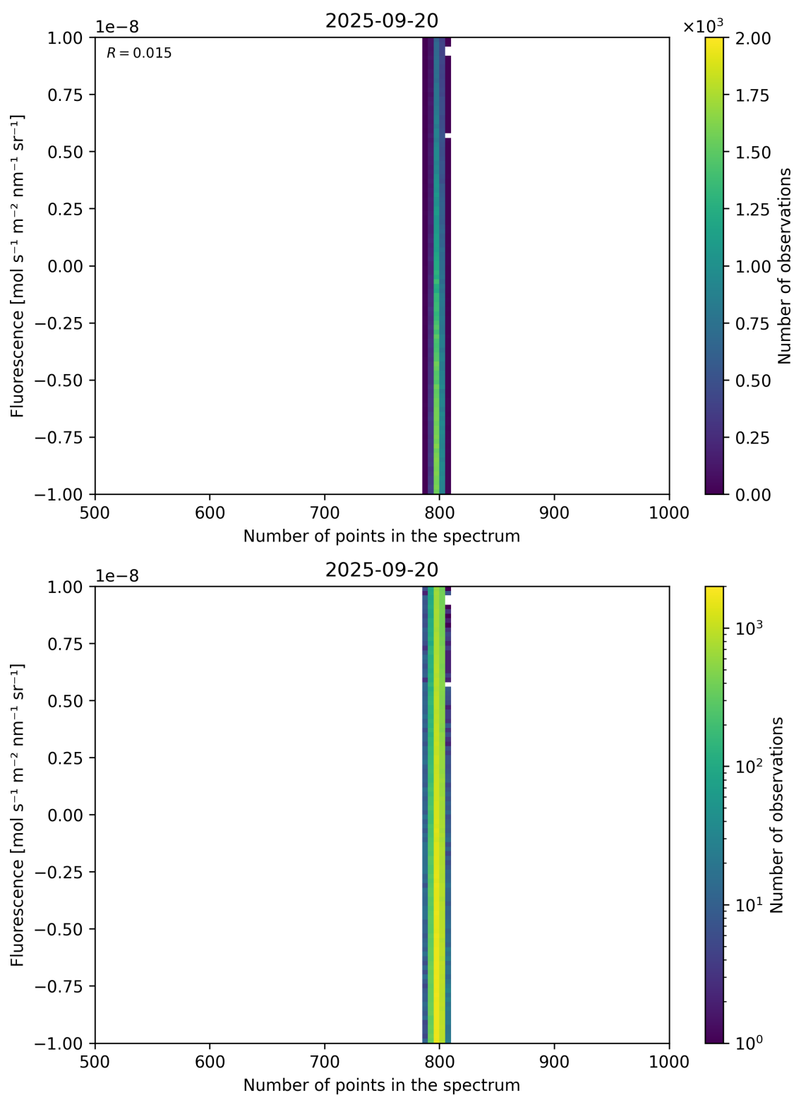
Figure 91: Scatter density plot of “Number of points in the spectrum” against “Fluorescence” for 2025-09-20 to 2025-09-21.
