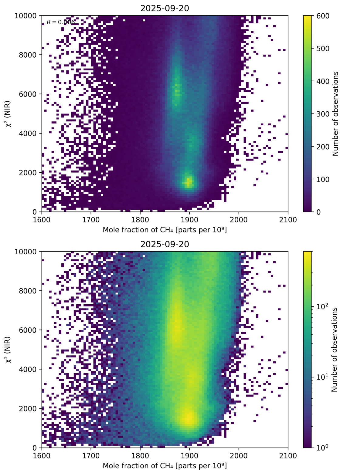
Figure 70: Scatter density plot of “Mole fraction of \text{CH}_4 ” against “ \chi^2 (NIR)” for 2025-09-20 to 2025-09-21.
