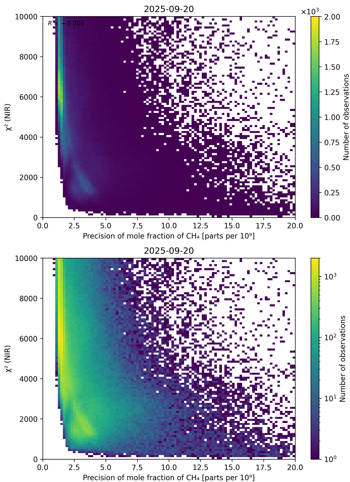
Figure 78: Scatter density plot of “Precision of mole fraction of \text{CH}_4 ” against “ \chi^2 (NIR)” for 2025-09-20 to 2025-09-21.
