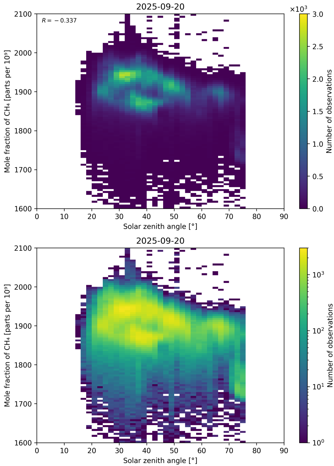
Figure 99: Scatter density plot of “Solar zenith angle” against “Mole fraction of CH 4 ” for 2025-09-20 to 2025-09-21.
