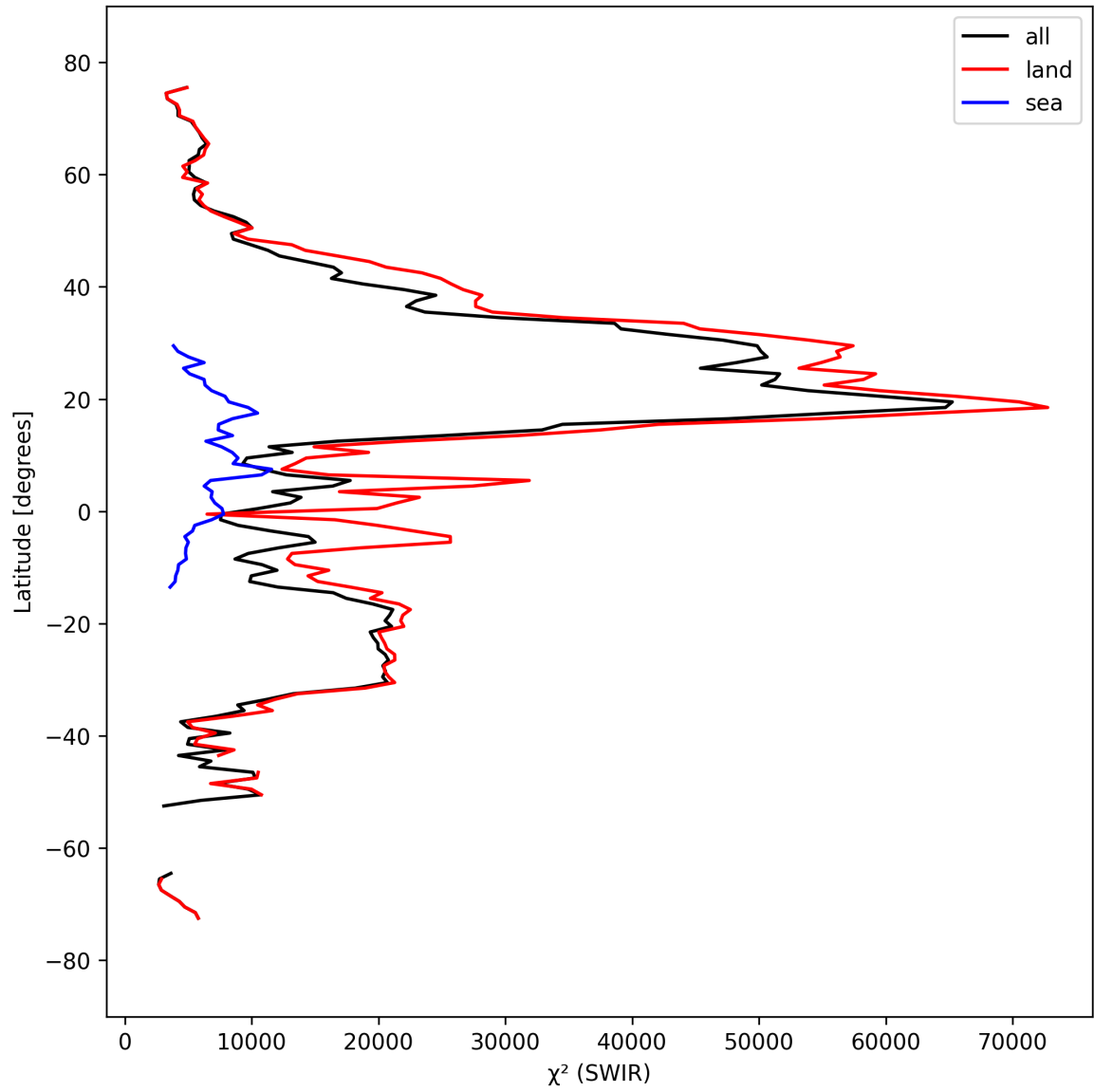
Figure 17: Zonal average of “ \chi^2 (SWIR)” for 2025-09-20 to 2025-09-21.
