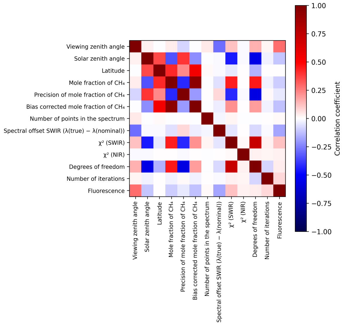
Figure 2: Map of correlation matrix for 2025-09-20 to 2025-09-21.
