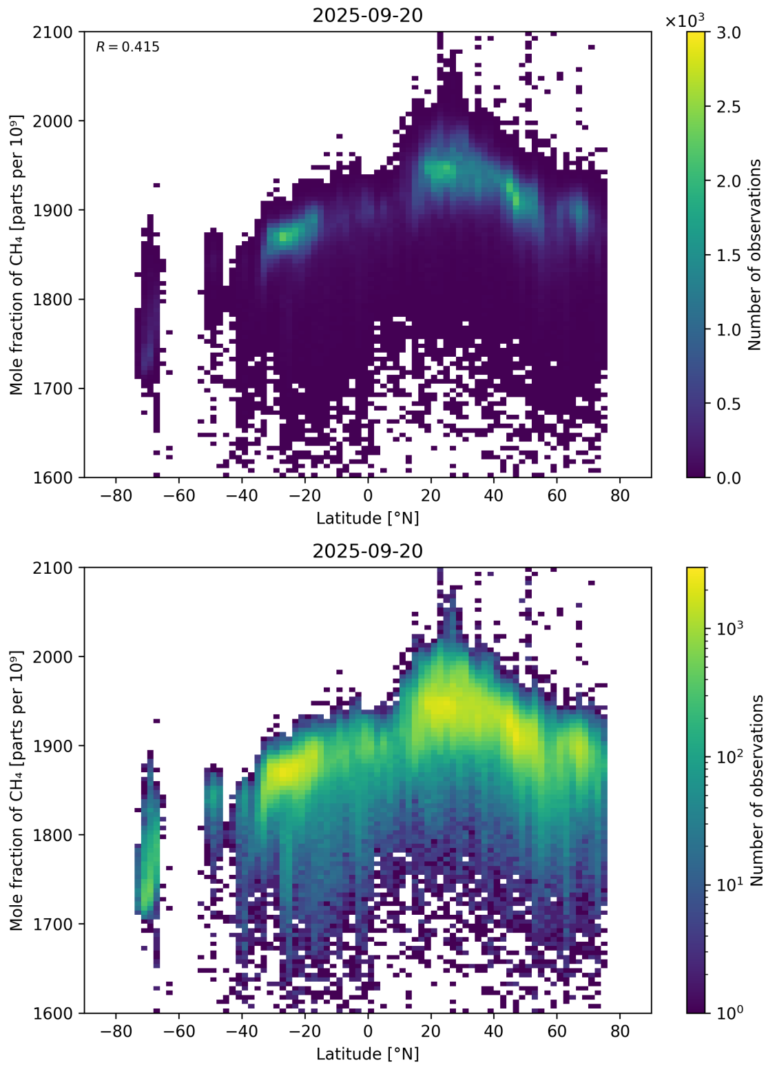
Figure 57: Scatter density plot of “Latitude” against “Mole fraction of \text{CH}_4 ” for 2025-09-20 to 2025-09-21.
