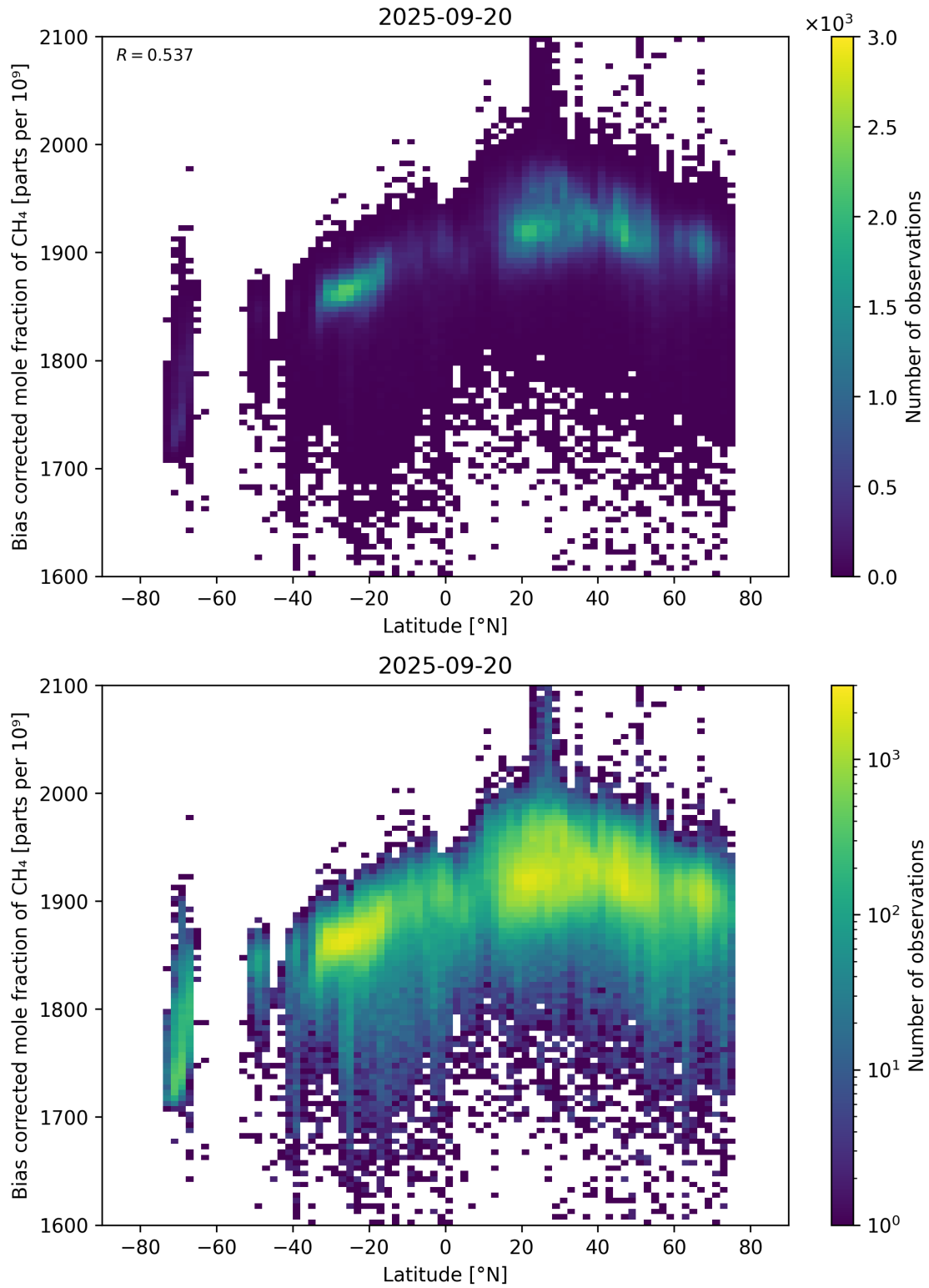
Figure 58: Scatter density plot of “Latitude” against “Bias corrected mole fraction of CH 4 ” for 2025-09-20 to 2025-09-21.
