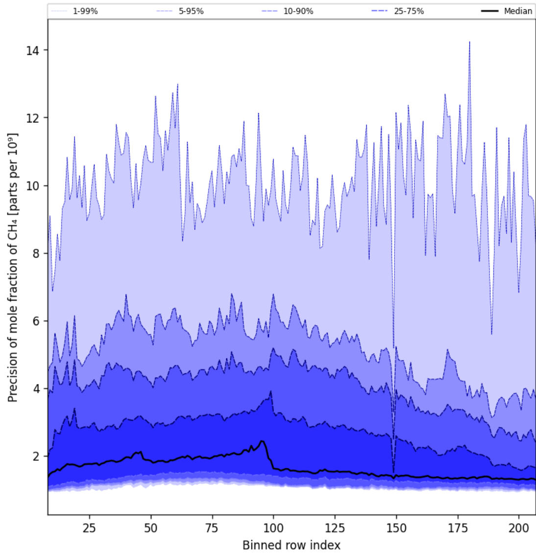
Figure 35: Along track statistics of “Precision of mole fraction of CH 4 ” for 2025-09-20 to 2025-09-21
