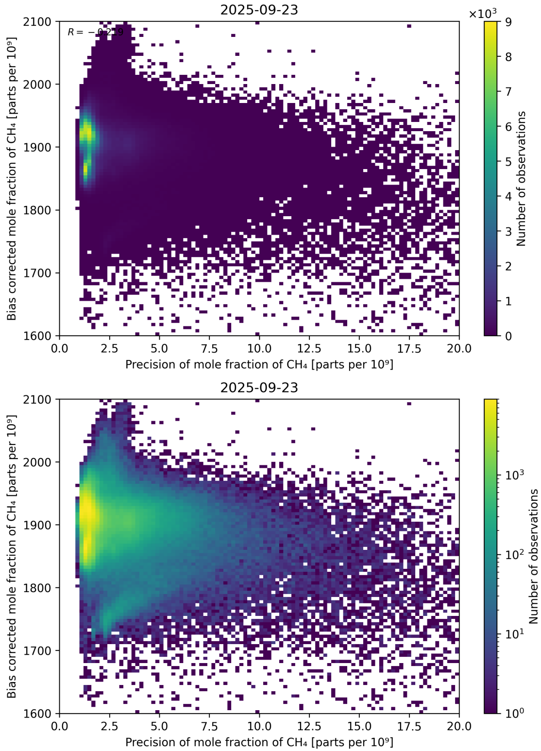
Figure 82: Scatter density plot of “Precision of mole fraction of CH 4 ” against “Bias corrected mole fraction of CH 4 ” for 2025-09-22 to 2025-09-24.
