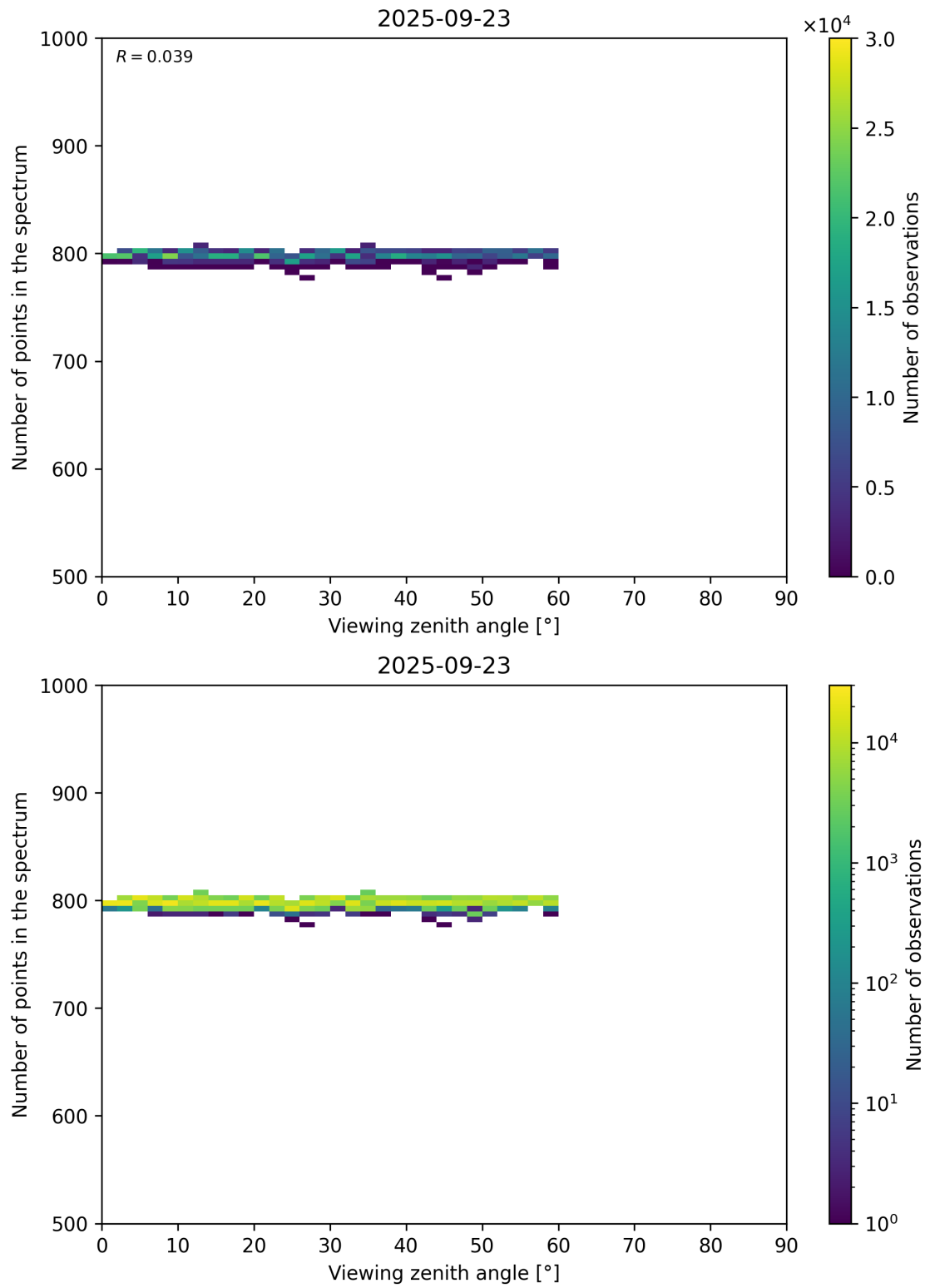
Figure 114: Scatter density plot of “Viewing zenith angle” against “Number of points in the spectrum” for 2025-09-22 to 2025-09-24.
