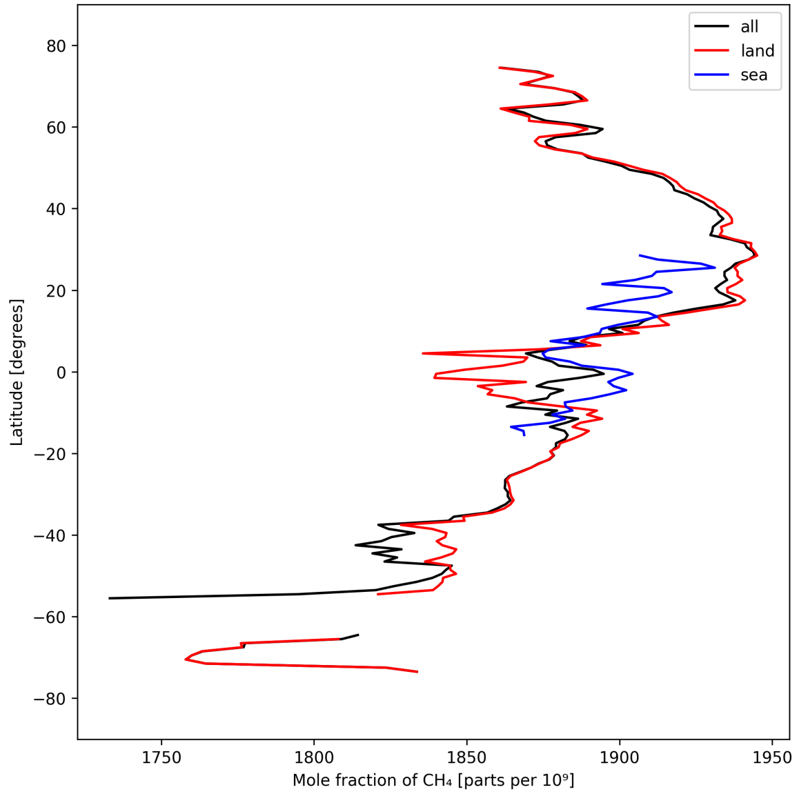
Figure 12: Zonal average of “Mole fraction of CH 4 ” for 2025-09-22 to 2025-09-24.
