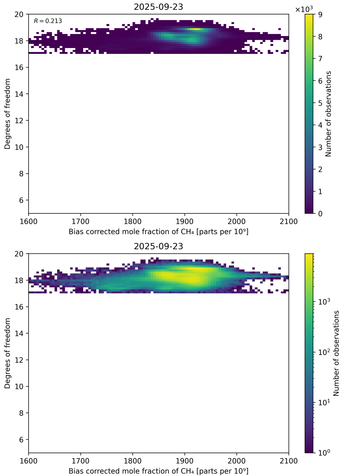
Figure 65: Scatter density plot of “Bias corrected mole fraction of CH 4 ” against “Degrees of freedom” for 2025-09-22 to 2025-09-24.
