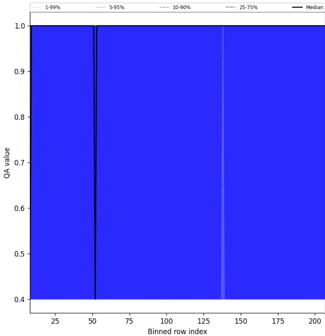
Figure 33: Along track statistics of “QA value” for 2025-09-22 to 2025-09-24
