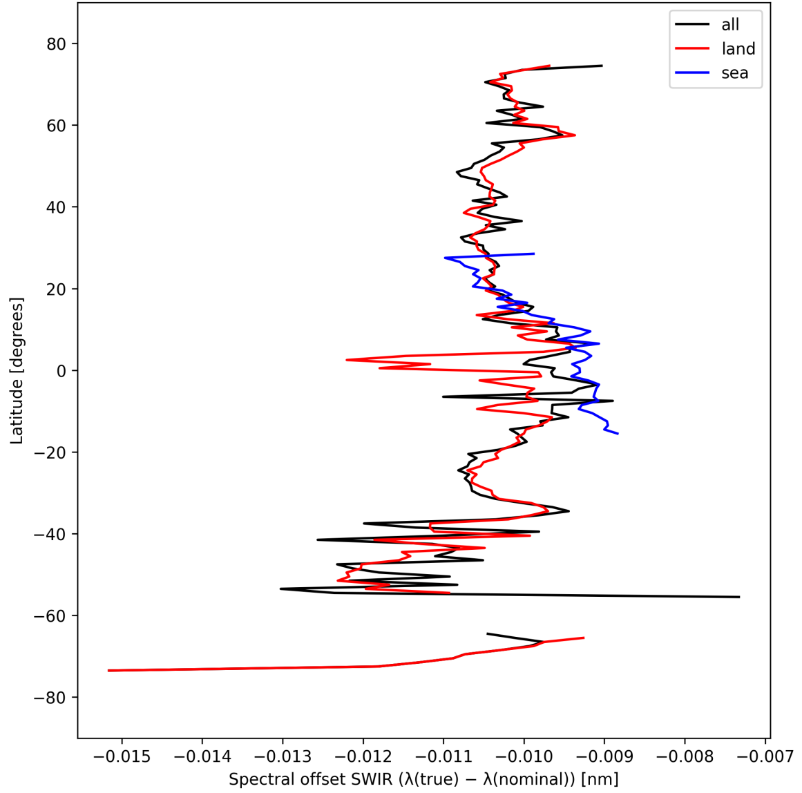
Figure 16: Zonal average of “Spectral offset SWIR ( \lambda_{\text{true}} - \lambda_{\text{nominal}} )” for 2025-09-22 to 2025-09-24.
