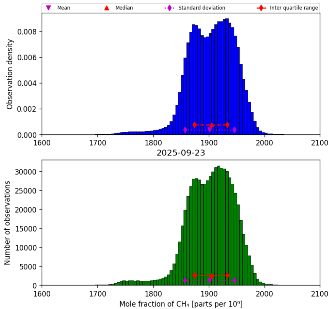
Figure 23: Histogram of “Mole fraction of CH 4 ” for 2025-09-22 to 2025-09-24
