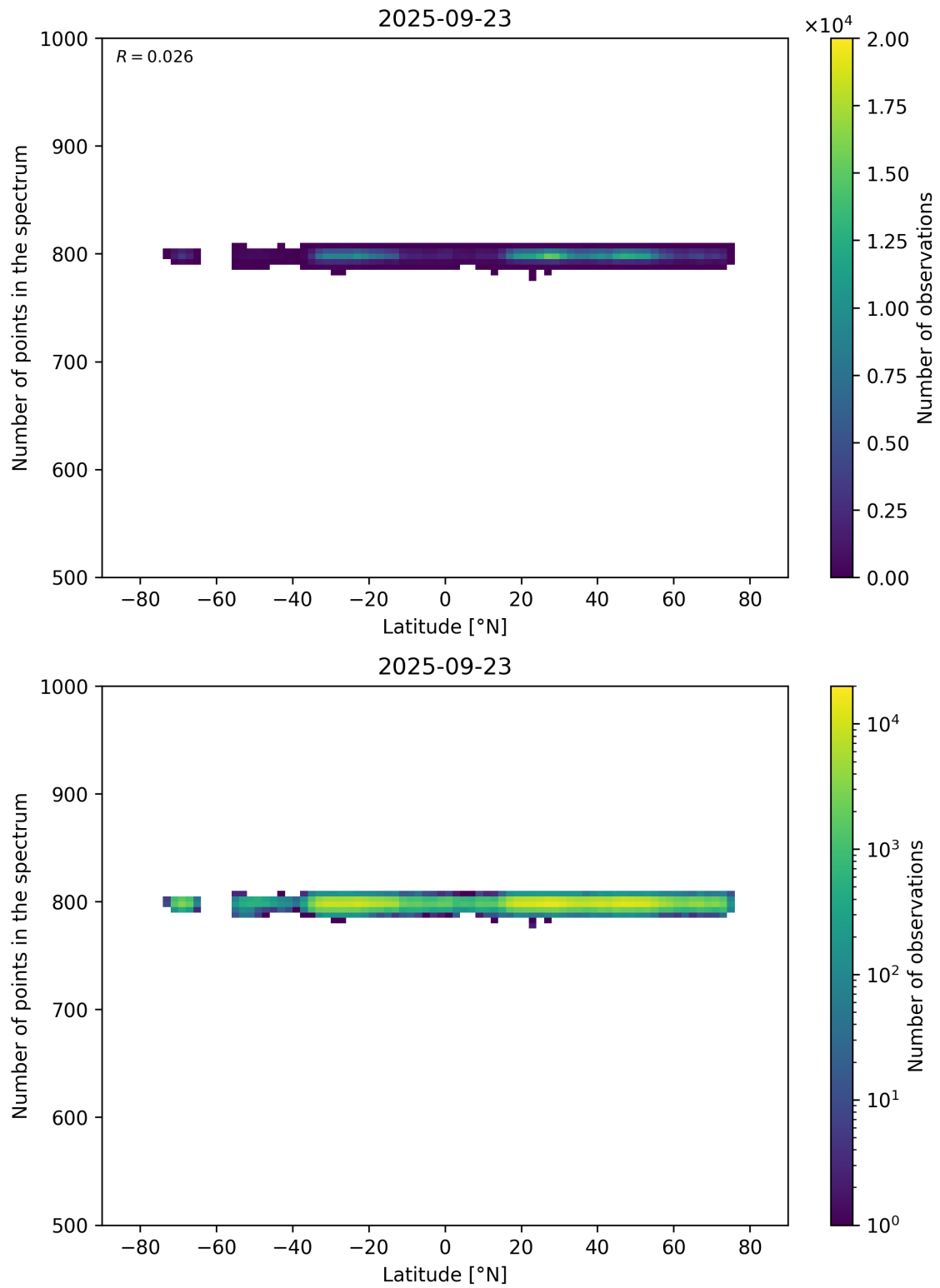
Figure 61: Scatter density plot of “Latitude” against “Number of points in the spectrum” for 2025-09-22 to 2025-09-24.
