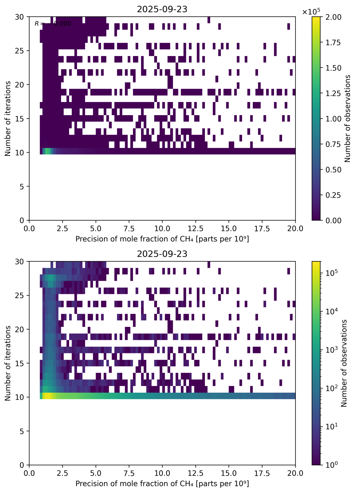
Figure 83: Scatter density plot of “Precision of mole fraction of CH 4 ” against “Number of iterations” for 2025-09-22 to 2025-09-24.
