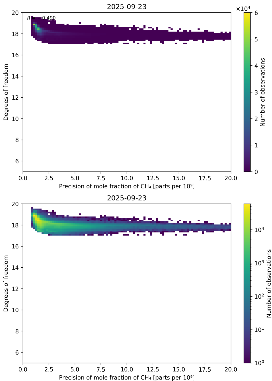
Figure 80: Scatter density plot of “Precision of mole fraction of CH 4 ” against “Degrees of freedom” for 2025-09-22 to 2025-09-24.
