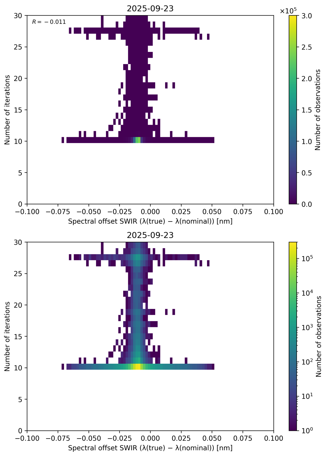
Figure 121: Scatter density plot of “Spectral offset SWIR ( \lambda_{\text{true}} - \lambda_{\text{nominal}} )” against “Number of iterations” for 2025-09-22 to 2025-09-24.
