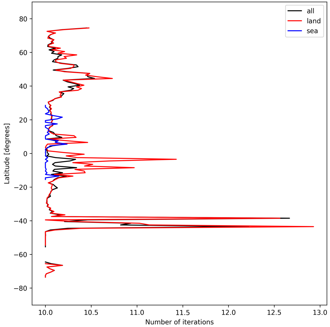
Figure 20: Zonal average of “Number of iterations” for 2025-09-22 to 2025-09-24.
