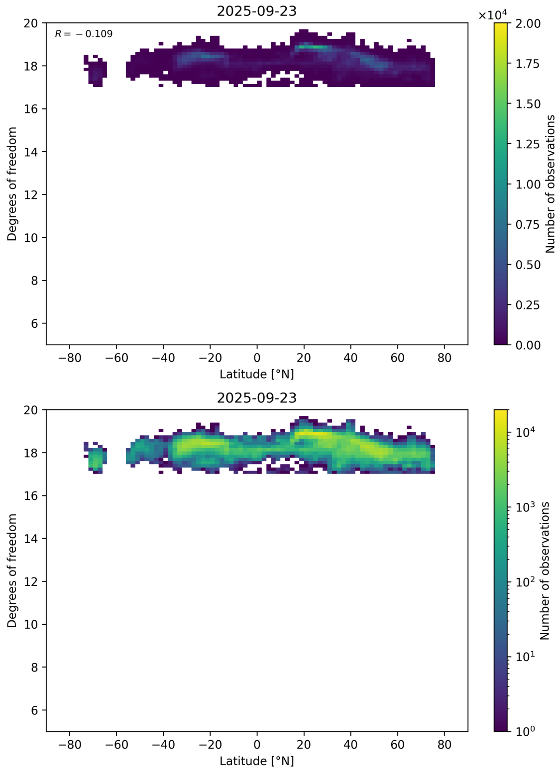
Figure 55: Scatter density plot of “Latitude” against “Degrees of freedom” for 2025-09-22 to 2025-09-24.
