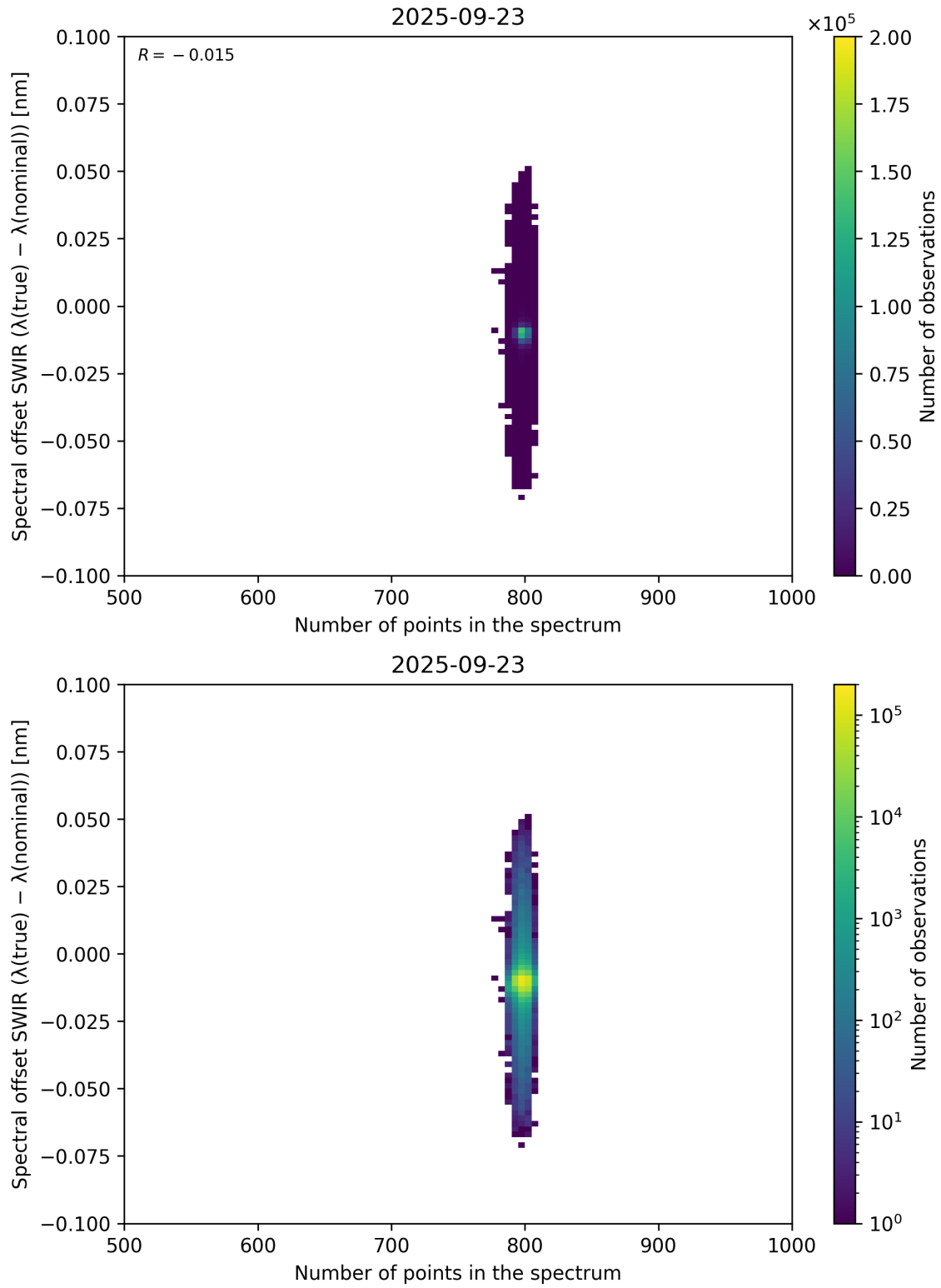
Figure 93: Scatter density plot of “Number of points in the spectrum” against “Spectral offset SWIR ( \lambda_{\text{true}} - \lambda_{\text{nominal}} )” for 2025-09-22 to 2025-09-24.
