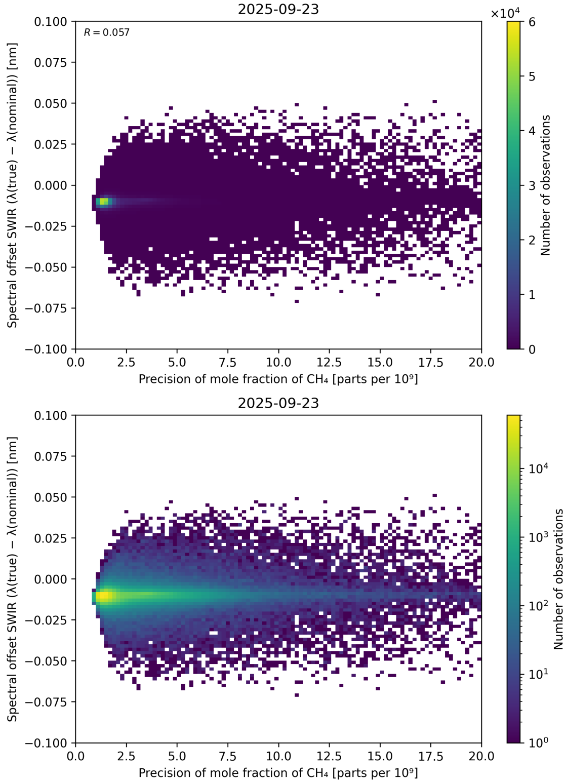
Figure 85: Scatter density plot of “Precision of mole fraction of CH 4 ” against “Spectral offset SWIR ( \lambda_{\text{true}} - \lambda_{\text{nominal}} )” for 2025-09-22 to 2025-09-24.
