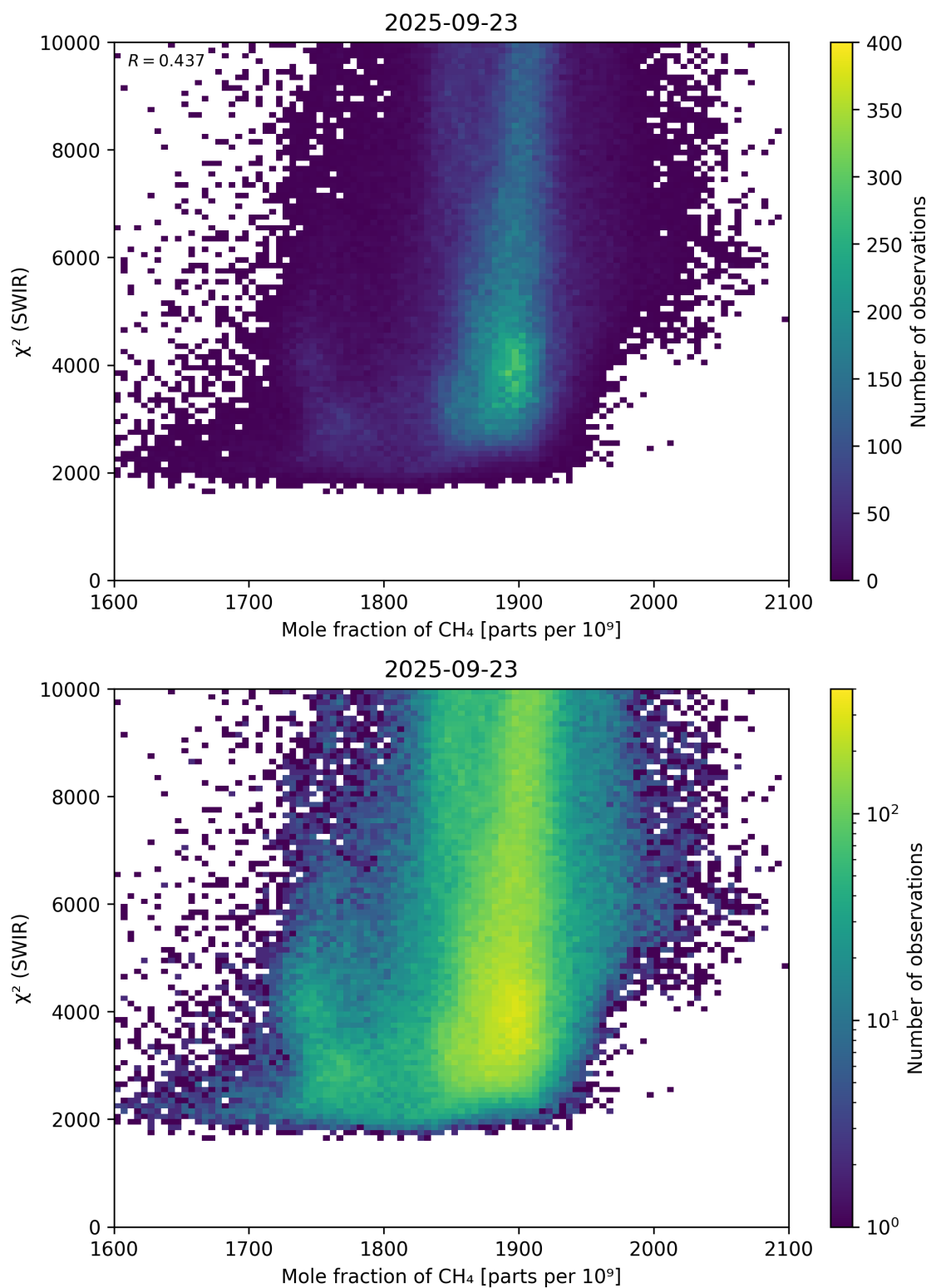
Figure 71: Scatter density plot of “Mole fraction of CH 4 ” against “ \chi^2 (SWIR)” for 2025-09-22 to 2025-09-24.
