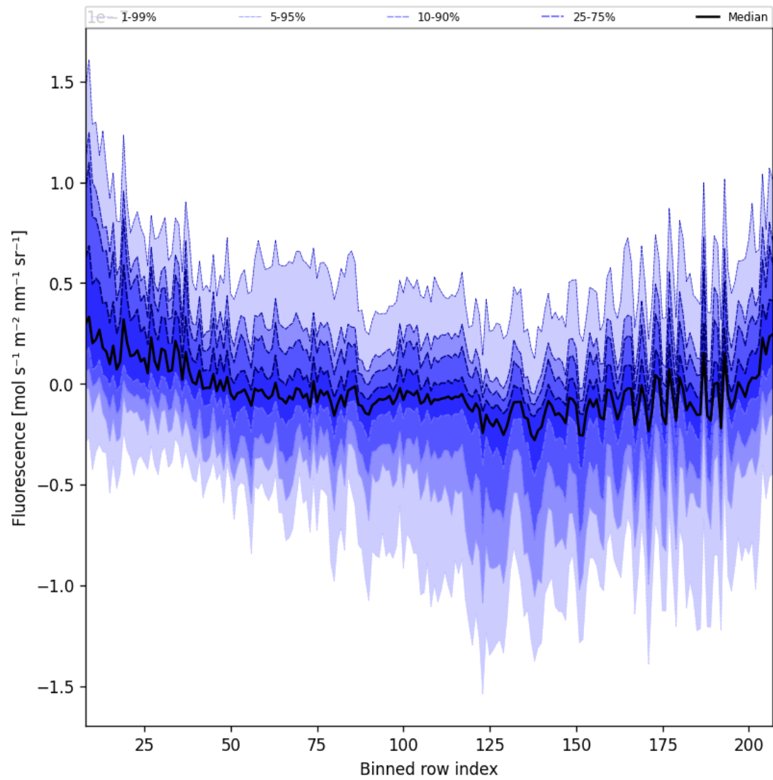
Figure 43: Along track statistics of “Fluorescence” for 2025-09-22 to 2025-09-24
