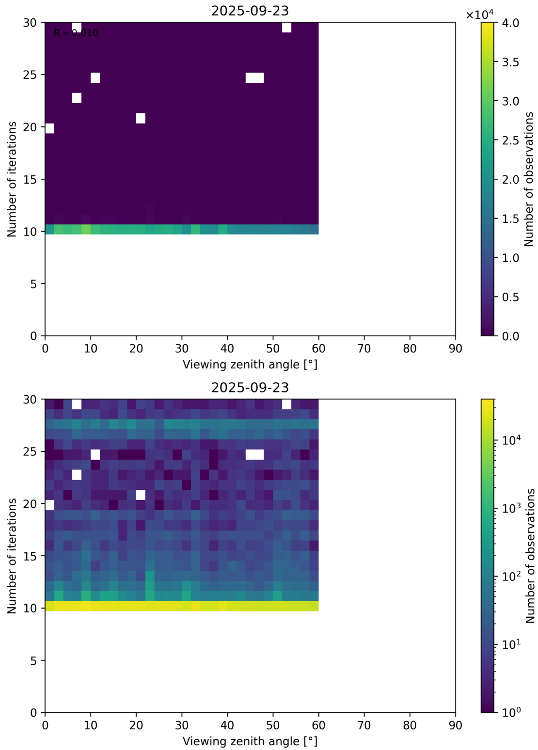
Figure 113: Scatter density plot of “Viewing zenith angle” against “Number of iterations” for 2025-09-22 to 2025-09-24.
