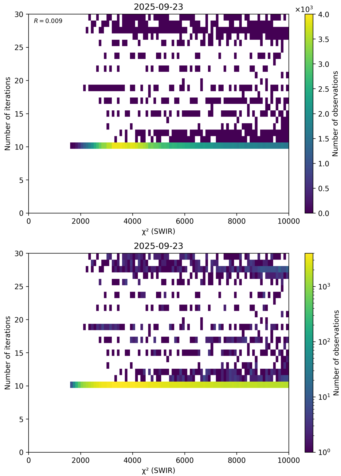
Figure 50: Scatter density plot of " \chi^2 (SWIR)" against "Number of iterations" for 2025-09-22 to 2025-09-24.
