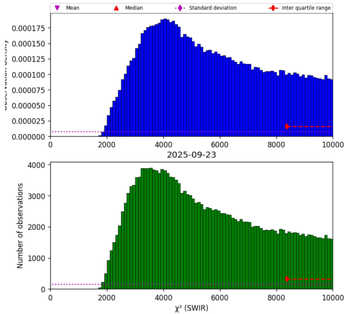
Figure 28: Histogram of “ \chi^2 (SWIR)” for 2025-09-22 to 2025-09-24
