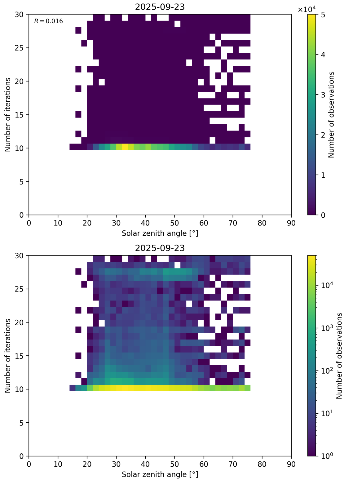
Figure 102: Scatter density plot of “Solar zenith angle” against “Number of iterations” for 2025-09-22 to 2025-09-24.
