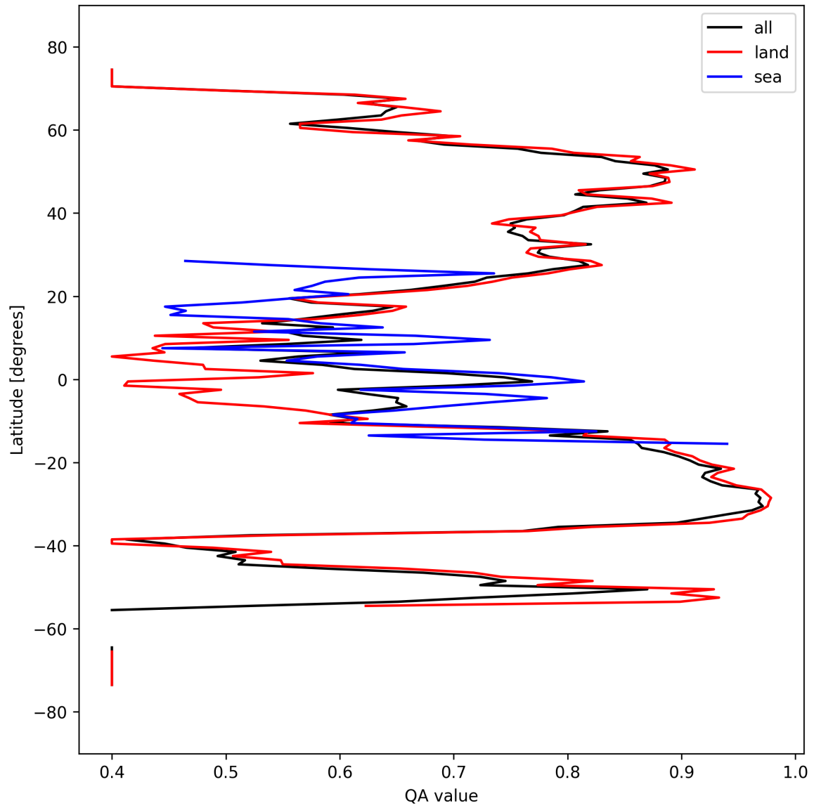
Figure 11: Zonal average of “QA value” for 2025-09-22 to 2025-09-24.
