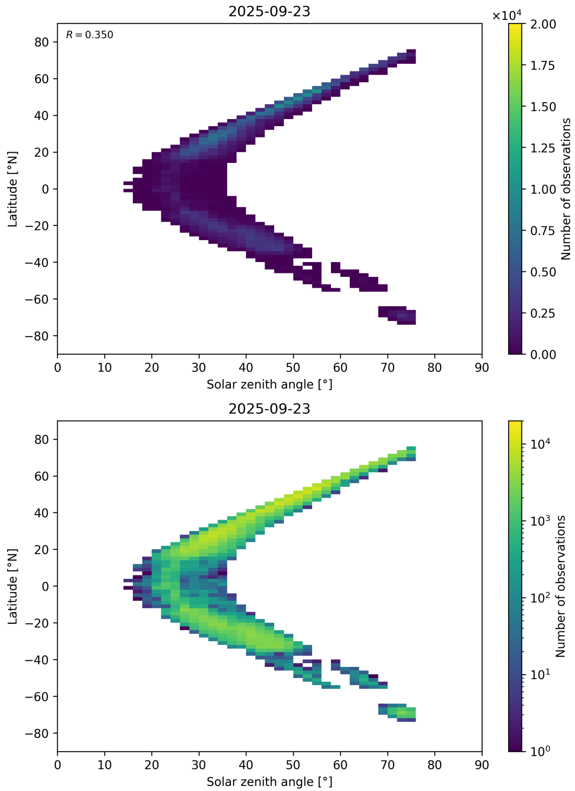
Figure 98: Scatter density plot of “Solar zenith angle” against “Latitude” for 2025-09-22 to 2025-09-24.
