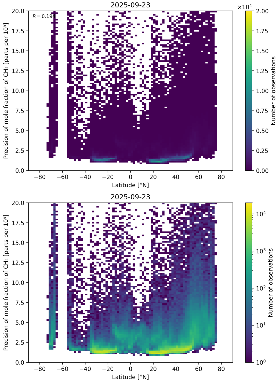
Figure 59: Scatter density plot of “Latitude” against “Precision of mole fraction of \text{CH}_4 ” for 2025-09-22 to 2025-09-24.
