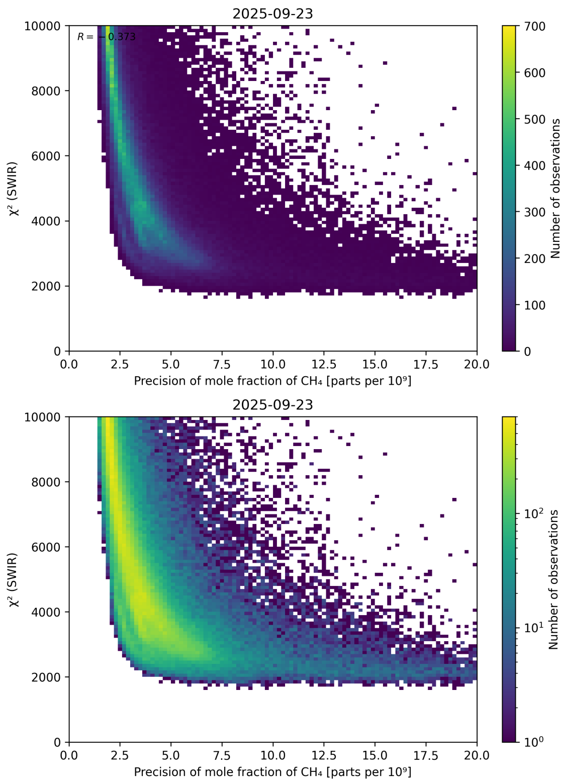
Figure 79: Scatter density plot of “Precision of mole fraction of \text{CH}_4 ” against “ \chi^2 (SWIR)” for 2025-09-22 to 2025-09-24.
