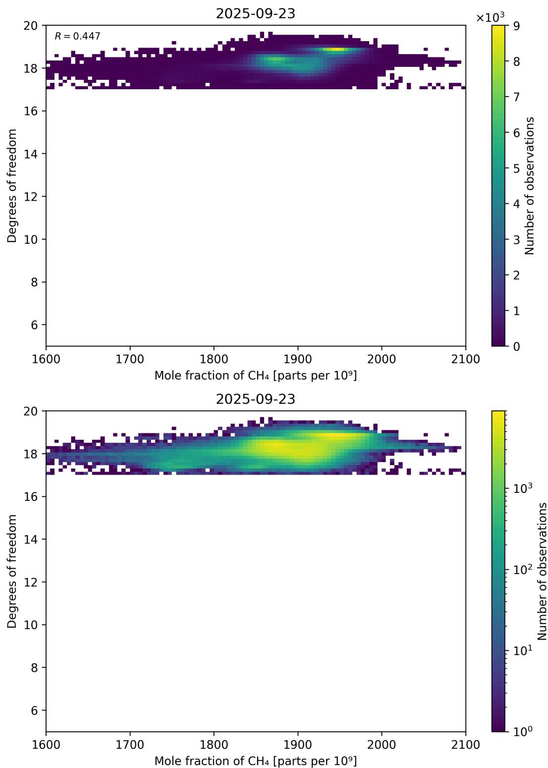
Figure 72: Scatter density plot of “Mole fraction of CH 4 ” against “Degrees of freedom” for 2025-09-22 to 2025-09-24.
