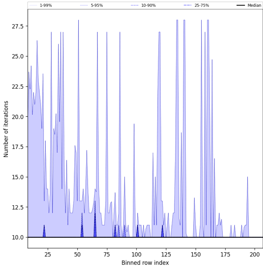
Figure 42: Along track statistics of “Number of iterations” for 2025-09-22 to 2025-09-24
