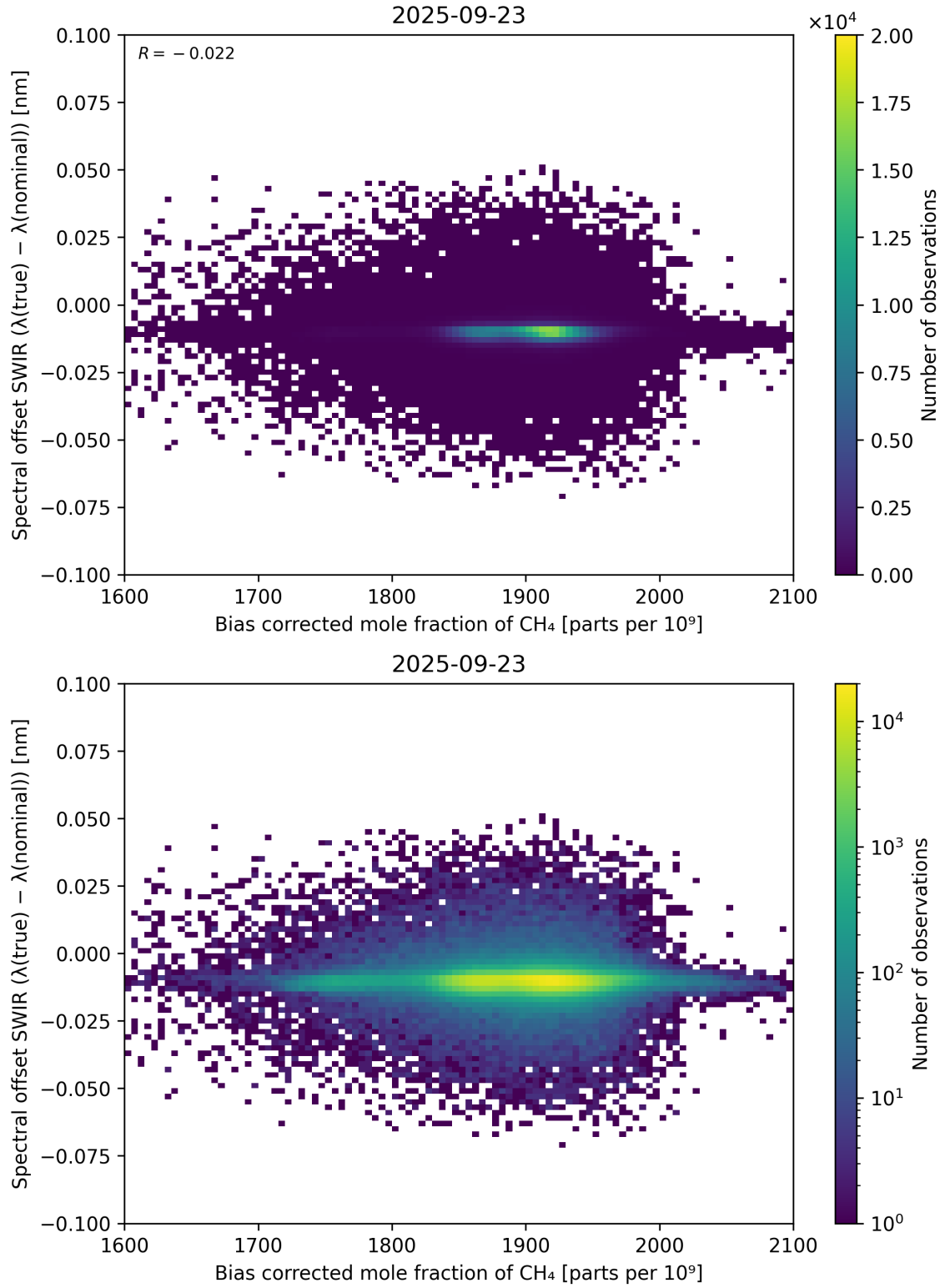
Figure 69: Scatter density plot of “Bias corrected mole fraction of \text{CH}_4 ” against “Spectral offset SWIR ( \lambda_{\text{true}} - \lambda_{\text{nominal}} )” for 2025-09-22 to 2025-09-24.
