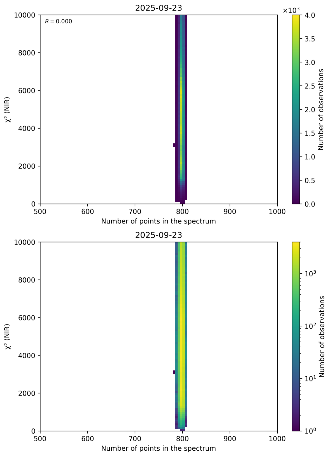
Figure 88: Scatter density plot of “Number of points in the spectrum” against “ \chi^2 (NIR)” for 2025-09-22 to 2025-09-24.
