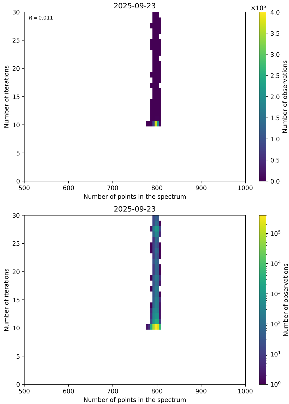
Figure 92: Scatter density plot of “Number of points in the spectrum” against “Number of iterations” for 2025-09-22 to 2025-09-24.
