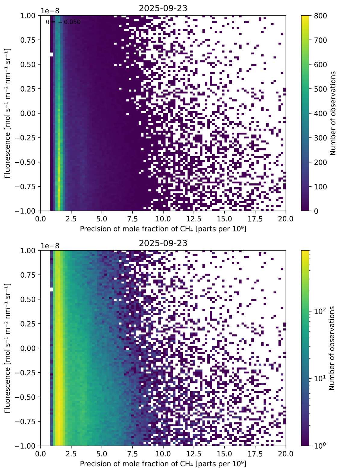
Figure 81: Scatter density plot of “Precision of mole fraction of \text{CH}_4 ” against “Fluorescence” for 2025-09-22 to 2025-09-24.
