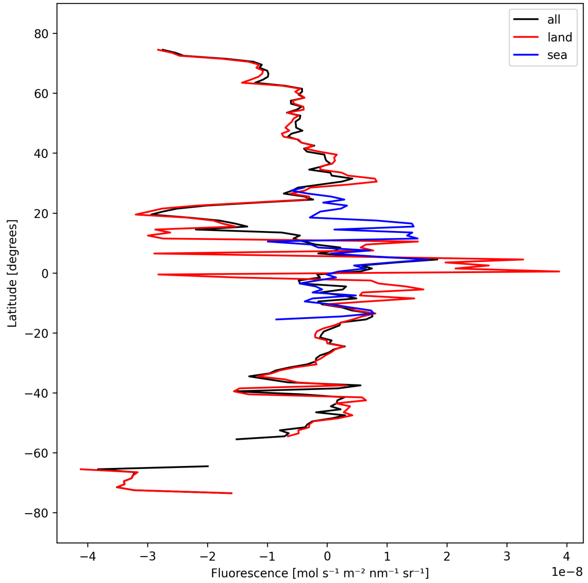
Figure 21: Zonal average of “Fluorescence” for 2025-09-22 to 2025-09-24.
