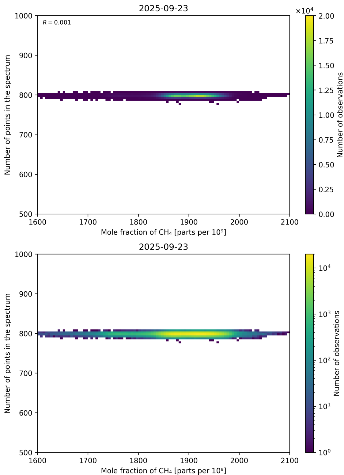
Figure 77: Scatter density plot of “Mole fraction of CH 4 ” against “Number of points in the spectrum” for 2025-09-22 to 2025-09-24.
