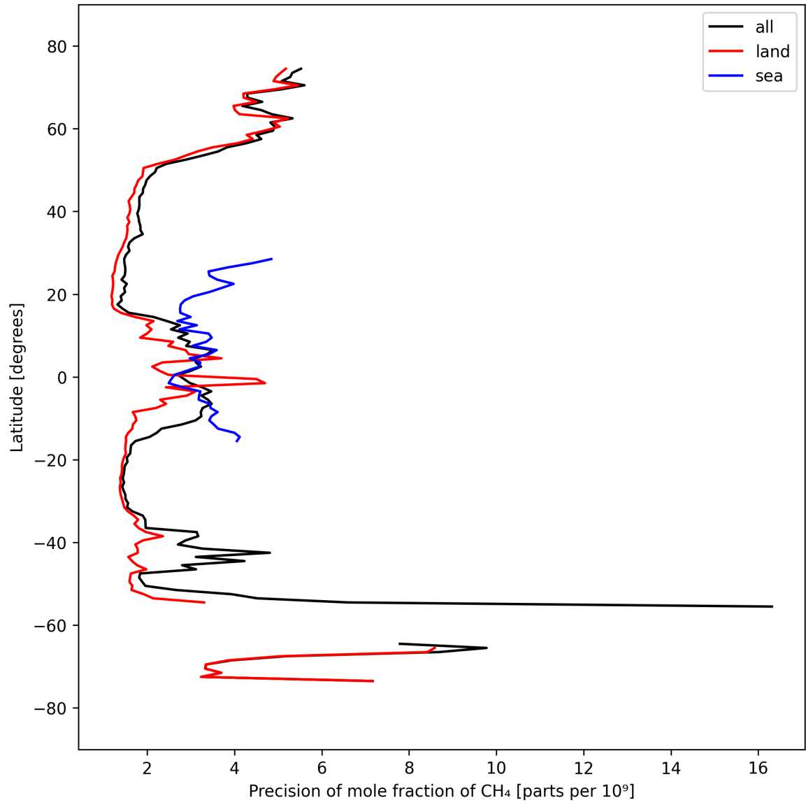
Figure 13: Zonal average of “Precision of mole fraction of CH 4 ” for 2025-09-22 to 2025-09-24.
