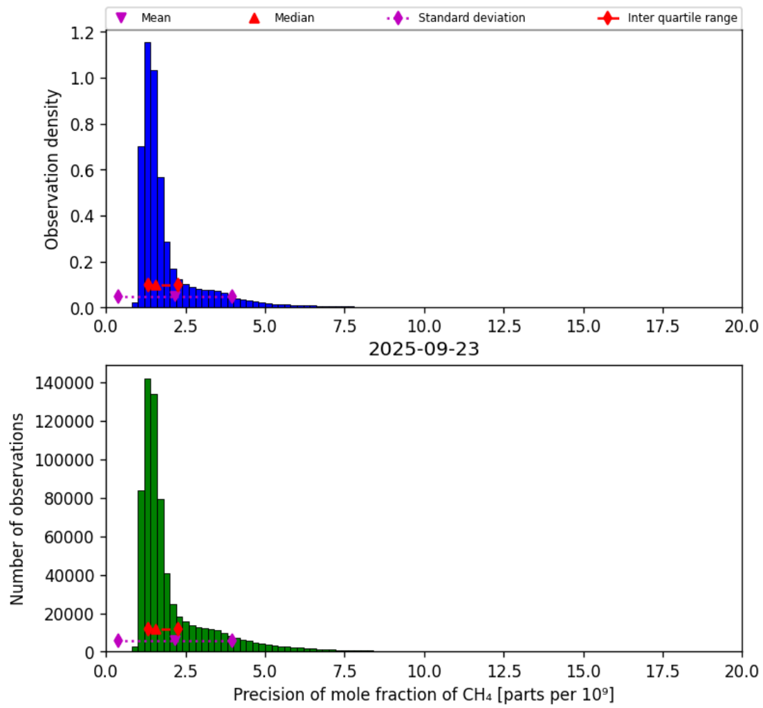
Figure 24: Histogram of “Precision of mole fraction of CH 4 ” for 2025-09-22 to 2025-09-24
