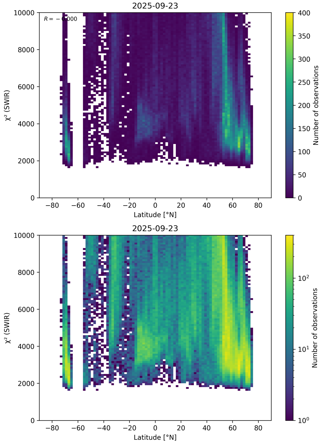
Figure 54: Scatter density plot of “Latitude” against “ \chi^2 (SWIR)” for 2025-09-22 to 2025-09-24.
