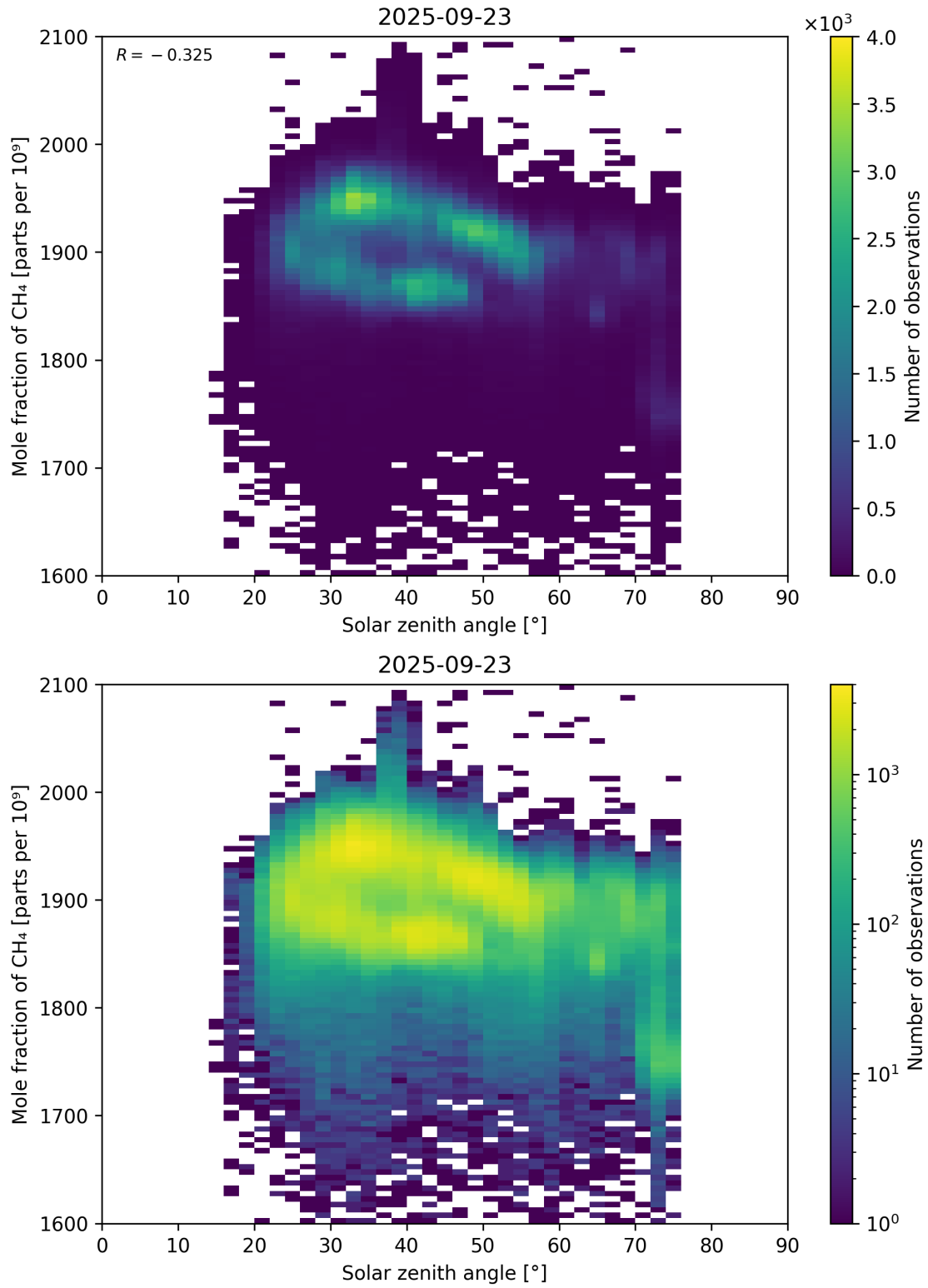
Figure 99: Scatter density plot of “Solar zenith angle” against “Mole fraction of \text{CH}_4 ” for 2025-09-22 to 2025-09-24.
