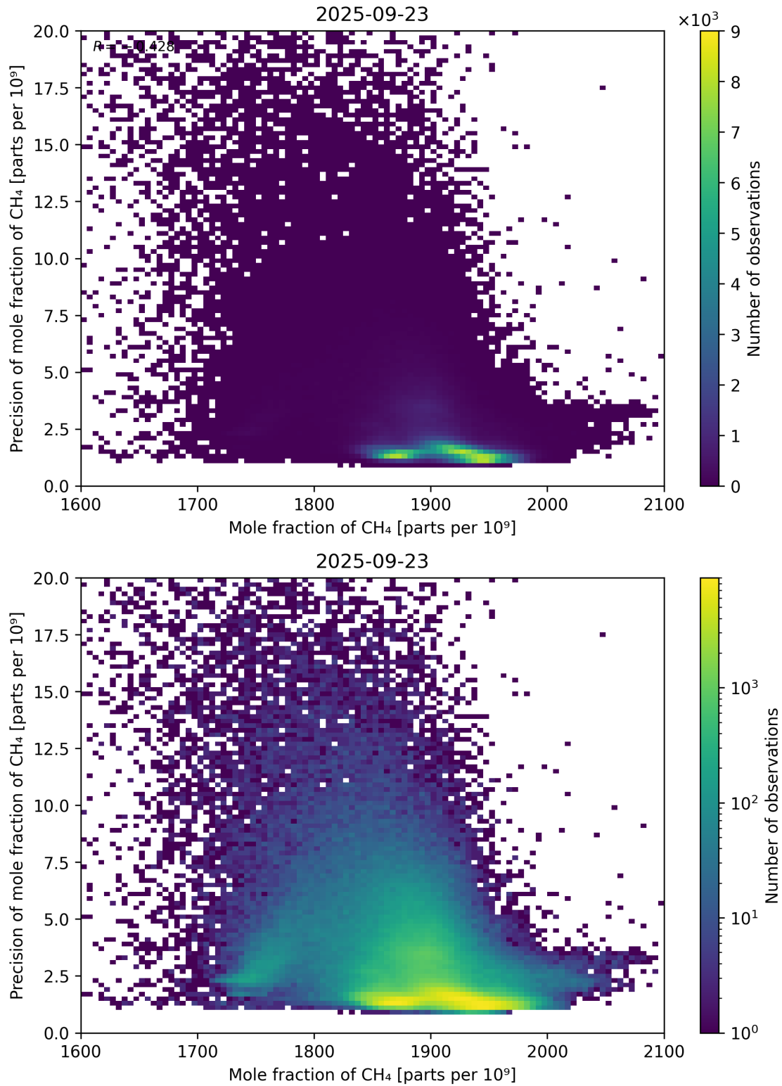
Figure 75: Scatter density plot of “Mole fraction of CH 4 ” against “Precision of mole fraction of CH 4 ” for 2025-09-22 to 2025-09-24.
