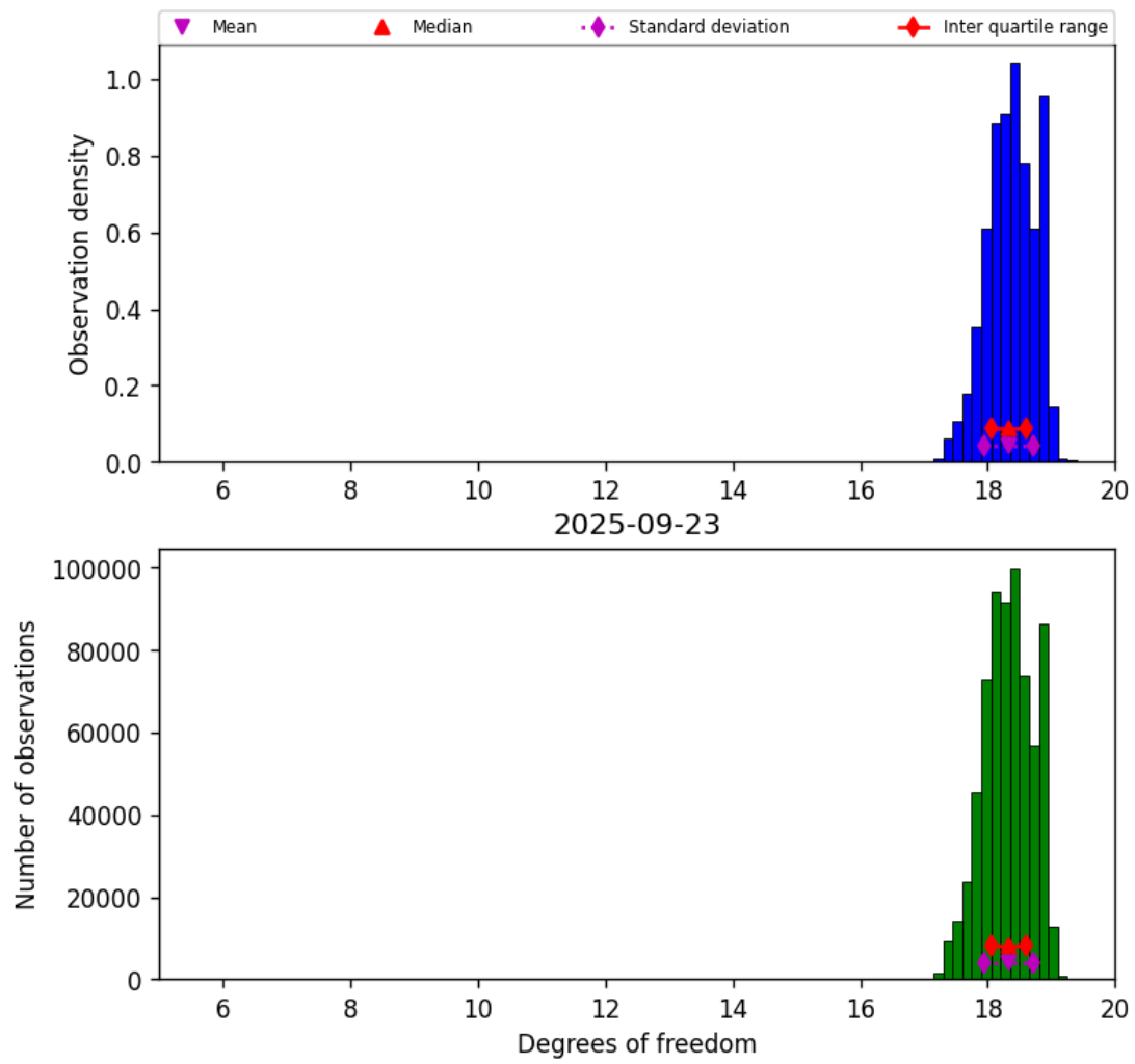
Figure 30: Histogram of “Degrees of freedom” for 2025-09-22 to 2025-09-24
