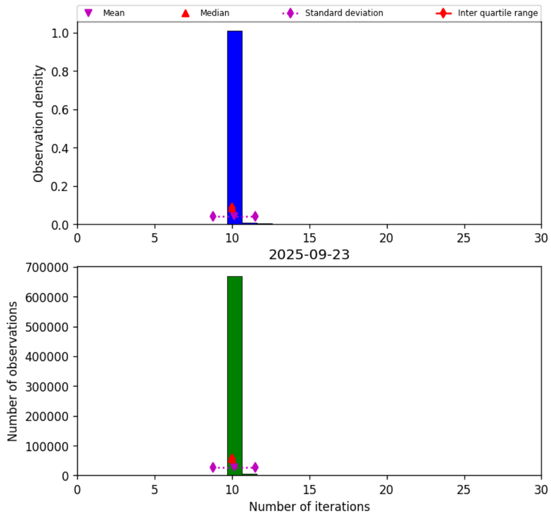
Figure 31: Histogram of “Number of iterations” for 2025-09-22 to 2025-09-24
