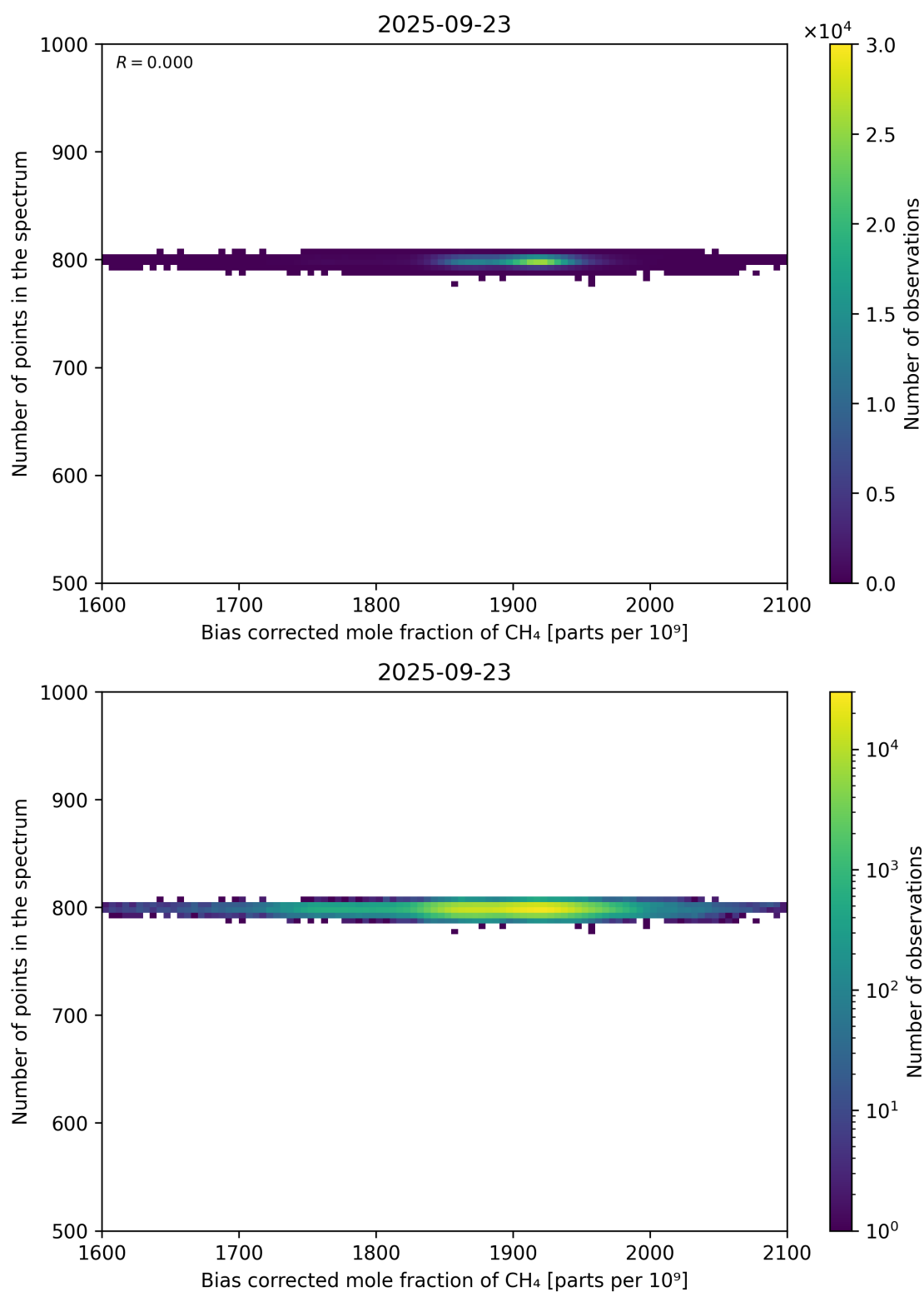
Figure 68: Scatter density plot of “Bias corrected mole fraction of CH 4 ” against “Number of points in the spectrum” for 2025-09-22 to 2025-09-24.
