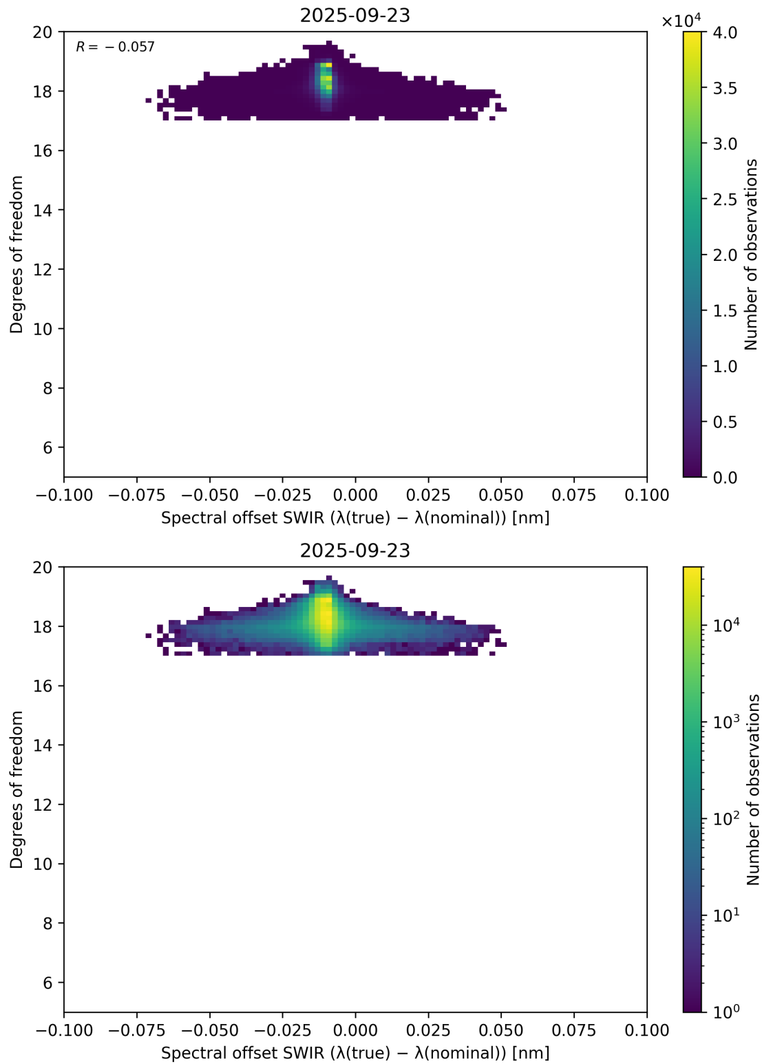
Figure 119: Scatter density plot of “Spectral offset SWIR ( \lambda_{\text{true}} - \lambda_{\text{nominal}} )” against “Degrees of freedom” for 2025-09-22 to 2025-09-24.
