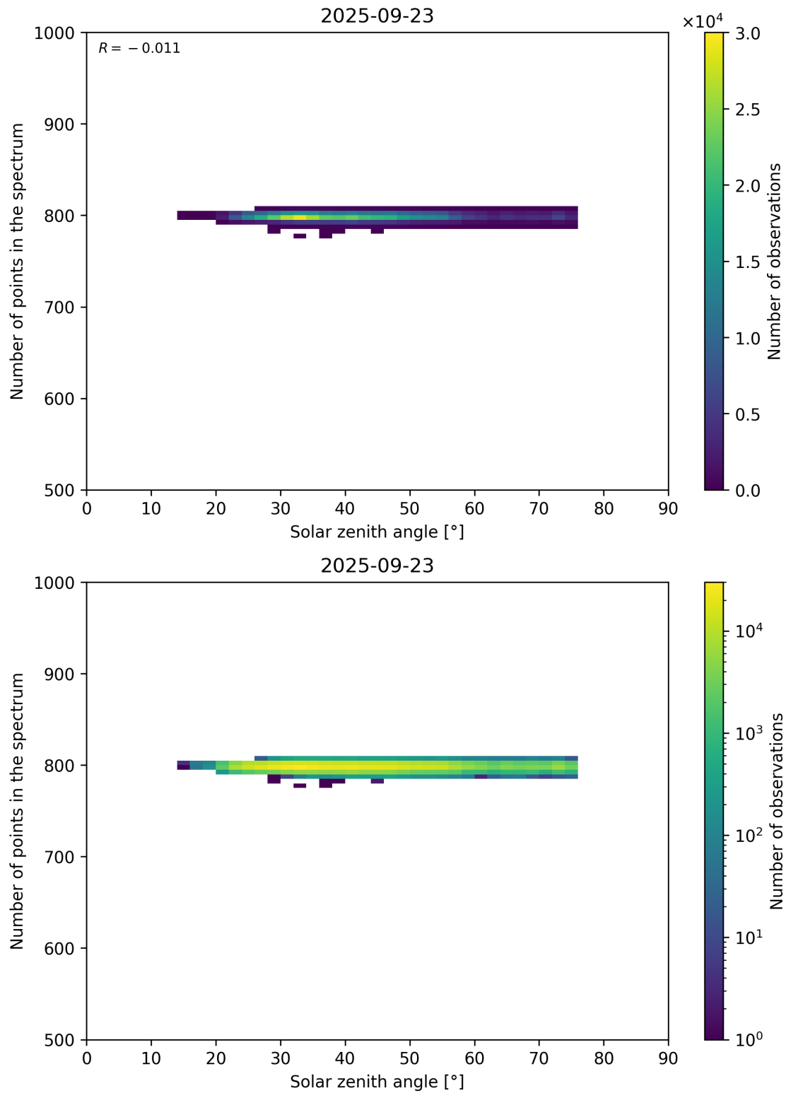
Figure 103: Scatter density plot of “Solar zenith angle” against “Number of points in the spectrum” for 2025-09-22 to 2025-09-24.
