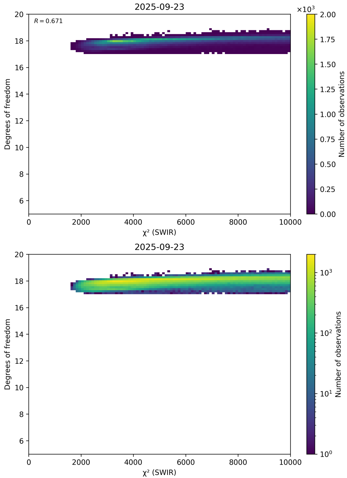
Figure 48: Scatter density plot of “ \chi^2 (SWIR)” against “Degrees of freedom” for 2025-09-22 to 2025-09-24.
