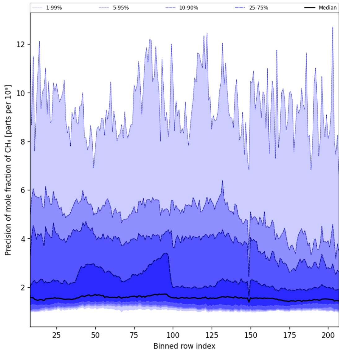
Figure 35: Along track statistics of “Precision of mole fraction of CH 4 ” for 2025-09-22 to 2025-09-24
