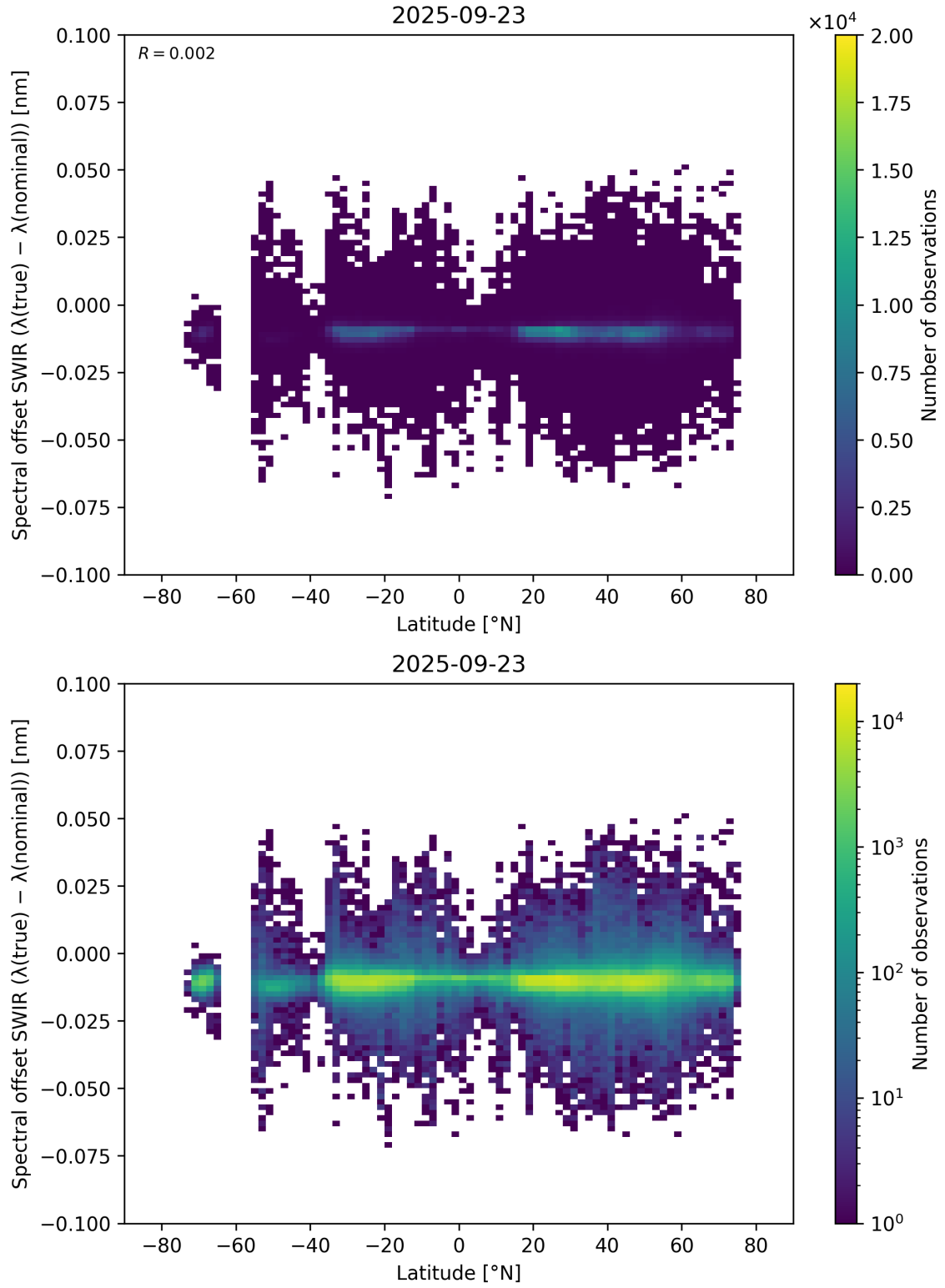
Figure 62: Scatter density plot of “Latitude” against “Spectral offset SWIR ( \lambda_{\text{true}} - \lambda_{\text{nominal}} )” for 2025-09-22 to 2025-09-24.
