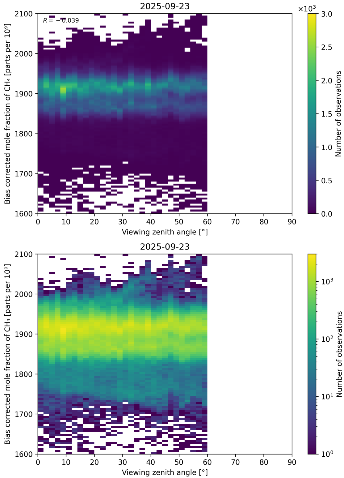
Figure 111: Scatter density plot of “Viewing zenith angle” against “Bias corrected mole fraction of CH 4 ” for 2025-09-22 to 2025-09-24.
