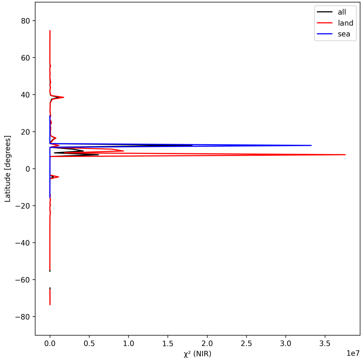
Figure 18: Zonal average of “ \chi^2 (NIR)” for 2025-09-22 to 2025-09-24.
