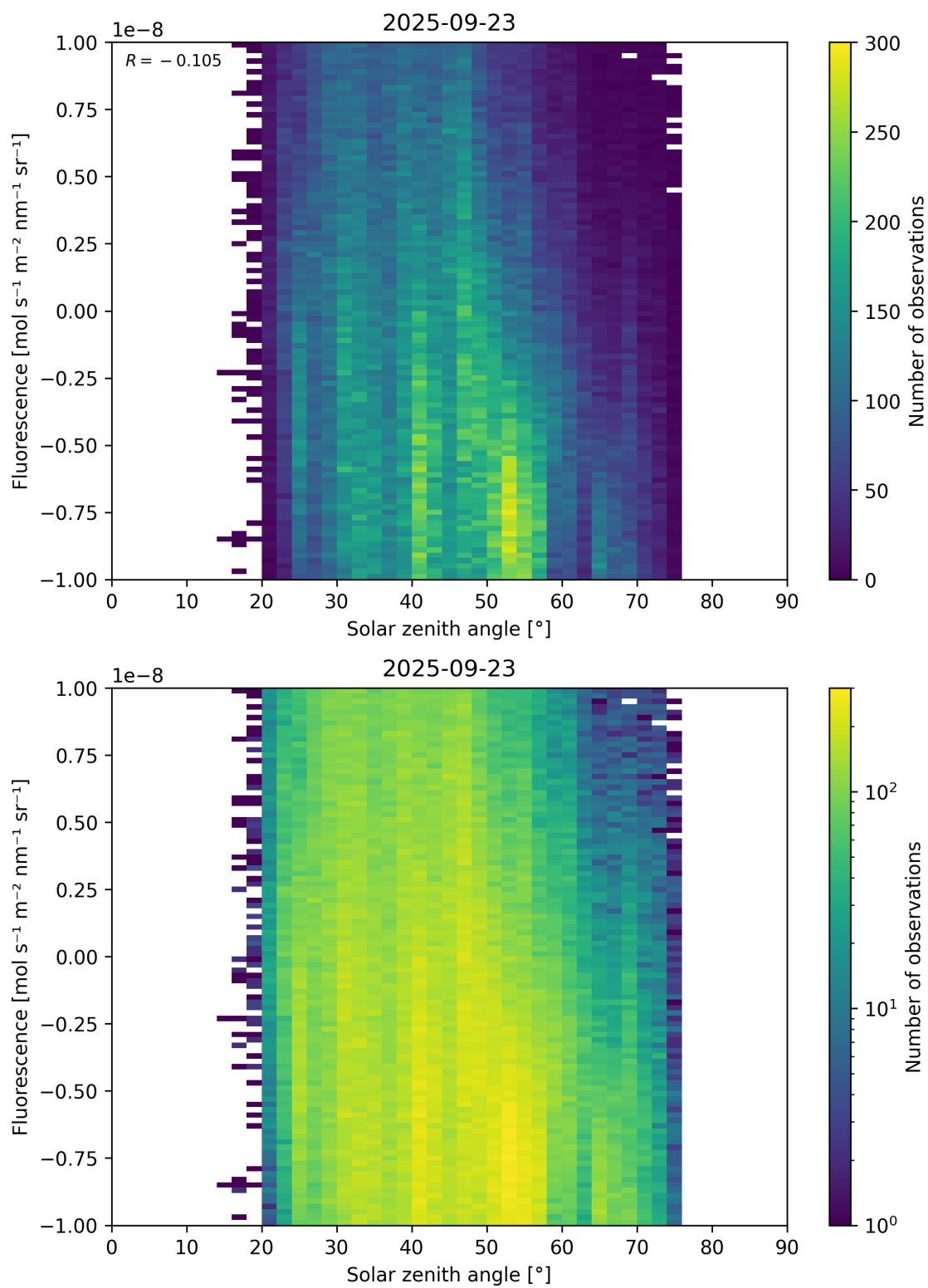
Figure 97: Scatter density plot of “Solar zenith angle” against “Fluorescence” for 2025-09-22 to 2025-09-24.
