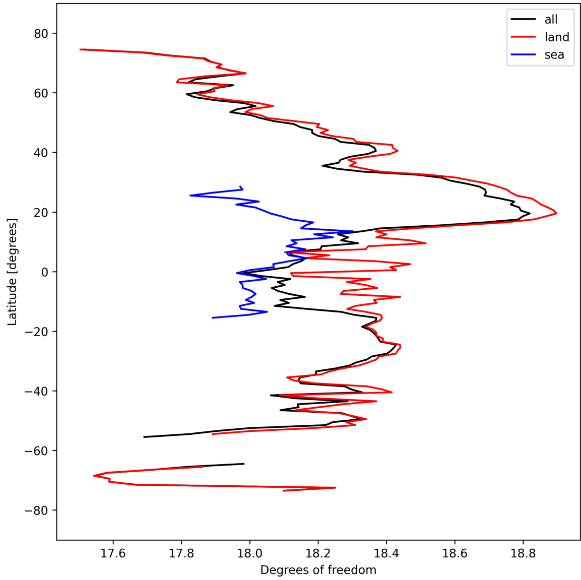
Figure 19: Zonal average of “Degrees of freedom” for 2025-09-22 to 2025-09-24.
