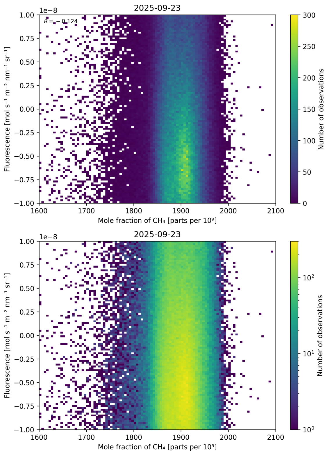
Figure 73: Scatter density plot of “Mole fraction of \text{CH}_4 ” against “Fluorescence” for 2025-09-22 to 2025-09-24.
