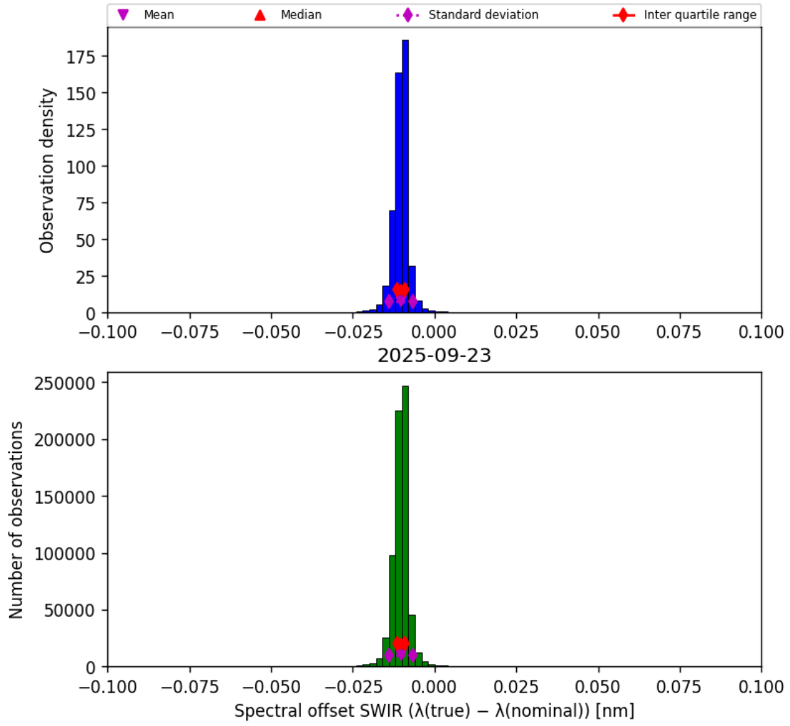
Figure 27: Histogram of “Spectral offset SWIR ( \lambda_{\text{true}} - \lambda_{\text{nominal}} )” for 2025-09-22 to 2025-09-24
