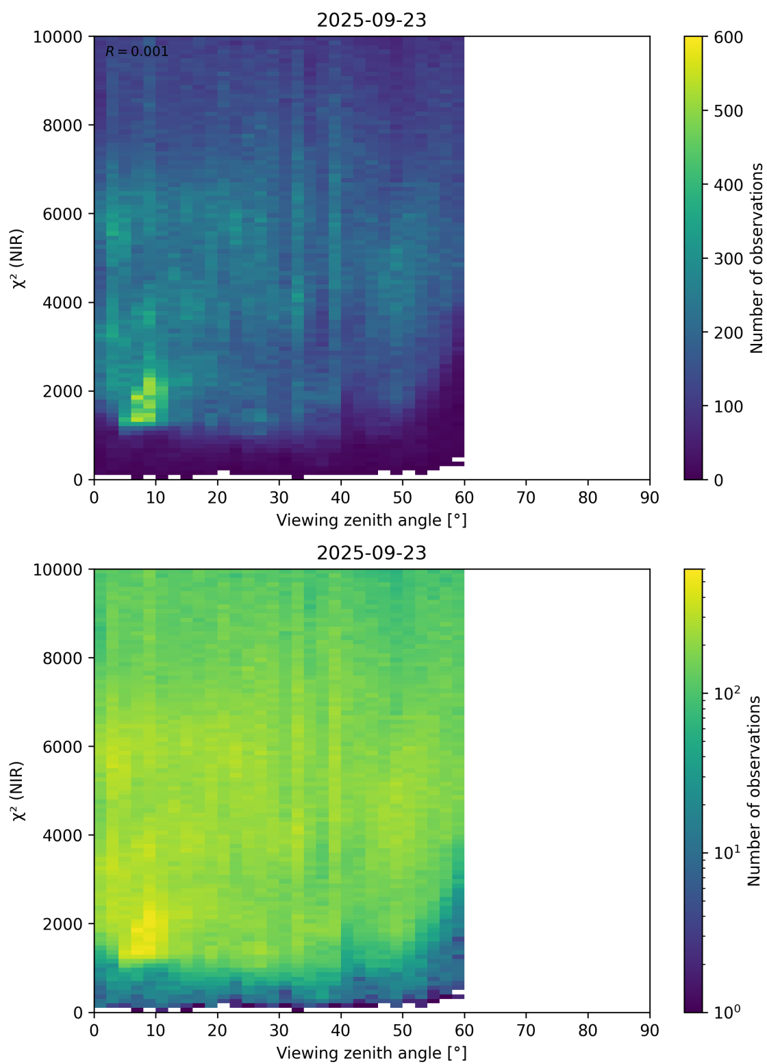
Figure 105: Scatter density plot of “Viewing zenith angle” against “ \chi^2 (NIR)” for 2025-09-22 to 2025-09-24.
