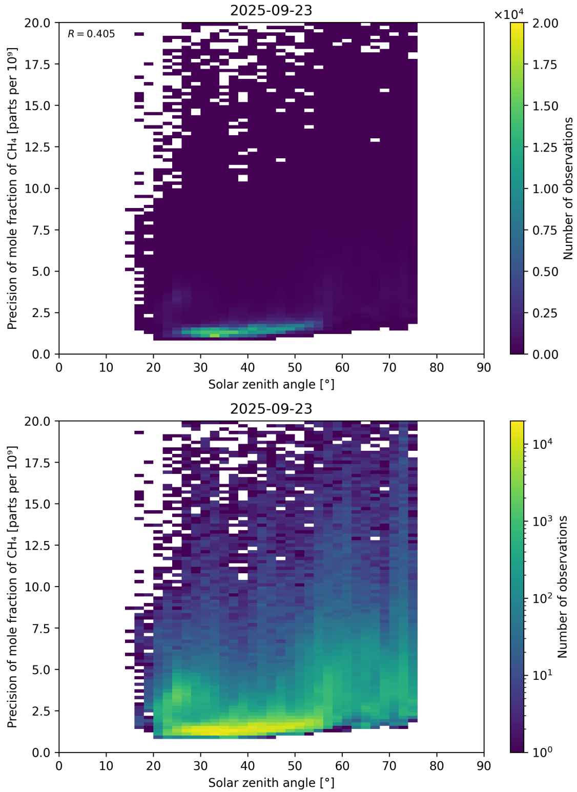
Figure 101: Scatter density plot of “Solar zenith angle” against “Precision of mole fraction of \text{CH}_4 ” for 2025-09-22 to 2025-09-24.
