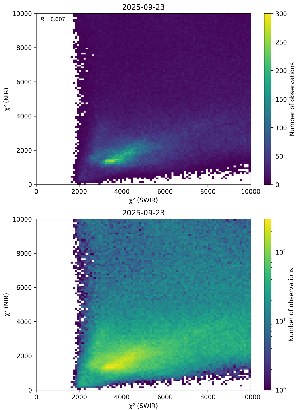
Figure 47: Scatter density plot of “ \chi^2 (SWIR)” against “ \chi^2 (NIR)” for 2025-09-22 to 2025-09-24.
