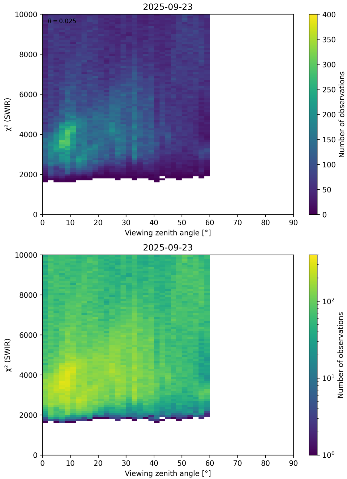
Figure 106: Scatter density plot of “Viewing zenith angle” against “ \chi^2 (SWIR)” for 2025-09-22 to 2025-09-24.
