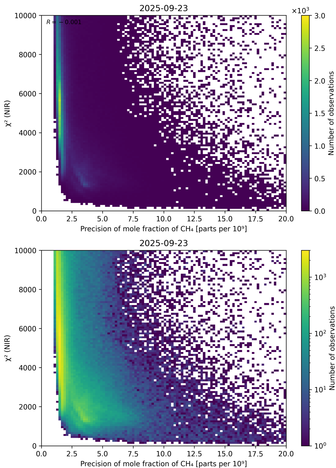
Figure 78: Scatter density plot of “Precision of mole fraction of CH 4 ” against “ \chi^2 (NIR)” for 2025-09-22 to 2025-09-24.
