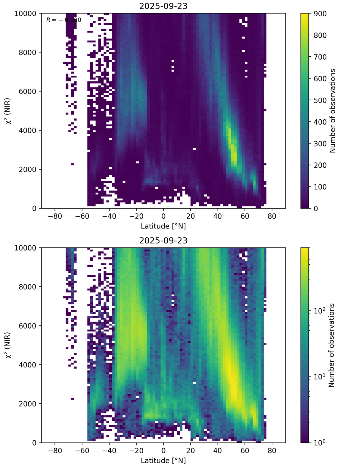
Figure 53: Scatter density plot of “Latitude” against “ \chi^2 (NIR)” for 2025-09-22 to 2025-09-24.
