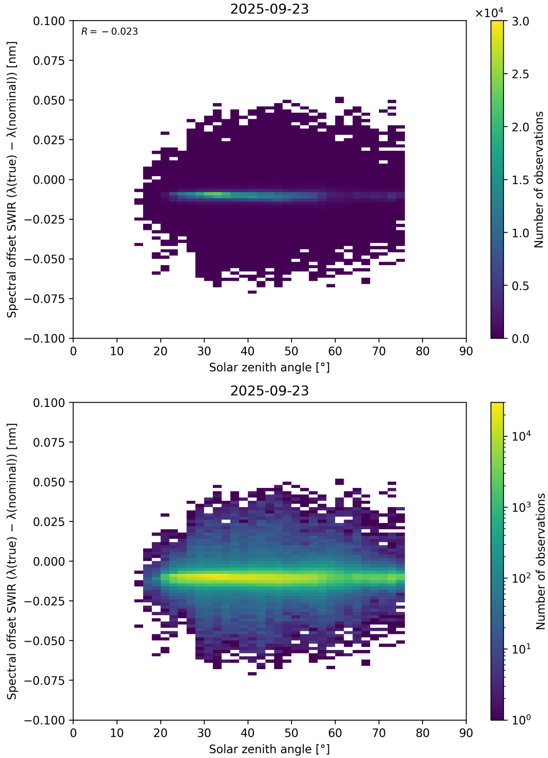
Figure 104: Scatter density plot of “Solar zenith angle” against “Spectral offset SWIR ( \lambda_{\text{true}} - \lambda_{\text{nominal}} )” for 2025-09-22 to 2025-09-24.
