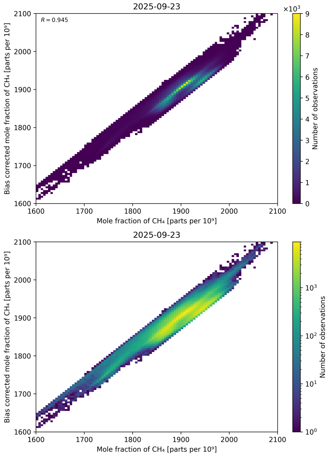
Figure 74: Scatter density plot of “Mole fraction of CH 4 ” against “Bias corrected mole fraction of CH 4 ” for 2025-09-22 to 2025-09-24.
