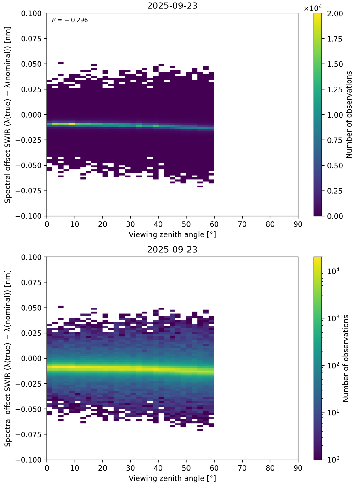
Figure 116: Scatter density plot of “Viewing zenith angle” against “Spectral offset SWIR ( \lambda_{\text{true}} - \lambda_{\text{nominal}} )” for 2025-09-22 to 2025-09-24.
