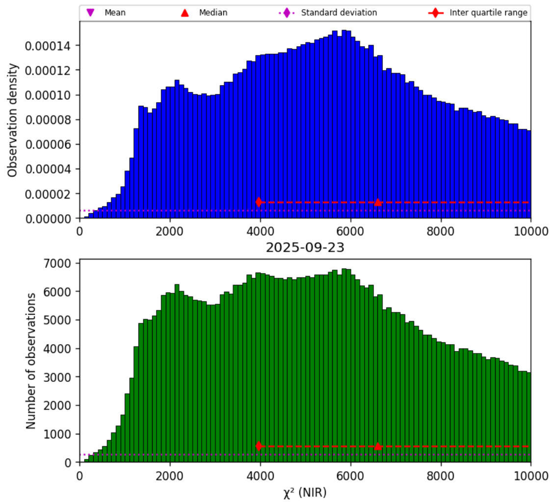
Figure 29: Histogram of “ \chi^2 (NIR)” for 2025-09-22 to 2025-09-24
