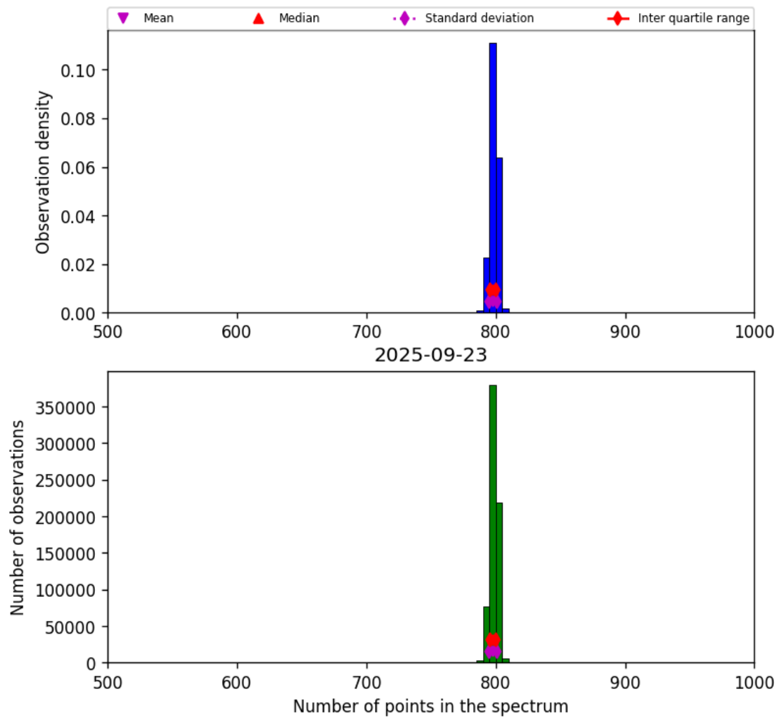
Figure 26: Histogram of “Number of points in the spectrum” for 2025-09-22 to 2025-09-24
