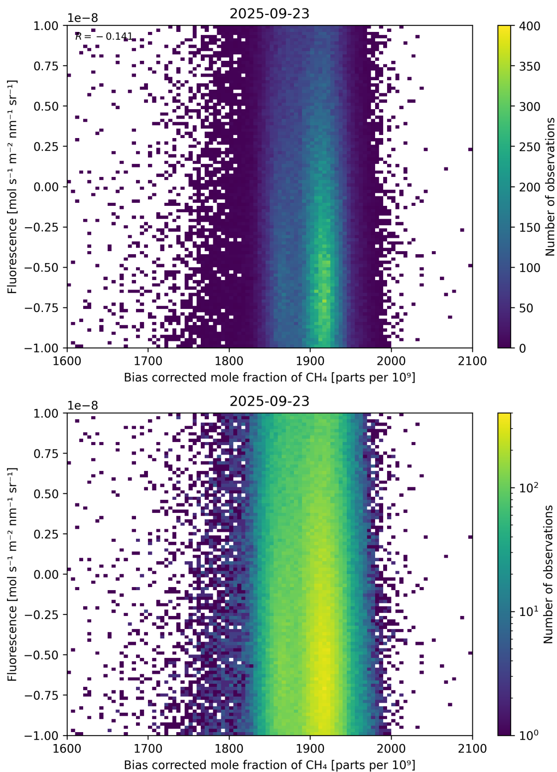
Figure 66: Scatter density plot of “Bias corrected mole fraction of \text{CH}_4 ” against “Fluorescence” for 2025-09-22 to 2025-09-24.
