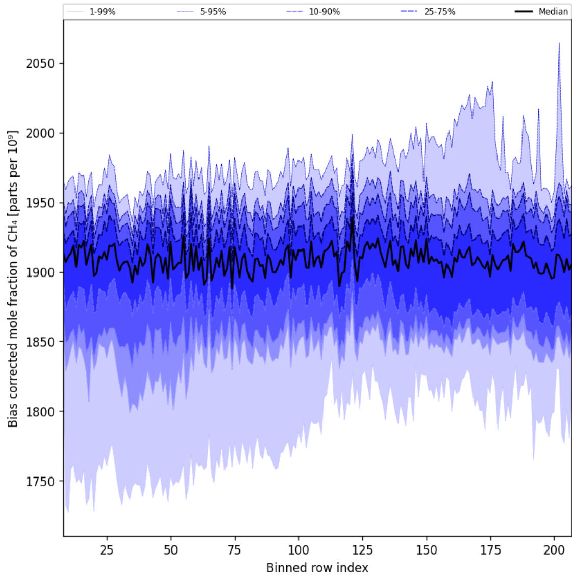
Figure 36: Along track statistics of “Bias corrected mole fraction of CH 4 ” for 2025-09-22 to 2025-09-24
