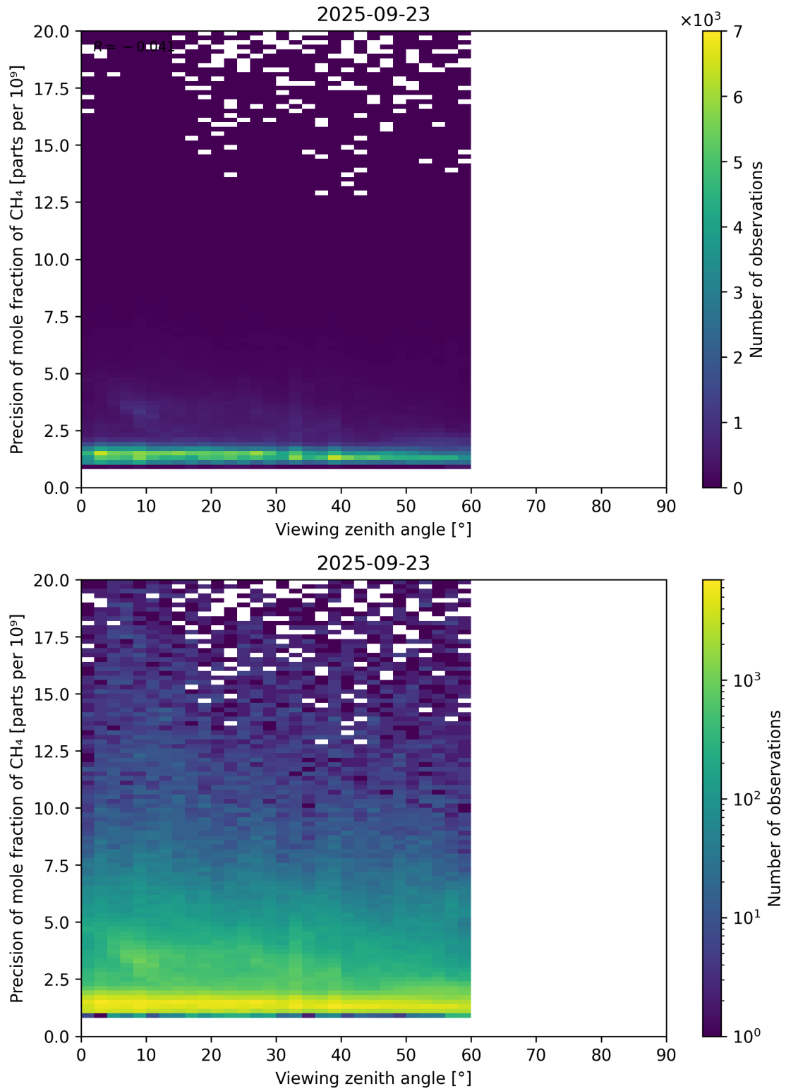
Figure 112: Scatter density plot of “Viewing zenith angle” against “Precision of mole fraction of CH 4 ” for 2025-09-22 to 2025-09-24.
