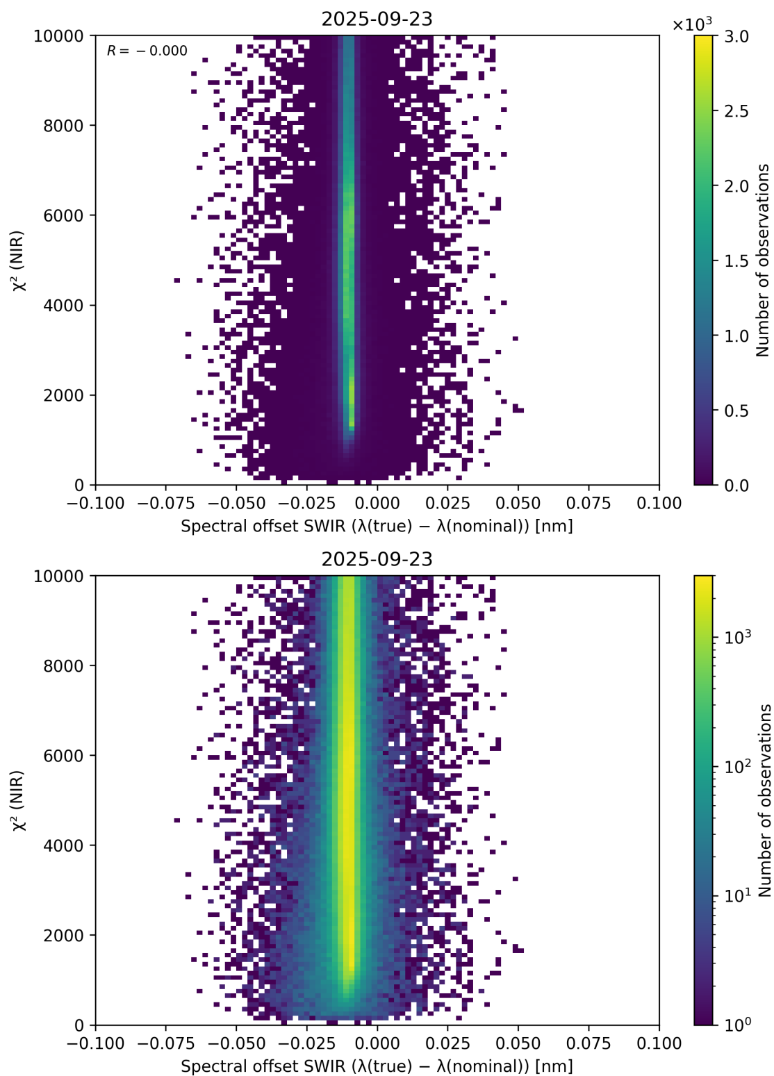
Figure 117: Scatter density plot of “Spectral offset SWIR ( \lambda_{\text{true}} - \lambda_{\text{nominal}} )” against “ \chi^2 (NIR)” for 2025-09-22 to 2025-09-24.
