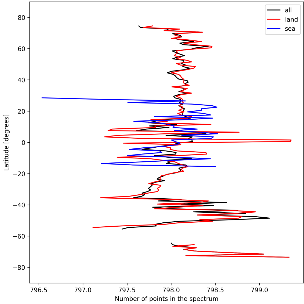
Figure 15: Zonal average of “Number of points in the spectrum” for 2025-09-22 to 2025-09-24.
