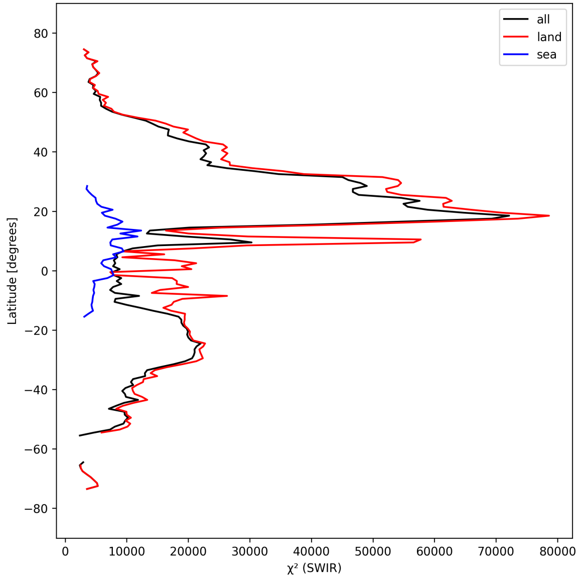
Figure 17: Zonal average of “ \chi^2 (SWIR)” for 2025-09-22 to 2025-09-24.
