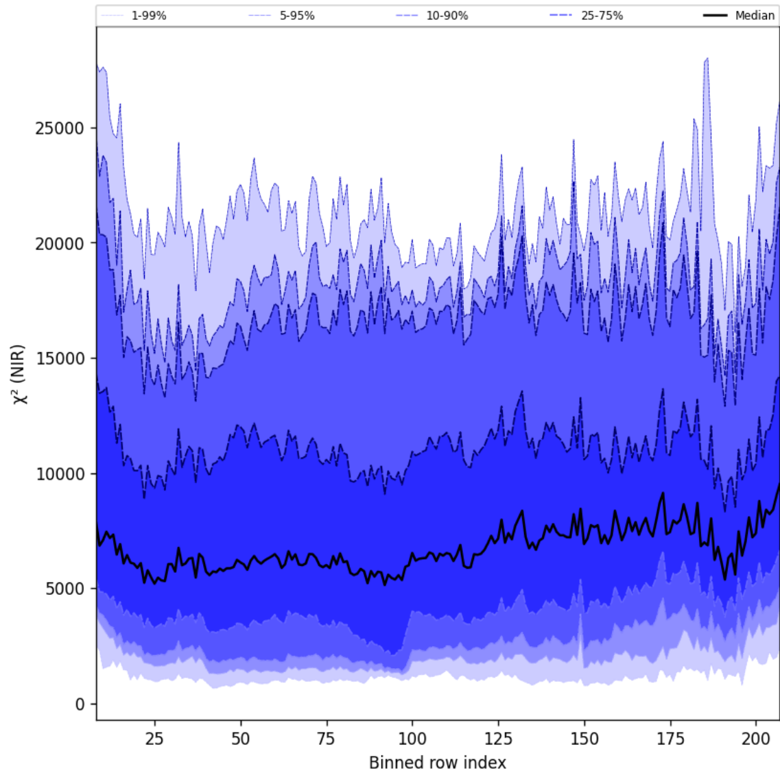
Figure 40: Along track statistics of “ \chi^2 (NIR)” for 2025-09-22 to 2025-09-24
