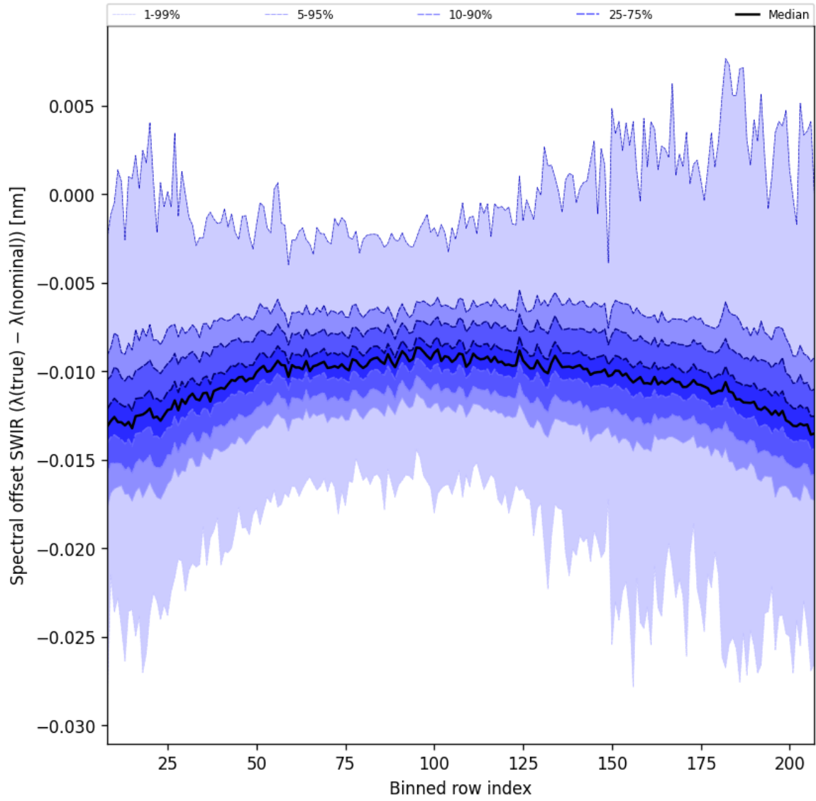
Figure 38: Along track statistics of “Spectral offset SWIR ( \lambda_{\text{true}} - \lambda_{\text{nominal}} )” for 2025-09-22 to 2025-09-24
