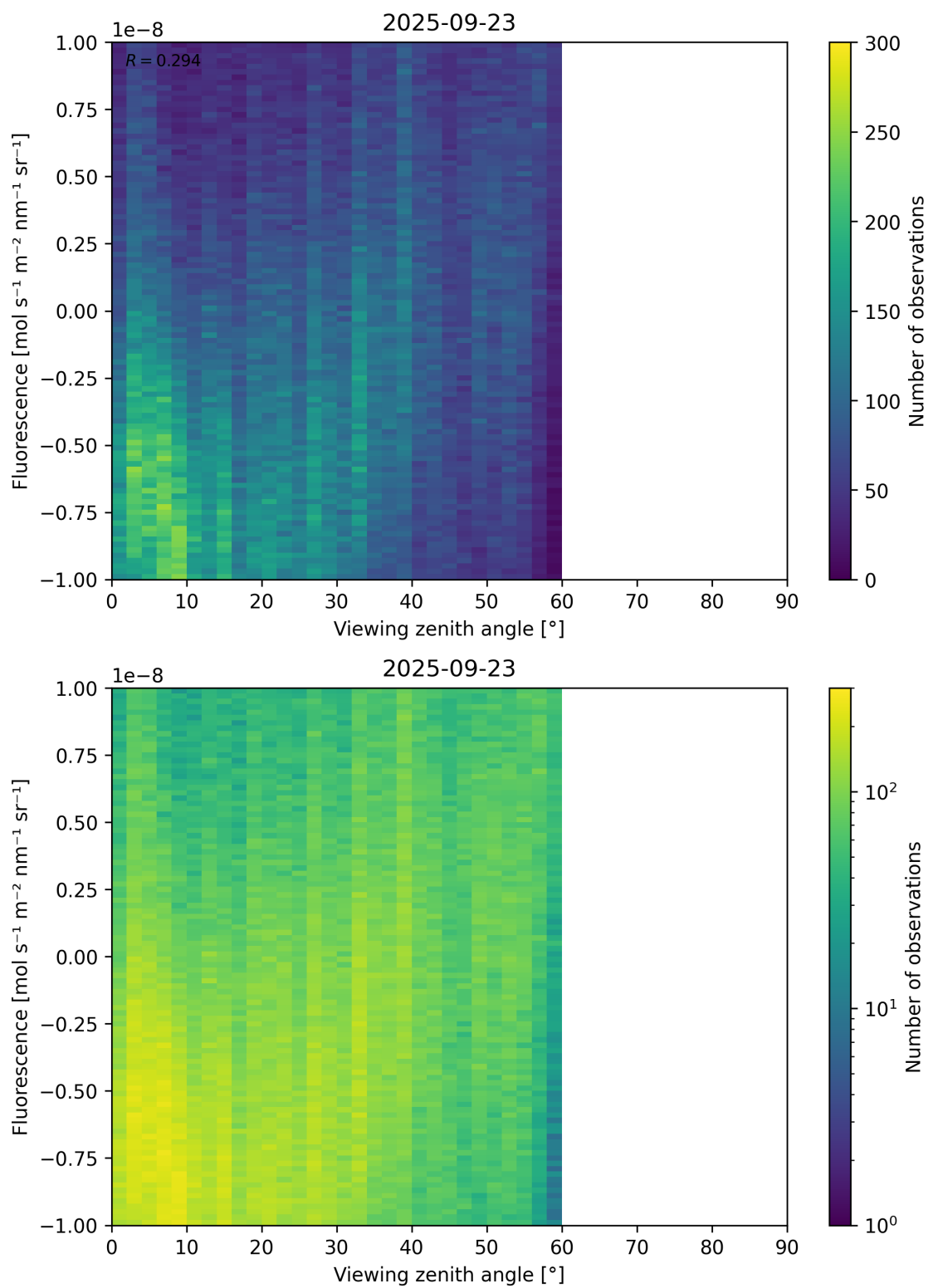
Figure 108: Scatter density plot of “Viewing zenith angle” against “Fluorescence” for 2025-09-22 to 2025-09-24.
