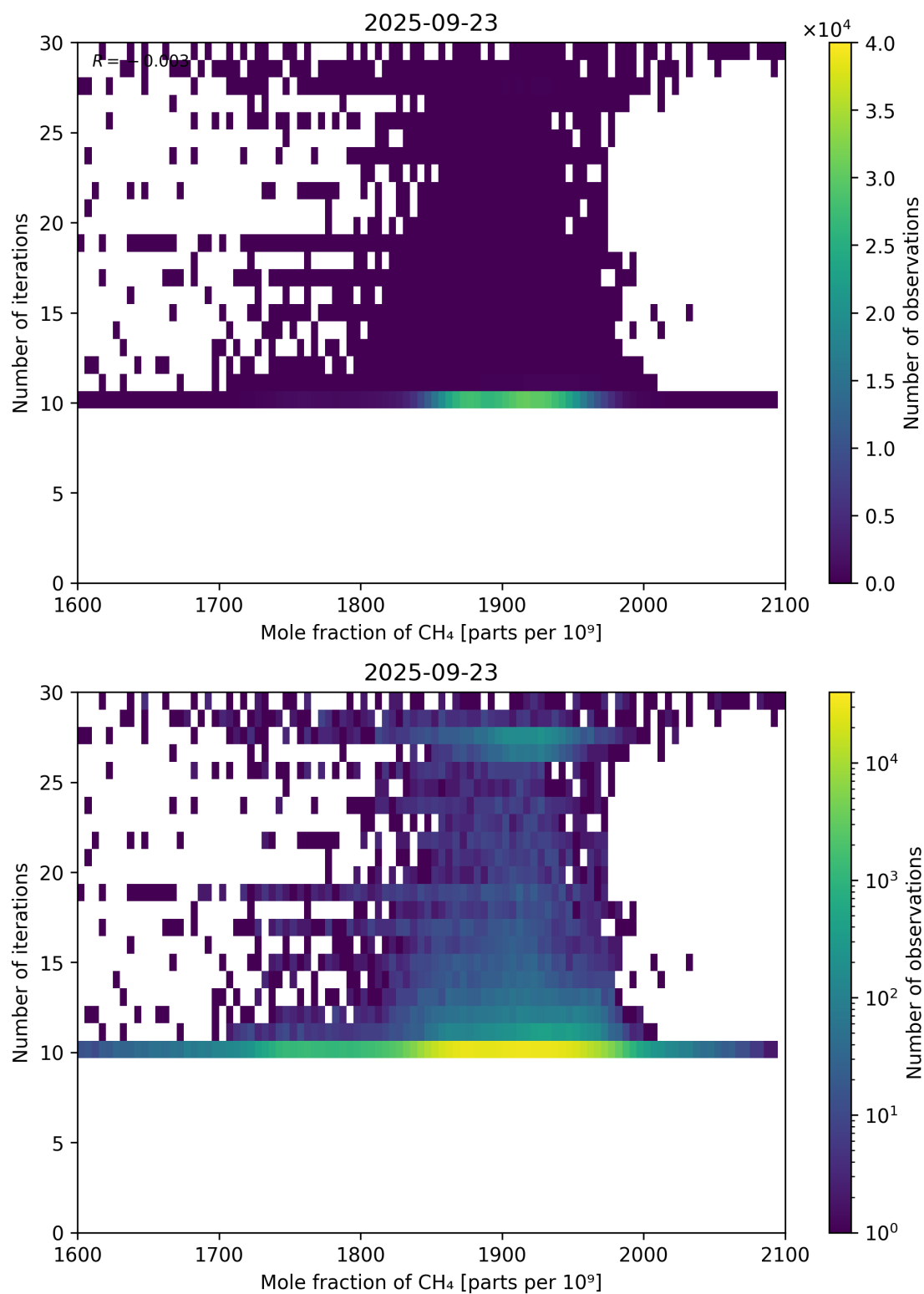
Figure 76: Scatter density plot of “Mole fraction of CH 4 ” against “Number of iterations” for 2025-09-22 to 2025-09-24.
