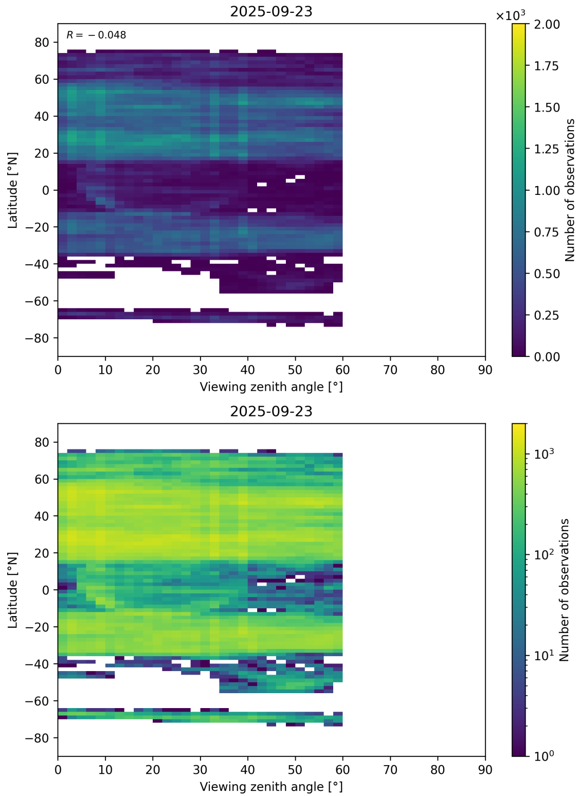
Figure 109: Scatter density plot of “Viewing zenith angle” against “Latitude” for 2025-09-22 to 2025-09-24.
