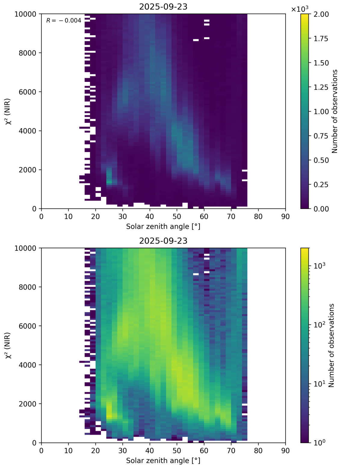
Figure 94: Scatter density plot of “Solar zenith angle” against “ \chi^2 (NIR)” for 2025-09-22 to 2025-09-24.
