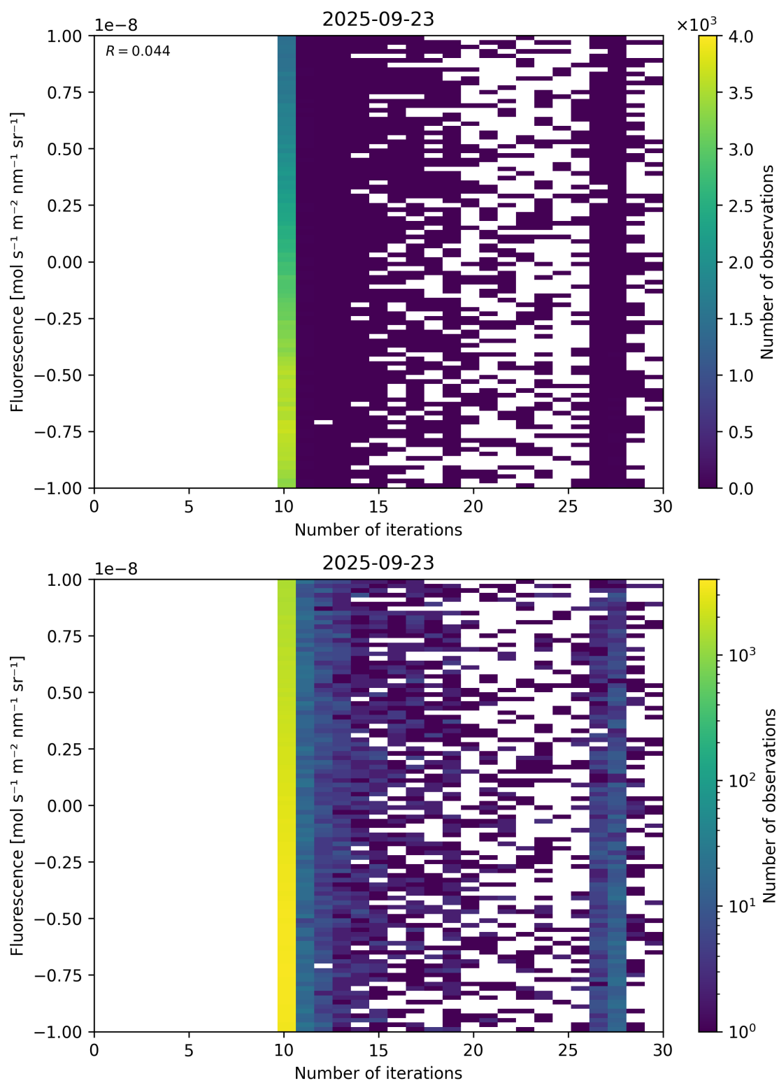
Figure 87: Scatter density plot of “Number of iterations” against “Fluorescence” for 2025-09-22 to 2025-09-24.
