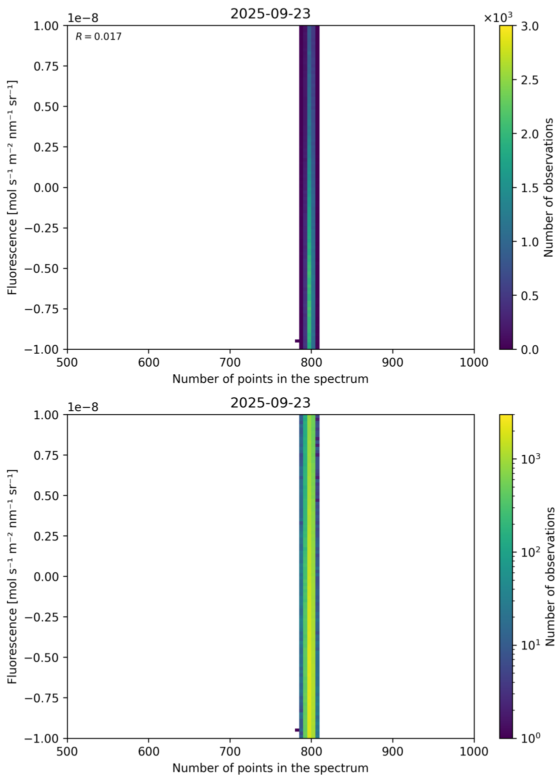
Figure 91: Scatter density plot of “Number of points in the spectrum” against “Fluorescence” for 2025-09-22 to 2025-09-24.
