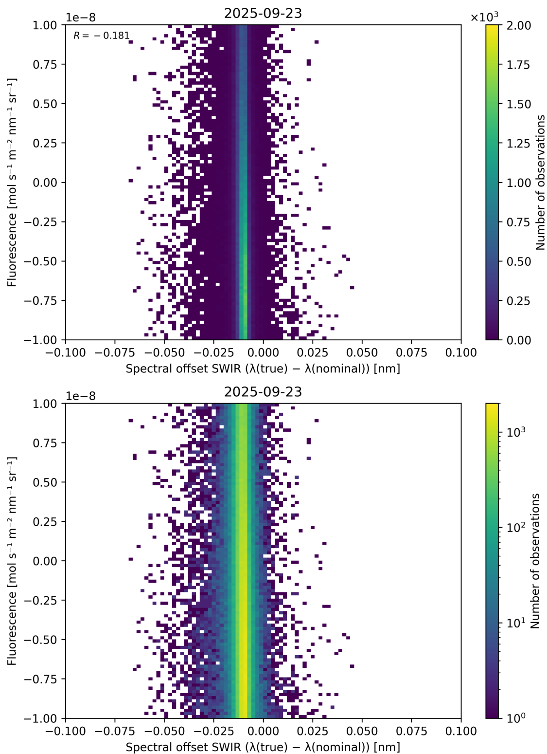
Figure 120: Scatter density plot of “Spectral offset SWIR ( \lambda_{\text{true}} - \lambda_{\text{nominal}} )” against “Fluorescence” for 2025-09-22 to 2025-09-24.
