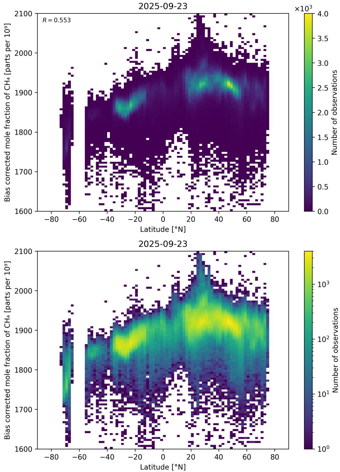
Figure 58: Scatter density plot of “Latitude” against “Bias corrected mole fraction of \text{CH}_4 ” for 2025-09-22 to 2025-09-24.
