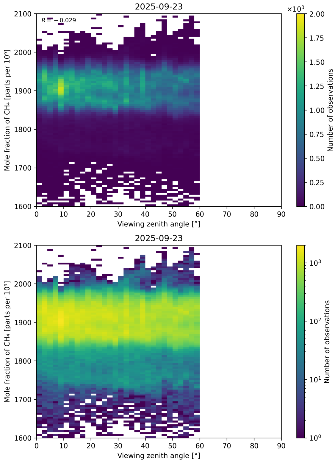
Figure 110: Scatter density plot of “Viewing zenith angle” against “Mole fraction of CH 4 ” for 2025-09-22 to 2025-09-24.
