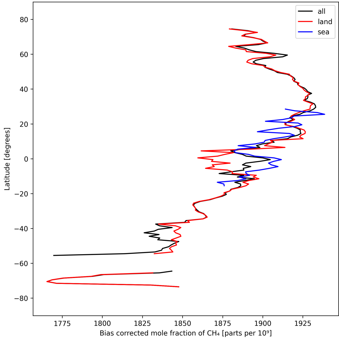
Figure 14: Zonal average of “Bias corrected mole fraction of CH 4 ” for 2025-09-22 to 2025-09-24.
