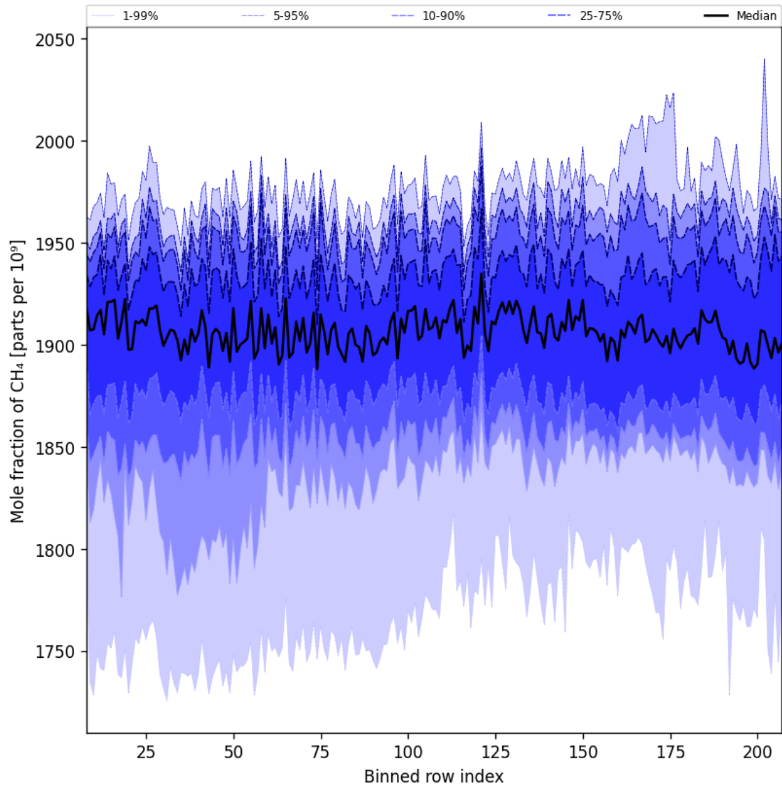
Figure 34: Along track statistics of “Mole fraction of CH 4 ” for 2025-09-22 to 2025-09-24
