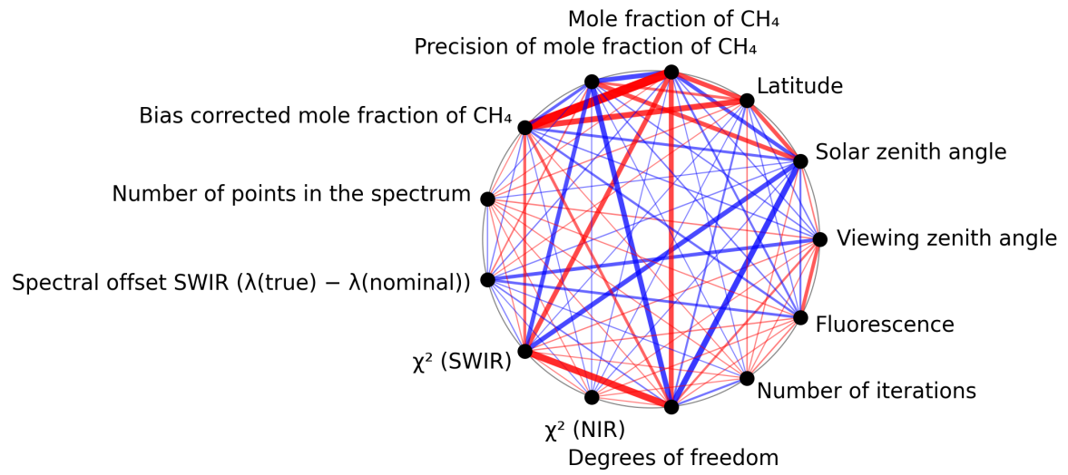
Figure 1: Map of correlation graph for 2025-09-22 to 2025-09-24.
