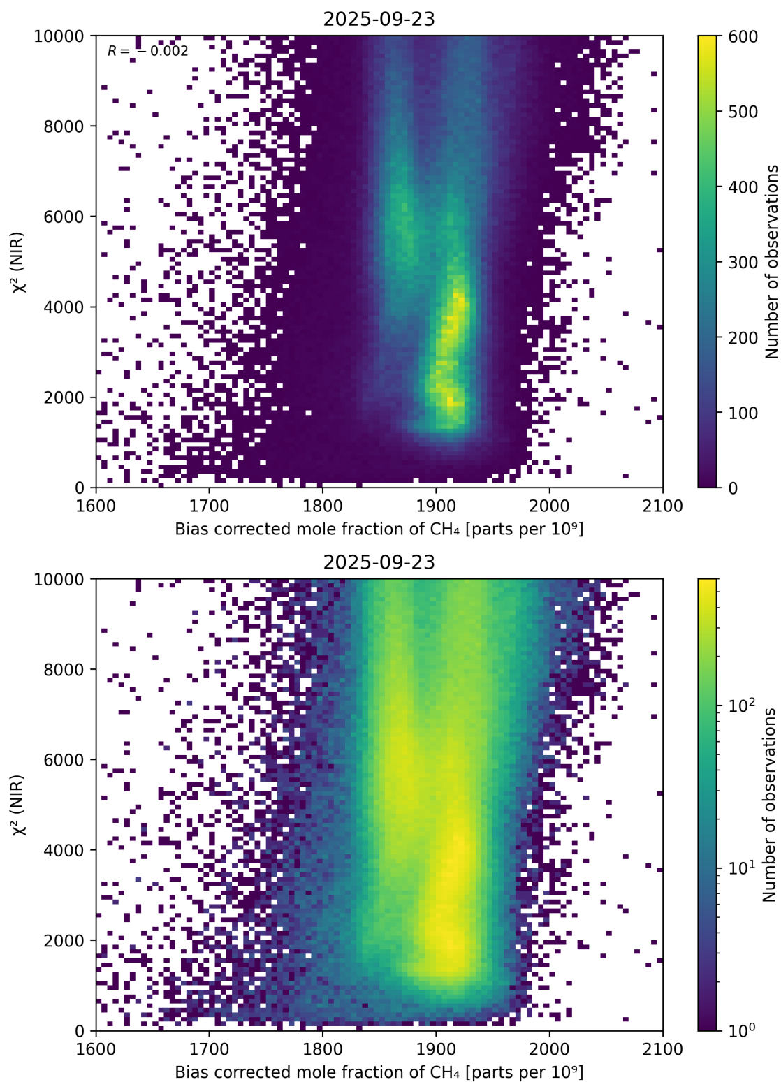
Figure 63: Scatter density plot of “Bias corrected mole fraction of CH 4 ” against “ \chi^2 (NIR)” for 2025-09-22 to 2025-09-24.
