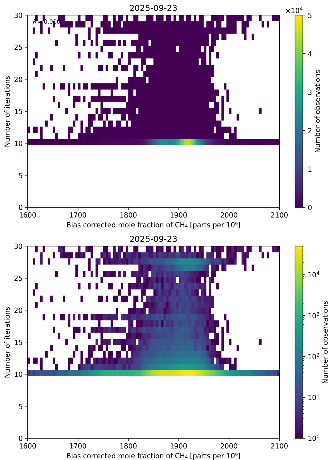
Figure 67: Scatter density plot of “Bias corrected mole fraction of CH 4 ” against “Number of iterations” for 2025-09-22 to 2025-09-24.
