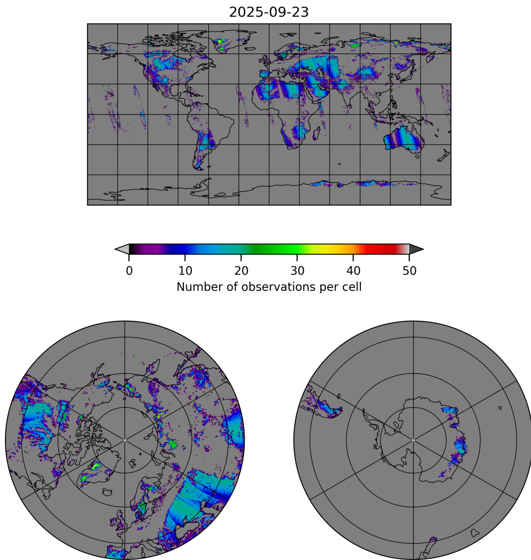
Figure 10: Map of the number of observations for 2025-09-22 to 2025-09-24
