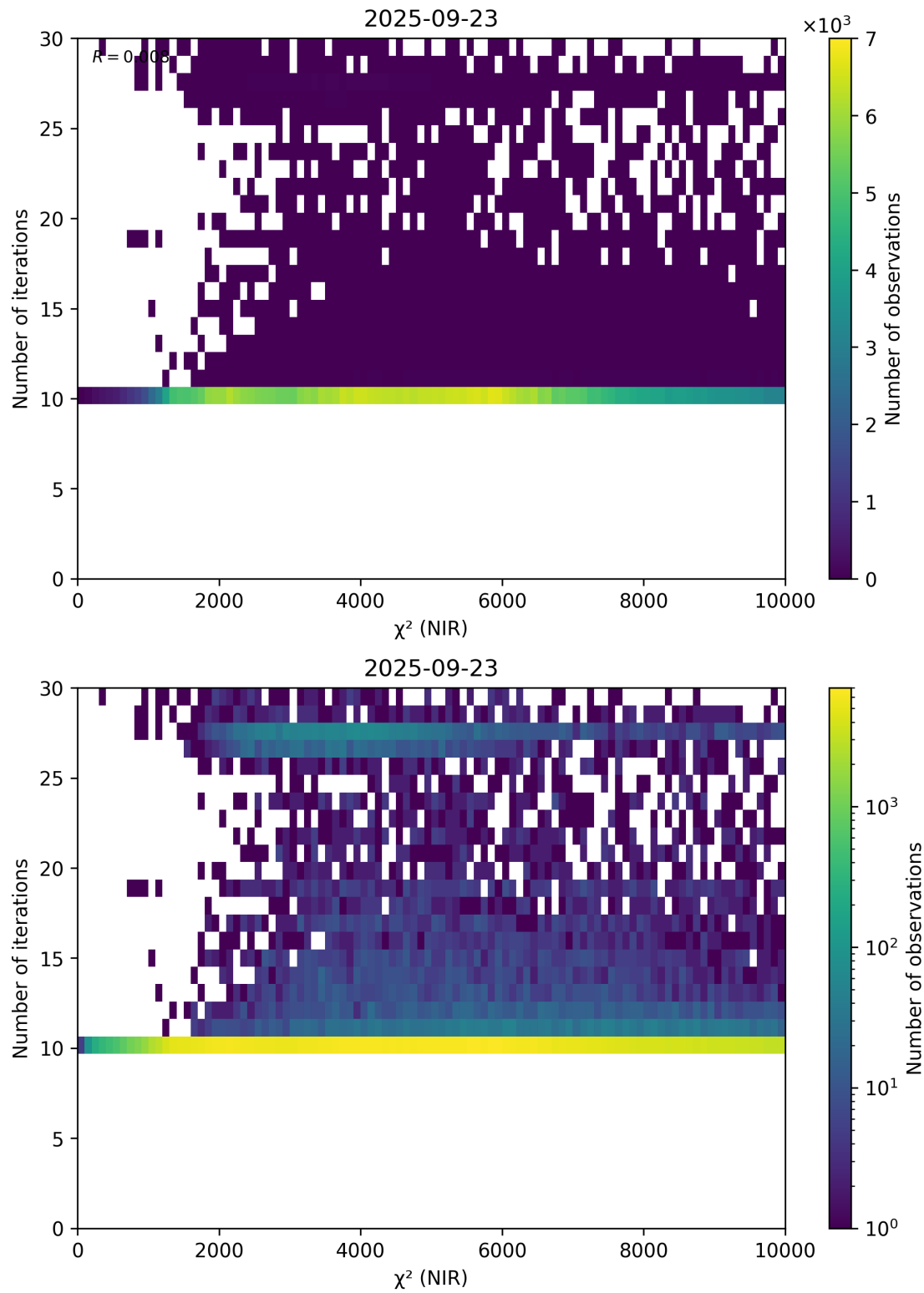
Figure 46: Scatter density plot of “ \chi^2 (NIR)” against “Number of iterations” for 2025-09-22 to 2025-09-24.
