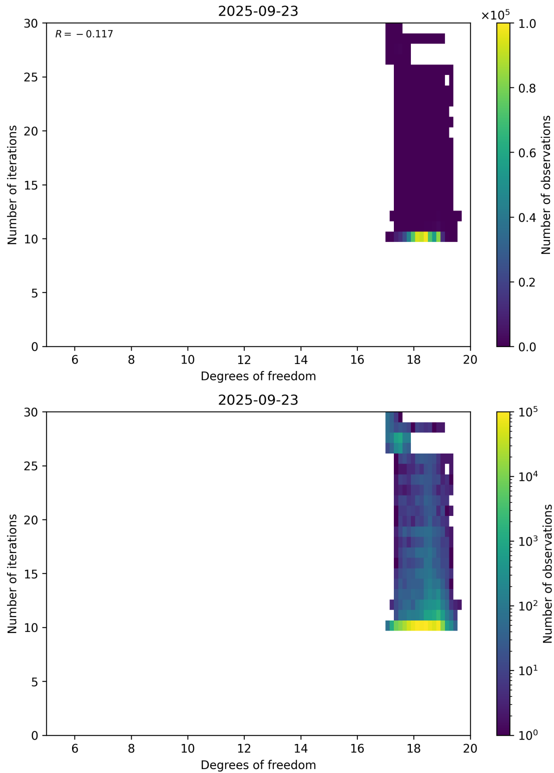
Figure 52: Scatter density plot of “Degrees of freedom” against “Number of iterations” for 2025-09-22 to 2025-09-24.
