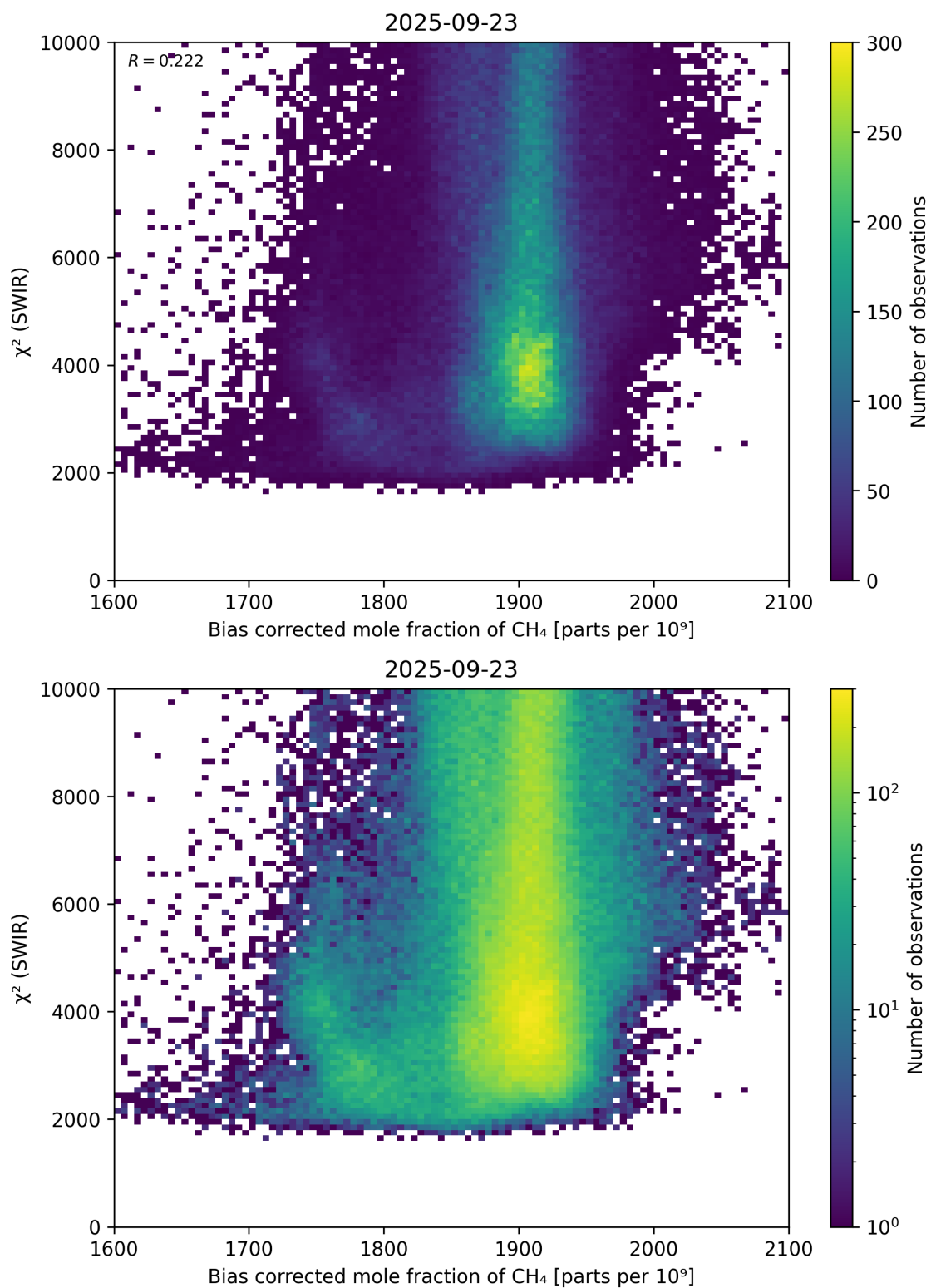
Figure 64: Scatter density plot of “Bias corrected mole fraction of \text{CH}_4 ” against “ \chi^2 (SWIR)” for 2025-09-22 to 2025-09-24.
