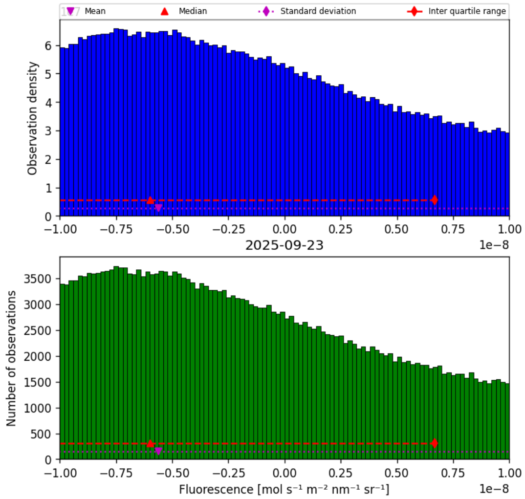
Figure 32: Histogram of “Fluorescence” for 2025-09-22 to 2025-09-24
