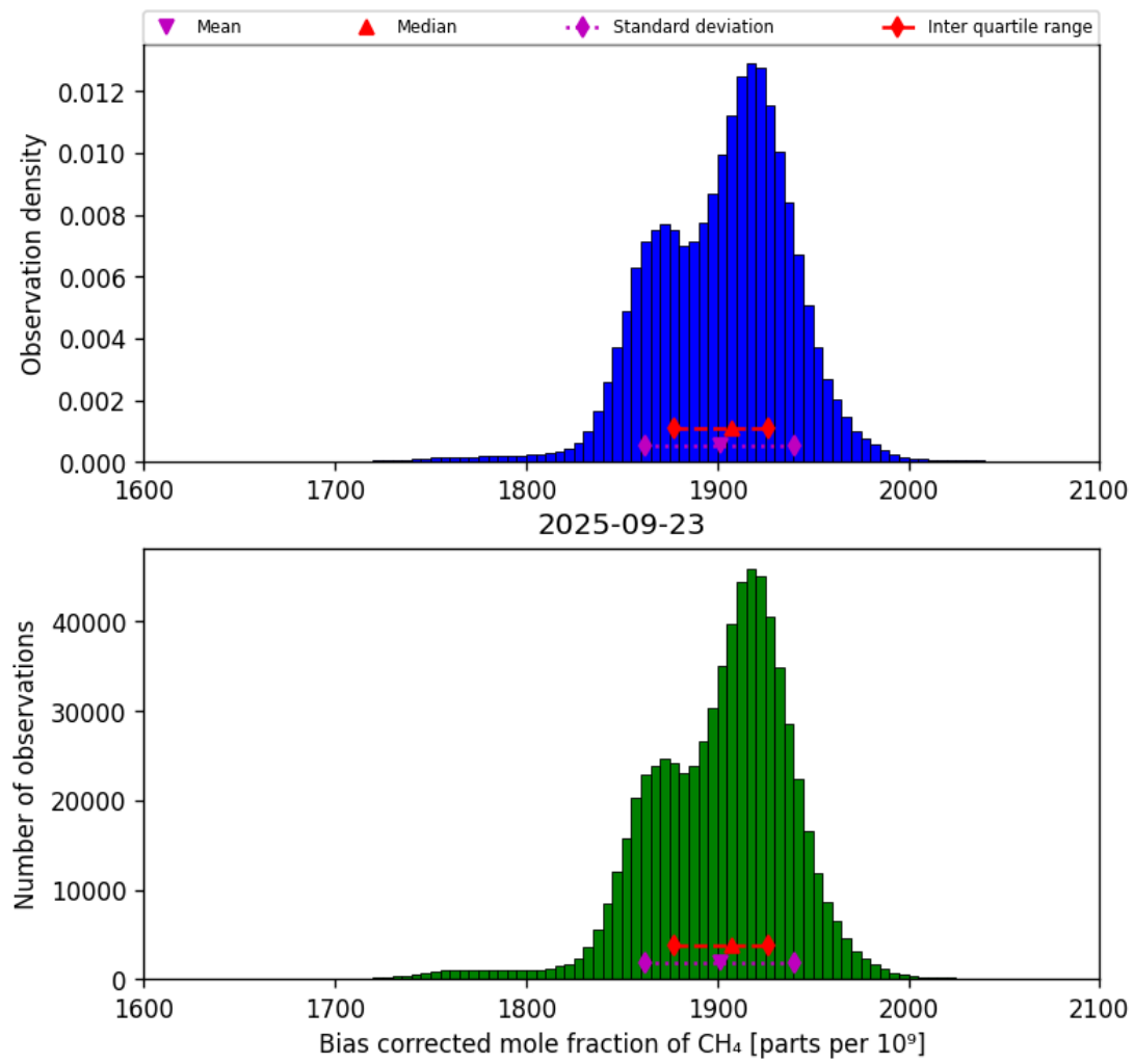
Figure 25: Histogram of “Bias corrected mole fraction of CH 4 ” for 2025-09-22 to 2025-09-24
