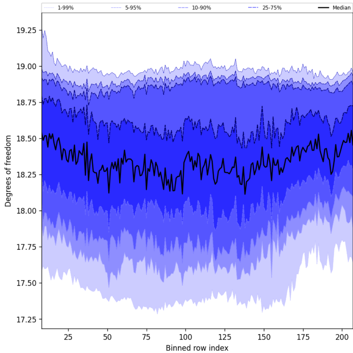
Figure 41: Along track statistics of “Degrees of freedom” for 2025-09-22 to 2025-09-24
