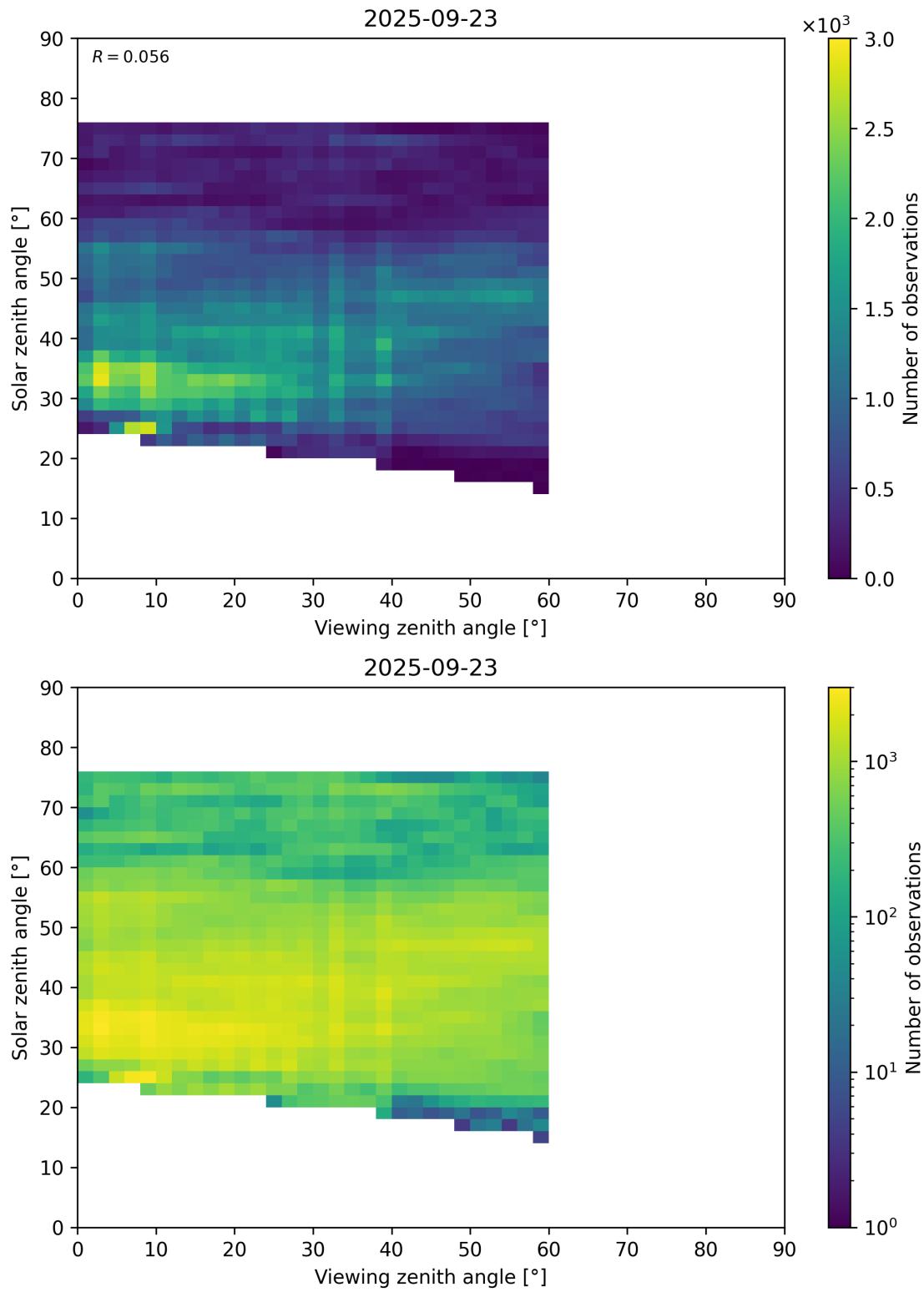
Figure 115: Scatter density plot of “Viewing zenith angle” against “Solar zenith angle” for 2025-09-22 to 2025-09-24.
