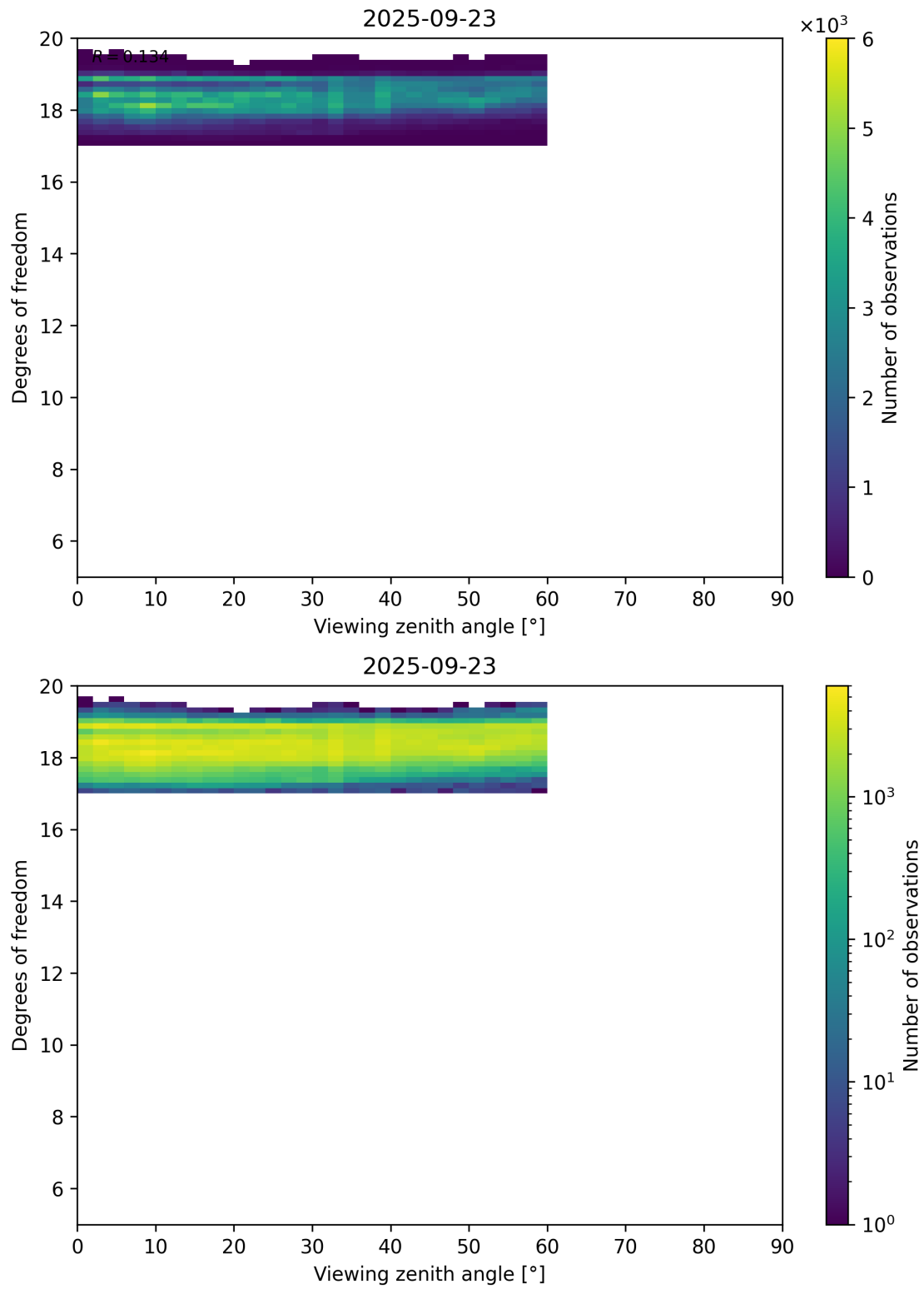
Figure 107: Scatter density plot of “Viewing zenith angle” against “Degrees of freedom” for 2025-09-22 to 2025-09-24.
