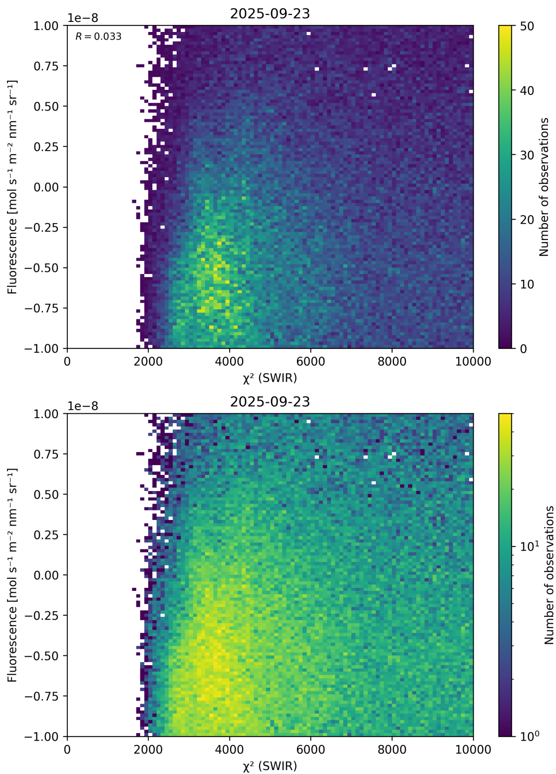
Figure 49: Scatter density plot of “ \chi^2 (SWIR)” against “Fluorescence” for 2025-09-22 to 2025-09-24.
