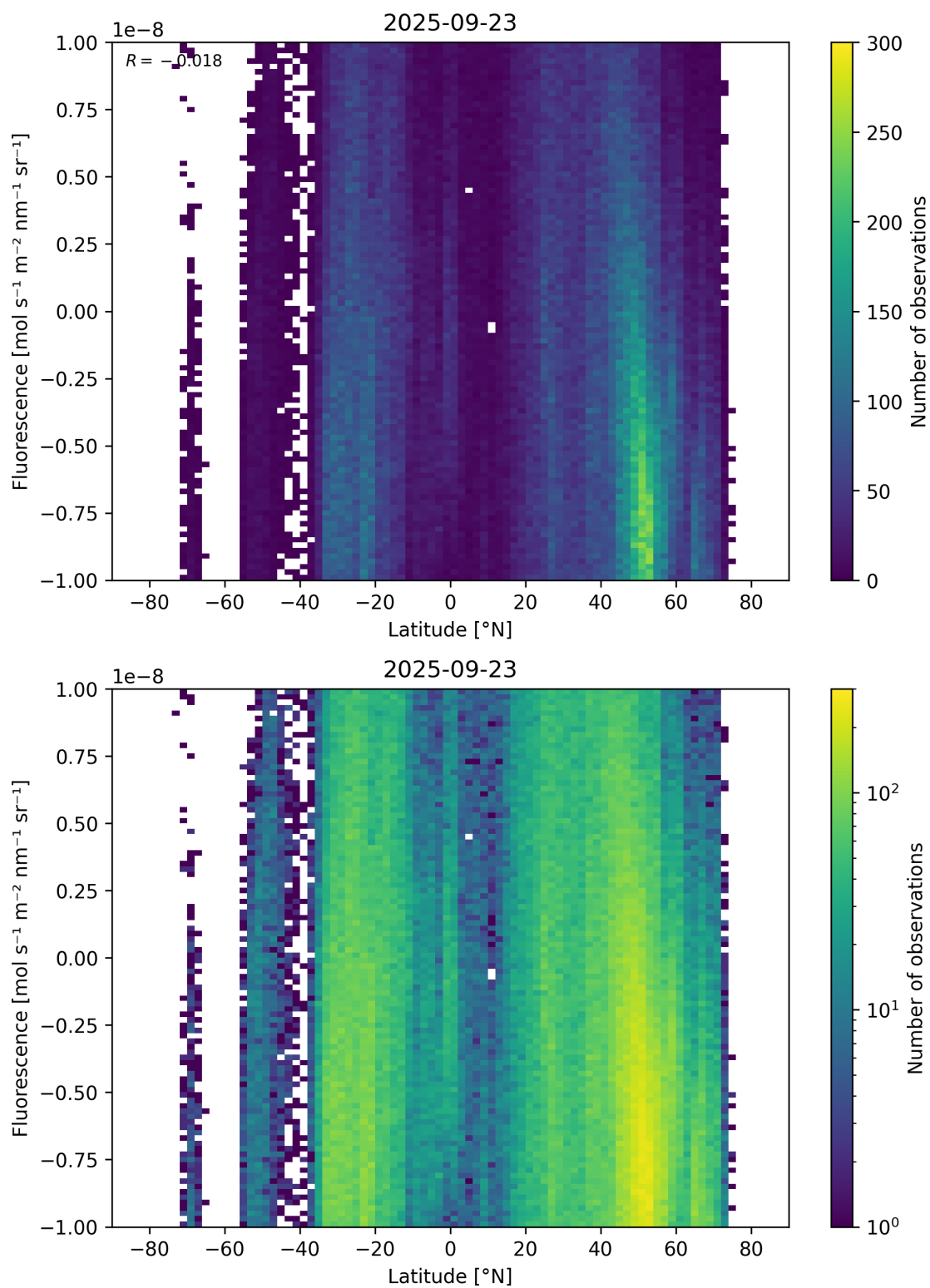
Figure 56: Scatter density plot of “Latitude” against “Fluorescence” for 2025-09-22 to 2025-09-24.
