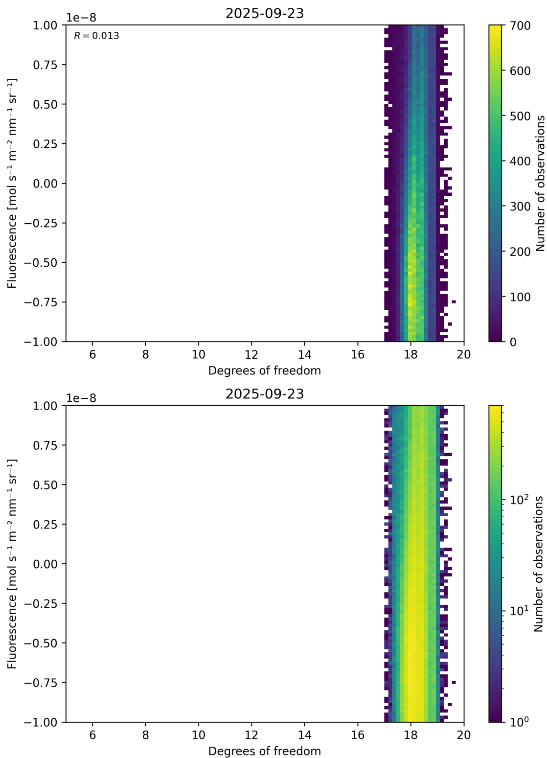
Figure 51: Scatter density plot of “Degrees of freedom” against “Fluorescence” for 2025-09-22 to 2025-09-24.
