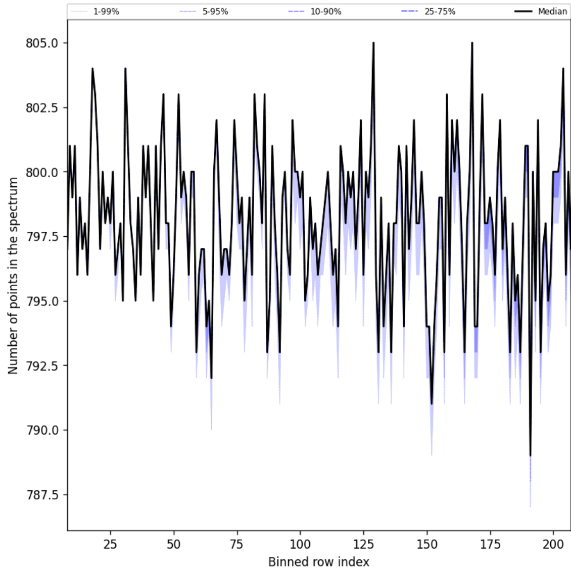
Figure 37: Along track statistics of “Number of points in the spectrum” for 2025-09-22 to 2025-09-24
