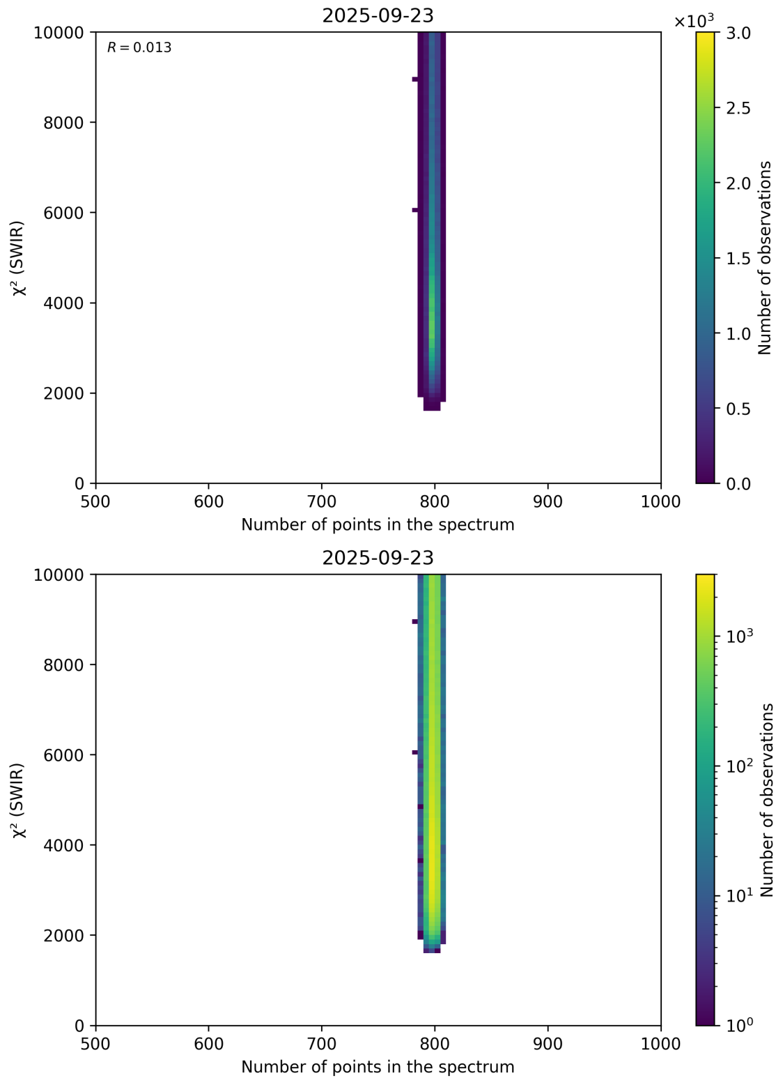
Figure 89: Scatter density plot of “Number of points in the spectrum” against “ \chi^2 (SWIR)” for 2025-09-22 to 2025-09-24.
