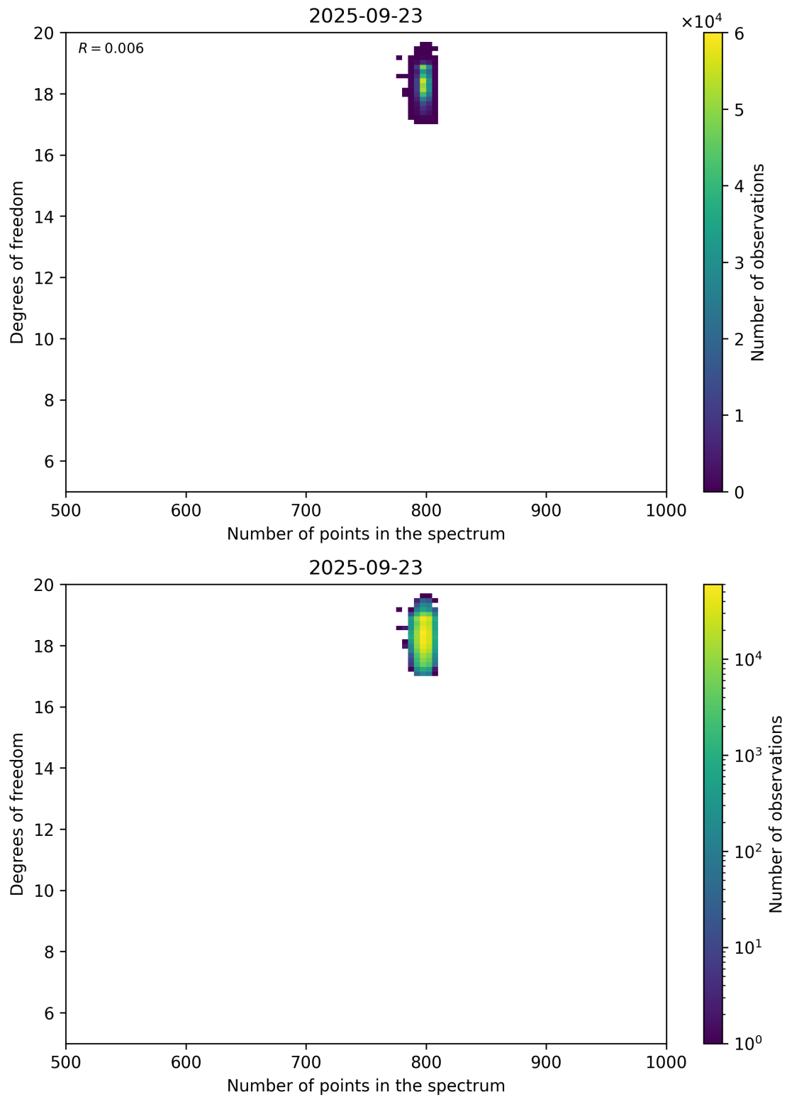
Figure 90: Scatter density plot of “Number of points in the spectrum” against “Degrees of freedom” for 2025-09-22 to 2025-09-24.
