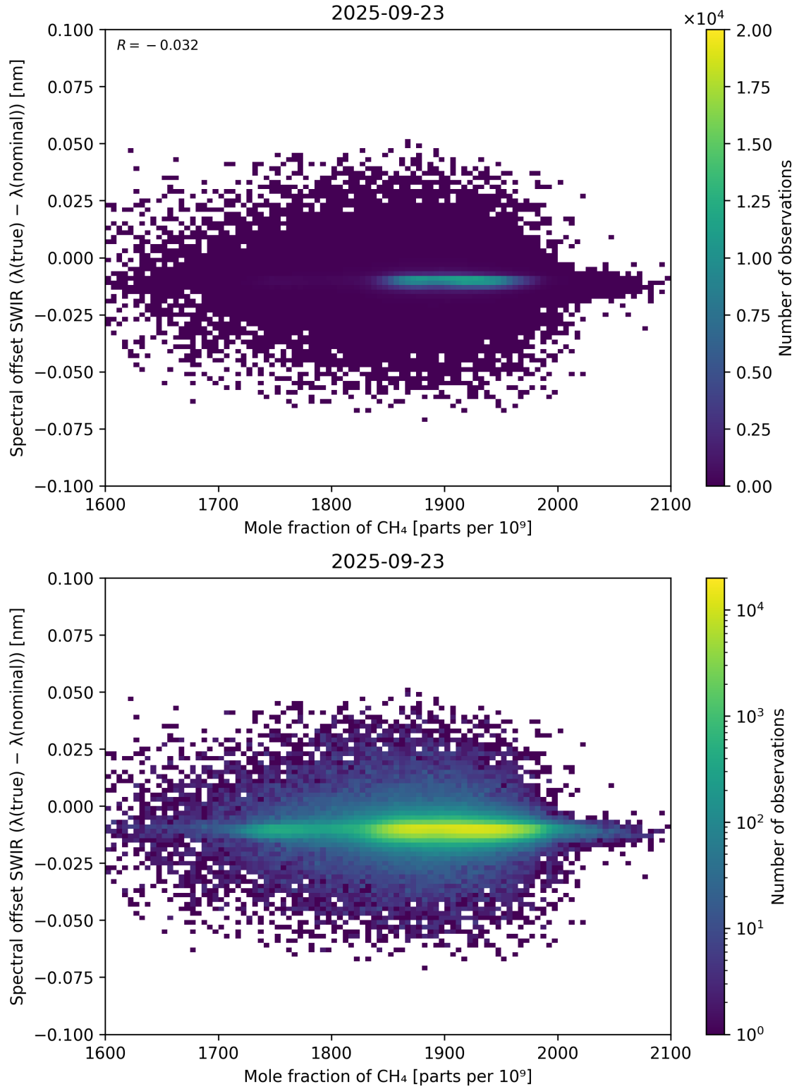
Figure 86: Scatter density plot of “Mole fraction of CH 4 ” against “Spectral offset SWIR ( \lambda_{\text{true}} - \lambda_{\text{nominal}} )” for 2025-09-22 to 2025-09-24.
