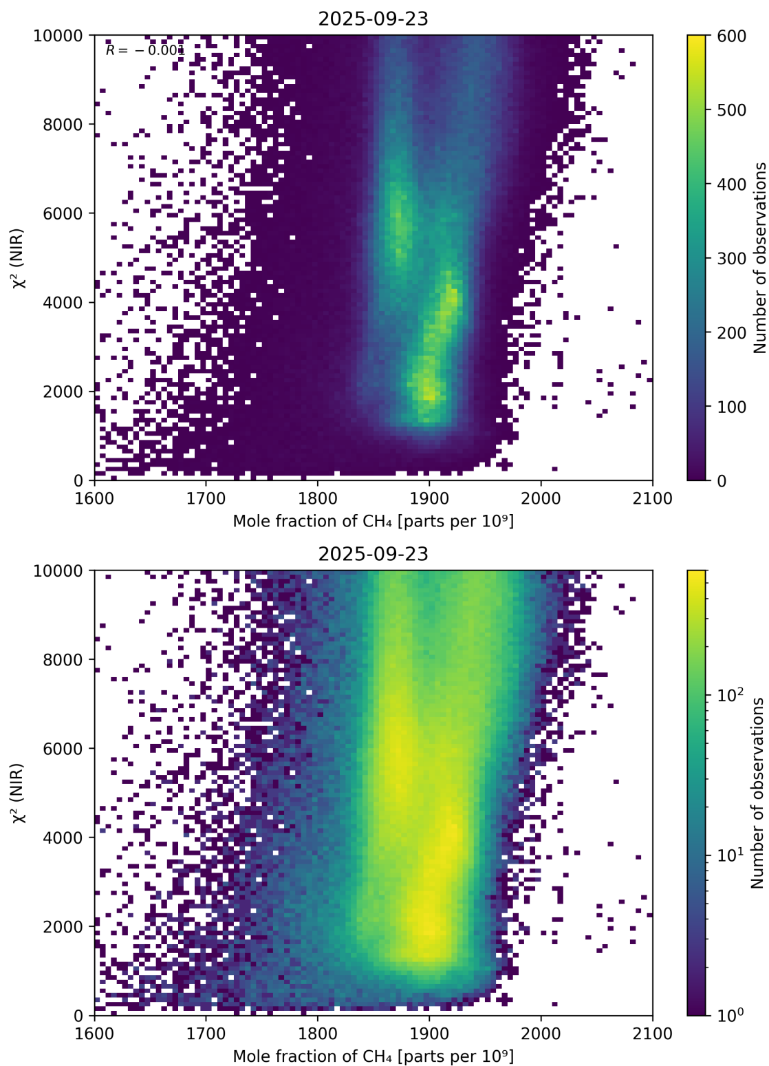
Figure 70: Scatter density plot of “Mole fraction of \text{CH}_4 ” against “ \chi^2 (NIR)” for 2025-09-22 to 2025-09-24.
