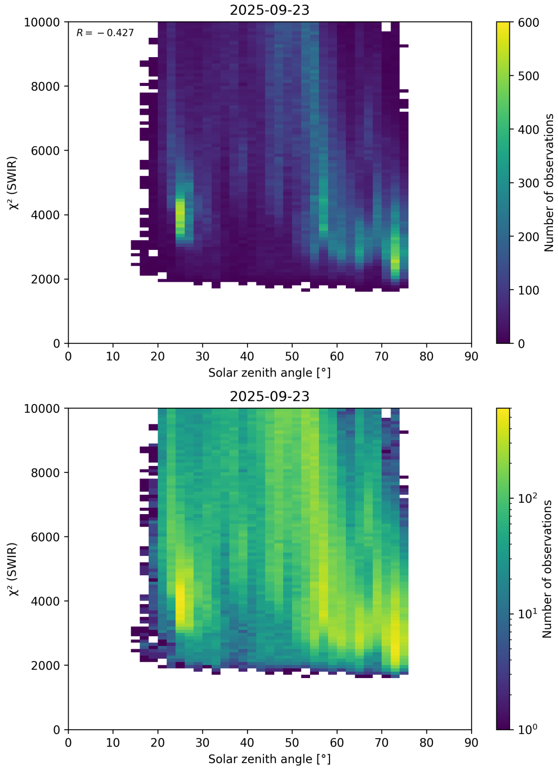
Figure 95: Scatter density plot of “Solar zenith angle” against “ \chi^2 (SWIR)” for 2025-09-22 to 2025-09-24.
