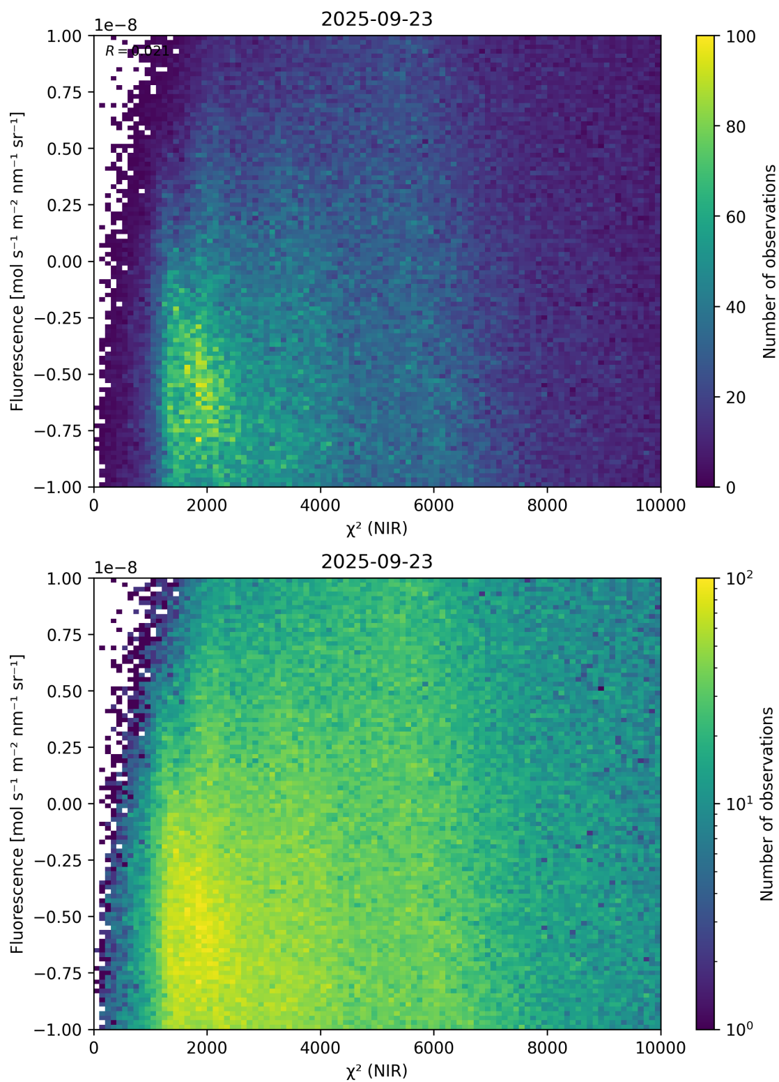
Figure 45: Scatter density plot of “ \chi^2 (NIR)” against “Fluorescence” for 2025-09-22 to 2025-09-24.
