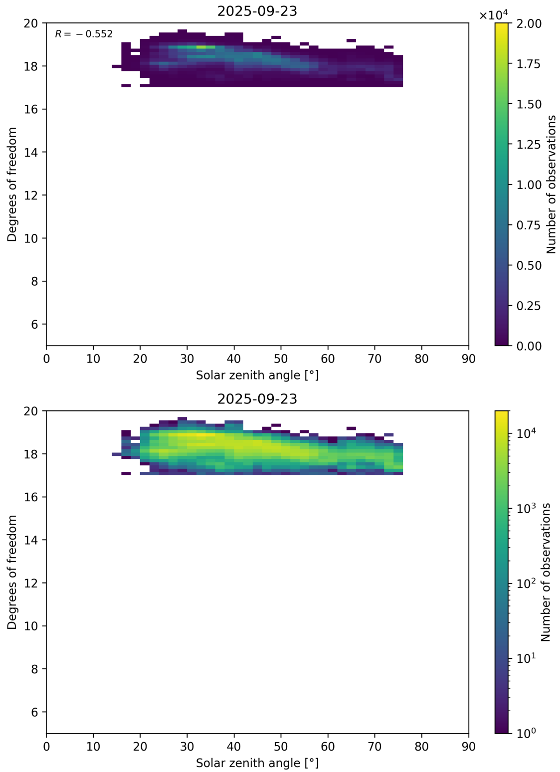
Figure 96: Scatter density plot of “Solar zenith angle” against “Degrees of freedom” for 2025-09-22 to 2025-09-24.
