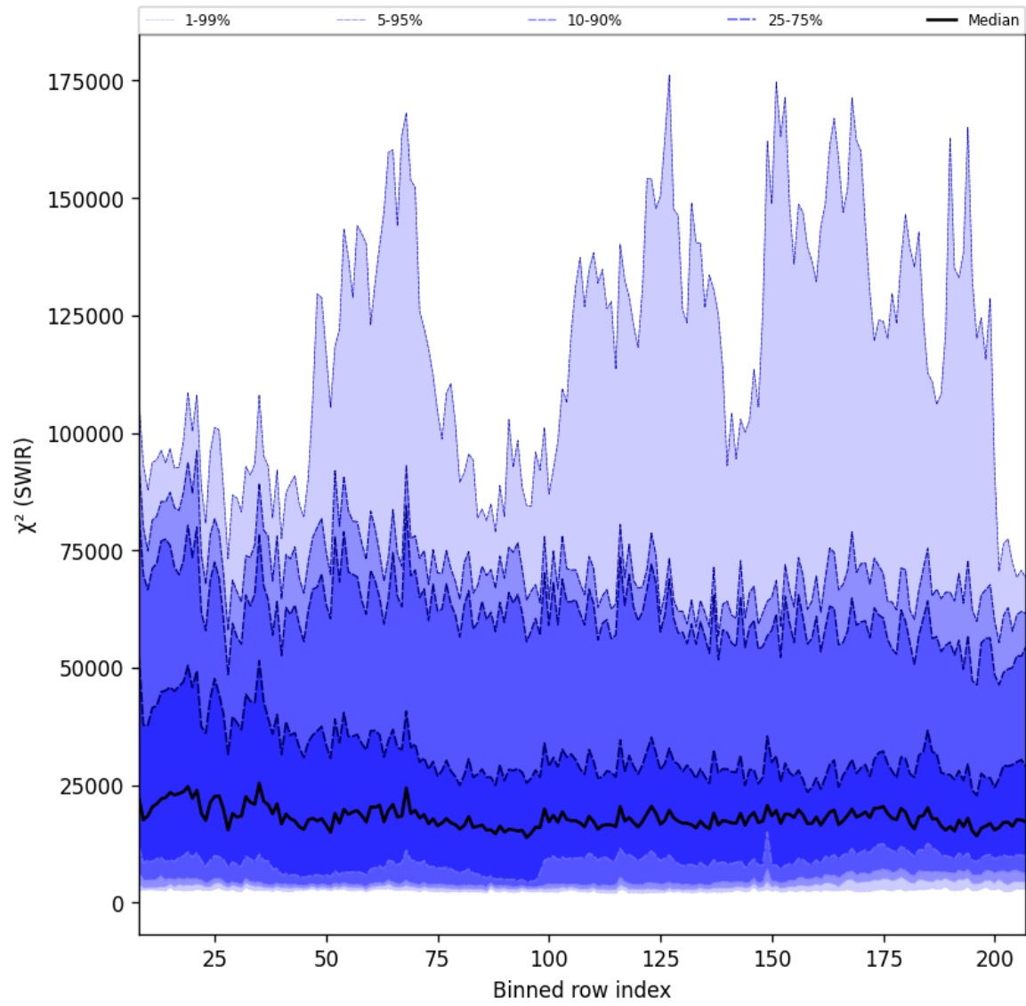
Figure 39: Along track statistics of “ \chi^2 (SWIR)” for 2025-09-22 to 2025-09-24
