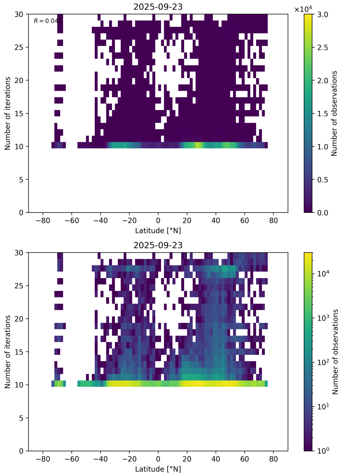
Figure 60: Scatter density plot of “Latitude” against “Number of iterations” for 2025-09-22 to 2025-09-24.
