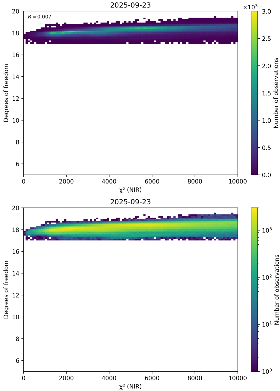
Figure 44: Scatter density plot of “ \chi^2 (NIR)” against “Degrees of freedom” for 2025-09-22 to 2025-09-24.
