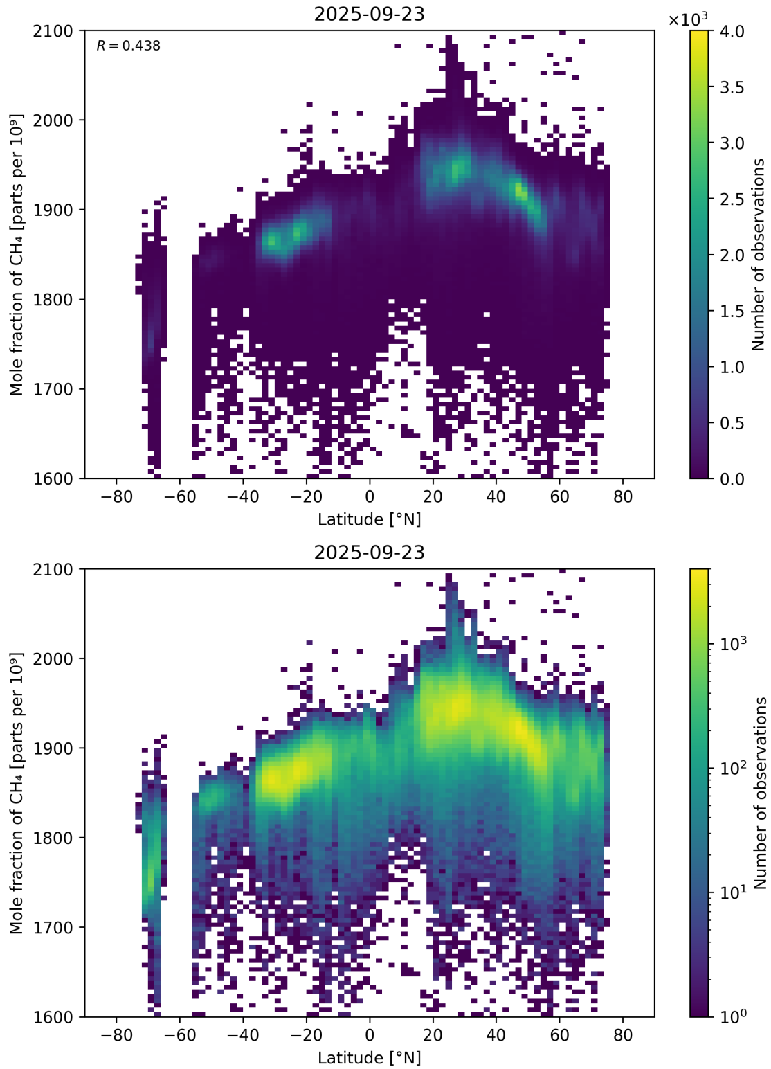
Figure 57: Scatter density plot of “Latitude” against “Mole fraction of CH 4 ” for 2025-09-22 to 2025-09-24.
