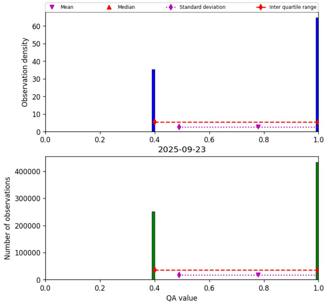
Figure 22: Histogram of “QA value” for 2025-09-22 to 2025-09-24
