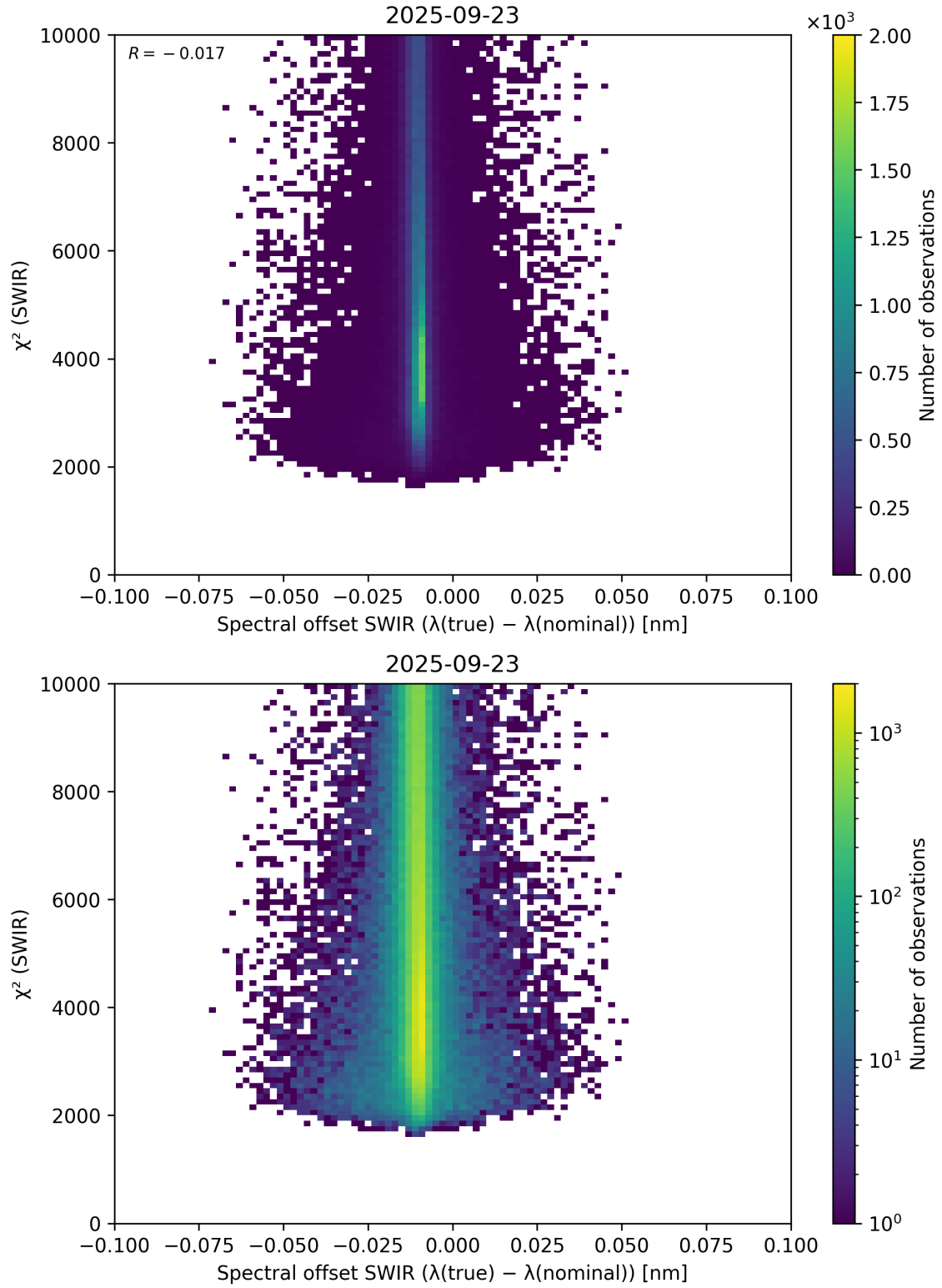
Figure 118: Scatter density plot of “Spectral offset SWIR ( \lambda_{\text{true}} - \lambda_{\text{nominal}} )” against “ \chi^2 (SWIR)” for 2025-09-22 to 2025-09-24.
