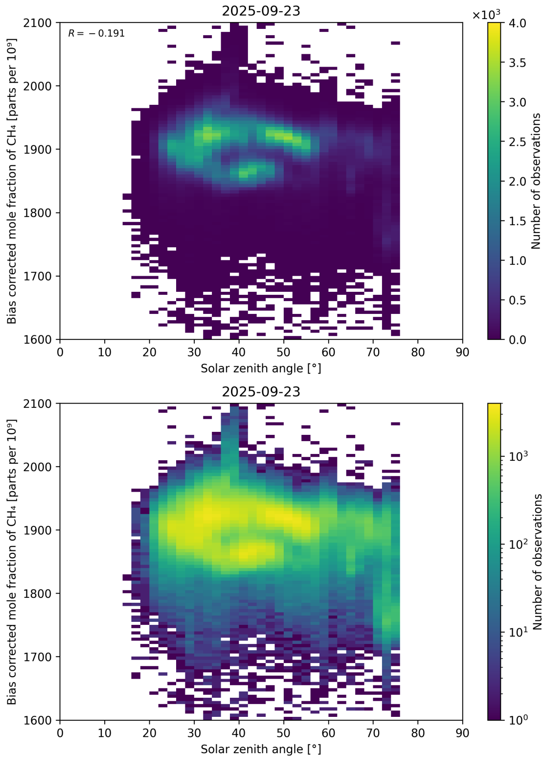
Figure 100: Scatter density plot of “Solar zenith angle” against “Bias corrected mole fraction of \text{CH}_4 ” for 2025-09-22 to 2025-09-24.
