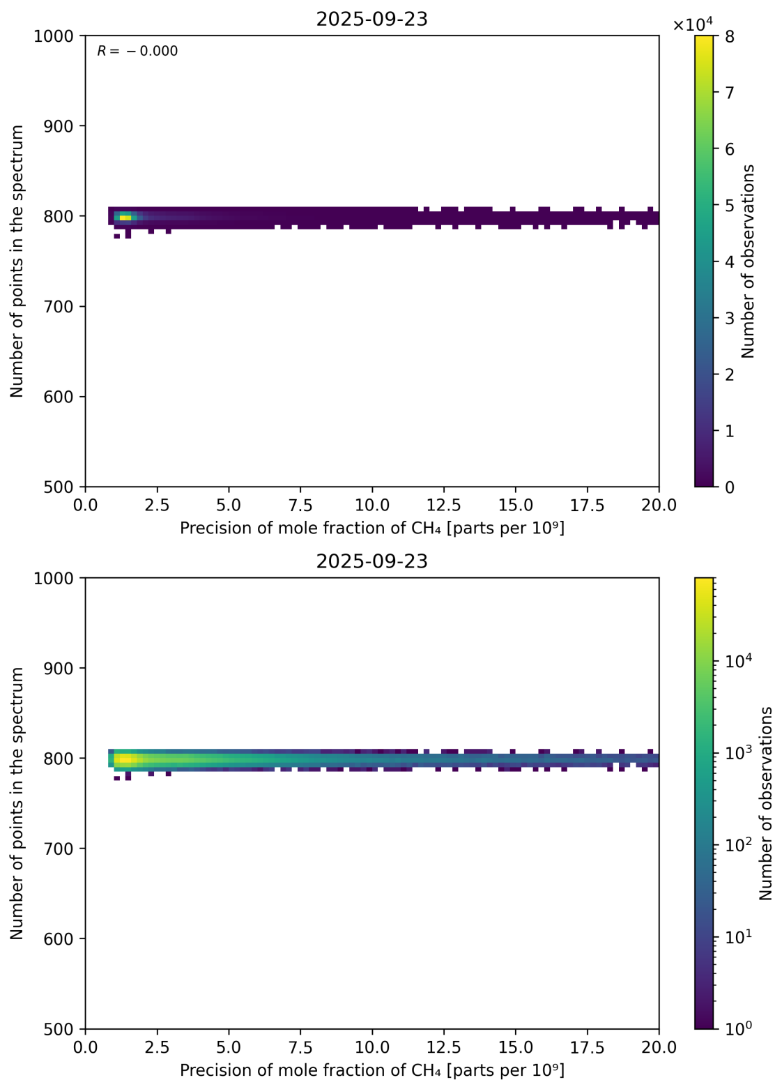
Figure 84: Scatter density plot of “Precision of mole fraction of CH 4 ” against “Number of points in the spectrum” for 2025-09-22 to 2025-09-24.
