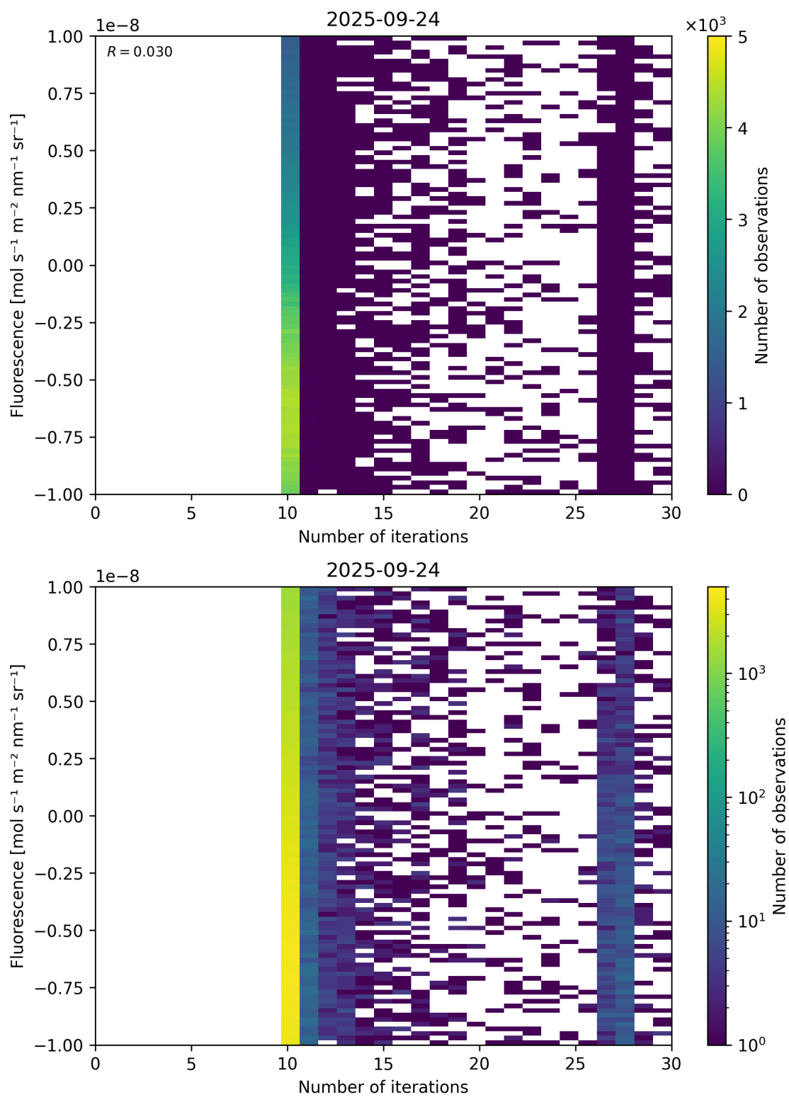
Figure 87: Scatter density plot of “Number of iterations” against “Fluorescence” for 2025-09-23 to 2025-09-25.
