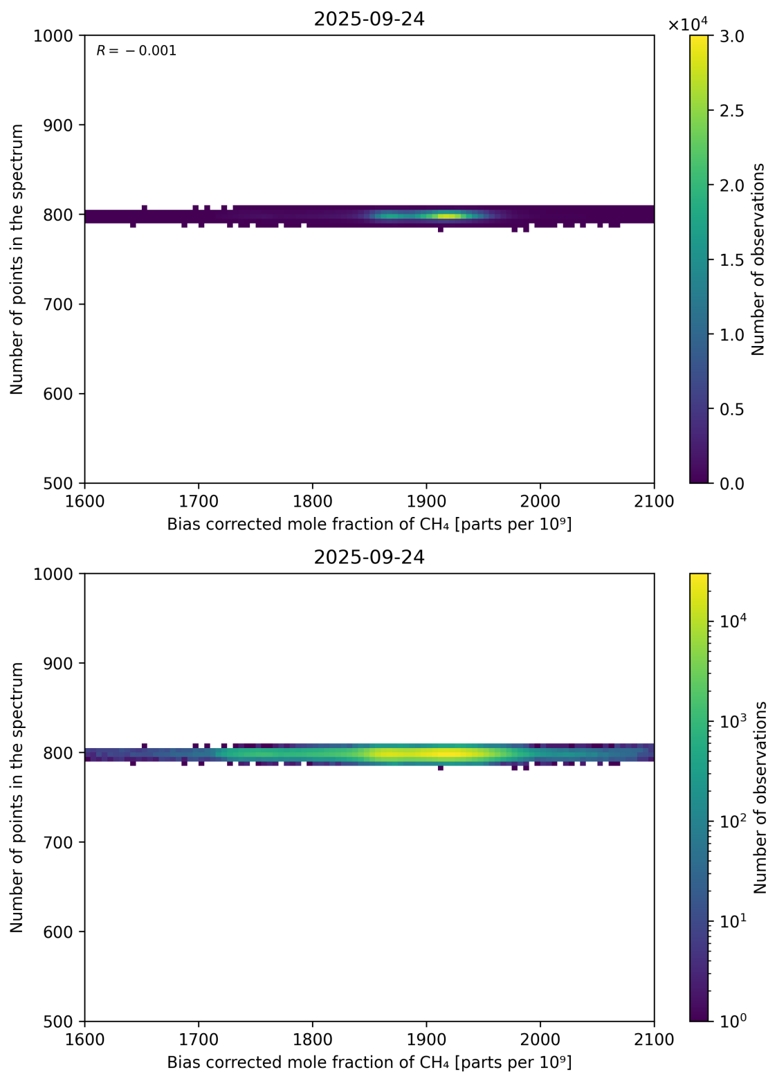
Figure 68: Scatter density plot of “Bias corrected mole fraction of CH 4 ” against “Number of points in the spectrum” for 2025-09-23 to 2025-09-25.
