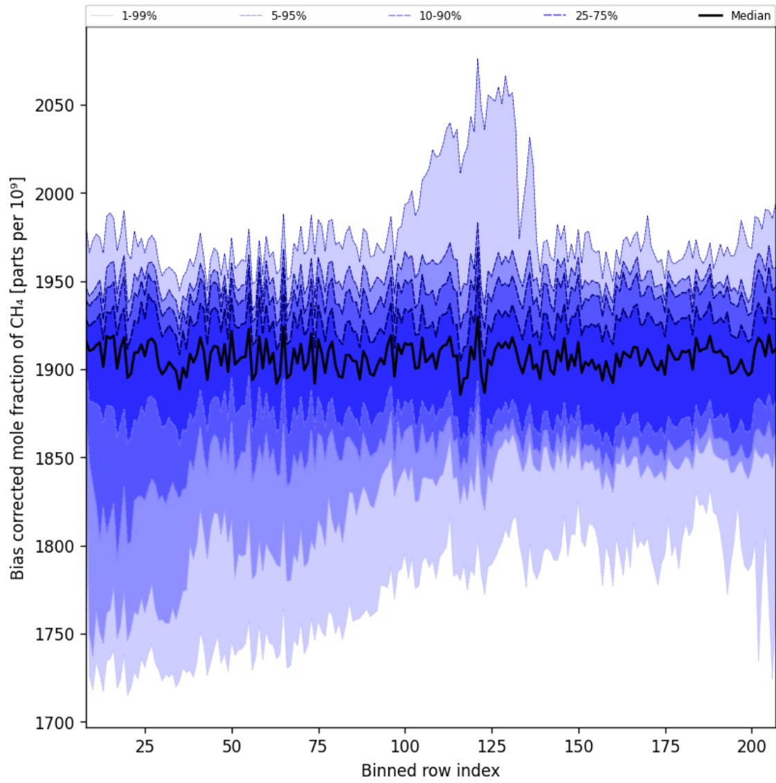
Figure 36: Along track statistics of “Bias corrected mole fraction of CH 4 ” for 2025-09-23 to 2025-09-25
