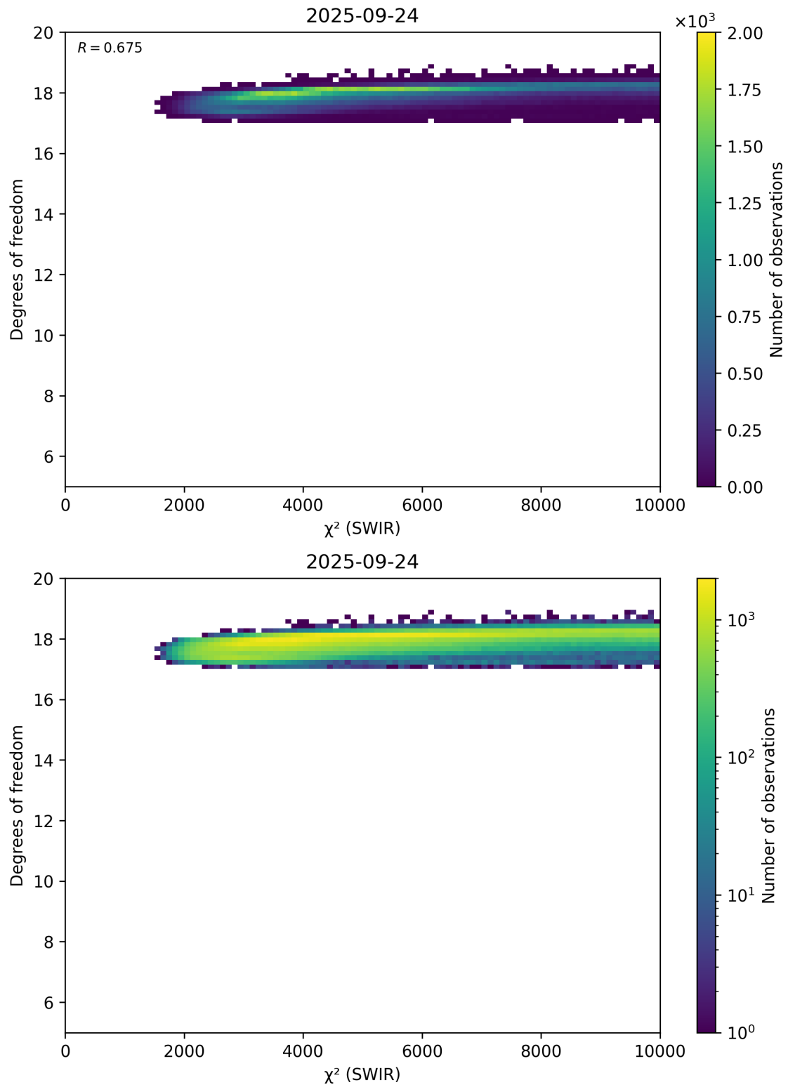
Figure 48: Scatter density plot of “ \chi^2 (SWIR)” against “Degrees of freedom” for 2025-09-23 to 2025-09-25.
