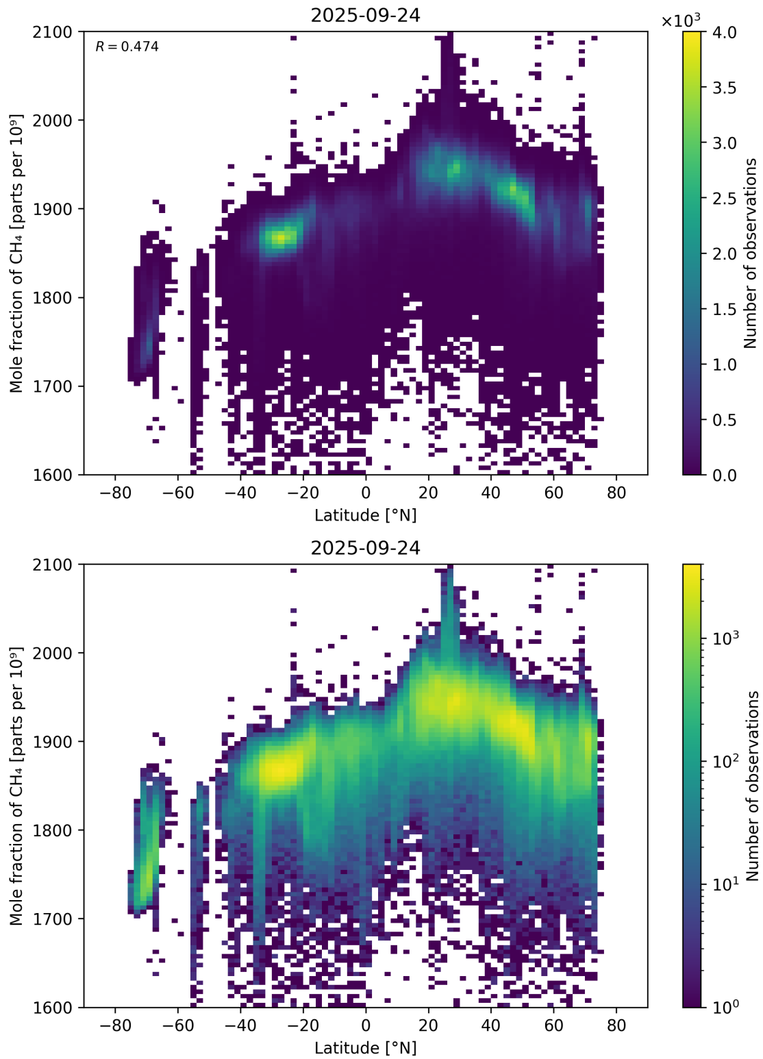
Figure 57: Scatter density plot of “Latitude” against “Mole fraction of CH 4 ” for 2025-09-23 to 2025-09-25.
