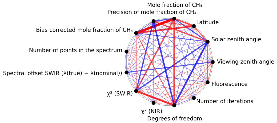
Figure 1: Map of correlation graph for 2025-09-23 to 2025-09-25.
