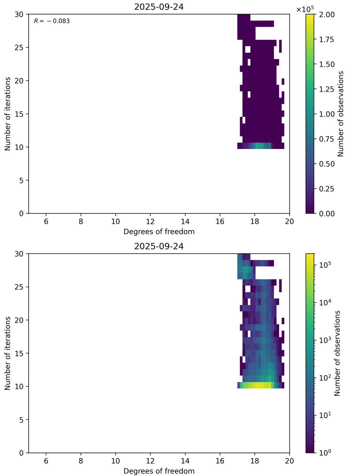
Figure 52: Scatter density plot of “Degrees of freedom” against “Number of iterations” for 2025-09-23 to 2025-09-25.
