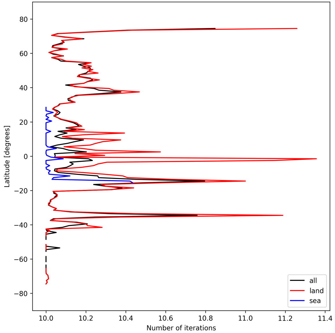
Figure 20: Zonal average of “Number of iterations” for 2025-09-23 to 2025-09-25.
