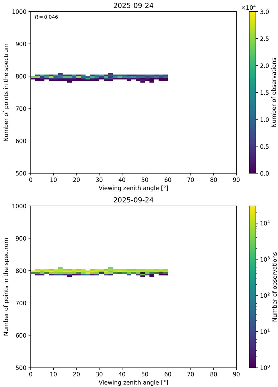
Figure 114: Scatter density plot of “Viewing zenith angle” against “Number of points in the spectrum” for 2025-09-23 to 2025-09-25.
