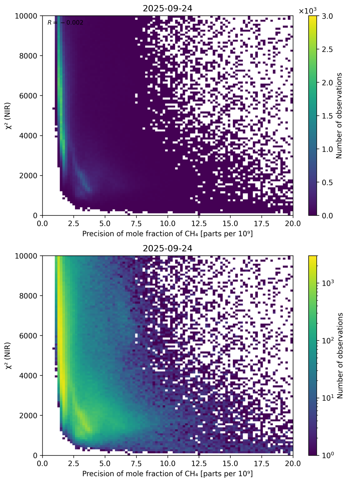
Figure 78: Scatter density plot of “Precision of mole fraction of CH 4 ” against “ \chi^2 (NIR)” for 2025-09-23 to 2025-09-25.
