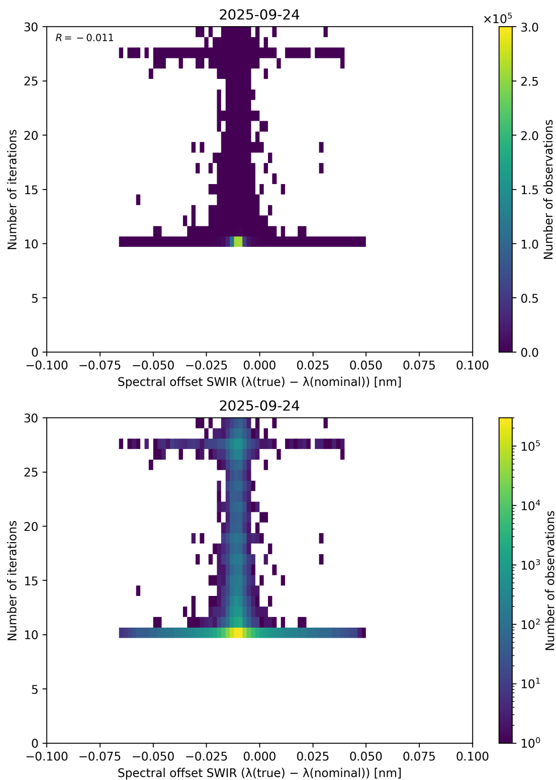
Figure 121: Scatter density plot of “Spectral offset SWIR ( \lambda_{\text{true}} - \lambda_{\text{nominal}} )” against “Number of iterations” for 2025-09-23 to 2025-09-25.
