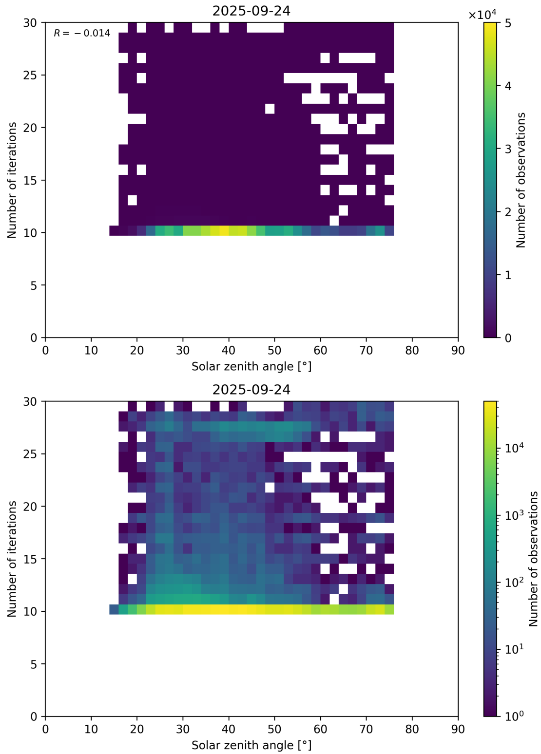
Figure 102: Scatter density plot of “Solar zenith angle” against “Number of iterations” for 2025-09-23 to 2025-09-25.
