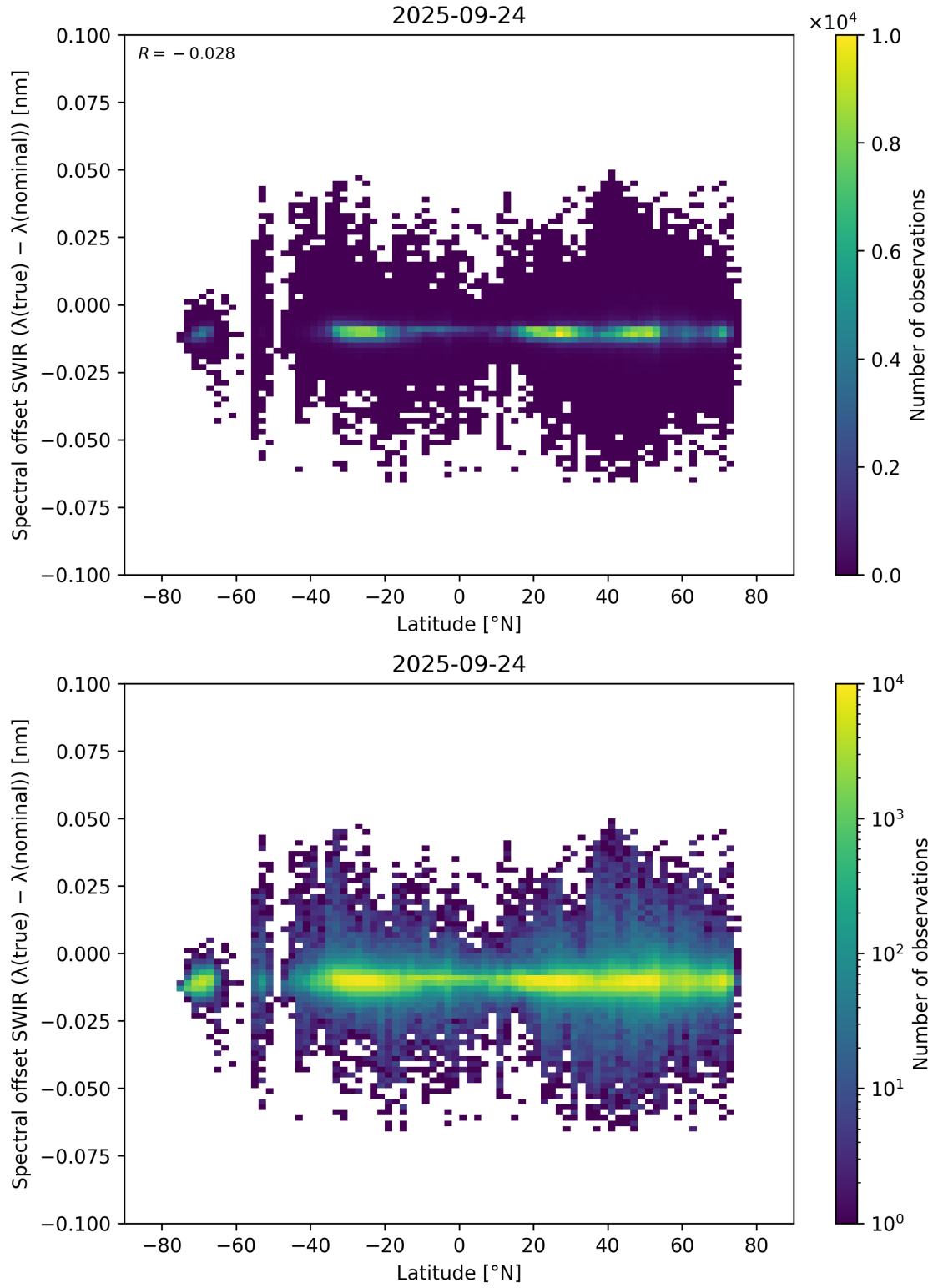
Figure 62: Scatter density plot of “Latitude” against “Spectral offset SWIR ( \lambda_{\text{true}} - \lambda_{\text{nominal}} )” for 2025-09-23 to 2025-09-25.
