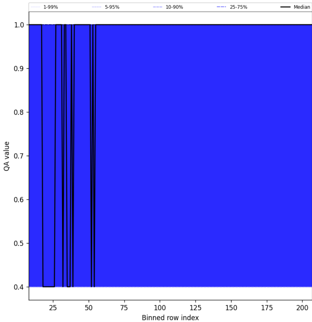
Figure 33: Along track statistics of “QA value” for 2025-09-23 to 2025-09-25
