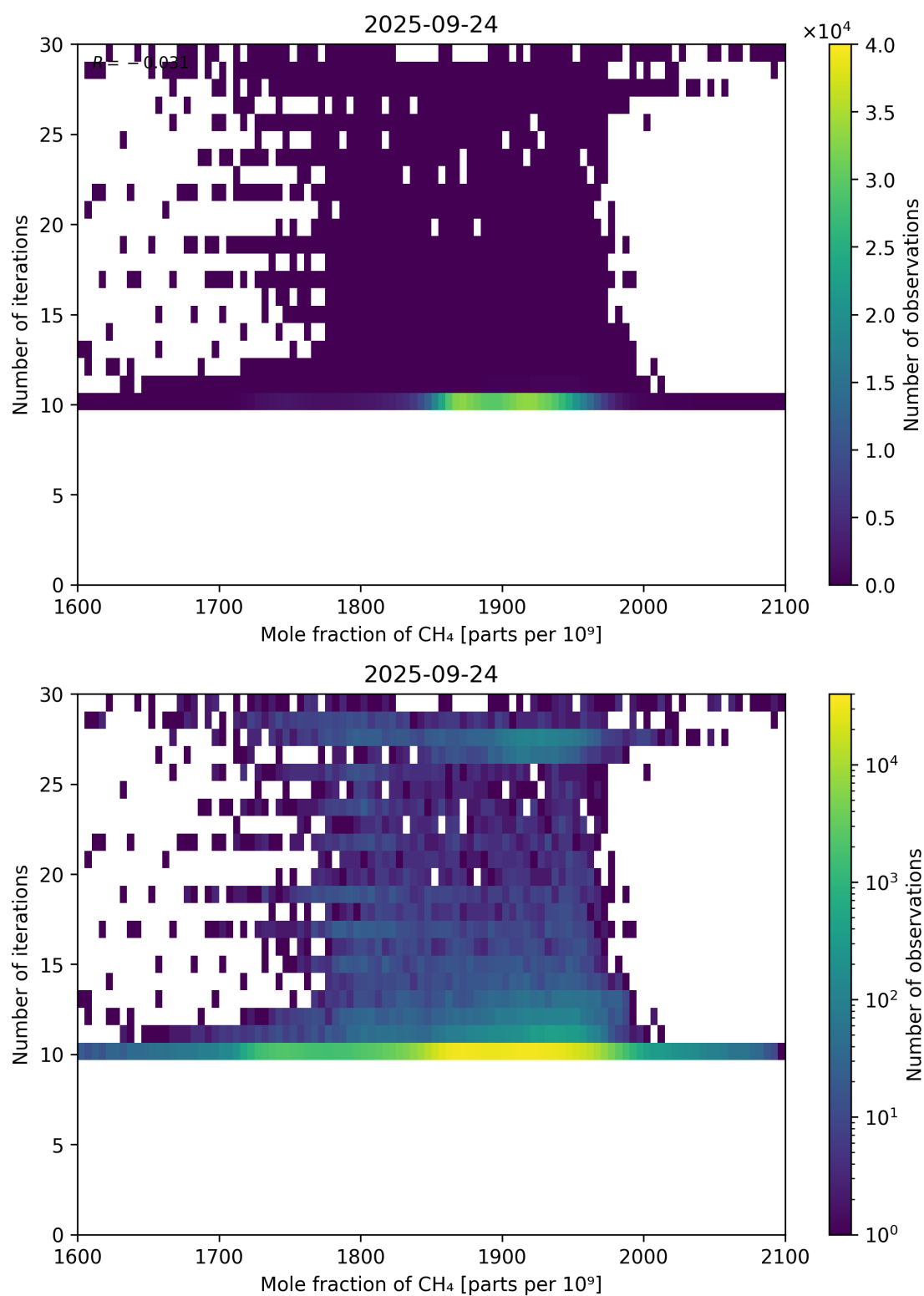
Figure 76: Scatter density plot of “Mole fraction of CH 4 ” against “Number of iterations” for 2025-09-23 to 2025-09-25.
