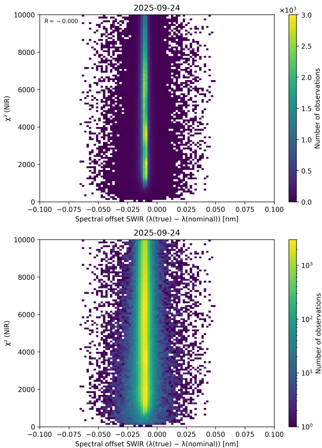
Figure 117: Scatter density plot of “Spectral offset SWIR ( \lambda_{\text{true}} - \lambda_{\text{nominal}} )” against “ \chi^2 (NIR)” for 2025-09-23 to 2025-09-25.
