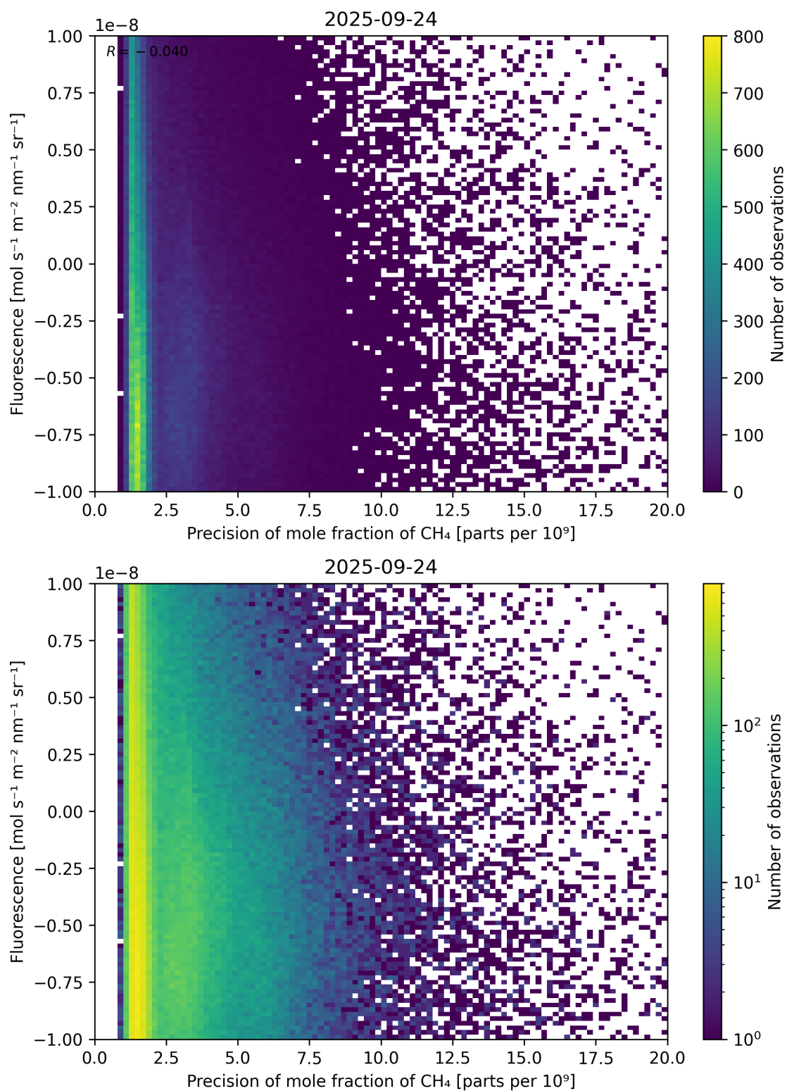
Figure 81: Scatter density plot of “Precision of mole fraction of CH 4 ” against “Fluorescence” for 2025-09-23 to 2025-09-25.
