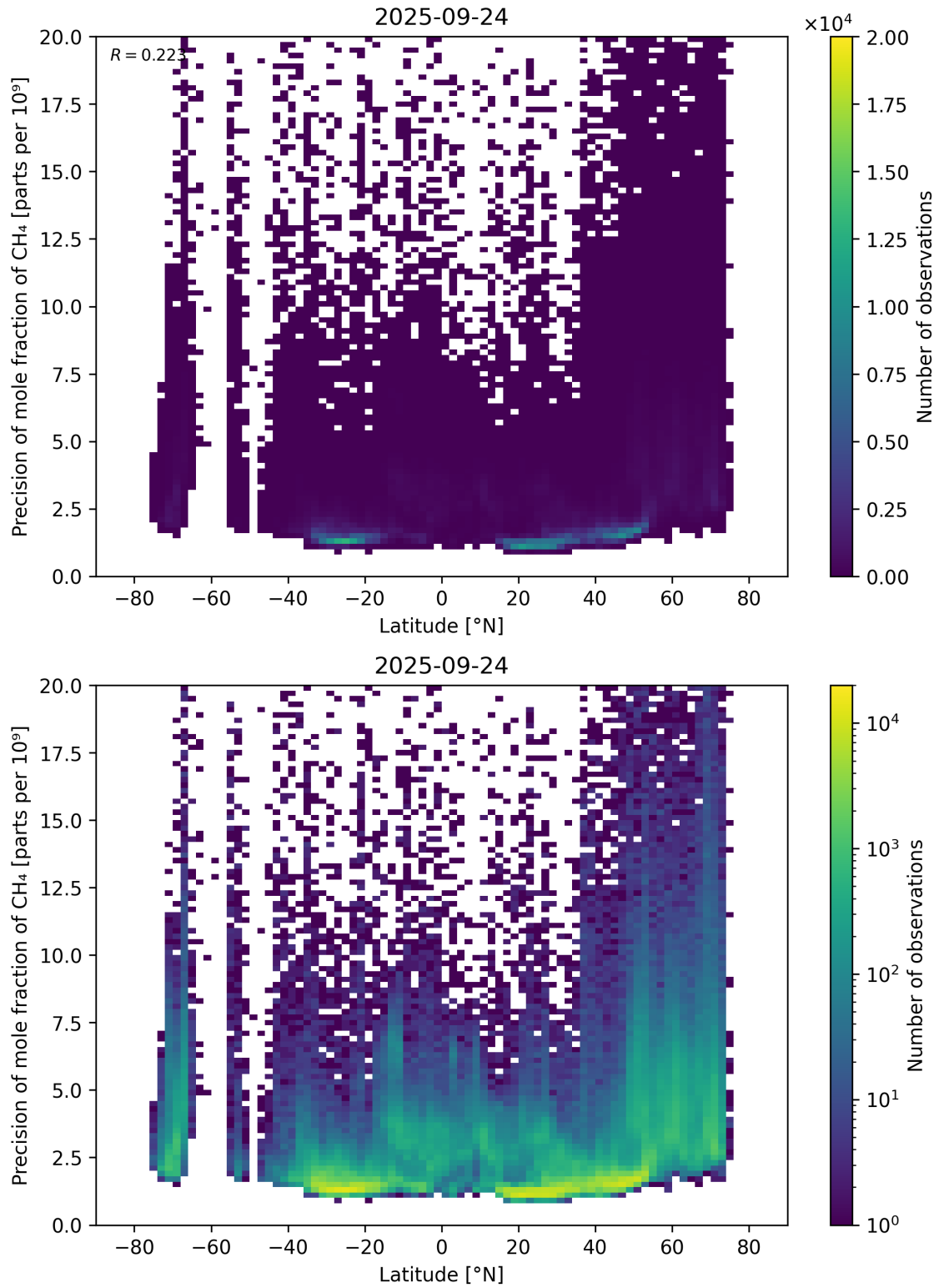
Figure 59: Scatter density plot of “Latitude” against “Precision of mole fraction of \text{CH}_4 ” for 2025-09-23 to 2025-09-25.
