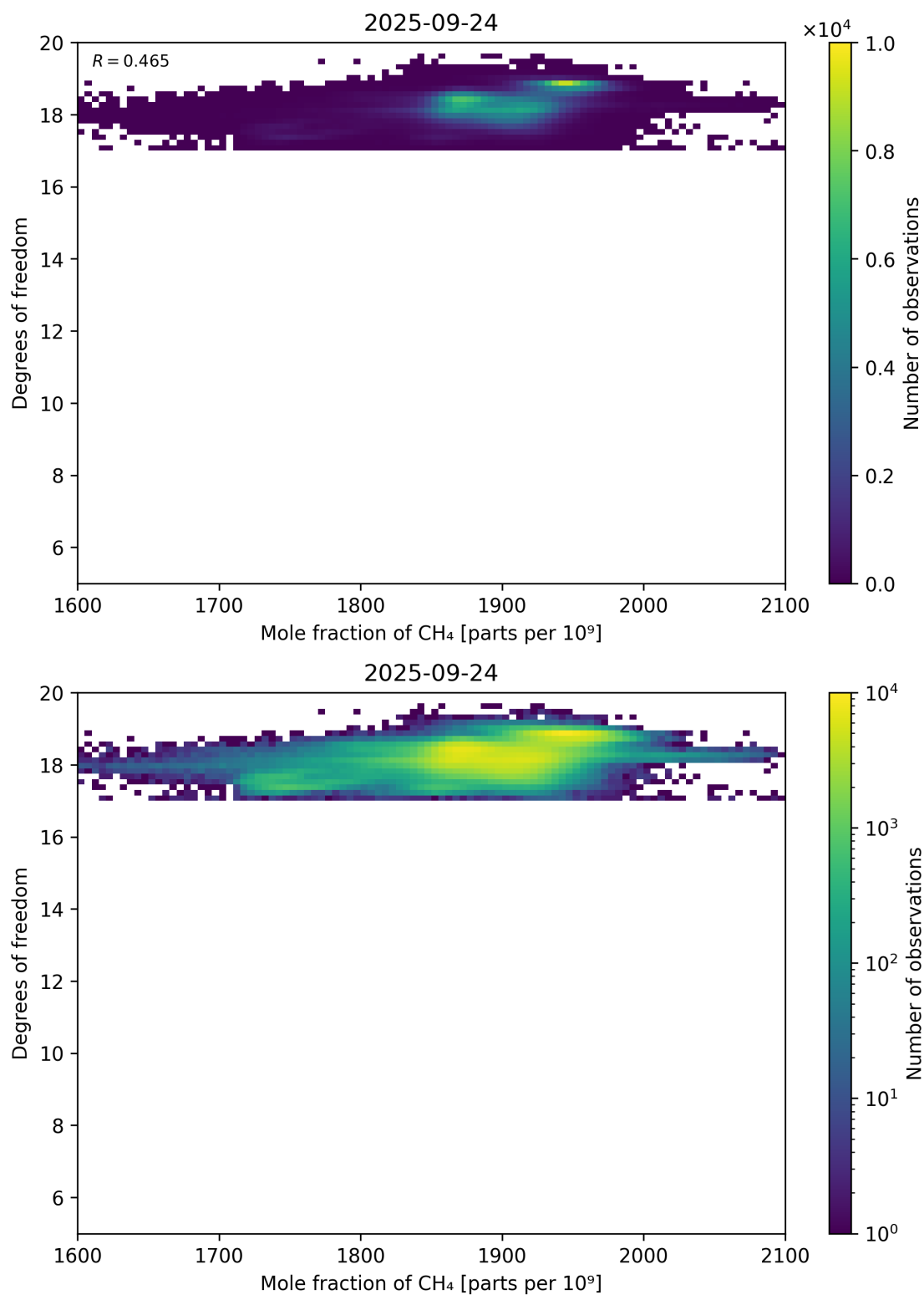
Figure 72: Scatter density plot of “Mole fraction of CH 4 ” against “Degrees of freedom” for 2025-09-23 to 2025-09-25.
