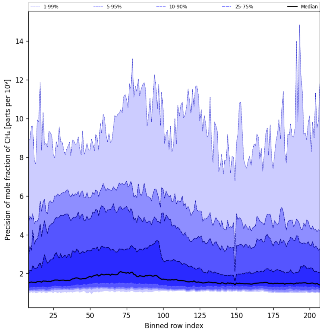
Figure 35: Along track statistics of “Precision of mole fraction of CH 4 ” for 2025-09-23 to 2025-09-25
