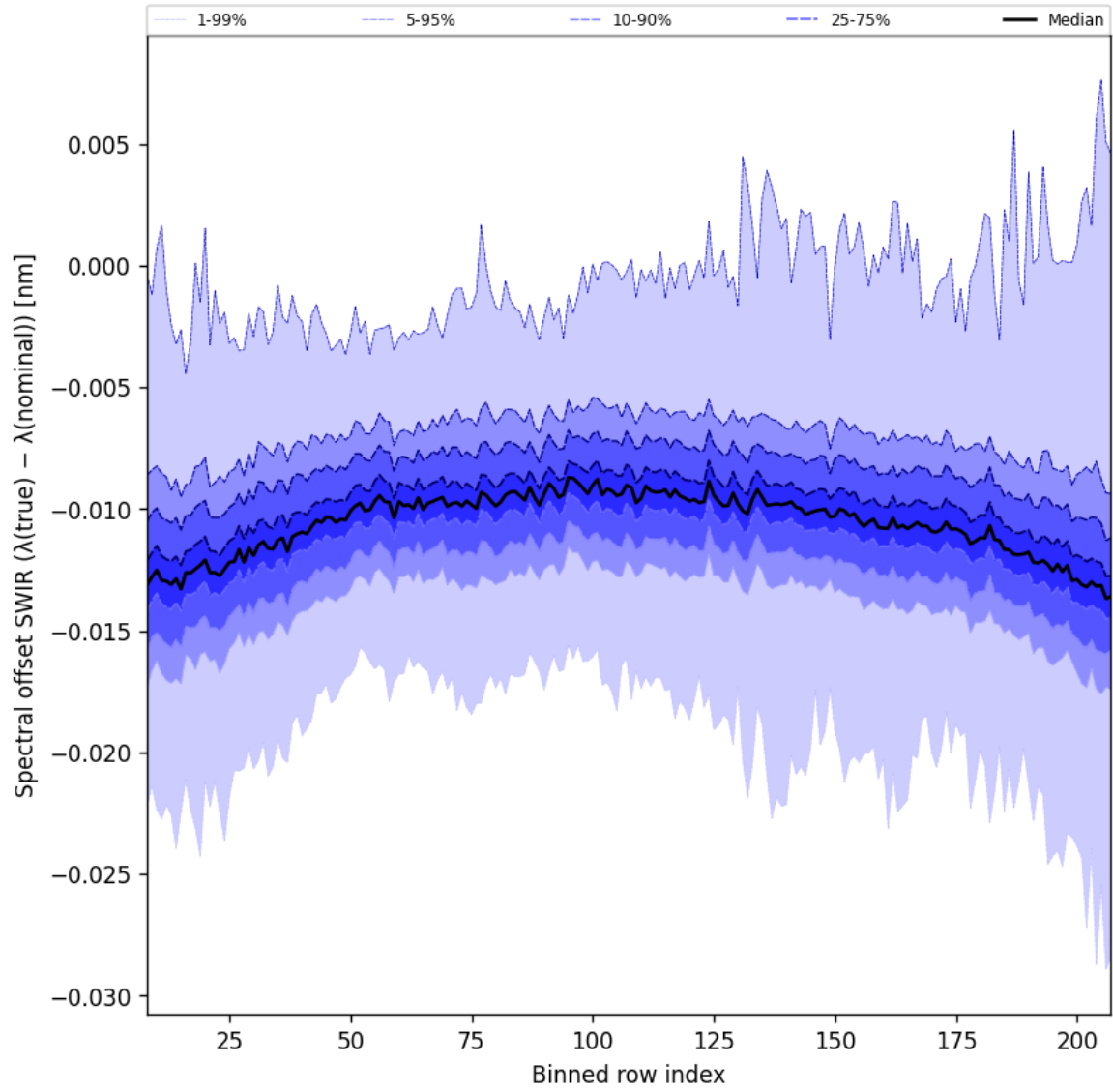
Figure 38: Along track statistics of “Spectral offset SWIR ( \lambda_{\text{true}} - \lambda_{\text{nominal}} )” for 2025-09-23 to 2025-09-25
