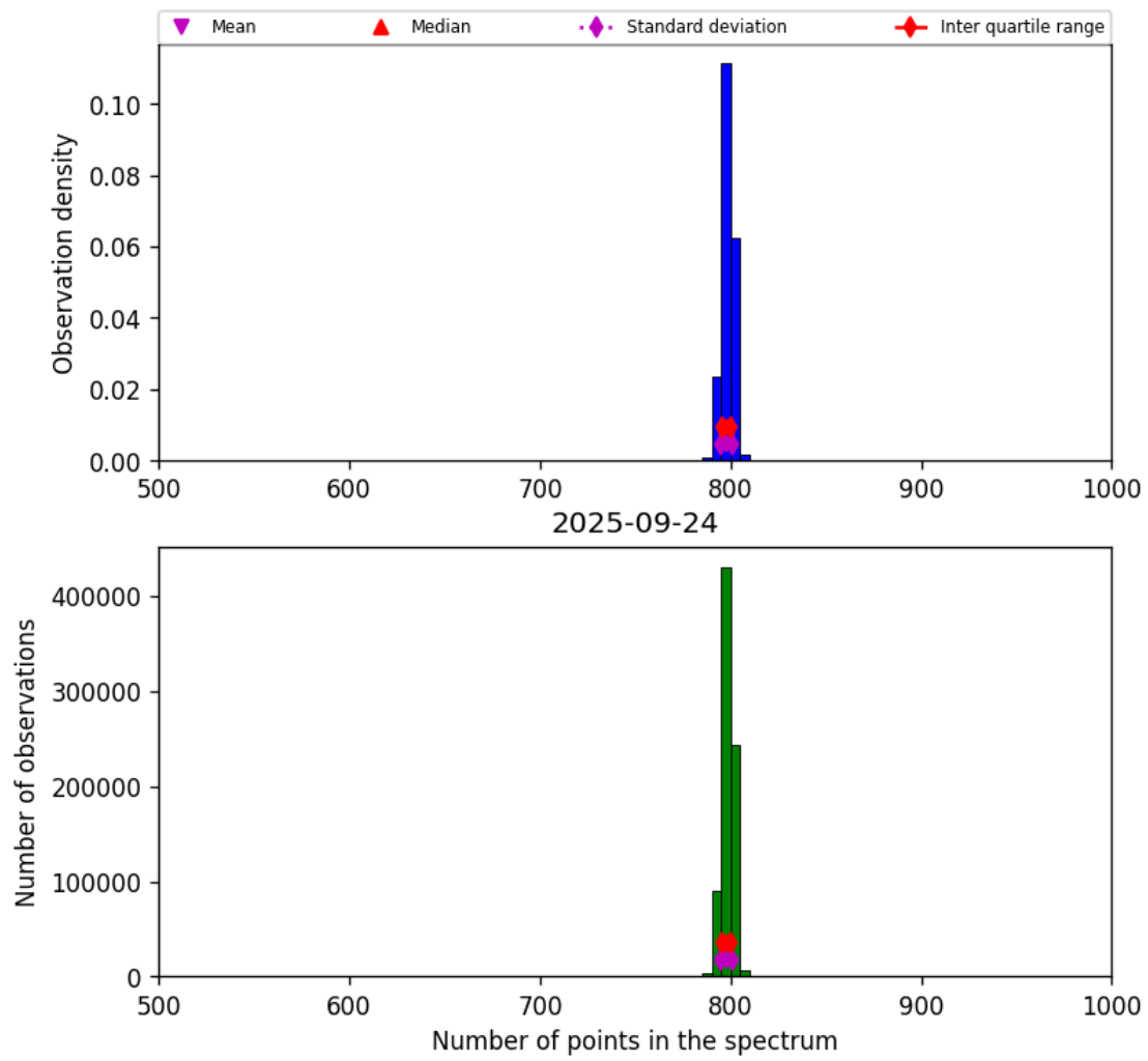
Figure 26: Histogram of “Number of points in the spectrum” for 2025-09-23 to 2025-09-25
