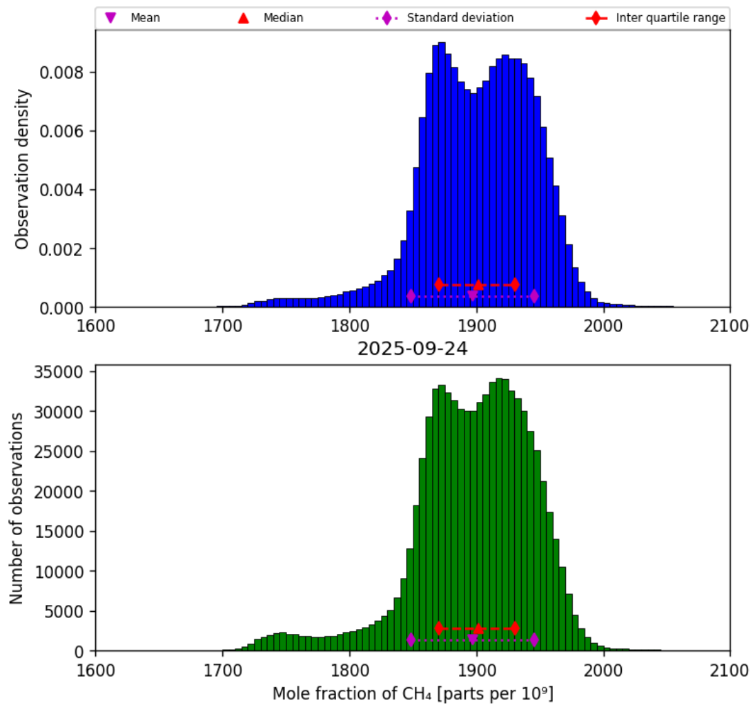
Figure 23: Histogram of “Mole fraction of CH 4 ” for 2025-09-23 to 2025-09-25
