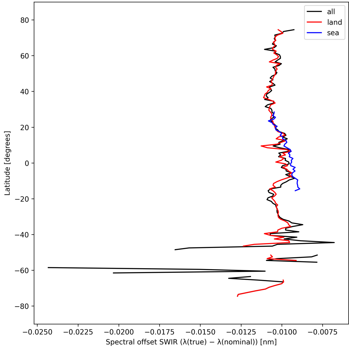
Figure 16: Zonal average of “Spectral offset SWIR ( \lambda_{\text{true}} - \lambda_{\text{nominal}} )” for 2025-09-23 to 2025-09-25.
