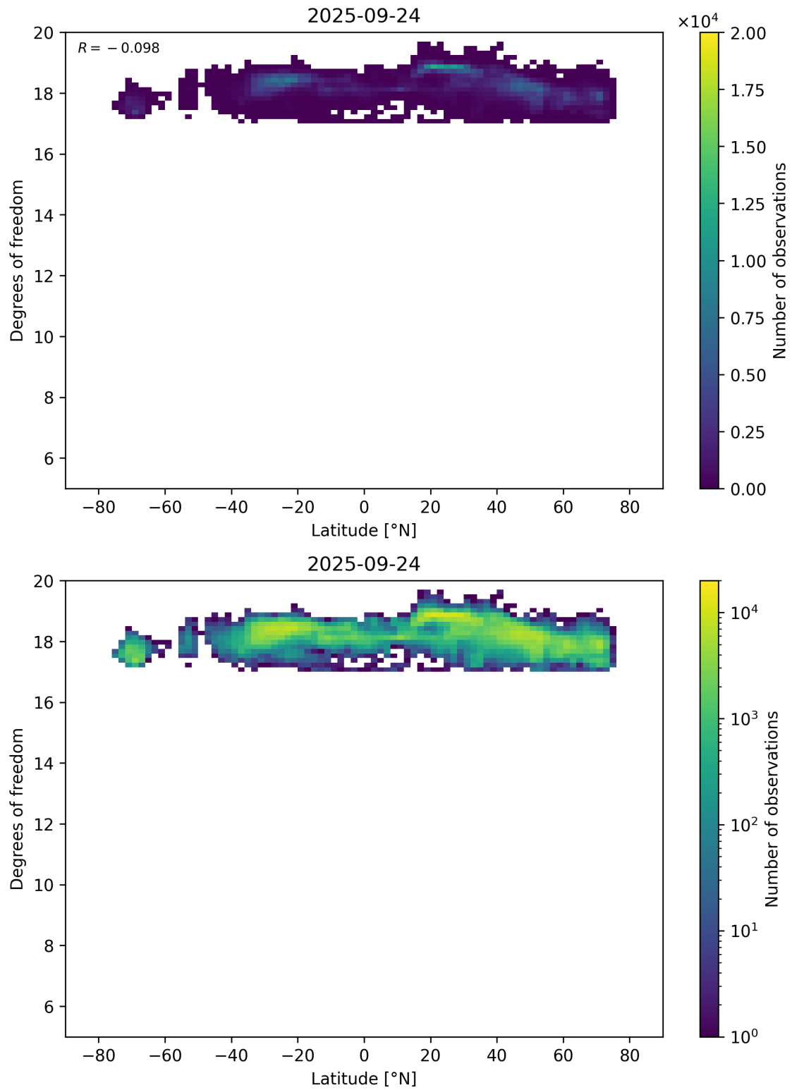
Figure 55: Scatter density plot of “Latitude” against “Degrees of freedom” for 2025-09-23 to 2025-09-25.
