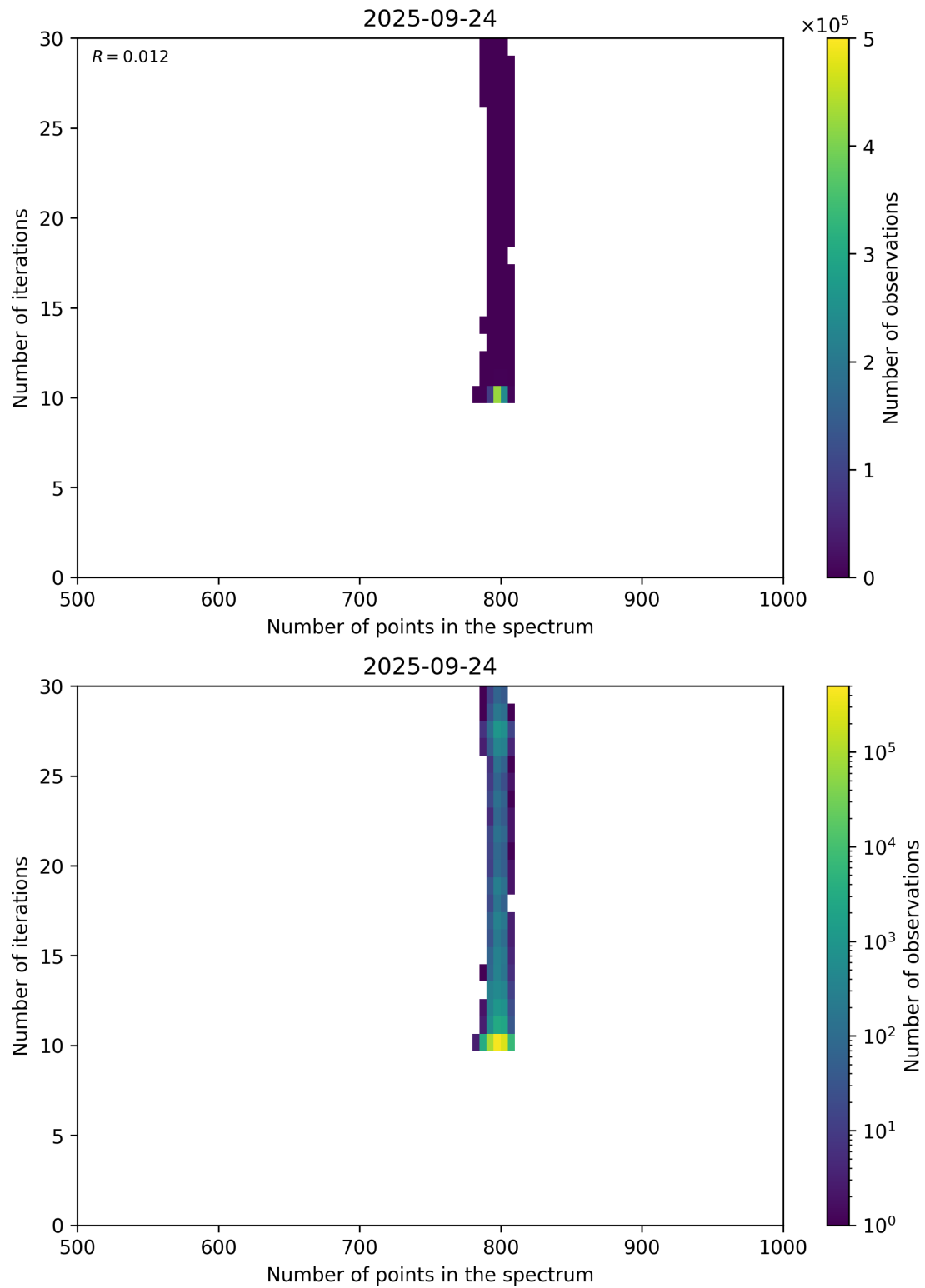
Figure 92: Scatter density plot of “Number of points in the spectrum” against “Number of iterations” for 2025-09-23 to 2025-09-25.
