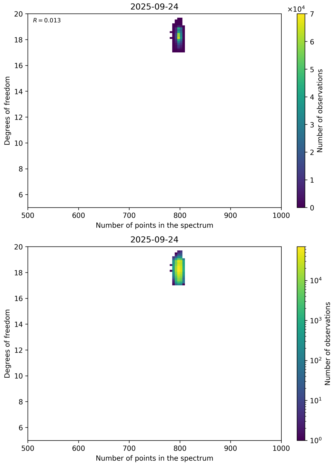
Figure 90: Scatter density plot of “Number of points in the spectrum” against “Degrees of freedom” for 2025-09-23 to 2025-09-25.
