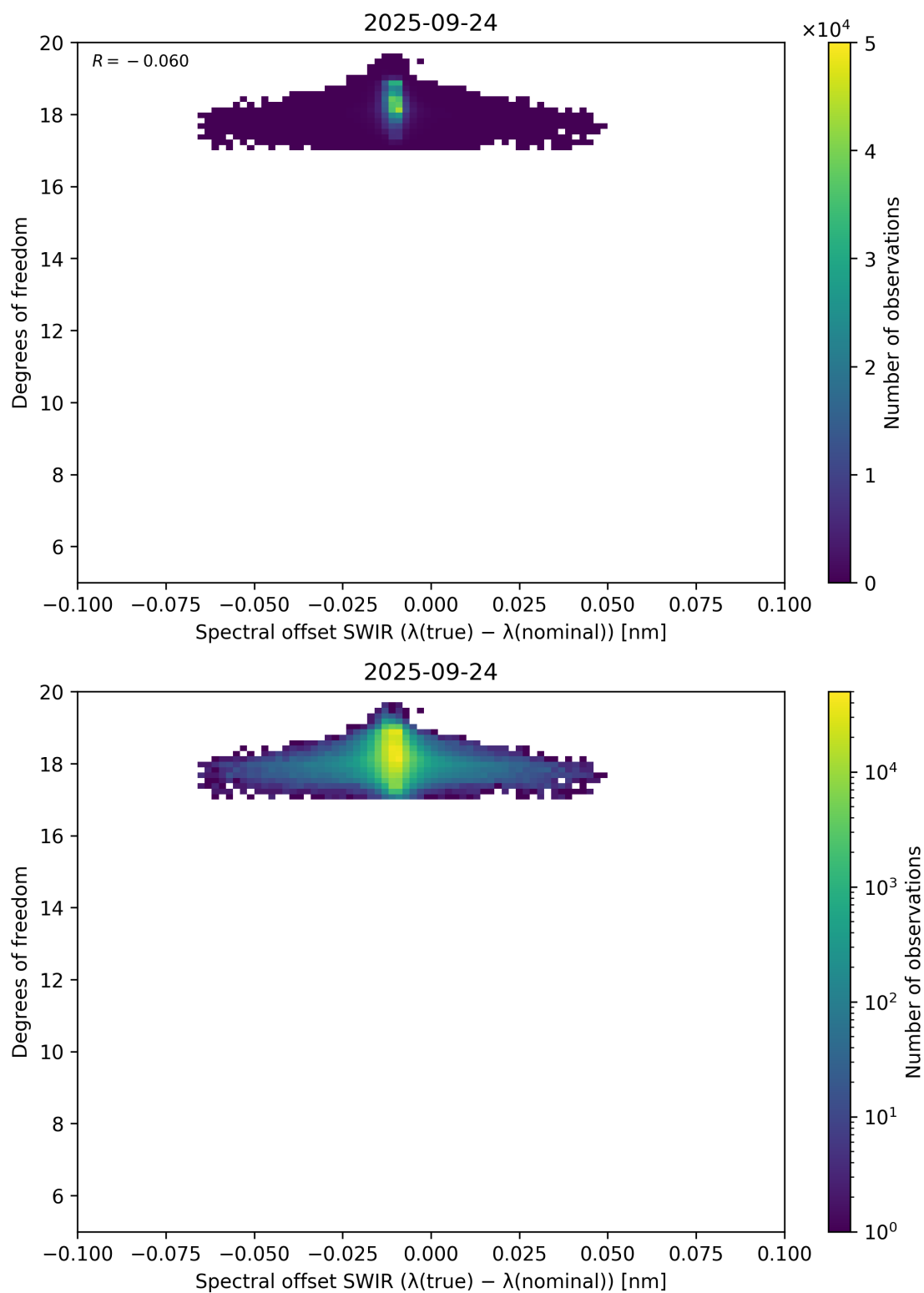
Figure 119: Scatter density plot of “Spectral offset SWIR ( \lambda_{\text{true}} - \lambda_{\text{nominal}} )” against “Degrees of freedom” for 2025-09-23 to 2025-09-25.
