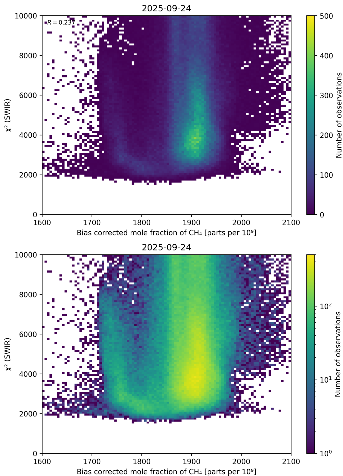
Figure 64: Scatter density plot of “Bias corrected mole fraction of CH 4 ” against “ \chi^2 (SWIR)” for 2025-09-23 to 2025-09-25.
