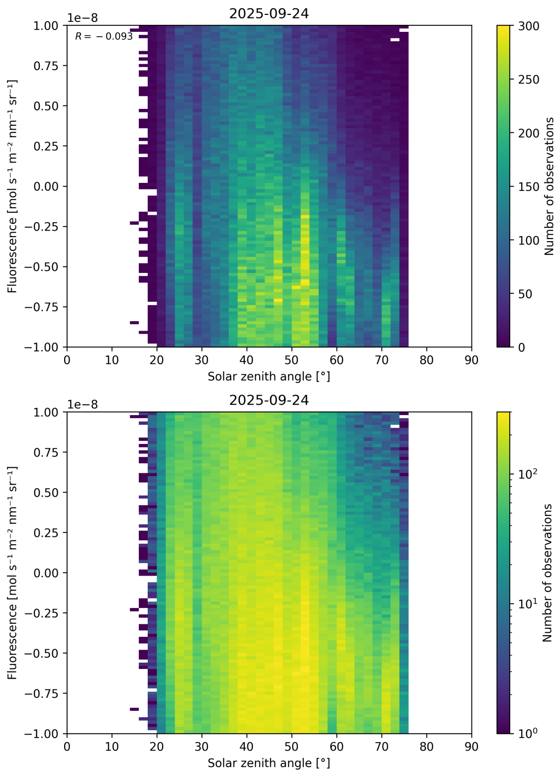
Figure 97: Scatter density plot of “Solar zenith angle” against “Fluorescence” for 2025-09-23 to 2025-09-25.
