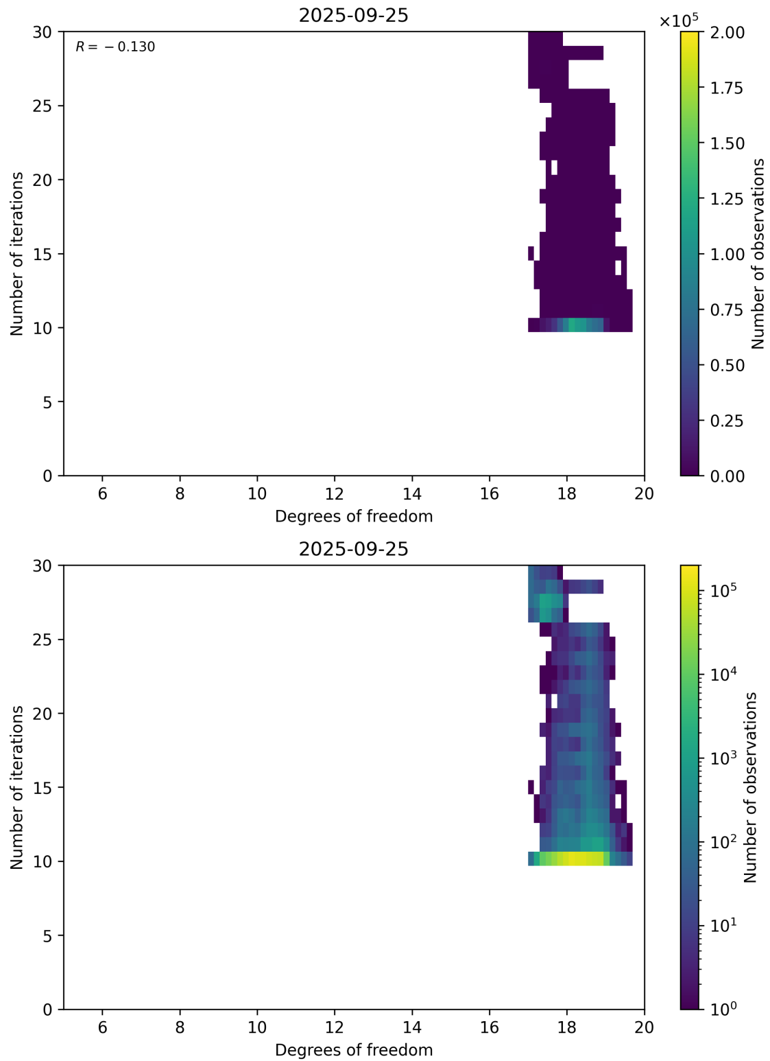
Figure 52: Scatter density plot of “Degrees of freedom” against “Number of iterations” for 2025-09-25 to 2025-09-26.
