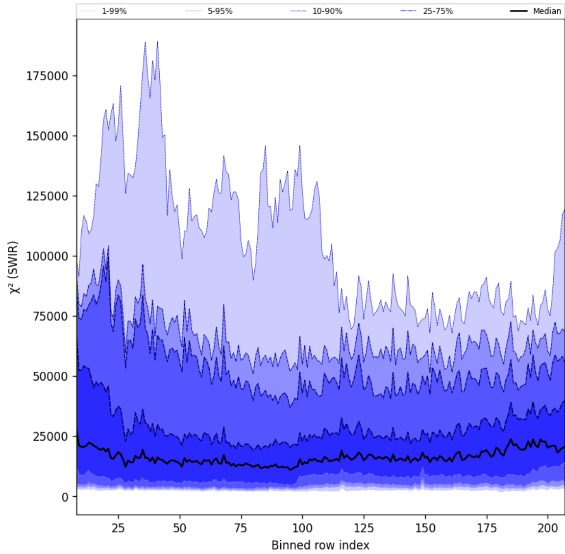
Figure 39: Along track statistics of “ \chi^2 (SWIR)” for 2025-09-25 to 2025-09-26
