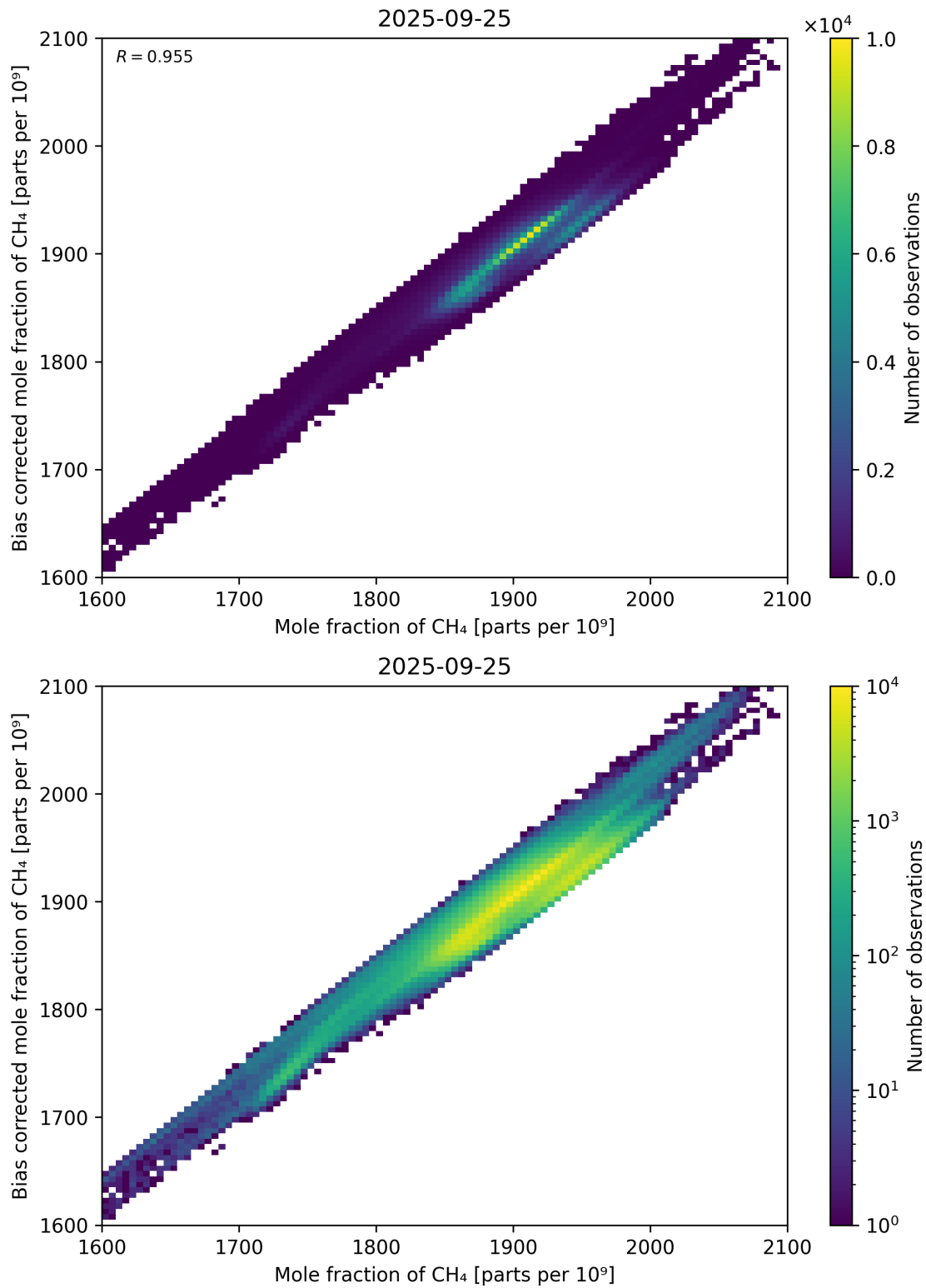
Figure 74: Scatter density plot of “Mole fraction of CH 4 ” against “Bias corrected mole fraction of CH 4 ” for 2025-09-25 to 2025-09-26.
