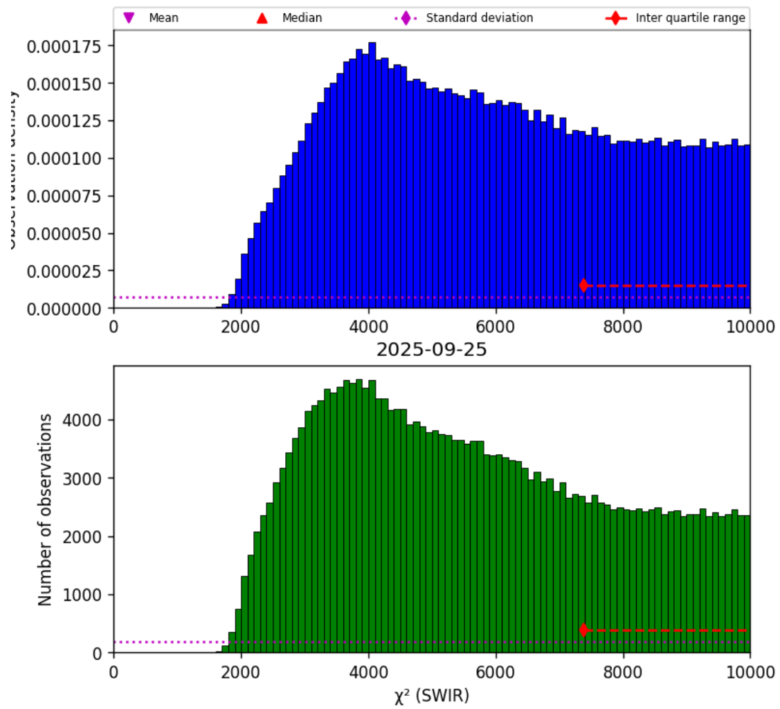
Figure 28: Histogram of “ \chi^2 (SWIR)” for 2025-09-25 to 2025-09-26
