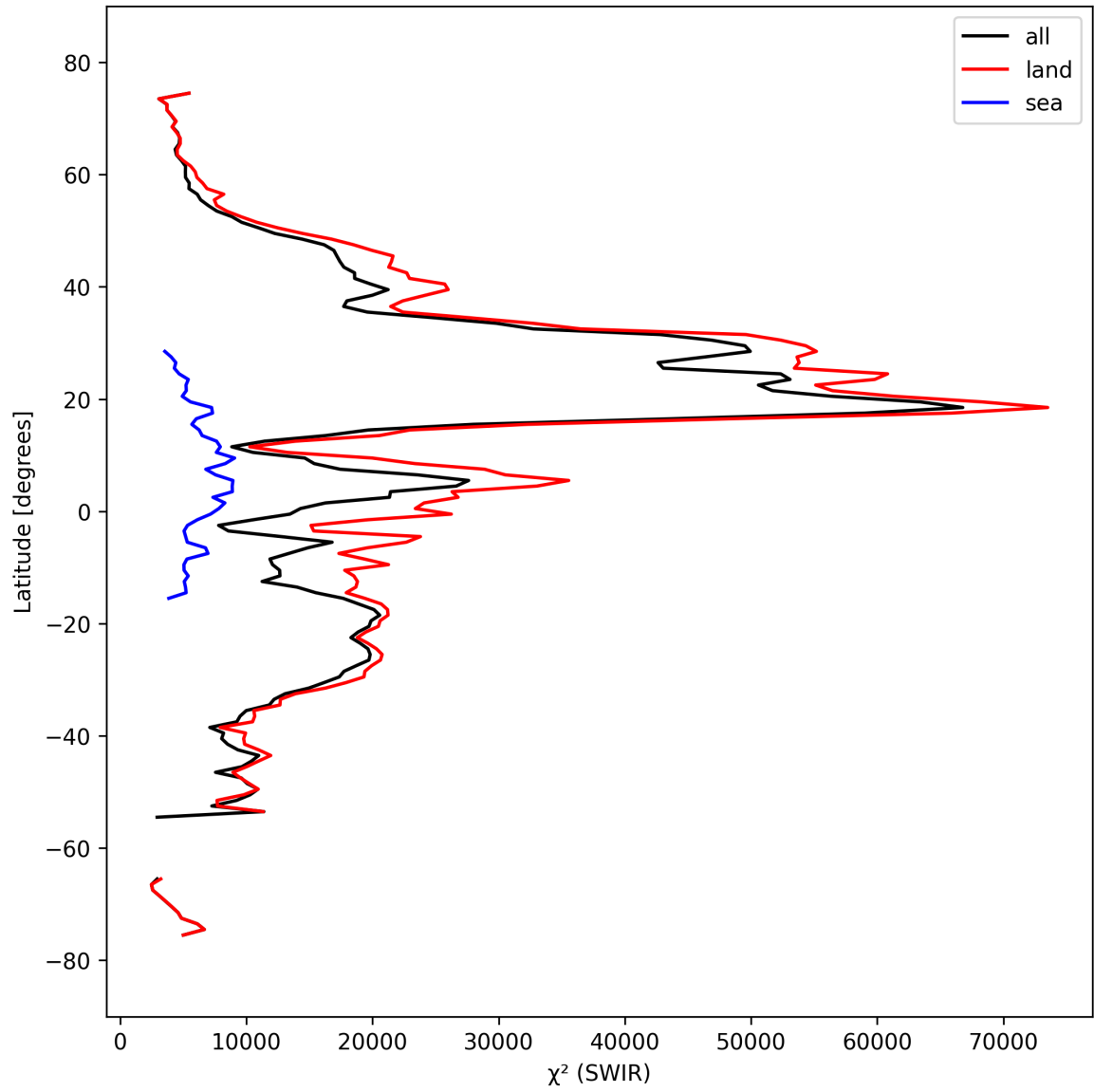
Figure 17: Zonal average of “ \chi^2 (SWIR)” for 2025-09-25 to 2025-09-26.
