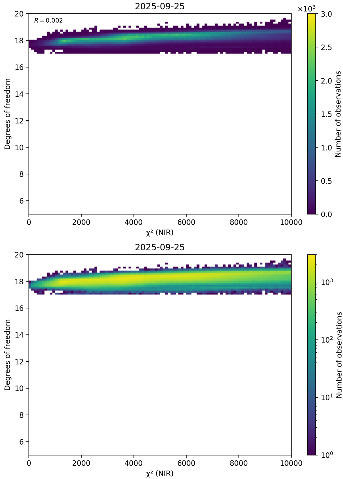
Figure 44: Scatter density plot of “ \chi^2 (NIR)” against “Degrees of freedom” for 2025-09-25 to 2025-09-26.
