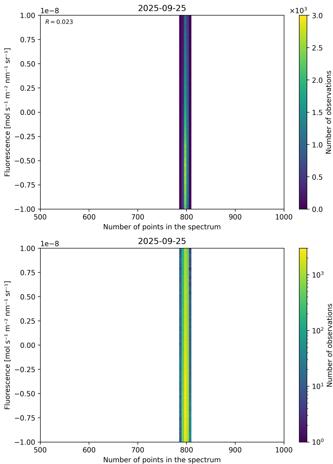
Figure 91: Scatter density plot of “Number of points in the spectrum” against “Fluorescence” for 2025-09-25 to 2025-09-26.
