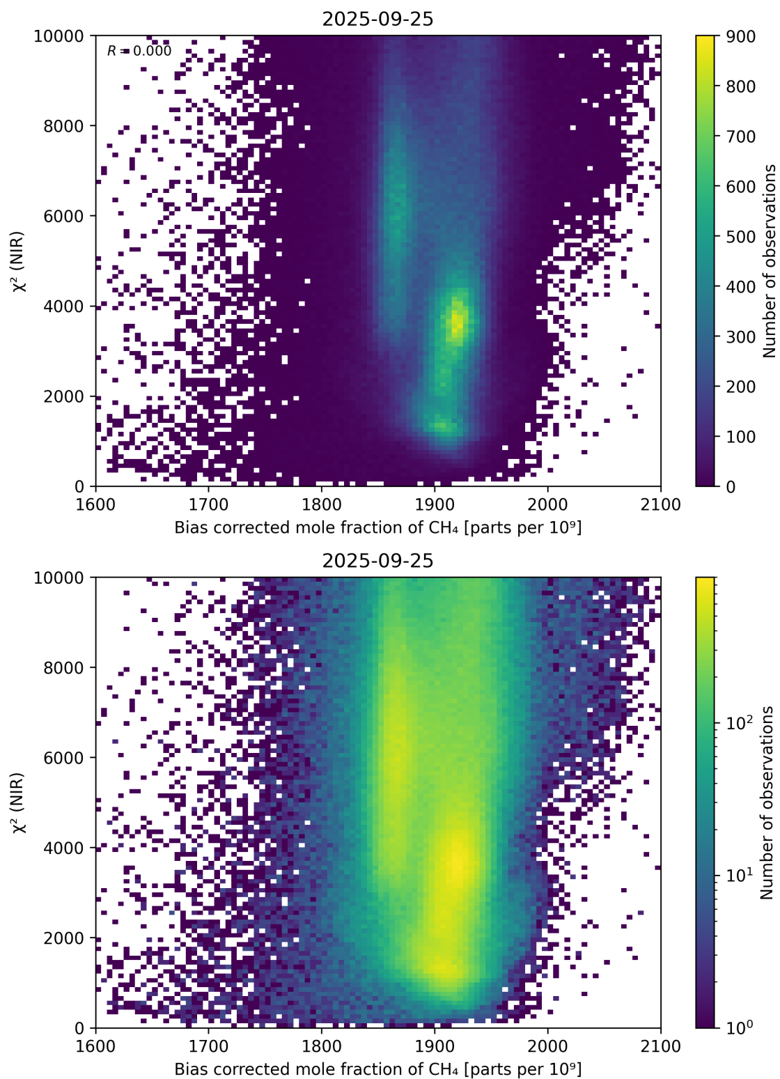
Figure 63: Scatter density plot of “Bias corrected mole fraction of CH 4 ” against “ \chi^2 (NIR)” for 2025-09-25 to 2025-09-26.
