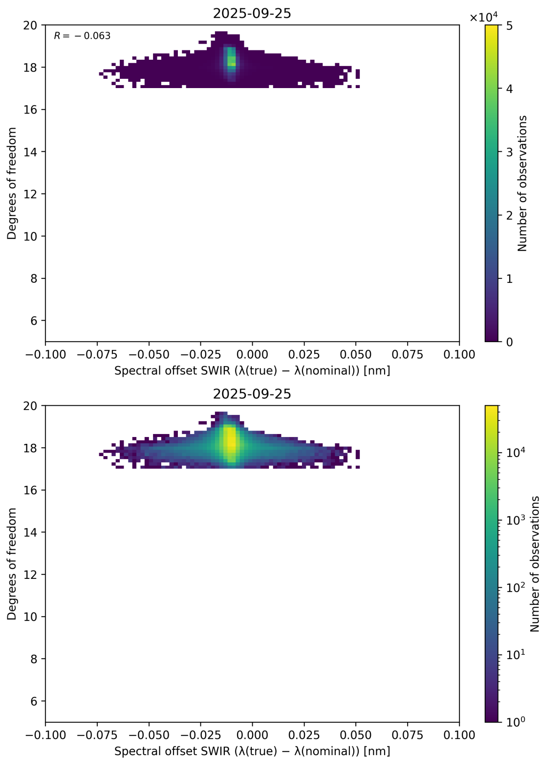
Figure 119: Scatter density plot of “Spectral offset SWIR ( \lambda_{\text{true}} - \lambda_{\text{nominal}} )” against “Degrees of freedom” for 2025-09-25 to 2025-09-26.
