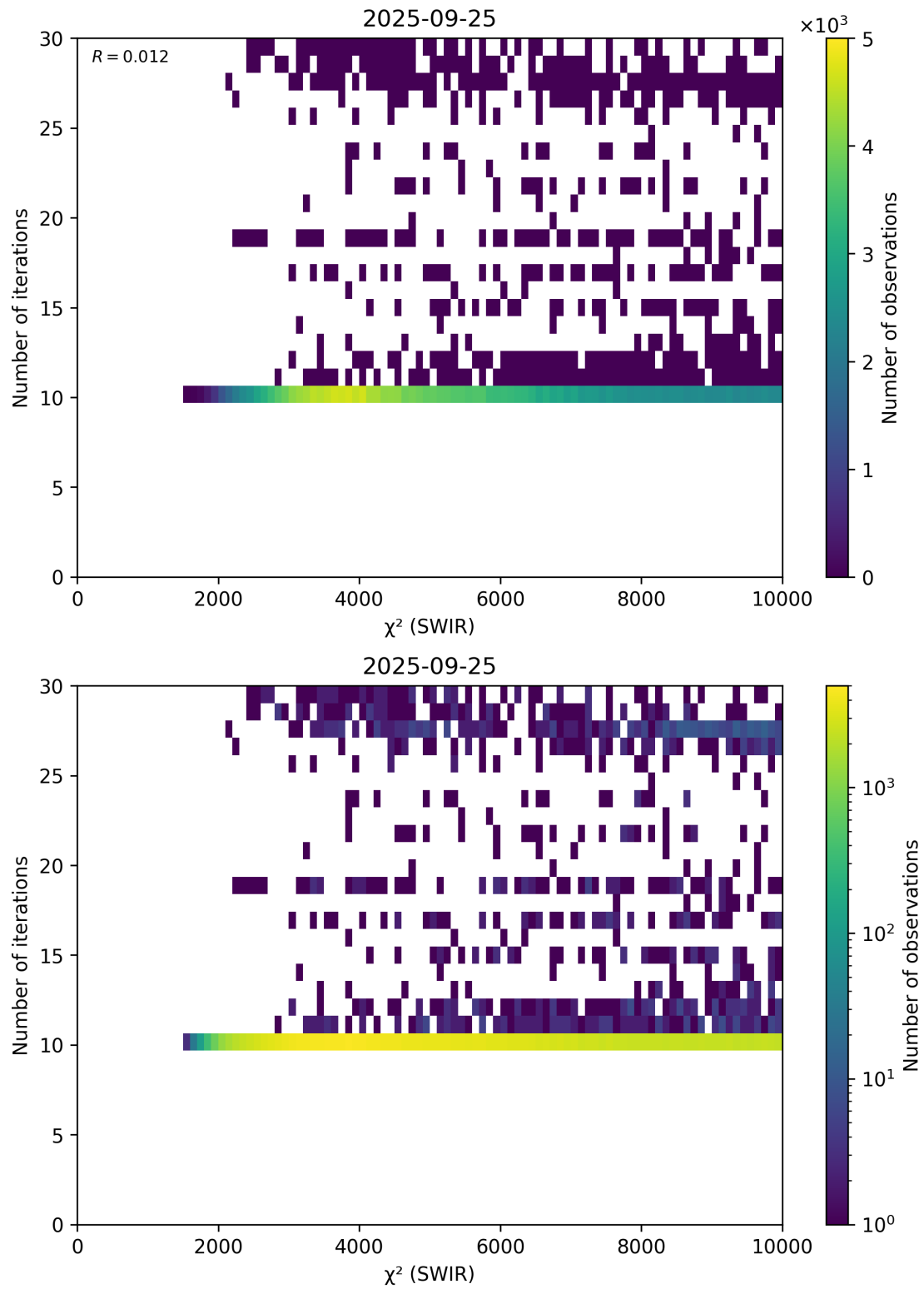
Figure 50: Scatter density plot of “ \chi^2 (SWIR)” against “Number of iterations” for 2025-09-25 to 2025-09-26.
