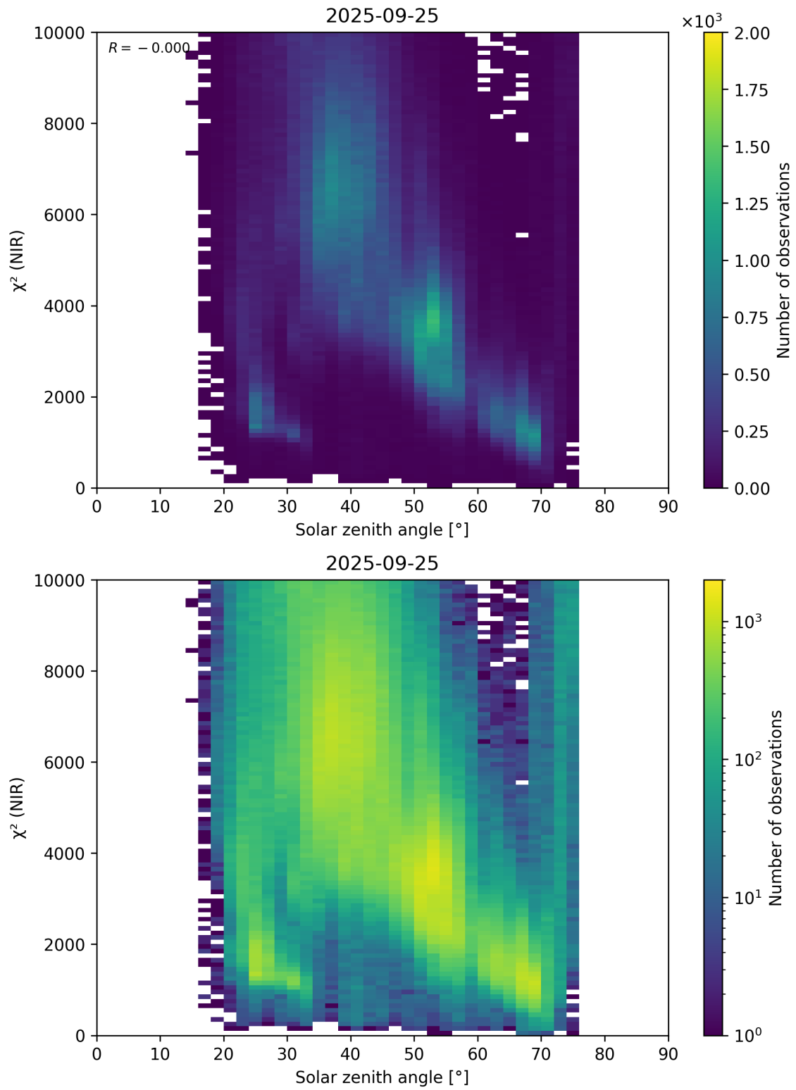
Figure 94: Scatter density plot of “Solar zenith angle” against “ \chi^2 (NIR)” for 2025-09-25 to 2025-09-26.
