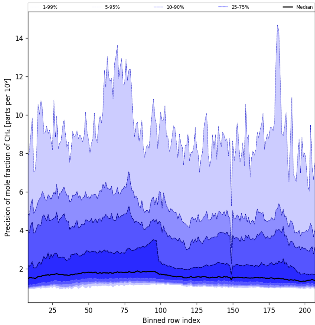
Figure 35: Along track statistics of “Precision of mole fraction of CH 4 ” for 2025-09-25 to 2025-09-26
