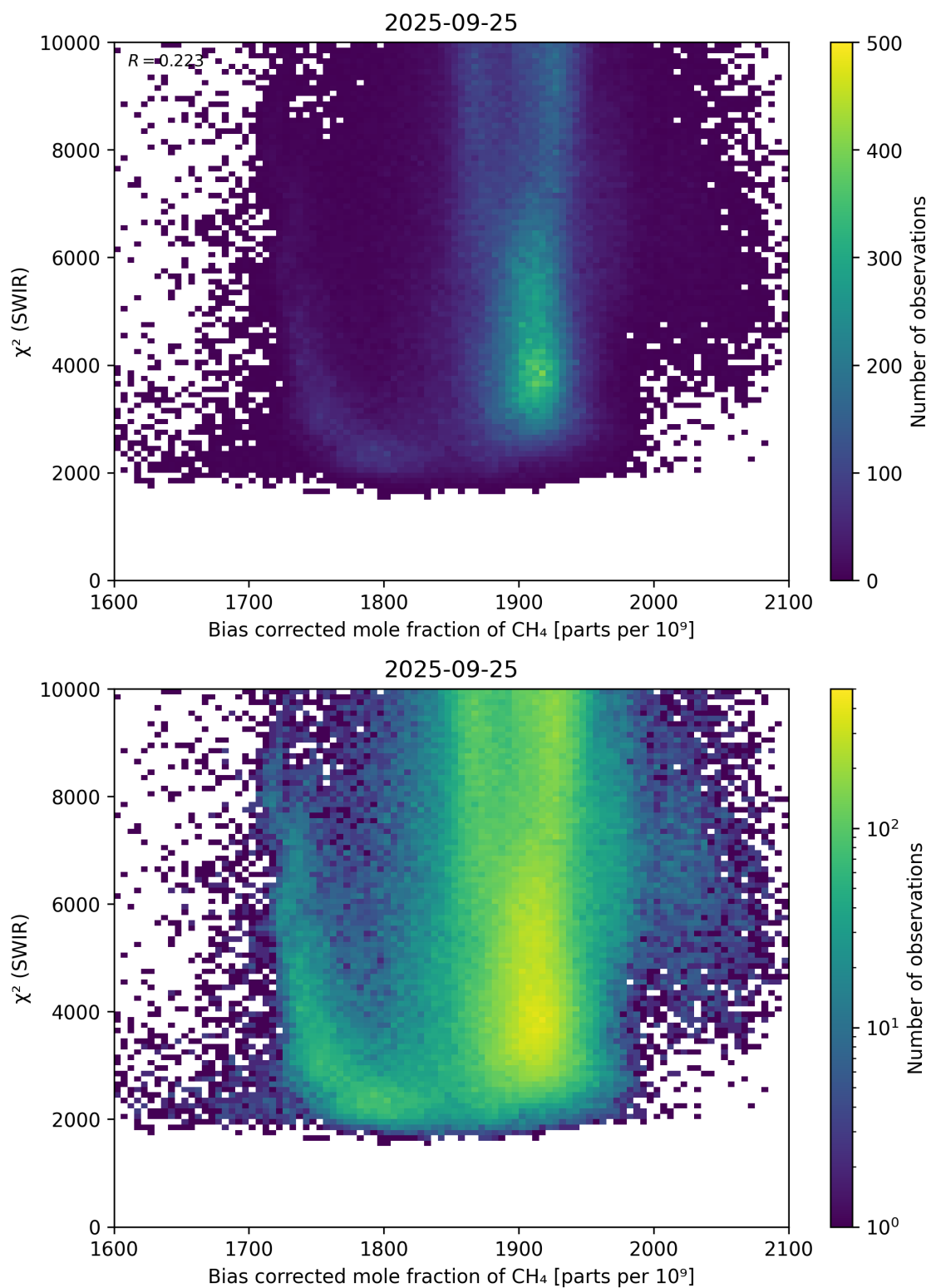
Figure 64: Scatter density plot of “Bias corrected mole fraction of \text{CH}_4 ” against “ \chi^2 (SWIR)” for 2025-09-25 to 2025-09-26.
