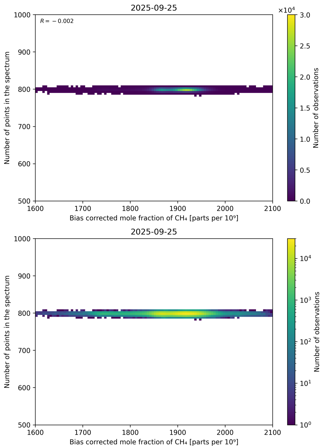
Figure 68: Scatter density plot of “Bias corrected mole fraction of CH 4 ” against “Number of points in the spectrum” for 2025-09-25 to 2025-09-26.
