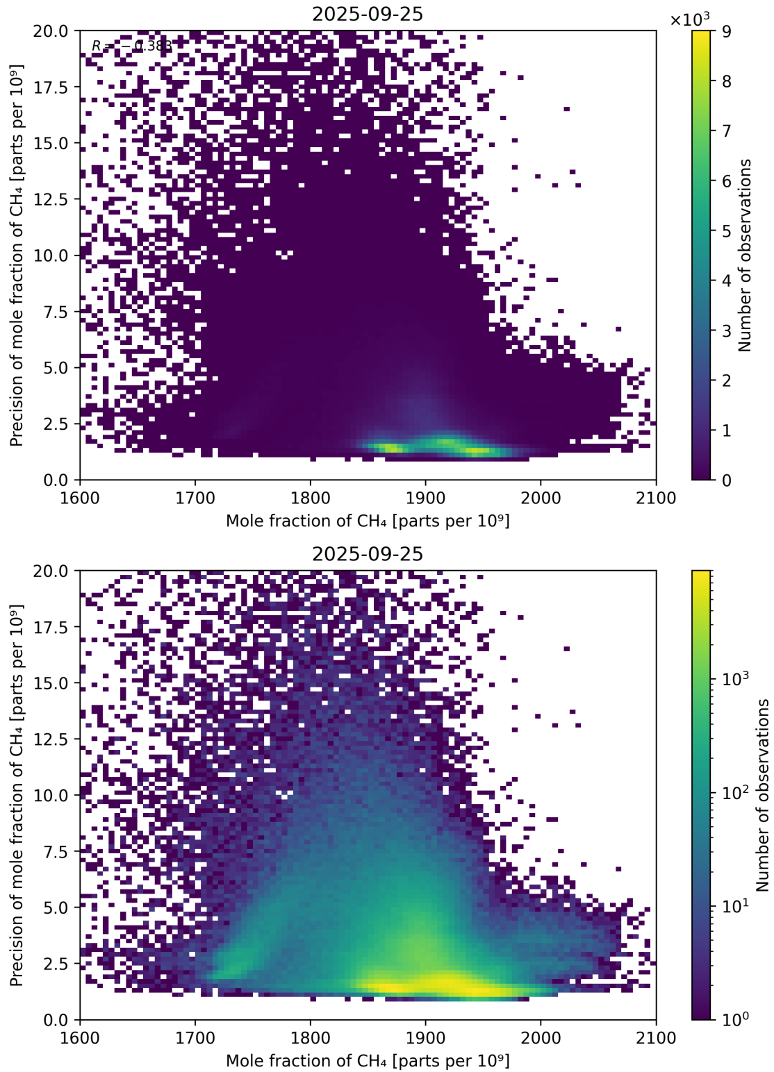
Figure 75: Scatter density plot of “Mole fraction of CH 4 ” against “Precision of mole fraction of CH 4 ” for 2025-09-25 to 2025-09-26.
