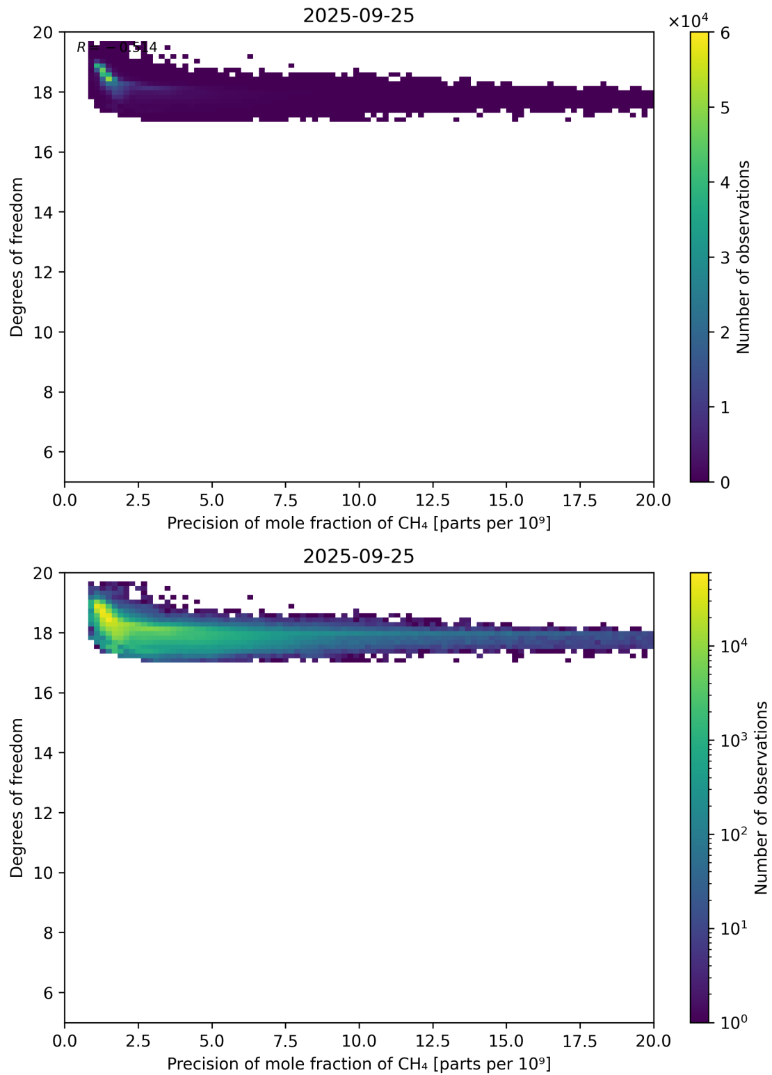
Figure 80: Scatter density plot of “Precision of mole fraction of CH 4 ” against “Degrees of freedom” for 2025-09-25 to 2025-09-26.
