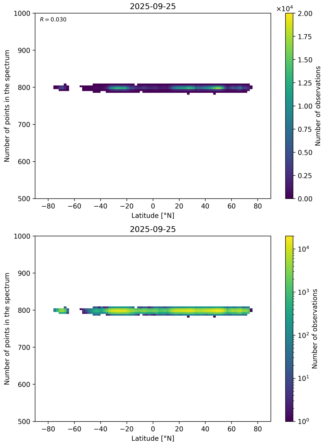
Figure 61: Scatter density plot of “Latitude” against “Number of points in the spectrum” for 2025-09-25 to 2025-09-26.
