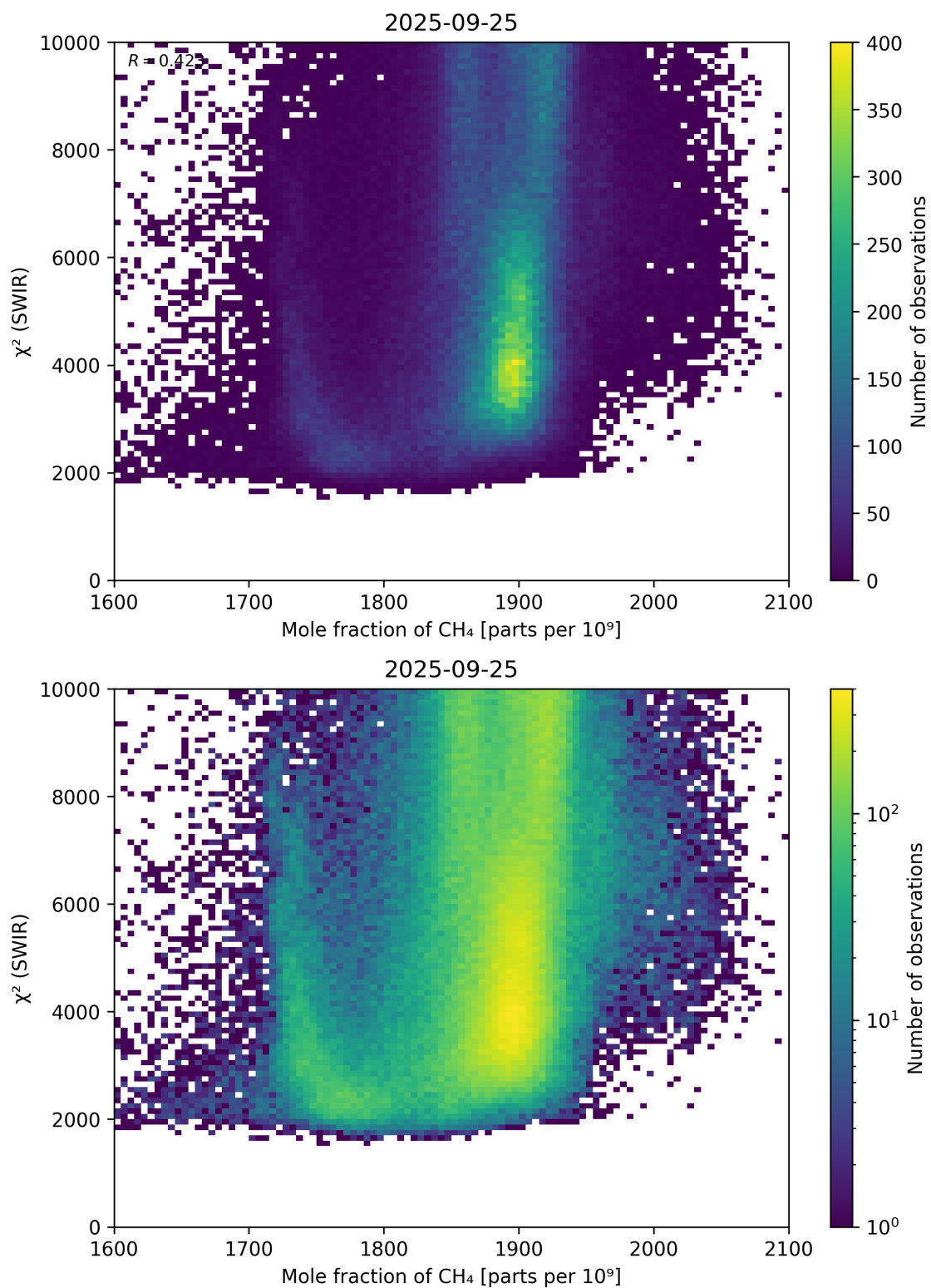
Figure 71: Scatter density plot of “Mole fraction of CH 4 ” against “ \chi^2 (SWIR)” for 2025-09-25 to 2025-09-26.
