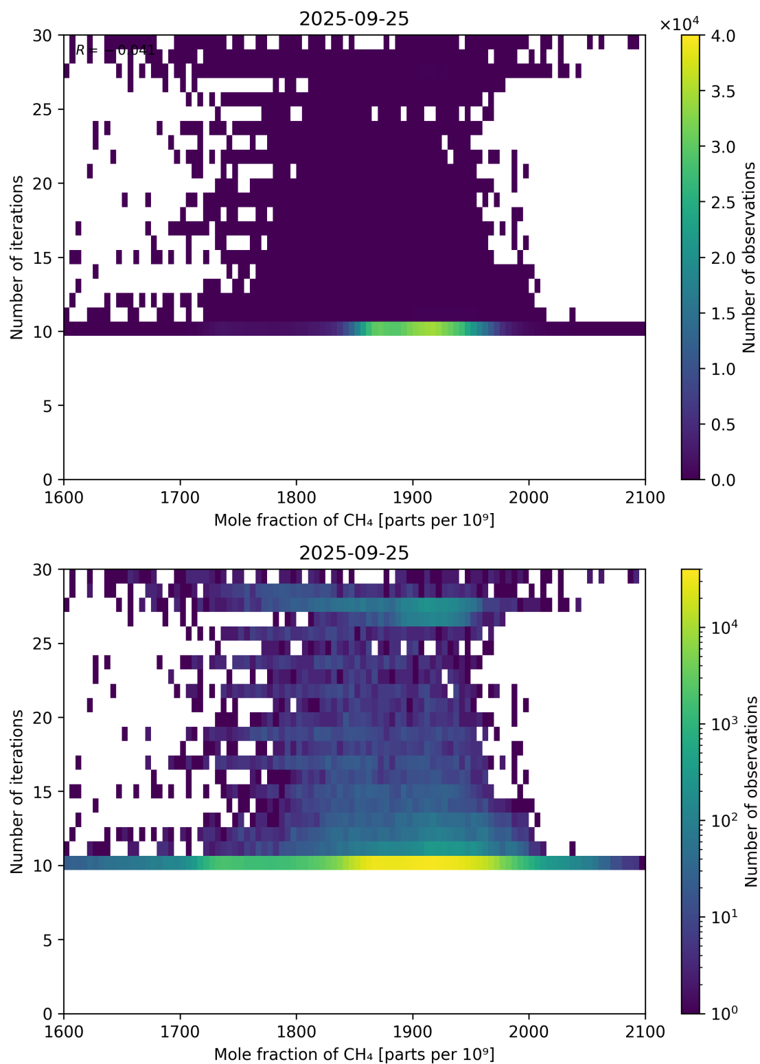
Figure 76: Scatter density plot of “Mole fraction of CH 4 ” against “Number of iterations” for 2025-09-25 to 2025-09-26.
