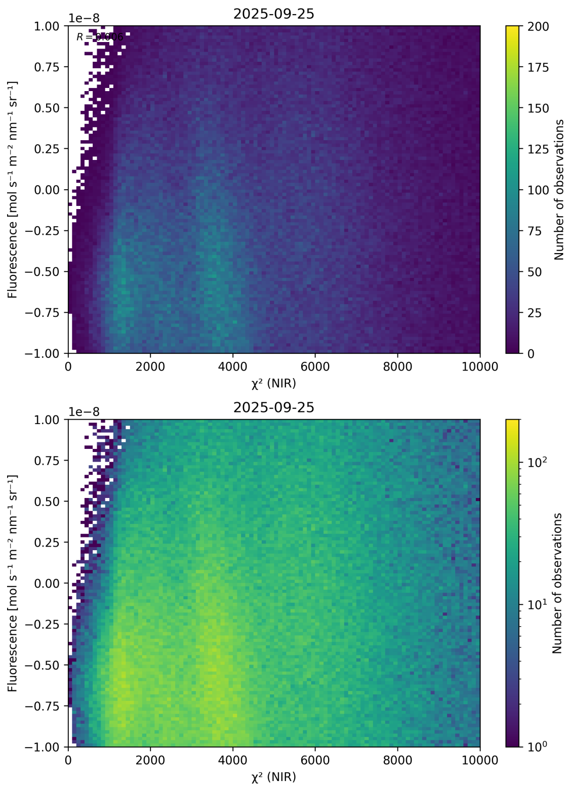
Figure 45: Scatter density plot of “ \chi^2 (NIR)” against “Fluorescence” for 2025-09-25 to 2025-09-26.
