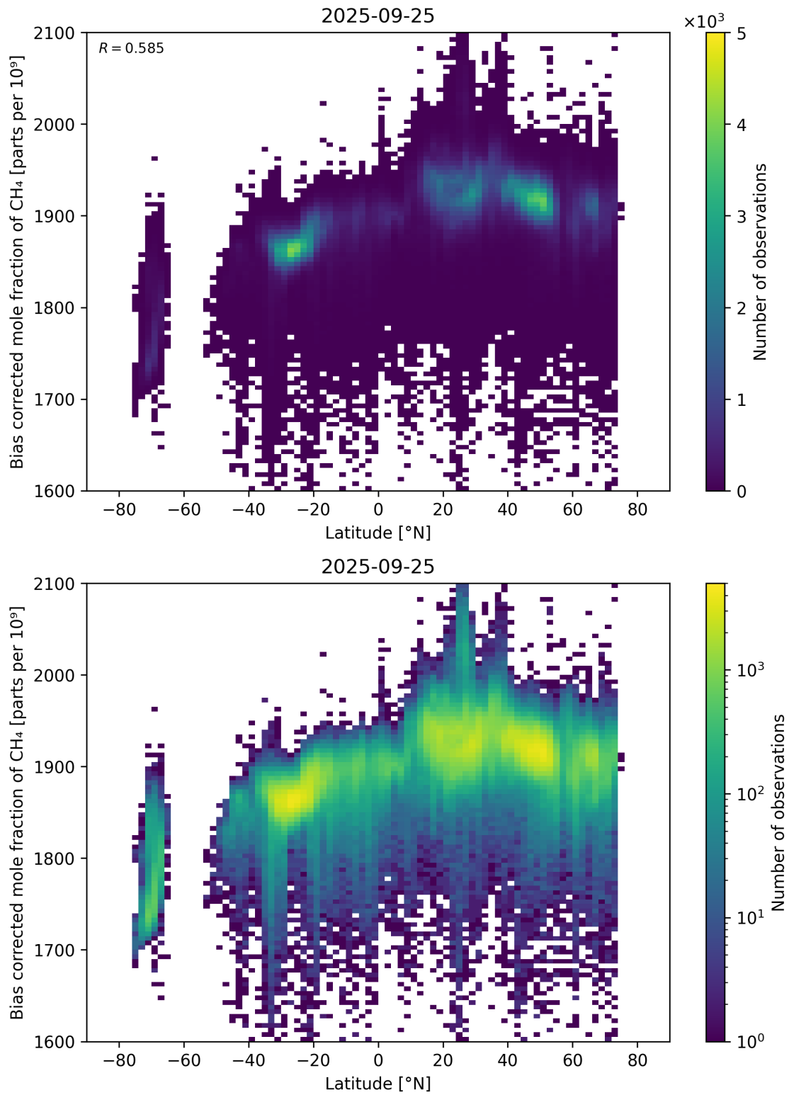
Figure 58: Scatter density plot of “Latitude” against “Bias corrected mole fraction of CH 4 ” for 2025-09-25 to 2025-09-26.
