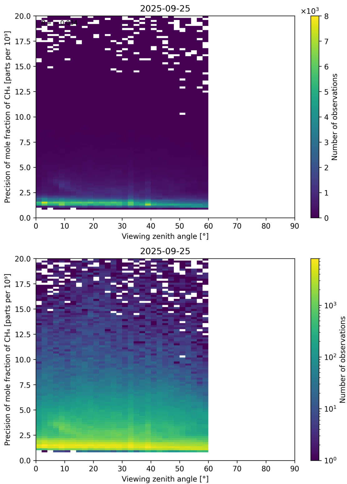
Figure 112: Scatter density plot of “Viewing zenith angle” against “Precision of mole fraction of CH 4 ” for 2025-09-25 to 2025-09-26.
