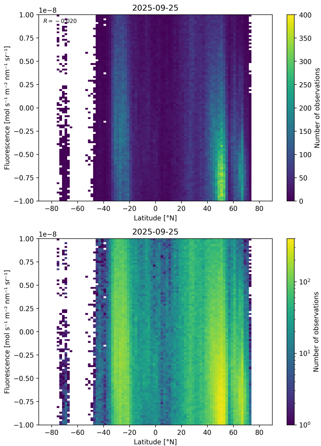
Figure 56: Scatter density plot of “Latitude” against “Fluorescence” for 2025-09-25 to 2025-09-26.
