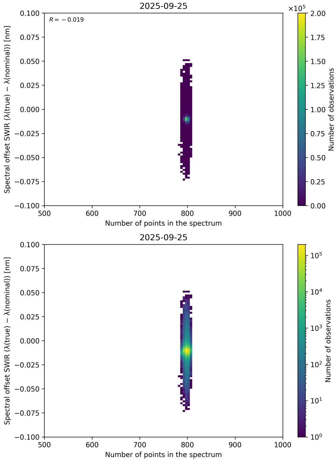
Figure 93: Scatter density plot of “Number of points in the spectrum” against “Spectral offset SWIR ( \lambda_{\text{true}} - \lambda_{\text{nominal}} )” for 2025-09-25 to 2025-09-26.
