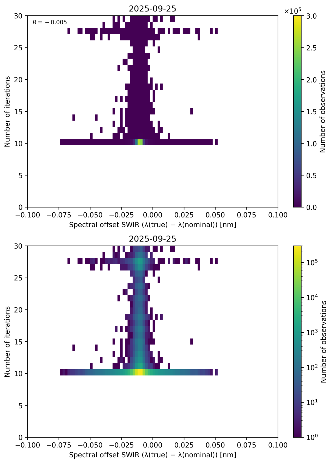
Figure 121: Scatter density plot of “Spectral offset SWIR ( \lambda_{\text{true}} - \lambda_{\text{nominal}} )” against “Number of iterations” for 2025-09-25 to 2025-09-26.
