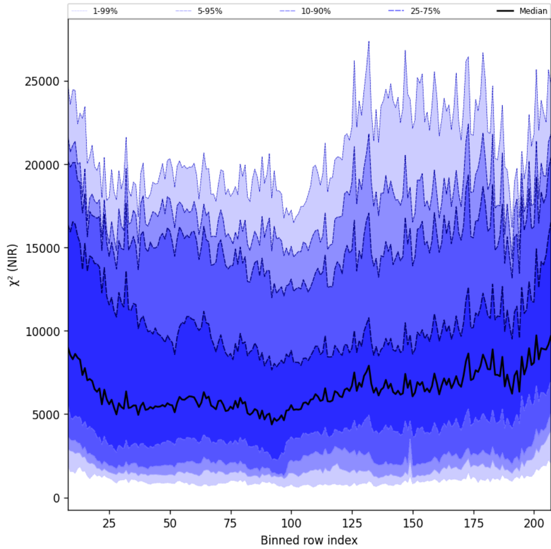
Figure 40: Along track statistics of “ \chi^2 (NIR)” for 2025-09-25 to 2025-09-26
