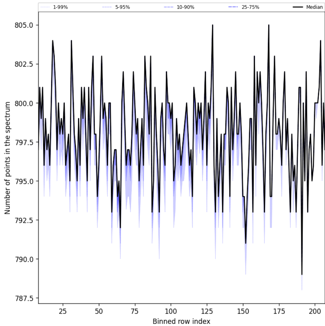
Figure 37: Along track statistics of “Number of points in the spectrum” for 2025-09-25 to 2025-09-26
