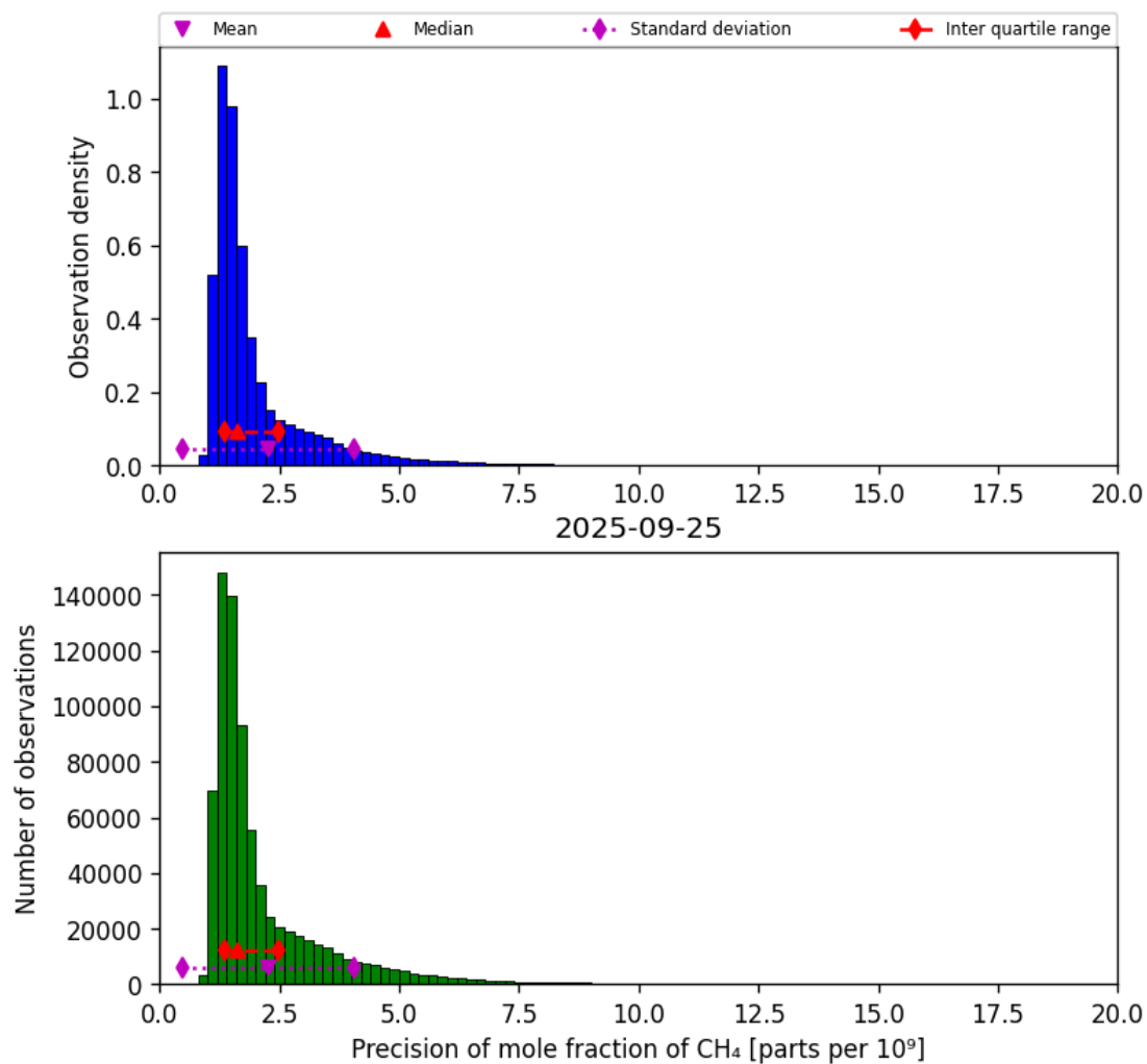
Figure 24: Histogram of “Precision of mole fraction of CH 4 ” for 2025-09-25 to 2025-09-26
