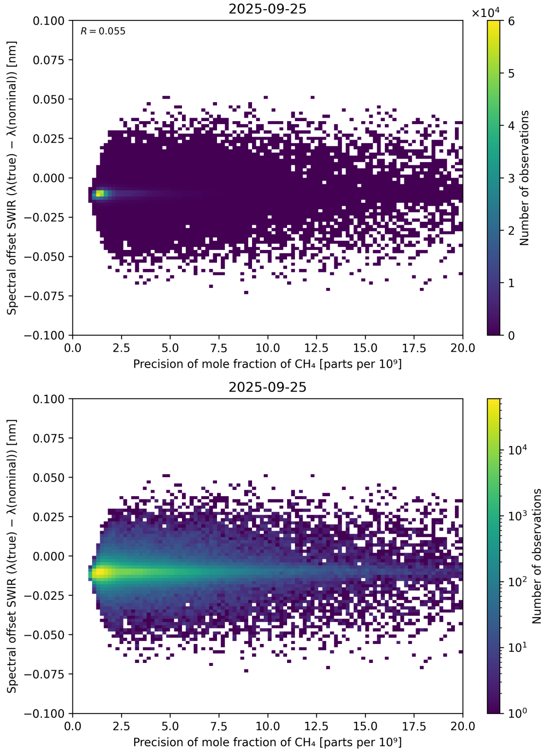
Figure 85: Scatter density plot of “Precision of mole fraction of CH 4 ” against “Spectral offset SWIR ( \lambda_{\text{true}} - \lambda_{\text{nominal}} )” for 2025-09-25 to 2025-09-26.
