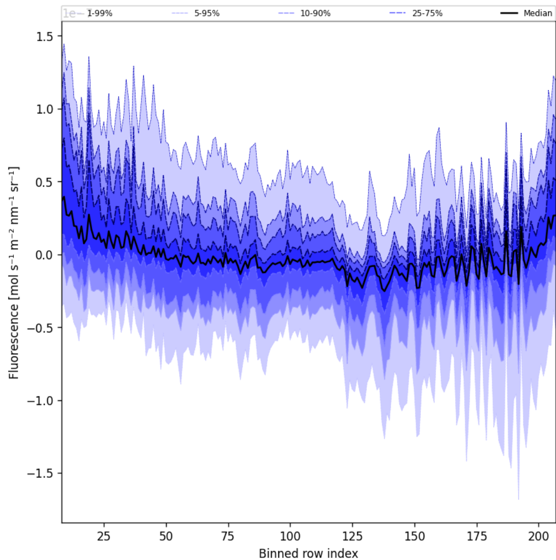
Figure 43: Along track statistics of “Fluorescence” for 2025-09-25 to 2025-09-26
