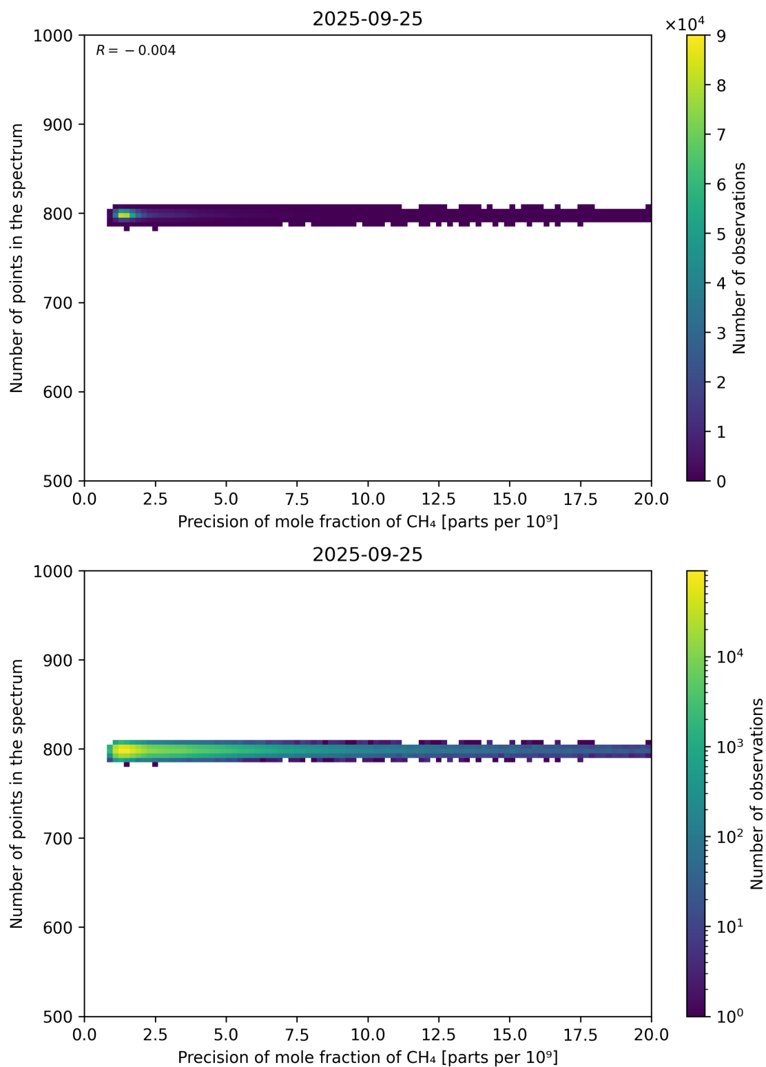
Figure 84: Scatter density plot of “Precision of mole fraction of CH 4 ” against “Number of points in the spectrum” for 2025-09-25 to 2025-09-26.
