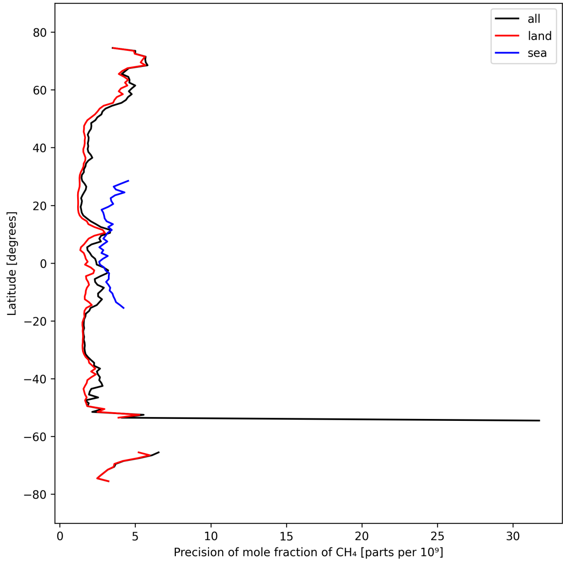
Figure 13: Zonal average of “Precision of mole fraction of CH 4 ” for 2025-09-25 to 2025-09-26.
