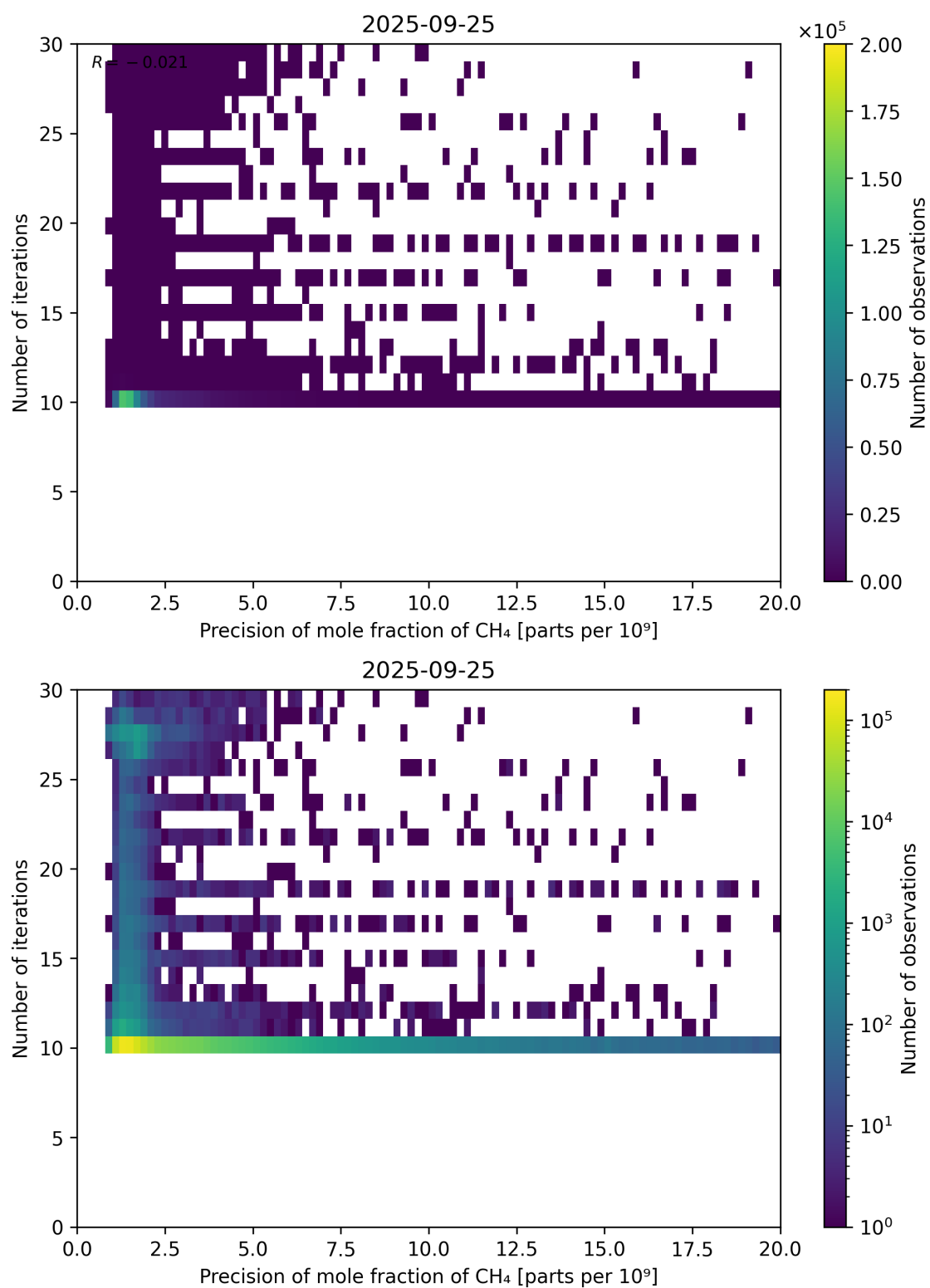
Figure 83: Scatter density plot of “Precision of mole fraction of CH 4 ” against “Number of iterations” for 2025-09-25 to 2025-09-26.
