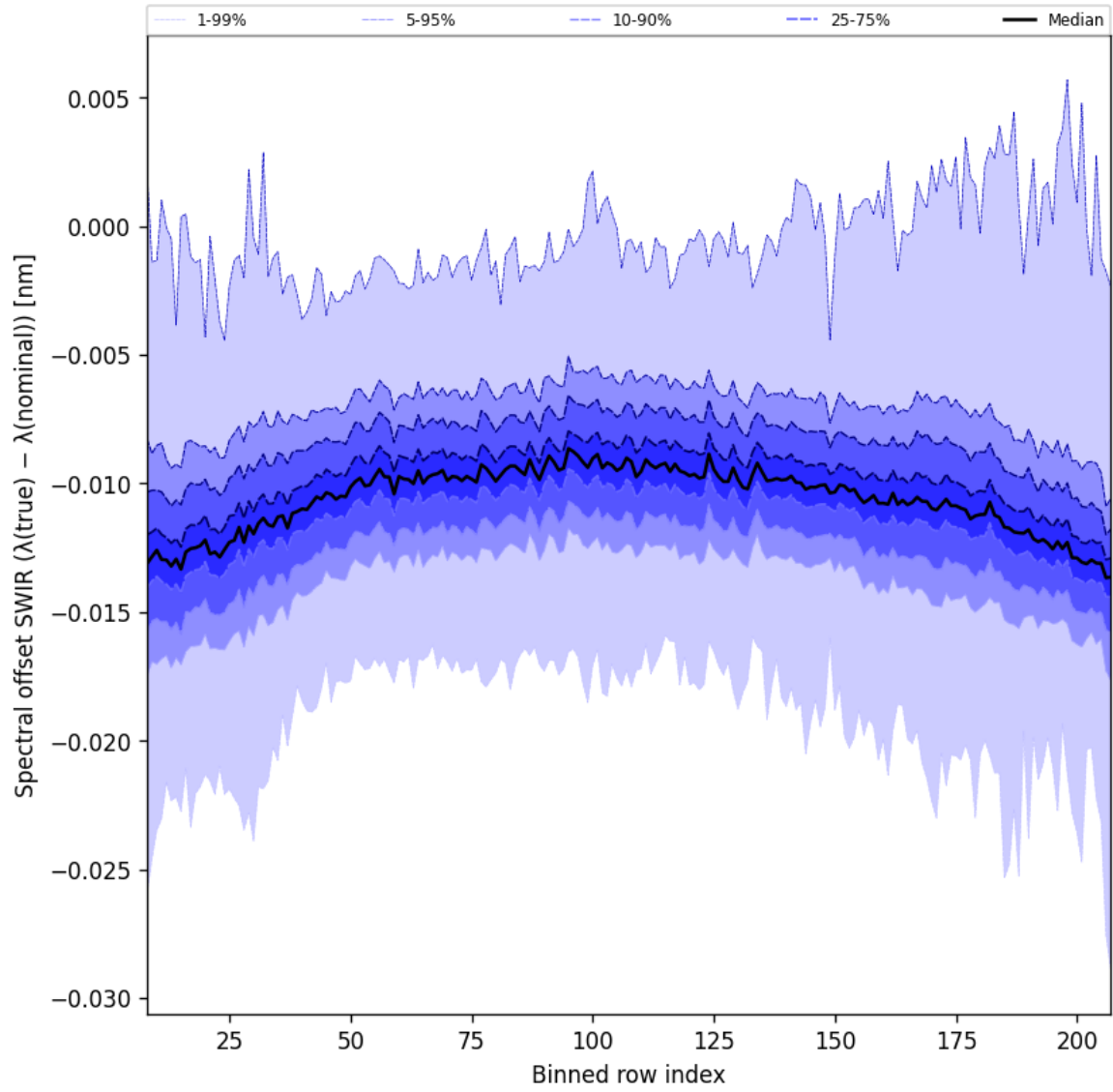
Figure 38: Along track statistics of “Spectral offset SWIR ( \lambda_{\text{true}} - \lambda_{\text{nominal}} )” for 2025-09-25 to 2025-09-26
