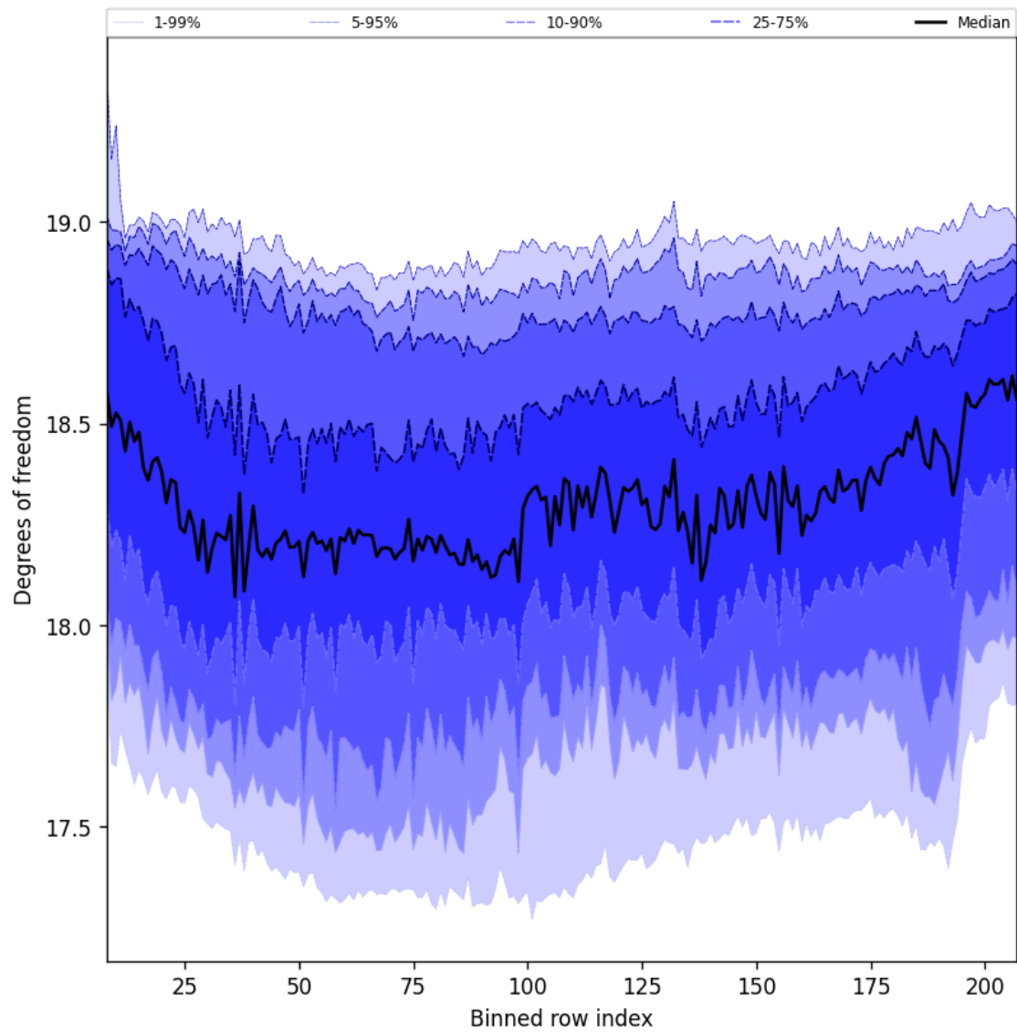
Figure 41: Along track statistics of “Degrees of freedom” for 2025-09-25 to 2025-09-26
