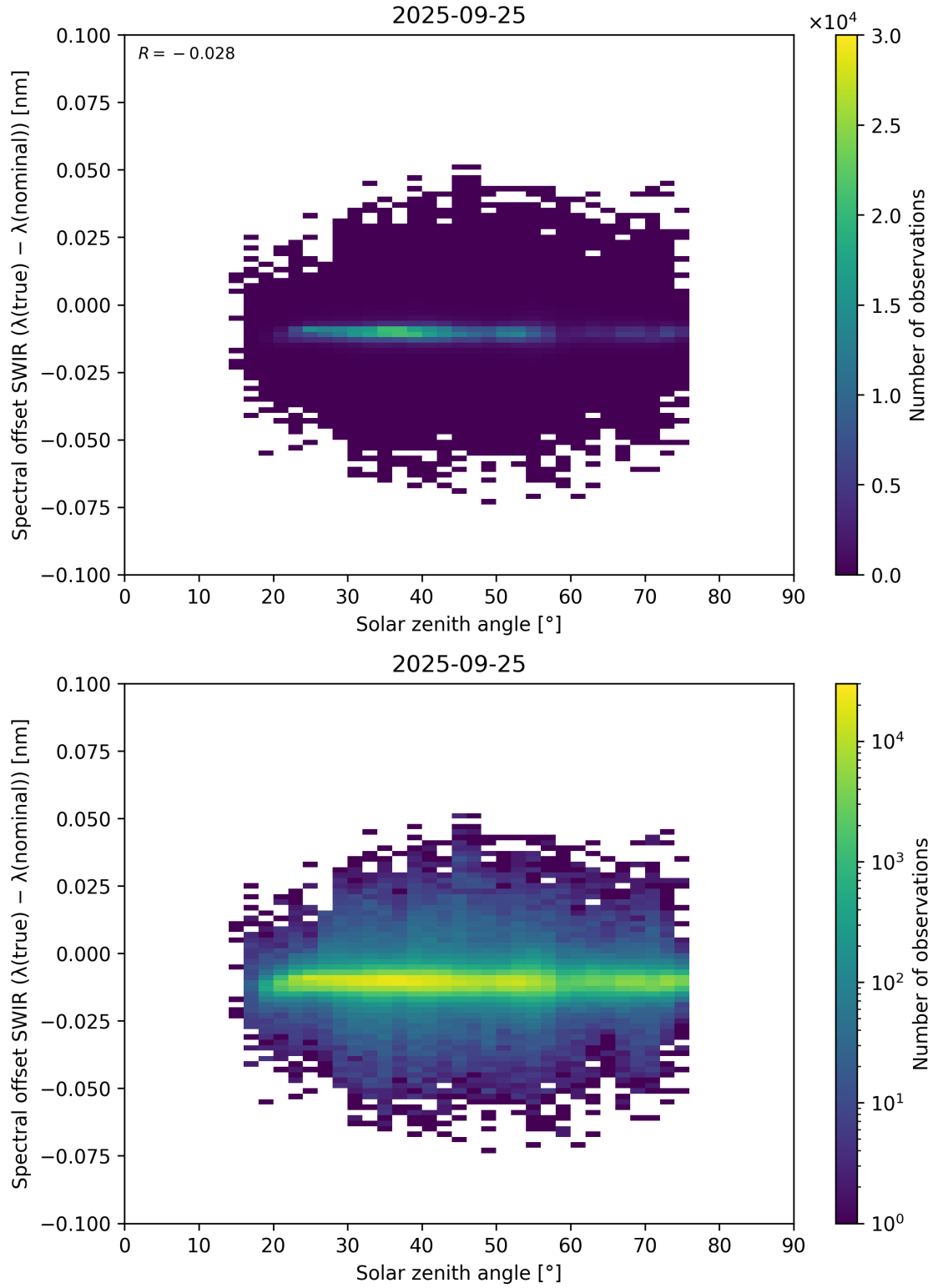
Figure 104: Scatter density plot of “Solar zenith angle” against “Spectral offset SWIR ( \lambda_{\text{true}} - \lambda_{\text{nominal}} )” for 2025-09-25 to 2025-09-26.
