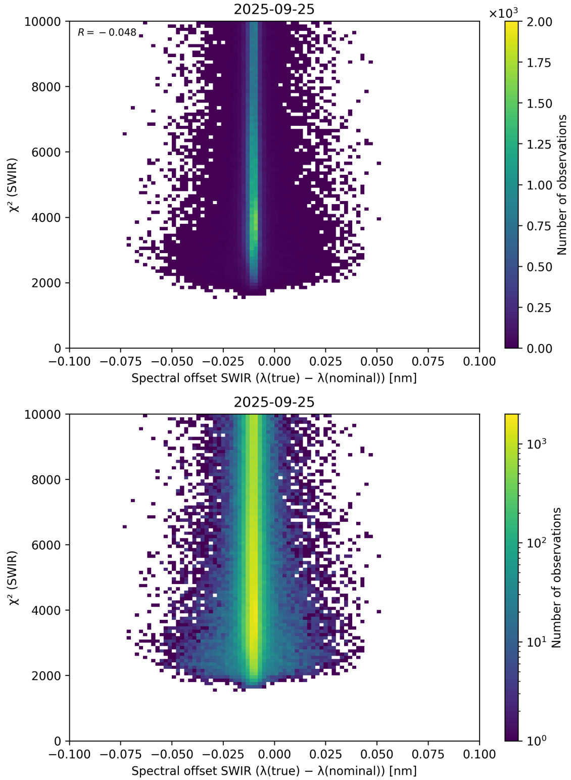
Figure 118: Scatter density plot of “Spectral offset SWIR ( \lambda_{\text{true}} - \lambda_{\text{nominal}} )” against “ \chi^2 (SWIR)” for 2025-09-25 to 2025-09-26.
