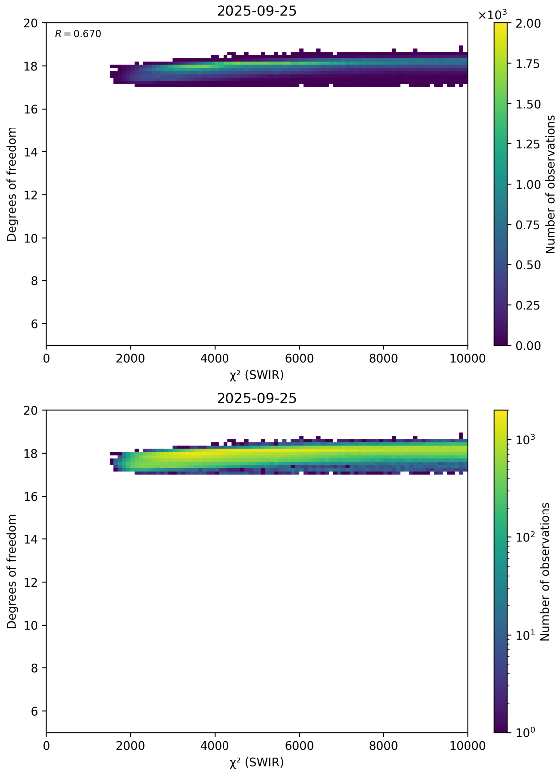
Figure 48: Scatter density plot of “ \chi^2 (SWIR)” against “Degrees of freedom” for 2025-09-25 to 2025-09-26.
