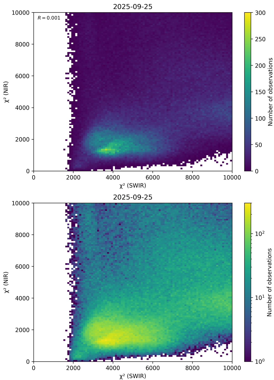
Figure 47: Scatter density plot of “ \chi^2 (SWIR)” against “ \chi^2 (NIR)” for 2025-09-25 to 2025-09-26.
