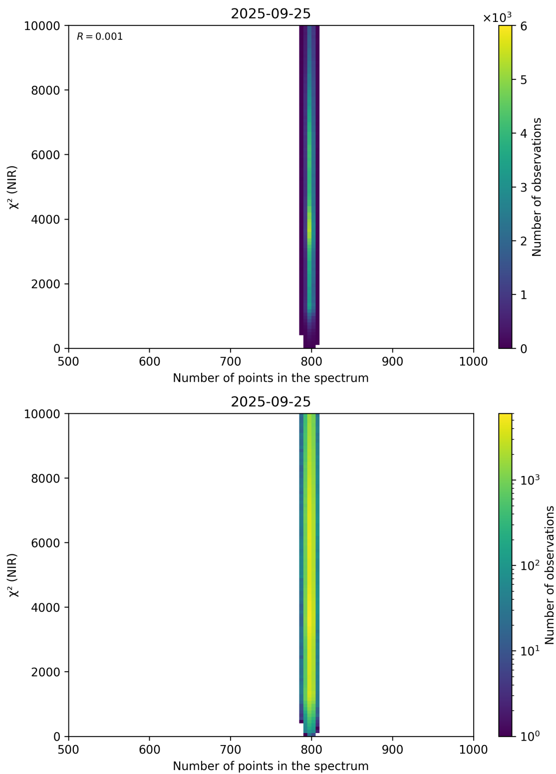
Figure 88: Scatter density plot of “Number of points in the spectrum” against “ \chi^2 (NIR)” for 2025-09-25 to 2025-09-26.
