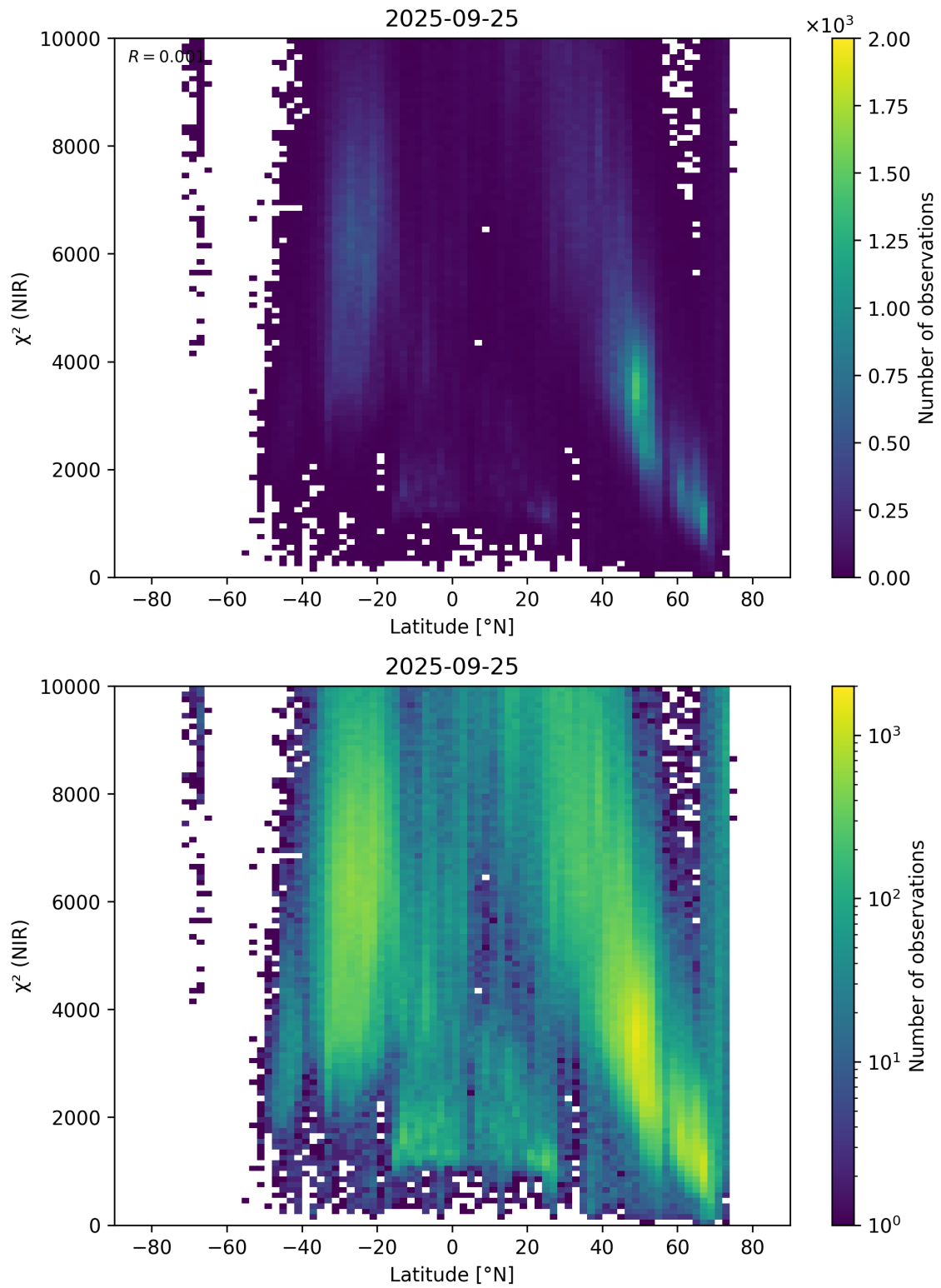
Figure 53: Scatter density plot of “Latitude” against “ \chi^2 (NIR)” for 2025-09-25 to 2025-09-26.
