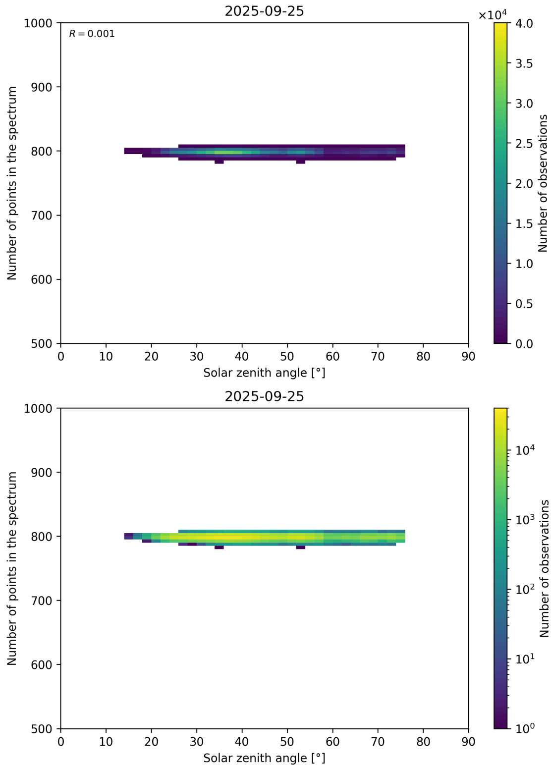
Figure 103: Scatter density plot of “Solar zenith angle” against “Number of points in the spectrum” for 2025-09-25 to 2025-09-26.
