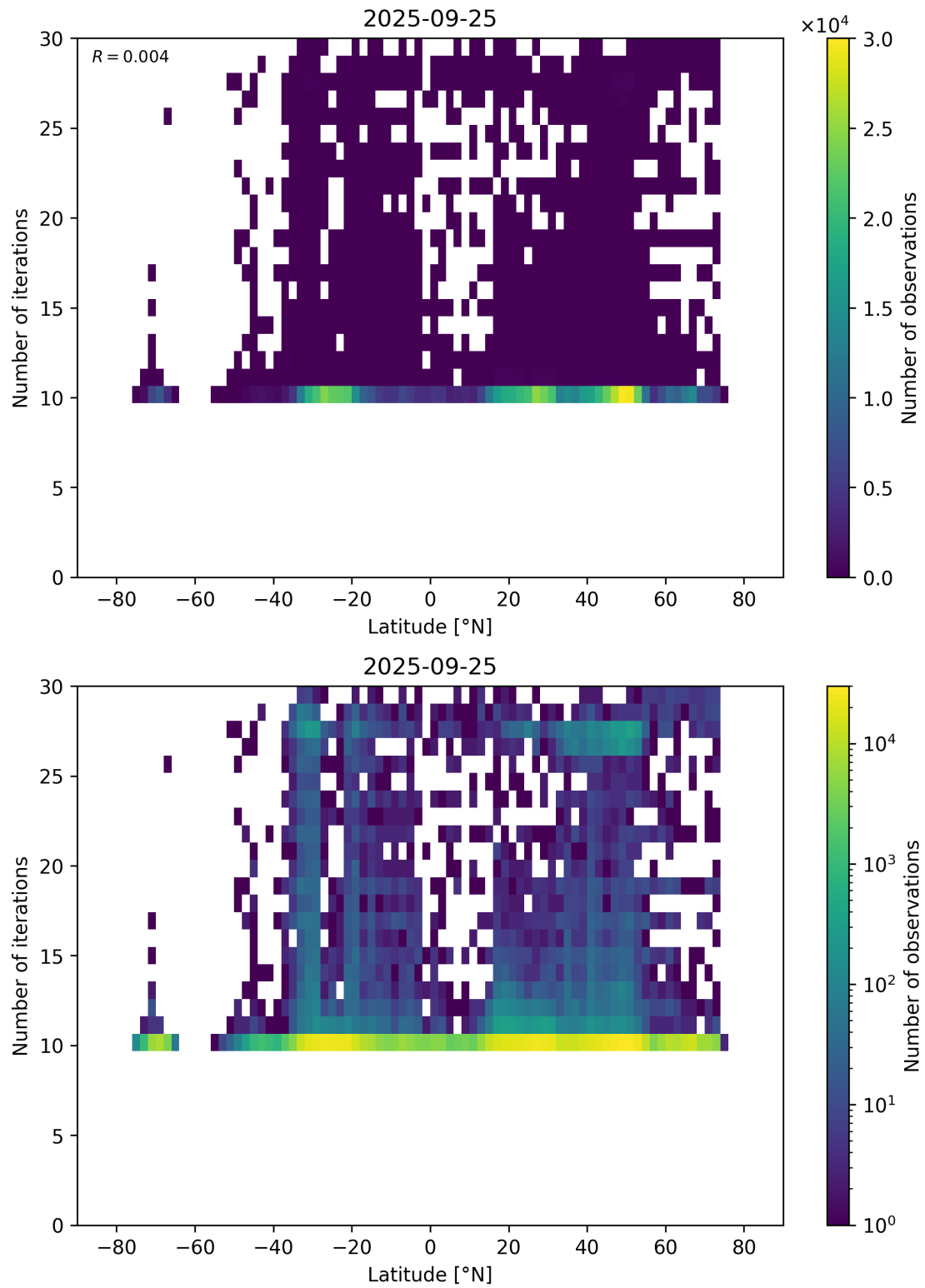
Figure 60: Scatter density plot of “Latitude” against “Number of iterations” for 2025-09-25 to 2025-09-26.
