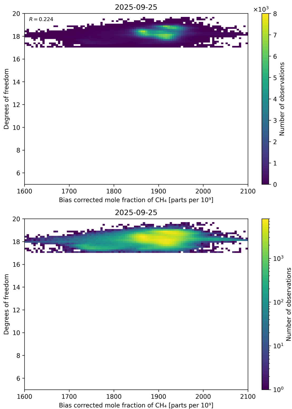
Figure 65: Scatter density plot of “Bias corrected mole fraction of CH 4 ” against “Degrees of freedom” for 2025-09-25 to 2025-09-26.
