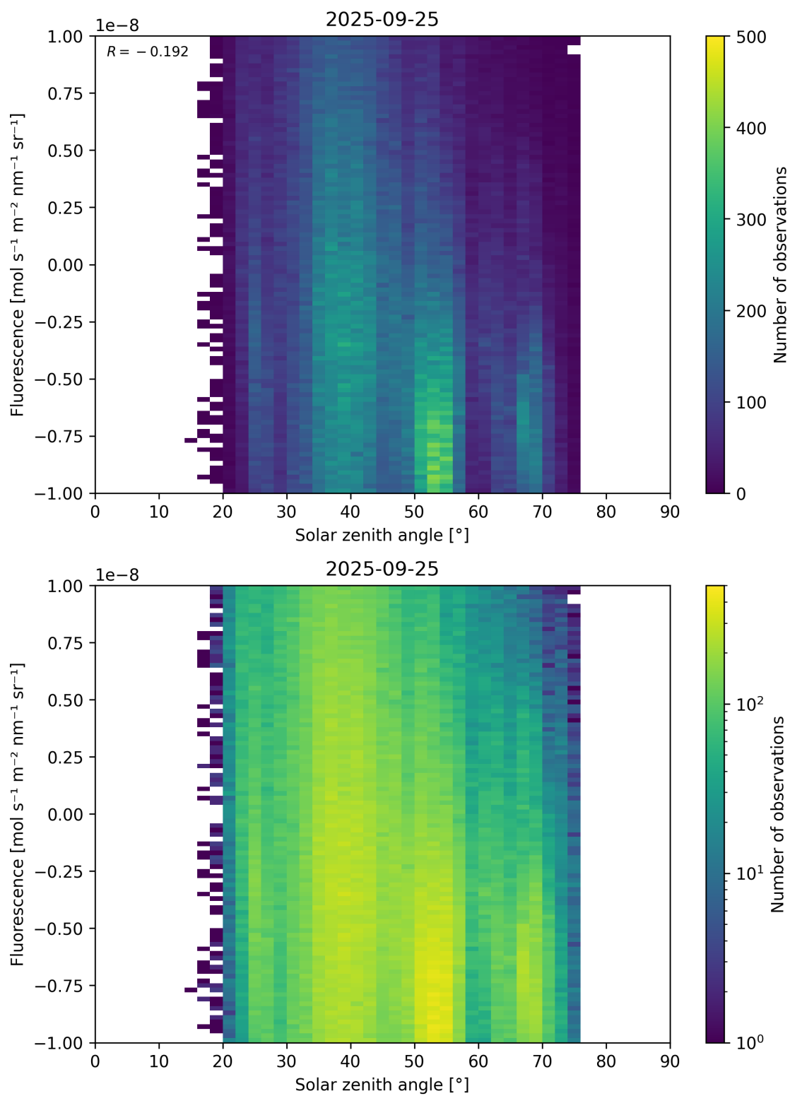
Figure 97: Scatter density plot of “Solar zenith angle” against “Fluorescence” for 2025-09-25 to 2025-09-26.
