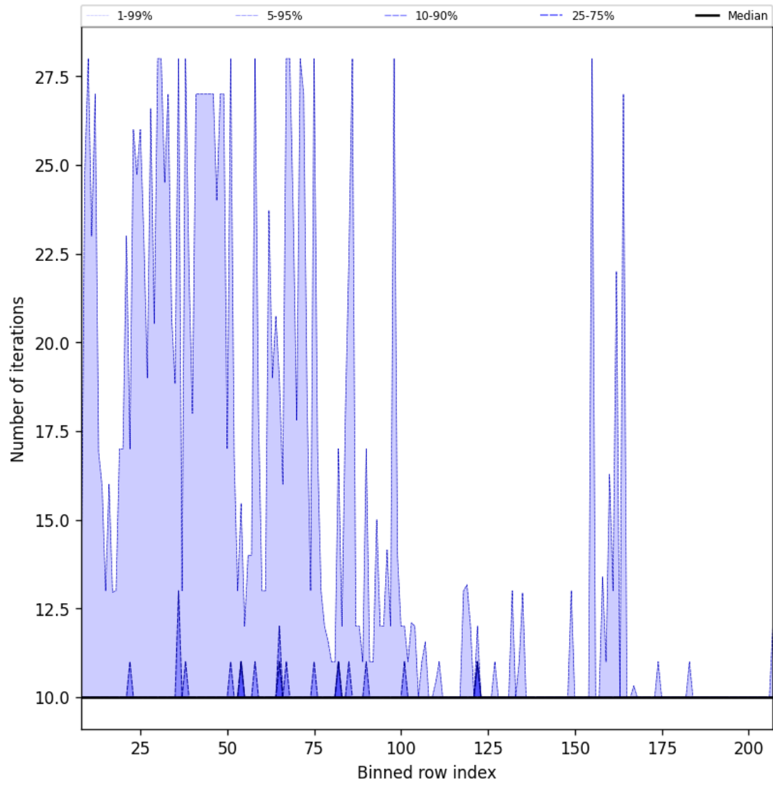
Figure 42: Along track statistics of “Number of iterations” for 2025-09-25 to 2025-09-26
