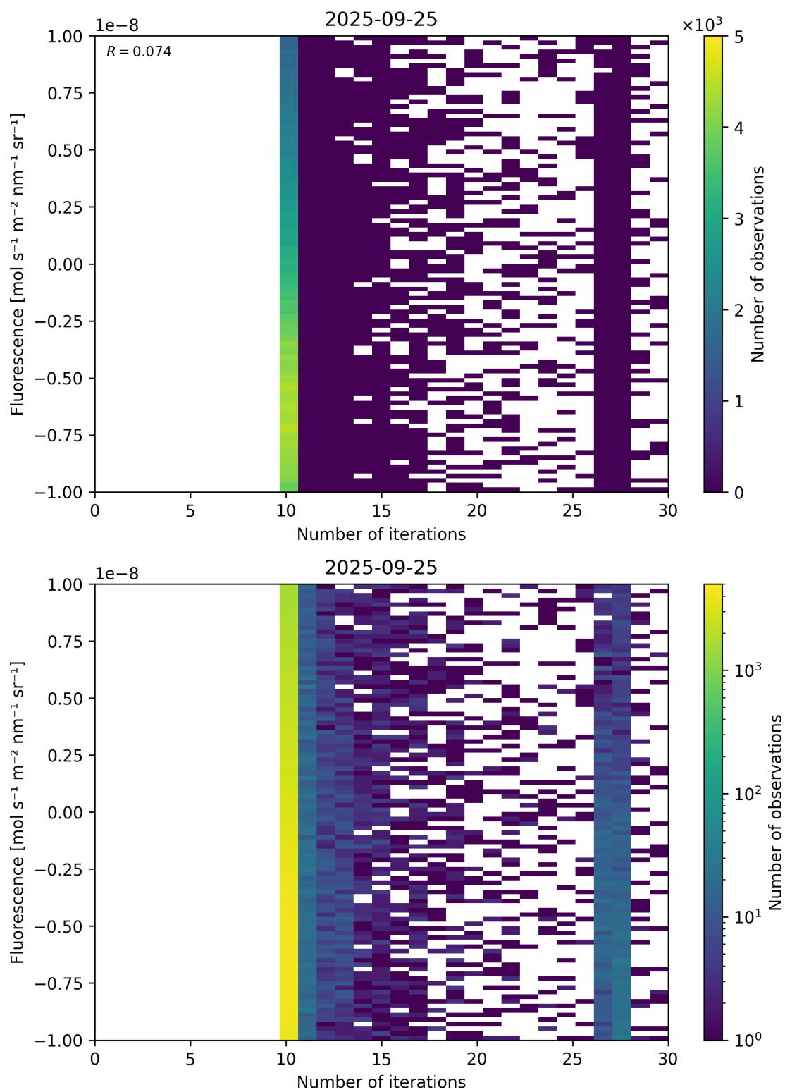
Figure 87: Scatter density plot of “Number of iterations” against “Fluorescence” for 2025-09-25 to 2025-09-26.
