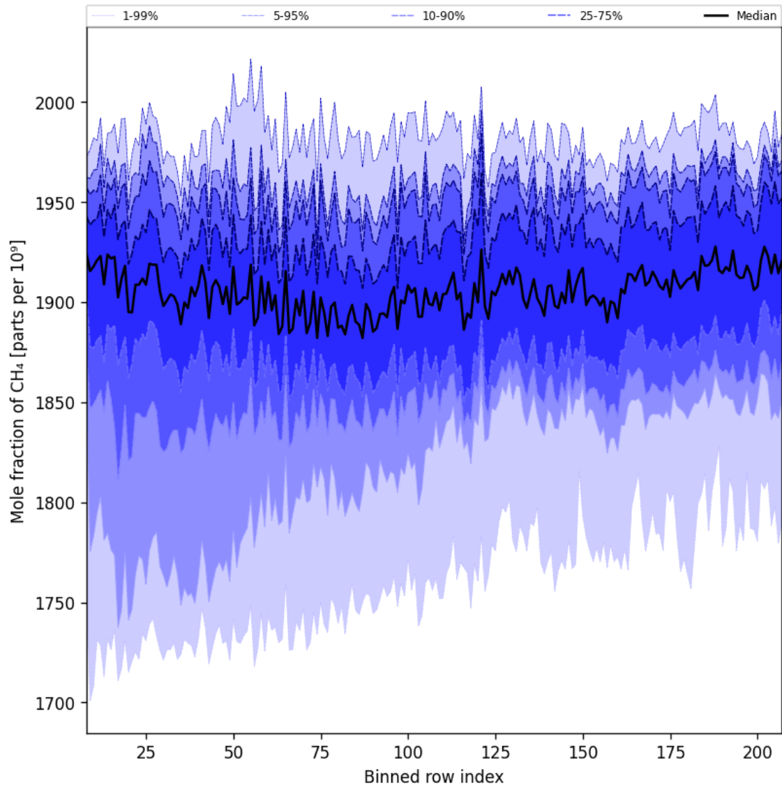
Figure 34: Along track statistics of “Mole fraction of CH 4 ” for 2025-09-25 to 2025-09-26
