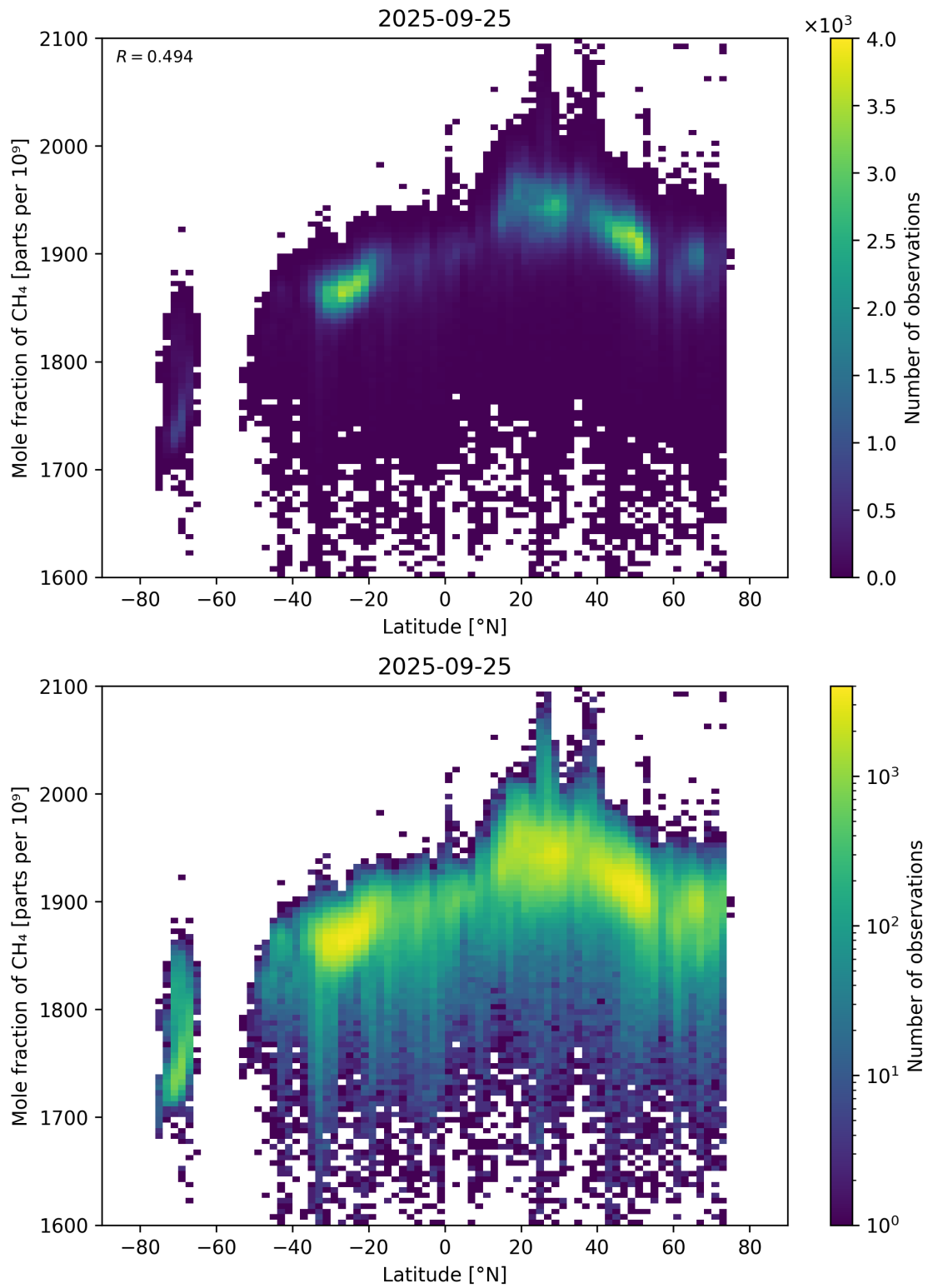
Figure 57: Scatter density plot of “Latitude” against “Mole fraction of \text{CH}_4 ” for 2025-09-25 to 2025-09-26.
