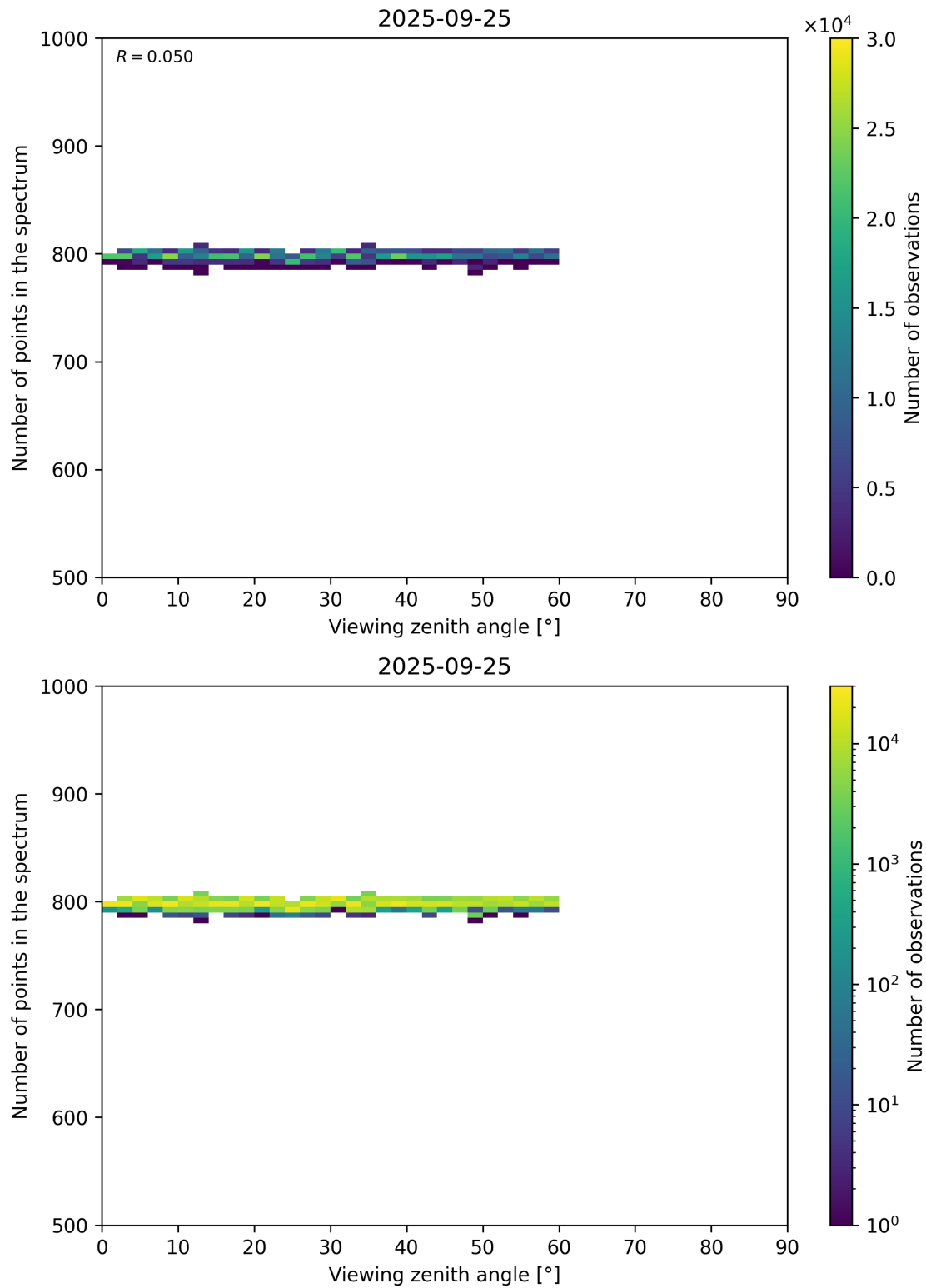
Figure 114: Scatter density plot of “Viewing zenith angle” against “Number of points in the spectrum” for 2025-09-25 to 2025-09-26.
