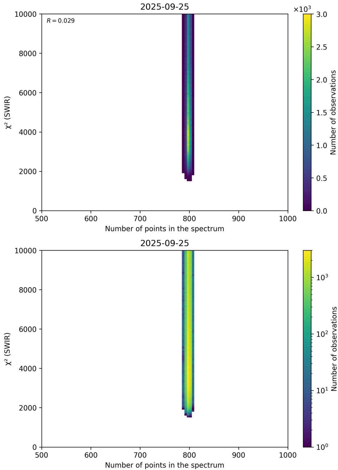
Figure 89: Scatter density plot of “Number of points in the spectrum” against “ \chi^2 (SWIR)” for 2025-09-25 to 2025-09-26.
