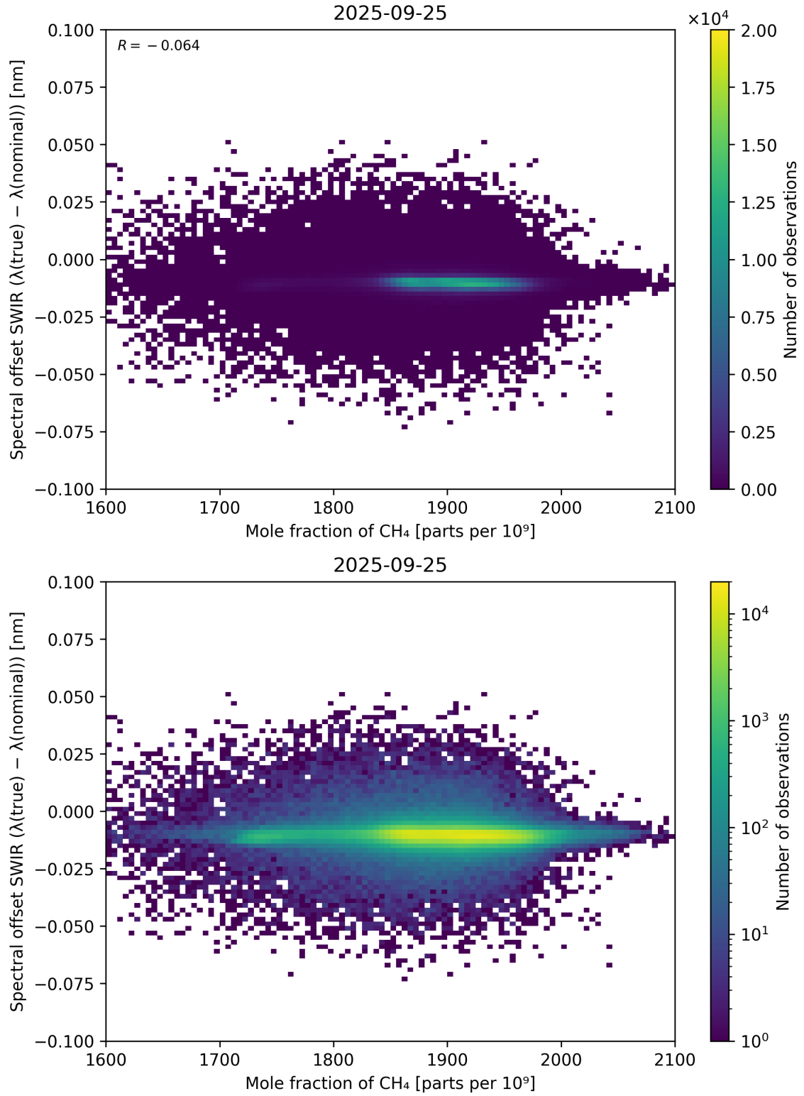
Figure 86: Scatter density plot of “Mole fraction of CH 4 ” against “Spectral offset SWIR ( \lambda_{\text{true}} - \lambda_{\text{nominal}} )” for 2025-09-25 to 2025-09-26.
