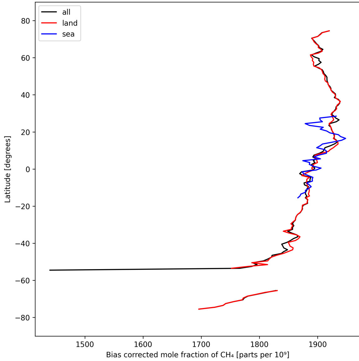
Figure 14: Zonal average of “Bias corrected mole fraction of CH 4 ” for 2025-09-25 to 2025-09-26.
