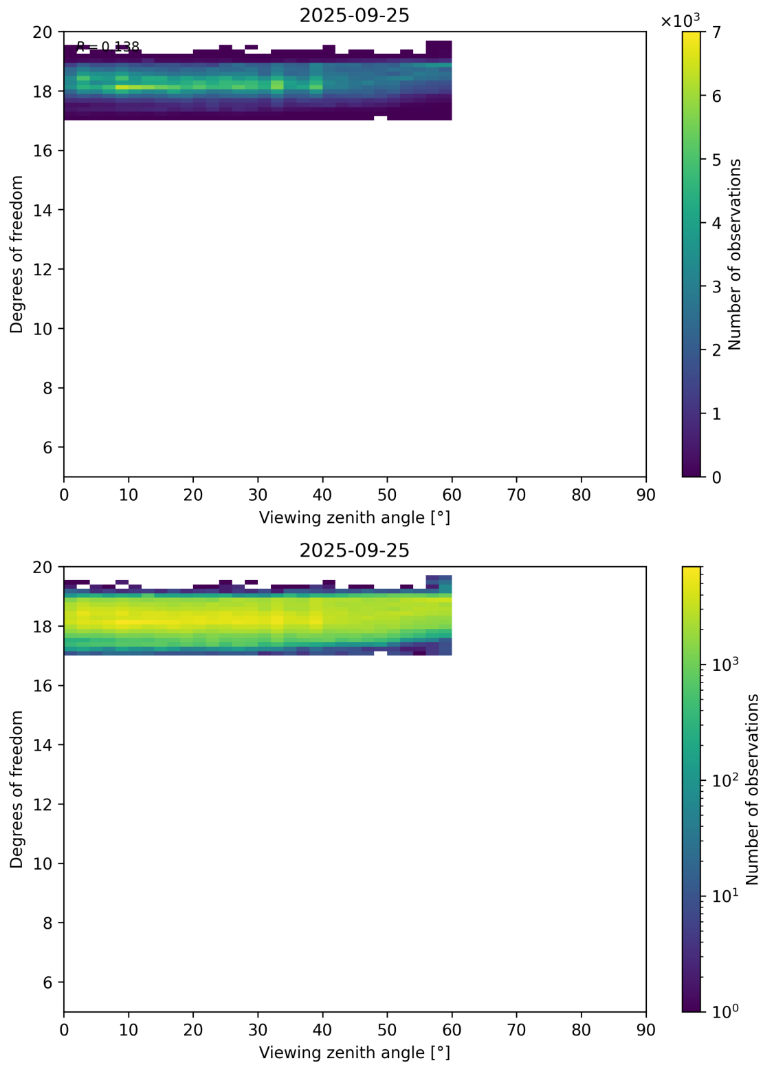
Figure 107: Scatter density plot of “Viewing zenith angle” against “Degrees of freedom” for 2025-09-25 to 2025-09-26.
