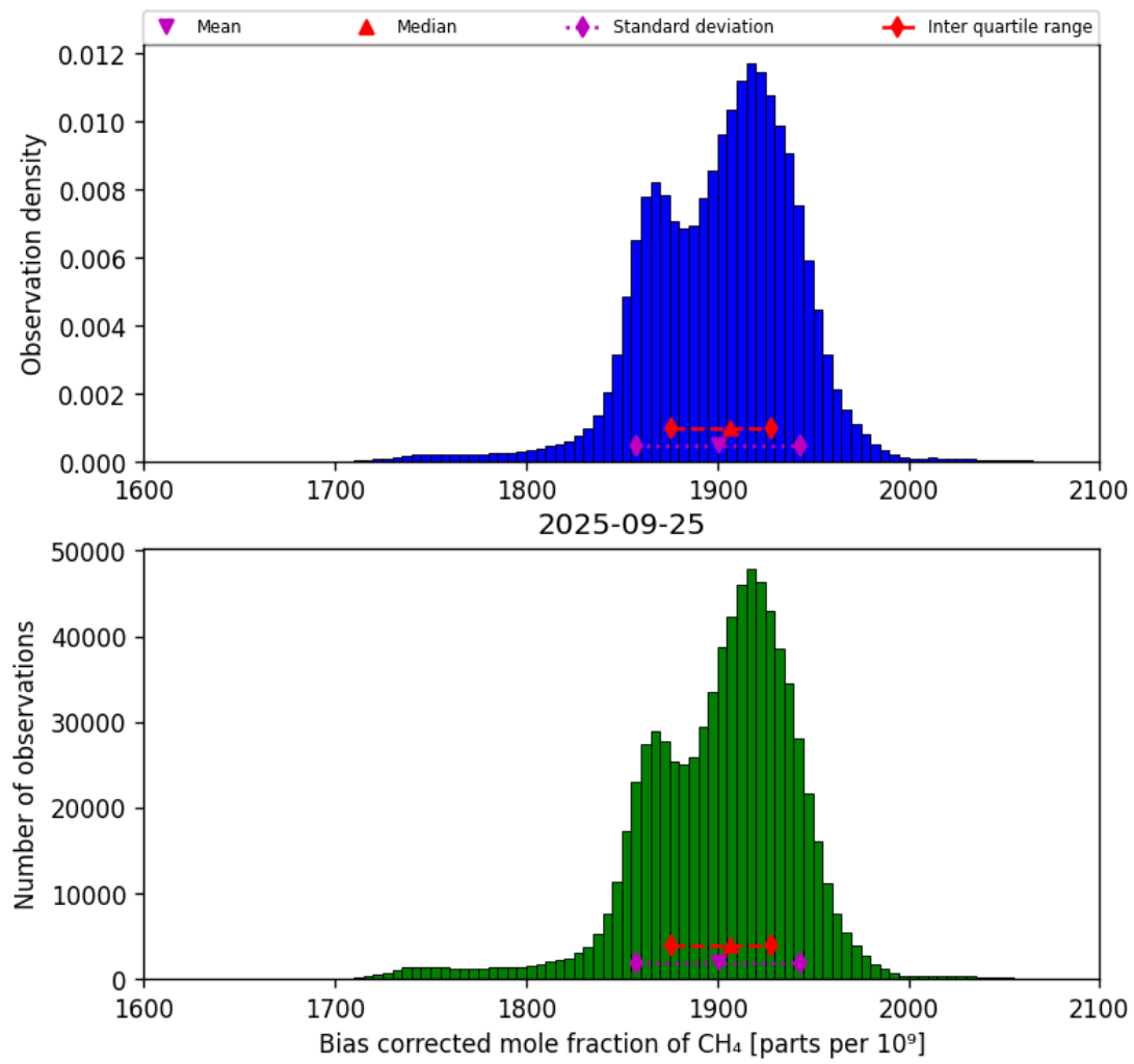
Figure 25: Histogram of “Bias corrected mole fraction of CH 4 ” for 2025-09-25 to 2025-09-26
