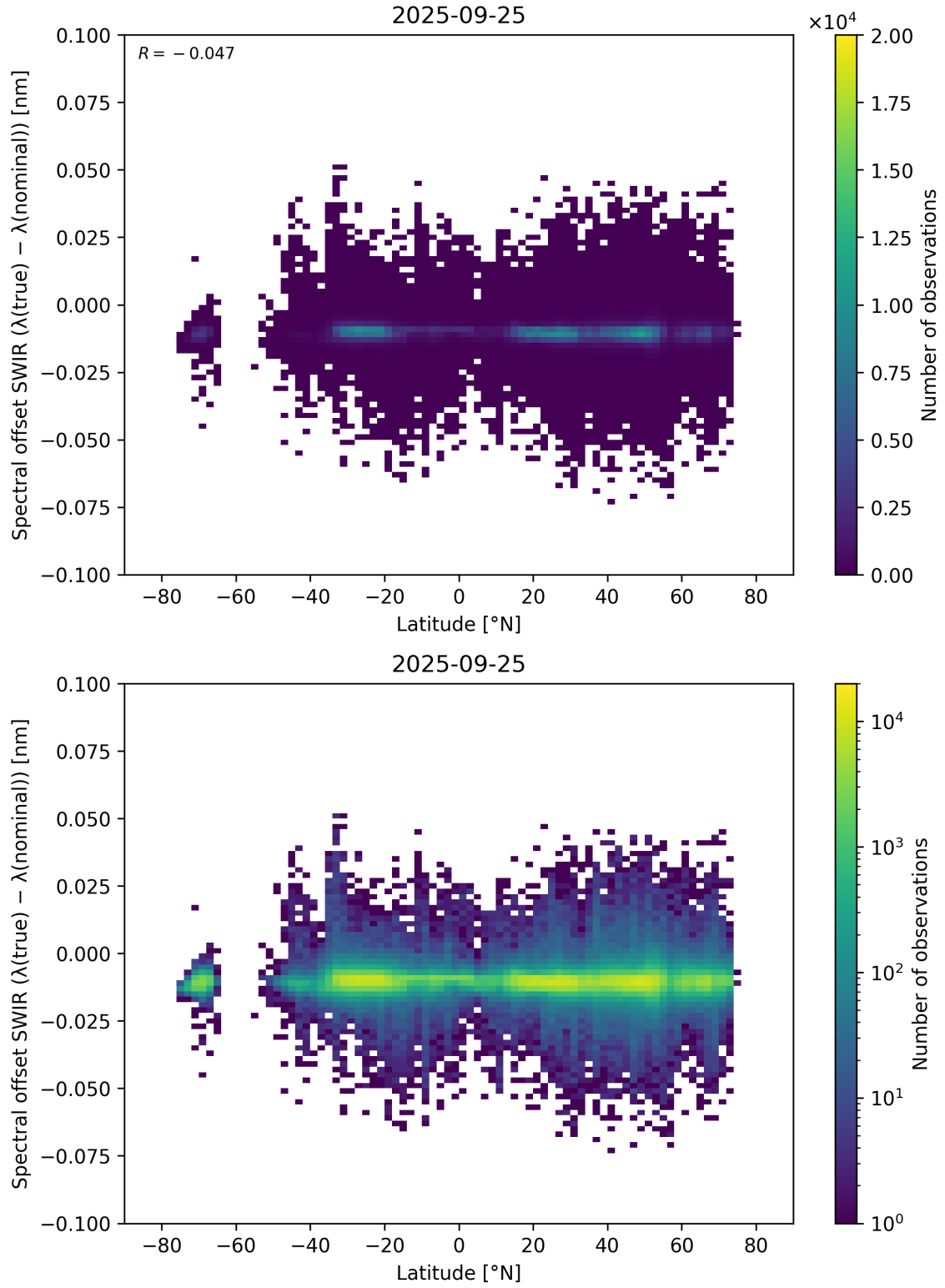
Figure 62: Scatter density plot of “Latitude” against “Spectral offset SWIR ( \lambda_{\text{true}} - \lambda_{\text{nominal}} )” for 2025-09-25 to 2025-09-26.
