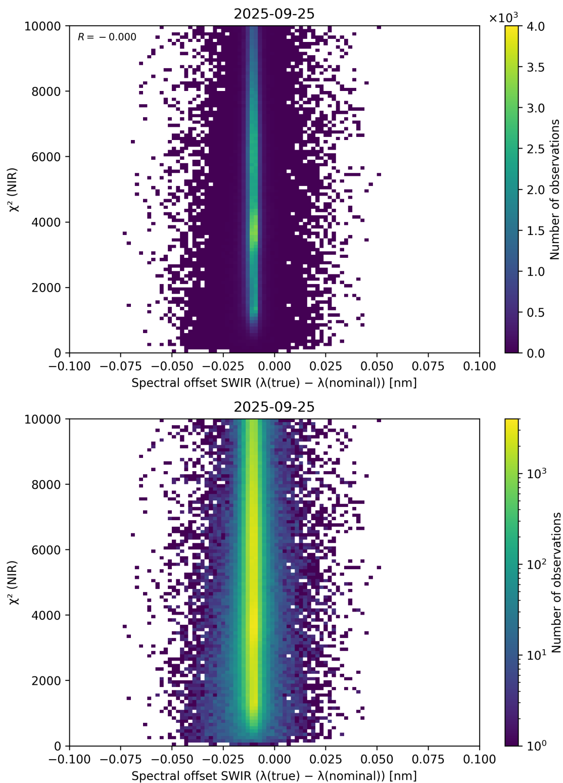
Figure 117: Scatter density plot of “Spectral offset SWIR ( \lambda_{\text{true}} - \lambda_{\text{nominal}} )” against “ \chi^2 (NIR)” for 2025-09-25 to 2025-09-26.
