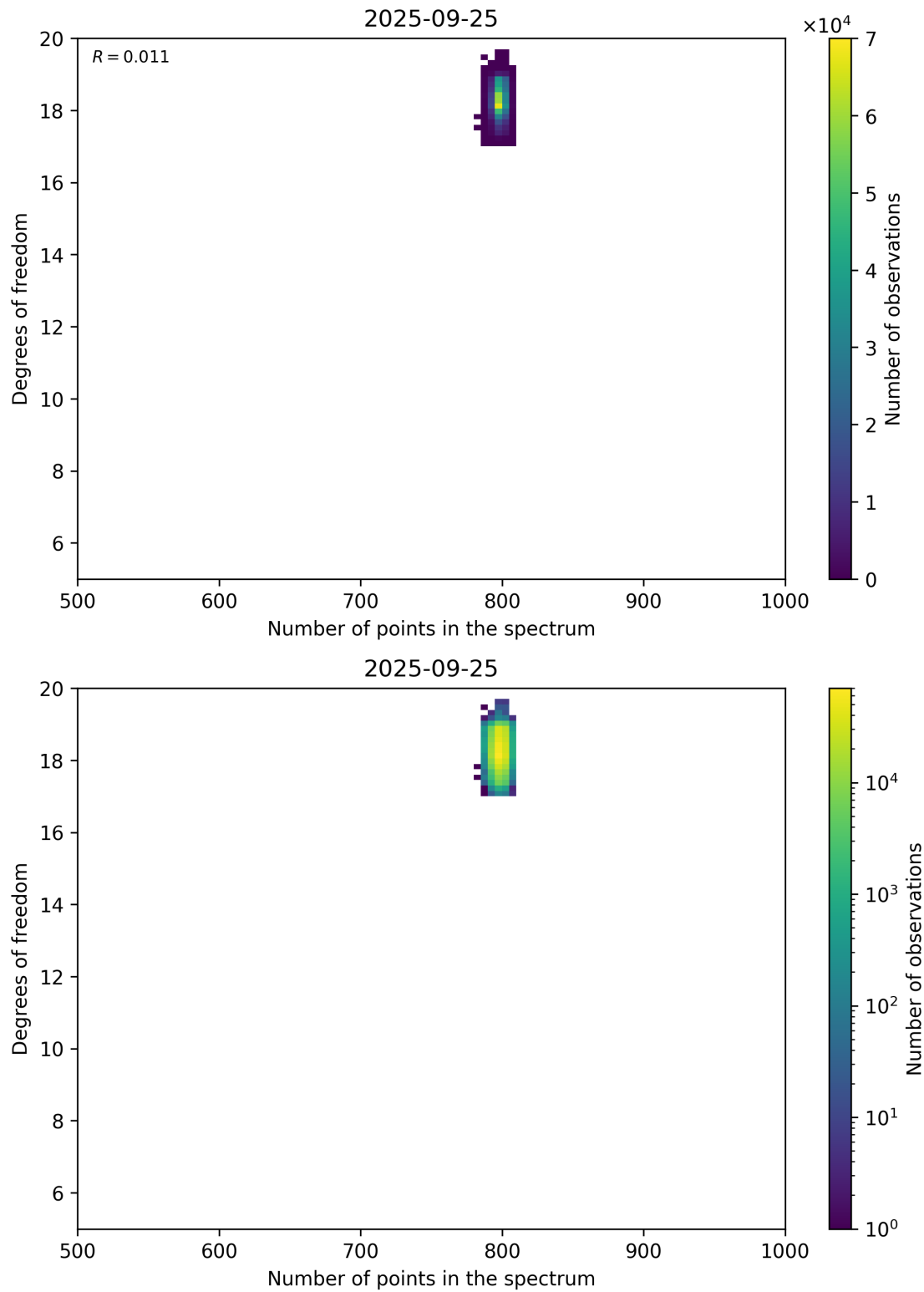
Figure 90: Scatter density plot of “Number of points in the spectrum” against “Degrees of freedom” for 2025-09-25 to 2025-09-26.
