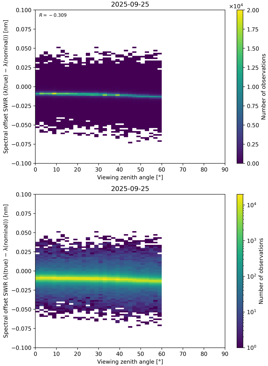
Figure 116: Scatter density plot of “Viewing zenith angle” against “Spectral offset SWIR ( \lambda_{\text{true}} - \lambda_{\text{nominal}} )” for 2025-09-25 to 2025-09-26.
