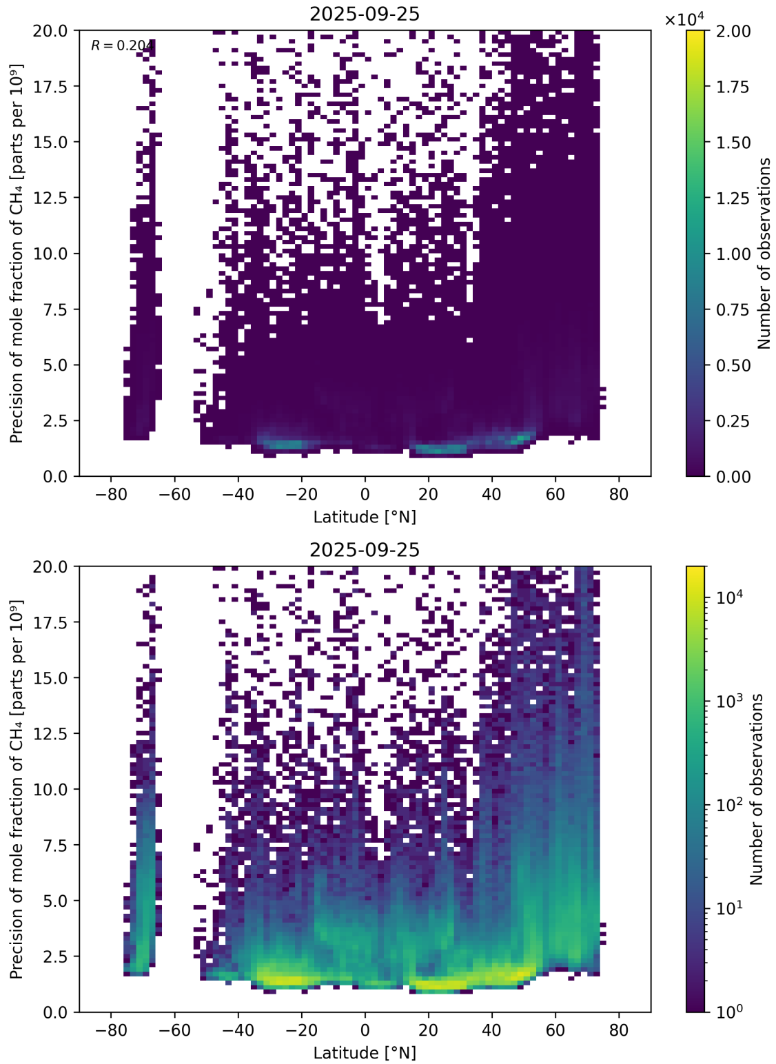
Figure 59: Scatter density plot of “Latitude” against “Precision of mole fraction of CH 4 ” for 2025-09-25 to 2025-09-26.
