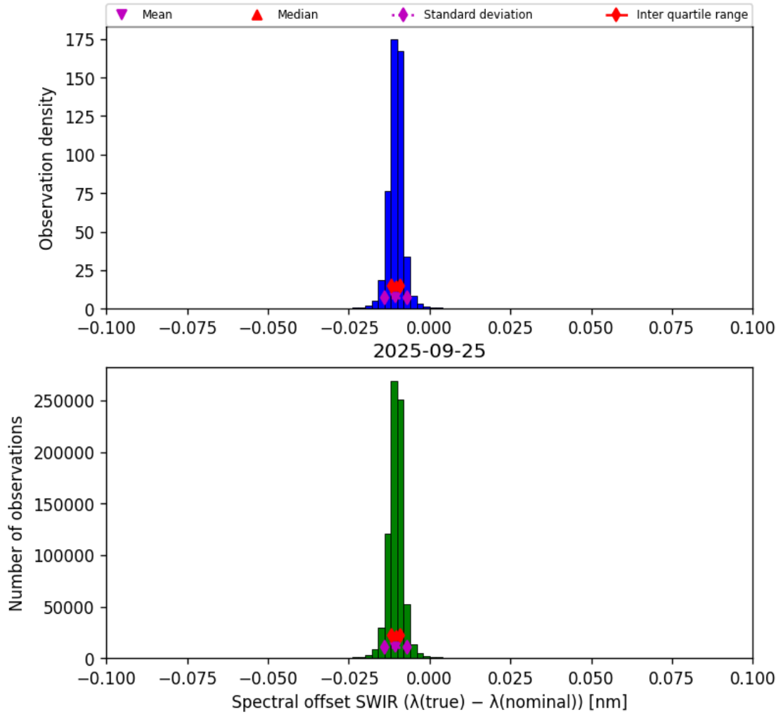
Figure 27: Histogram of “Spectral offset SWIR ( \lambda_{\text{true}} - \lambda_{\text{nominal}} )” for 2025-09-25 to 2025-09-26
