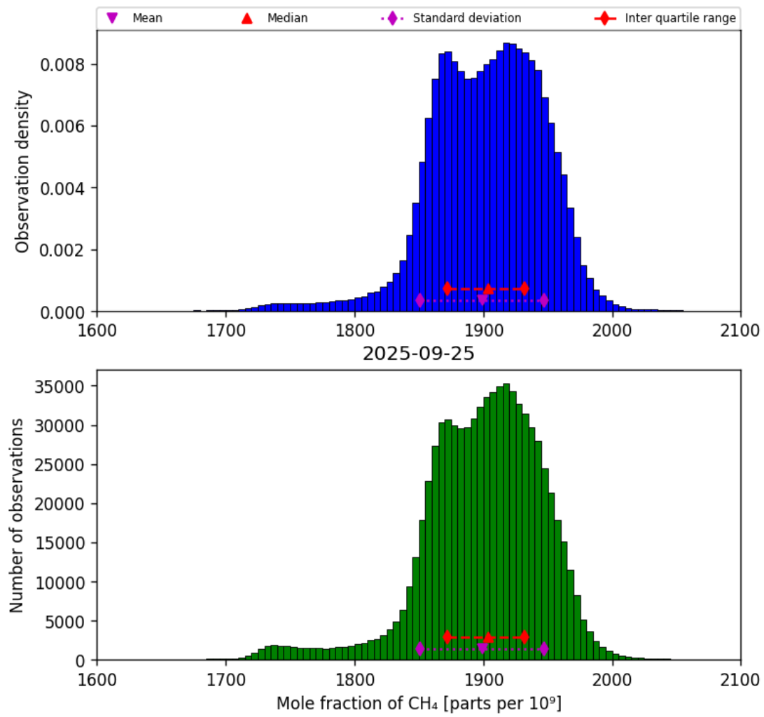
Figure 23: Histogram of “Mole fraction of CH 4 ” for 2025-09-25 to 2025-09-26
