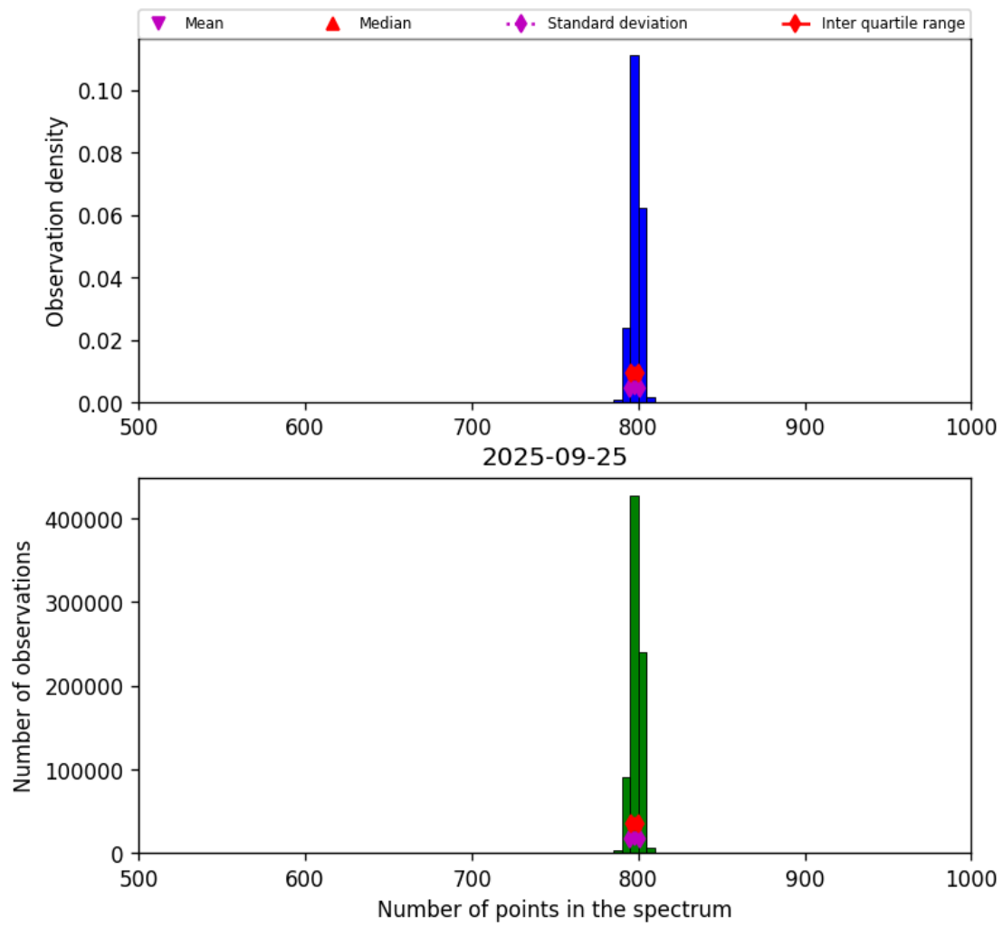
Figure 26: Histogram of “Number of points in the spectrum” for 2025-09-25 to 2025-09-26
