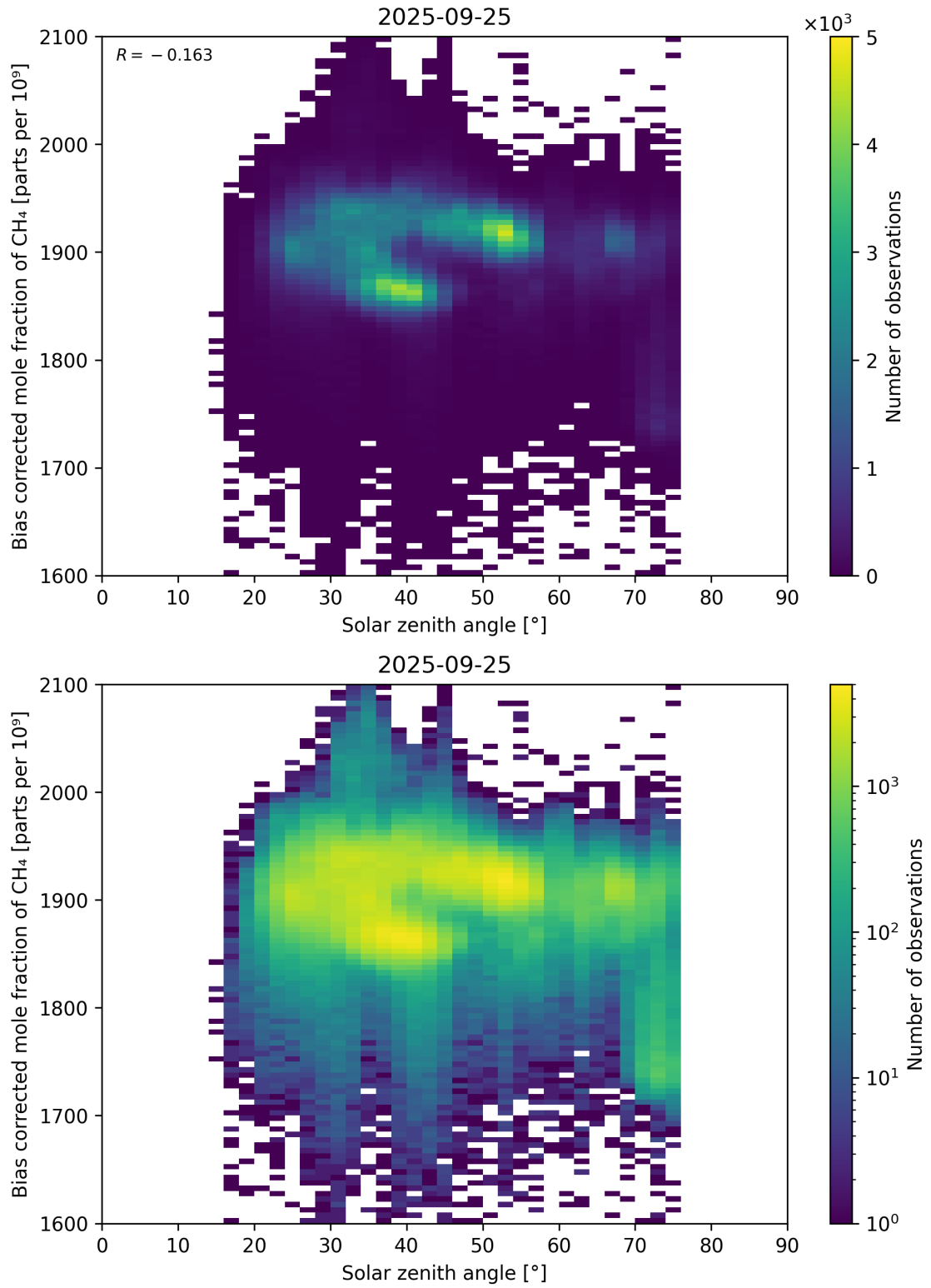
Figure 100: Scatter density plot of “Solar zenith angle” against “Bias corrected mole fraction of CH 4 ” for 2025-09-25 to 2025-09-26.
