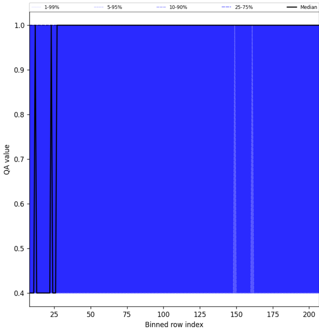
Figure 33: Along track statistics of “QA value” for 2025-09-25 to 2025-09-26
