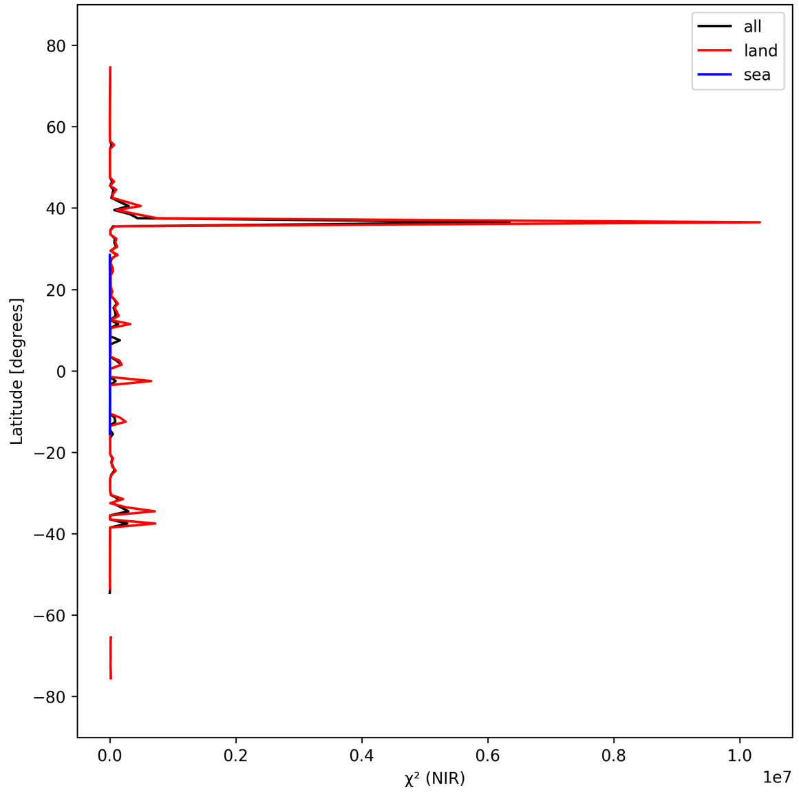
Figure 18: Zonal average of “ \chi^2 (NIR)” for 2025-09-25 to 2025-09-26.
