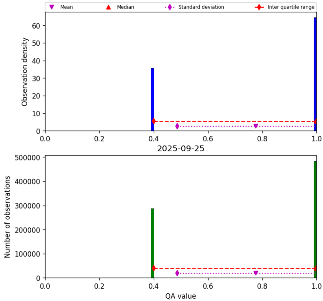
Figure 22: Histogram of “QA value” for 2025-09-25 to 2025-09-26
