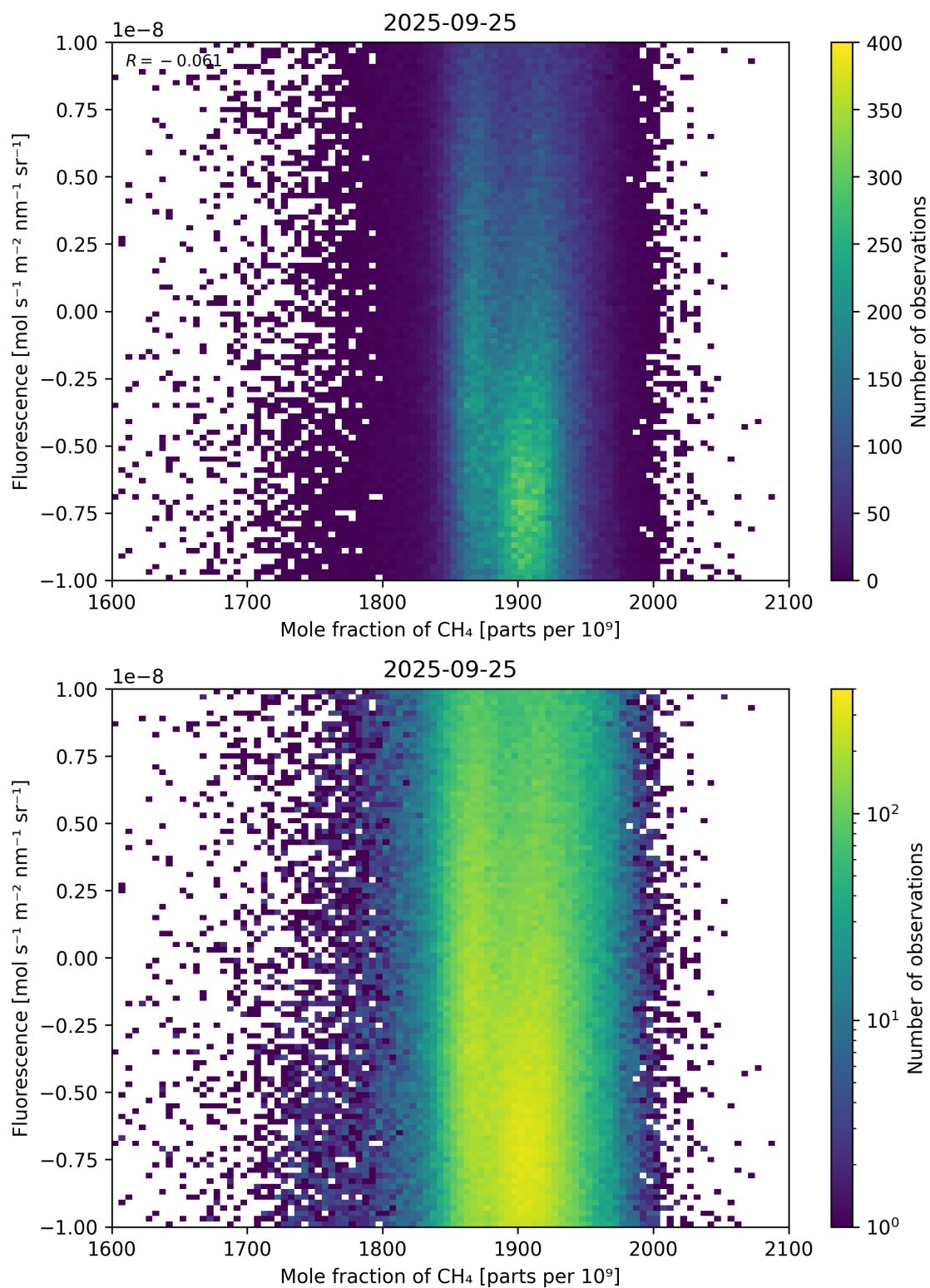
Figure 73: Scatter density plot of “Mole fraction of \text{CH}_4 ” against “Fluorescence” for 2025-09-25 to 2025-09-26.
