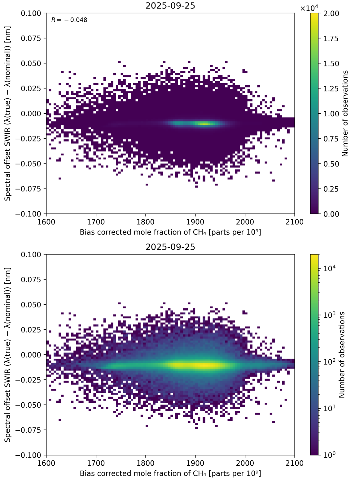
Figure 69: Scatter density plot of “Bias corrected mole fraction of \text{CH}_4 ” against “Spectral offset SWIR ( \lambda_{\text{true}} - \lambda_{\text{nominal}} )” for 2025-09-25 to 2025-09-26.
