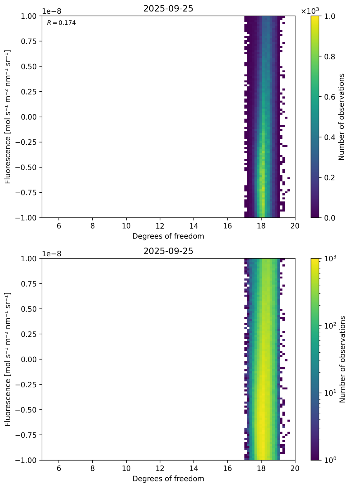
Figure 51: Scatter density plot of “Degrees of freedom” against “Fluorescence” for 2025-09-25 to 2025-09-26.
