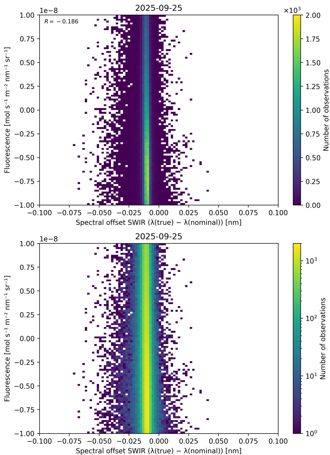
Figure 120: Scatter density plot of “Spectral offset SWIR ( \lambda_{\text{true}} - \lambda_{\text{nominal}} )” against “Fluorescence” for 2025-09-25 to 2025-09-26.
