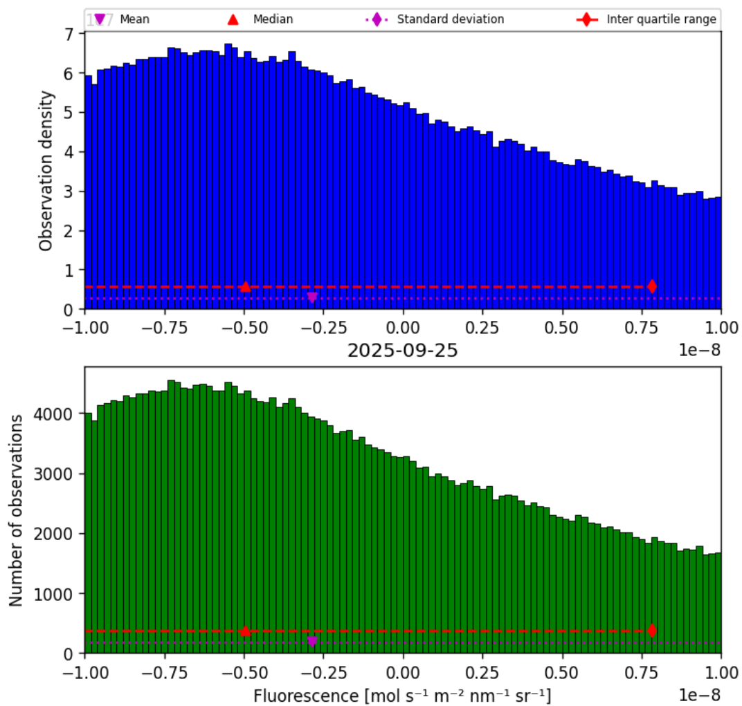
Figure 32: Histogram of “Fluorescence” for 2025-09-25 to 2025-09-26
