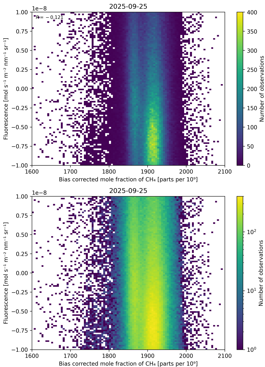
Figure 66: Scatter density plot of “Bias corrected mole fraction of \text{CH}_4 ” against “Fluorescence” for 2025-09-25 to 2025-09-26.
