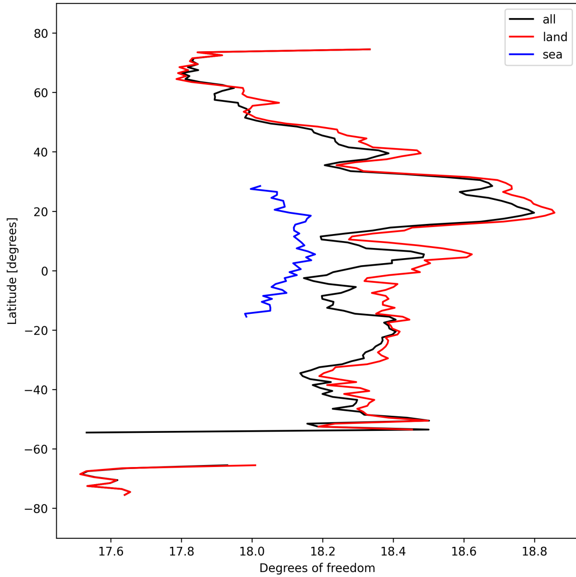
Figure 19: Zonal average of “Degrees of freedom” for 2025-09-25 to 2025-09-26.
