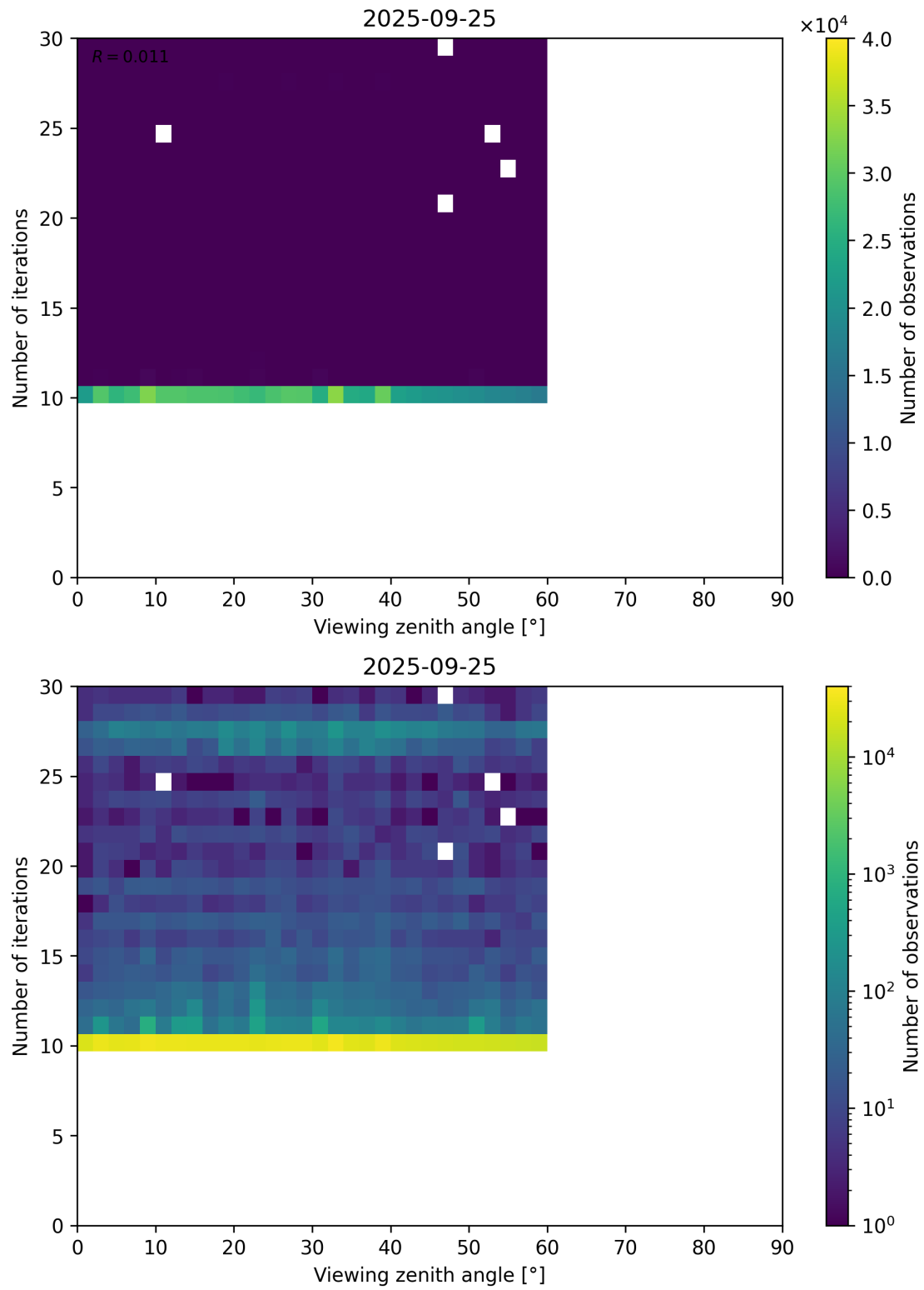
Figure 113: Scatter density plot of “Viewing zenith angle” against “Number of iterations” for 2025-09-25 to 2025-09-26.
