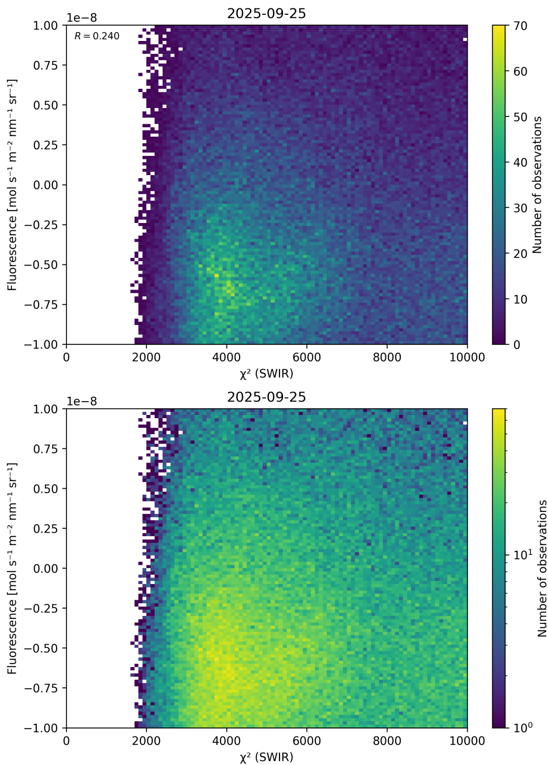
Figure 49: Scatter density plot of “ \chi^2 (SWIR)” against “Fluorescence” for 2025-09-25 to 2025-09-26.
