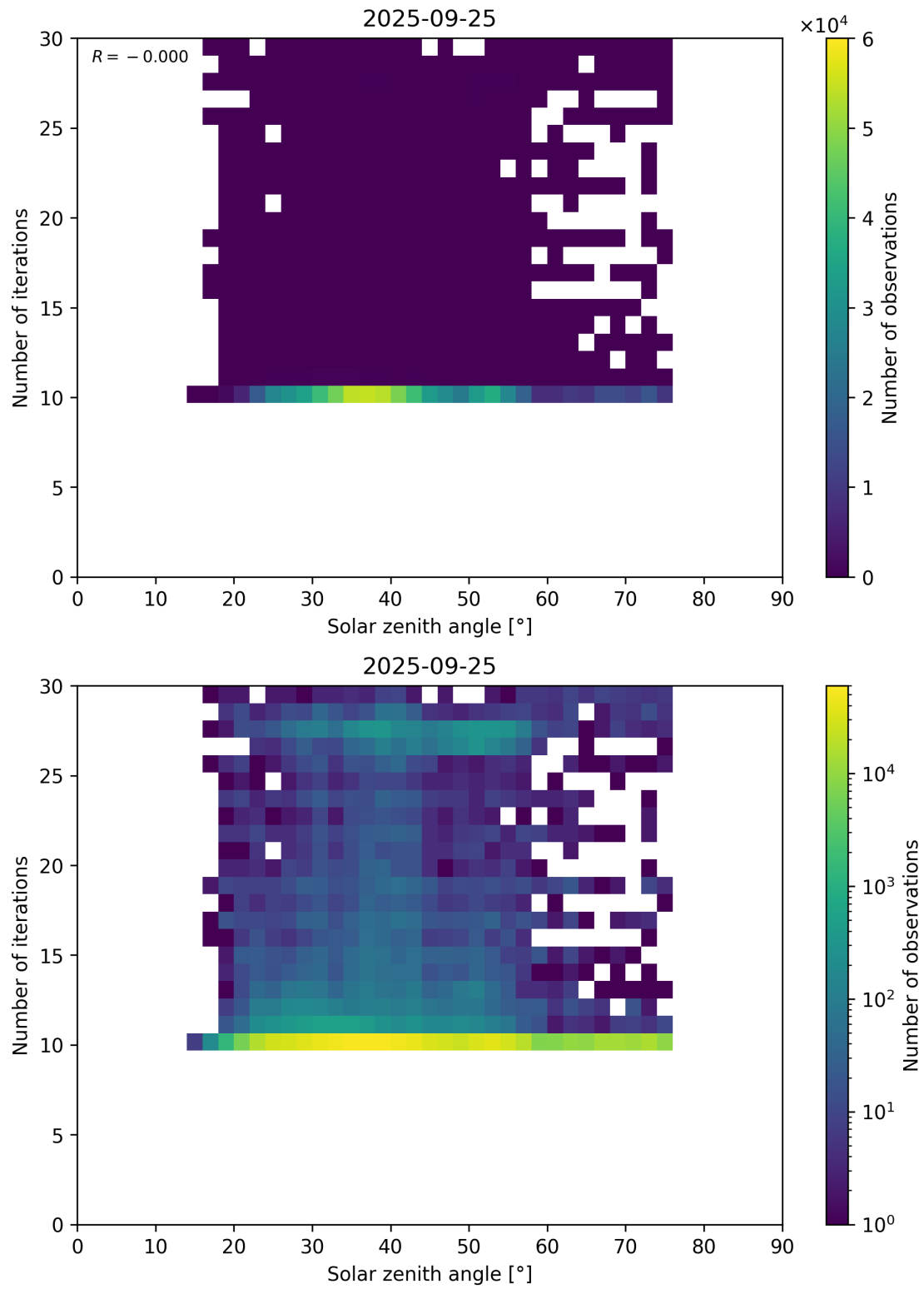
Figure 102: Scatter density plot of “Solar zenith angle” against “Number of iterations” for 2025-09-25 to 2025-09-26.
