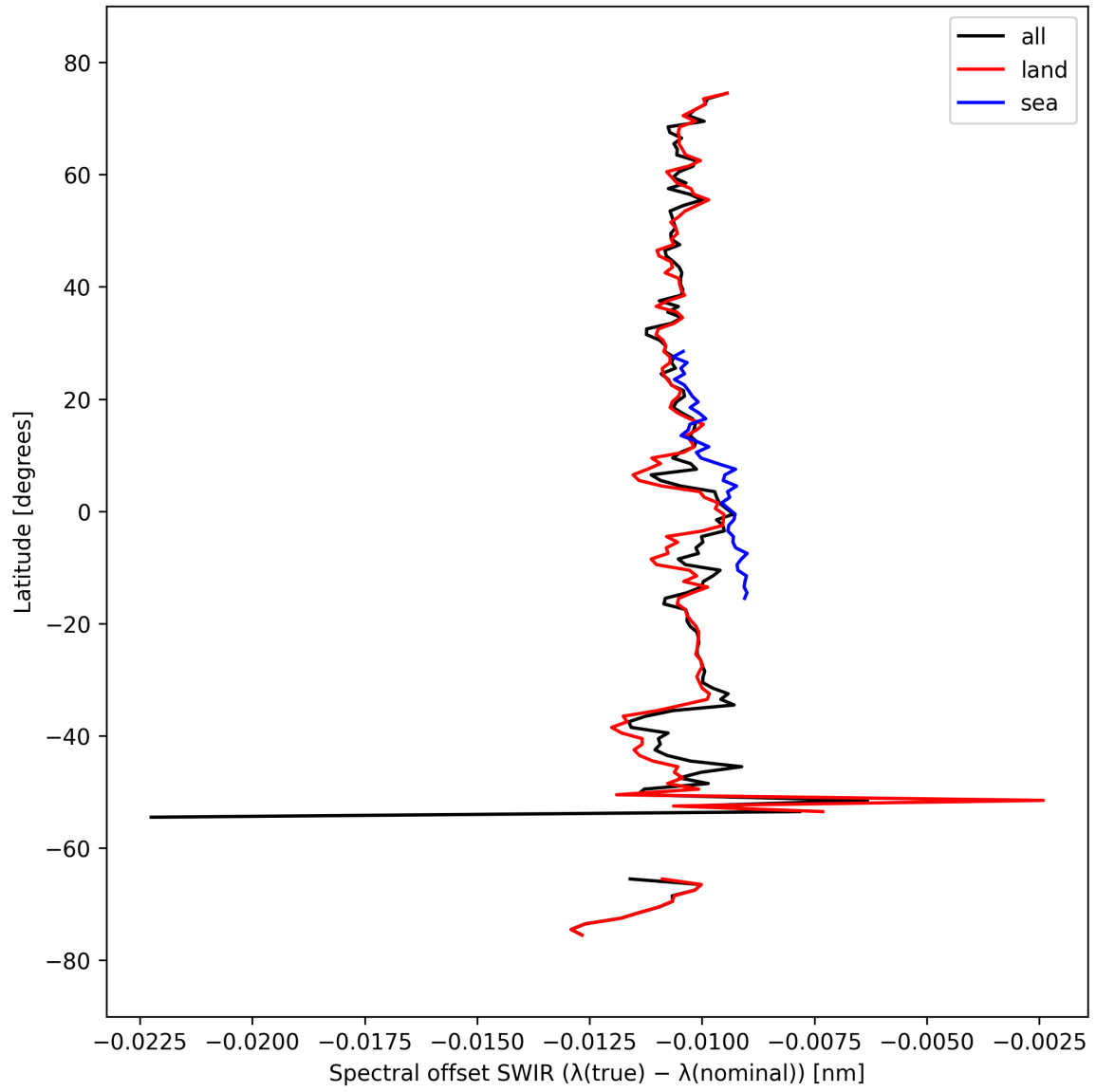
Figure 16: Zonal average of “Spectral offset SWIR ( \lambda_{\text{true}} - \lambda_{\text{nominal}} )” for 2025-09-25 to 2025-09-26.
