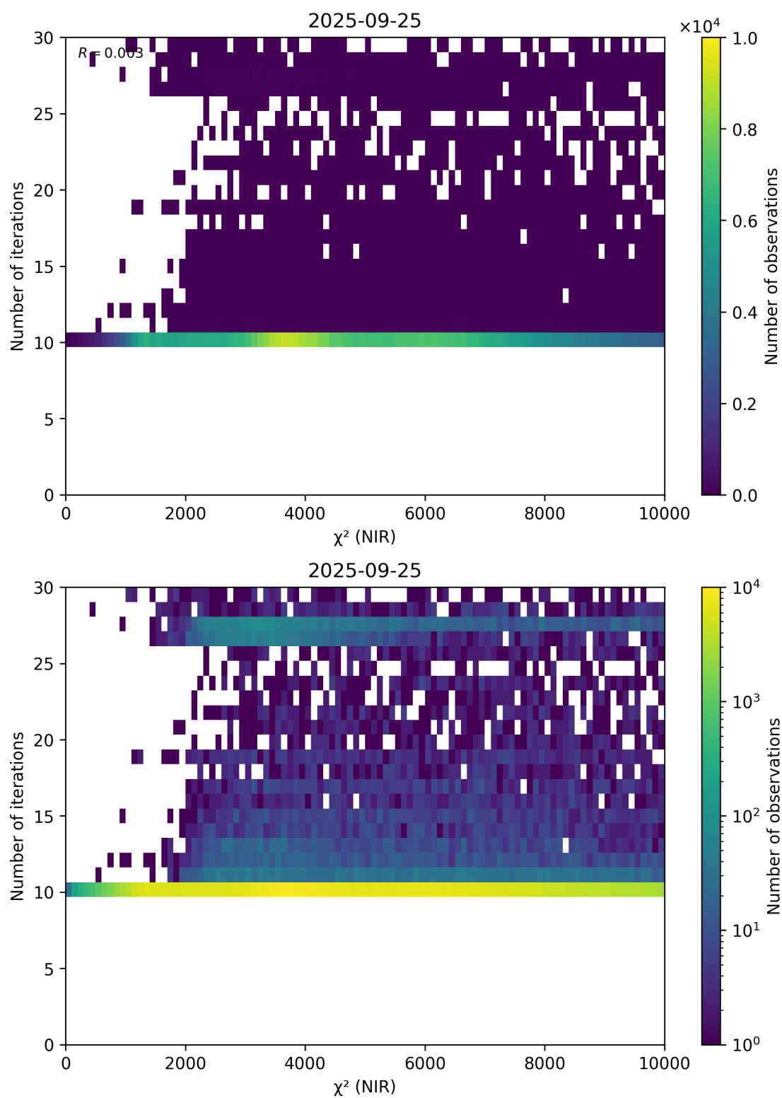
Figure 46: Scatter density plot of “ \chi^2 (NIR)” against “Number of iterations” for 2025-09-25 to 2025-09-26.
