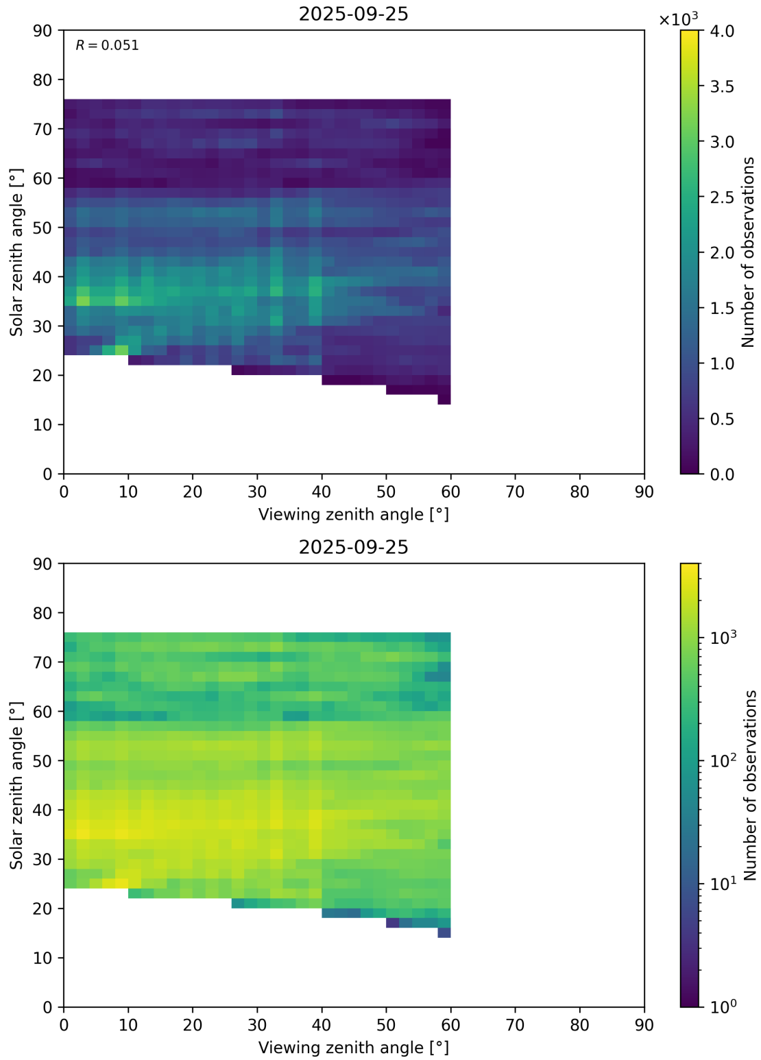
Figure 115: Scatter density plot of “Viewing zenith angle” against “Solar zenith angle” for 2025-09-25 to 2025-09-26.
