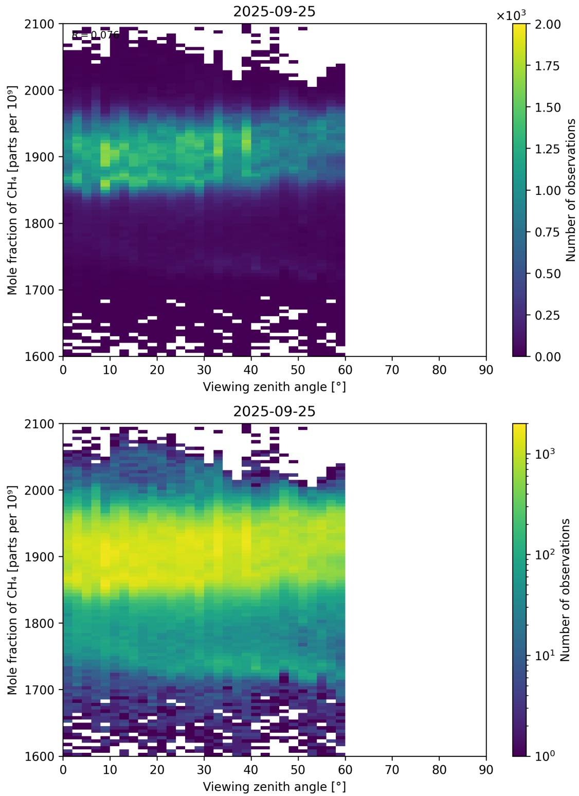
Figure 110: Scatter density plot of “Viewing zenith angle” against “Mole fraction of CH 4 ” for 2025-09-25 to 2025-09-26.
