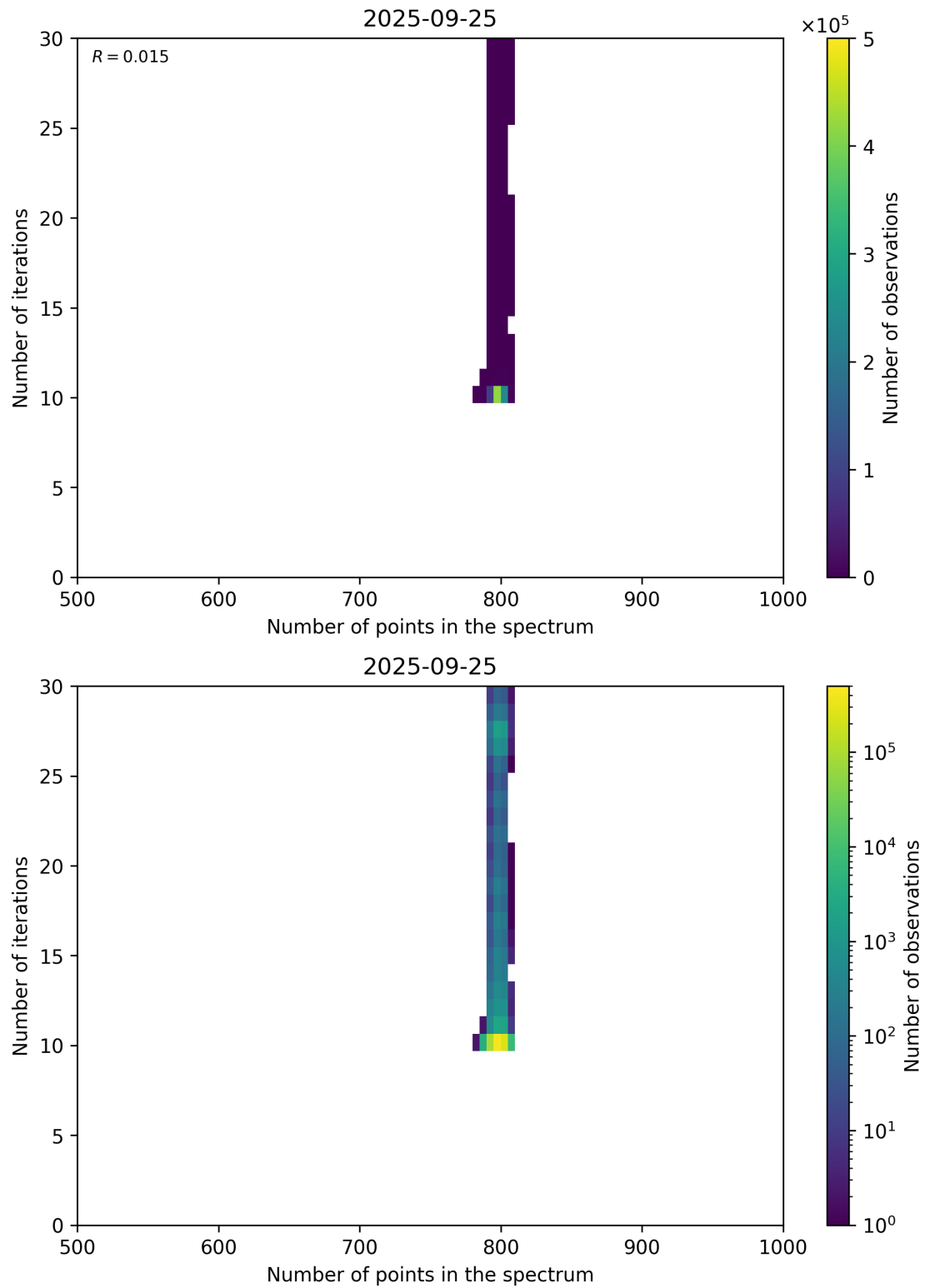
Figure 92: Scatter density plot of “Number of points in the spectrum” against “Number of iterations” for 2025-09-25 to 2025-09-26.
