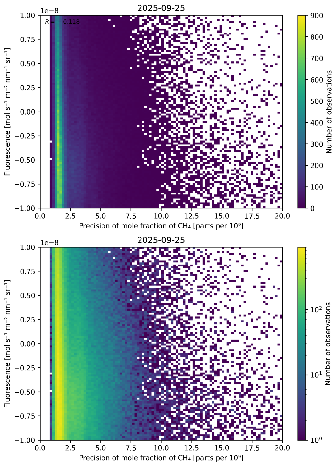
Figure 81: Scatter density plot of “Precision of mole fraction of CH 4 ” against “Fluorescence” for 2025-09-25 to 2025-09-26.
