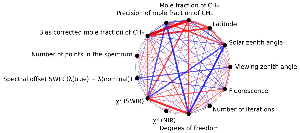
Figure 1: Map of correlation graph for 2025-09-25 to 2025-09-26.
