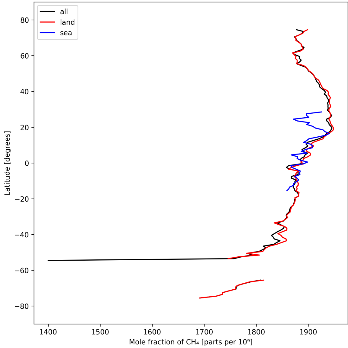
Figure 12: Zonal average of “Mole fraction of CH 4 ” for 2025-09-25 to 2025-09-26.
