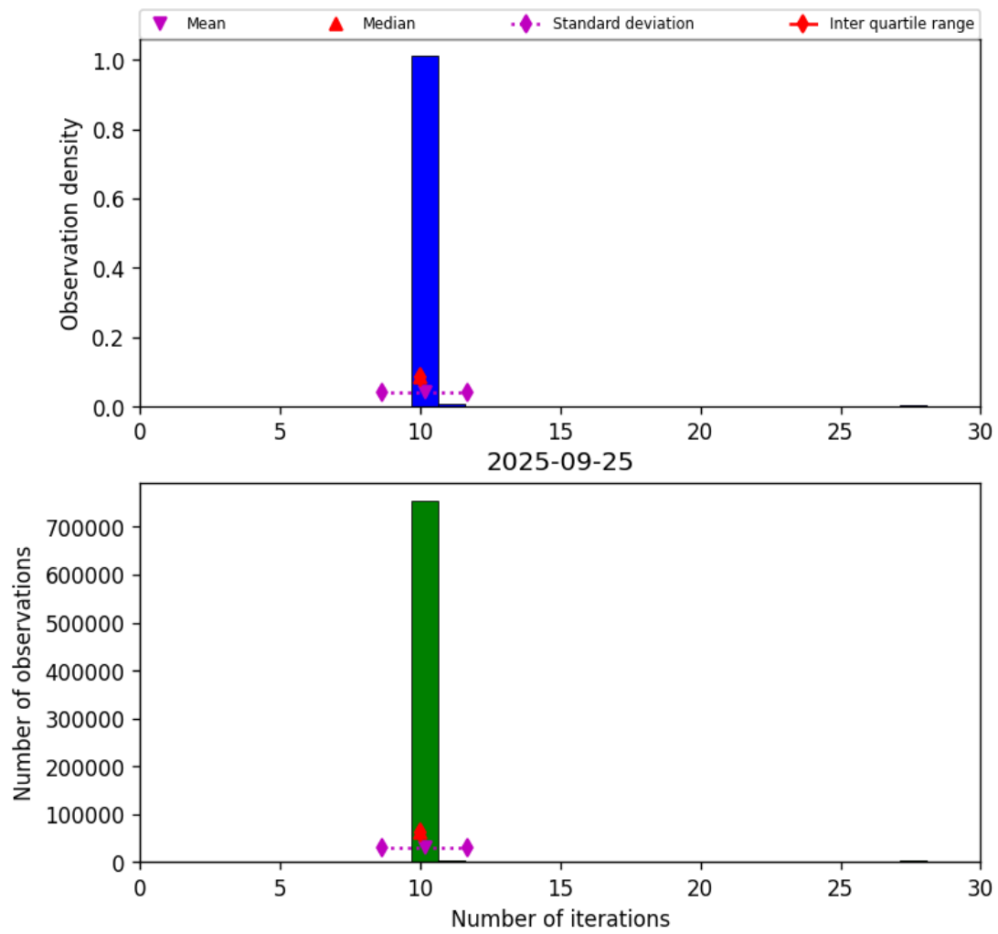
Figure 31: Histogram of “Number of iterations” for 2025-09-25 to 2025-09-26
