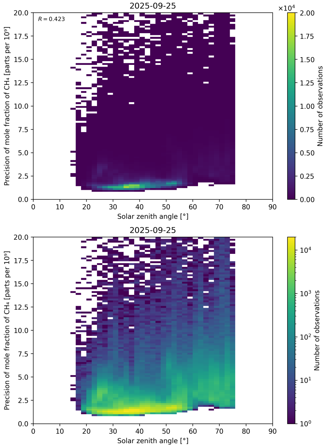
Figure 101: Scatter density plot of “Solar zenith angle” against “Precision of mole fraction of \text{CH}_4 ” for 2025-09-25 to 2025-09-26.
