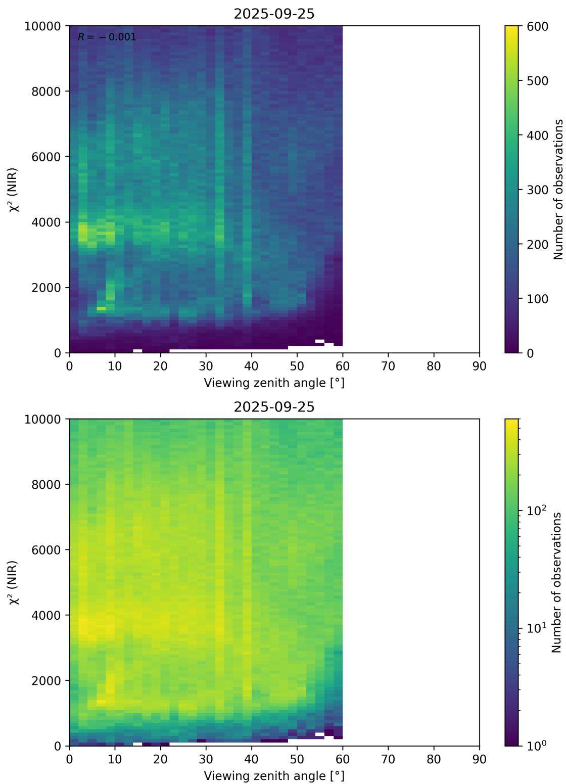
Figure 105: Scatter density plot of “Viewing zenith angle” against “ \chi^2 (NIR)” for 2025-09-25 to 2025-09-26.
