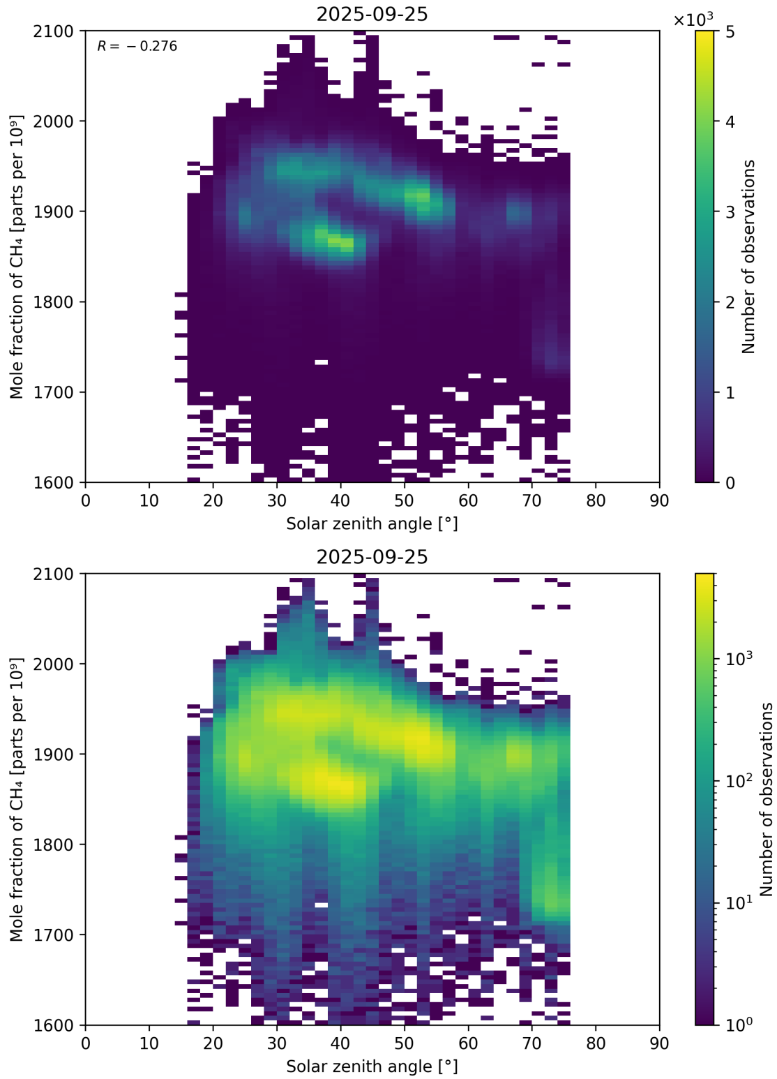
Figure 99: Scatter density plot of “Solar zenith angle” against “Mole fraction of CH 4 ” for 2025-09-25 to 2025-09-26.
