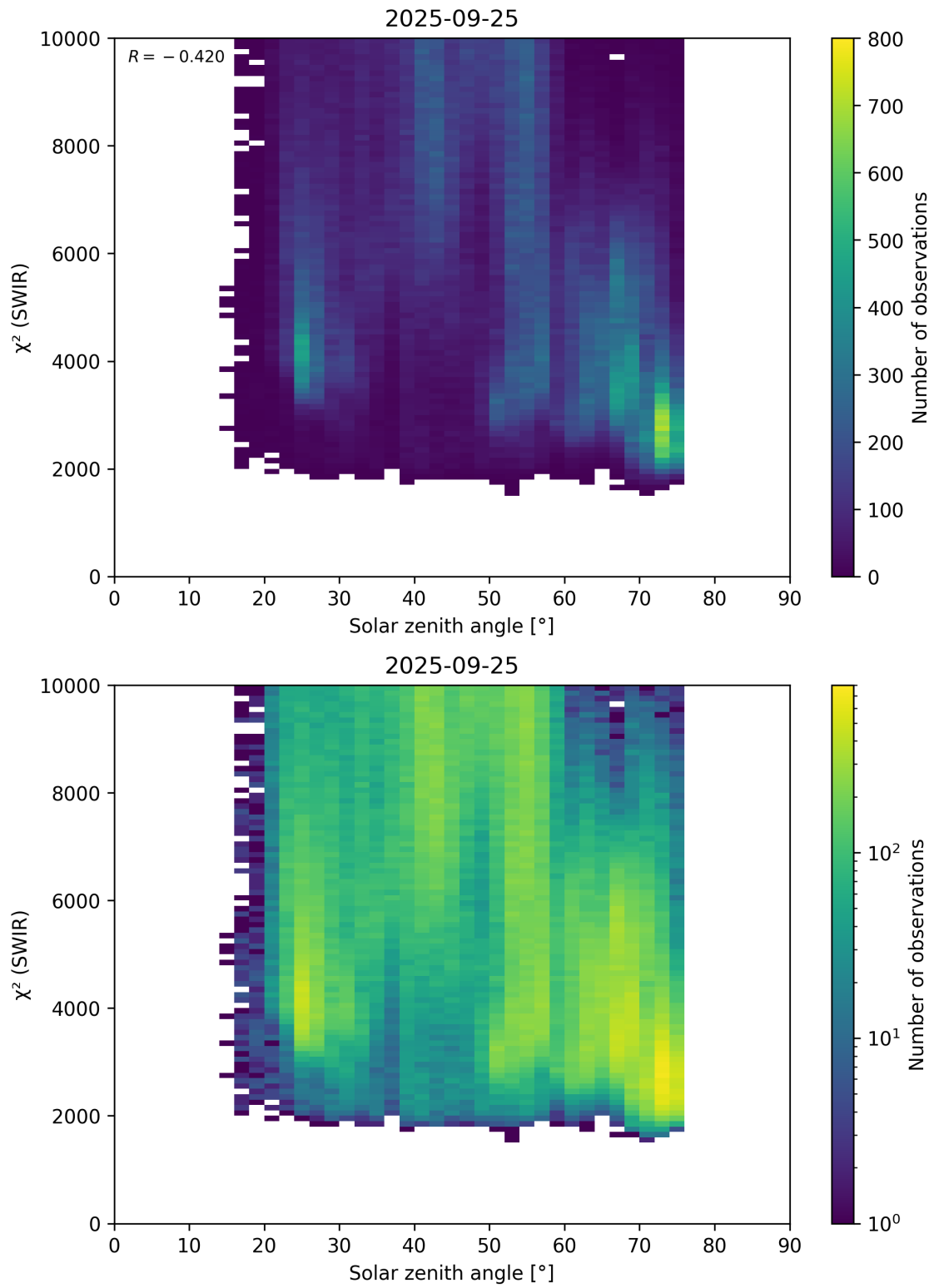
Figure 95: Scatter density plot of “Solar zenith angle” against “ \chi^2 (SWIR)” for 2025-09-25 to 2025-09-26.
