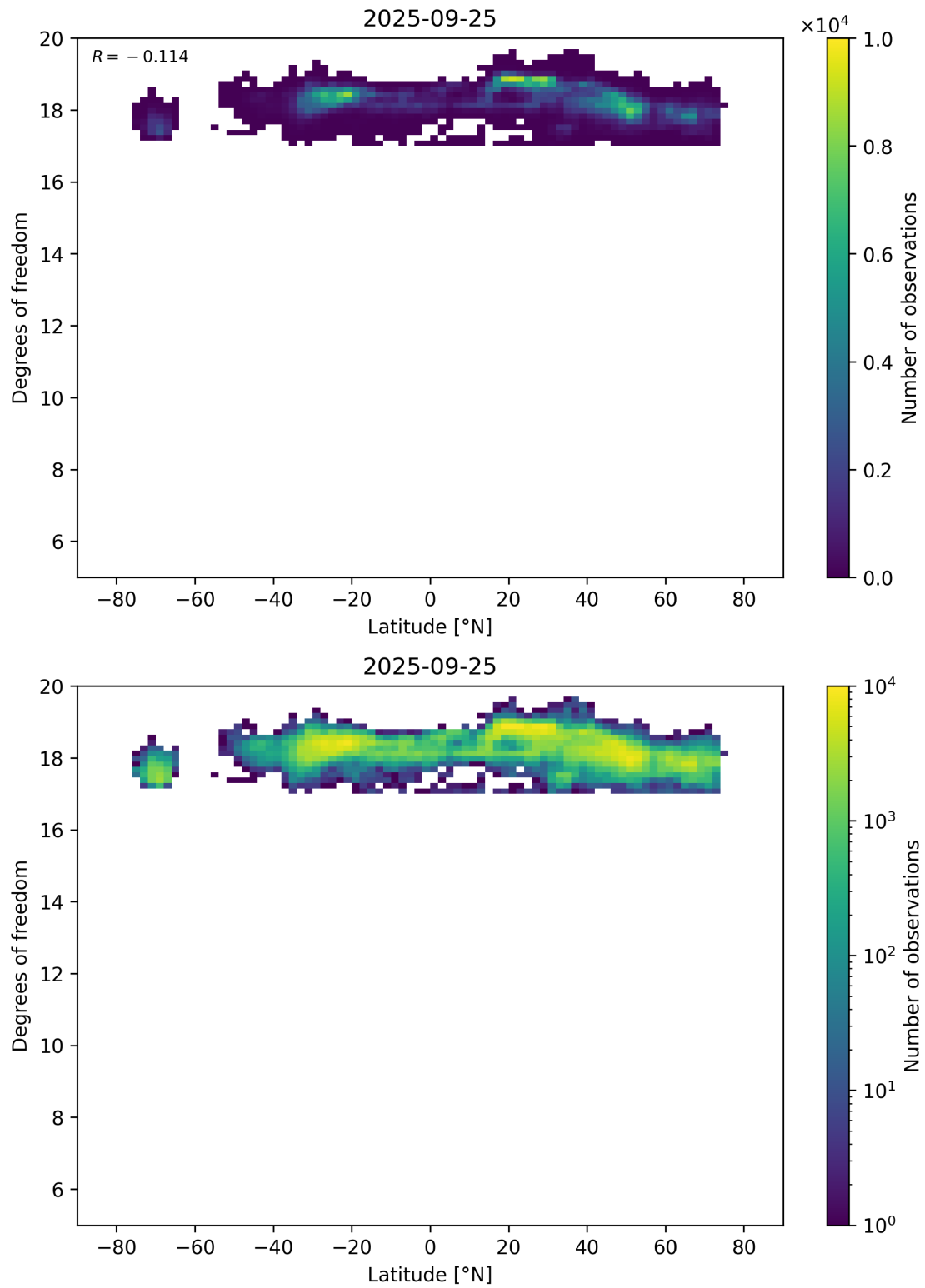
Figure 55: Scatter density plot of “Latitude” against “Degrees of freedom” for 2025-09-25 to 2025-09-26.
