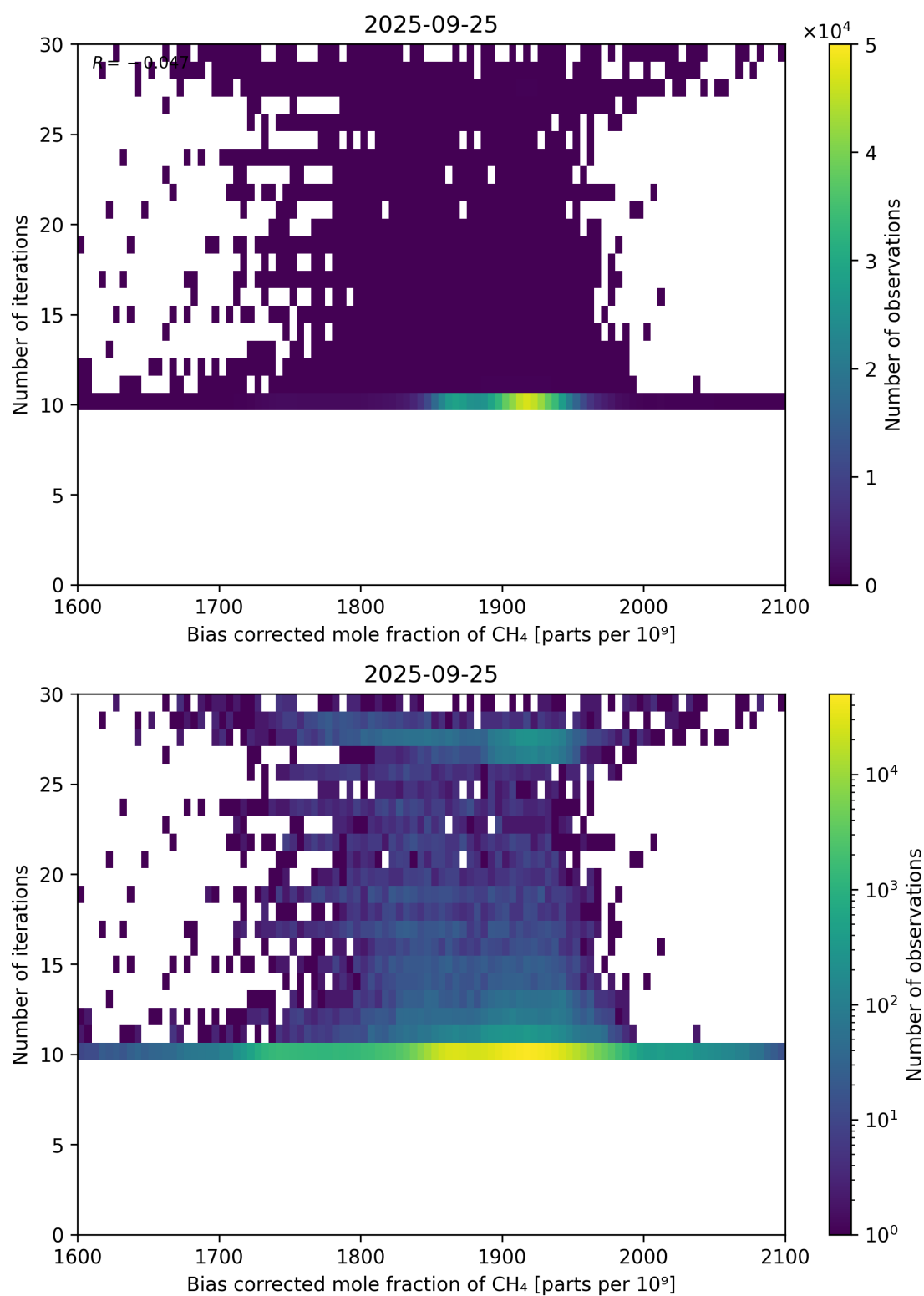
Figure 67: Scatter density plot of “Bias corrected mole fraction of CH 4 ” against “Number of iterations” for 2025-09-25 to 2025-09-26.
