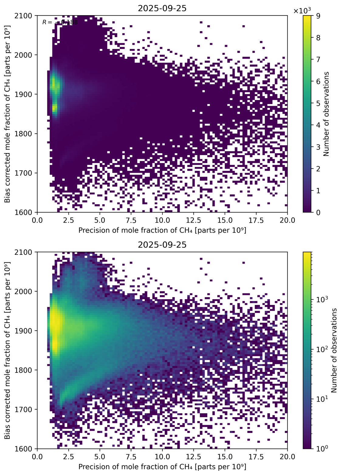
Figure 82: Scatter density plot of “Precision of mole fraction of CH 4 ” against “Bias corrected mole fraction of CH 4 ” for 2025-09-25 to 2025-09-26.
