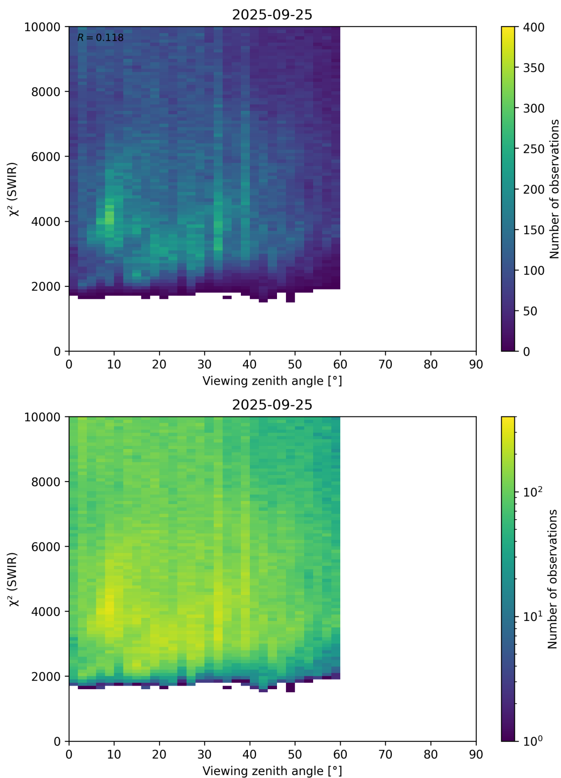
Figure 106: Scatter density plot of “Viewing zenith angle” against “ \chi^2 (SWIR)” for 2025-09-25 to 2025-09-26.
