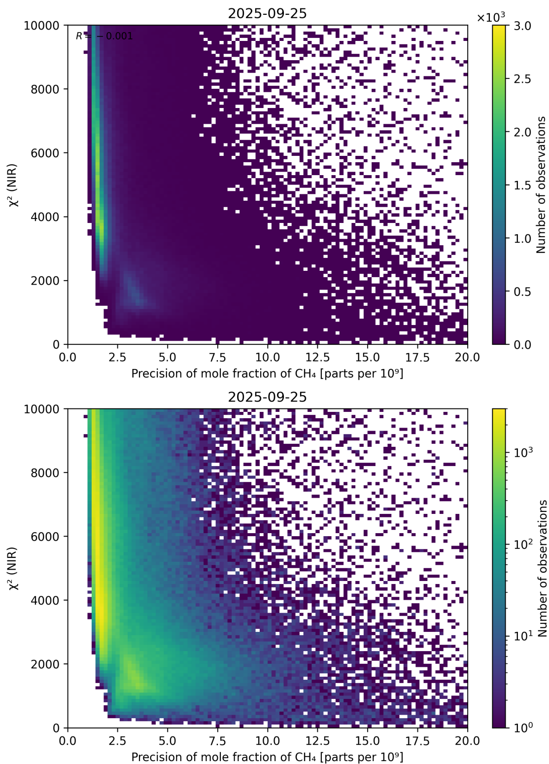
Figure 78: Scatter density plot of “Precision of mole fraction of \text{CH}_4 ” against “ \chi^2 (NIR)” for 2025-09-25 to 2025-09-26.
