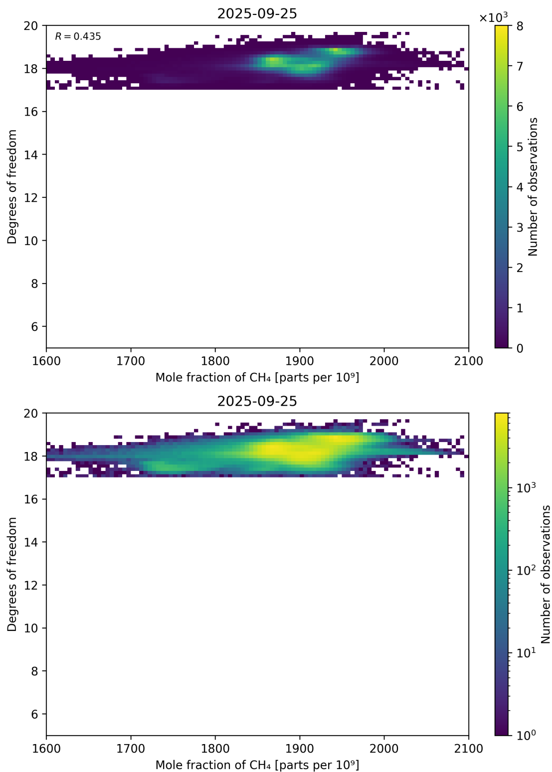
Figure 72: Scatter density plot of “Mole fraction of CH 4 ” against “Degrees of freedom” for 2025-09-25 to 2025-09-26.
