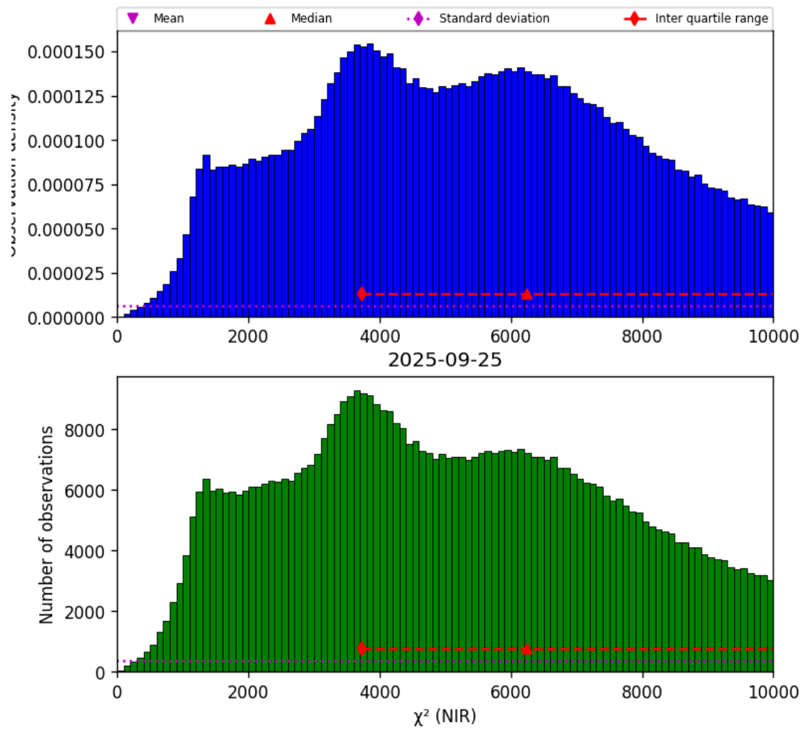
Figure 29: Histogram of “ \chi^2 (NIR)” for 2025-09-25 to 2025-09-26
