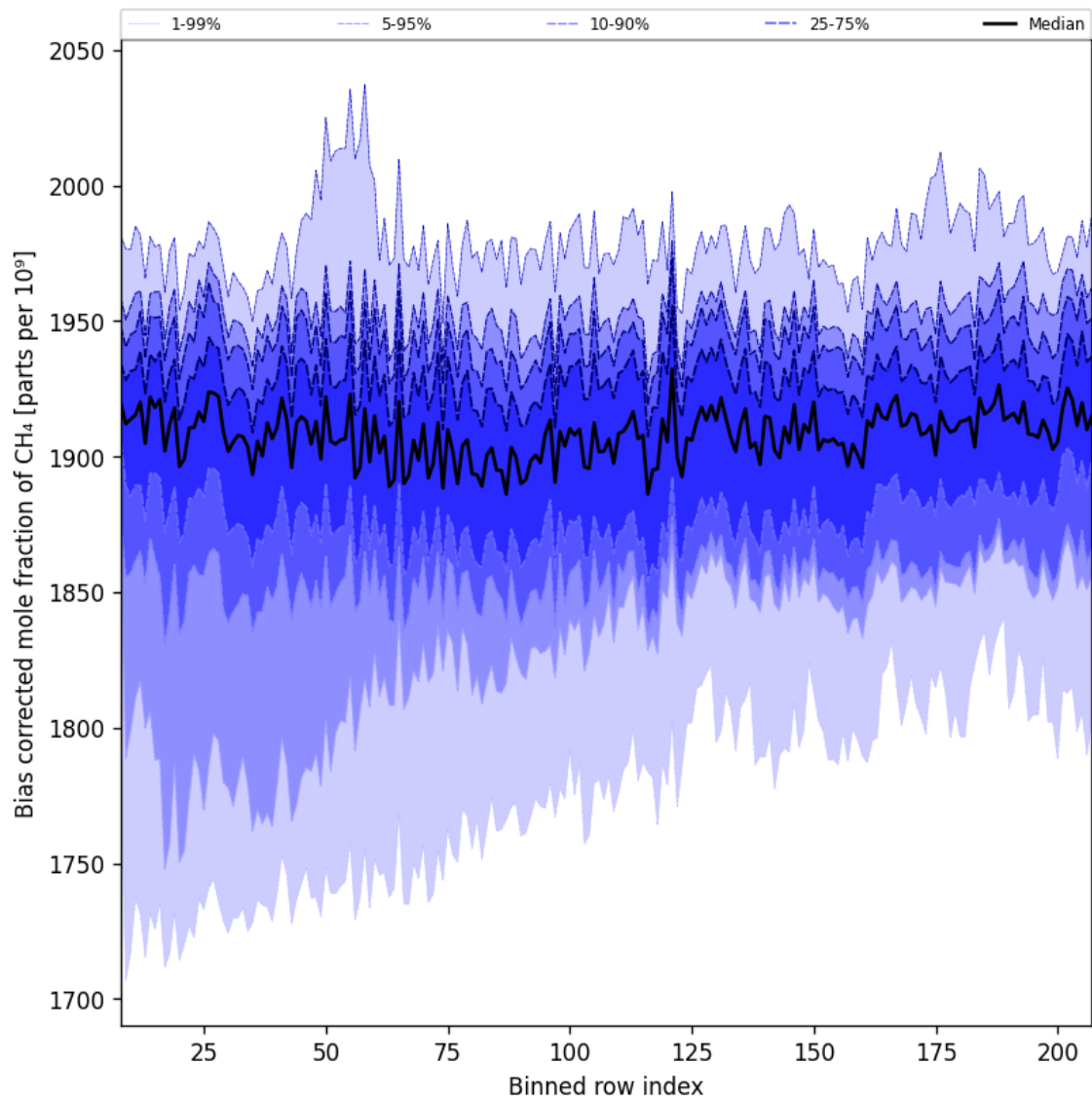
Figure 36: Along track statistics of “Bias corrected mole fraction of CH 4 ” for 2025-09-25 to 2025-09-26
