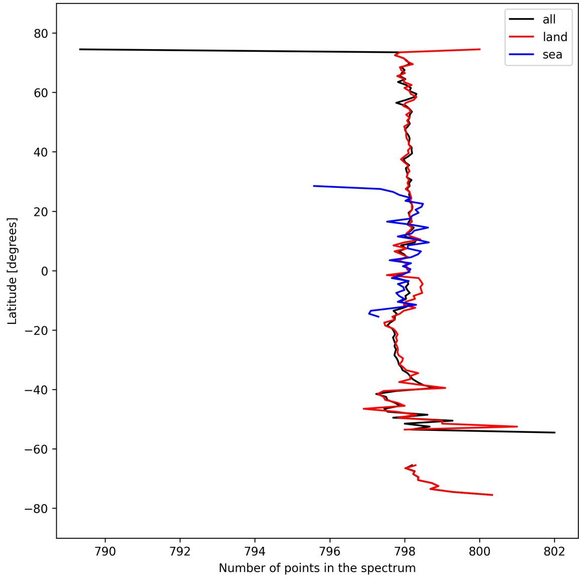
Figure 15: Zonal average of “Number of points in the spectrum” for 2025-09-25 to 2025-09-26.
