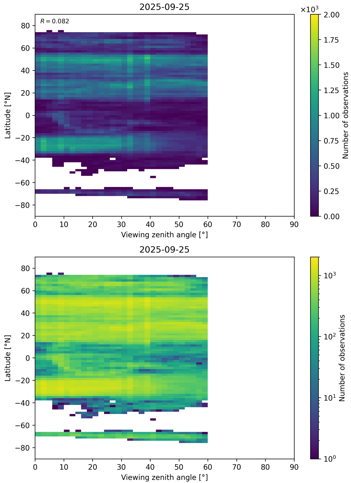
Figure 109: Scatter density plot of “Viewing zenith angle” against “Latitude” for 2025-09-25 to 2025-09-26.
