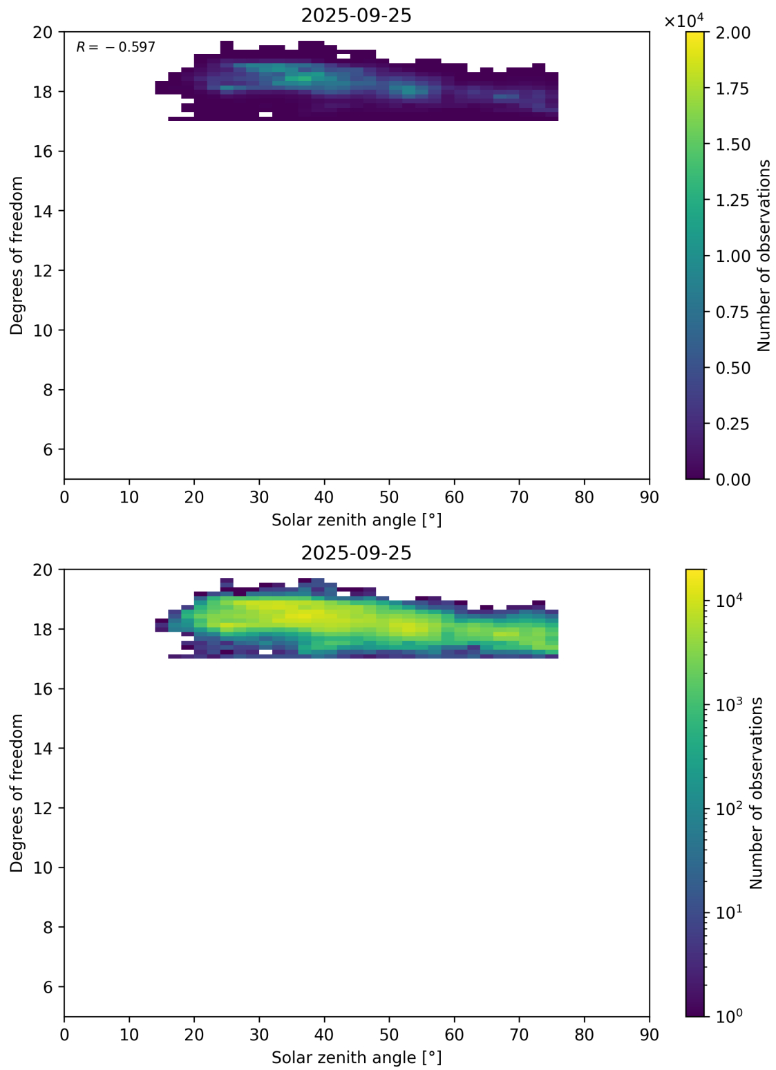
Figure 96: Scatter density plot of “Solar zenith angle” against “Degrees of freedom” for 2025-09-25 to 2025-09-26.
