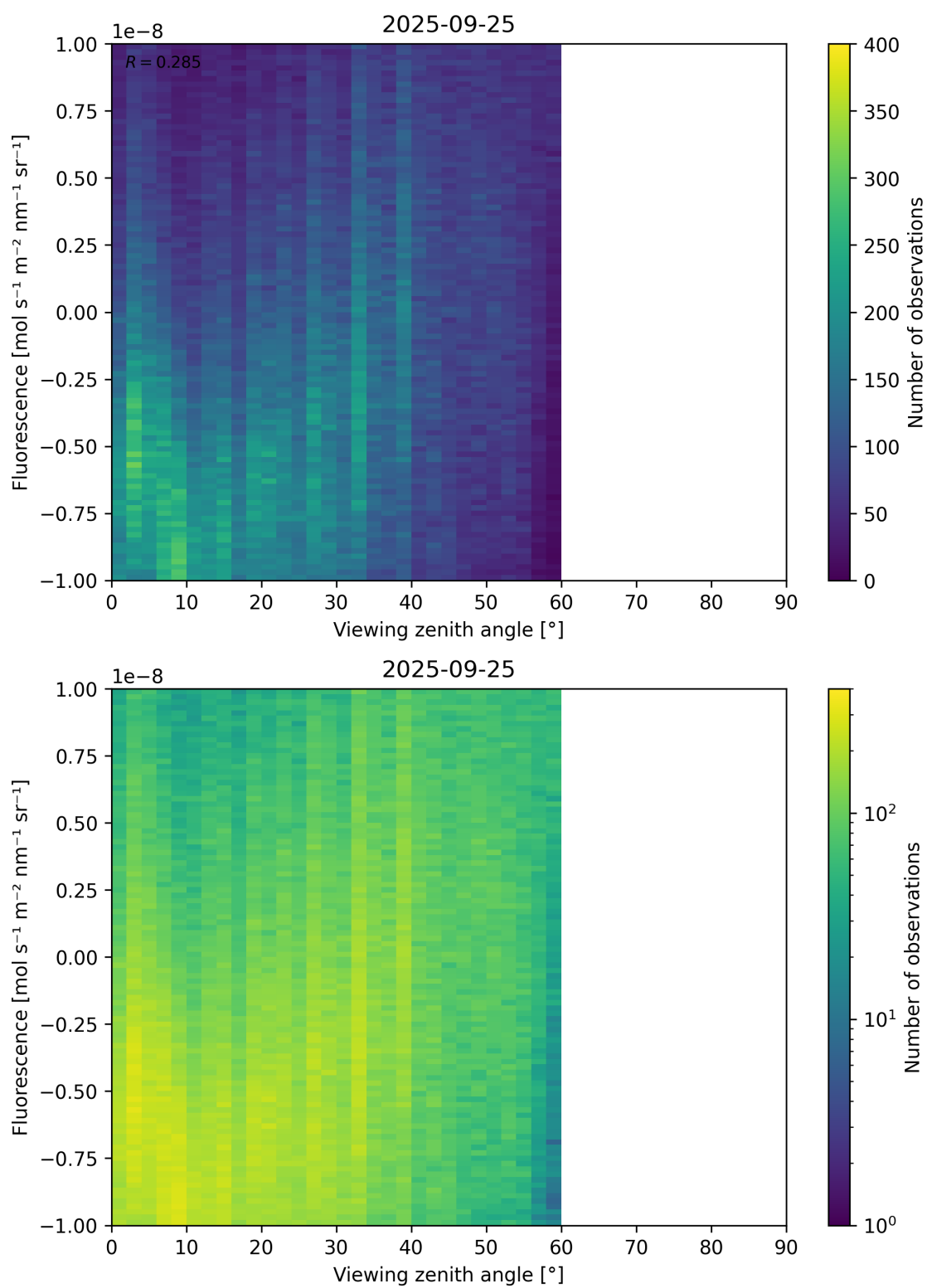
Figure 108: Scatter density plot of “Viewing zenith angle” against “Fluorescence” for 2025-09-25 to 2025-09-26.
