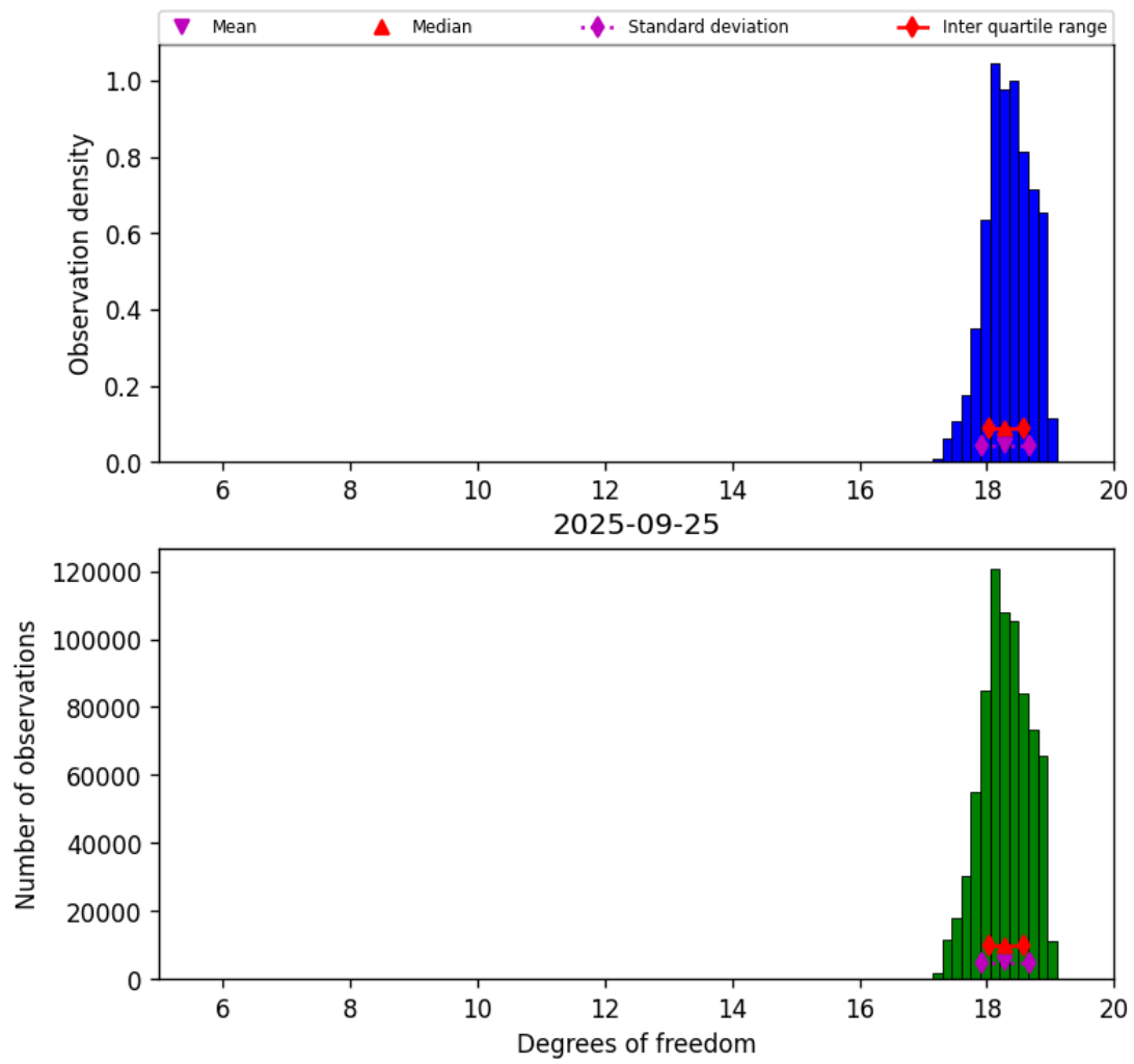
Figure 30: Histogram of “Degrees of freedom” for 2025-09-25 to 2025-09-26
