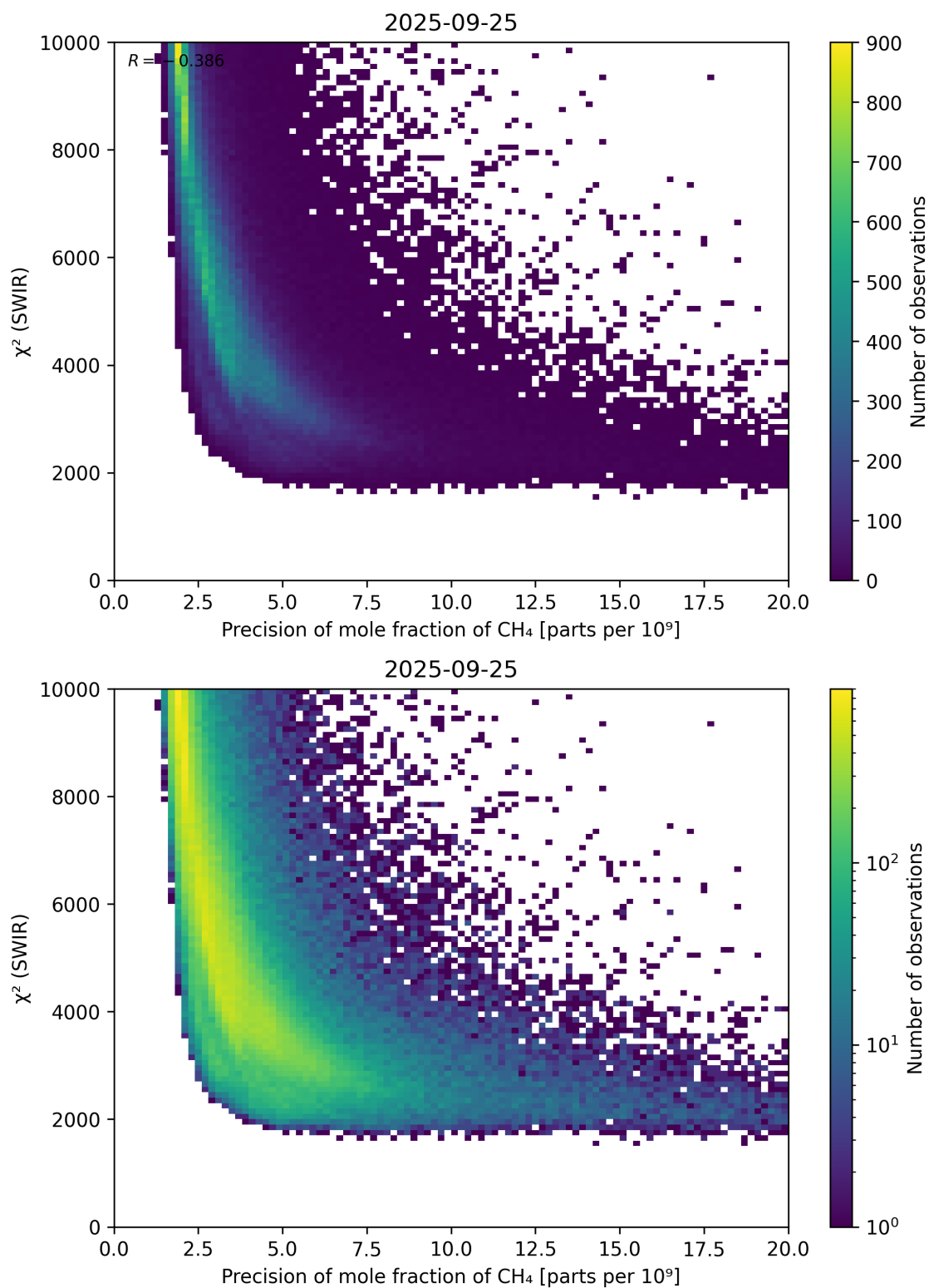
Figure 79: Scatter density plot of “Precision of mole fraction of \text{CH}_4 ” against “ \chi^2 (SWIR)” for 2025-09-25 to 2025-09-26.
