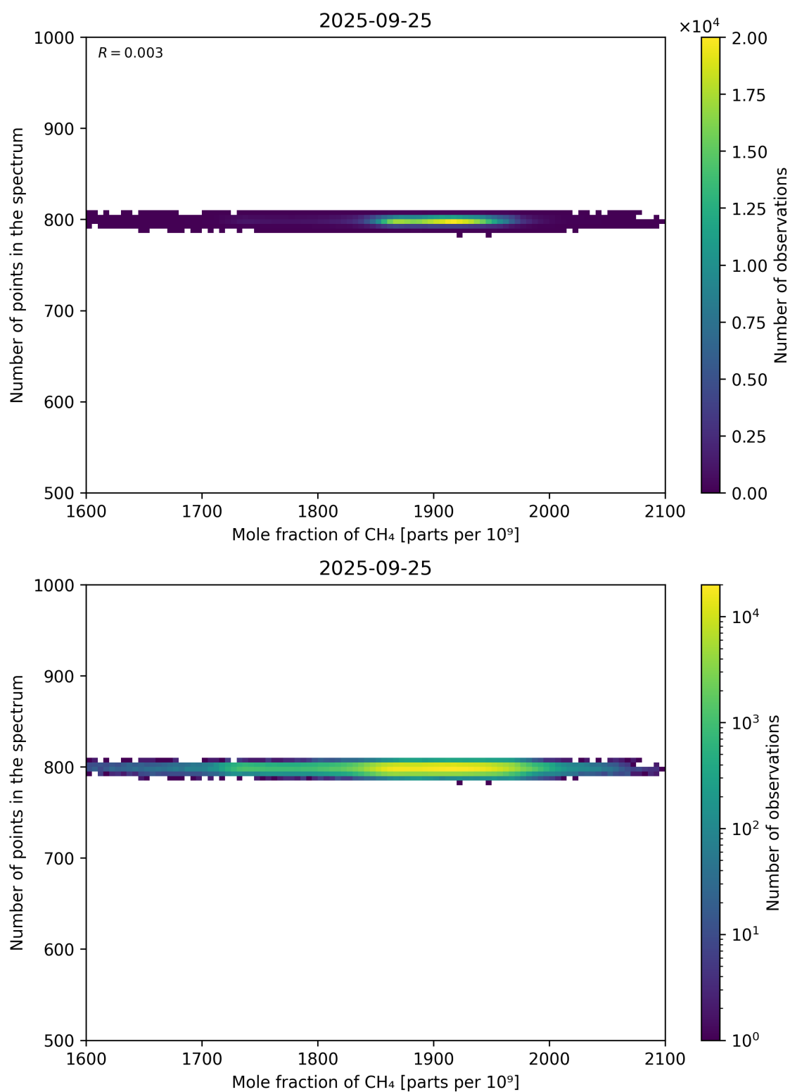
Figure 77: Scatter density plot of “Mole fraction of CH 4 ” against “Number of points in the spectrum” for 2025-09-25 to 2025-09-26.
