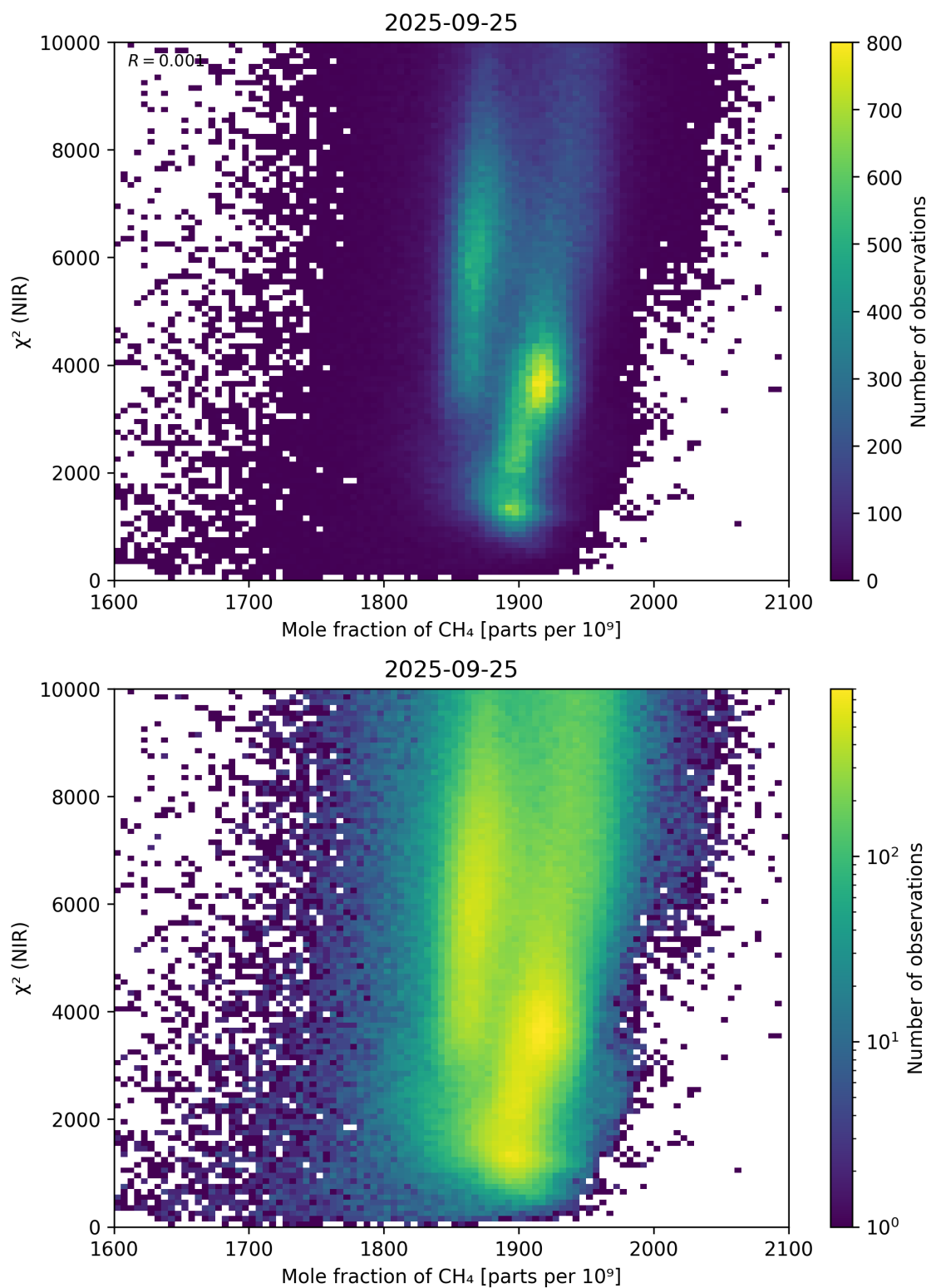
Figure 70: Scatter density plot of “Mole fraction of \text{CH}_4 ” against “ \chi^2 (NIR)” for 2025-09-25 to 2025-09-26.
