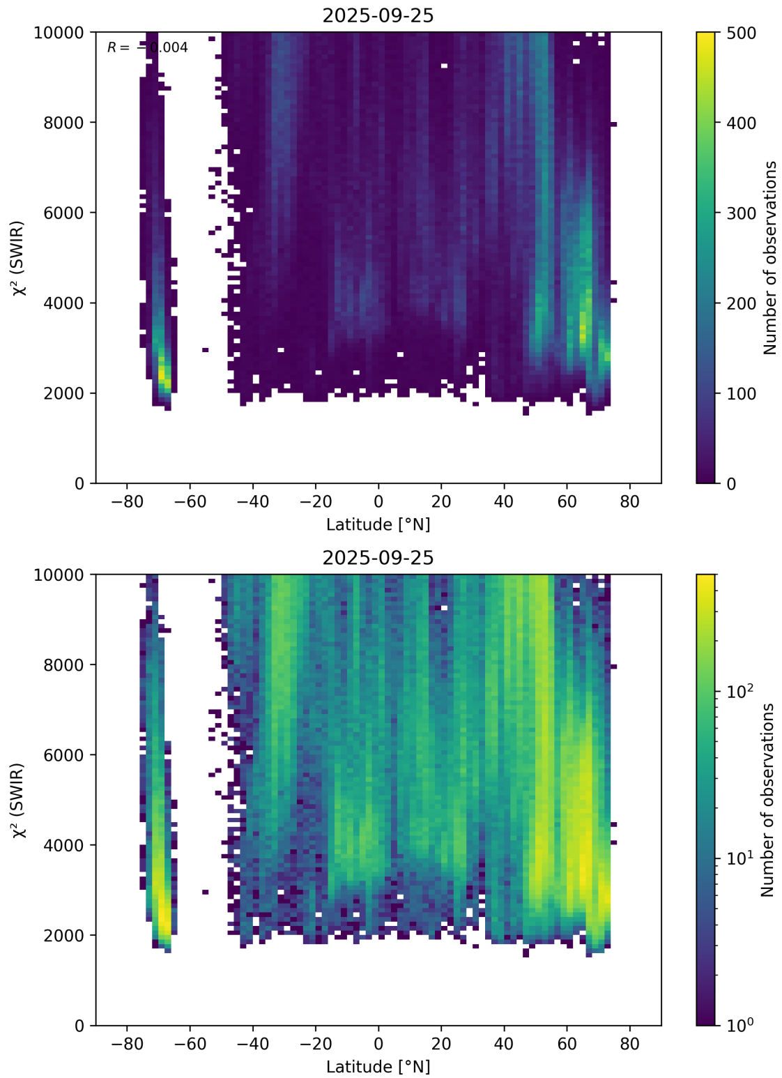
Figure 54: Scatter density plot of “Latitude” against “ \chi^2 (SWIR)” for 2025-09-25 to 2025-09-26.
