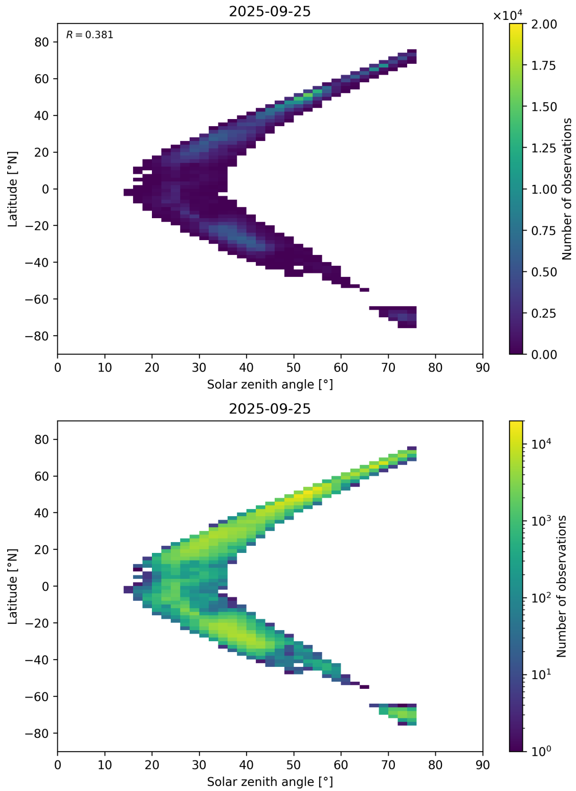
Figure 98: Scatter density plot of “Solar zenith angle” against “Latitude” for 2025-09-25 to 2025-09-26.
