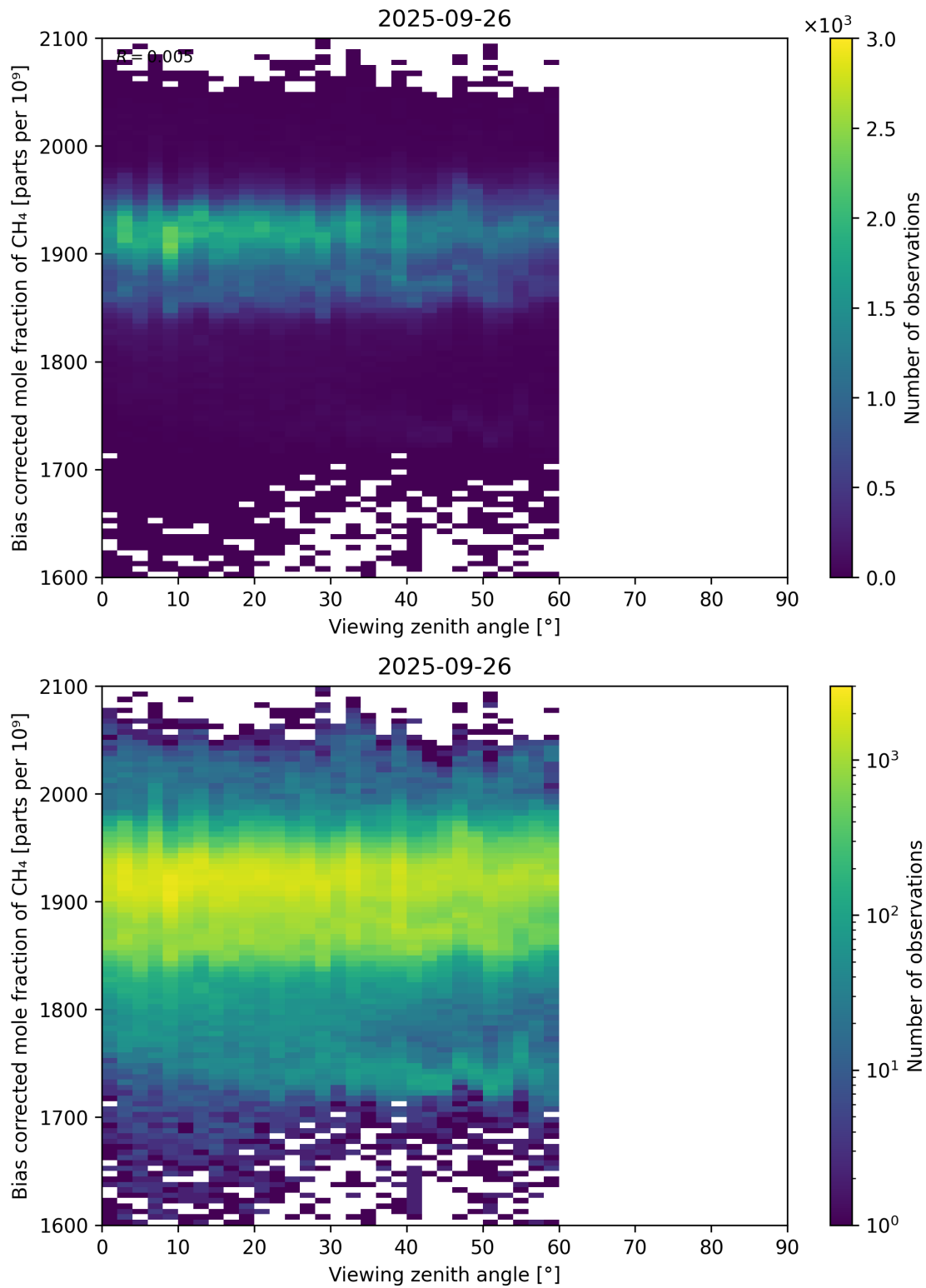
Figure 111: Scatter density plot of “Viewing zenith angle” against “Bias corrected mole fraction of CH 4 ” for 2025-09-26 to 2025-09-27.
