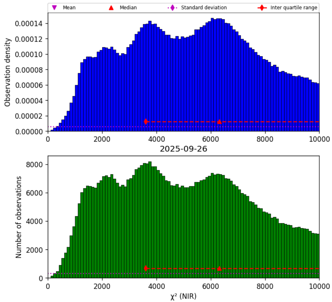
Figure 29: Histogram of " \chi^2 (NIR)" for 2025-09-26 to 2025-09-27
