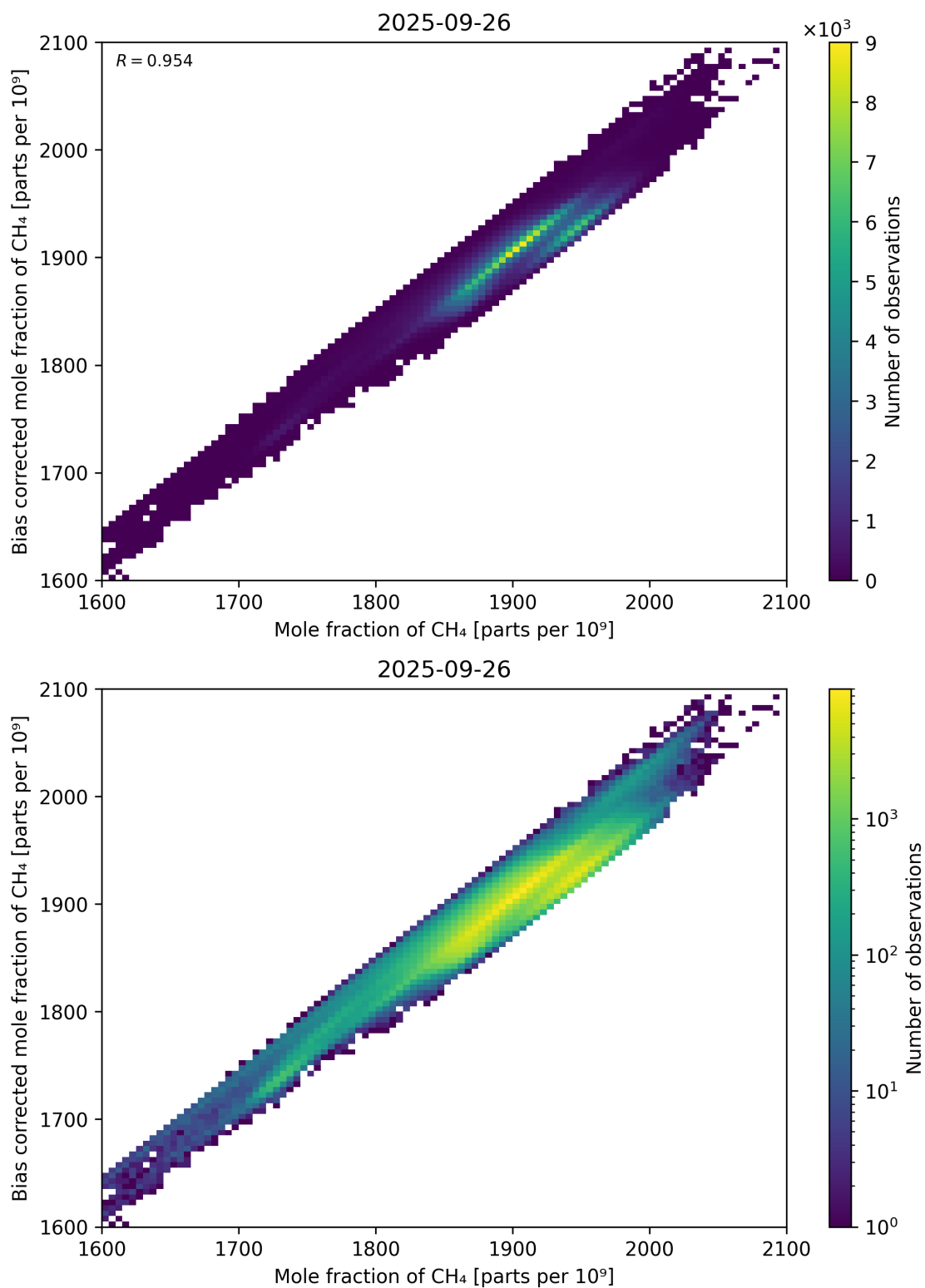
Figure 74: Scatter density plot of “Mole fraction of CH 4 ” against “Bias corrected mole fraction of CH 4 ” for 2025-09-26 to 2025-09-27.
