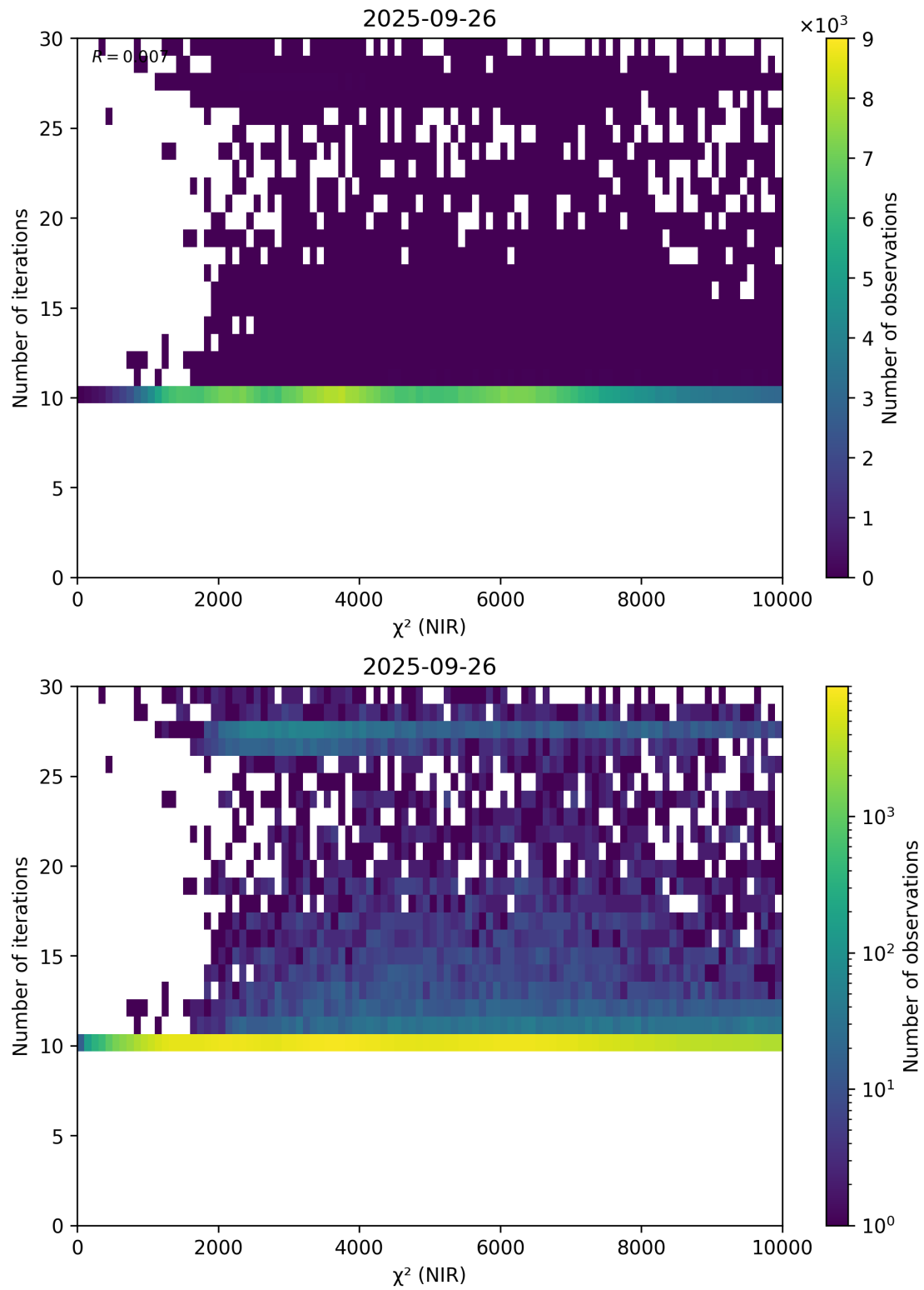
Figure 46: Scatter density plot of “ \chi^2 (NIR)” against “Number of iterations” for 2025-09-26 to 2025-09-27.
