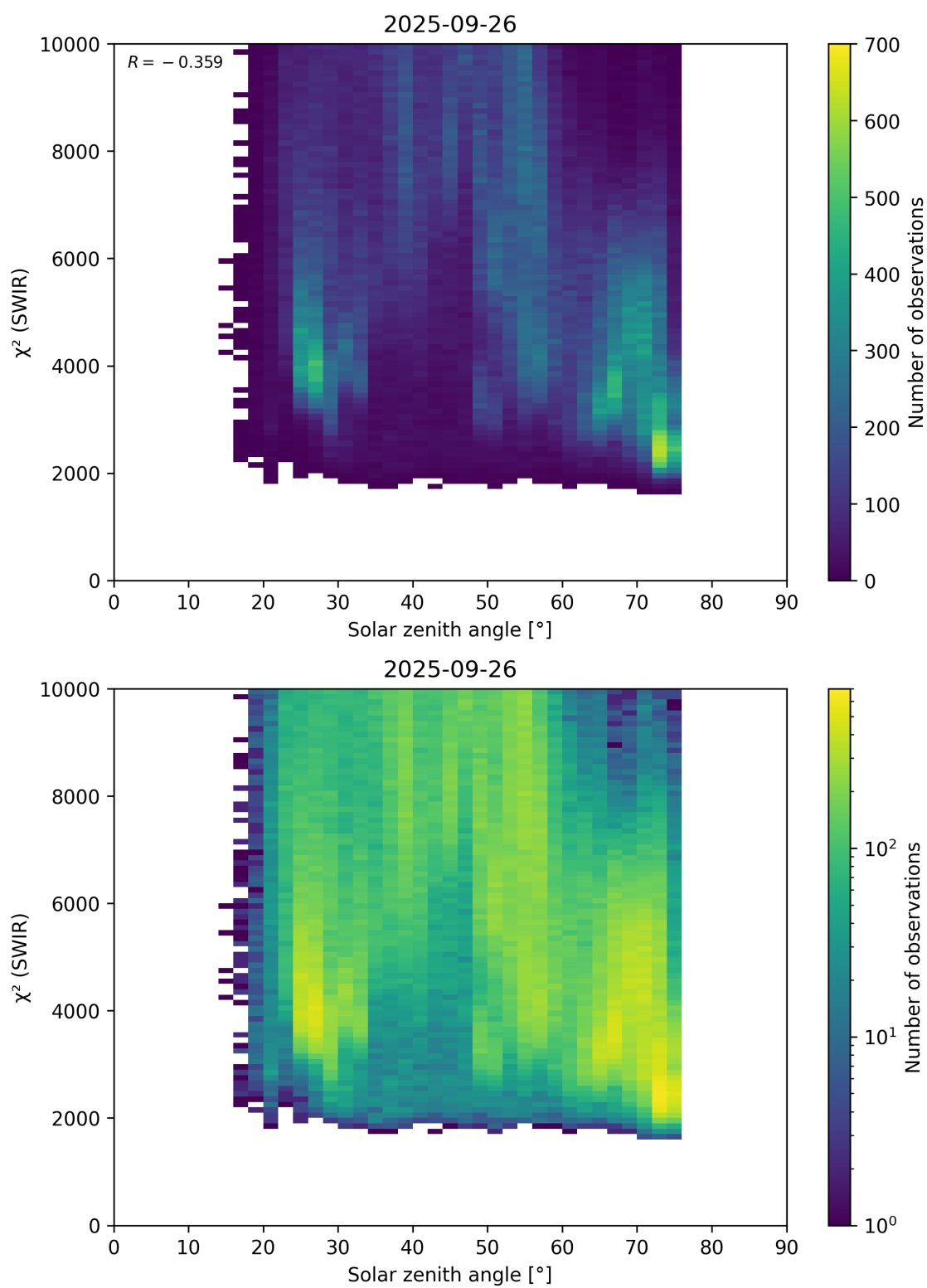
Figure 95: Scatter density plot of “Solar zenith angle” against “ \chi^2 (SWIR)” for 2025-09-26 to 2025-09-27.
