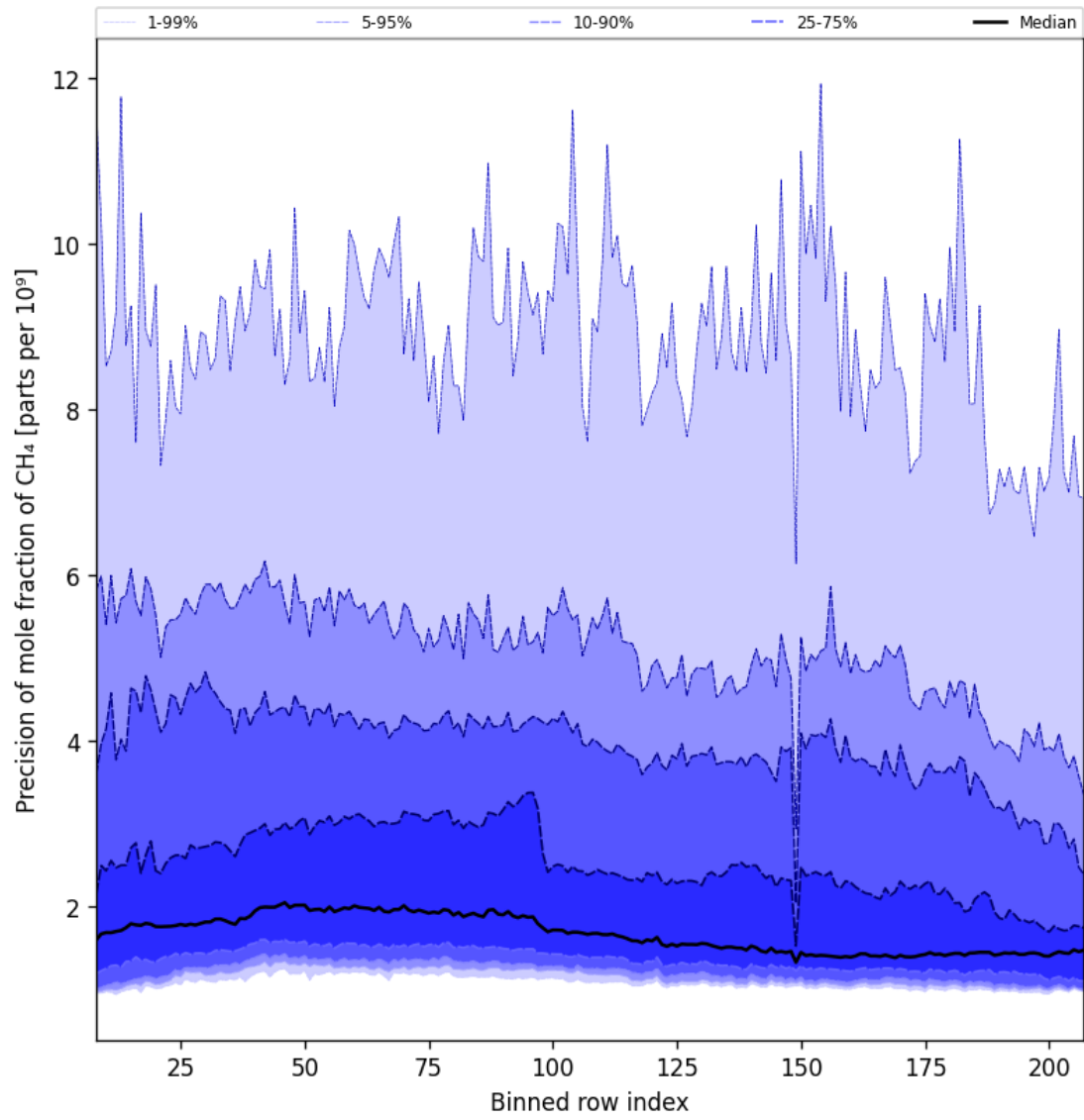
Figure 35: Along track statistics of "Precision of mole fraction of CH 4 " for 2025-09-26 to 2025-09-27
