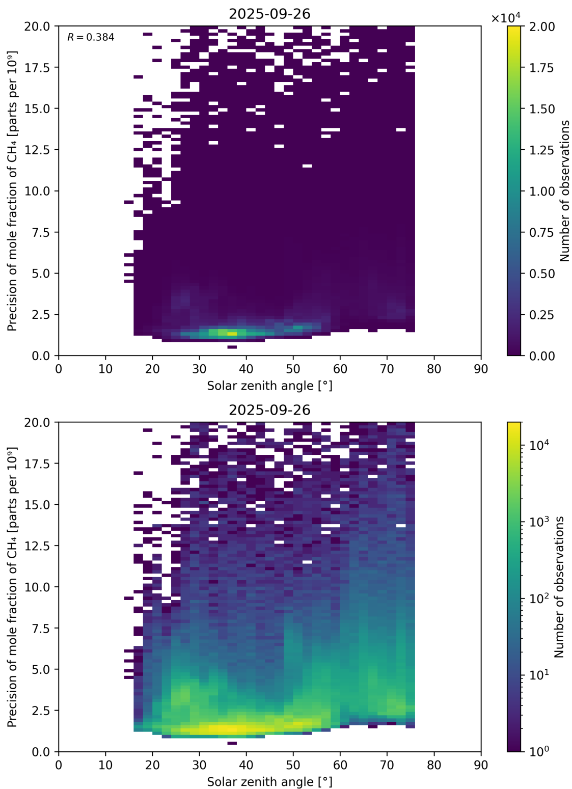
Figure 101: Scatter density plot of “Solar zenith angle” against “Precision of mole fraction of \text{CH}_4 ” for 2025-09-26 to 2025-09-27.
