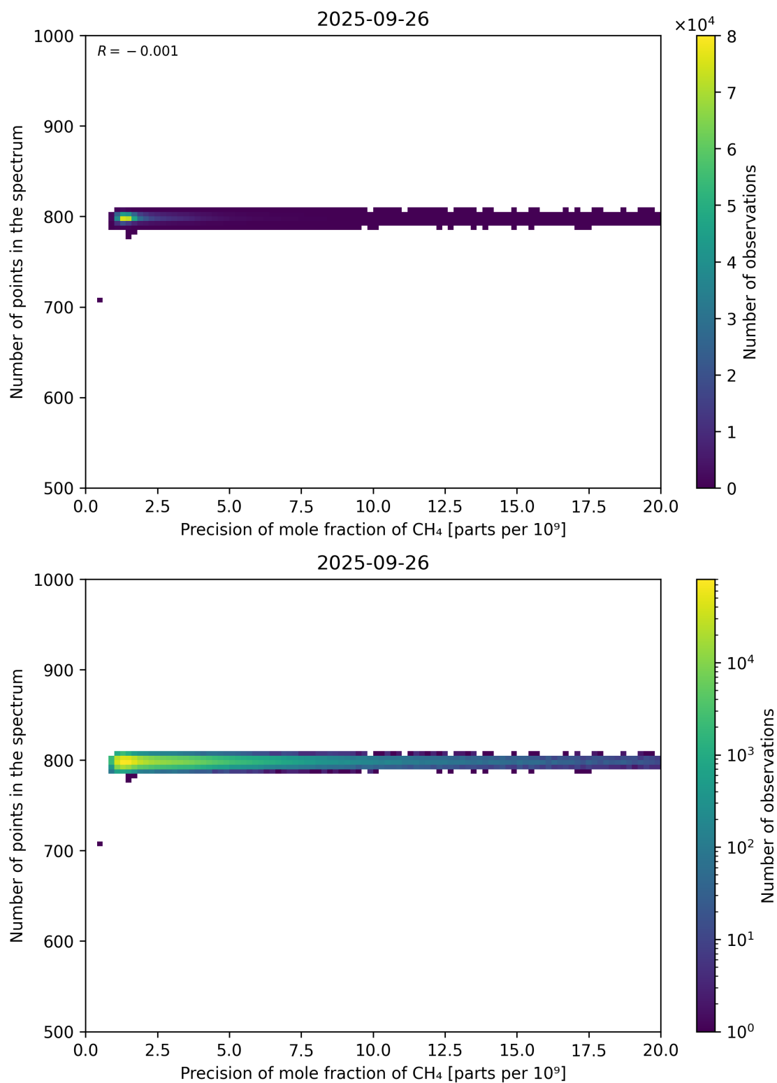
Figure 84: Scatter density plot of “Precision of mole fraction of CH 4 ” against “Number of points in the spectrum” for 2025-09-26 to 2025-09-27.
