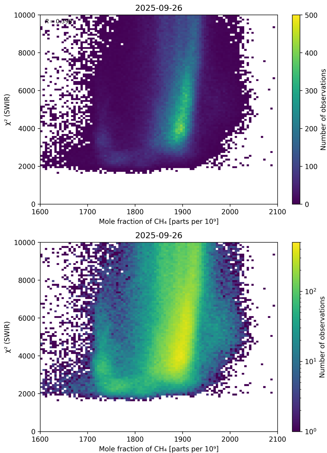
Figure 71: Scatter density plot of “Mole fraction of CH 4 ” against “ \chi^2 (SWIR)” for 2025-09-26 to 2025-09-27.
