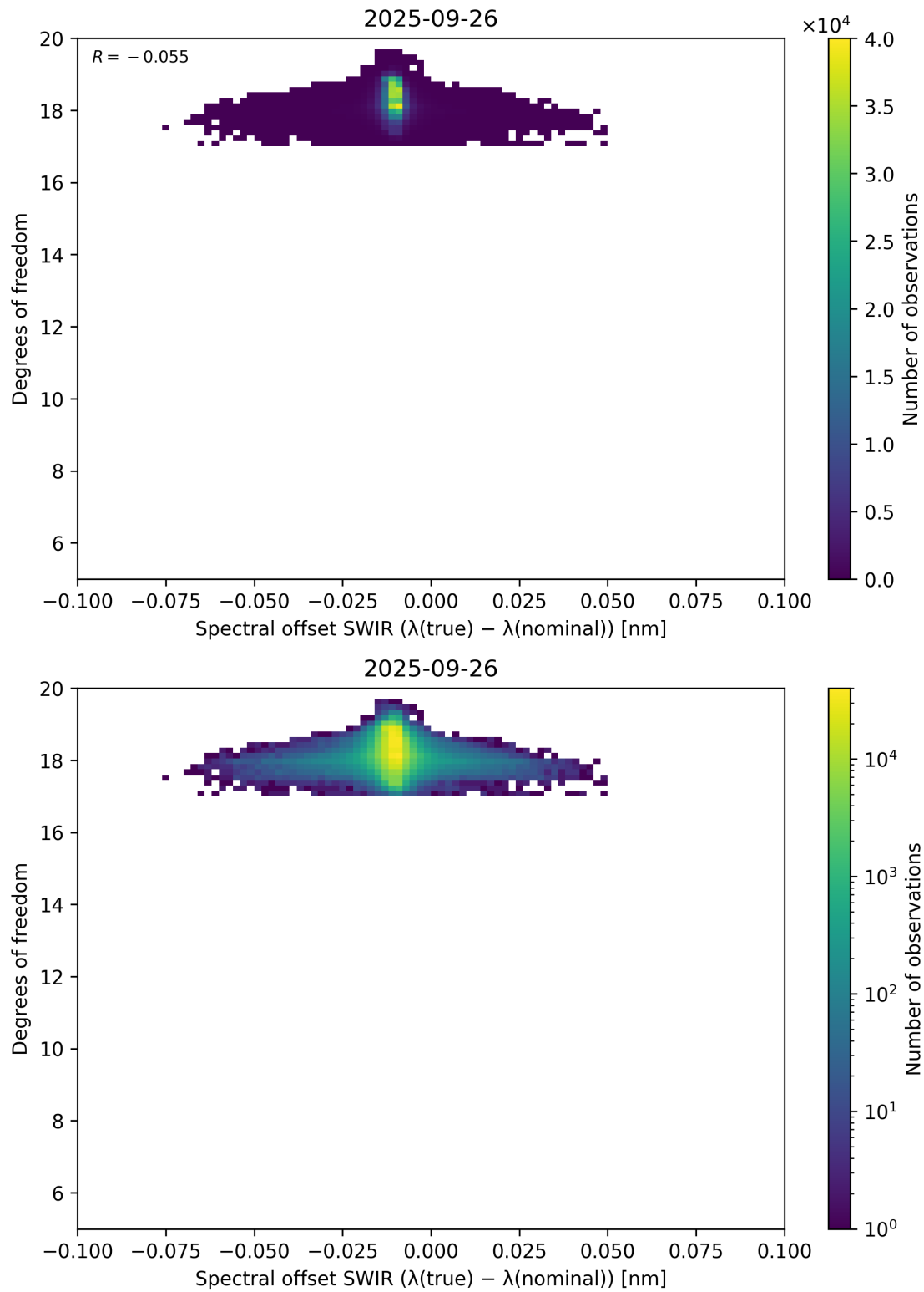
Figure 119: Scatter density plot of “Spectral offset SWIR ( \lambda_{\text{true}} - \lambda_{\text{nominal}} )” against “Degrees of freedom” for 2025-09-26 to 2025-09-27.
