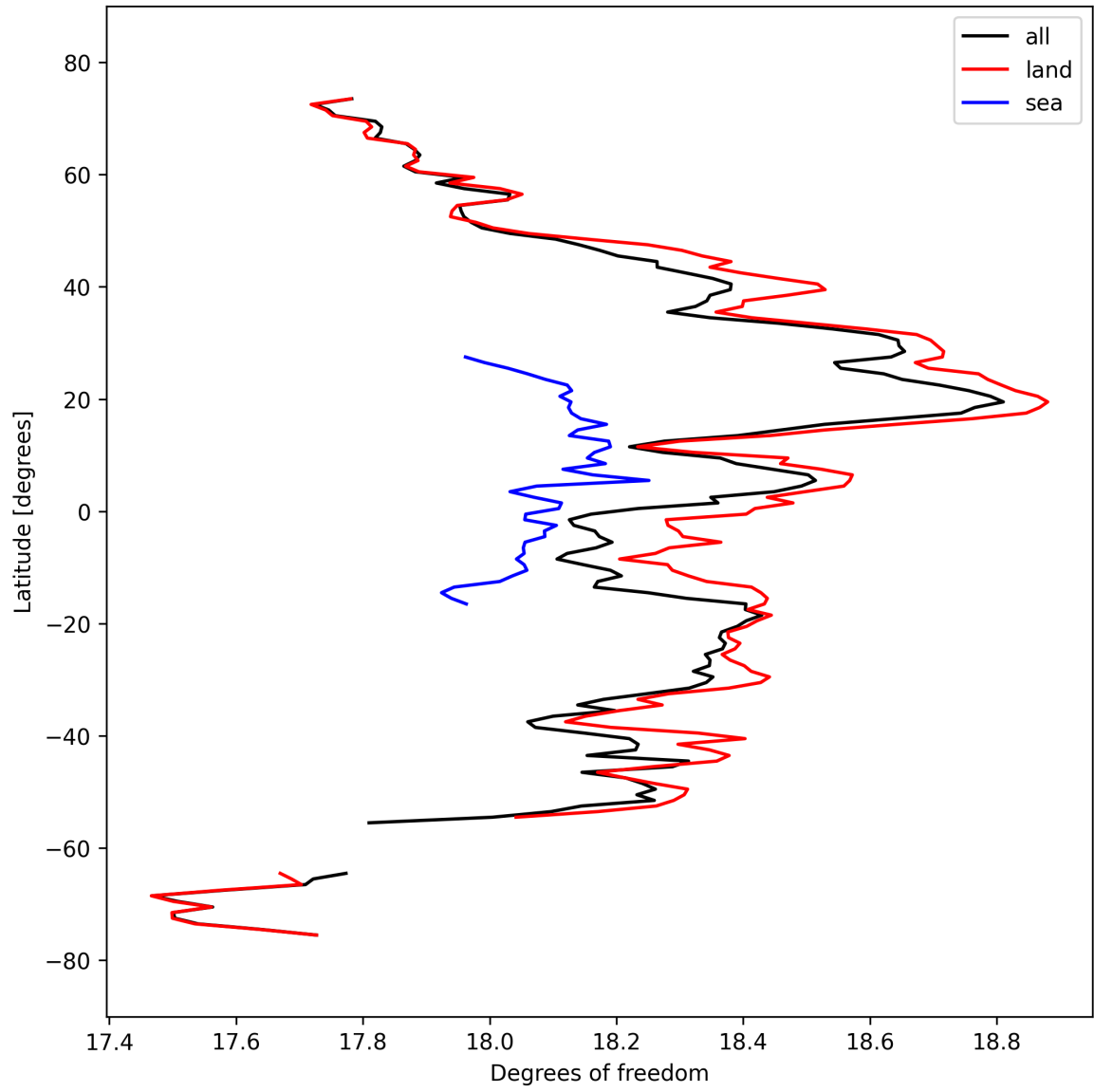
Figure 19: Zonal average of “Degrees of freedom” for 2025-09-26 to 2025-09-27.
