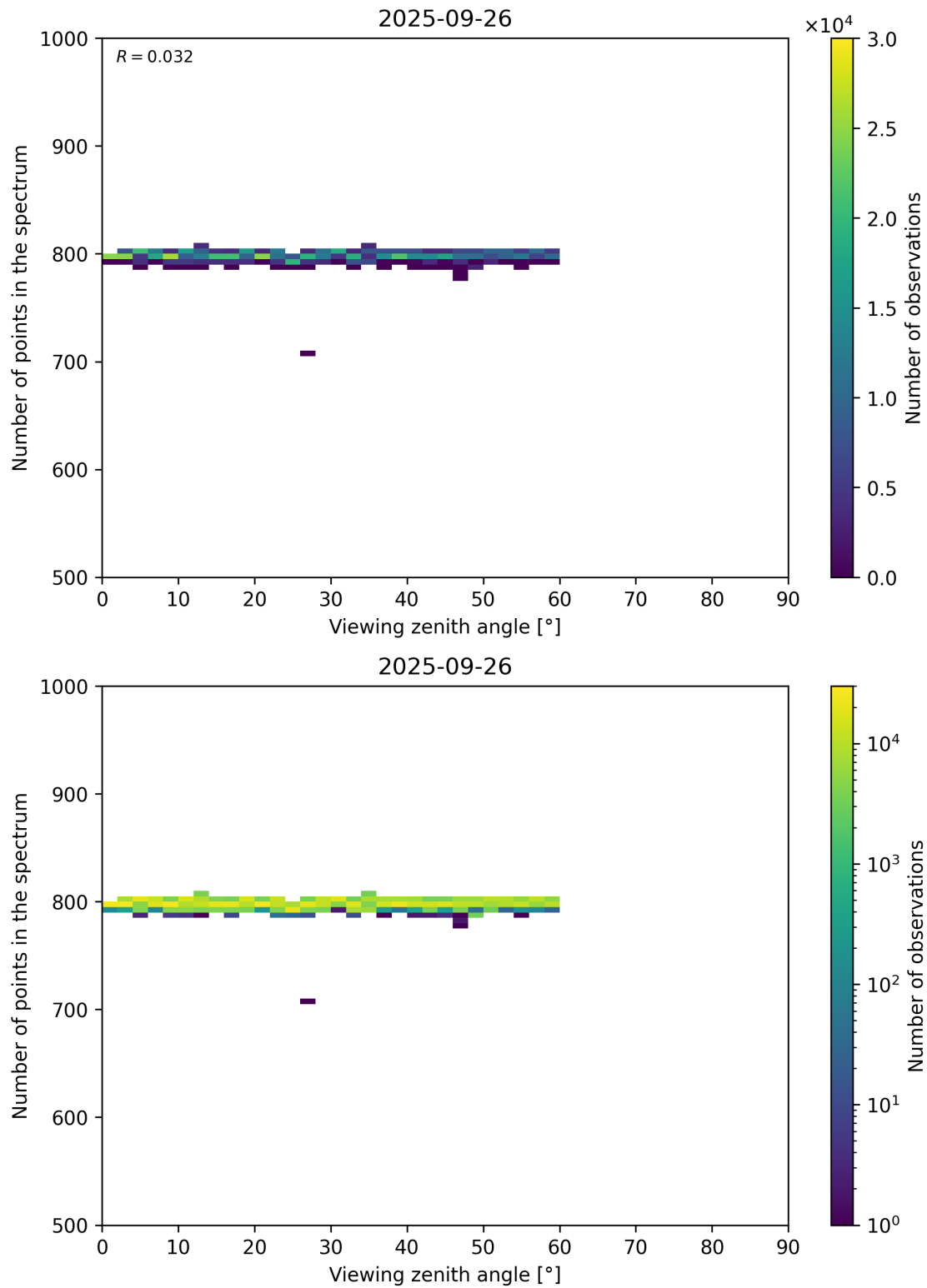
Figure 114: Scatter density plot of “Viewing zenith angle” against “Number of points in the spectrum” for 2025-09-26 to 2025-09-27.
