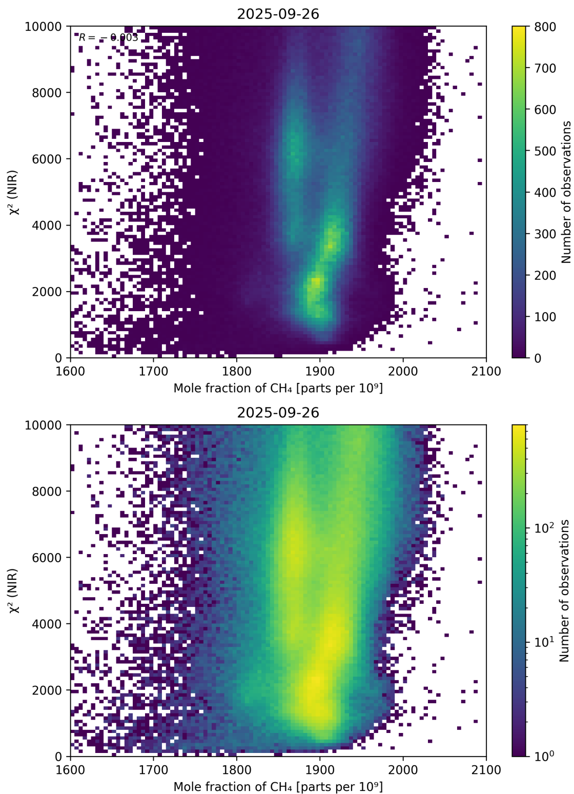
Figure 70: Scatter density plot of “Mole fraction of CH 4 ” against “ \chi^2 (NIR)” for 2025-09-26 to 2025-09-27.
