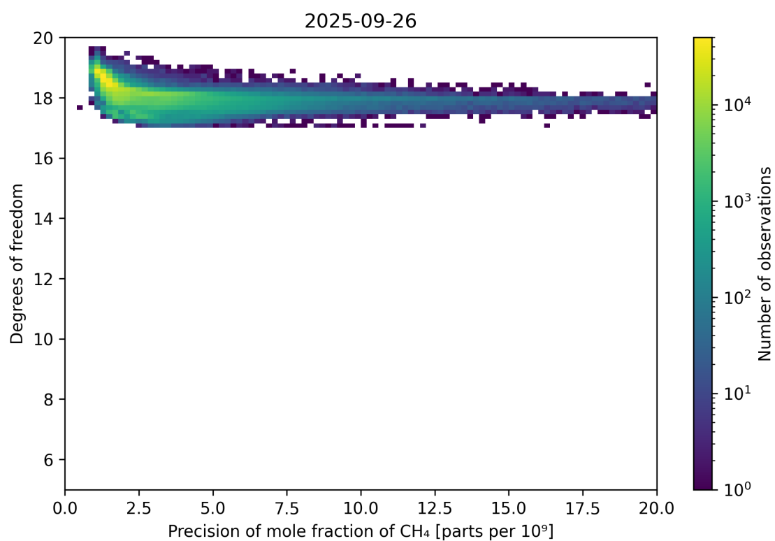
Figure 80: Scatter density plot of “Precision of mole fraction of CH 4 ” against “Degrees of freedom” for 2025-09-26 to 2025-09-27.
