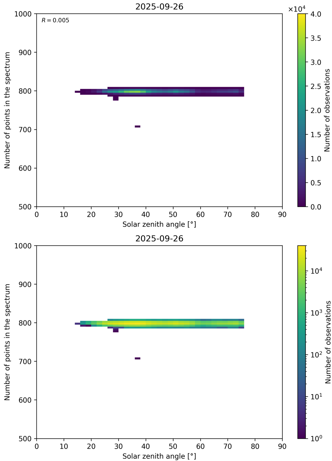
Figure 103: Scatter density plot of “Solar zenith angle” against “Number of points in the spectrum” for 2025-09-26 to 2025-09-27.
