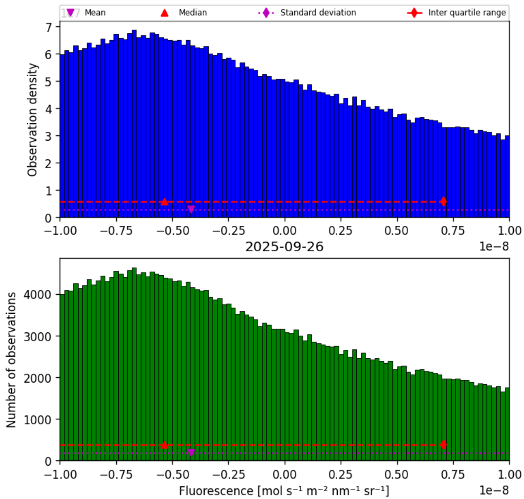
Figure 32: Histogram of “Fluorescence” for 2025-09-26 to 2025-09-27
