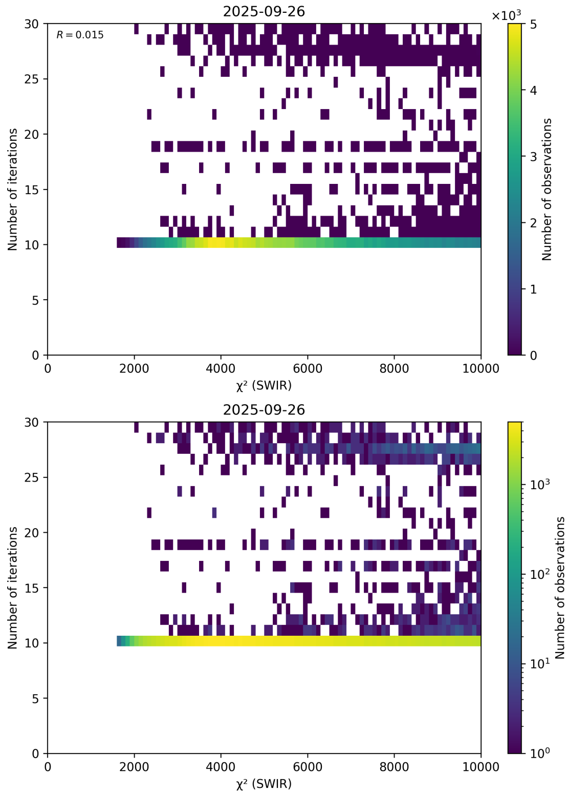
Figure 50: Scatter density plot of “ \chi^2 (SWIR)” against “Number of iterations” for 2025-09-26 to 2025-09-27.
