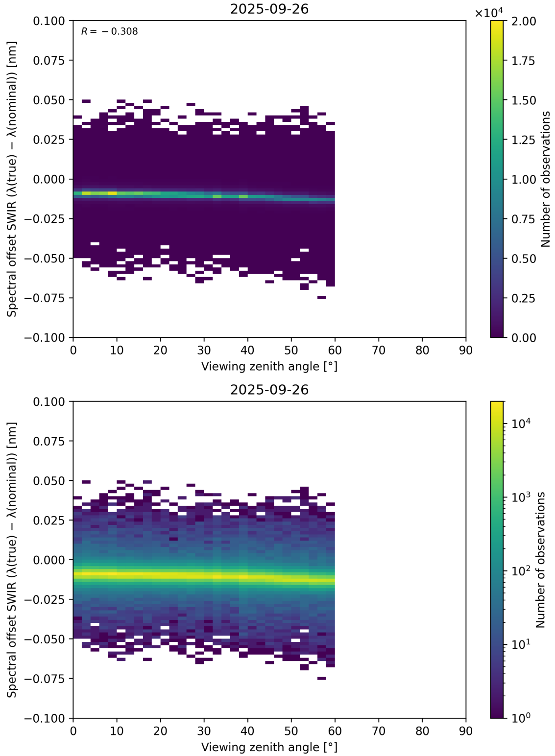
Figure 116: Scatter density plot of “Viewing zenith angle” against “Spectral offset SWIR ( \lambda_{\text{true}} - \lambda_{\text{nominal}} )” for 2025-09-26 to 2025-09-27.
