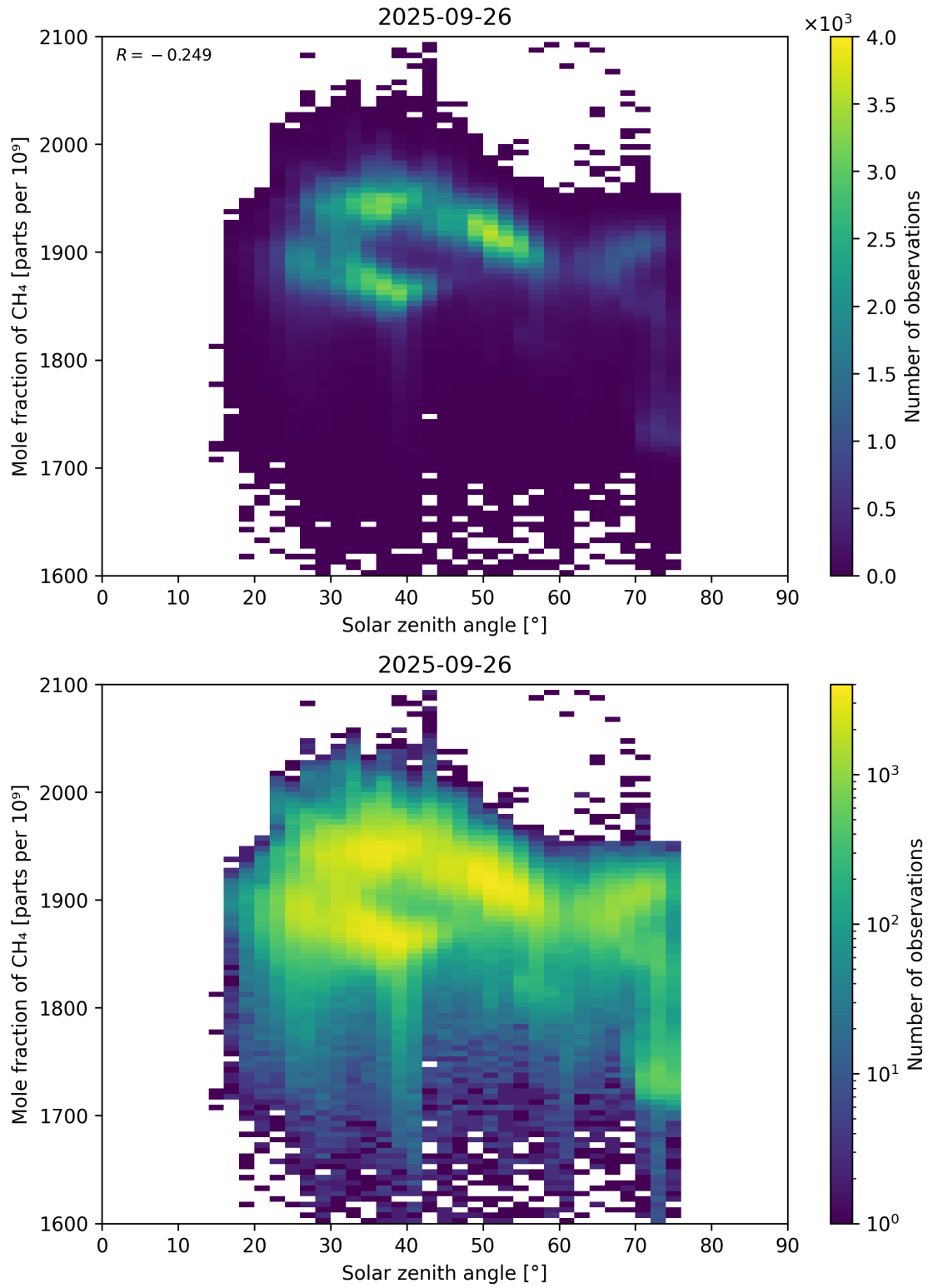
Figure 99: Scatter density plot of “Solar zenith angle” against “Mole fraction of \text{CH}_4 ” for 2025-09-26 to 2025-09-27.
