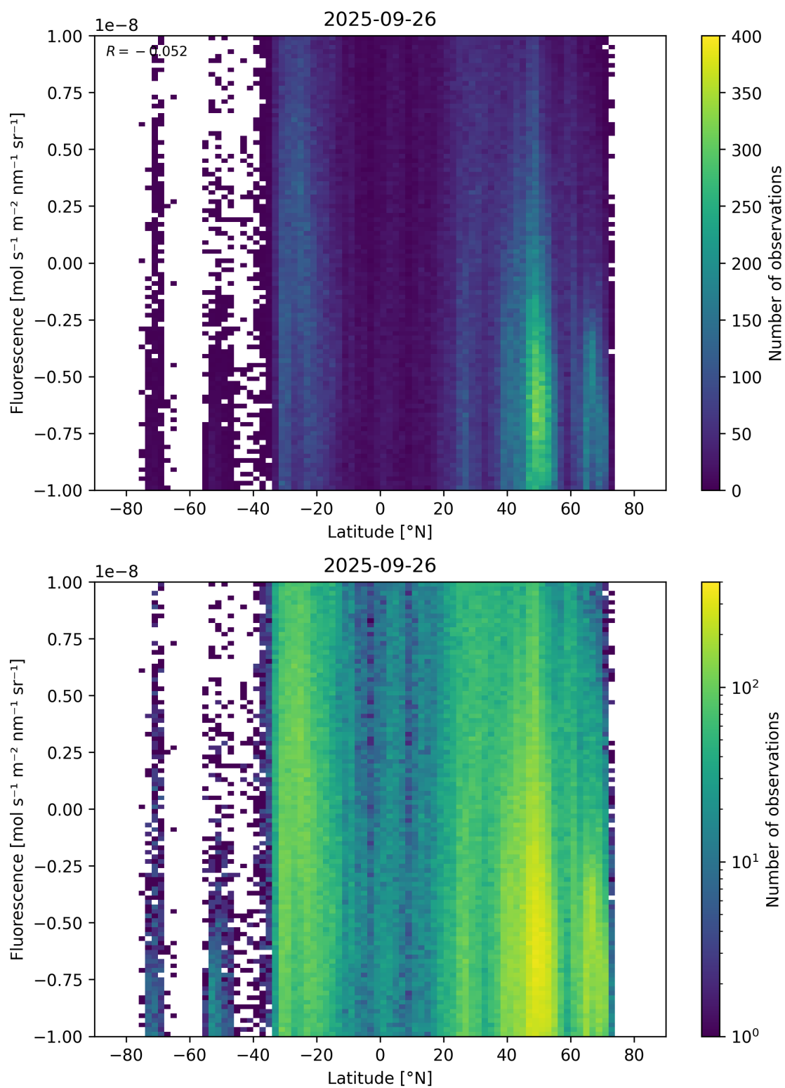
Figure 56: Scatter density plot of “Latitude” against “Fluorescence” for 2025-09-26 to 2025-09-27.
