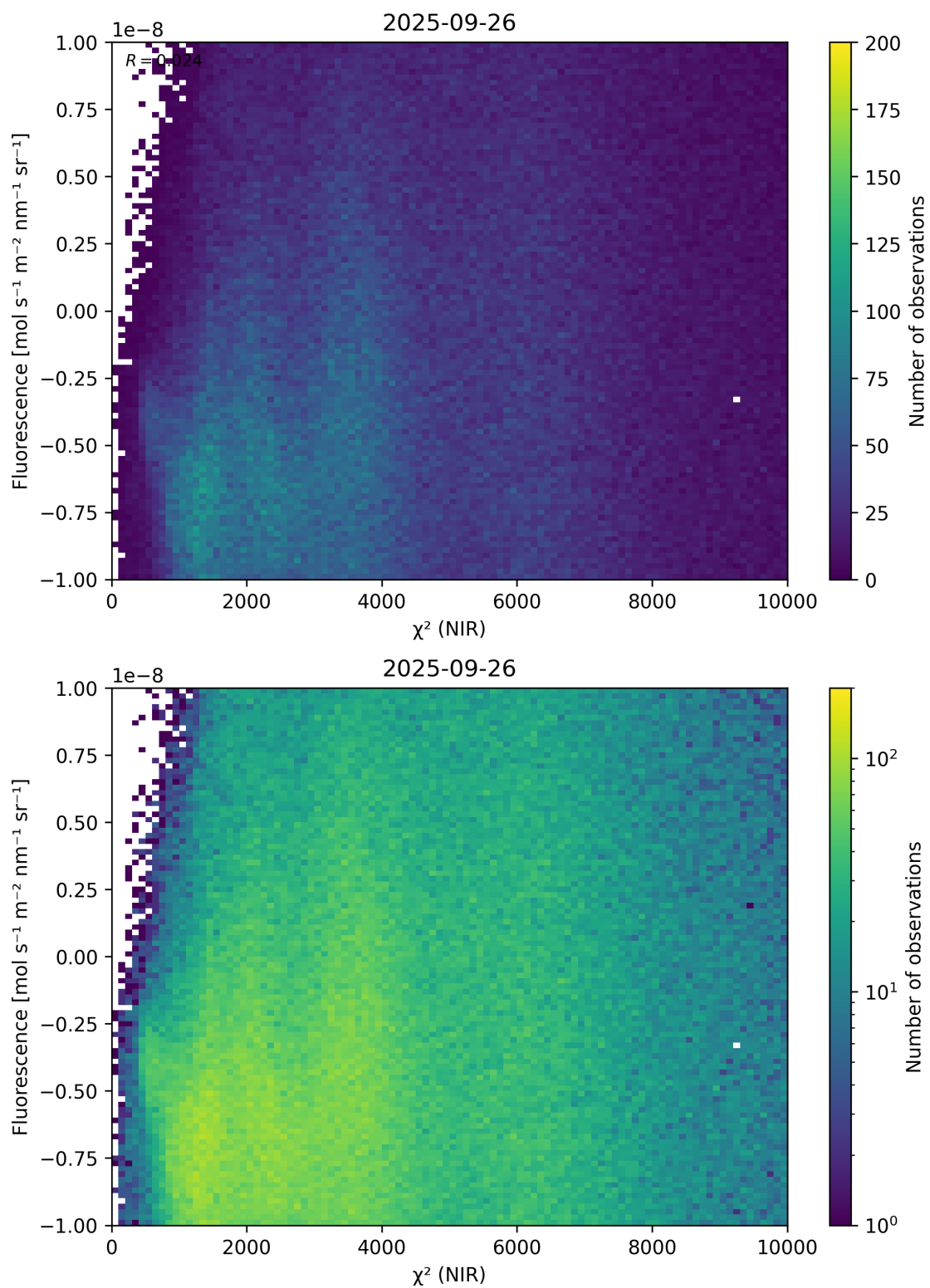
Figure 45: Scatter density plot of “ \chi^2 (NIR)” against “Fluorescence” for 2025-09-26 to 2025-09-27.
