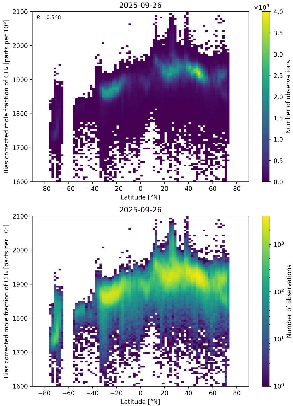
Figure 58: Scatter density plot of “Latitude” against “Bias corrected mole fraction of CH 4 ” for 2025-09-26 to 2025-09-27.
