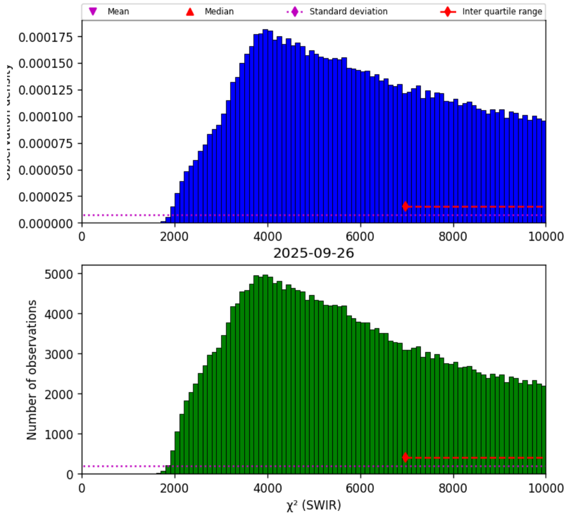
Figure 28: Histogram of “ \chi^2 (SWIR)” for 2025-09-26 to 2025-09-27
