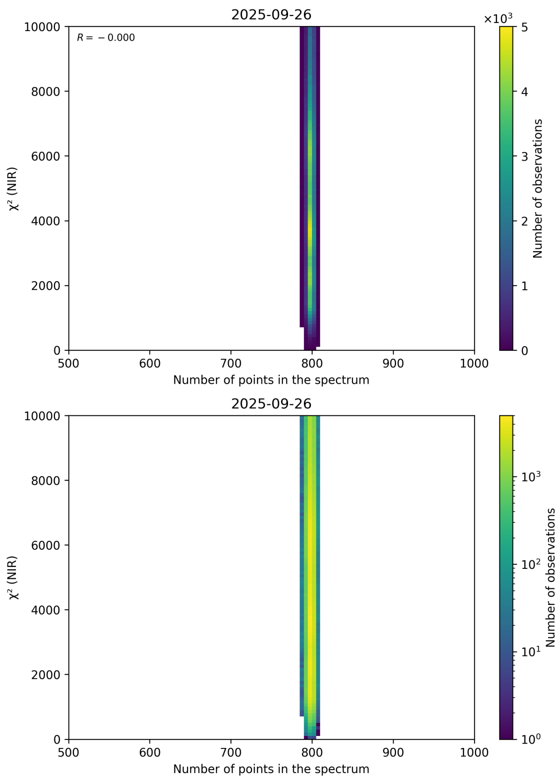
Figure 88: Scatter density plot of “Number of points in the spectrum” against “ \chi^2 (NIR)” for 2025-09-26 to 2025-09-27.
