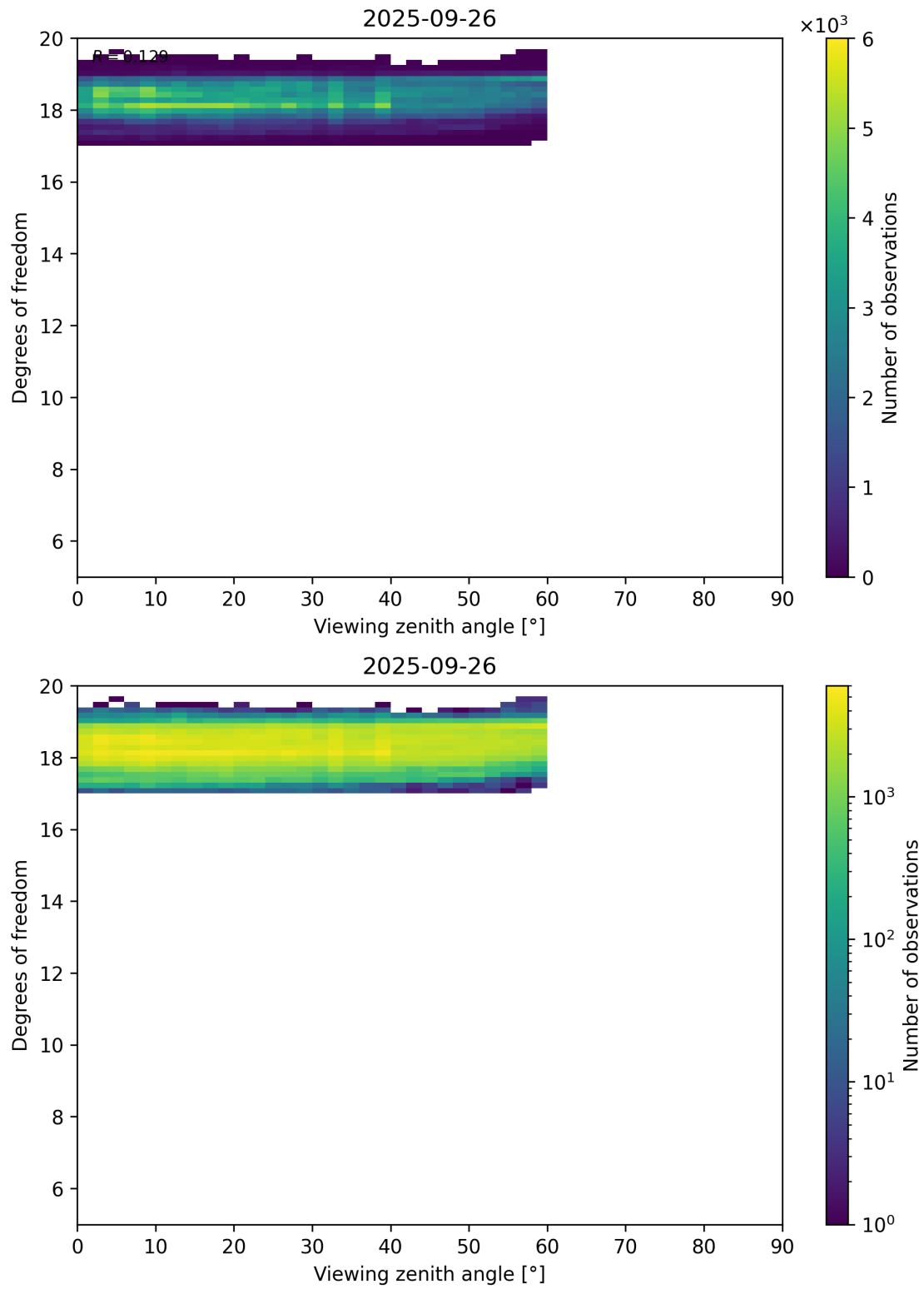
Figure 107: Scatter density plot of “Viewing zenith angle” against “Degrees of freedom” for 2025-09-26 to 2025-09-27.
