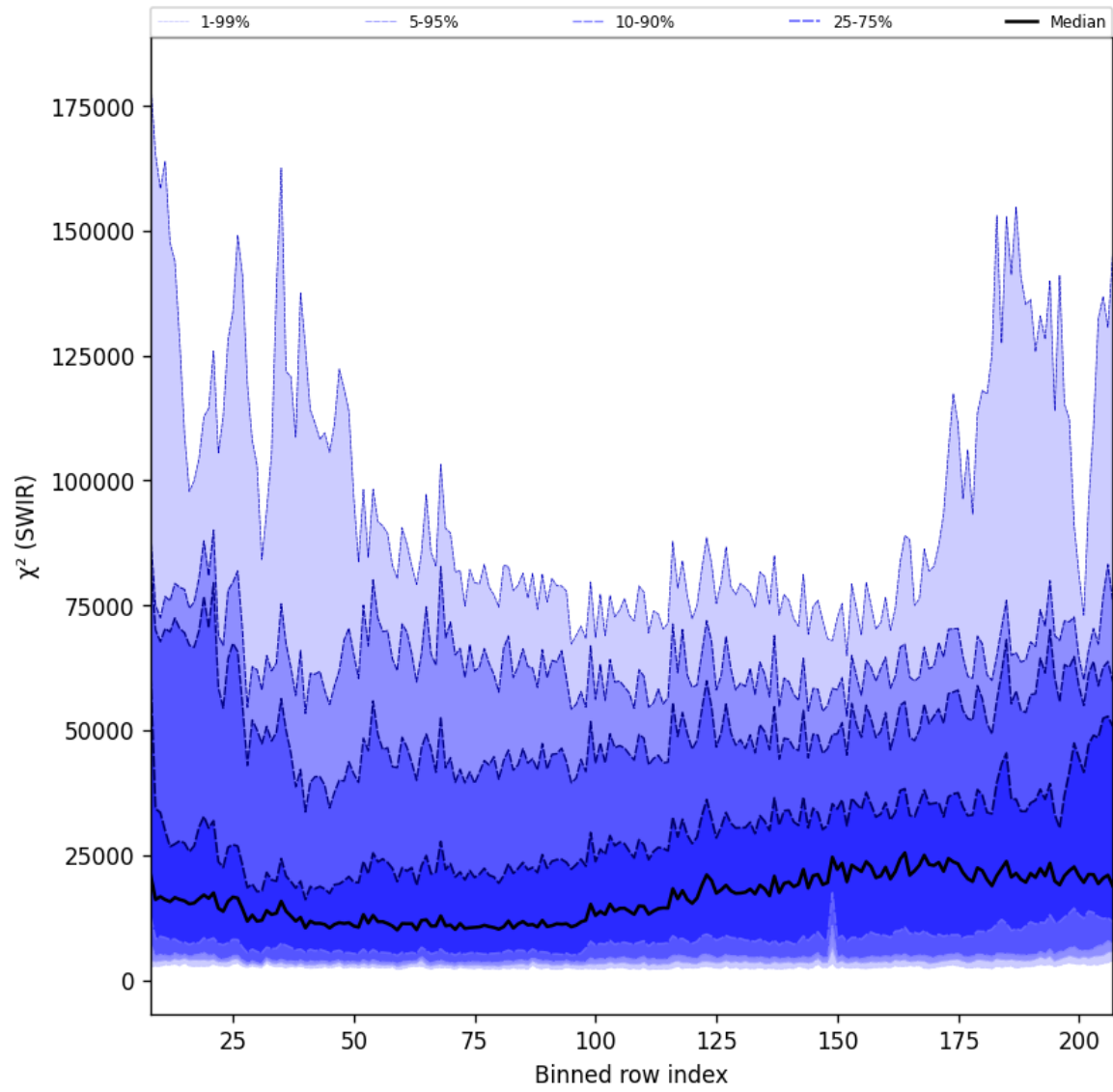
Figure 39: Along track statistics of " \chi^2 (SWIR)" for 2025-09-26 to 2025-09-27
