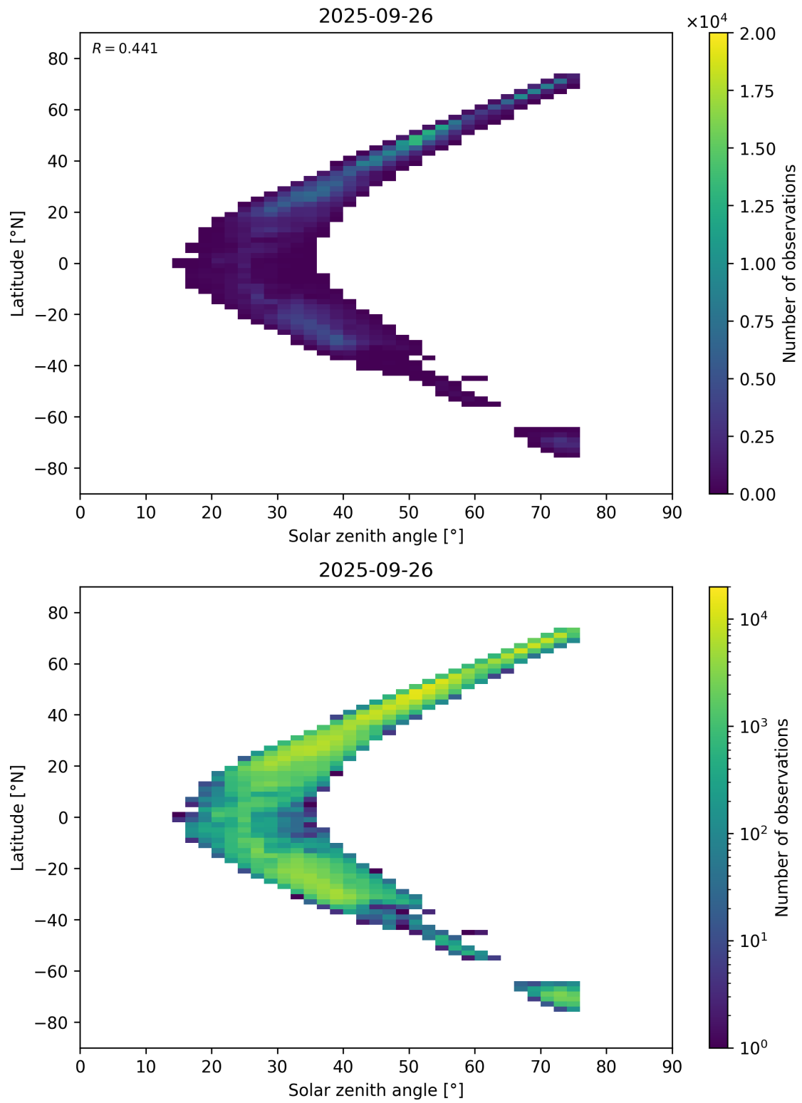
Figure 98: Scatter density plot of “Solar zenith angle” against “Latitude” for 2025-09-26 to 2025-09-27.
