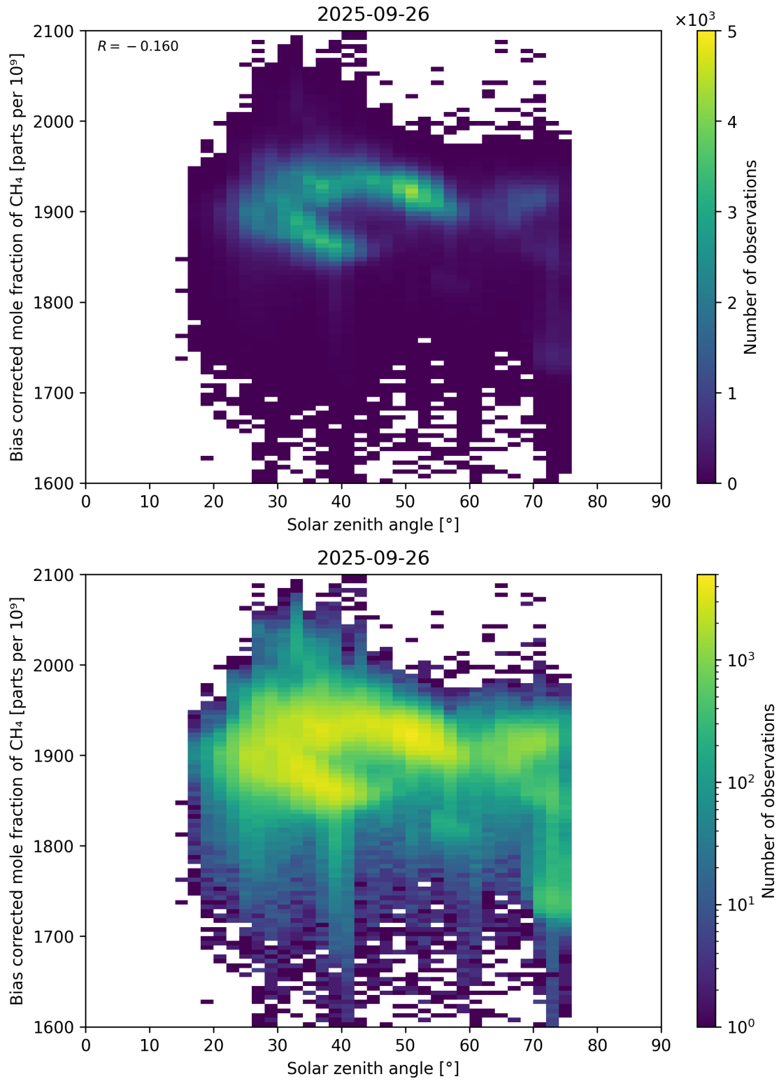
Figure 100: Scatter density plot of “Solar zenith angle” against “Bias corrected mole fraction of CH 4 ” for 2025-09-26 to 2025-09-27.
