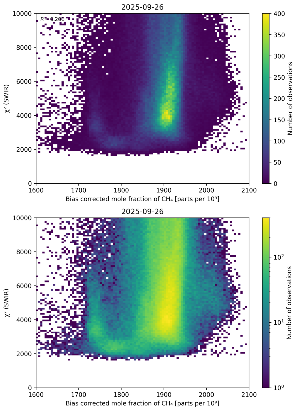
Figure 64: Scatter density plot of “Bias corrected mole fraction of \text{CH}_4 ” against “ \chi^2 (SWIR)” for 2025-09-26 to 2025-09-27.
