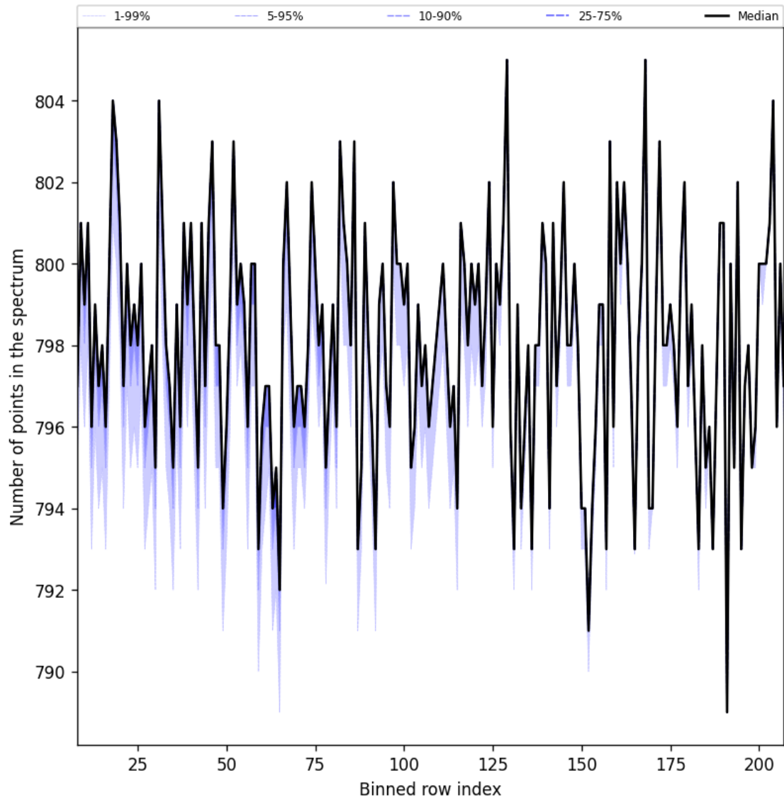
Figure 37: Along track statistics of “Number of points in the spectrum” for 2025-09-26 to 2025-09-27
