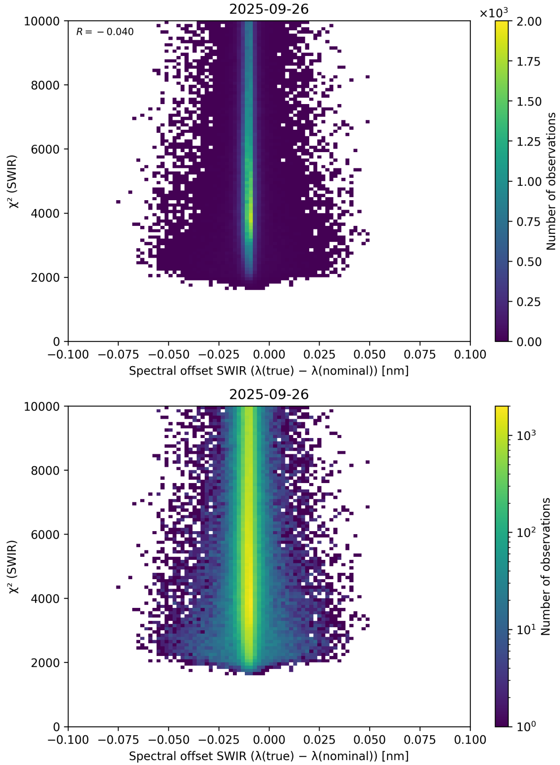
Figure 118: Scatter density plot of “Spectral offset SWIR ( \lambda_{\text{true}} - \lambda_{\text{nominal}} )” against “ \chi^2 (SWIR)” for 2025-09-26 to 2025-09-27.
