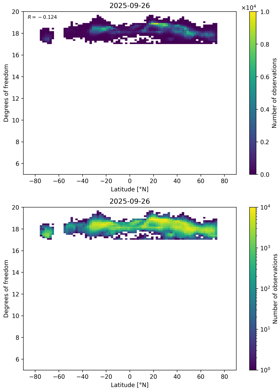
Figure 55: Scatter density plot of “Latitude” against “Degrees of freedom” for 2025-09-26 to 2025-09-27.
