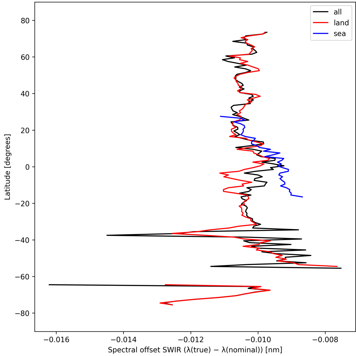
Figure 16: Zonal average of “Spectral offset SWIR ( \lambda_{\text{true}} - \lambda_{\text{nominal}} )” for 2025-09-26 to 2025-09-27.
