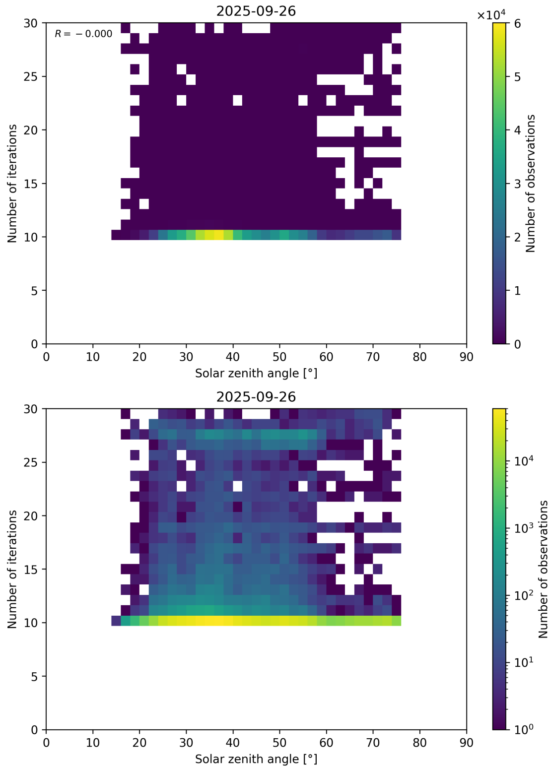
Figure 102: Scatter density plot of “Solar zenith angle” against “Number of iterations” for 2025-09-26 to 2025-09-27.
