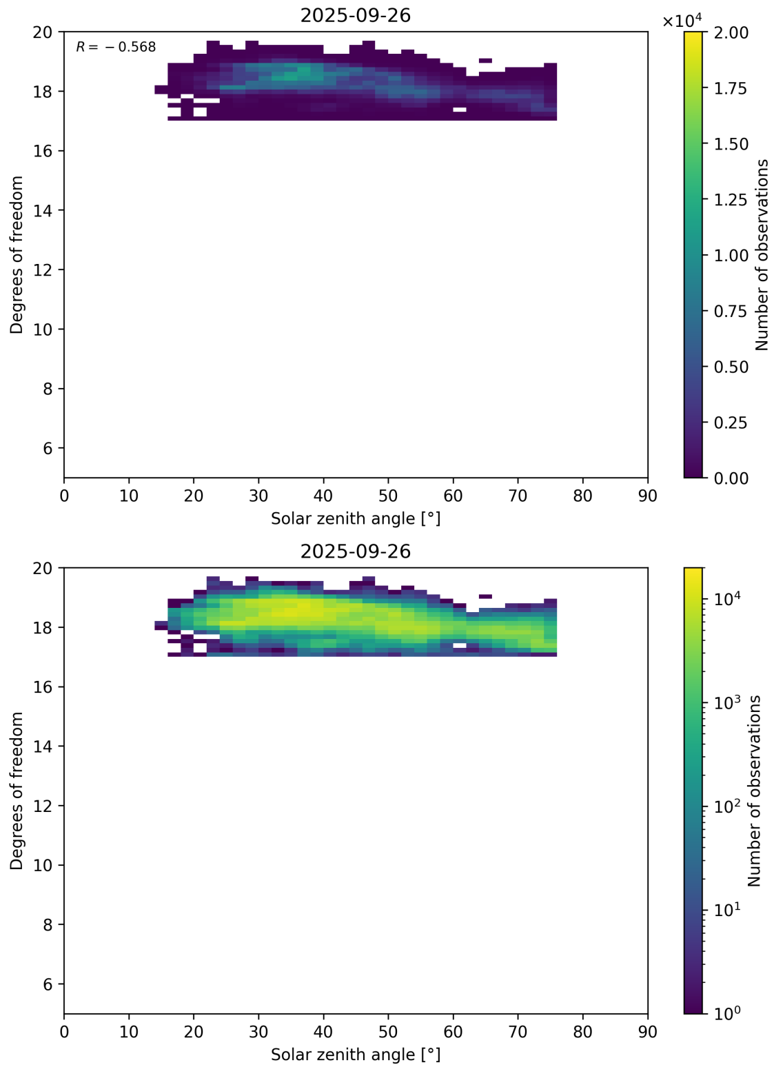
Figure 96: Scatter density plot of “Solar zenith angle” against “Degrees of freedom” for 2025-09-26 to 2025-09-27.
