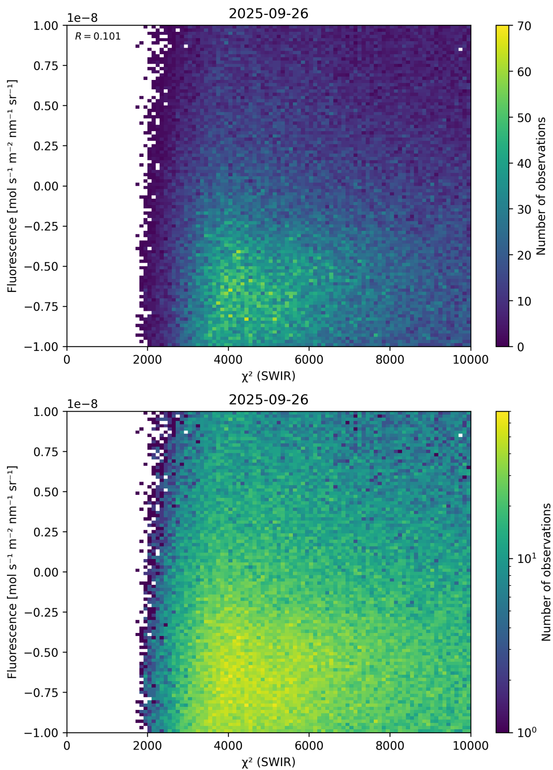
Figure 49: Scatter density plot of “ \chi^2 (SWIR)” against “Fluorescence” for 2025-09-26 to 2025-09-27.
