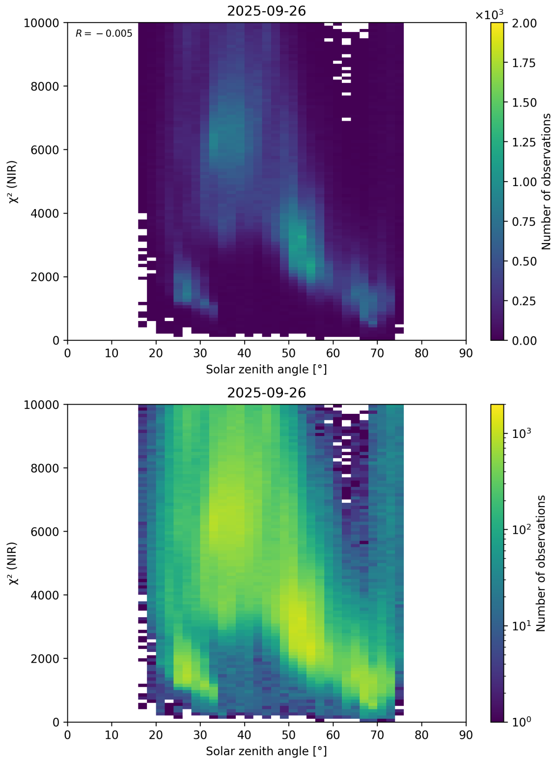
Figure 94: Scatter density plot of “Solar zenith angle” against “ \chi^2 (NIR)” for 2025-09-26 to 2025-09-27.
