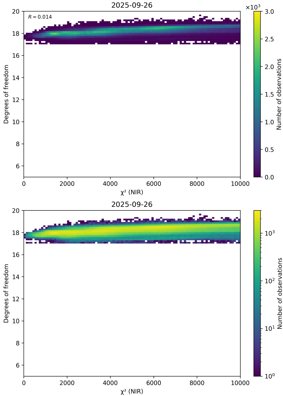
Figure 44: Scatter density plot of “ \chi^2 (NIR)” against “Degrees of freedom” for 2025-09-26 to 2025-09-27.
