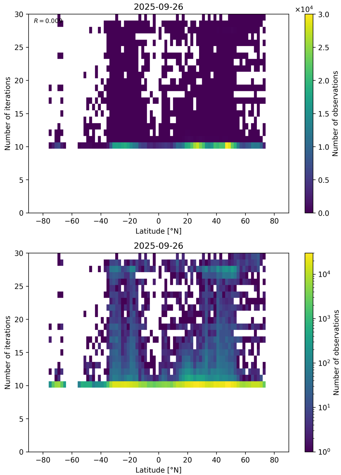
Figure 60: Scatter density plot of “Latitude” against “Number of iterations” for 2025-09-26 to 2025-09-27.
