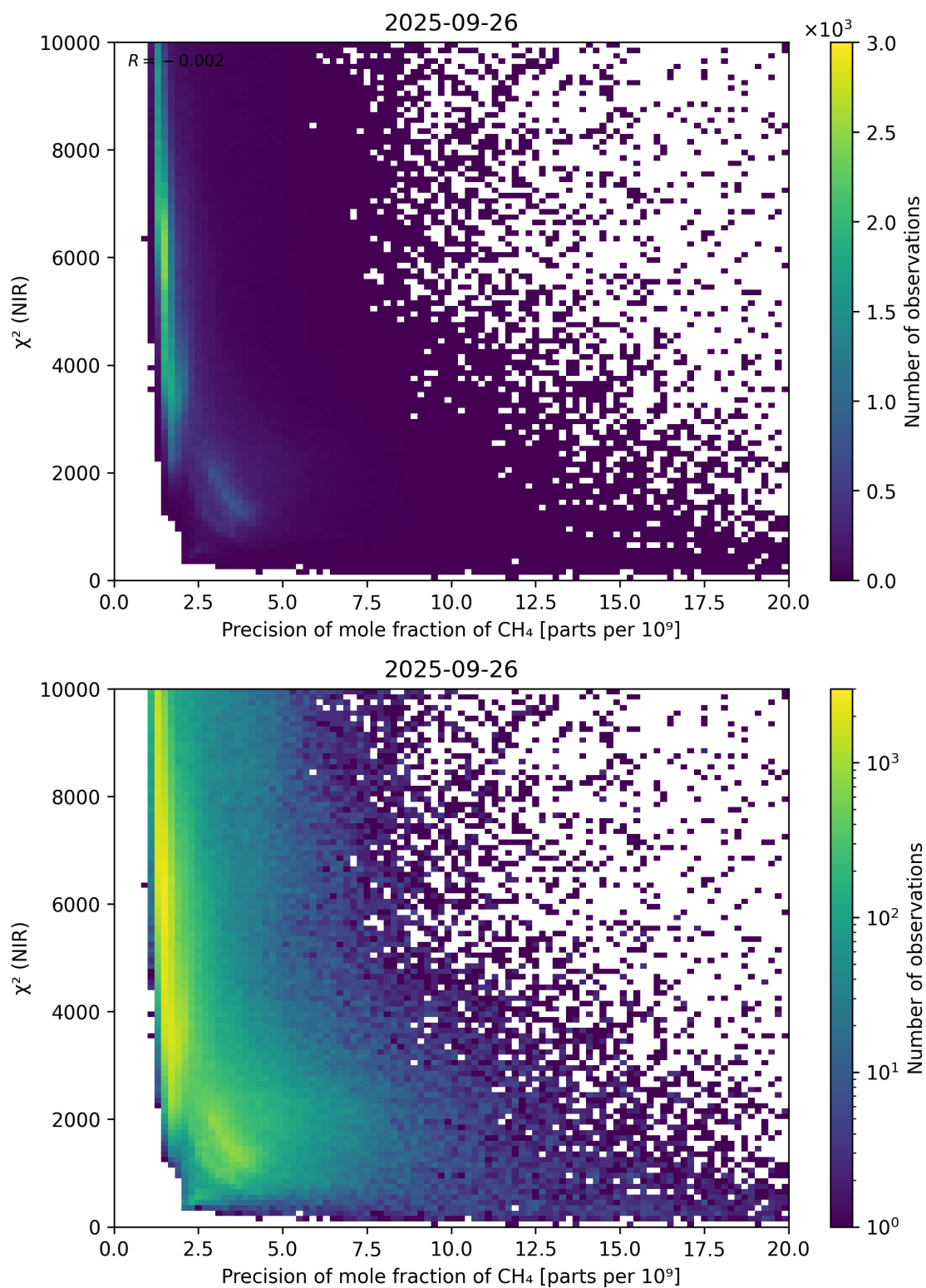
Figure 78: Scatter density plot of “Precision of mole fraction of CH 4 ” against “ \chi^2 (NIR)” for 2025-09-26 to 2025-09-27.
