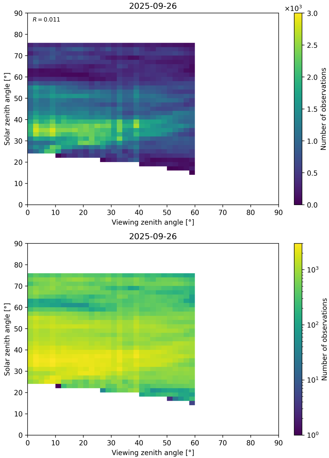
Figure 115: Scatter density plot of “Viewing zenith angle” against “Solar zenith angle” for 2025-09-26 to 2025-09-27.
