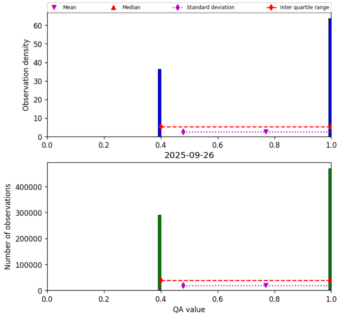
Figure 22: Histogram of “QA value” for 2025-09-26 to 2025-09-27
