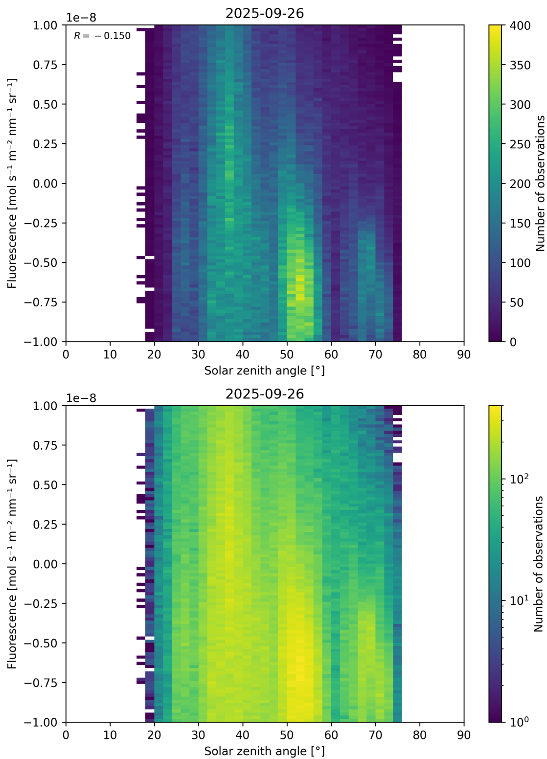
Figure 97: Scatter density plot of “Solar zenith angle” against “Fluorescence” for 2025-09-26 to 2025-09-27.
