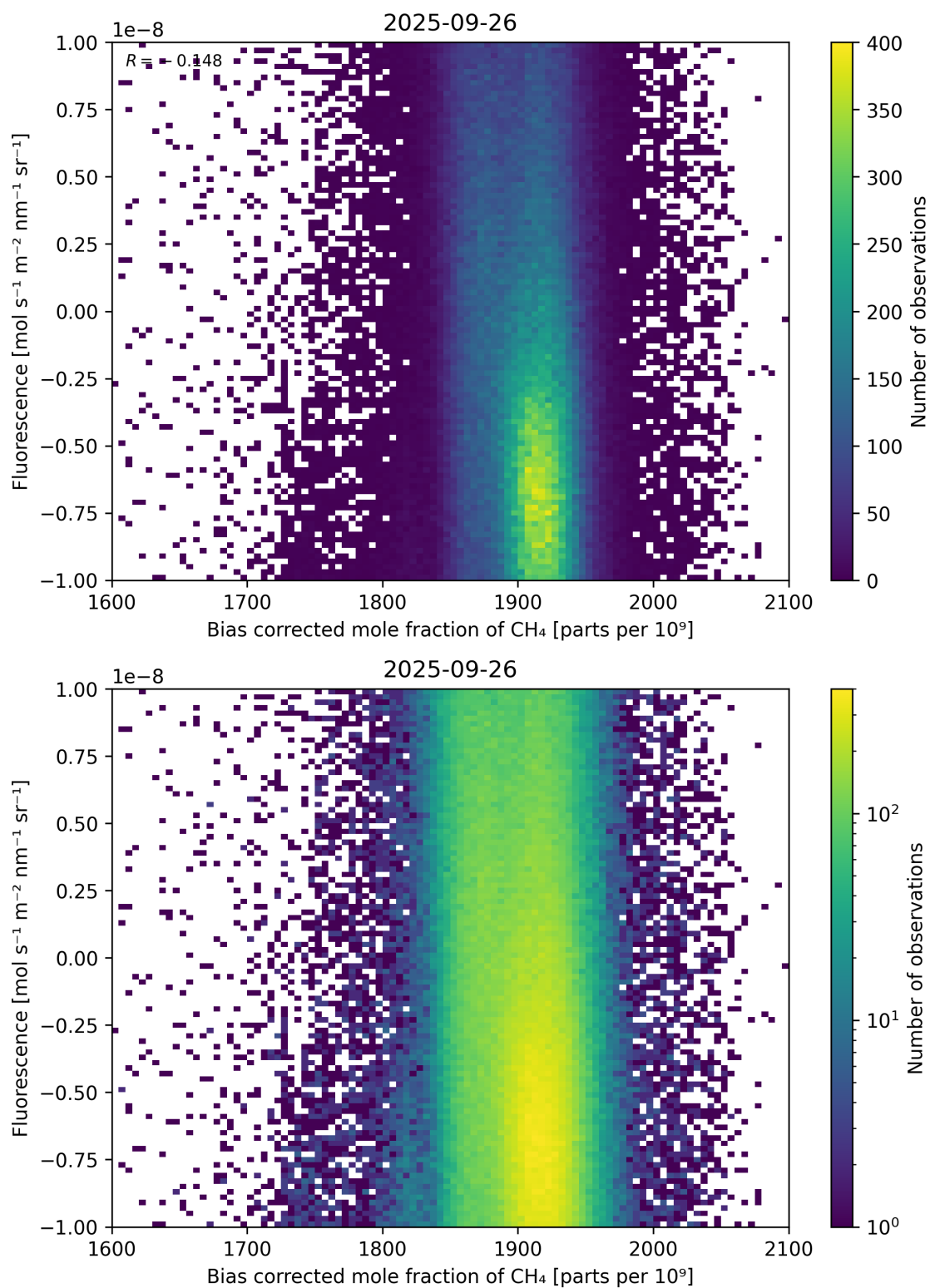
Figure 66: Scatter density plot of “Bias corrected mole fraction of \text{CH}_4 ” against “Fluorescence” for 2025-09-26 to 2025-09-27.
