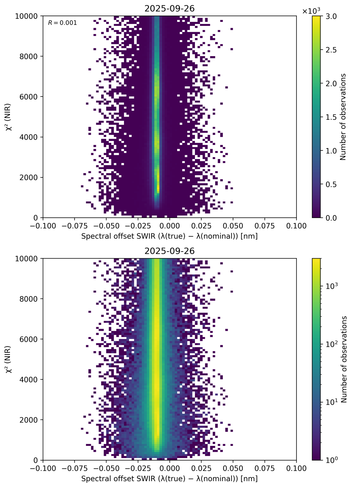
Figure 117: Scatter density plot of “Spectral offset SWIR ( \lambda_{\text{true}} - \lambda_{\text{nominal}} )” against “ \chi^2 (NIR)” for 2025-09-26 to 2025-09-27.
