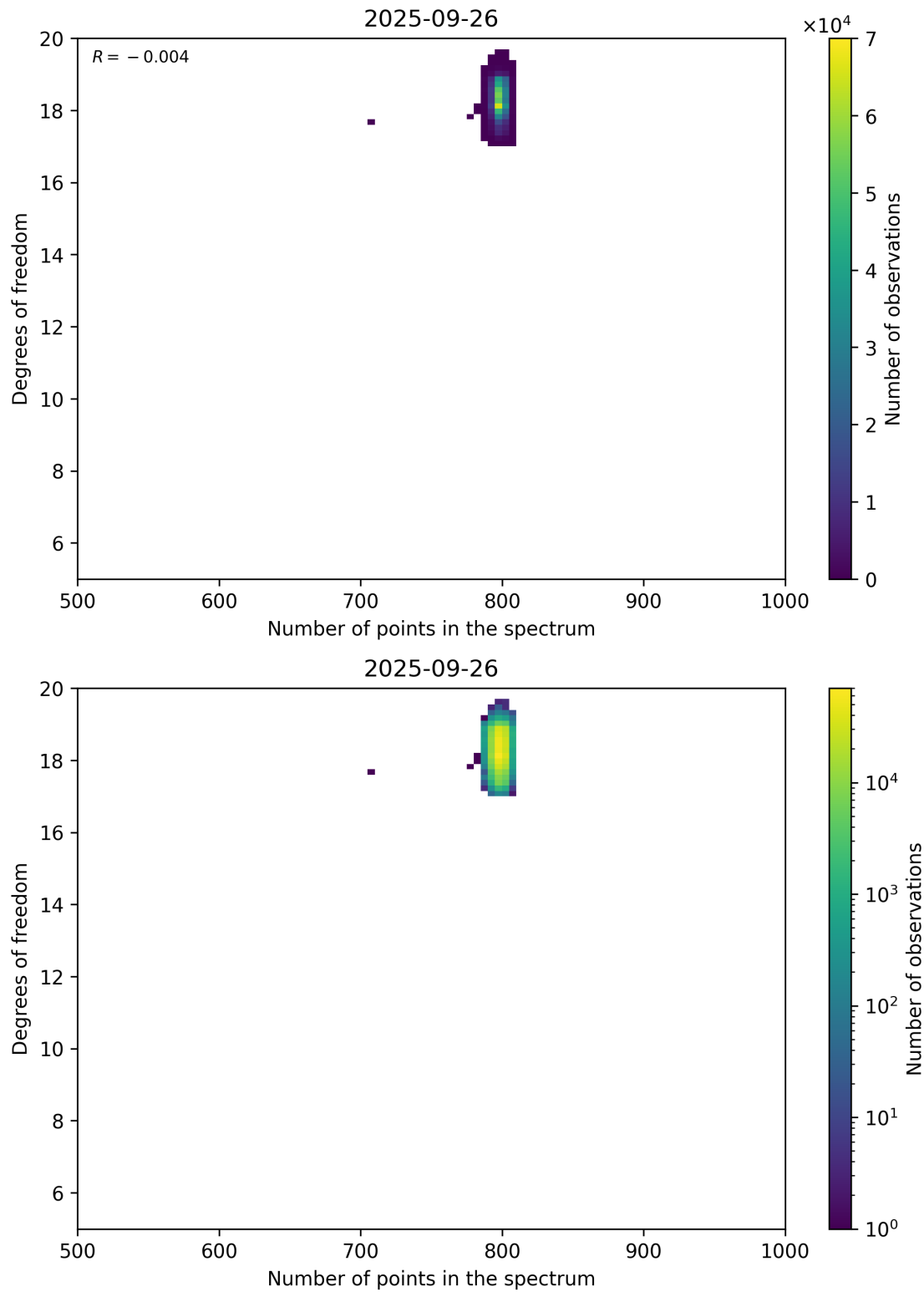
Figure 90: Scatter density plot of “Number of points in the spectrum” against “Degrees of freedom” for 2025-09-26 to 2025-09-27.
