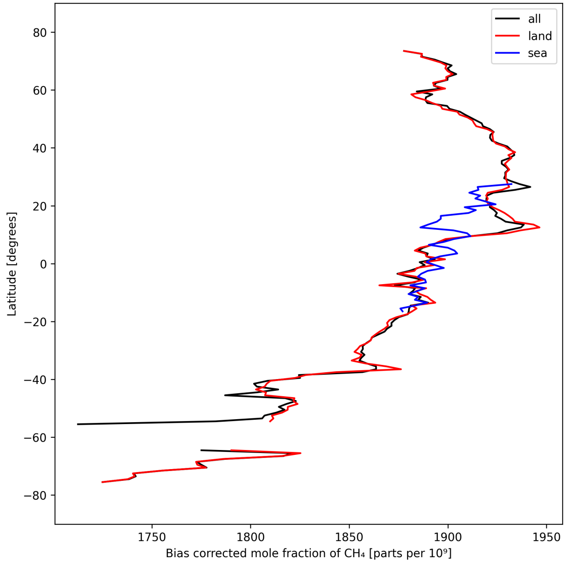
Figure 14: Zonal average of “Bias corrected mole fraction of \text{CH}_4 ” for 2025-09-26 to 2025-09-27.
