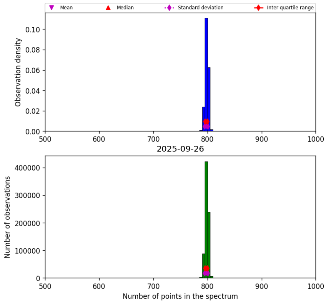
Figure 26: Histogram of “Number of points in the spectrum” for 2025-09-26 to 2025-09-27
