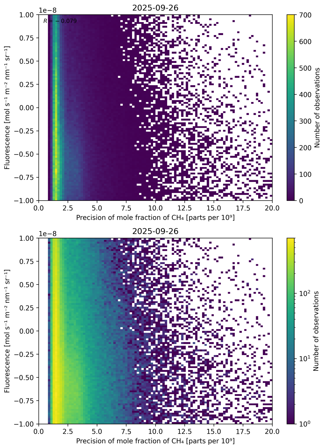
Figure 81: Scatter density plot of “Precision of mole fraction of CH 4 ” against “Fluorescence” for 2025-09-26 to 2025-09-27.
