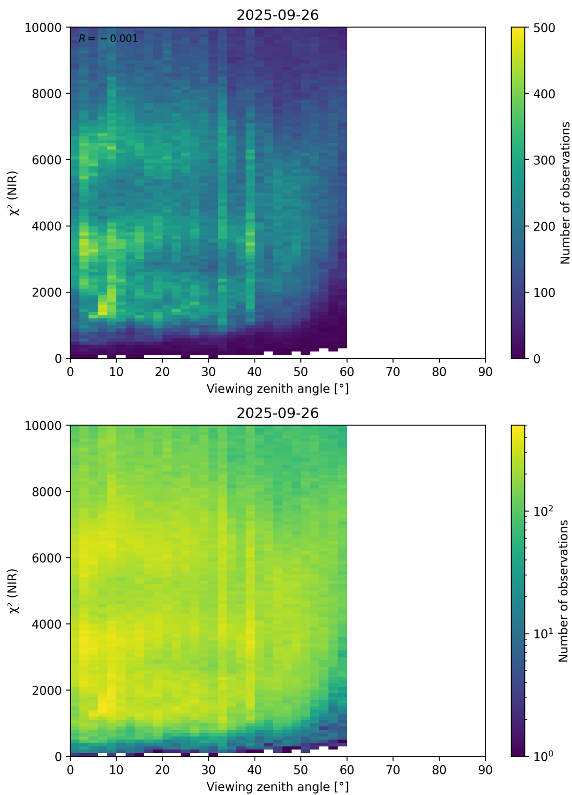
Figure 105: Scatter density plot of “Viewing zenith angle” against “ \chi^2 (NIR)” for 2025-09-26 to 2025-09-27.
