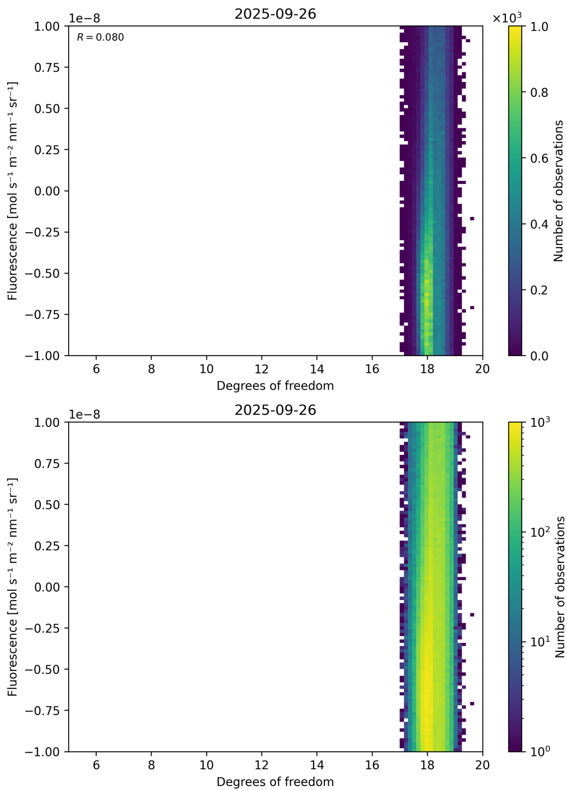
Figure 51: Scatter density plot of “Degrees of freedom” against “Fluorescence” for 2025-09-26 to 2025-09-27.
