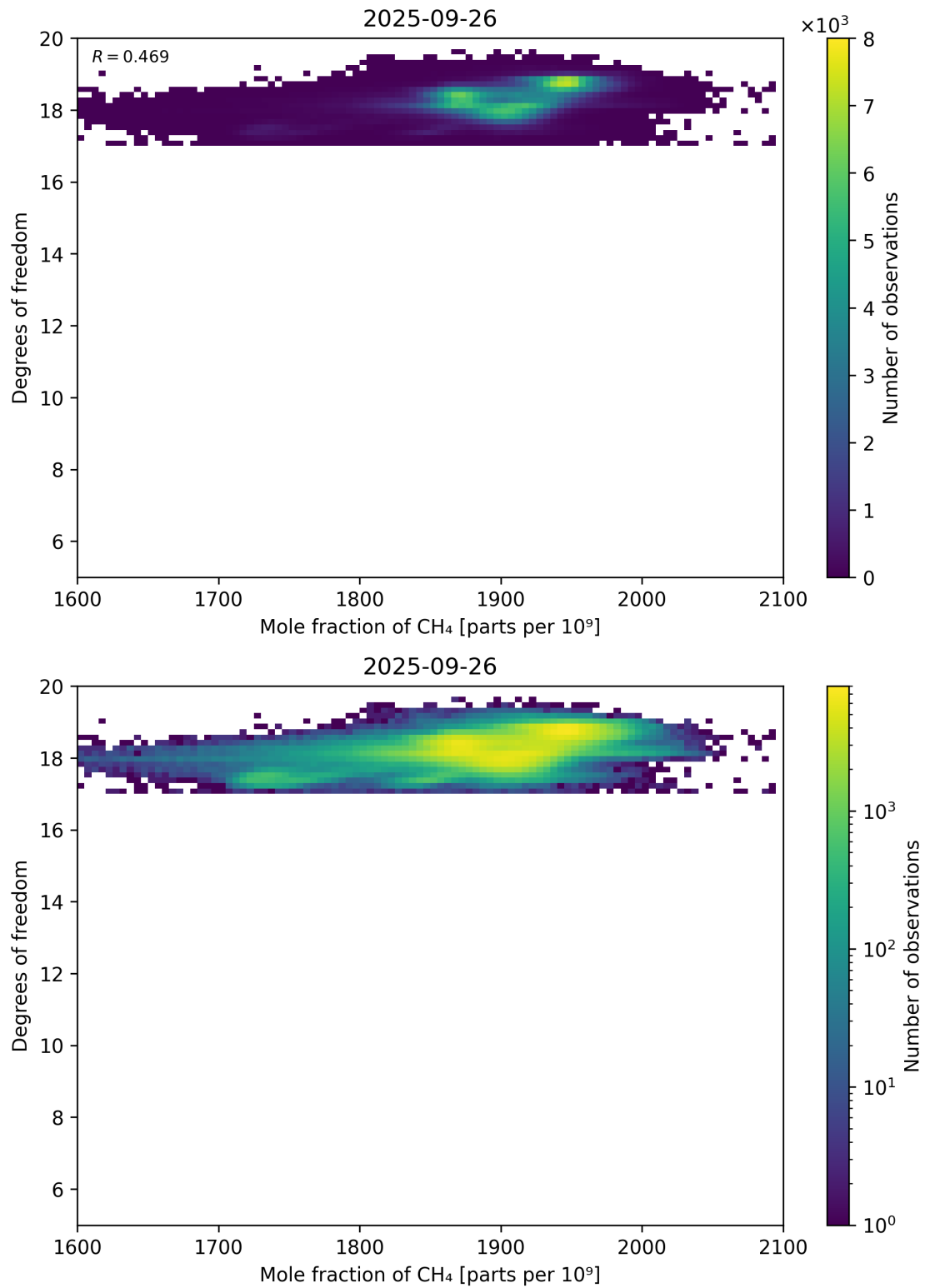
Figure 72: Scatter density plot of “Mole fraction of CH 4 ” against “Degrees of freedom” for 2025-09-26 to 2025-09-27.
