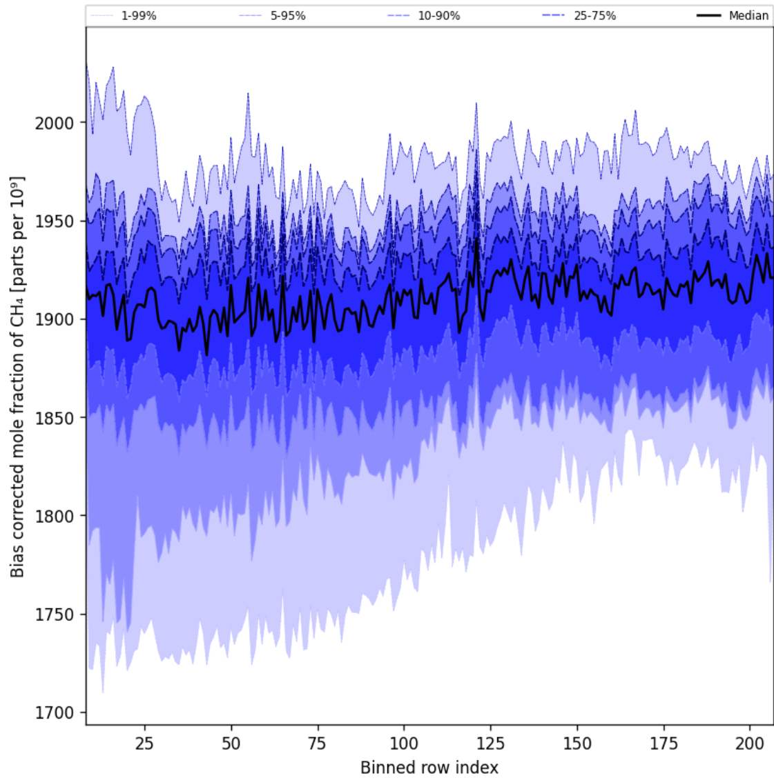
Figure 36: Along track statistics of “Bias corrected mole fraction of CH 4 ” for 2025-09-26 to 2025-09-27
