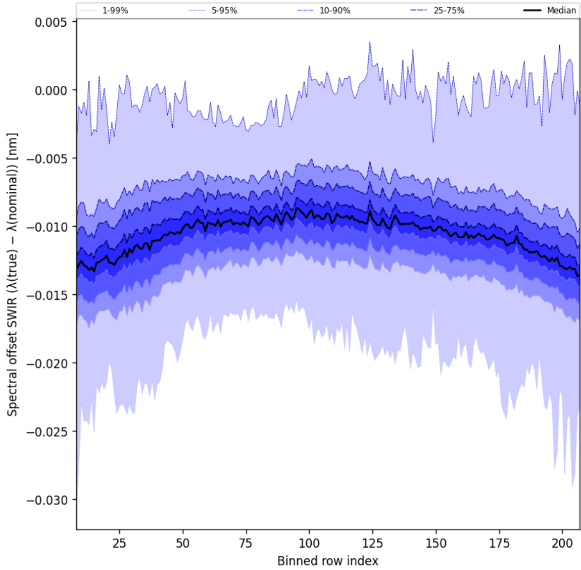
Figure 38: Along track statistics of “Spectral offset SWIR ( \lambda_{\text{true}} - \lambda_{\text{nominal}} )” for 2025-09-26 to 2025-09-27
