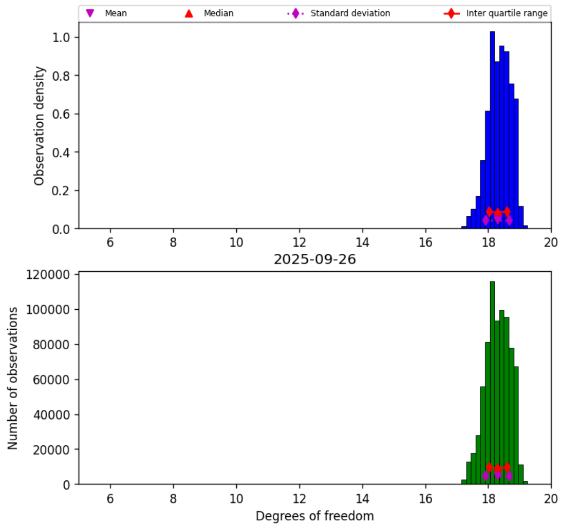
Figure 30: Histogram of “Degrees of freedom” for 2025-09-26 to 2025-09-27
