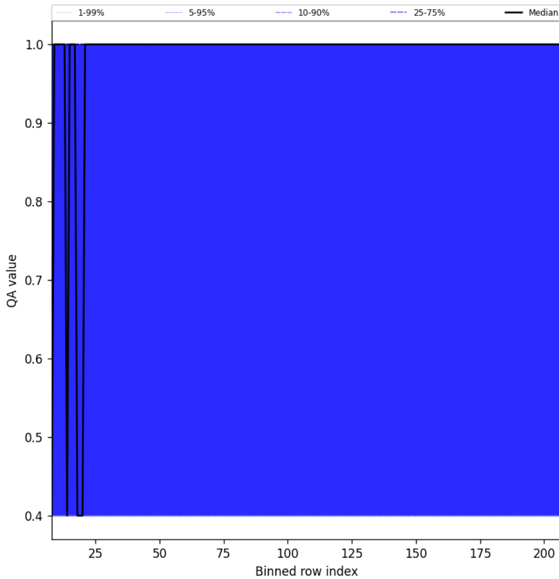
Figure 33: Along track statistics of “QA value” for 2025-09-26 to 2025-09-27
