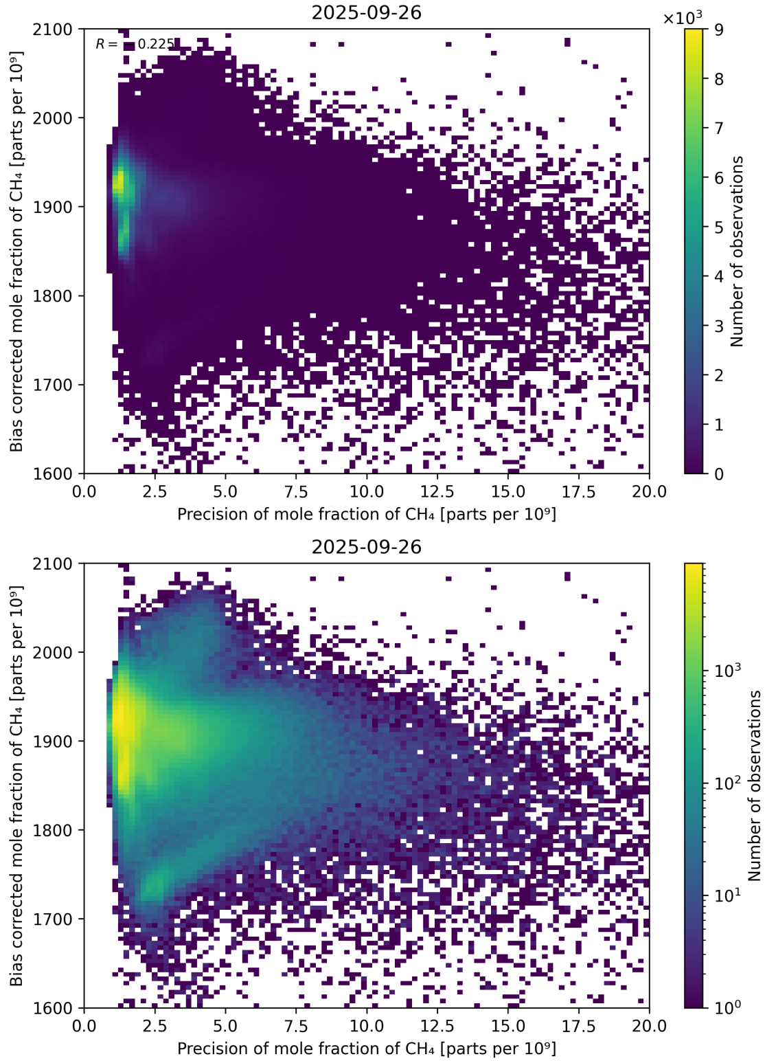
Figure 82: Scatter density plot of “Precision of mole fraction of \text{CH}_4 ” against “Bias corrected mole fraction of \text{CH}_4 ” for 2025-09-26 to 2025-09-27.
