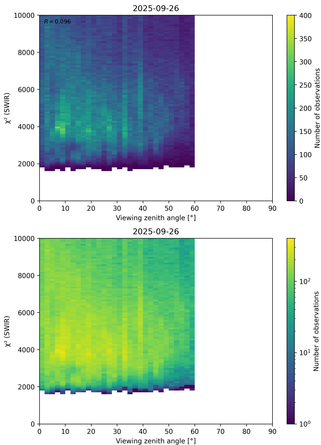
Figure 106: Scatter density plot of “Viewing zenith angle” against “ \chi^2 (SWIR)” for 2025-09-26 to 2025-09-27.
