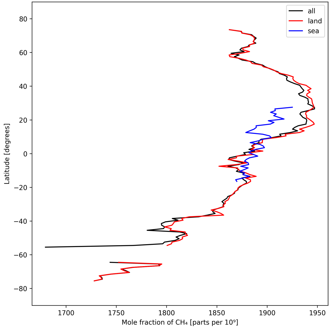
Figure 12: Zonal average of “Mole fraction of \text{CH}_4 ” for 2025-09-26 to 2025-09-27.
