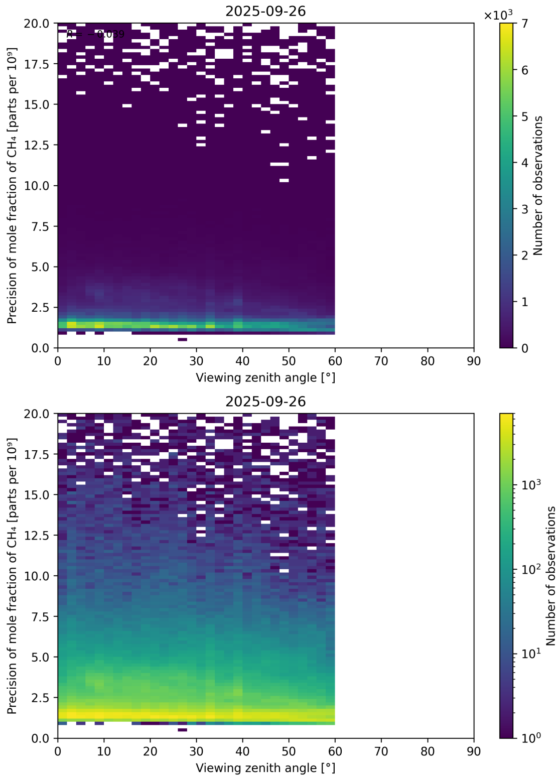
Figure 112: Scatter density plot of “Viewing zenith angle” against “Precision of mole fraction of CH 4 ” for 2025-09-26 to 2025-09-27.
