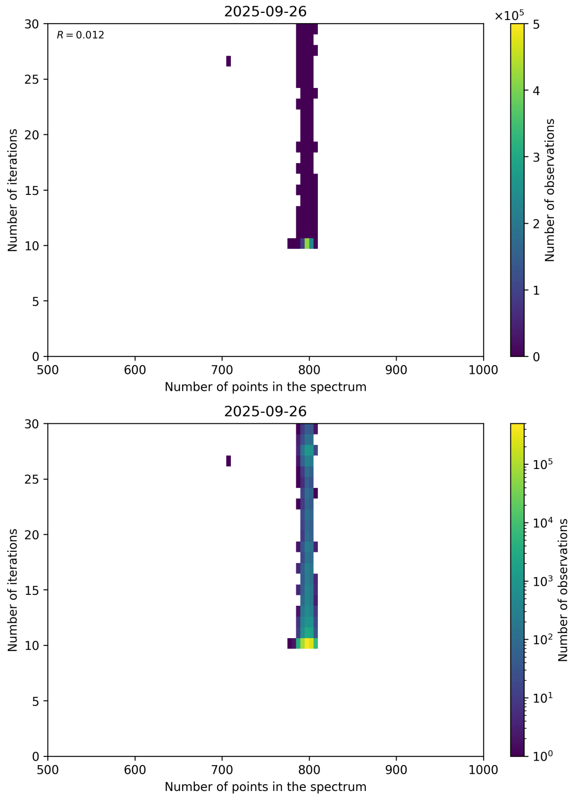
Figure 92: Scatter density plot of “Number of points in the spectrum” against “Number of iterations” for 2025-09-26 to 2025-09-27.
