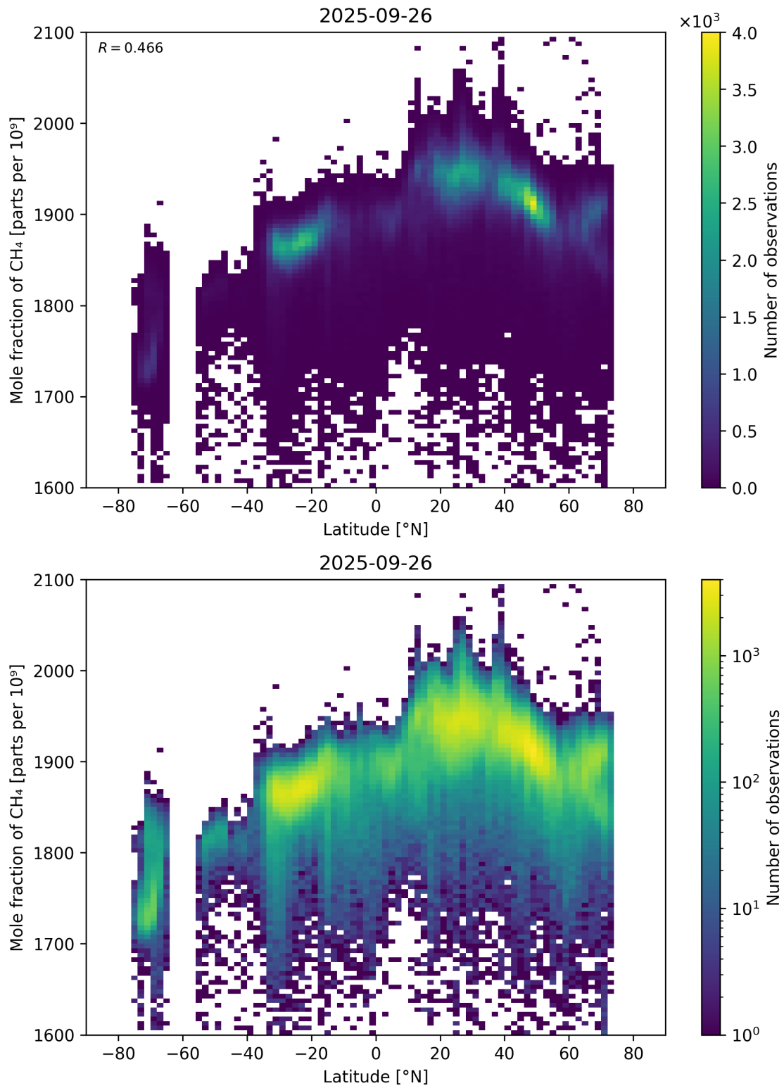
Figure 57: Scatter density plot of “Latitude” against “Mole fraction of CH 4 ” for 2025-09-26 to 2025-09-27.
