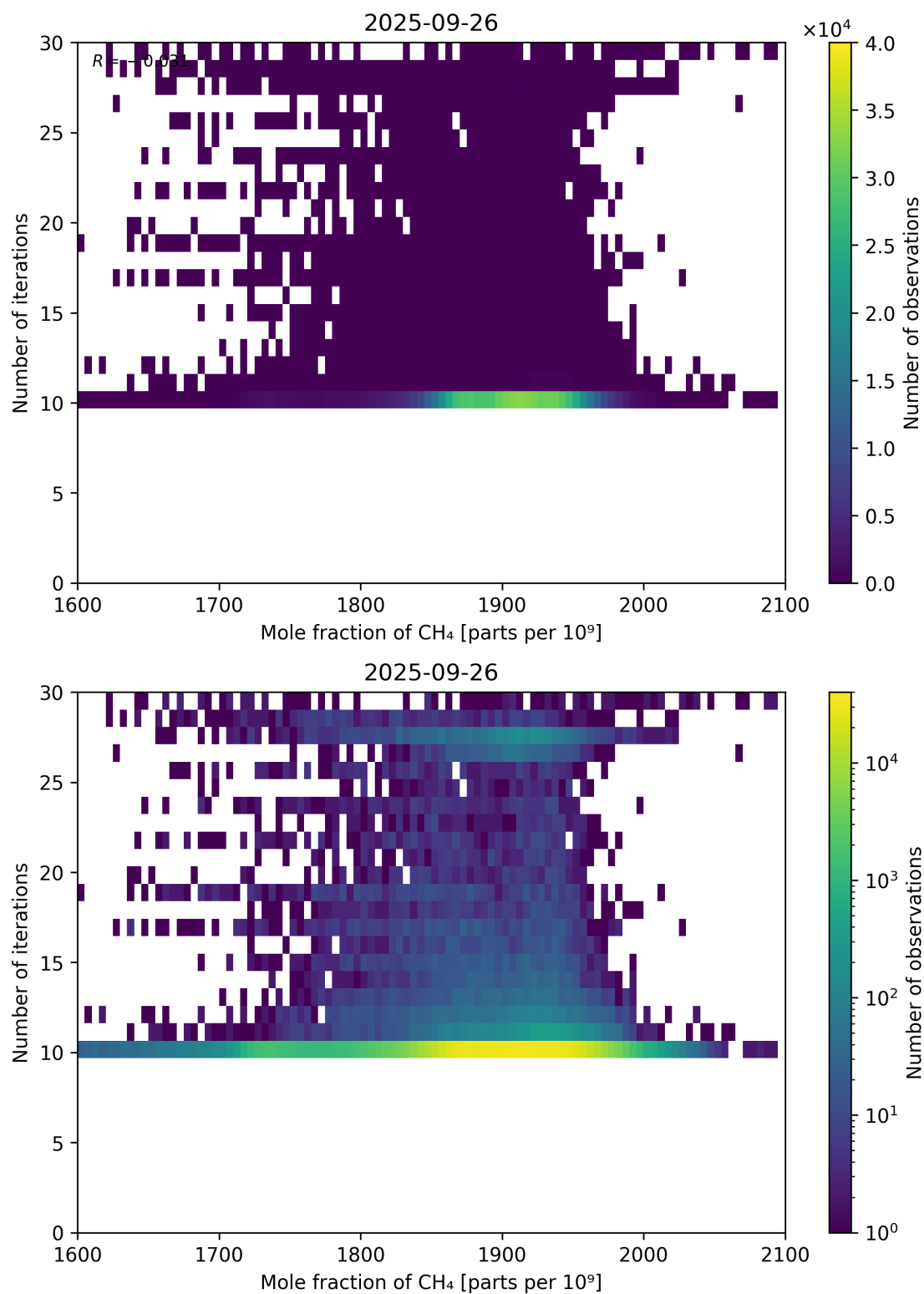
Figure 76: Scatter density plot of “Mole fraction of CH 4 ” against “Number of iterations” for 2025-09-26 to 2025-09-27.
