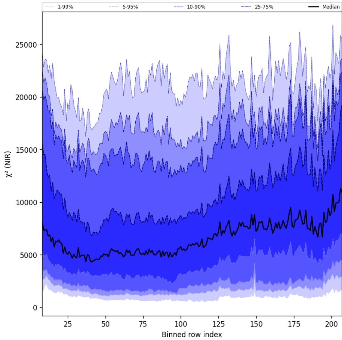
Figure 40: Along track statistics of “ \chi^2 (NIR)” for 2025-09-26 to 2025-09-27
