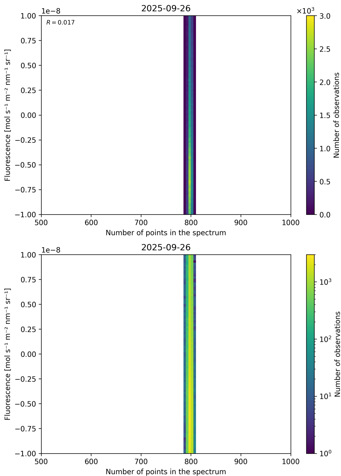
Figure 91: Scatter density plot of “Number of points in the spectrum” against “Fluorescence” for 2025-09-26 to 2025-09-27.
