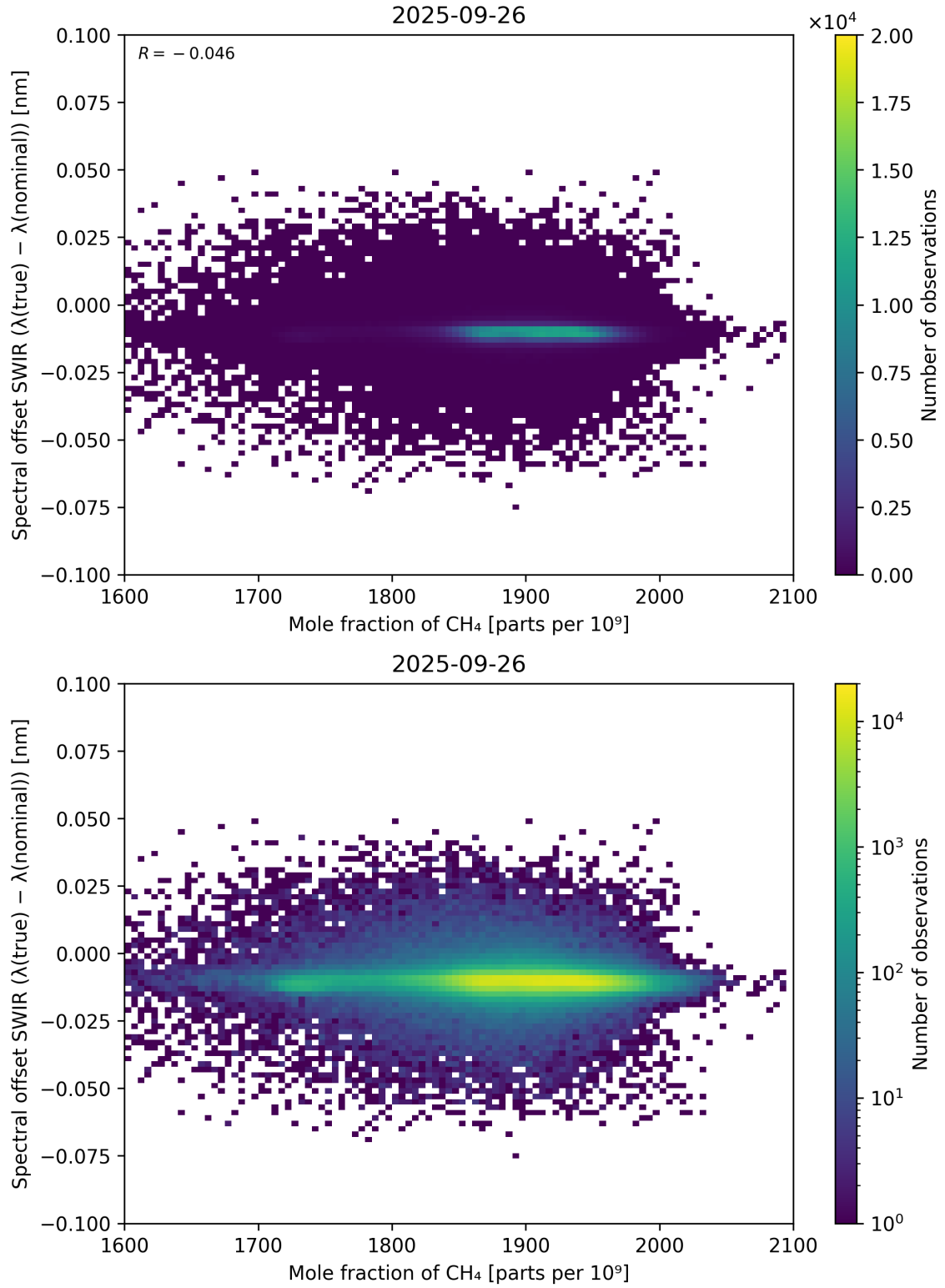
Figure 86: Scatter density plot of “Mole fraction of CH 4 ” against “Spectral offset SWIR ( \lambda_{\text{true}} - \lambda_{\text{nominal}} )” for 2025-09-26 to 2025-09-27.
