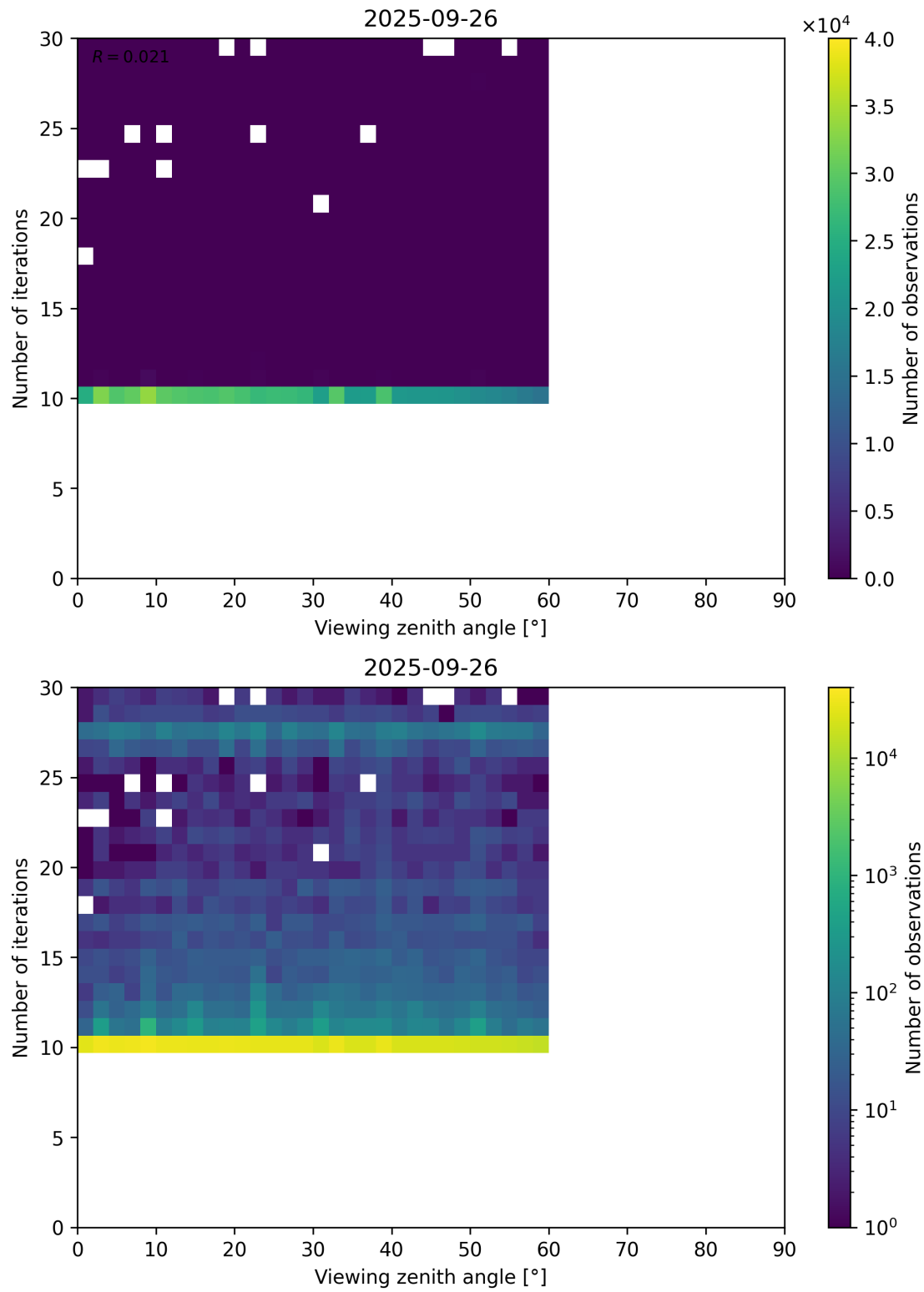
Figure 113: Scatter density plot of “Viewing zenith angle” against “Number of iterations” for 2025-09-26 to 2025-09-27.
