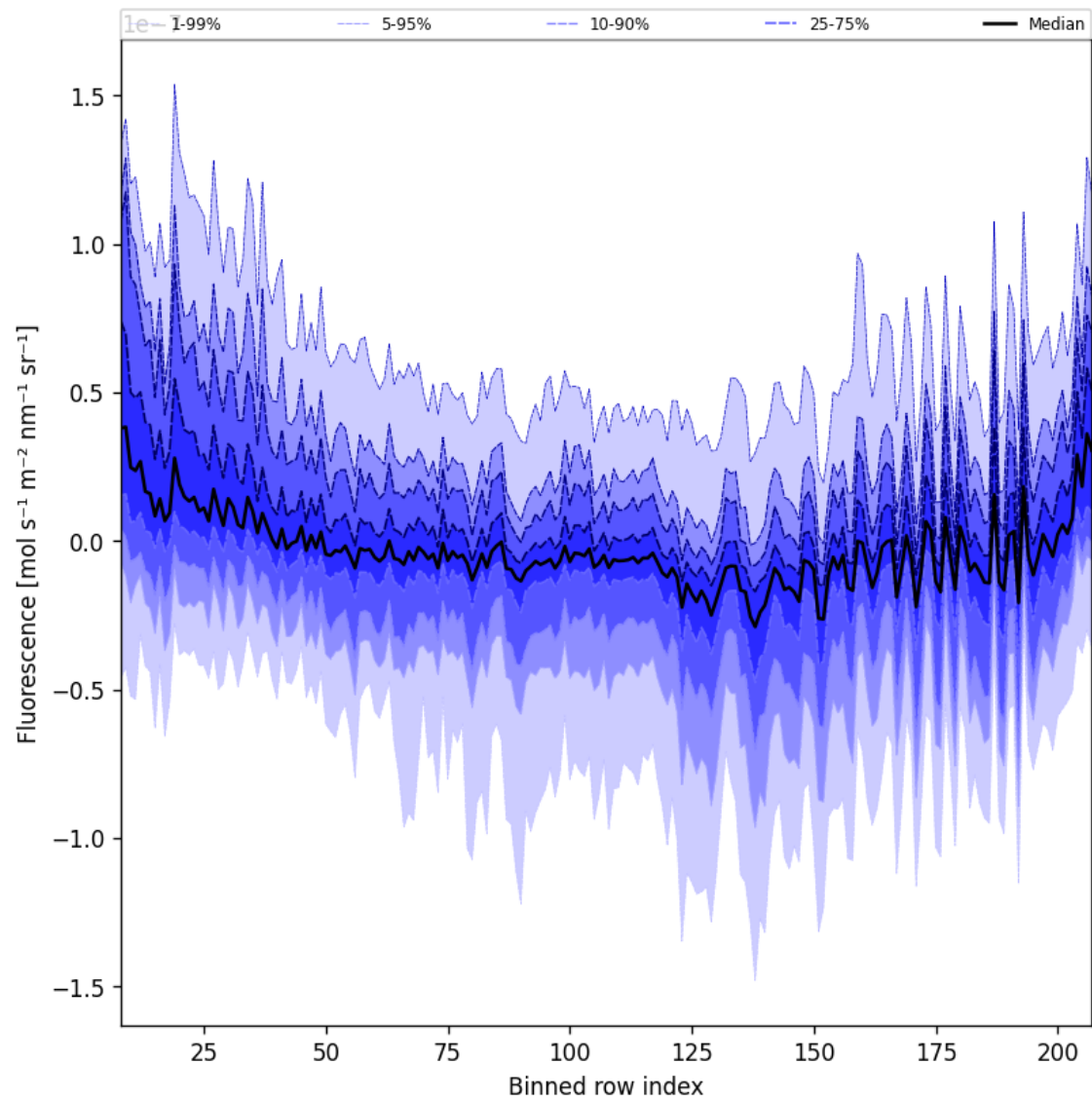
Figure 43: Along track statistics of “Fluorescence” for 2025-09-26 to 2025-09-27
