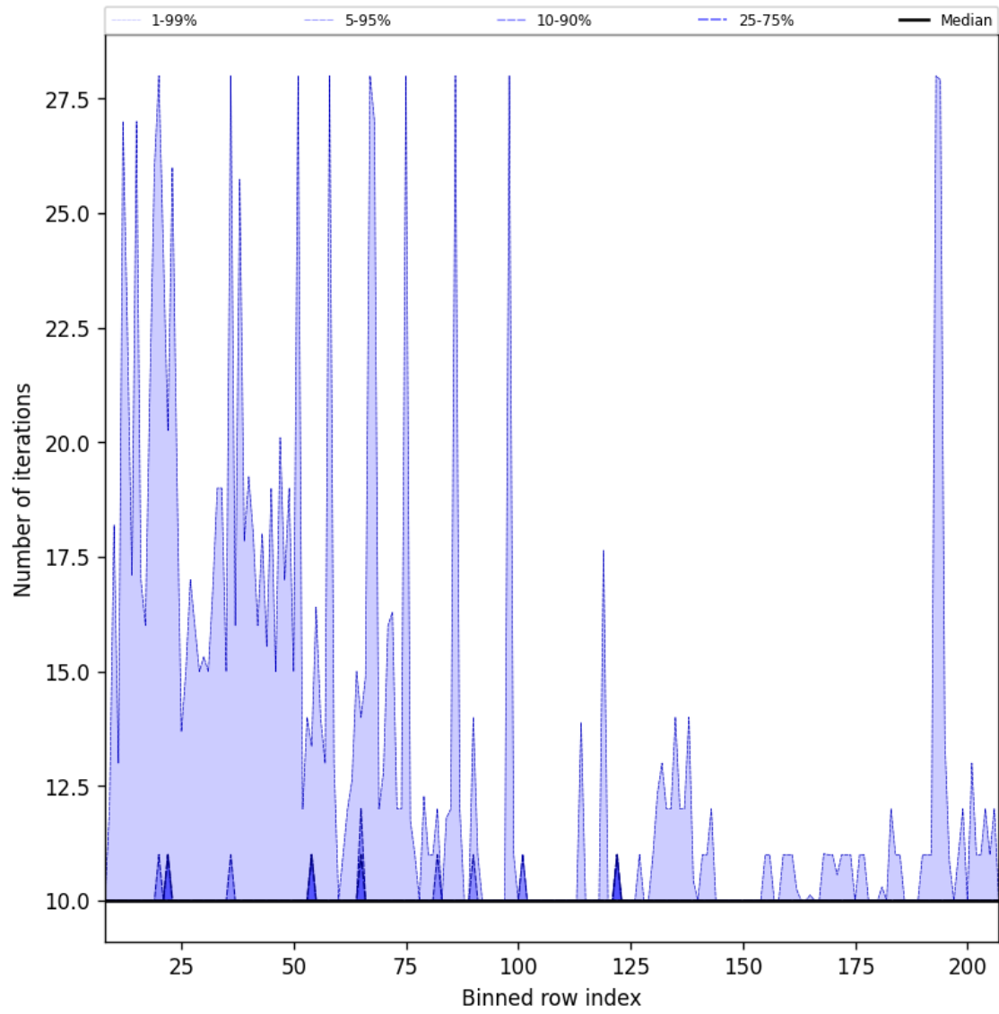
Figure 42: Along track statistics of “Number of iterations” for 2025-09-26 to 2025-09-27
