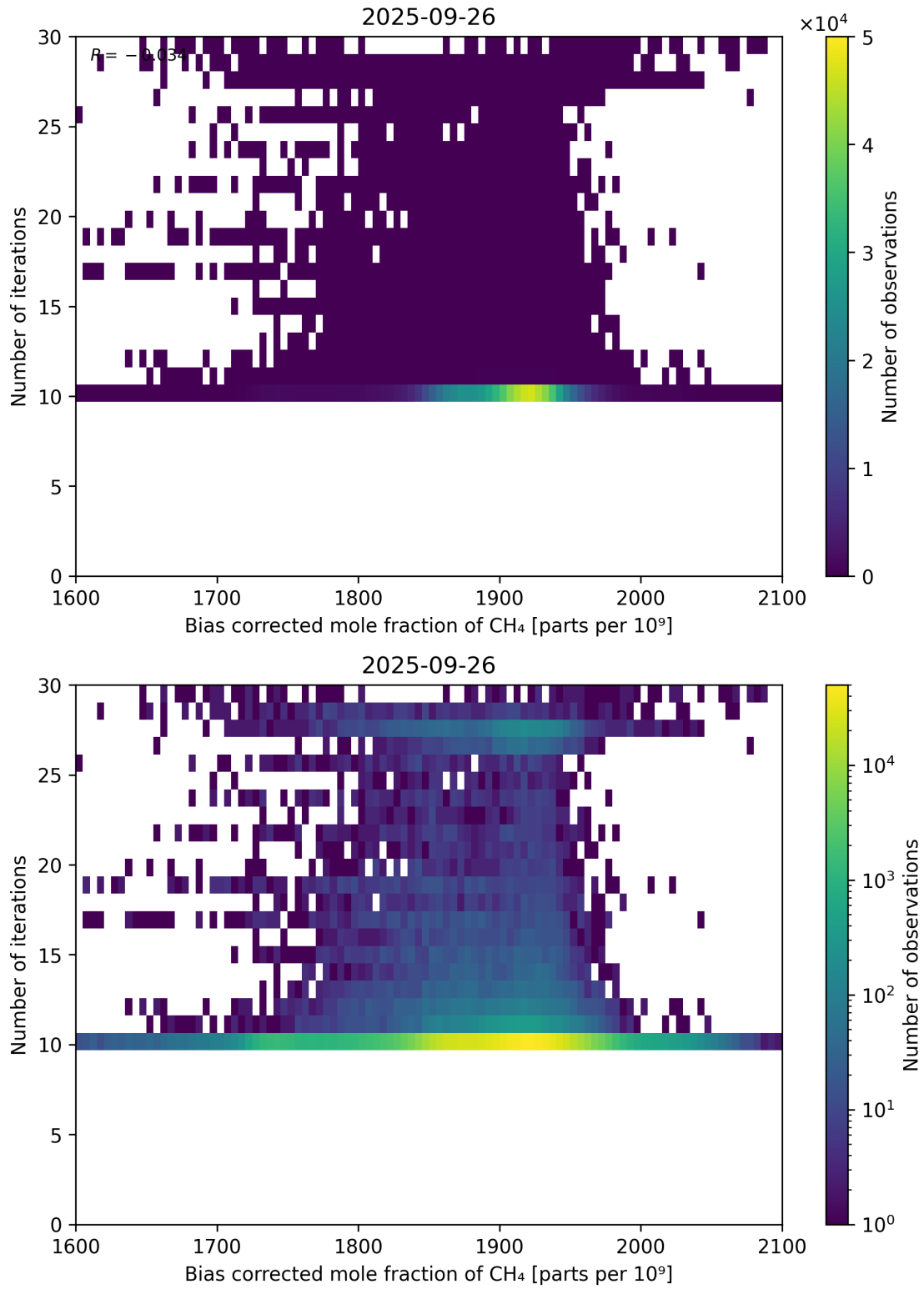
Figure 67: Scatter density plot of “Bias corrected mole fraction of CH 4 ” against “Number of iterations” for 2025-09-26 to 2025-09-27.
