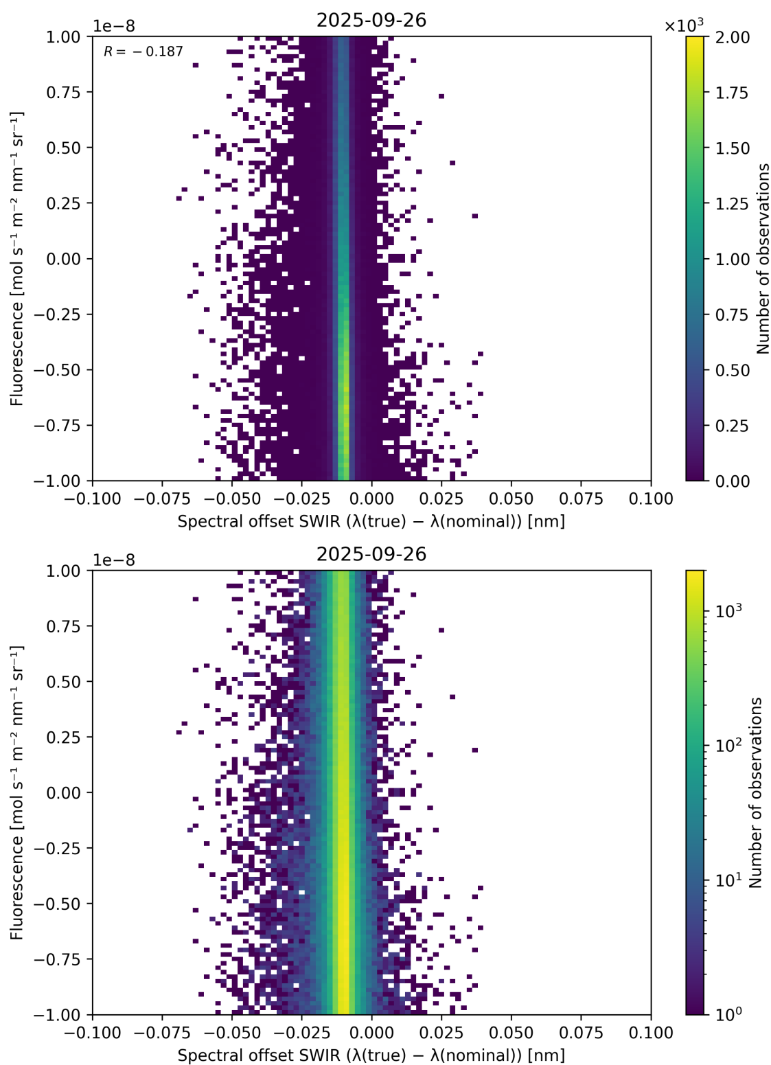
Figure 120: Scatter density plot of “Spectral offset SWIR ( \lambda_{\text{true}} - \lambda_{\text{nominal}} )” against “Fluorescence” for 2025-09-26 to 2025-09-27.
