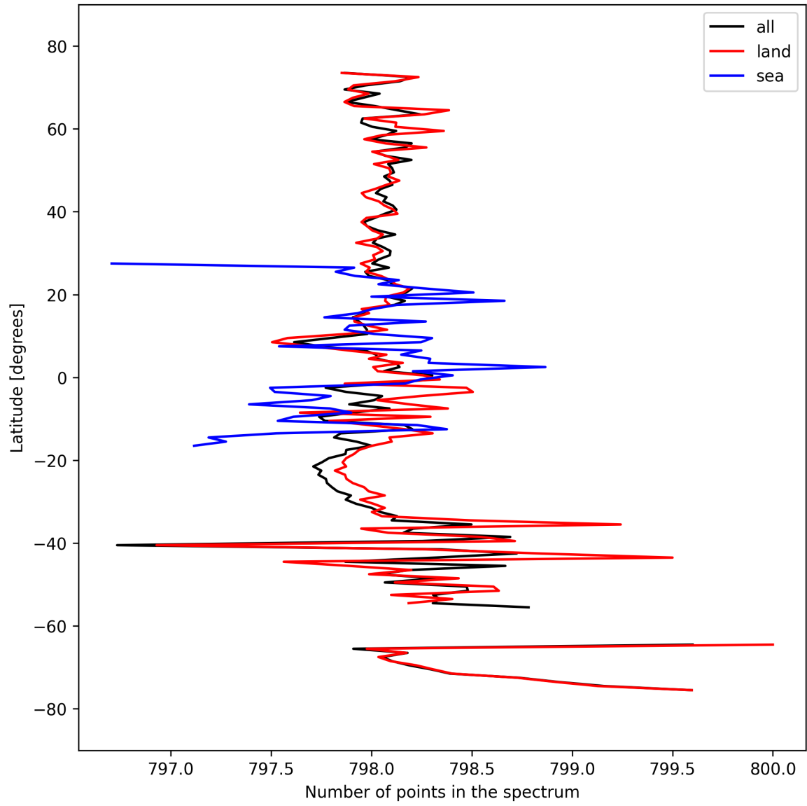
Figure 15: Zonal average of “Number of points in the spectrum” for 2025-09-26 to 2025-09-27.
