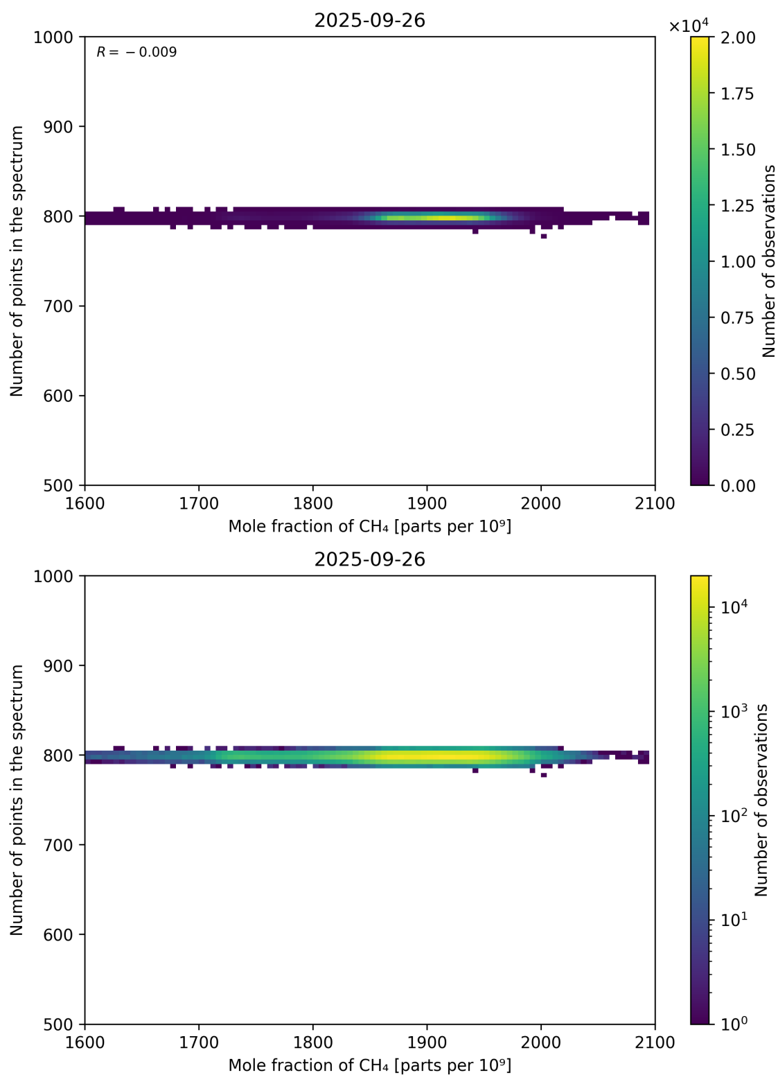
Figure 77: Scatter density plot of “Mole fraction of CH 4 ” against “Number of points in the spectrum” for 2025-09-26 to 2025-09-27.
