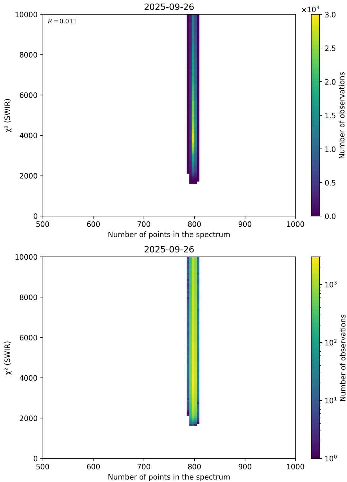
Figure 89: Scatter density plot of “Number of points in the spectrum” against “ \chi^2 (SWIR)” for 2025-09-26 to 2025-09-27.
