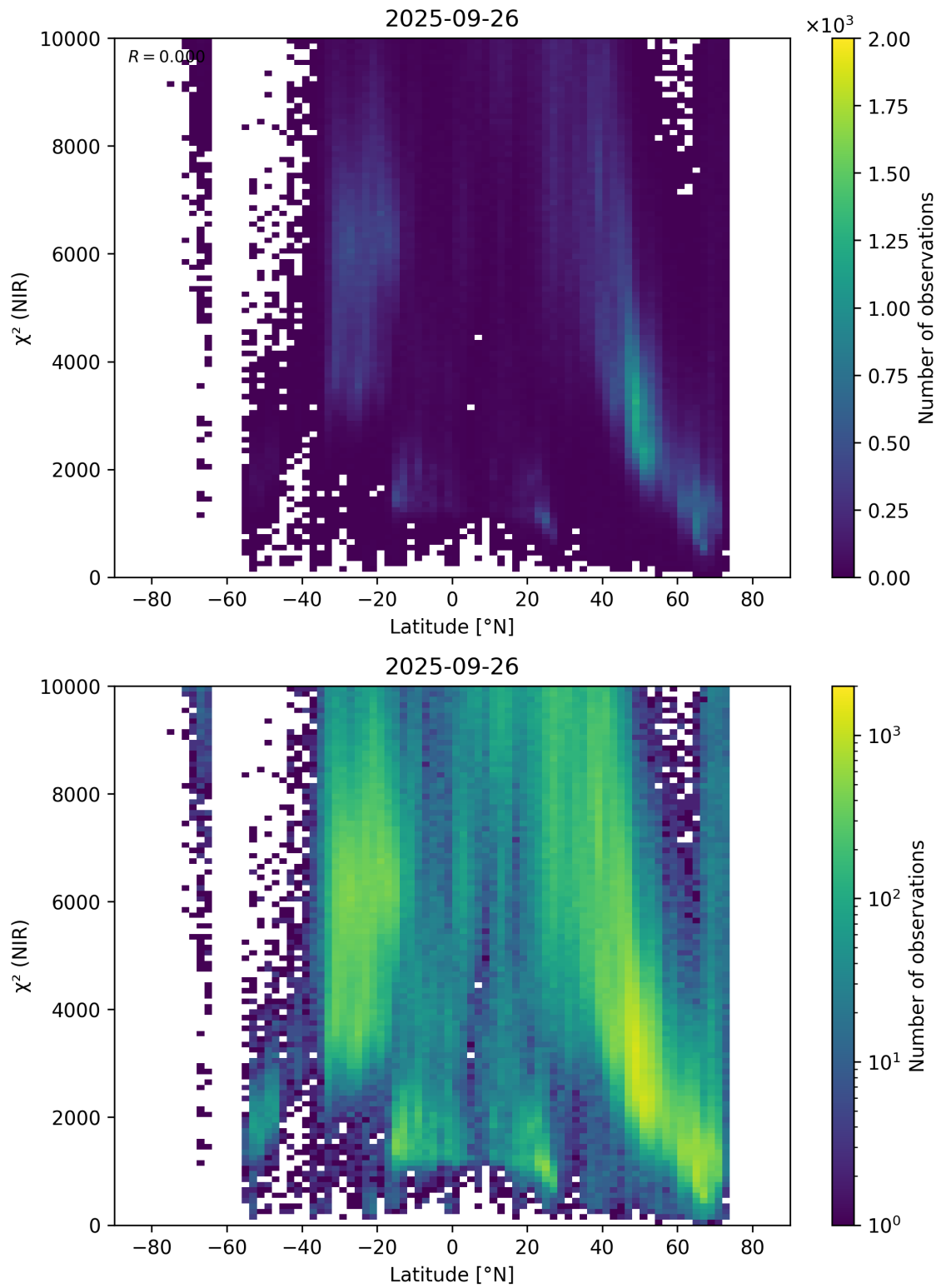
Figure 53: Scatter density plot of “Latitude” against “ \chi^2 (NIR)” for 2025-09-26 to 2025-09-27.
