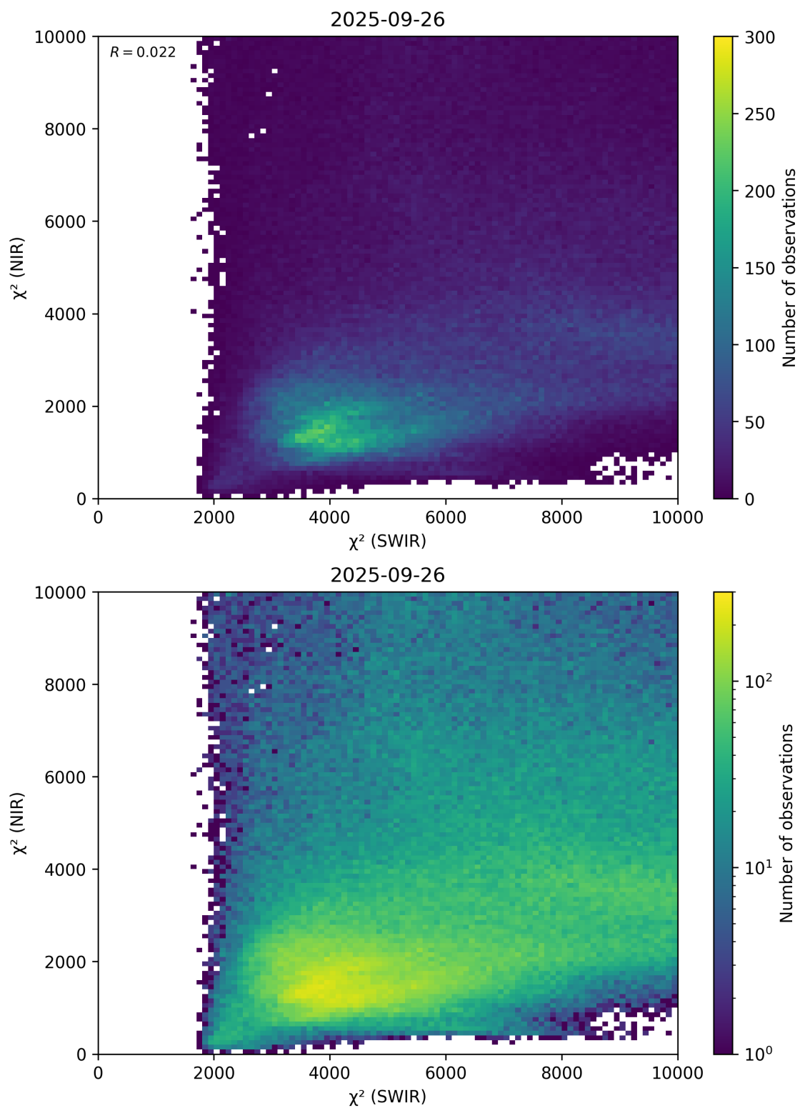
Figure 47: Scatter density plot of “ \chi^2 (SWIR)” against “ \chi^2 (NIR)” for 2025-09-26 to 2025-09-27.
