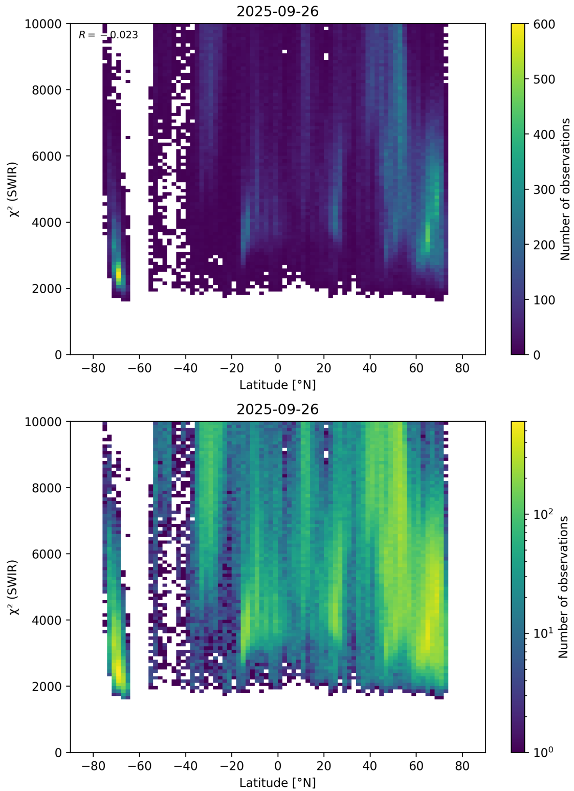
Figure 54: Scatter density plot of “Latitude” against “ \chi^2 (SWIR)” for 2025-09-26 to 2025-09-27.
