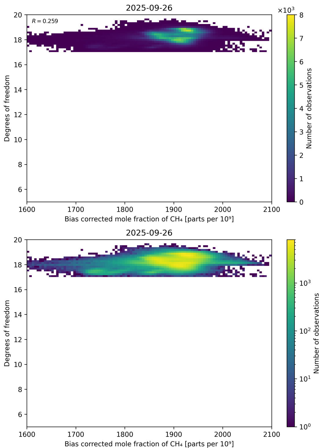
Figure 65: Scatter density plot of “Bias corrected mole fraction of CH 4 ” against “Degrees of freedom” for 2025-09-26 to 2025-09-27.
