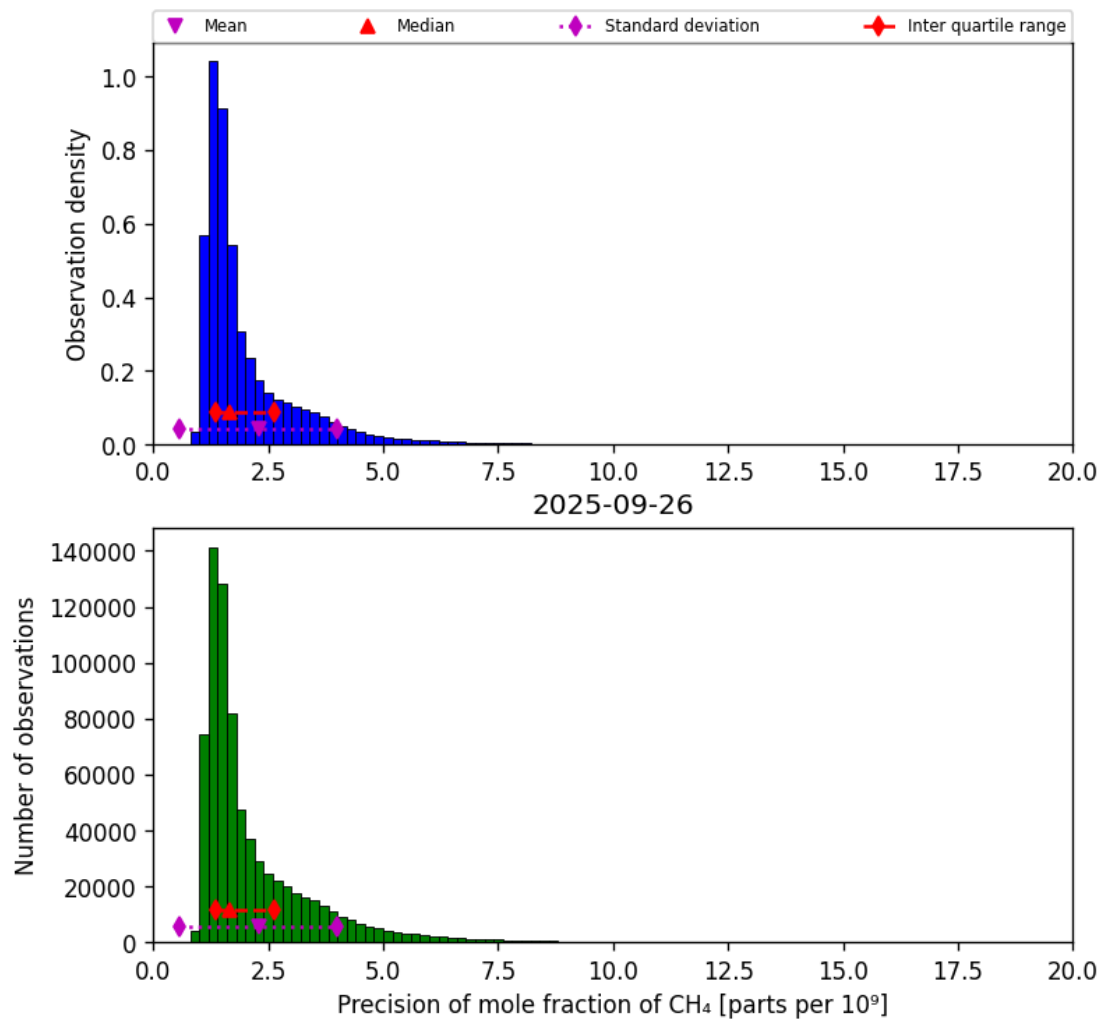
Figure 24: Histogram of “Precision of mole fraction of CH 4 ” for 2025-09-26 to 2025-09-27
