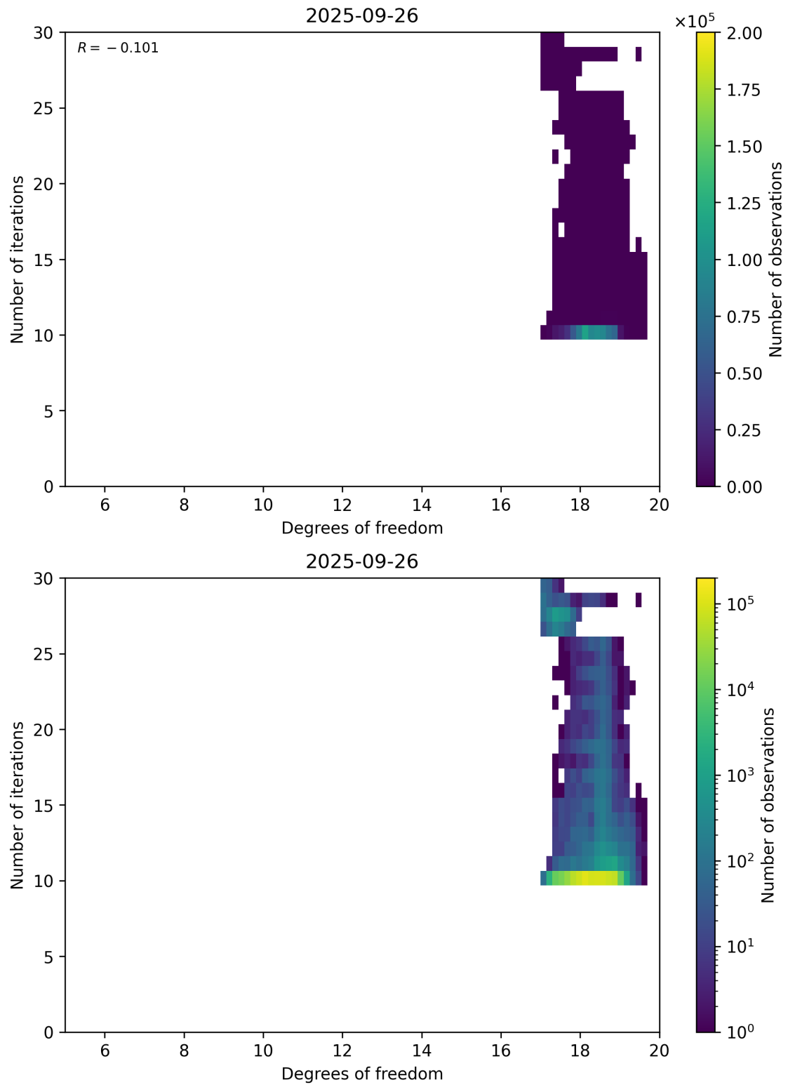
Figure 52: Scatter density plot of “Degrees of freedom” against “Number of iterations” for 2025-09-26 to 2025-09-27.
