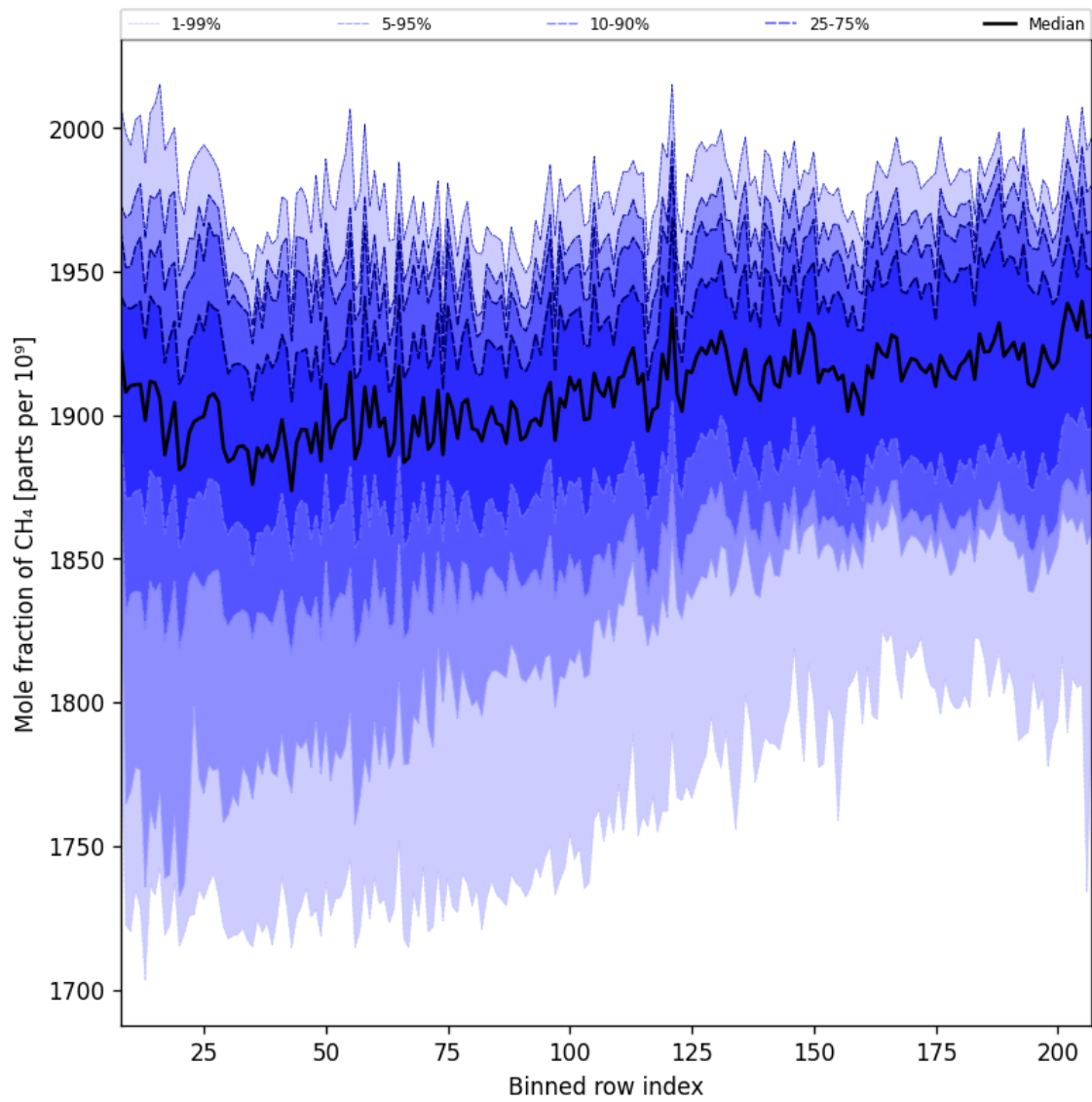
Figure 34: Along track statistics of “Mole fraction of CH 4 ” for 2025-09-26 to 2025-09-27
