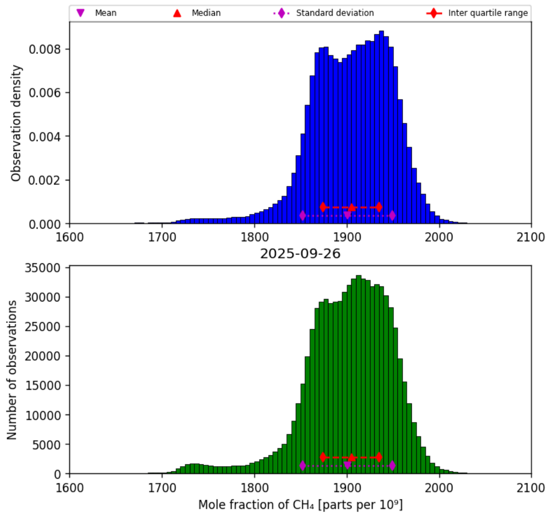
Figure 23: Histogram of “Mole fraction of CH 4 ” for 2025-09-26 to 2025-09-27
