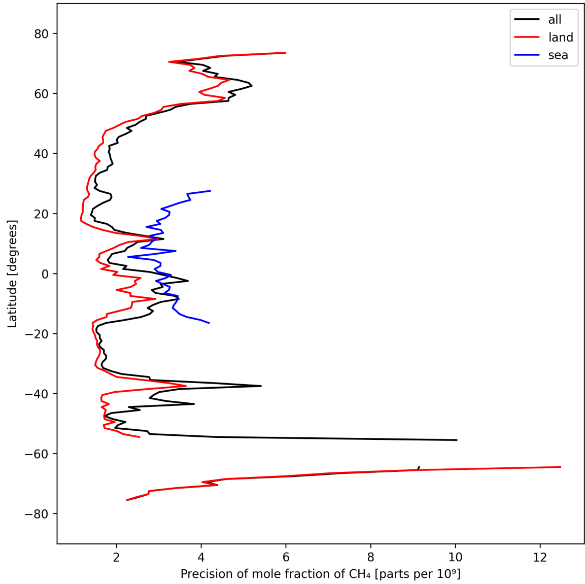
Figure 13: Zonal average of “Precision of mole fraction of CH 4 ” for 2025-09-26 to 2025-09-27.
