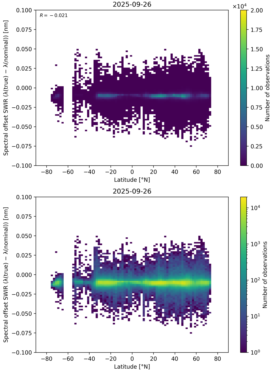
Figure 62: Scatter density plot of “Latitude” against “Spectral offset SWIR ( \lambda_{\text{true}} - \lambda_{\text{nominal}} )” for 2025-09-26 to 2025-09-27.
