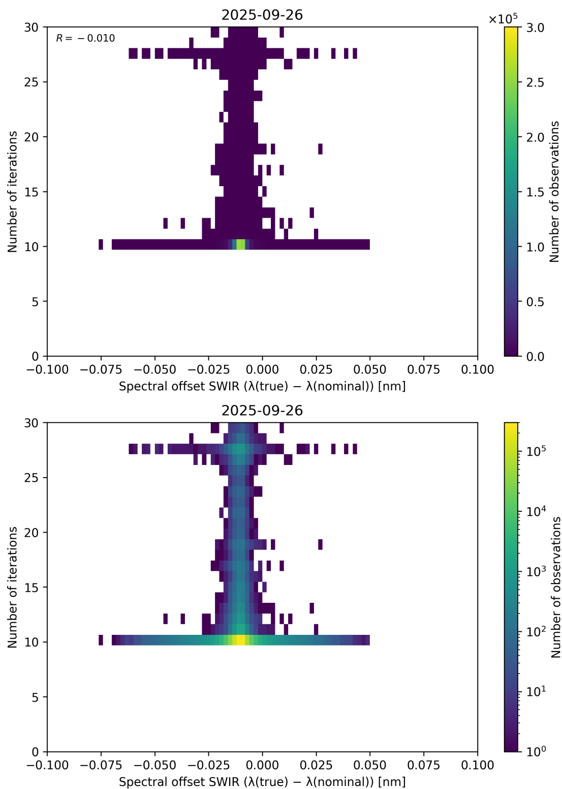
Figure 121: Scatter density plot of “Spectral offset SWIR ( \lambda_{\text{true}} - \lambda_{\text{nominal}} )” against “Number of iterations” for 2025-09-26 to 2025-09-27.
