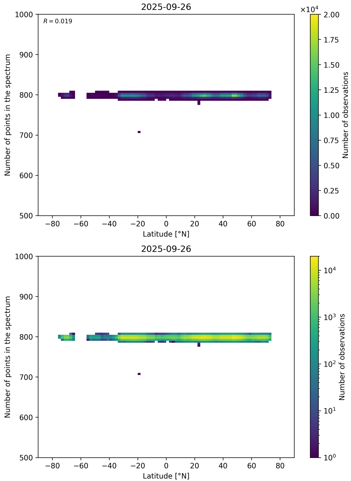
Figure 61: Scatter density plot of “Latitude” against “Number of points in the spectrum” for 2025-09-26 to 2025-09-27.
