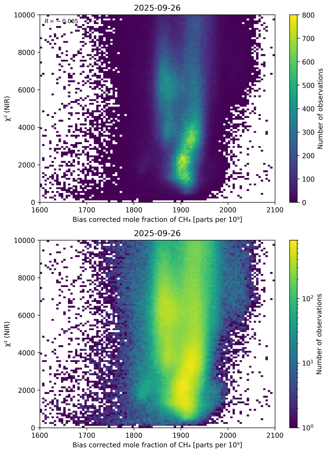
Figure 63: Scatter density plot of “Bias corrected mole fraction of \text{CH}_4 ” against “ \chi^2 (NIR)” for 2025-09-26 to 2025-09-27.
