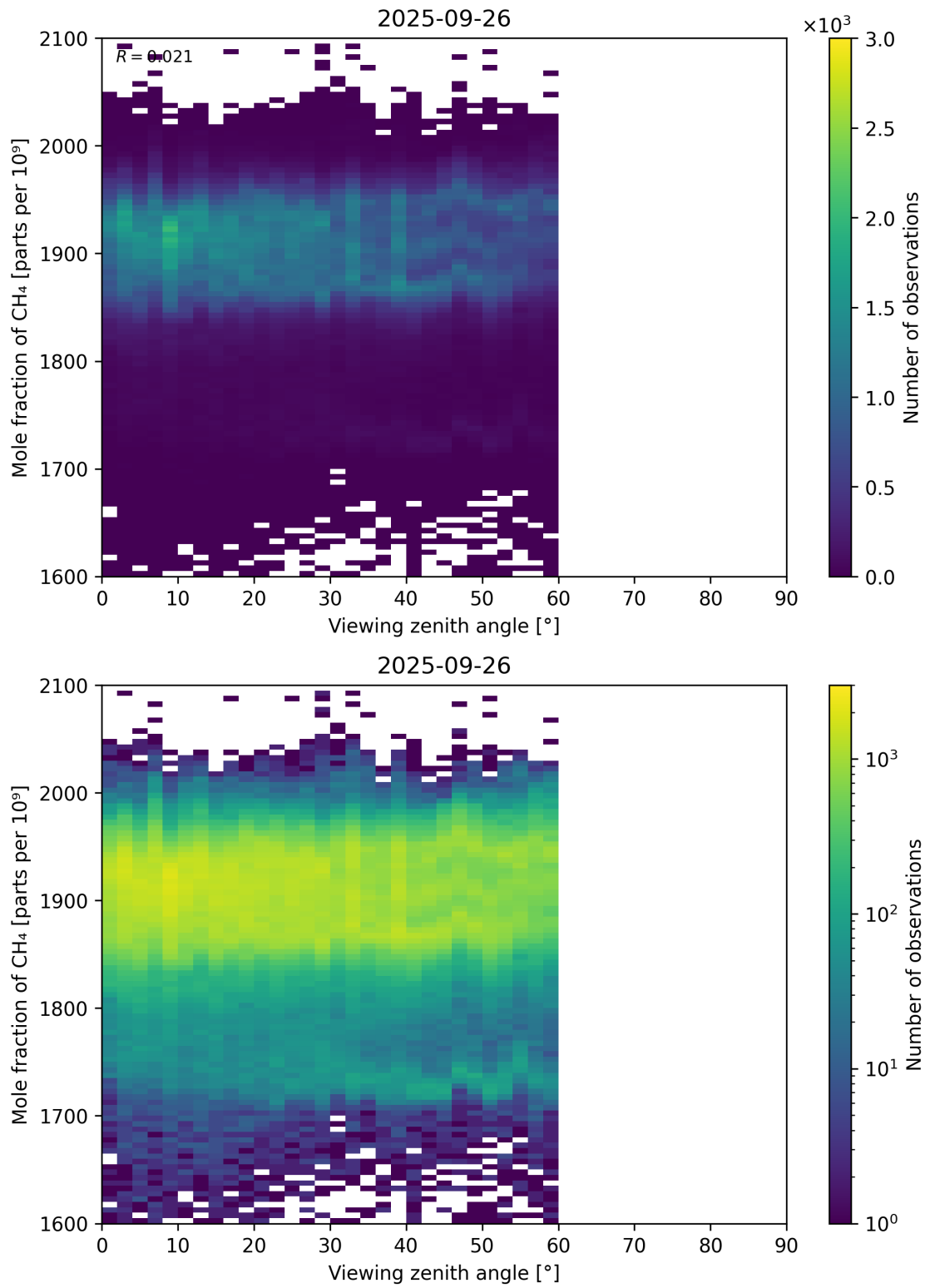
Figure 110: Scatter density plot of “Viewing zenith angle” against “Mole fraction of CH 4 ” for 2025-09-26 to 2025-09-27.
