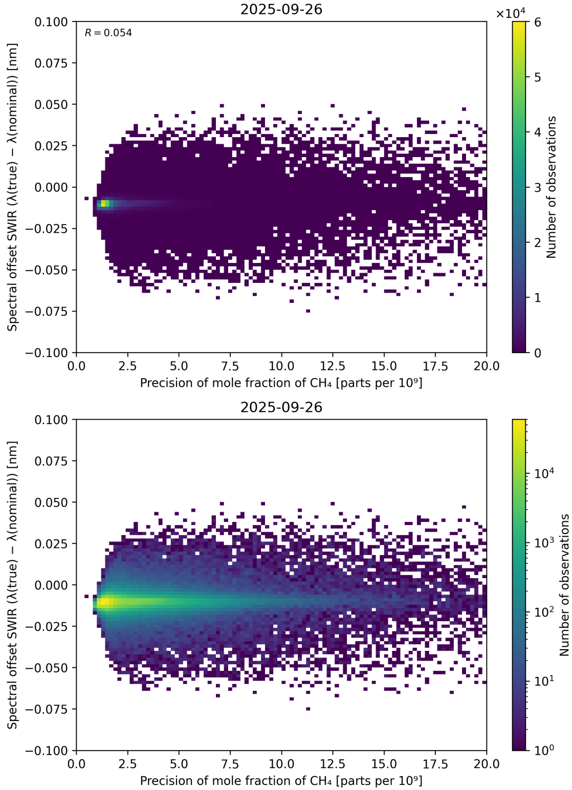
Figure 85: Scatter density plot of “Precision of mole fraction of \text{CH}_4 ” against “Spectral offset SWIR ( \lambda_{\text{true}} - \lambda_{\text{nominal}} )” for 2025-09-26 to 2025-09-27.
