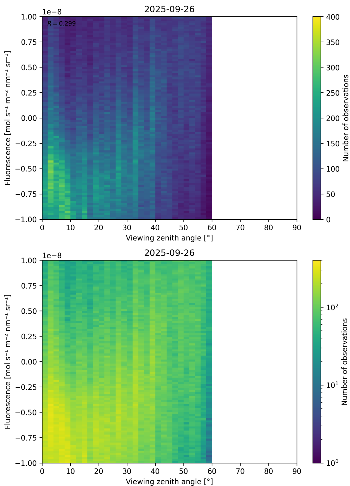
Figure 108: Scatter density plot of “Viewing zenith angle” against “Fluorescence” for 2025-09-26 to 2025-09-27.
