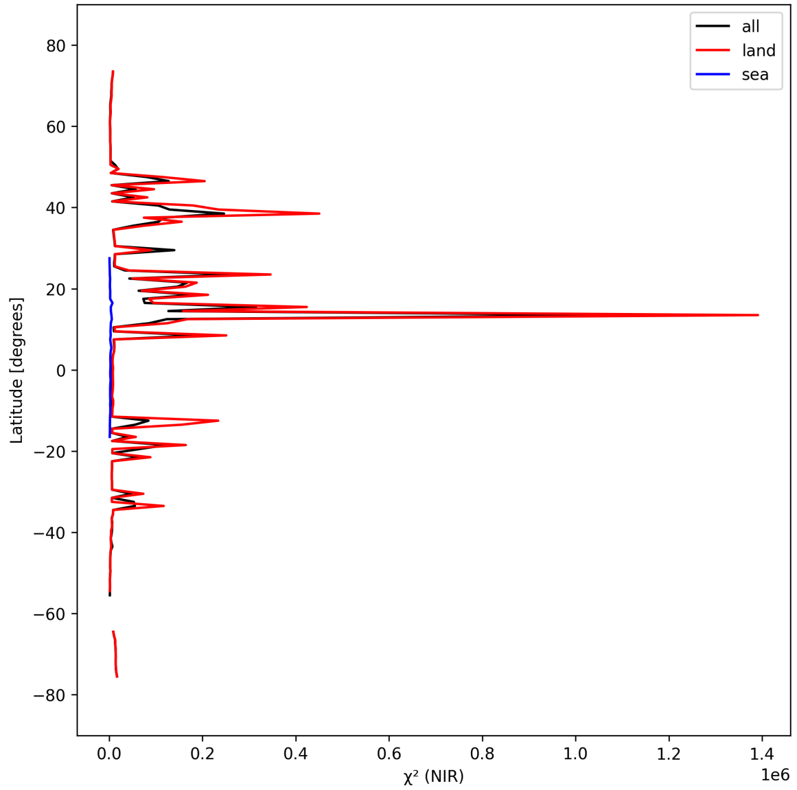
Figure 18: Zonal average of “ \chi^2 (NIR)” for 2025-09-26 to 2025-09-27.
