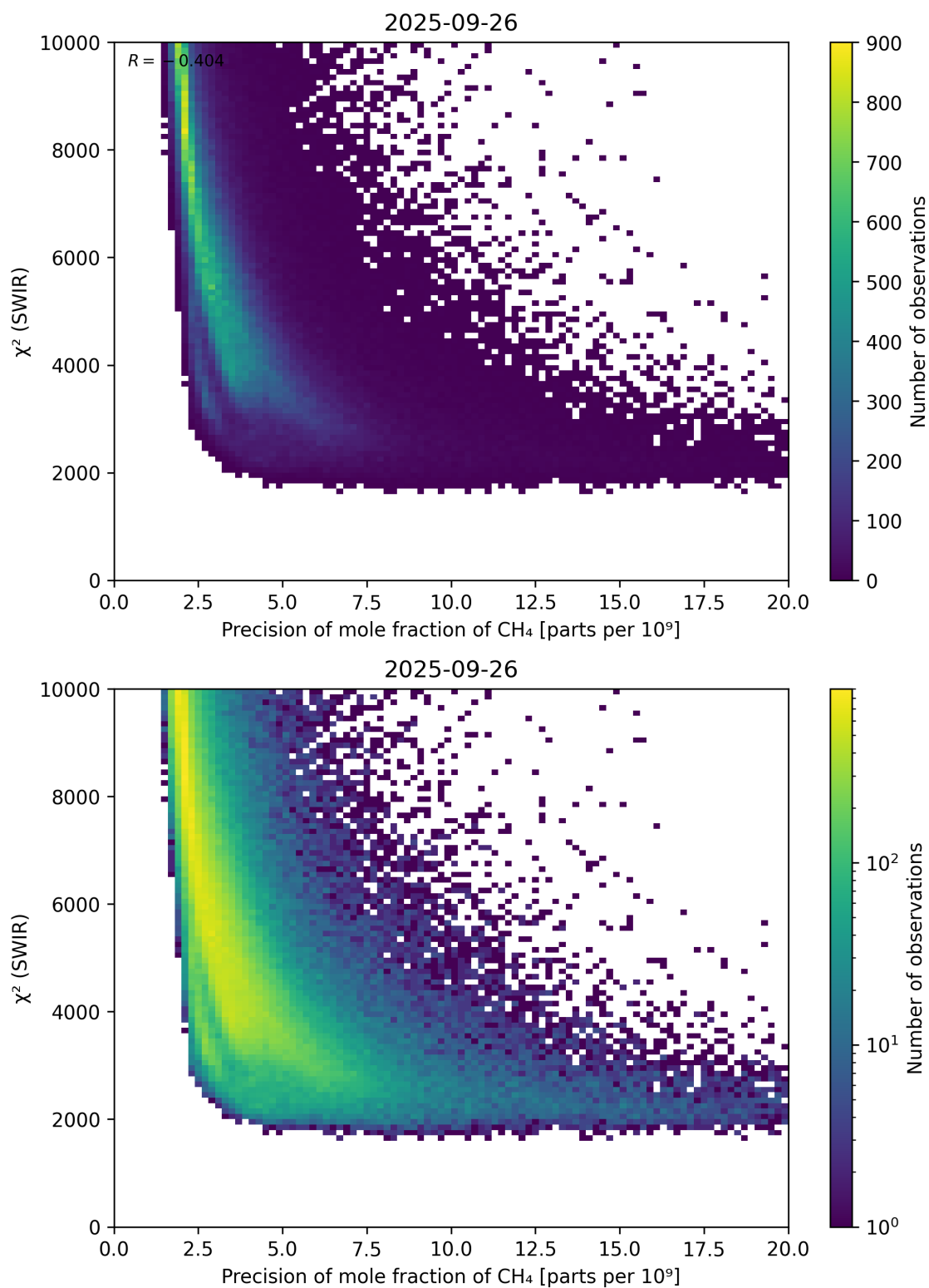
Figure 79: Scatter density plot of “Precision of mole fraction of \text{CH}_4 ” against “ \chi^2 (SWIR)” for 2025-09-26 to 2025-09-27.
