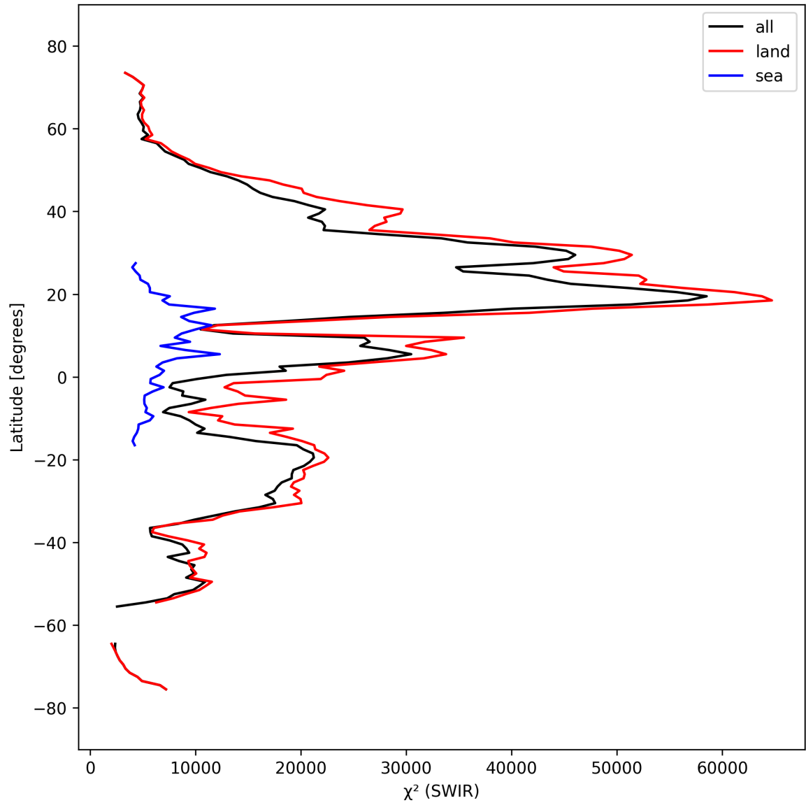
Figure 17: Zonal average of “ \chi^2 (SWIR)” for 2025-09-26 to 2025-09-27.
