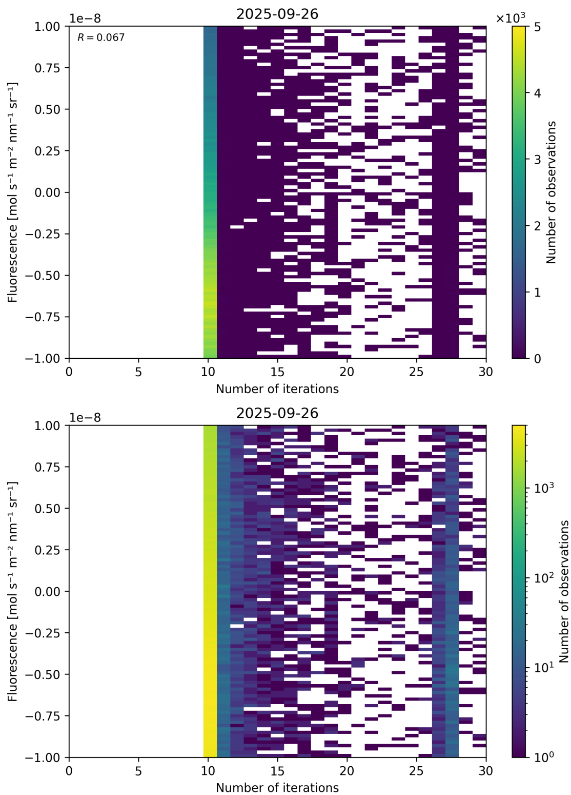
Figure 87: Scatter density plot of "Number of iterations" against "Fluorescence" for 2025-09-26 to 2025-09-27.
