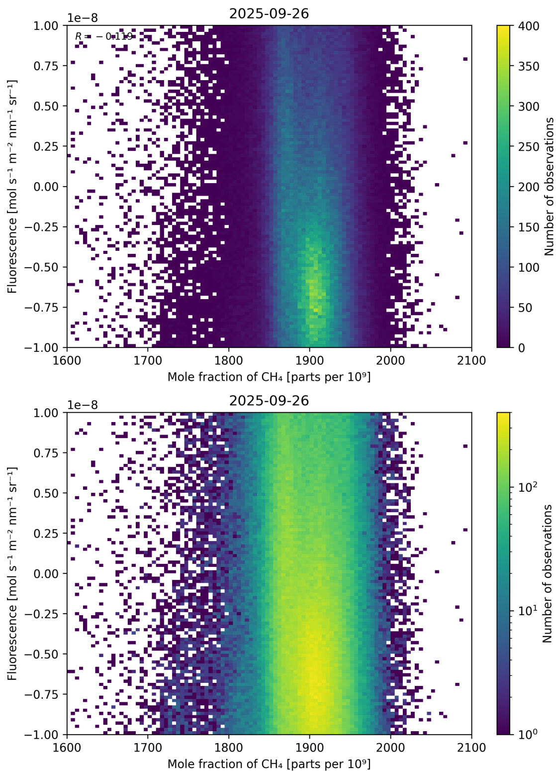
Figure 73: Scatter density plot of “Mole fraction of \text{CH}_4 ” against “Fluorescence” for 2025-09-26 to 2025-09-27.
