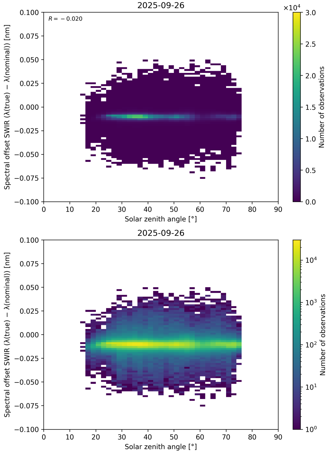
Figure 104: Scatter density plot of “Solar zenith angle” against “Spectral offset SWIR ( \lambda_{\text{true}} - \lambda_{\text{nominal}} )” for 2025-09-26 to 2025-09-27.
