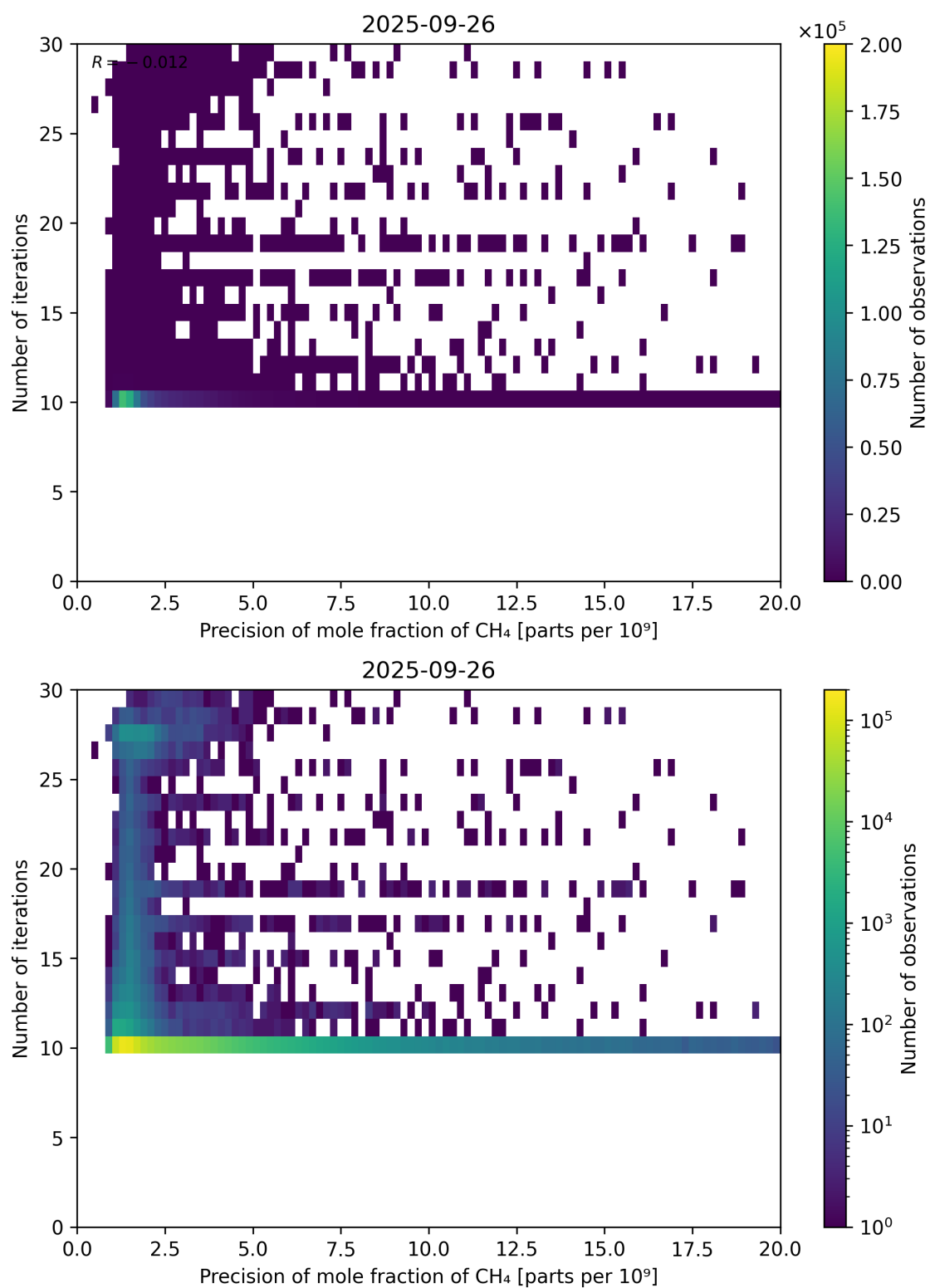
Figure 83: Scatter density plot of “Precision of mole fraction of CH 4 ” against “Number of iterations” for 2025-09-26 to 2025-09-27.
