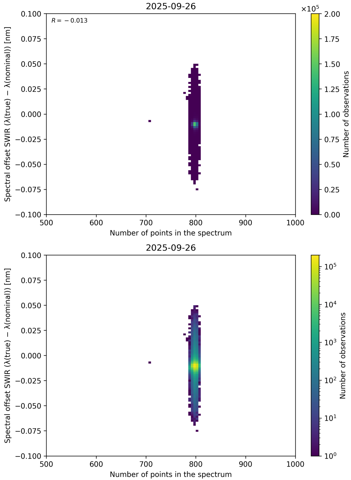
Figure 93: Scatter density plot of “Number of points in the spectrum” against “Spectral offset SWIR ( \lambda_{\text{true}} - \lambda_{\text{nominal}} )” for 2025-09-26 to 2025-09-27.
