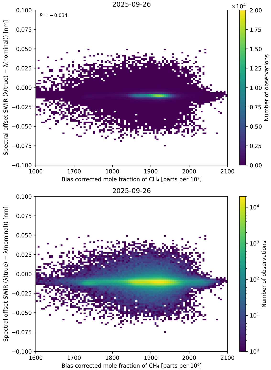
Figure 69: Scatter density plot of “Bias corrected mole fraction of \text{CH}_4 ” against “Spectral offset SWIR ( \lambda_{\text{true}} - \lambda_{\text{nominal}} )” for 2025-09-26 to 2025-09-27.
