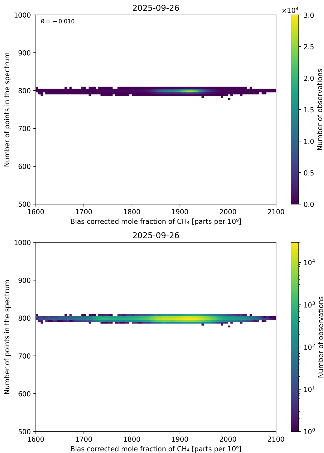
Figure 68: Scatter density plot of “Bias corrected mole fraction of CH 4 ” against “Number of points in the spectrum” for 2025-09-26 to 2025-09-27.
