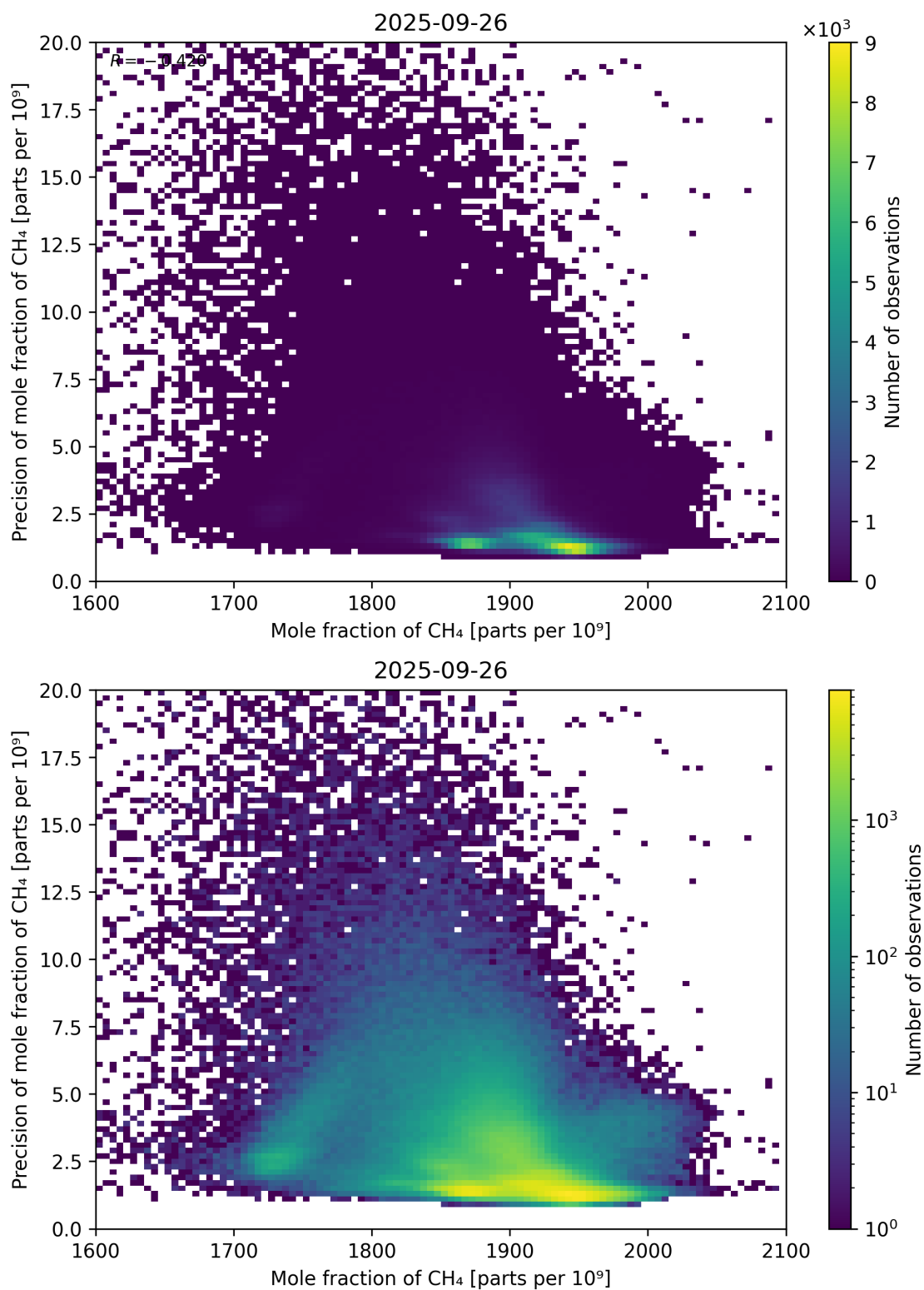
Figure 75: Scatter density plot of “Mole fraction of CH 4 ” against “Precision of mole fraction of CH 4 ” for 2025-09-26 to 2025-09-27.
