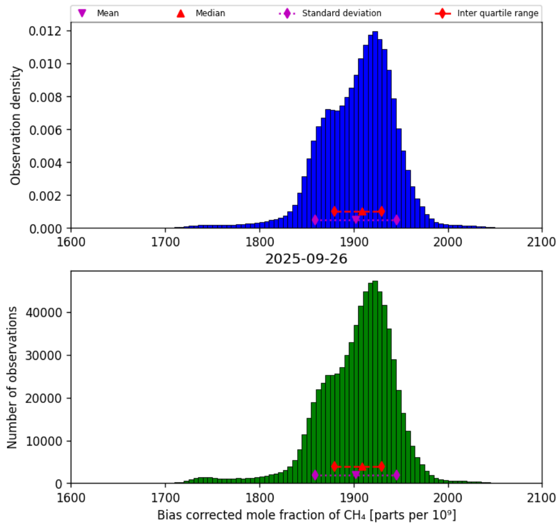
Figure 25: Histogram of “Bias corrected mole fraction of CH 4 ” for 2025-09-26 to 2025-09-27
