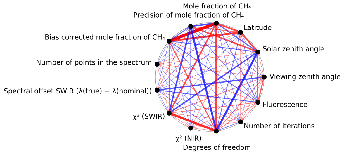
Figure 1: Map of correlation graph for 2025-09-26 to 2025-09-27.
