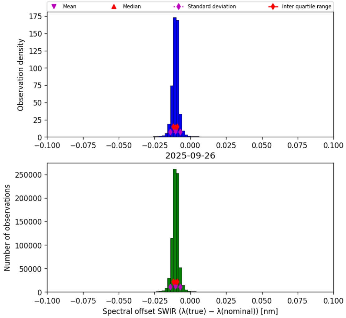
Figure 27: Histogram of “Spectral offset SWIR ( \lambda_{\text{true}} - \lambda_{\text{nominal}} )” for 2025-09-26 to 2025-09-27
