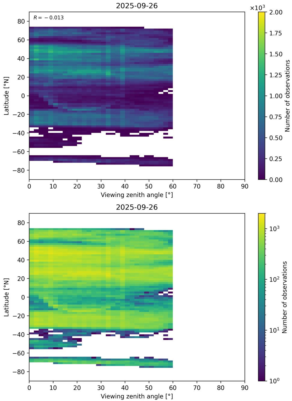
Figure 109: Scatter density plot of “Viewing zenith angle” against “Latitude” for 2025-09-26 to 2025-09-27.
