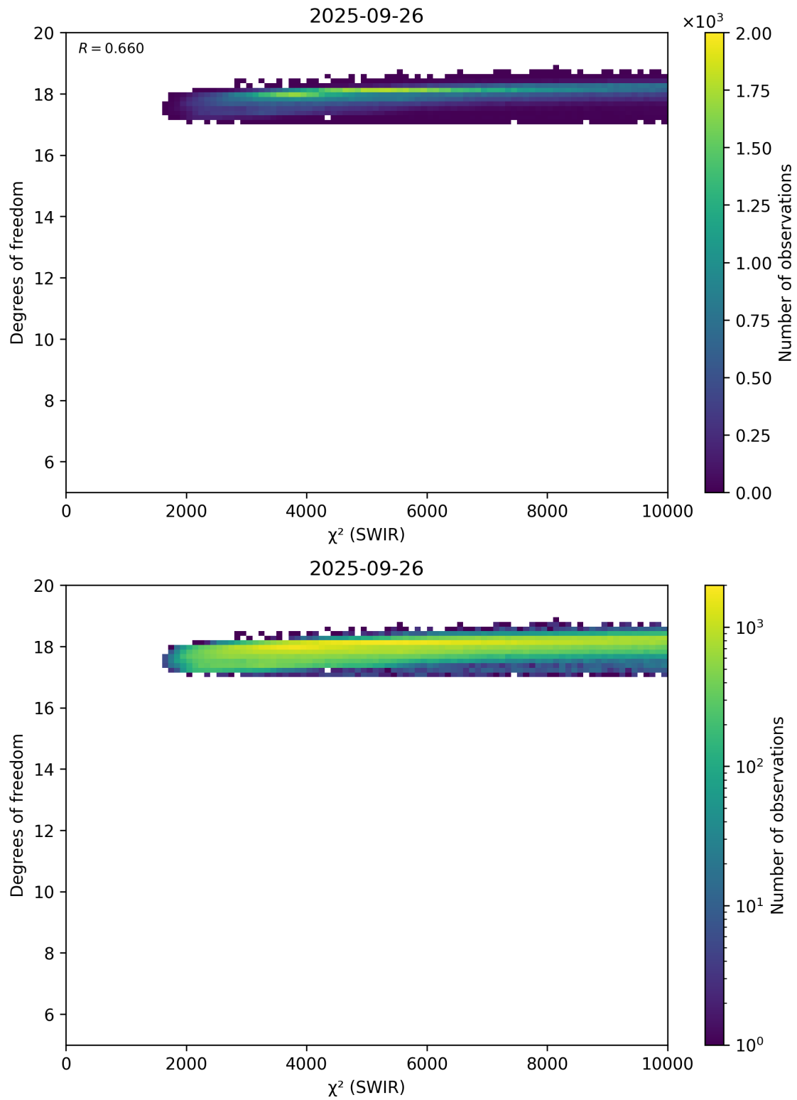
Figure 48: Scatter density plot of “ \chi^2 (SWIR)” against “Degrees of freedom” for 2025-09-26 to 2025-09-27.
