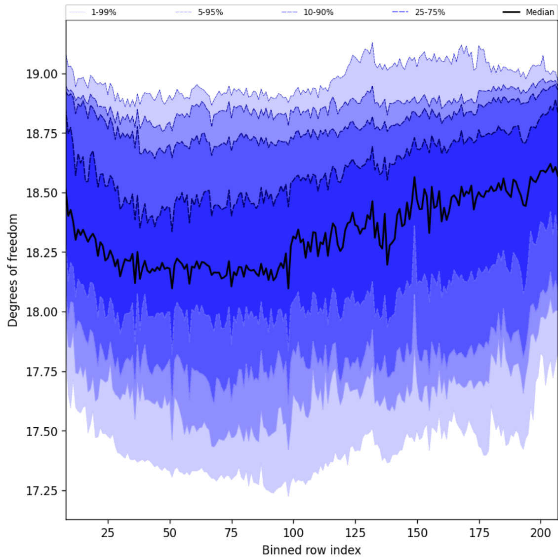
Figure 41: Along track statistics of “Degrees of freedom” for 2025-09-26 to 2025-09-27
