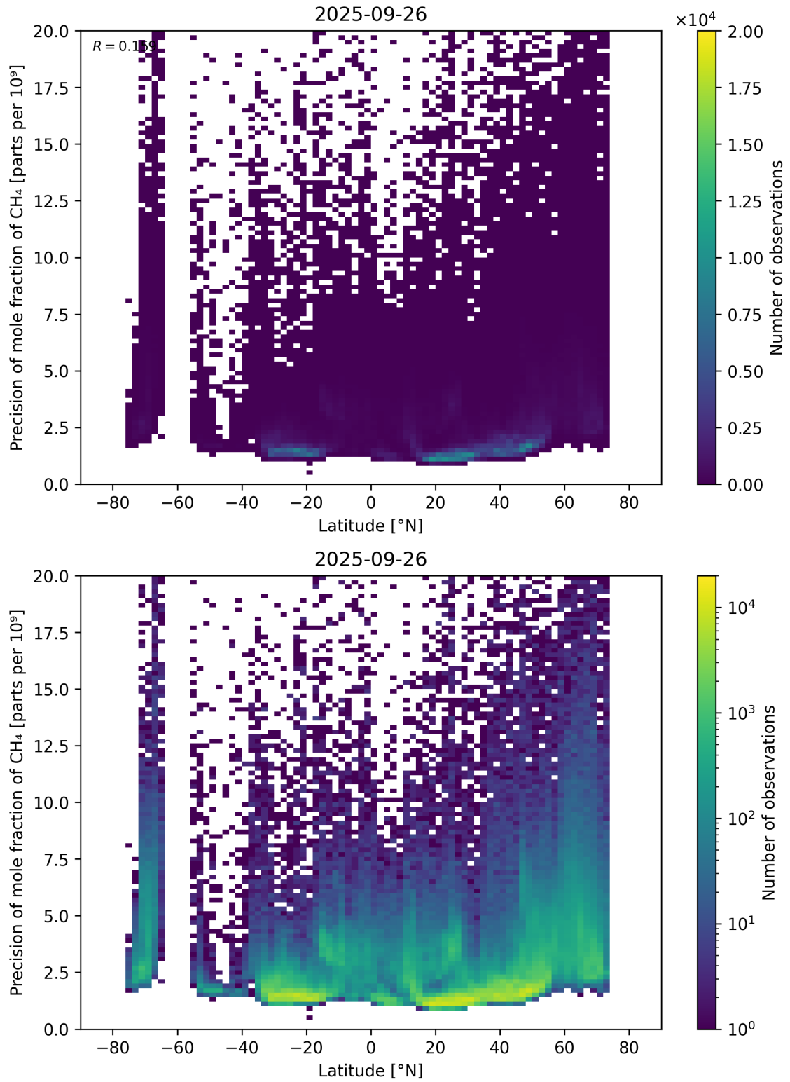
Figure 59: Scatter density plot of “Latitude” against “Precision of mole fraction of \text{CH}_4 ” for 2025-09-26 to 2025-09-27.
