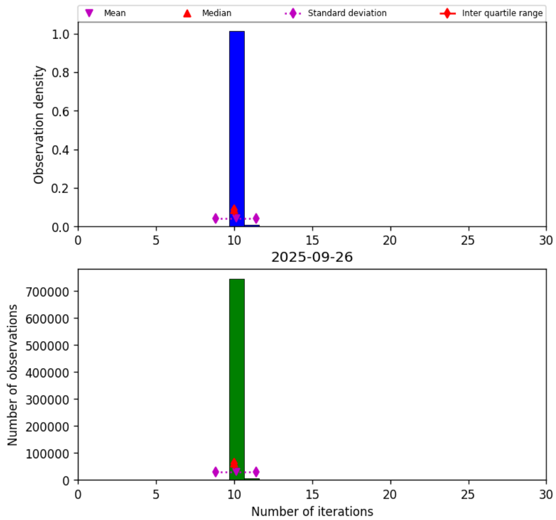
Figure 31: Histogram of “Number of iterations” for 2025-09-26 to 2025-09-27
