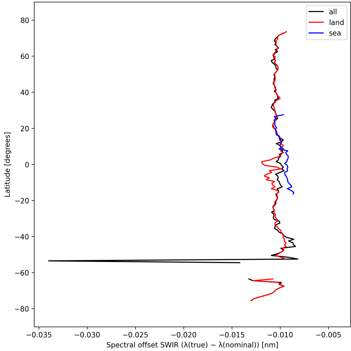
Figure 16: Zonal average of “Spectral offset SWIR ( \lambda_{\text{true}} - \lambda_{\text{nominal}} )” for 2025-09-26 to 2025-09-28.
