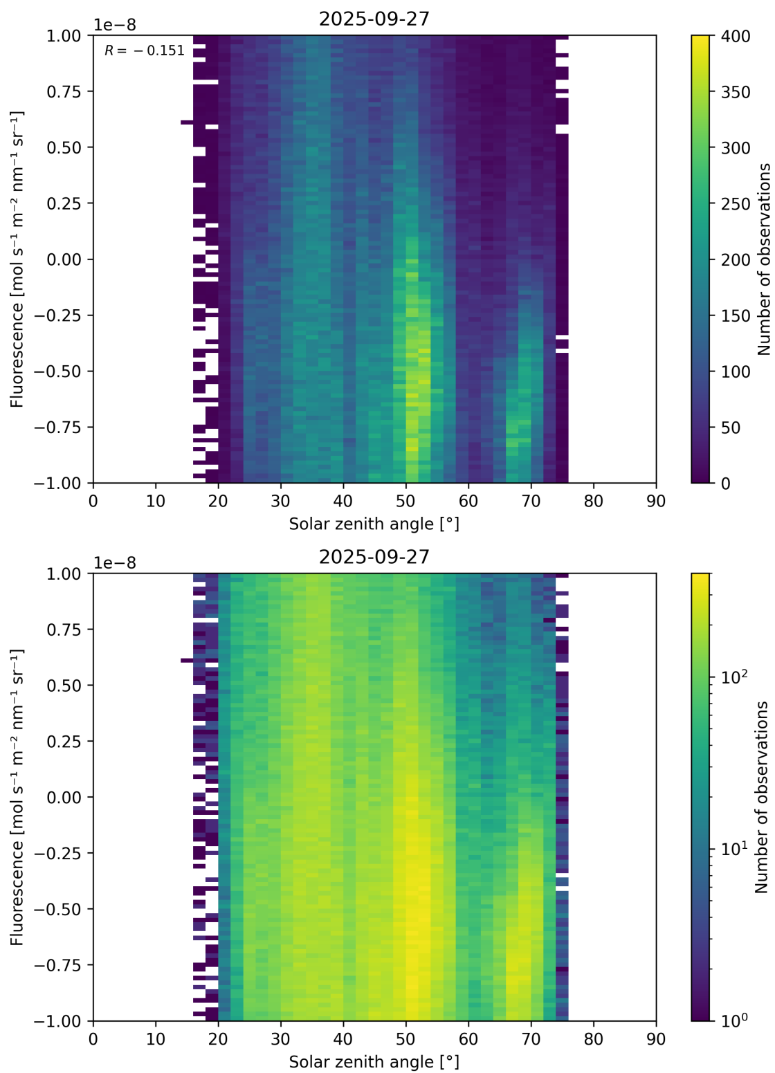
Figure 97: Scatter density plot of “Solar zenith angle” against “Fluorescence” for 2025-09-26 to 2025-09-28.
