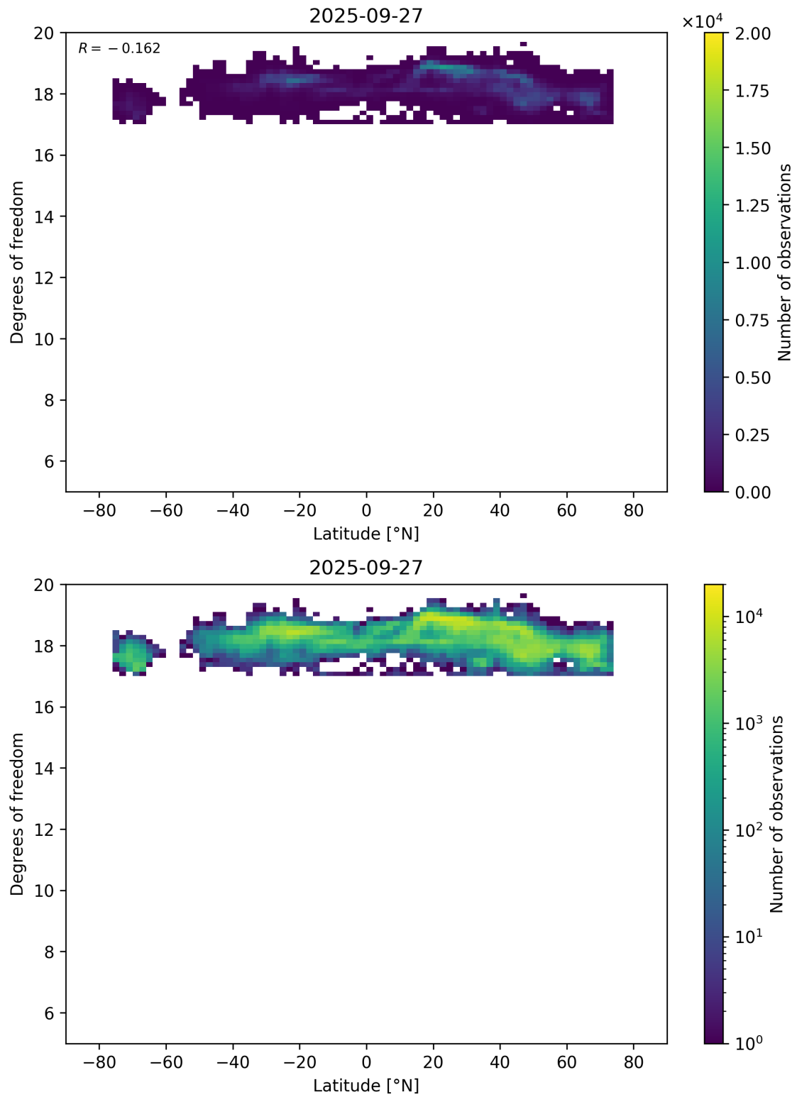
Figure 55: Scatter density plot of “Latitude” against “Degrees of freedom” for 2025-09-26 to 2025-09-28.
