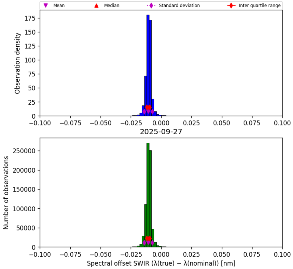
Figure 27: Histogram of “Spectral offset SWIR ( \lambda_{\text{true}} - \lambda_{\text{nominal}} )” for 2025-09-26 to 2025-09-28
