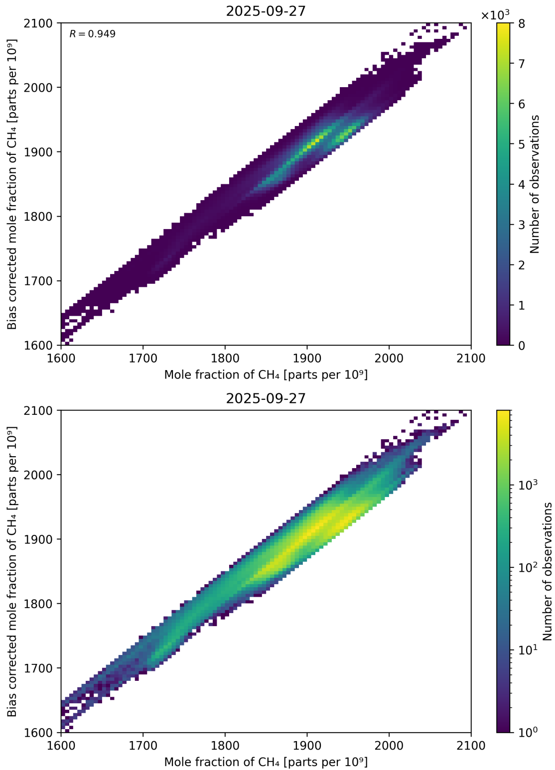
Figure 74: Scatter density plot of “Mole fraction of CH 4 ” against “Bias corrected mole fraction of CH 4 ” for 2025-09-26 to 2025-09-28.
