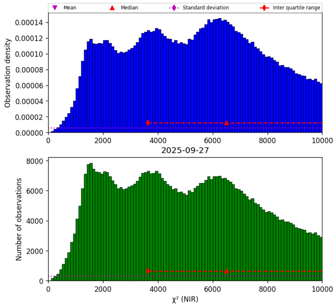
Figure 29: Histogram of “ \chi^2 (NIR)” for 2025-09-26 to 2025-09-28
