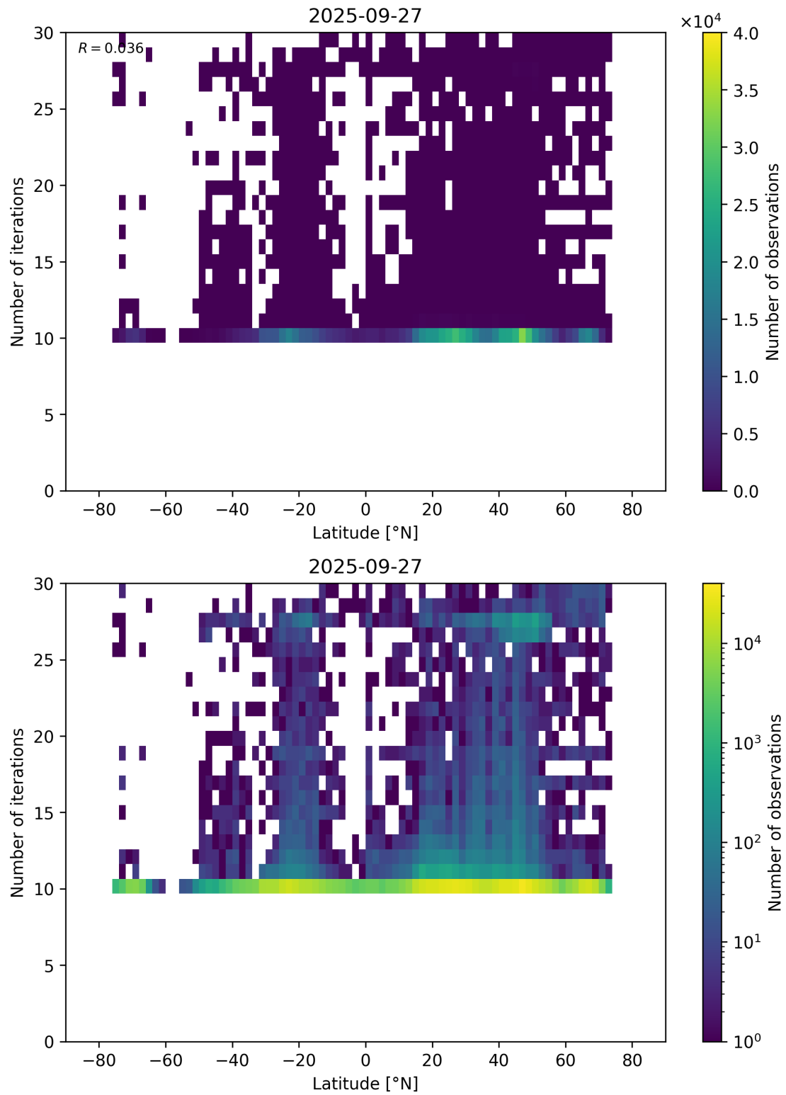
Figure 60: Scatter density plot of “Latitude” against “Number of iterations” for 2025-09-26 to 2025-09-28.
