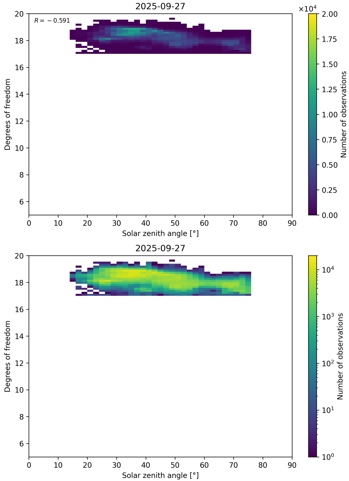
Figure 96: Scatter density plot of “Solar zenith angle” against “Degrees of freedom” for 2025-09-26 to 2025-09-28.
