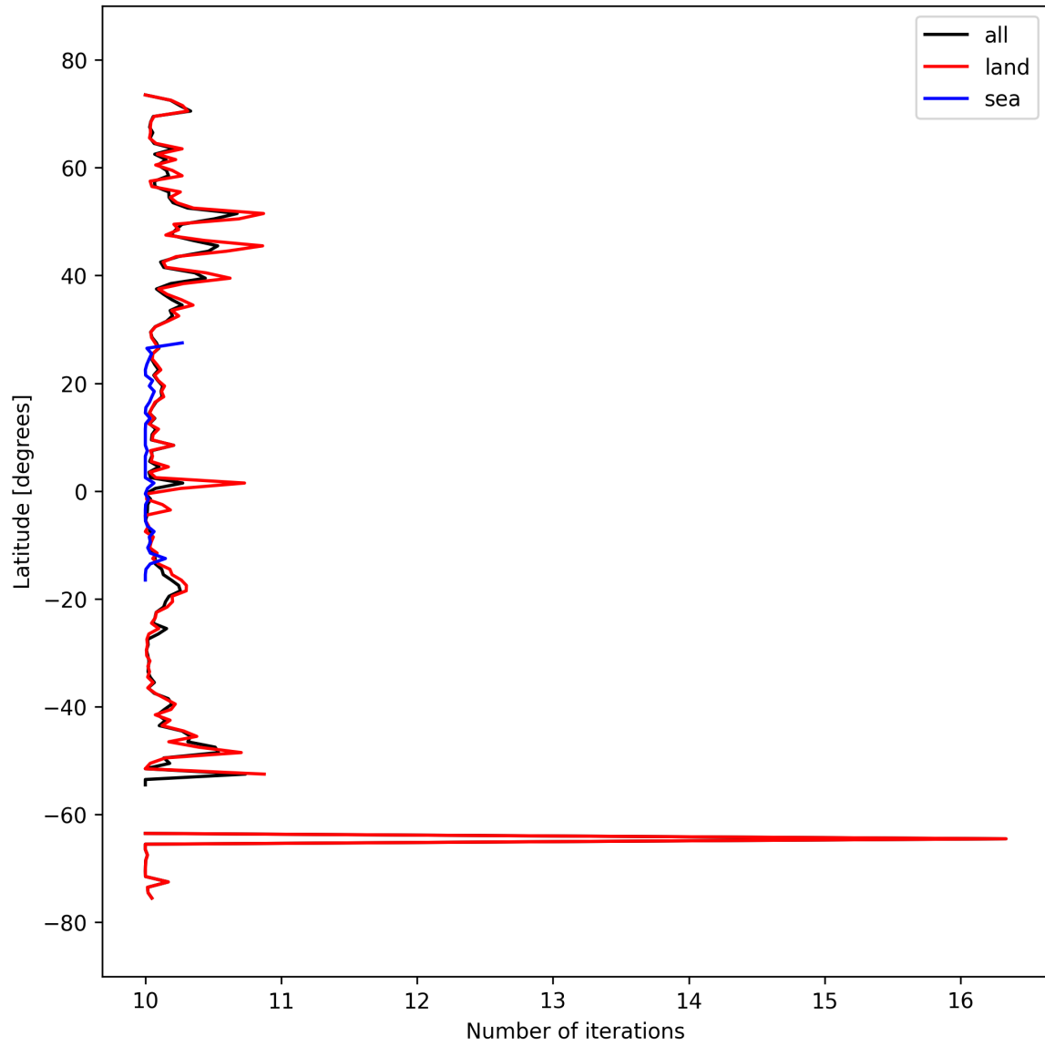
Figure 20: Zonal average of “Number of iterations” for 2025-09-26 to 2025-09-28.
