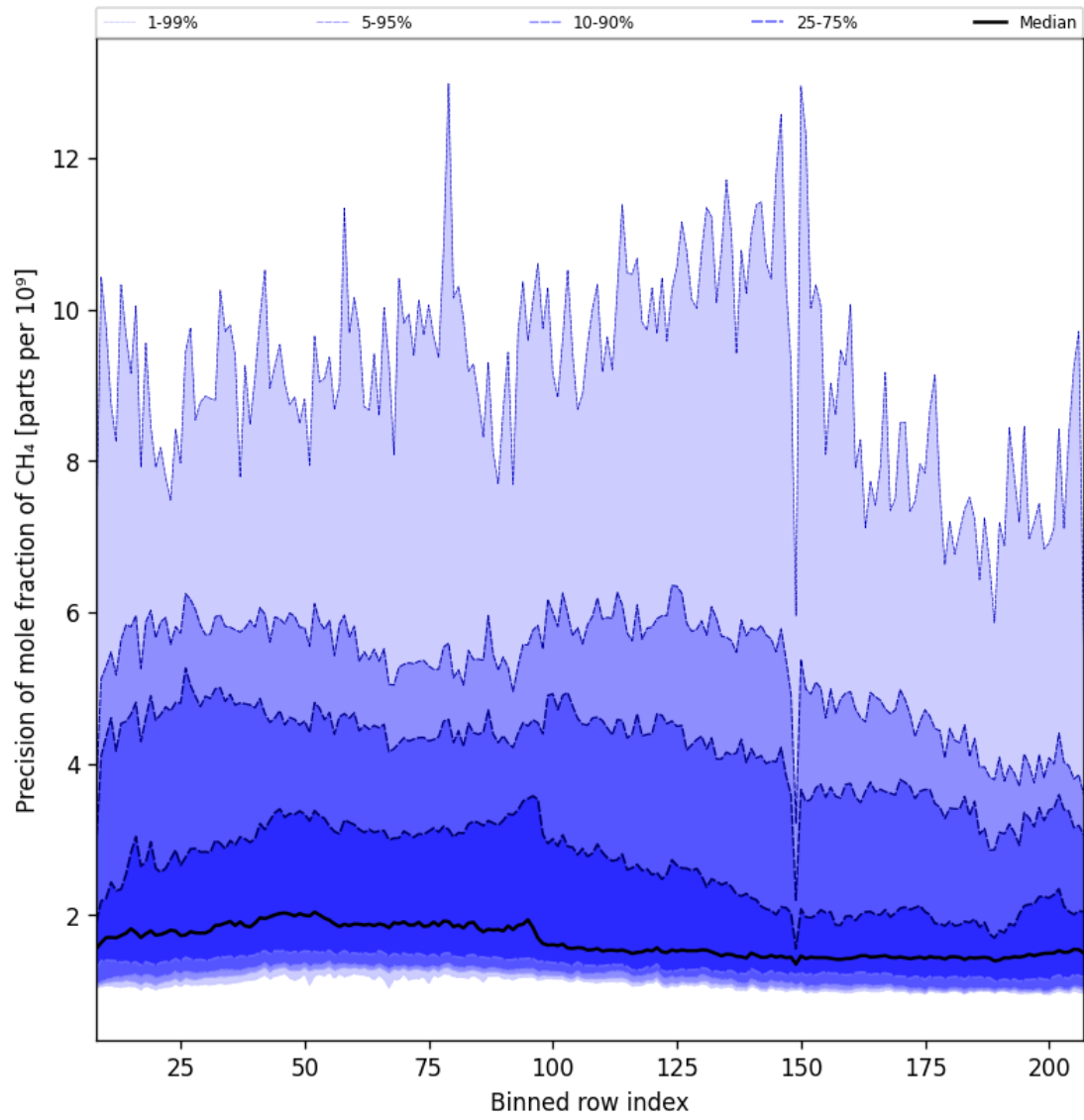
Figure 35: Along track statistics of “Precision of mole fraction of CH 4 ” for 2025-09-26 to 2025-09-28
