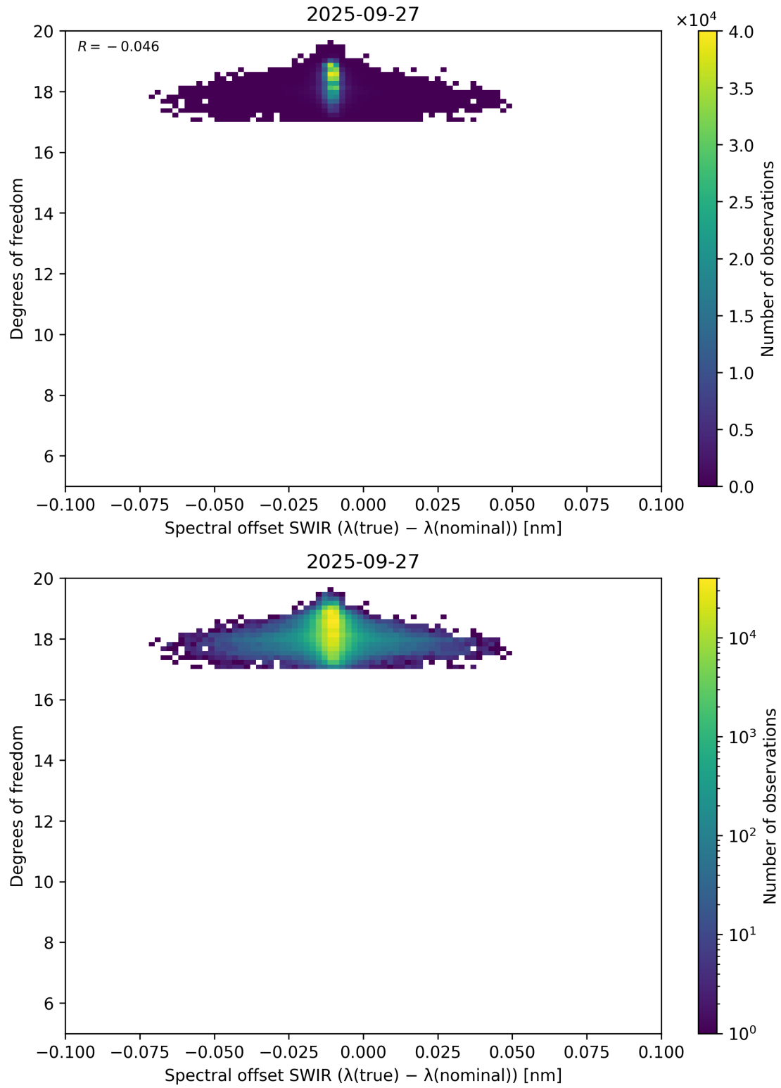
Figure 119: Scatter density plot of “Spectral offset SWIR ( \lambda_{\text{true}} - \lambda_{\text{nominal}} )” against “Degrees of freedom” for 2025-09-26 to 2025-09-28.
