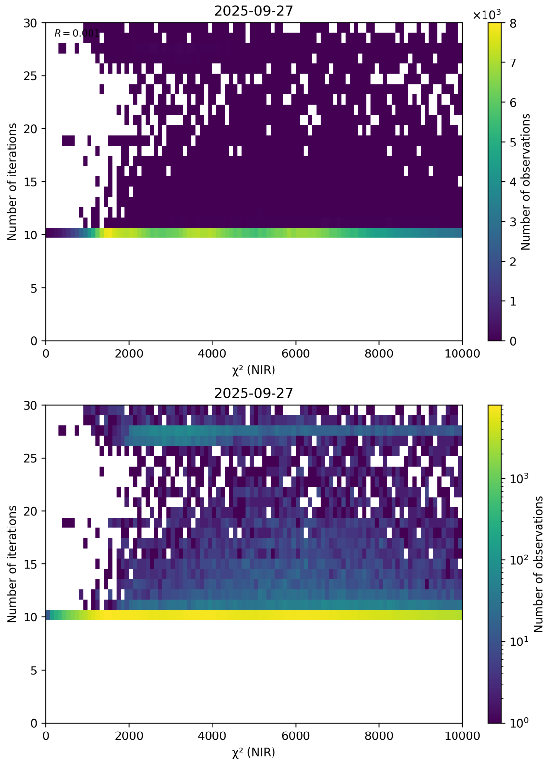
Figure 46: Scatter density plot of “ \chi^2 (NIR)” against “Number of iterations” for 2025-09-26 to 2025-09-28.
