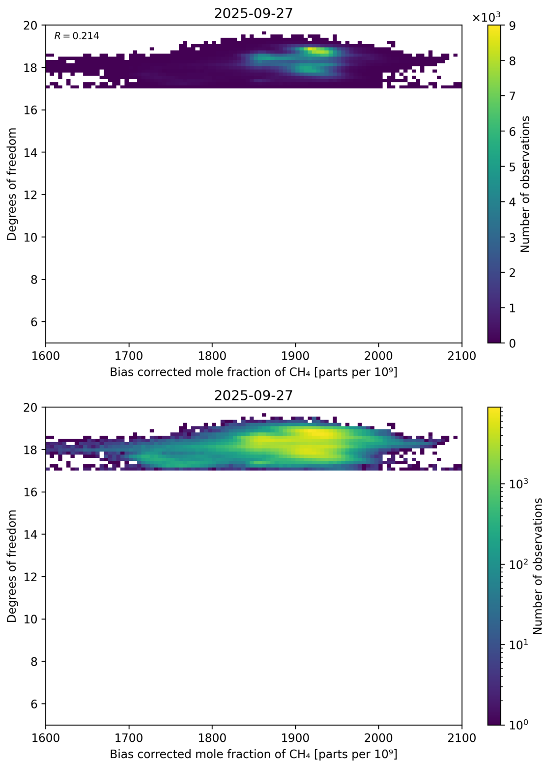
Figure 65: Scatter density plot of “Bias corrected mole fraction of CH 4 ” against “Degrees of freedom” for 2025-09-26 to 2025-09-28.
