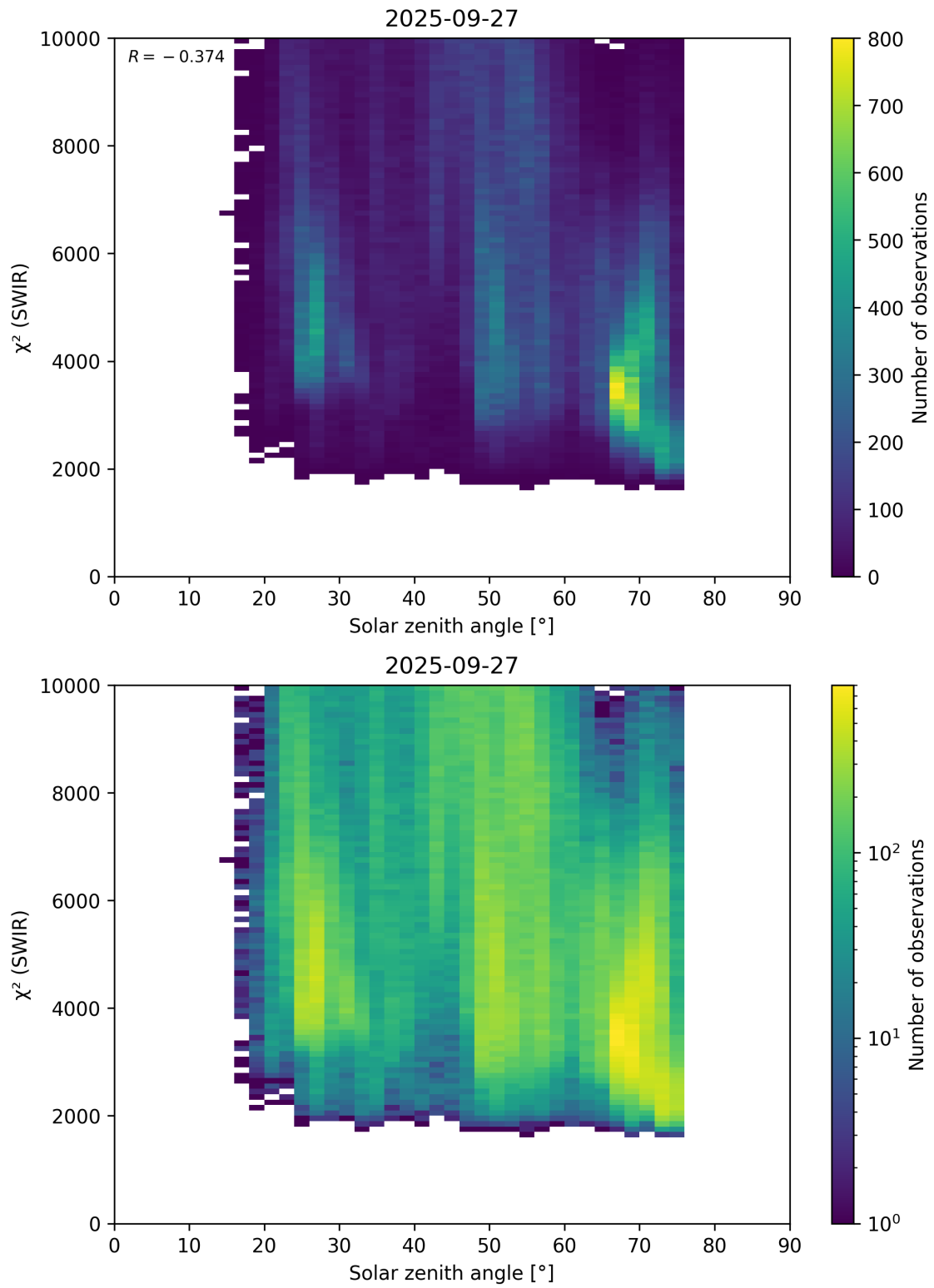
Figure 95: Scatter density plot of “Solar zenith angle” against “ \chi^2 (SWIR)” for 2025-09-26 to 2025-09-28.
