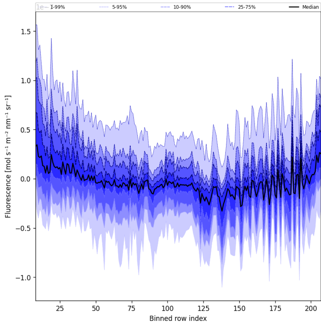
Figure 43: Along track statistics of “Fluorescence” for 2025-09-26 to 2025-09-28
