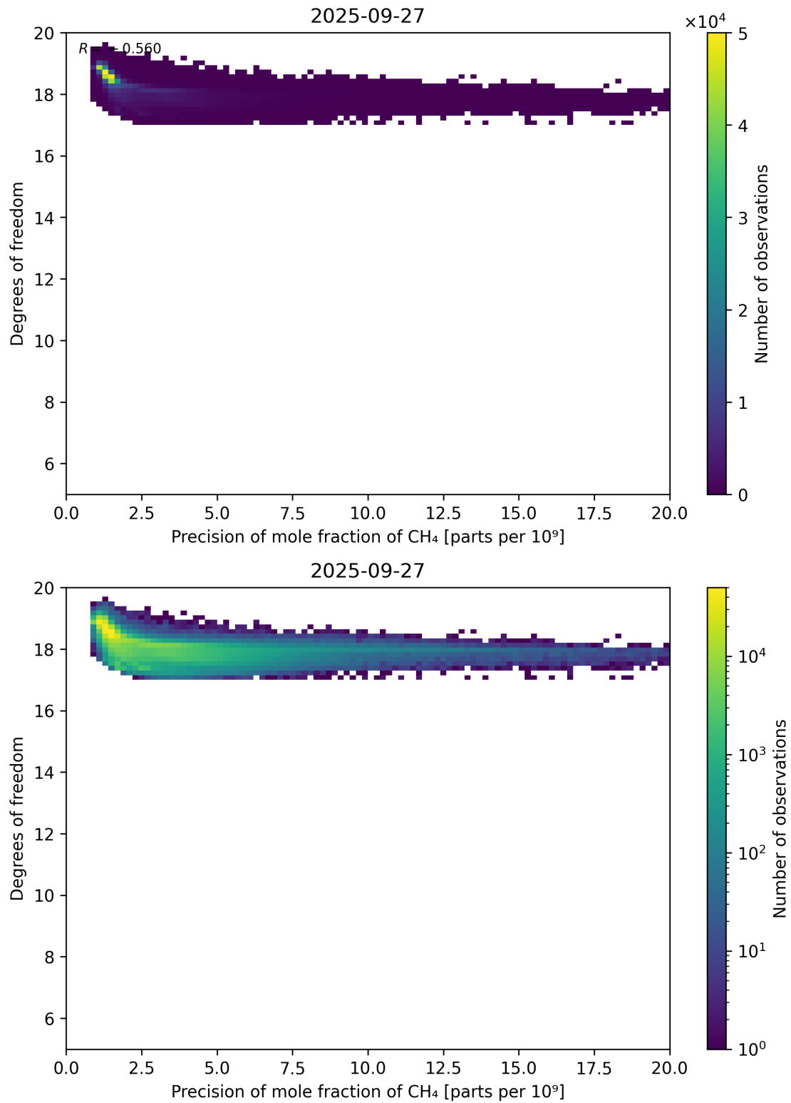
Figure 80: Scatter density plot of “Precision of mole fraction of CH 4 ” against “Degrees of freedom” for 2025-09-26 to 2025-09-28.
