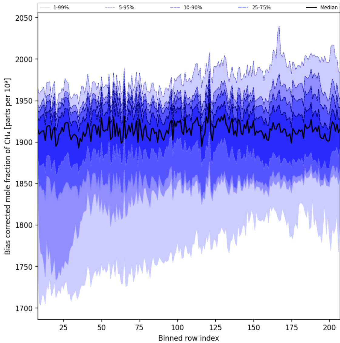
Figure 36: Along track statistics of “Bias corrected mole fraction of CH 4 ” for 2025-09-26 to 2025-09-28
