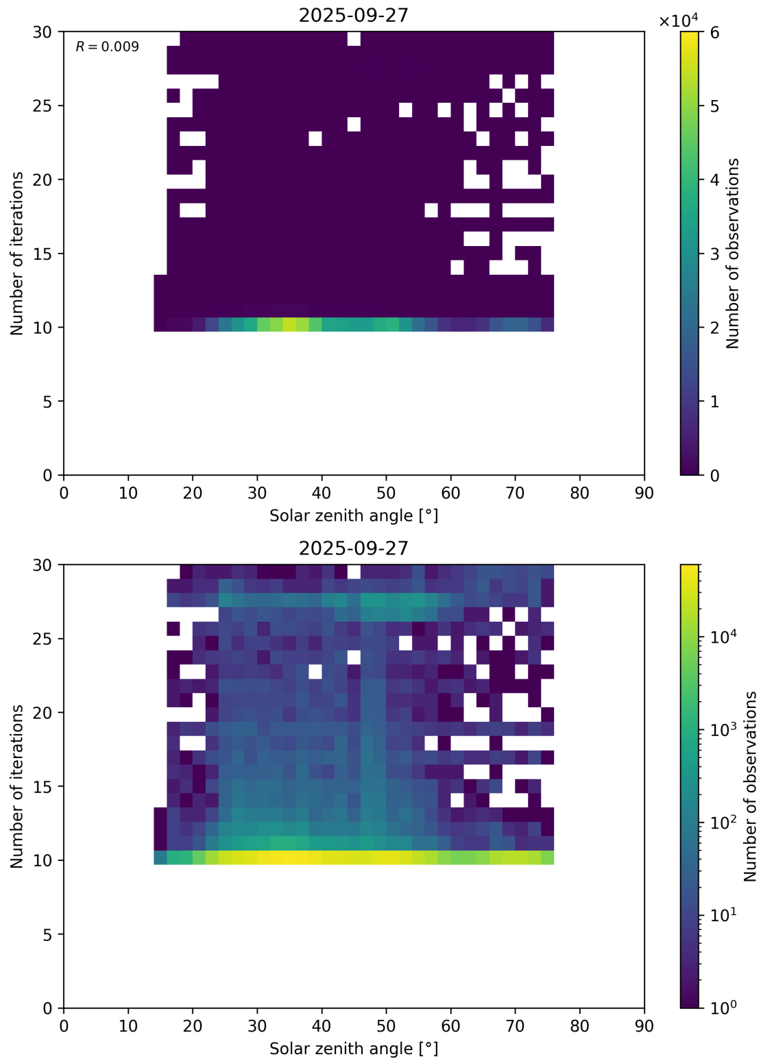
Figure 102: Scatter density plot of “Solar zenith angle” against “Number of iterations” for 2025-09-26 to 2025-09-28.
