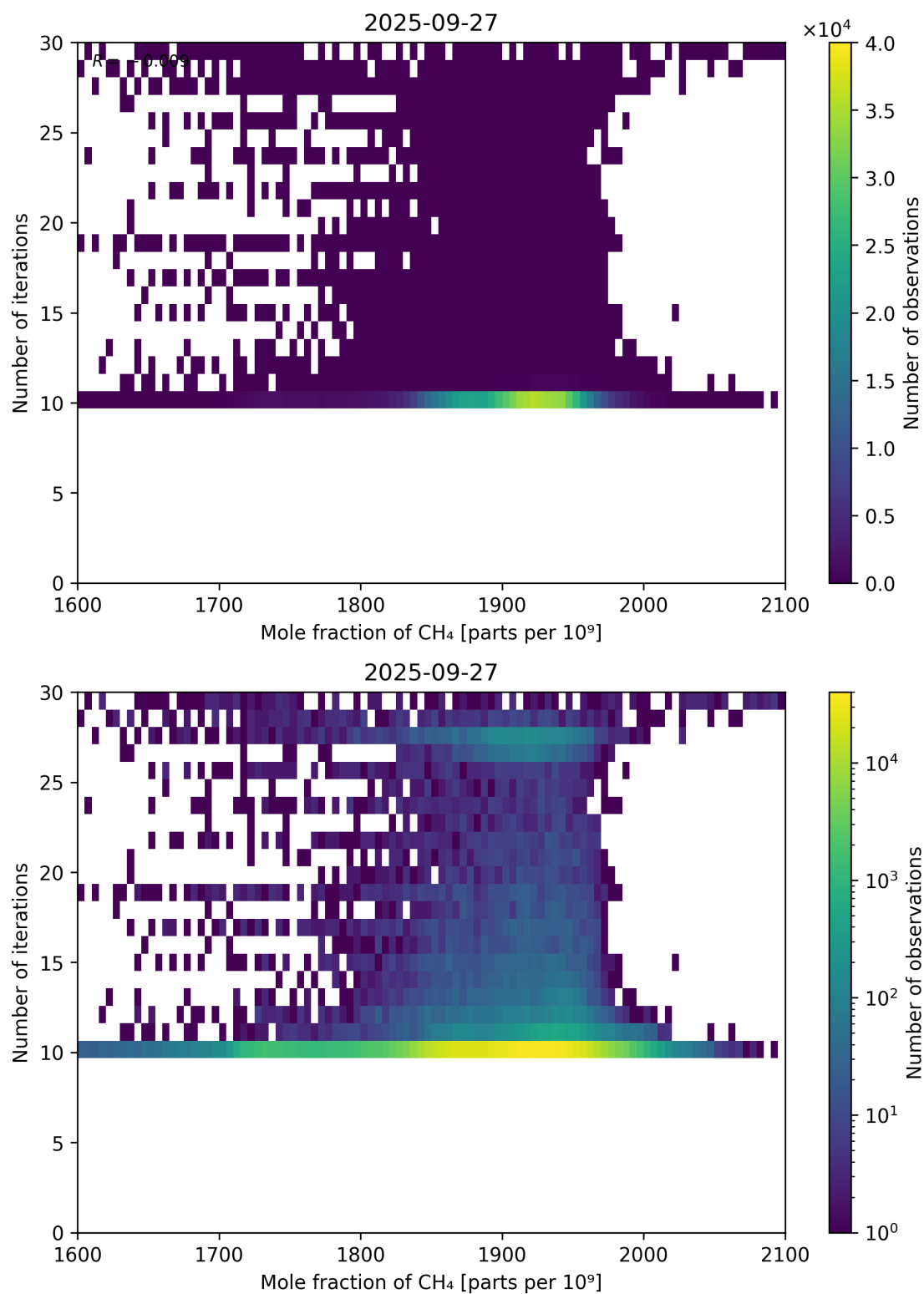
Figure 76: Scatter density plot of “Mole fraction of CH 4 ” against “Number of iterations” for 2025-09-26 to 2025-09-28.
