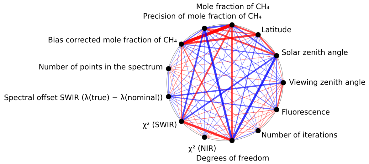
Figure 1: Map of correlation graph for 2025-09-26 to 2025-09-28.
