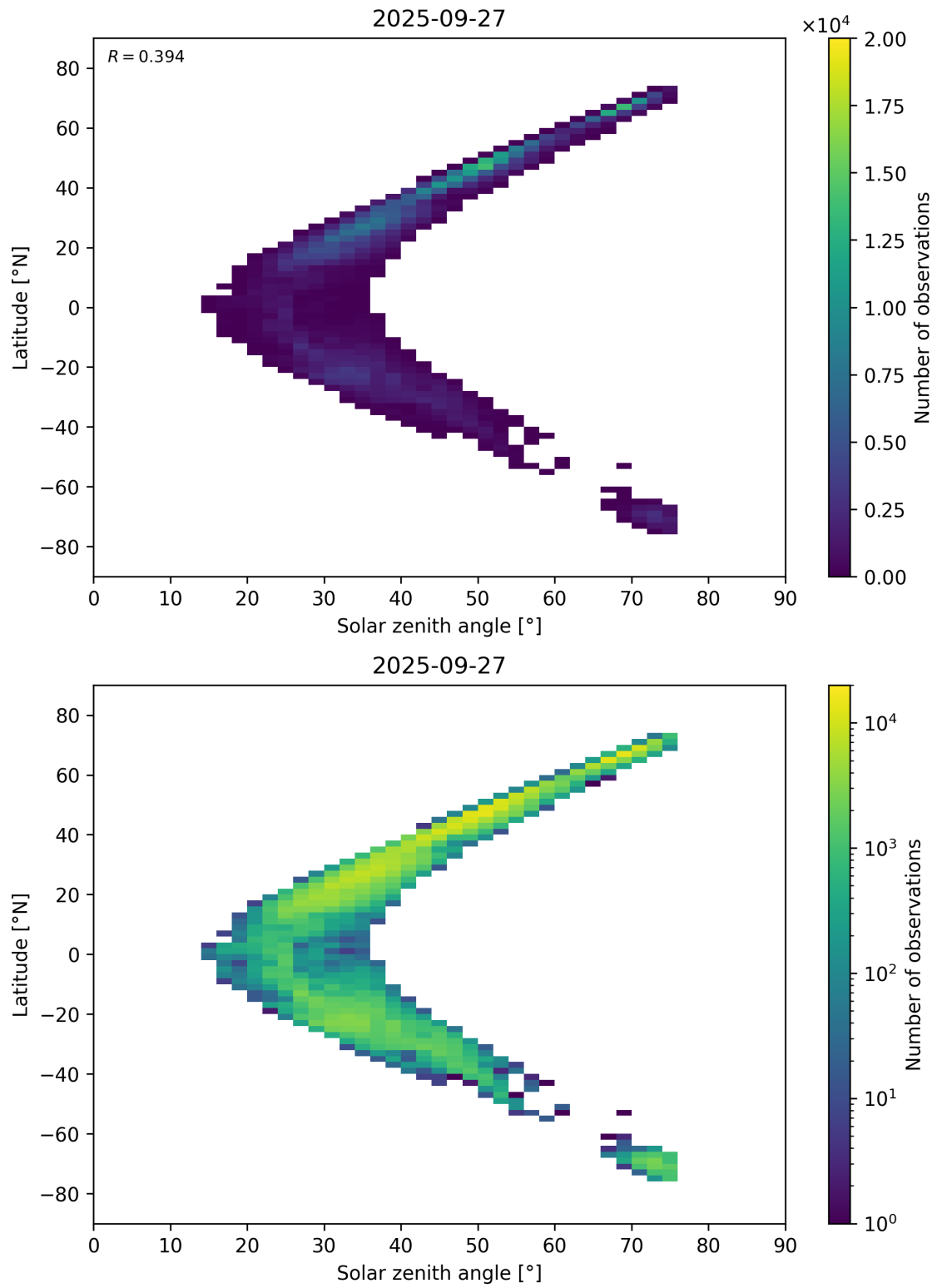
Figure 98: Scatter density plot of “Solar zenith angle” against “Latitude” for 2025-09-26 to 2025-09-28.
