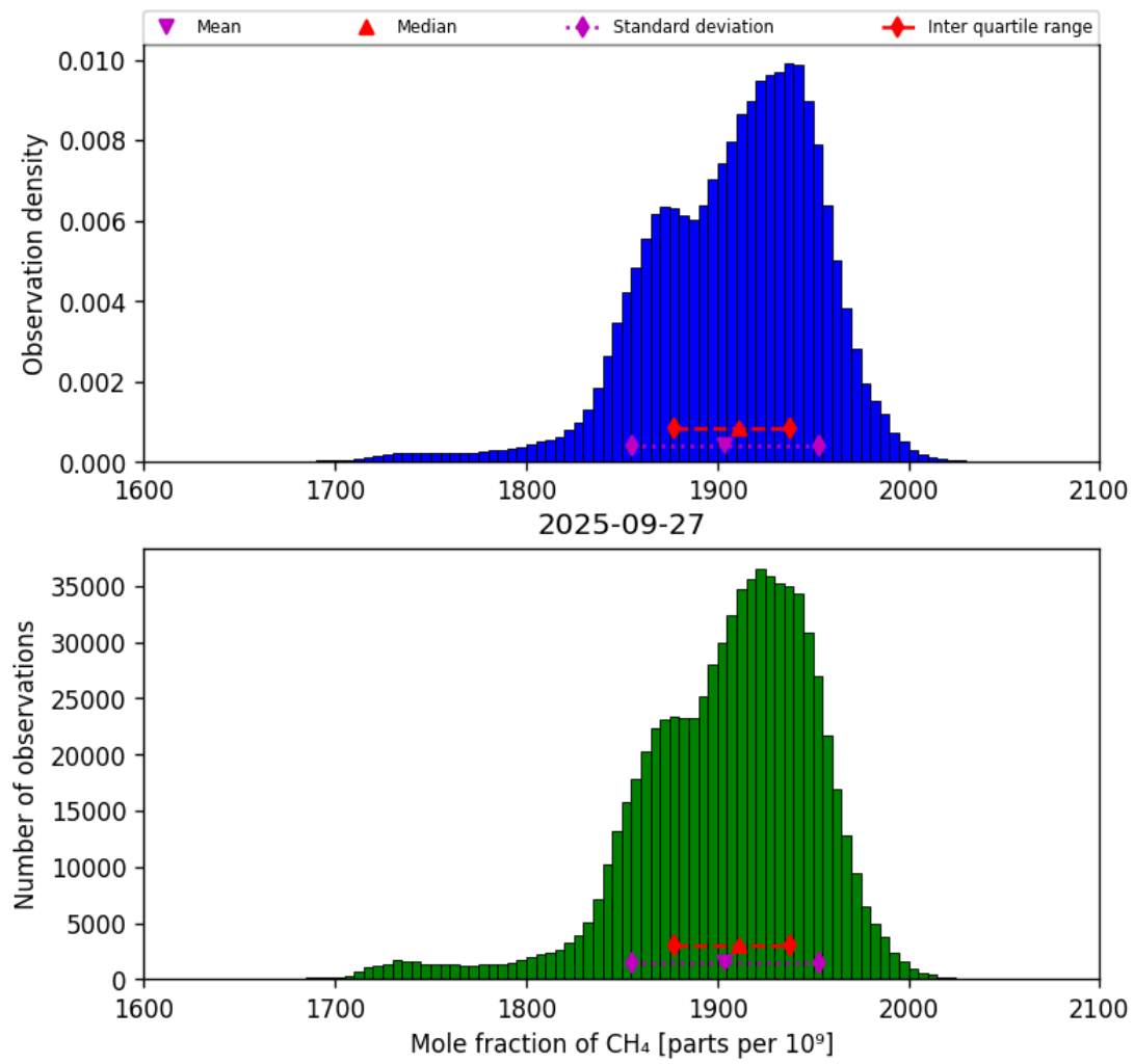
Figure 23: Histogram of “Mole fraction of CH 4 ” for 2025-09-26 to 2025-09-28
