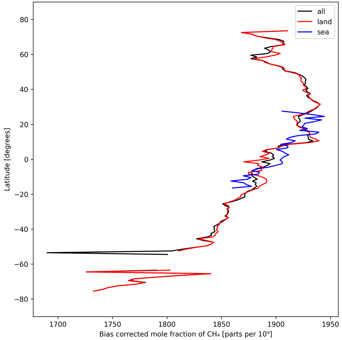
Figure 14: Zonal average of “Bias corrected mole fraction of CH 4 ” for 2025-09-26 to 2025-09-28.
