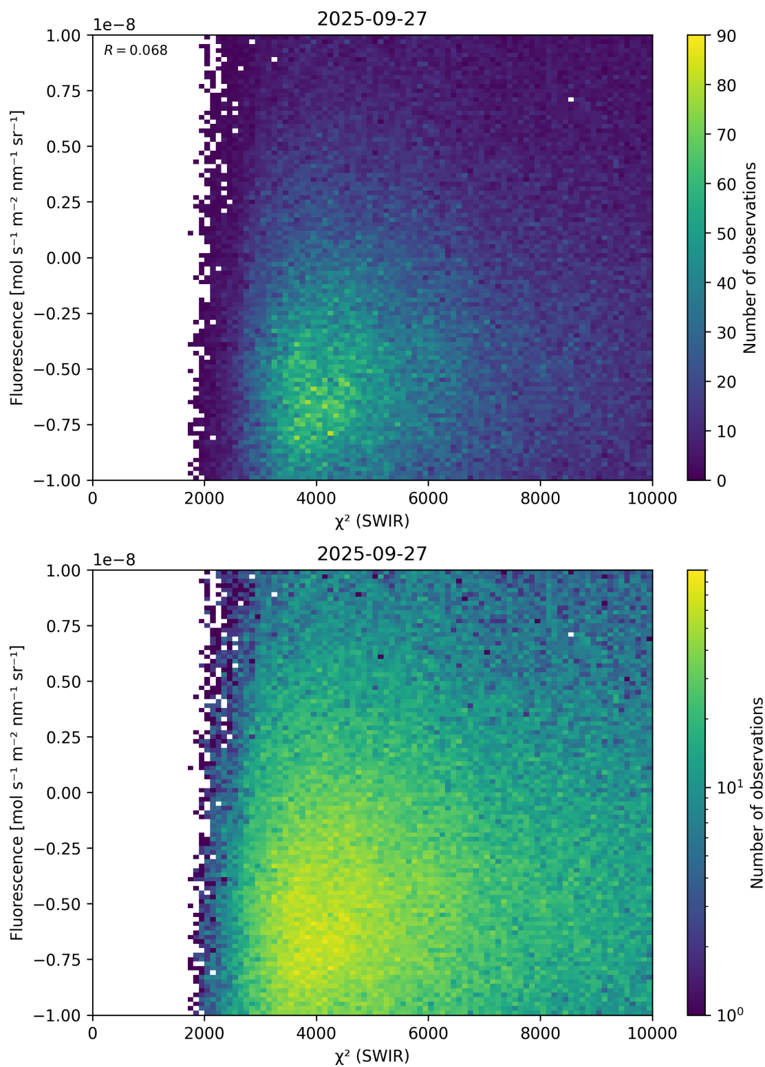
Figure 49: Scatter density plot of “ \chi^2 (SWIR)” against “Fluorescence” for 2025-09-26 to 2025-09-28.
