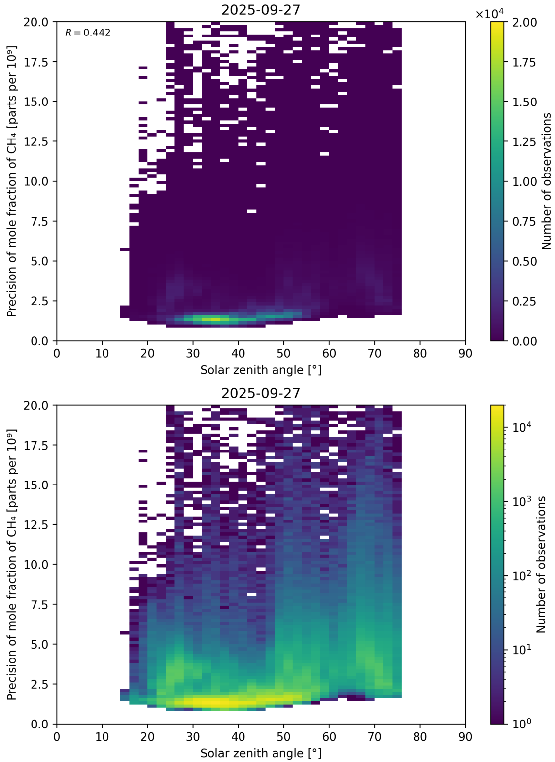
Figure 101: Scatter density plot of “Solar zenith angle” against “Precision of mole fraction of \text{CH}_4 ” for 2025-09-26 to 2025-09-28.
