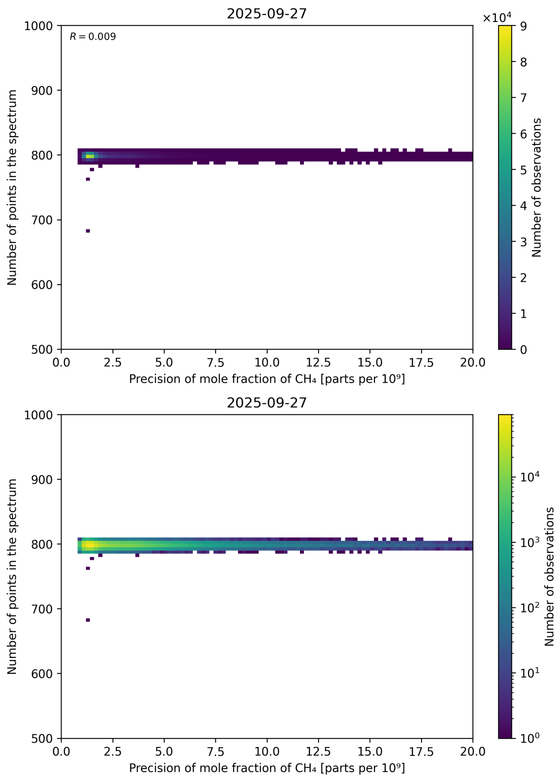
Figure 84: Scatter density plot of “Precision of mole fraction of CH 4 ” against “Number of points in the spectrum” for 2025-09-26 to 2025-09-28.
