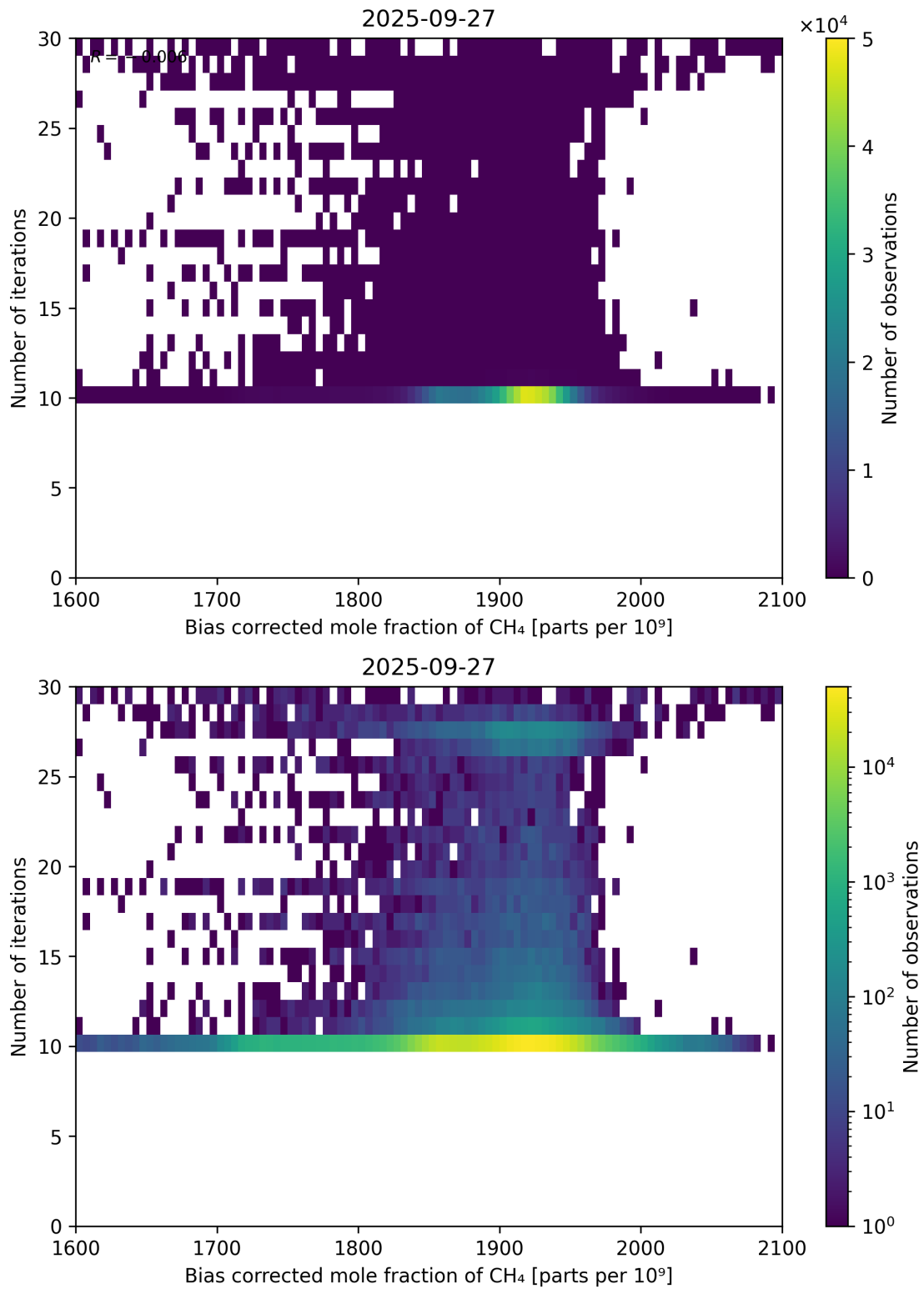
Figure 67: Scatter density plot of “Bias corrected mole fraction of CH 4 ” against “Number of iterations” for 2025-09-26 to 2025-09-28.
