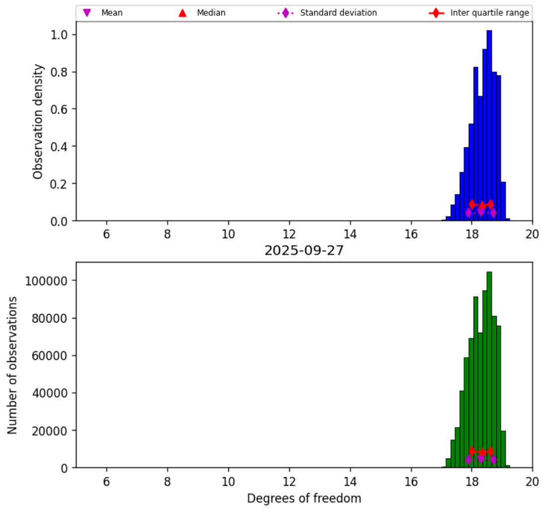
Figure 30: Histogram of “Degrees of freedom” for 2025-09-26 to 2025-09-28
