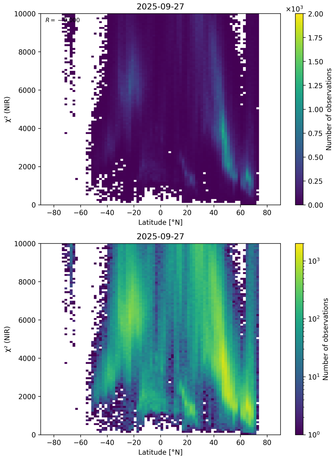
Figure 53: Scatter density plot of “Latitude” against “ \chi^2 (NIR)” for 2025-09-26 to 2025-09-28.
