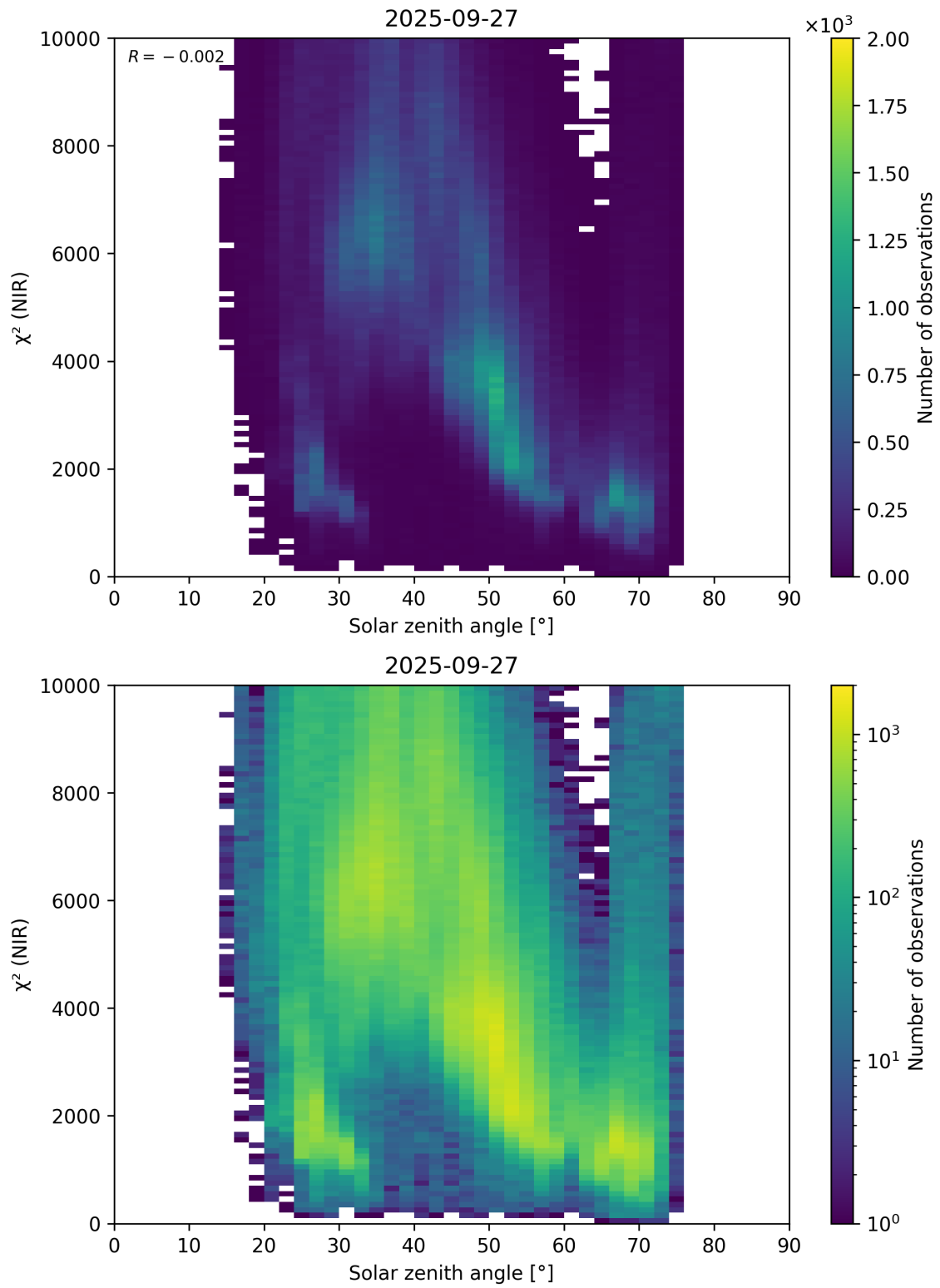
Figure 94: Scatter density plot of “Solar zenith angle” against “ \chi^2 (NIR)” for 2025-09-26 to 2025-09-28.
