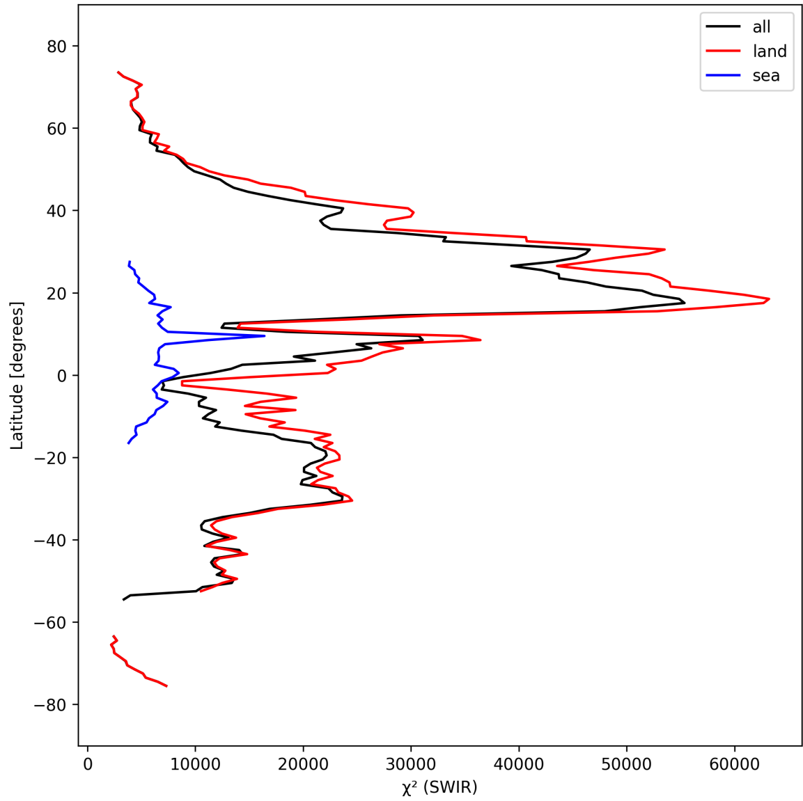
Figure 17: Zonal average of “ \chi^2 (SWIR)” for 2025-09-26 to 2025-09-28.
