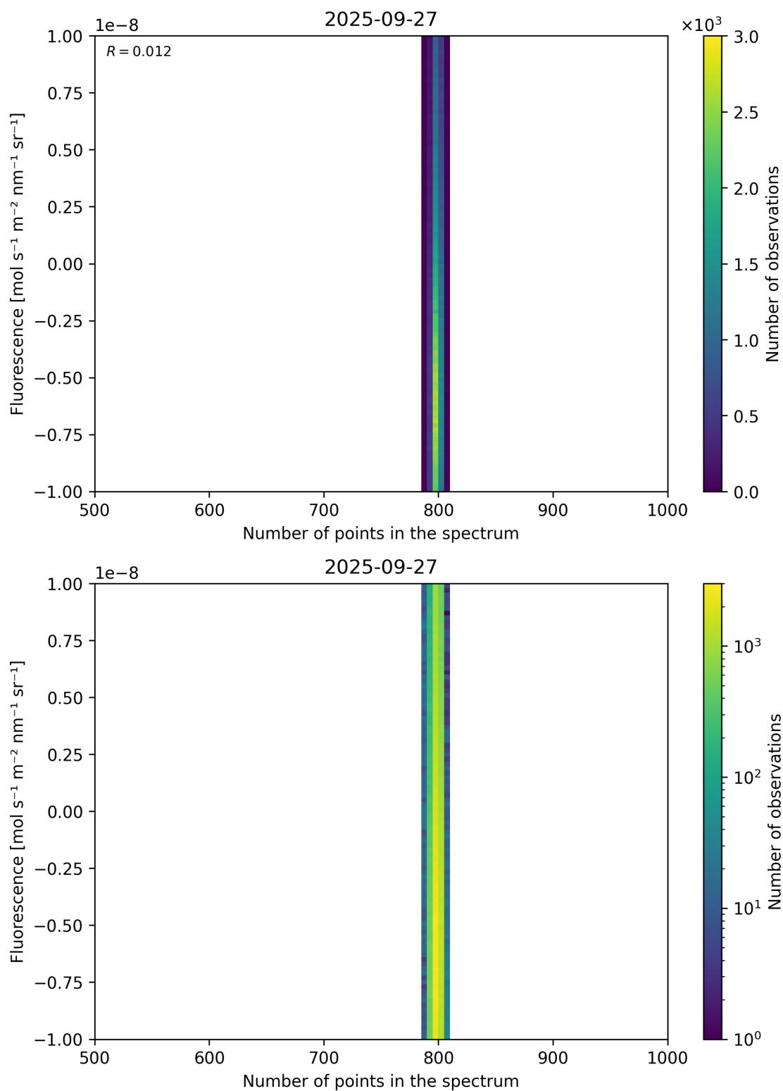
Figure 91: Scatter density plot of “Number of points in the spectrum” against “Fluorescence” for 2025-09-26 to 2025-09-28.
