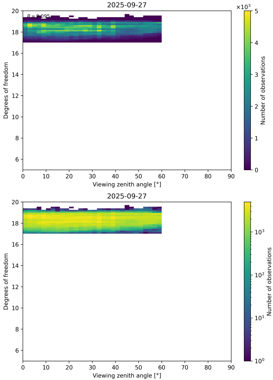
Figure 107: Scatter density plot of “Viewing zenith angle” against “Degrees of freedom” for 2025-09-26 to 2025-09-28.
