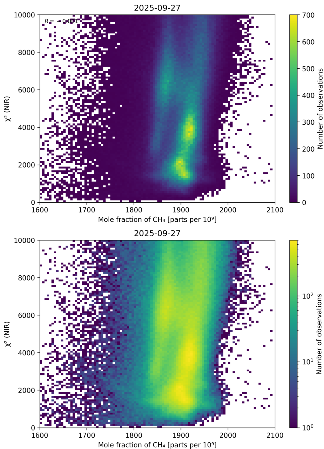
Figure 70: Scatter density plot of “Mole fraction of \text{CH}_4 ” against “ \chi^2 (NIR)” for 2025-09-26 to 2025-09-28.
