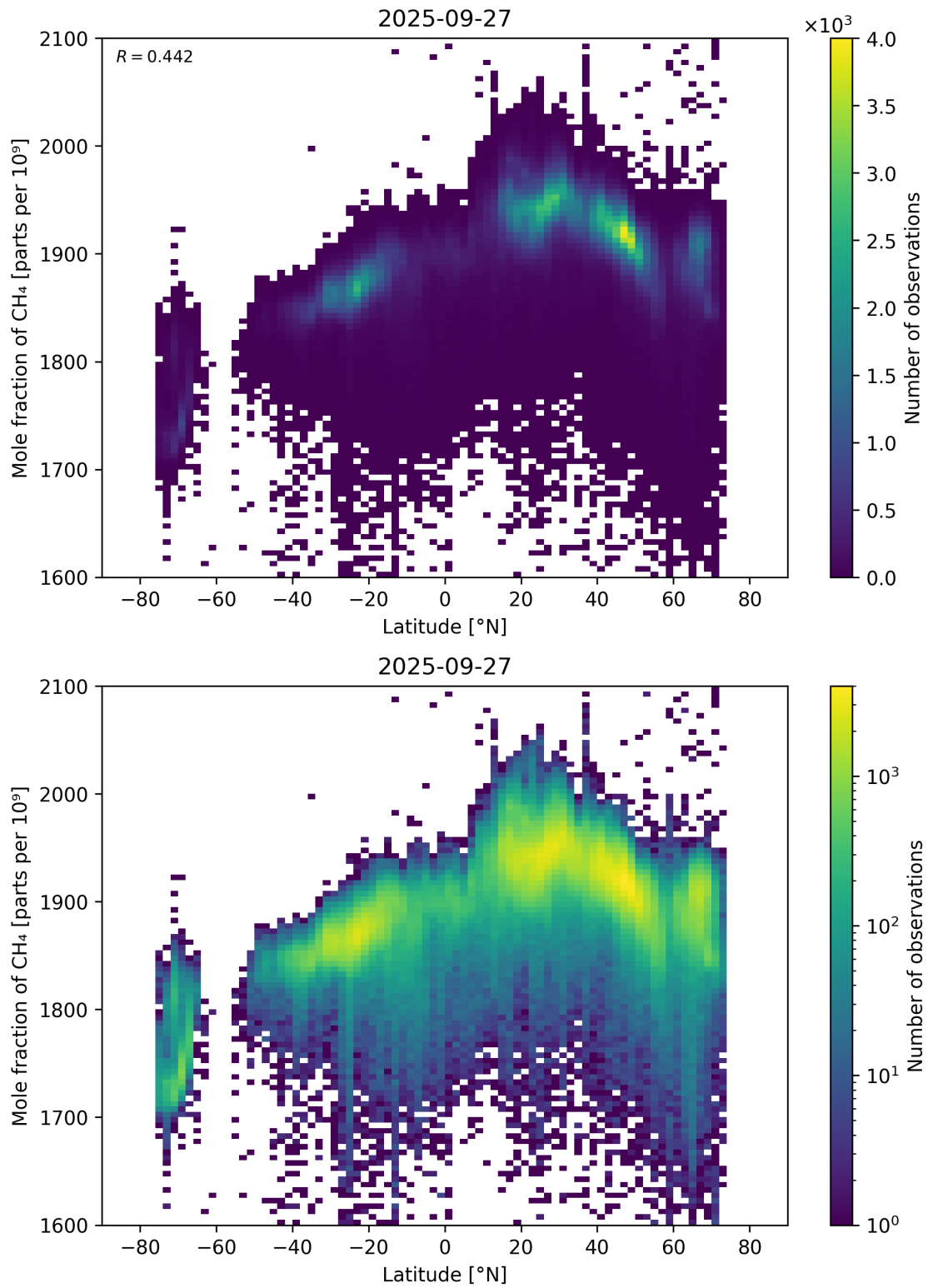
Figure 57: Scatter density plot of “Latitude” against “Mole fraction of CH 4 ” for 2025-09-26 to 2025-09-28.
