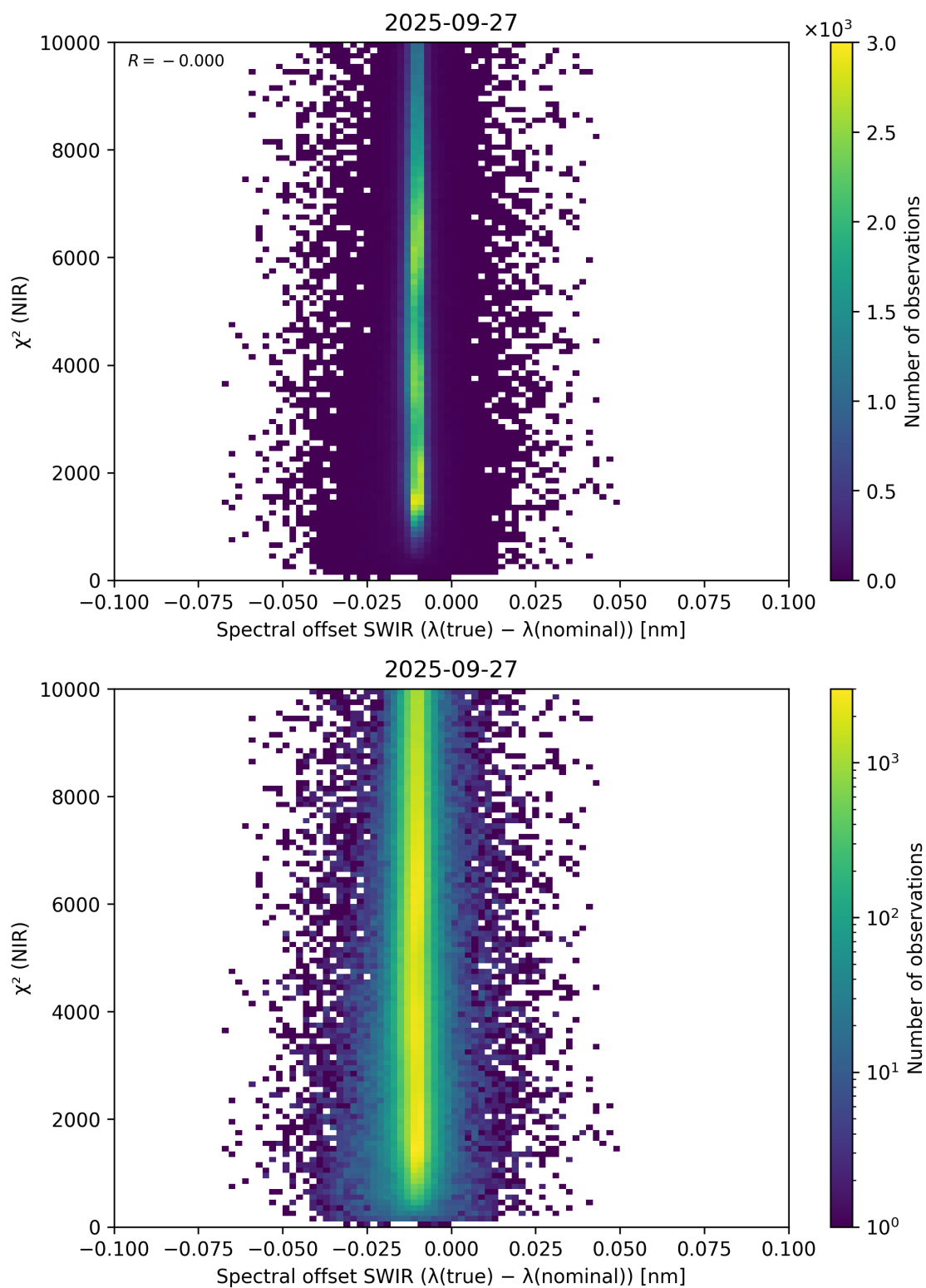
Figure 117: Scatter density plot of “Spectral offset SWIR ( \lambda_{\text{true}} - \lambda_{\text{nominal}} )” against “ \chi^2 (NIR)” for 2025-09-26 to 2025-09-28.
