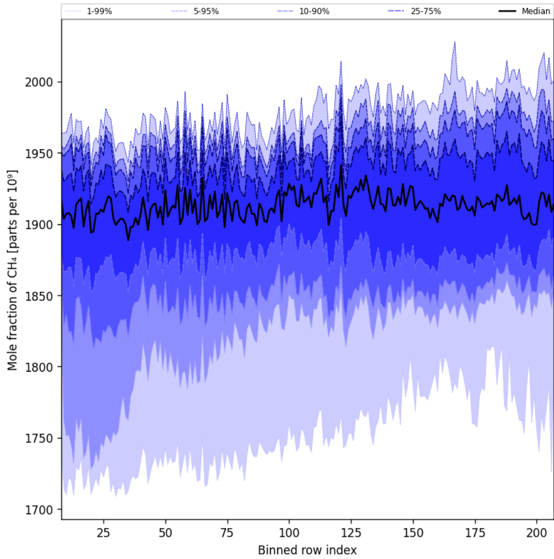
Figure 34: Along track statistics of “Mole fraction of CH 4 ” for 2025-09-26 to 2025-09-28
