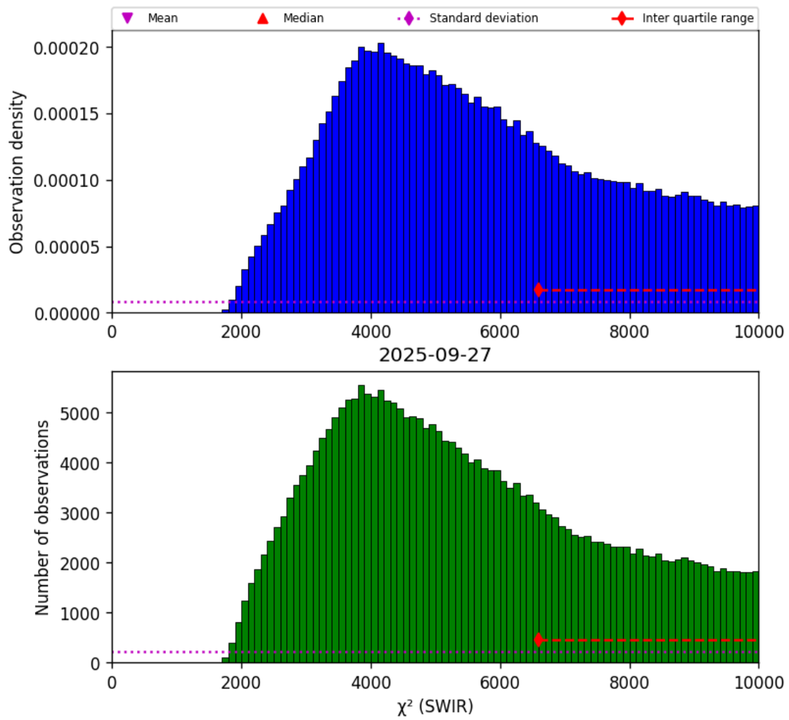
Figure 28: Histogram of " \chi^2 (SWIR)" for 2025-09-26 to 2025-09-28
