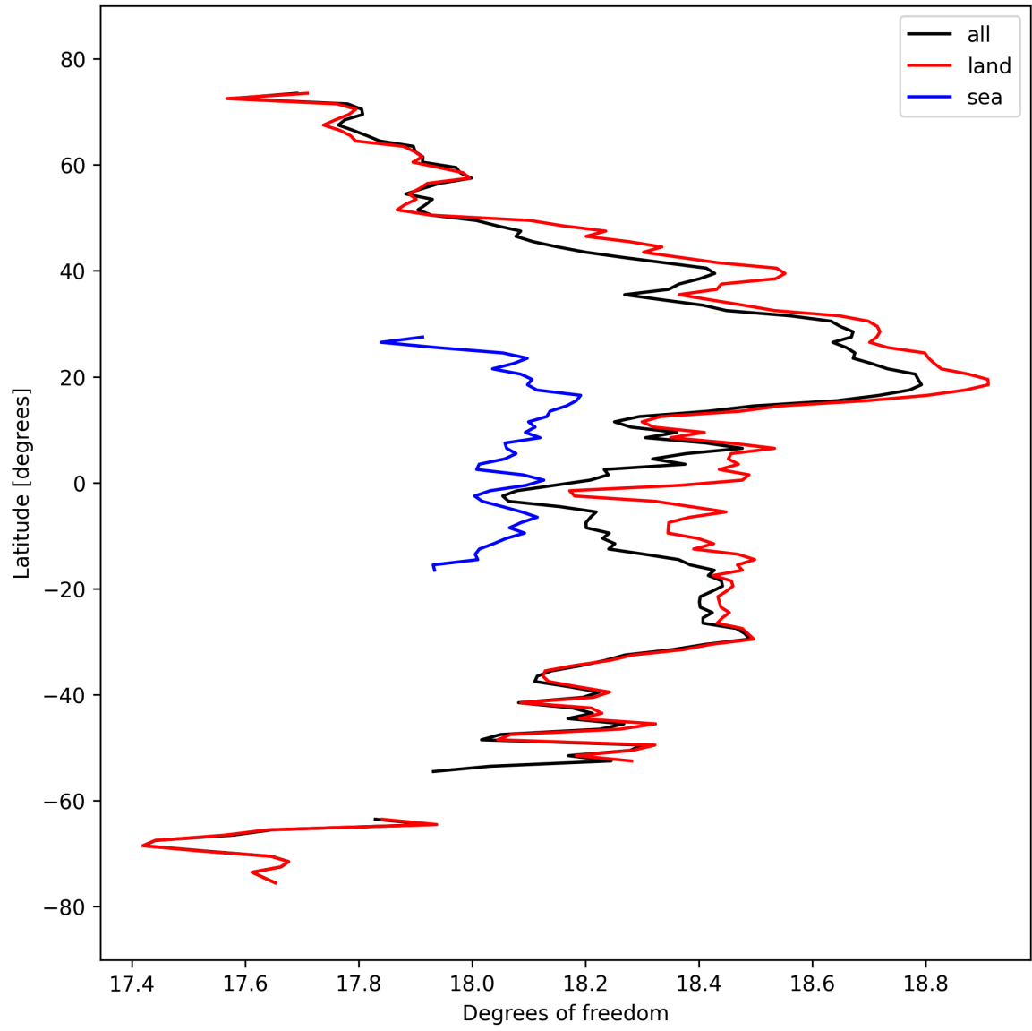
Figure 19: Zonal average of “Degrees of freedom” for 2025-09-26 to 2025-09-28.
