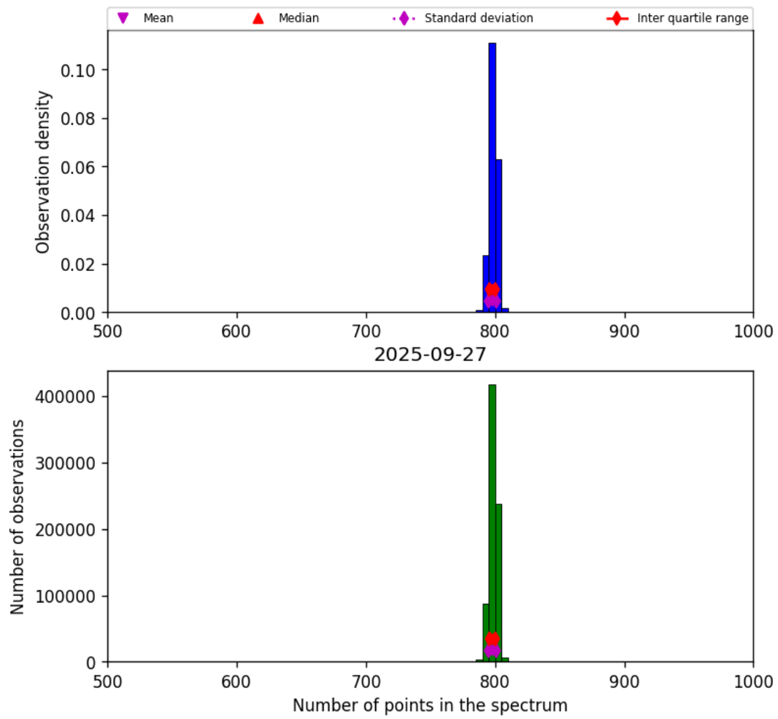
Figure 26: Histogram of “Number of points in the spectrum” for 2025-09-26 to 2025-09-28
