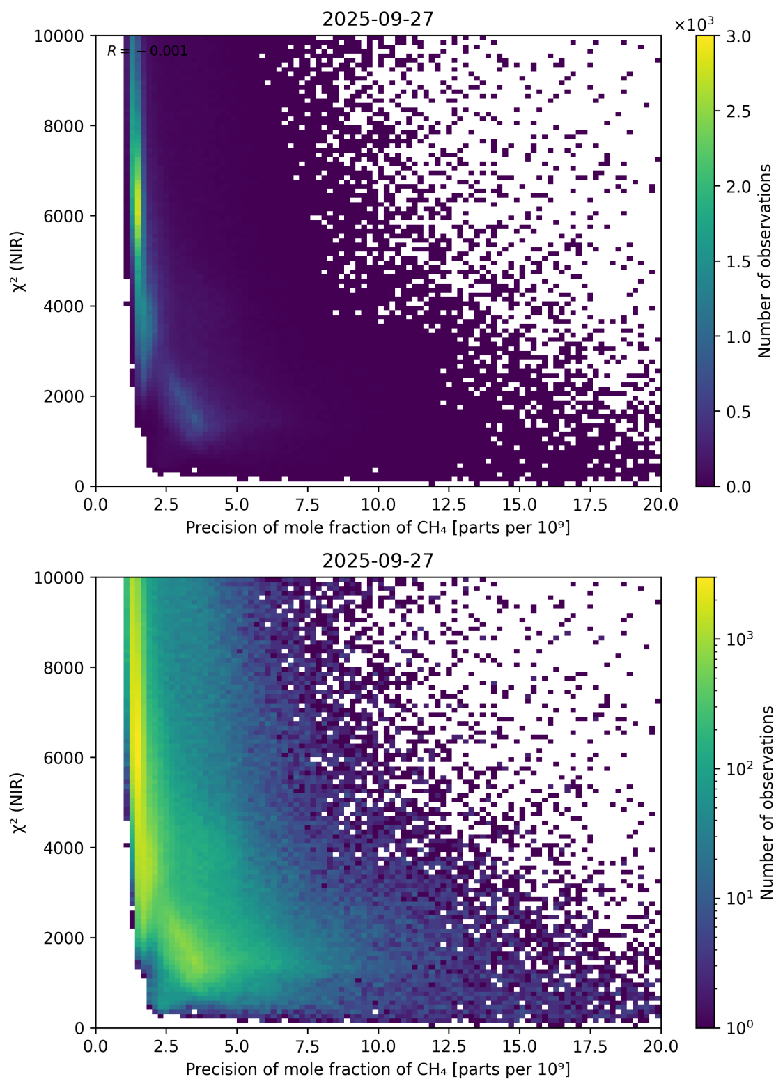
Figure 78: Scatter density plot of “Precision of mole fraction of \text{CH}_4 ” against “ \chi^2 (NIR)” for 2025-09-26 to 2025-09-28.
