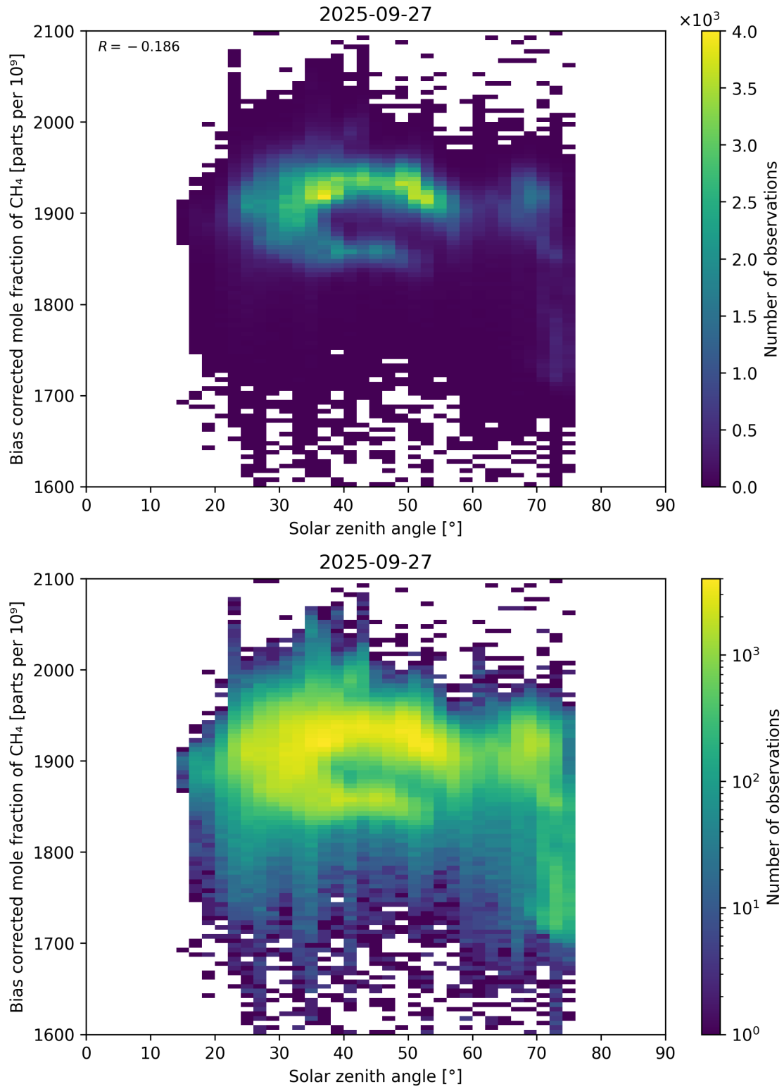
Figure 100: Scatter density plot of “Solar zenith angle” against “Bias corrected mole fraction of CH 4 ” for 2025-09-26 to 2025-09-28.
