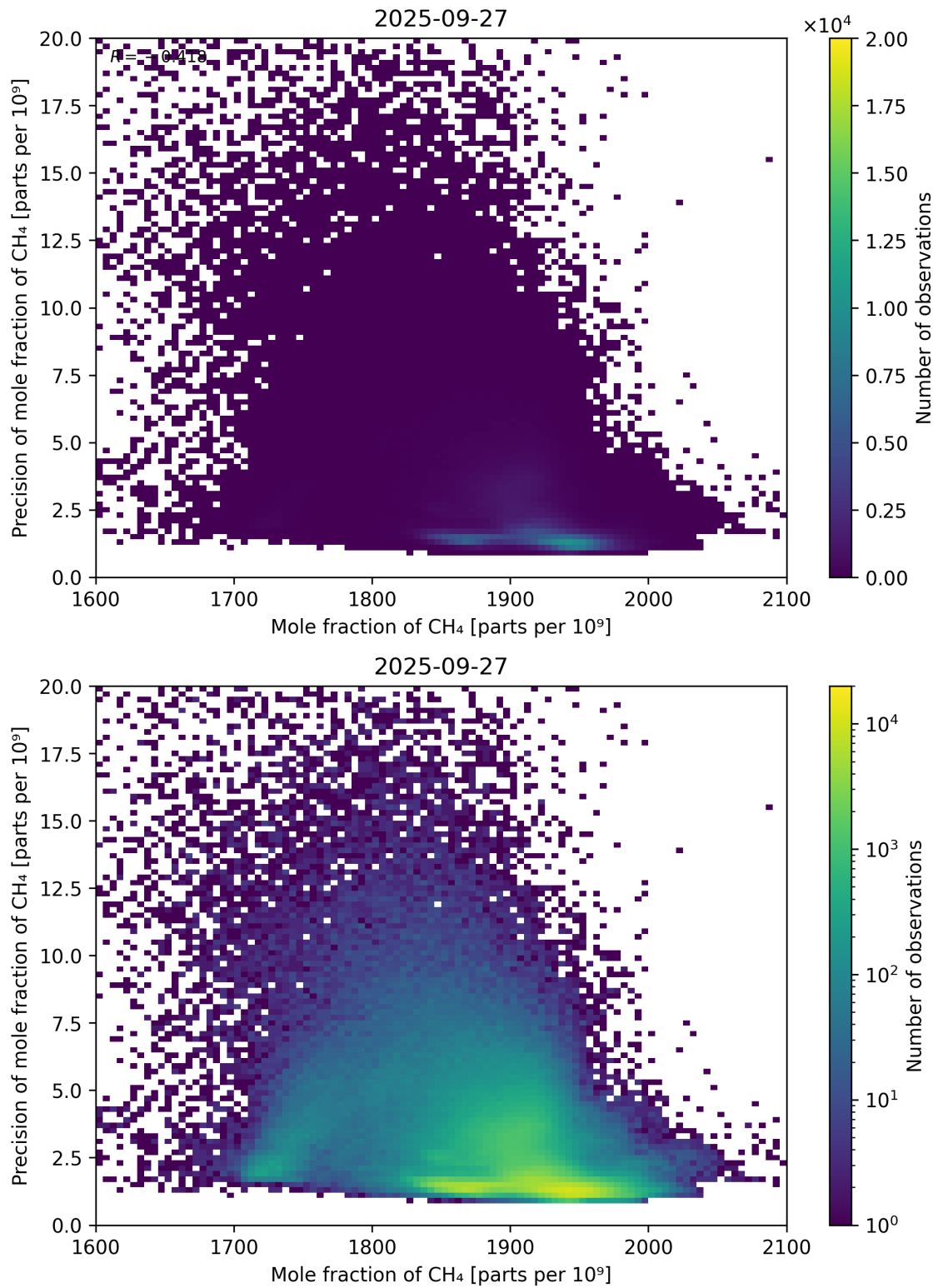
Figure 75: Scatter density plot of “Mole fraction of CH 4 ” against “Precision of mole fraction of CH 4 ” for 2025-09-26 to 2025-09-28.
