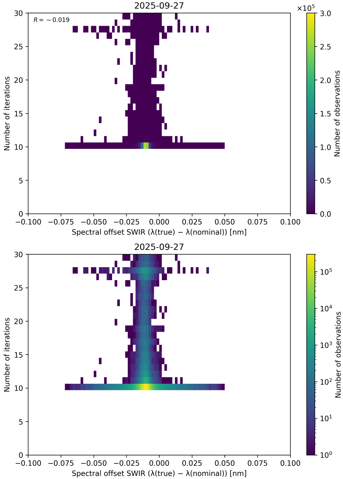
Figure 121: Scatter density plot of “Spectral offset SWIR ( \lambda_{\text{true}} - \lambda_{\text{nominal}} )” against “Number of iterations” for 2025-09-26 to 2025-09-28.
