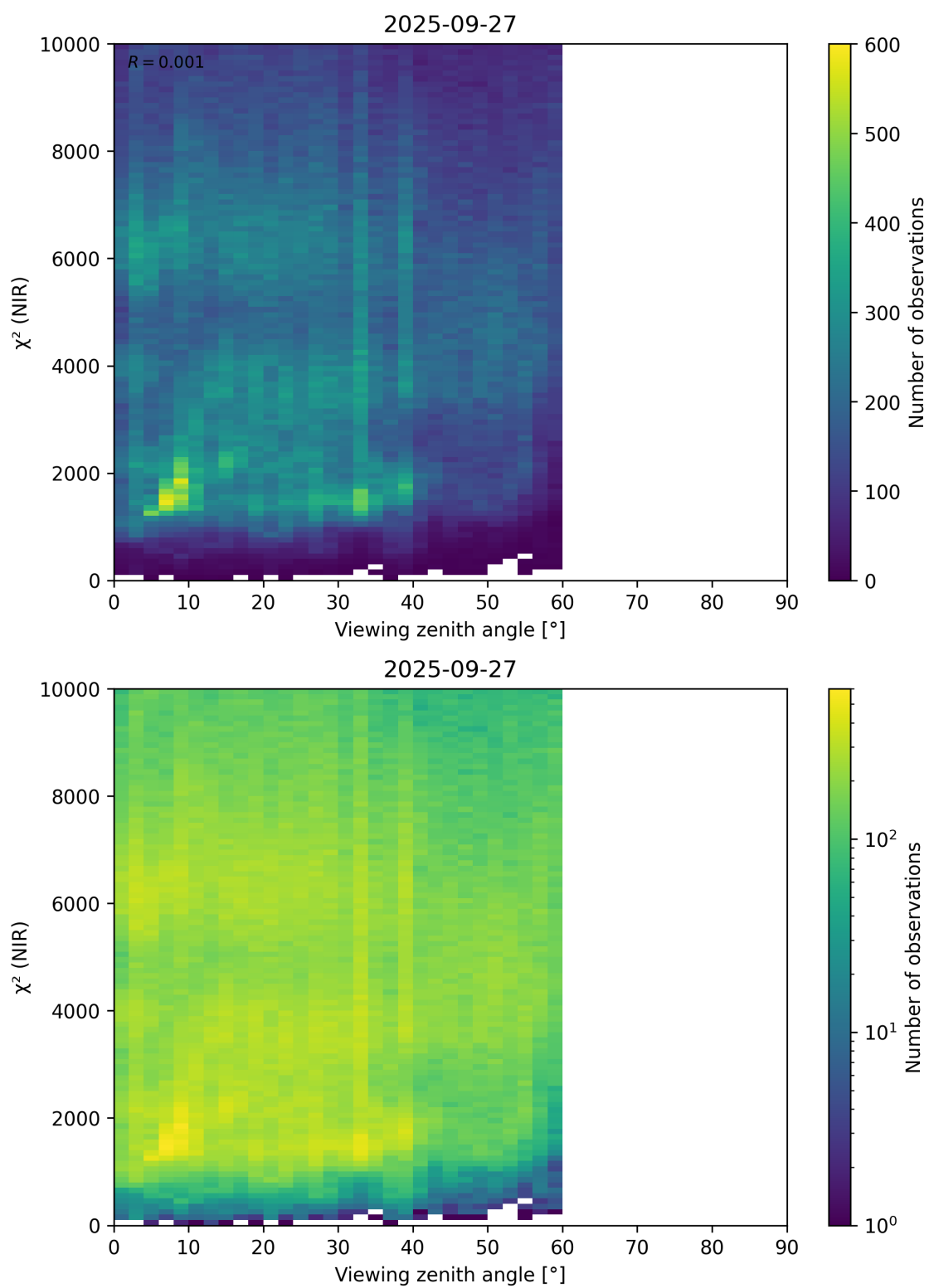
Figure 105: Scatter density plot of “Viewing zenith angle” against “ \chi^2 (NIR)” for 2025-09-26 to 2025-09-28.
