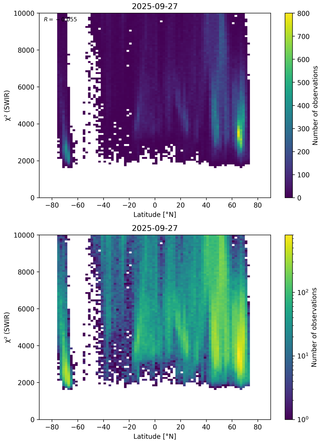
Figure 54: Scatter density plot of “Latitude” against “ \chi^2 (SWIR)” for 2025-09-26 to 2025-09-28.
