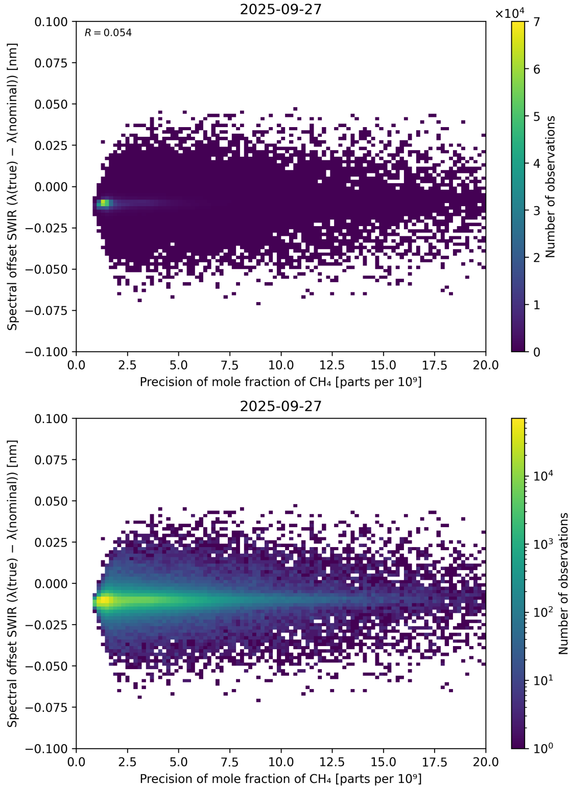
Figure 85: Scatter density plot of “Precision of mole fraction of CH 4 ” against “Spectral offset SWIR ( \lambda_{\text{true}} - \lambda_{\text{nominal}} )” for 2025-09-26 to 2025-09-28.
