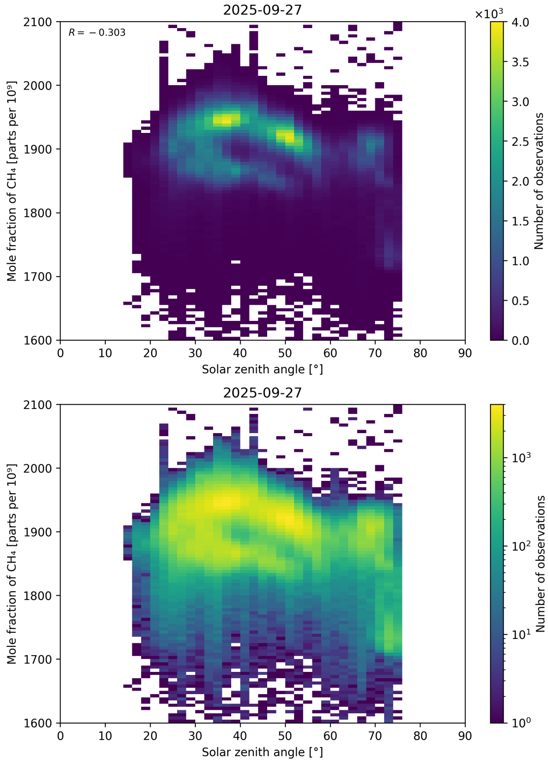
Figure 99: Scatter density plot of “Solar zenith angle” against “Mole fraction of CH 4 ” for 2025-09-26 to 2025-09-28.
