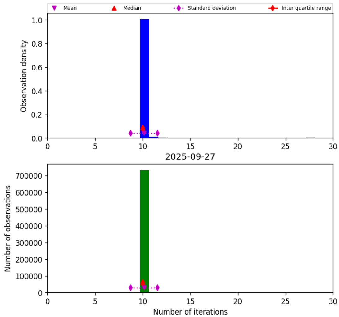
Figure 31: Histogram of “Number of iterations” for 2025-09-26 to 2025-09-28
