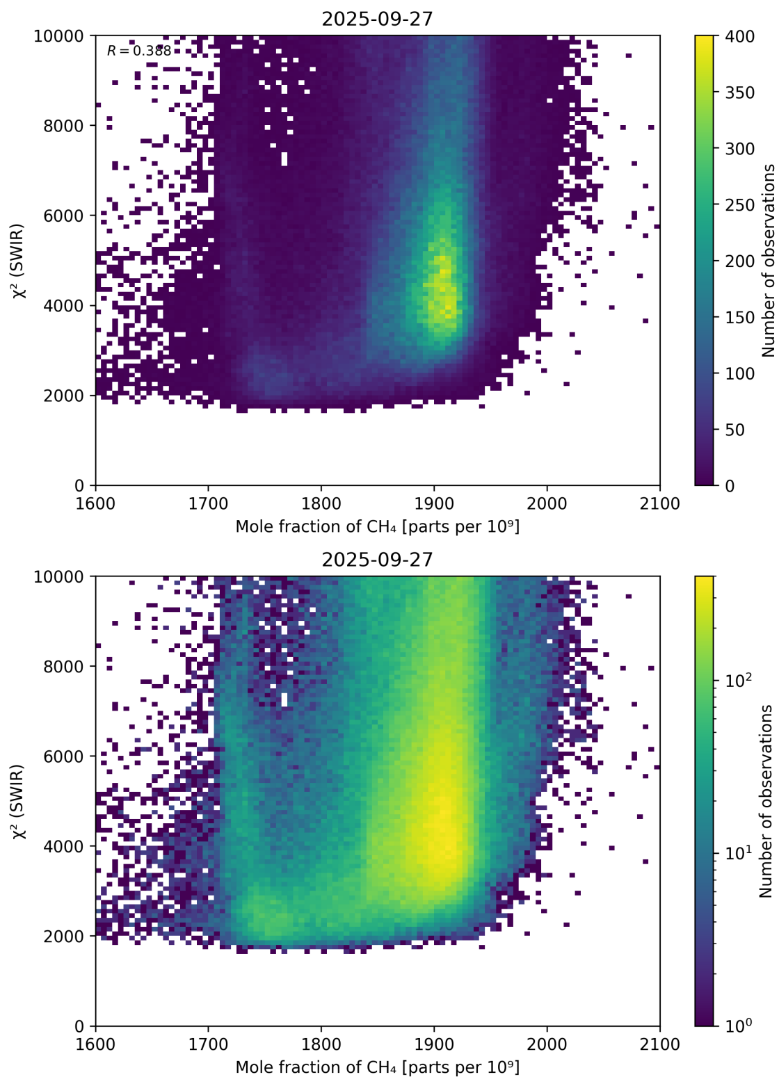
Figure 71: Scatter density plot of “Mole fraction of \text{CH}_4 ” against “ \chi^2 (SWIR)” for 2025-09-26 to 2025-09-28.
