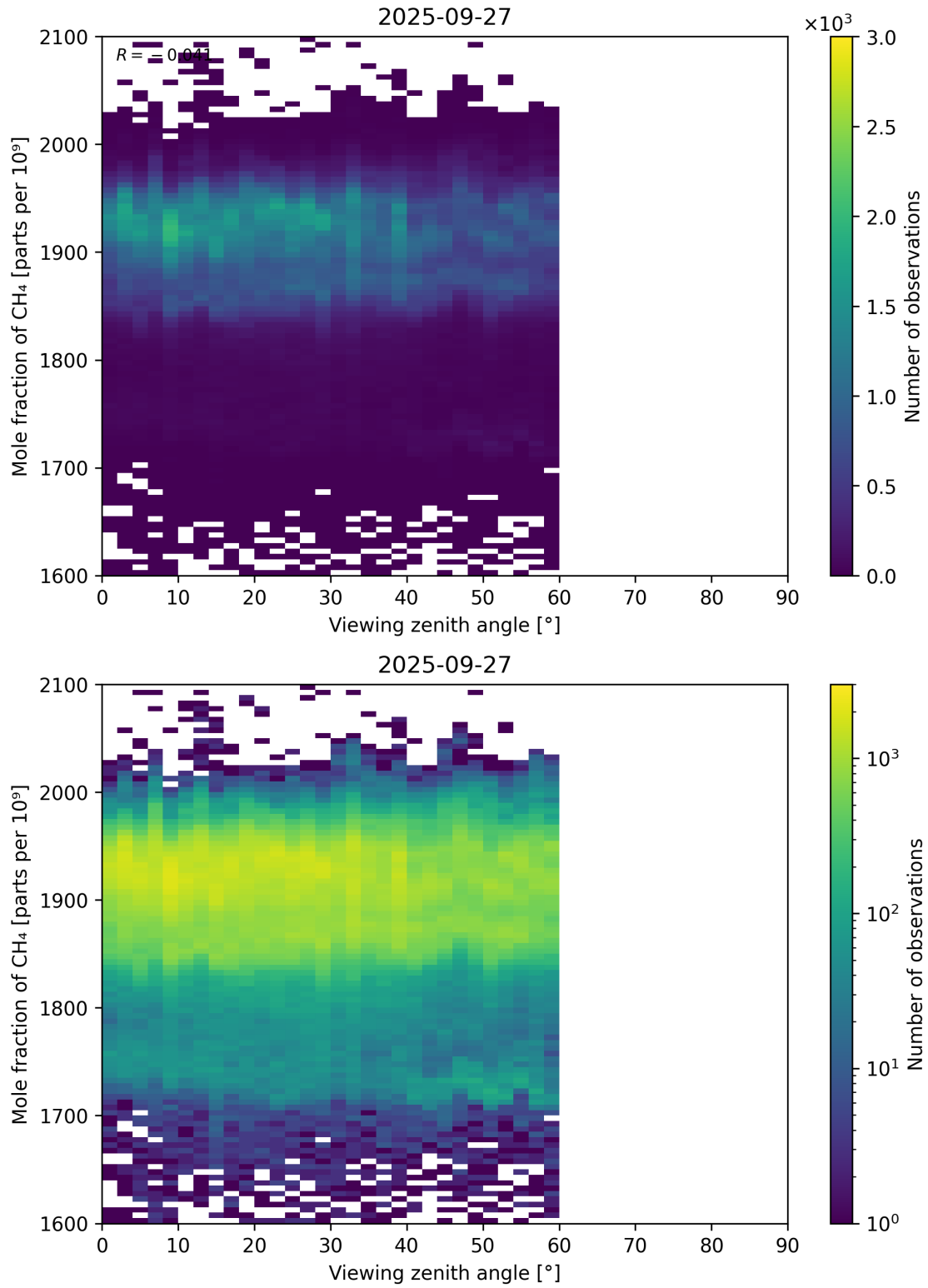
Figure 110: Scatter density plot of “Viewing zenith angle” against “Mole fraction of CH 4 ” for 2025-09-26 to 2025-09-28.
