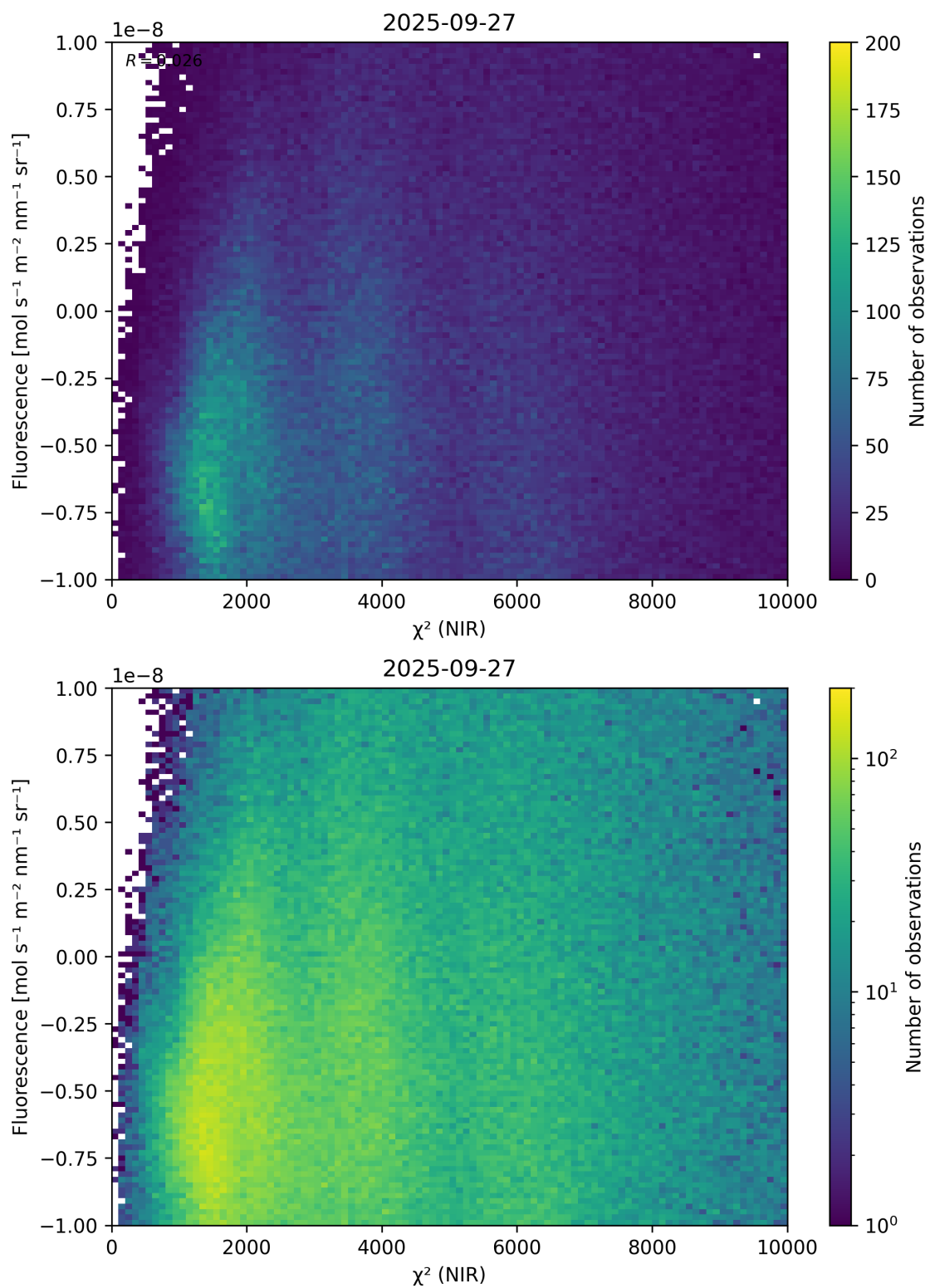
Figure 45: Scatter density plot of “ \chi^2 (NIR)” against “Fluorescence” for 2025-09-26 to 2025-09-28.
