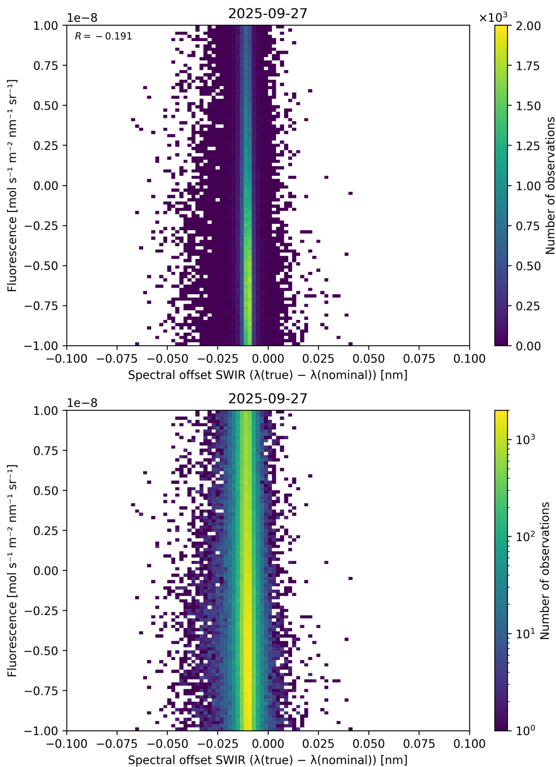
Figure 120: Scatter density plot of “Spectral offset SWIR ( \lambda_{\text{true}} - \lambda_{\text{nominal}} )” against “Fluorescence” for 2025-09-26 to 2025-09-28.
