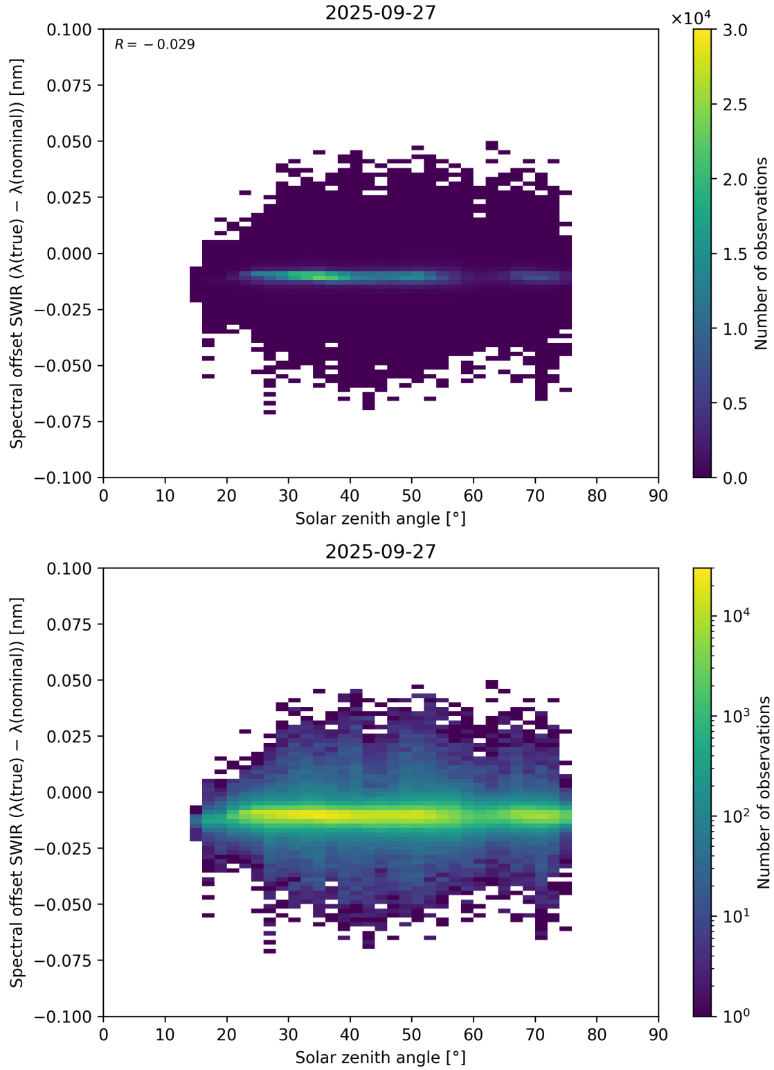
Figure 104: Scatter density plot of “Solar zenith angle” against “Spectral offset SWIR ( \lambda_{\text{true}} - \lambda_{\text{nominal}} )” for 2025-09-26 to 2025-09-28.
