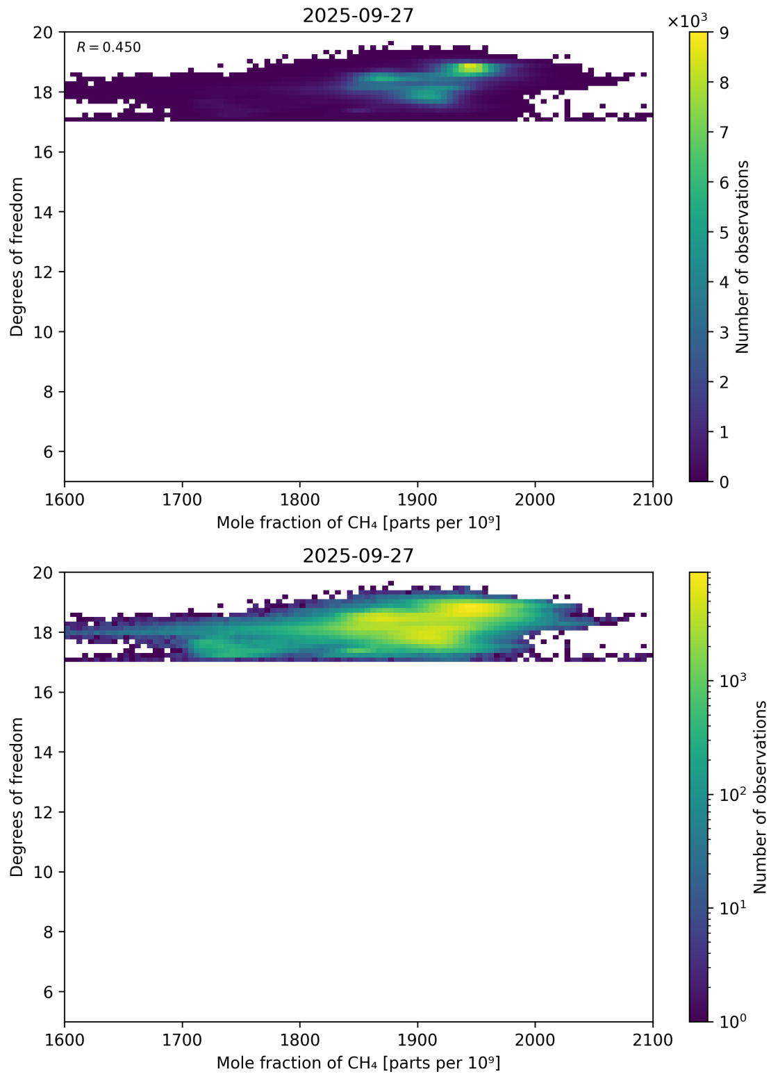
Figure 72: Scatter density plot of “Mole fraction of CH 4 ” against “Degrees of freedom” for 2025-09-26 to 2025-09-28.
