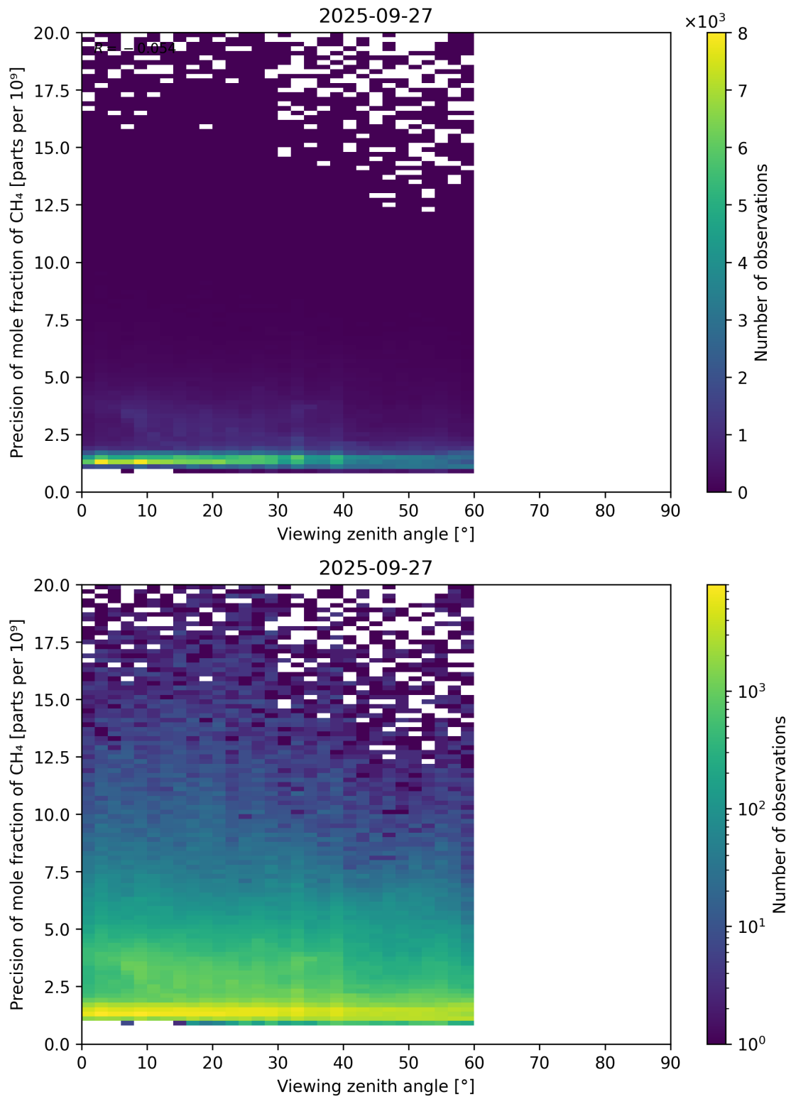
Figure 112: Scatter density plot of “Viewing zenith angle” against “Precision of mole fraction of CH 4 ” for 2025-09-26 to 2025-09-28.
