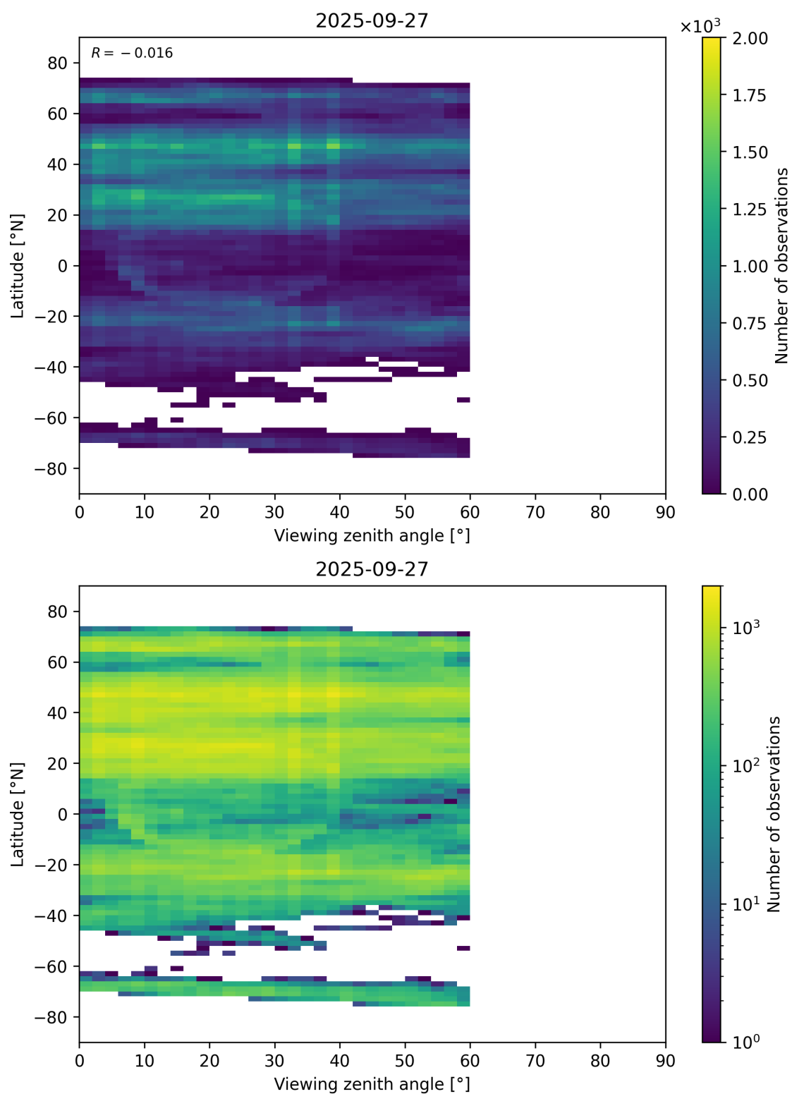
Figure 109: Scatter density plot of “Viewing zenith angle” against “Latitude” for 2025-09-26 to 2025-09-28.
