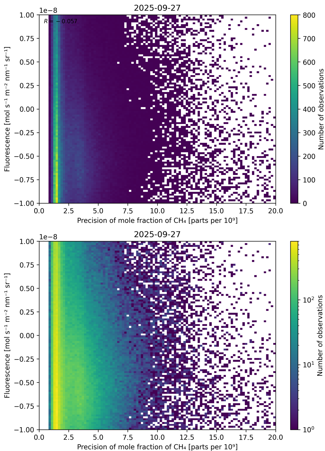
Figure 81: Scatter density plot of “Precision of mole fraction of CH 4 ” against “Fluorescence” for 2025-09-26 to 2025-09-28.
