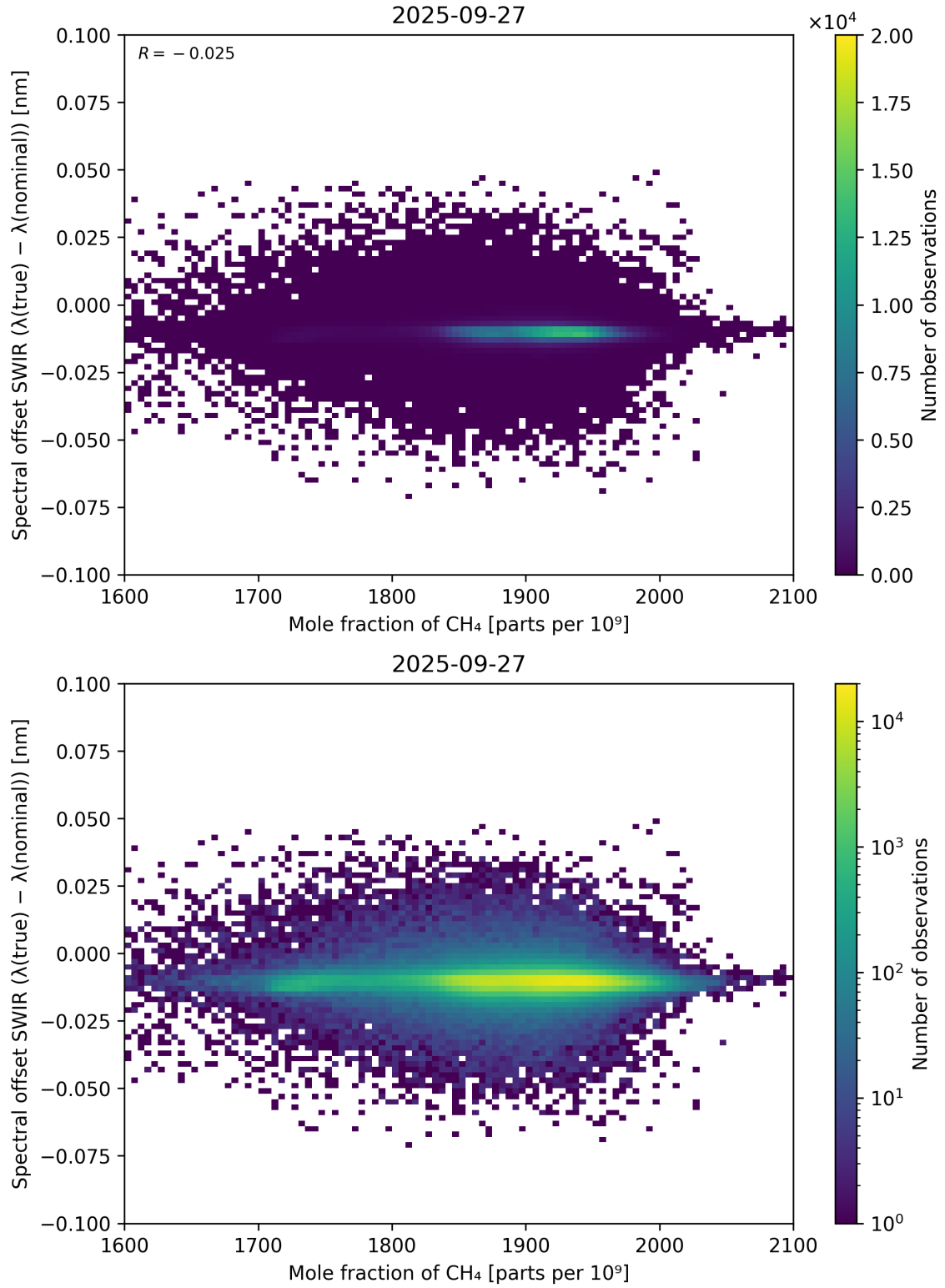
Figure 86: Scatter density plot of “Mole fraction of \text{CH}_4 ” against “Spectral offset SWIR ( \lambda_{\text{true}} - \lambda_{\text{nominal}} )” for 2025-09-26 to 2025-09-28.
