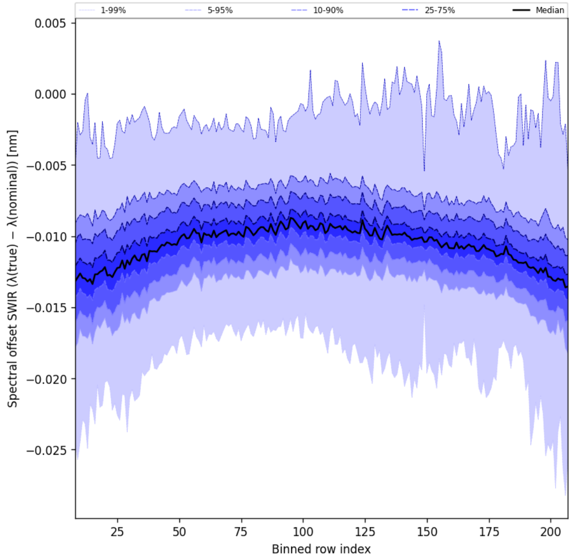
Figure 38: Along track statistics of “Spectral offset SWIR ( \lambda_{\text{true}} - \lambda_{\text{nominal}} )” for 2025-09-26 to 2025-09-28
