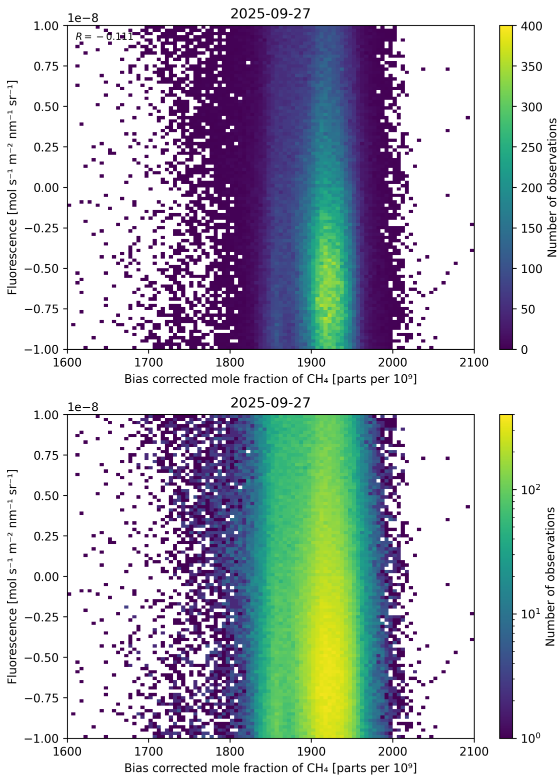
Figure 66: Scatter density plot of “Bias corrected mole fraction of \text{CH}_4 ” against “Fluorescence” for 2025-09-26 to 2025-09-28.
