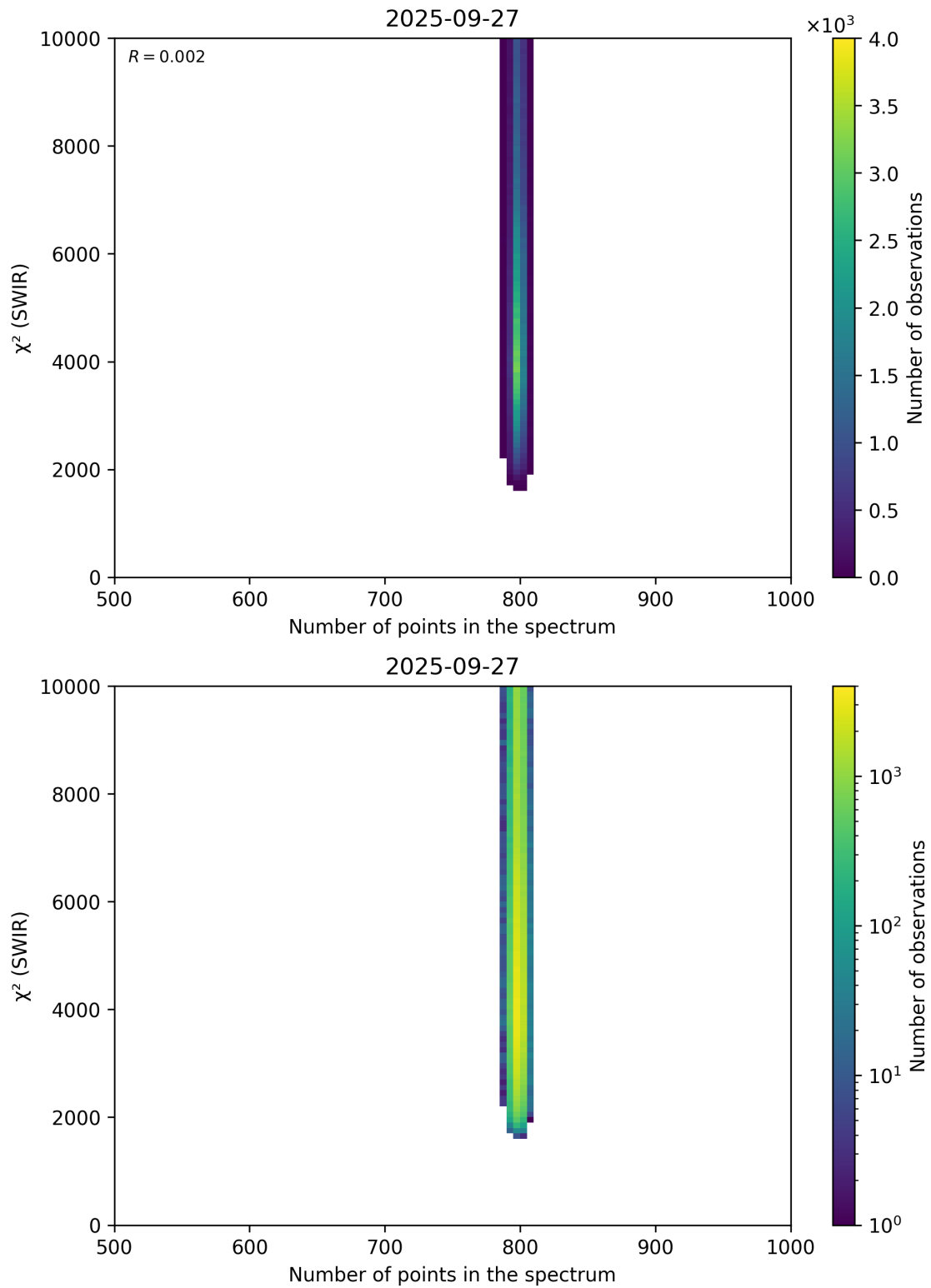
Figure 89: Scatter density plot of “Number of points in the spectrum” against “ \chi^2 (SWIR)” for 2025-09-26 to 2025-09-28.
