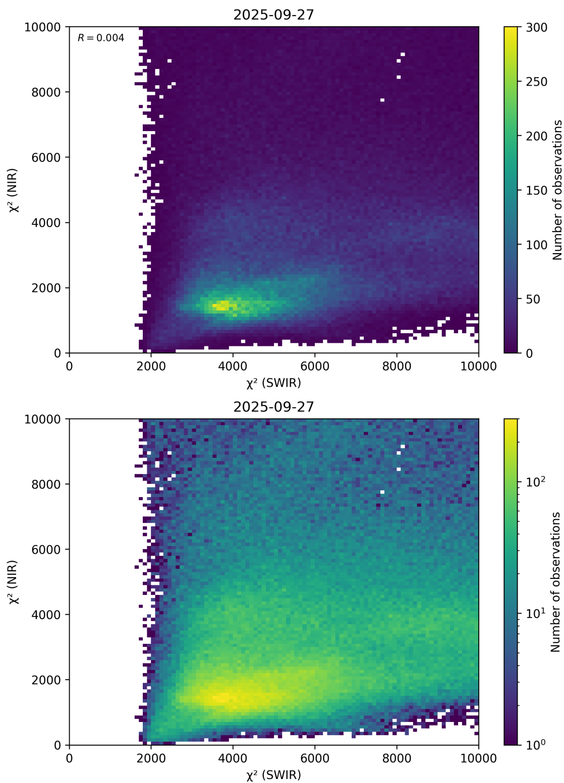
Figure 47: Scatter density plot of “ \chi^2 (SWIR)” against “ \chi^2 (NIR)” for 2025-09-26 to 2025-09-28.
