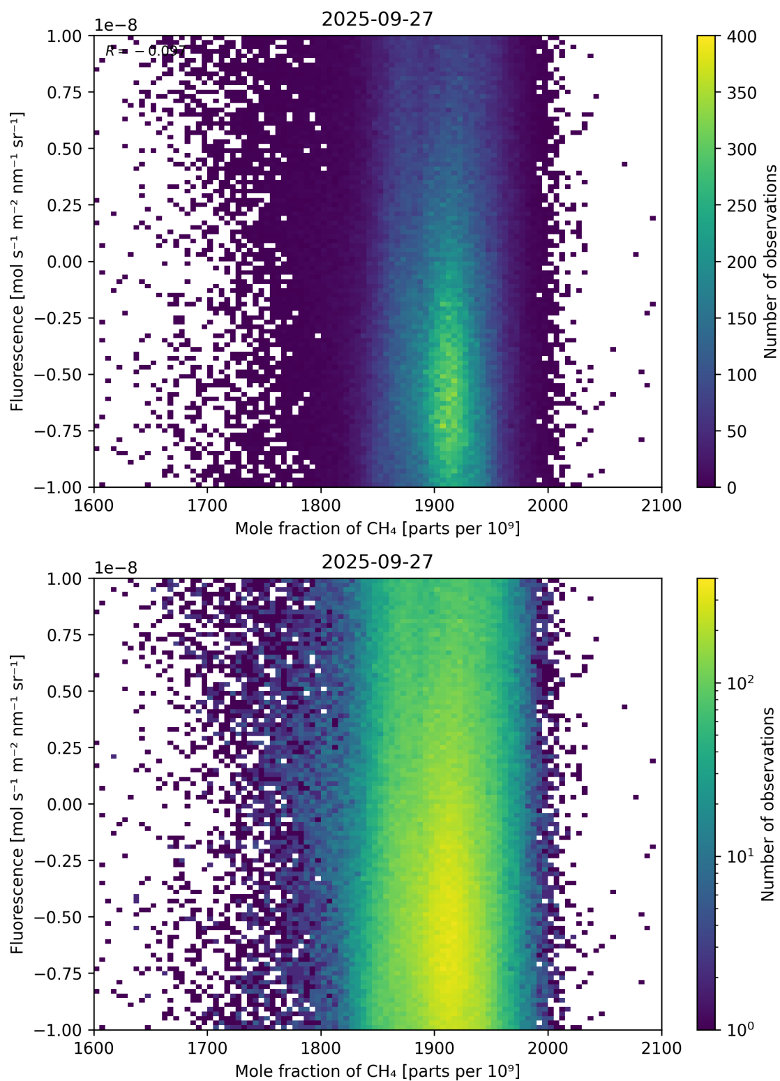
Figure 73: Scatter density plot of “Mole fraction of \text{CH}_4 ” against “Fluorescence” for 2025-09-26 to 2025-09-28.
