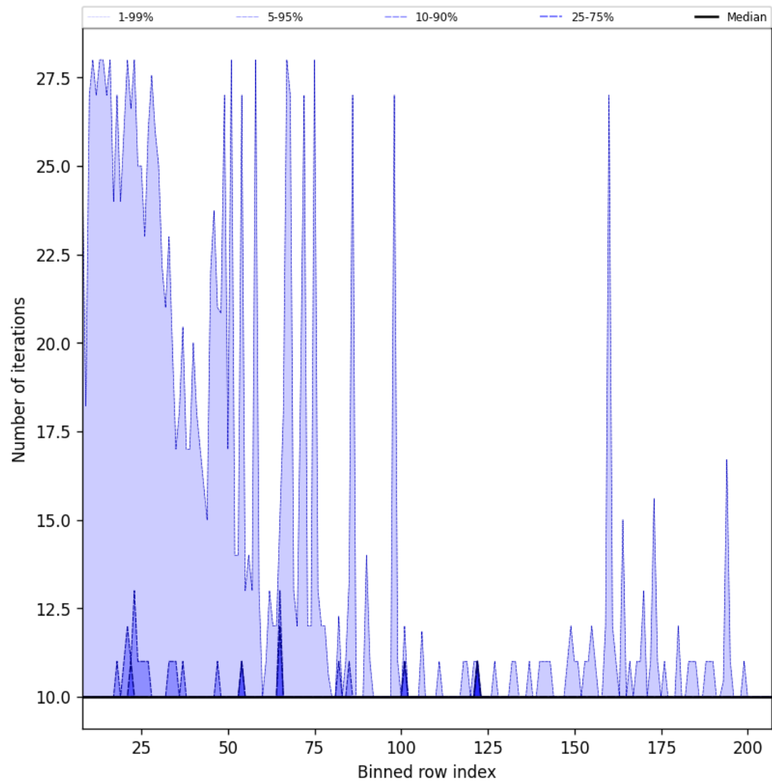
Figure 42: Along track statistics of “Number of iterations” for 2025-09-26 to 2025-09-28
