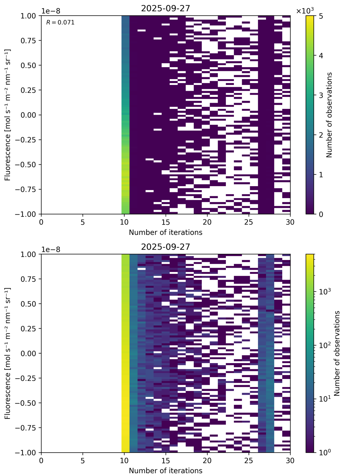
Figure 87: Scatter density plot of “Number of iterations” against “Fluorescence” for 2025-09-26 to 2025-09-28.
