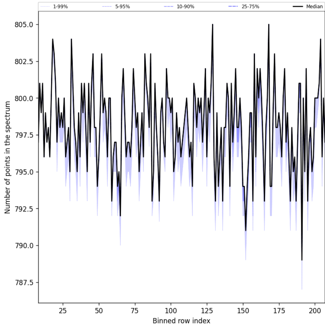
Figure 37: Along track statistics of “Number of points in the spectrum” for 2025-09-26 to 2025-09-28
