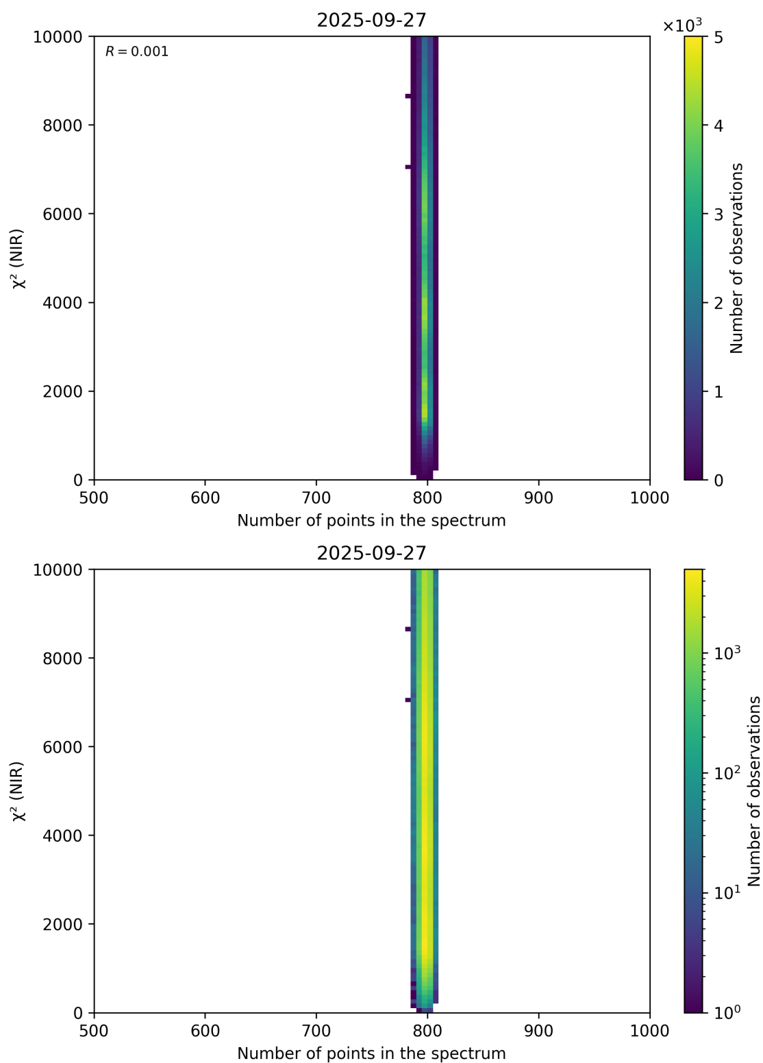
Figure 88: Scatter density plot of “Number of points in the spectrum” against “ \chi^2 (NIR)” for 2025-09-26 to 2025-09-28.
