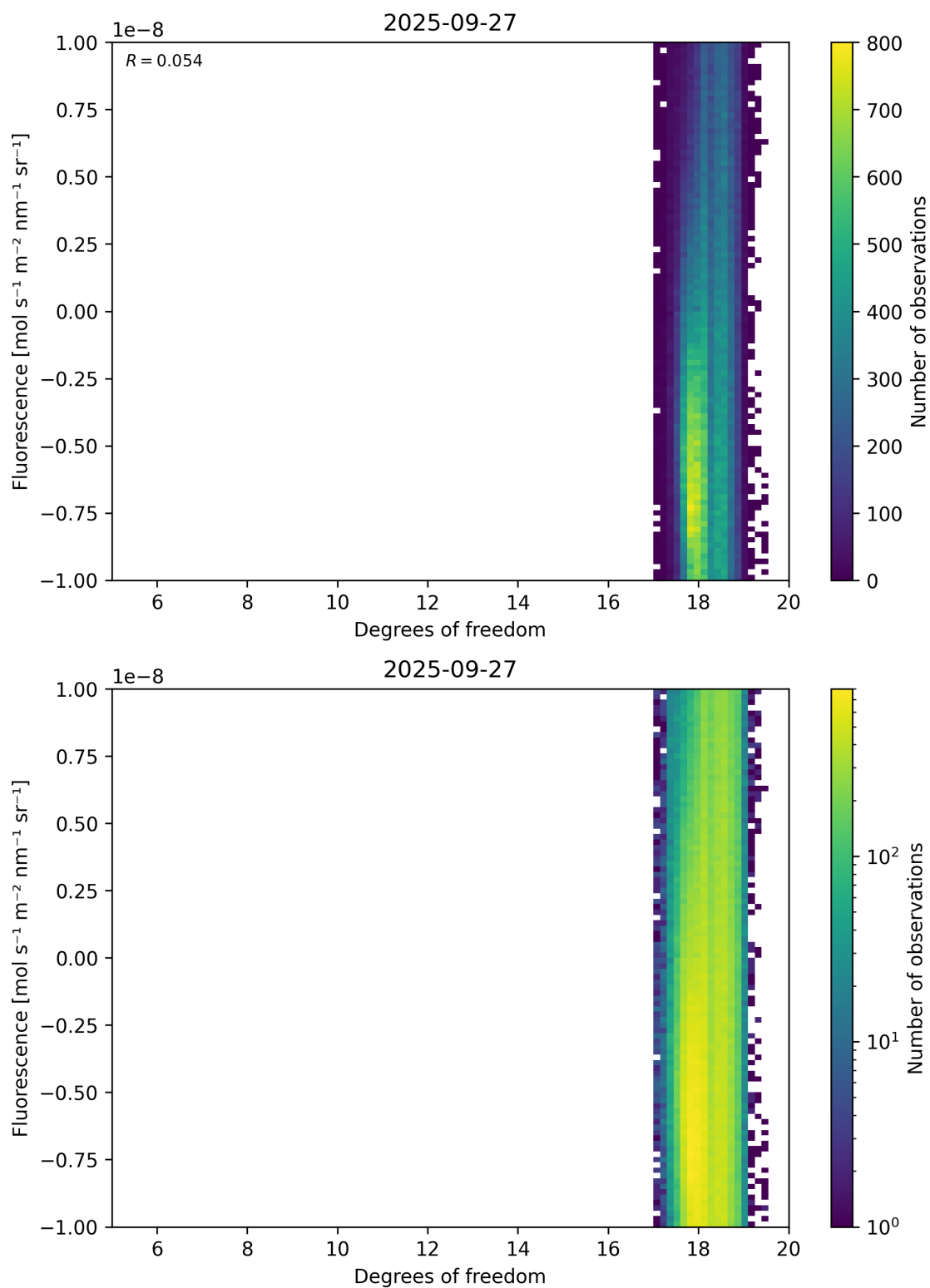
Figure 51: Scatter density plot of “Degrees of freedom” against “Fluorescence” for 2025-09-26 to 2025-09-28.
