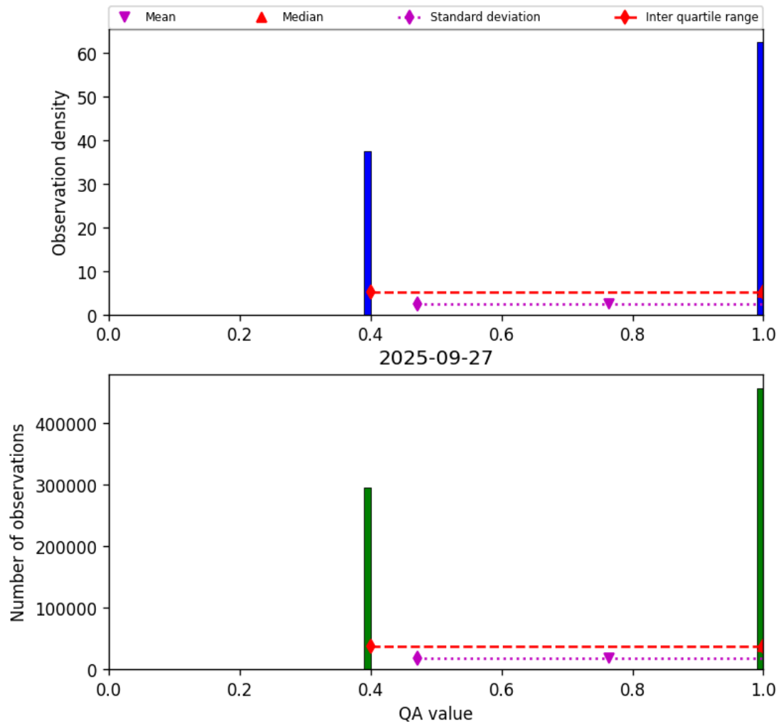
Figure 22: Histogram of “QA value” for 2025-09-26 to 2025-09-28
