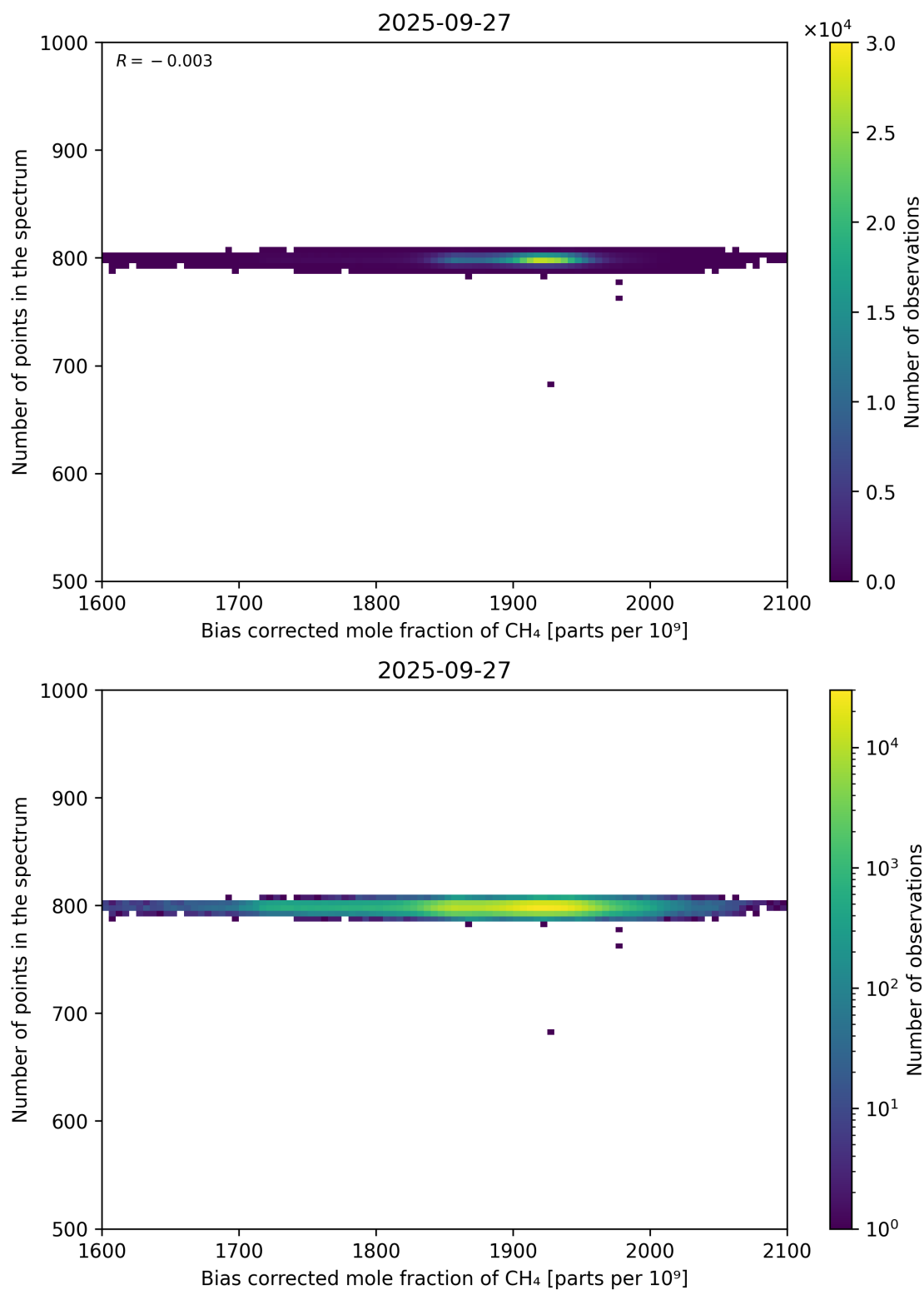
Figure 68: Scatter density plot of “Bias corrected mole fraction of CH 4 ” against “Number of points in the spectrum” for 2025-09-26 to 2025-09-28.
