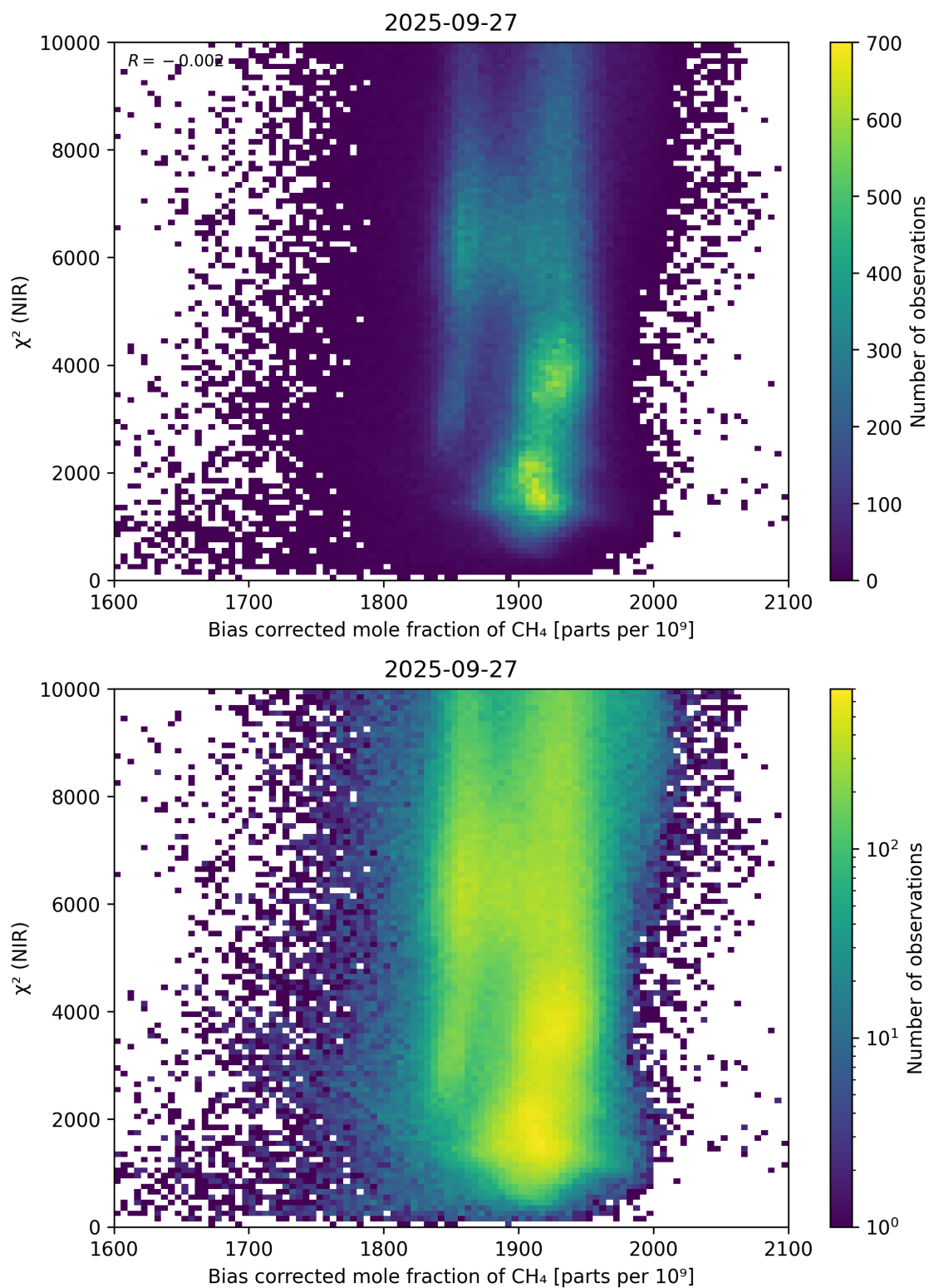
Figure 63: Scatter density plot of “Bias corrected mole fraction of CH 4 ” against “ \chi^2 (NIR)” for 2025-09-26 to 2025-09-28.
