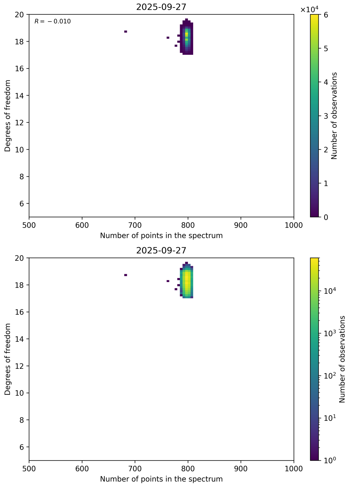
Figure 90: Scatter density plot of “Number of points in the spectrum” against “Degrees of freedom” for 2025-09-26 to 2025-09-28.
