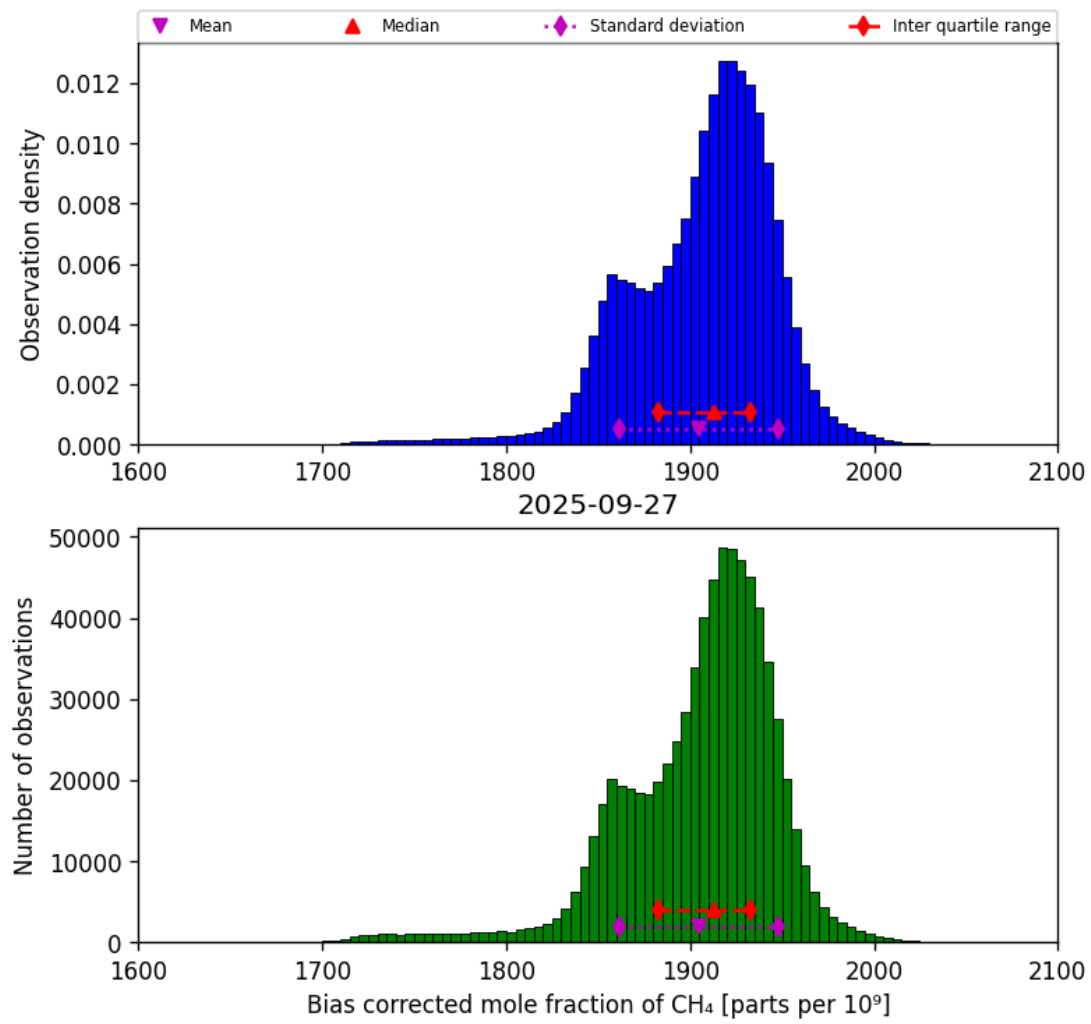
Figure 25: Histogram of “Bias corrected mole fraction of CH 4 ” for 2025-09-26 to 2025-09-28
