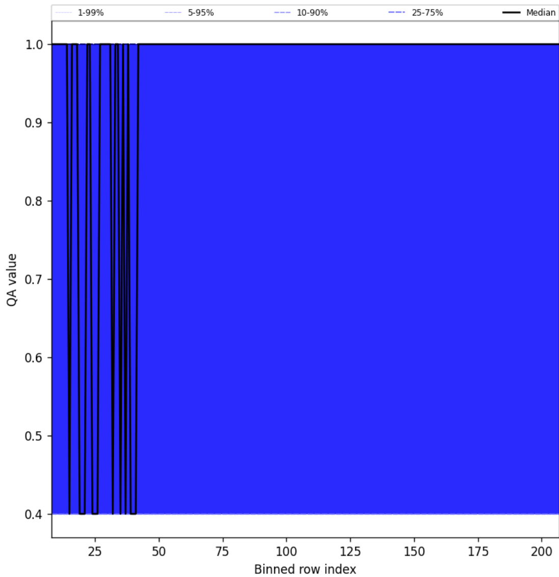
Figure 33: Along track statistics of “QA value” for 2025-09-26 to 2025-09-28
