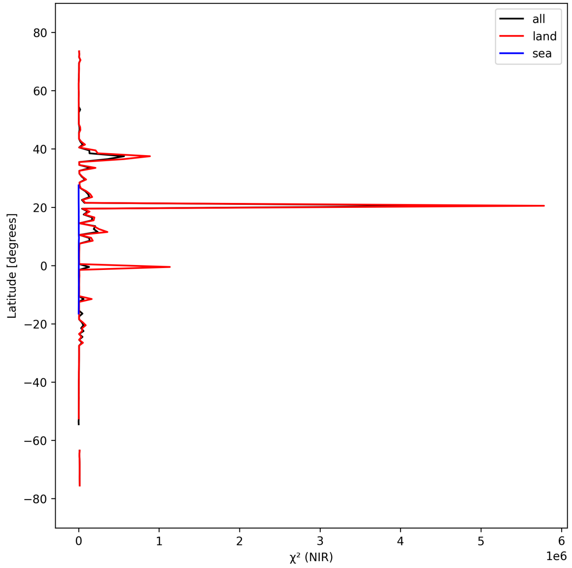
Figure 18: Zonal average of “ \chi^2 (NIR)” for 2025-09-26 to 2025-09-28.
