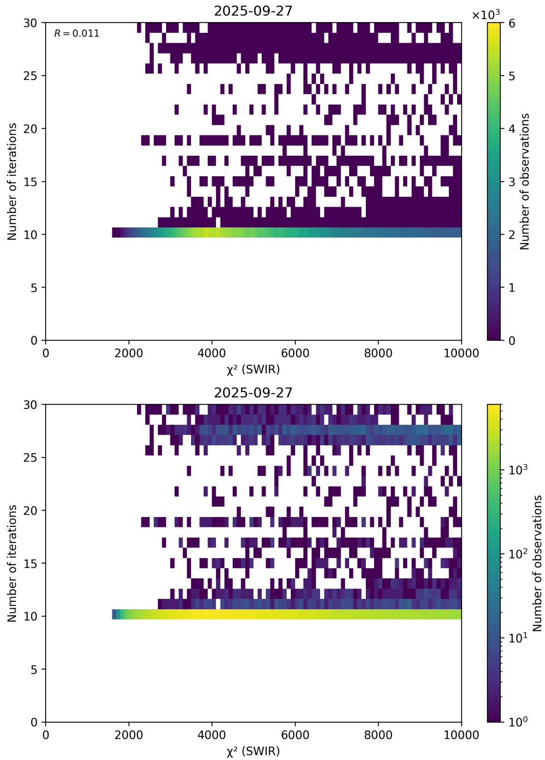
Figure 50: Scatter density plot of “ \chi^2 (SWIR)” against “Number of iterations” for 2025-09-26 to 2025-09-28.
