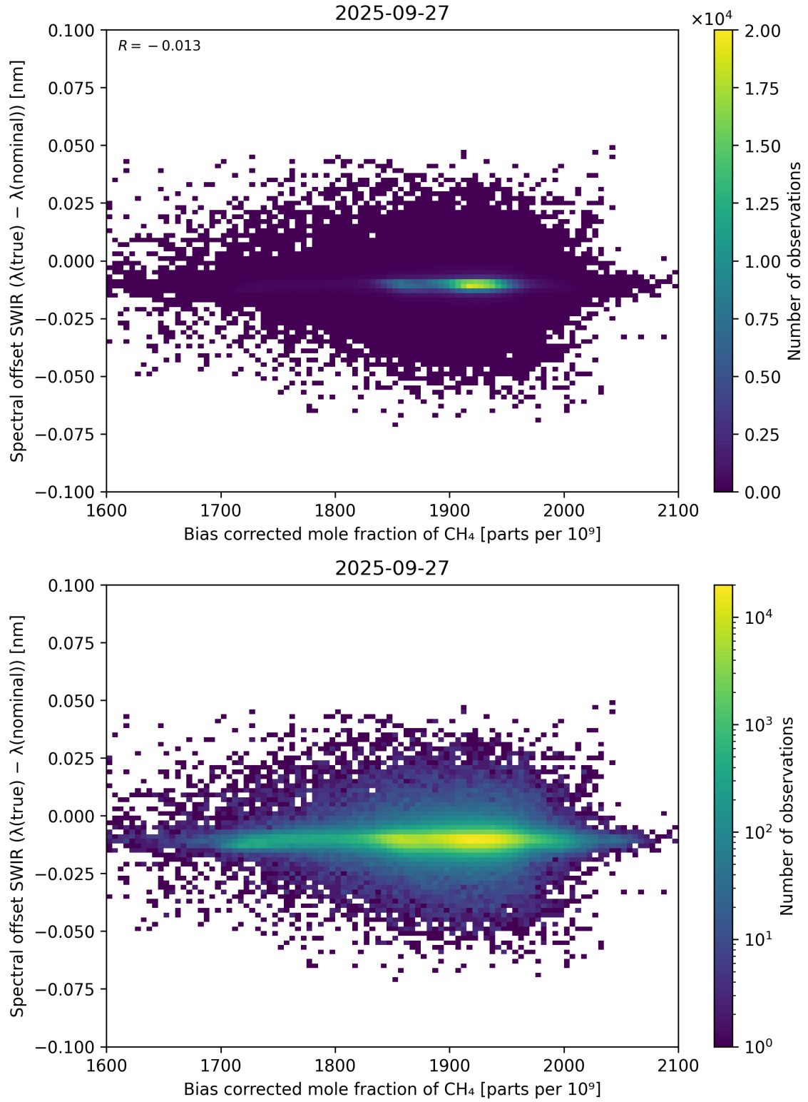
Figure 69: Scatter density plot of “Bias corrected mole fraction of CH 4 ” against “Spectral offset SWIR ( \lambda_{\text{true}} - \lambda_{\text{nominal}} )” for 2025-09-26 to 2025-09-28.
