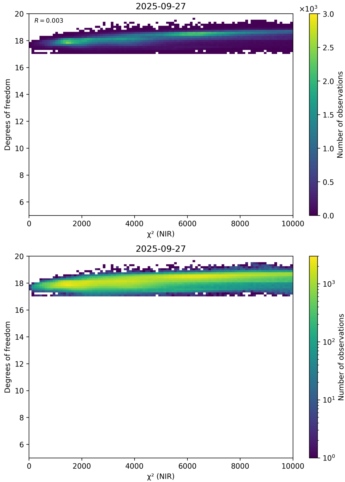
Figure 44: Scatter density plot of “ \chi^2 (NIR)” against “Degrees of freedom” for 2025-09-26 to 2025-09-28.
