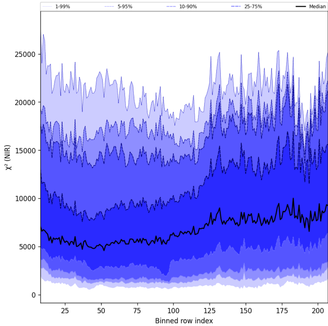
Figure 40: Along track statistics of “ \chi^2 (NIR)” for 2025-09-26 to 2025-09-28
