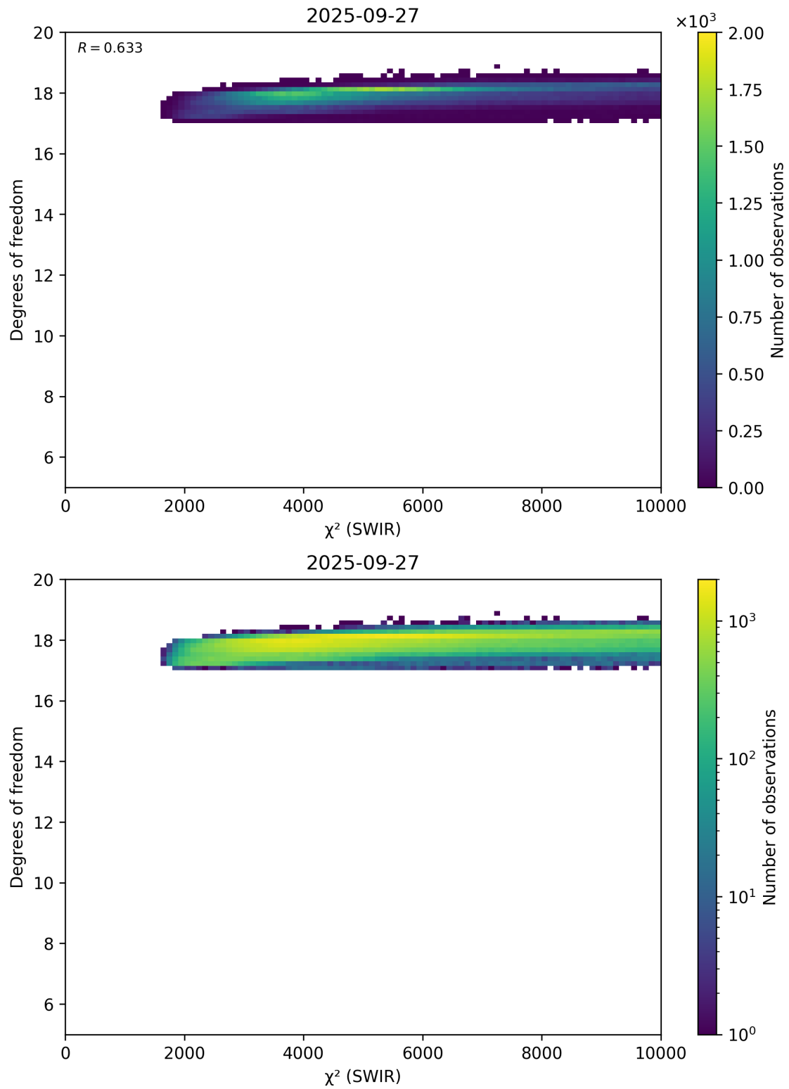
Figure 48: Scatter density plot of “ \chi^2 (SWIR)” against “Degrees of freedom” for 2025-09-26 to 2025-09-28.
