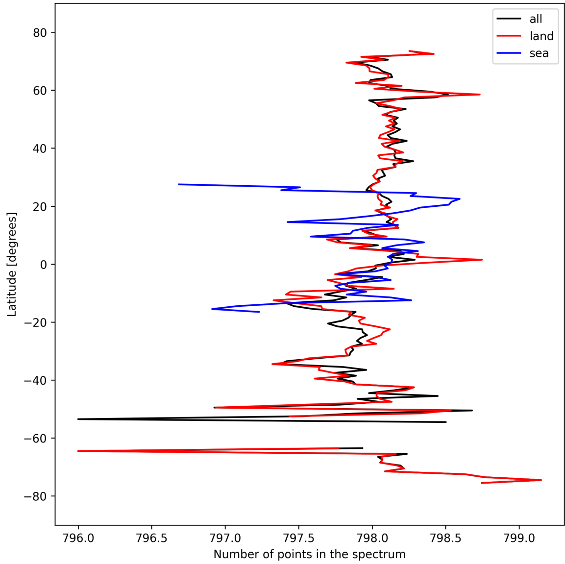
Figure 15: Zonal average of “Number of points in the spectrum” for 2025-09-26 to 2025-09-28.
