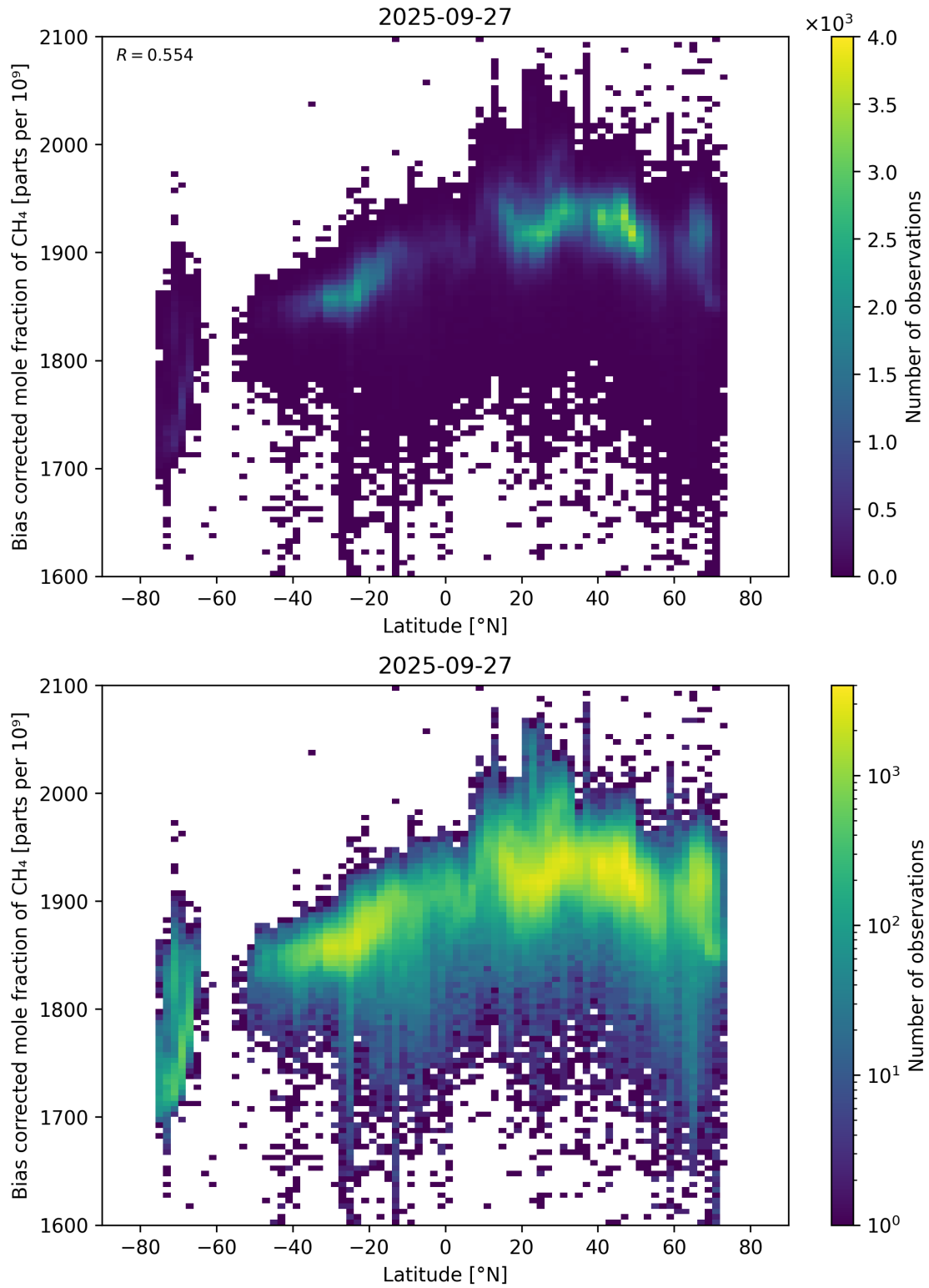
Figure 58: Scatter density plot of “Latitude” against “Bias corrected mole fraction of CH 4 ” for 2025-09-26 to 2025-09-28.
