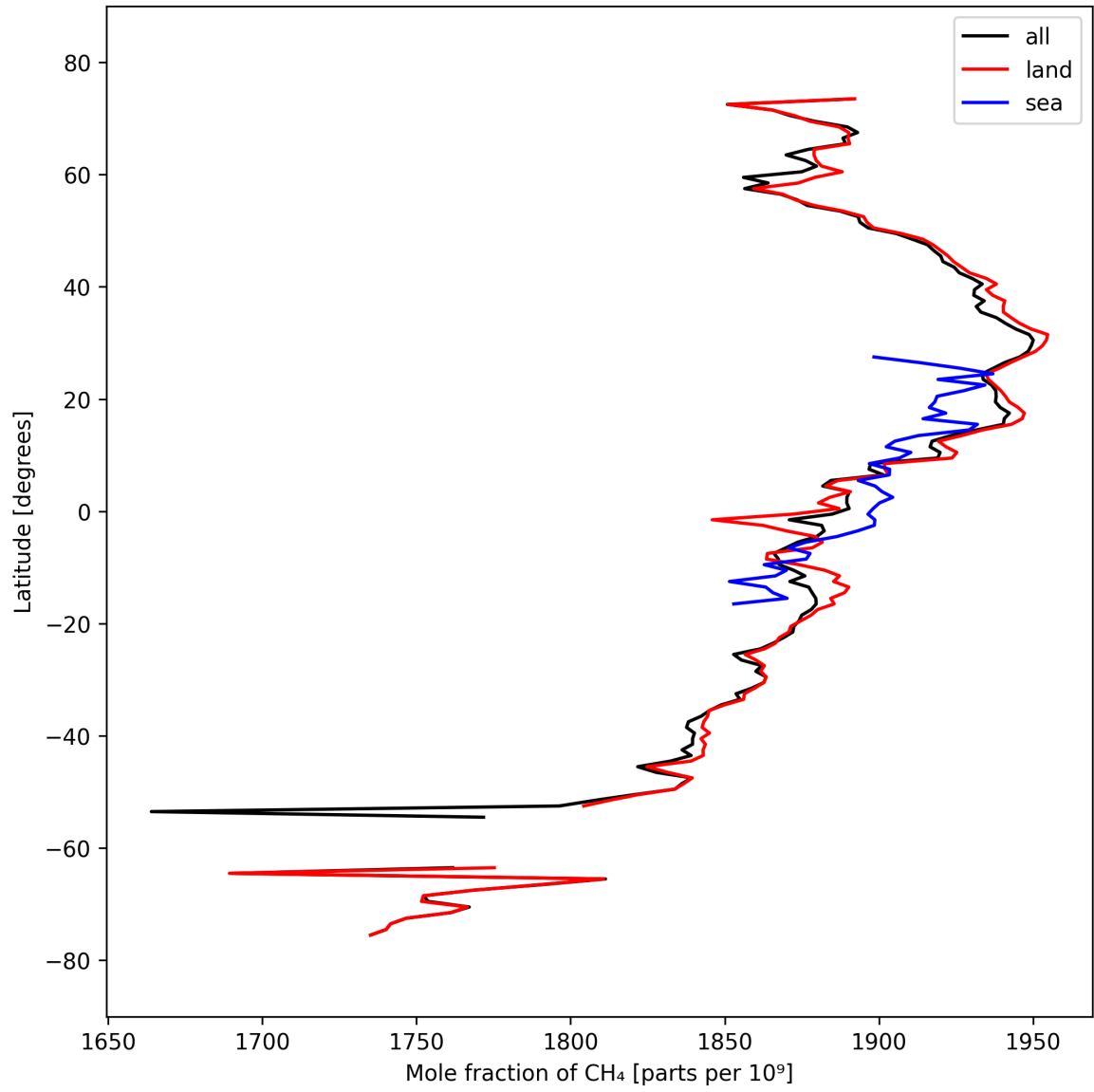
Figure 12: Zonal average of “Mole fraction of CH 4 ” for 2025-09-26 to 2025-09-28.
