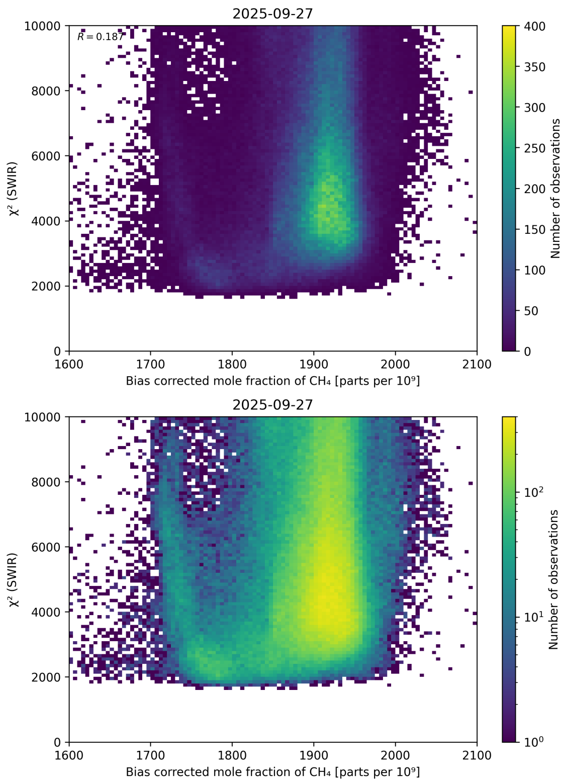
Figure 64: Scatter density plot of “Bias corrected mole fraction of CH 4 ” against “ \chi^2 (SWIR)” for 2025-09-26 to 2025-09-28.
