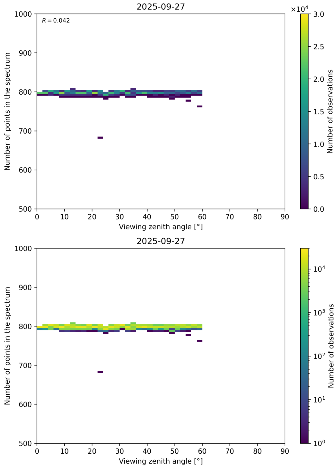
Figure 114: Scatter density plot of “Viewing zenith angle” against “Number of points in the spectrum” for 2025-09-26 to 2025-09-28.
