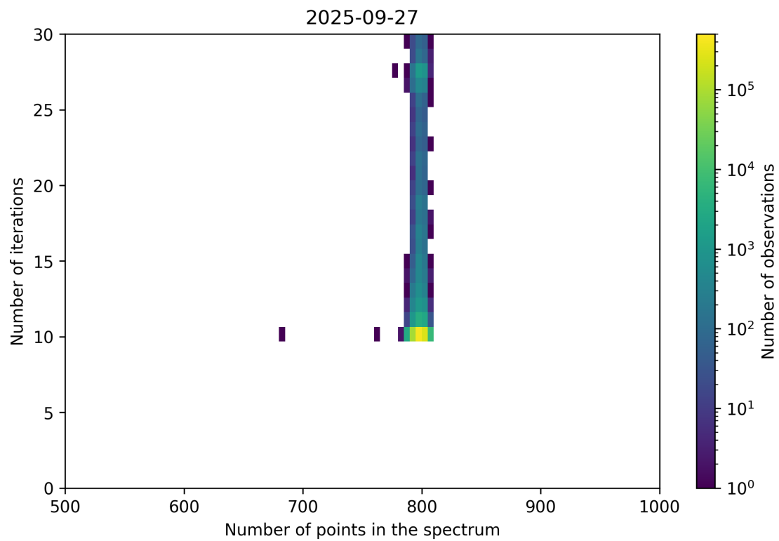
Figure 92: Scatter density plot of “Number of points in the spectrum” against “Number of iterations” for 2025-09-26 to 2025-09-28.
