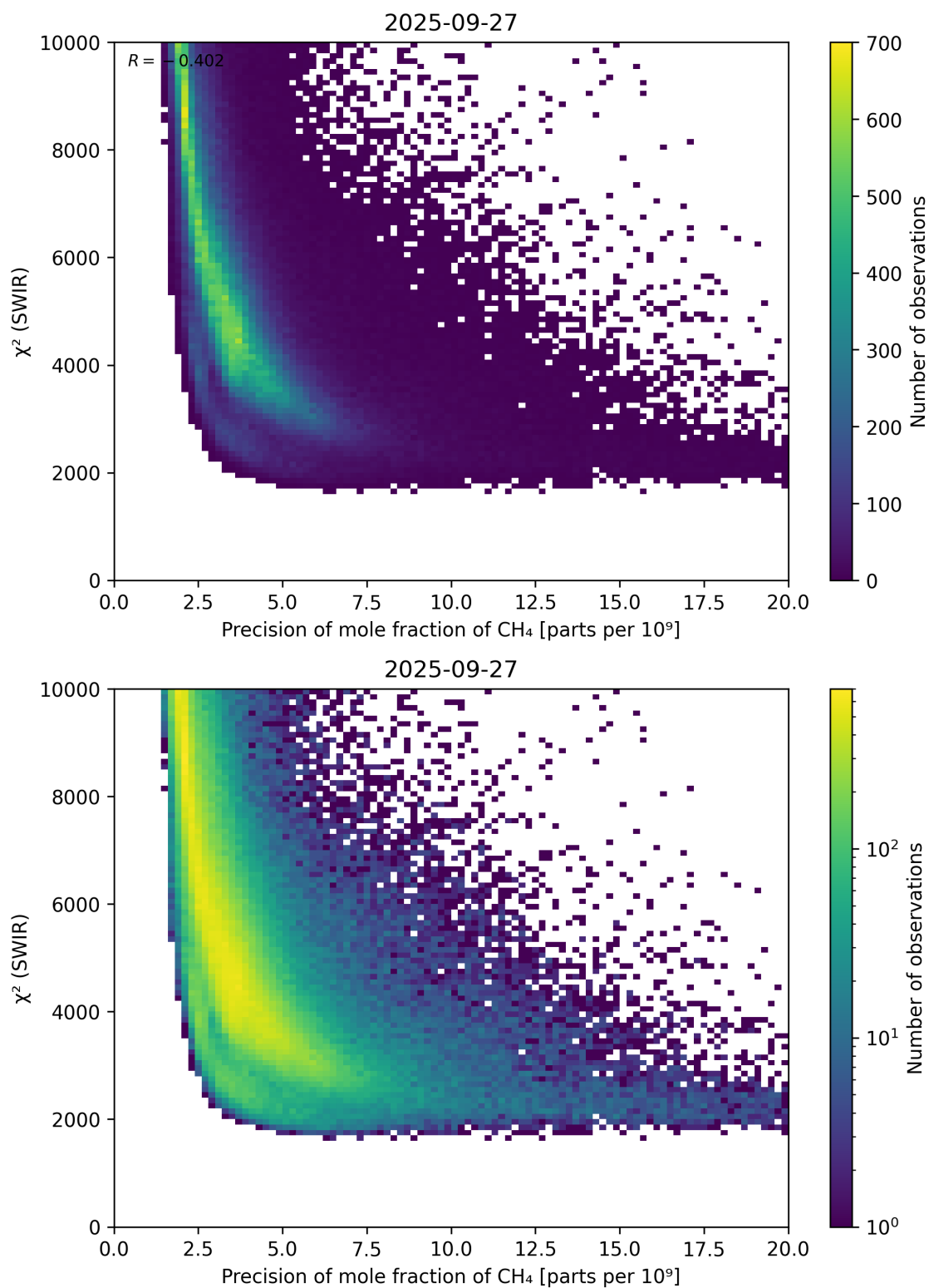
Figure 79: Scatter density plot of “Precision of mole fraction of \text{CH}_4 ” against “ \chi^2 (SWIR)” for 2025-09-26 to 2025-09-28.
