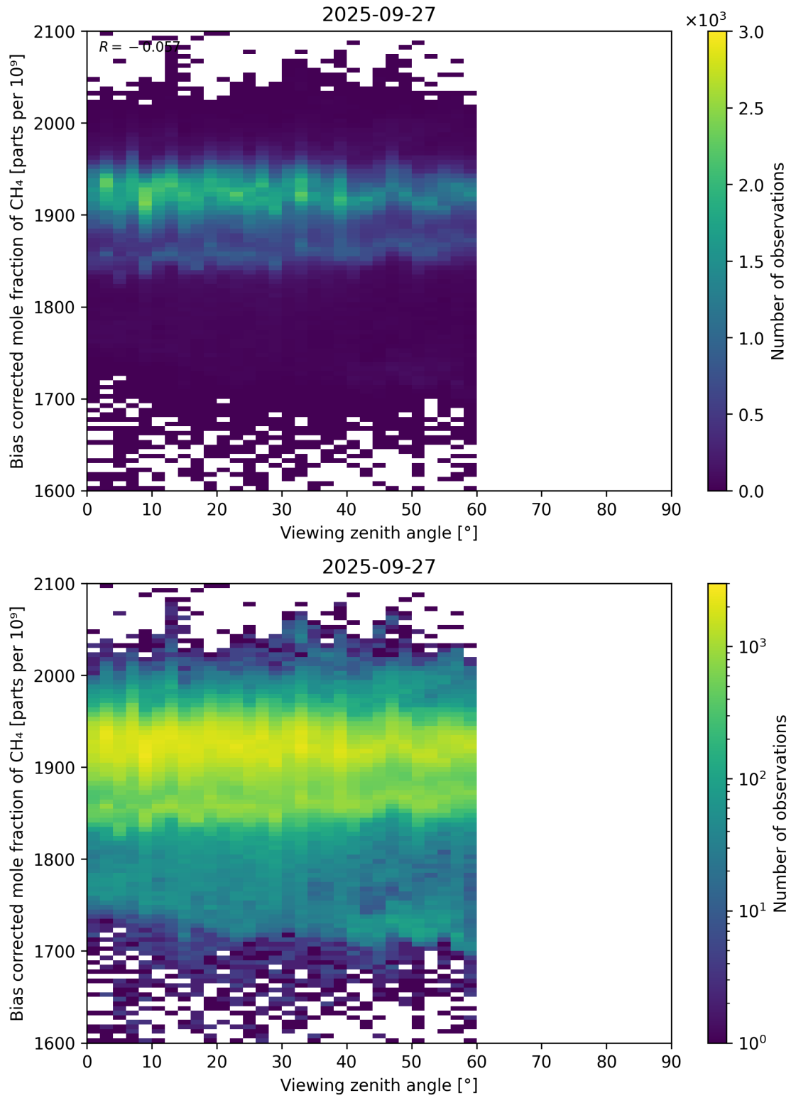
Figure 111: Scatter density plot of “Viewing zenith angle” against “Bias corrected mole fraction of CH 4 ” for 2025-09-26 to 2025-09-28.
