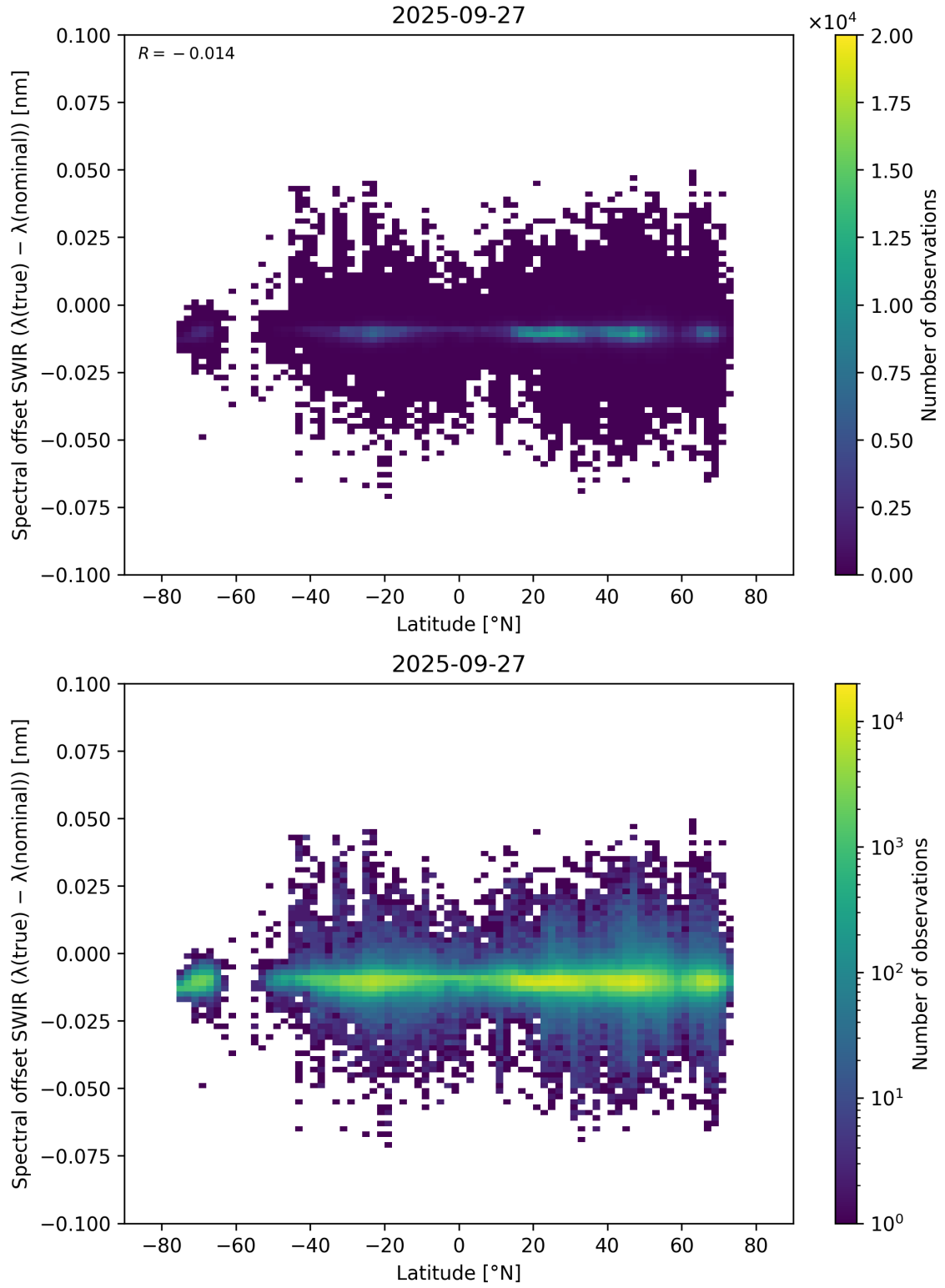
Figure 62: Scatter density plot of “Latitude” against “Spectral offset SWIR ( \lambda_{\text{true}} - \lambda_{\text{nominal}} )” for 2025-09-26 to 2025-09-28.
