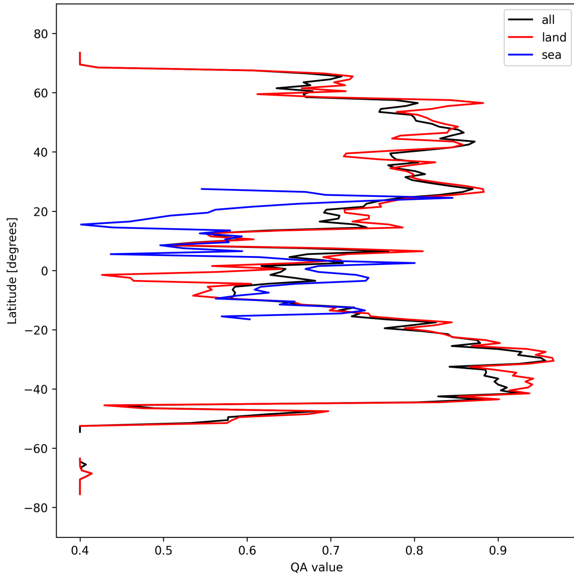
Figure 11: Zonal average of “QA value” for 2025-09-26 to 2025-09-28.
