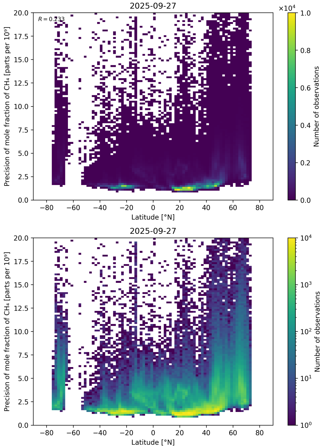
Figure 59: Scatter density plot of “Latitude” against “Precision of mole fraction of \text{CH}_4 ” for 2025-09-26 to 2025-09-28.
