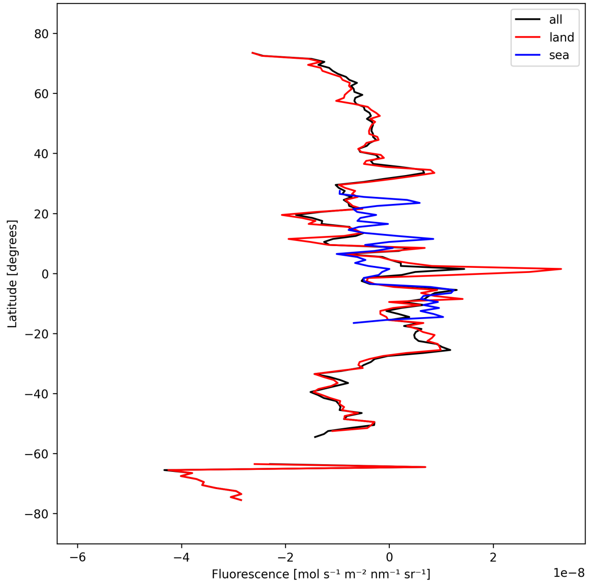
Figure 21: Zonal average of “Fluorescence” for 2025-09-26 to 2025-09-28.
