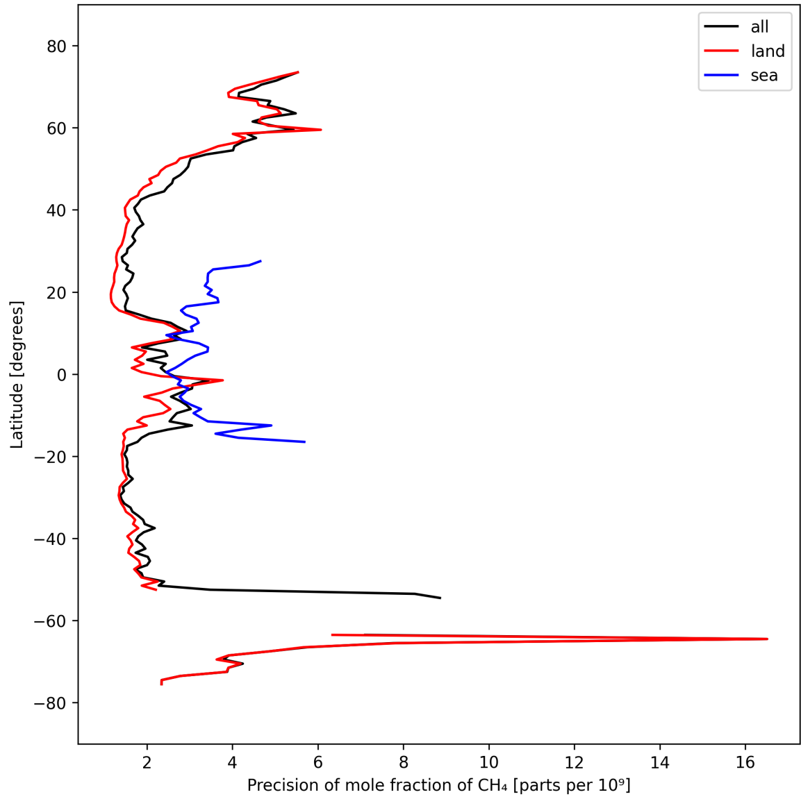
Figure 13: Zonal average of “Precision of mole fraction of CH 4 ” for 2025-09-26 to 2025-09-28.
