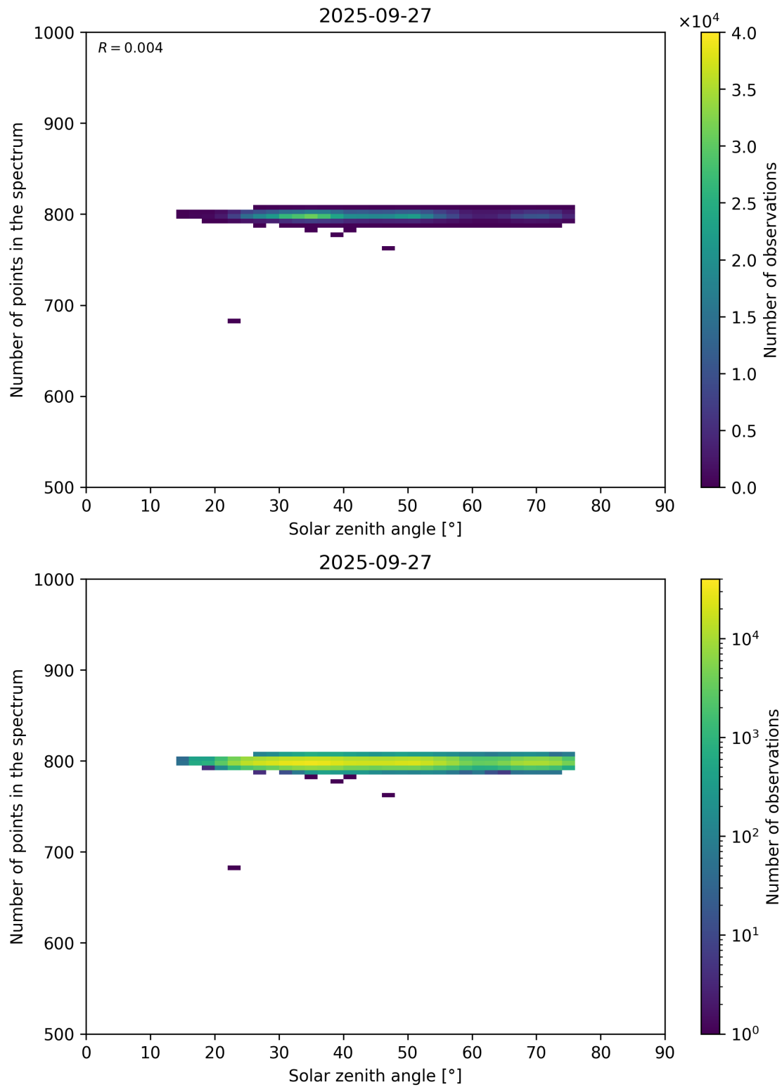
Figure 103: Scatter density plot of “Solar zenith angle” against “Number of points in the spectrum” for 2025-09-26 to 2025-09-28.
