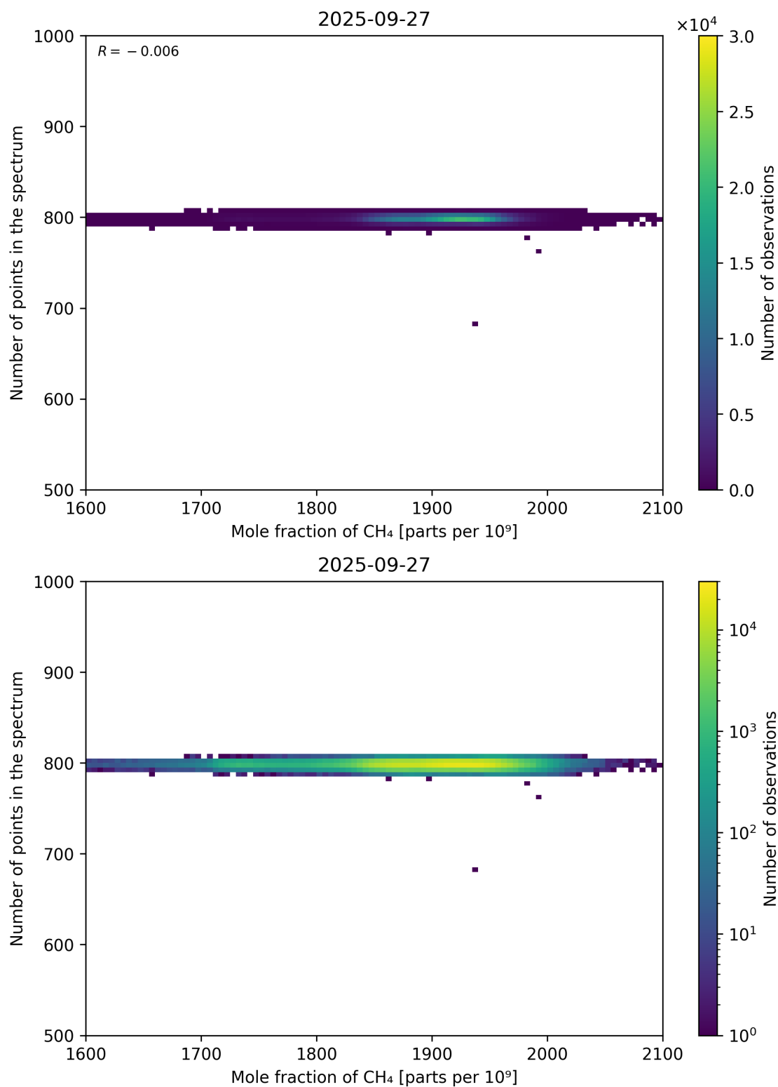
Figure 77: Scatter density plot of “Mole fraction of CH 4 ” against “Number of points in the spectrum” for 2025-09-26 to 2025-09-28.
