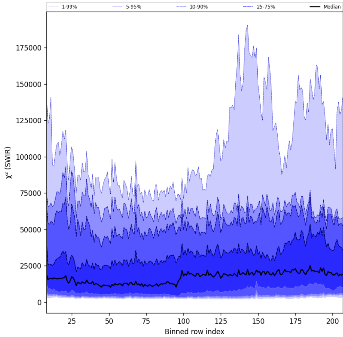
Figure 39: Along track statistics of " \chi^2 (SWIR)" for 2025-09-26 to 2025-09-28
