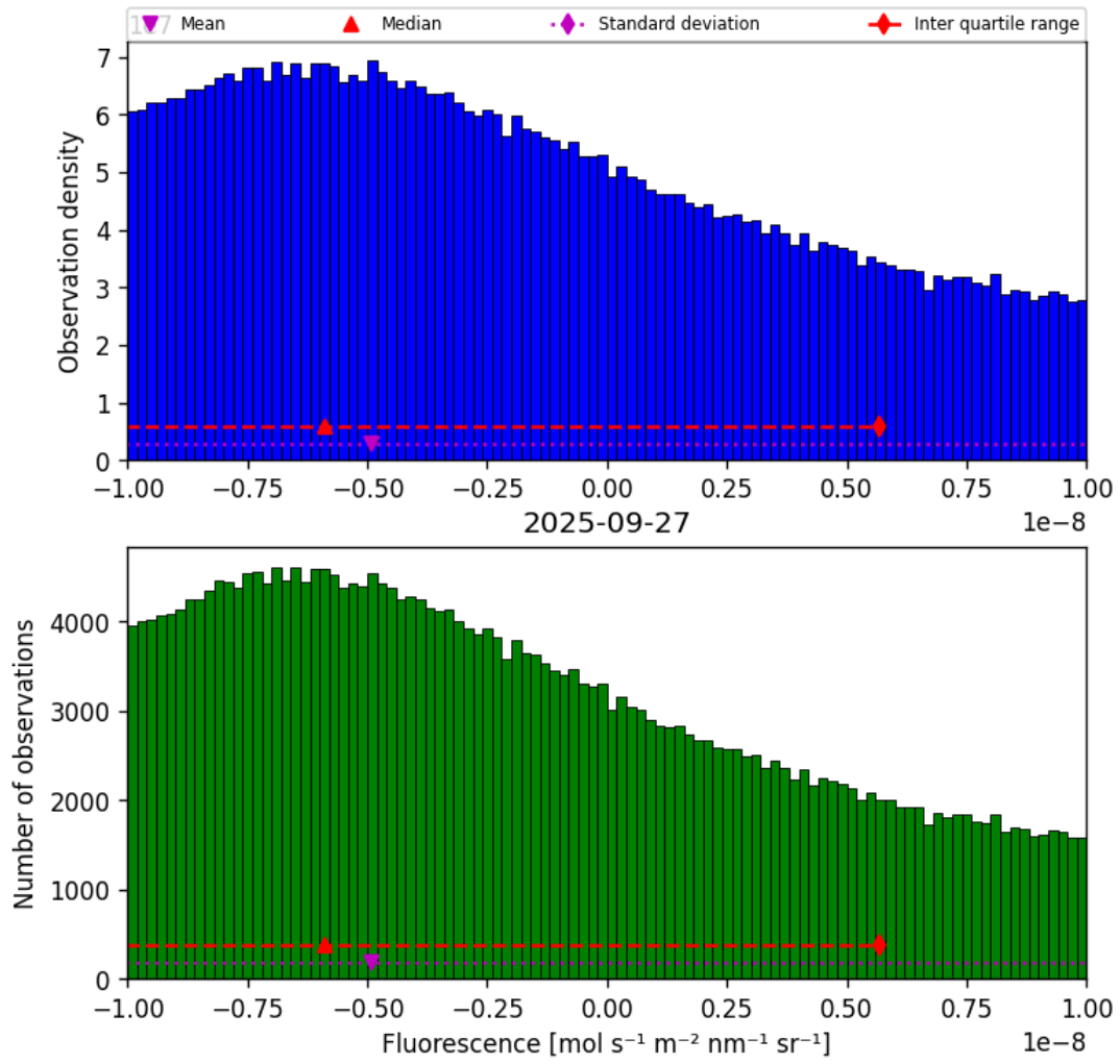
Figure 32: Histogram of “Fluorescence” for 2025-09-26 to 2025-09-28
