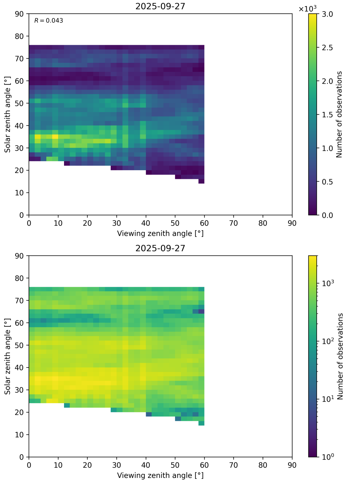
Figure 115: Scatter density plot of “Viewing zenith angle” against “Solar zenith angle” for 2025-09-26 to 2025-09-28.
