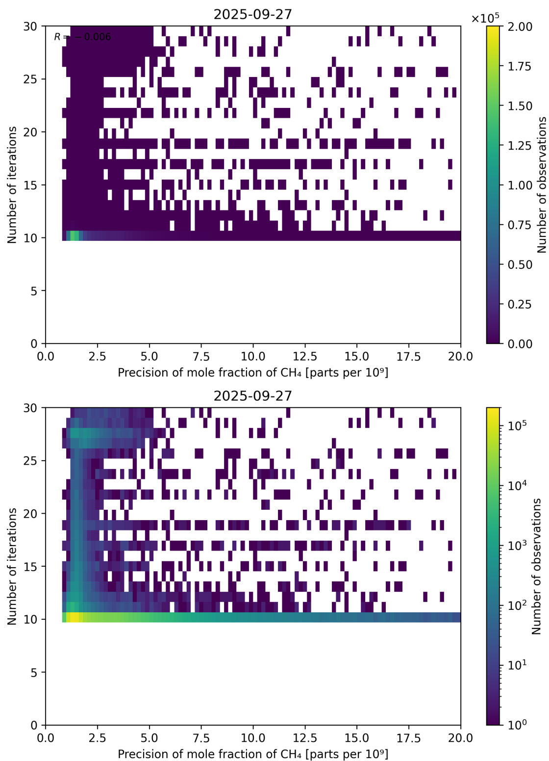
Figure 83: Scatter density plot of “Precision of mole fraction of CH 4 ” against “Number of iterations” for 2025-09-26 to 2025-09-28.
