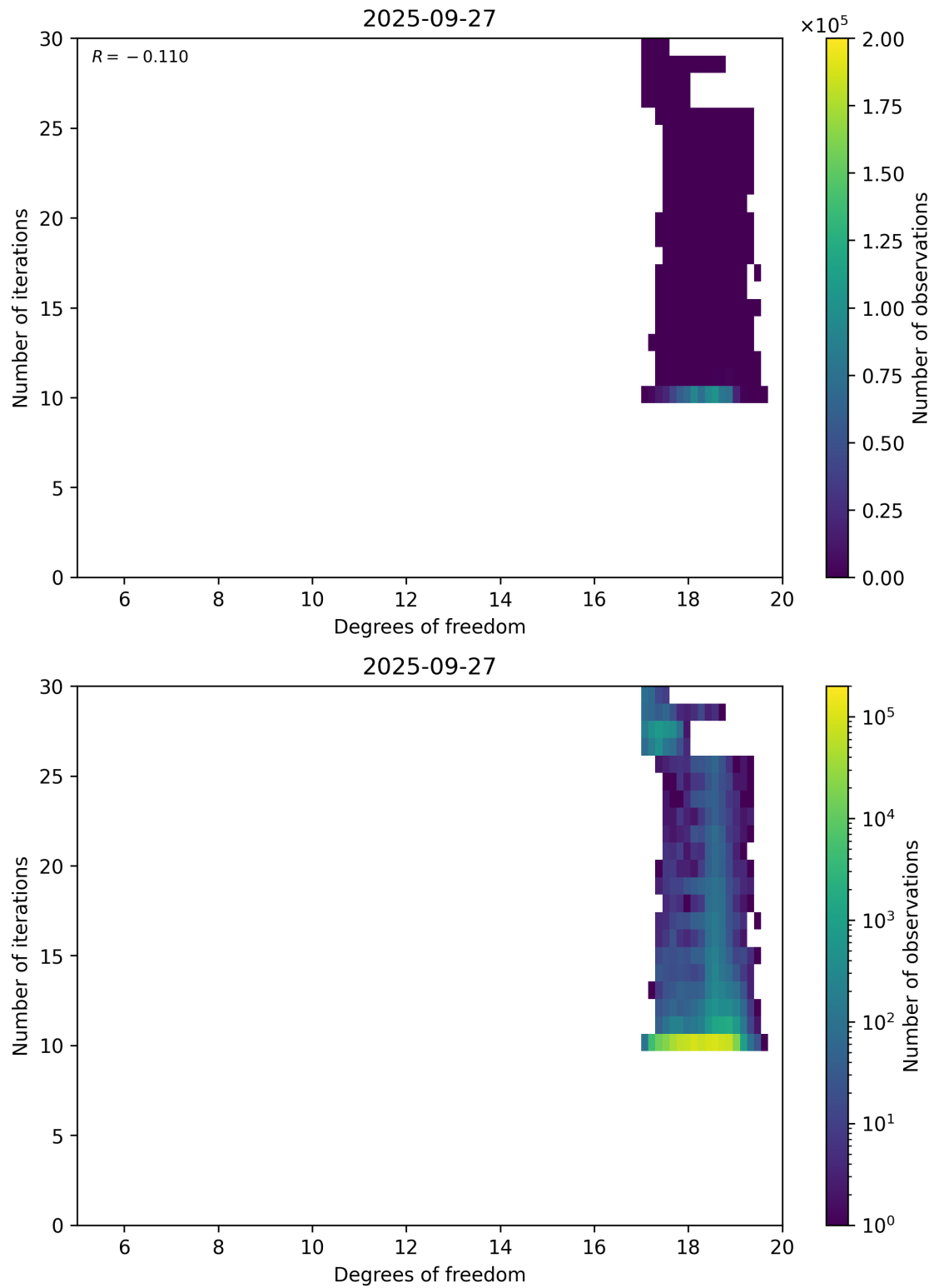
Figure 52: Scatter density plot of “Degrees of freedom” against “Number of iterations” for 2025-09-26 to 2025-09-28.
