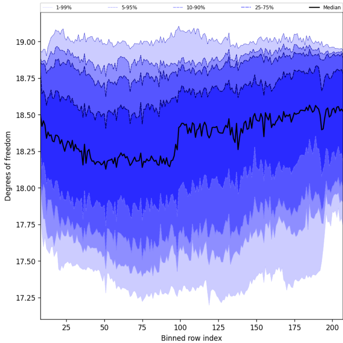
Figure 41: Along track statistics of “Degrees of freedom” for 2025-09-26 to 2025-09-28
