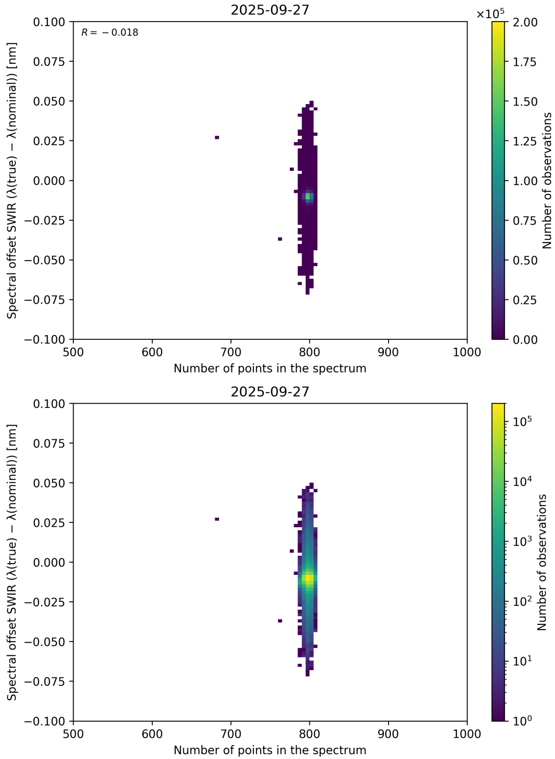
Figure 93: Scatter density plot of “Number of points in the spectrum” against “Spectral offset SWIR ( \lambda_{\text{true}} - \lambda_{\text{nominal}} )” for 2025-09-26 to 2025-09-28.
