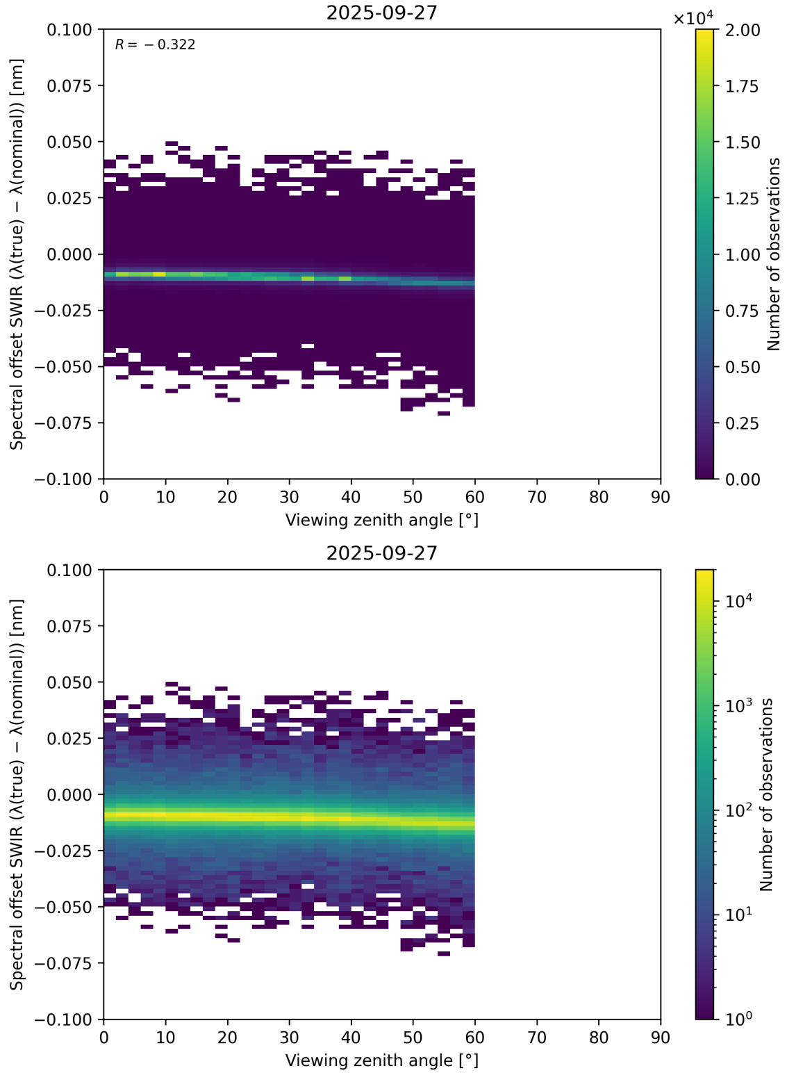
Figure 116: Scatter density plot of “Viewing zenith angle” against “Spectral offset SWIR ( \lambda_{\text{true}} - \lambda_{\text{nominal}} )” for 2025-09-26 to 2025-09-28.
