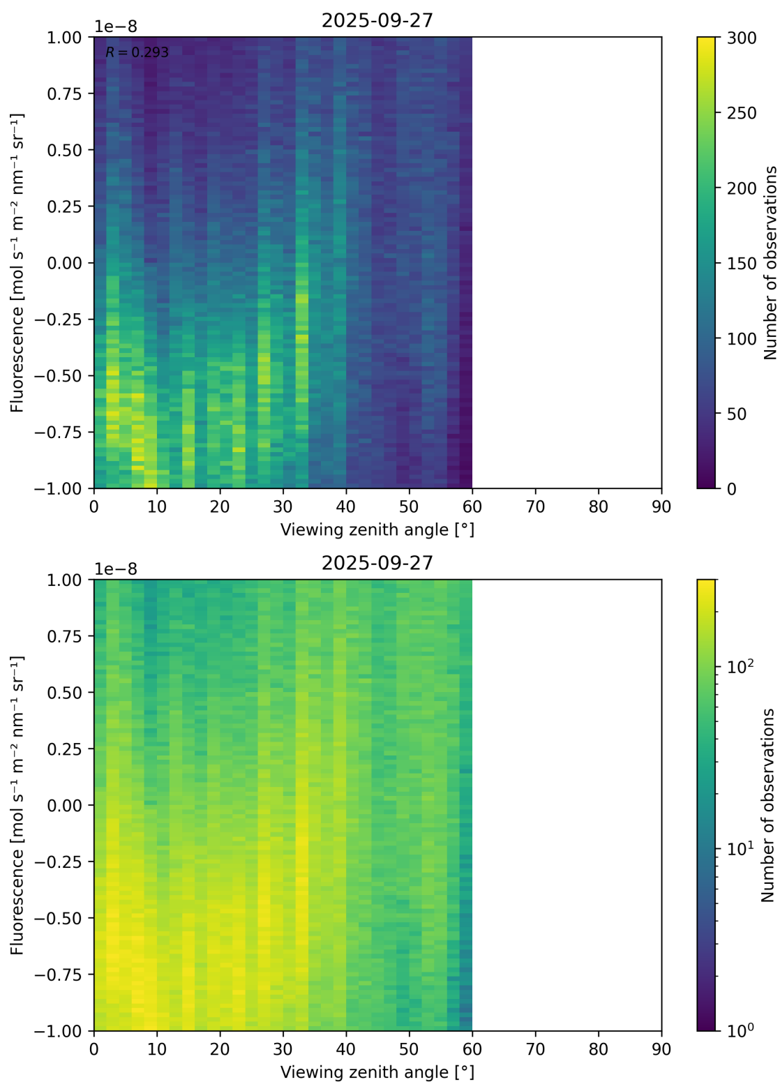
Figure 108: Scatter density plot of “Viewing zenith angle” against “Fluorescence” for 2025-09-26 to 2025-09-28.
