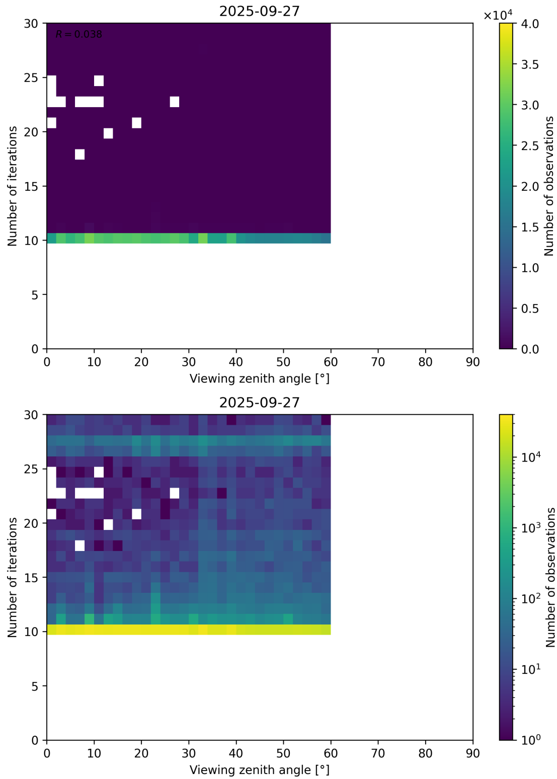
Figure 113: Scatter density plot of “Viewing zenith angle” against “Number of iterations” for 2025-09-26 to 2025-09-28.
