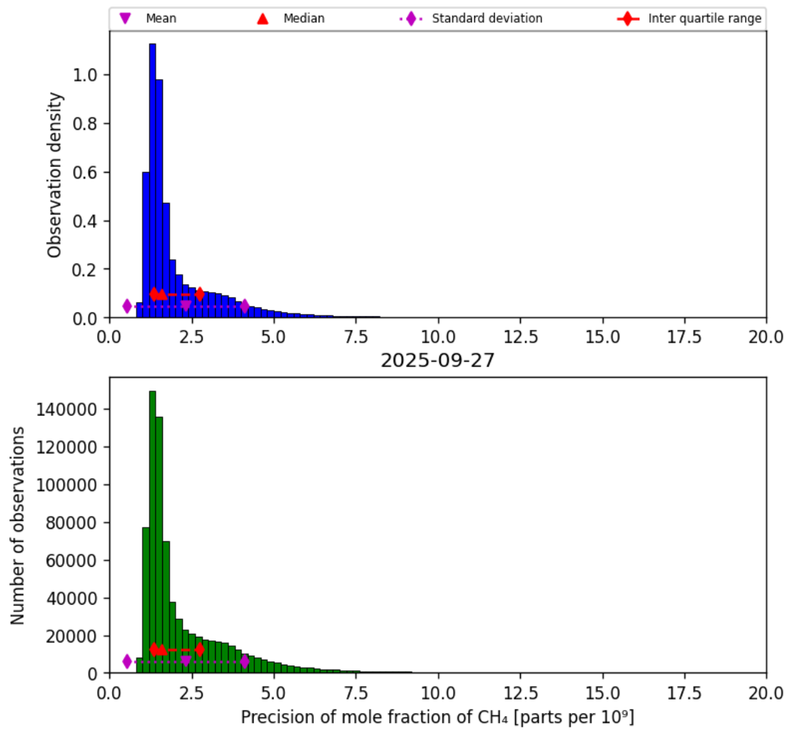
Figure 24: Histogram of “Precision of mole fraction of CH 4 ” for 2025-09-26 to 2025-09-28
