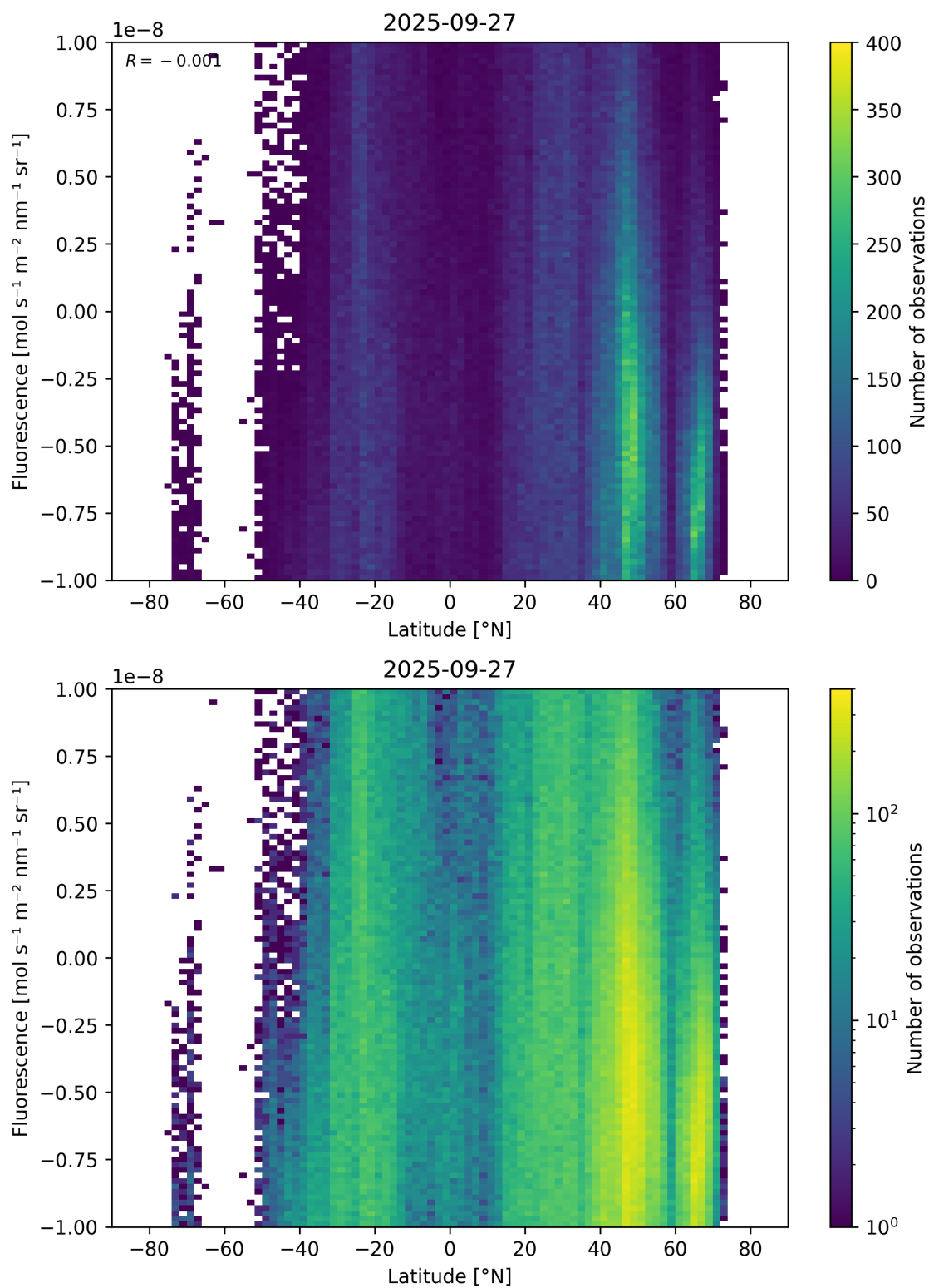
Figure 56: Scatter density plot of “Latitude” against “Fluorescence” for 2025-09-26 to 2025-09-28.
