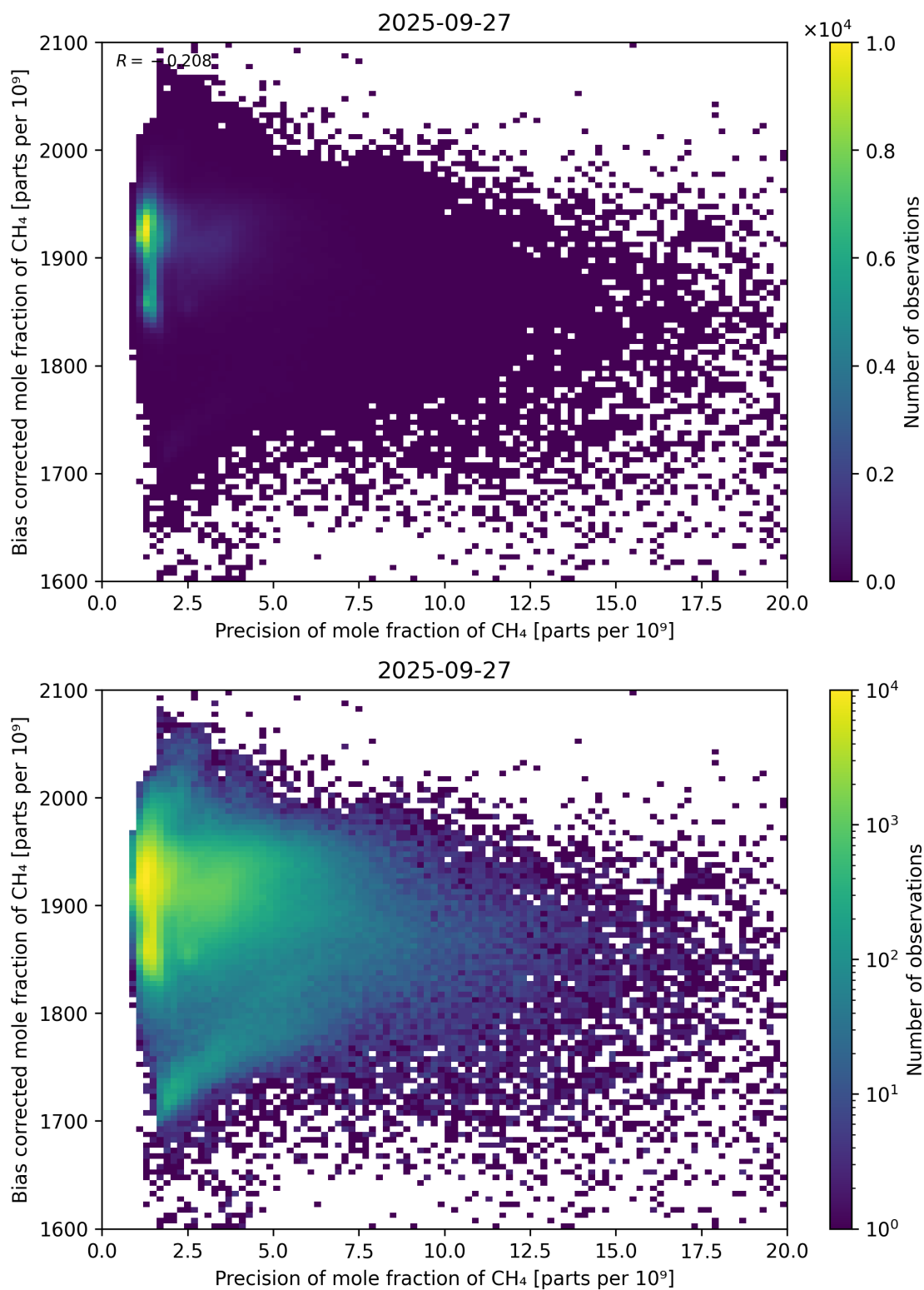
Figure 82: Scatter density plot of “Precision of mole fraction of CH 4 ” against “Bias corrected mole fraction of CH 4 ” for 2025-09-26 to 2025-09-28.
