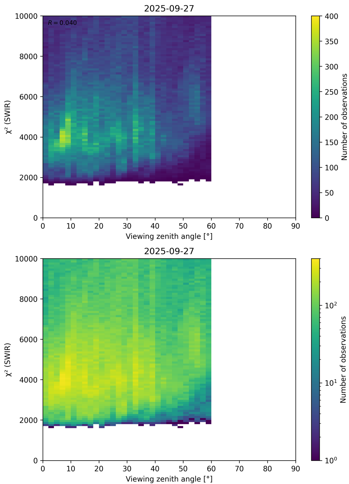
Figure 106: Scatter density plot of “Viewing zenith angle” against “ \chi^2 (SWIR)” for 2025-09-26 to 2025-09-28.
