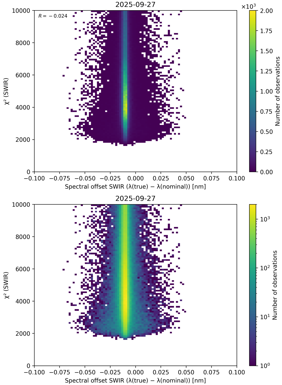
Figure 118: Scatter density plot of “Spectral offset SWIR ( \lambda_{\text{true}} - \lambda_{\text{nominal}} )” against “ \chi^2 (SWIR)” for 2025-09-26 to 2025-09-28.
