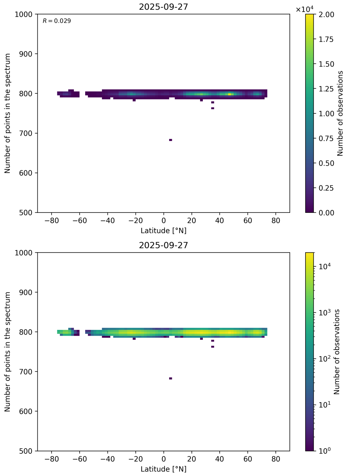
Figure 61: Scatter density plot of “Latitude” against “Number of points in the spectrum” for 2025-09-26 to 2025-09-28.
