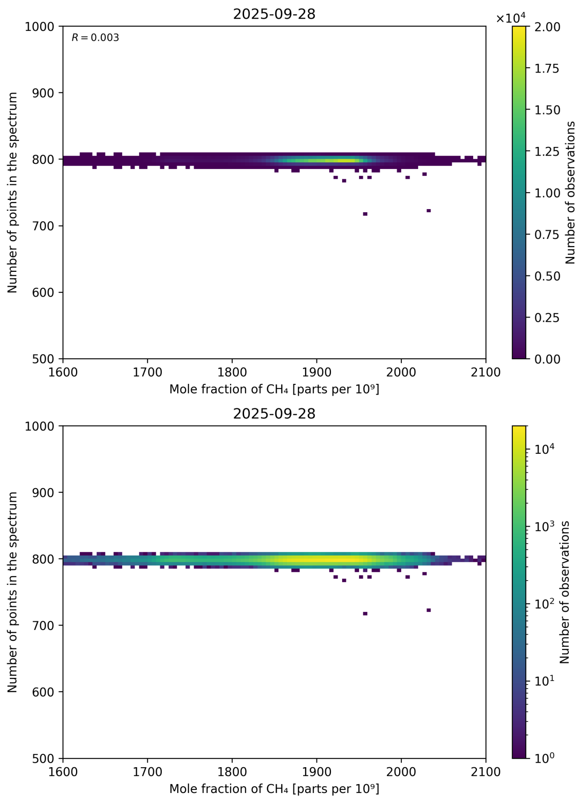
Figure 77: Scatter density plot of “Mole fraction of CH 4 ” against “Number of points in the spectrum” for 2025-09-27 to 2025-09-29.
