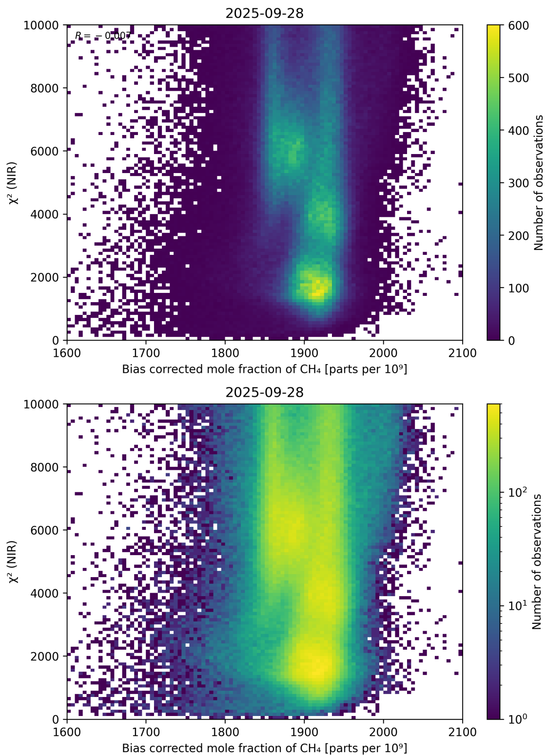
Figure 63: Scatter density plot of “Bias corrected mole fraction of \text{CH}_4 ” against “ \chi^2 (NIR)” for 2025-09-27 to 2025-09-29.
