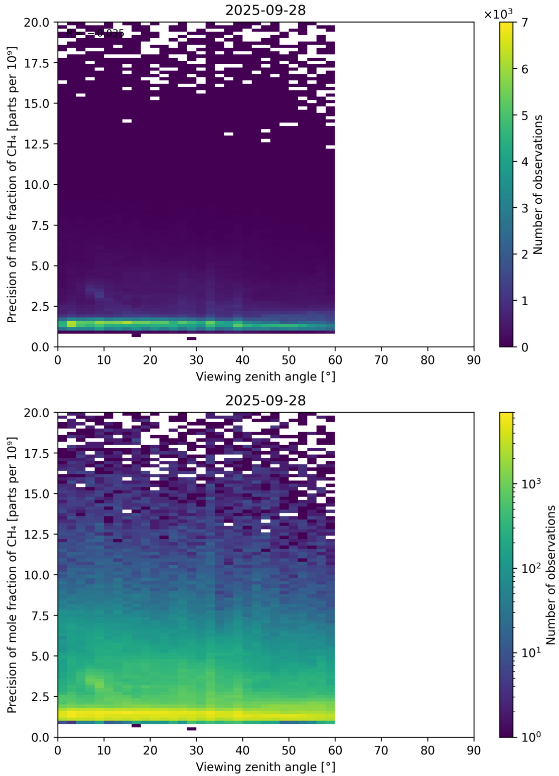
Figure 112: Scatter density plot of “Viewing zenith angle” against “Precision of mole fraction of CH 4 ” for 2025-09-27 to 2025-09-29.
