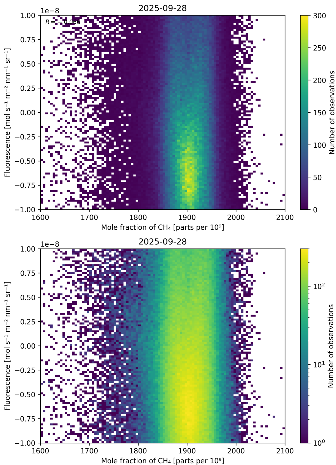
Figure 73: Scatter density plot of “Mole fraction of \text{CH}_4 ” against “Fluorescence” for 2025-09-27 to 2025-09-29.
