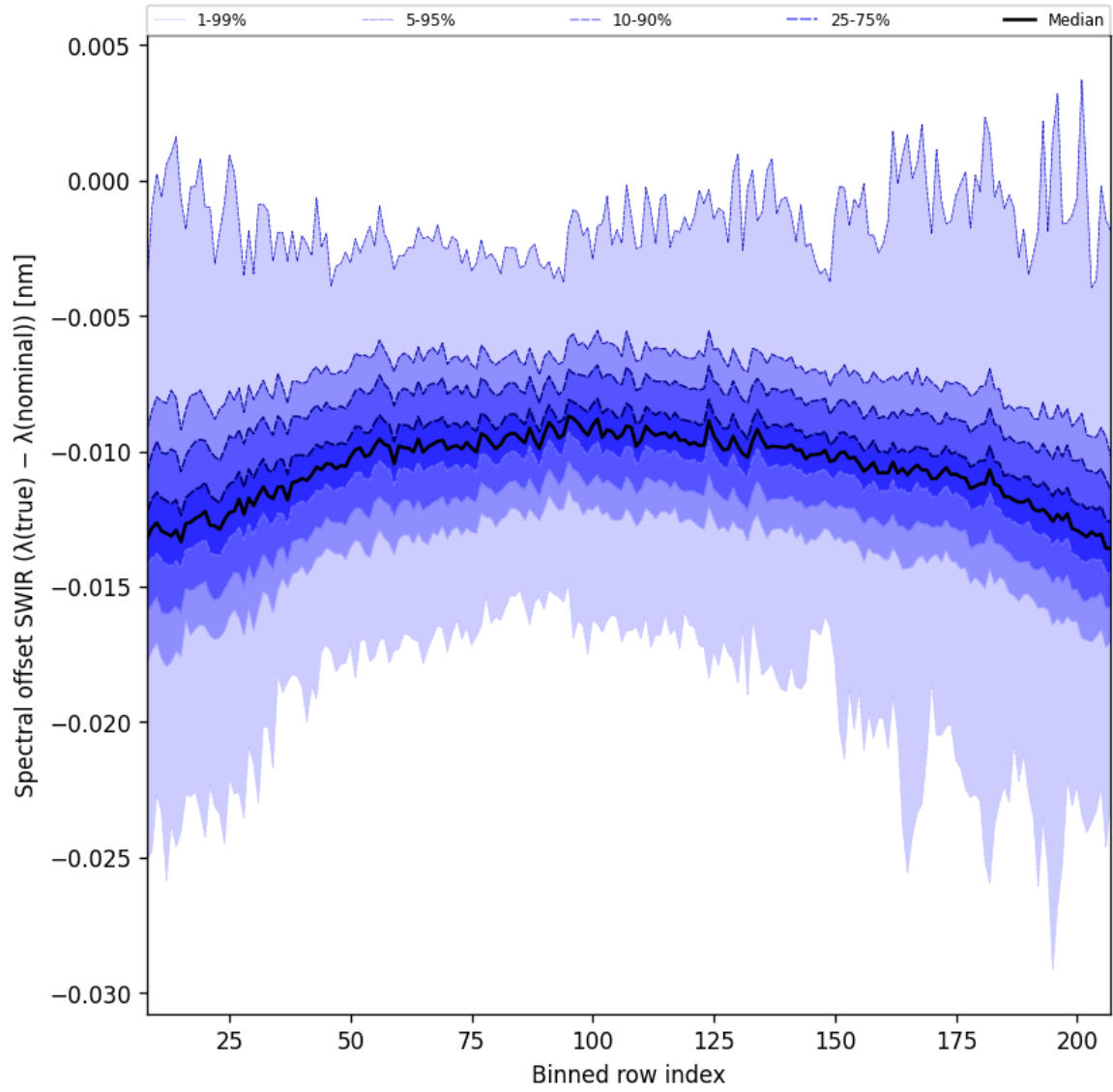
Figure 38: Along track statistics of “Spectral offset SWIR ( \lambda_{\text{true}} - \lambda_{\text{nominal}} )” for 2025-09-27 to 2025-09-29
