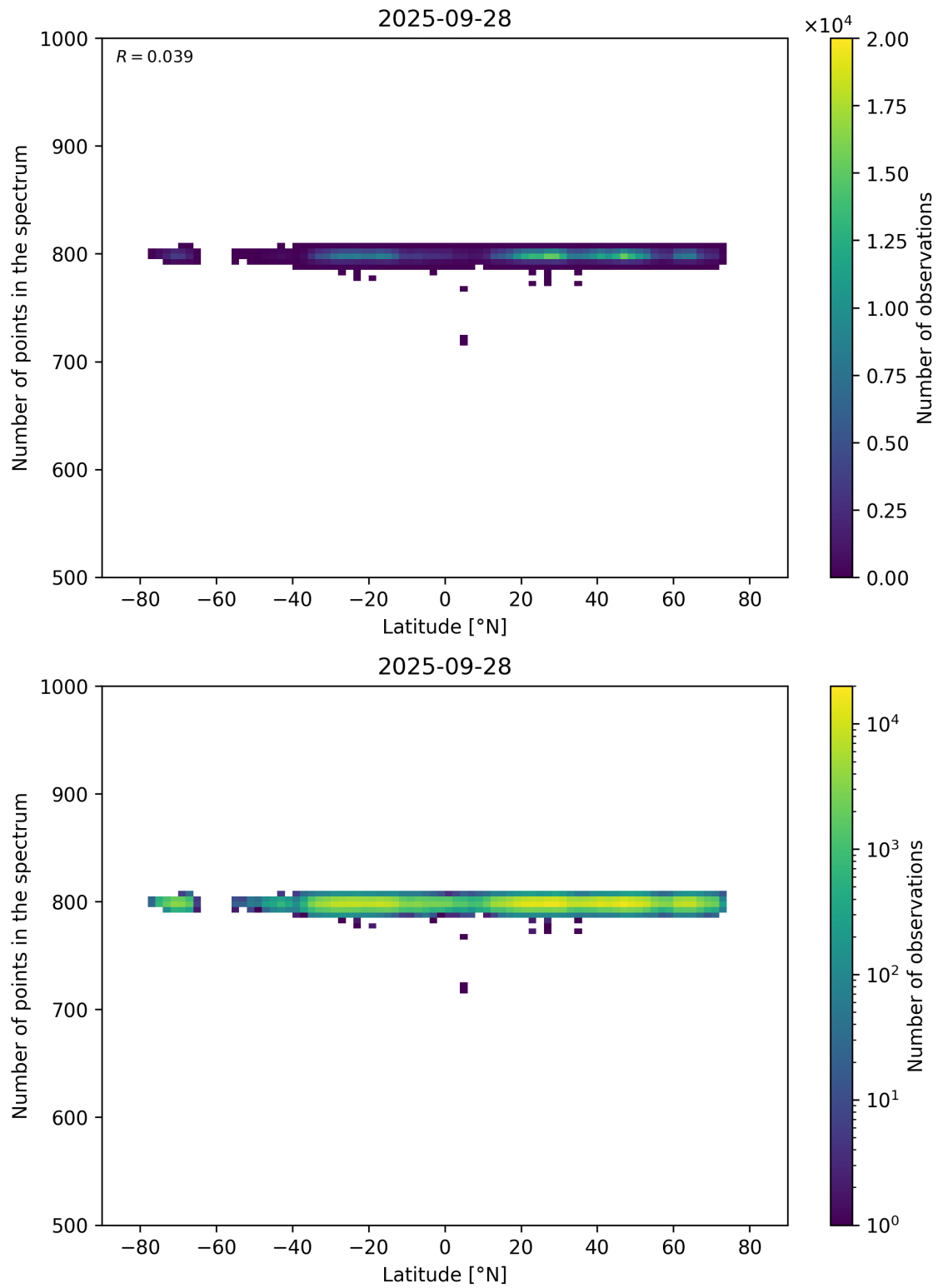
Figure 61: Scatter density plot of “Latitude” against “Number of points in the spectrum” for 2025-09-27 to 2025-09-29.
