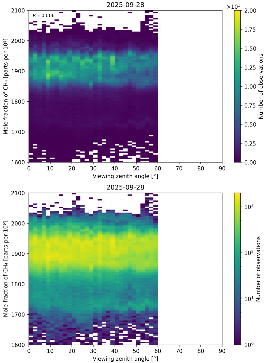
Figure 110: Scatter density plot of “Viewing zenith angle” against “Mole fraction of CH 4 ” for 2025-09-27 to 2025-09-29.
