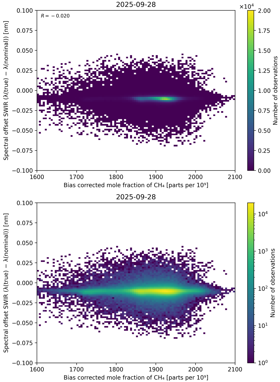
Figure 69: Scatter density plot of “Bias corrected mole fraction of \text{CH}_4 ” against “Spectral offset SWIR ( \lambda_{\text{true}} - \lambda_{\text{nominal}} )” for 2025-09-27 to 2025-09-29.
