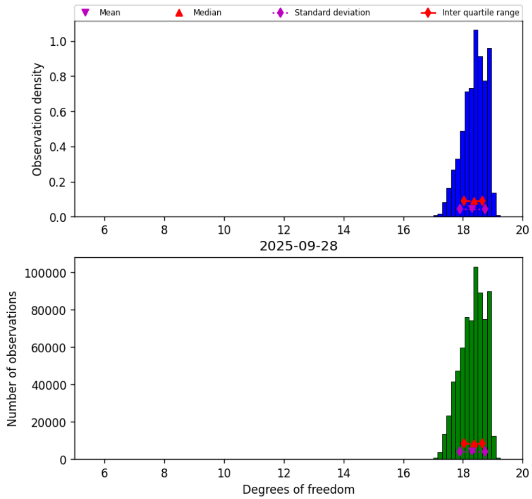
Figure 30: Histogram of “Degrees of freedom” for 2025-09-27 to 2025-09-29
