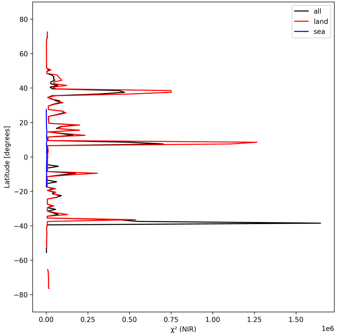
Figure 18: Zonal average of “ \chi^2 (NIR)” for 2025-09-27 to 2025-09-29.
