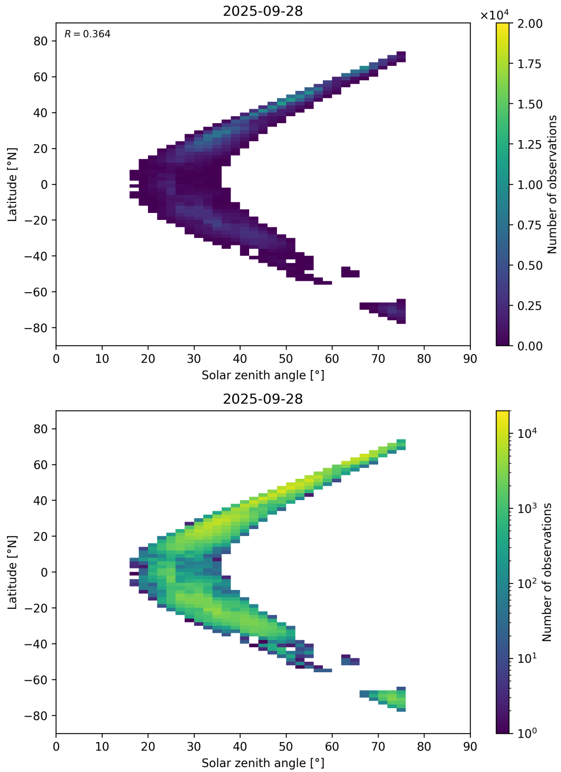
Figure 98: Scatter density plot of “Solar zenith angle” against “Latitude” for 2025-09-27 to 2025-09-29.
