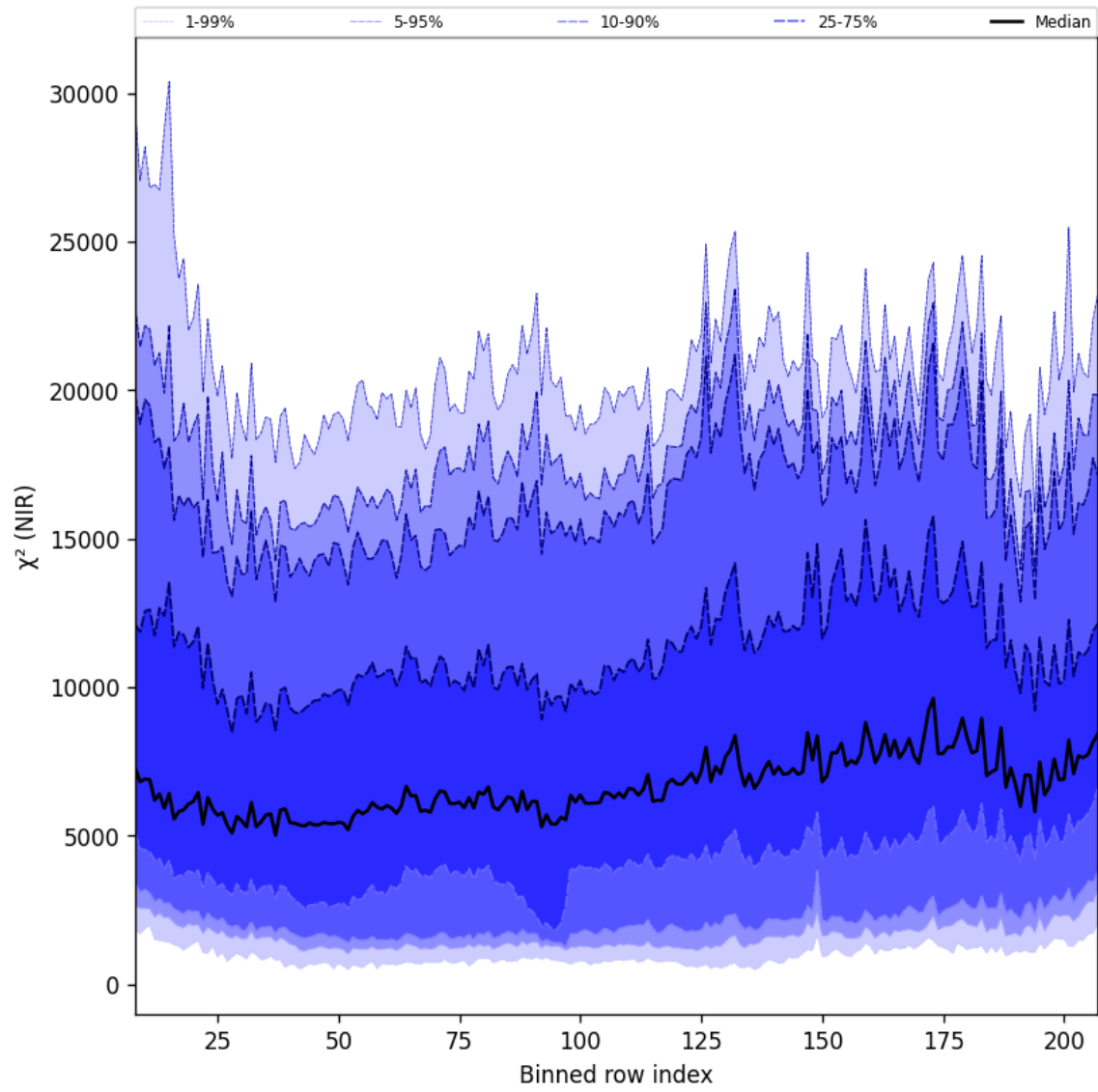
Figure 40: Along track statistics of “ \chi^2 (NIR)” for 2025-09-27 to 2025-09-29
