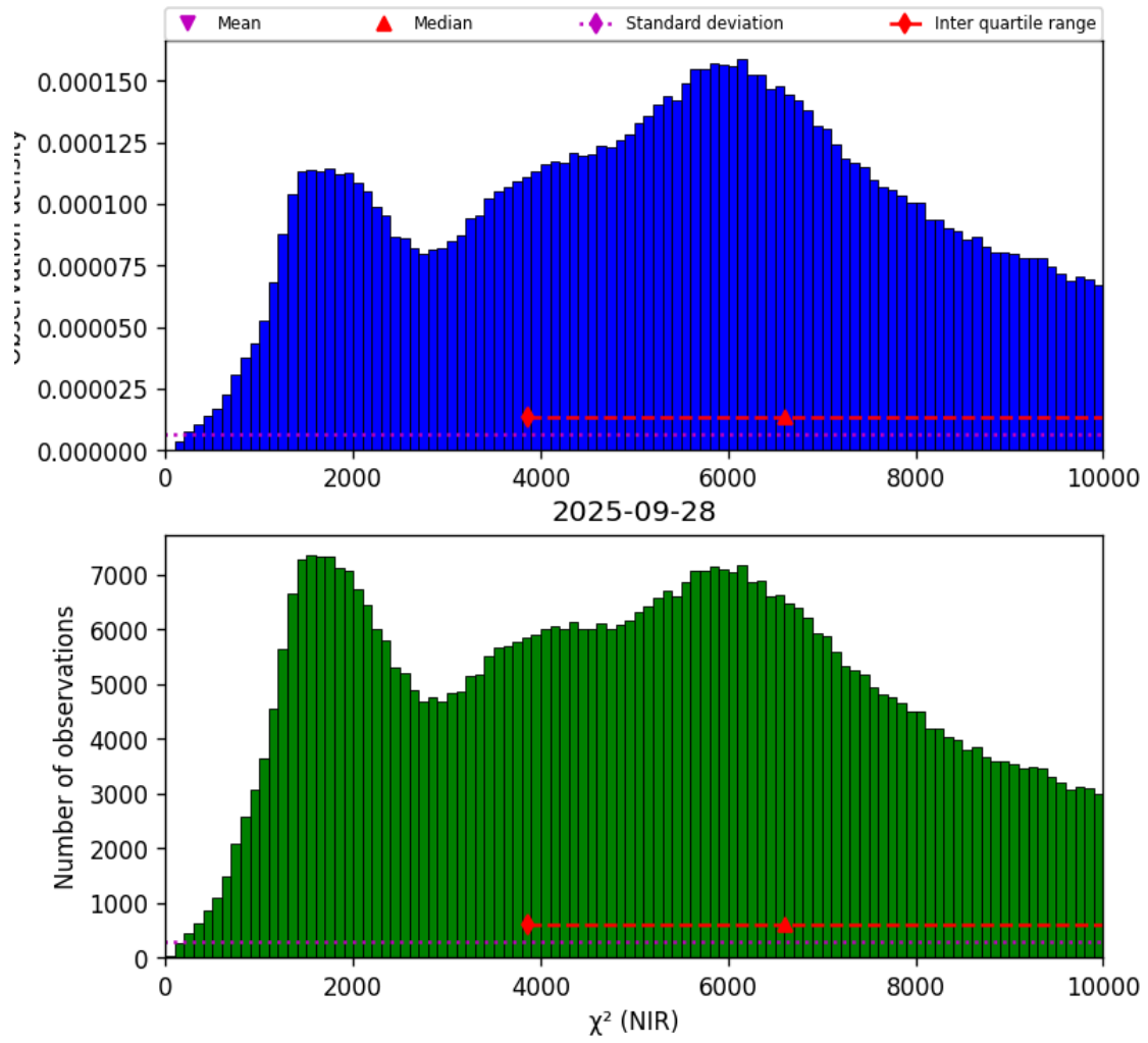
Figure 29: Histogram of “ \chi^2 (NIR)” for 2025-09-27 to 2025-09-29
