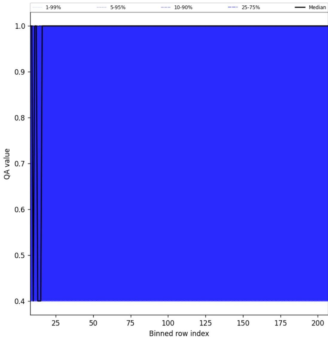
Figure 33: Along track statistics of “QA value” for 2025-09-27 to 2025-09-29
