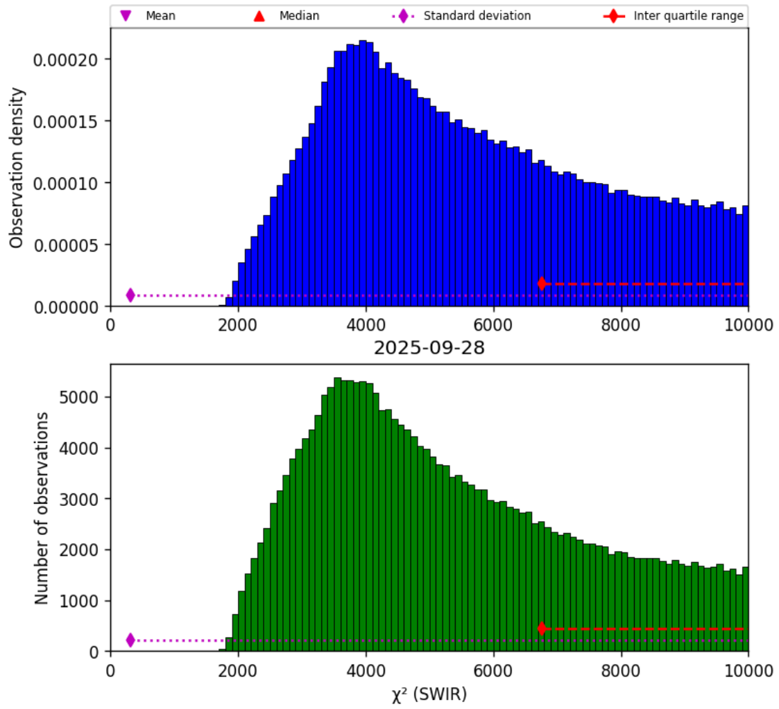
Figure 28: Histogram of " \chi^2 (SWIR)" for 2025-09-27 to 2025-09-29
