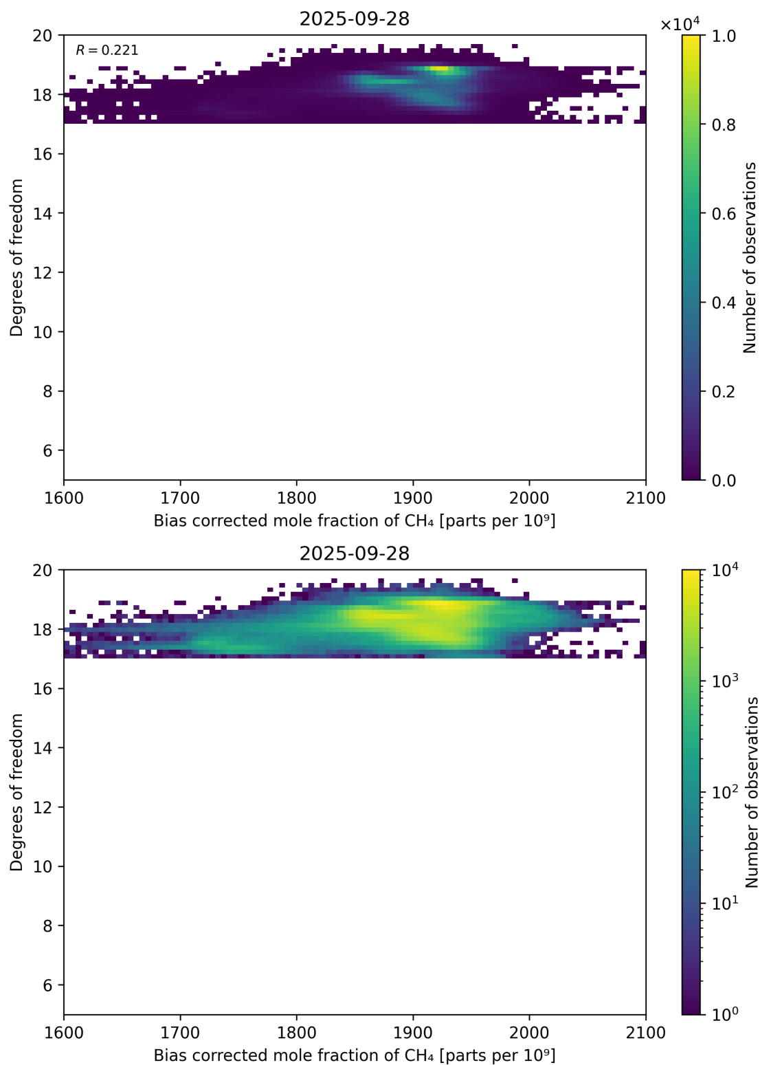
Figure 65: Scatter density plot of “Bias corrected mole fraction of \text{CH}_4 ” against “Degrees of freedom” for 2025-09-27 to 2025-09-29.
