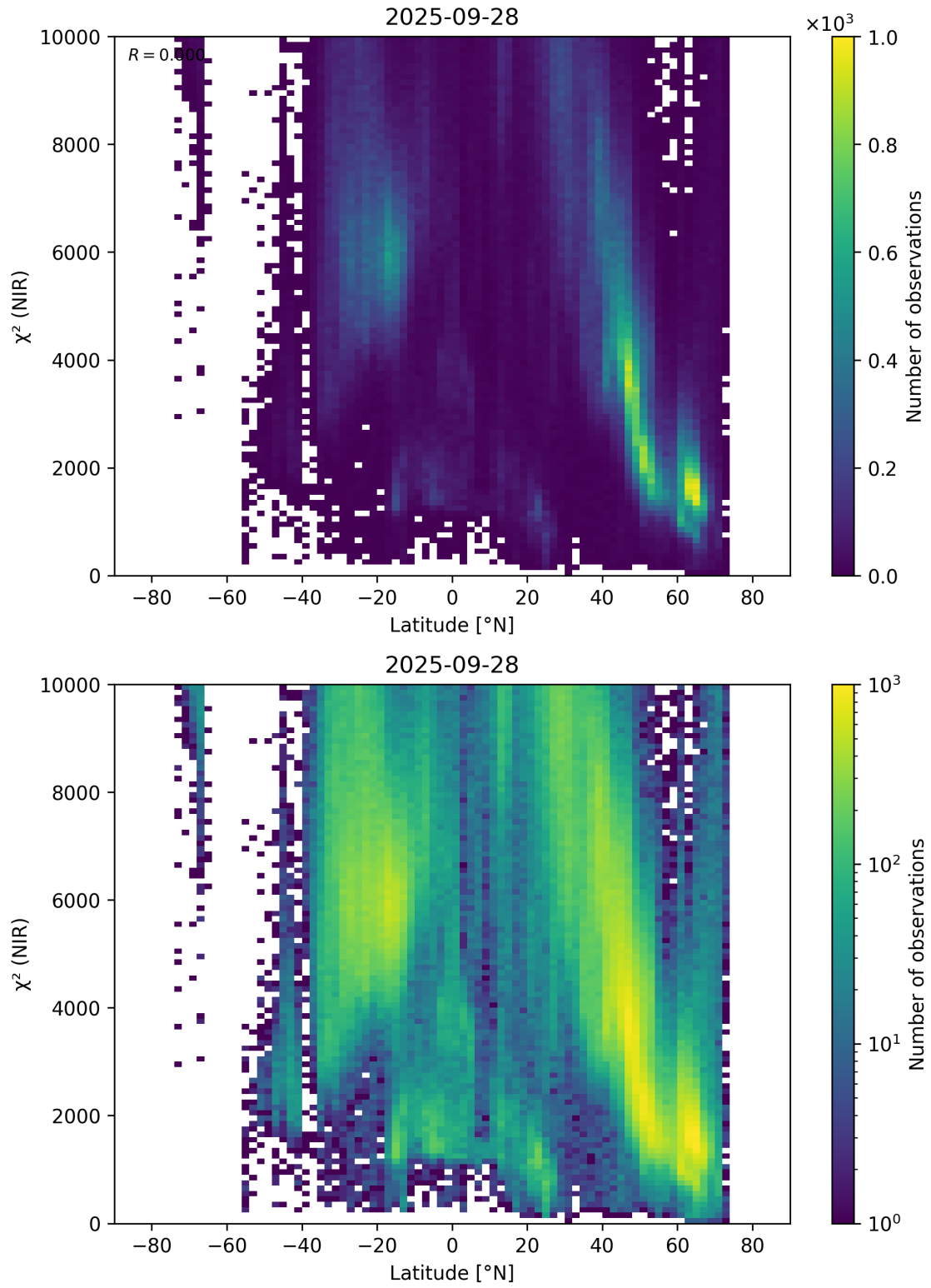
Figure 53: Scatter density plot of “Latitude” against “ \chi^2 (NIR)” for 2025-09-27 to 2025-09-29.
