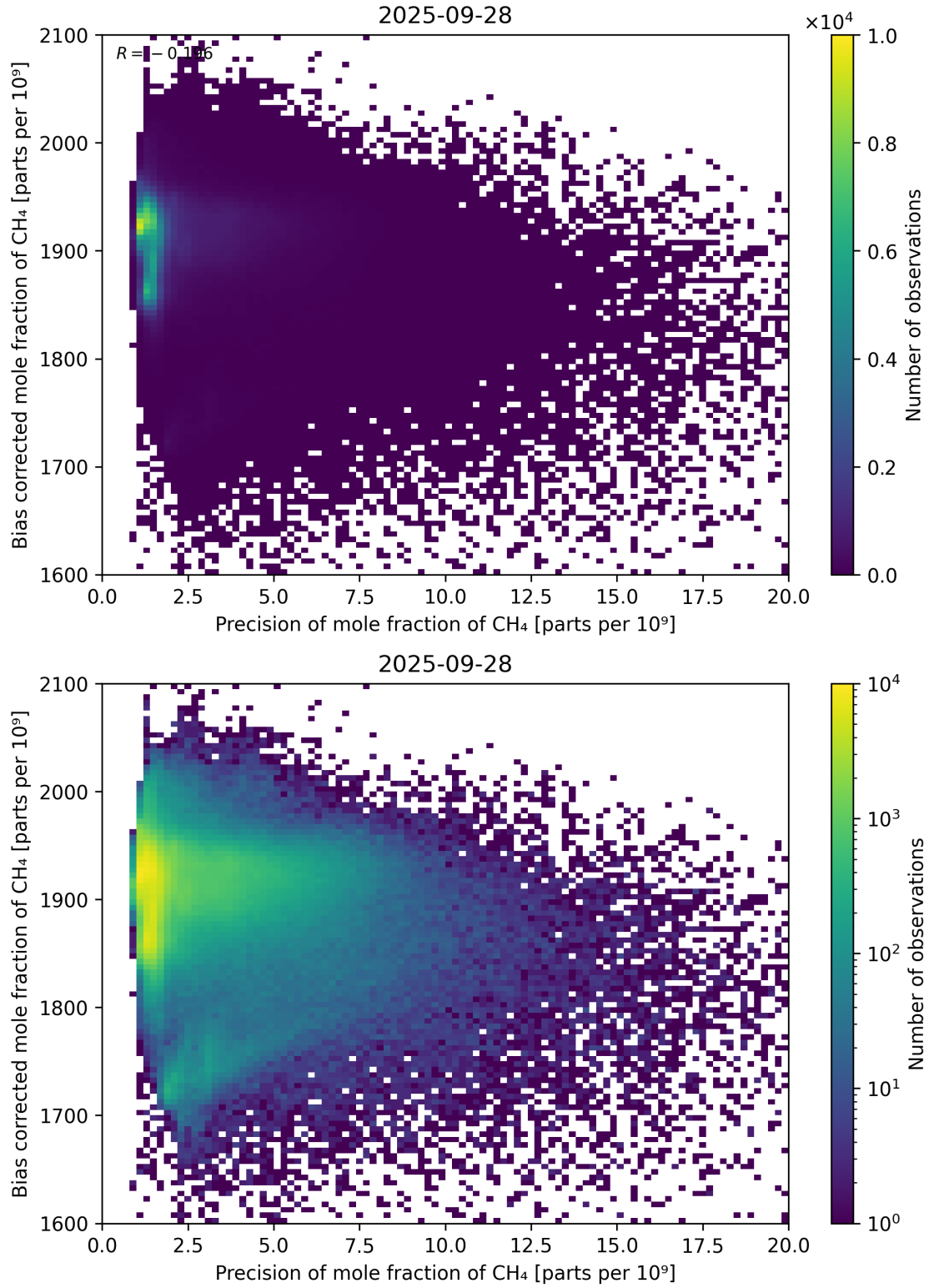
Figure 82: Scatter density plot of “Precision of mole fraction of CH 4 ” against “Bias corrected mole fraction of CH 4 ” for 2025-09-27 to 2025-09-29.
