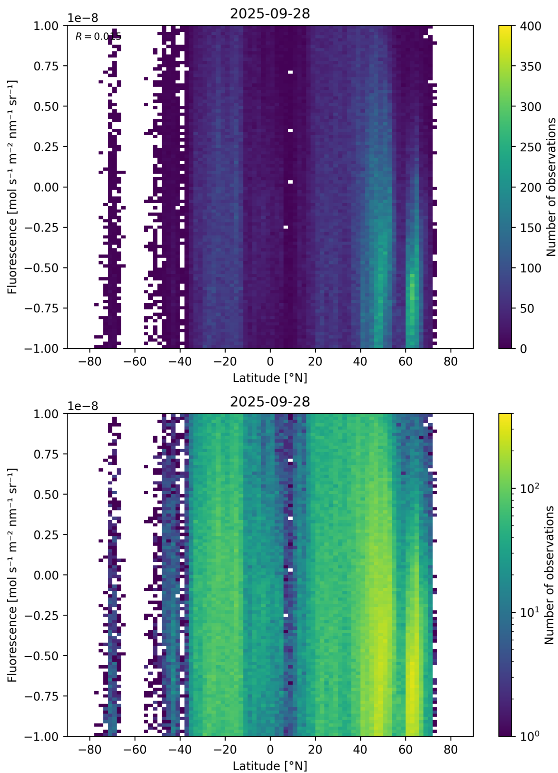
Figure 56: Scatter density plot of “Latitude” against “Fluorescence” for 2025-09-27 to 2025-09-29.
