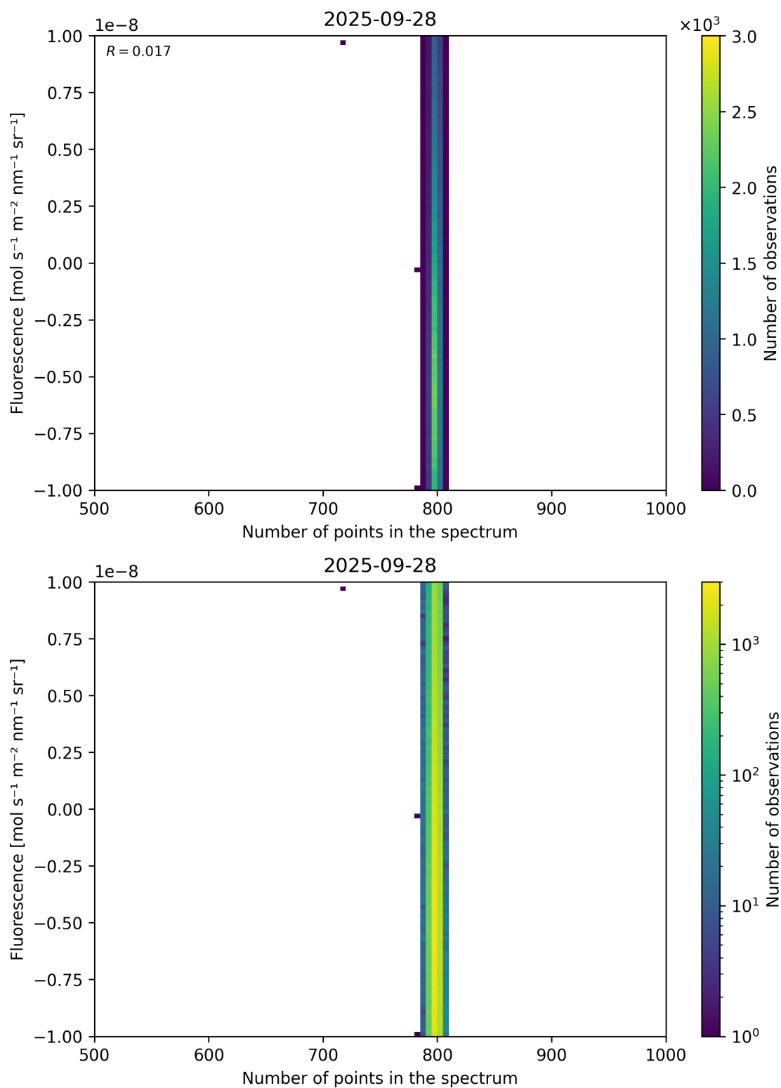
Figure 91: Scatter density plot of “Number of points in the spectrum” against “Fluorescence” for 2025-09-27 to 2025-09-29.
