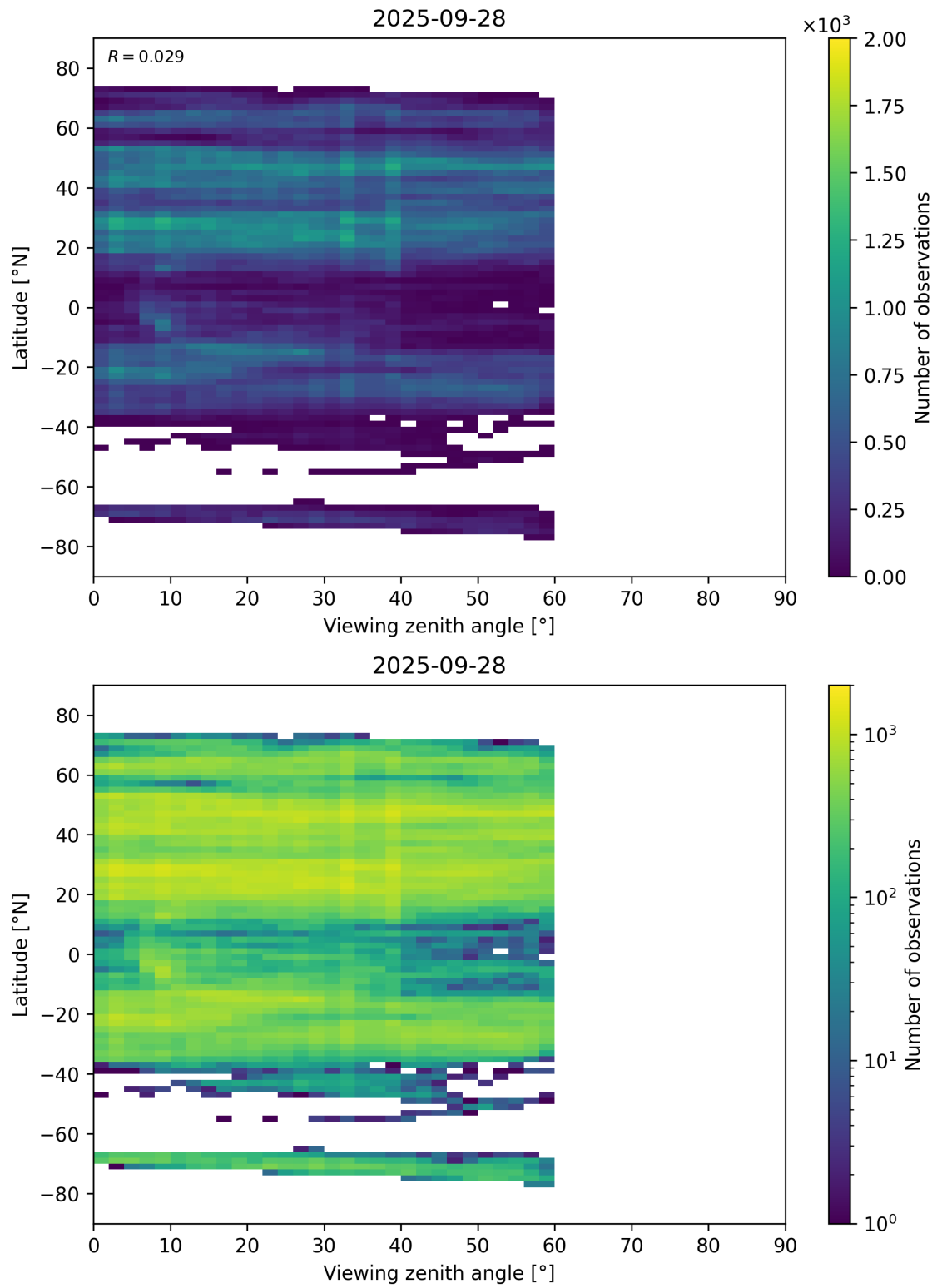
Figure 109: Scatter density plot of “Viewing zenith angle” against “Latitude” for 2025-09-27 to 2025-09-29.
