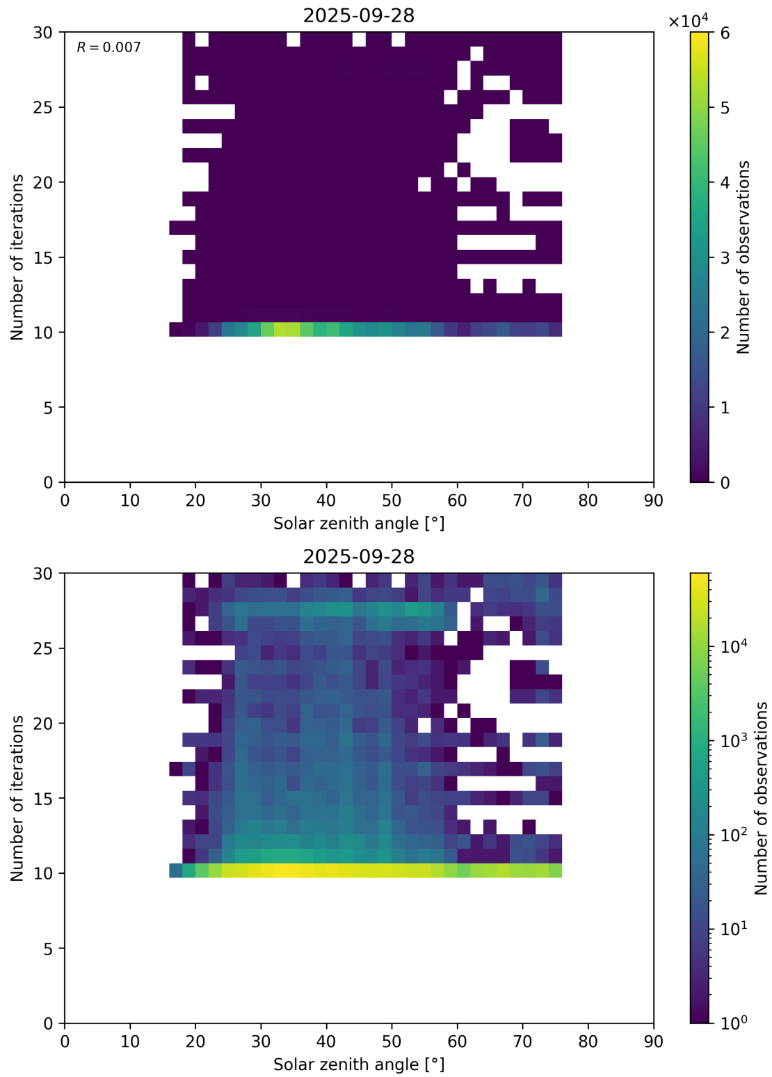
Figure 102: Scatter density plot of “Solar zenith angle” against “Number of iterations” for 2025-09-27 to 2025-09-29.
