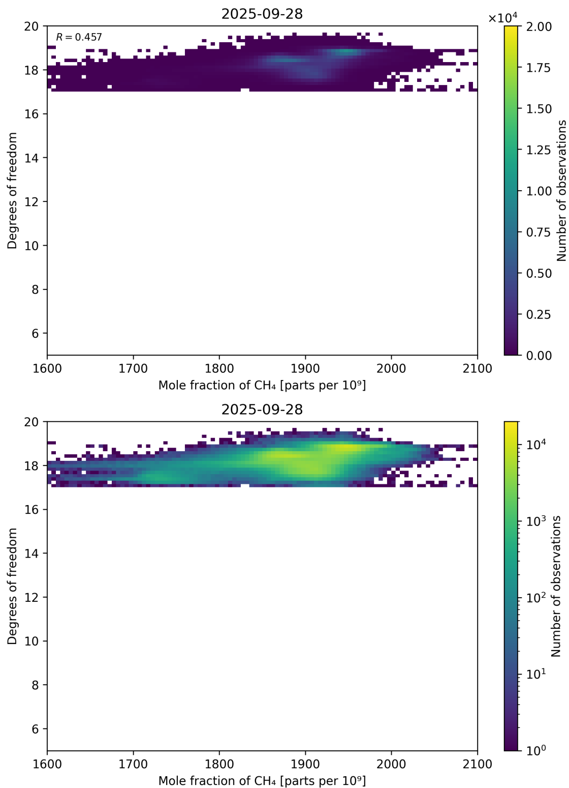
Figure 72: Scatter density plot of “Mole fraction of CH 4 ” against “Degrees of freedom” for 2025-09-27 to 2025-09-29.
