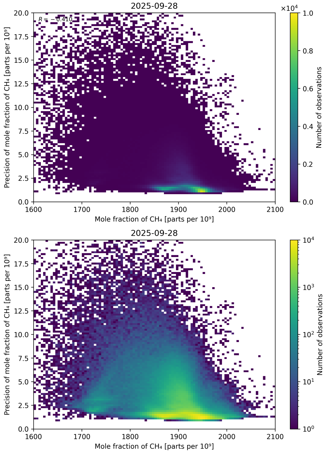
Figure 75: Scatter density plot of “Mole fraction of CH 4 ” against “Precision of mole fraction of CH 4 ” for 2025-09-27 to 2025-09-29.
