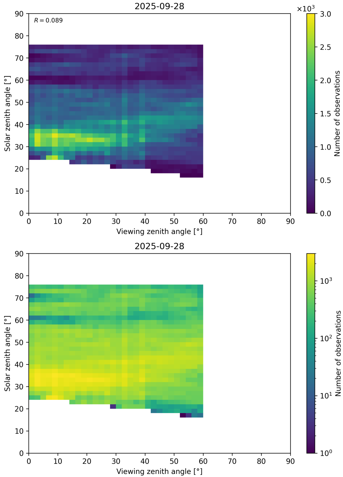
Figure 115: Scatter density plot of “Viewing zenith angle” against “Solar zenith angle” for 2025-09-27 to 2025-09-29.
