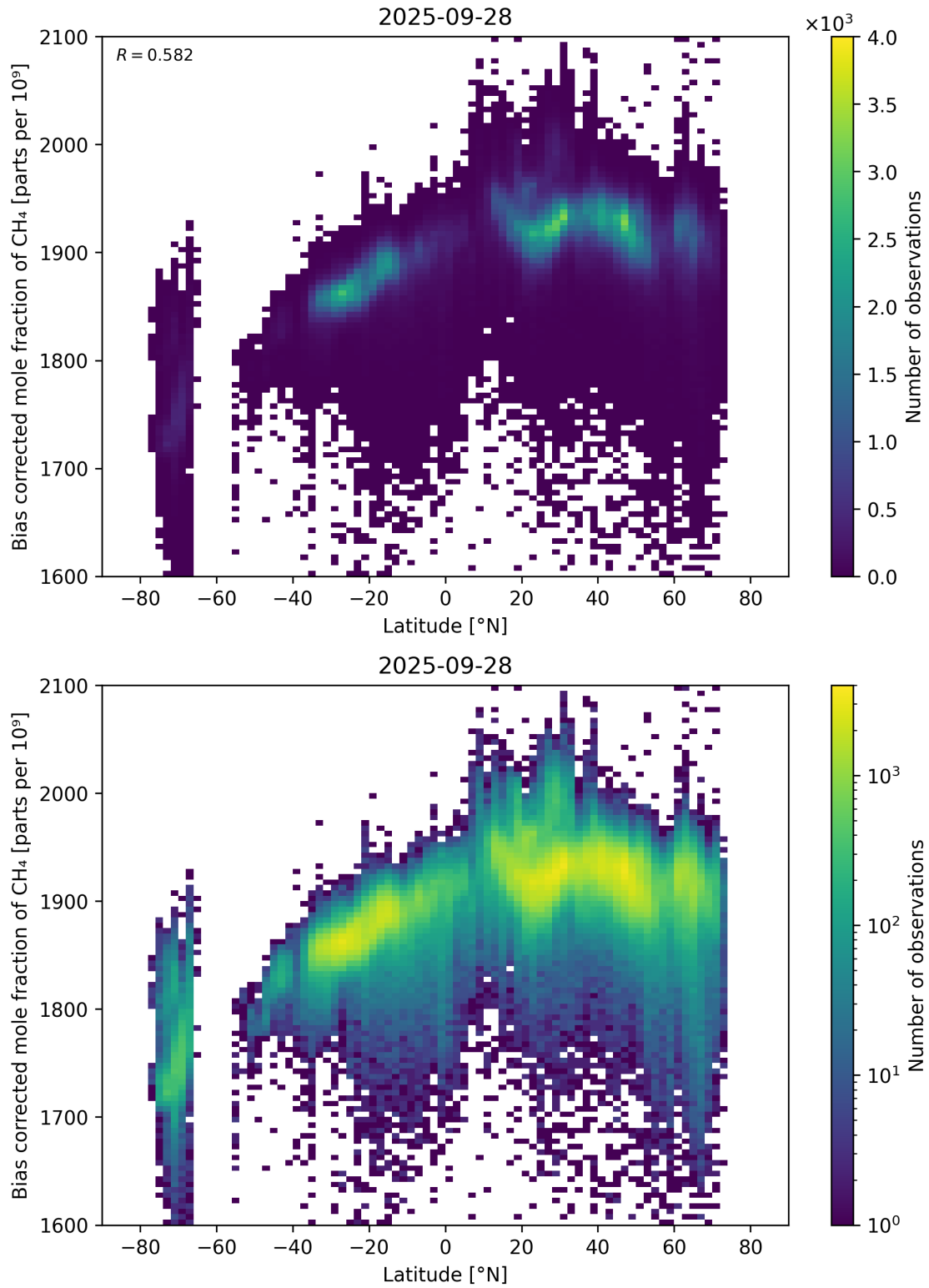
Figure 58: Scatter density plot of “Latitude” against “Bias corrected mole fraction of \text{CH}_4 ” for 2025-09-27 to 2025-09-29.
