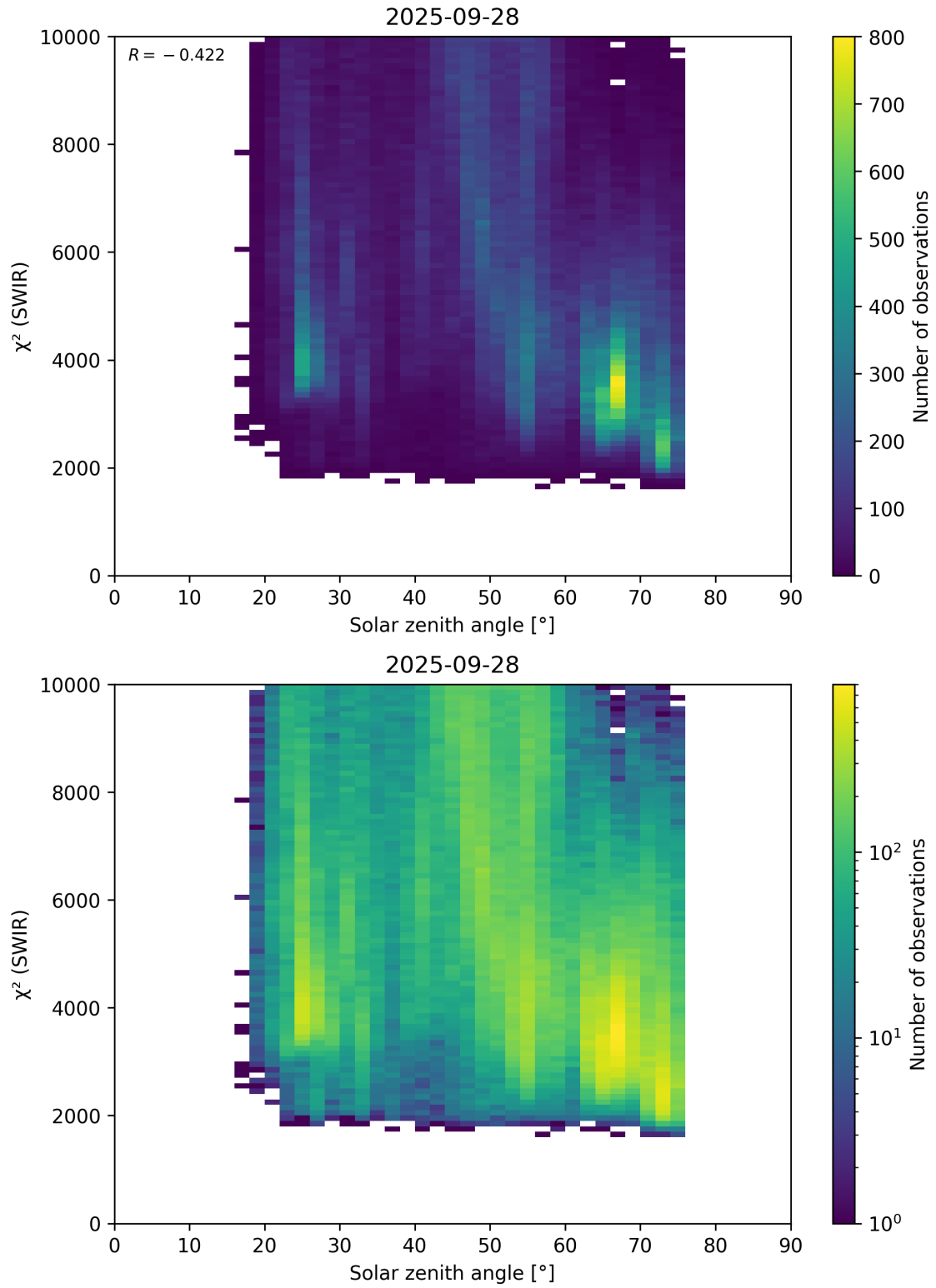
Figure 95: Scatter density plot of “Solar zenith angle” against “ \chi^2 (SWIR)” for 2025-09-27 to 2025-09-29.
