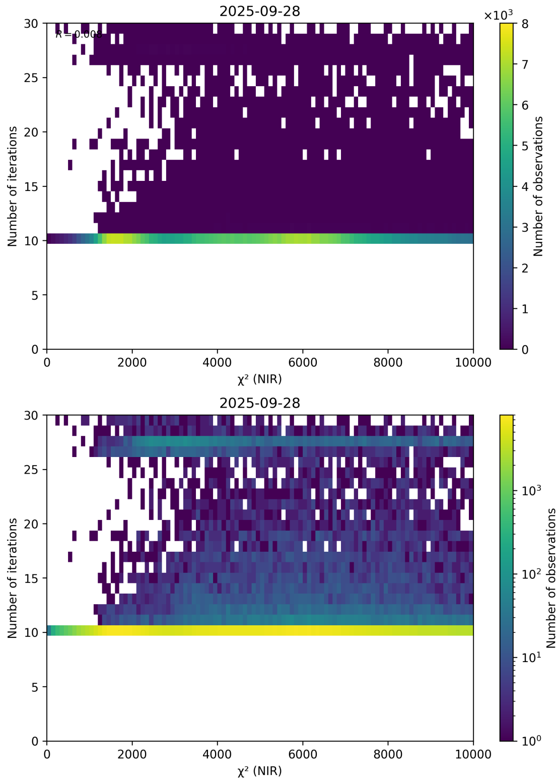
Figure 46: Scatter density plot of “ \chi^2 (NIR)” against “Number of iterations” for 2025-09-27 to 2025-09-29.
