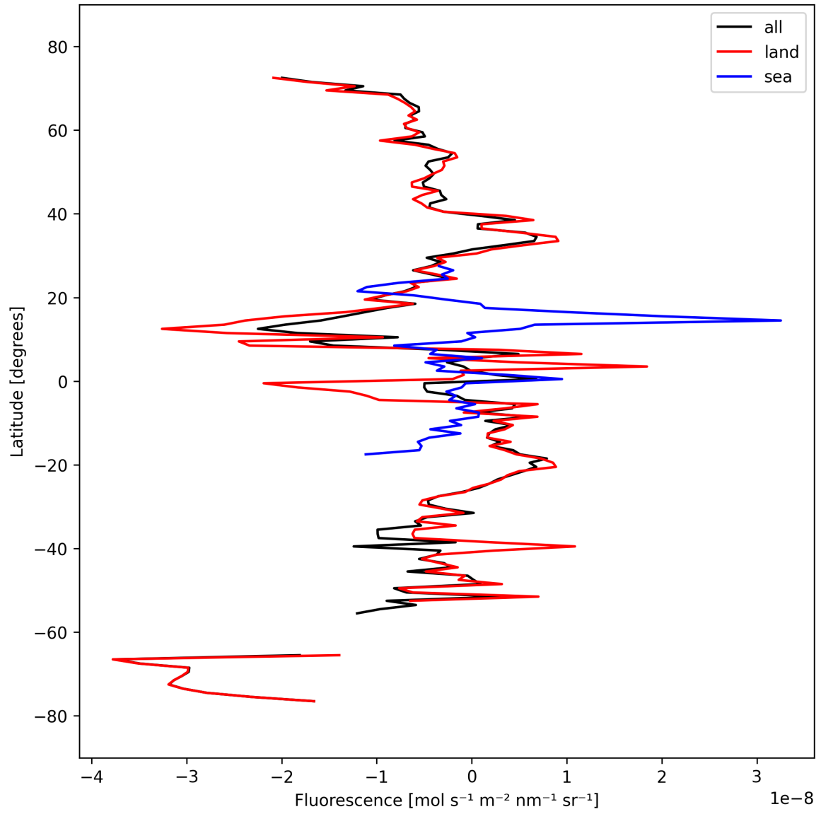
Figure 21: Zonal average of “Fluorescence” for 2025-09-27 to 2025-09-29.
