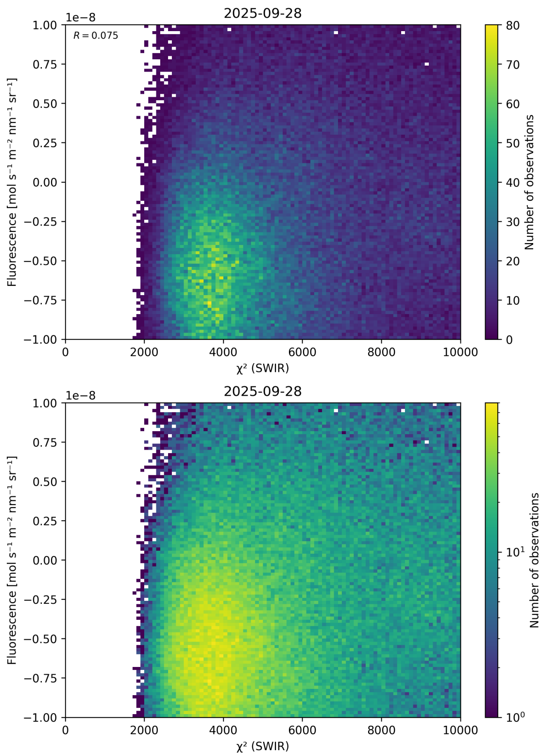
Figure 49: Scatter density plot of “ \chi^2 (SWIR)” against “Fluorescence” for 2025-09-27 to 2025-09-29.
