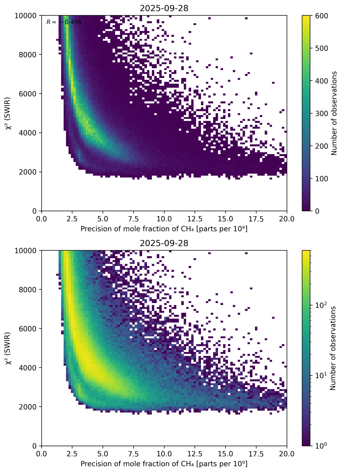
Figure 79: Scatter density plot of “Precision of mole fraction of \text{CH}_4 ” against “ \chi^2 (SWIR)” for 2025-09-27 to 2025-09-29.
