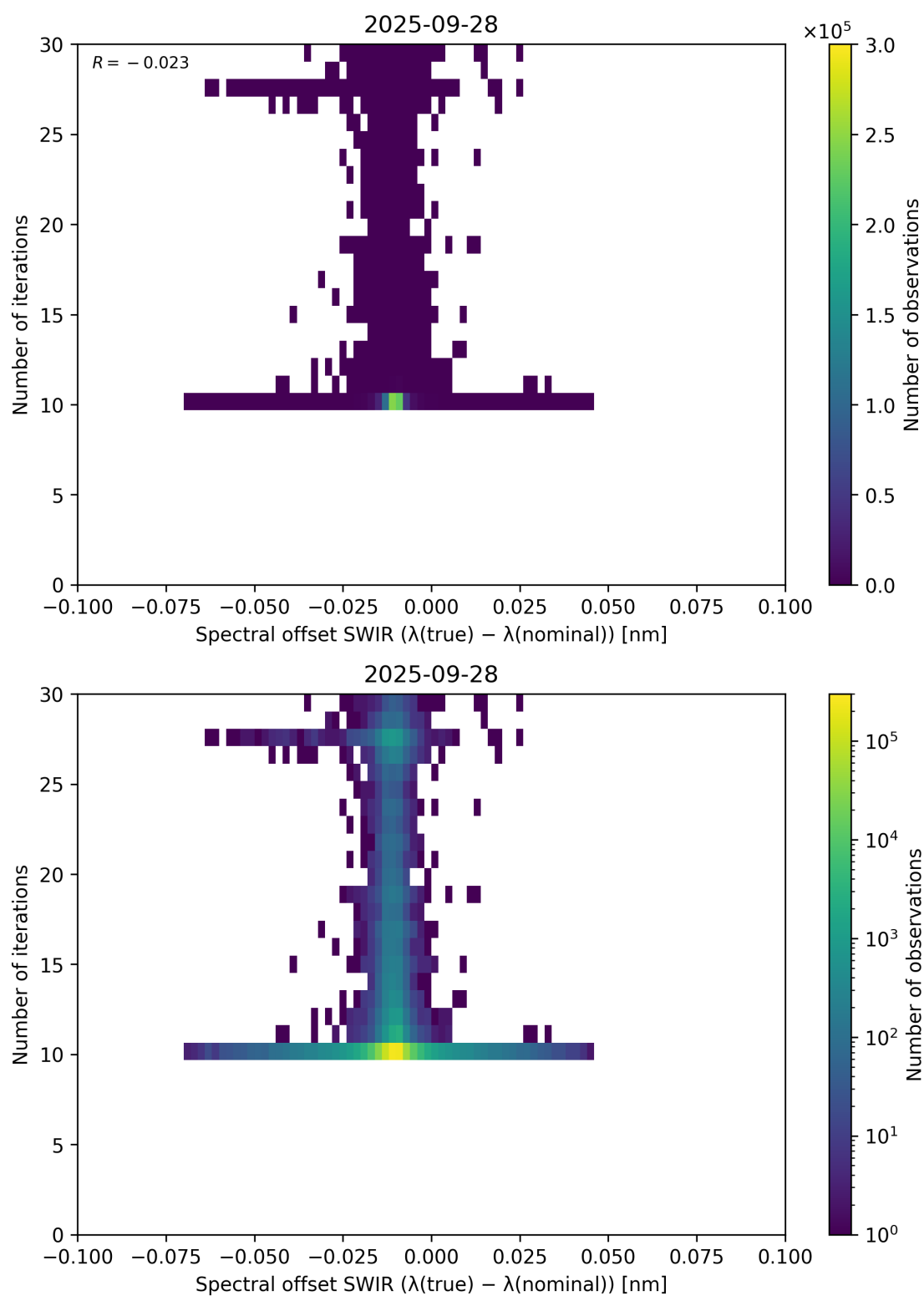
Figure 121: Scatter density plot of “Spectral offset SWIR ( \lambda_{\text{true}} - \lambda_{\text{nominal}} )” against “Number of iterations” for 2025-09-27 to 2025-09-29.
