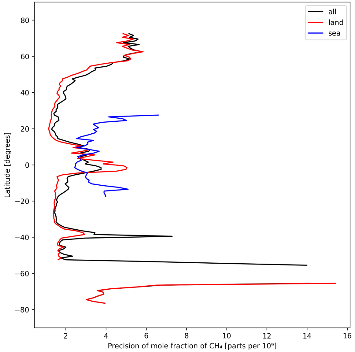
Figure 13: Zonal average of “Precision of mole fraction of CH 4 ” for 2025-09-27 to 2025-09-29.
