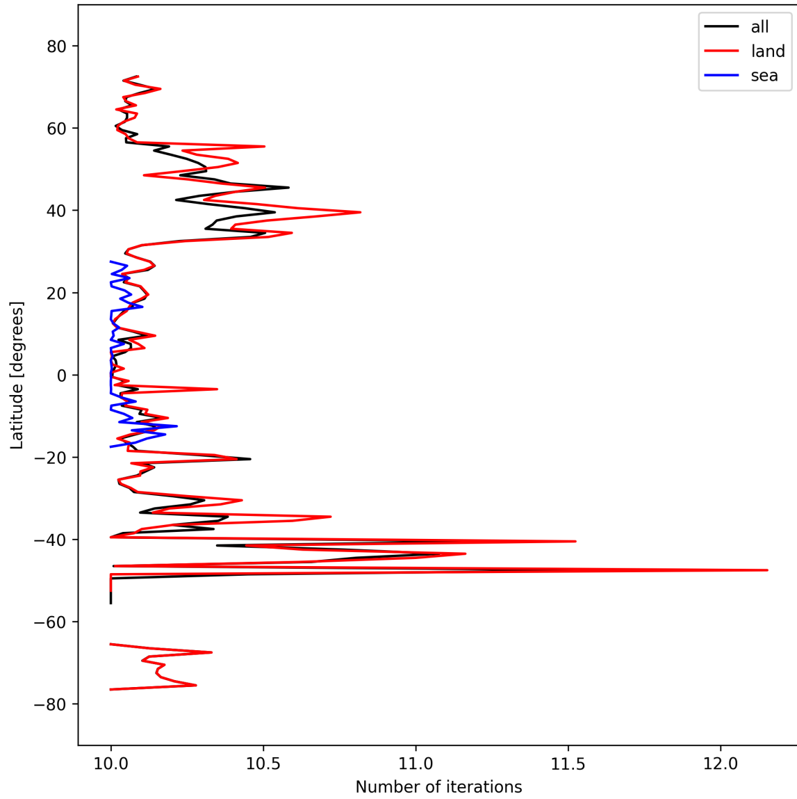
Figure 20: Zonal average of “Number of iterations” for 2025-09-27 to 2025-09-29.
