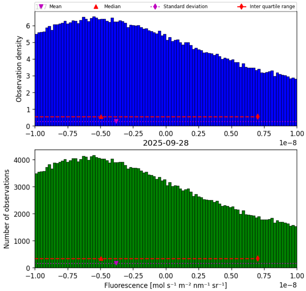
Figure 32: Histogram of “Fluorescence” for 2025-09-27 to 2025-09-29
