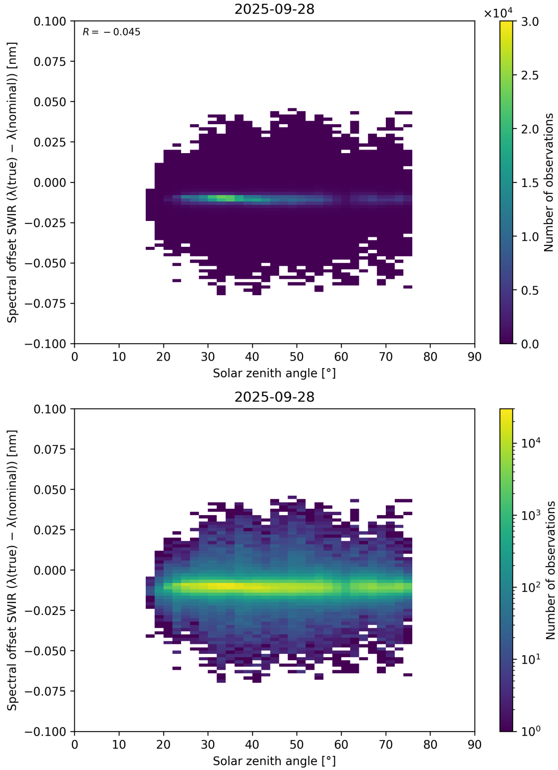
Figure 104: Scatter density plot of “Solar zenith angle” against “Spectral offset SWIR ( \lambda_{\text{true}} - \lambda_{\text{nominal}} )” for 2025-09-27 to 2025-09-29.
