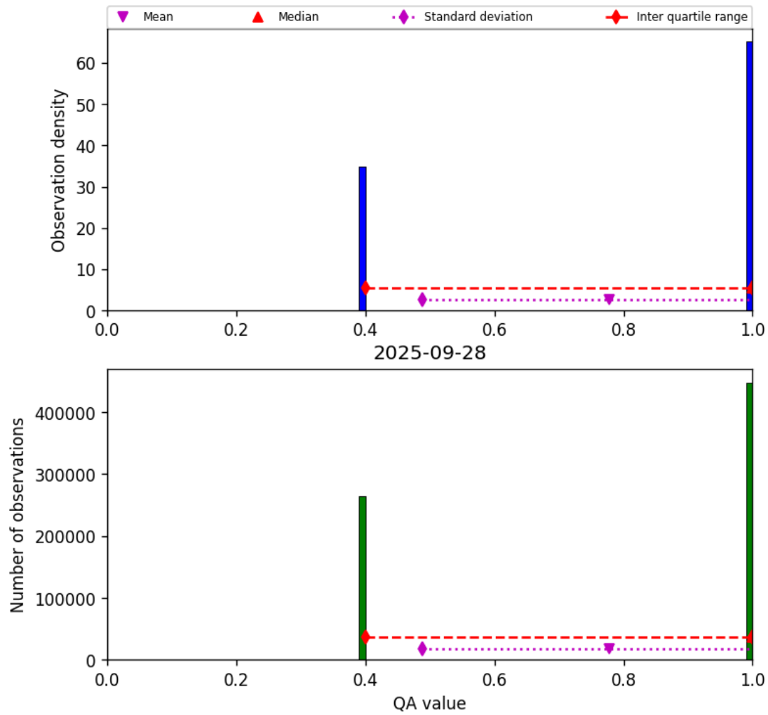
Figure 22: Histogram of “QA value” for 2025-09-27 to 2025-09-29
