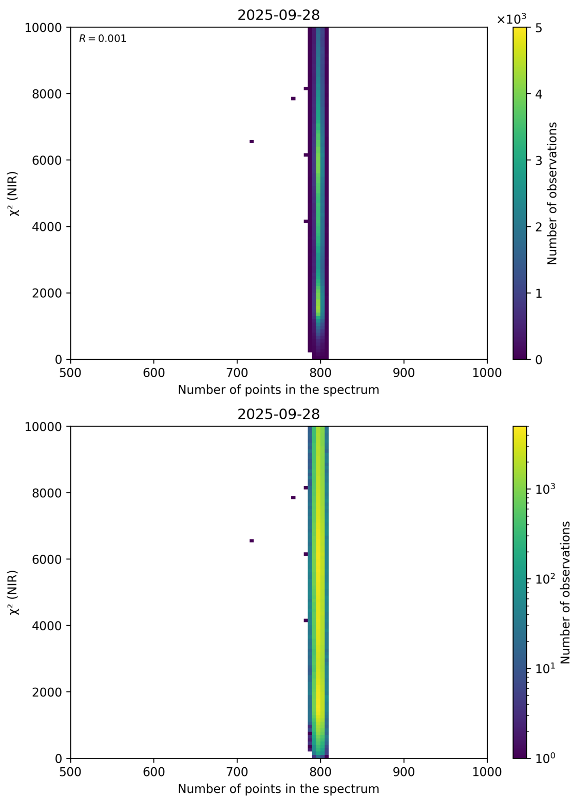
Figure 88: Scatter density plot of “Number of points in the spectrum” against “ \chi^2 (NIR)” for 2025-09-27 to 2025-09-29.
