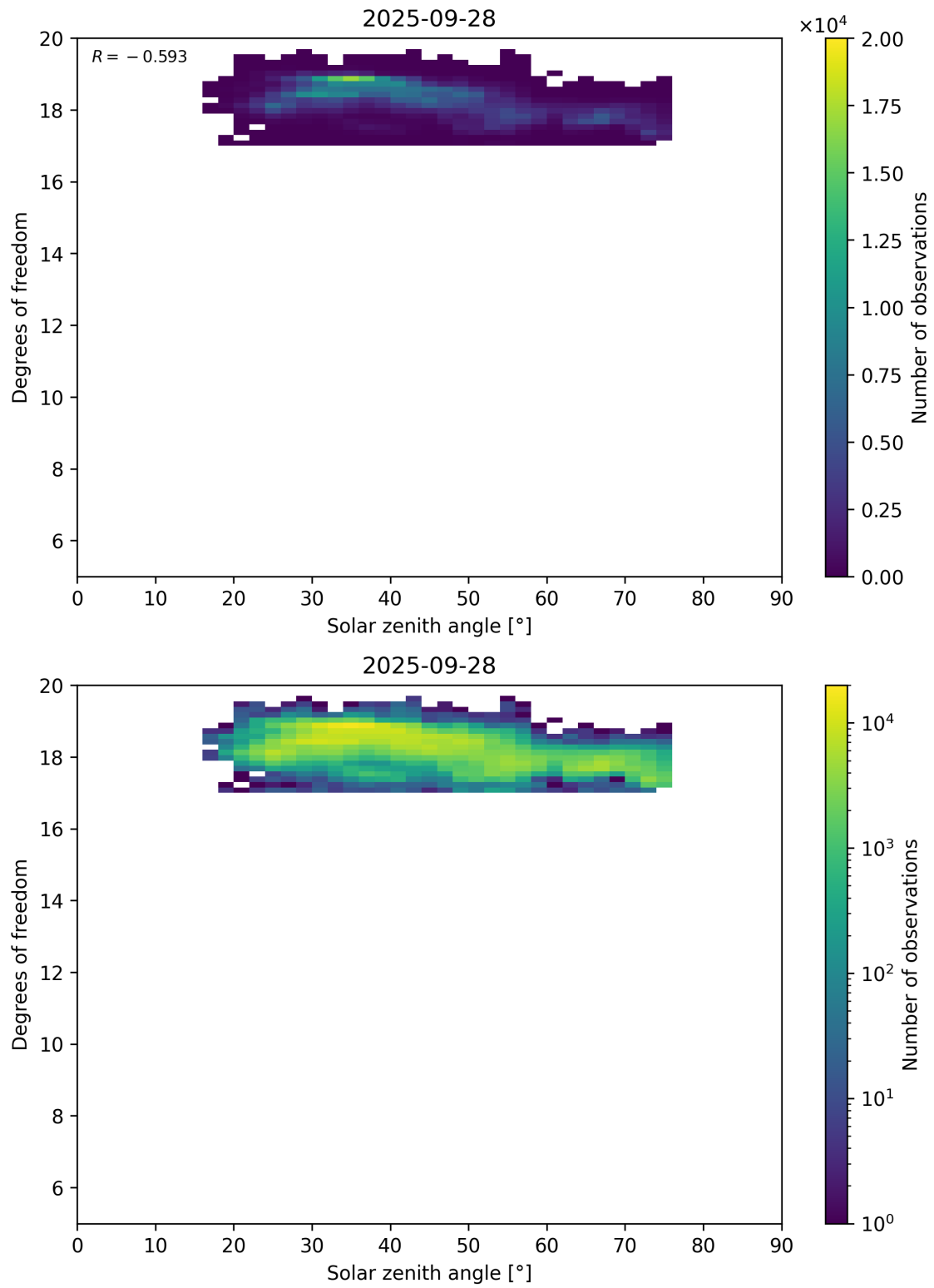
Figure 96: Scatter density plot of “Solar zenith angle” against “Degrees of freedom” for 2025-09-27 to 2025-09-29.
