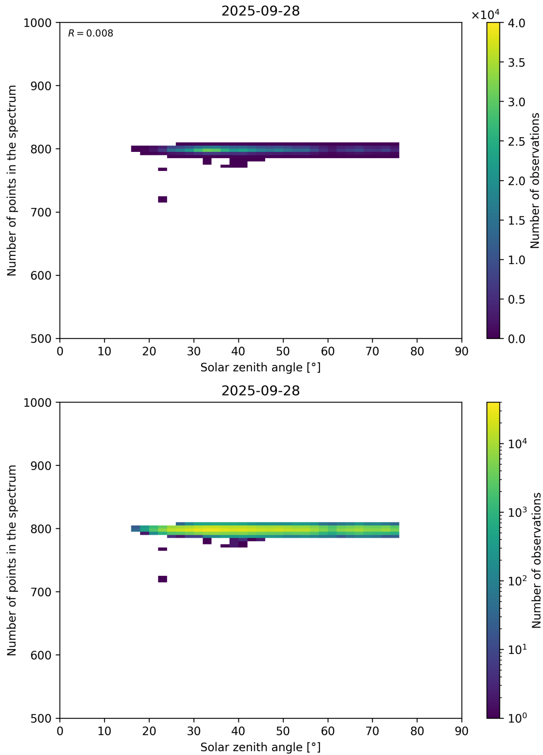
Figure 103: Scatter density plot of “Solar zenith angle” against “Number of points in the spectrum” for 2025-09-27 to 2025-09-29.
