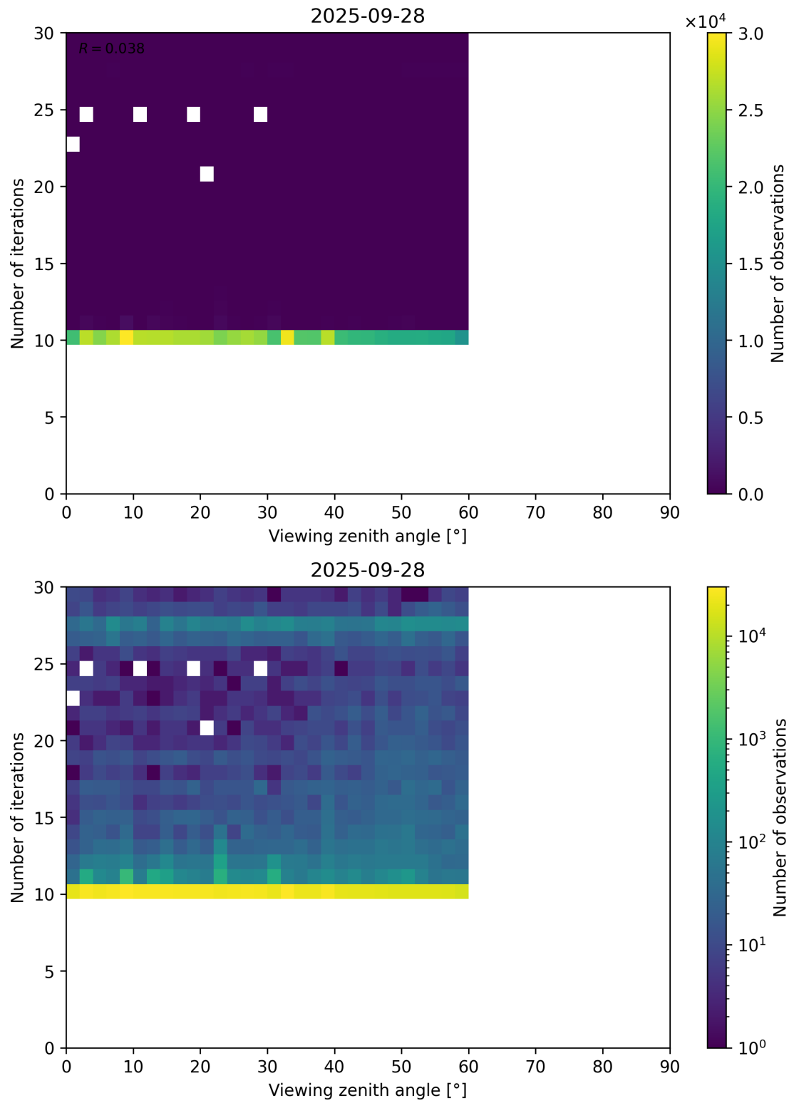
Figure 113: Scatter density plot of “Viewing zenith angle” against “Number of iterations” for 2025-09-27 to 2025-09-29.
