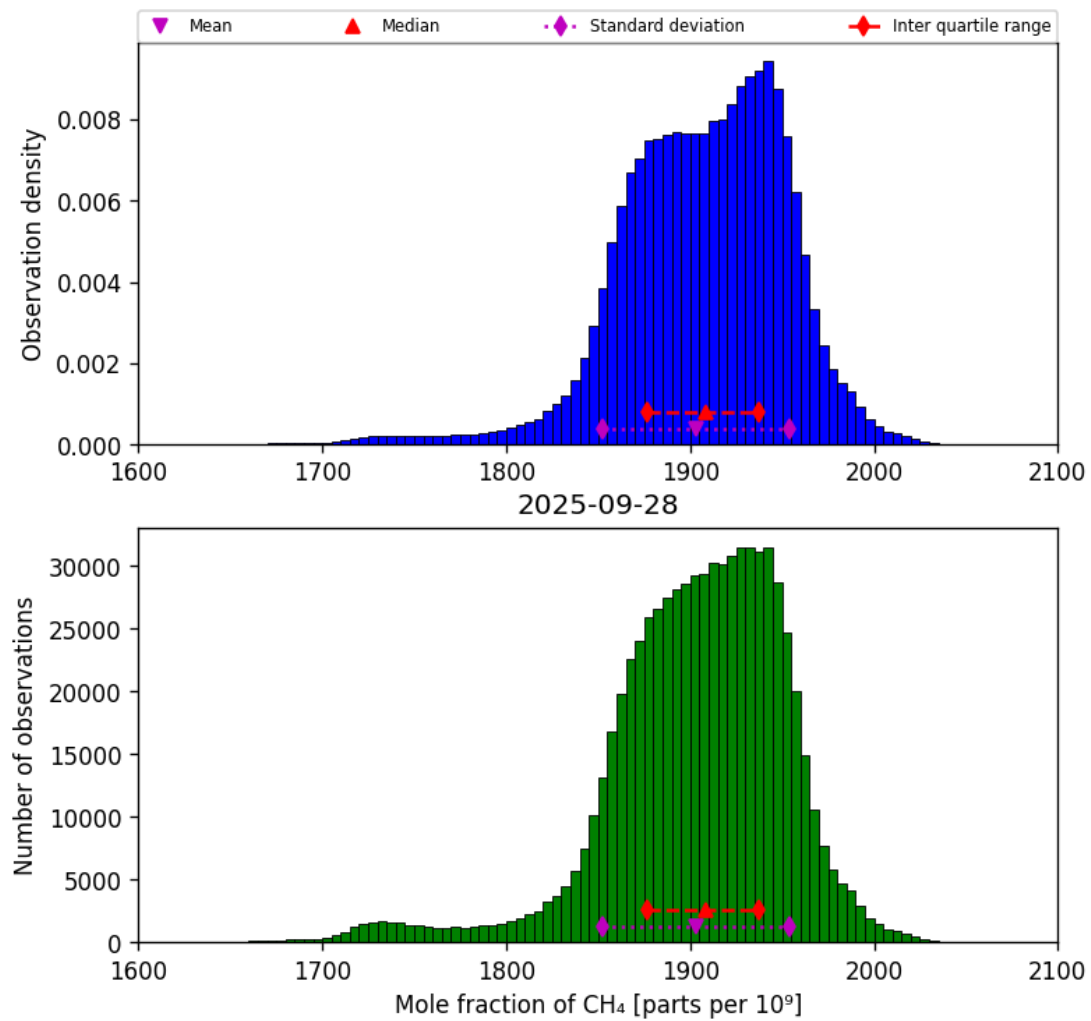
Figure 23: Histogram of “Mole fraction of CH 4 ” for 2025-09-27 to 2025-09-29
