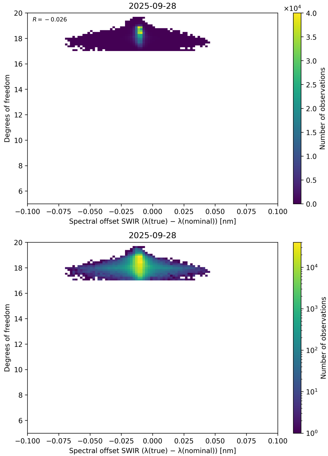
Figure 119: Scatter density plot of “Spectral offset SWIR ( \lambda_{\text{true}} - \lambda_{\text{nominal}} )” against “Degrees of freedom” for 2025-09-27 to 2025-09-29.
