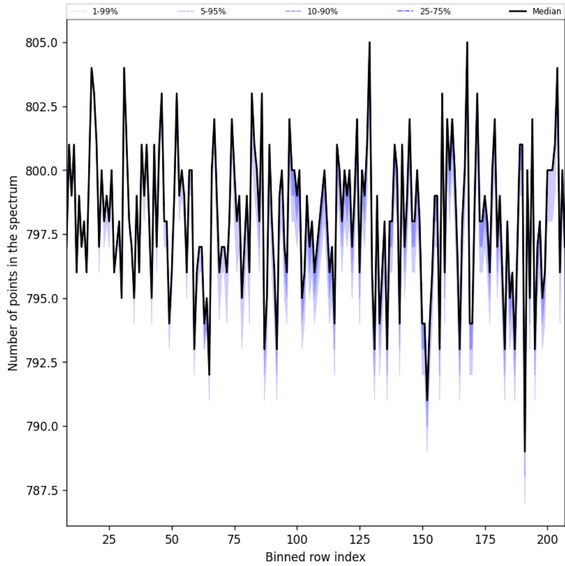
Figure 37: Along track statistics of “Number of points in the spectrum” for 2025-09-27 to 2025-09-29
