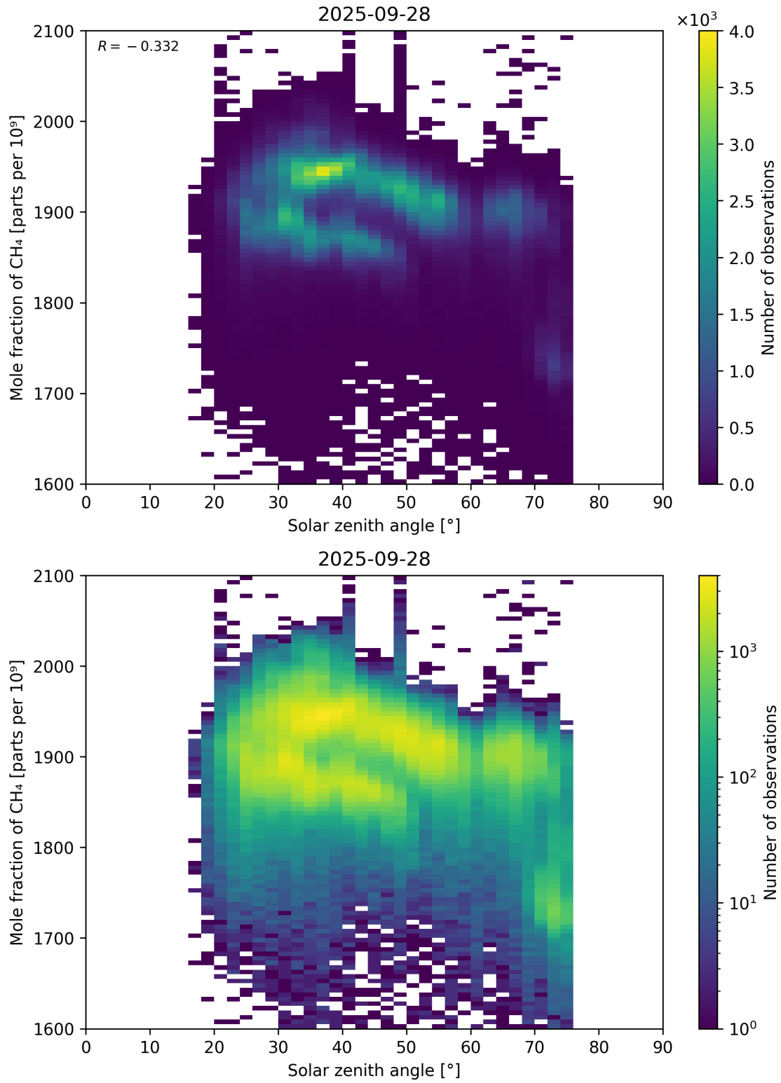
Figure 99: Scatter density plot of “Solar zenith angle” against “Mole fraction of CH 4 ” for 2025-09-27 to 2025-09-29.
