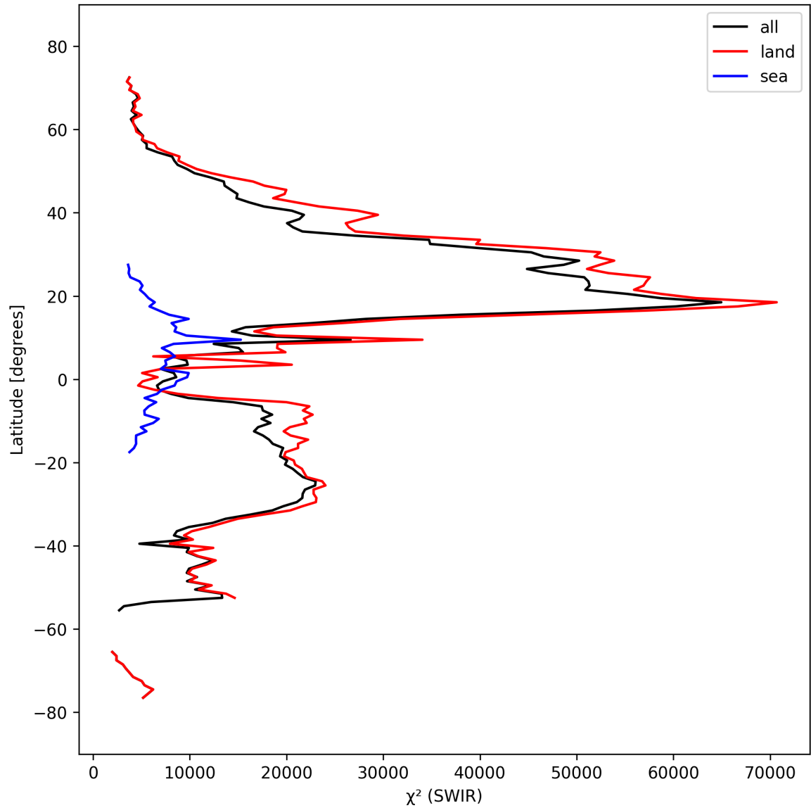
Figure 17: Zonal average of “ \chi^2 (SWIR)” for 2025-09-27 to 2025-09-29.
