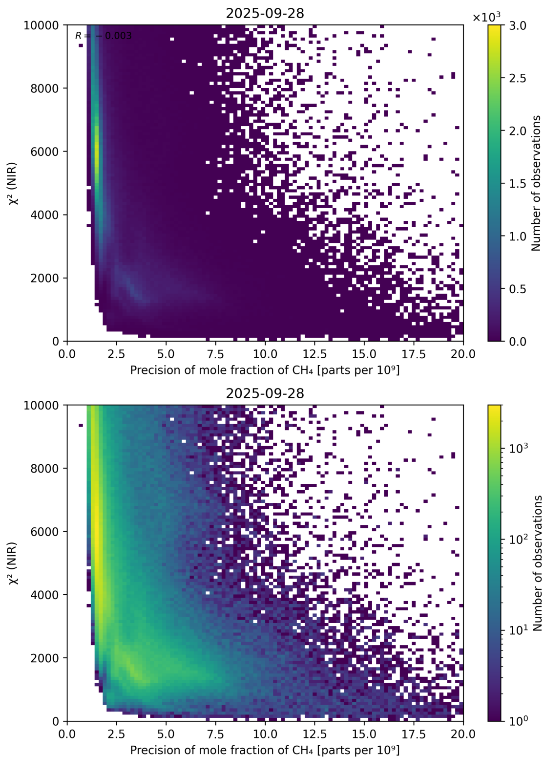
Figure 78: Scatter density plot of “Precision of mole fraction of CH 4 ” against “ \chi^2 (NIR)” for 2025-09-27 to 2025-09-29.
