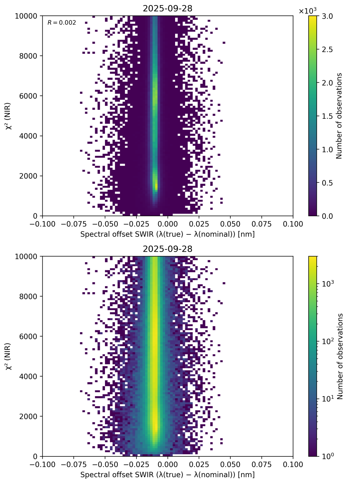
Figure 117: Scatter density plot of “Spectral offset SWIR ( \lambda_{\text{true}} - \lambda_{\text{nominal}} )” against “ \chi^2 (NIR)” for 2025-09-27 to 2025-09-29.
