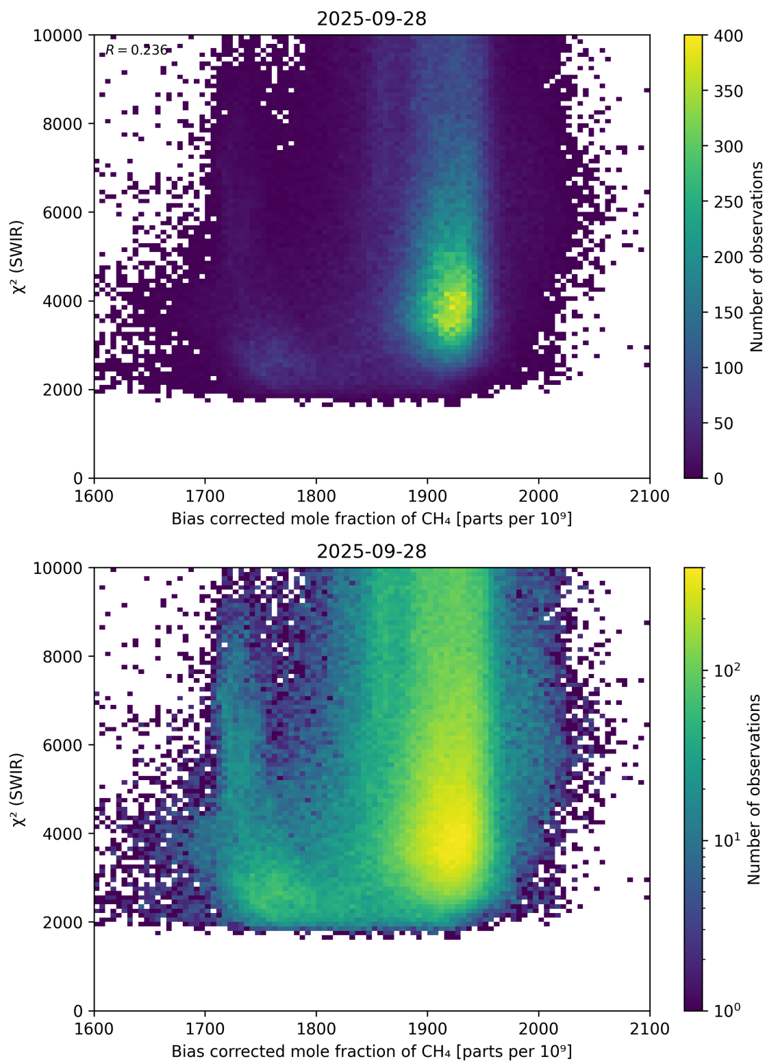
Figure 64: Scatter density plot of “Bias corrected mole fraction of \text{CH}_4 ” against “ \chi^2 (SWIR)” for 2025-09-27 to 2025-09-29.
