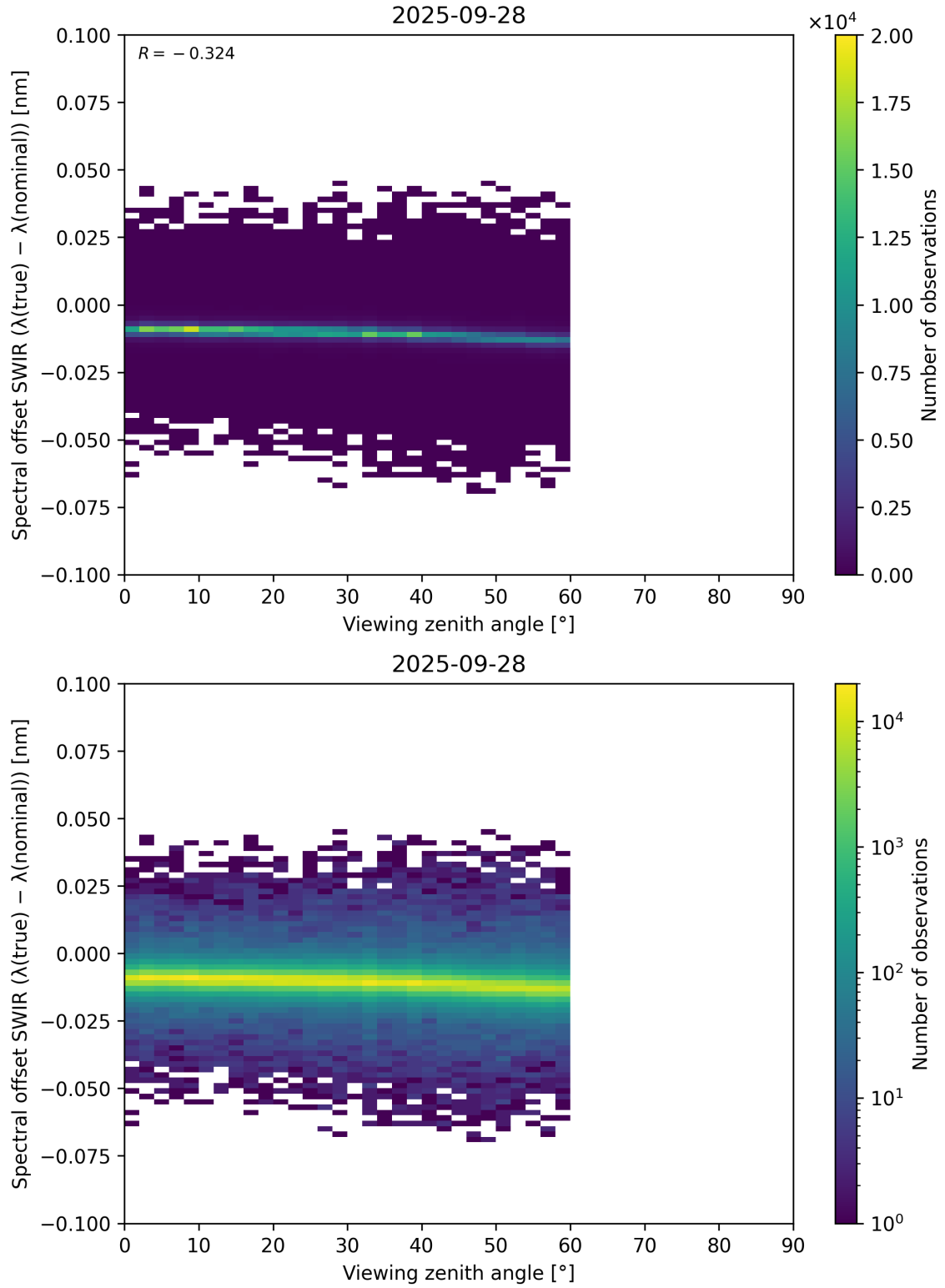
Figure 116: Scatter density plot of “Viewing zenith angle” against “Spectral offset SWIR ( \lambda_{\text{true}} - \lambda_{\text{nominal}} )” for 2025-09-27 to 2025-09-29.
