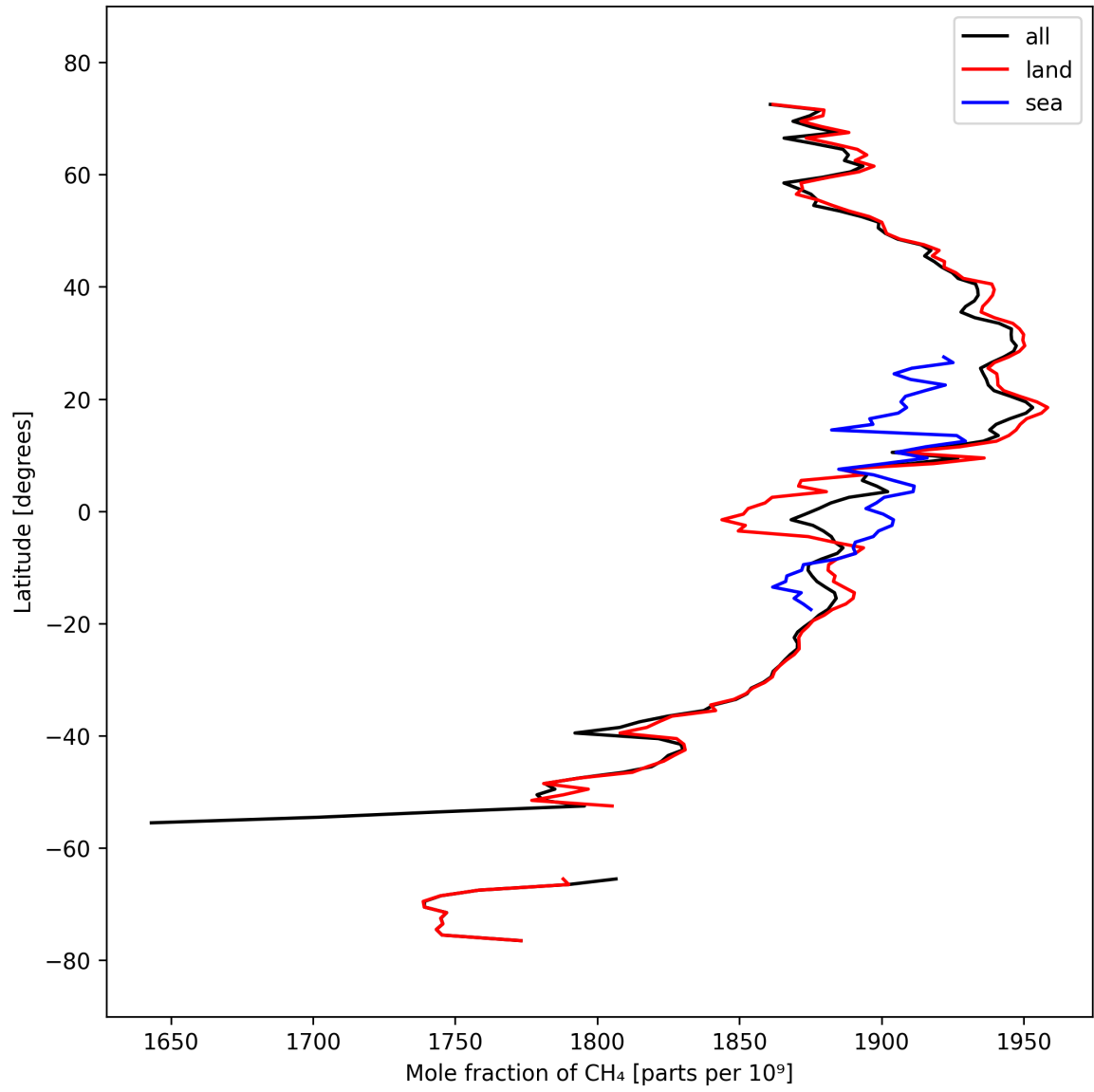
Figure 12: Zonal average of “Mole fraction of CH 4 ” for 2025-09-27 to 2025-09-29.
