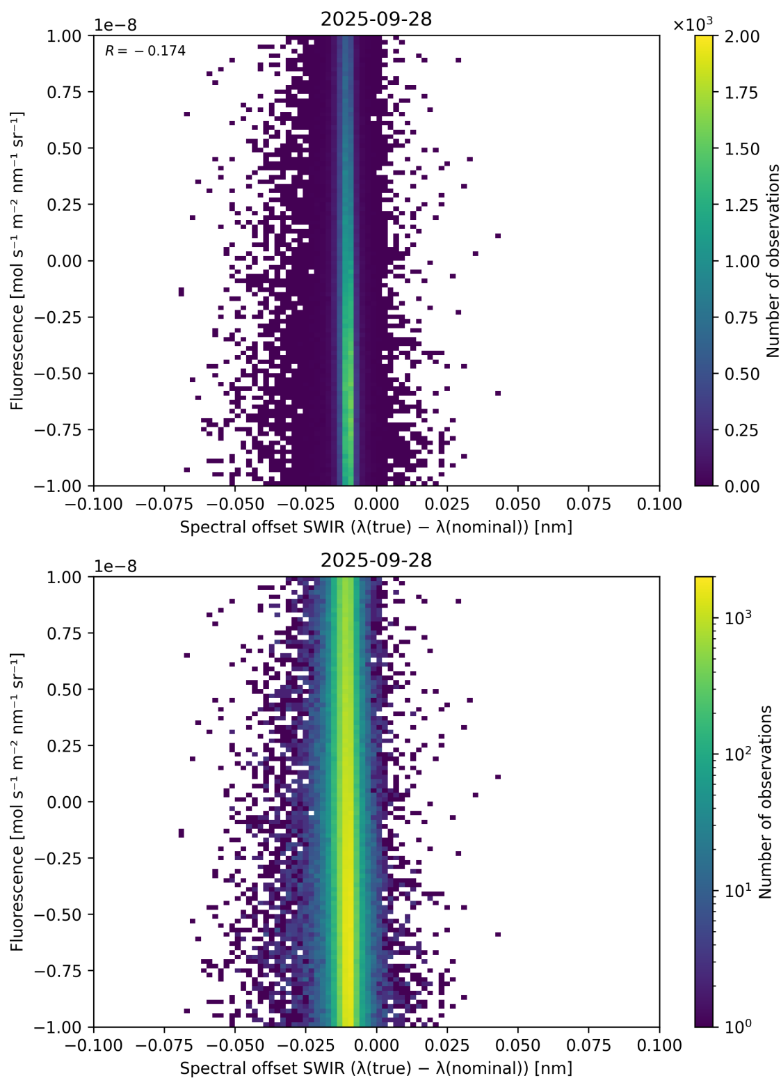
Figure 120: Scatter density plot of “Spectral offset SWIR ( \lambda_{\text{true}} - \lambda_{\text{nominal}} )” against “Fluorescence” for 2025-09-27 to 2025-09-29.
