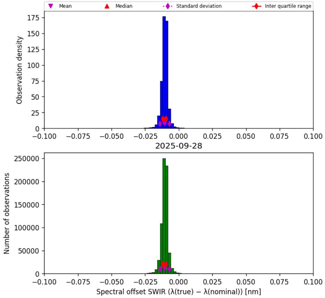
Figure 27: Histogram of “Spectral offset SWIR ( \lambda_{\text{true}} - \lambda_{\text{nominal}} )” for 2025-09-27 to 2025-09-29
