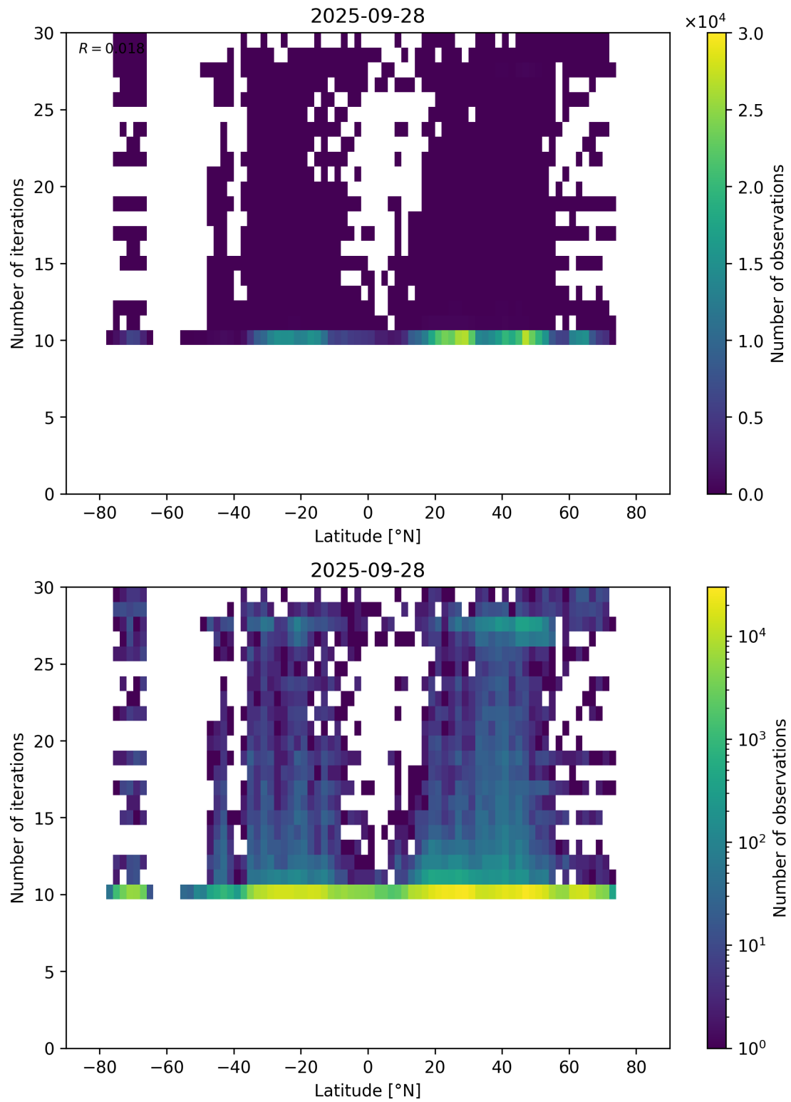
Figure 60: Scatter density plot of “Latitude” against “Number of iterations” for 2025-09-27 to 2025-09-29.
