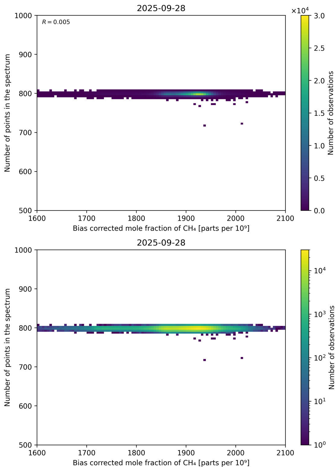
Figure 68: Scatter density plot of “Bias corrected mole fraction of CH 4 ” against “Number of points in the spectrum” for 2025-09-27 to 2025-09-29.
