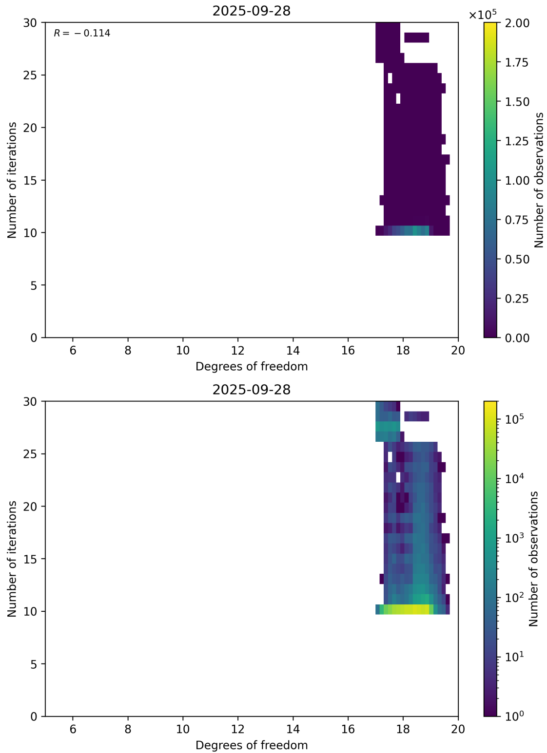
Figure 52: Scatter density plot of “Degrees of freedom” against “Number of iterations” for 2025-09-27 to 2025-09-29.
