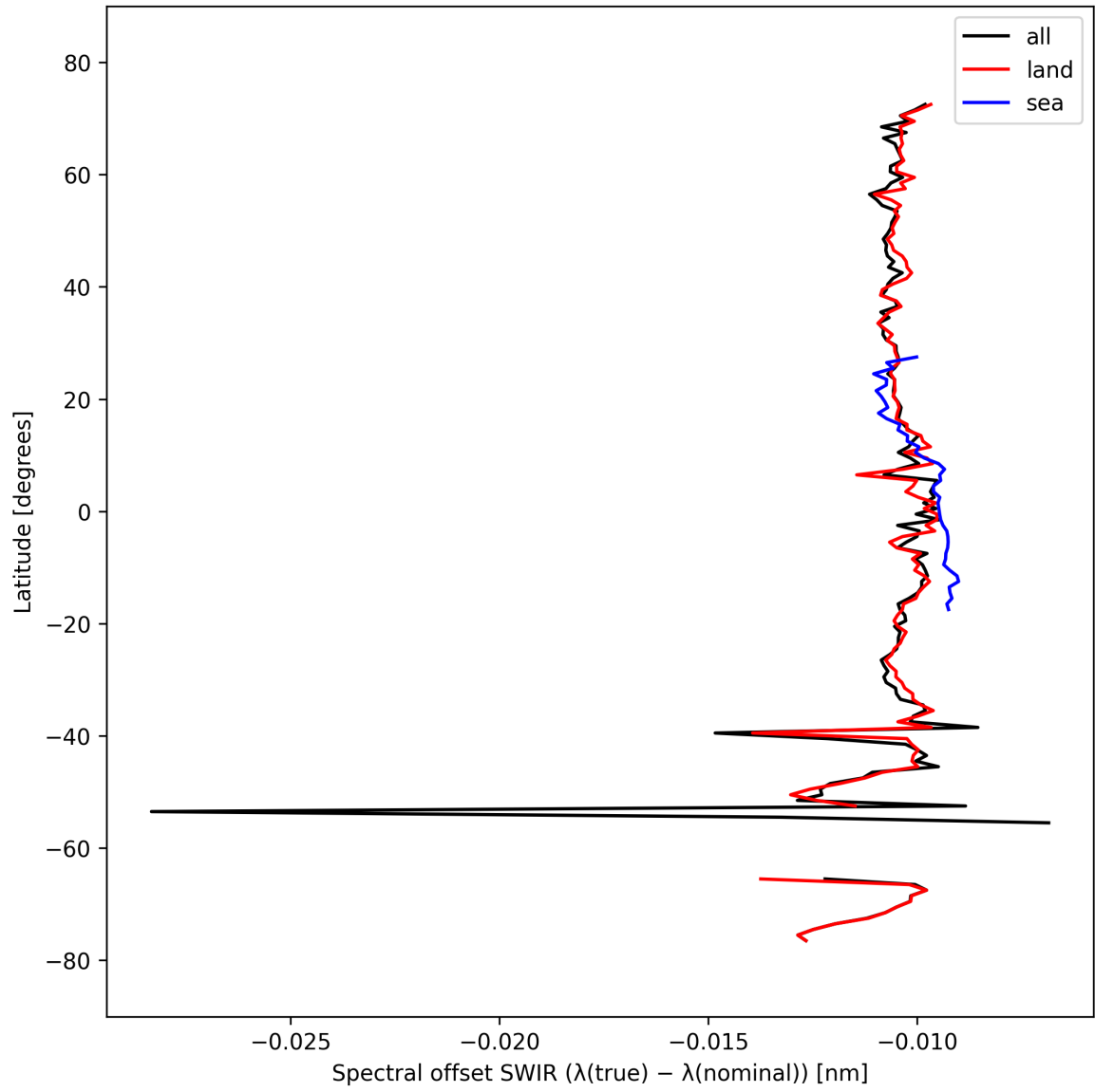
Figure 16: Zonal average of “Spectral offset SWIR ( \lambda_{\text{true}} - \lambda_{\text{nominal}} )” for 2025-09-27 to 2025-09-29.
