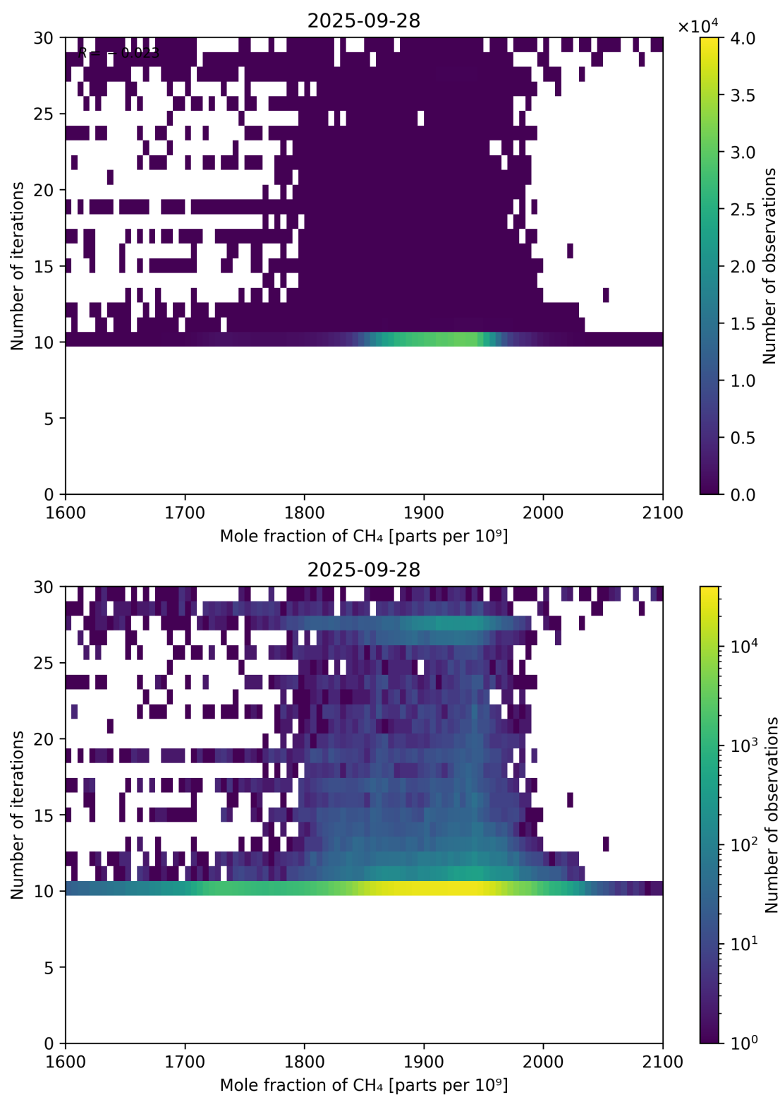
Figure 76: Scatter density plot of “Mole fraction of CH 4 ” against “Number of iterations” for 2025-09-27 to 2025-09-29.
