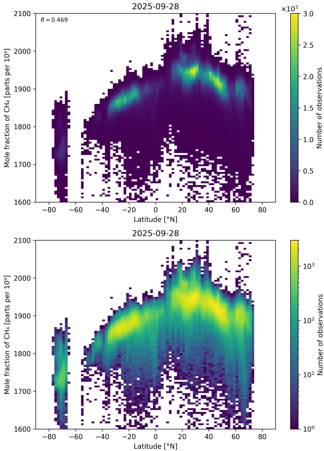
Figure 57: Scatter density plot of “Latitude” against “Mole fraction of CH 4 ” for 2025-09-27 to 2025-09-29.
