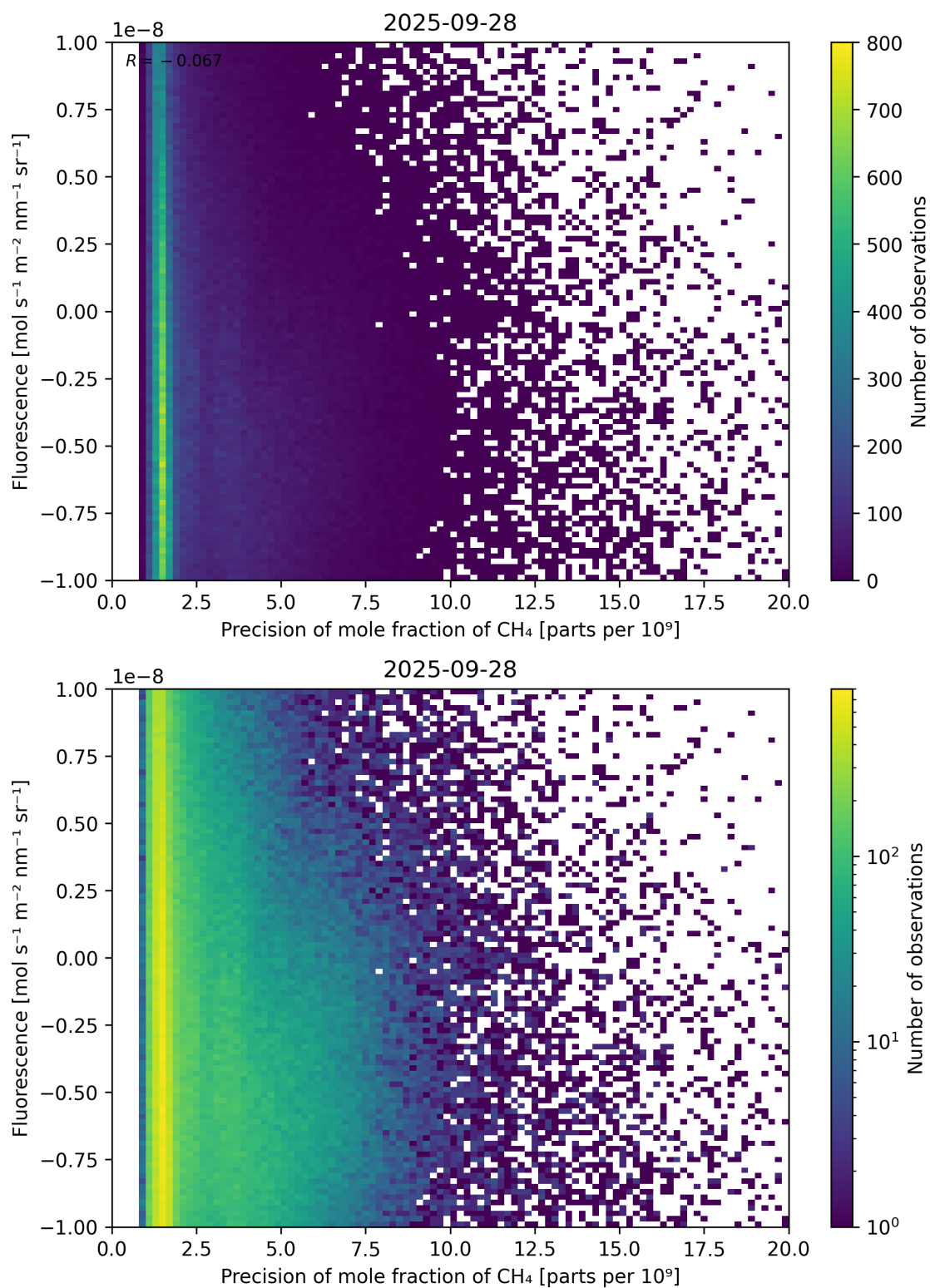
Figure 81: Scatter density plot of “Precision of mole fraction of \text{CH}_4 ” against “Fluorescence” for 2025-09-27 to 2025-09-29.
