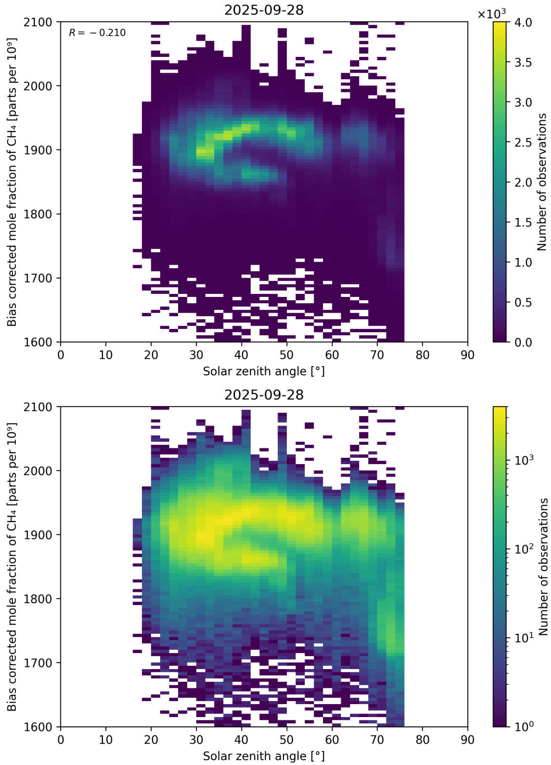
Figure 100: Scatter density plot of “Solar zenith angle” against “Bias corrected mole fraction of \text{CH}_4 ” for 2025-09-27 to 2025-09-29.
