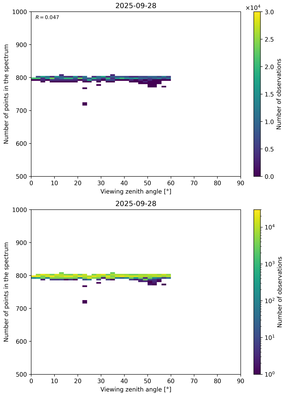
Figure 114: Scatter density plot of “Viewing zenith angle” against “Number of points in the spectrum” for 2025-09-27 to 2025-09-29.
