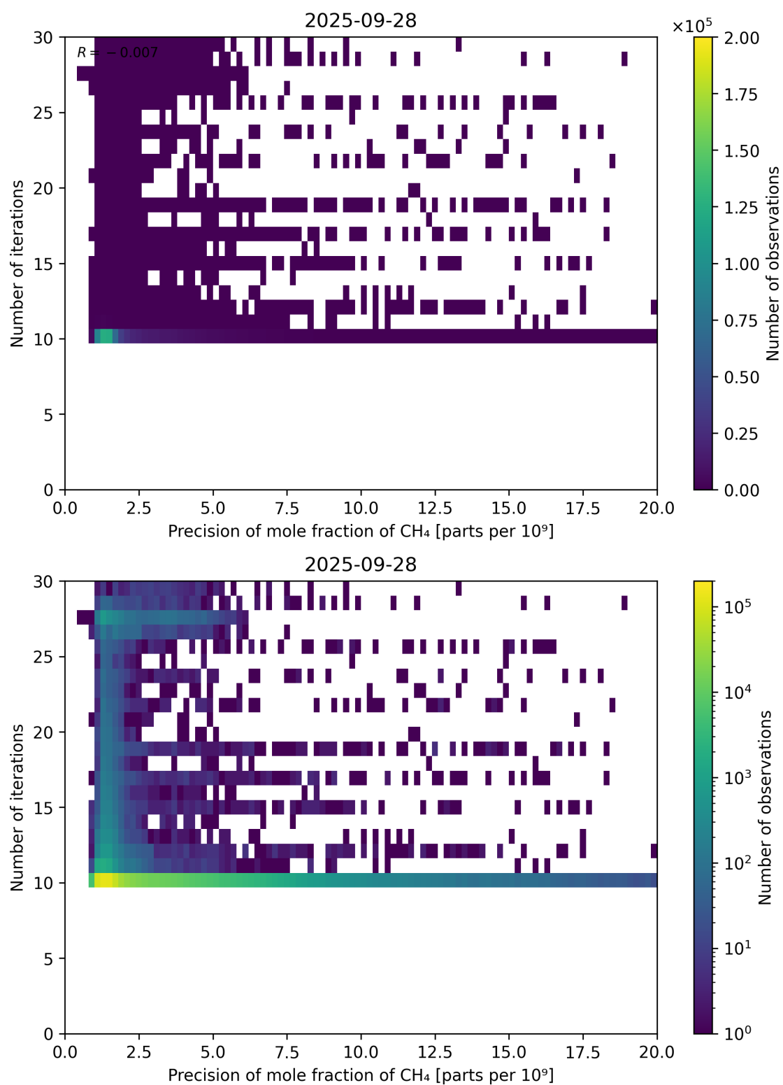
Figure 83: Scatter density plot of “Precision of mole fraction of CH 4 ” against “Number of iterations” for 2025-09-27 to 2025-09-29.
