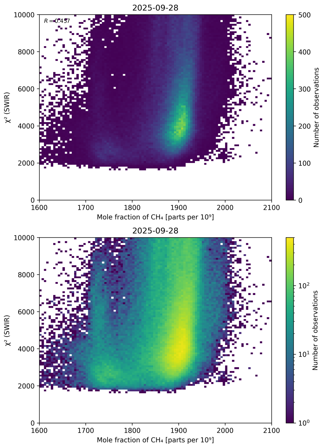
Figure 71: Scatter density plot of “Mole fraction of CH 4 ” against “ \chi^2 (SWIR)” for 2025-09-27 to 2025-09-29.
