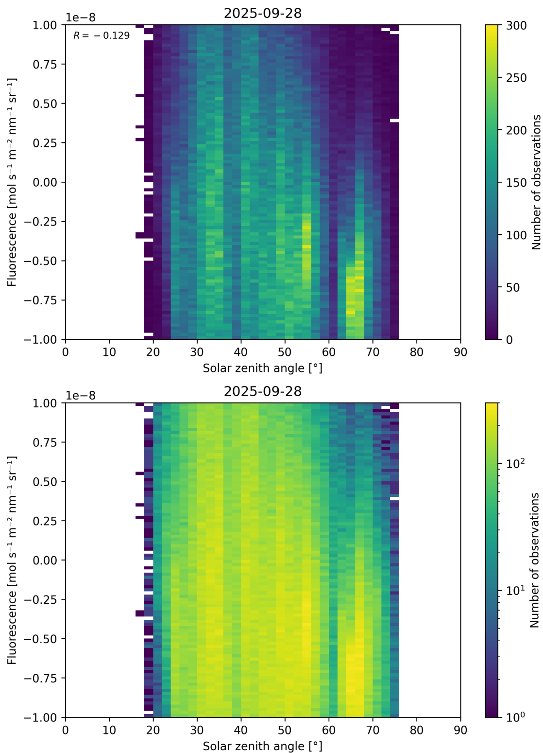
Figure 97: Scatter density plot of “Solar zenith angle” against “Fluorescence” for 2025-09-27 to 2025-09-29.
