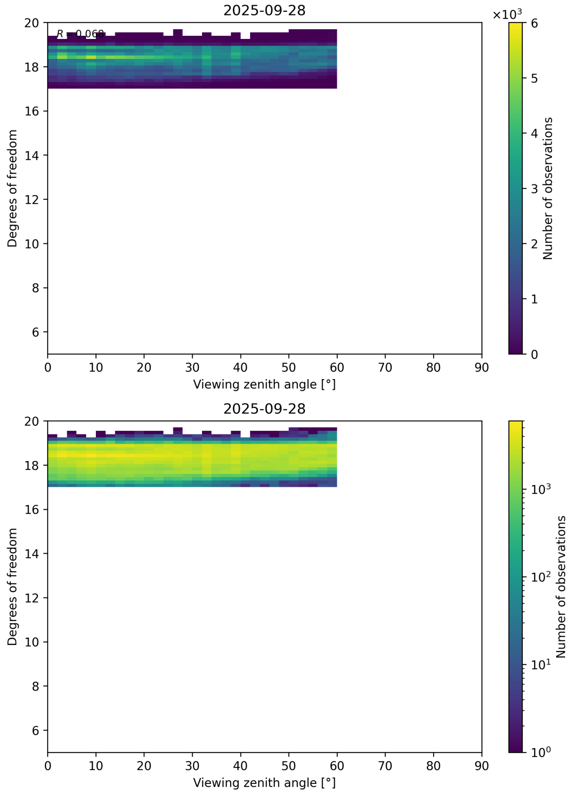
Figure 107: Scatter density plot of “Viewing zenith angle” against “Degrees of freedom” for 2025-09-27 to 2025-09-29.
