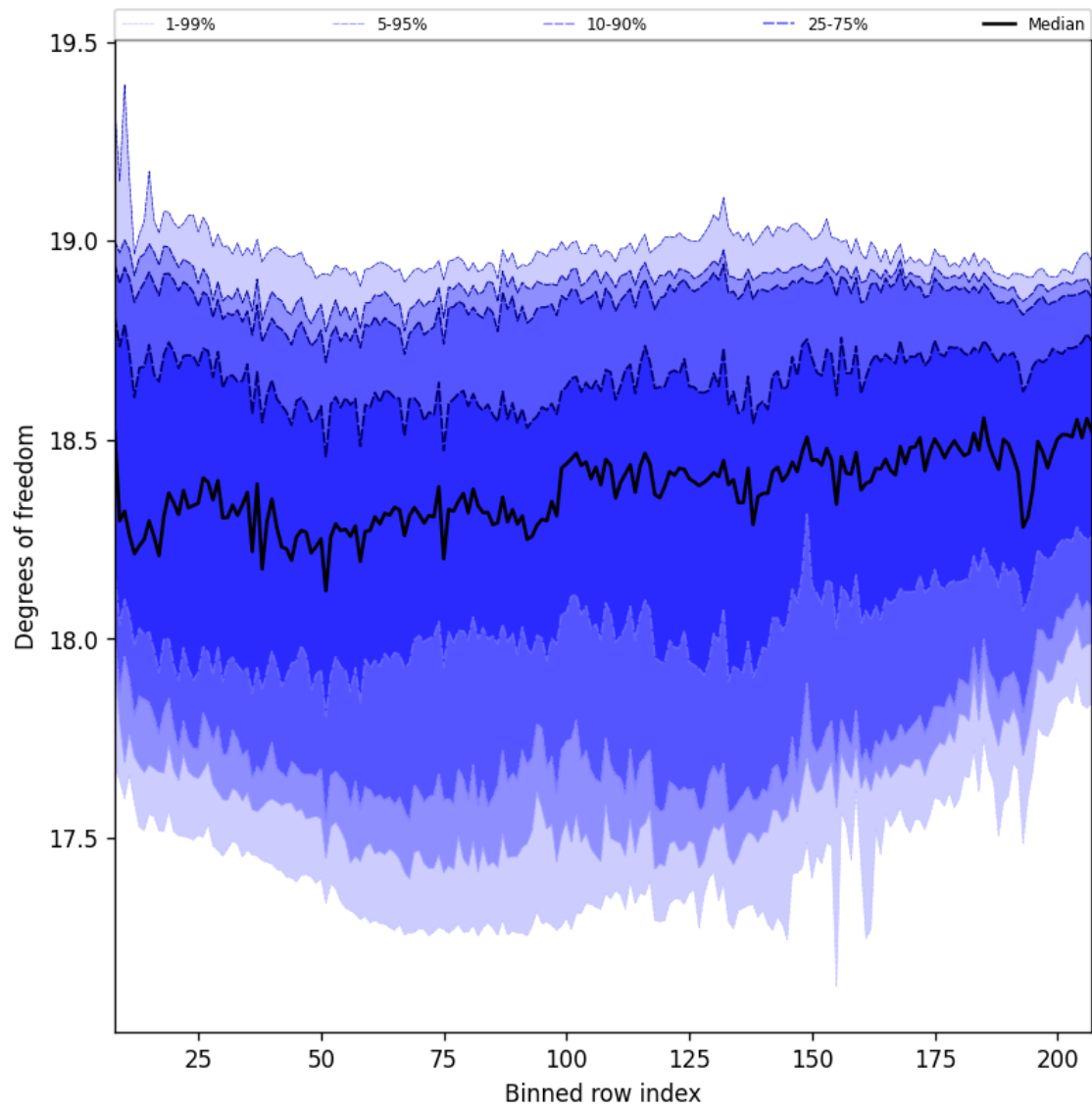
Figure 41: Along track statistics of “Degrees of freedom” for 2025-09-27 to 2025-09-29
