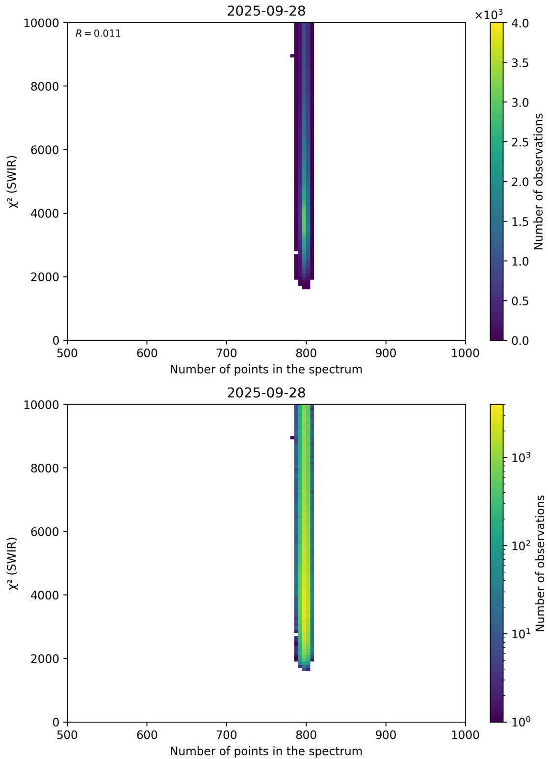
Figure 89: Scatter density plot of “Number of points in the spectrum” against “ \chi^2 (SWIR)” for 2025-09-27 to 2025-09-29.
