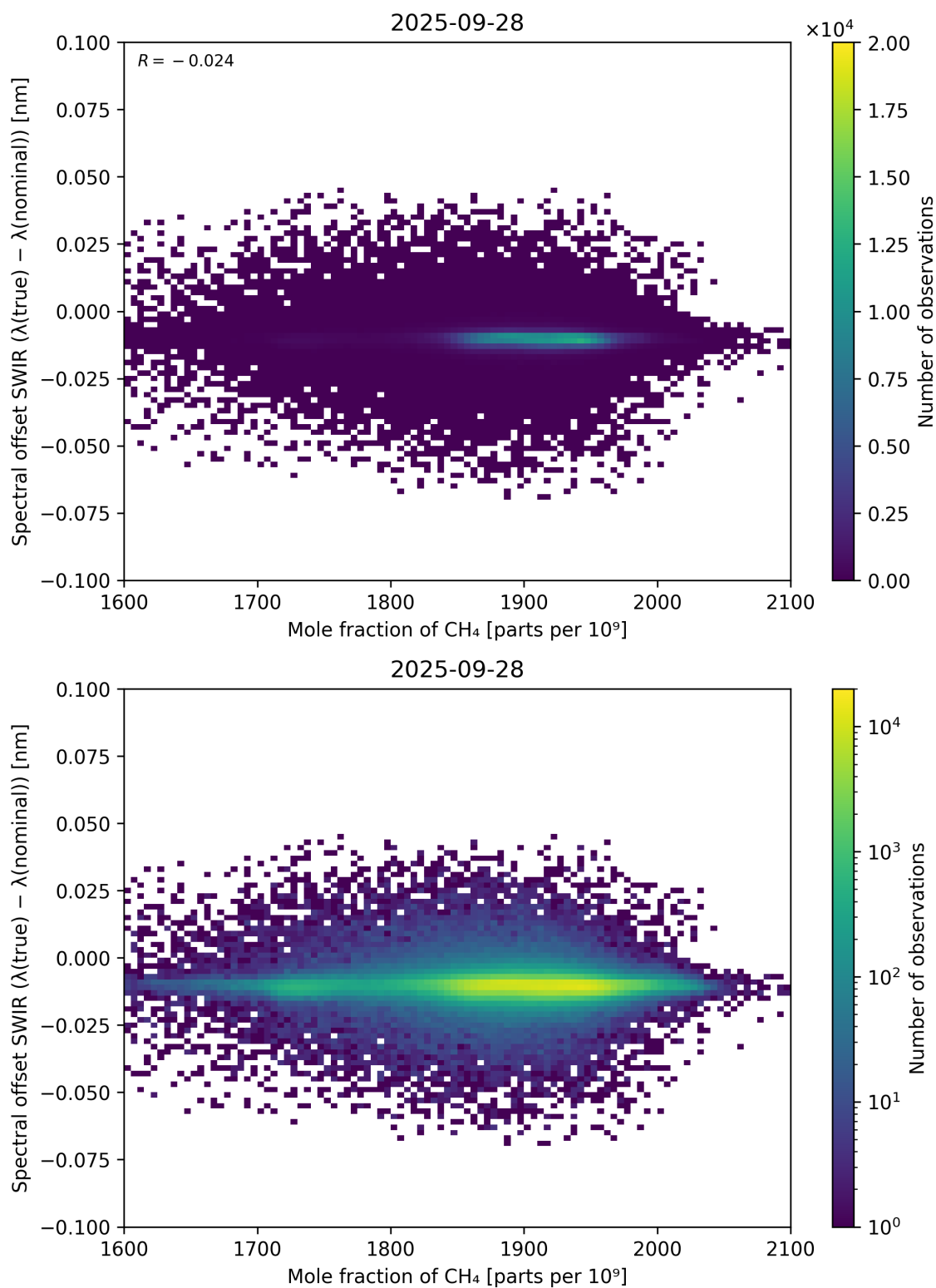
Figure 86: Scatter density plot of “Mole fraction of CH 4 ” against “Spectral offset SWIR ( \lambda_{\text{true}} - \lambda_{\text{nominal}} )” for 2025-09-27 to 2025-09-29.
