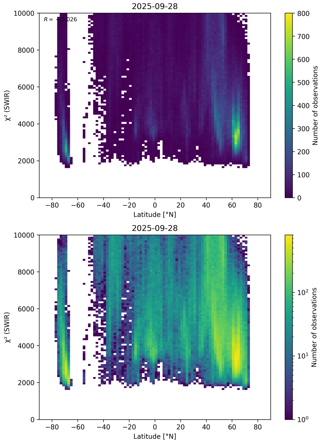
Figure 54: Scatter density plot of “Latitude” against “ \chi^2 (SWIR)” for 2025-09-27 to 2025-09-29.
