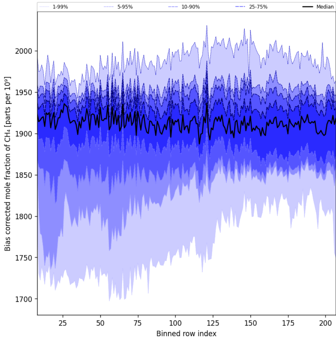
Figure 36: Along track statistics of “Bias corrected mole fraction of CH 4 ” for 2025-09-27 to 2025-09-29
