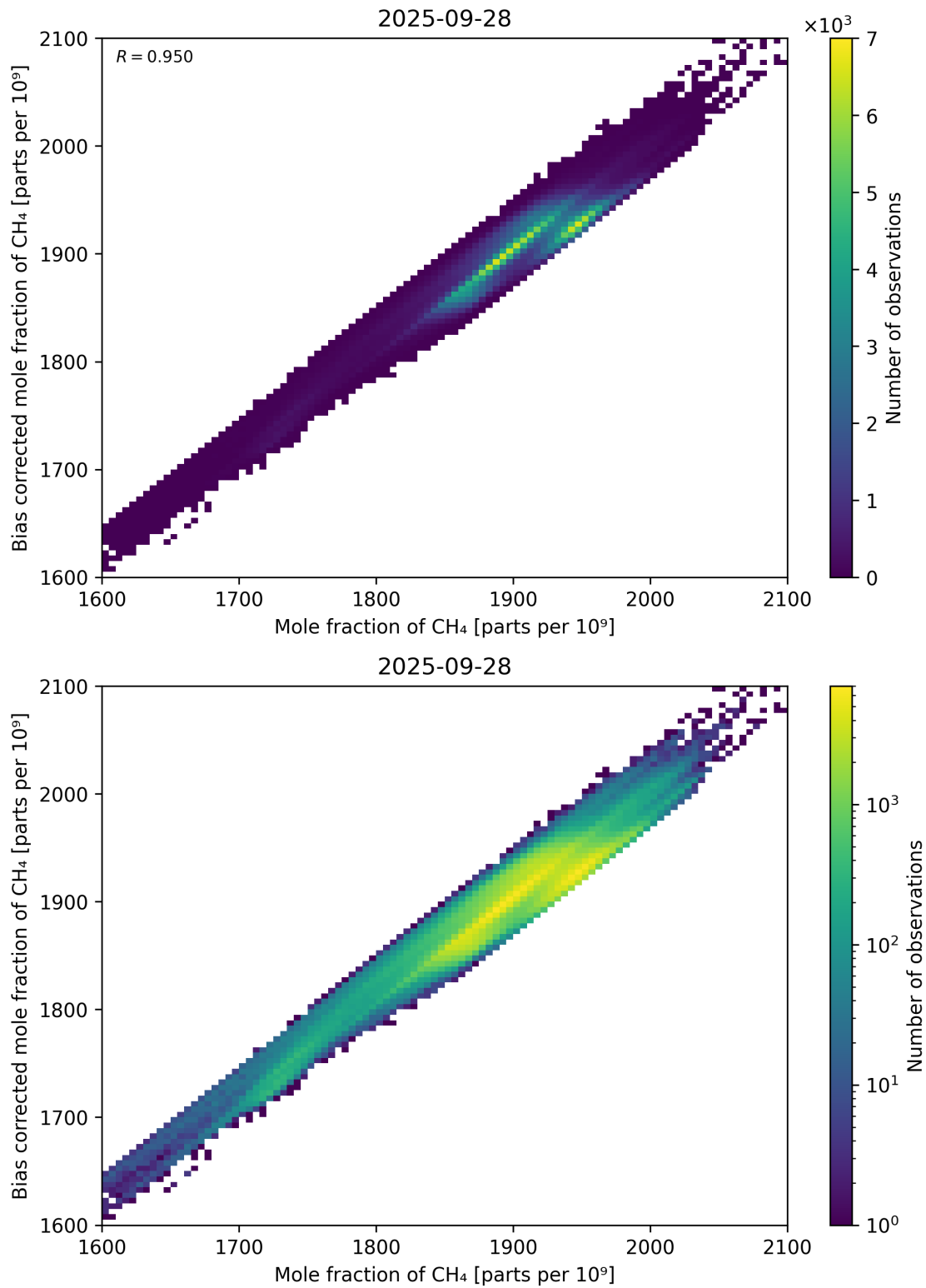
Figure 74: Scatter density plot of “Mole fraction of CH 4 ” against “Bias corrected mole fraction of CH 4 ” for 2025-09-27 to 2025-09-29.
