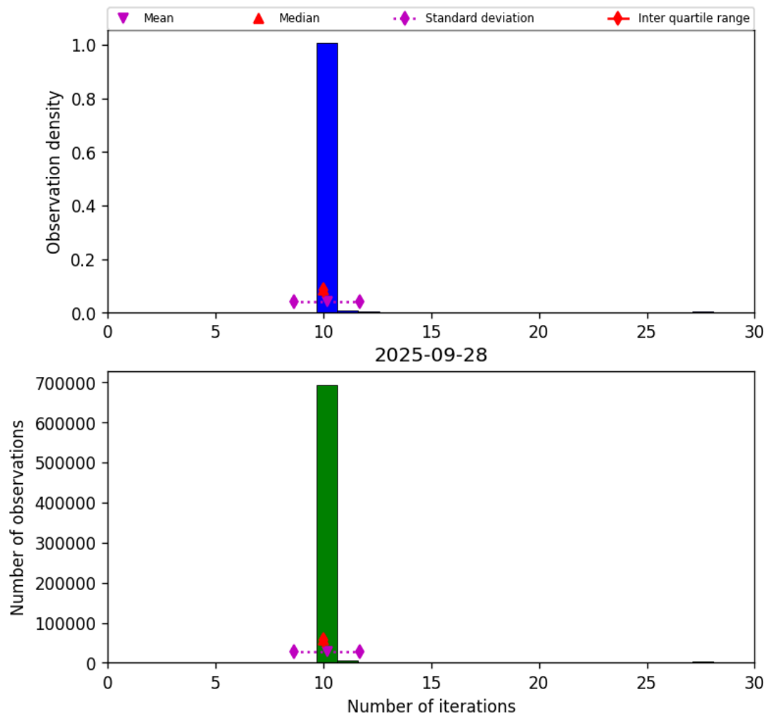
Figure 31: Histogram of “Number of iterations” for 2025-09-27 to 2025-09-29
