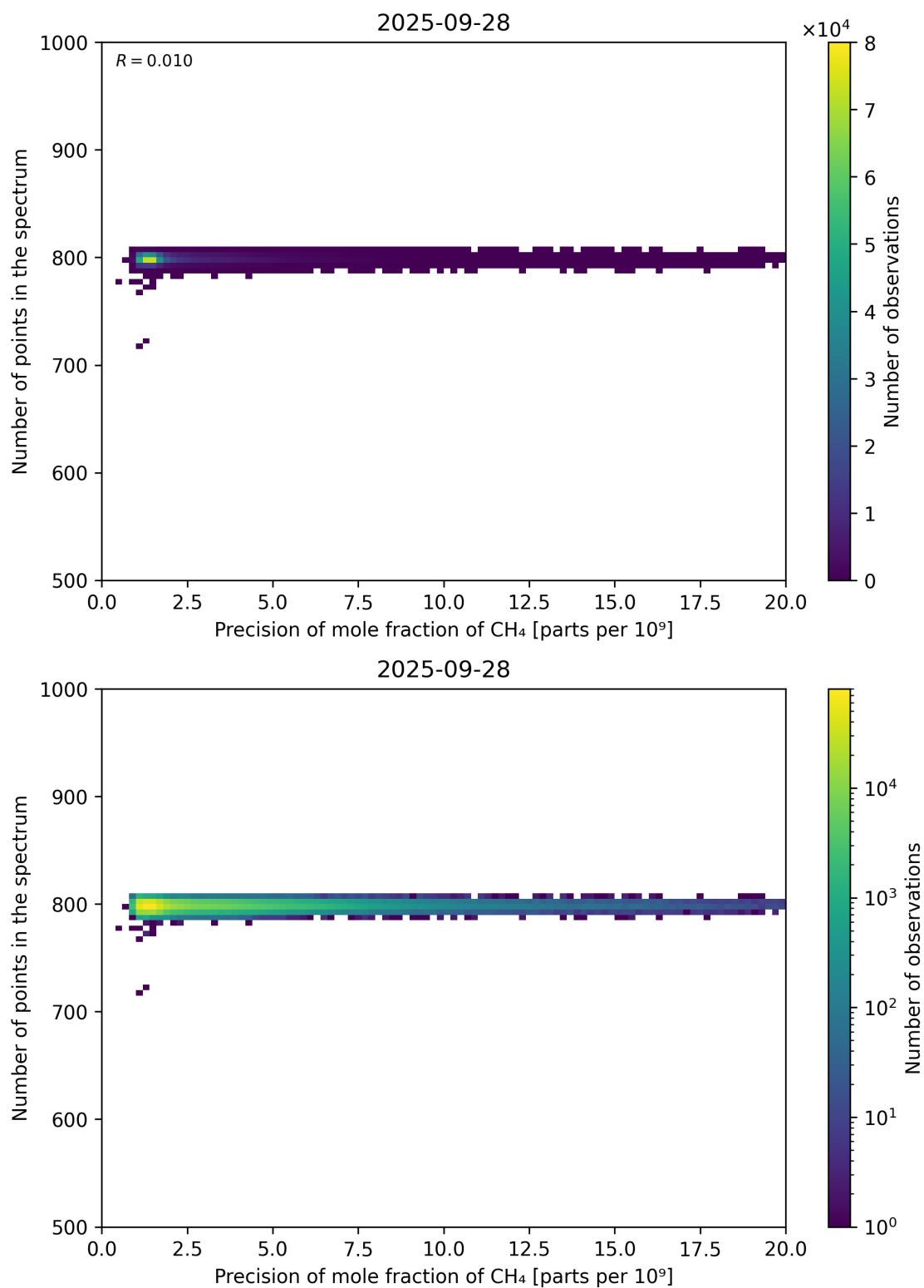
Figure 84: Scatter density plot of “Precision of mole fraction of CH 4 ” against “Number of points in the spectrum” for 2025-09-27 to 2025-09-29.
