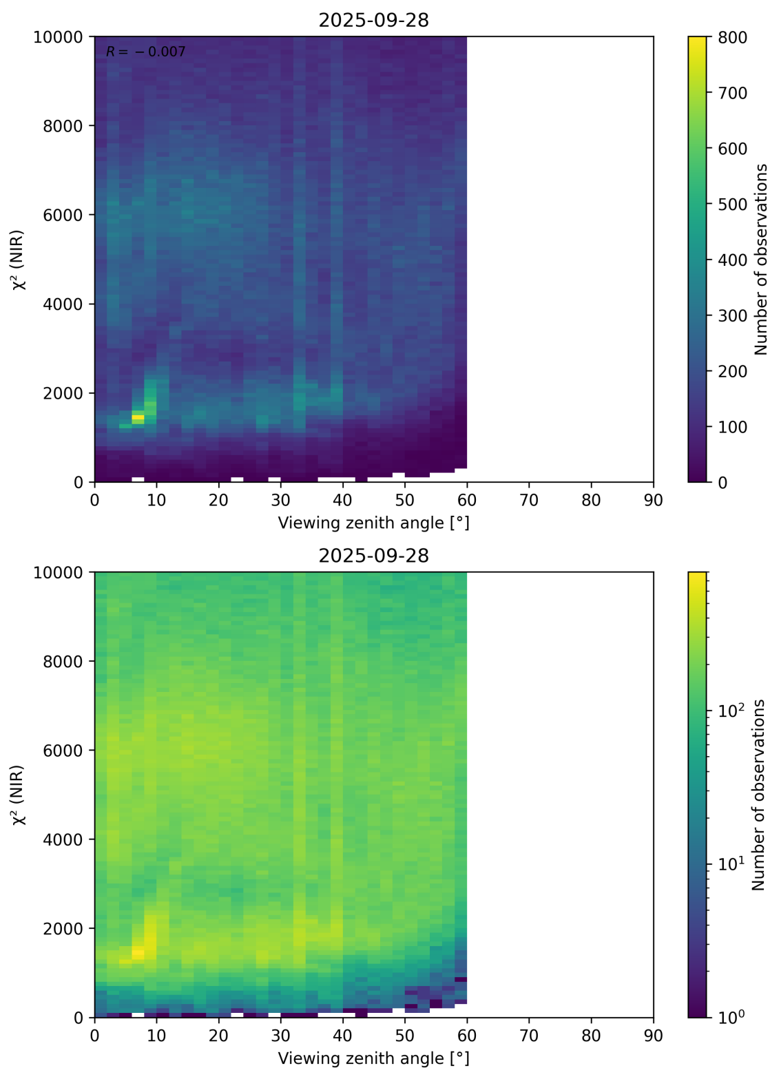
Figure 105: Scatter density plot of “Viewing zenith angle” against “ \chi^2 (NIR)” for 2025-09-27 to 2025-09-29.
