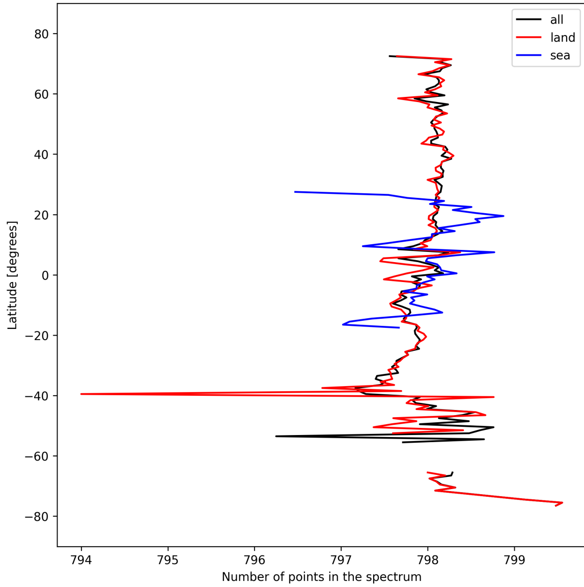
Figure 15: Zonal average of “Number of points in the spectrum” for 2025-09-27 to 2025-09-29.
