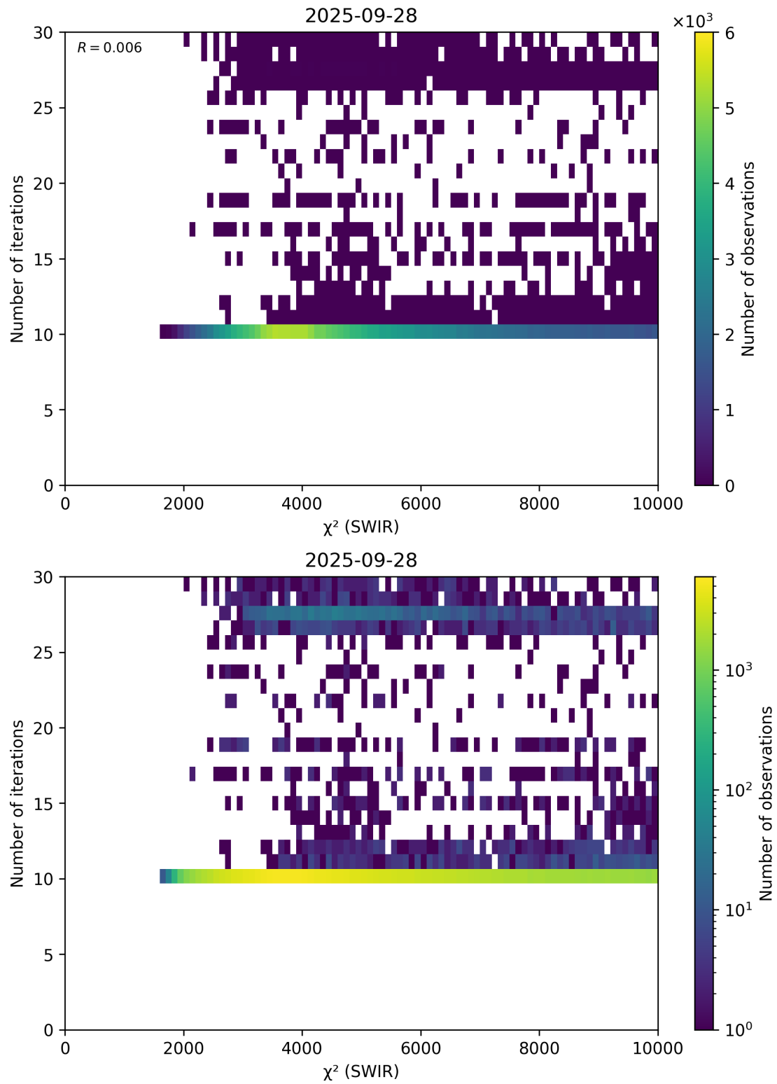
Figure 50: Scatter density plot of “ \chi^2 (SWIR)” against “Number of iterations” for 2025-09-27 to 2025-09-29.
