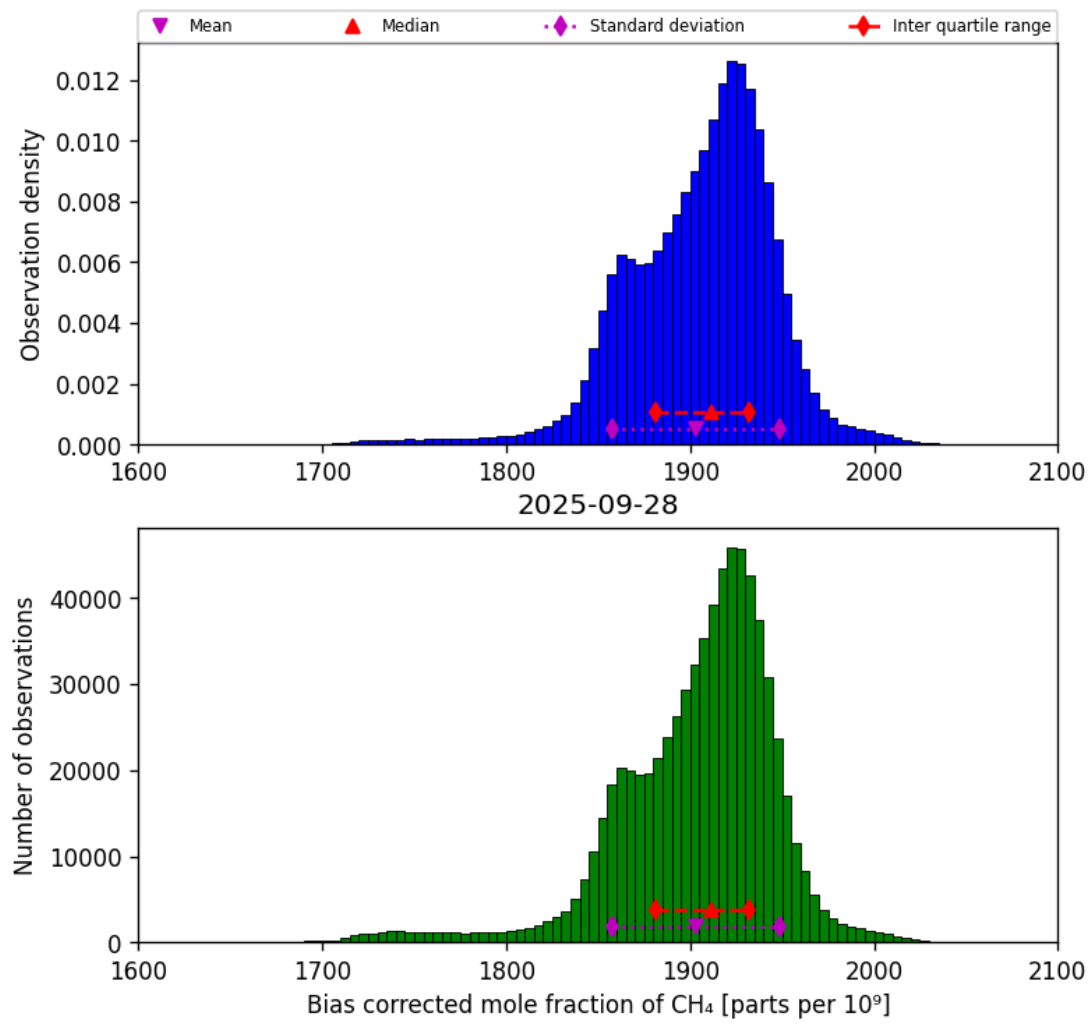
Figure 25: Histogram of “Bias corrected mole fraction of CH 4 ” for 2025-09-27 to 2025-09-29
