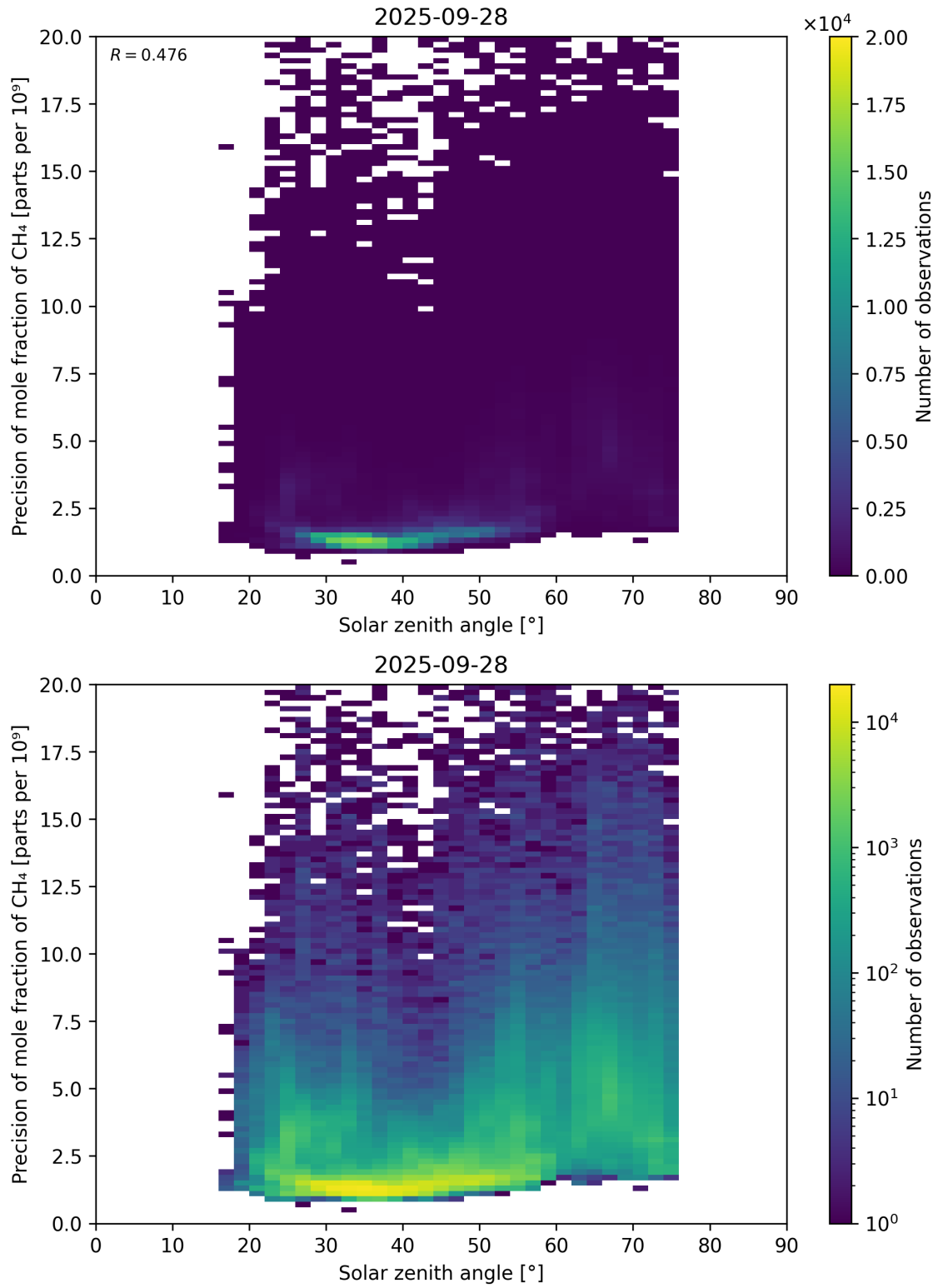
Figure 101: Scatter density plot of “Solar zenith angle” against “Precision of mole fraction of CH 4 ” for 2025-09-27 to 2025-09-29.
