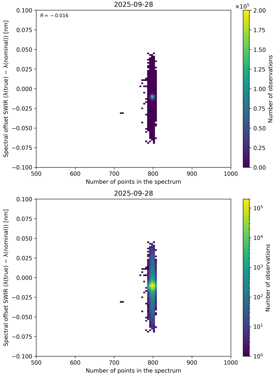
Figure 93: Scatter density plot of “Number of points in the spectrum” against “Spectral offset SWIR ( \lambda_{\text{true}} - \lambda_{\text{nominal}} )” for 2025-09-27 to 2025-09-29.
