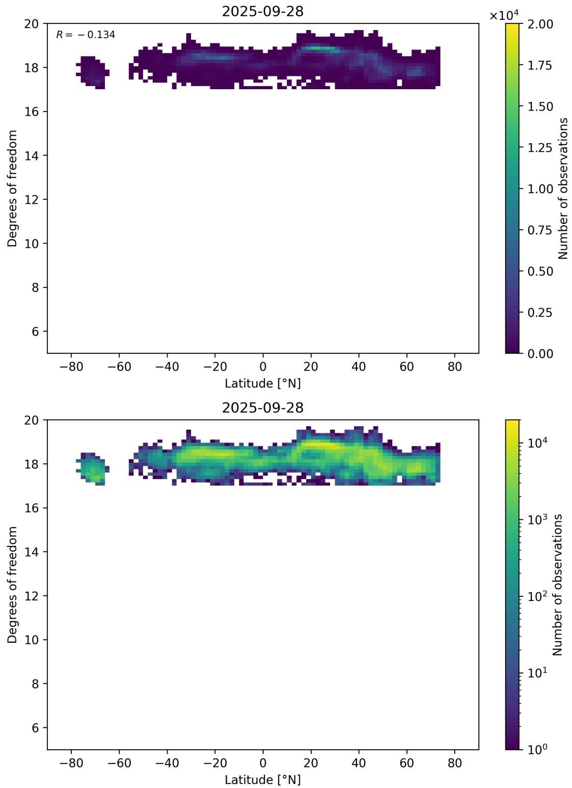
Figure 55: Scatter density plot of “Latitude” against “Degrees of freedom” for 2025-09-27 to 2025-09-29.
