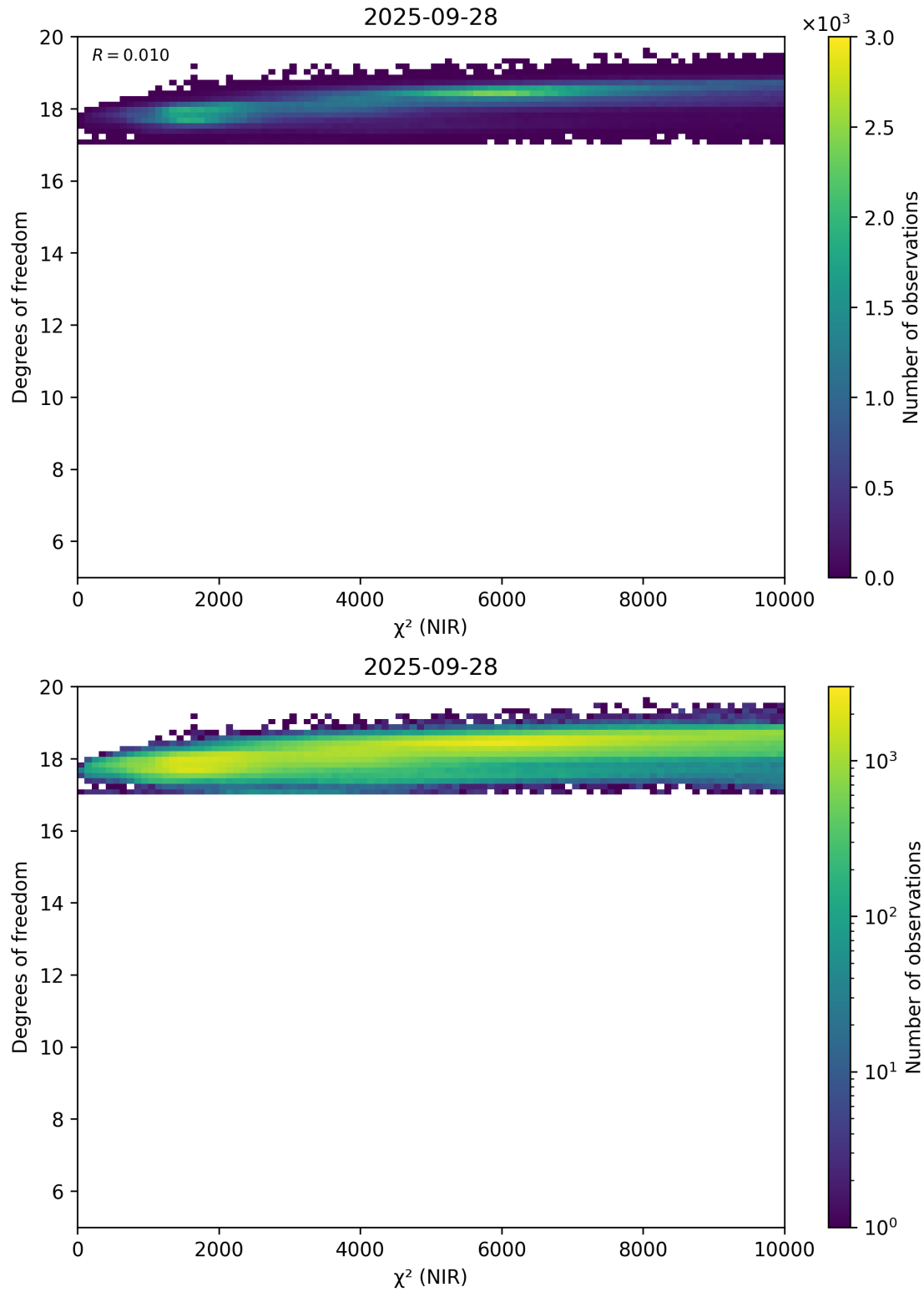
Figure 44: Scatter density plot of “ \chi^2 (NIR)” against “Degrees of freedom” for 2025-09-27 to 2025-09-29.
