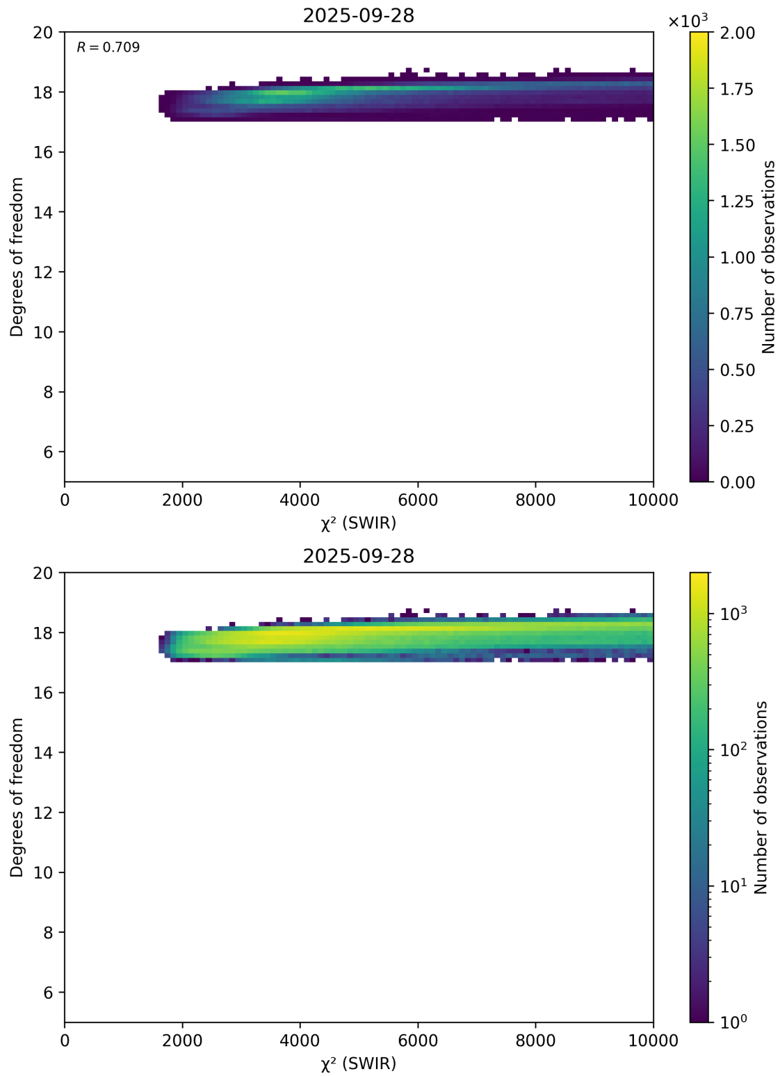
Figure 48: Scatter density plot of “ \chi^2 (SWIR)” against “Degrees of freedom” for 2025-09-27 to 2025-09-29.
