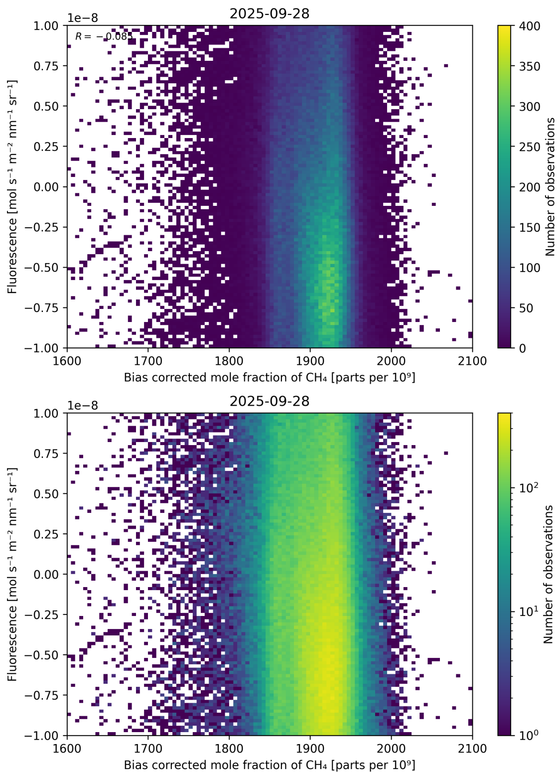
Figure 66: Scatter density plot of “Bias corrected mole fraction of \text{CH}_4 ” against “Fluorescence” for 2025-09-27 to 2025-09-29.
