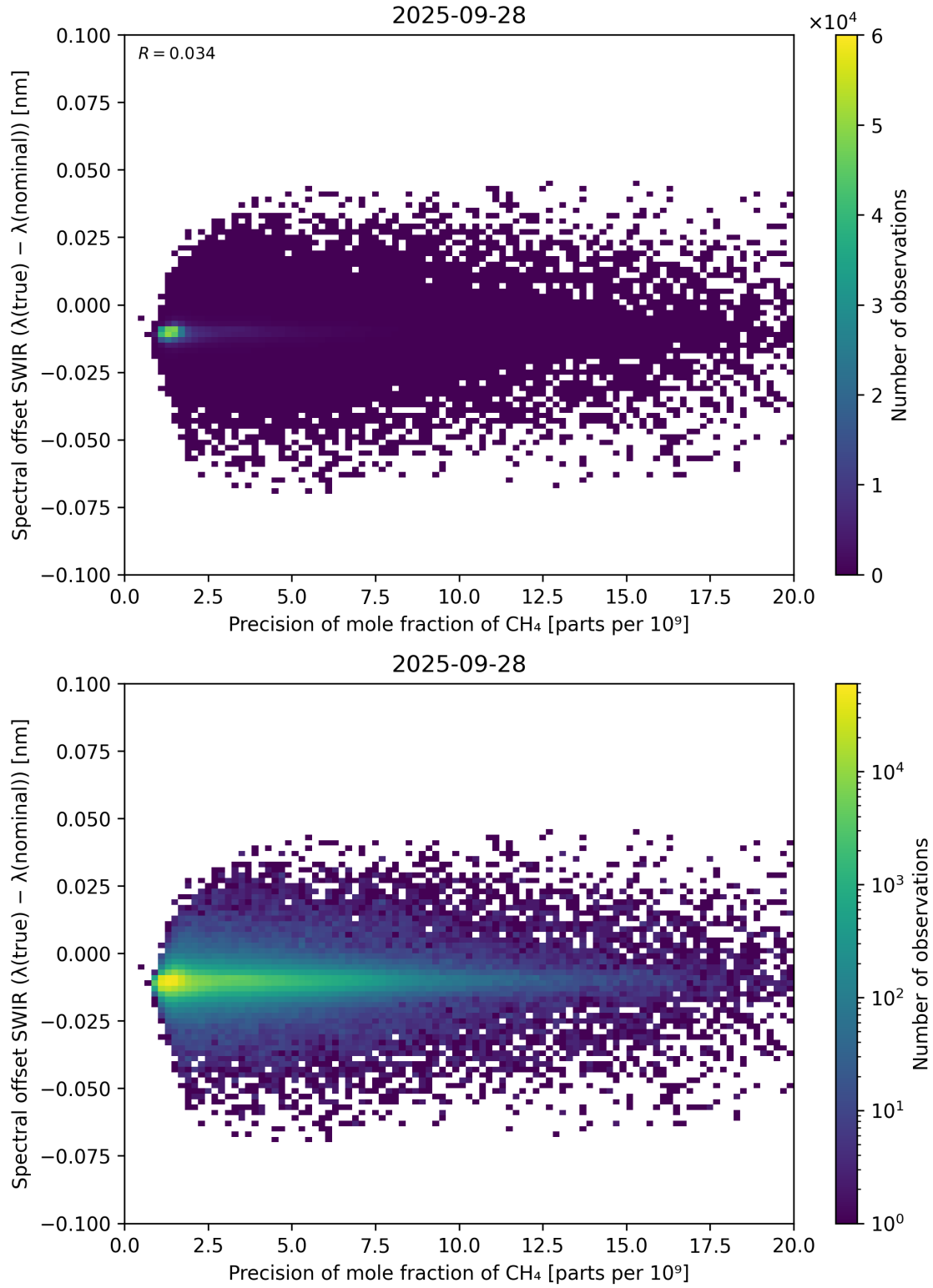
Figure 85: Scatter density plot of “Precision of mole fraction of \text{CH}_4 ” against “Spectral offset SWIR ( \lambda_{\text{true}} - \lambda_{\text{nominal}} )” for 2025-09-27 to 2025-09-29.
