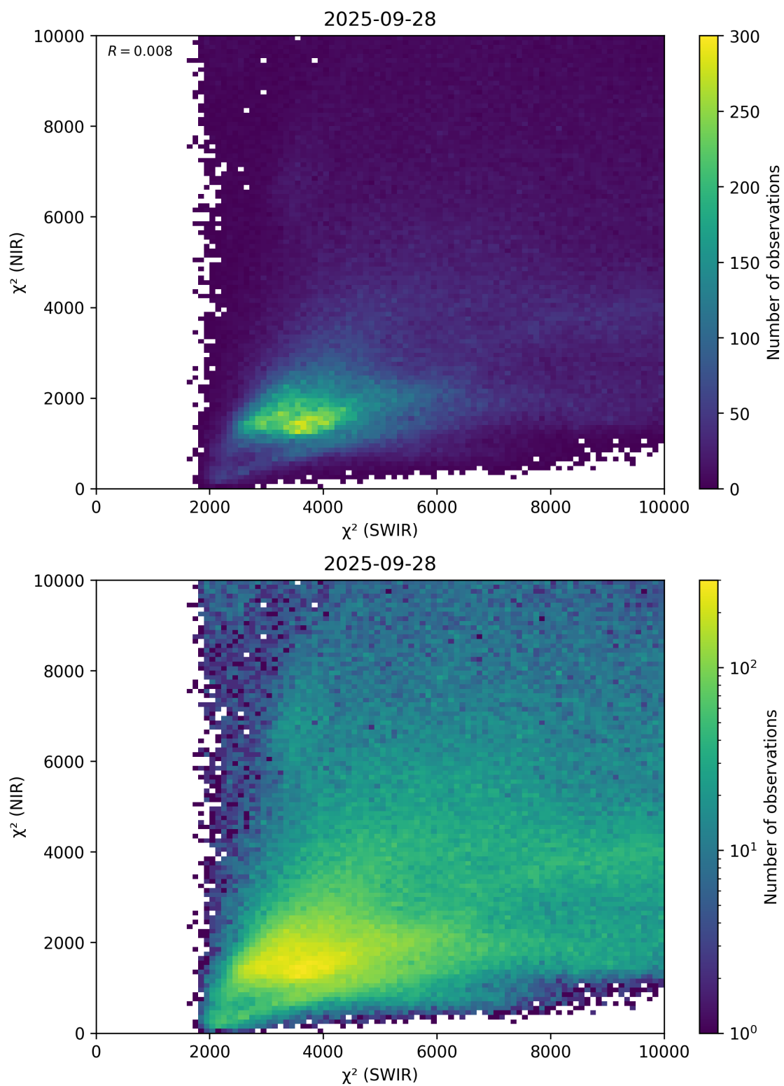
Figure 47: Scatter density plot of “ \chi^2 (SWIR)” against “ \chi^2 (NIR)” for 2025-09-27 to 2025-09-29.
