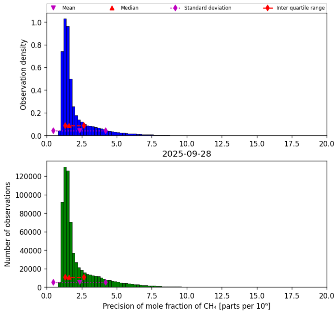
Figure 24: Histogram of “Precision of mole fraction of CH 4 ” for 2025-09-27 to 2025-09-29
