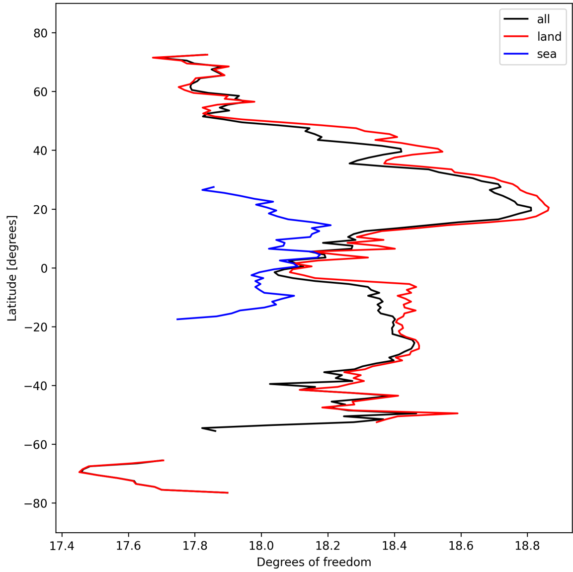
Figure 19: Zonal average of “Degrees of freedom” for 2025-09-27 to 2025-09-29.
