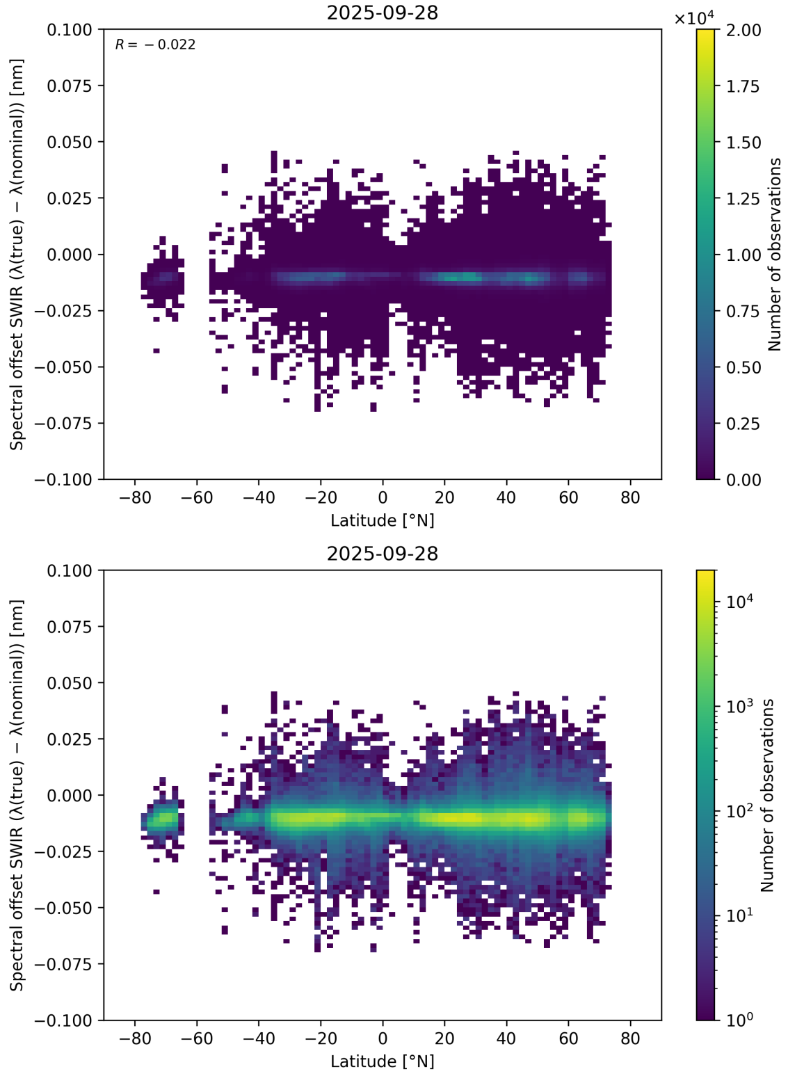
Figure 62: Scatter density plot of “Latitude” against “Spectral offset SWIR ( \lambda_{\text{true}} - \lambda_{\text{nominal}} )” for 2025-09-27 to 2025-09-29.
