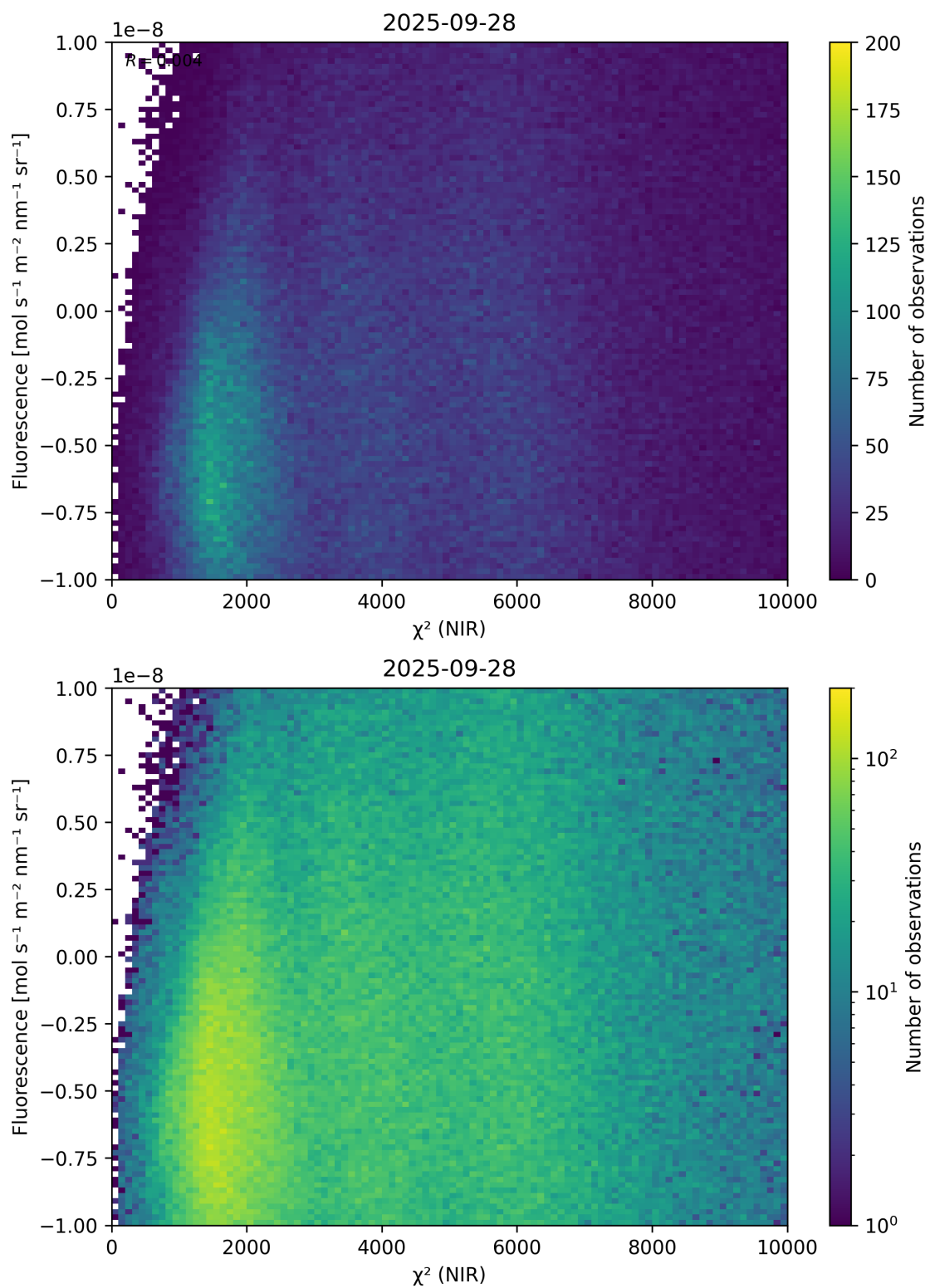
Figure 45: Scatter density plot of “ \chi^2 (NIR)” against “Fluorescence” for 2025-09-27 to 2025-09-29.
