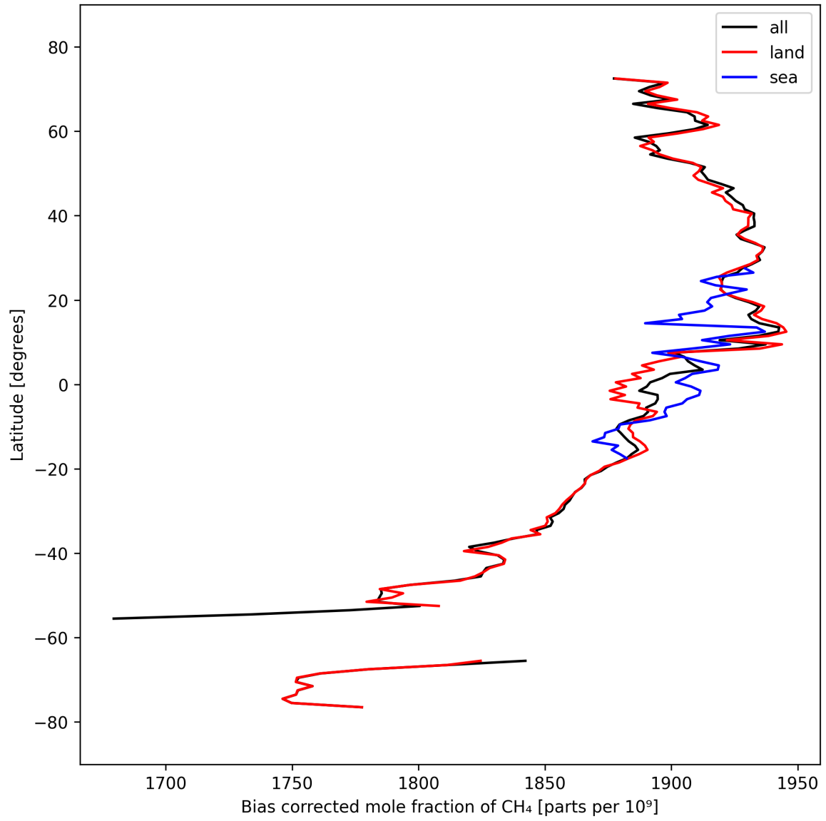
Figure 14: Zonal average of “Bias corrected mole fraction of CH 4 ” for 2025-09-27 to 2025-09-29.
