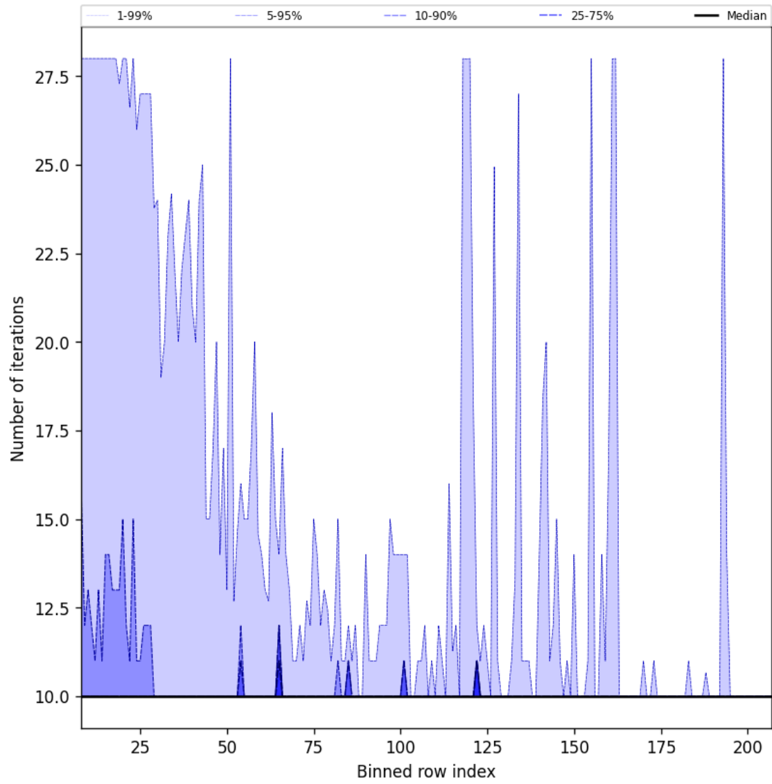
Figure 42: Along track statistics of “Number of iterations” for 2025-09-27 to 2025-09-29
