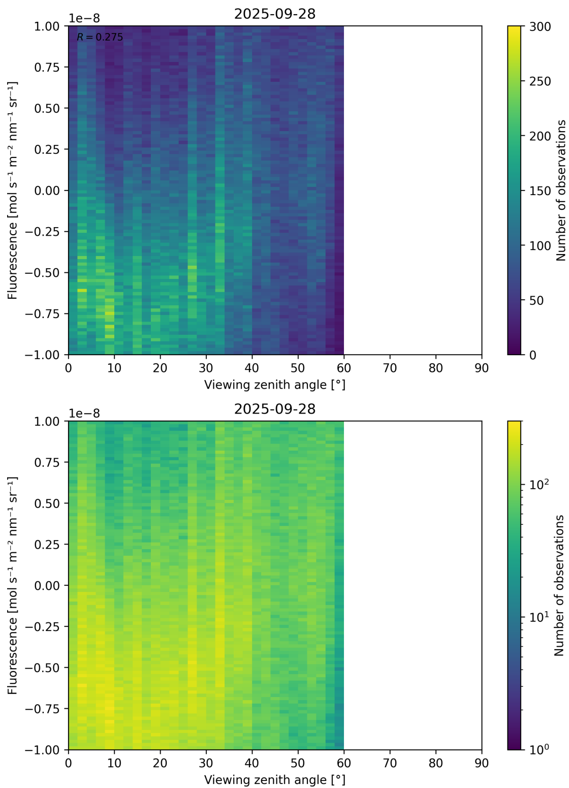
Figure 108: Scatter density plot of “Viewing zenith angle” against “Fluorescence” for 2025-09-27 to 2025-09-29.
