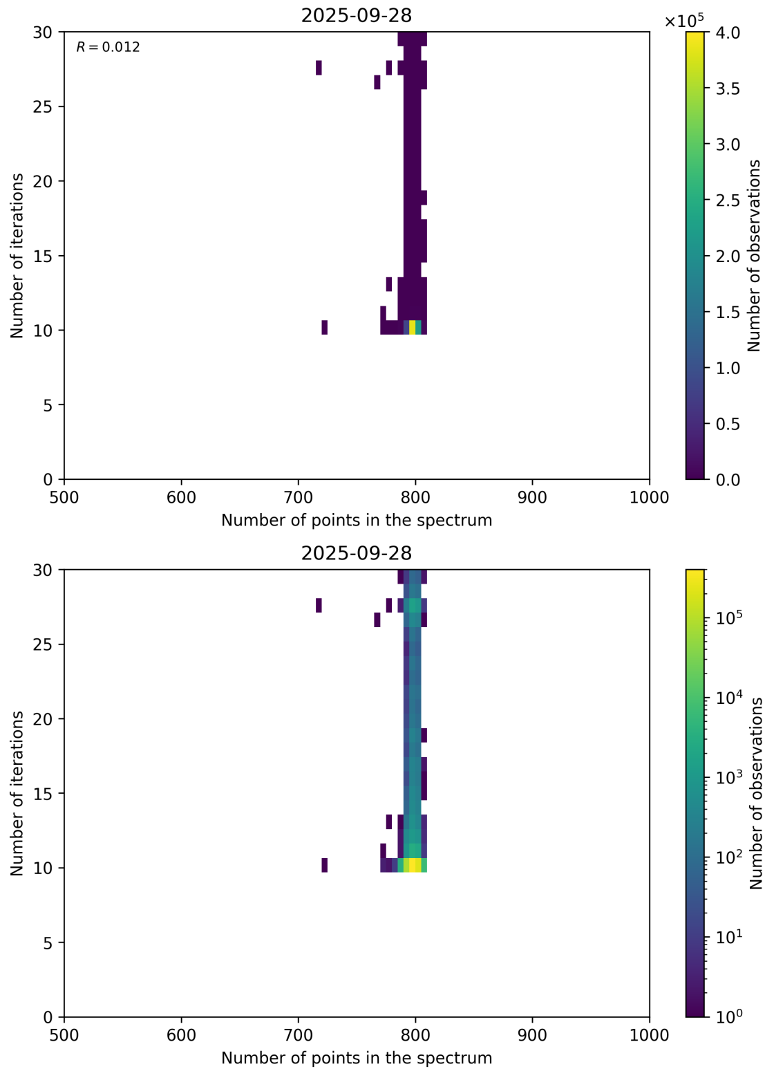
Figure 92: Scatter density plot of “Number of points in the spectrum” against “Number of iterations” for 2025-09-27 to 2025-09-29.
