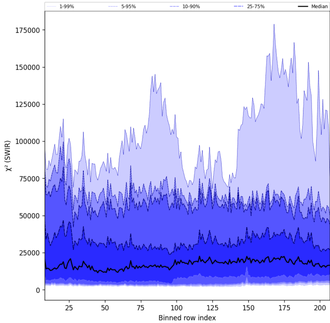
Figure 39: Along track statistics of “ \chi^2 (SWIR)” for 2025-09-27 to 2025-09-29
