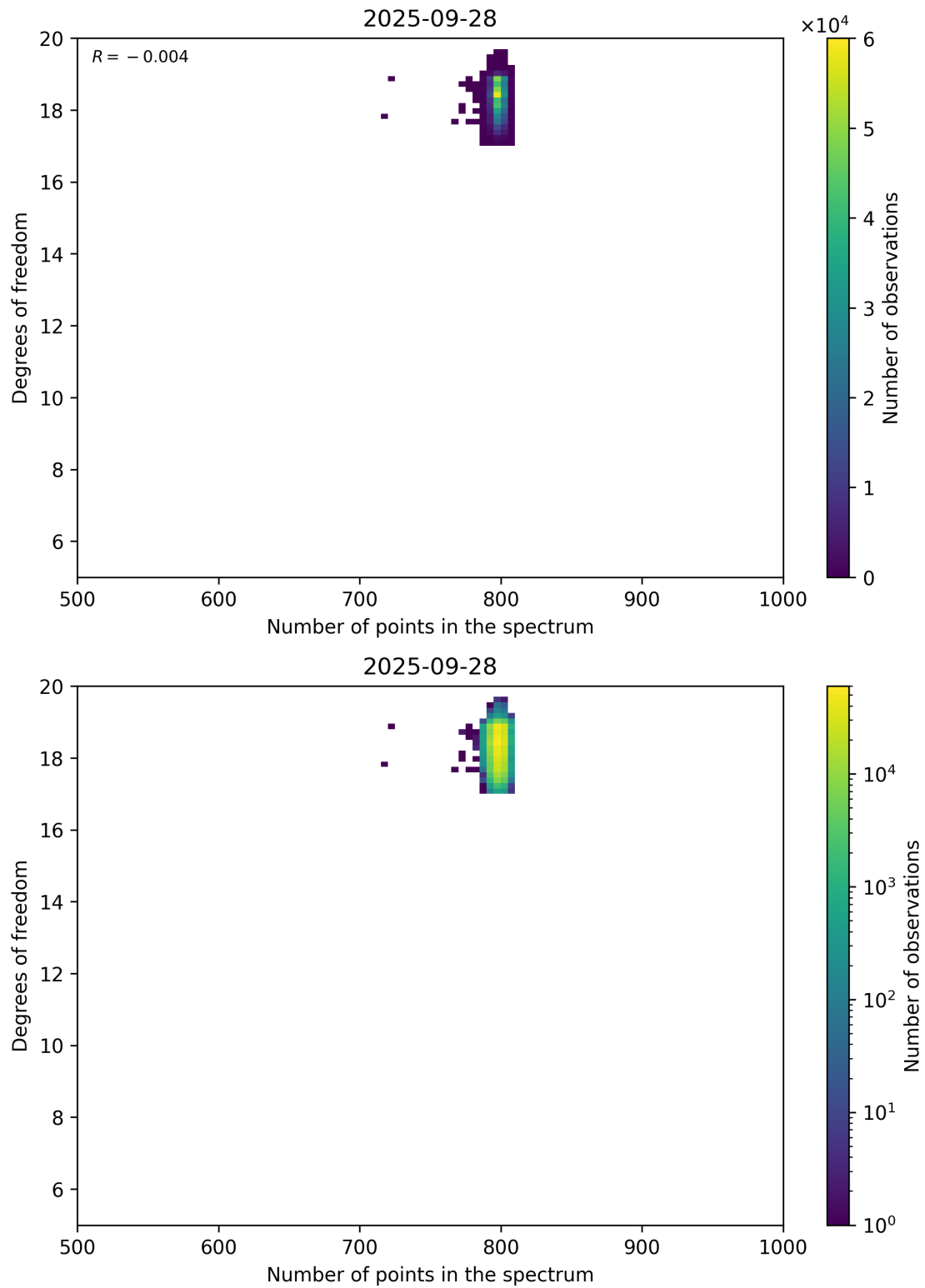
Figure 90: Scatter density plot of “Number of points in the spectrum” against “Degrees of freedom” for 2025-09-27 to 2025-09-29.
