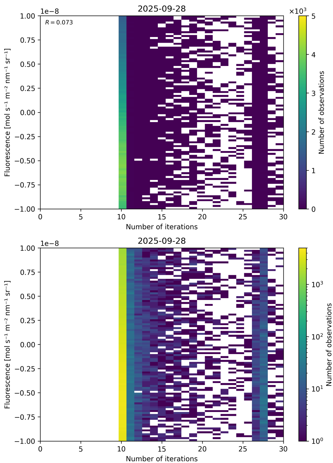
Figure 87: Scatter density plot of “Number of iterations” against “Fluorescence” for 2025-09-27 to 2025-09-29.
