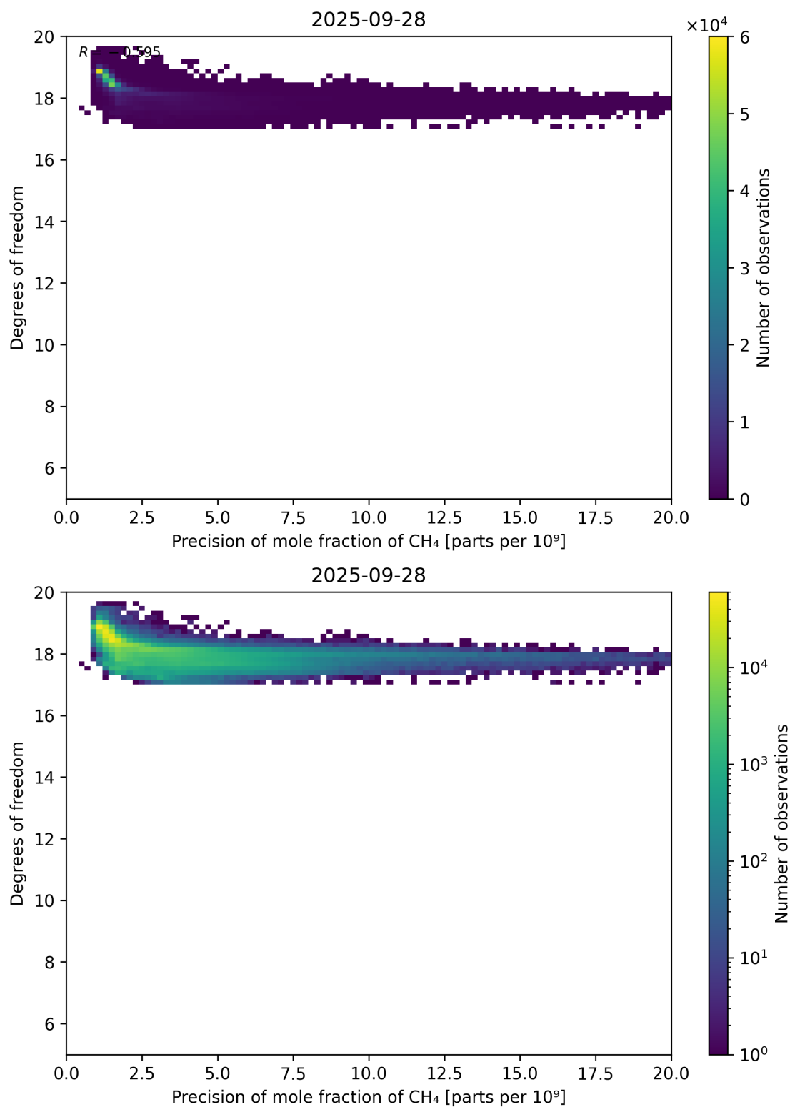
Figure 80: Scatter density plot of “Precision of mole fraction of CH 4 ” against “Degrees of freedom” for 2025-09-27 to 2025-09-29.
