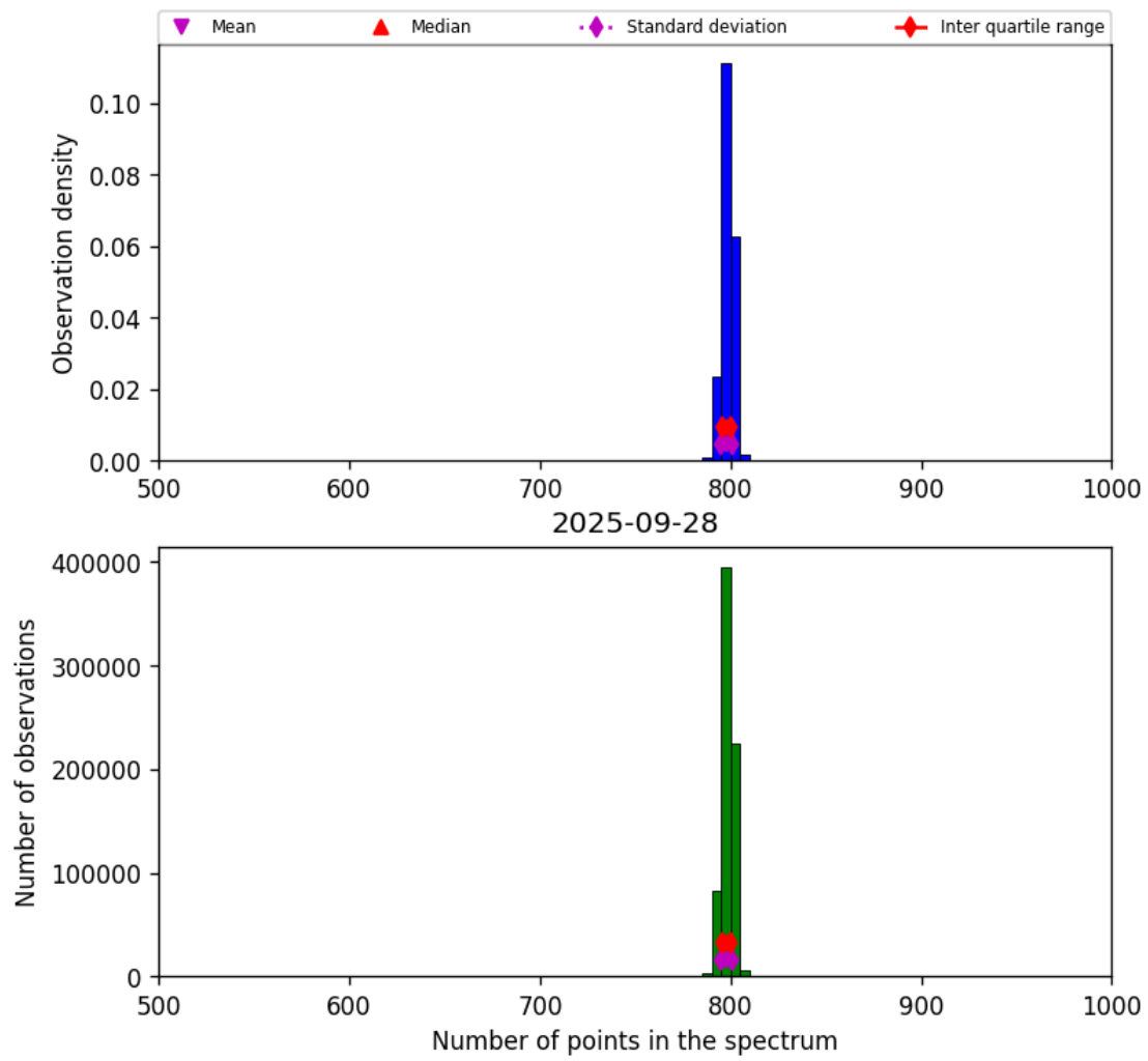
Figure 26: Histogram of “Number of points in the spectrum” for 2025-09-27 to 2025-09-29
