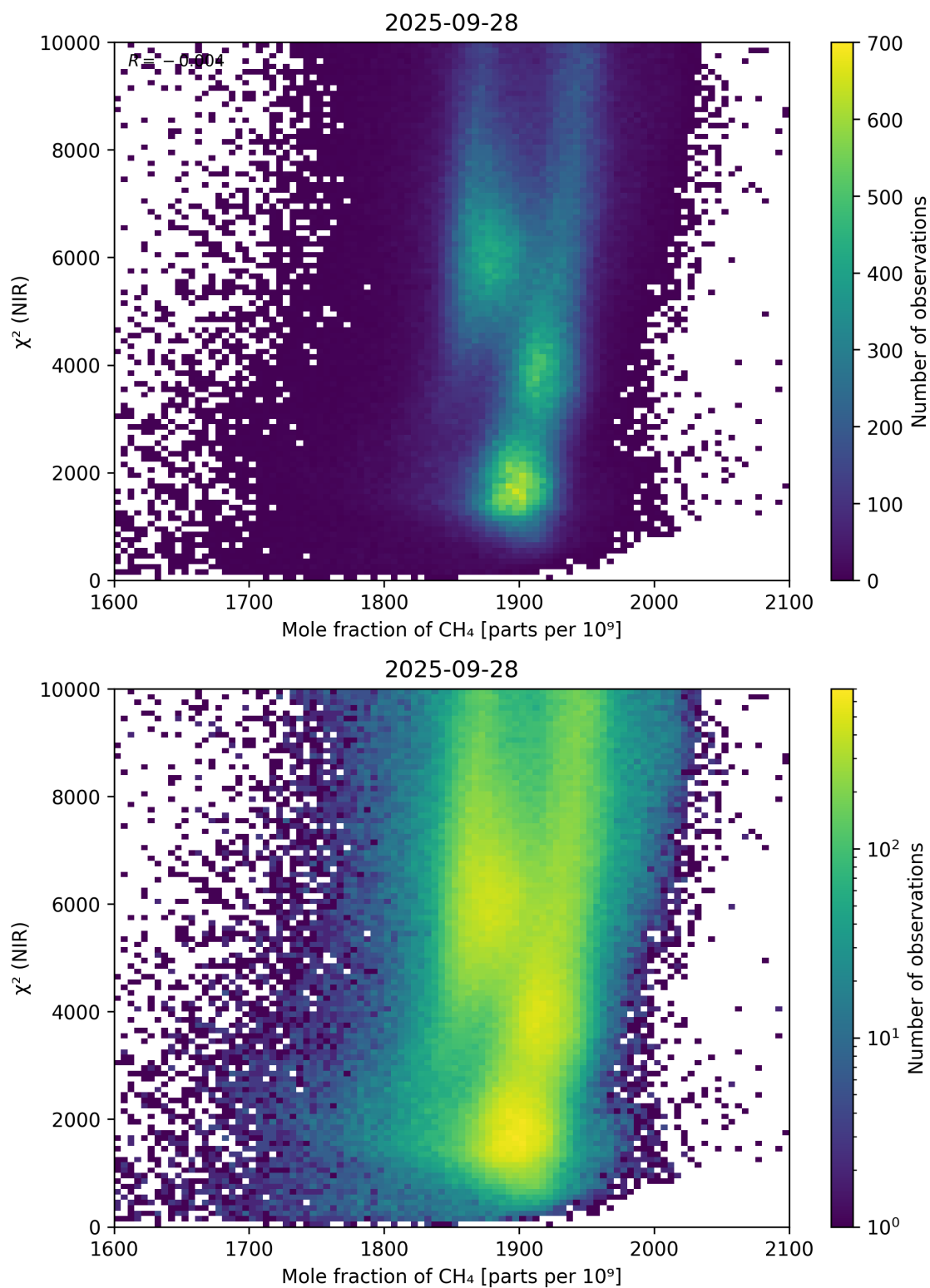
Figure 70: Scatter density plot of “Mole fraction of \text{CH}_4 ” against “ \chi^2 (NIR)” for 2025-09-27 to 2025-09-29.
