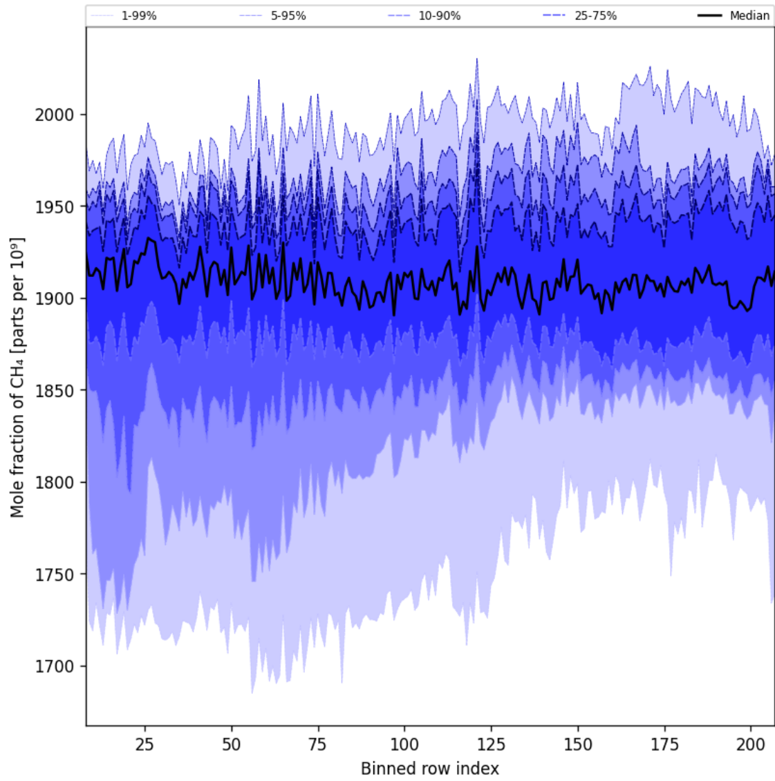
Figure 34: Along track statistics of “Mole fraction of CH 4 ” for 2025-09-27 to 2025-09-29
