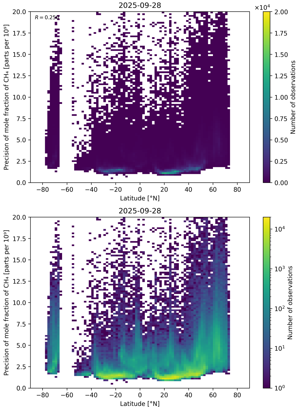
Figure 59: Scatter density plot of “Latitude” against “Precision of mole fraction of CH 4 ” for 2025-09-27 to 2025-09-29.
