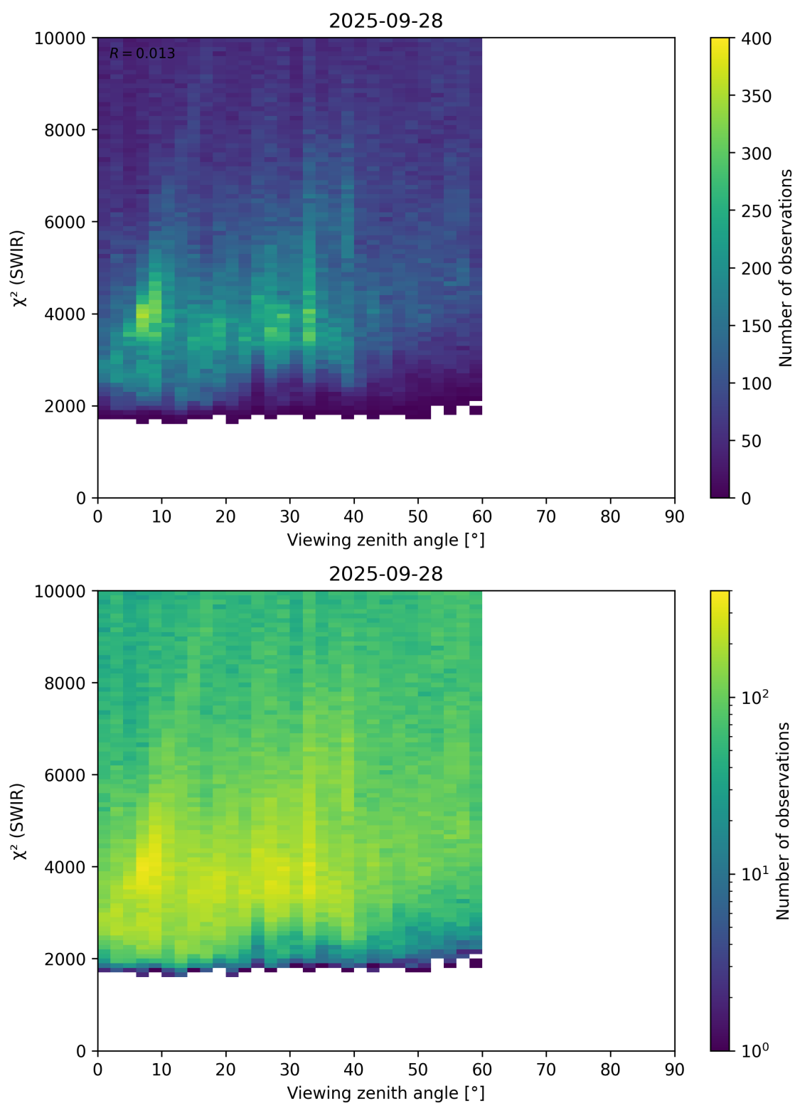
Figure 106: Scatter density plot of “Viewing zenith angle” against “ \chi^2 (SWIR)” for 2025-09-27 to 2025-09-29.
