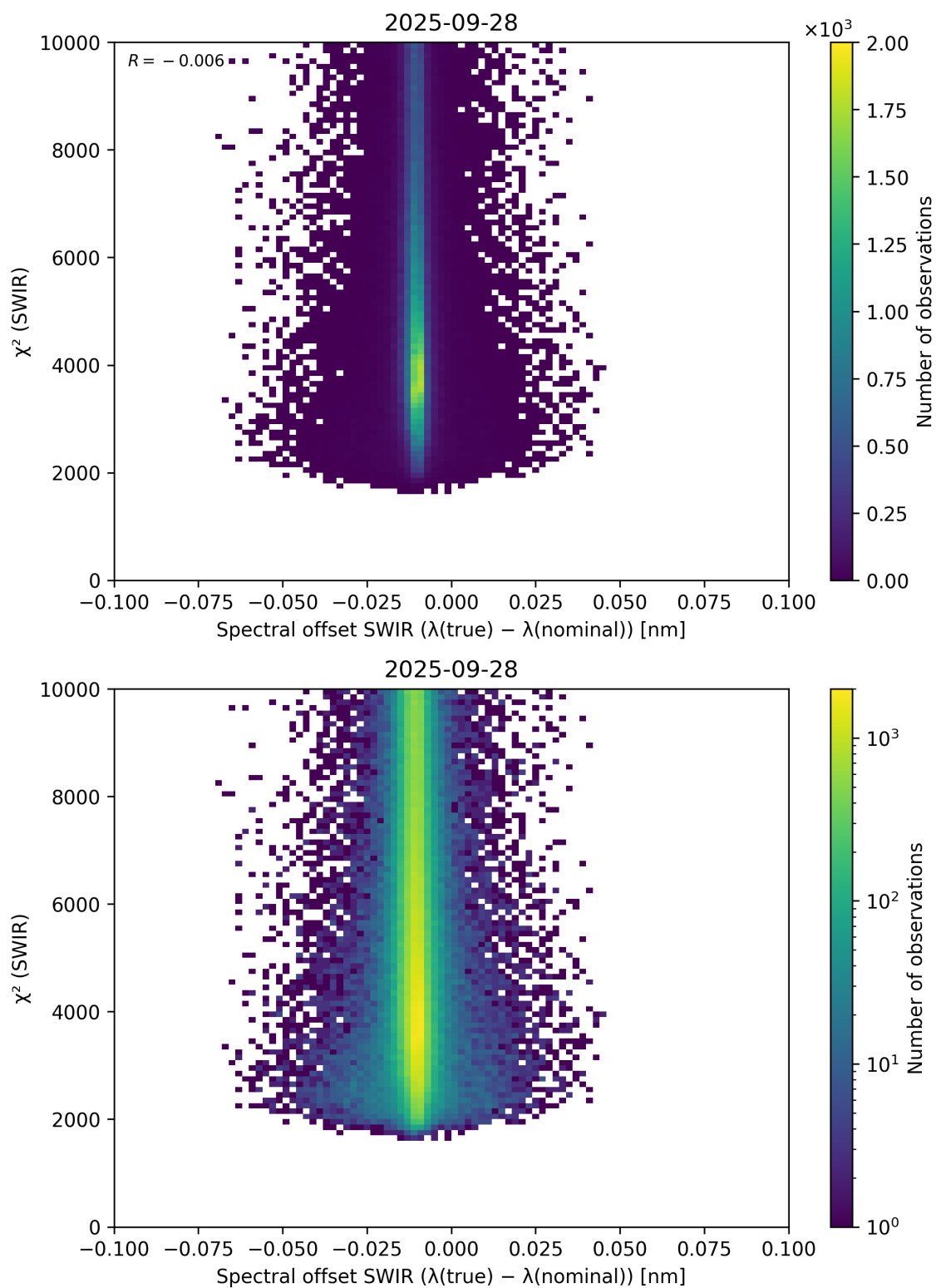
Figure 118: Scatter density plot of “Spectral offset SWIR ( \lambda_{\text{true}} - \lambda_{\text{nominal}} )” against “ \chi^2 (SWIR)” for 2025-09-27 to 2025-09-29.
