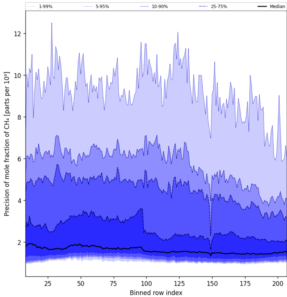
Figure 35: Along track statistics of “Precision of mole fraction of CH 4 ” for 2025-09-27 to 2025-09-29
