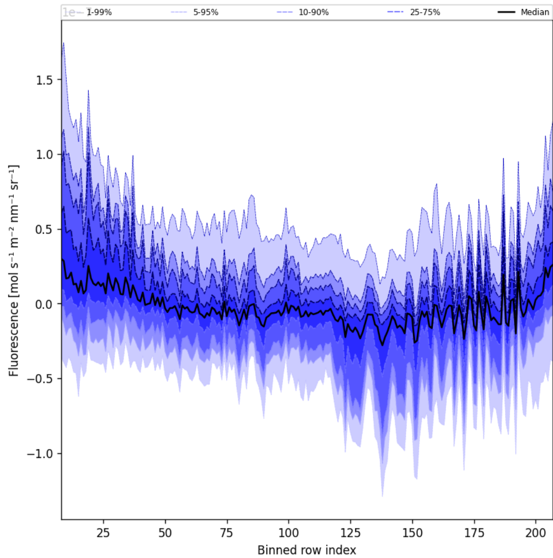
Figure 43: Along track statistics of “Fluorescence” for 2025-09-27 to 2025-09-29
