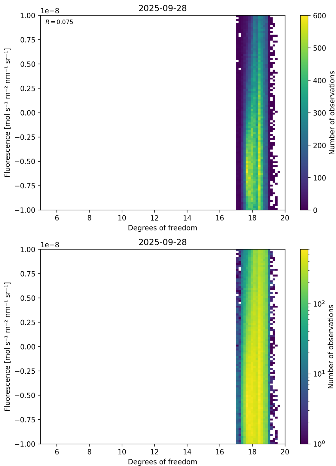
Figure 51: Scatter density plot of “Degrees of freedom” against “Fluorescence” for 2025-09-27 to 2025-09-29.
