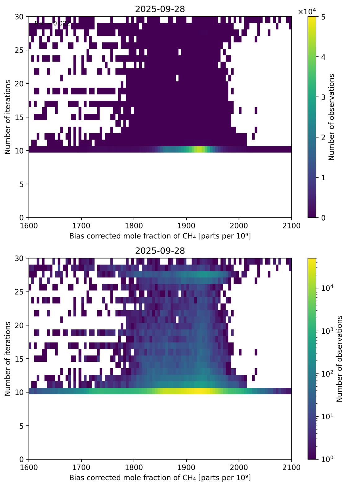
Figure 67: Scatter density plot of “Bias corrected mole fraction of \text{CH}_4 ” against “Number of iterations” for 2025-09-27 to 2025-09-29.
