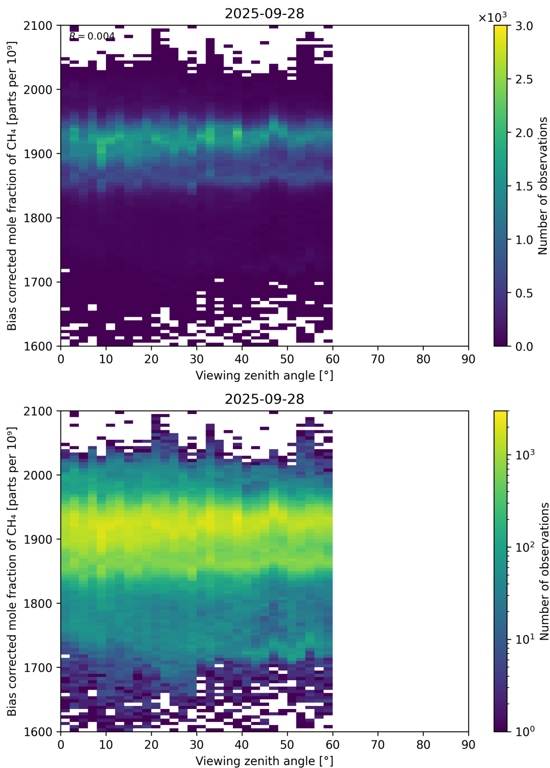
Figure 111: Scatter density plot of “Viewing zenith angle” against “Bias corrected mole fraction of CH 4 ” for 2025-09-27 to 2025-09-29.
