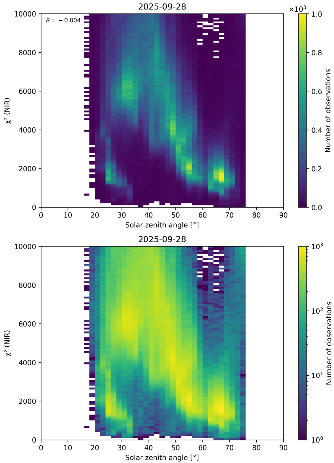
Figure 94: Scatter density plot of “Solar zenith angle” against “ \chi^2 (NIR)” for 2025-09-27 to 2025-09-29.
