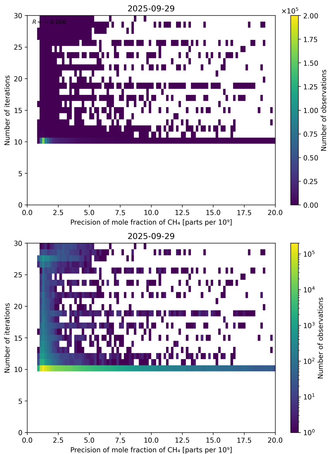
Figure 83: Scatter density plot of “Precision of mole fraction of CH 4 ” against “Number of iterations” for 2025-09-28 to 2025-09-30.
