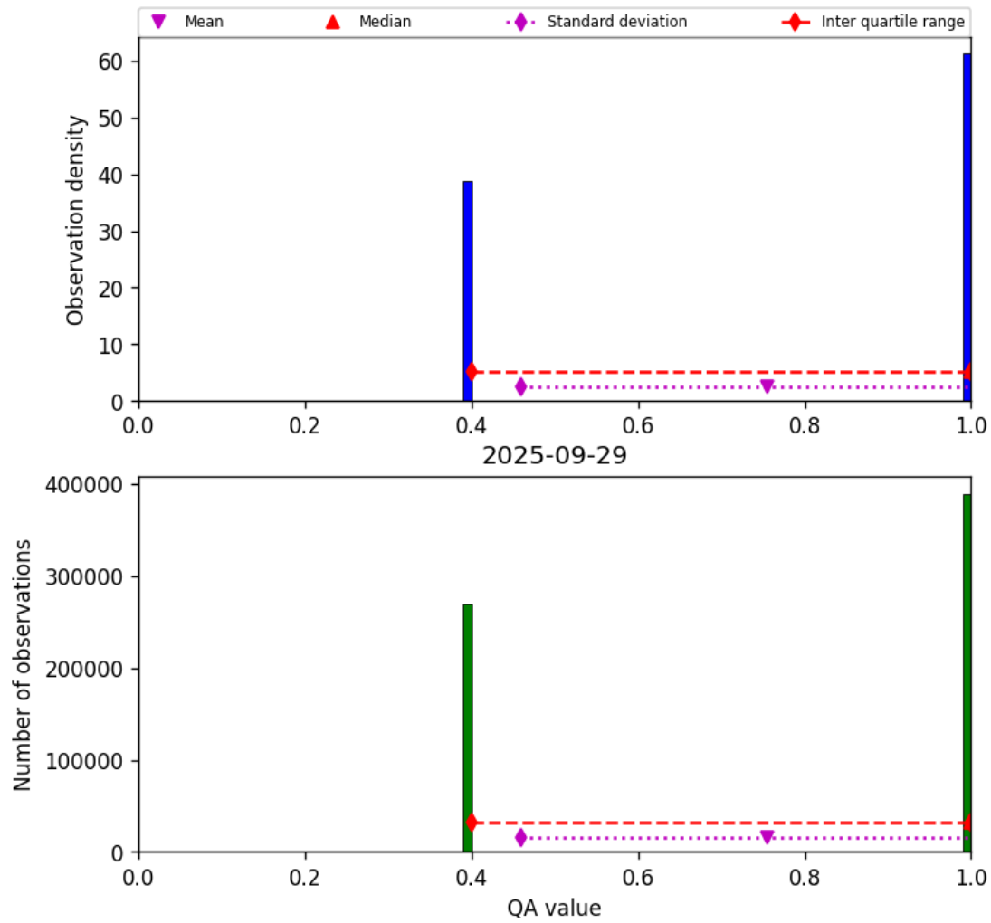
Figure 22: Histogram of “QA value” for 2025-09-28 to 2025-09-30
