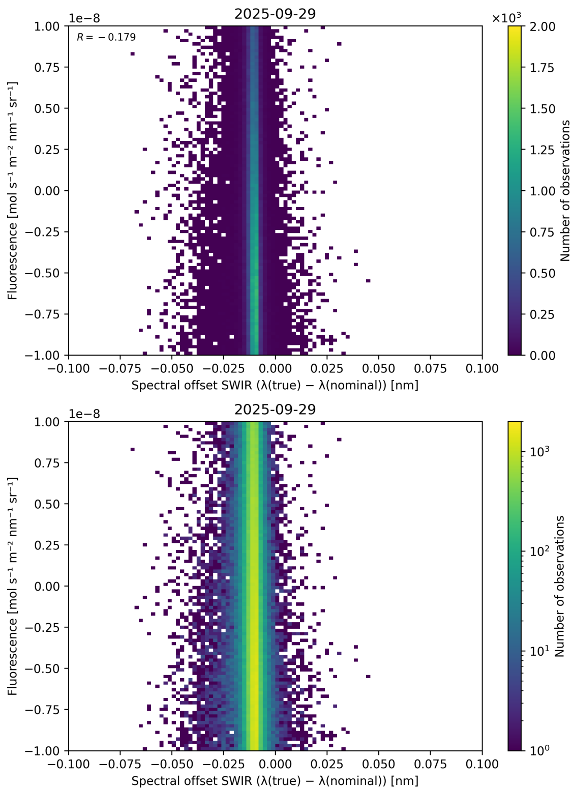
Figure 120: Scatter density plot of “Spectral offset SWIR ( \lambda_{\text{true}} - \lambda_{\text{nominal}} )” against “Fluorescence” for 2025-09-28 to 2025-09-30.
