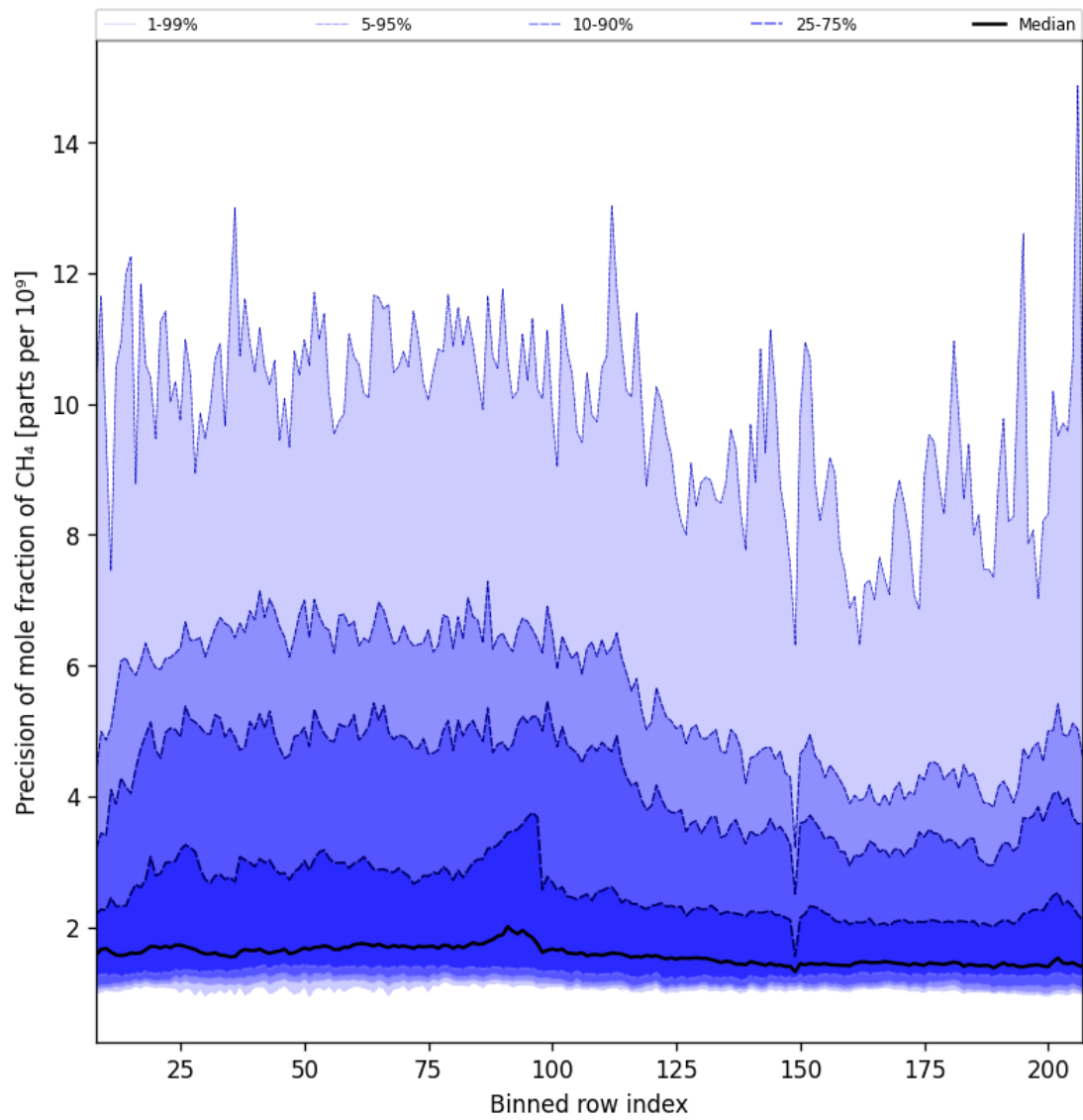
Figure 35: Along track statistics of “Precision of mole fraction of CH 4 ” for 2025-09-28 to 2025-09-30
