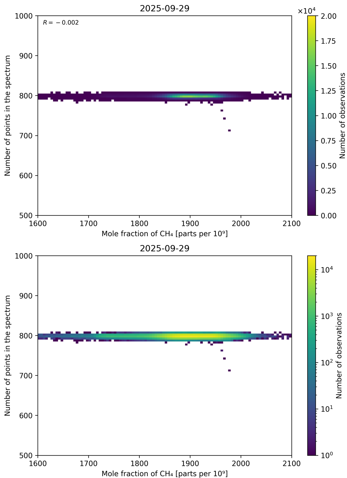
Figure 77: Scatter density plot of “Mole fraction of CH 4 ” against “Number of points in the spectrum” for 2025-09-28 to 2025-09-30.
