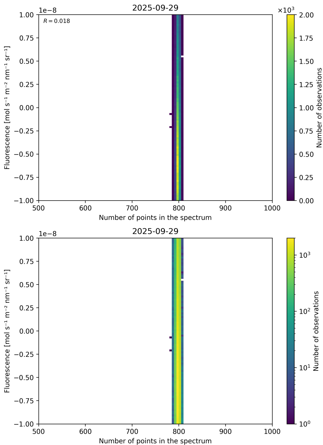
Figure 91: Scatter density plot of “Number of points in the spectrum” against “Fluorescence” for 2025-09-28 to 2025-09-30.
