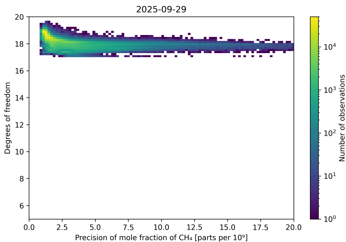
Figure 80: Scatter density plot of “Precision of mole fraction of CH 4 ” against “Degrees of freedom” for 2025-09-28 to 2025-09-30.
