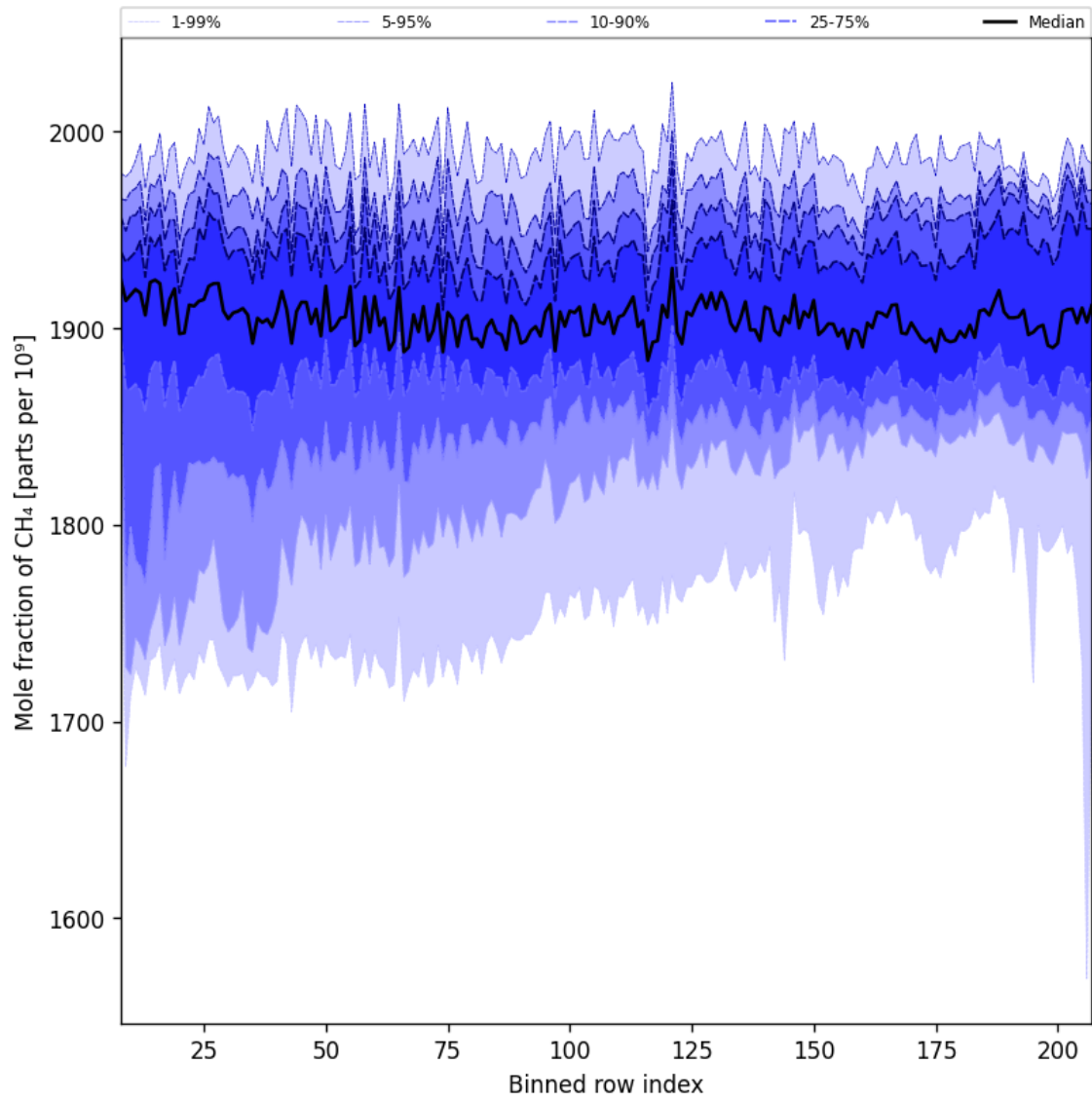
Figure 34: Along track statistics of “Mole fraction of CH 4 ” for 2025-09-28 to 2025-09-30
