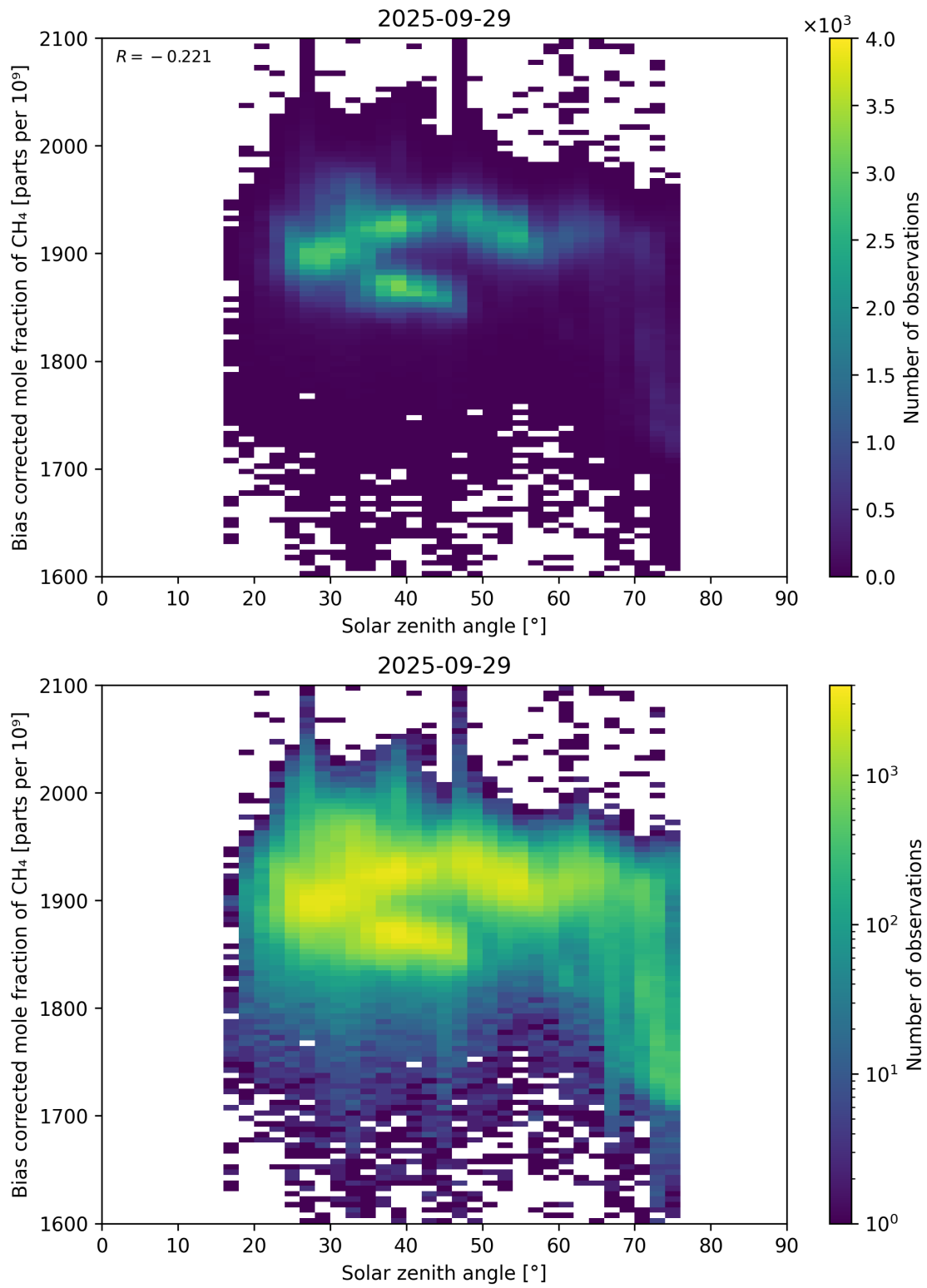
Figure 100: Scatter density plot of “Solar zenith angle” against “Bias corrected mole fraction of CH 4 ” for 2025-09-28 to 2025-09-30.
