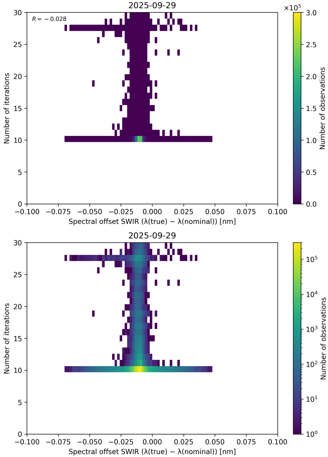
Figure 121: Scatter density plot of “Spectral offset SWIR ( \lambda_{\text{true}} - \lambda_{\text{nominal}} )” against “Number of iterations” for 2025-09-28 to 2025-09-30.
