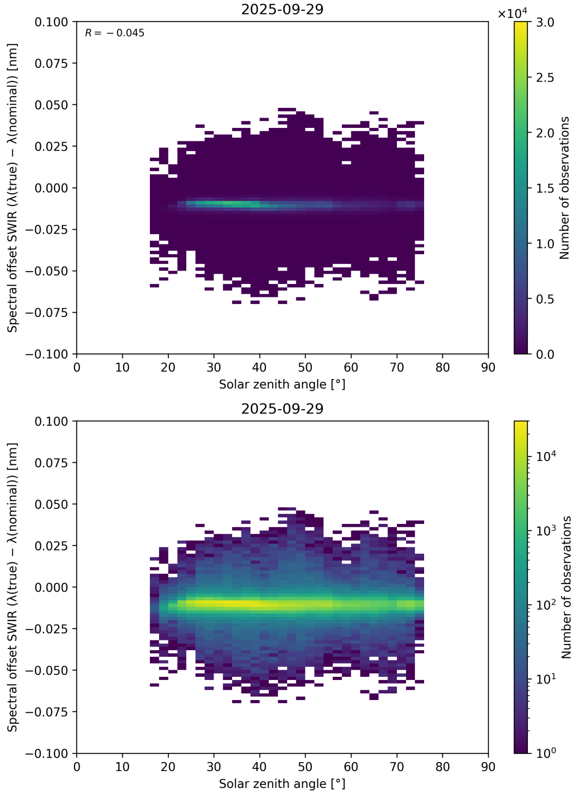
Figure 104: Scatter density plot of “Solar zenith angle” against “Spectral offset SWIR ( \lambda_{\text{true}} - \lambda_{\text{nominal}} )” for 2025-09-28 to 2025-09-30.
