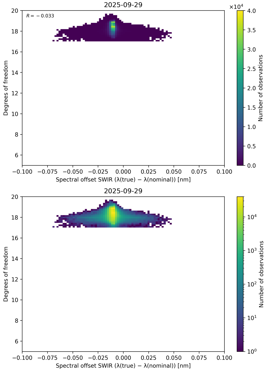
Figure 119: Scatter density plot of “Spectral offset SWIR ( \lambda_{\text{true}} - \lambda_{\text{nominal}} )” against “Degrees of freedom” for 2025-09-28 to 2025-09-30.
