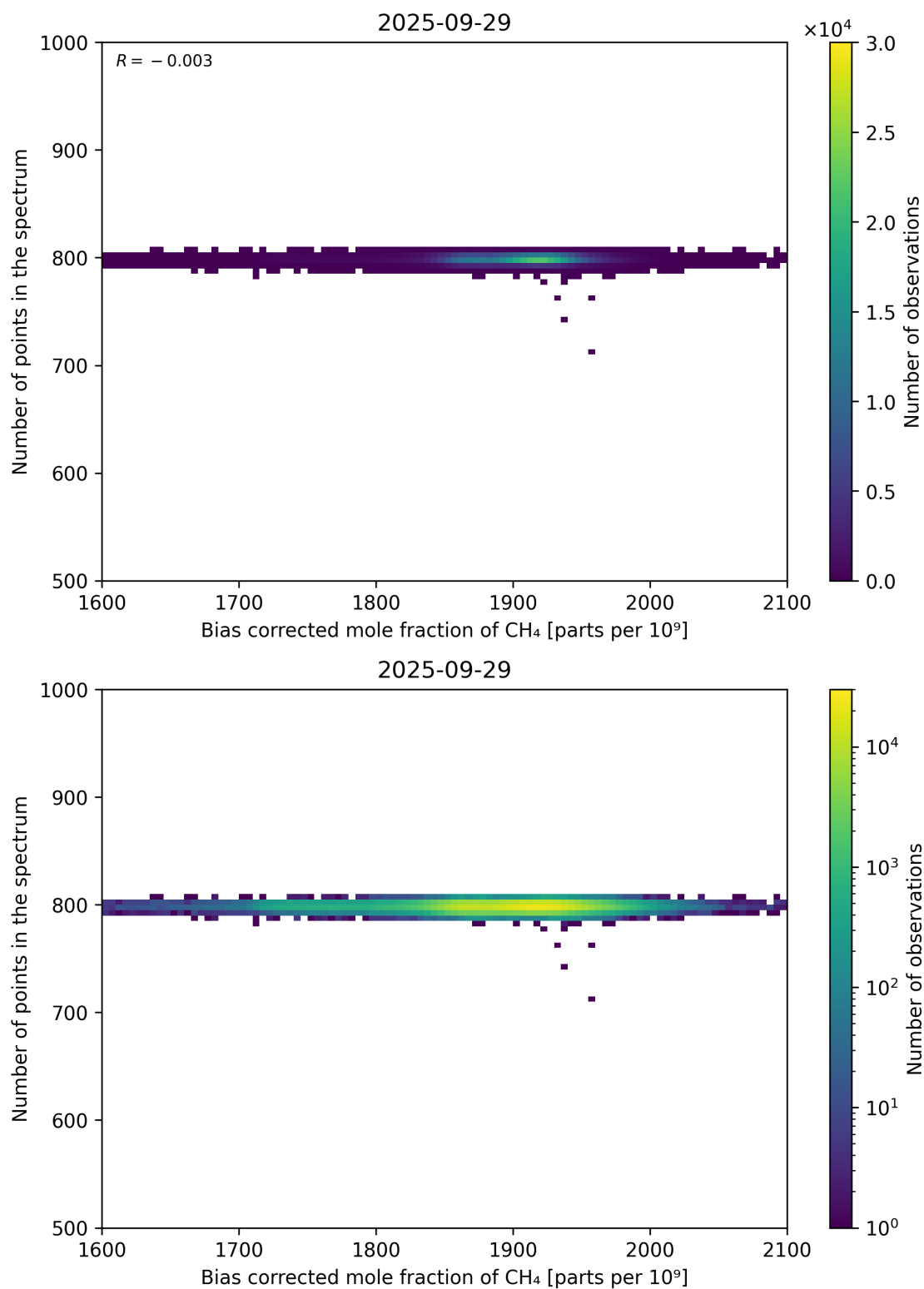
Figure 68: Scatter density plot of “Bias corrected mole fraction of CH 4 ” against “Number of points in the spectrum” for 2025-09-28 to 2025-09-30.
