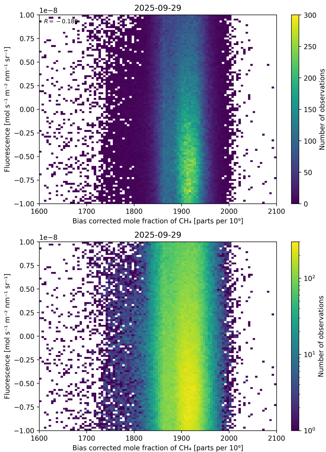
Figure 66: Scatter density plot of “Bias corrected mole fraction of CH 4 ” against “Fluorescence” for 2025-09-28 to 2025-09-30.
