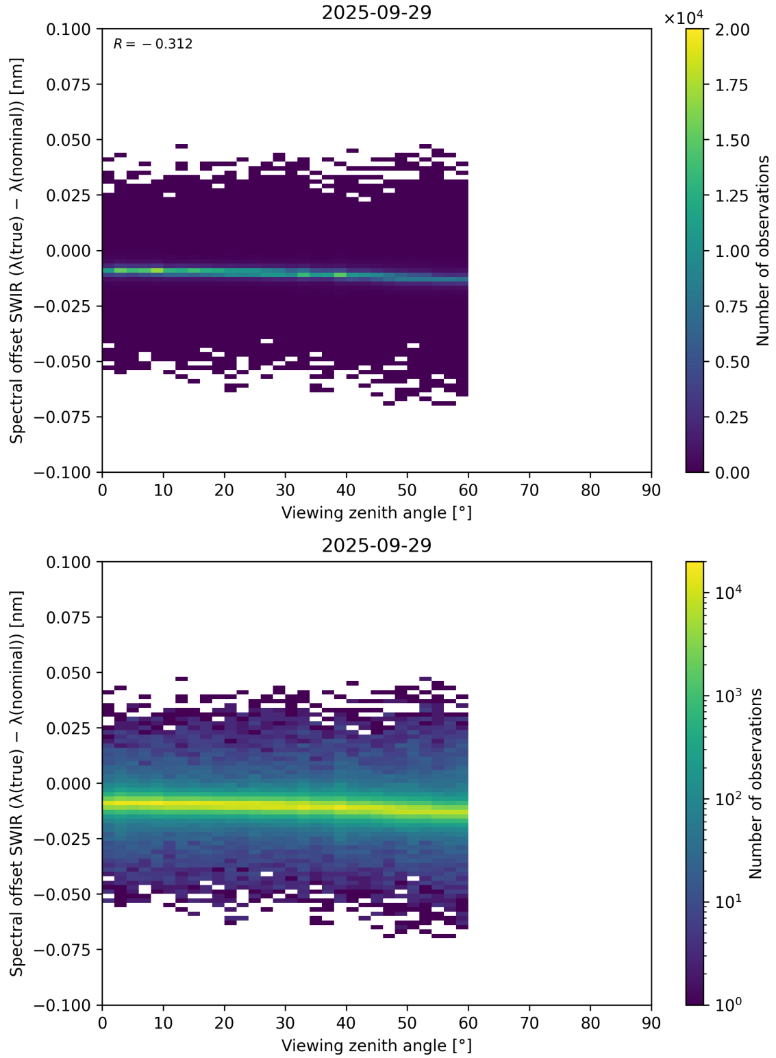
Figure 116: Scatter density plot of “Viewing zenith angle” against “Spectral offset SWIR ( \lambda_{\text{true}} - \lambda_{\text{nominal}} )” for 2025-09-28 to 2025-09-30.
