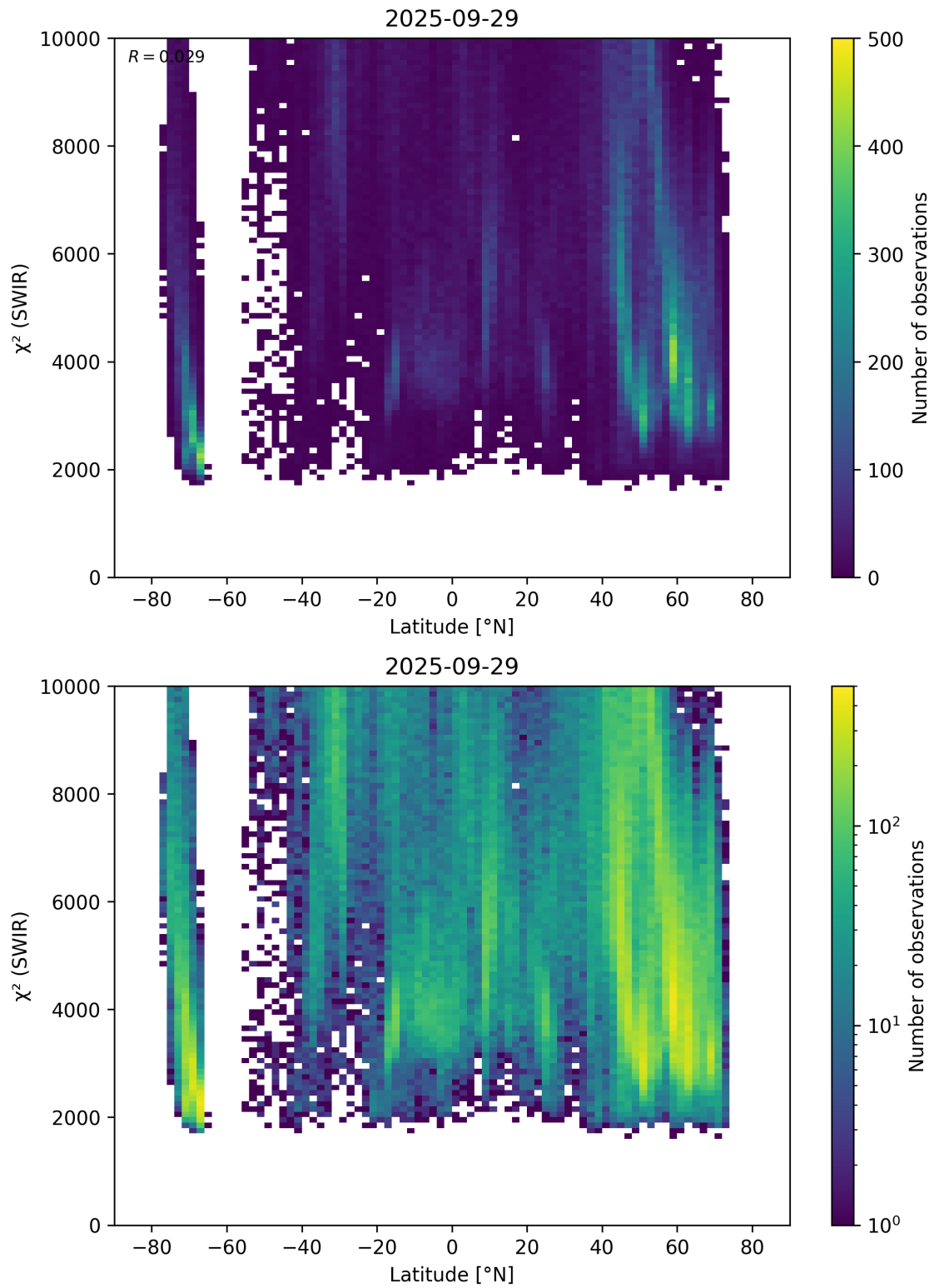
Figure 54: Scatter density plot of “Latitude” against “ \chi^2 (SWIR)” for 2025-09-28 to 2025-09-30.
