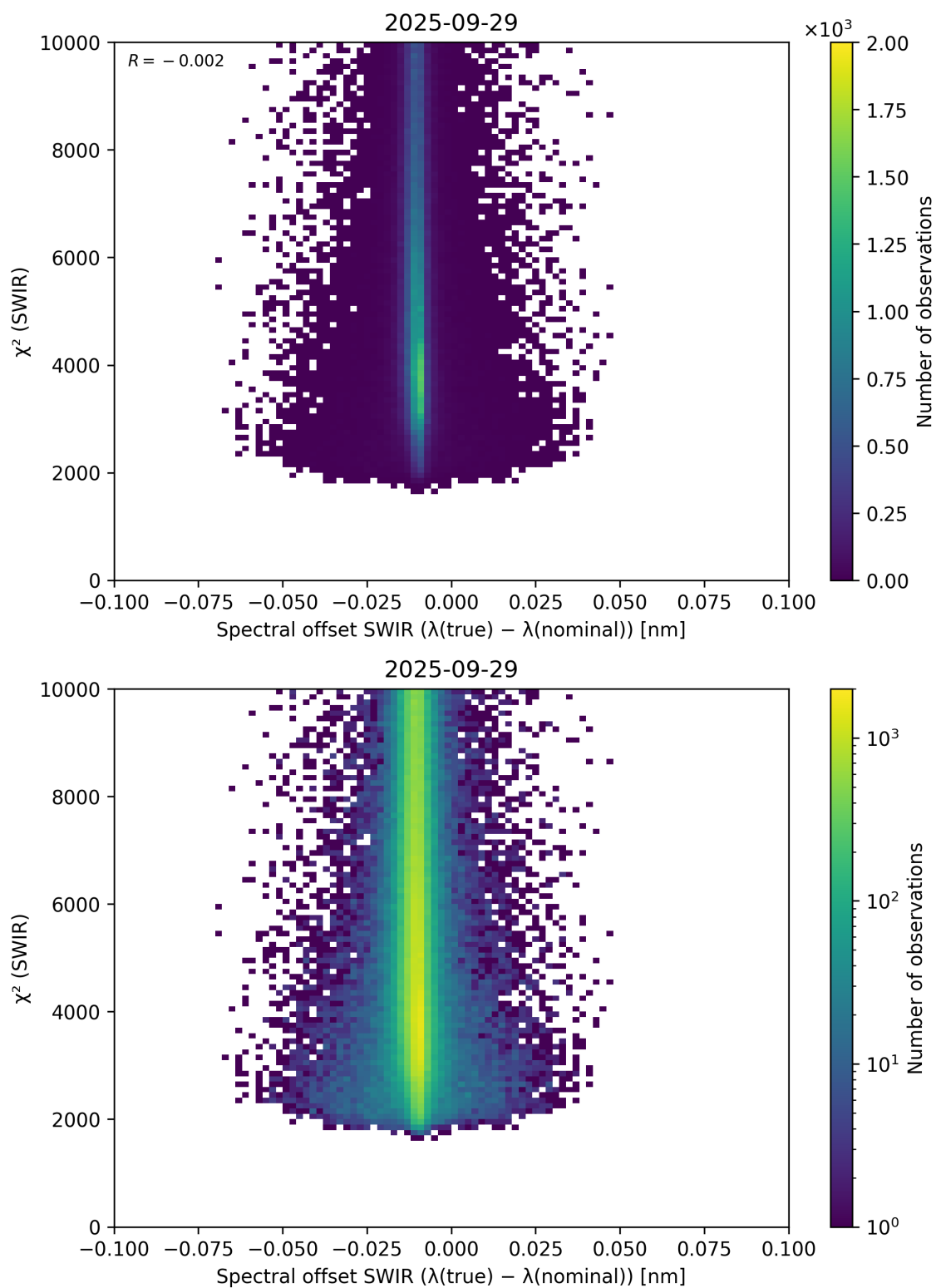
Figure 118: Scatter density plot of “Spectral offset SWIR ( \lambda_{\text{true}} - \lambda_{\text{nominal}} )” against “ \chi^2 (SWIR)” for 2025-09-28 to 2025-09-30.
