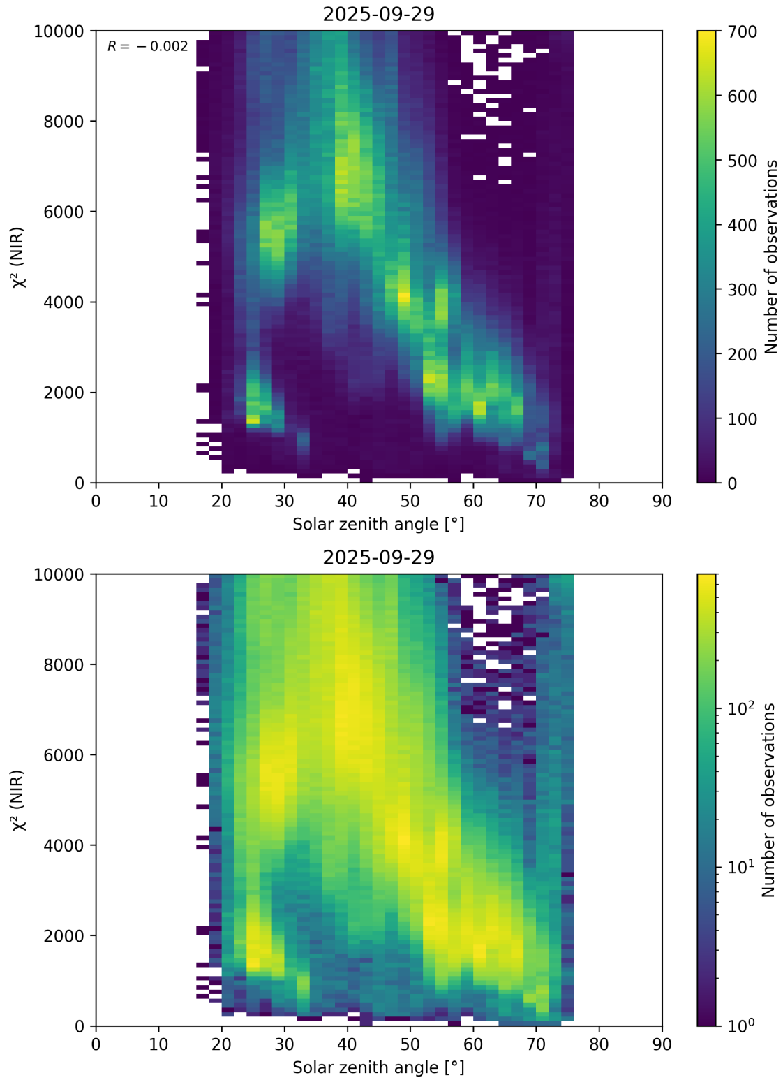
Figure 94: Scatter density plot of “Solar zenith angle” against “ \chi^2 (NIR)” for 2025-09-28 to 2025-09-30.
