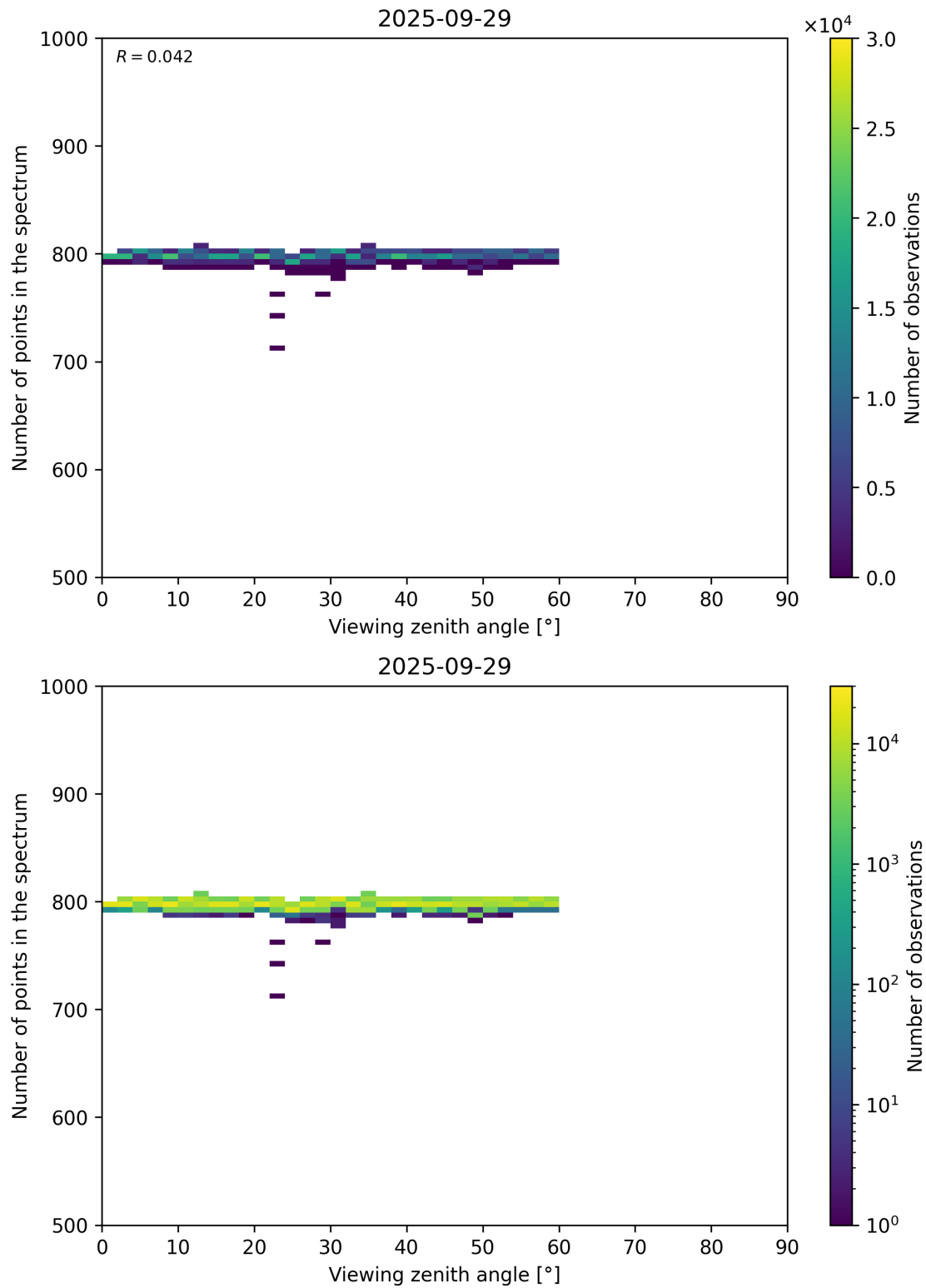
Figure 114: Scatter density plot of “Viewing zenith angle” against “Number of points in the spectrum” for 2025-09-28 to 2025-09-30.
