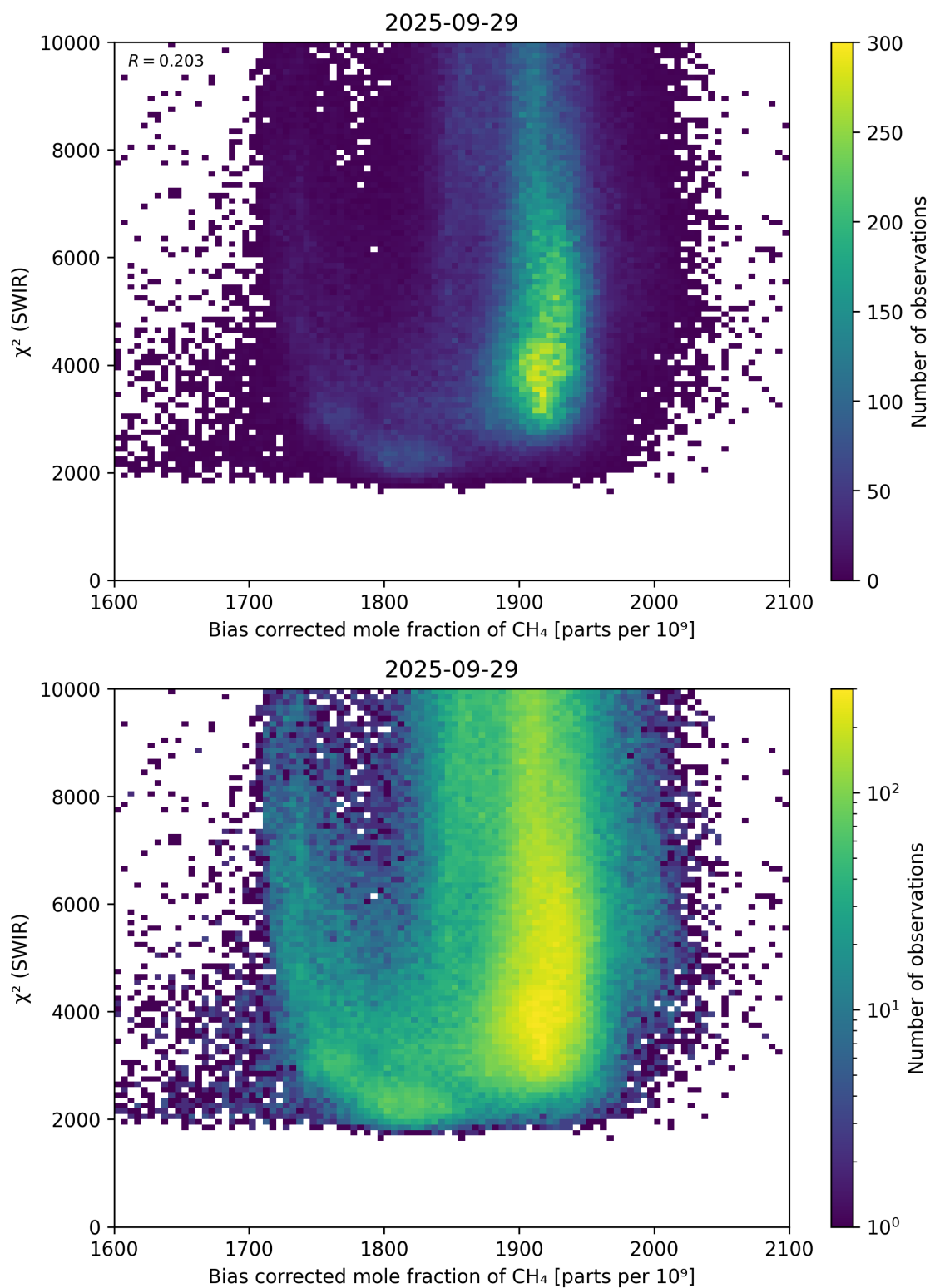
Figure 64: Scatter density plot of “Bias corrected mole fraction of \text{CH}_4 ” against “ \chi^2 (SWIR)” for 2025-09-28 to 2025-09-30.
