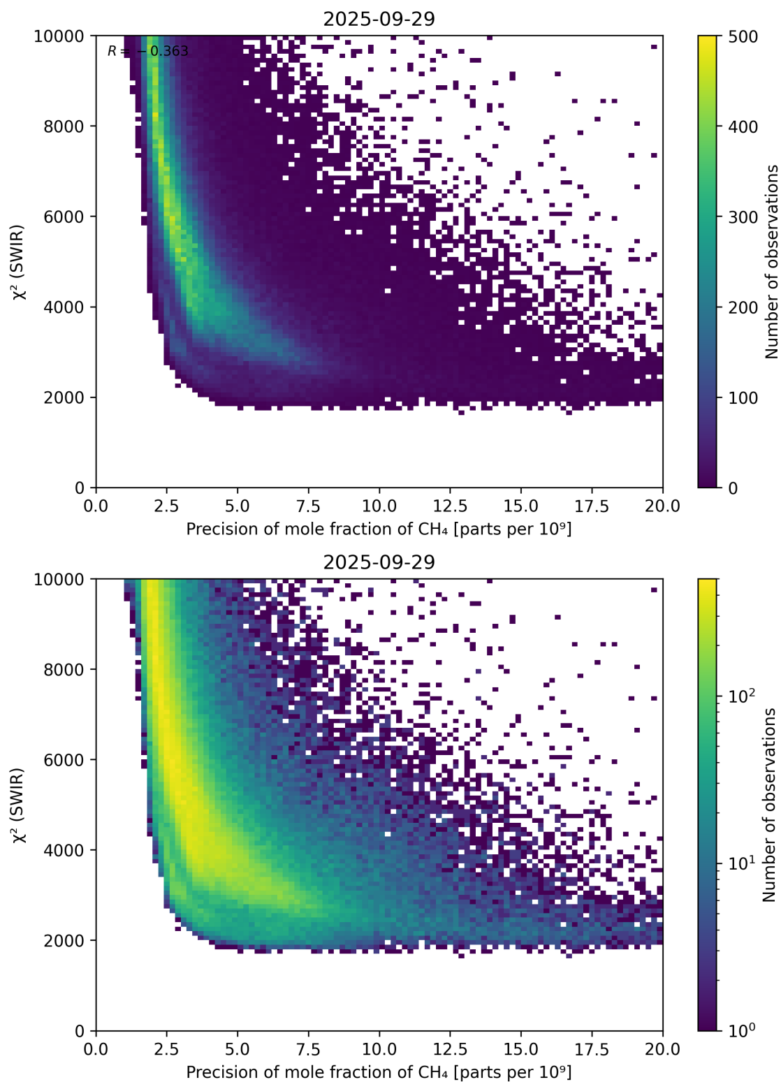
Figure 79: Scatter density plot of “Precision of mole fraction of \text{CH}_4 ” against “ \chi^2 (SWIR)” for 2025-09-28 to 2025-09-30.
