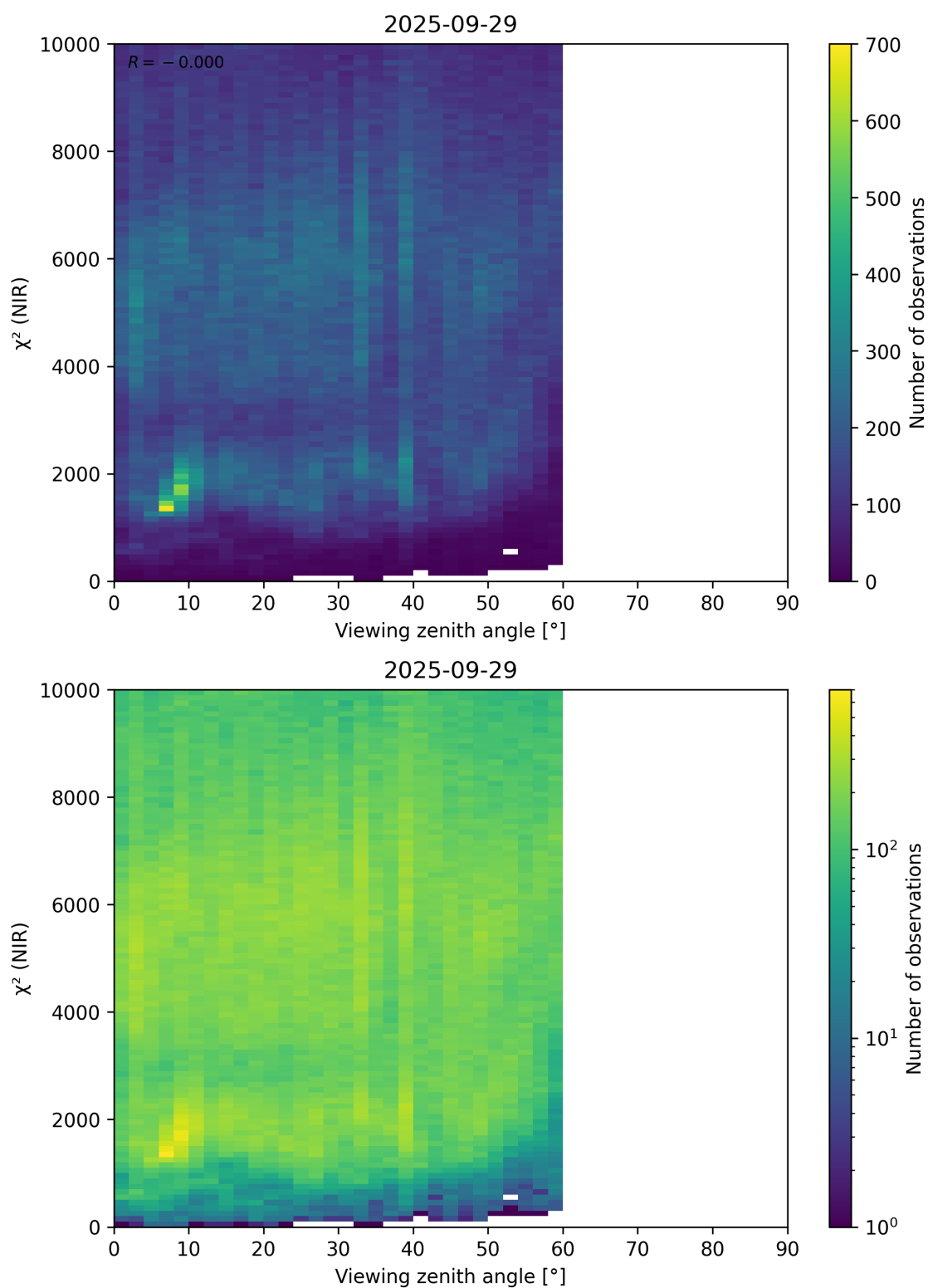
Figure 105: Scatter density plot of “Viewing zenith angle” against “ \chi^2 (NIR)” for 2025-09-28 to 2025-09-30.
