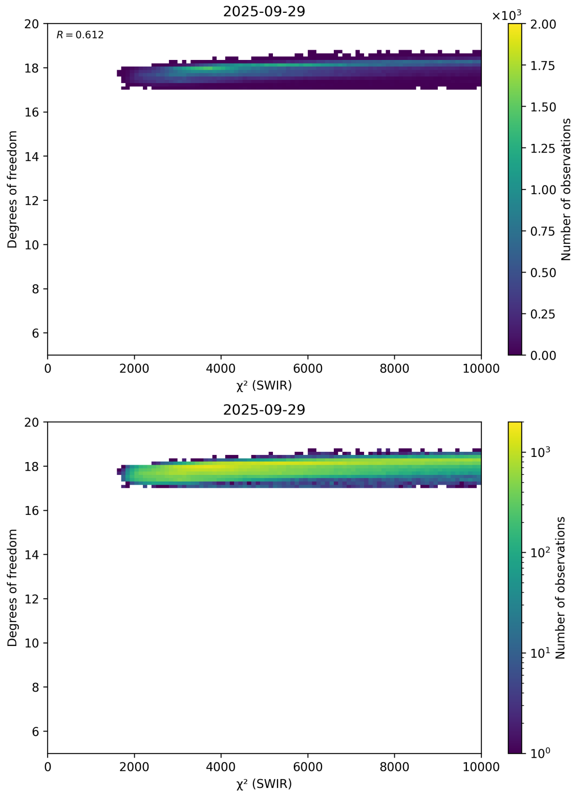
Figure 48: Scatter density plot of “ \chi^2 (SWIR)” against “Degrees of freedom” for 2025-09-28 to 2025-09-30.
