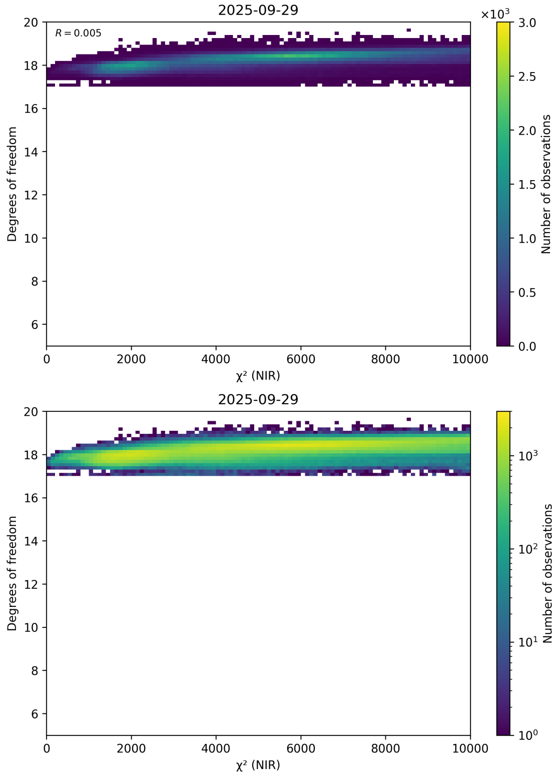
Figure 44: Scatter density plot of “ \chi^2 (NIR)” against “Degrees of freedom” for 2025-09-28 to 2025-09-30.
