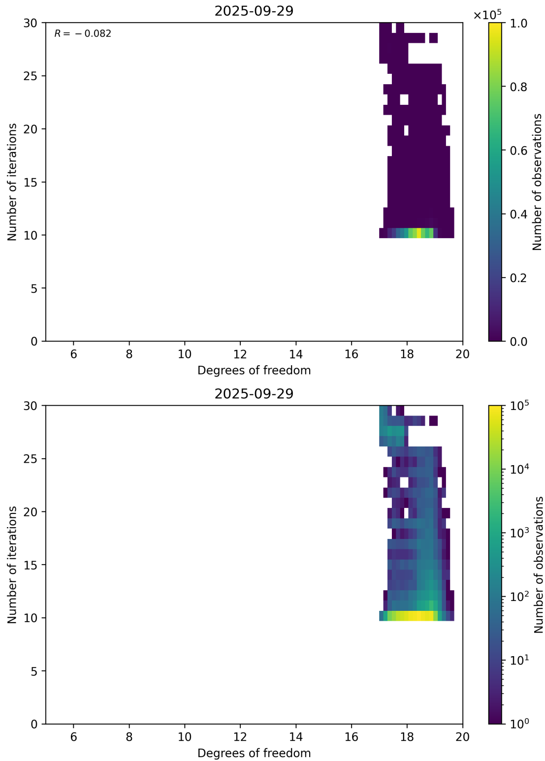
Figure 52: Scatter density plot of “Degrees of freedom” against “Number of iterations” for 2025-09-28 to 2025-09-30.
