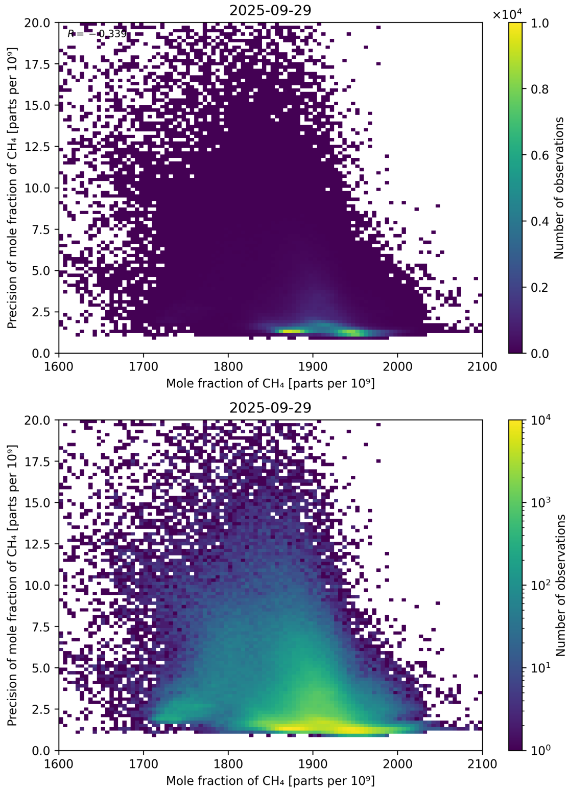
Figure 75: Scatter density plot of “Mole fraction of CH 4 ” against “Precision of mole fraction of CH 4 ” for 2025-09-28 to 2025-09-30.
