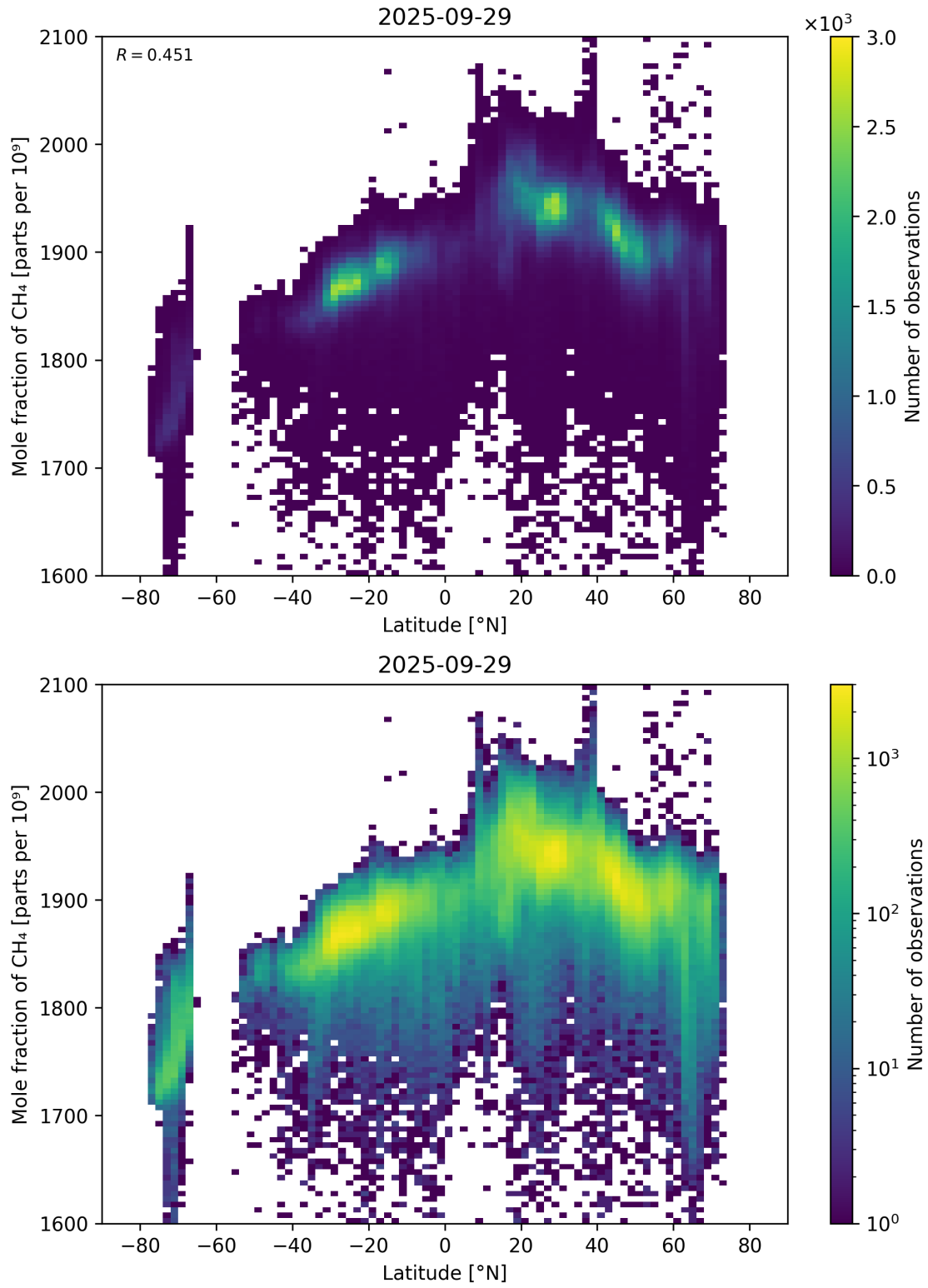
Figure 57: Scatter density plot of “Latitude” against “Mole fraction of CH 4 ” for 2025-09-28 to 2025-09-30.
