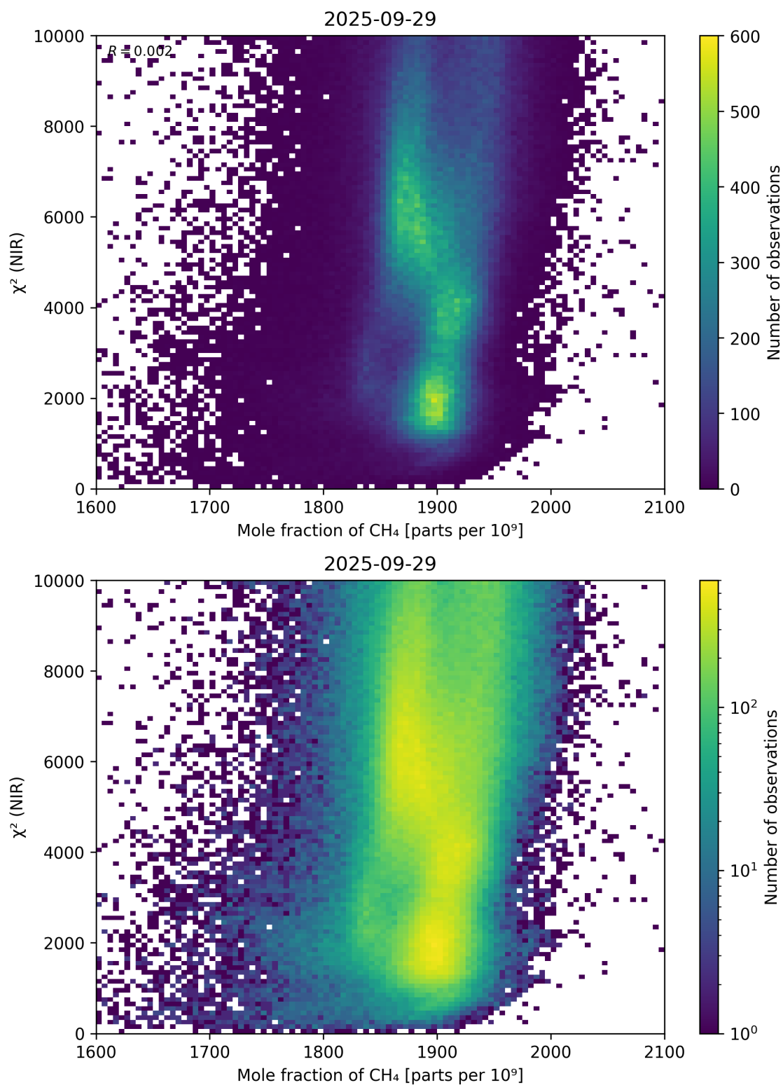
Figure 70: Scatter density plot of “Mole fraction of \text{CH}_4 ” against “ \chi^2 (NIR)” for 2025-09-28 to 2025-09-30.
