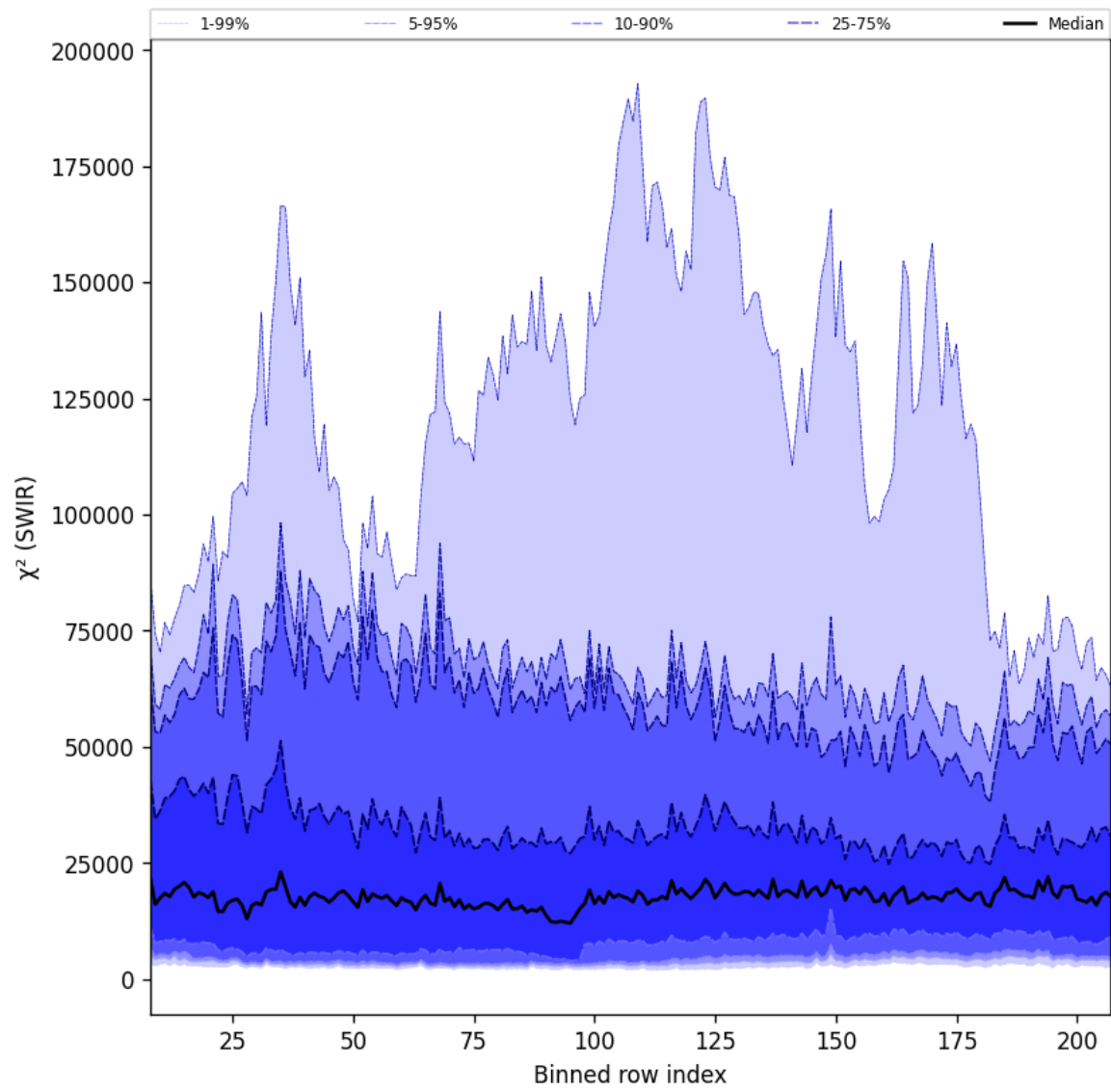
Figure 39: Along track statistics of “ \chi^2 (SWIR)” for 2025-09-28 to 2025-09-30
