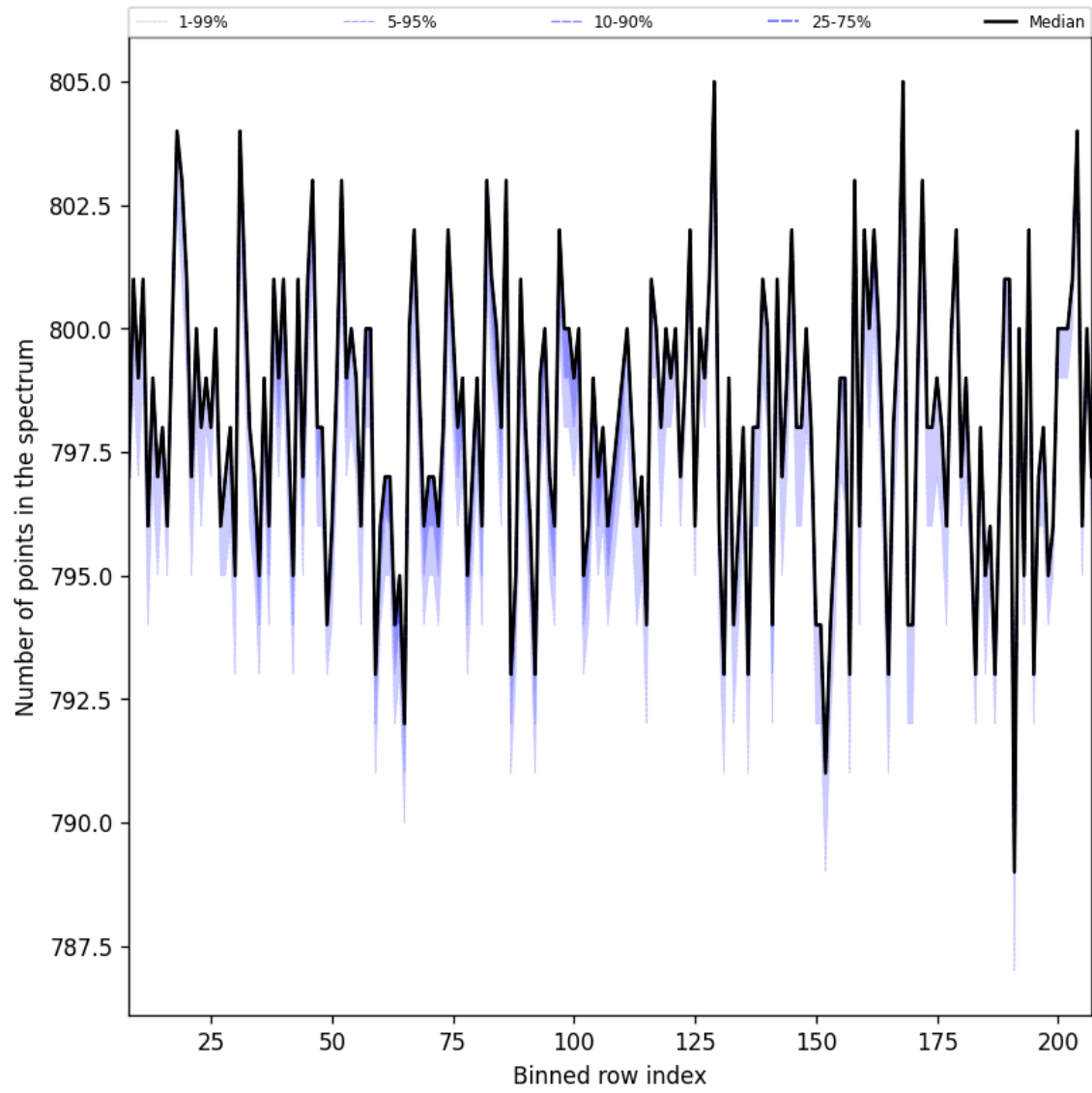
Figure 37: Along track statistics of “Number of points in the spectrum” for 2025-09-28 to 2025-09-30
