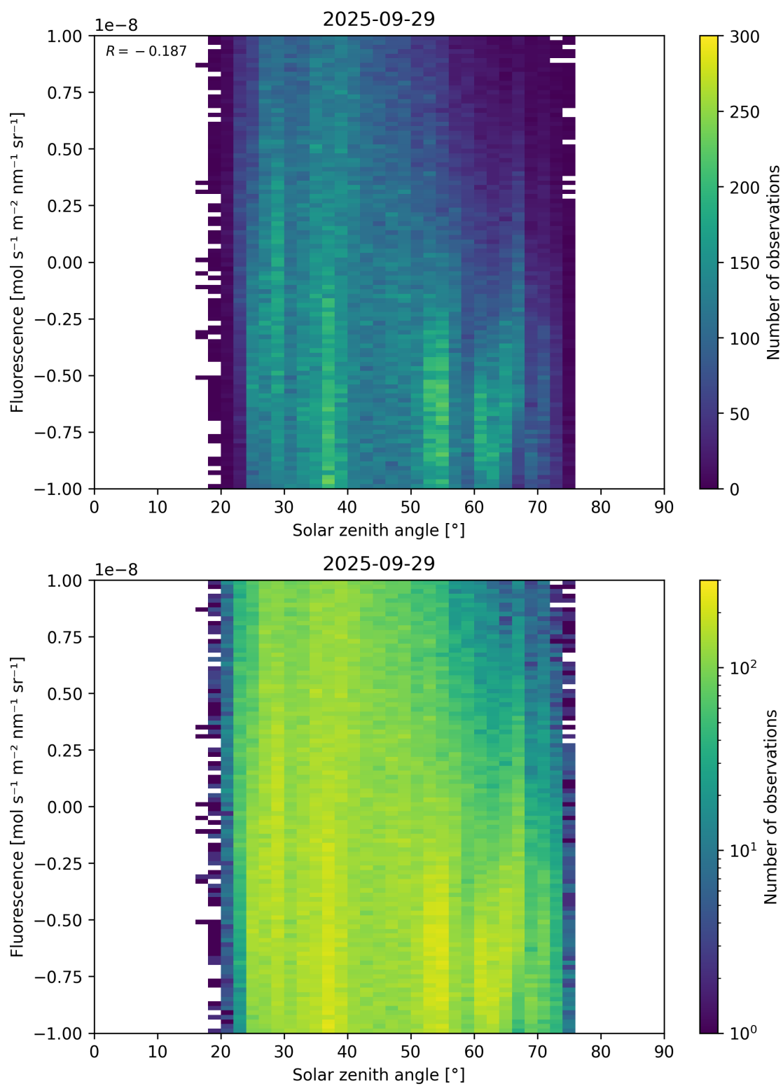
Figure 97: Scatter density plot of “Solar zenith angle” against “Fluorescence” for 2025-09-28 to 2025-09-30.
