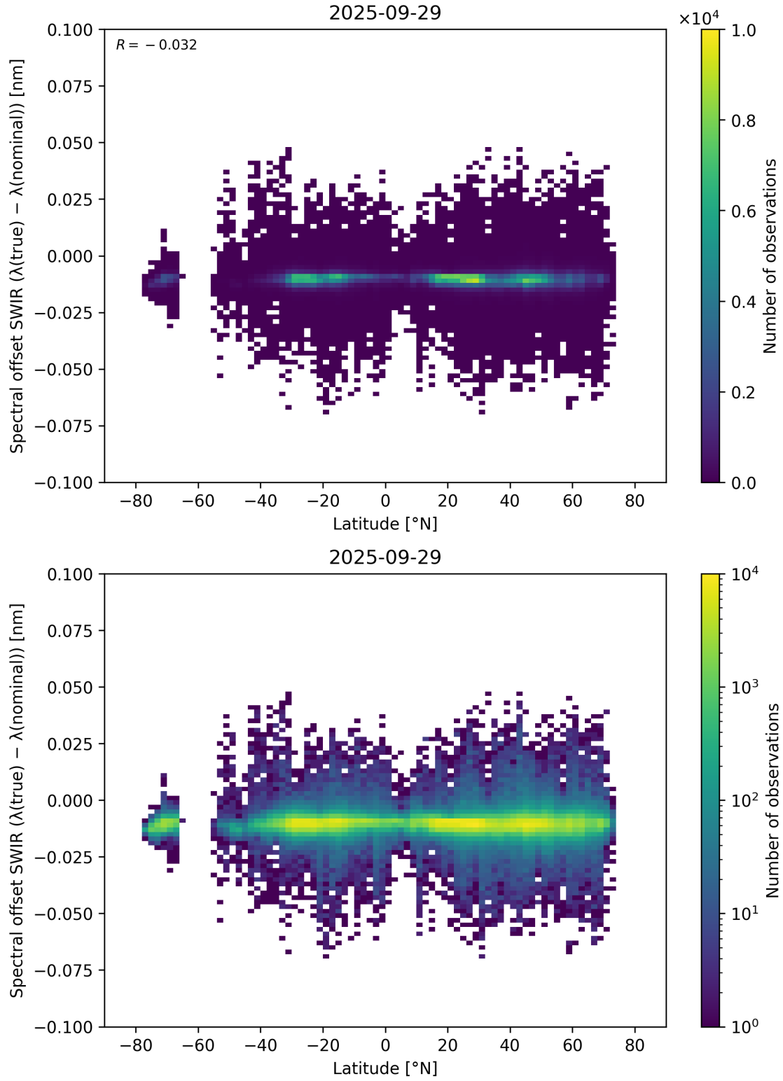
Figure 62: Scatter density plot of “Latitude” against “Spectral offset SWIR ( \lambda_{\text{true}} - \lambda_{\text{nominal}} )” for 2025-09-28 to 2025-09-30.
