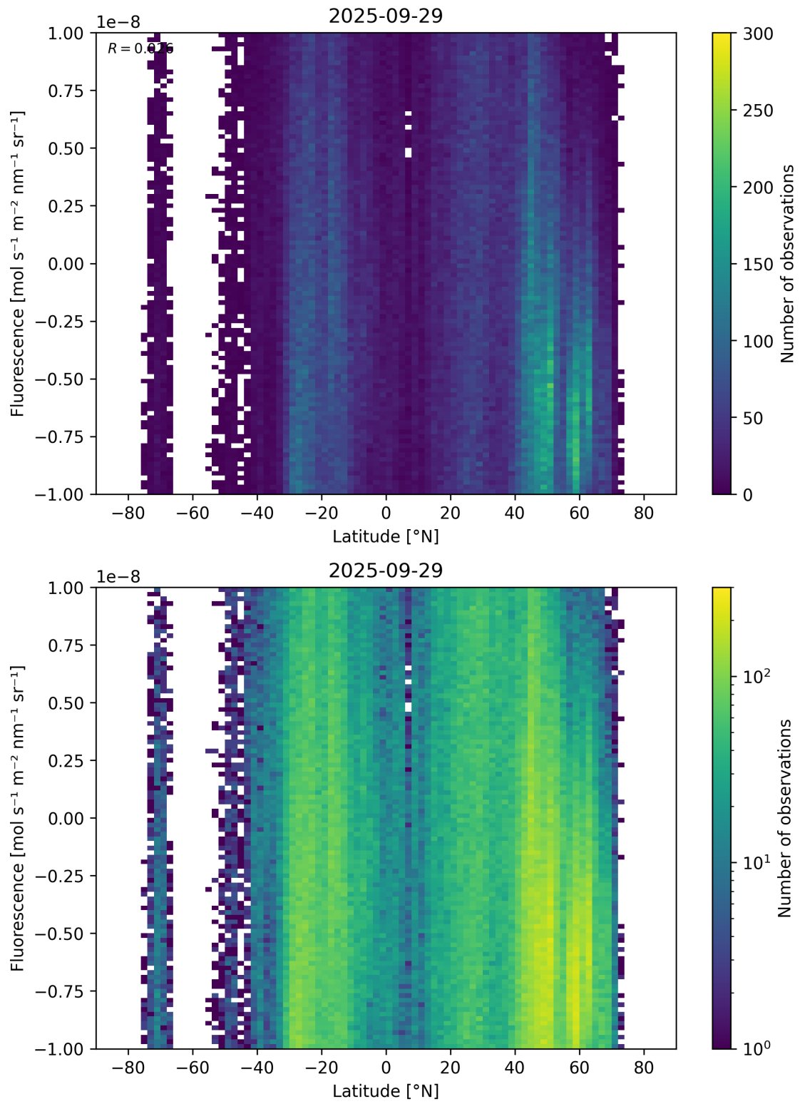
Figure 56: Scatter density plot of “Latitude” against “Fluorescence” for 2025-09-28 to 2025-09-30.
