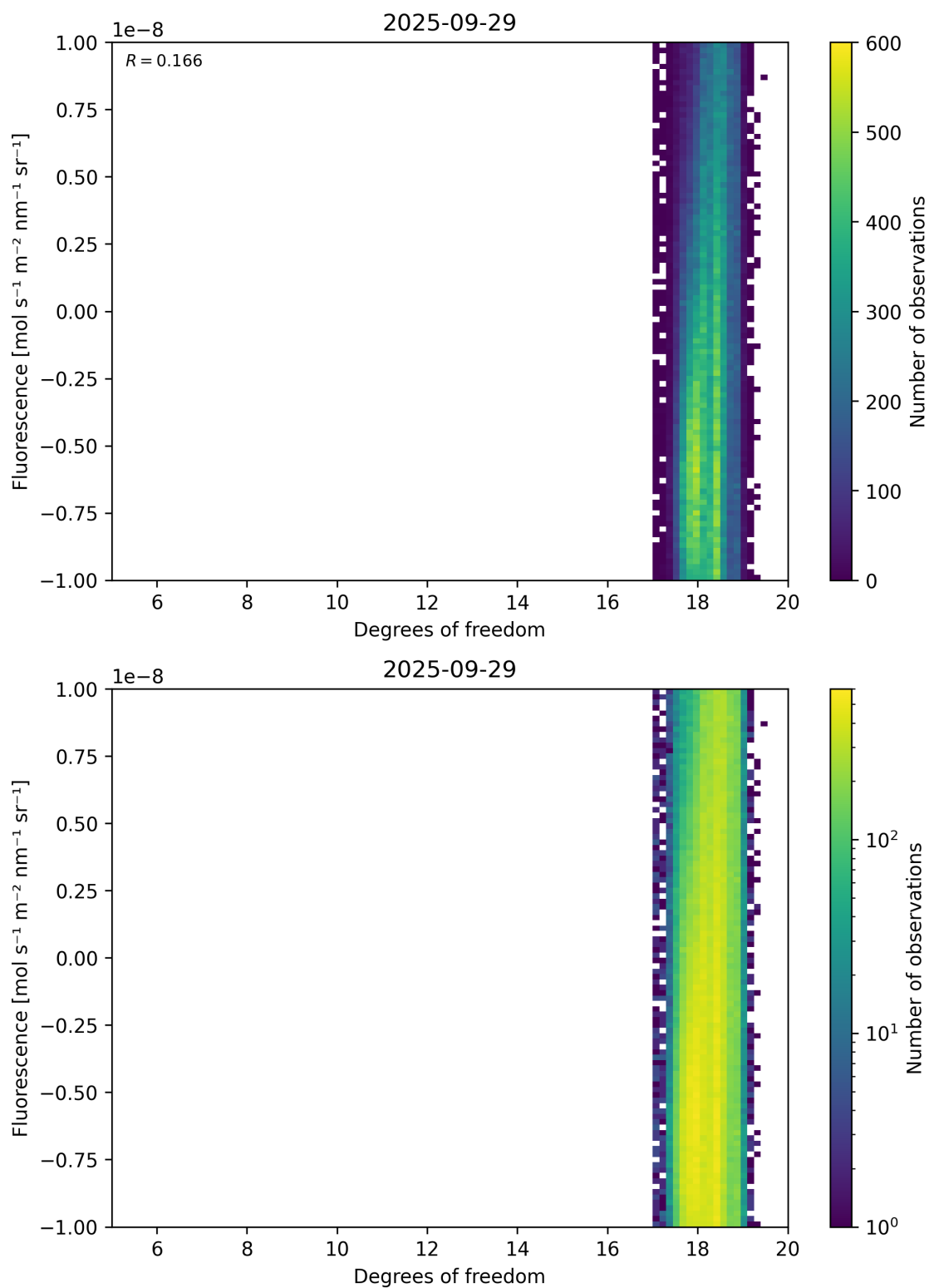
Figure 51: Scatter density plot of “Degrees of freedom” against “Fluorescence” for 2025-09-28 to 2025-09-30.
