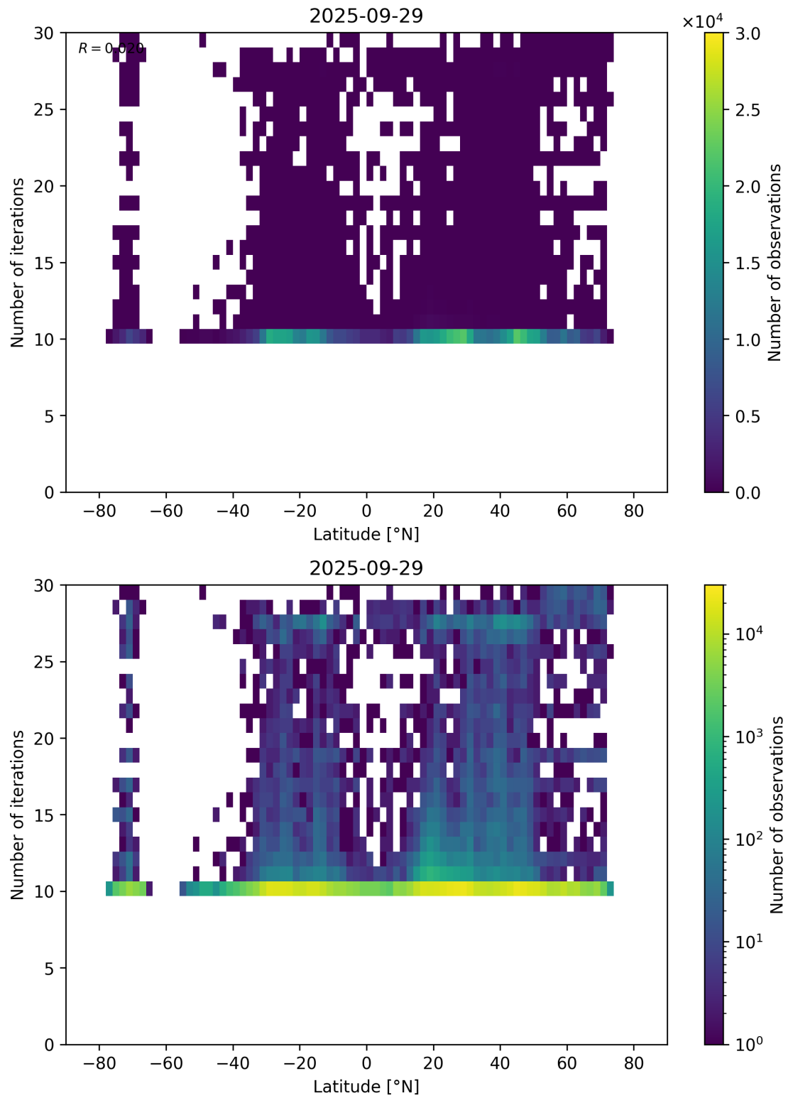
Figure 60: Scatter density plot of “Latitude” against “Number of iterations” for 2025-09-28 to 2025-09-30.
