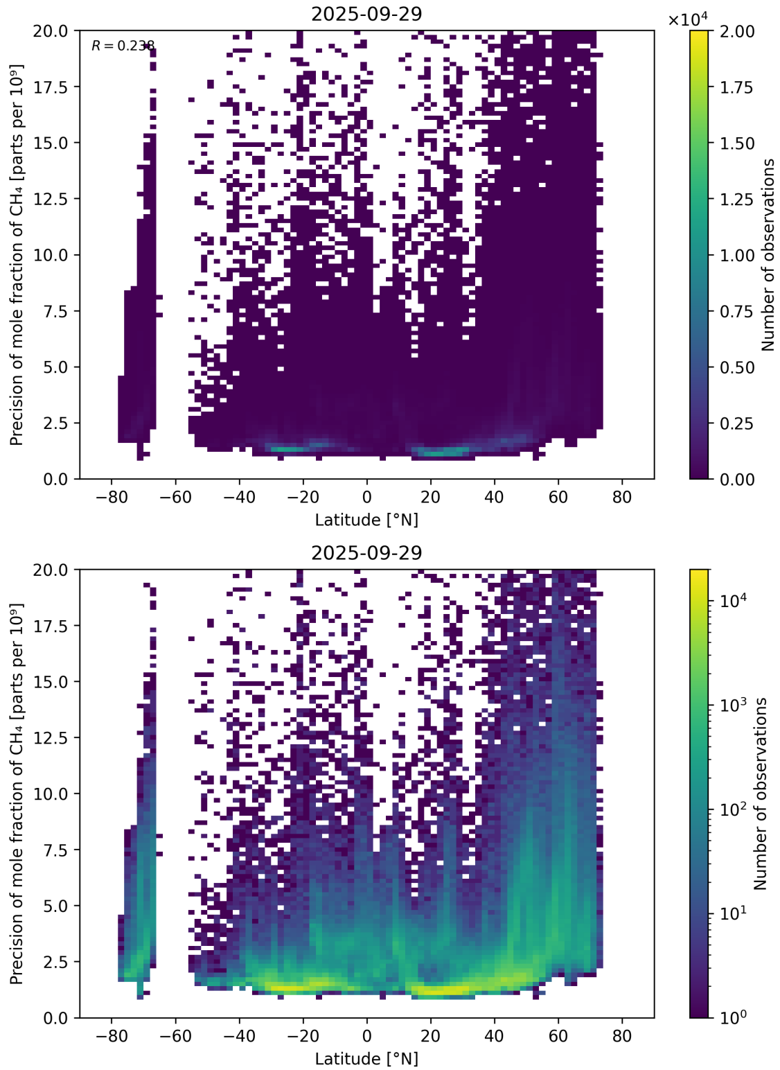
Figure 59: Scatter density plot of “Latitude” against “Precision of mole fraction of \text{CH}_4 ” for 2025-09-28 to 2025-09-30.
