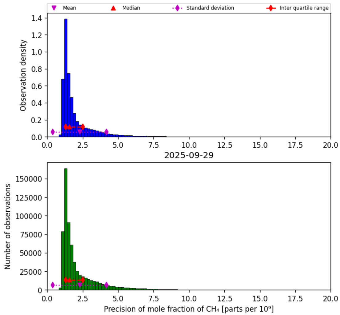
Figure 24: Histogram of “Precision of mole fraction of CH 4 ” for 2025-09-28 to 2025-09-30
