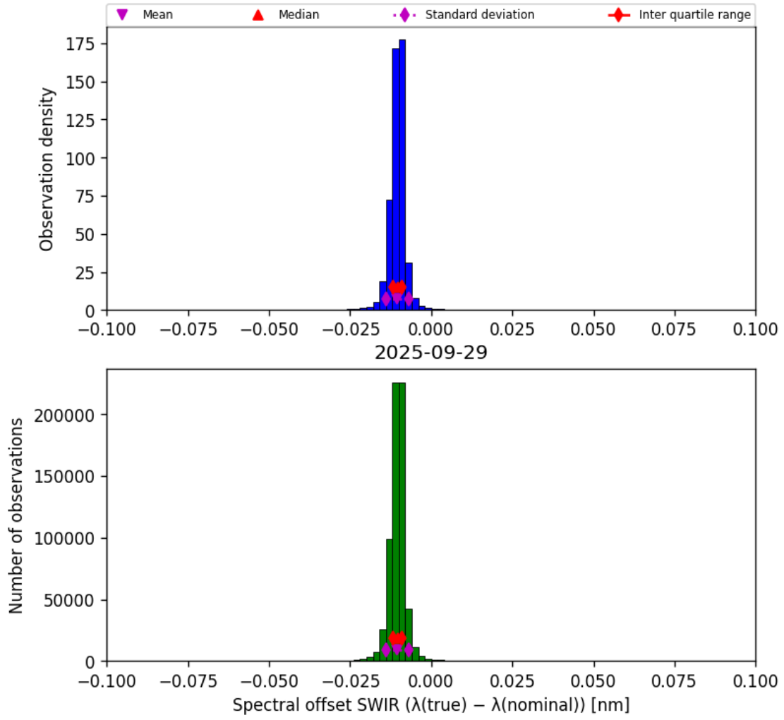
Figure 27: Histogram of “Spectral offset SWIR ( \lambda_{\text{true}} - \lambda_{\text{nominal}} )” for 2025-09-28 to 2025-09-30
