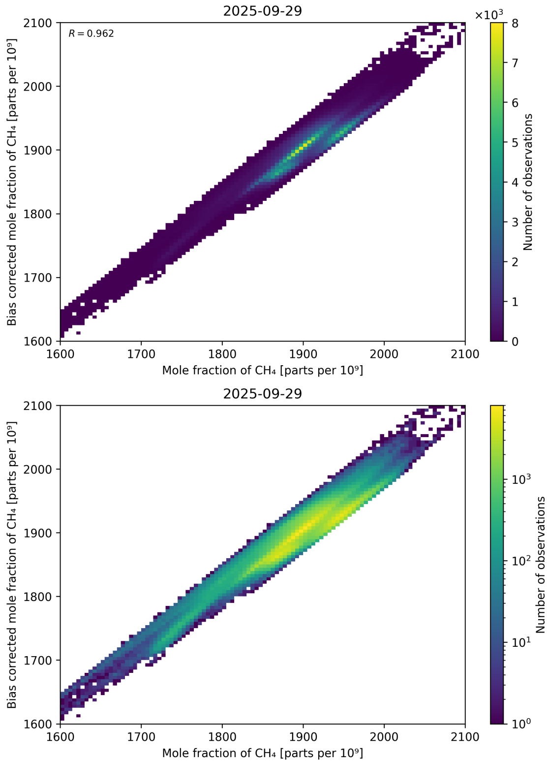
Figure 74: Scatter density plot of “Mole fraction of CH 4 ” against “Bias corrected mole fraction of CH 4 ” for 2025-09-28 to 2025-09-30.
