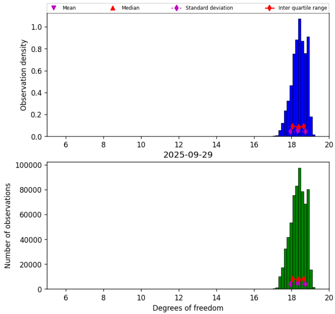
Figure 30: Histogram of “Degrees of freedom” for 2025-09-28 to 2025-09-30
