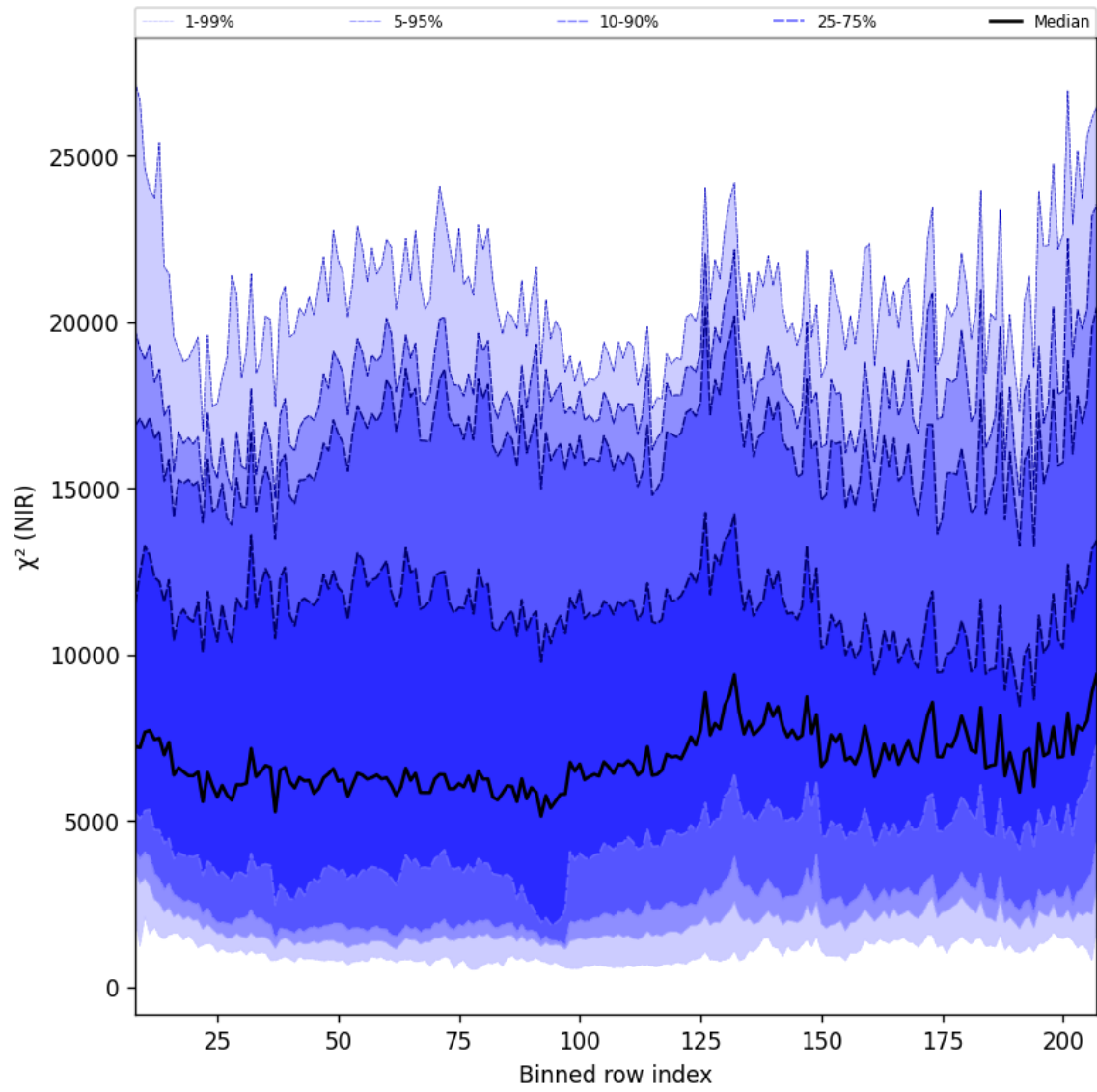
Figure 40: Along track statistics of " \chi^2 (NIR)" for 2025-09-28 to 2025-09-30
