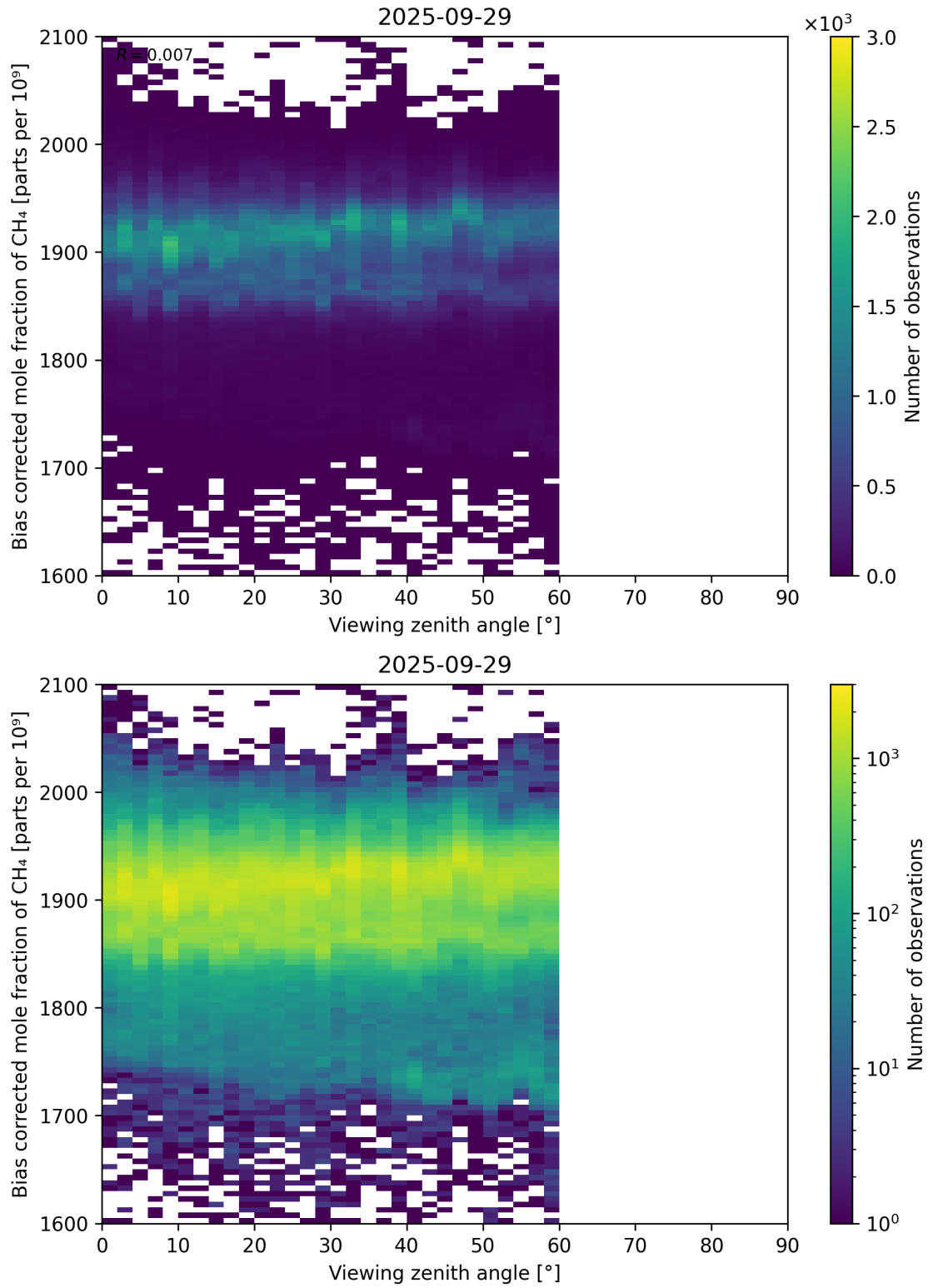
Figure 111: Scatter density plot of “Viewing zenith angle” against “Bias corrected mole fraction of CH 4 ” for 2025-09-28 to 2025-09-30.
