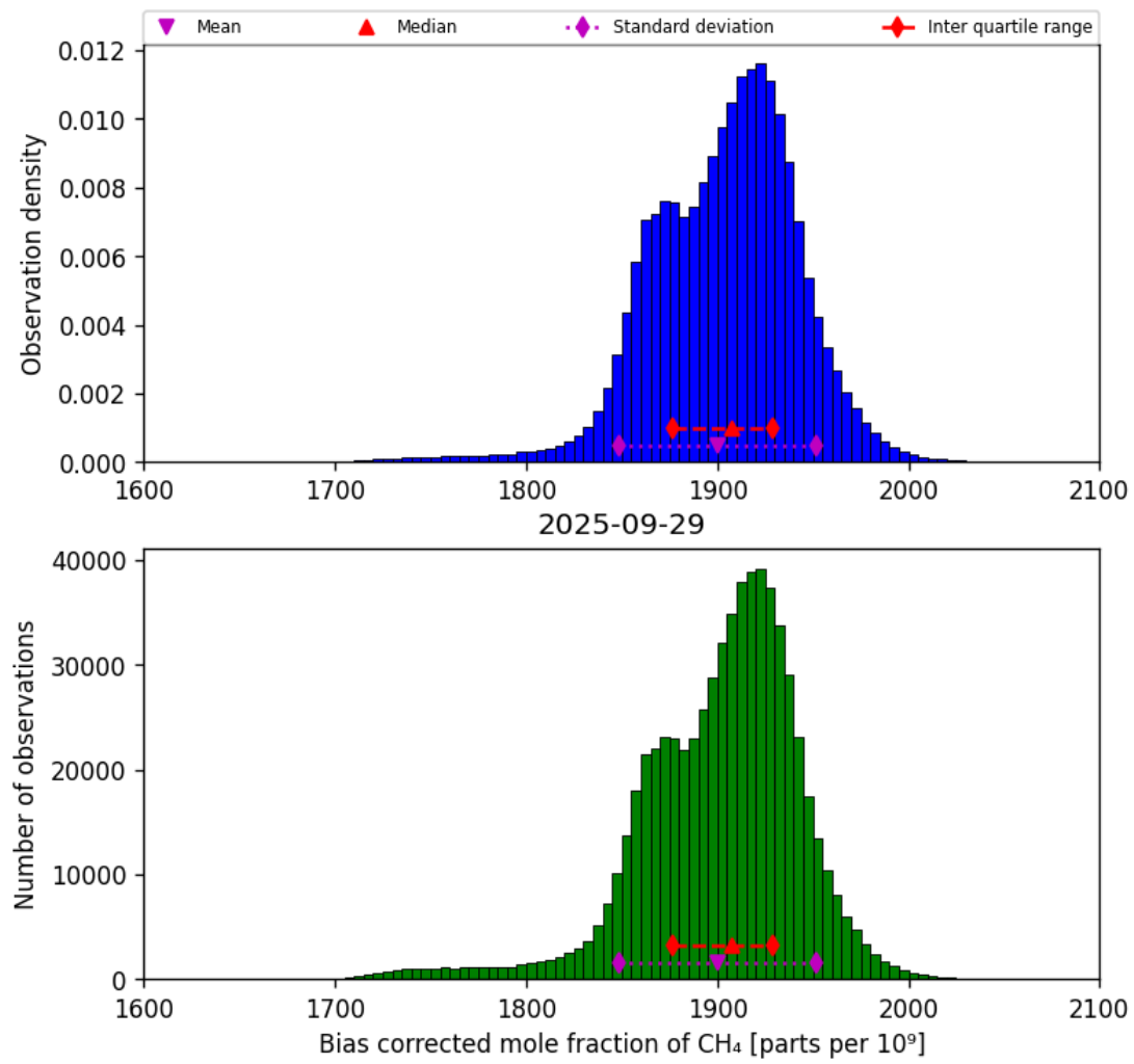
Figure 25: Histogram of “Bias corrected mole fraction of CH 4 ” for 2025-09-28 to 2025-09-30
