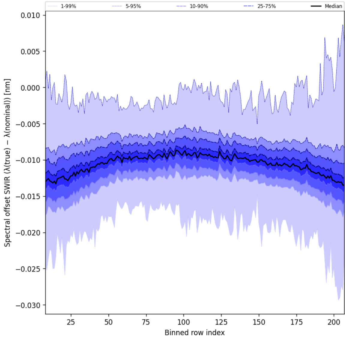
Figure 38: Along track statistics of “Spectral offset SWIR ( \lambda_{\text{true}} - \lambda_{\text{nominal}} )” for 2025-09-28 to 2025-09-30
