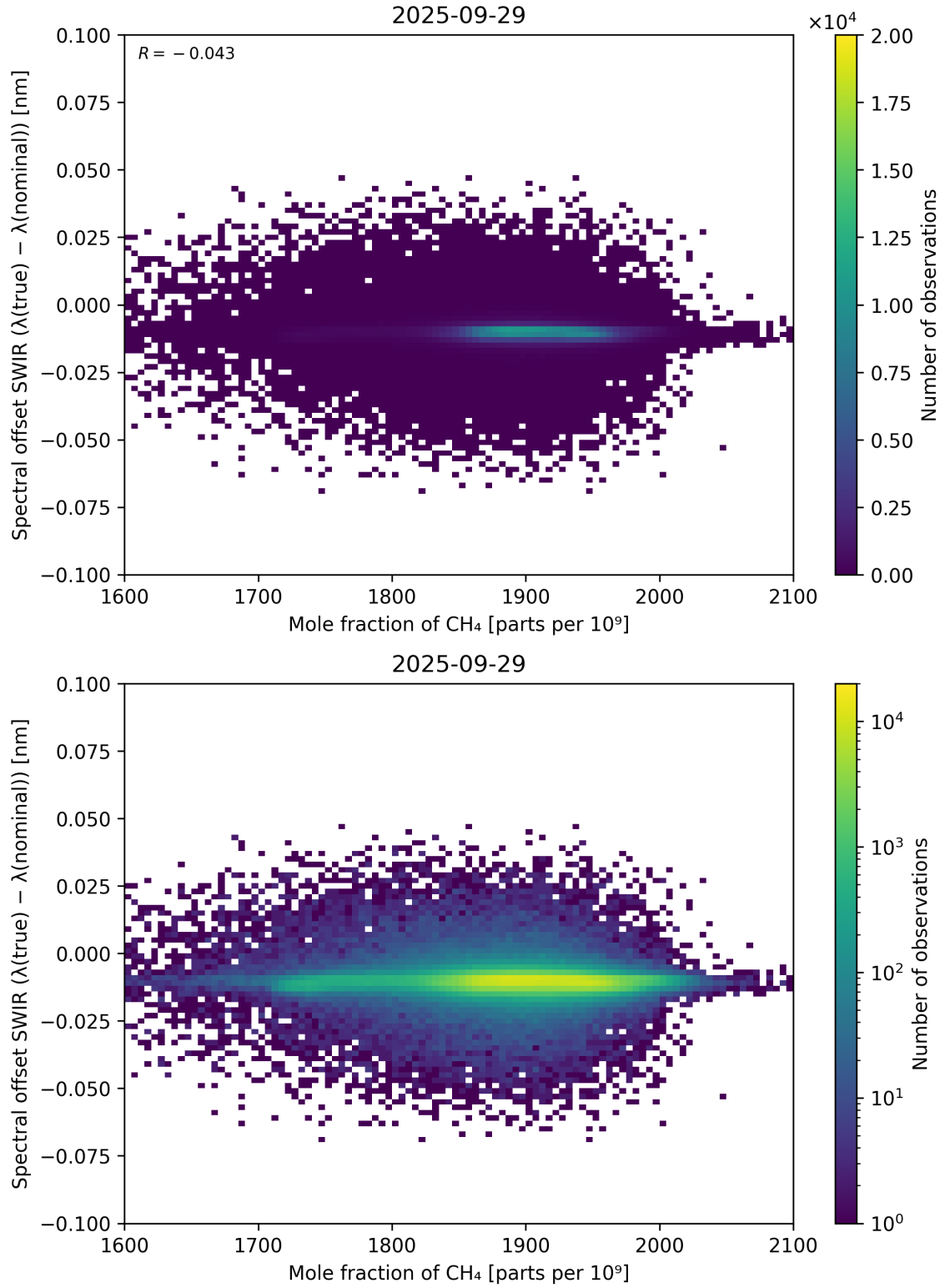
Figure 86: Scatter density plot of “Mole fraction of \text{CH}_4 ” against “Spectral offset SWIR ( \lambda_{\text{true}} - \lambda_{\text{nominal}} )” for 2025-09-28 to 2025-09-30.
