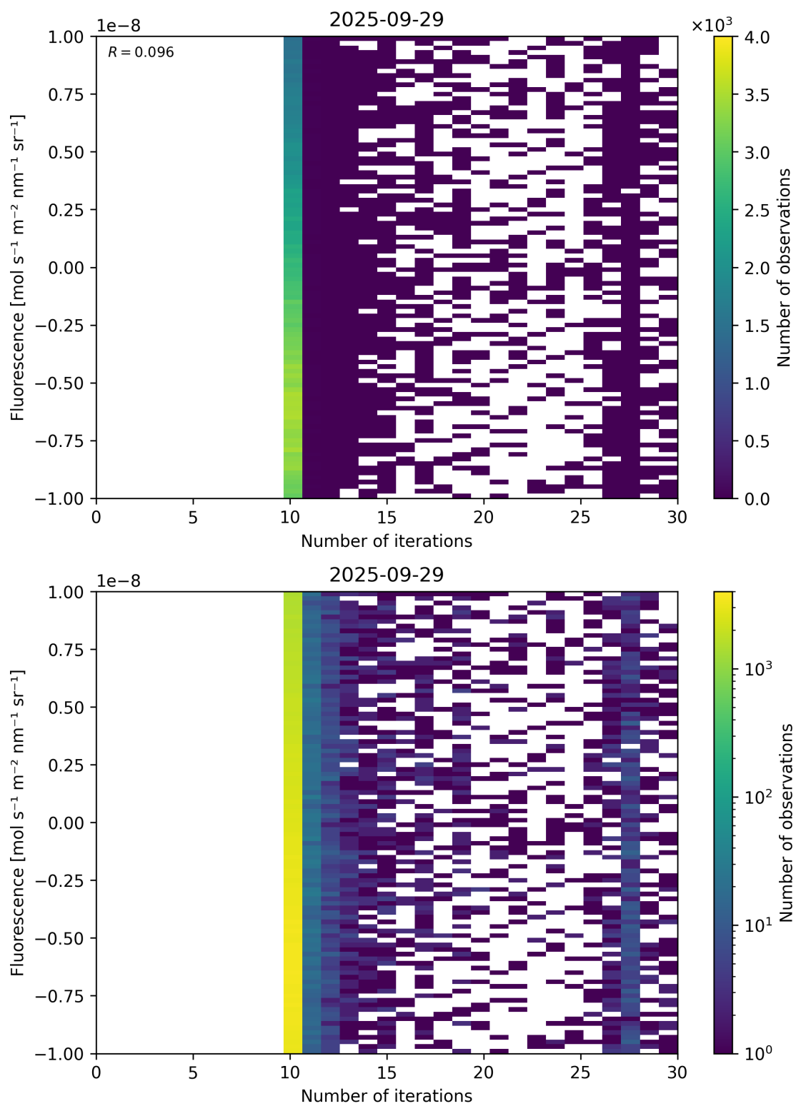
Figure 87: Scatter density plot of “Number of iterations” against “Fluorescence” for 2025-09-28 to 2025-09-30.
