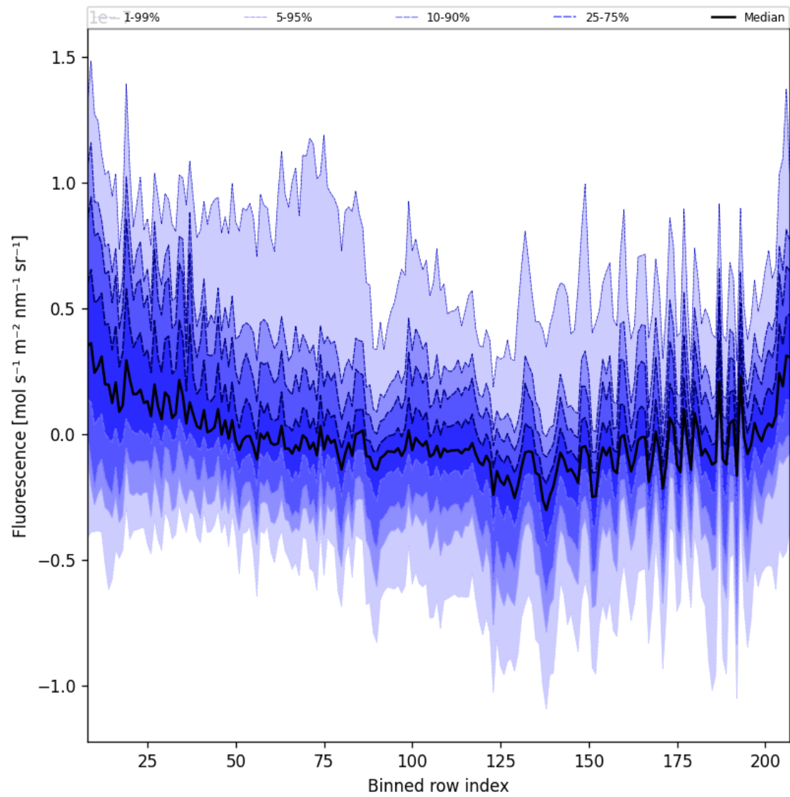
Figure 43: Along track statistics of “Fluorescence” for 2025-09-28 to 2025-09-30
