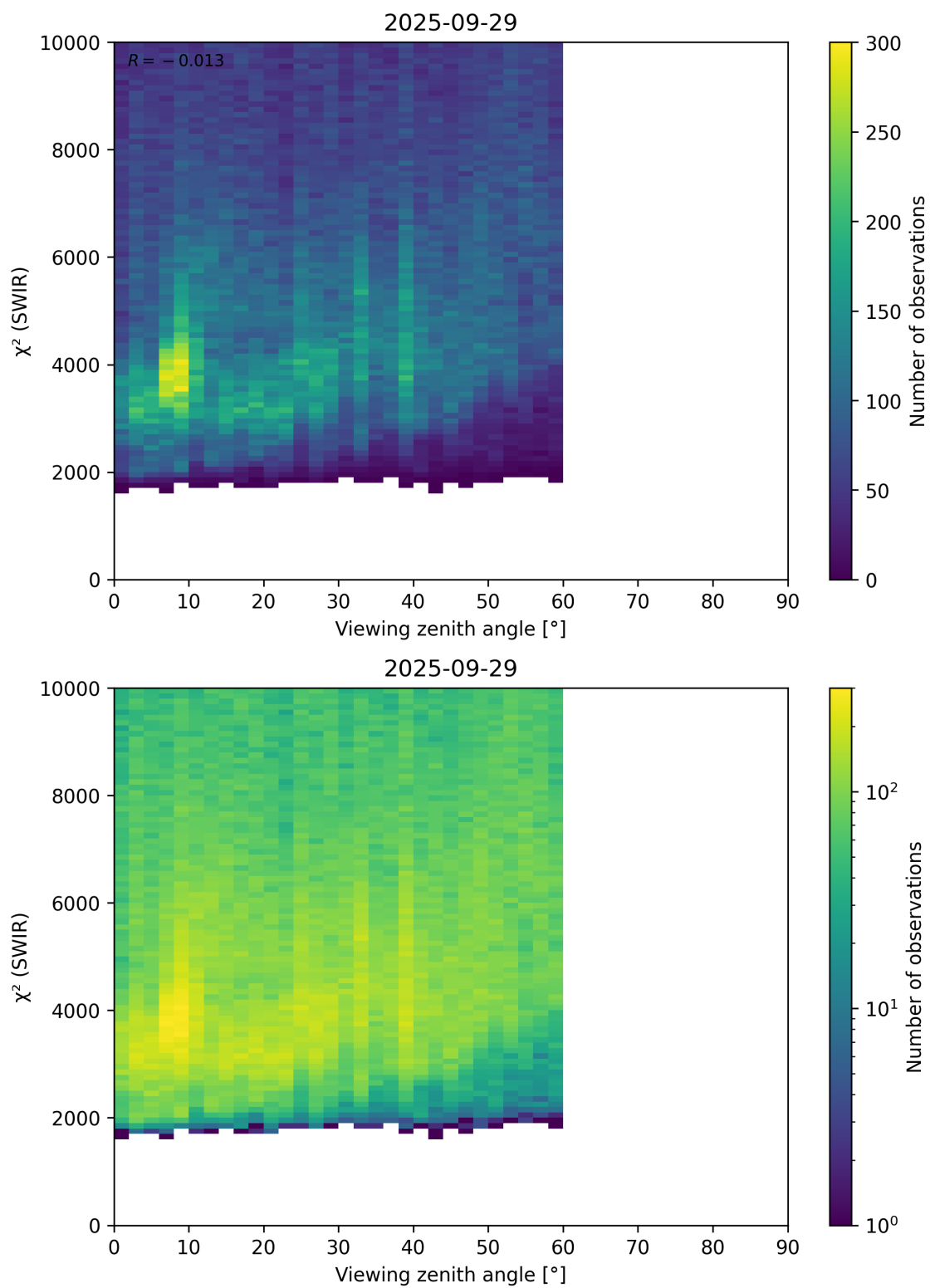
Figure 106: Scatter density plot of “Viewing zenith angle” against “ \chi^2 (SWIR)” for 2025-09-28 to 2025-09-30.
