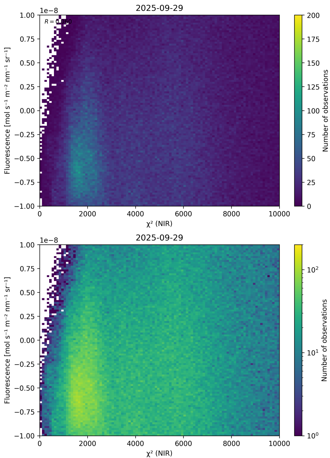
Figure 45: Scatter density plot of “ \chi^2 (NIR)” against “Fluorescence” for 2025-09-28 to 2025-09-30.
