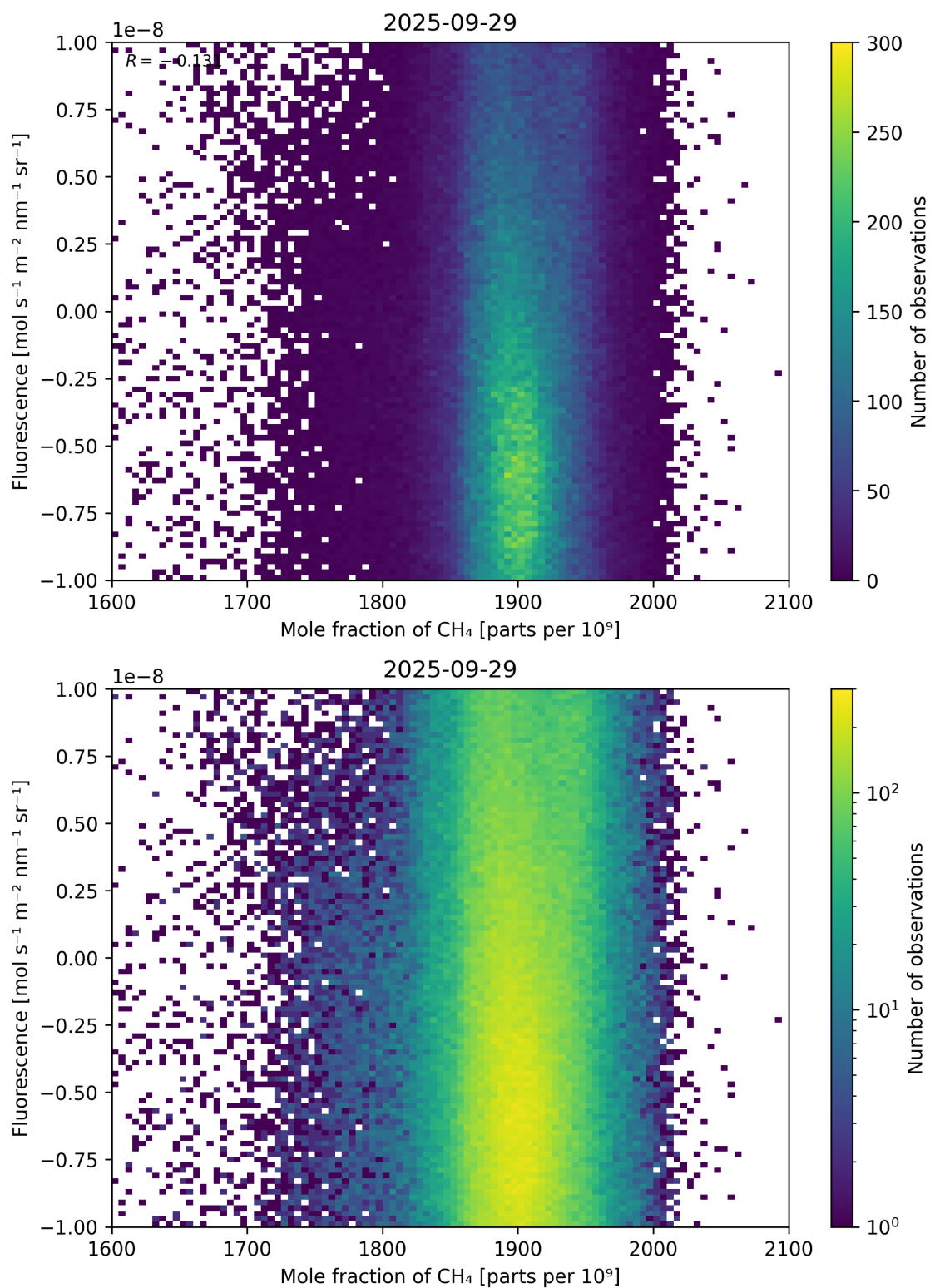
Figure 73: Scatter density plot of “Mole fraction of \text{CH}_4 ” against “Fluorescence” for 2025-09-28 to 2025-09-30.
