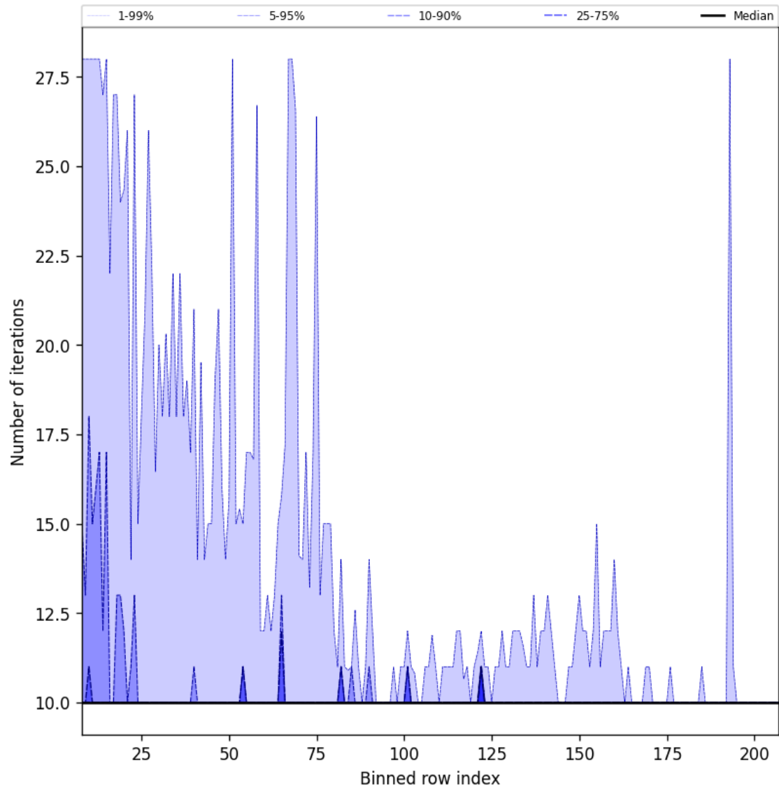
Figure 42: Along track statistics of “Number of iterations” for 2025-09-28 to 2025-09-30
