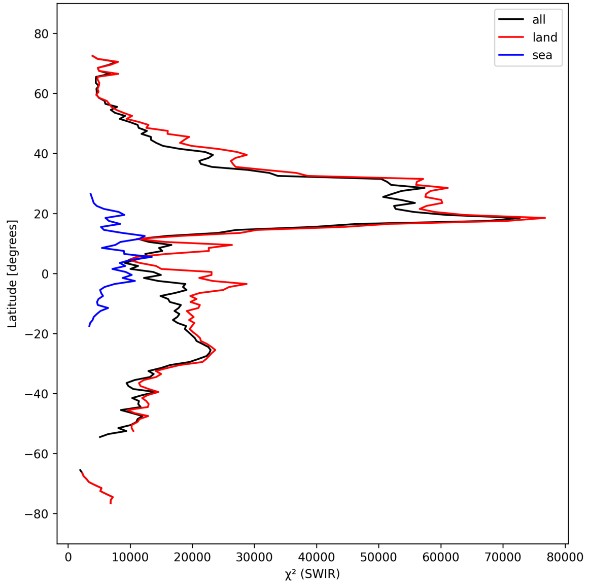
Figure 17: Zonal average of “ \chi^2 (SWIR)” for 2025-09-28 to 2025-09-30.
