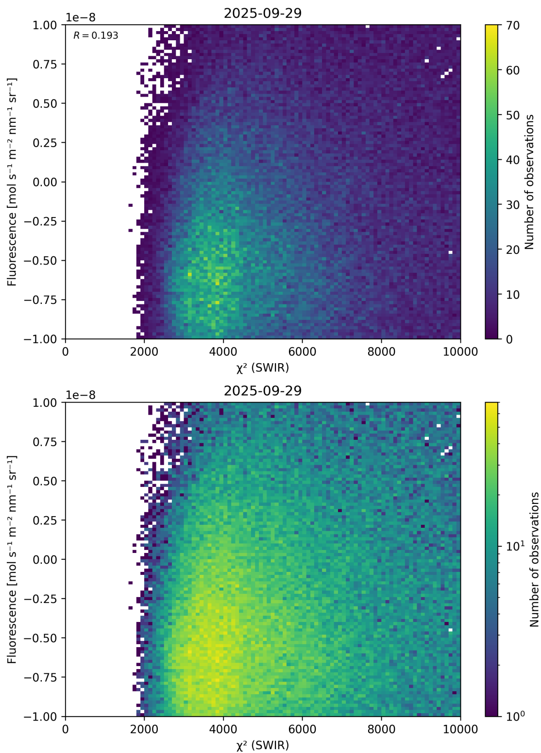
Figure 49: Scatter density plot of “ \chi^2 (SWIR)” against “Fluorescence” for 2025-09-28 to 2025-09-30.
