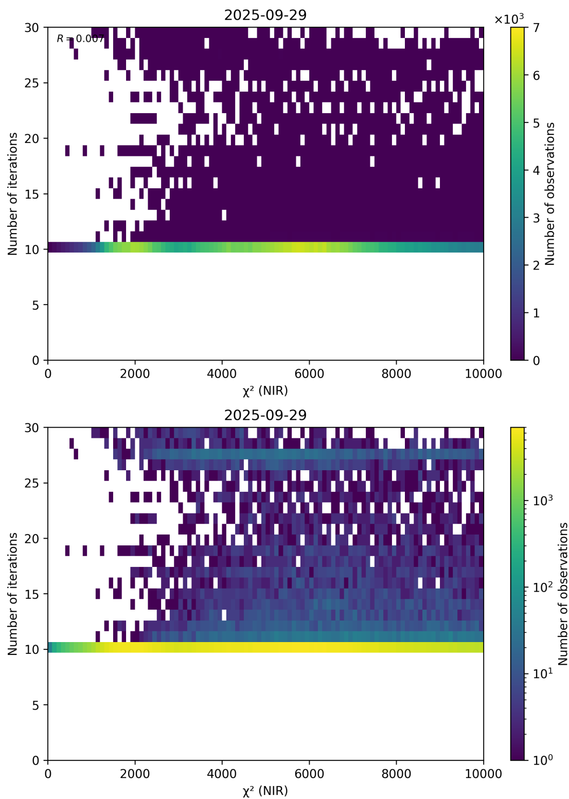
Figure 46: Scatter density plot of “ \chi^2 (NIR)” against “Number of iterations” for 2025-09-28 to 2025-09-30.
