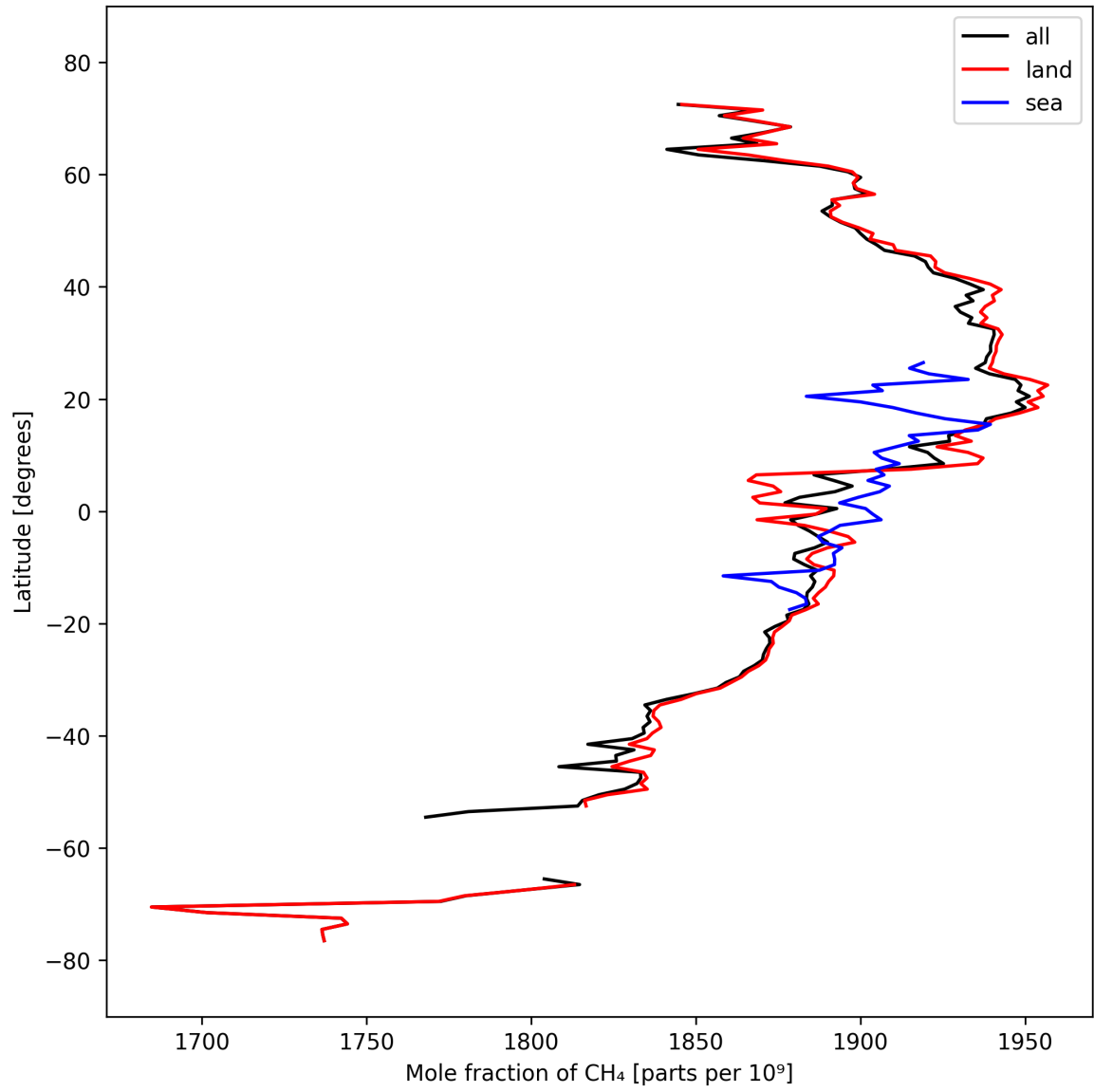
Figure 12: Zonal average of “Mole fraction of \text{CH}_4 ” for 2025-09-28 to 2025-09-30.
