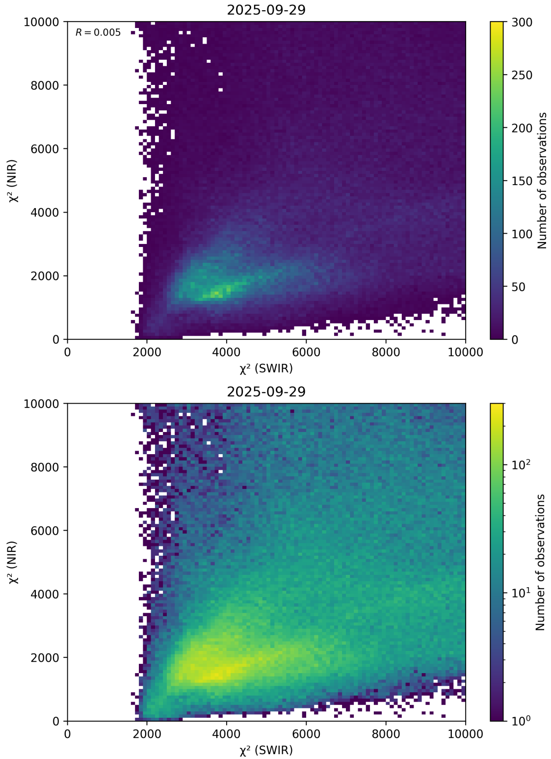
Figure 47: Scatter density plot of “ \chi^2 (SWIR)” against “ \chi^2 (NIR)” for 2025-09-28 to 2025-09-30.
