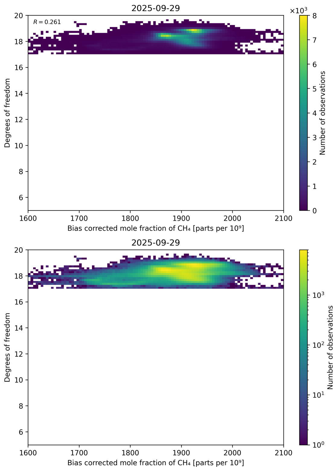
Figure 65: Scatter density plot of “Bias corrected mole fraction of CH 4 ” against “Degrees of freedom” for 2025-09-28 to 2025-09-30.
