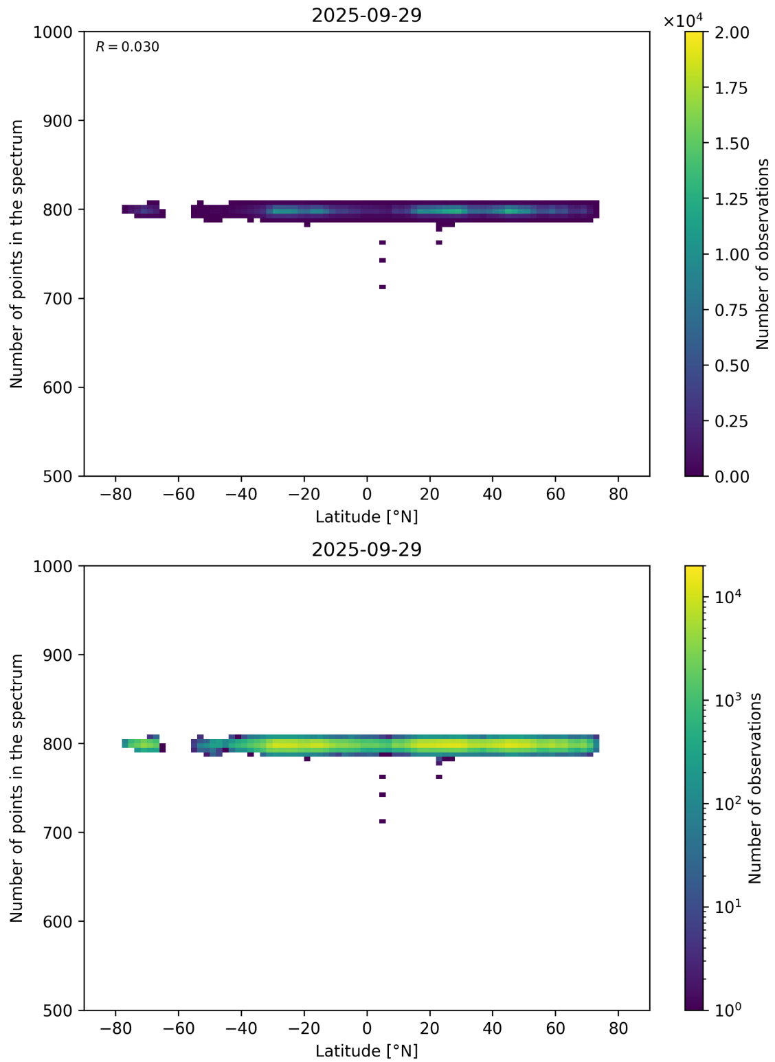
Figure 61: Scatter density plot of “Latitude” against “Number of points in the spectrum” for 2025-09-28 to 2025-09-30.
