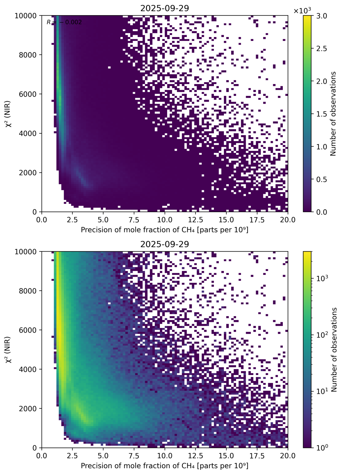
Figure 78: Scatter density plot of “Precision of mole fraction of CH 4 ” against “ \chi^2 (NIR)” for 2025-09-28 to 2025-09-30.
