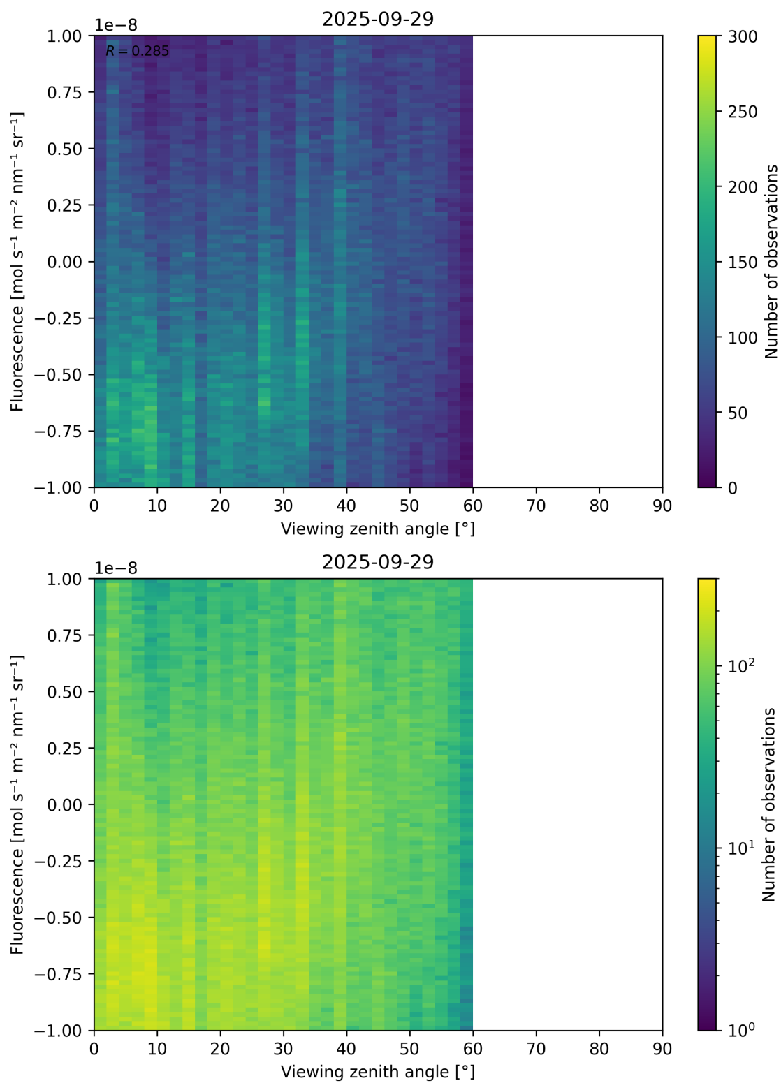
Figure 108: Scatter density plot of “Viewing zenith angle” against “Fluorescence” for 2025-09-28 to 2025-09-30.
