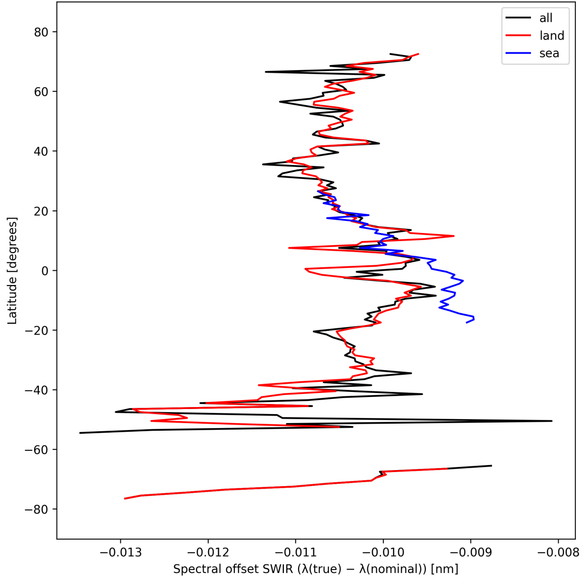
Figure 16: Zonal average of “Spectral offset SWIR ( \lambda_{\text{true}} - \lambda_{\text{nominal}} )” for 2025-09-28 to 2025-09-30.
