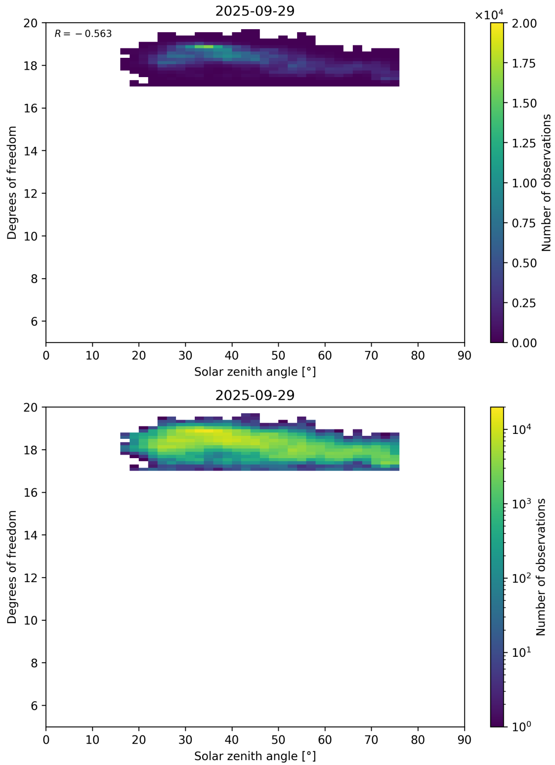
Figure 96: Scatter density plot of “Solar zenith angle” against “Degrees of freedom” for 2025-09-28 to 2025-09-30.
