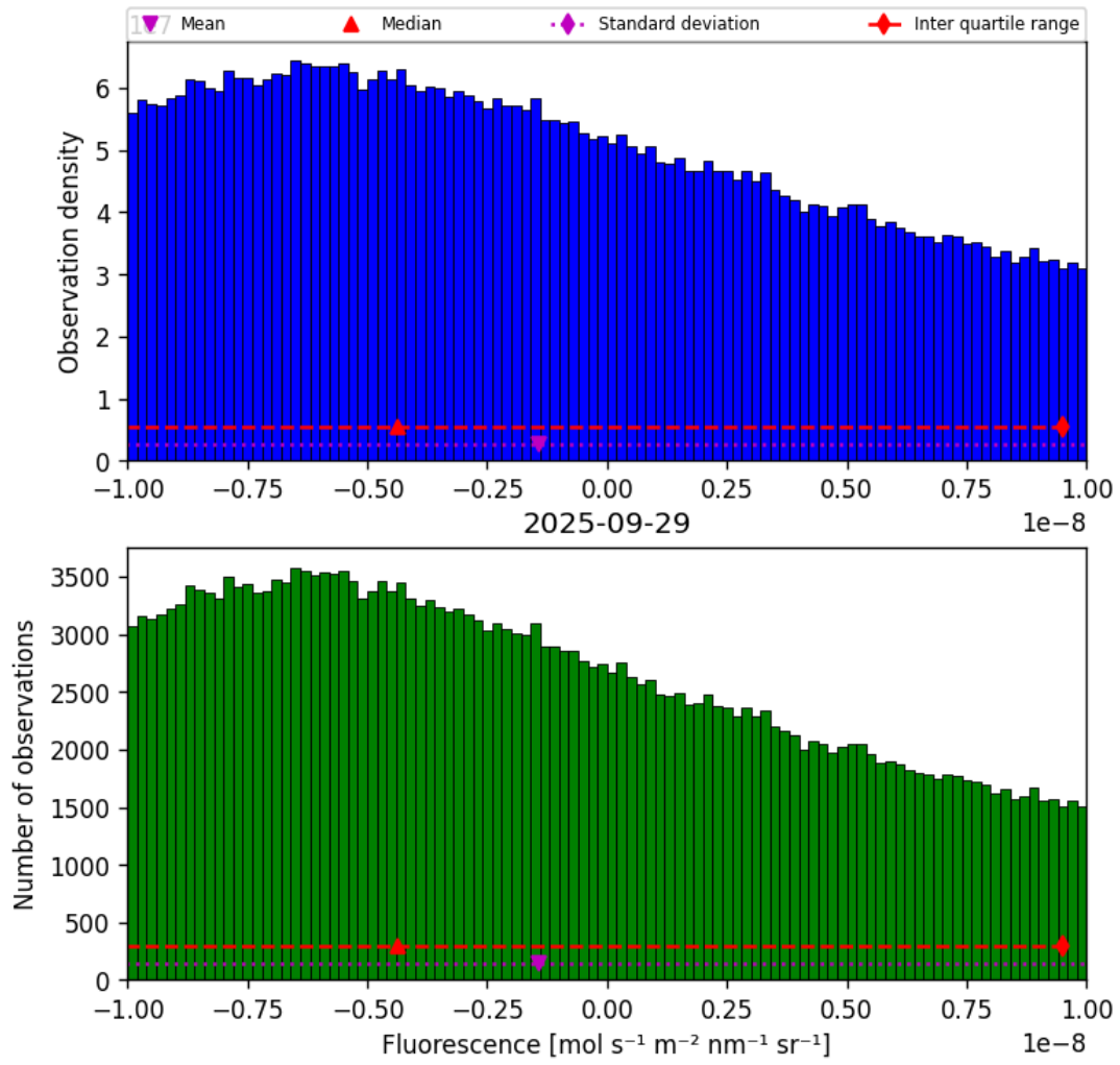
Figure 32: Histogram of “Fluorescence” for 2025-09-28 to 2025-09-30
