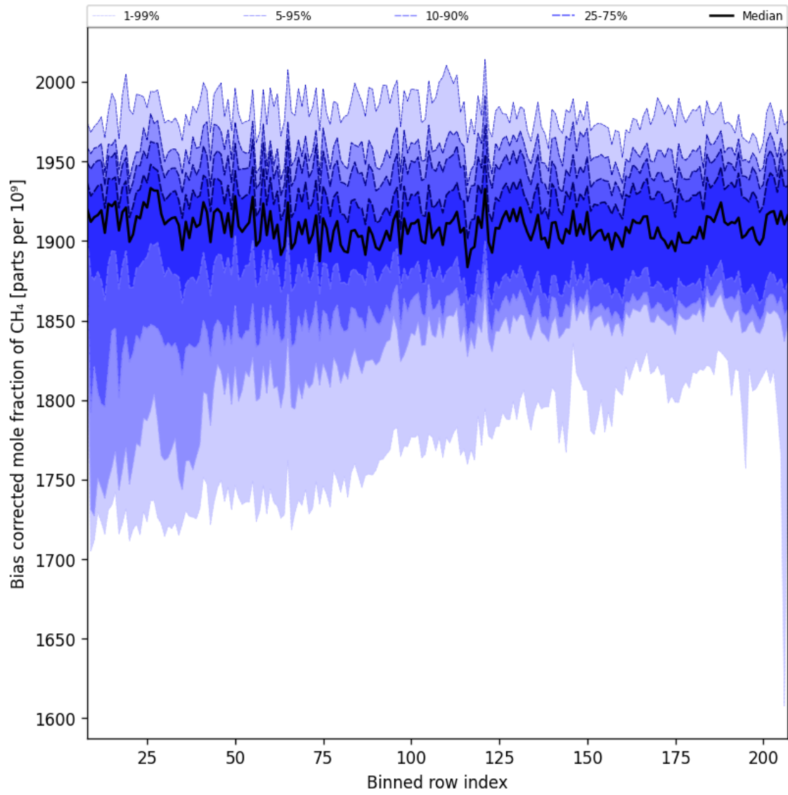
Figure 36: Along track statistics of “Bias corrected mole fraction of CH 4 ” for 2025-09-28 to 2025-09-30
