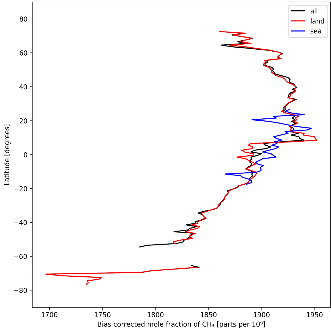
Figure 14: Zonal average of “Bias corrected mole fraction of CH 4 ” for 2025-09-28 to 2025-09-30.
