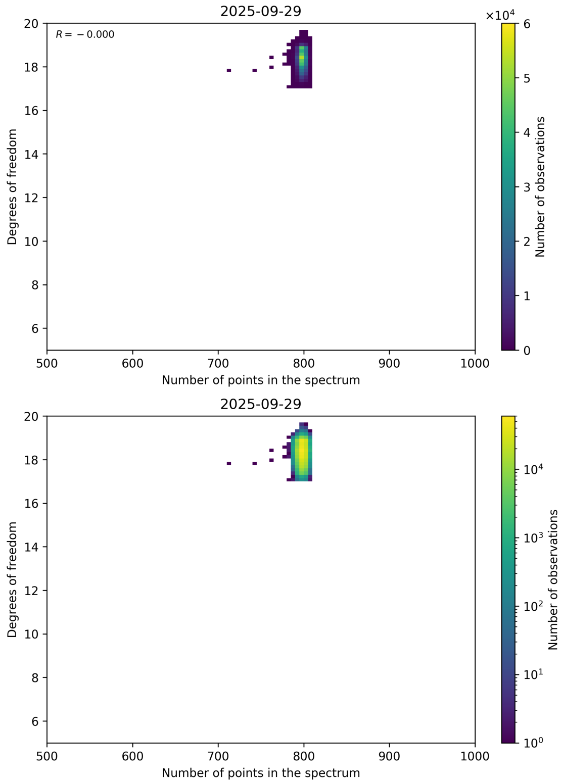
Figure 90: Scatter density plot of “Number of points in the spectrum” against “Degrees of freedom” for 2025-09-28 to 2025-09-30.
