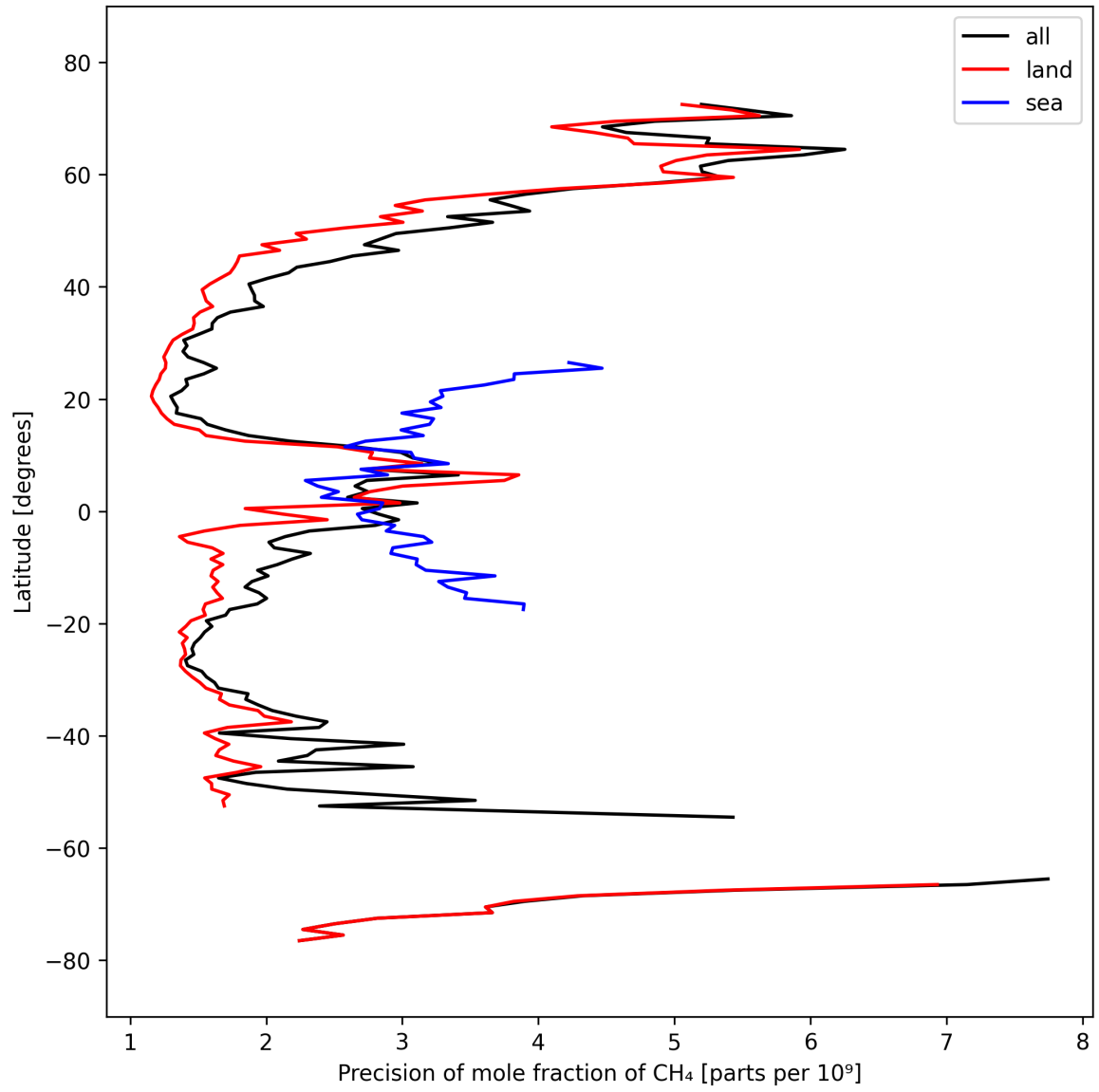
Figure 13: Zonal average of “Precision of mole fraction of CH 4 ” for 2025-09-28 to 2025-09-30.
