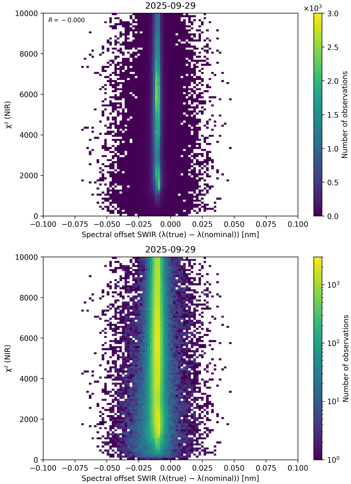
Figure 117: Scatter density plot of “Spectral offset SWIR ( \lambda_{\text{true}} - \lambda_{\text{nominal}} )” against “ \chi^2 (NIR)” for 2025-09-28 to 2025-09-30.
