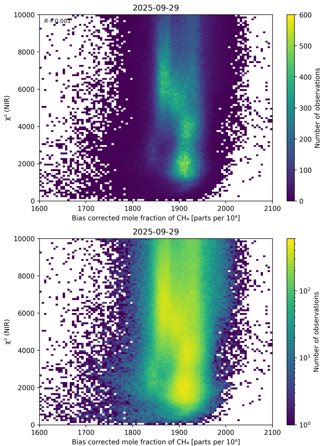
Figure 63: Scatter density plot of “Bias corrected mole fraction of CH 4 ” against “ \chi^2 (NIR)” for 2025-09-28 to 2025-09-30.
