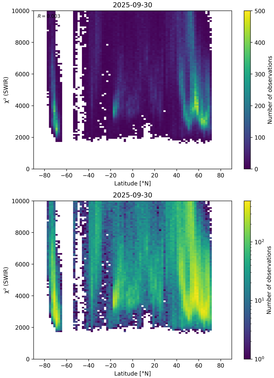
Figure 54: Scatter density plot of “Latitude” against “ \chi^2 (SWIR)” for 2025-09-29 to 2025-10-01.
