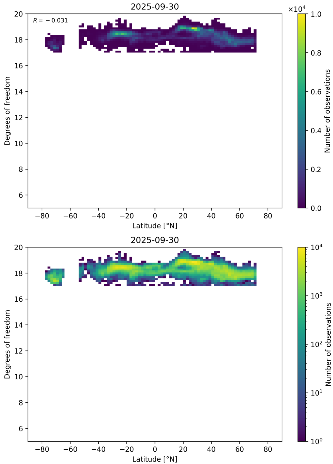
Figure 55: Scatter density plot of “Latitude” against “Degrees of freedom” for 2025-09-29 to 2025-10-01.
