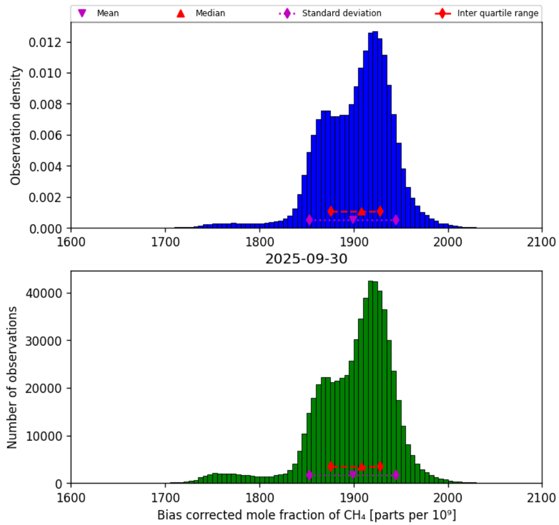
Figure 25: Histogram of “Bias corrected mole fraction of CH 4 ” for 2025-09-29 to 2025-10-01
