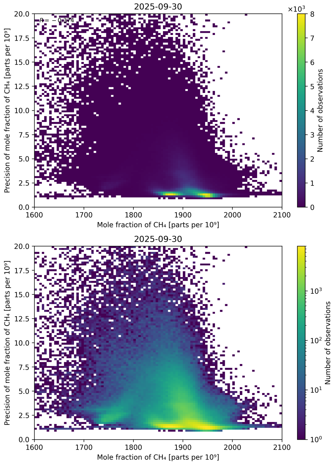
Figure 75: Scatter density plot of “Mole fraction of CH 4 ” against “Precision of mole fraction of CH 4 ” for 2025-09-29 to 2025-10-01.
