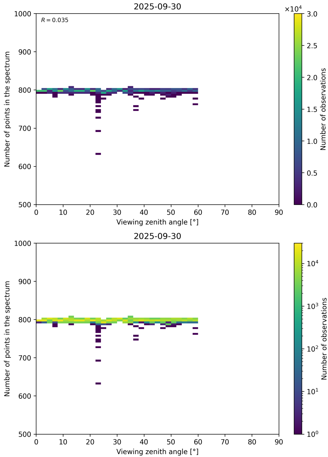
Figure 114: Scatter density plot of “Viewing zenith angle” against “Number of points in the spectrum” for 2025-09-29 to 2025-10-01.
