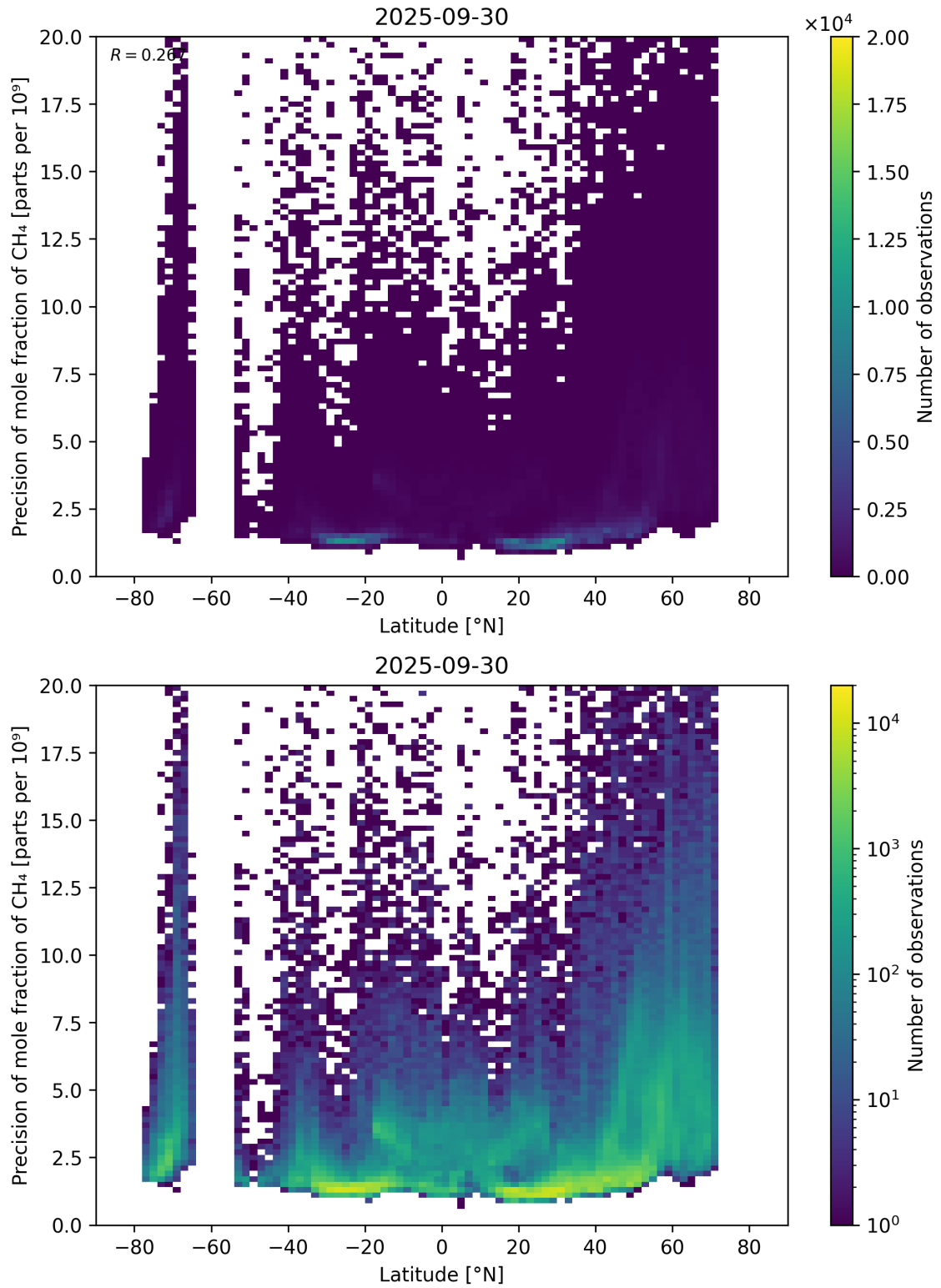
Figure 59: Scatter density plot of “Latitude” against “Precision of mole fraction of \text{CH}_4 ” for 2025-09-29 to 2025-10-01.
