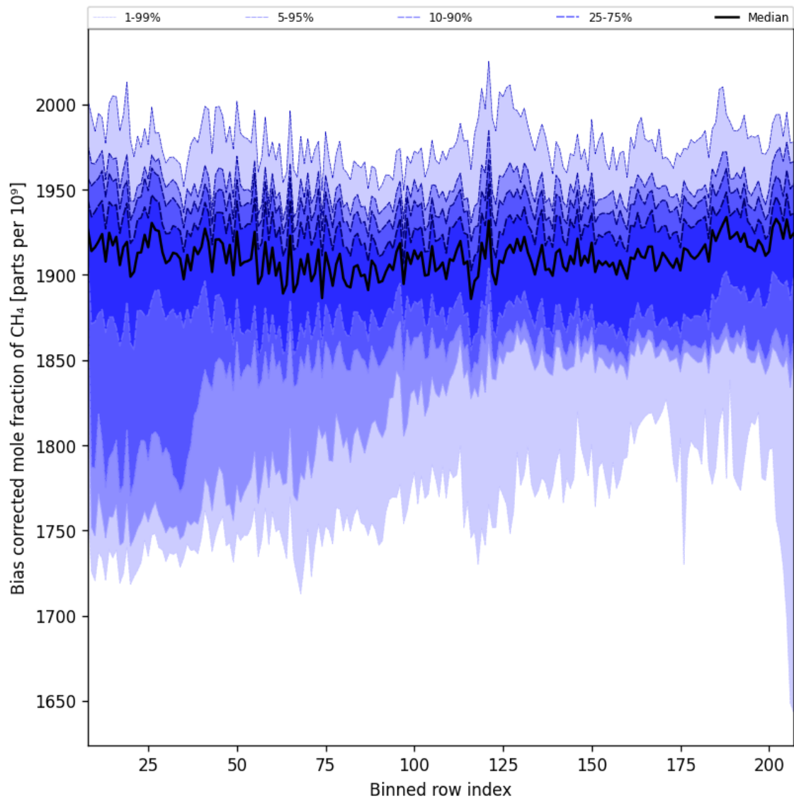
Figure 36: Along track statistics of “Bias corrected mole fraction of CH 4 ” for 2025-09-29 to 2025-10-01
