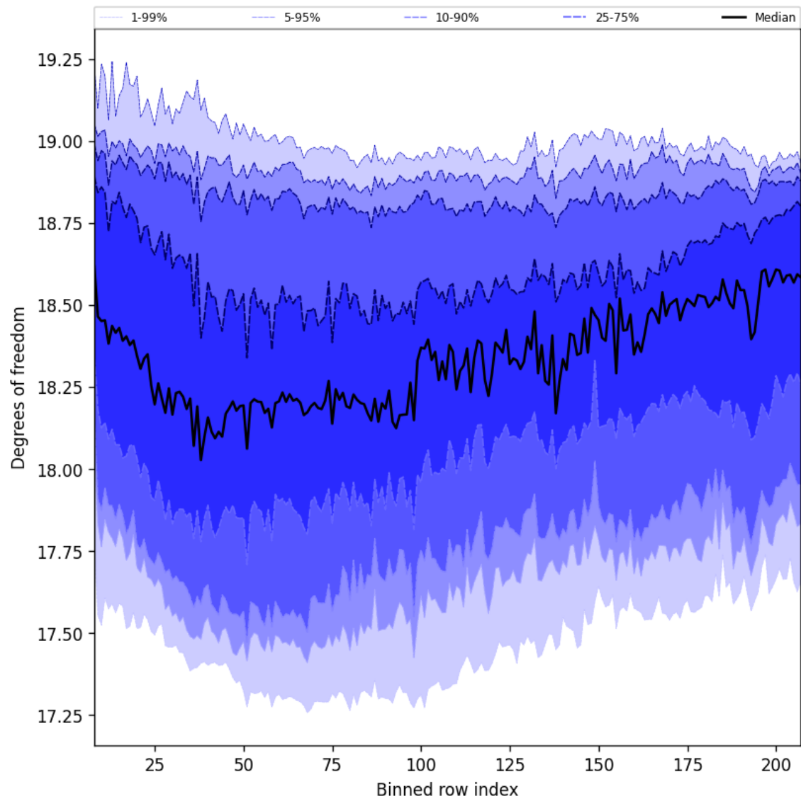
Figure 41: Along track statistics of “Degrees of freedom” for 2025-09-29 to 2025-10-01
