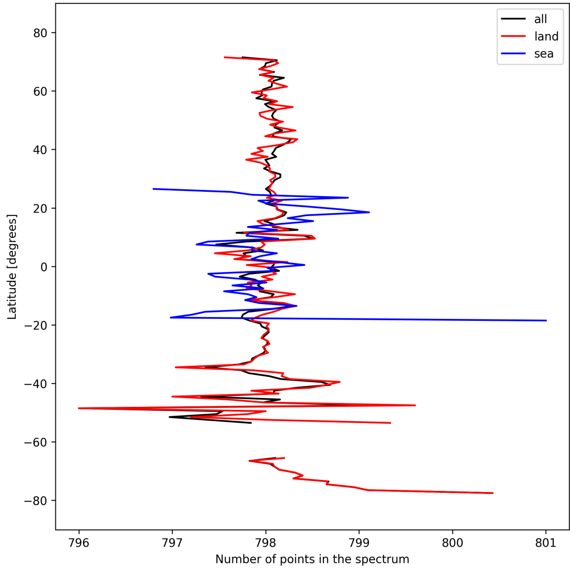
Figure 15: Zonal average of “Number of points in the spectrum” for 2025-09-29 to 2025-10-01.
