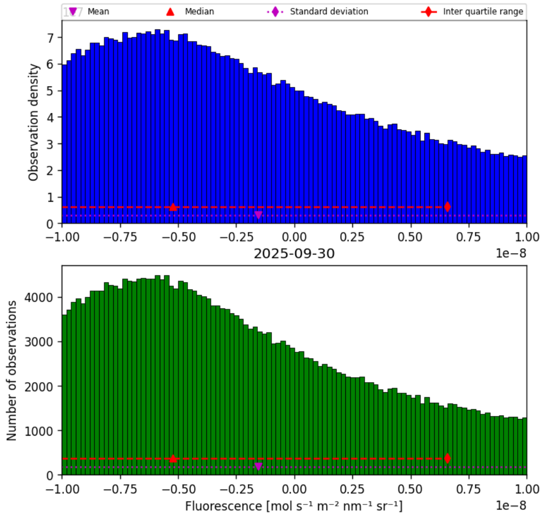
Figure 32: Histogram of “Fluorescence” for 2025-09-29 to 2025-10-01
