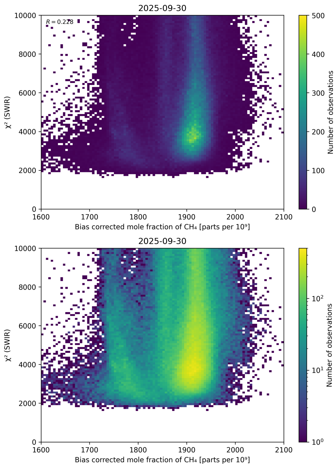
Figure 64: Scatter density plot of “Bias corrected mole fraction of \text{CH}_4 ” against “ \chi^2 (SWIR)” for 2025-09-29 to 2025-10-01.
