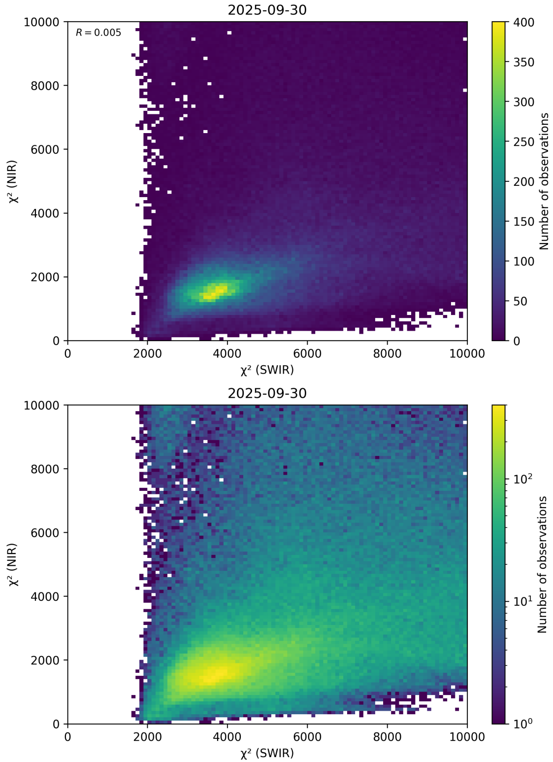
Figure 47: Scatter density plot of “ \chi^2 (SWIR)” against “ \chi^2 (NIR)” for 2025-09-29 to 2025-10-01.
