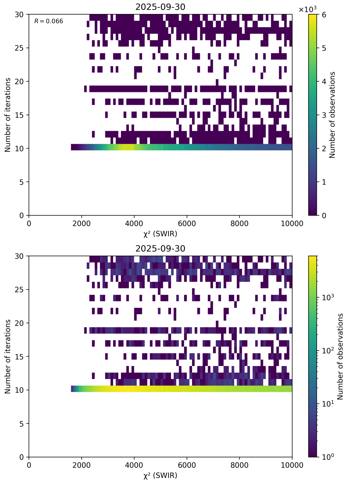
Figure 50: Scatter density plot of “ \chi^2 (SWIR)” against “Number of iterations” for 2025-09-29 to 2025-10-01.
