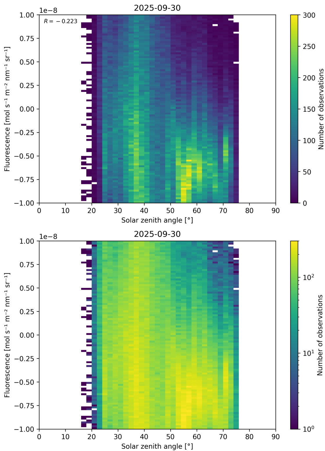
Figure 97: Scatter density plot of “Solar zenith angle” against “Fluorescence” for 2025-09-29 to 2025-10-01.
