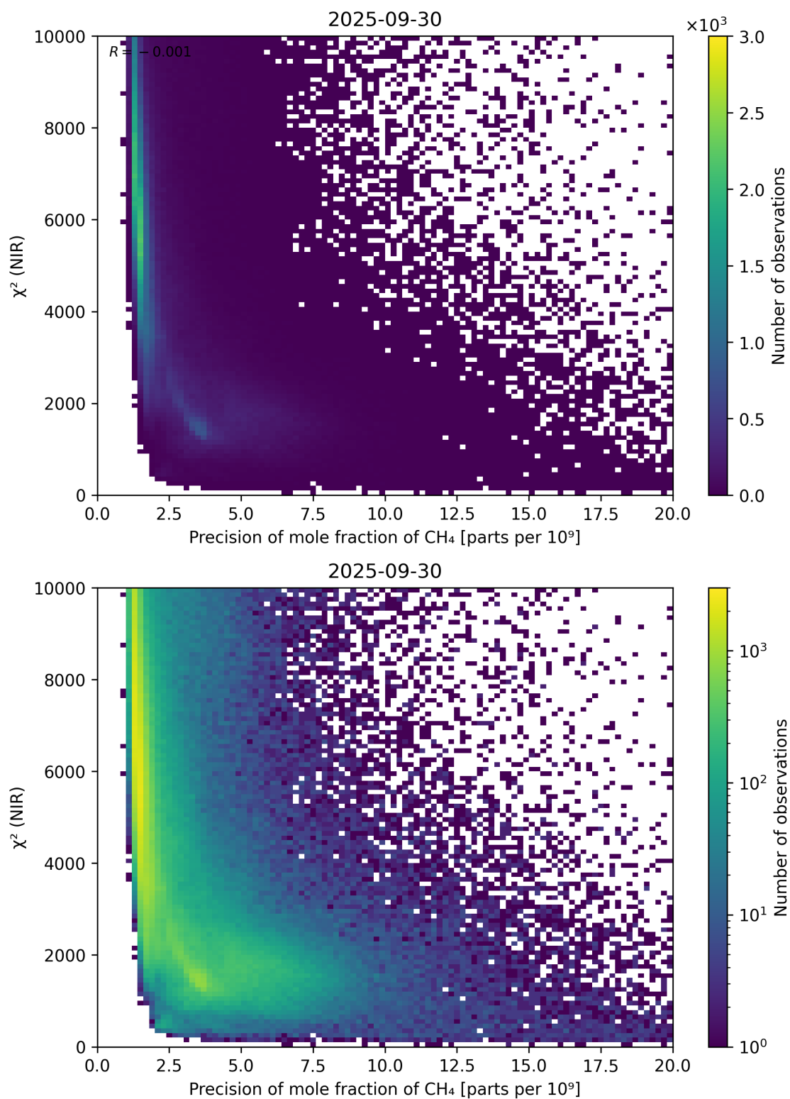
Figure 78: Scatter density plot of “Precision of mole fraction of CH 4 ” against “ \chi^2 (NIR)” for 2025-09-29 to 2025-10-01.
