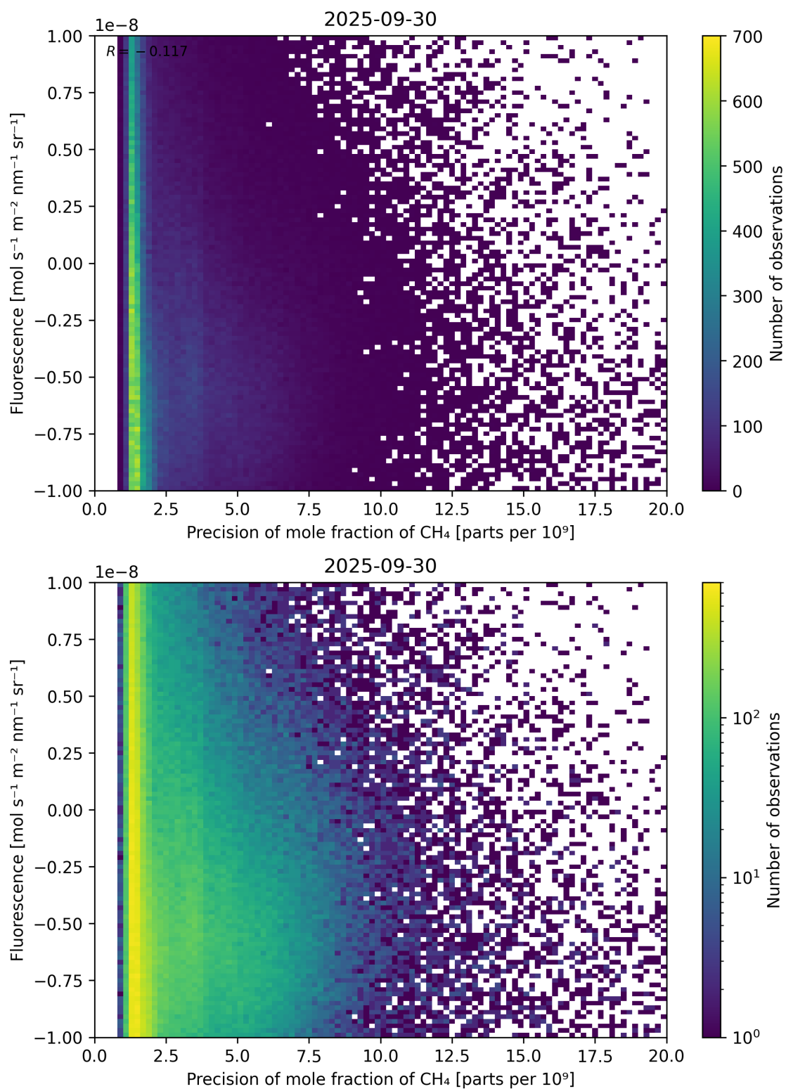
Figure 81: Scatter density plot of “Precision of mole fraction of CH 4 ” against “Fluorescence” for 2025-09-29 to 2025-10-01.
