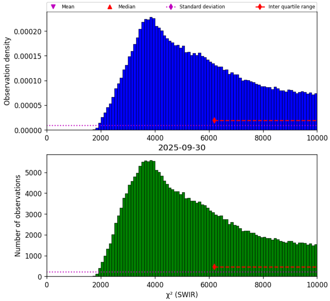
Figure 28: Histogram of “ \chi^2 (SWIR)” for 2025-09-29 to 2025-10-01
