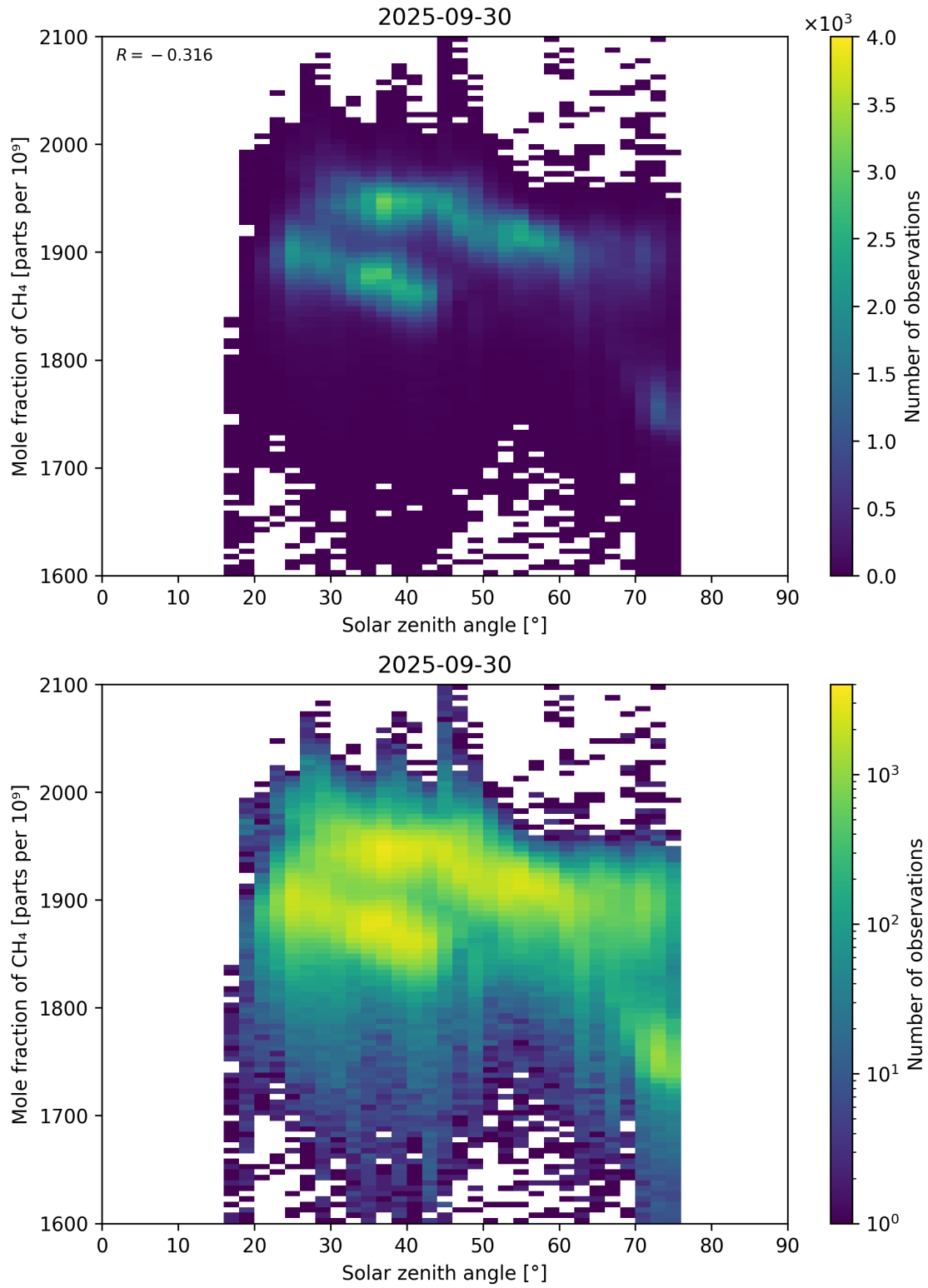
Figure 99: Scatter density plot of “Solar zenith angle” against “Mole fraction of CH 4 ” for 2025-09-29 to 2025-10-01.
