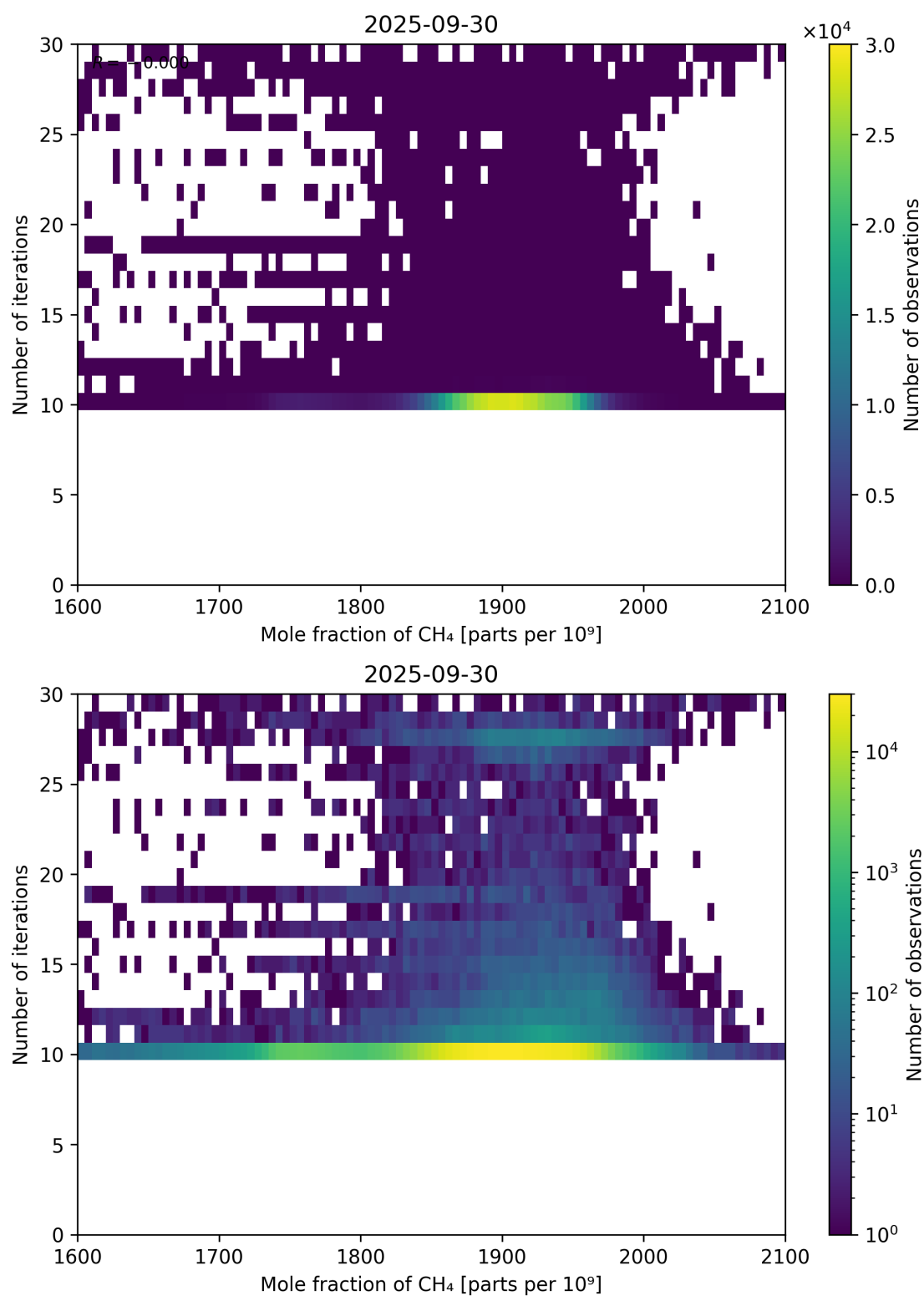
Figure 76: Scatter density plot of “Mole fraction of CH 4 ” against “Number of iterations” for 2025-09-29 to 2025-10-01.
