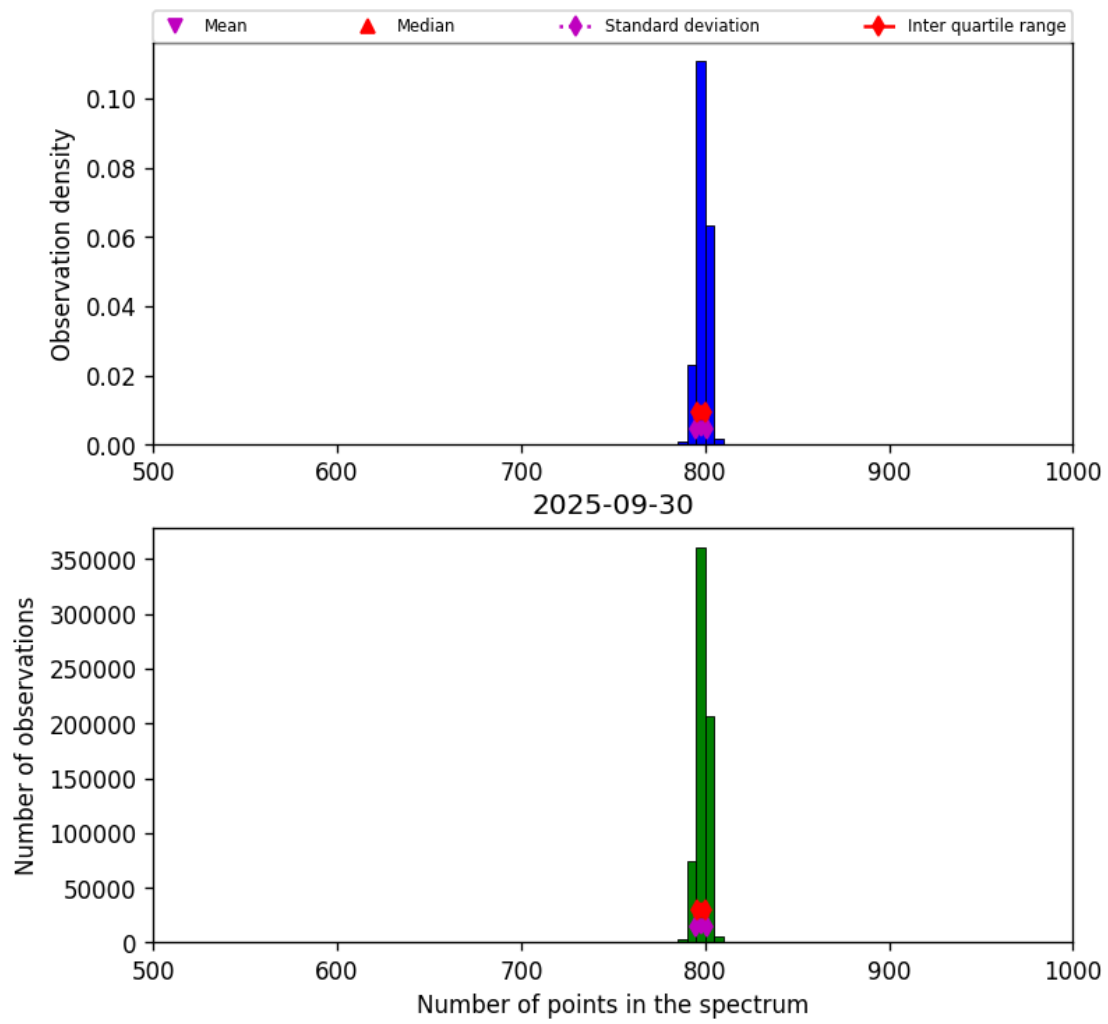
Figure 26: Histogram of “Number of points in the spectrum” for 2025-09-29 to 2025-10-01
