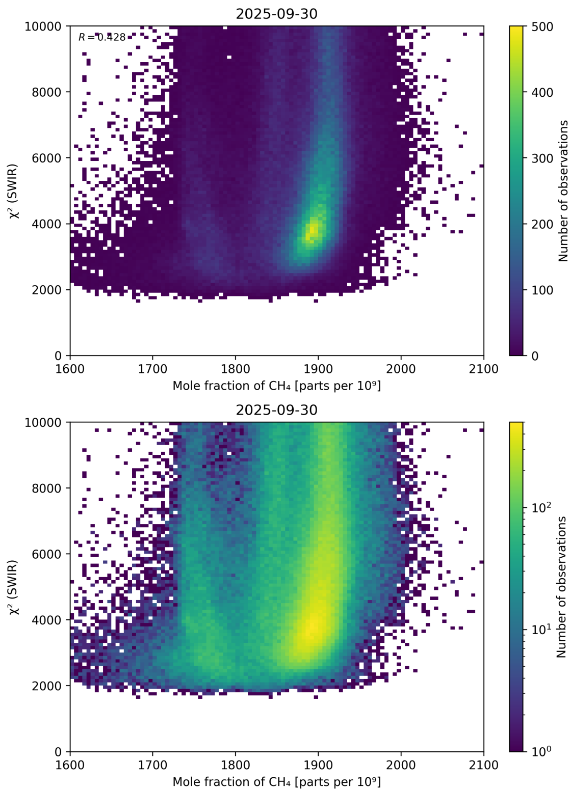
Figure 71: Scatter density plot of “Mole fraction of \text{CH}_4 ” against “ \chi^2 (SWIR)” for 2025-09-29 to 2025-10-01.
