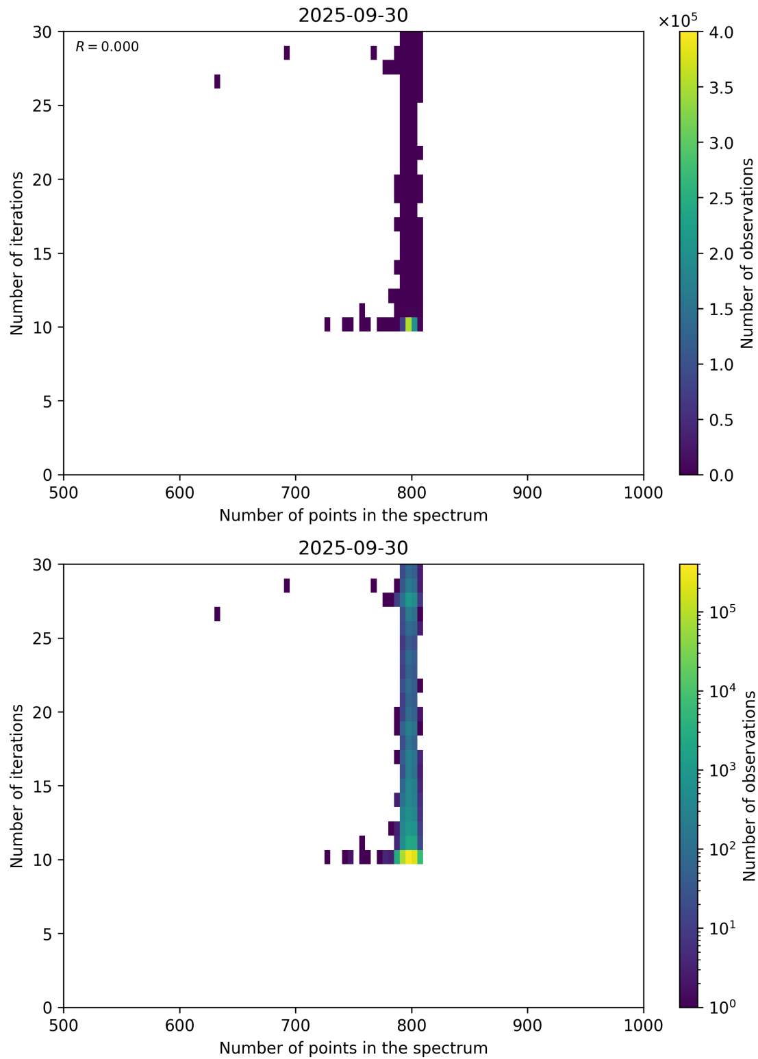
Figure 92: Scatter density plot of “Number of points in the spectrum” against “Number of iterations” for 2025-09-29 to 2025-10-01.
