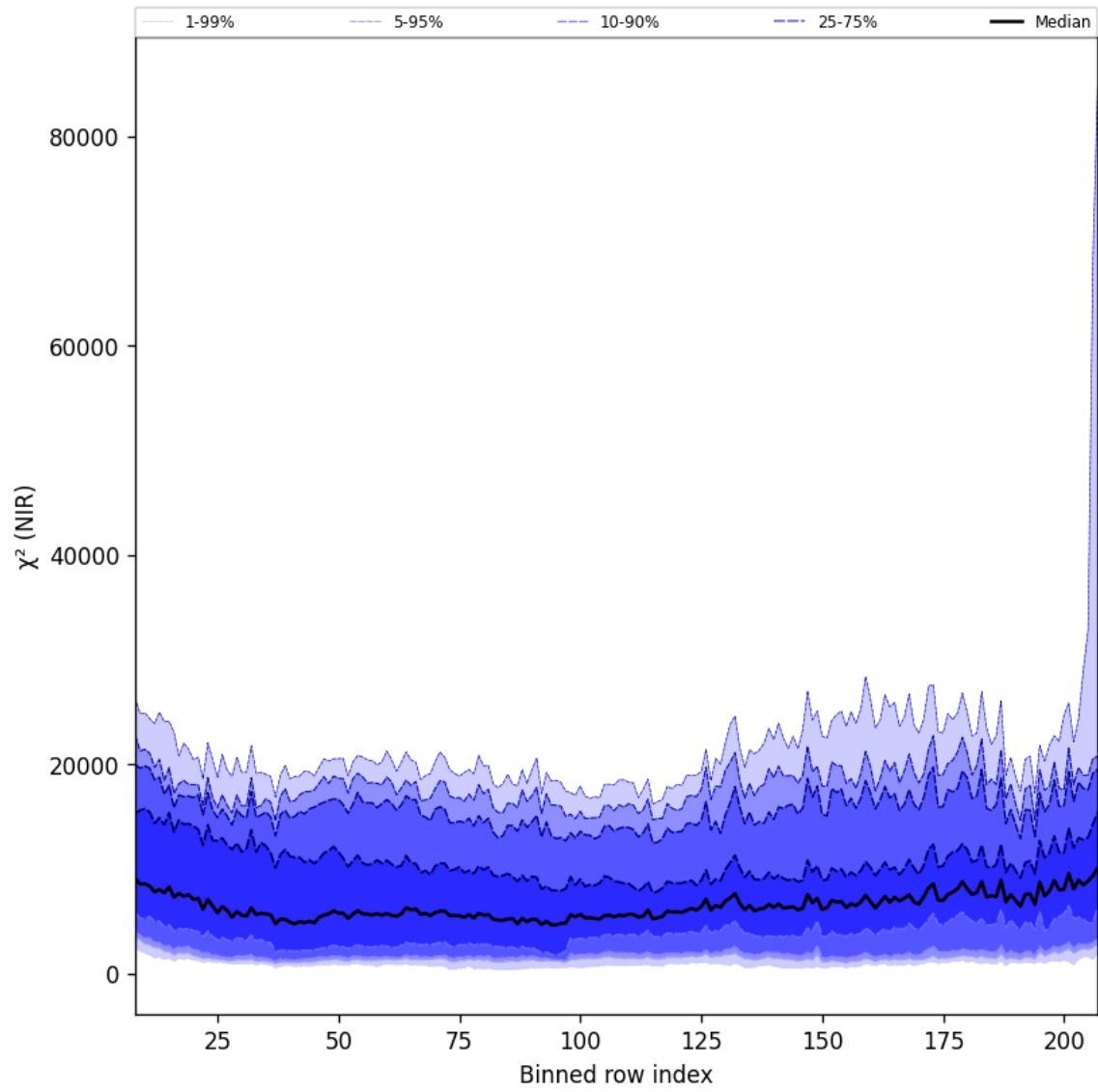
Figure 40: Along track statistics of “ \chi^2 (NIR)” for 2025-09-29 to 2025-10-01
