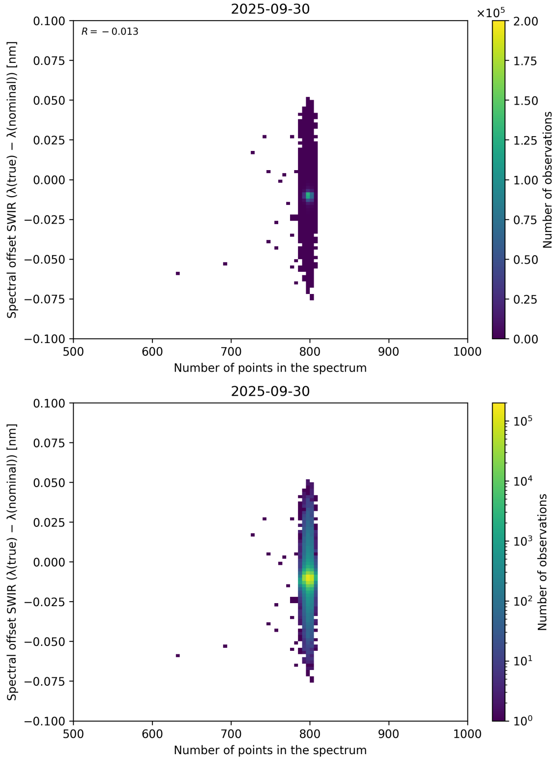
Figure 93: Scatter density plot of “Number of points in the spectrum” against “Spectral offset SWIR ( \lambda_{\text{true}} - \lambda_{\text{nominal}} )” for 2025-09-29 to 2025-10-01.
