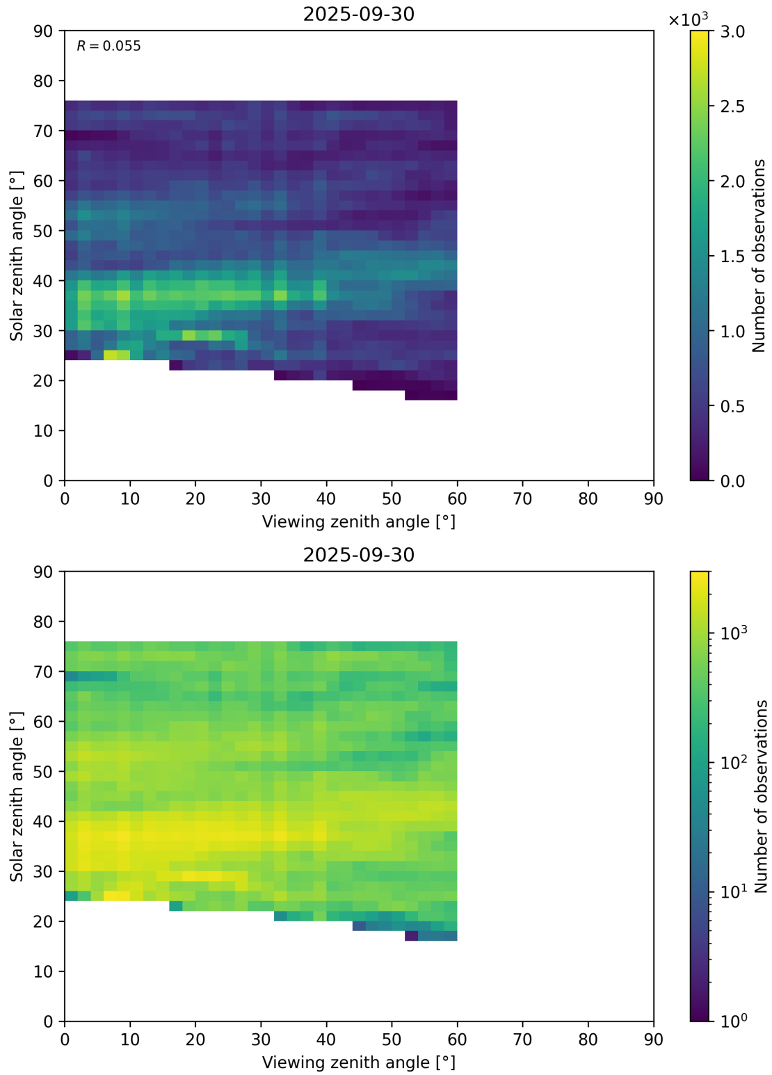
Figure 115: Scatter density plot of “Viewing zenith angle” against “Solar zenith angle” for 2025-09-29 to 2025-10-01.
