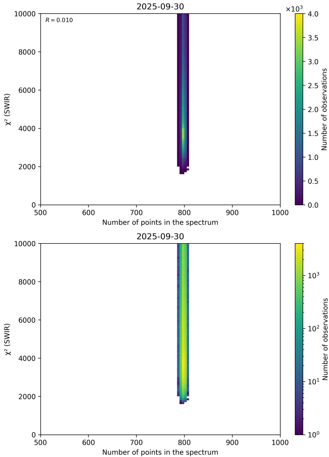
Figure 89: Scatter density plot of “Number of points in the spectrum” against “ \chi^2 (SWIR)” for 2025-09-29 to 2025-10-01.
