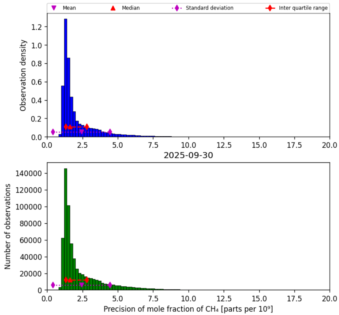
Figure 24: Histogram of “Precision of mole fraction of CH 4 ” for 2025-09-29 to 2025-10-01
