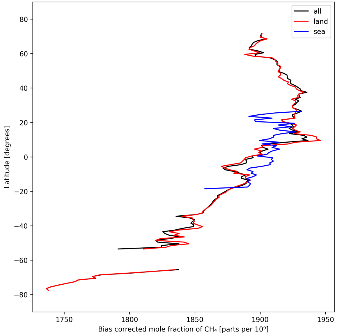
Figure 14: Zonal average of “Bias corrected mole fraction of CH 4 ” for 2025-09-29 to 2025-10-01.
