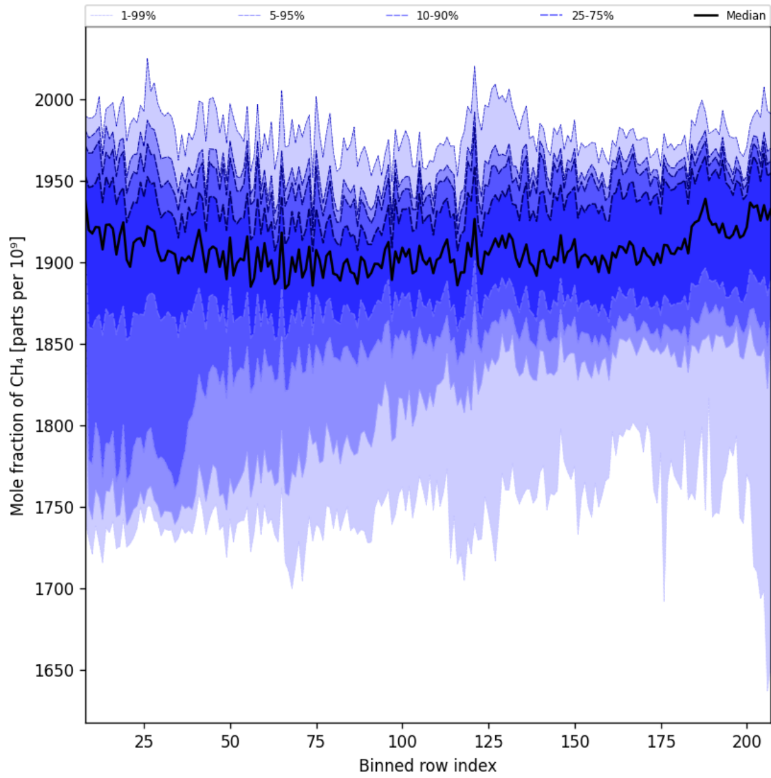
Figure 34: Along track statistics of “Mole fraction of CH 4 ” for 2025-09-29 to 2025-10-01
