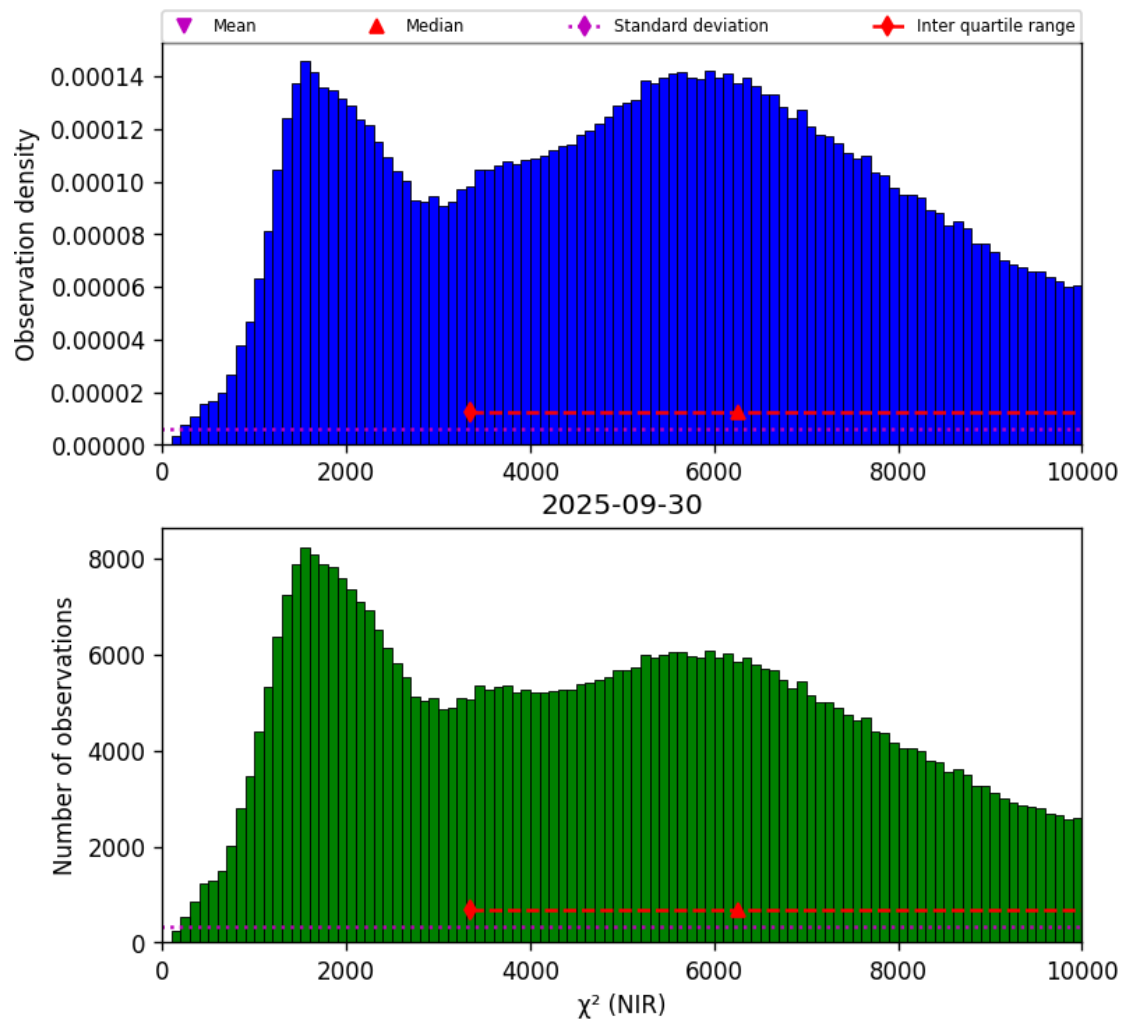
Figure 29: Histogram of " \chi^2 (NIR)" for 2025-09-29 to 2025-10-01
