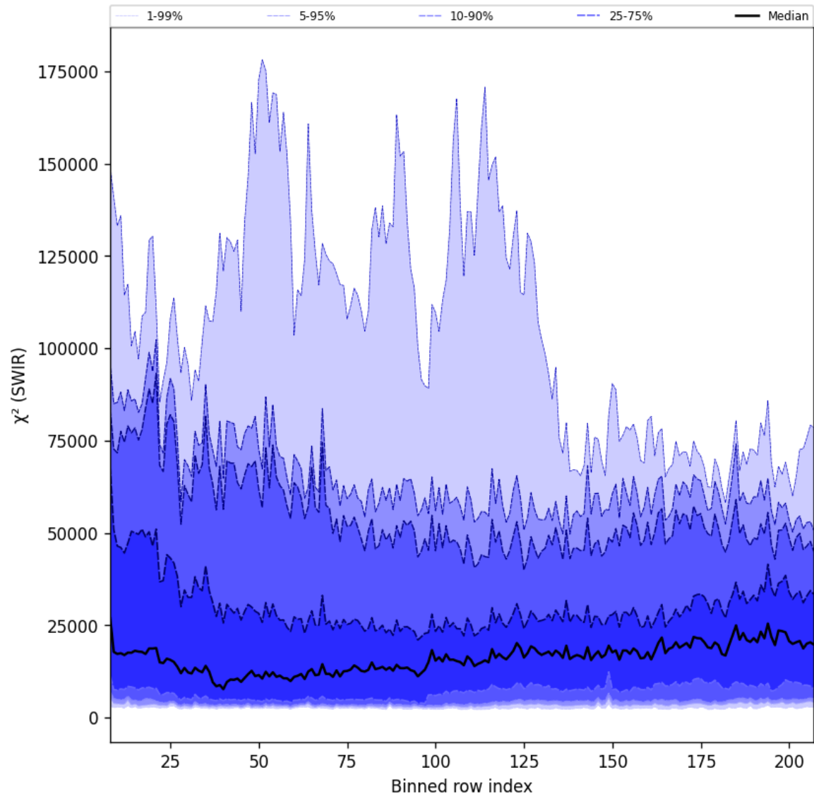
Figure 39: Along track statistics of “ \chi^2 (SWIR)” for 2025-09-29 to 2025-10-01
