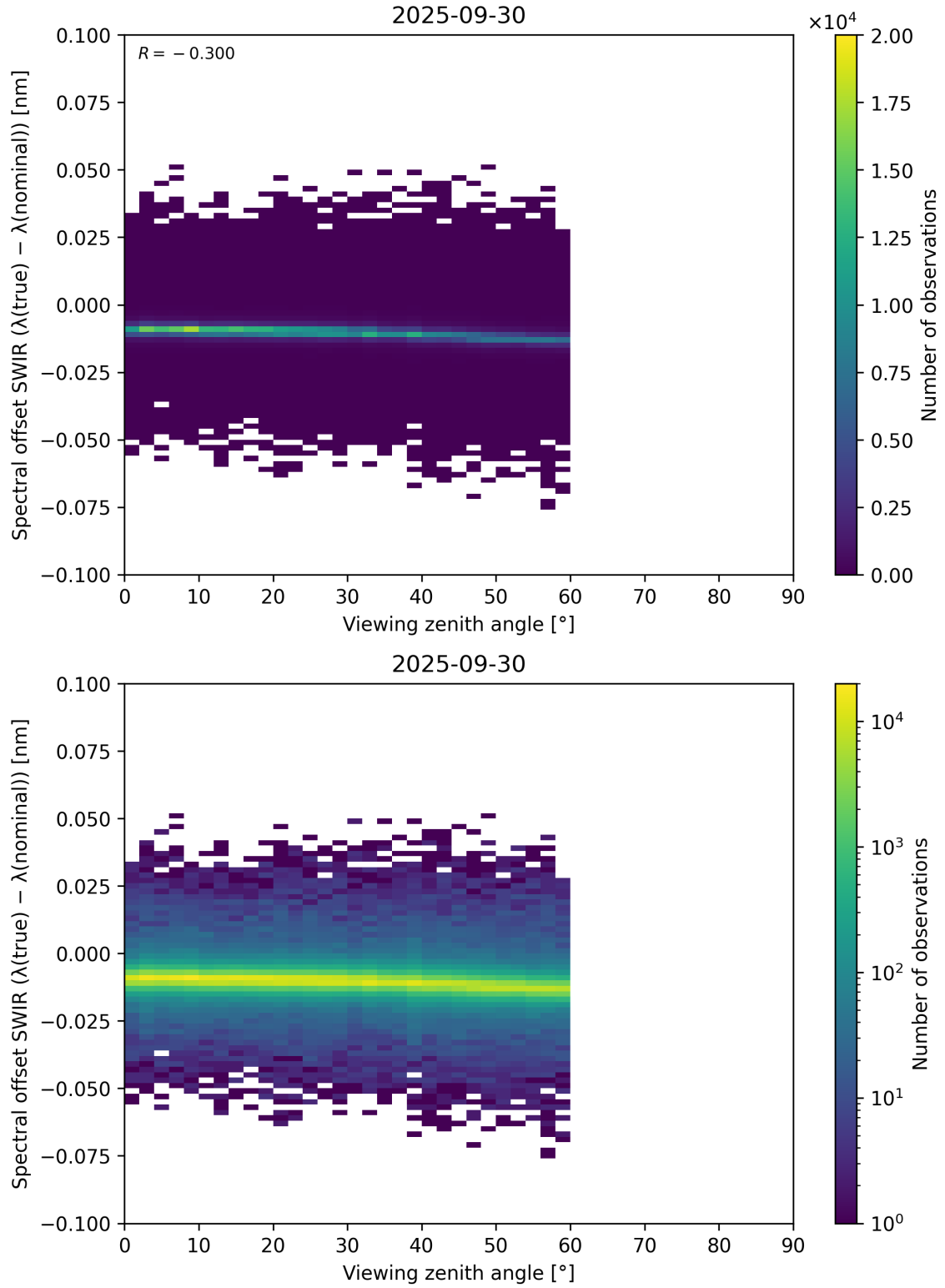
Figure 116: Scatter density plot of “Viewing zenith angle” against “Spectral offset SWIR ( \lambda_{\text{true}} - \lambda_{\text{nominal}} )” for 2025-09-29 to 2025-10-01.
