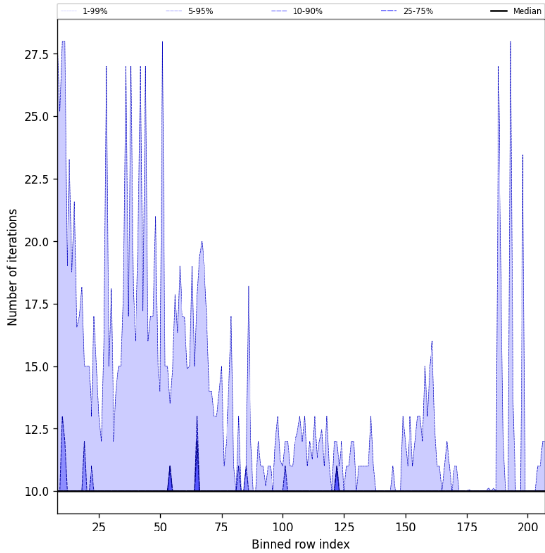
Figure 42: Along track statistics of “Number of iterations” for 2025-09-29 to 2025-10-01
