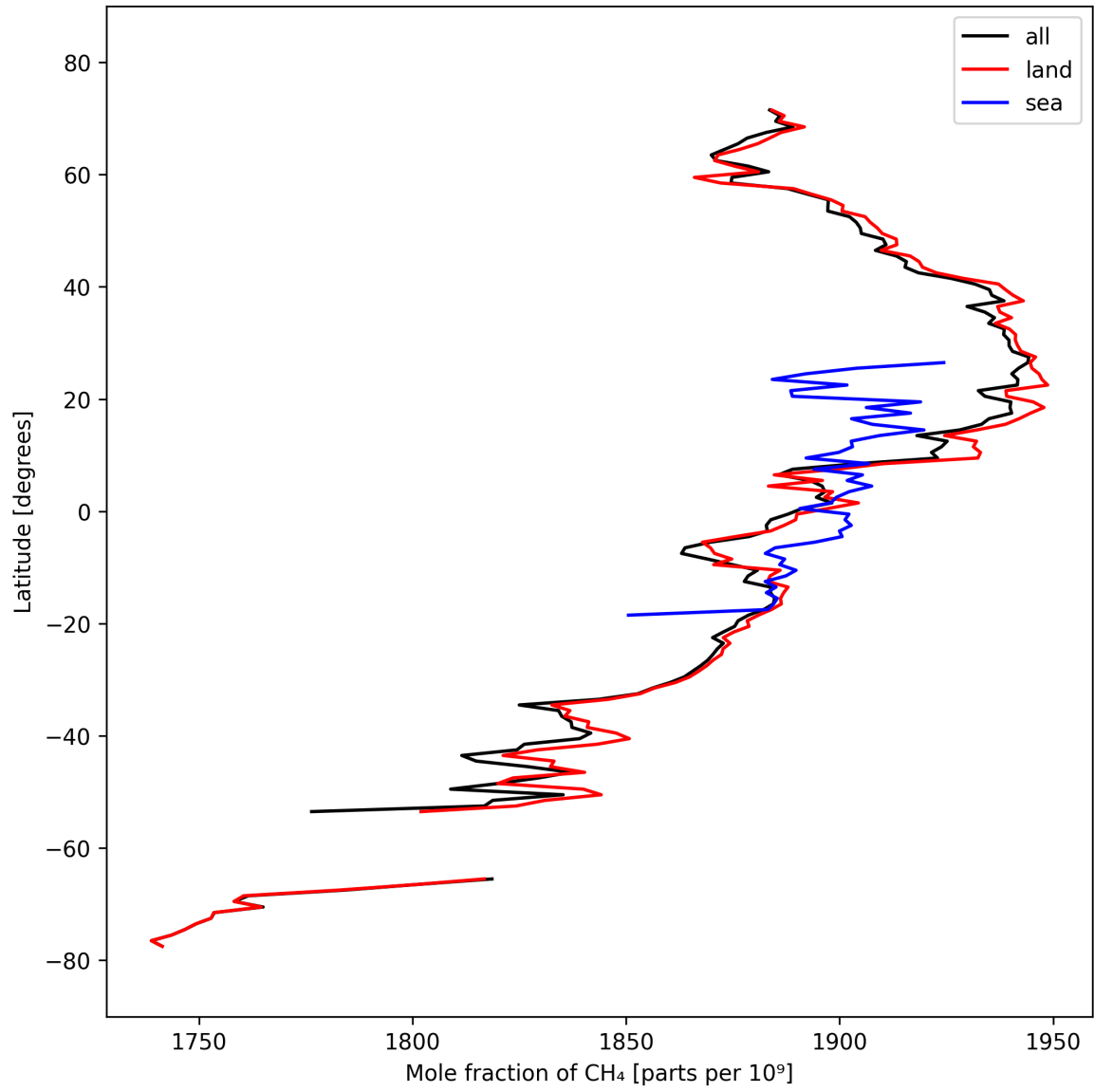
Figure 12: Zonal average of “Mole fraction of CH 4 ” for 2025-09-29 to 2025-10-01.
