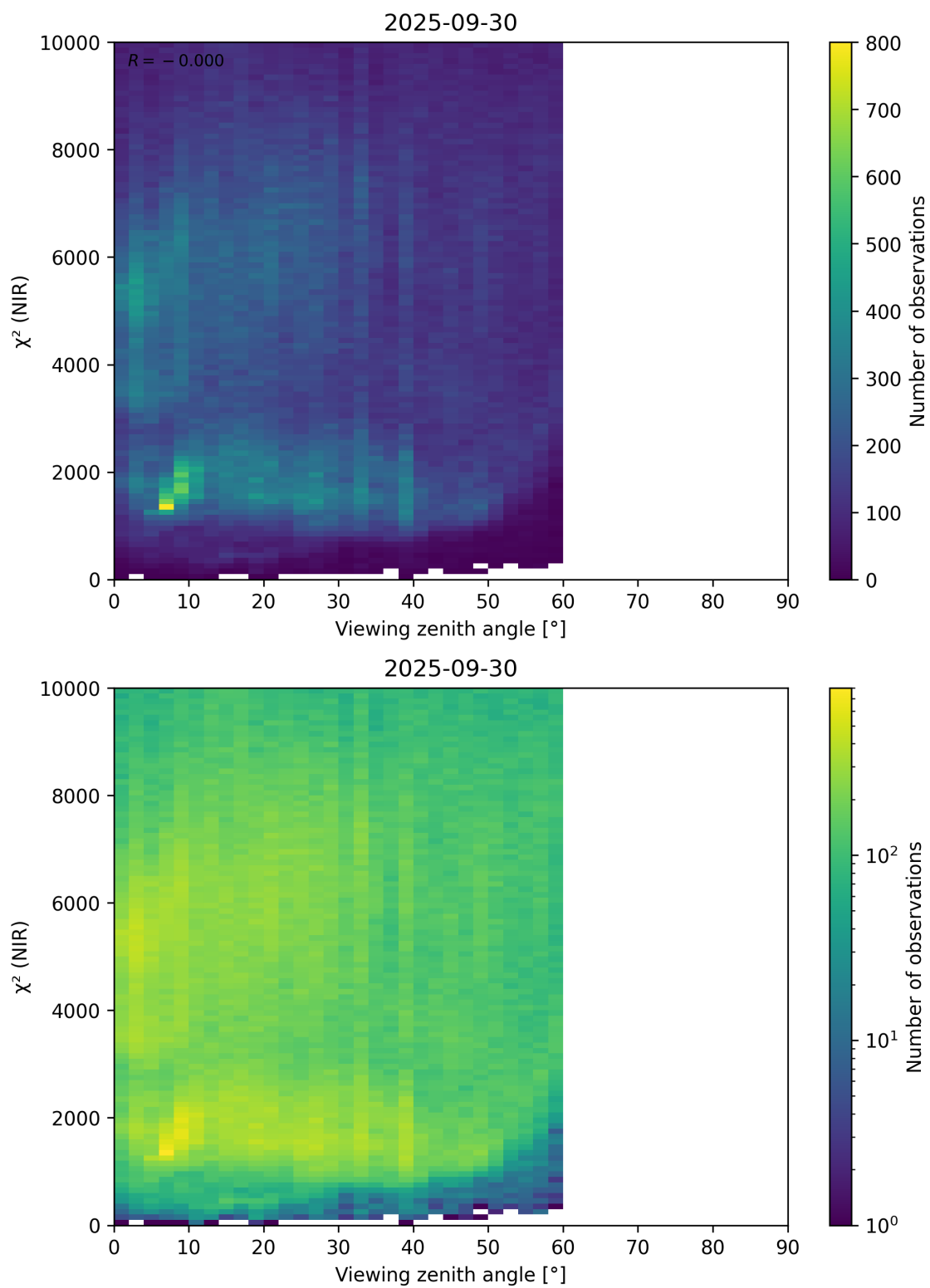
Figure 105: Scatter density plot of “Viewing zenith angle” against “ \chi^2 (NIR)” for 2025-09-29 to 2025-10-01.
