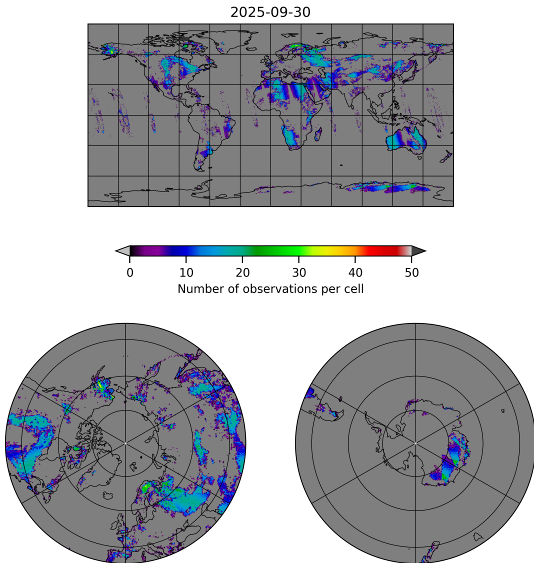
Figure 10: Map of the number of observations for 2025-09-29 to 2025-10-01
