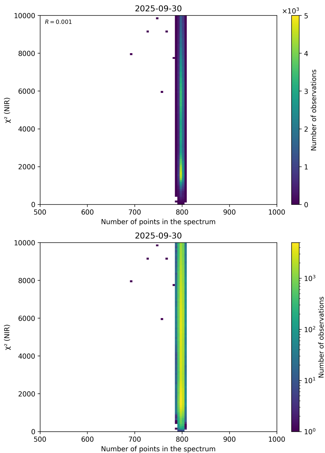
Figure 88: Scatter density plot of “Number of points in the spectrum” against “ \chi^2 (NIR)” for 2025-09-29 to 2025-10-01.
