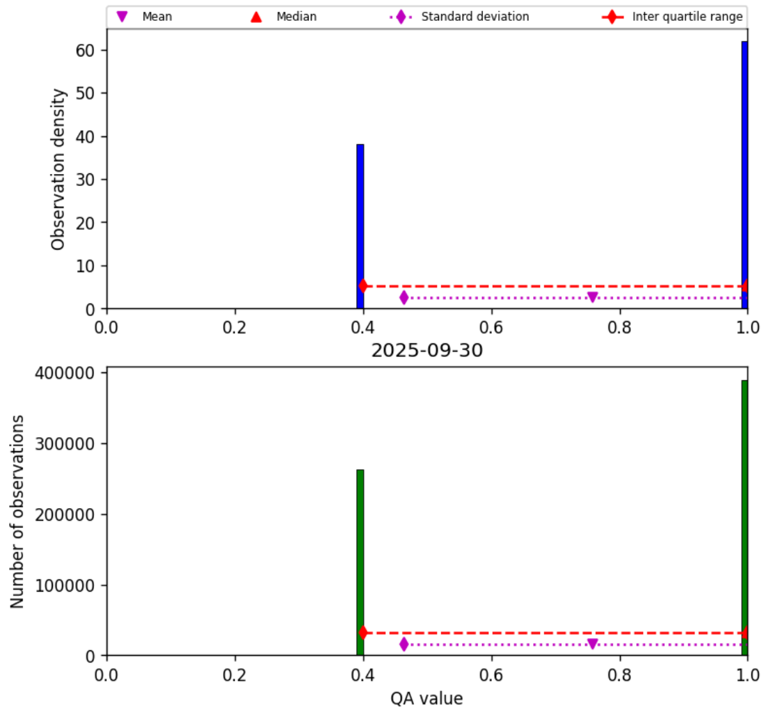
Figure 22: Histogram of “QA value” for 2025-09-29 to 2025-10-01
