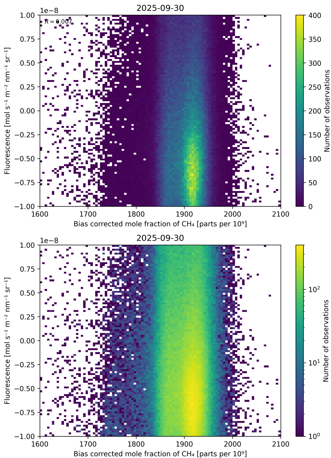
Figure 66: Scatter density plot of “Bias corrected mole fraction of \text{CH}_4 ” against “Fluorescence” for 2025-09-29 to 2025-10-01.
