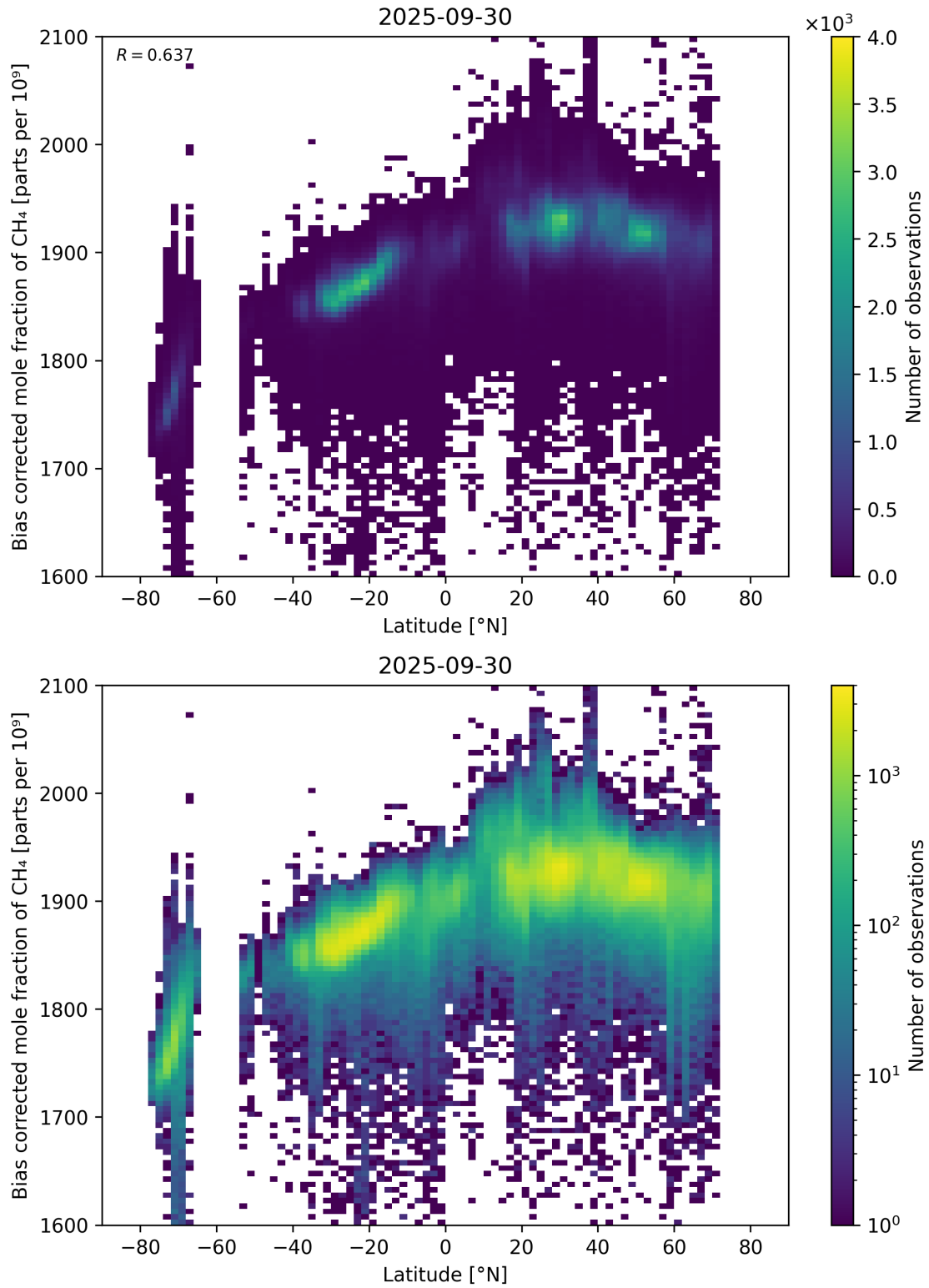
Figure 58: Scatter density plot of “Latitude” against “Bias corrected mole fraction of CH 4 ” for 2025-09-29 to 2025-10-01.
