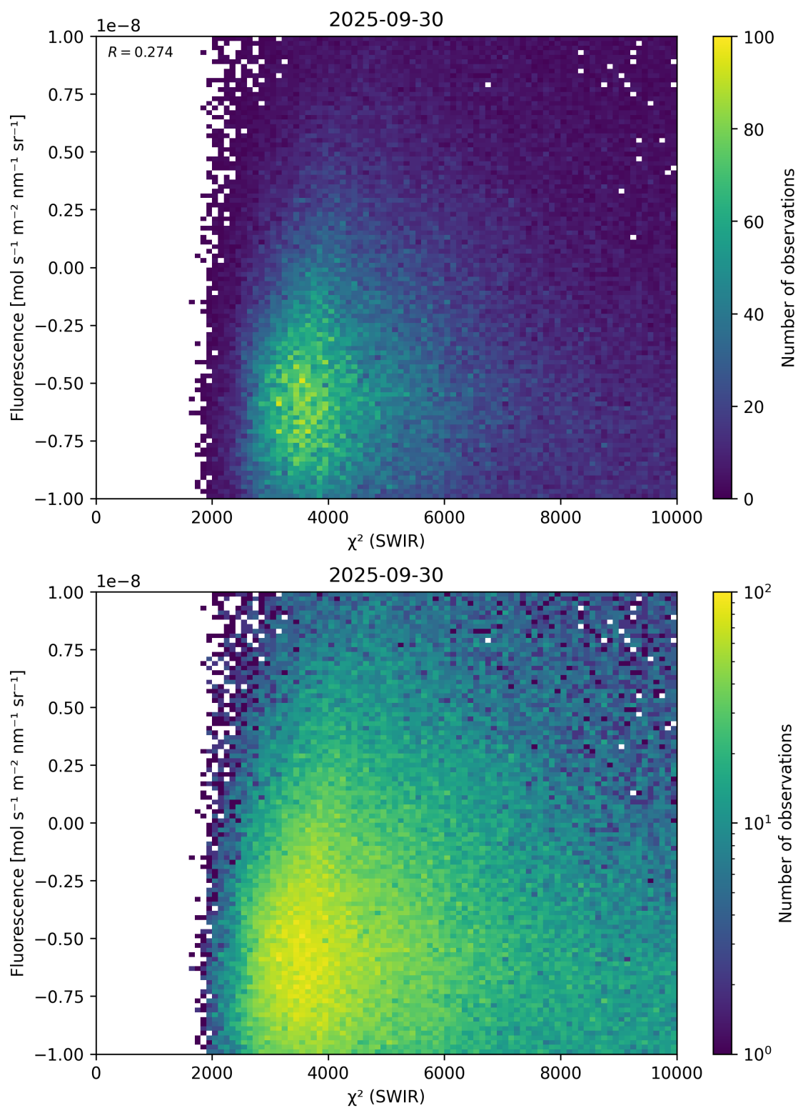
Figure 49: Scatter density plot of “ \chi^2 (SWIR)” against “Fluorescence” for 2025-09-29 to 2025-10-01.
