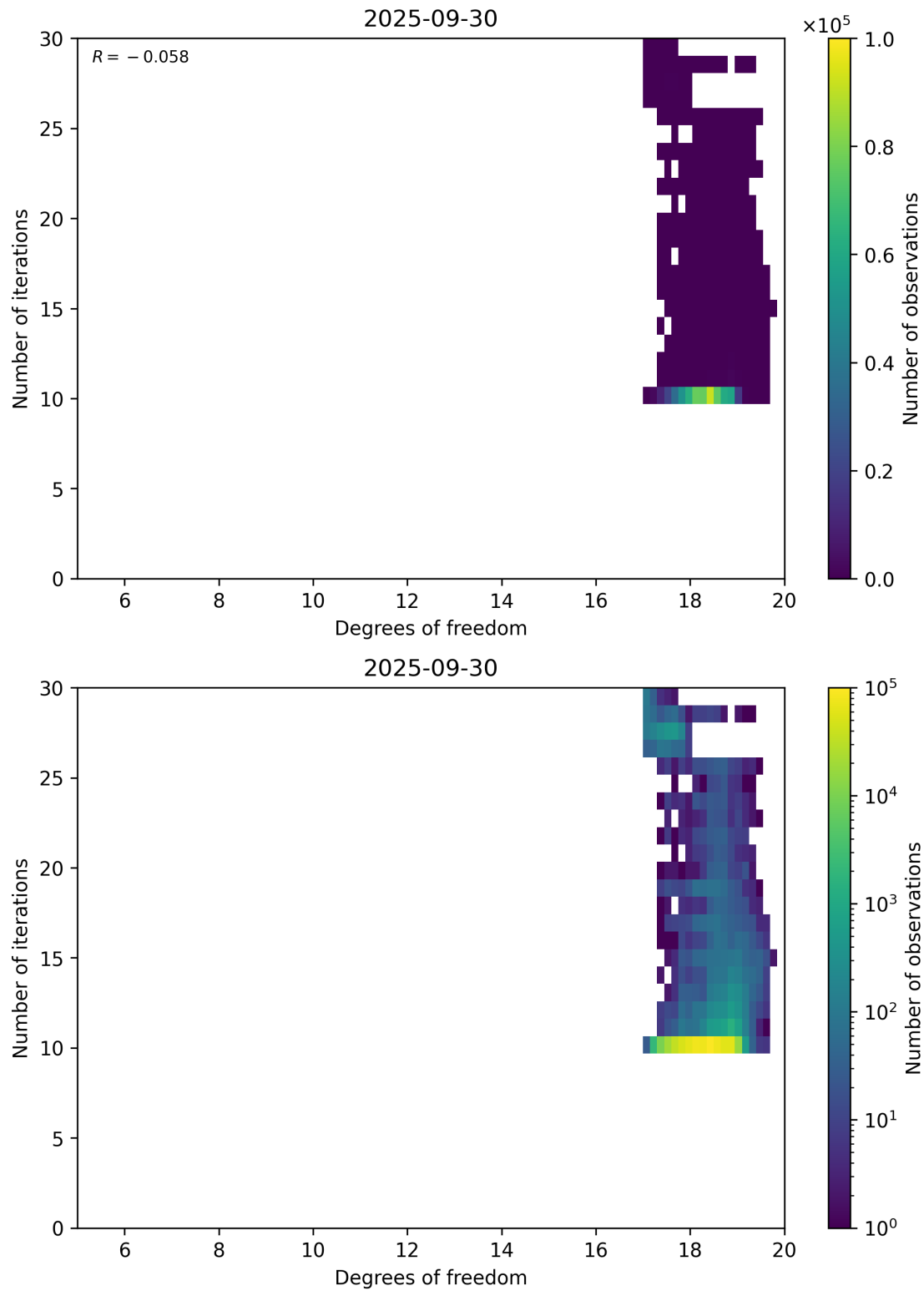
Figure 52: Scatter density plot of “Degrees of freedom” against “Number of iterations” for 2025-09-29 to 2025-10-01.
