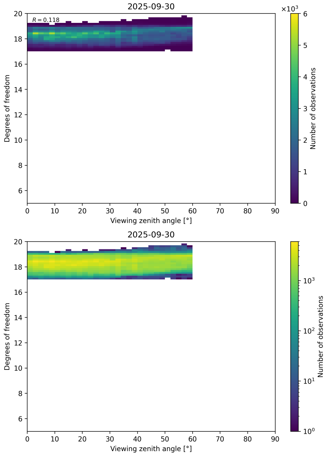
Figure 107: Scatter density plot of “Viewing zenith angle” against “Degrees of freedom” for 2025-09-29 to 2025-10-01.
