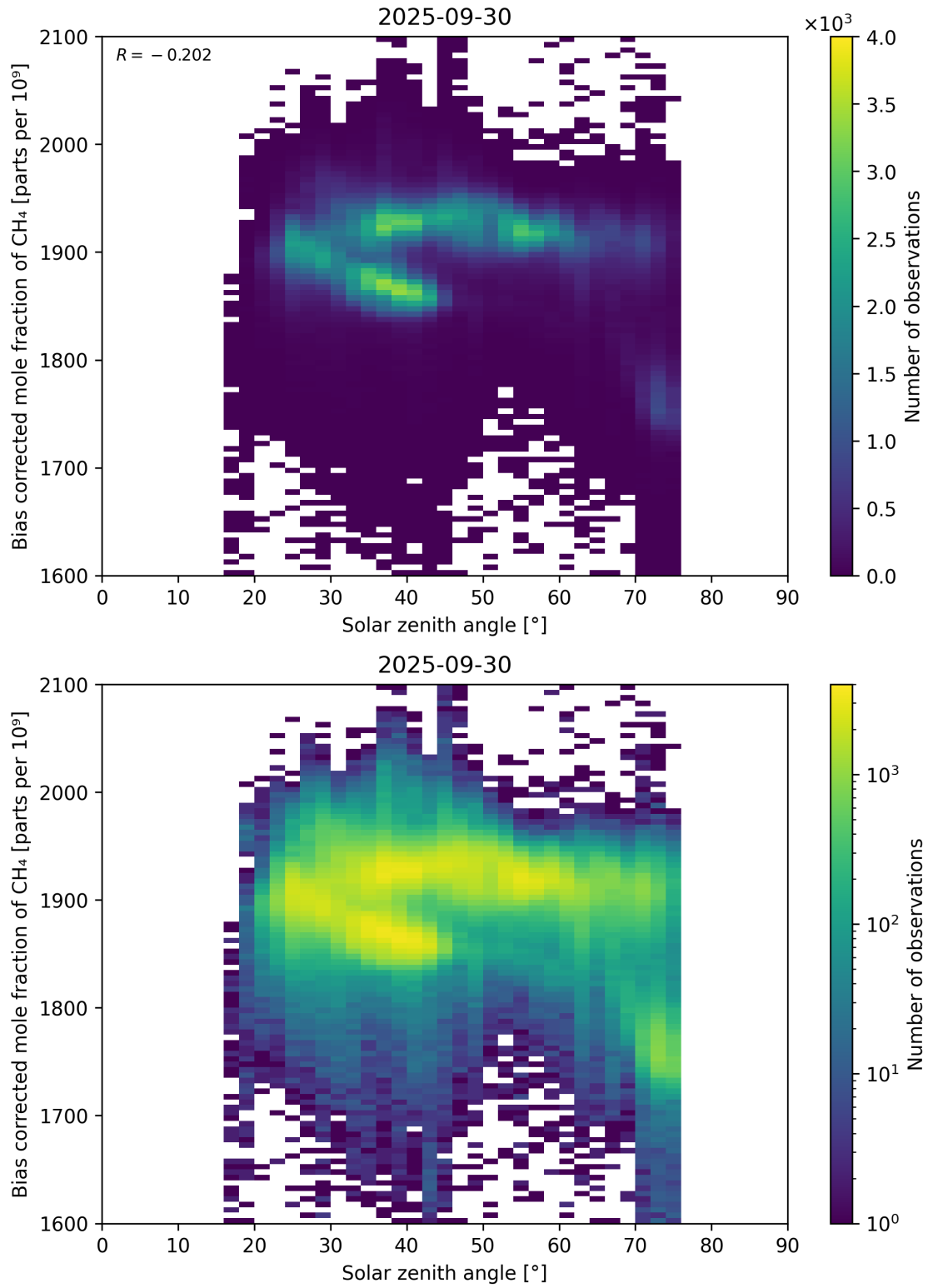
Figure 100: Scatter density plot of “Solar zenith angle” against “Bias corrected mole fraction of \text{CH}_4 ” for 2025-09-29 to 2025-10-01.
