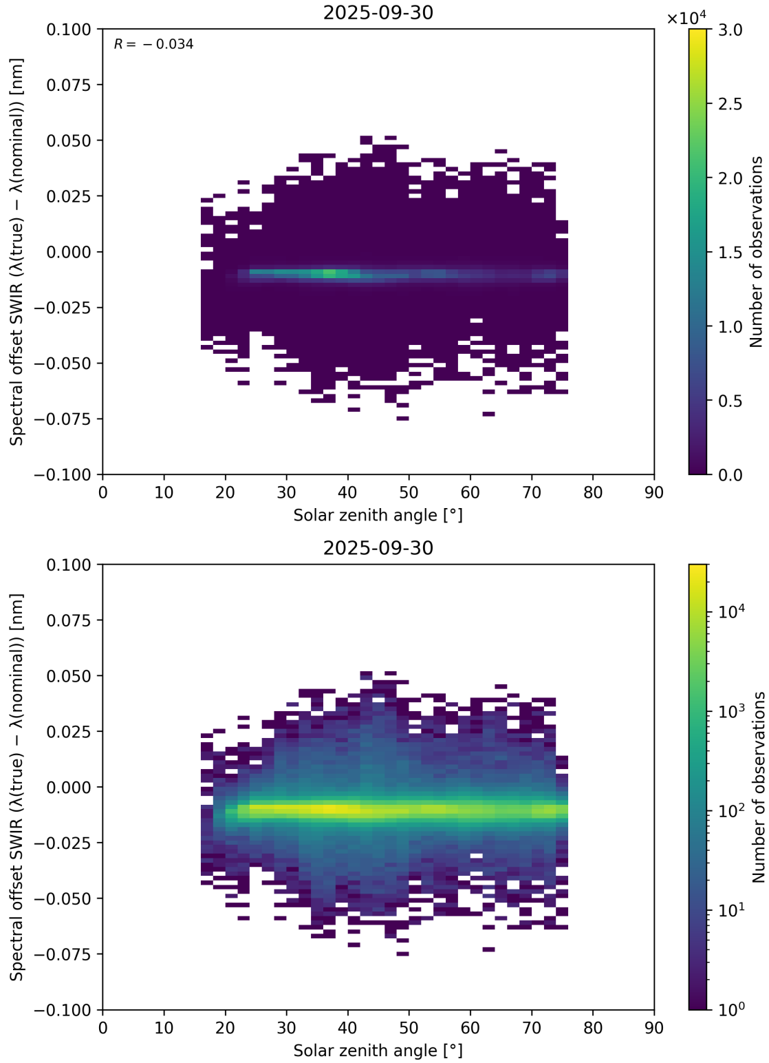
Figure 104: Scatter density plot of “Solar zenith angle” against “Spectral offset SWIR ( \lambda_{\text{true}} - \lambda_{\text{nominal}} )” for 2025-09-29 to 2025-10-01.
