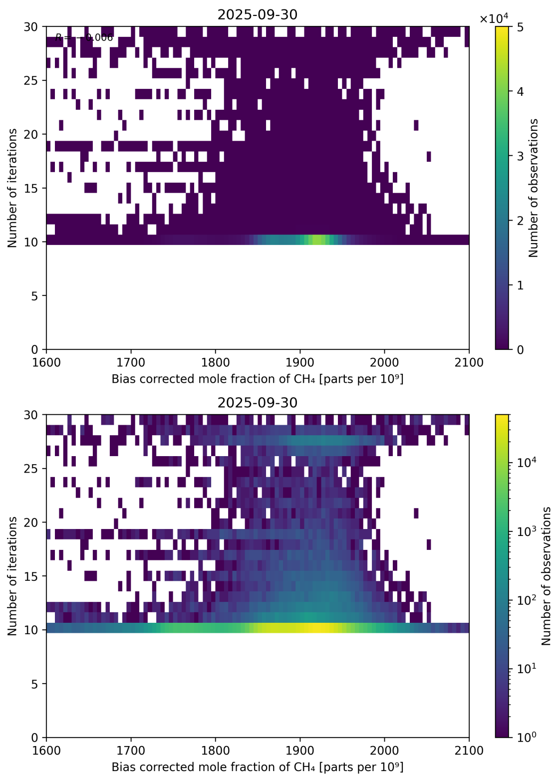
Figure 67: Scatter density plot of “Bias corrected mole fraction of \text{CH}_4 ” against “Number of iterations” for 2025-09-29 to 2025-10-01.
