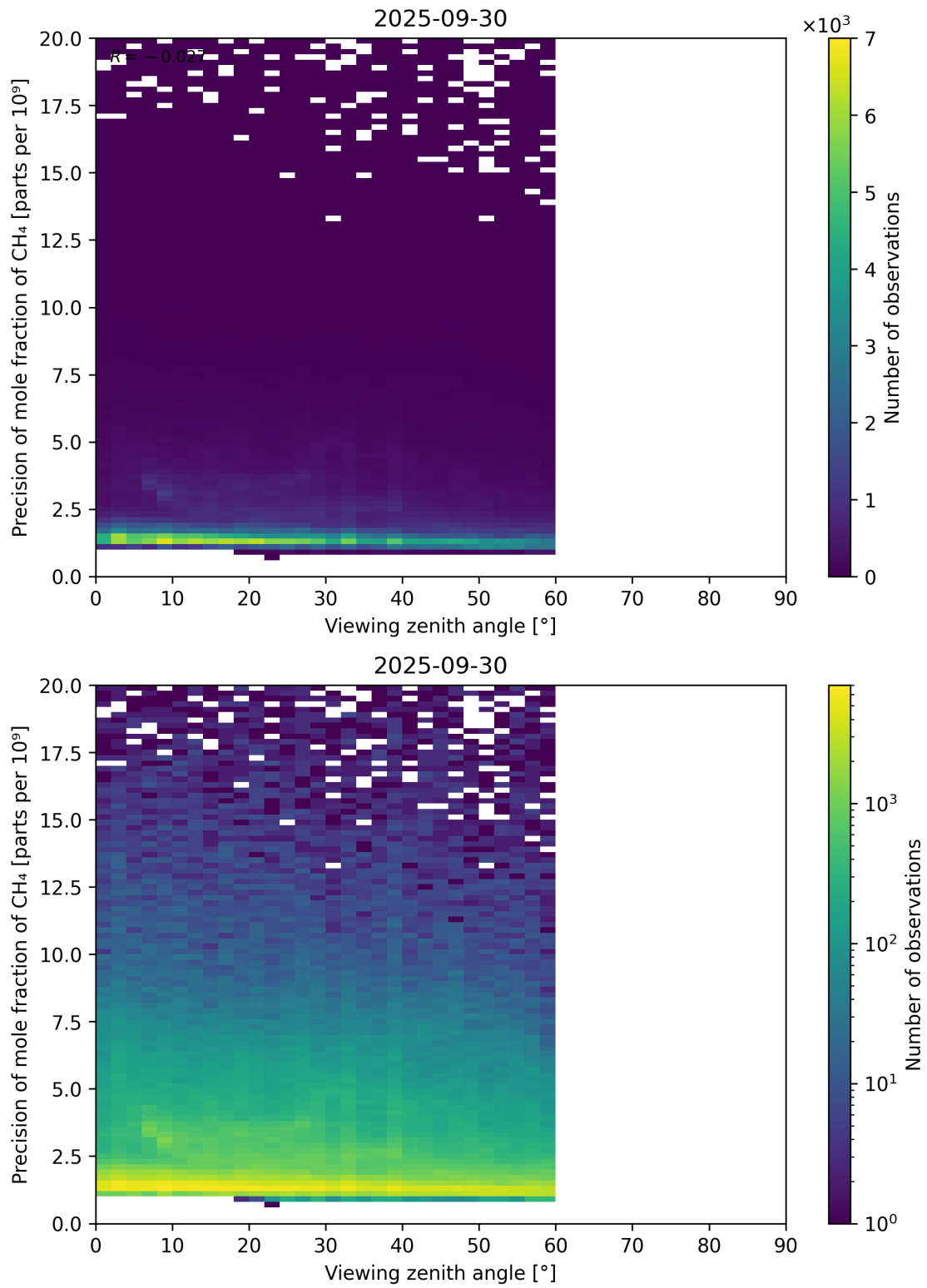
Figure 112: Scatter density plot of “Viewing zenith angle” against “Precision of mole fraction of CH 4 ” for 2025-09-29 to 2025-10-01.
