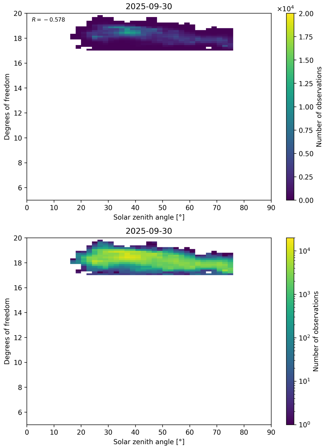
Figure 96: Scatter density plot of “Solar zenith angle” against “Degrees of freedom” for 2025-09-29 to 2025-10-01.
