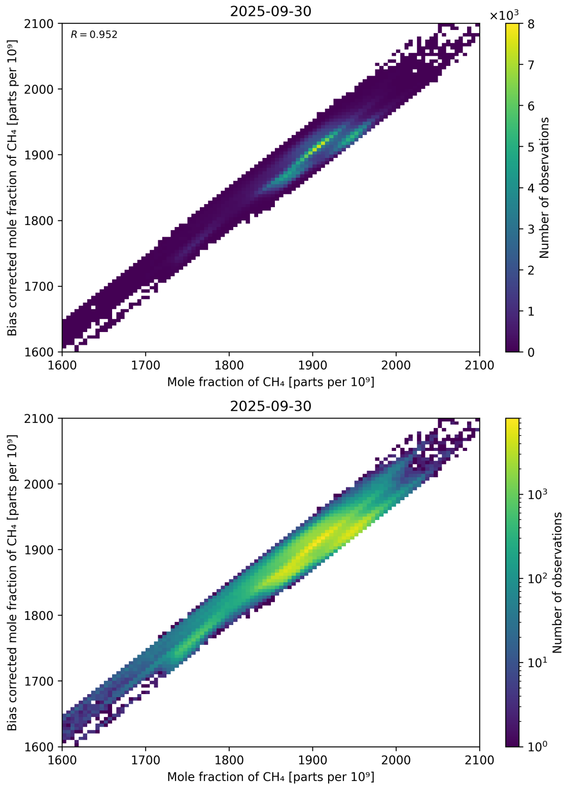
Figure 74: Scatter density plot of “Mole fraction of CH 4 ” against “Bias corrected mole fraction of CH 4 ” for 2025-09-29 to 2025-10-01.
