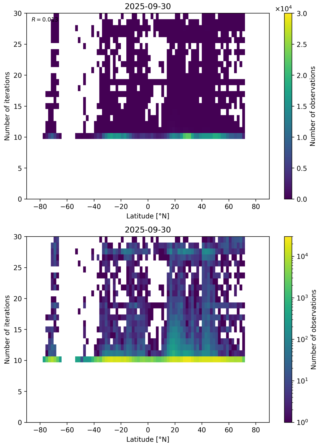
Figure 60: Scatter density plot of “Latitude” against “Number of iterations” for 2025-09-29 to 2025-10-01.
