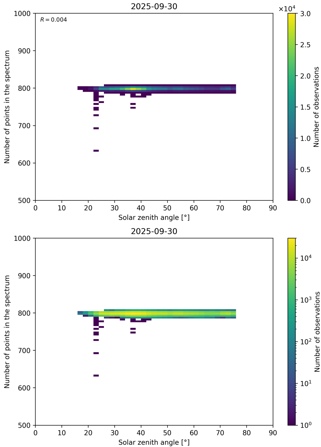
Figure 103: Scatter density plot of “Solar zenith angle” against “Number of points in the spectrum” for 2025-09-29 to 2025-10-01.
