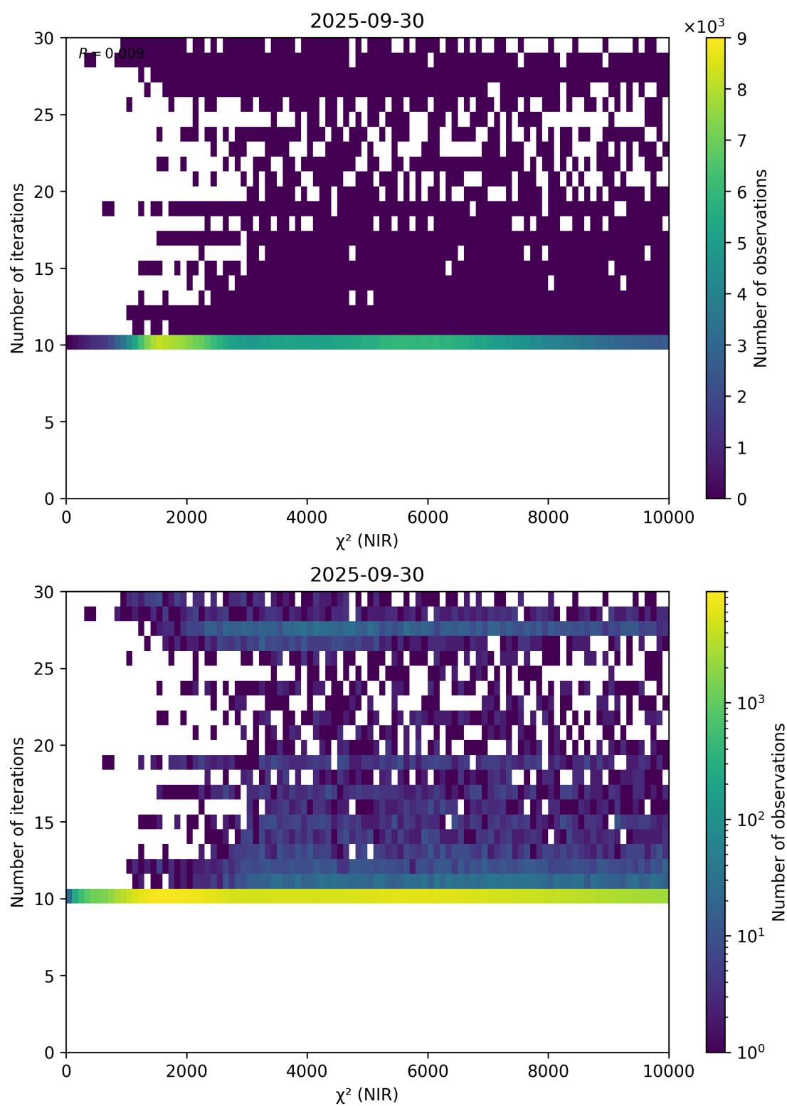
Figure 46: Scatter density plot of “ \chi^2 (NIR)” against “Number of iterations” for 2025-09-29 to 2025-10-01.
