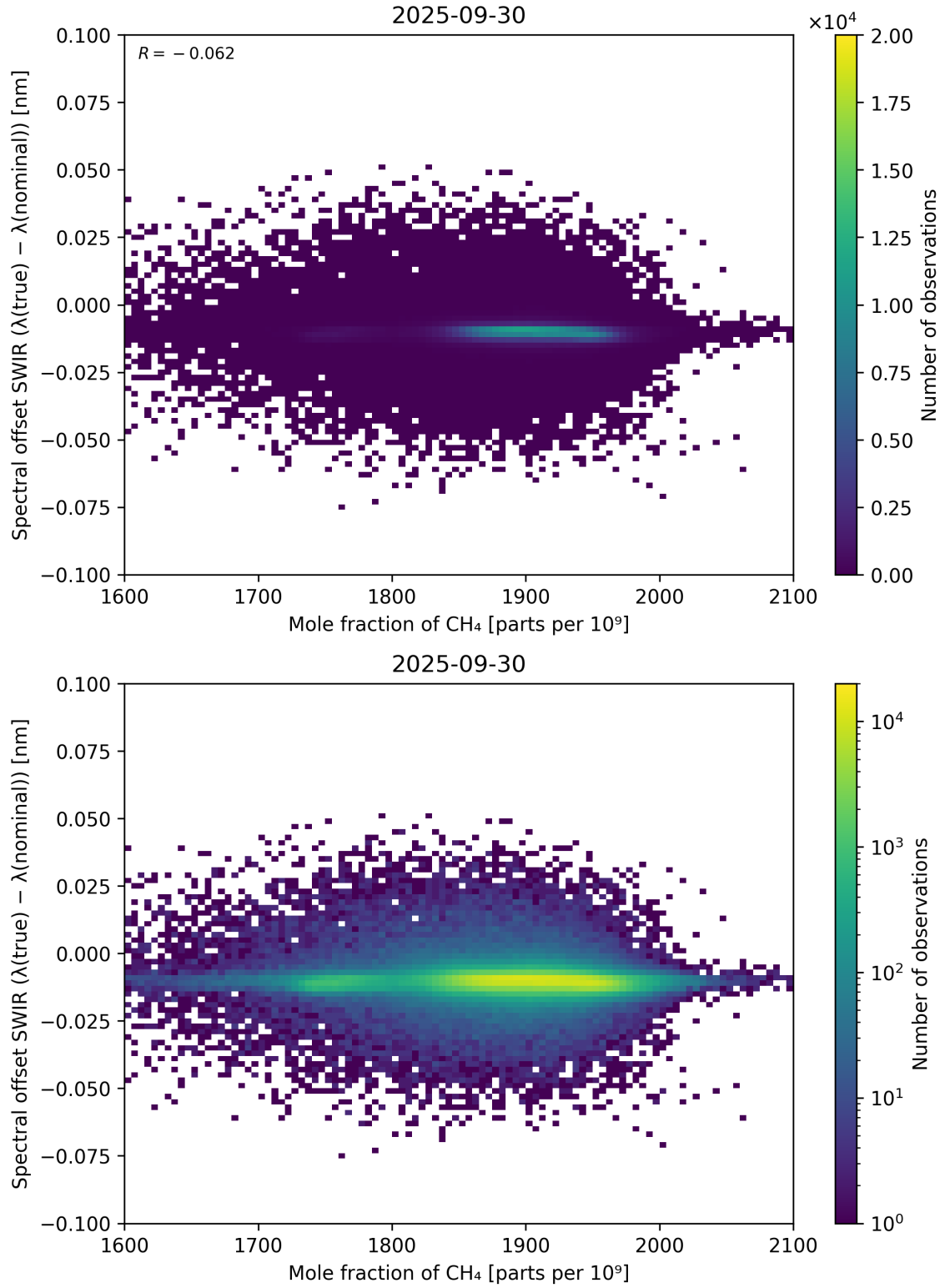
Figure 86: Scatter density plot of “Mole fraction of CH 4 ” against “Spectral offset SWIR ( \lambda_{\text{true}} - \lambda_{\text{nominal}} )” for 2025-09-29 to 2025-10-01.
