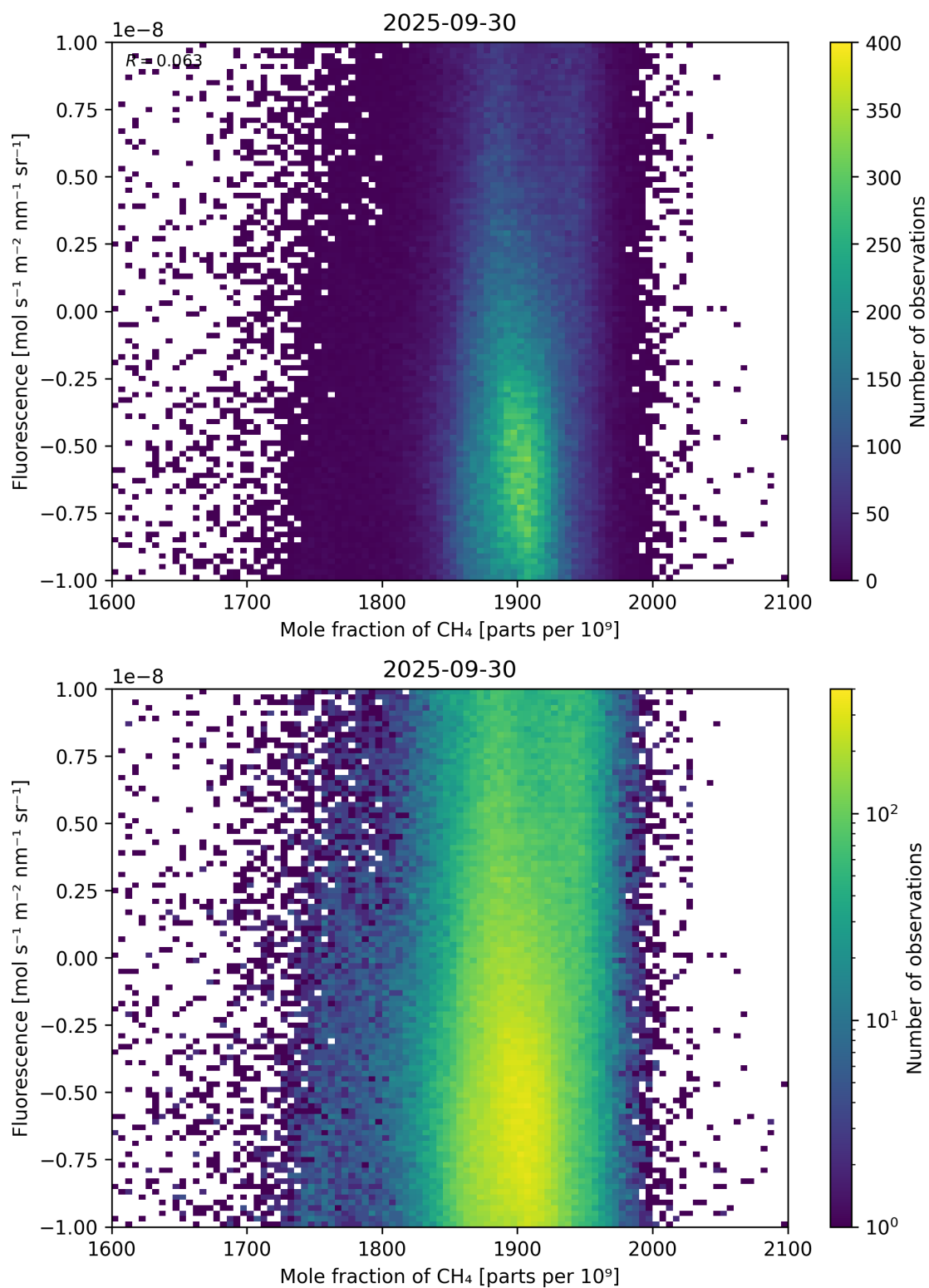
Figure 73: Scatter density plot of “Mole fraction of \text{CH}_4 ” against “Fluorescence” for 2025-09-29 to 2025-10-01.
