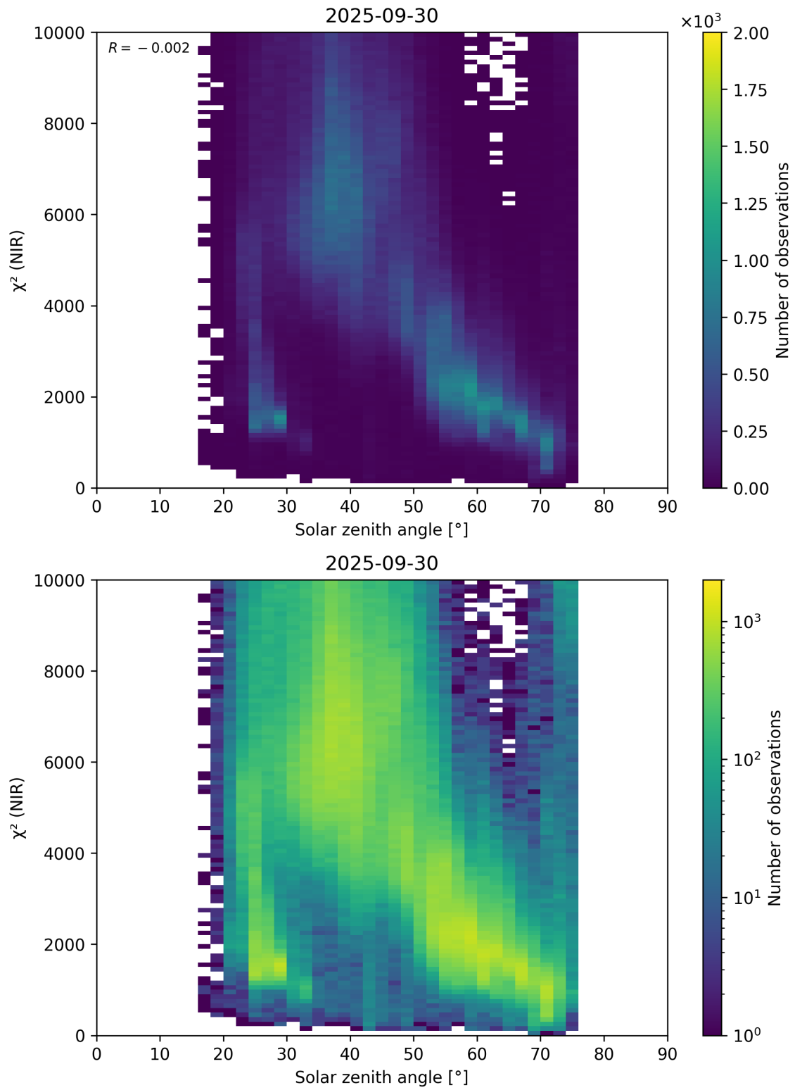
Figure 94: Scatter density plot of “Solar zenith angle” against “ \chi^2 (NIR)” for 2025-09-29 to 2025-10-01.
