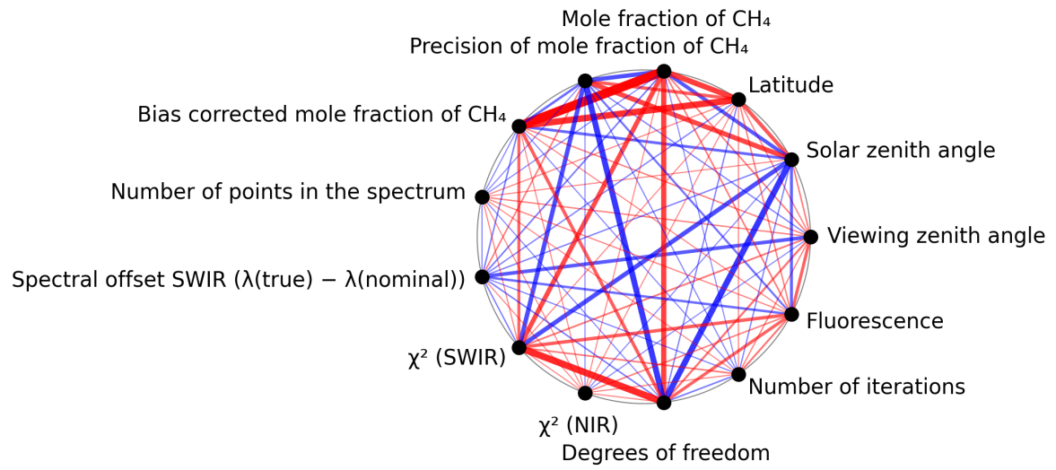
Figure 1: Map of correlation graph for 2025-09-29 to 2025-10-01.
