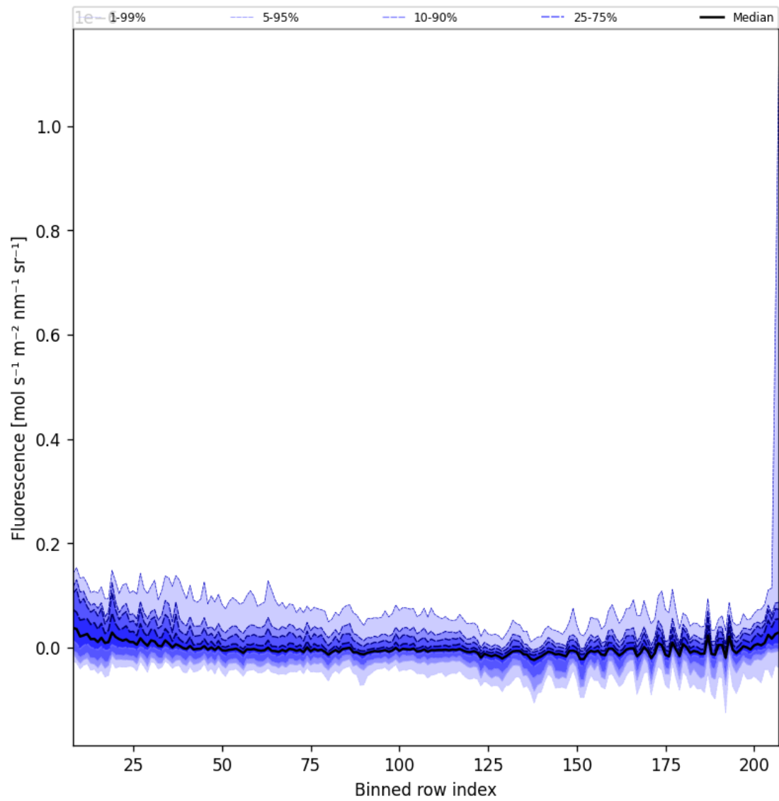
Figure 43: Along track statistics of “Fluorescence” for 2025-09-29 to 2025-10-01
