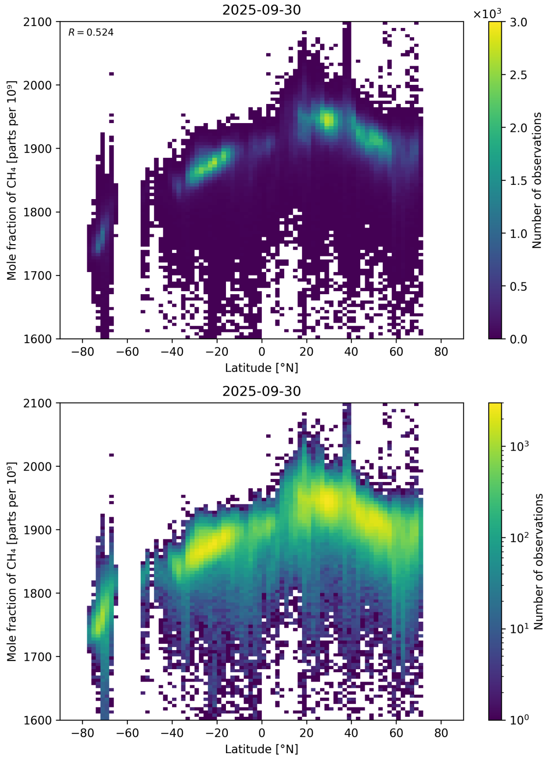
Figure 57: Scatter density plot of “Latitude” against “Mole fraction of CH 4 ” for 2025-09-29 to 2025-10-01.
