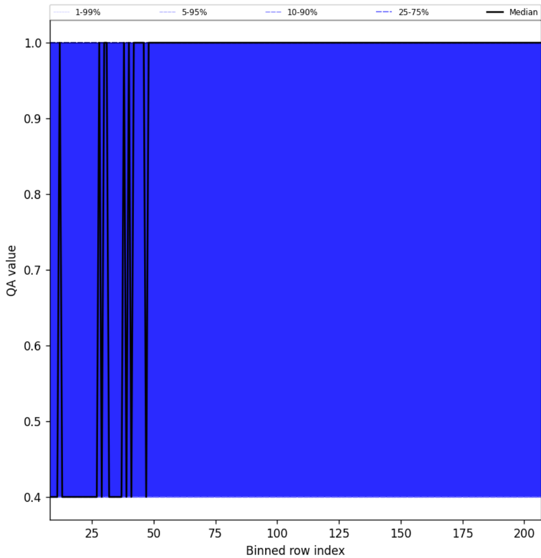
Figure 33: Along track statistics of “QA value” for 2025-09-29 to 2025-10-01
