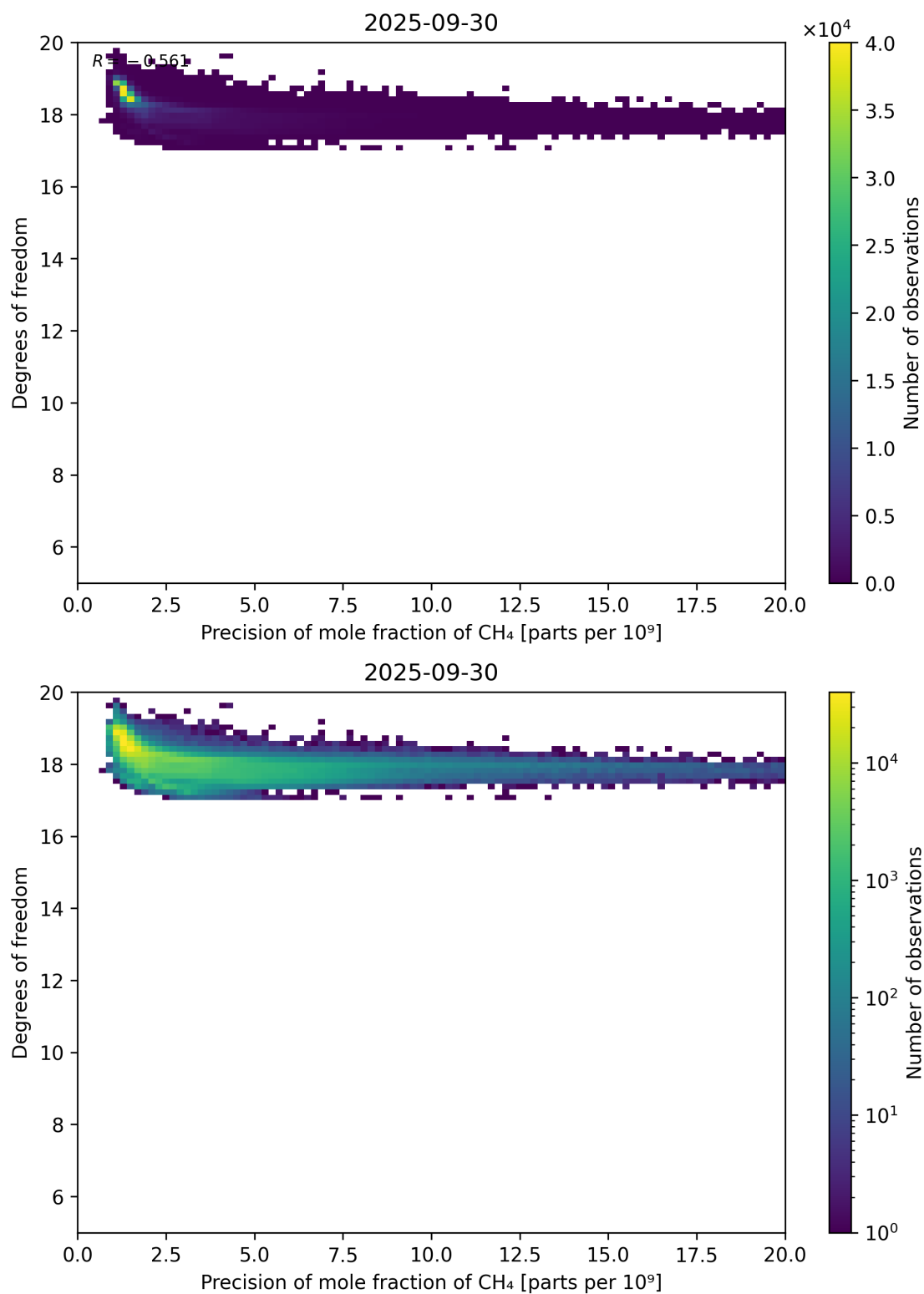
Figure 80: Scatter density plot of “Precision of mole fraction of CH 4 ” against “Degrees of freedom” for 2025-09-29 to 2025-10-01.
