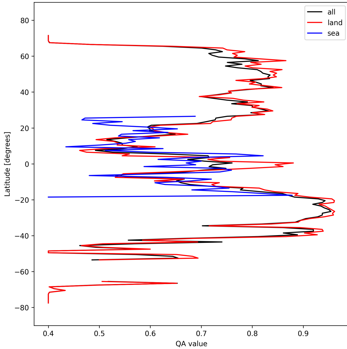
Figure 11: Zonal average of “QA value” for 2025-09-29 to 2025-10-01.
