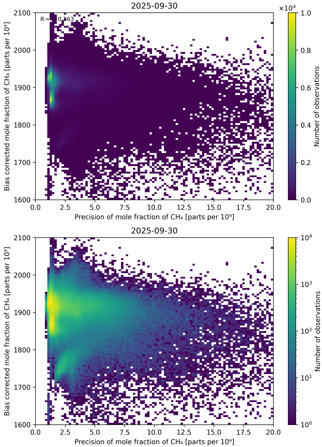
Figure 82: Scatter density plot of “Precision of mole fraction of CH 4 ” against “Bias corrected mole fraction of CH 4 ” for 2025-09-29 to 2025-10-01.
