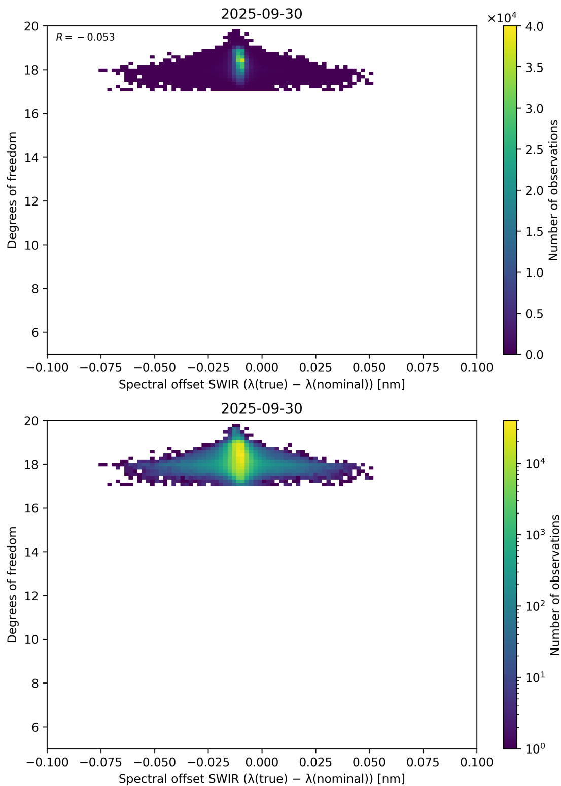
Figure 119: Scatter density plot of “Spectral offset SWIR ( \lambda_{\text{true}} - \lambda_{\text{nominal}} )” against “Degrees of freedom” for 2025-09-29 to 2025-10-01.
