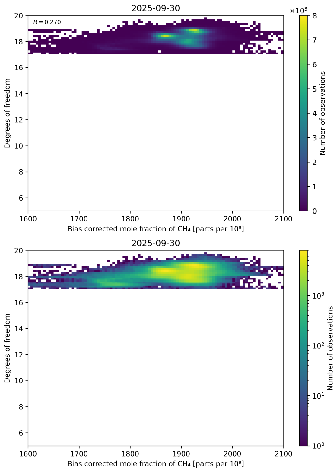
Figure 65: Scatter density plot of “Bias corrected mole fraction of CH 4 ” against “Degrees of freedom” for 2025-09-29 to 2025-10-01.
