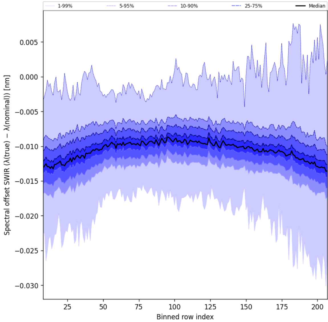
Figure 38: Along track statistics of “Spectral offset SWIR ( \lambda_{\text{true}} - \lambda_{\text{nominal}} )” for 2025-09-29 to 2025-10-01
