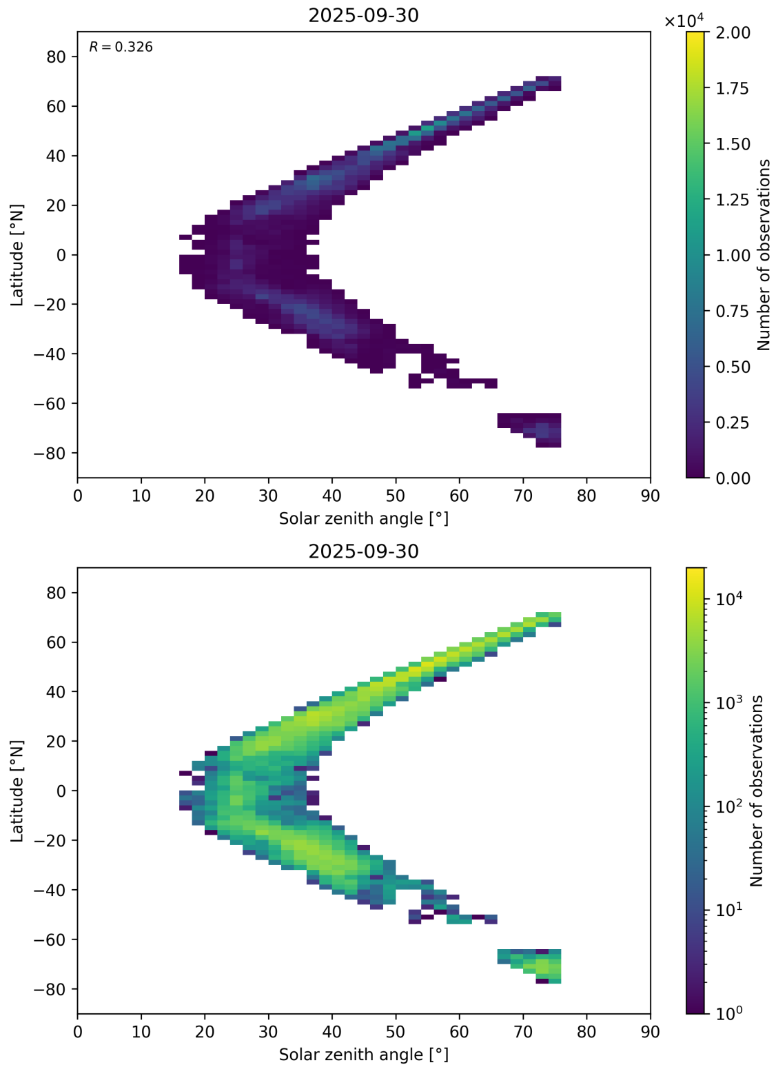
Figure 98: Scatter density plot of “Solar zenith angle” against “Latitude” for 2025-09-29 to 2025-10-01.
