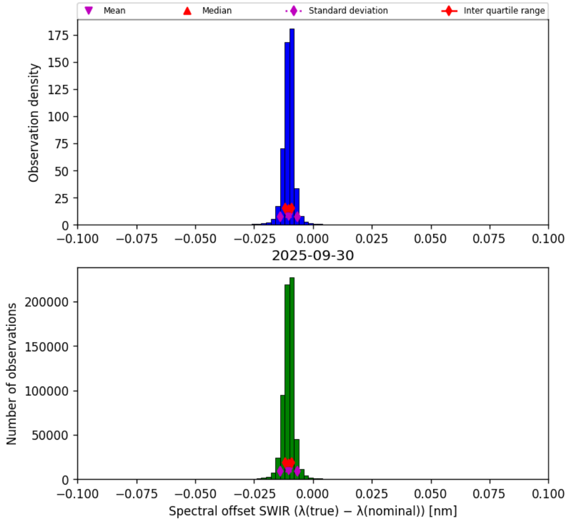
Figure 27: Histogram of “Spectral offset SWIR ( \lambda_{\text{true}} - \lambda_{\text{nominal}} )” for 2025-09-29 to 2025-10-01
