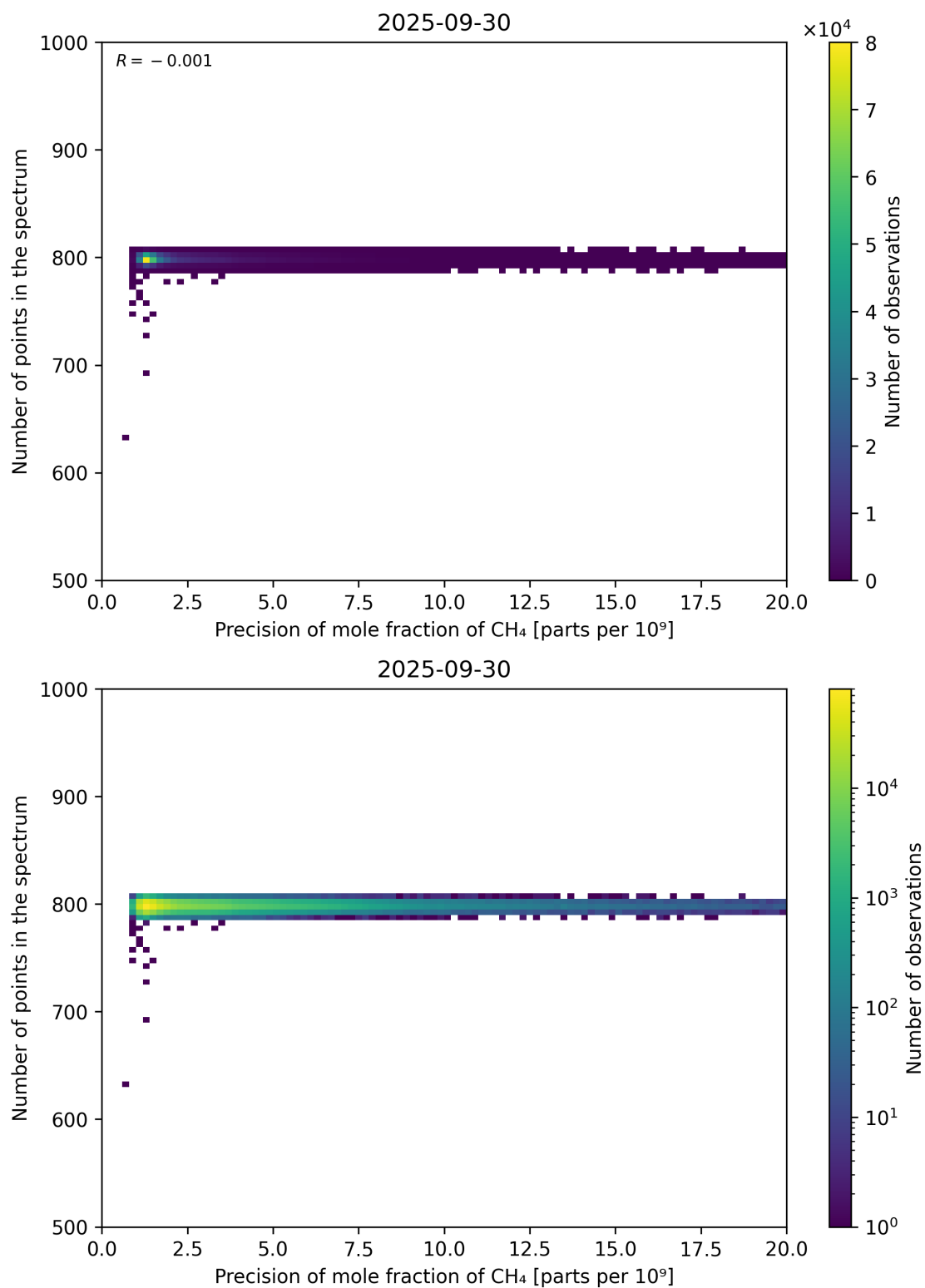
Figure 84: Scatter density plot of “Precision of mole fraction of CH 4 ” against “Number of points in the spectrum” for 2025-09-29 to 2025-10-01.
