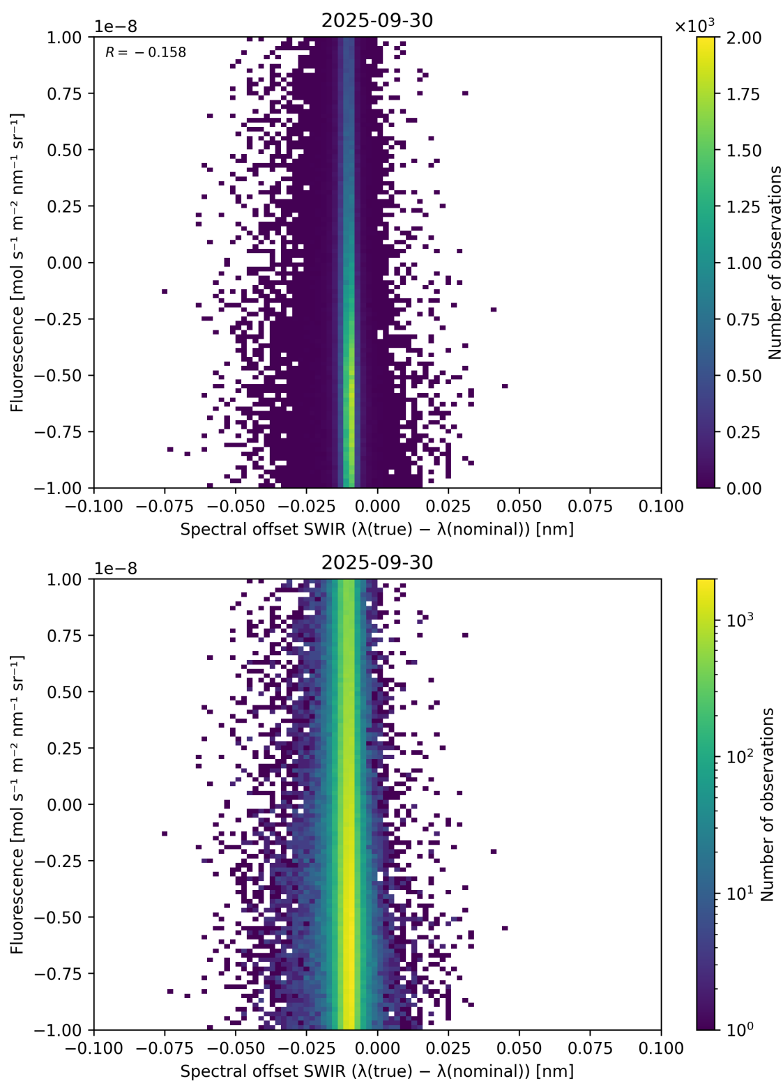
Figure 120: Scatter density plot of “Spectral offset SWIR ( \lambda_{\text{true}} - \lambda_{\text{nominal}} )” against “Fluorescence” for 2025-09-29 to 2025-10-01.
