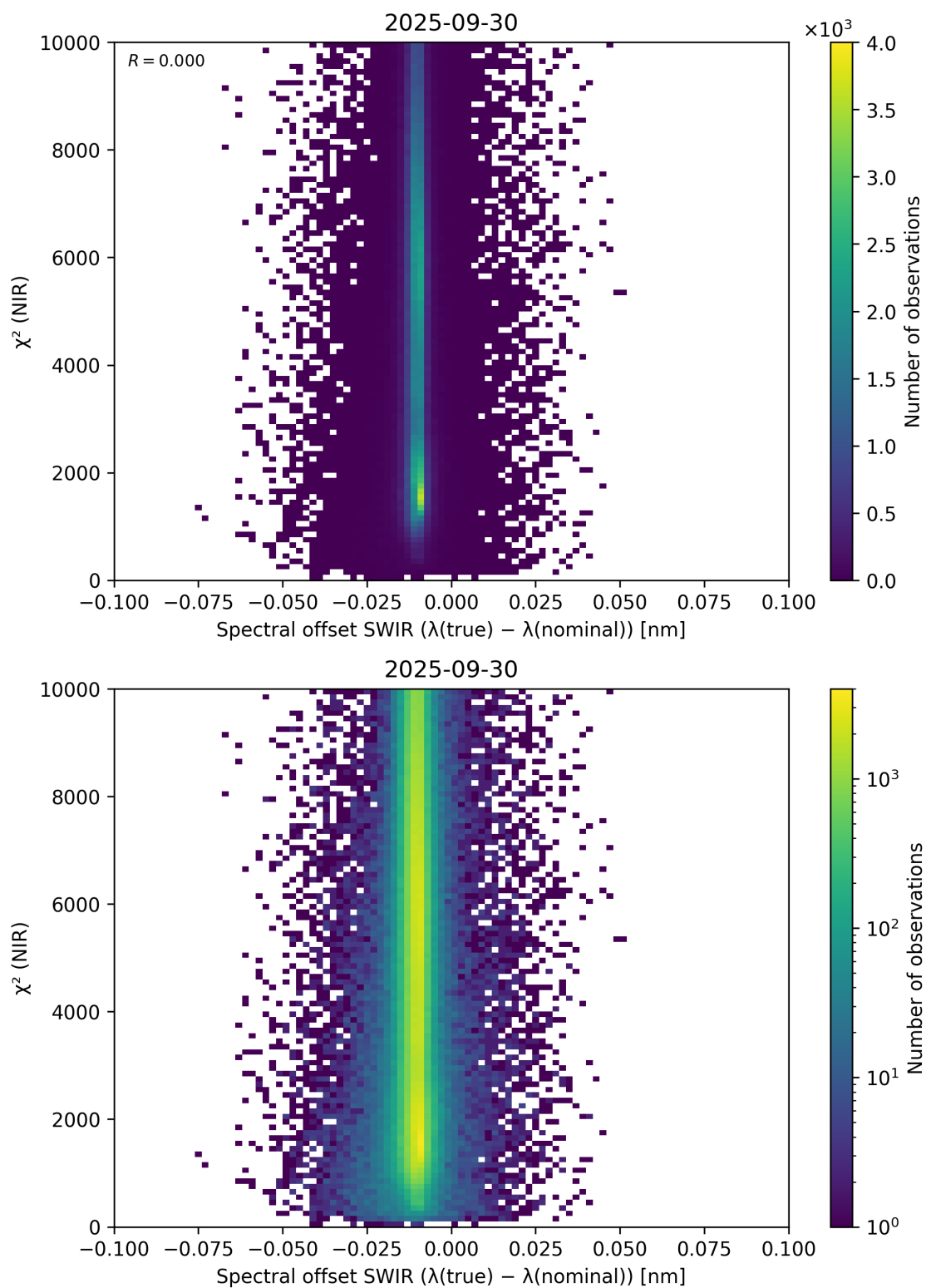
Figure 117: Scatter density plot of “Spectral offset SWIR ( \lambda_{\text{true}} - \lambda_{\text{nominal}} )” against “ \chi^2 (NIR)” for 2025-09-29 to 2025-10-01.
