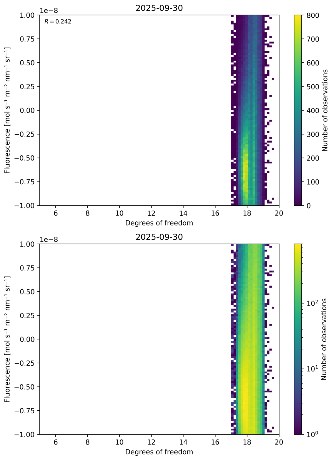
Figure 51: Scatter density plot of “Degrees of freedom” against “Fluorescence” for 2025-09-29 to 2025-10-01.
