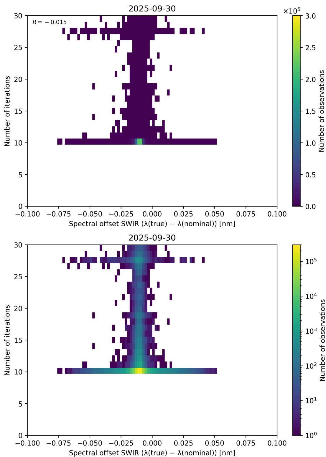
Figure 121: Scatter density plot of “Spectral offset SWIR ( \lambda_{\text{true}} - \lambda_{\text{nominal}} )” against “Number of iterations” for 2025-09-29 to 2025-10-01.
