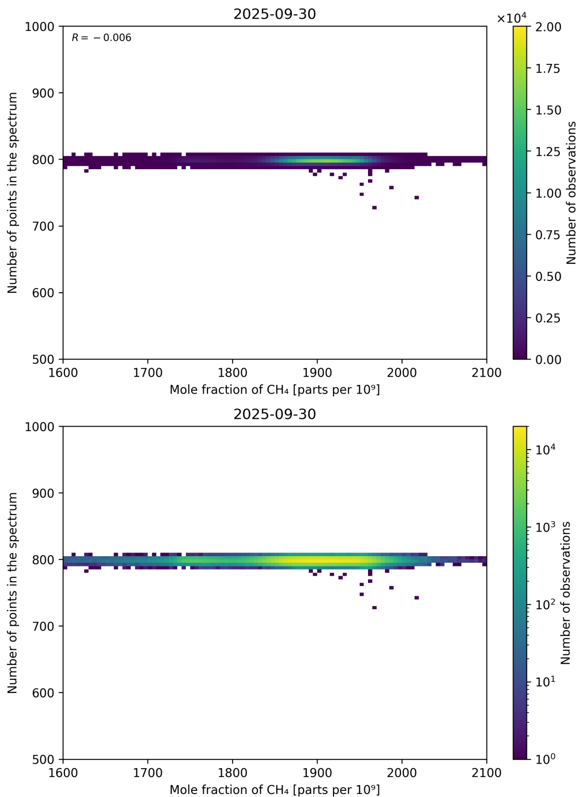
Figure 77: Scatter density plot of “Mole fraction of CH 4 ” against “Number of points in the spectrum” for 2025-09-29 to 2025-10-01.
