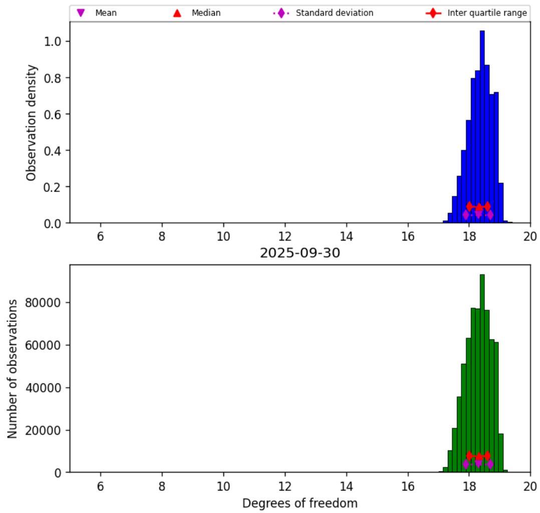
Figure 30: Histogram of “Degrees of freedom” for 2025-09-29 to 2025-10-01
