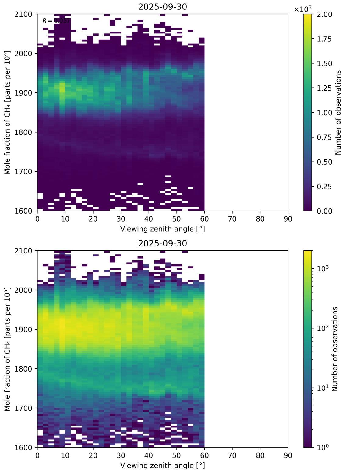
Figure 110: Scatter density plot of “Viewing zenith angle” against “Mole fraction of CH 4 ” for 2025-09-29 to 2025-10-01.
