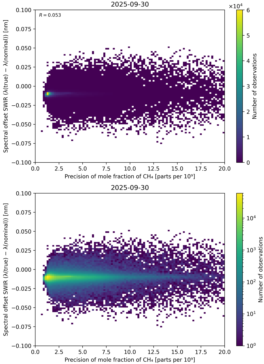
Figure 85: Scatter density plot of “Precision of mole fraction of CH 4 ” against “Spectral offset SWIR ( \lambda_{\text{true}} - \lambda_{\text{nominal}} )” for 2025-09-29 to 2025-10-01.
