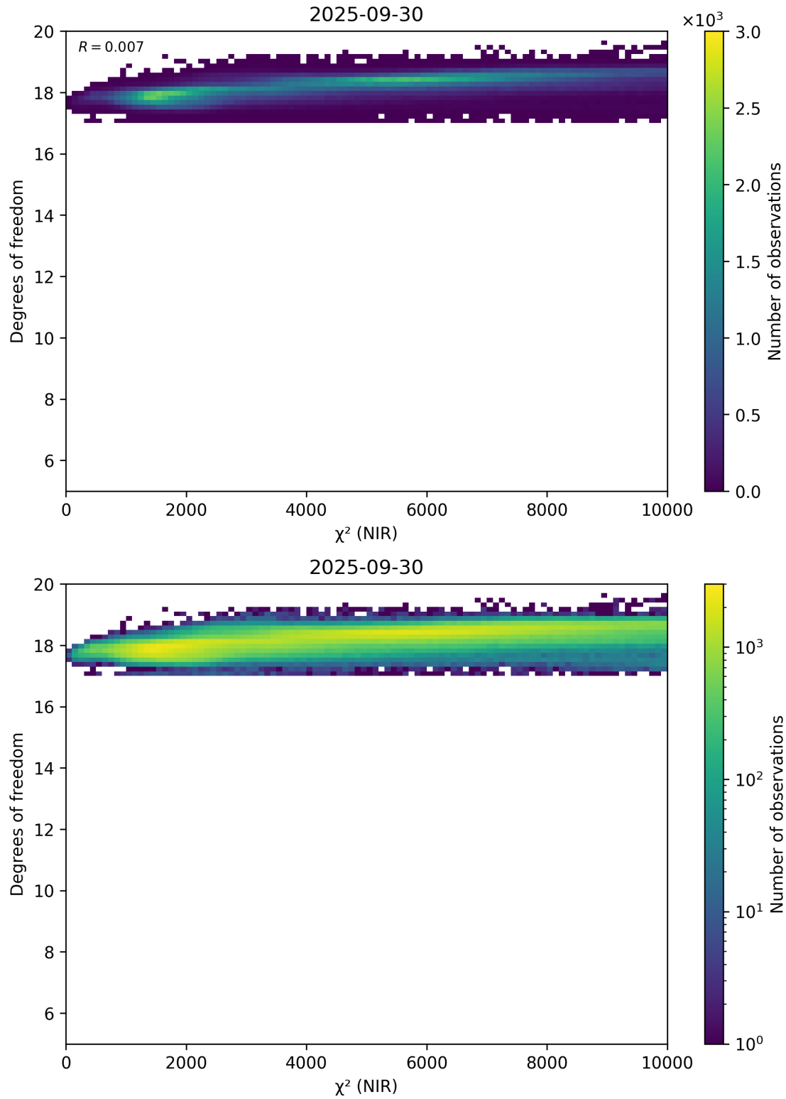
Figure 44: Scatter density plot of “ \chi^2 (NIR)” against “Degrees of freedom” for 2025-09-29 to 2025-10-01.
