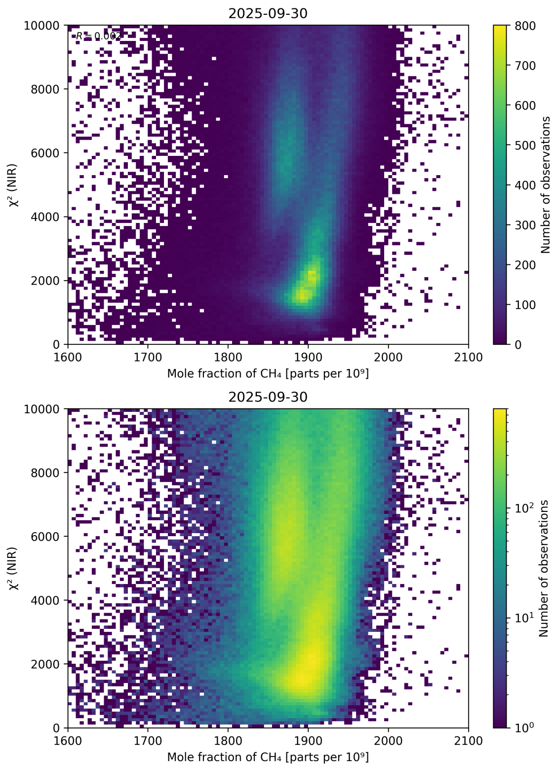
Figure 70: Scatter density plot of “Mole fraction of \text{CH}_4 ” against “ \chi^2 (NIR)” for 2025-09-29 to 2025-10-01.
