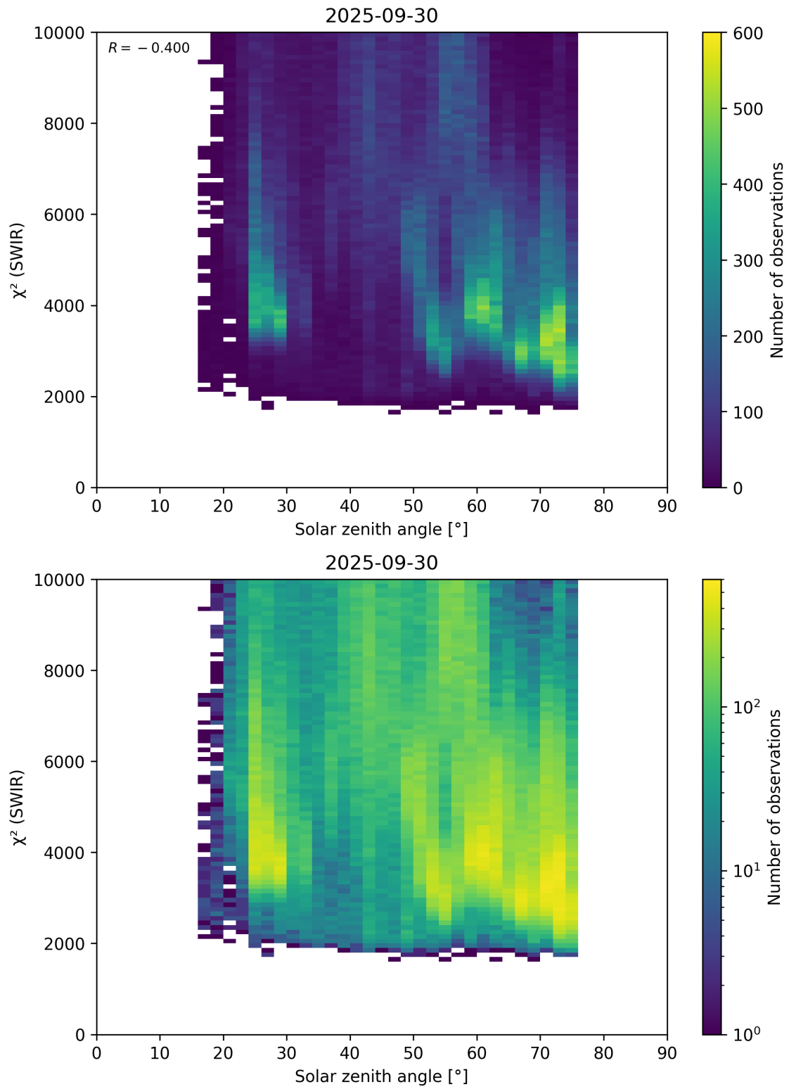
Figure 95: Scatter density plot of “Solar zenith angle” against “ \chi^2 (SWIR)” for 2025-09-29 to 2025-10-01.
