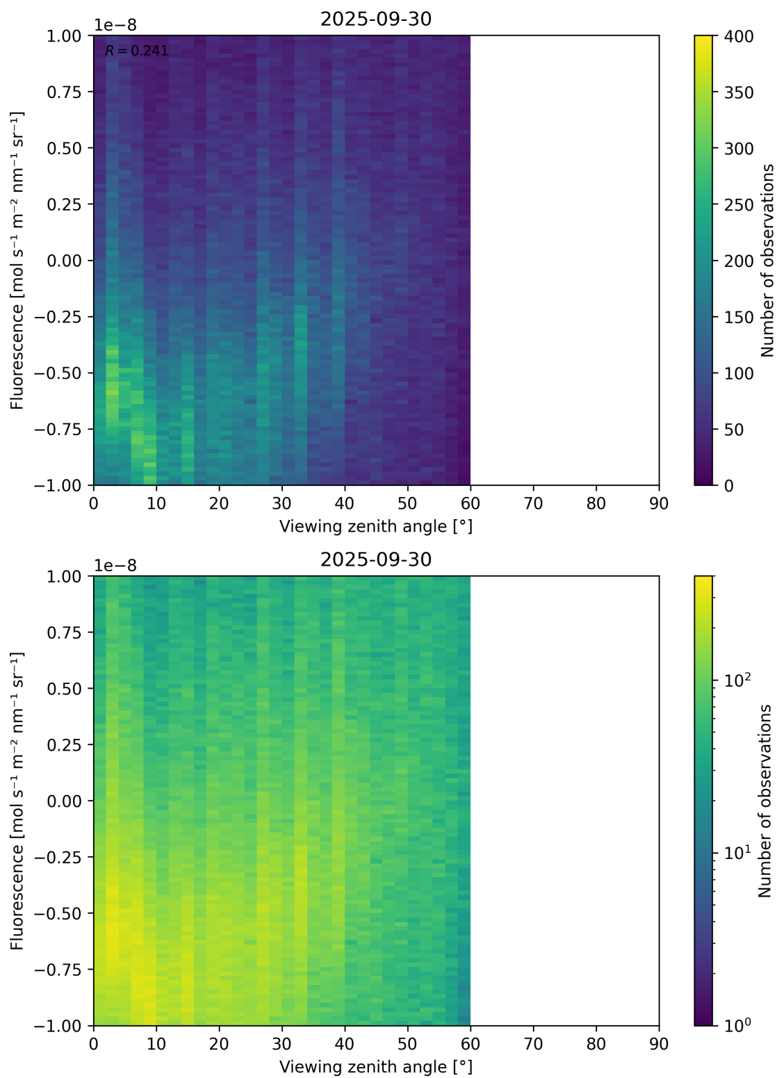
Figure 108: Scatter density plot of “Viewing zenith angle” against “Fluorescence” for 2025-09-29 to 2025-10-01.
