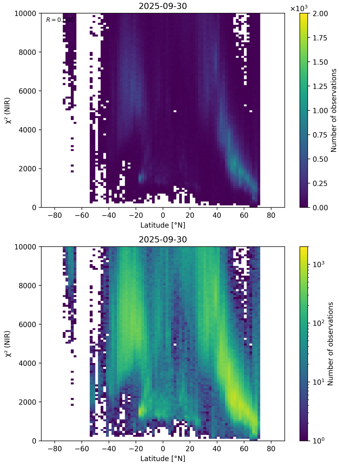
Figure 53: Scatter density plot of “Latitude” against “ \chi^2 (NIR)” for 2025-09-29 to 2025-10-01.
