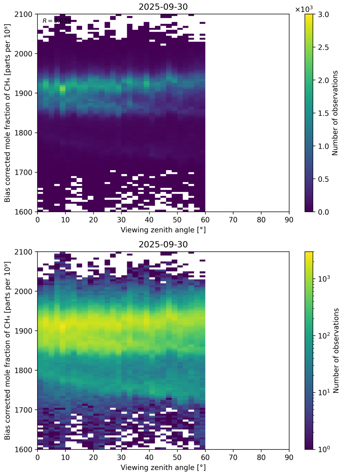
Figure 111: Scatter density plot of “Viewing zenith angle” against “Bias corrected mole fraction of CH 4 ” for 2025-09-29 to 2025-10-01.
