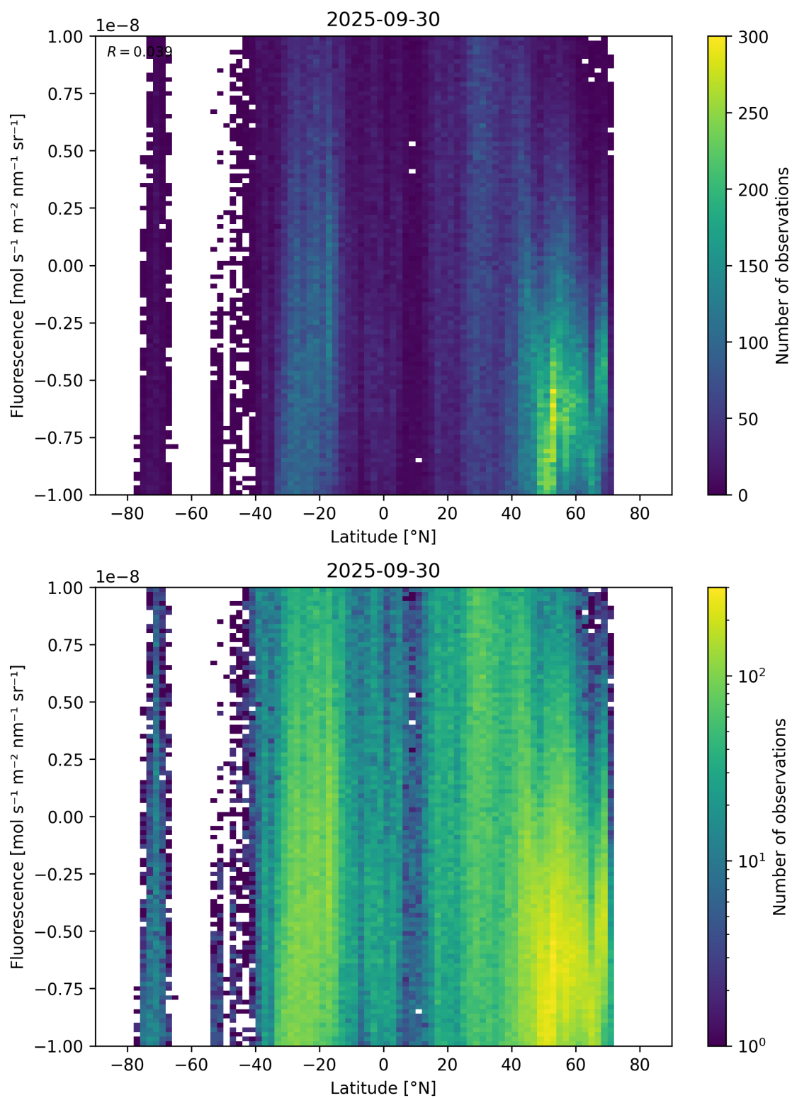
Figure 56: Scatter density plot of “Latitude” against “Fluorescence” for 2025-09-29 to 2025-10-01.
