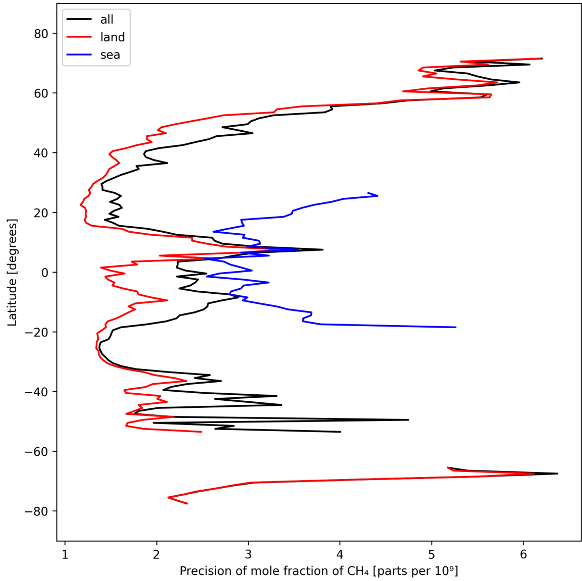
Figure 13: Zonal average of “Precision of mole fraction of CH 4 ” for 2025-09-29 to 2025-10-01.
