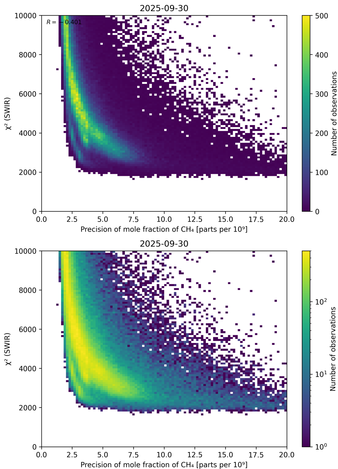
Figure 79: Scatter density plot of “Precision of mole fraction of \text{CH}_4 ” against “ \chi^2 (SWIR)” for 2025-09-29 to 2025-10-01.
