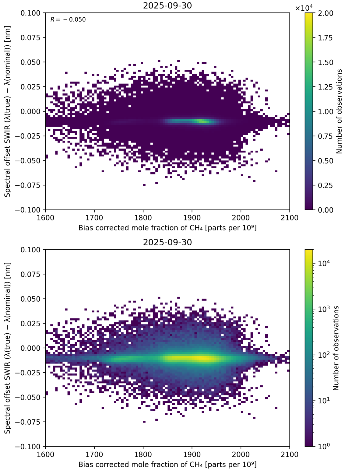
Figure 69: Scatter density plot of “Bias corrected mole fraction of \text{CH}_4 ” against “Spectral offset SWIR ( \lambda_{\text{true}} - \lambda_{\text{nominal}} )” for 2025-09-29 to 2025-10-01.
