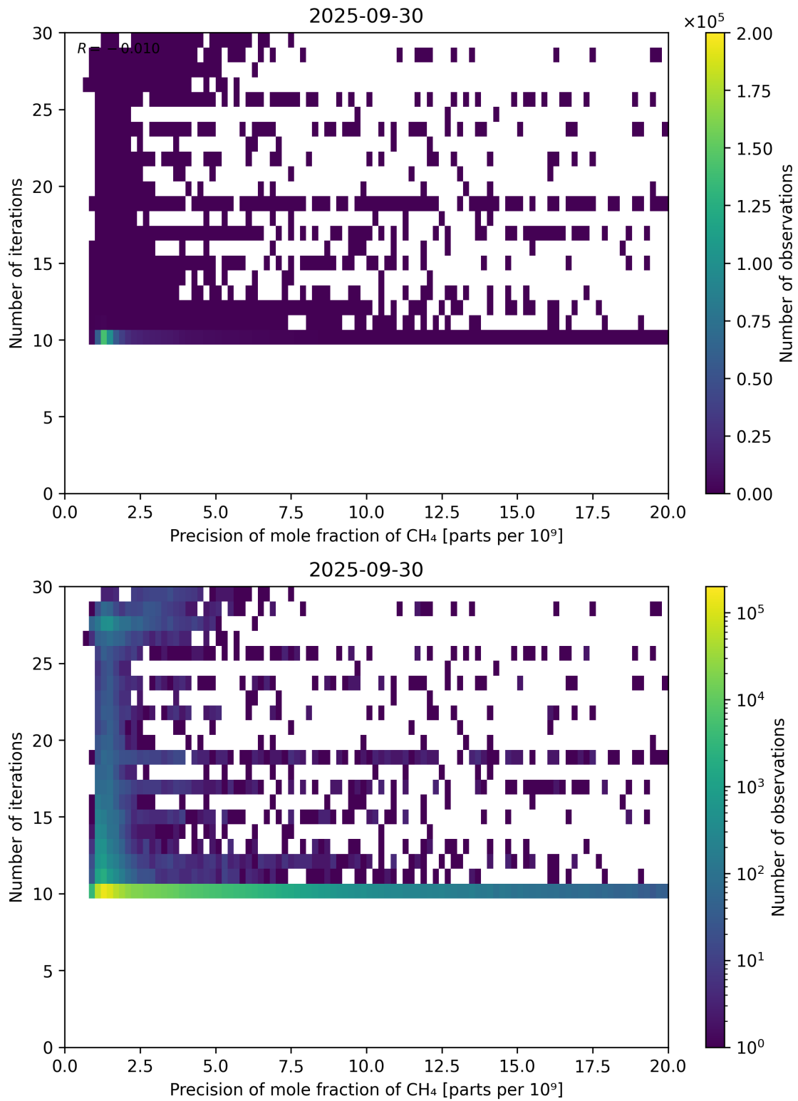
Figure 83: Scatter density plot of “Precision of mole fraction of CH 4 ” against “Number of iterations” for 2025-09-29 to 2025-10-01.
