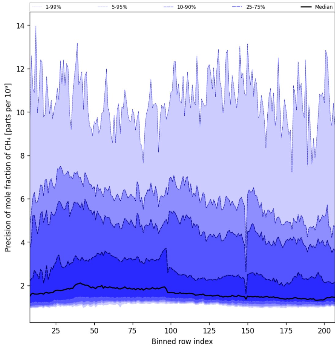
Figure 35: Along track statistics of “Precision of mole fraction of CH 4 ” for 2025-09-29 to 2025-10-01
