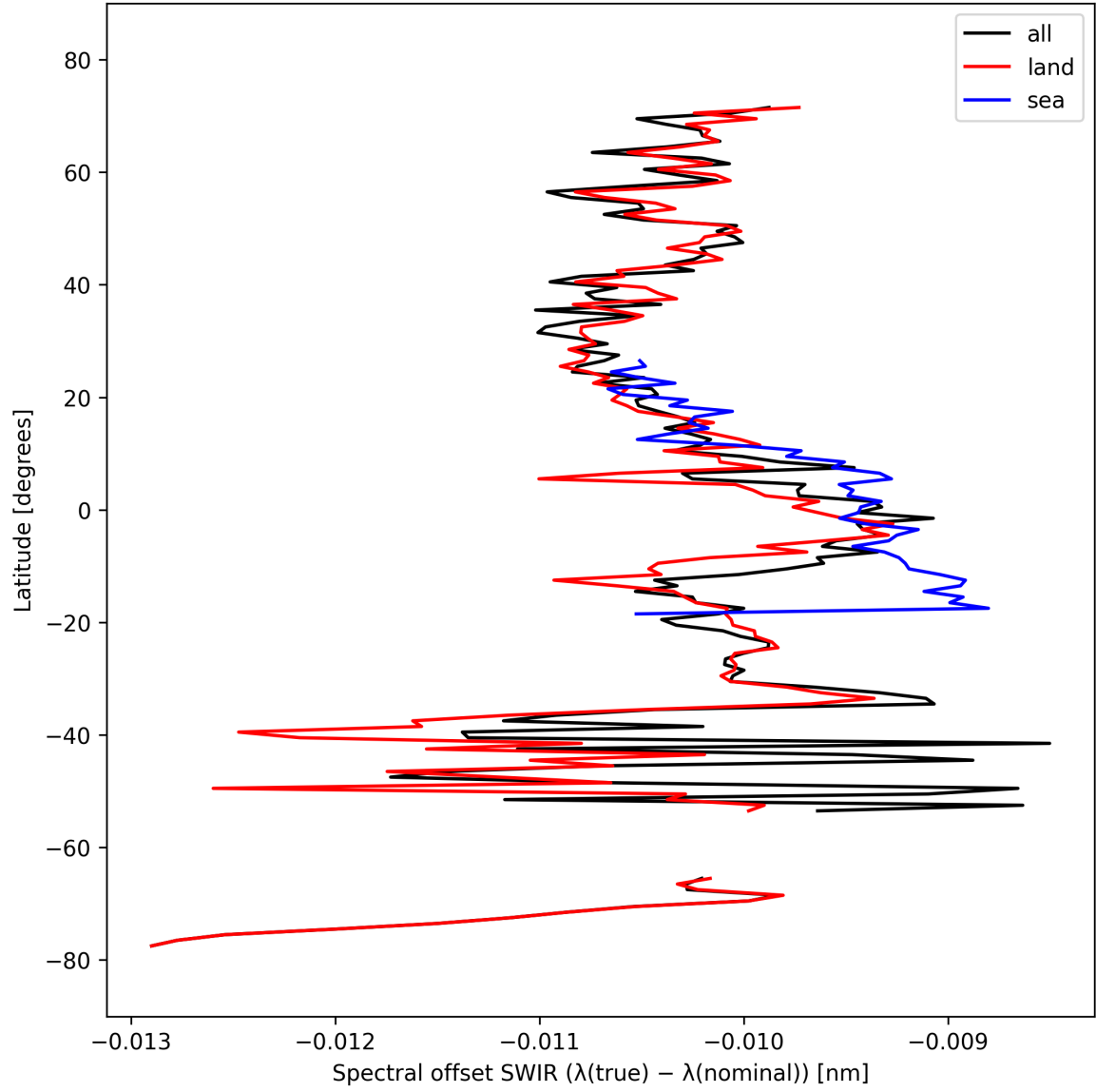
Figure 16: Zonal average of “Spectral offset SWIR ( \lambda_{\text{true}} - \lambda_{\text{nominal}} )” for 2025-09-29 to 2025-10-01.
