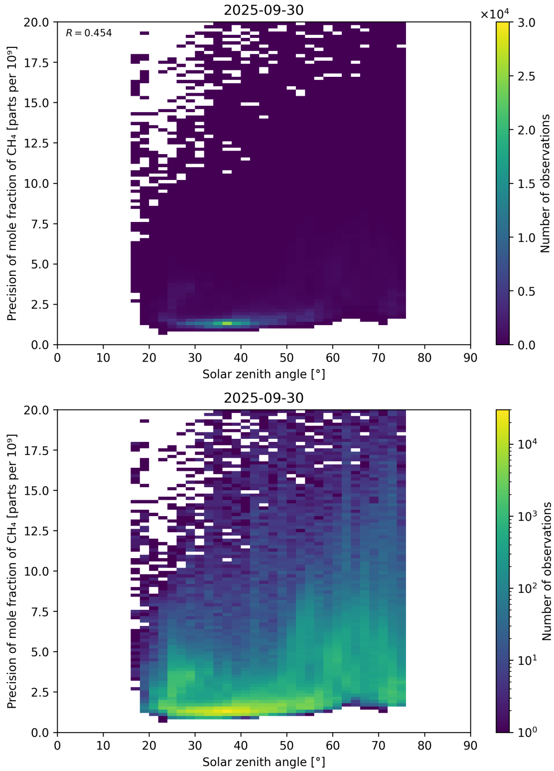
Figure 101: Scatter density plot of “Solar zenith angle” against “Precision of mole fraction of CH 4 ” for 2025-09-29 to 2025-10-01.
