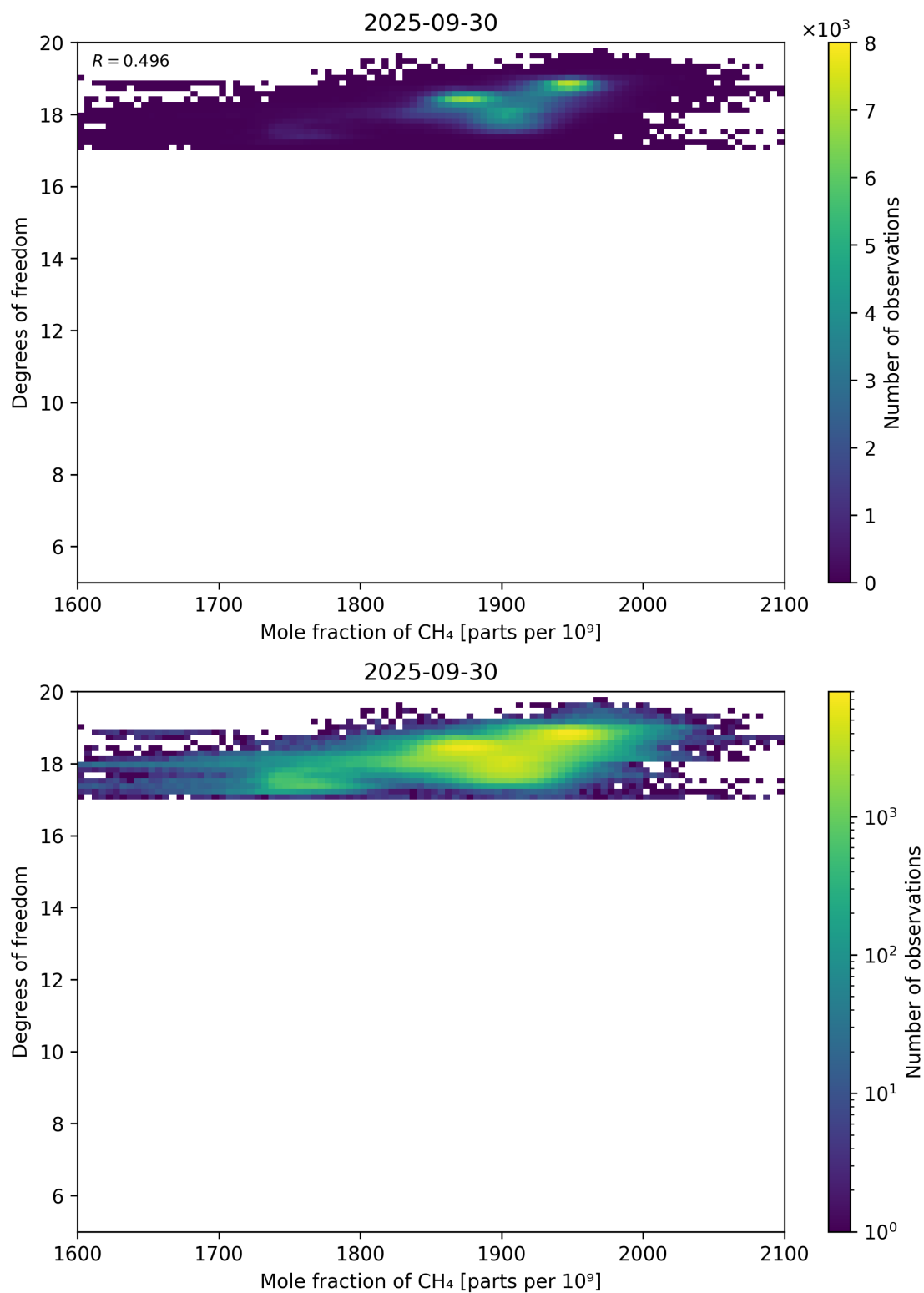
Figure 72: Scatter density plot of “Mole fraction of CH 4 ” against “Degrees of freedom” for 2025-09-29 to 2025-10-01.
