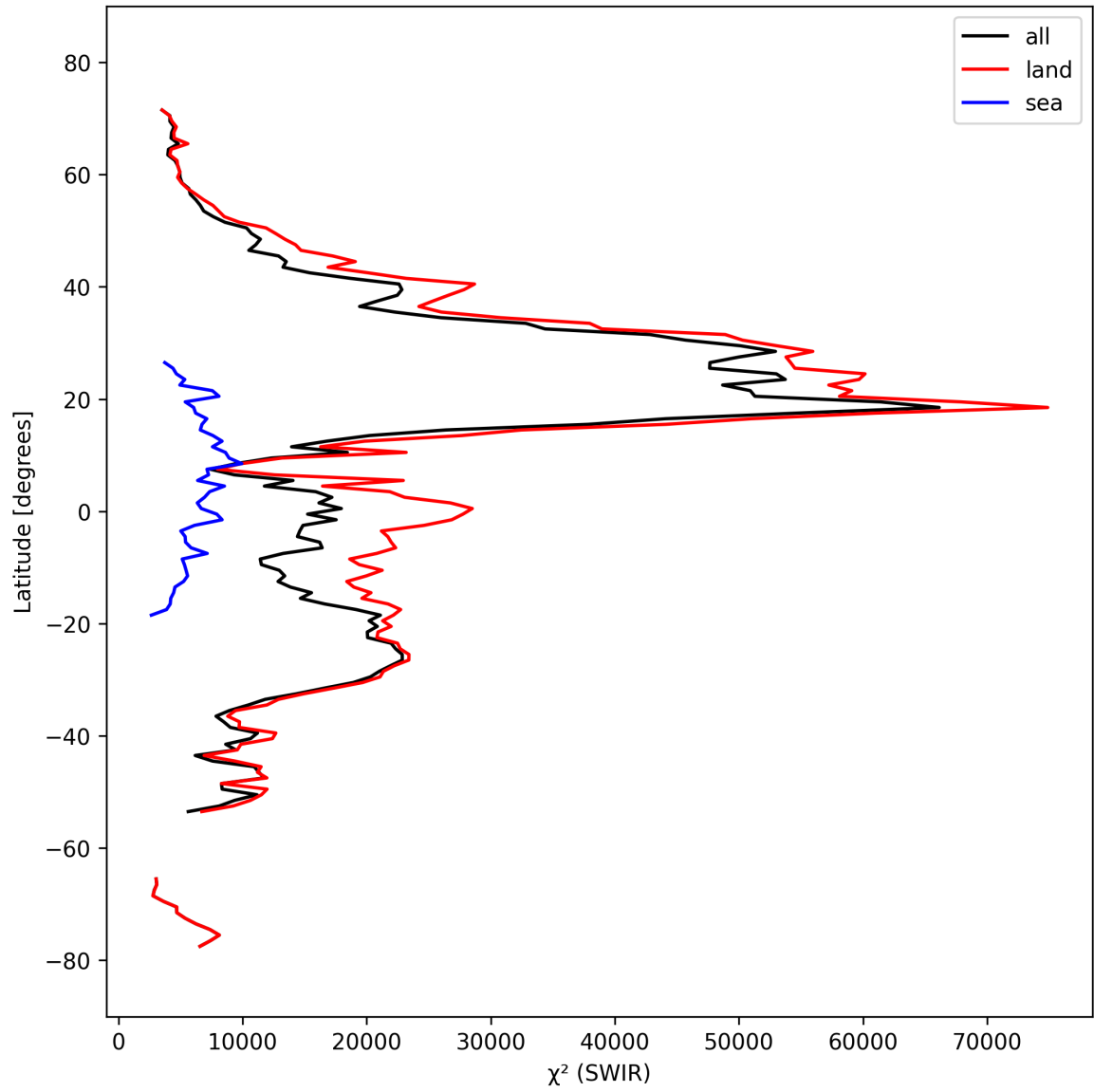
Figure 17: Zonal average of “ \chi^2 (SWIR)” for 2025-09-29 to 2025-10-01.
