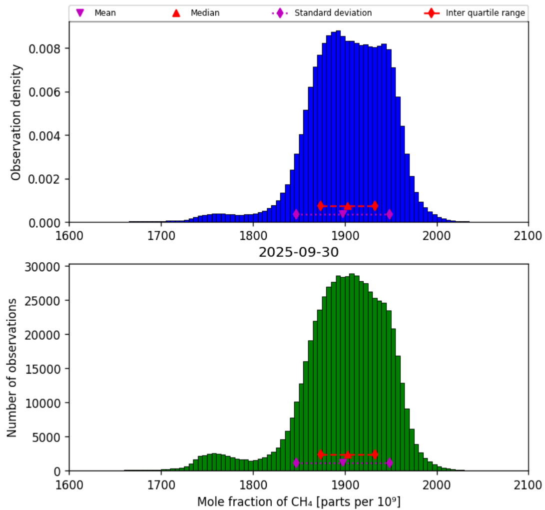
Figure 23: Histogram of “Mole fraction of CH 4 ” for 2025-09-29 to 2025-10-01
