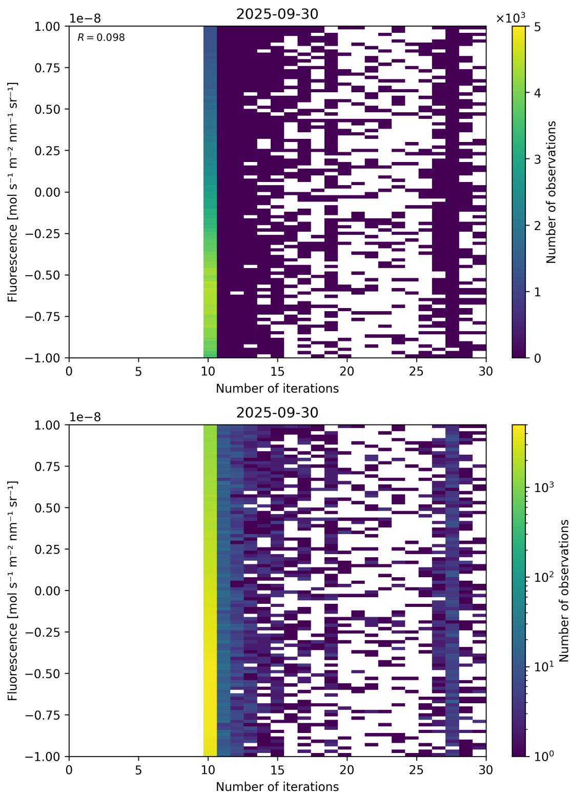
Figure 87: Scatter density plot of “Number of iterations” against “Fluorescence” for 2025-09-29 to 2025-10-01.
