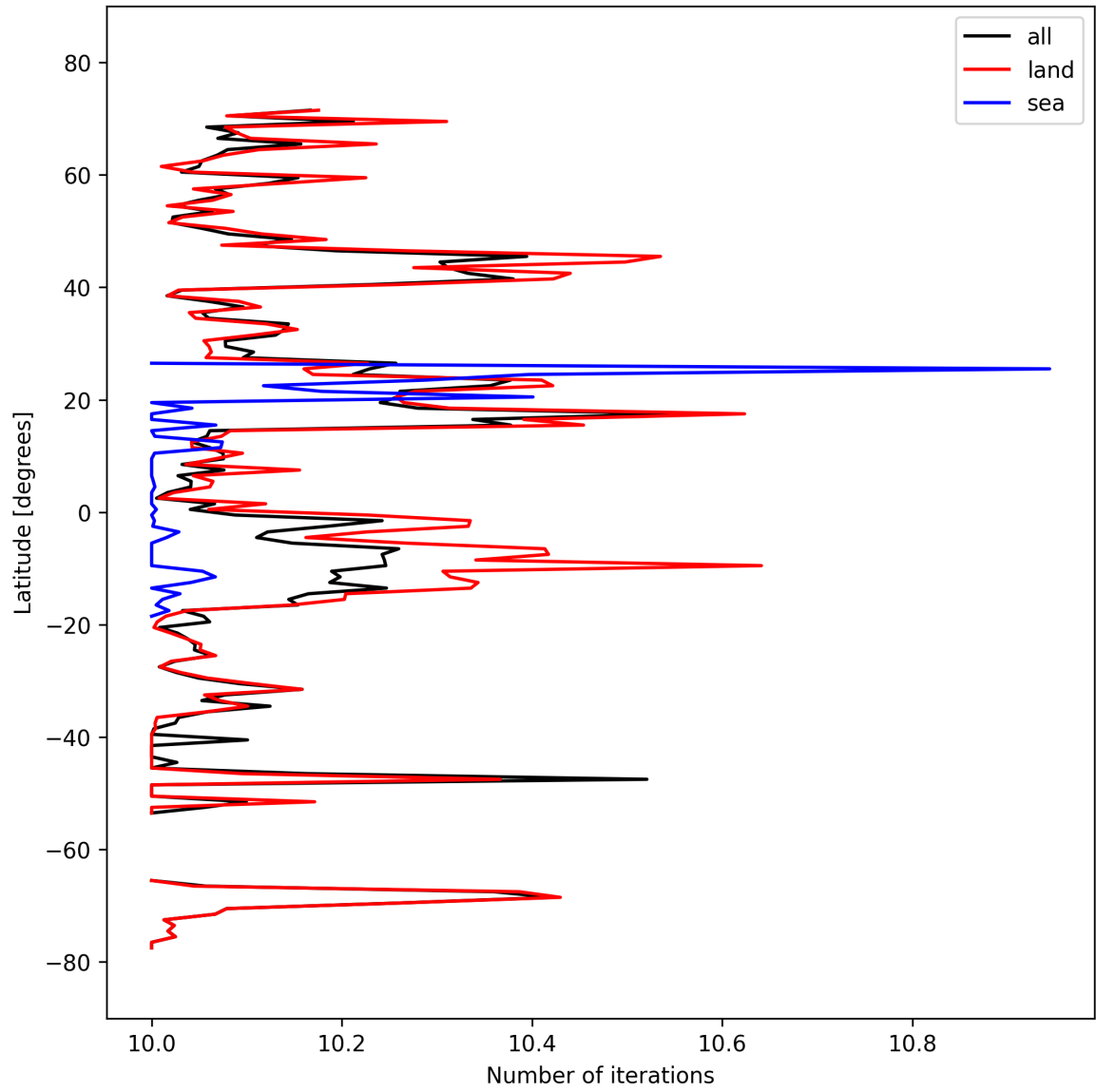
Figure 20: Zonal average of “Number of iterations” for 2025-09-29 to 2025-10-01.
