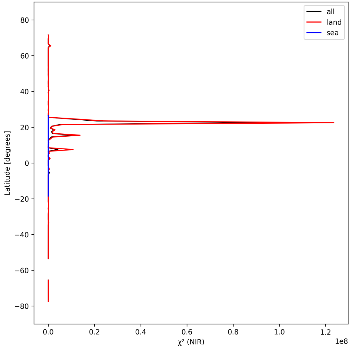
Figure 18: Zonal average of “ \chi^2 (NIR)” for 2025-09-29 to 2025-10-01.
