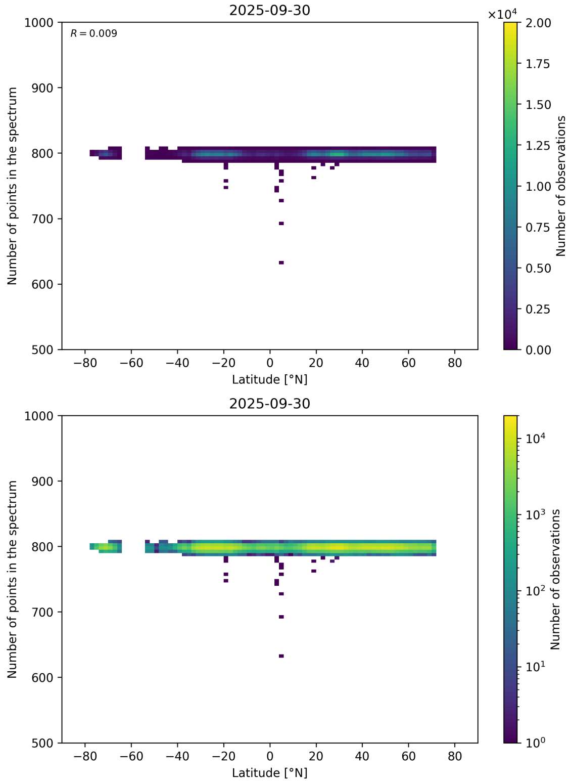
Figure 61: Scatter density plot of “Latitude” against “Number of points in the spectrum” for 2025-09-29 to 2025-10-01.
