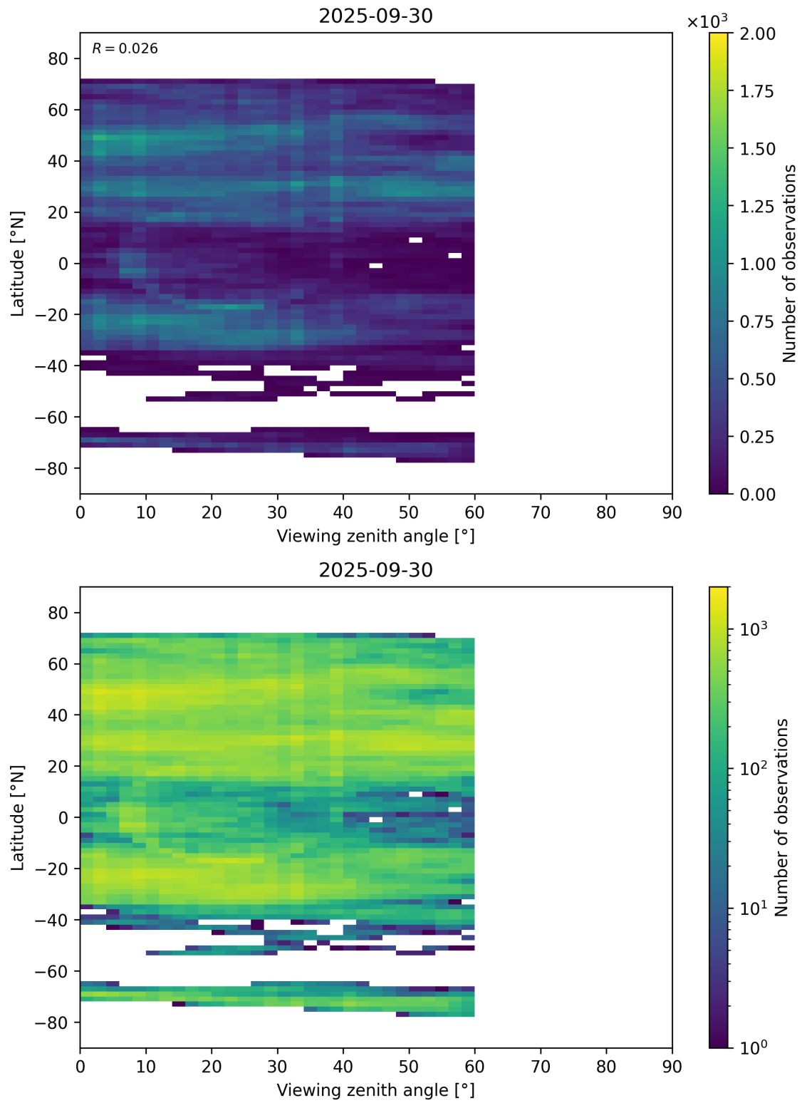
Figure 109: Scatter density plot of “Viewing zenith angle” against “Latitude” for 2025-09-29 to 2025-10-01.
