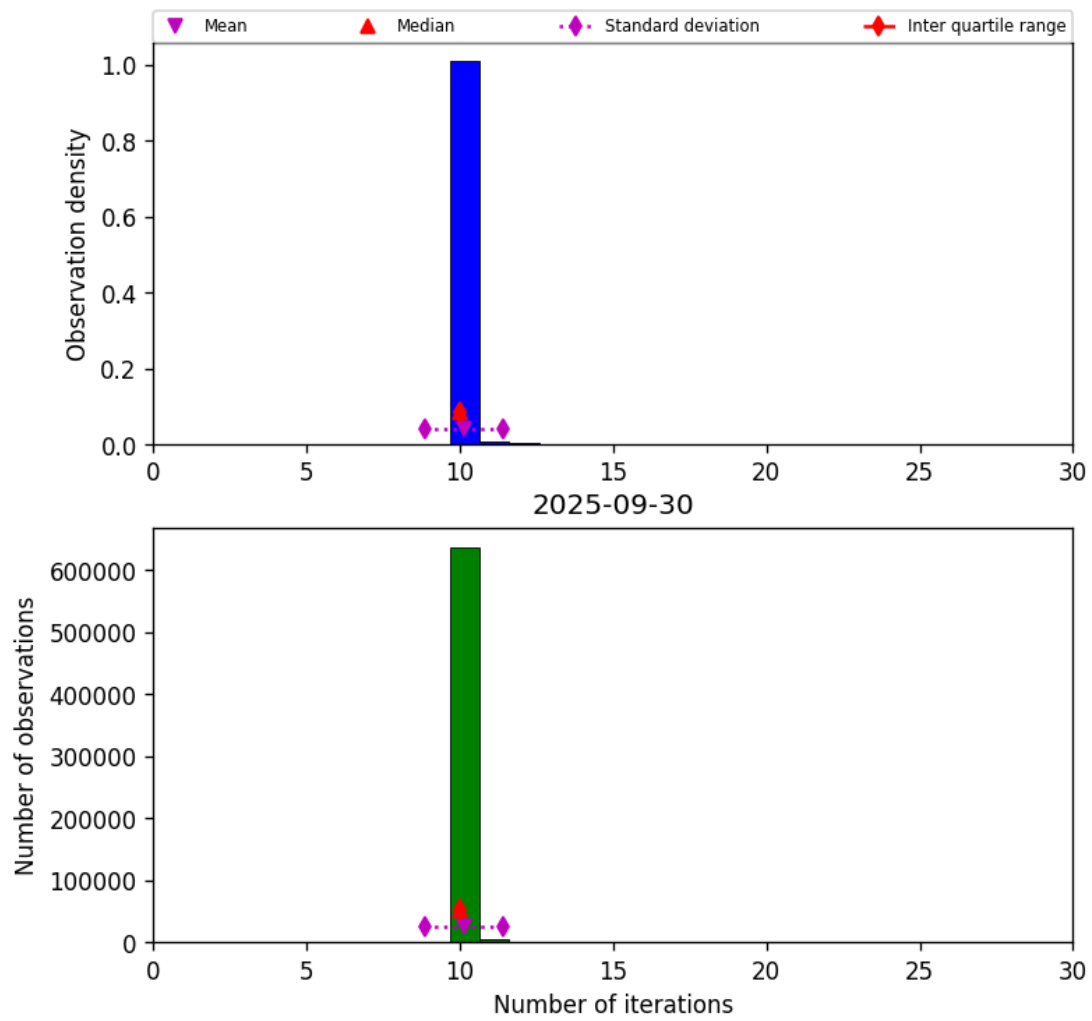
Figure 31: Histogram of “Number of iterations” for 2025-09-29 to 2025-10-01
