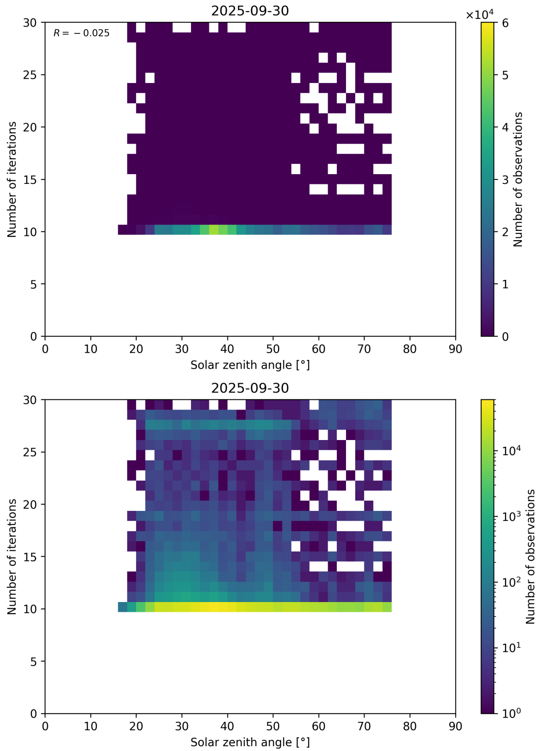
Figure 102: Scatter density plot of “Solar zenith angle” against “Number of iterations” for 2025-09-29 to 2025-10-01.
