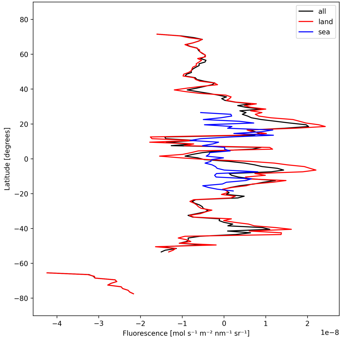
Figure 21: Zonal average of “Fluorescence” for 2025-09-29 to 2025-10-01.
