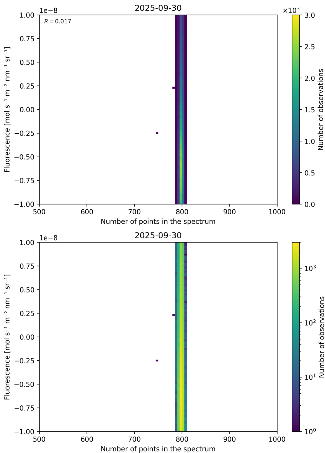
Figure 91: Scatter density plot of “Number of points in the spectrum” against “Fluorescence” for 2025-09-29 to 2025-10-01.
