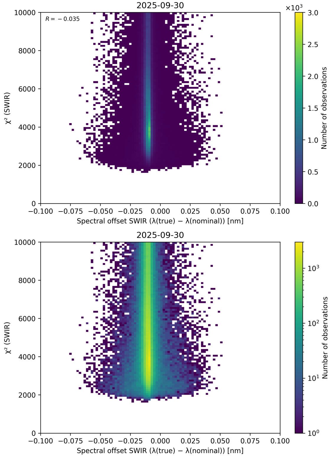
Figure 118: Scatter density plot of “Spectral offset SWIR ( \lambda_{\text{true}} - \lambda_{\text{nominal}} )” against “ \chi^2 (SWIR)” for 2025-09-29 to 2025-10-01.
