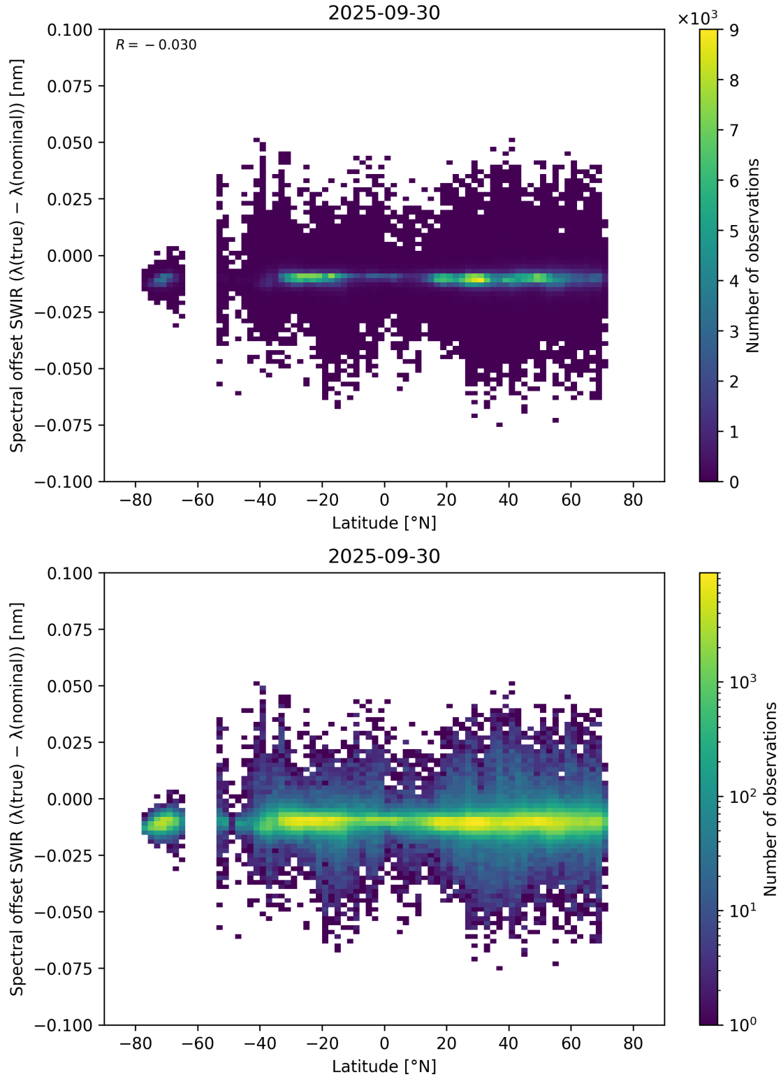
Figure 62: Scatter density plot of “Latitude” against “Spectral offset SWIR ( \lambda_{\text{true}} - \lambda_{\text{nominal}} )” for 2025-09-29 to 2025-10-01.
