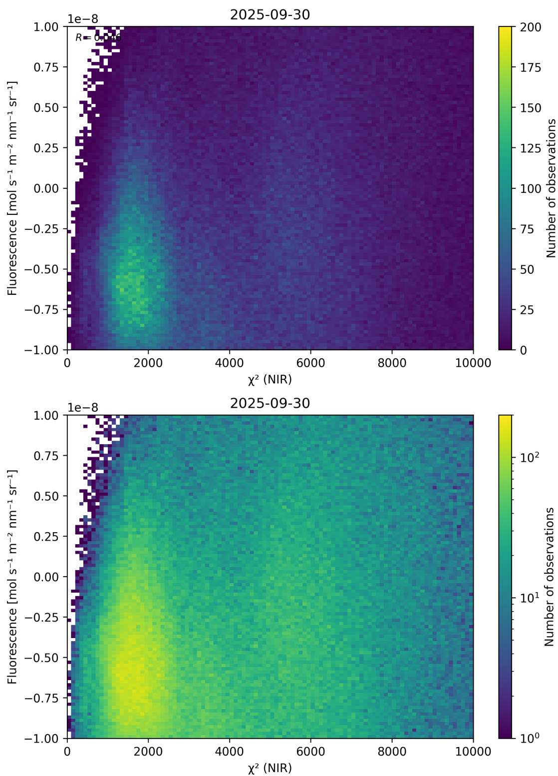
Figure 45: Scatter density plot of “ \chi^2 (NIR)” against “Fluorescence” for 2025-09-29 to 2025-10-01.
