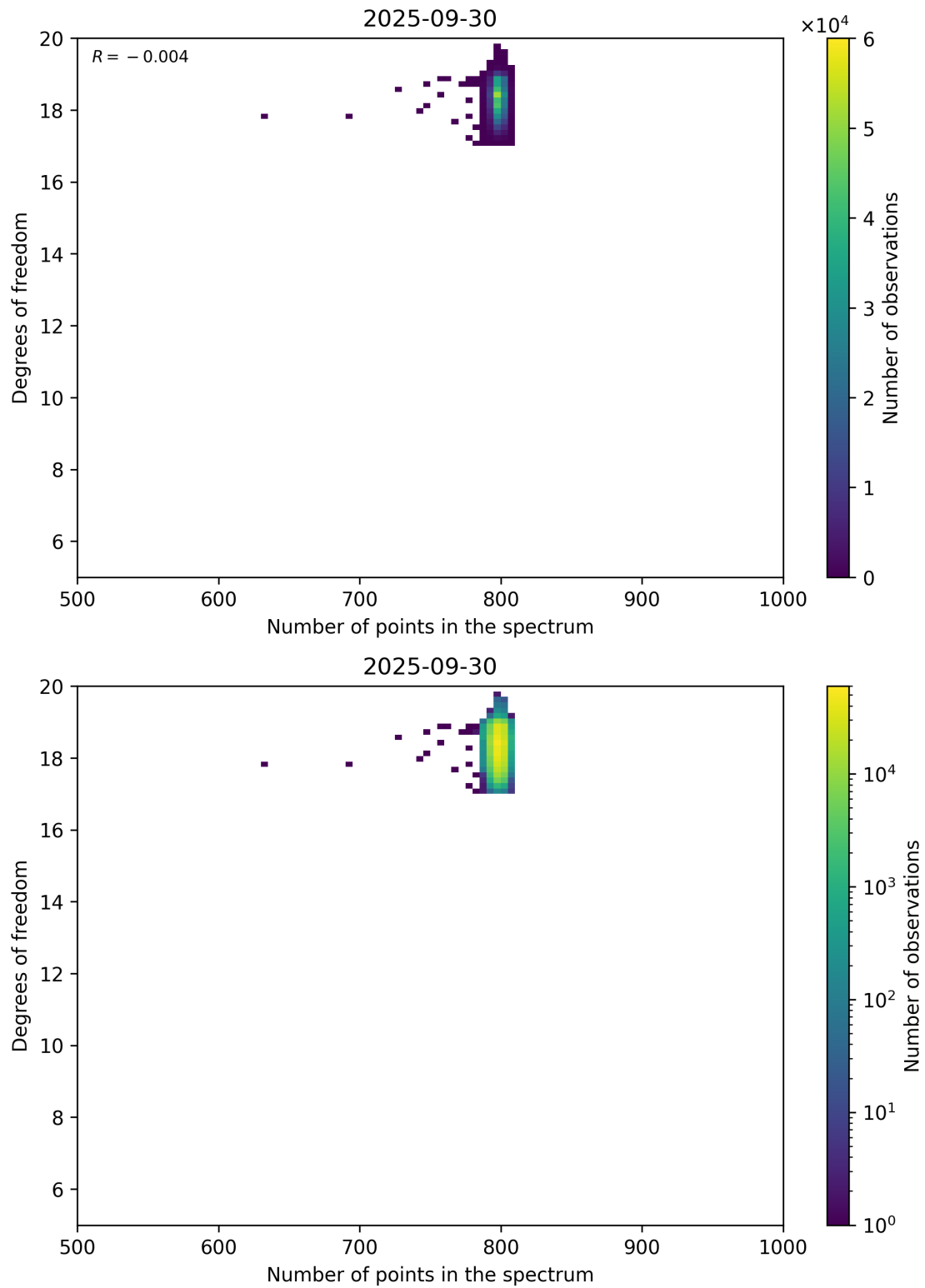
Figure 90: Scatter density plot of “Number of points in the spectrum” against “Degrees of freedom” for 2025-09-29 to 2025-10-01.
