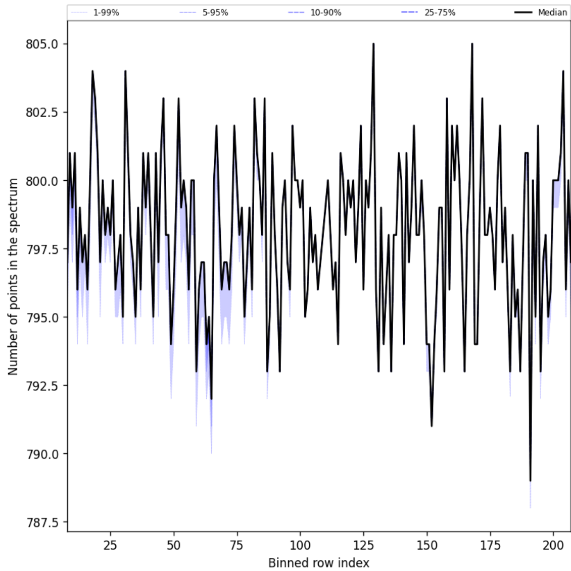
Figure 37: Along track statistics of “Number of points in the spectrum” for 2025-09-29 to 2025-10-01
