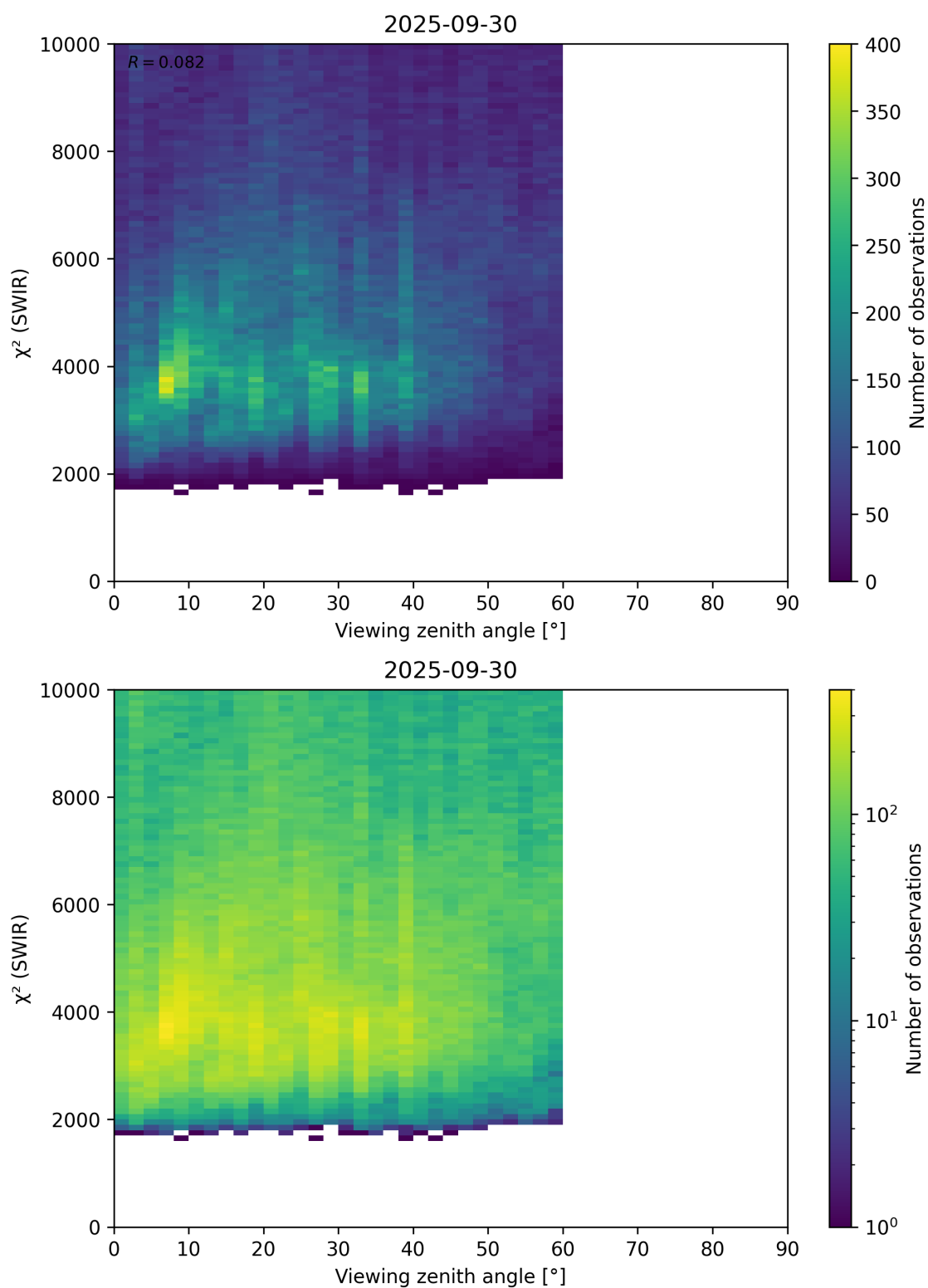
Figure 106: Scatter density plot of “Viewing zenith angle” against “ \chi^2 (SWIR)” for 2025-09-29 to 2025-10-01.
