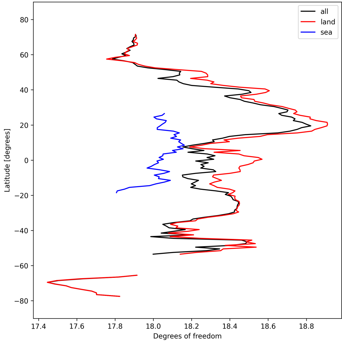
Figure 19: Zonal average of “Degrees of freedom” for 2025-09-29 to 2025-10-01.
