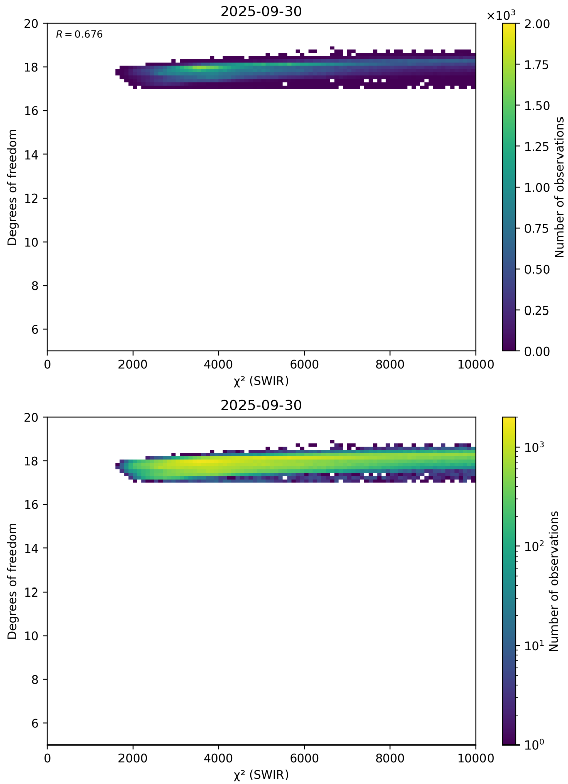
Figure 48: Scatter density plot of " \chi^2 (SWIR)" against "Degrees of freedom" for 2025-09-29 to 2025-10-01.
