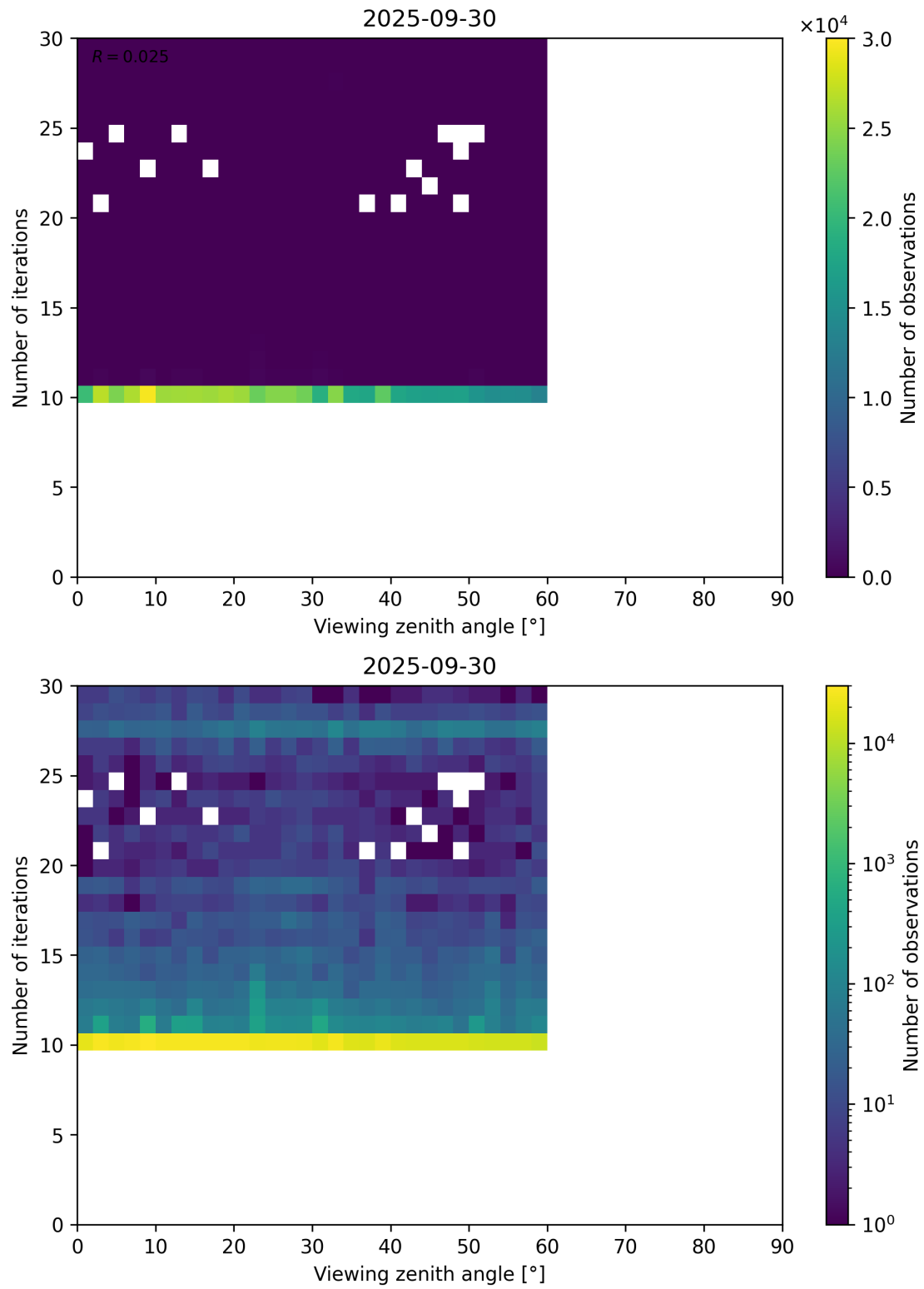
Figure 113: Scatter density plot of “Viewing zenith angle” against “Number of iterations” for 2025-09-29 to 2025-10-01.
