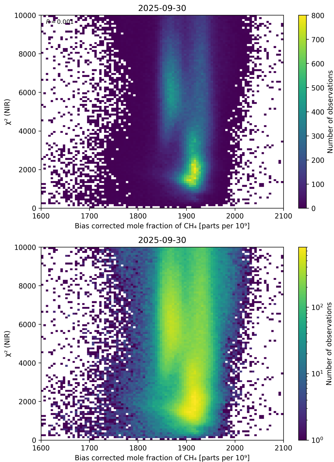
Figure 63: Scatter density plot of “Bias corrected mole fraction of CH 4 ” against “ \chi^2 (NIR)” for 2025-09-29 to 2025-10-01.
