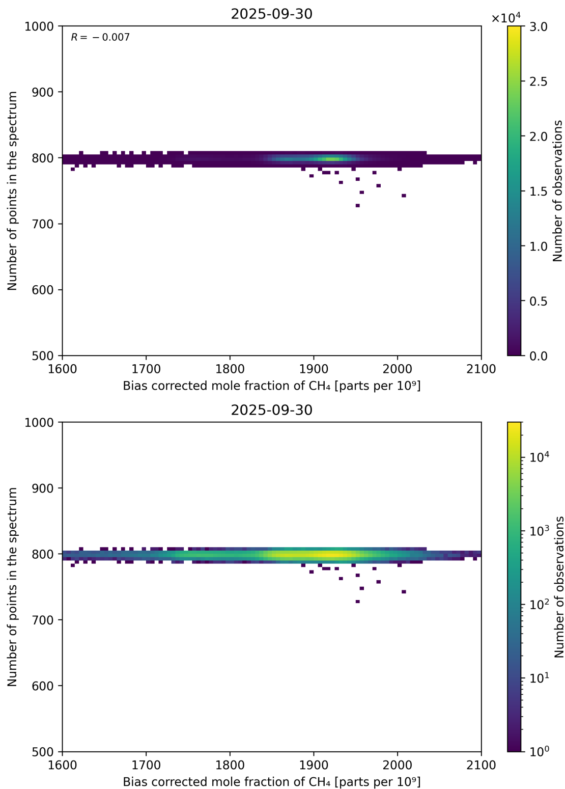
Figure 68: Scatter density plot of “Bias corrected mole fraction of CH 4 ” against “Number of points in the spectrum” for 2025-09-29 to 2025-10-01.
