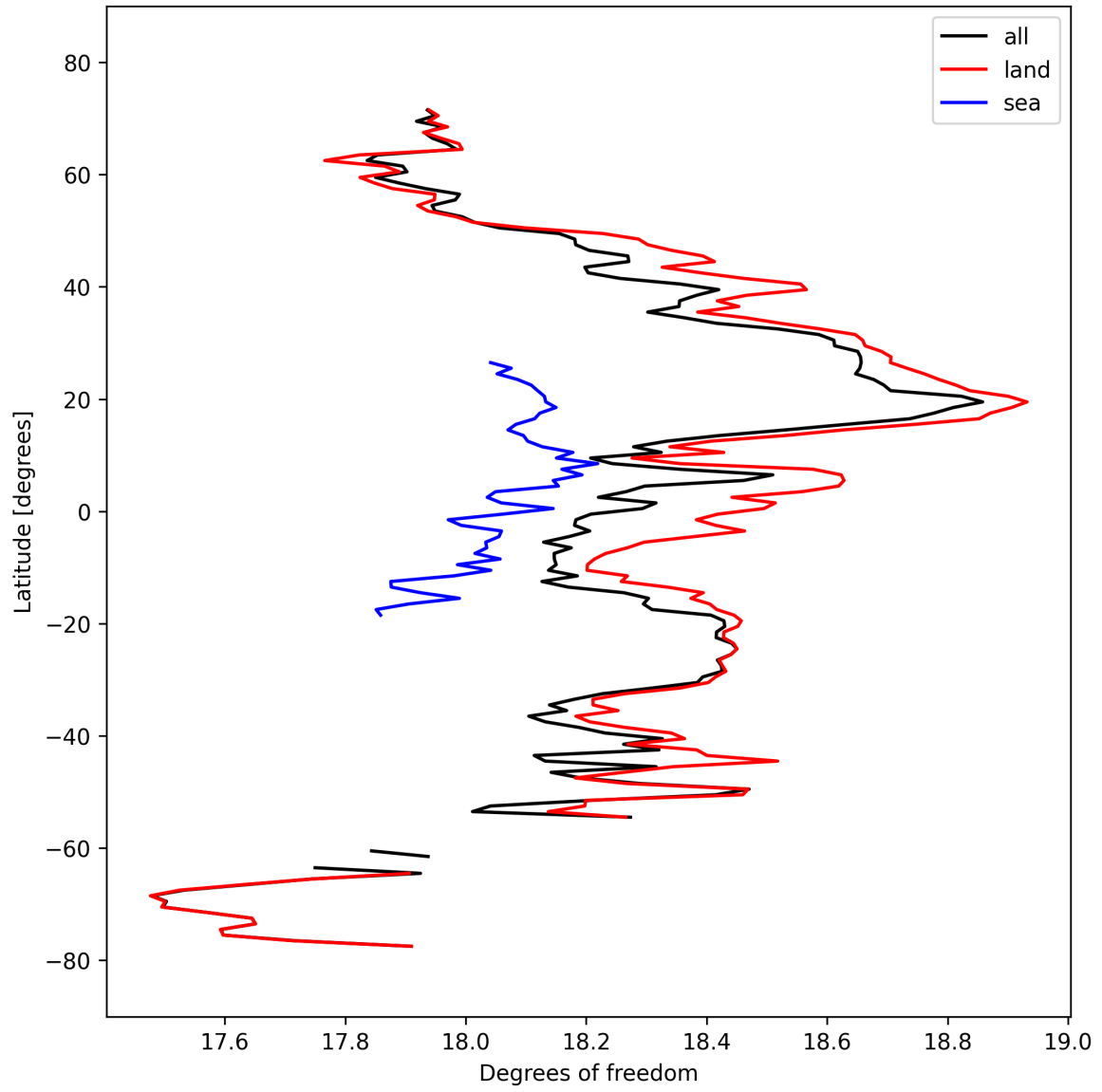
Figure 19: Zonal average of “Degrees of freedom” for 2025-10-01 to 2025-10-02.
