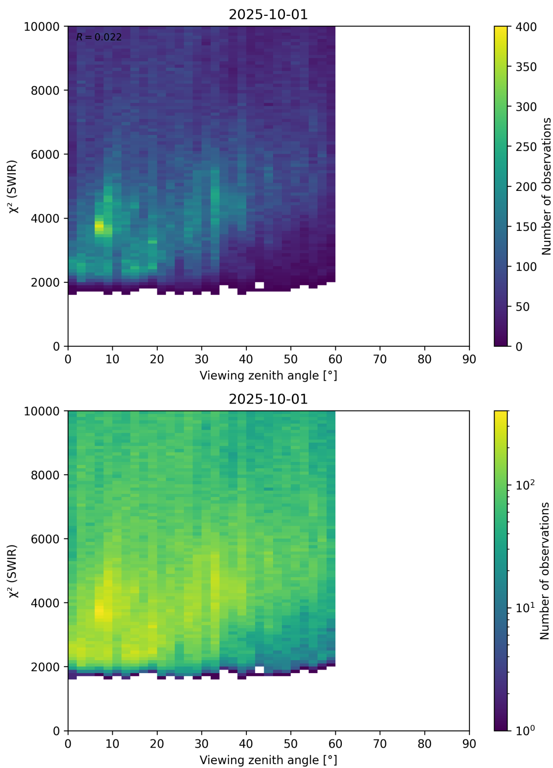
Figure 106: Scatter density plot of “Viewing zenith angle” against “ \chi^2 (SWIR)” for 2025-10-01 to 2025-10-02.
