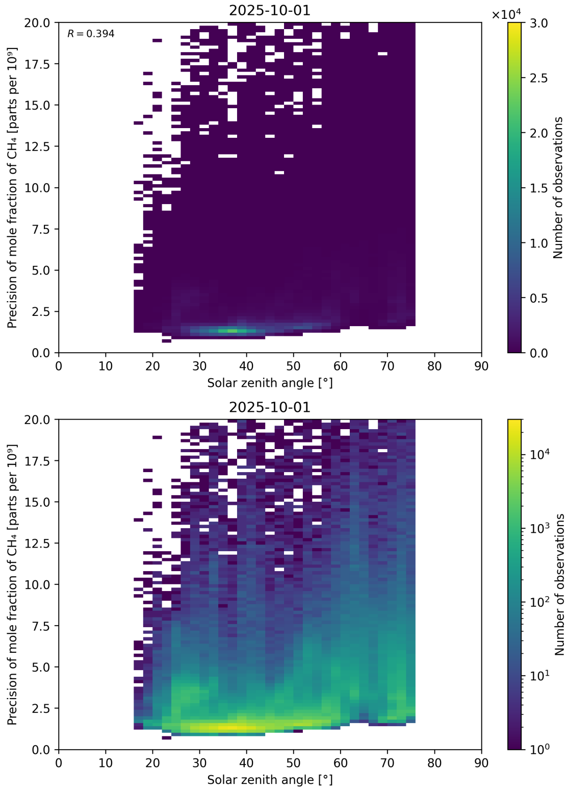
Figure 101: Scatter density plot of “Solar zenith angle” against “Precision of mole fraction of CH 4 ” for 2025-10-01 to 2025-10-02.
