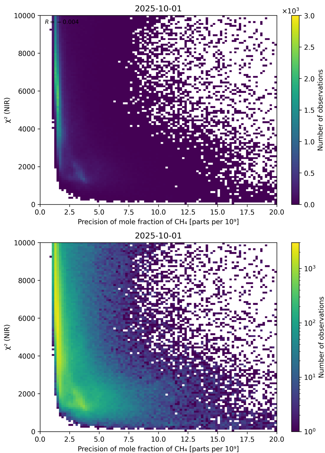
Figure 78: Scatter density plot of “Precision of mole fraction of \text{CH}_4 ” against “ \chi^2 (NIR)” for 2025-10-01 to 2025-10-02.
