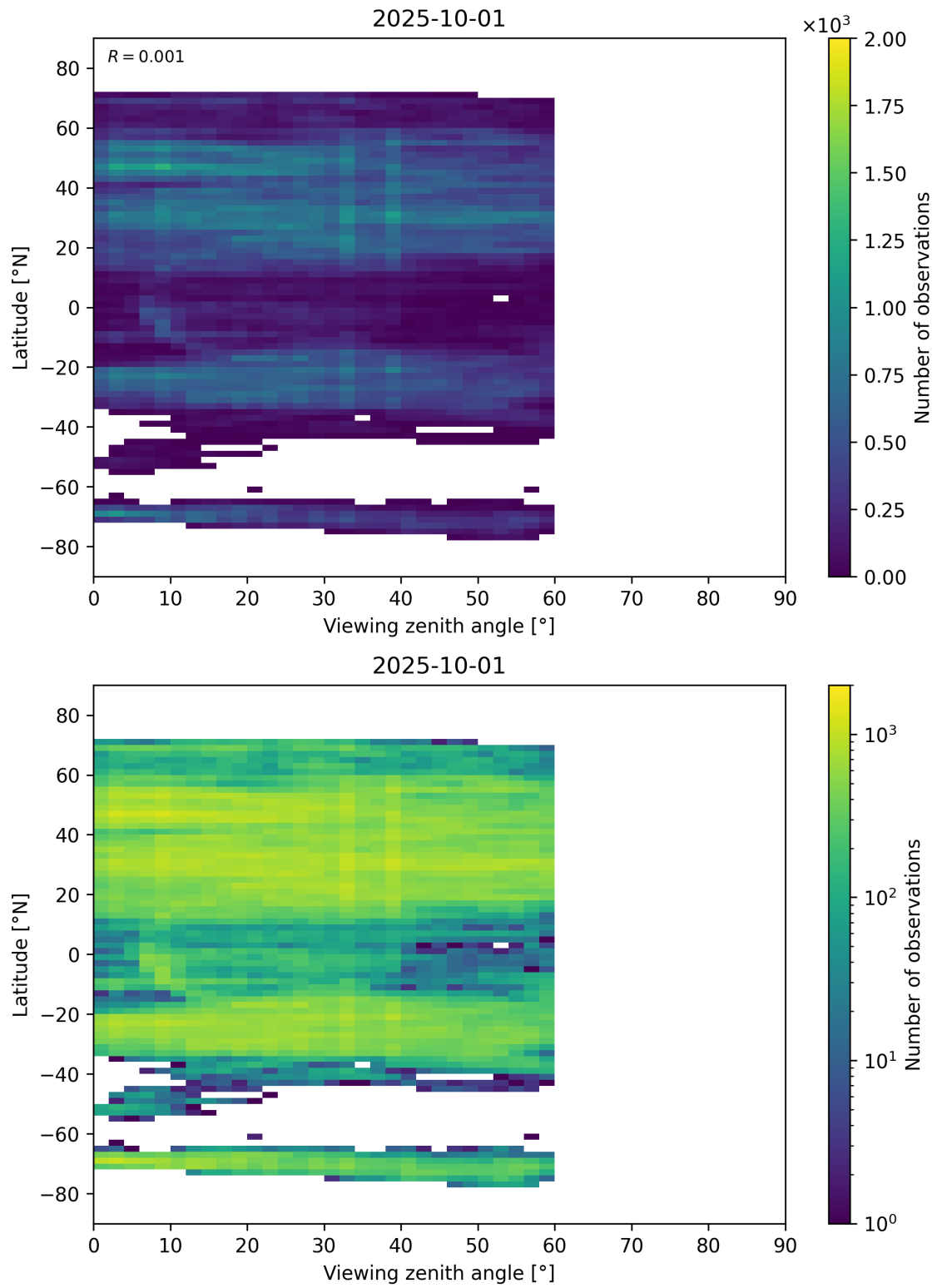
Figure 109: Scatter density plot of “Viewing zenith angle” against “Latitude” for 2025-10-01 to 2025-10-02.
