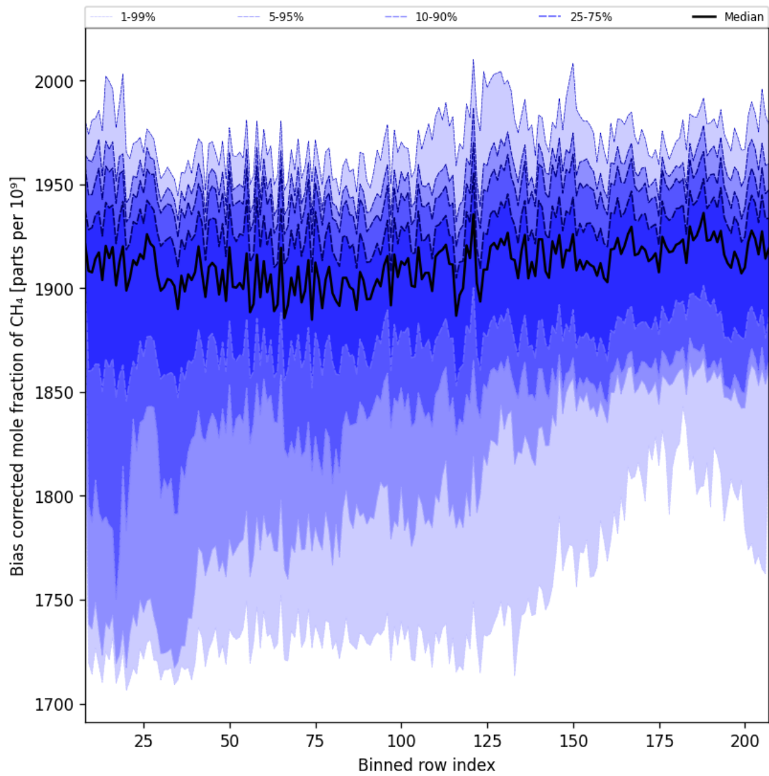
Figure 36: Along track statistics of “Bias corrected mole fraction of CH 4 ” for 2025-10-01 to 2025-10-02
