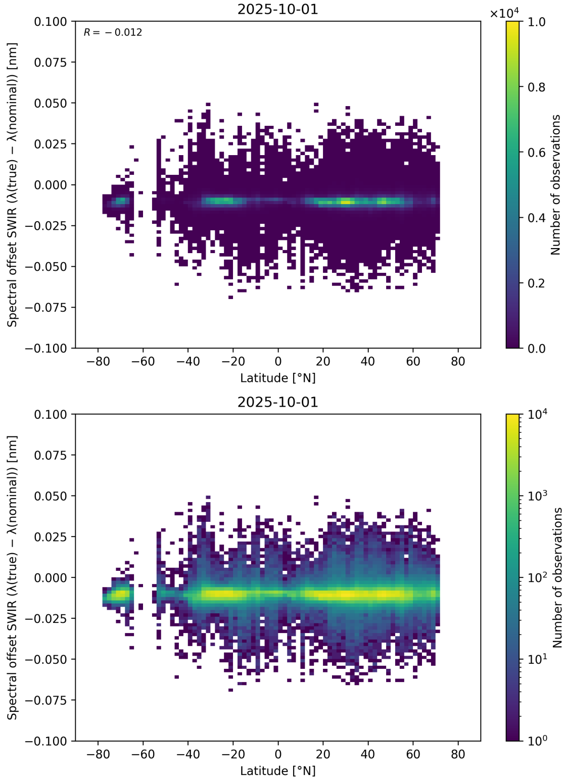
Figure 62: Scatter density plot of “Latitude” against “Spectral offset SWIR ( \lambda_{\text{true}} - \lambda_{\text{nominal}} )” for 2025-10-01 to 2025-10-02.
