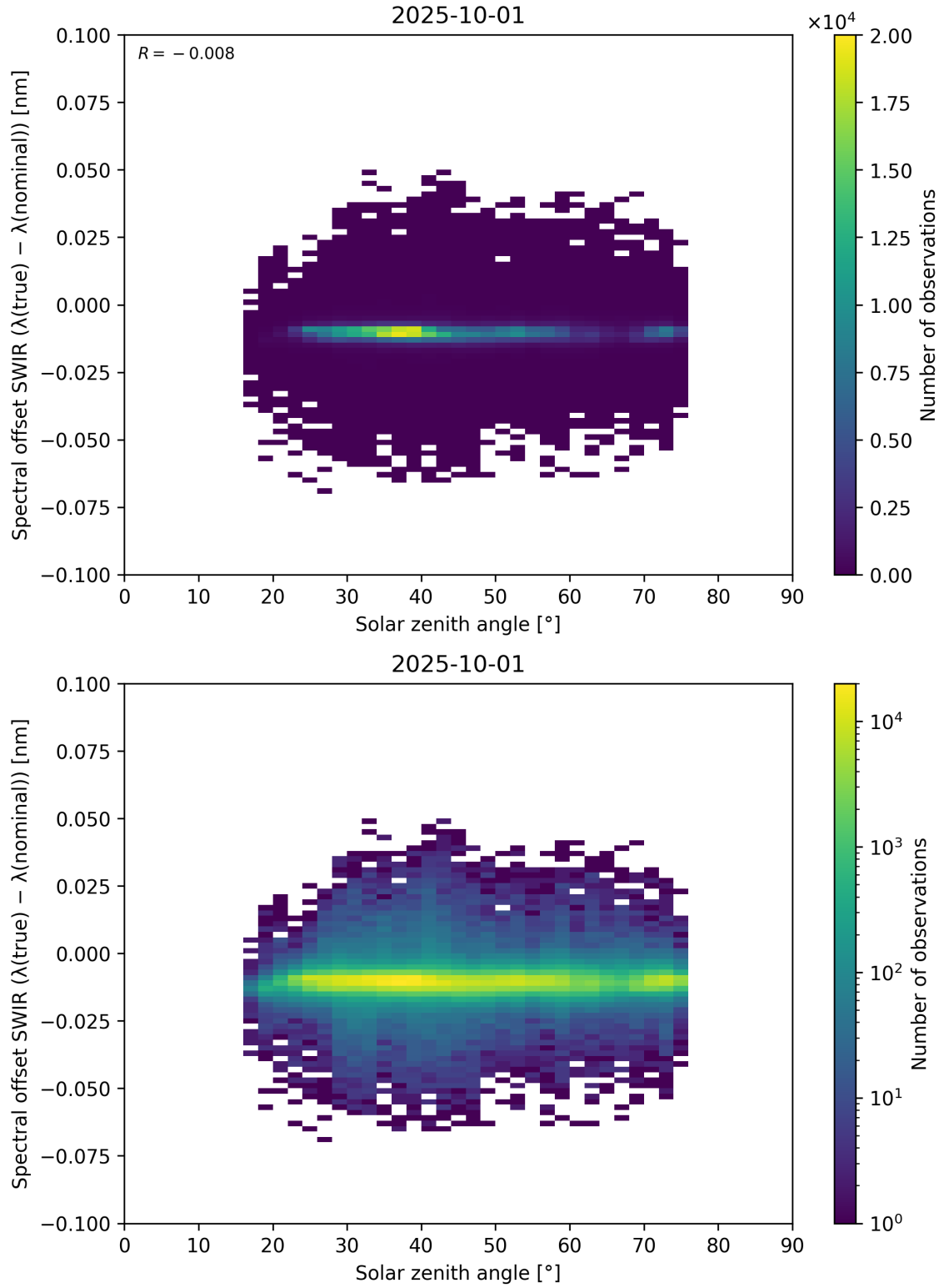
Figure 104: Scatter density plot of “Solar zenith angle” against “Spectral offset SWIR ( \lambda_{\text{true}} - \lambda_{\text{nominal}} )” for 2025-10-01 to 2025-10-02.
