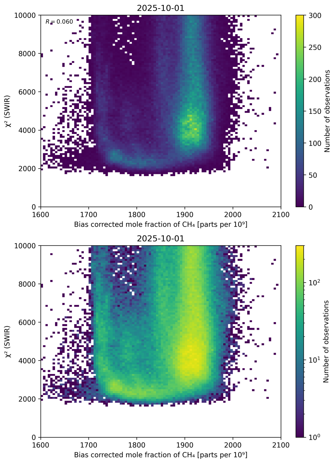
Figure 64: Scatter density plot of “Bias corrected mole fraction of \text{CH}_4 ” against “ \chi^2 (SWIR)” for 2025-10-01 to 2025-10-02.
