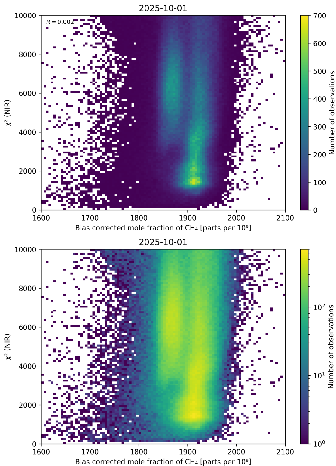
Figure 63: Scatter density plot of “Bias corrected mole fraction of \text{CH}_4 ” against “ \chi^2 (NIR)” for 2025-10-01 to 2025-10-02.
