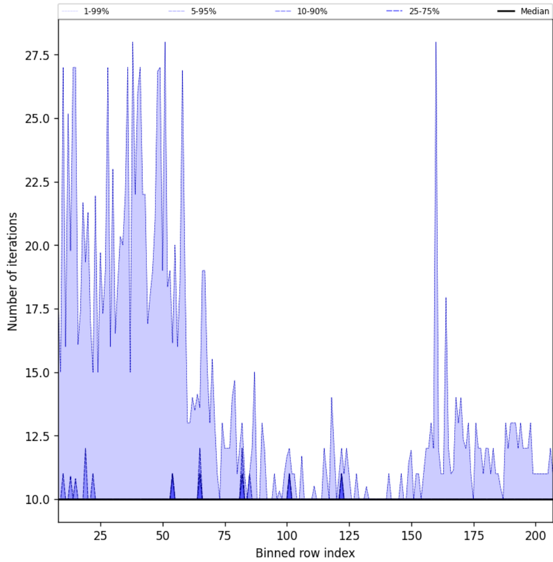
Figure 42: Along track statistics of “Number of iterations” for 2025-10-01 to 2025-10-02
