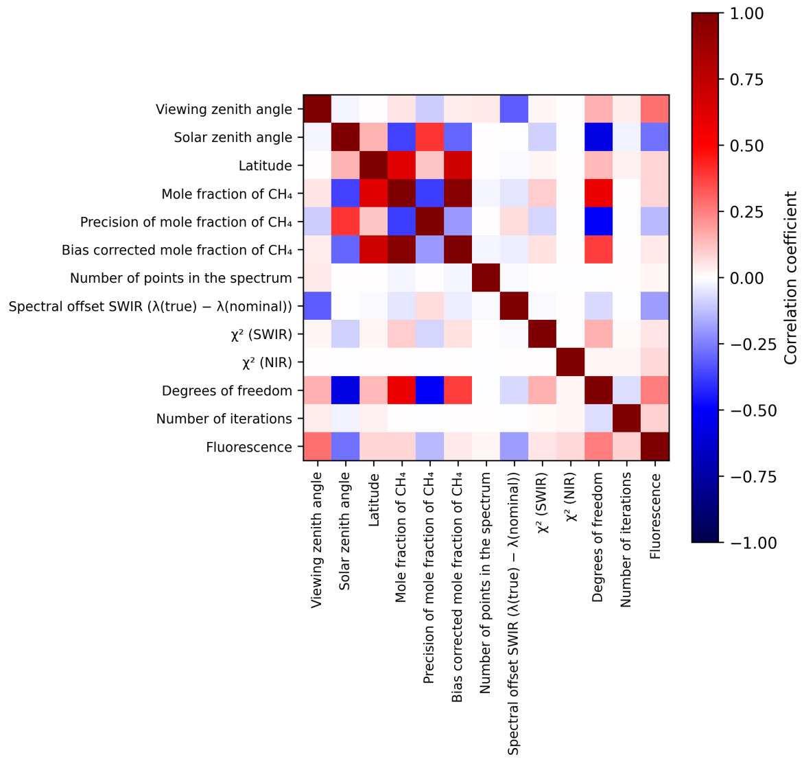
Figure 2: Map of correlation matrix for 2025-10-01 to 2025-10-02.
