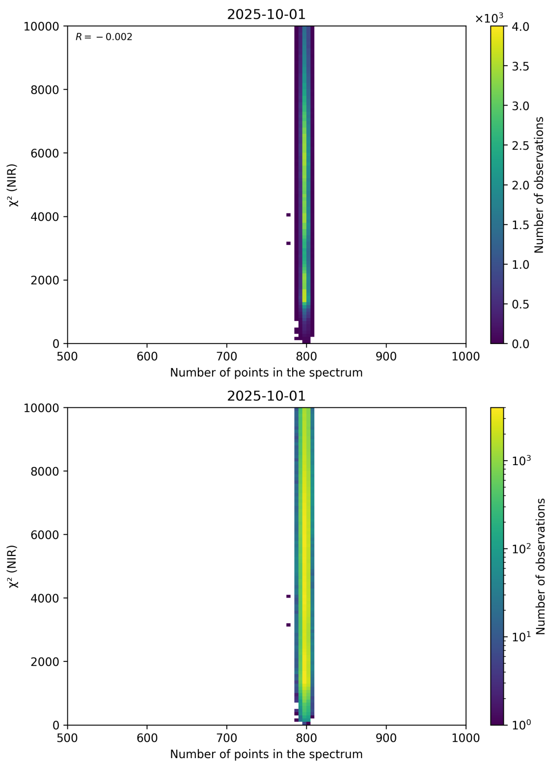
Figure 88: Scatter density plot of “Number of points in the spectrum” against “ \chi^2 (NIR)” for 2025-10-01 to 2025-10-02.
