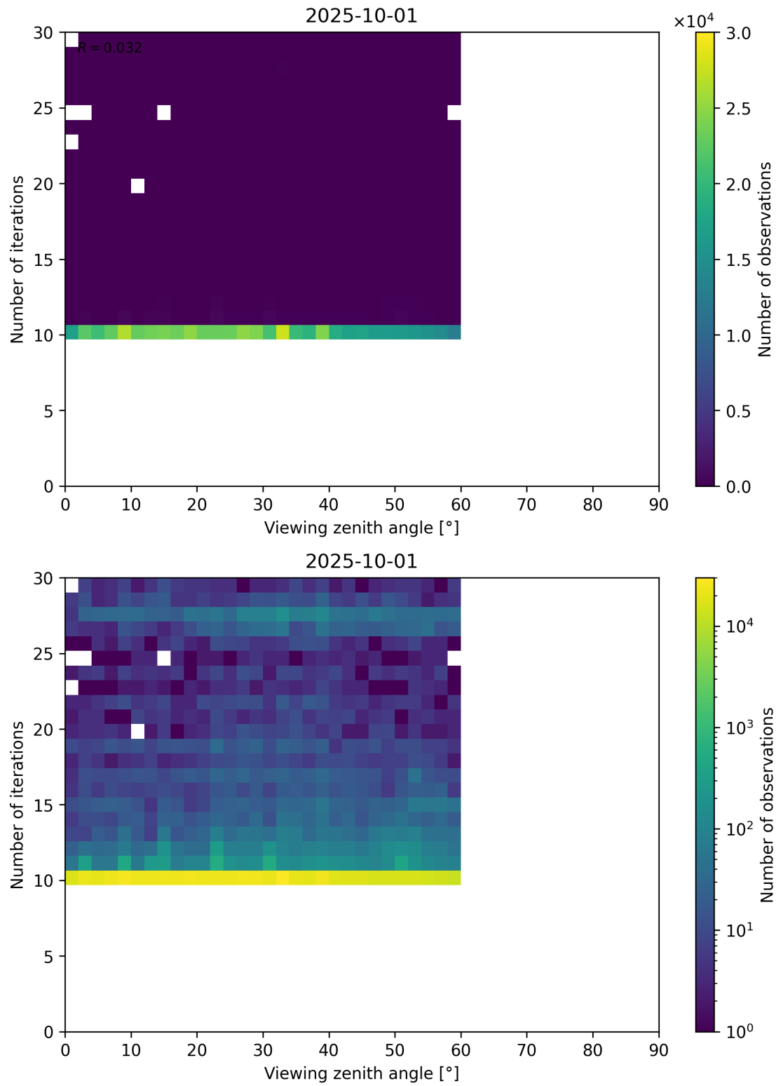
Figure 113: Scatter density plot of “Viewing zenith angle” against “Number of iterations” for 2025-10-01 to 2025-10-02.
