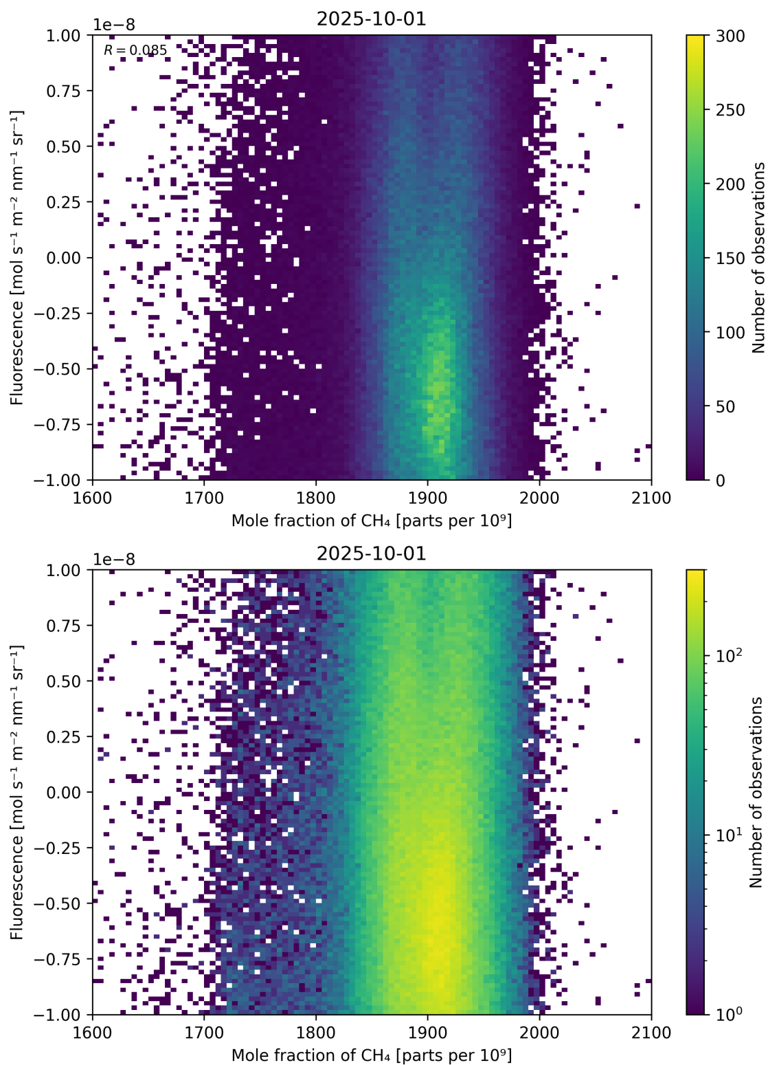
Figure 73: Scatter density plot of “Mole fraction of \text{CH}_4 ” against “Fluorescence” for 2025-10-01 to 2025-10-02.
