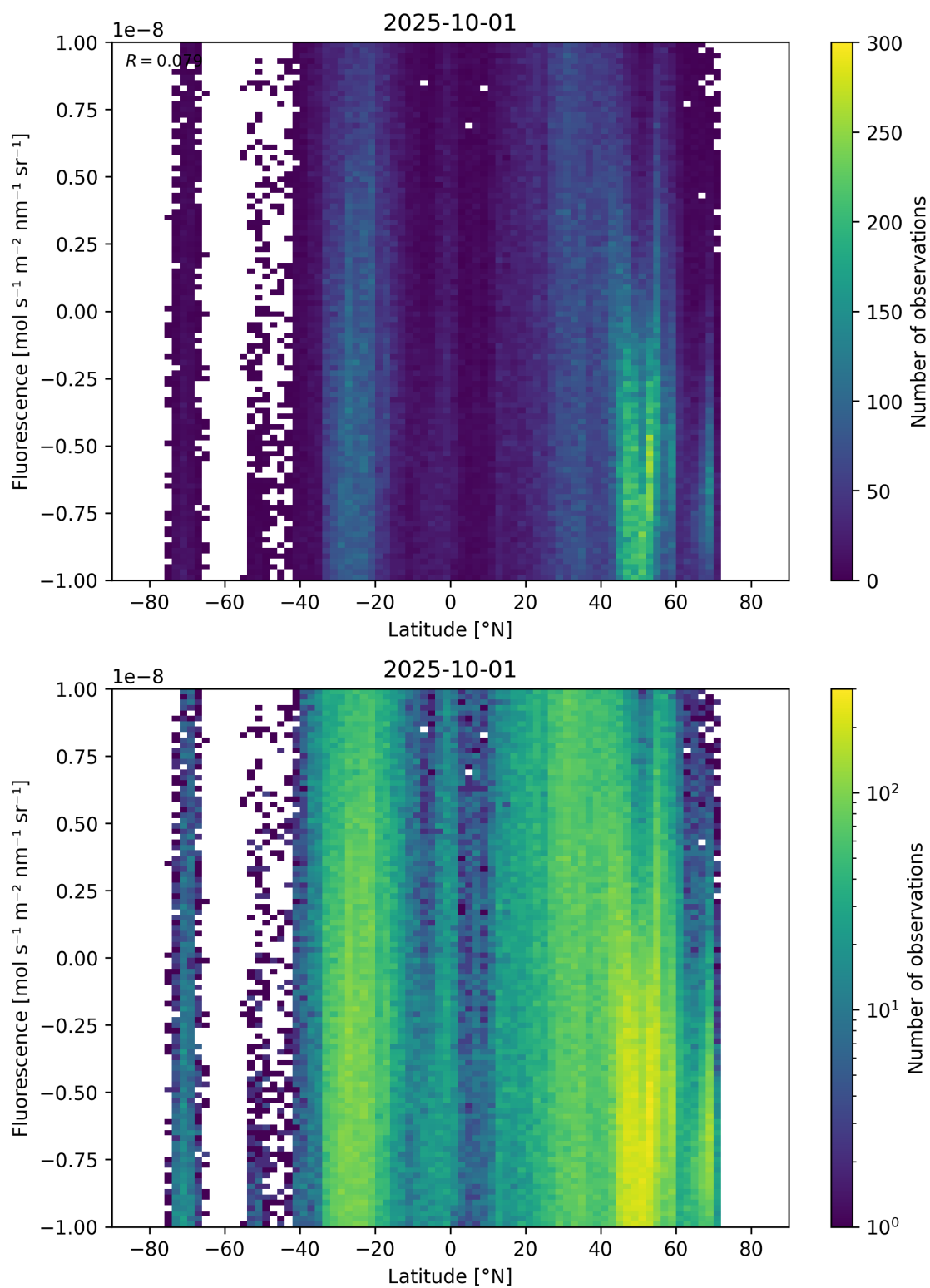
Figure 56: Scatter density plot of “Latitude” against “Fluorescence” for 2025-10-01 to 2025-10-02.
