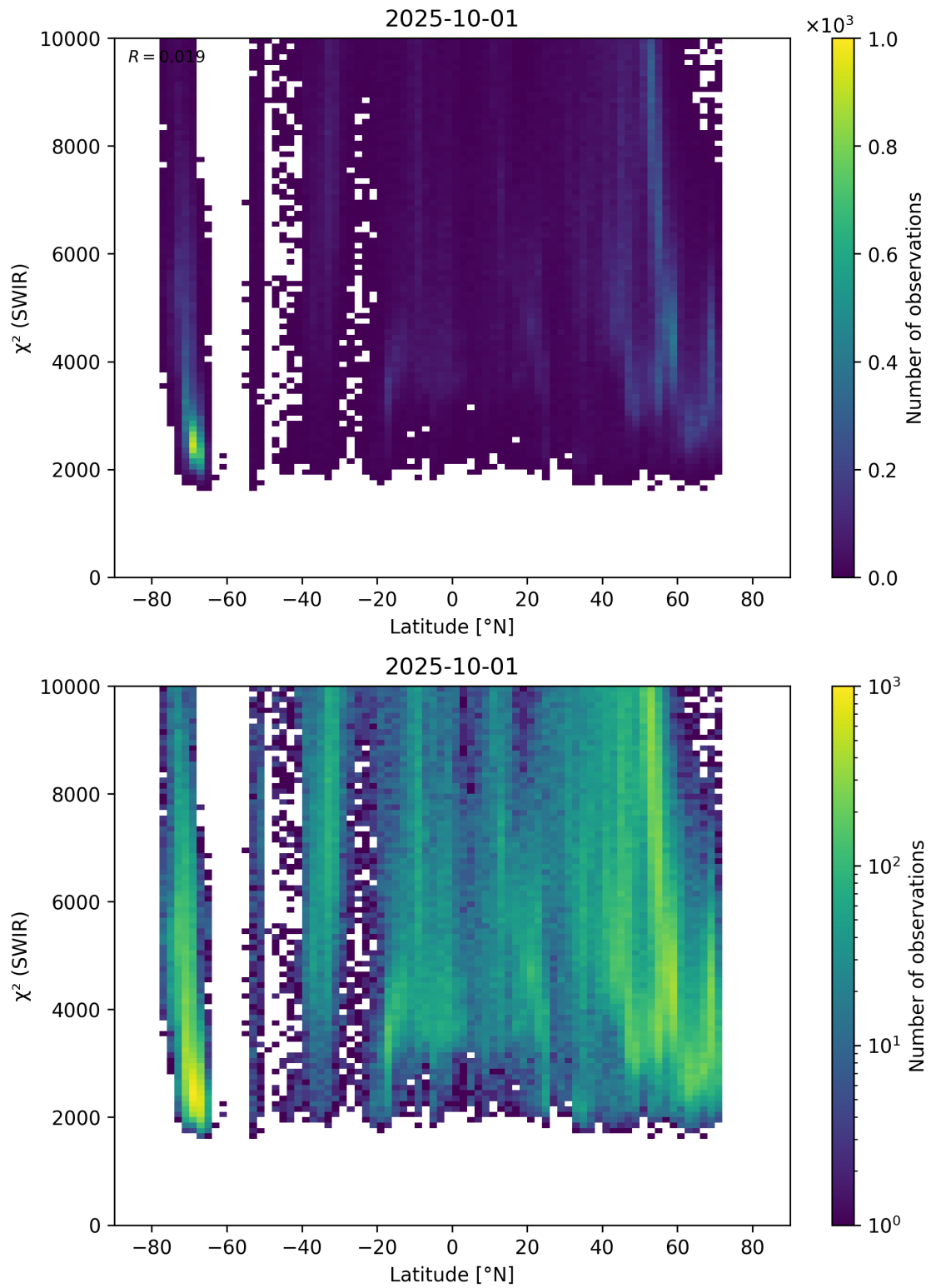
Figure 54: Scatter density plot of “Latitude” against “ \chi^2 (SWIR)” for 2025-10-01 to 2025-10-02.
