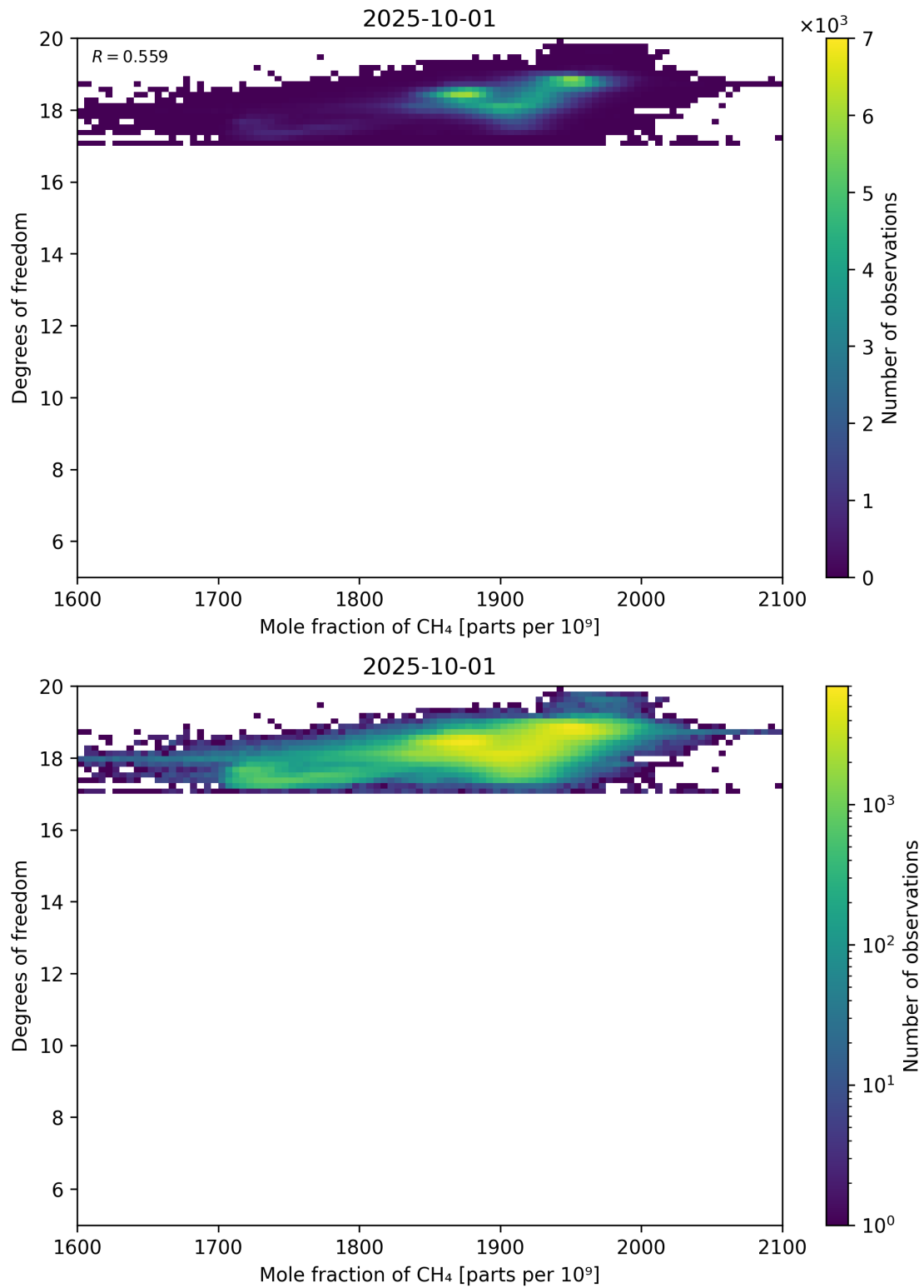
Figure 72: Scatter density plot of “Mole fraction of CH 4 ” against “Degrees of freedom” for 2025-10-01 to 2025-10-02.
