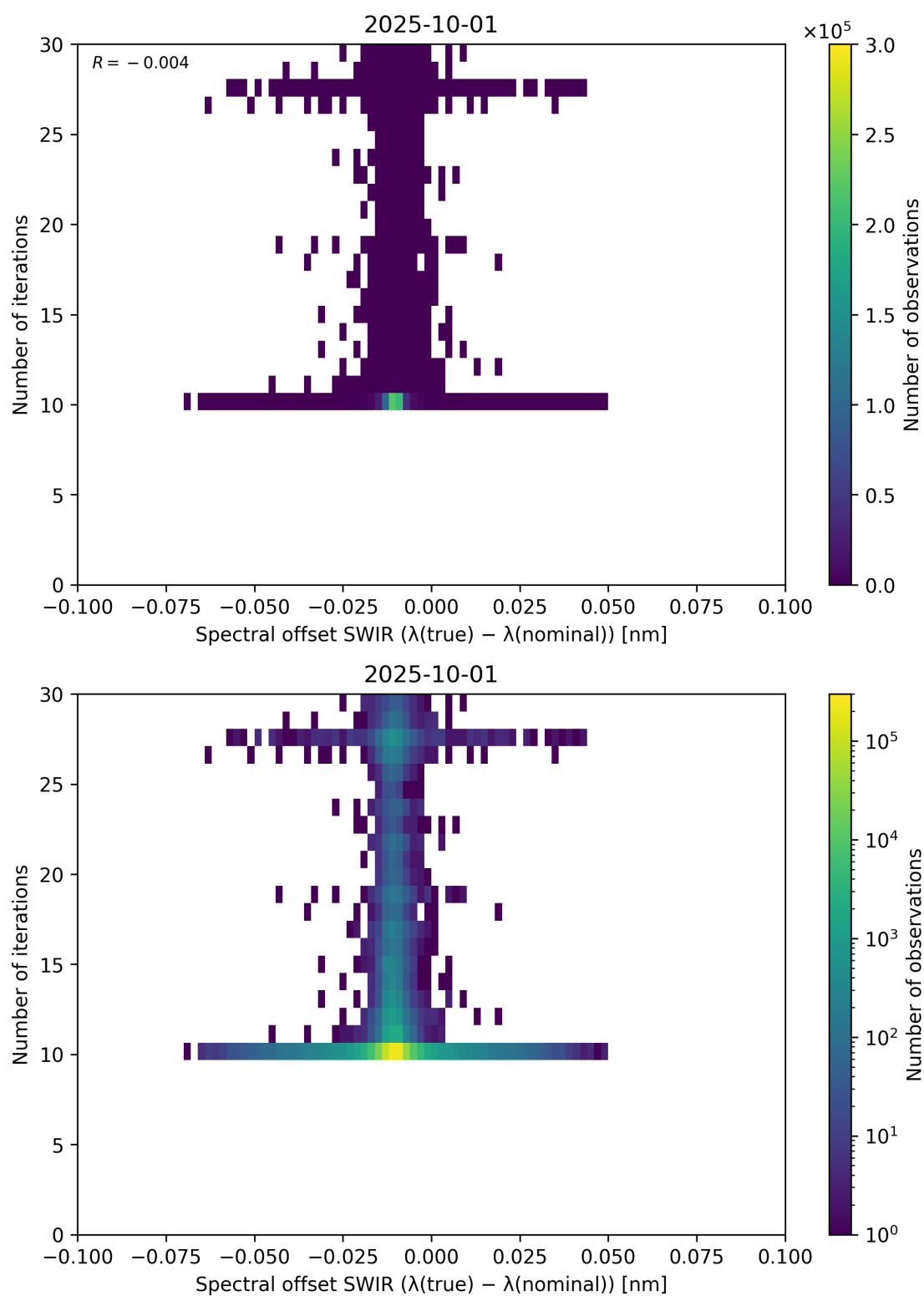
Figure 121: Scatter density plot of “Spectral offset SWIR ( \lambda_{\text{true}} - \lambda_{\text{nominal}} )” against “Number of iterations” for 2025-10-01 to 2025-10-02.
