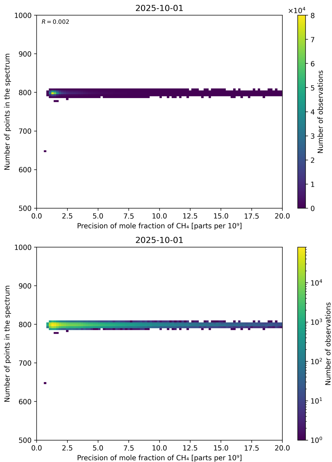
Figure 84: Scatter density plot of “Precision of mole fraction of CH 4 ” against “Number of points in the spectrum” for 2025-10-01 to 2025-10-02.
