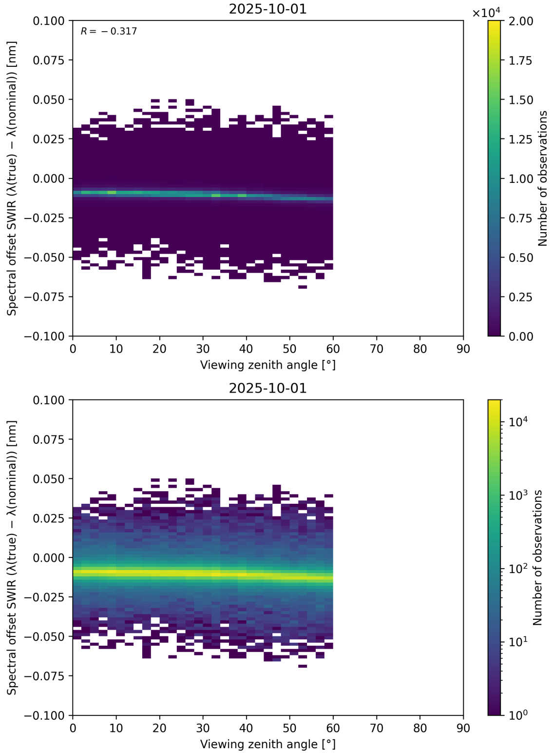
Figure 116: Scatter density plot of “Viewing zenith angle” against “Spectral offset SWIR ( \lambda_{\text{true}} - \lambda_{\text{nominal}} )” for 2025-10-01 to 2025-10-02.
