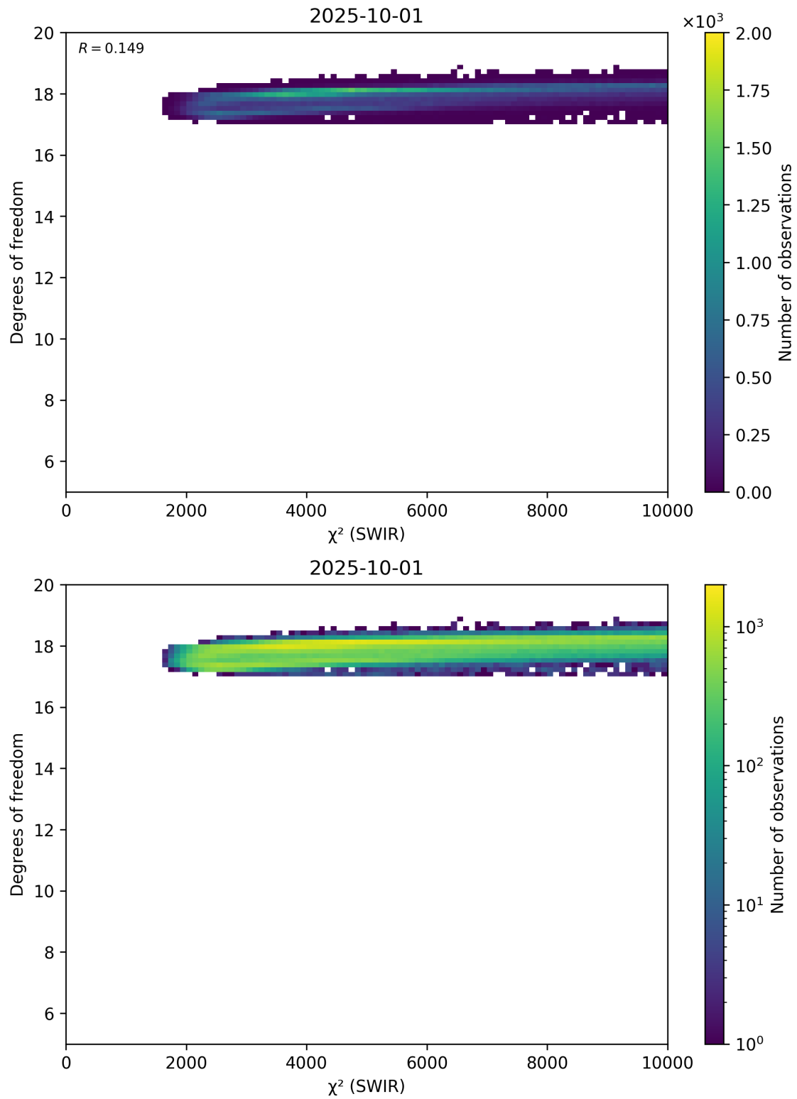
Figure 48: Scatter density plot of “ \chi^2 (SWIR)” against “Degrees of freedom” for 2025-10-01 to 2025-10-02.
