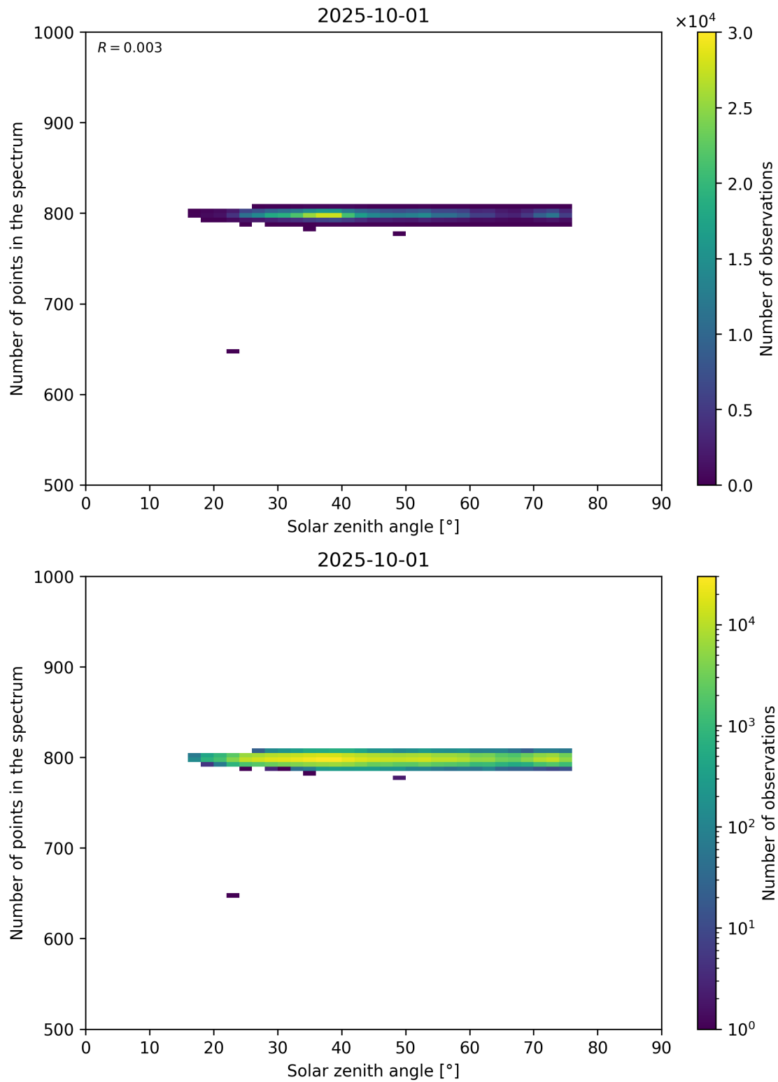
Figure 103: Scatter density plot of “Solar zenith angle” against “Number of points in the spectrum” for 2025-10-01 to 2025-10-02.
