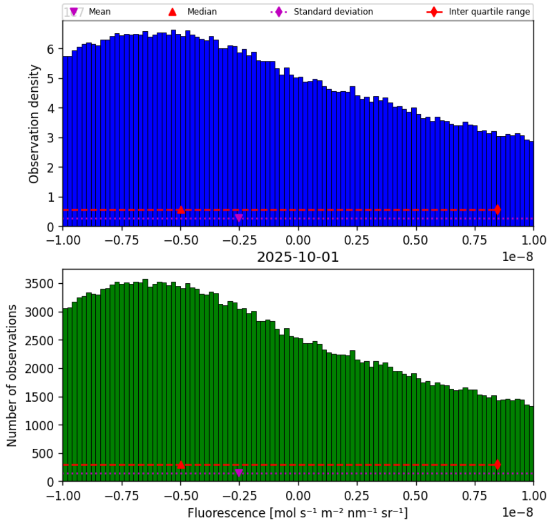
Figure 32: Histogram of “Fluorescence” for 2025-10-01 to 2025-10-02
