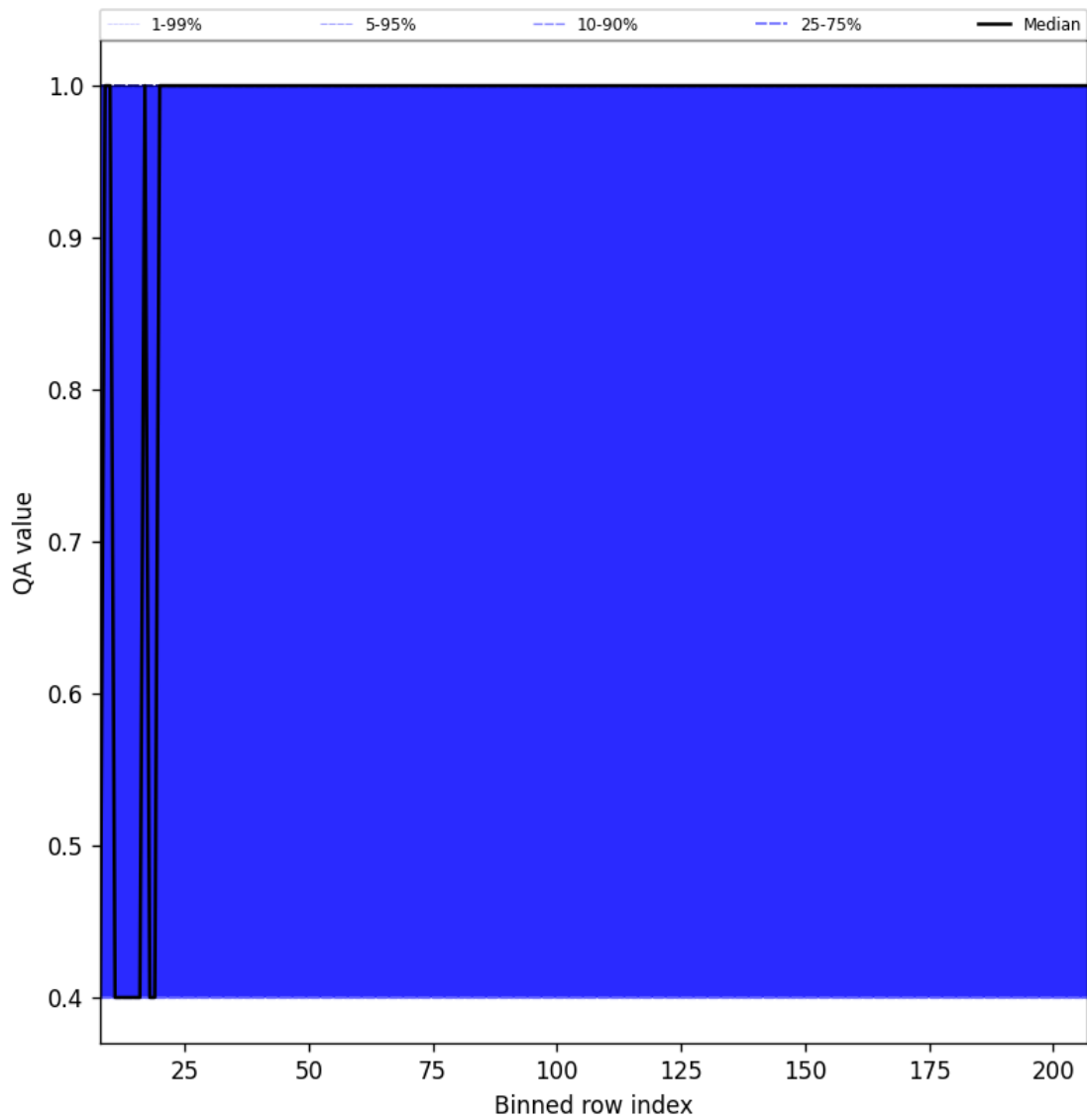
Figure 33: Along track statistics of “QA value” for 2025-10-01 to 2025-10-02
