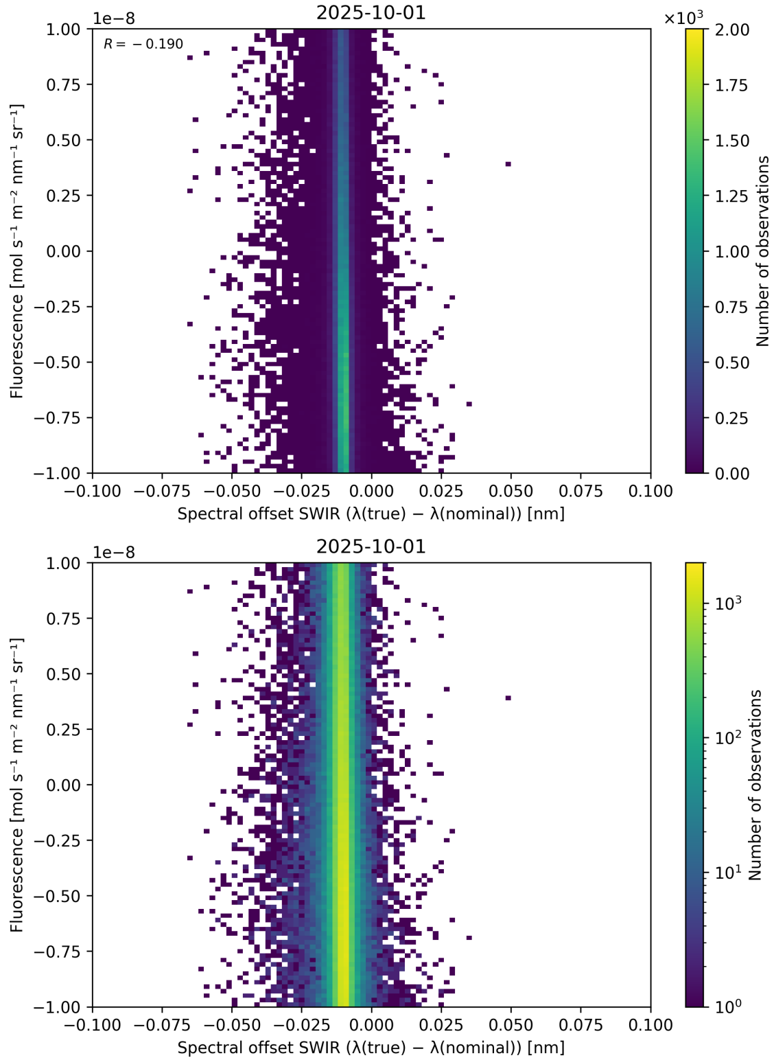
Figure 120: Scatter density plot of “Spectral offset SWIR ( \lambda_{\text{true}} - \lambda_{\text{nominal}} )” against “Fluorescence” for 2025-10-01 to 2025-10-02.
