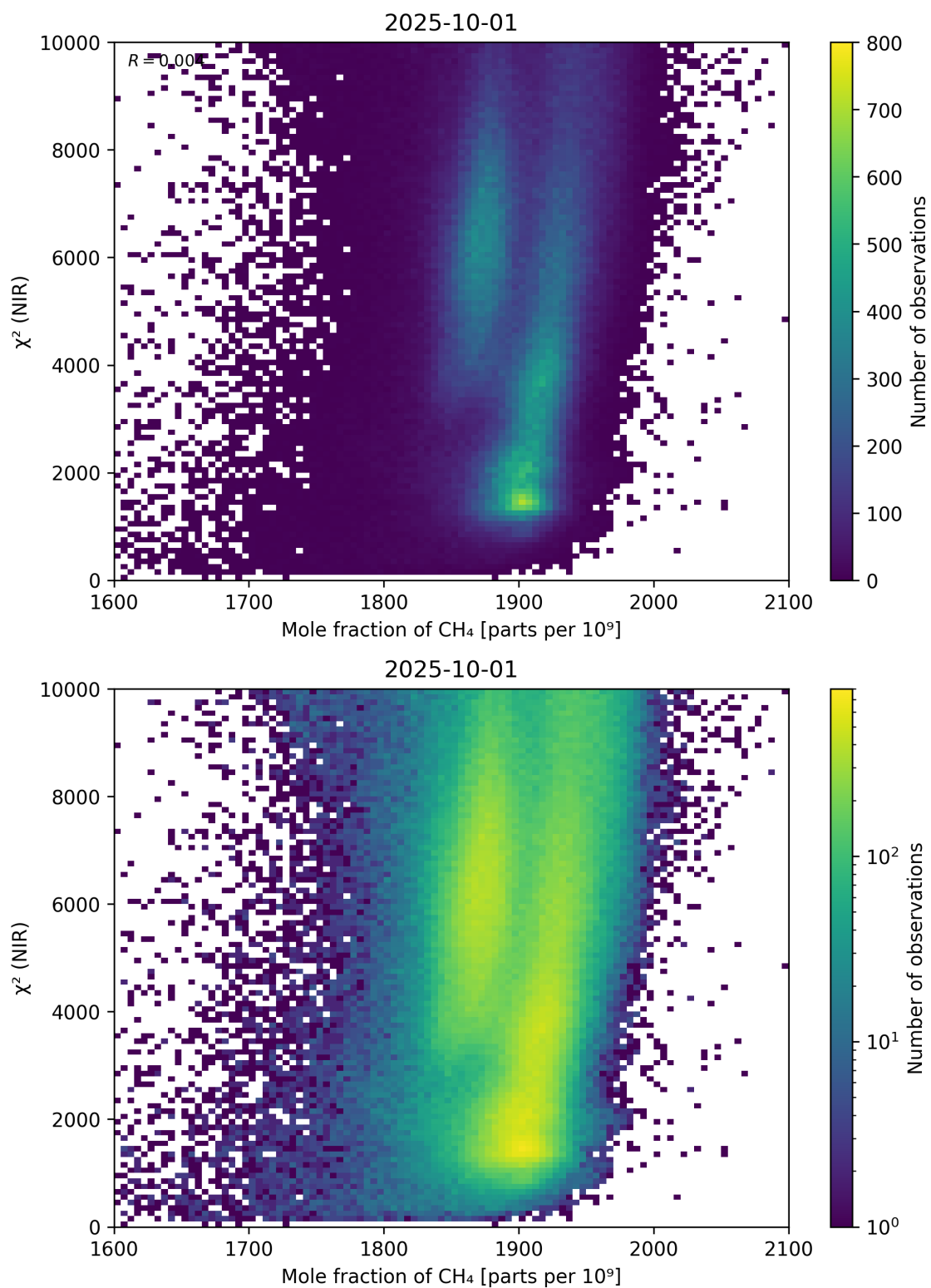
Figure 70: Scatter density plot of “Mole fraction of \text{CH}_4 ” against “ \chi^2 (NIR)” for 2025-10-01 to 2025-10-02.
