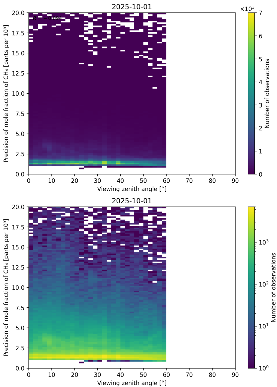
Figure 112: Scatter density plot of “Viewing zenith angle” against “Precision of mole fraction of CH 4 ” for 2025-10-01 to 2025-10-02.
