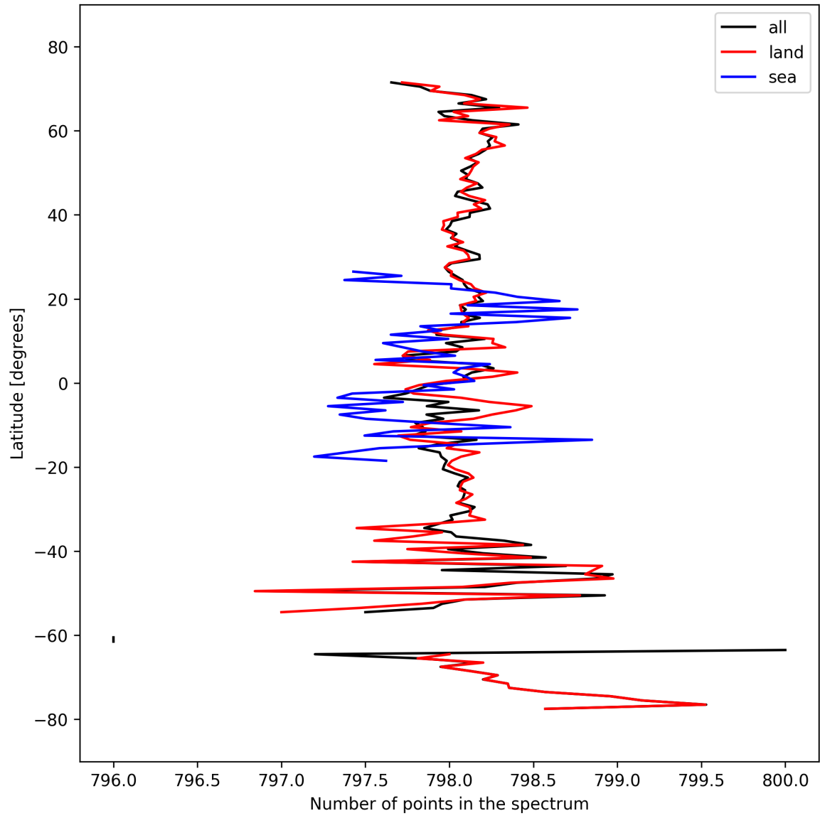
Figure 15: Zonal average of “Number of points in the spectrum” for 2025-10-01 to 2025-10-02.
