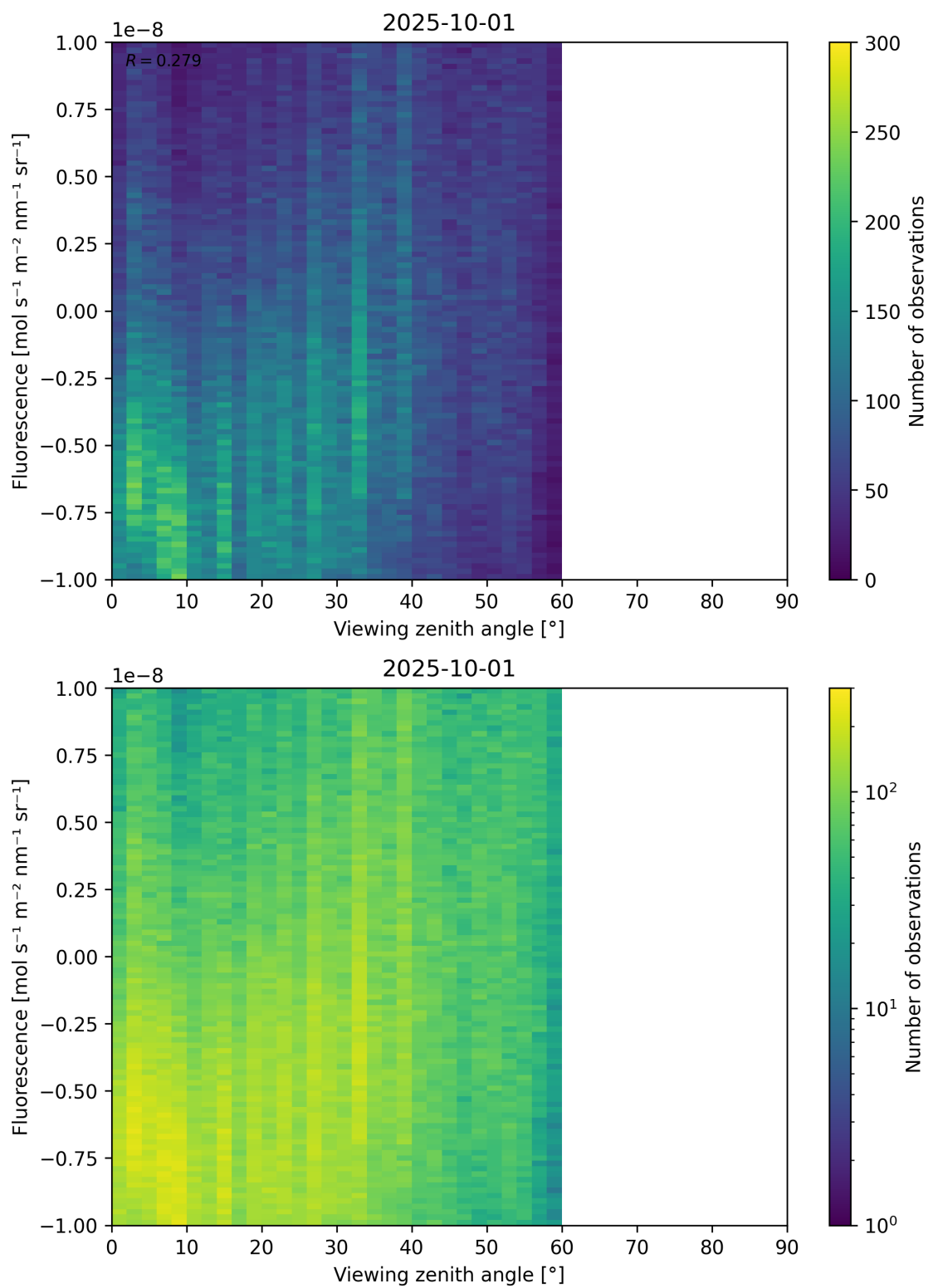
Figure 108: Scatter density plot of “Viewing zenith angle” against “Fluorescence” for 2025-10-01 to 2025-10-02.
