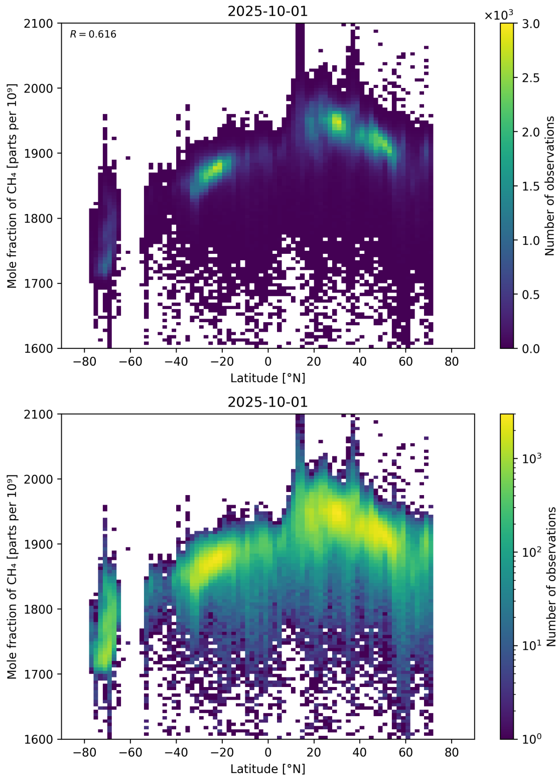
Figure 57: Scatter density plot of “Latitude” against “Mole fraction of CH 4 ” for 2025-10-01 to 2025-10-02.
