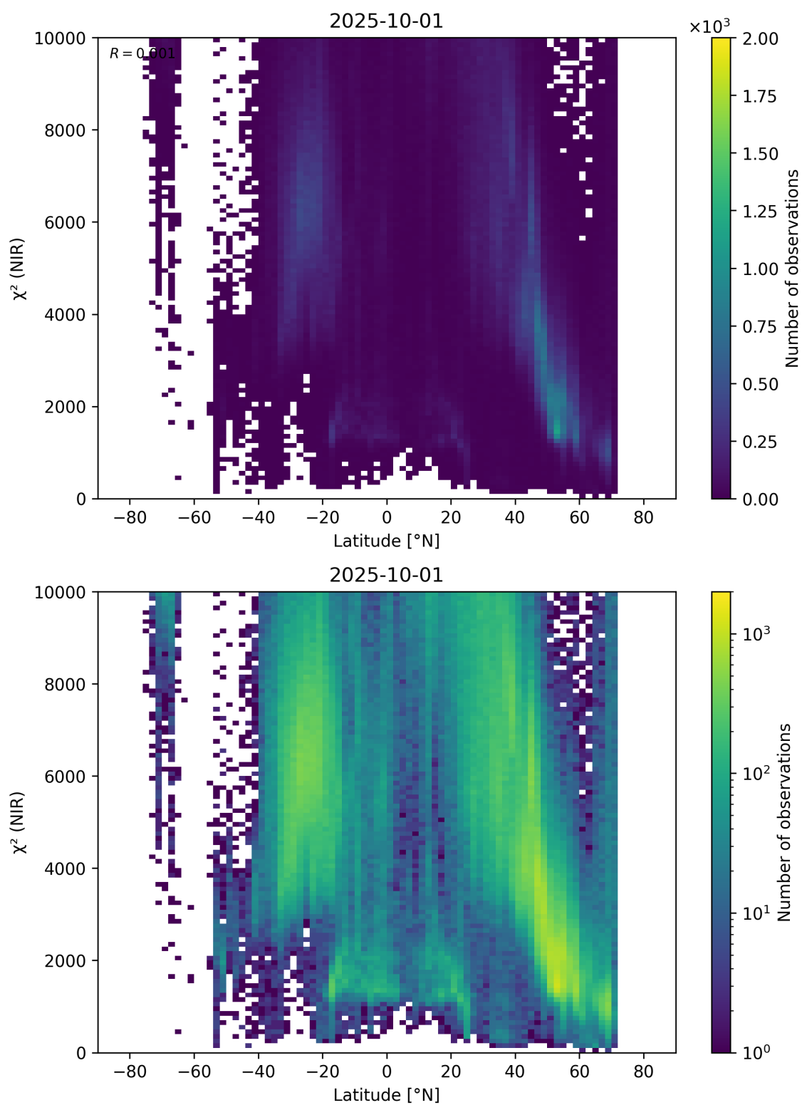
Figure 53: Scatter density plot of “Latitude” against “ \chi^2 (NIR)” for 2025-10-01 to 2025-10-02.
