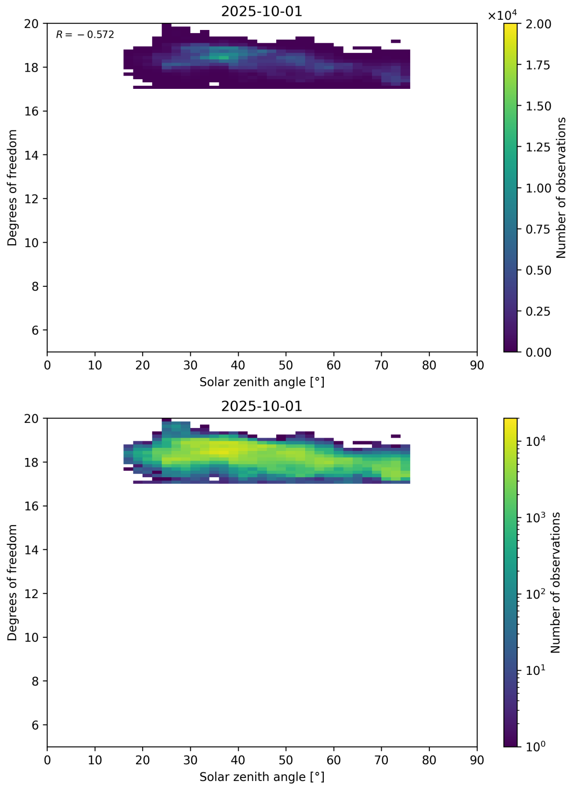
Figure 96: Scatter density plot of “Solar zenith angle” against “Degrees of freedom” for 2025-10-01 to 2025-10-02.
