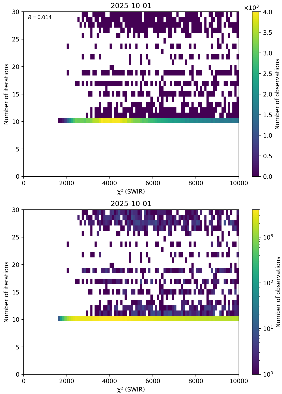
Figure 50: Scatter density plot of “ \chi^2 (SWIR)” against “Number of iterations” for 2025-10-01 to 2025-10-02.
