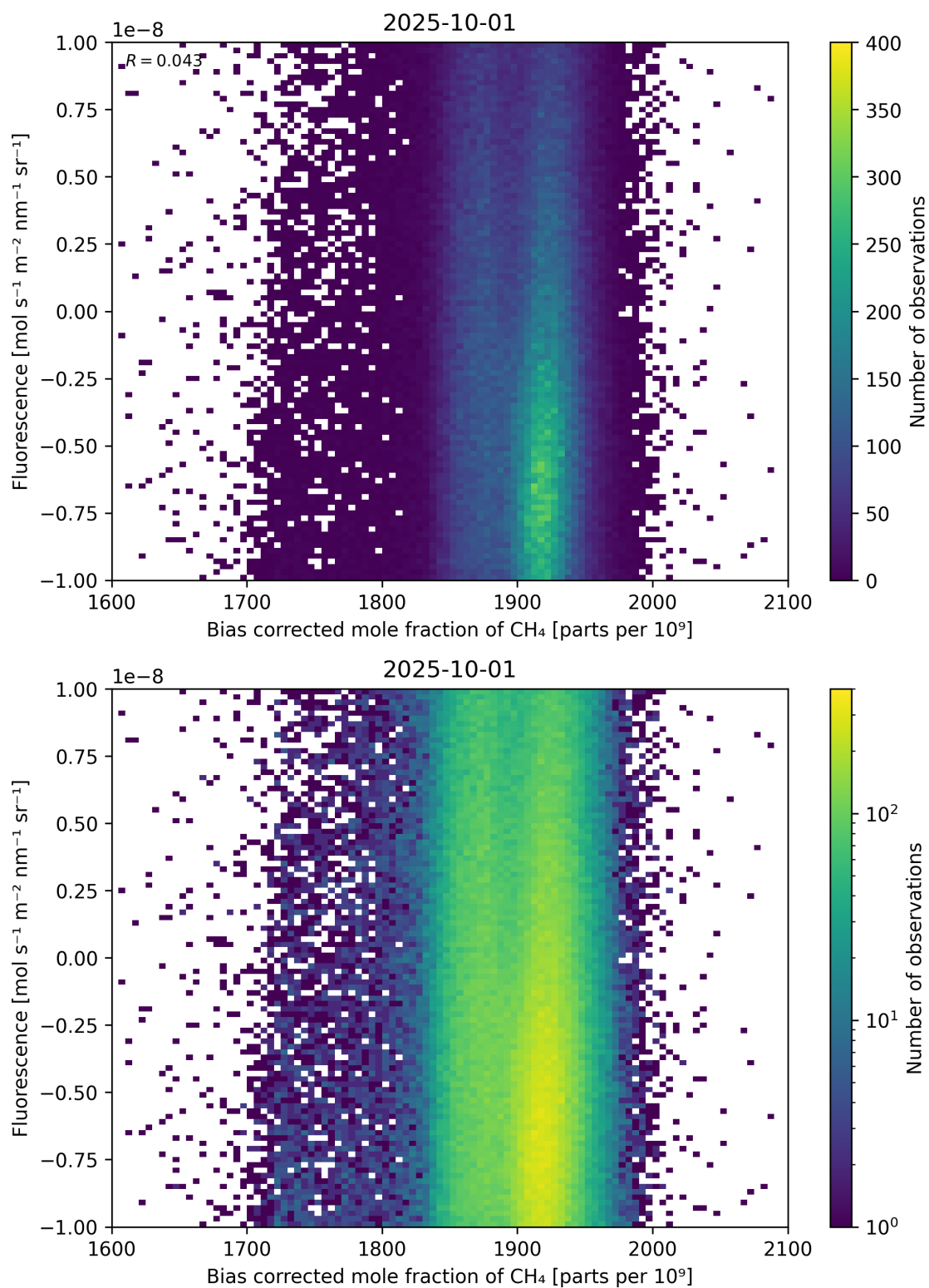
Figure 66: Scatter density plot of “Bias corrected mole fraction of CH 4 ” against “Fluorescence” for 2025-10-01 to 2025-10-02.
