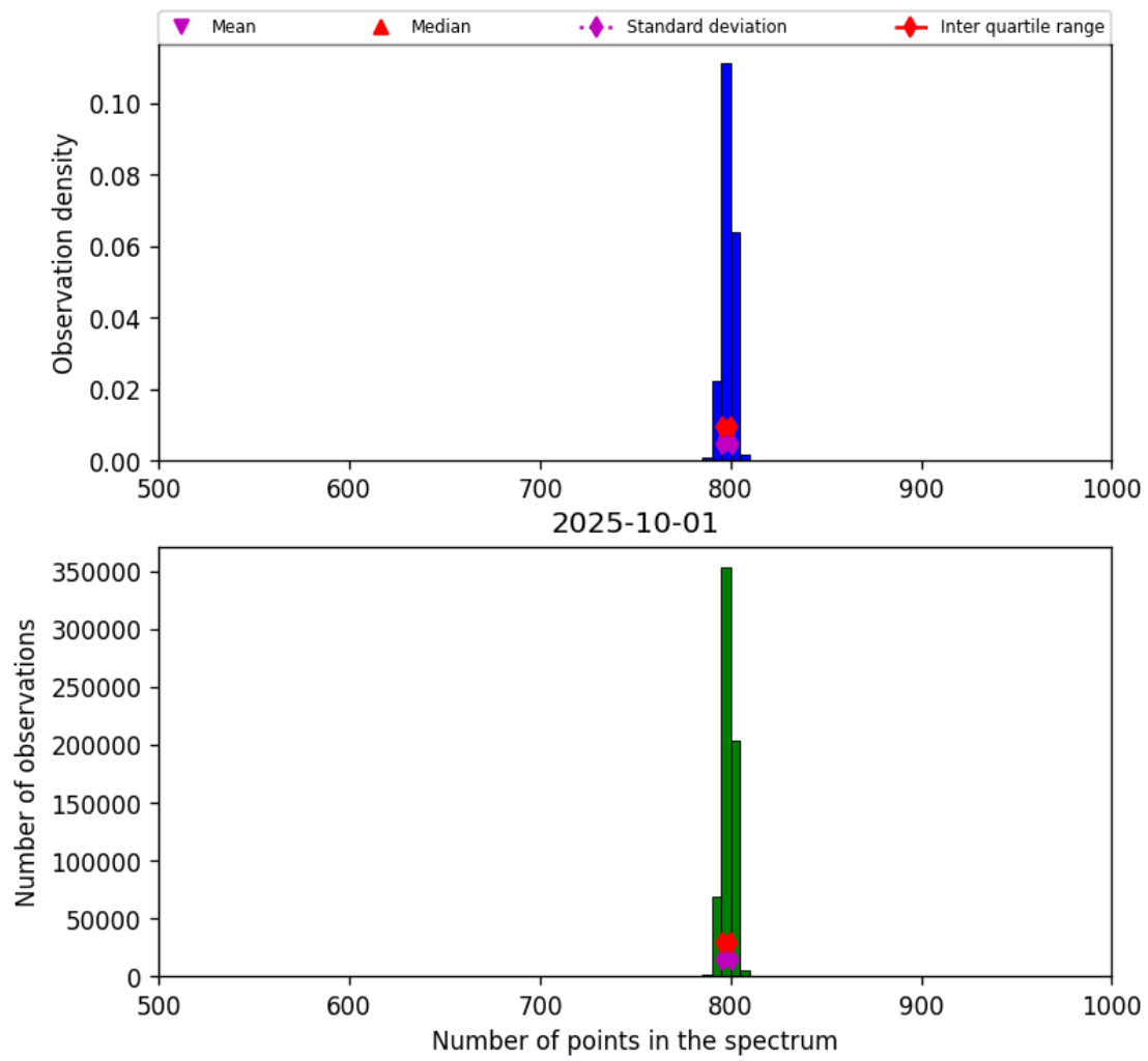
Figure 26: Histogram of “Number of points in the spectrum” for 2025-10-01 to 2025-10-02
