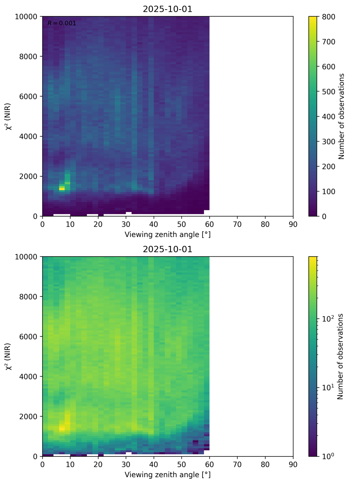
Figure 105: Scatter density plot of “Viewing zenith angle” against “ \chi^2 (NIR)” for 2025-10-01 to 2025-10-02.
