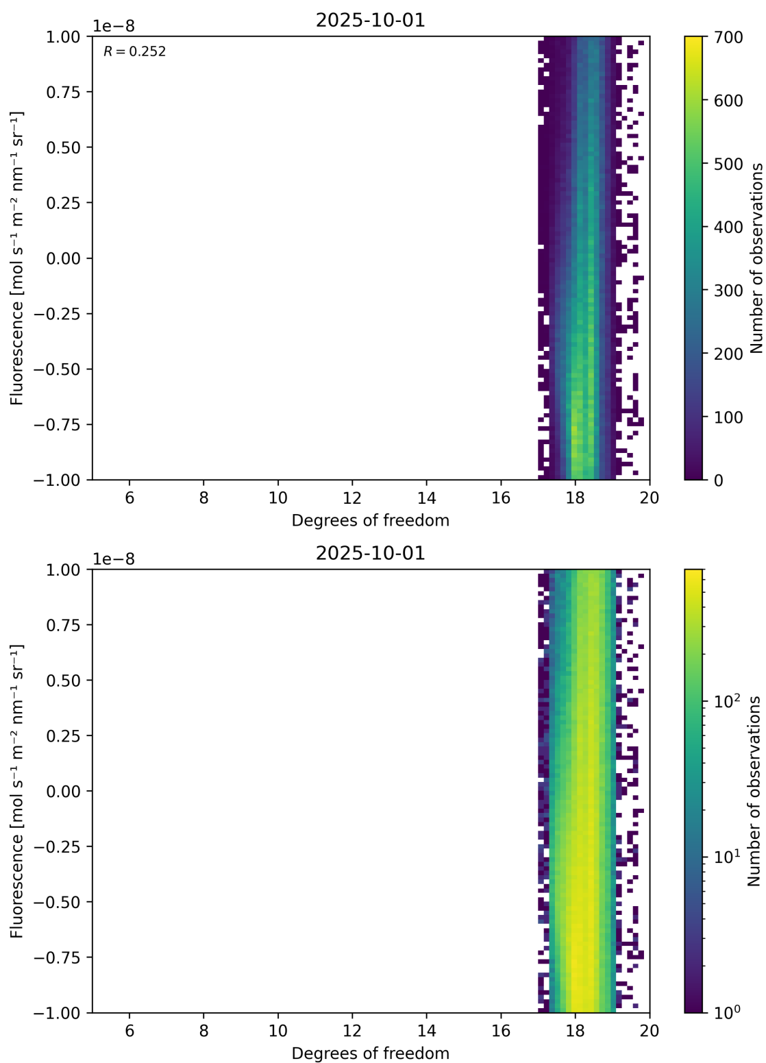
Figure 51: Scatter density plot of “Degrees of freedom” against “Fluorescence” for 2025-10-01 to 2025-10-02.
