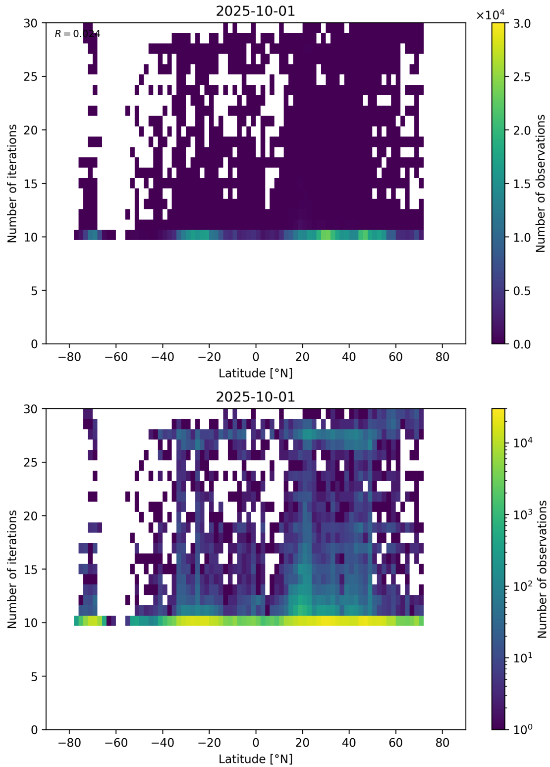
Figure 60: Scatter density plot of “Latitude” against “Number of iterations” for 2025-10-01 to 2025-10-02.
