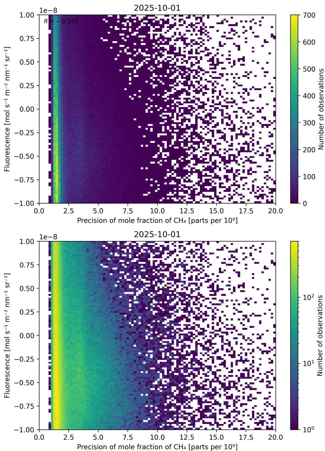
Figure 81: Scatter density plot of “Precision of mole fraction of \text{CH}_4 ” against “Fluorescence” for 2025-10-01 to 2025-10-02.
