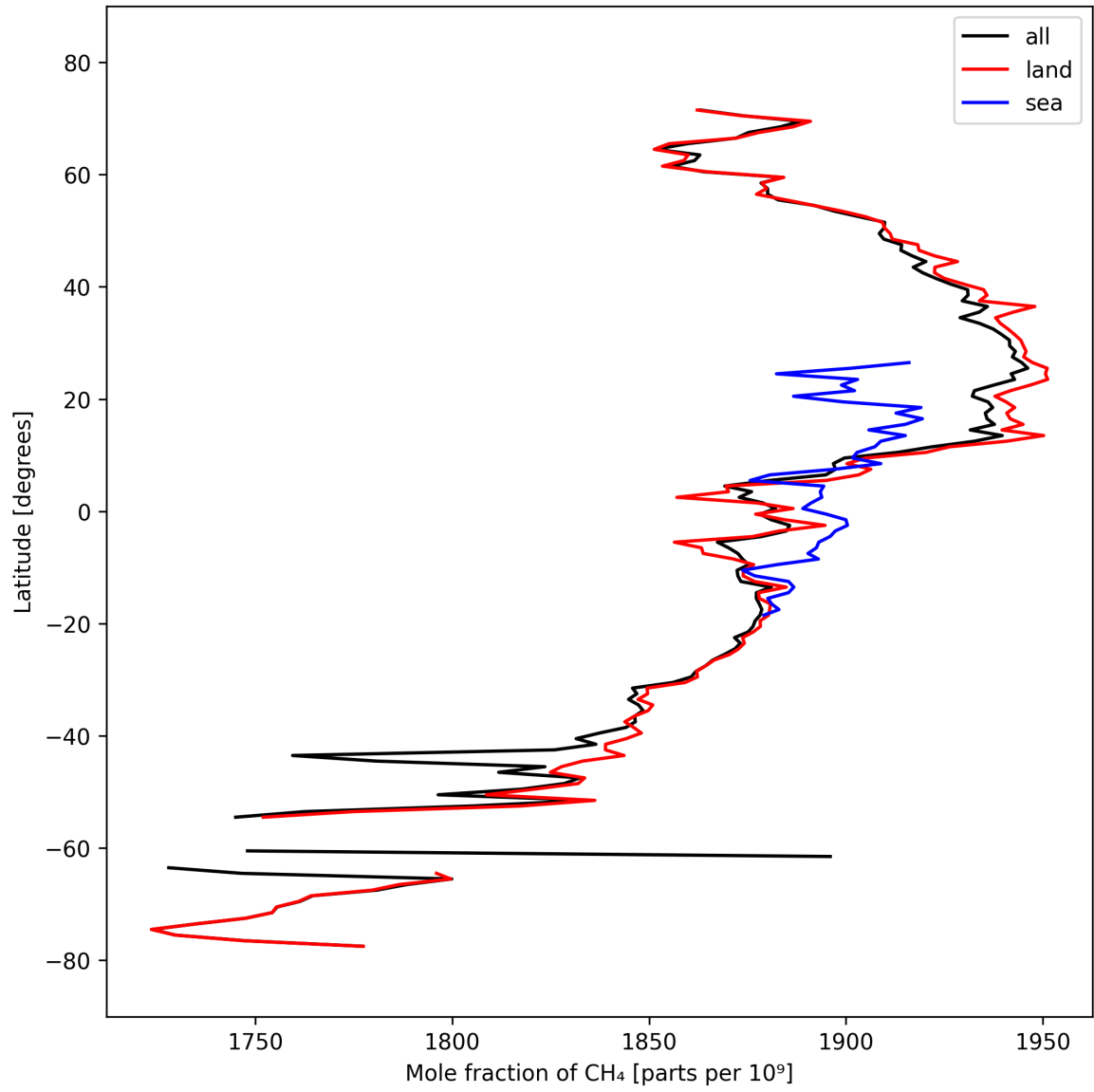
Figure 12: Zonal average of “Mole fraction of CH 4 ” for 2025-10-01 to 2025-10-02.
