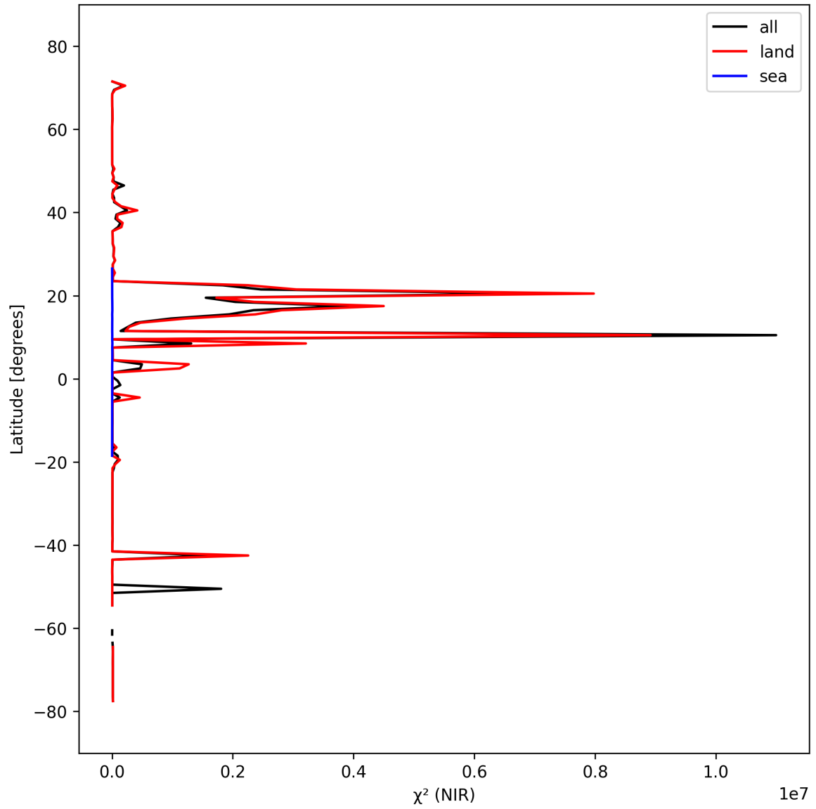
Figure 18: Zonal average of “ \chi^2 (NIR)” for 2025-10-01 to 2025-10-02.
