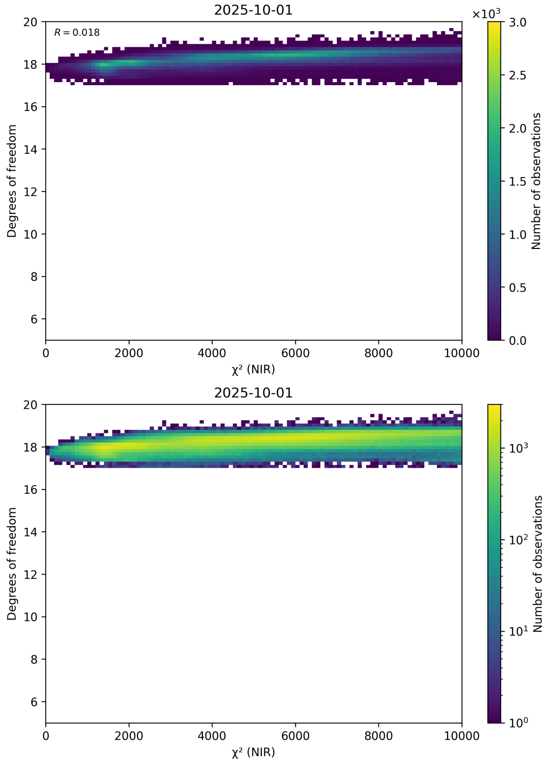
Figure 44: Scatter density plot of “ \chi^2 (NIR)” against “Degrees of freedom” for 2025-10-01 to 2025-10-02.
