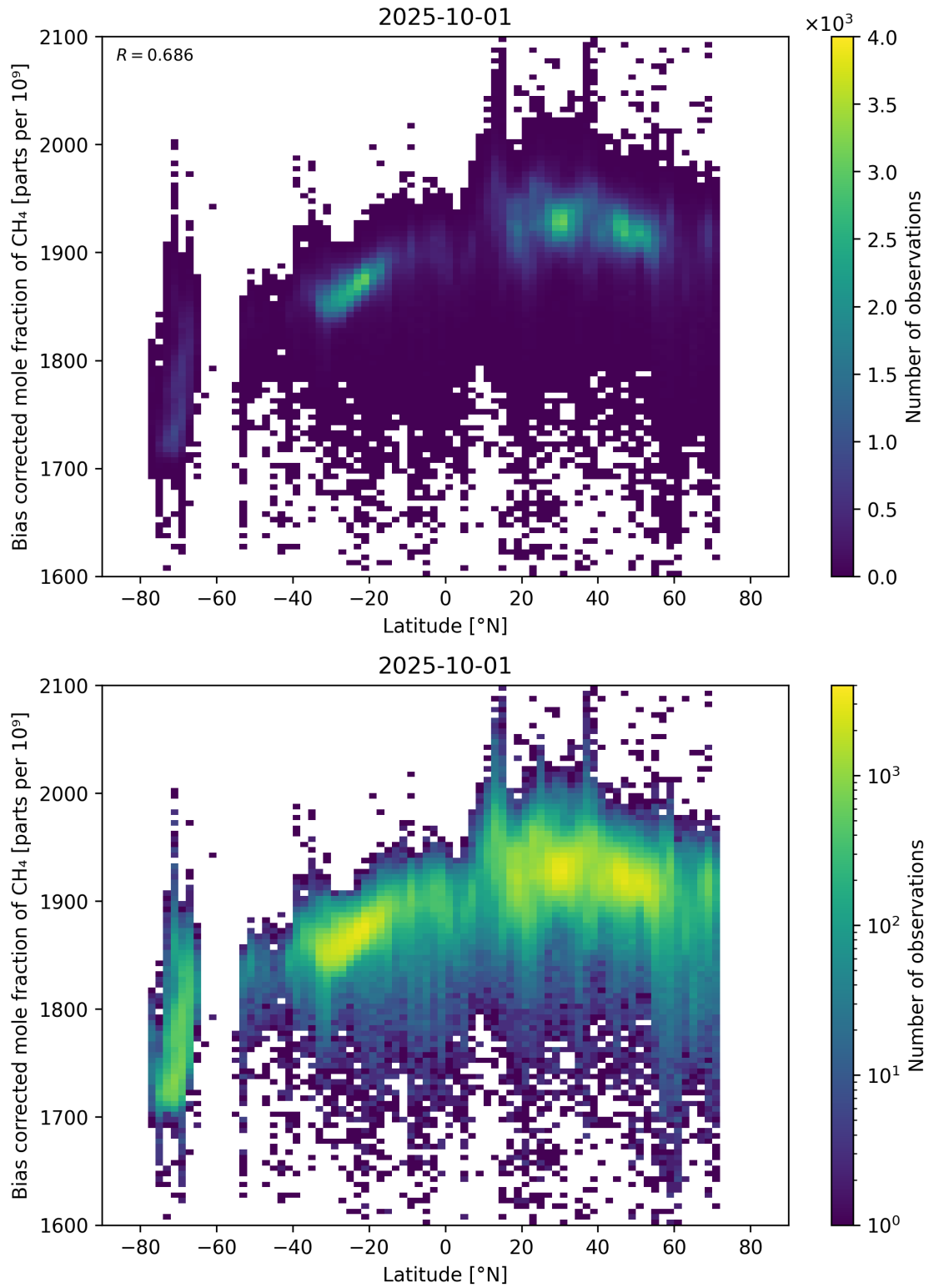
Figure 58: Scatter density plot of “Latitude” against “Bias corrected mole fraction of CH 4 ” for 2025-10-01 to 2025-10-02.
