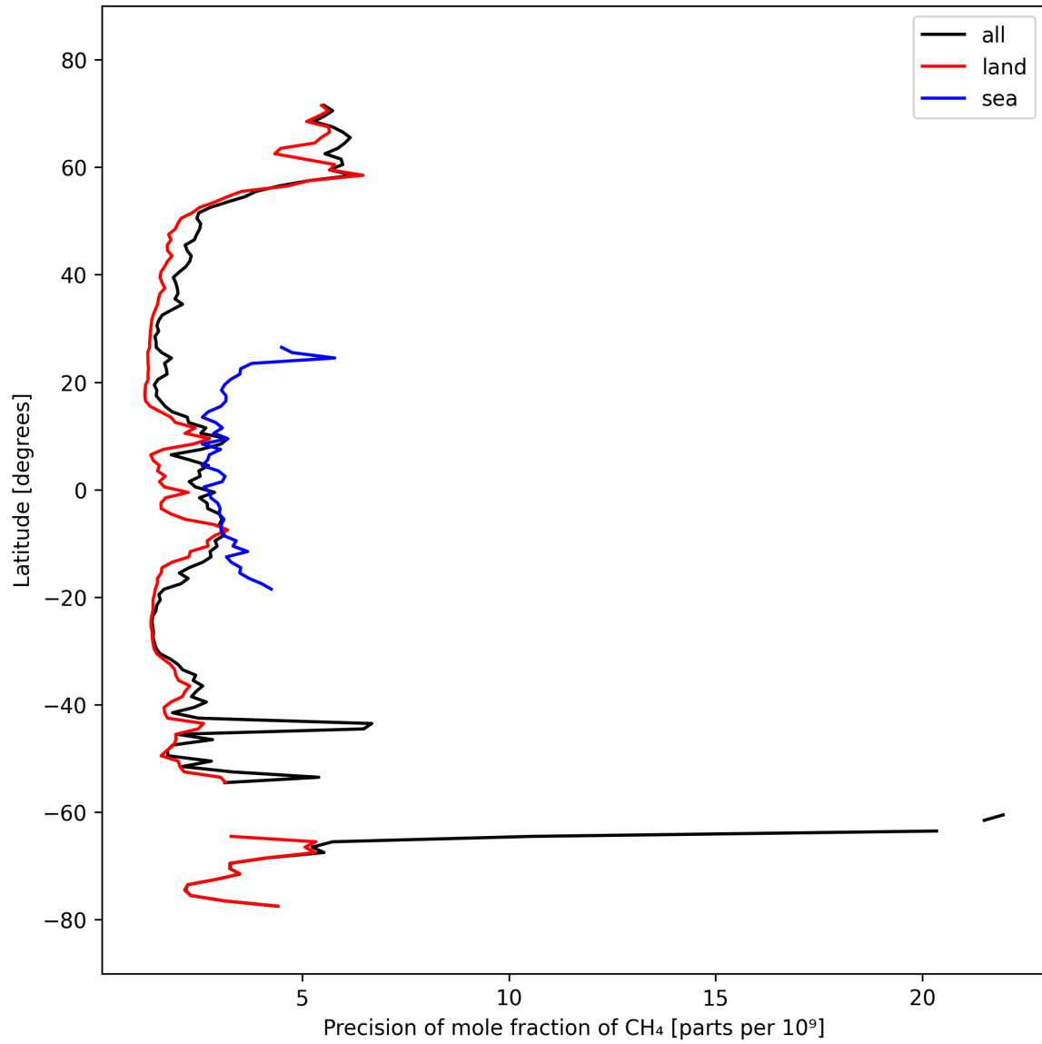
Figure 13: Zonal average of “Precision of mole fraction of CH 4 ” for 2025-10-01 to 2025-10-02.
