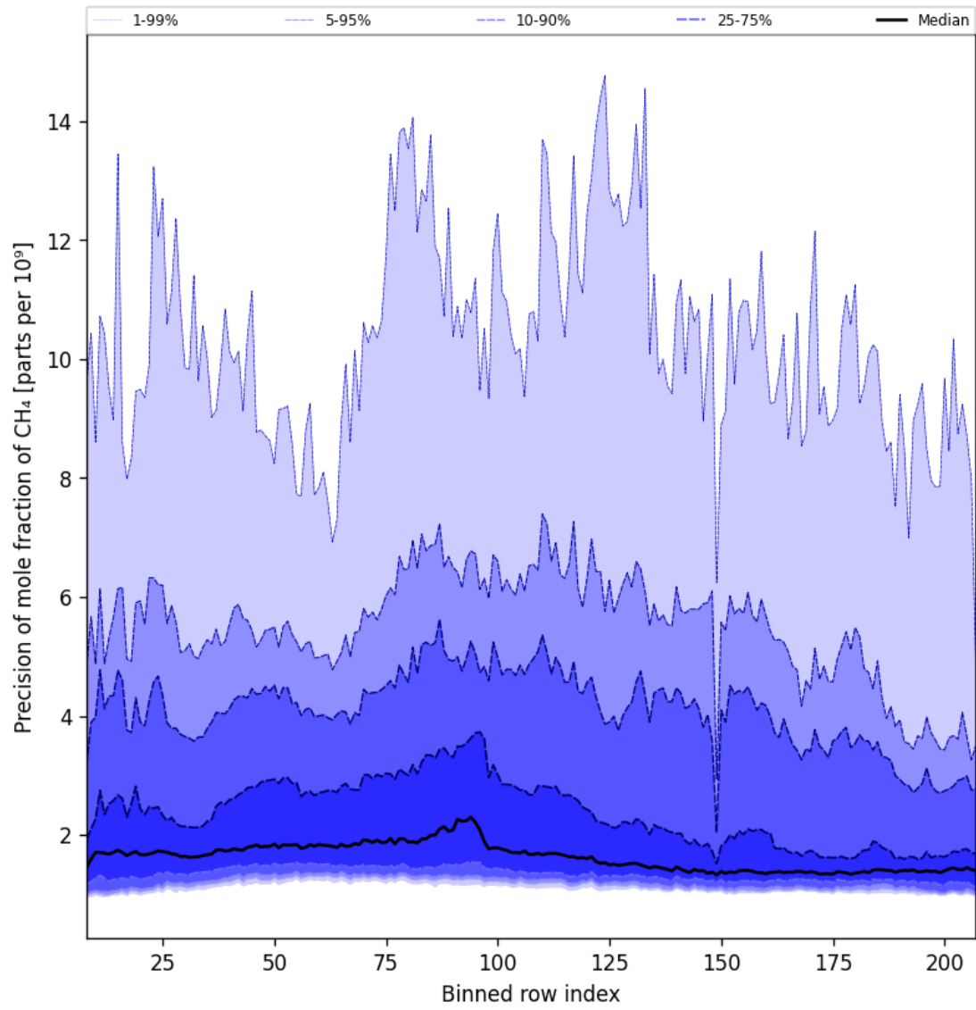
Figure 35: Along track statistics of “Precision of mole fraction of CH 4 ” for 2025-10-01 to 2025-10-02
