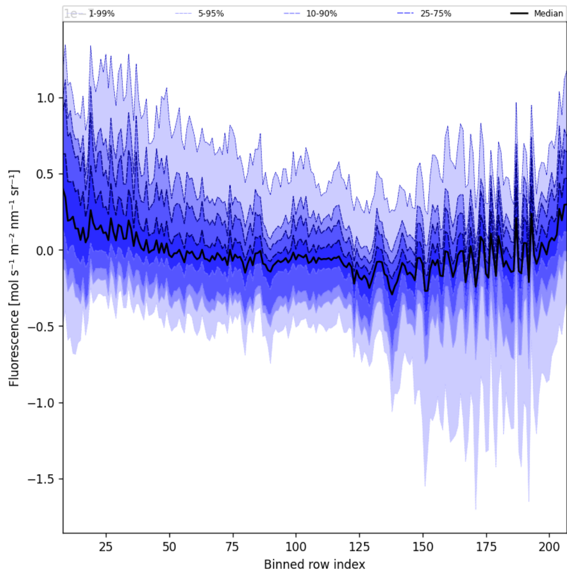
Figure 43: Along track statistics of “Fluorescence” for 2025-10-01 to 2025-10-02
