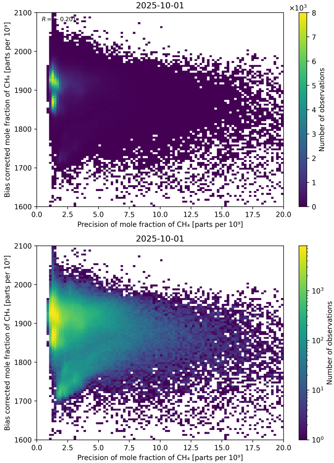
Figure 82: Scatter density plot of “Precision of mole fraction of CH 4 ” against “Bias corrected mole fraction of CH 4 ” for 2025-10-01 to 2025-10-02.
