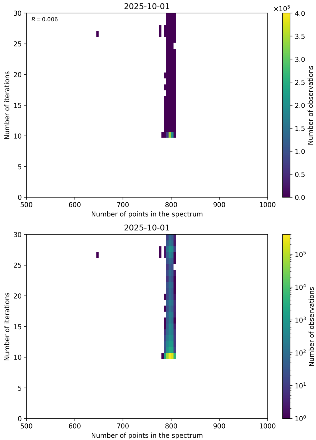
Figure 92: Scatter density plot of “Number of points in the spectrum” against “Number of iterations” for 2025-10-01 to 2025-10-02.
