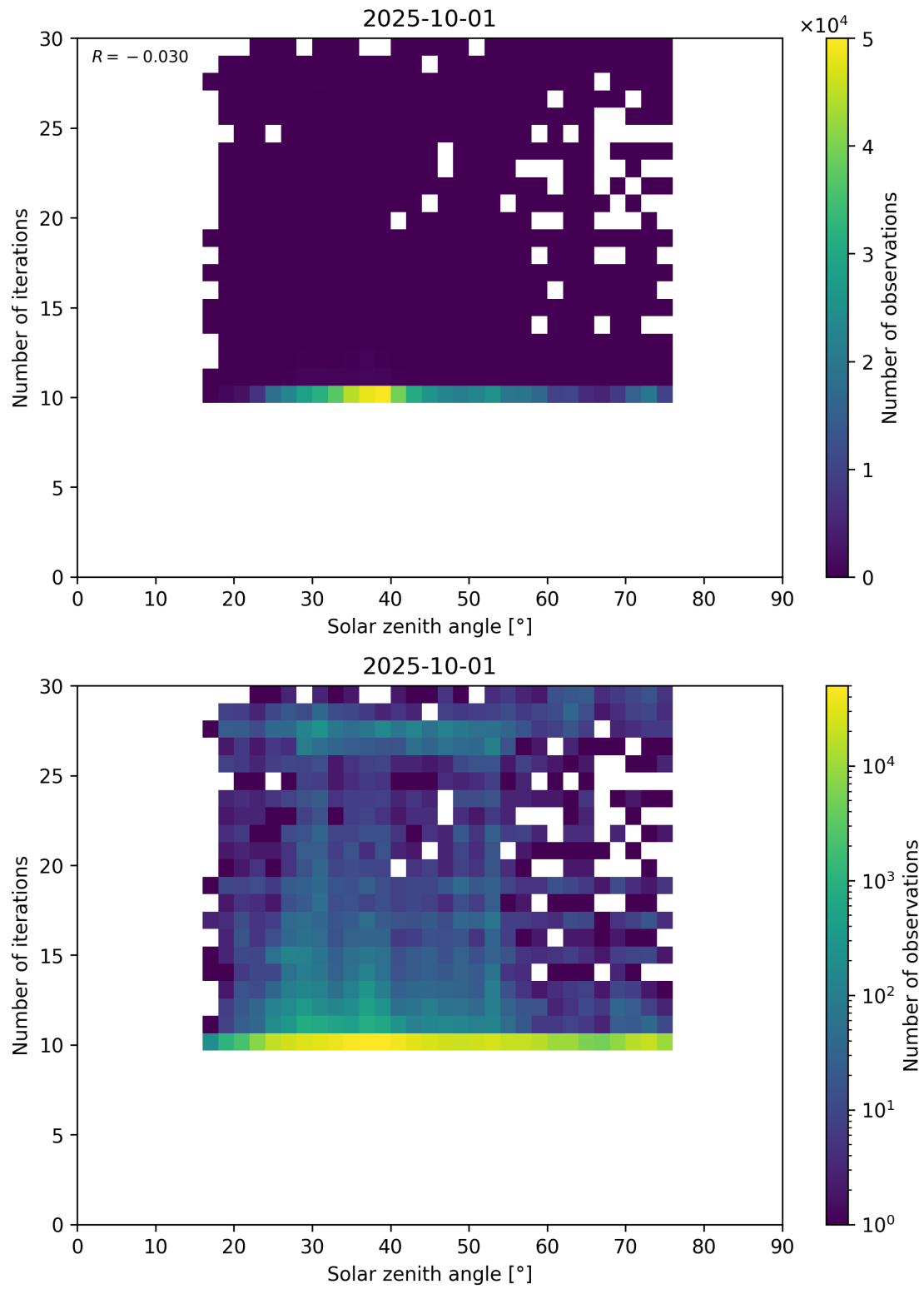
Figure 102: Scatter density plot of “Solar zenith angle” against “Number of iterations” for 2025-10-01 to 2025-10-02.
