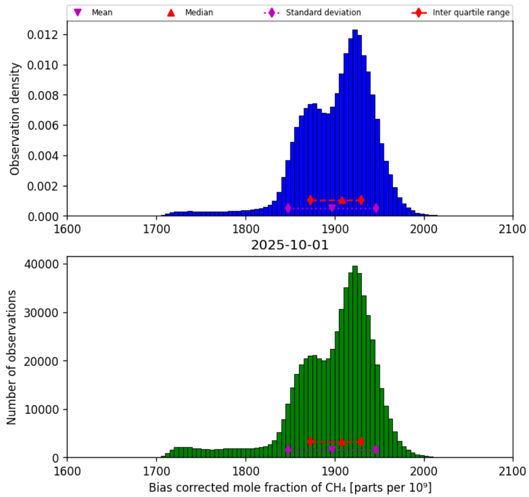
Figure 25: Histogram of “Bias corrected mole fraction of CH 4 ” for 2025-10-01 to 2025-10-02
