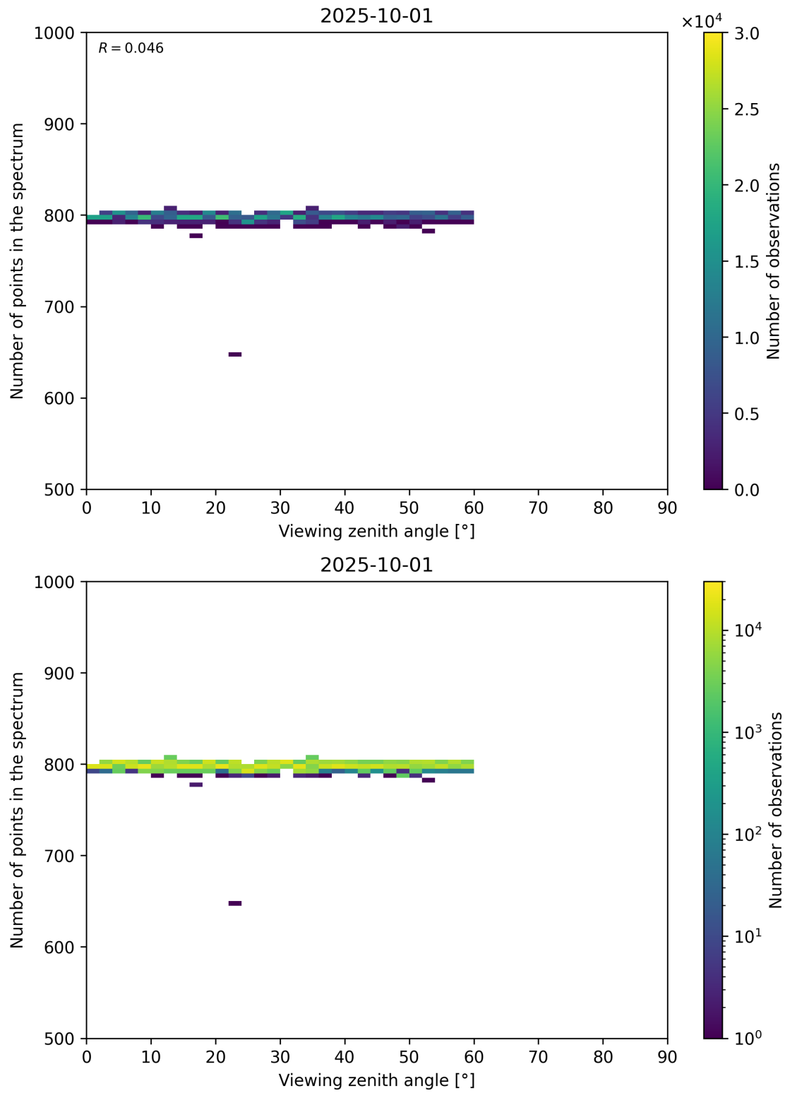
Figure 114: Scatter density plot of “Viewing zenith angle” against “Number of points in the spectrum” for 2025-10-01 to 2025-10-02.
