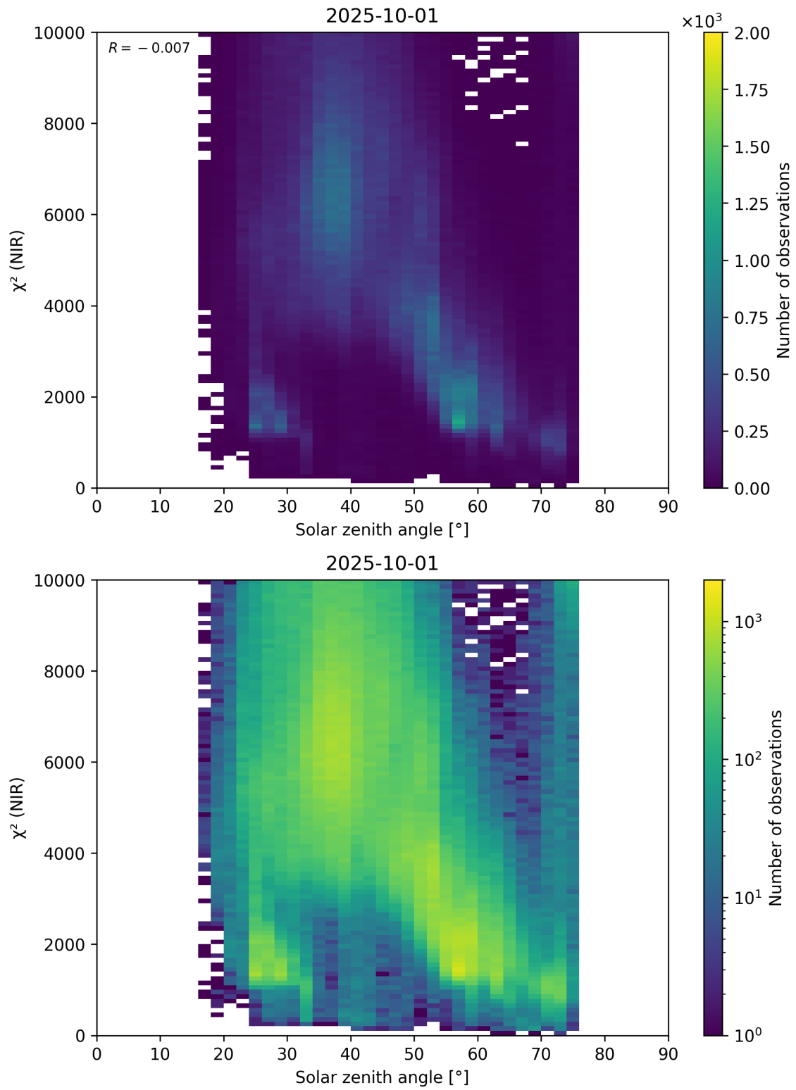
Figure 94: Scatter density plot of “Solar zenith angle” against “ \chi^2 (NIR)” for 2025-10-01 to 2025-10-02.
