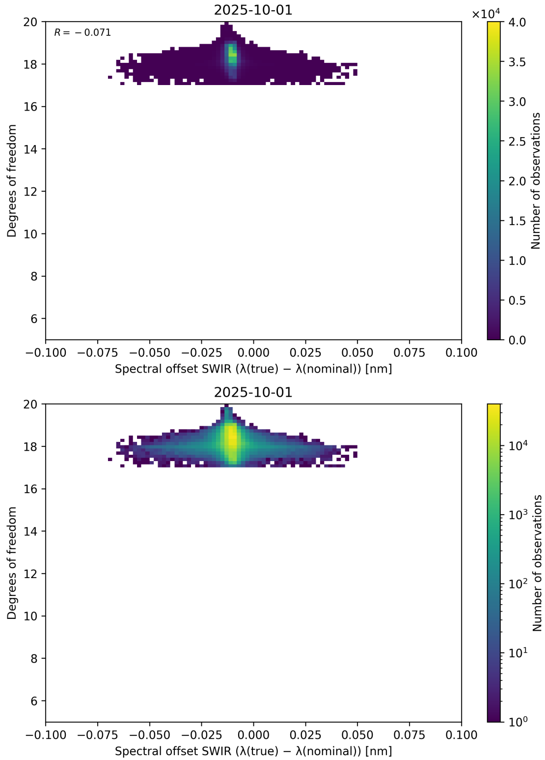
Figure 119: Scatter density plot of “Spectral offset SWIR ( \lambda_{\text{true}} - \lambda_{\text{nominal}} )” against “Degrees of freedom” for 2025-10-01 to 2025-10-02.
