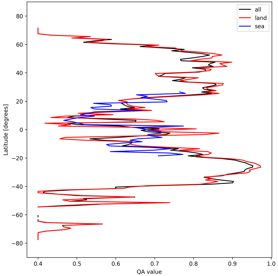
Figure 11: Zonal average of “QA value” for 2025-10-01 to 2025-10-02.
