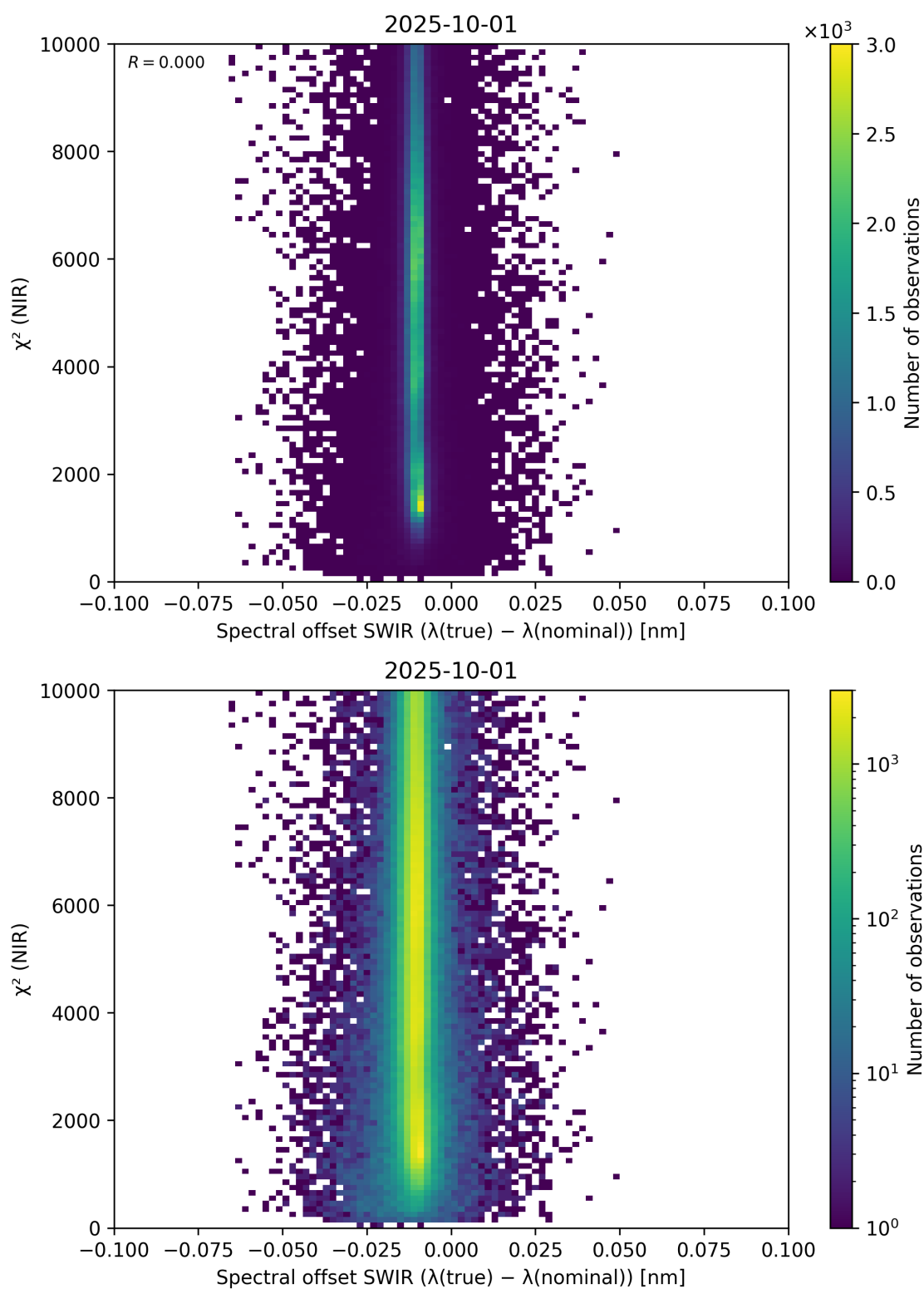
Figure 117: Scatter density plot of “Spectral offset SWIR ( \lambda_{\text{true}} - \lambda_{\text{nominal}} )” against “ \chi^2 (NIR)” for 2025-10-01 to 2025-10-02.
