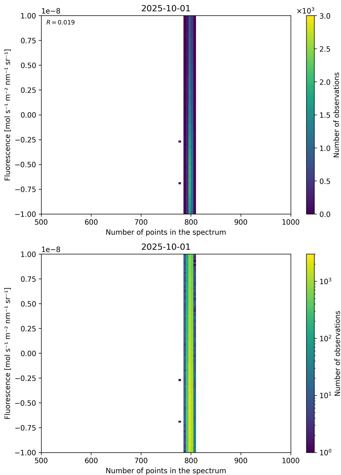
Figure 91: Scatter density plot of “Number of points in the spectrum” against “Fluorescence” for 2025-10-01 to 2025-10-02.
