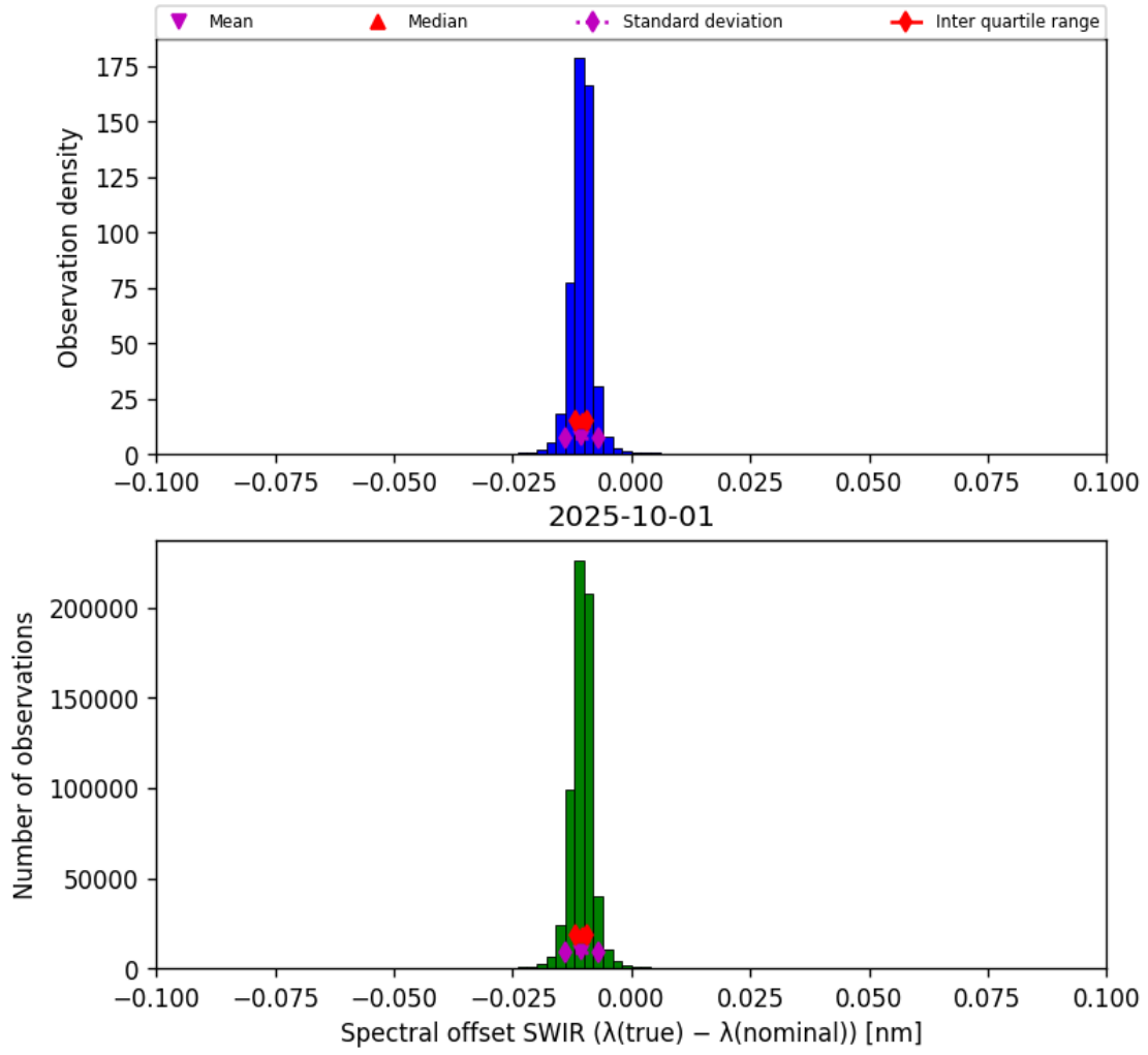
Figure 27: Histogram of “Spectral offset SWIR ( \lambda_{\text{true}} - \lambda_{\text{nominal}} )” for 2025-10-01 to 2025-10-02
