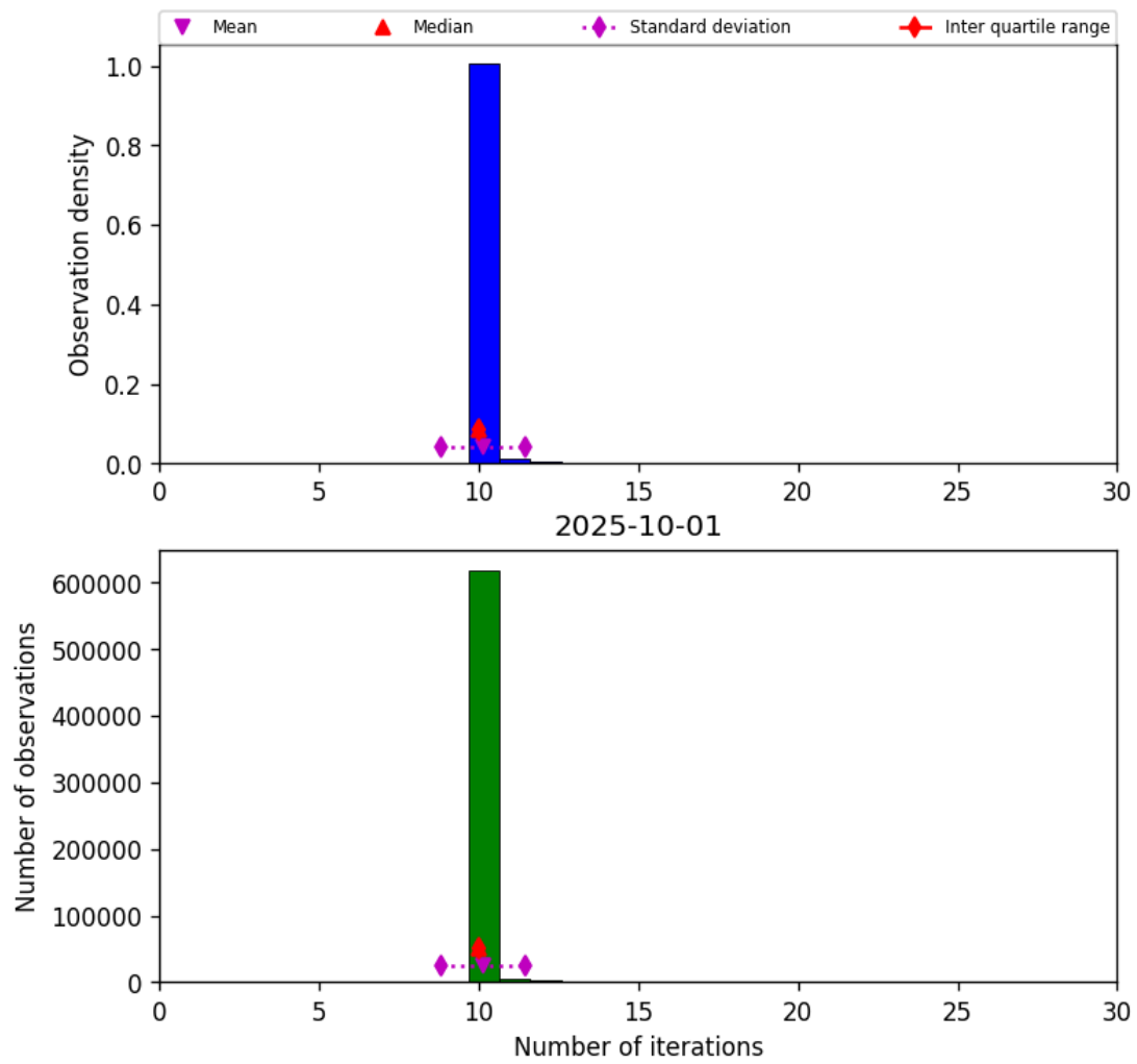
Figure 31: Histogram of “Number of iterations” for 2025-10-01 to 2025-10-02
