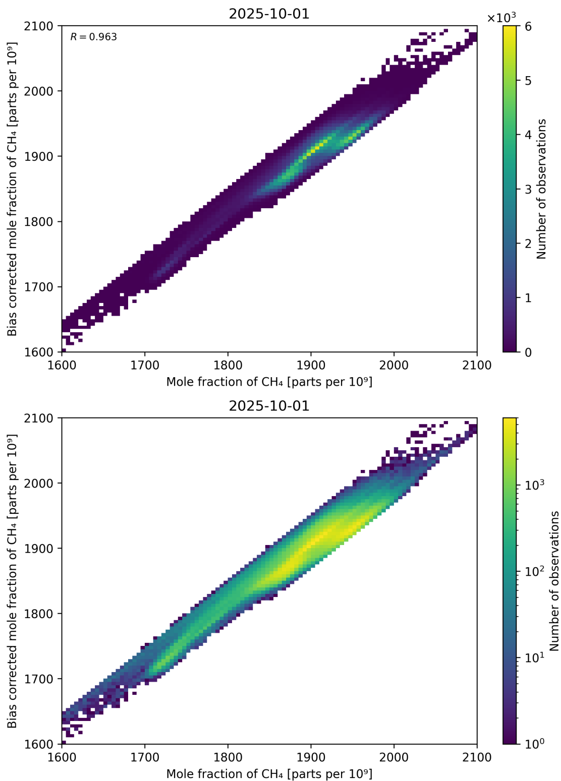
Figure 74: Scatter density plot of “Mole fraction of CH 4 ” against “Bias corrected mole fraction of CH 4 ” for 2025-10-01 to 2025-10-02.
