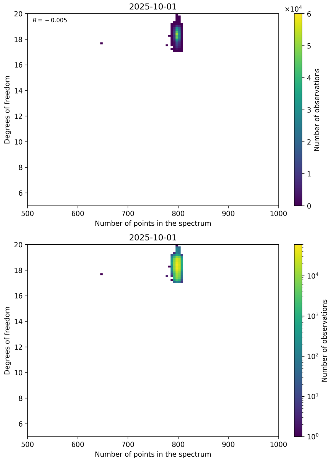
Figure 90: Scatter density plot of “Number of points in the spectrum” against “Degrees of freedom” for 2025-10-01 to 2025-10-02.
