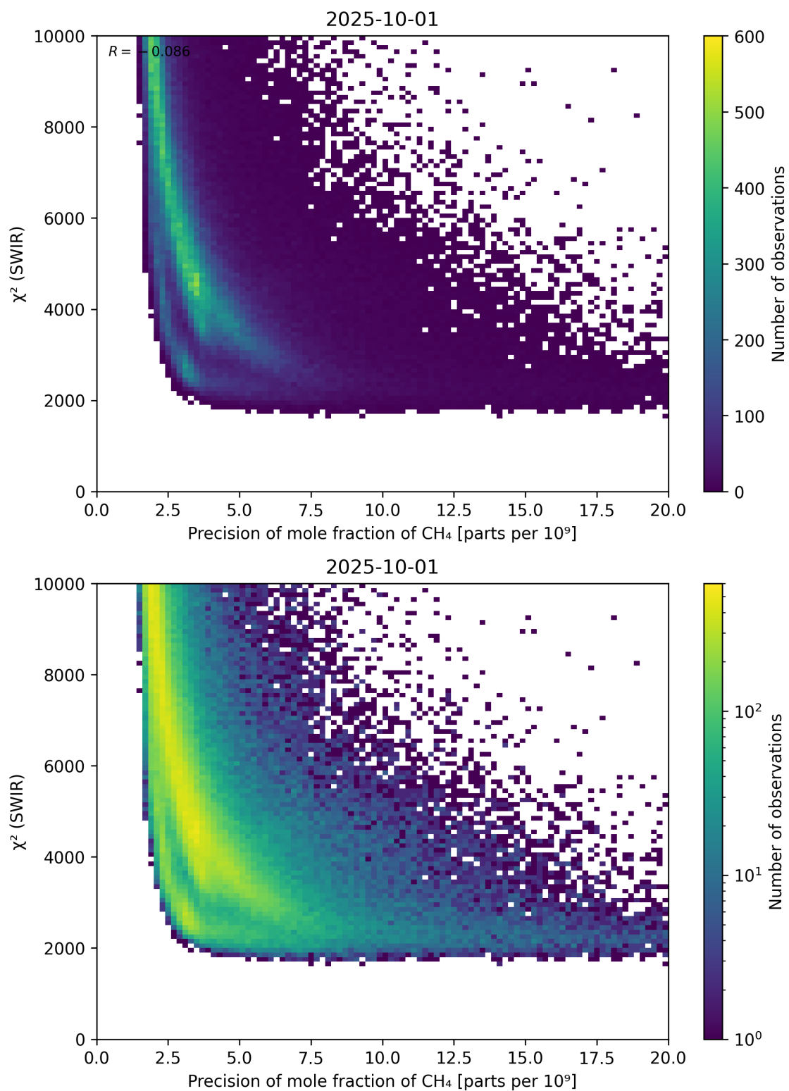
Figure 79: Scatter density plot of “Precision of mole fraction of \text{CH}_4 ” against “ \chi^2 (SWIR)” for 2025-10-01 to 2025-10-02.
