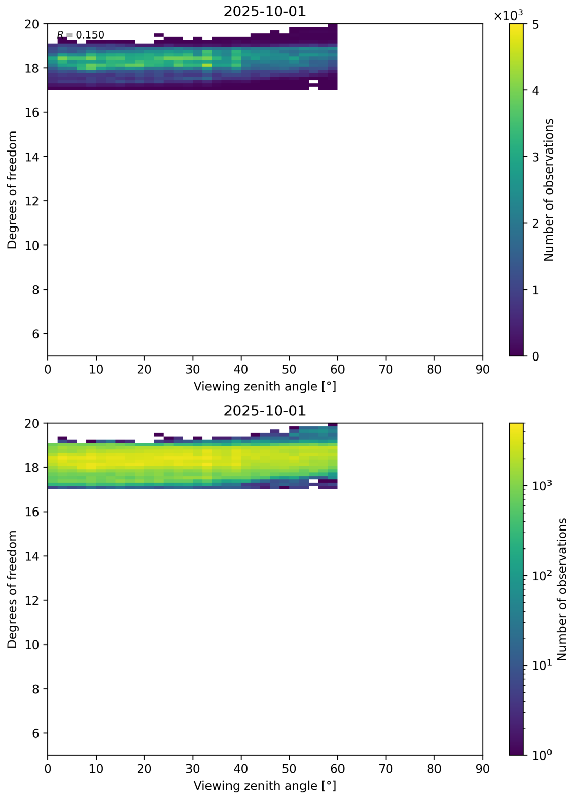
Figure 107: Scatter density plot of “Viewing zenith angle” against “Degrees of freedom” for 2025-10-01 to 2025-10-02.
