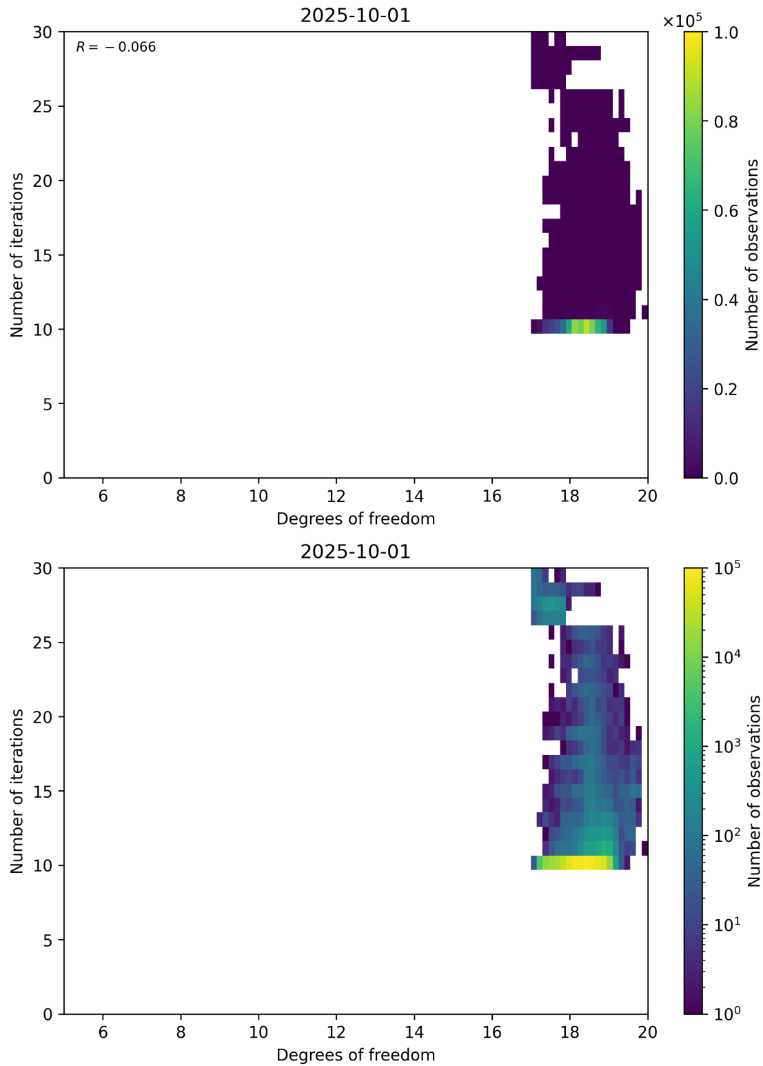
Figure 52: Scatter density plot of “Degrees of freedom” against “Number of iterations” for 2025-10-01 to 2025-10-02.
