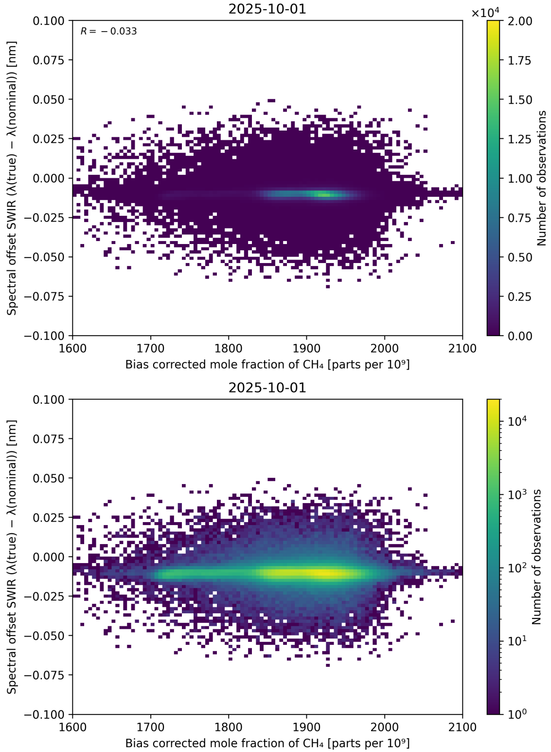
Figure 69: Scatter density plot of “Bias corrected mole fraction of CH 4 ” against “Spectral offset SWIR ( \lambda_{\text{true}} - \lambda_{\text{nominal}} )” for 2025-10-01 to 2025-10-02.
