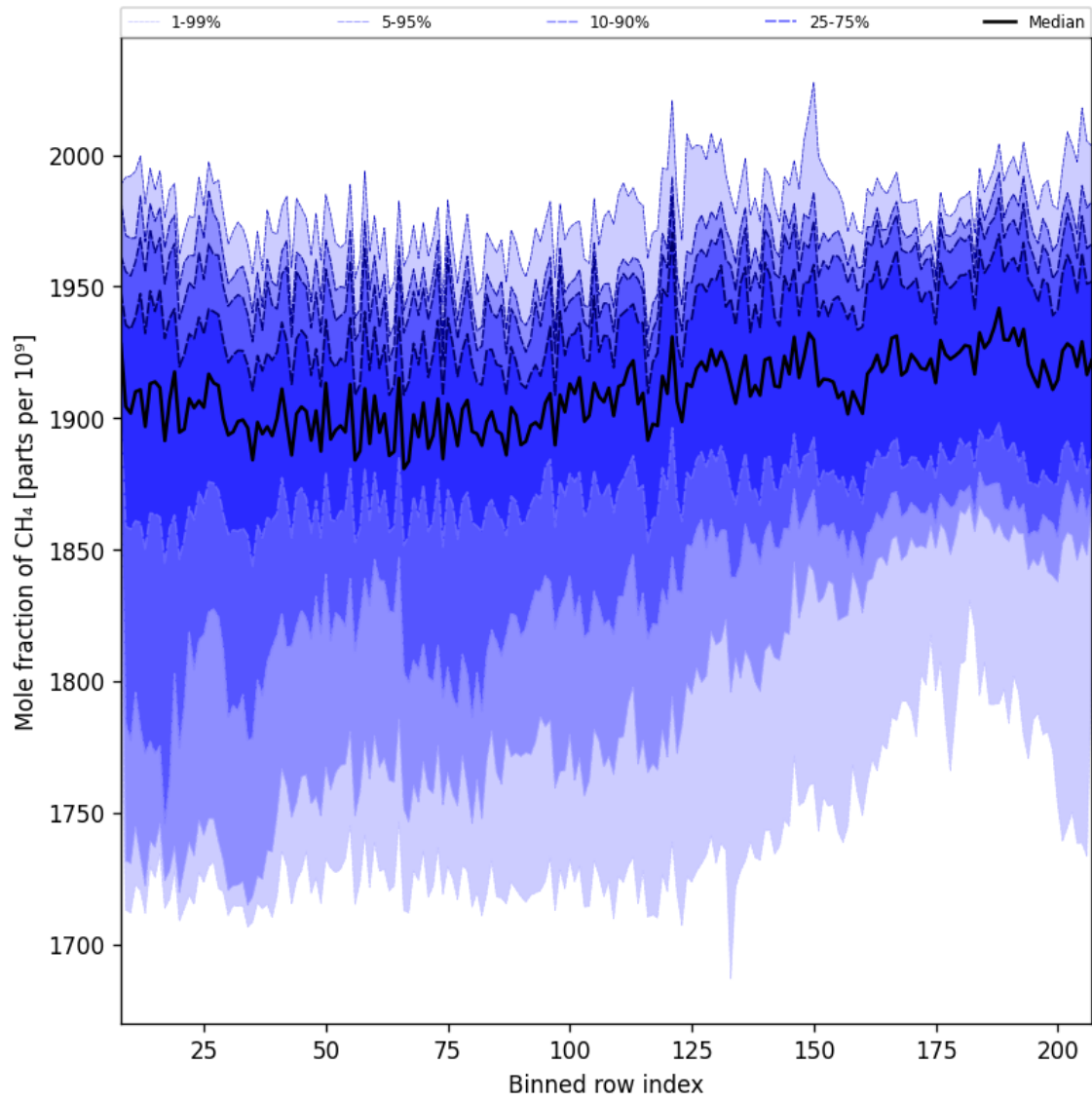
Figure 34: Along track statistics of “Mole fraction of CH 4 ” for 2025-10-01 to 2025-10-02
