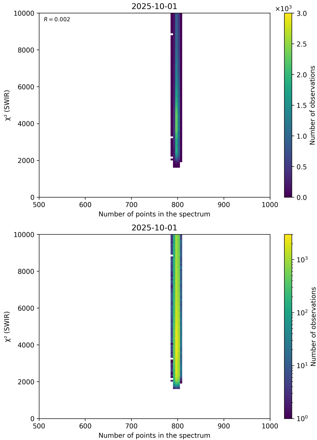
Figure 89: Scatter density plot of “Number of points in the spectrum” against “ \chi^2 (SWIR)” for 2025-10-01 to 2025-10-02.
