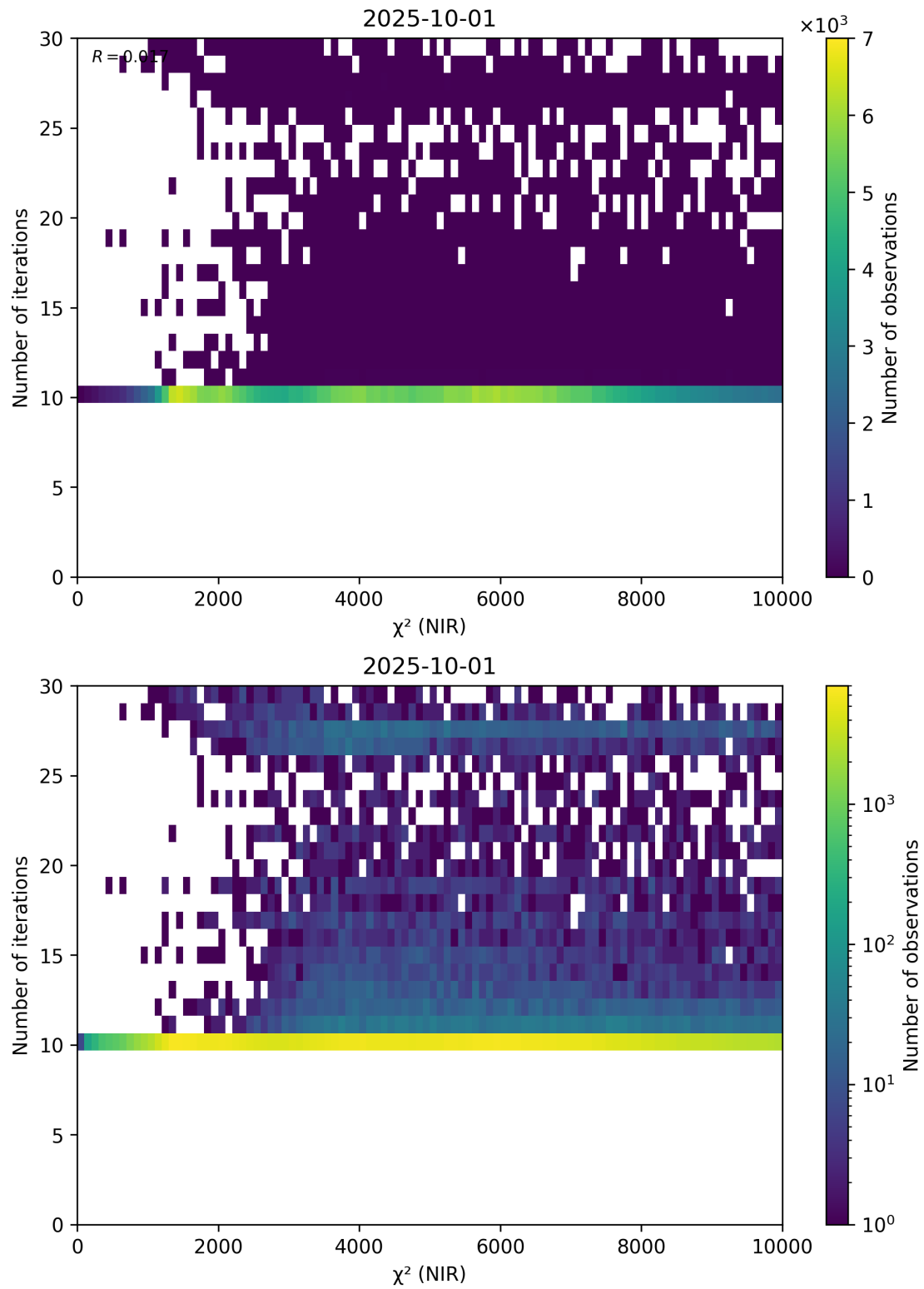
Figure 46: Scatter density plot of “ \chi^2 (NIR)” against “Number of iterations” for 2025-10-01 to 2025-10-02.
