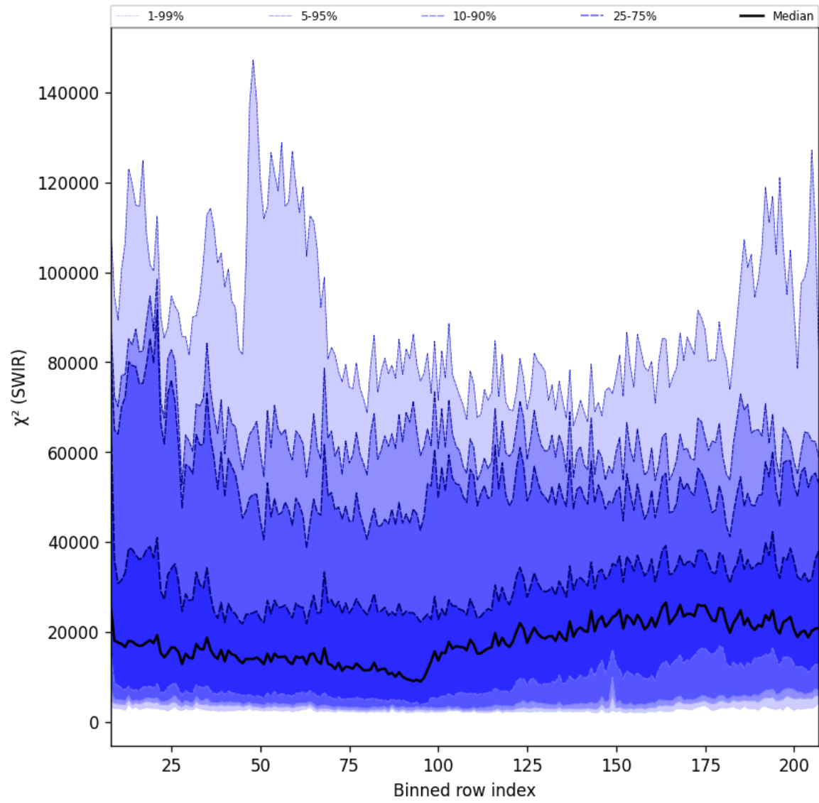
Figure 39: Along track statistics of “ \chi^2 (SWIR)” for 2025-10-01 to 2025-10-02
