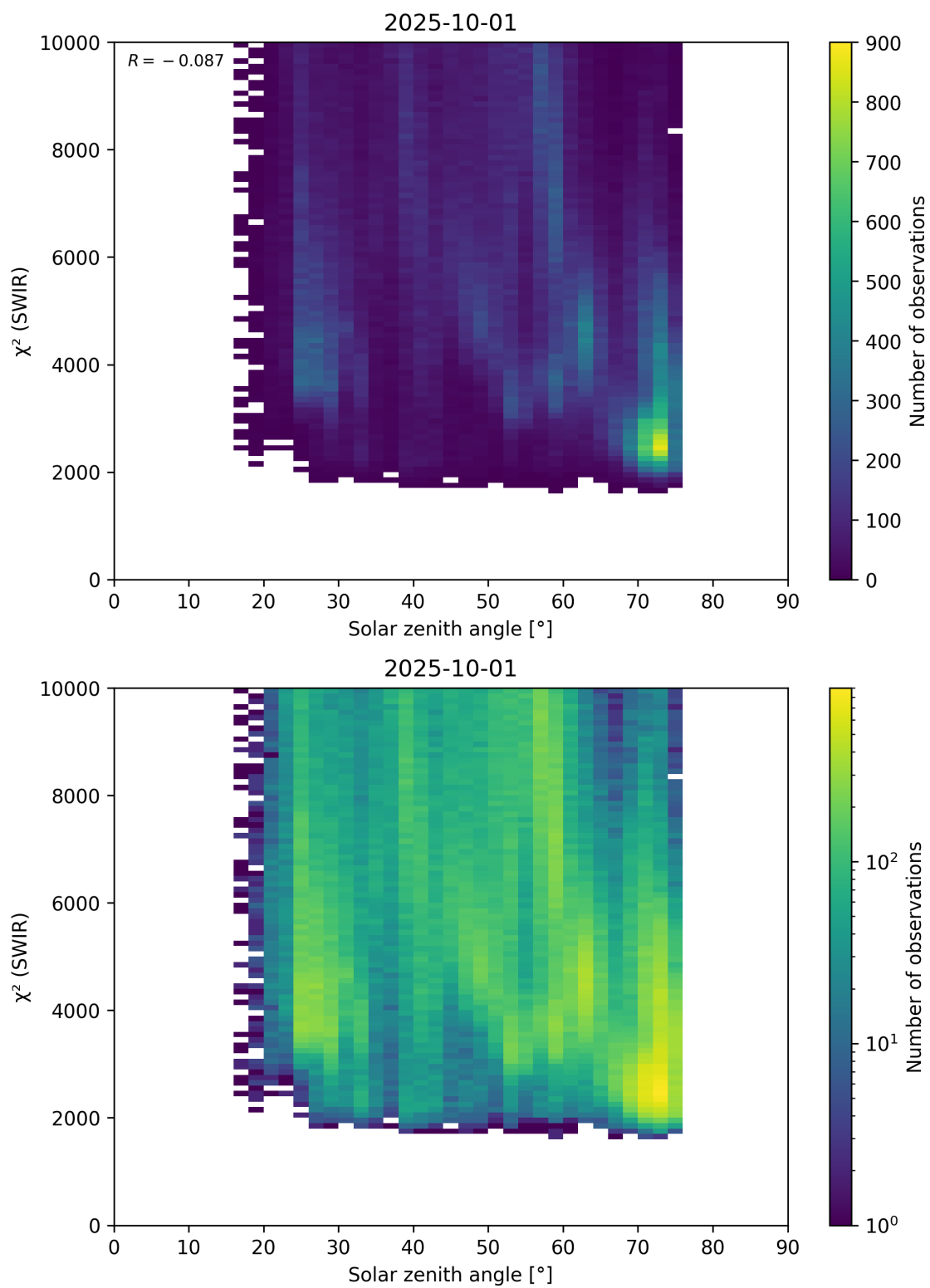
Figure 95: Scatter density plot of “Solar zenith angle” against “ \chi^2 (SWIR)” for 2025-10-01 to 2025-10-02.
