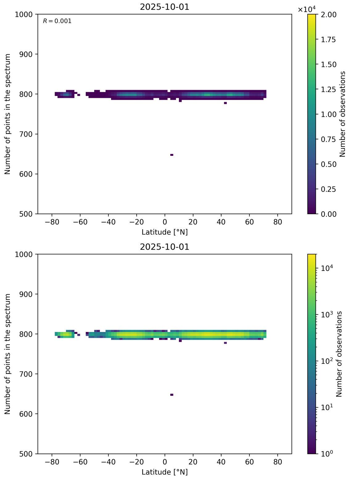
Figure 61: Scatter density plot of “Latitude” against “Number of points in the spectrum” for 2025-10-01 to 2025-10-02.
