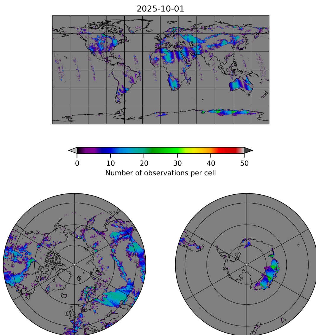
Figure 10: Map of the number of observations for 2025-10-01 to 2025-10-02
