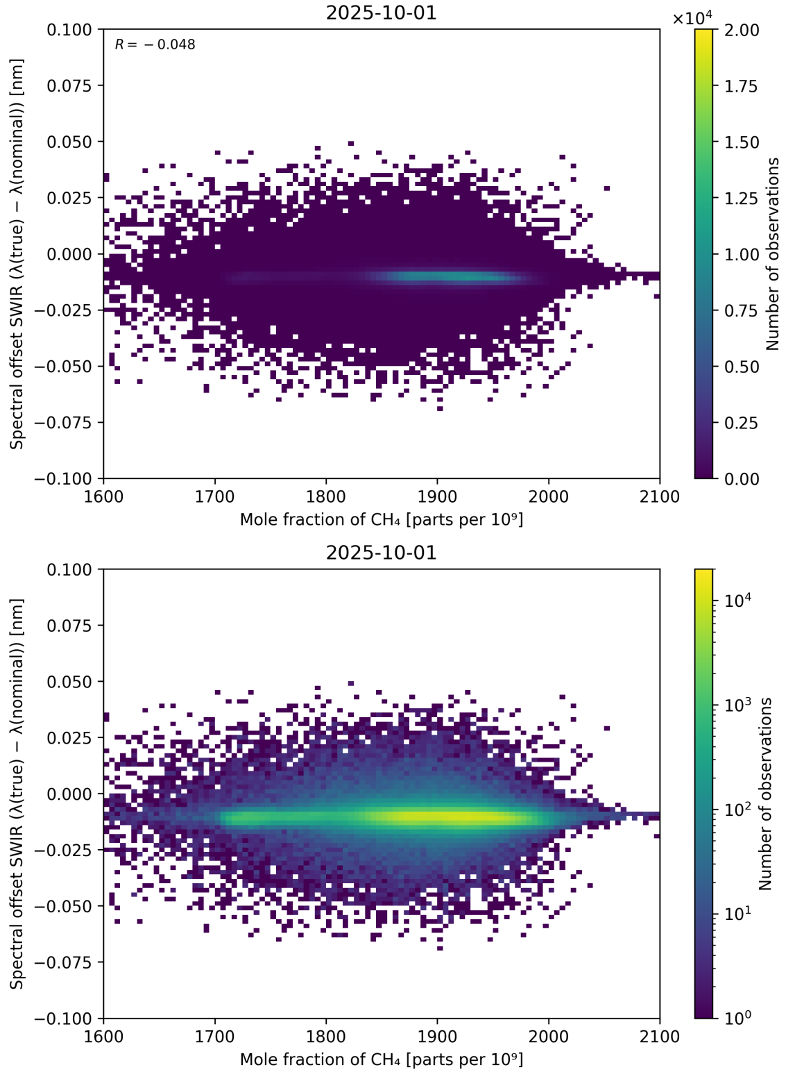
Figure 86: Scatter density plot of “Mole fraction of \text{CH}_4 ” against “Spectral offset SWIR ( \lambda_{\text{true}} - \lambda_{\text{nominal}} )” for 2025-10-01 to 2025-10-02.
