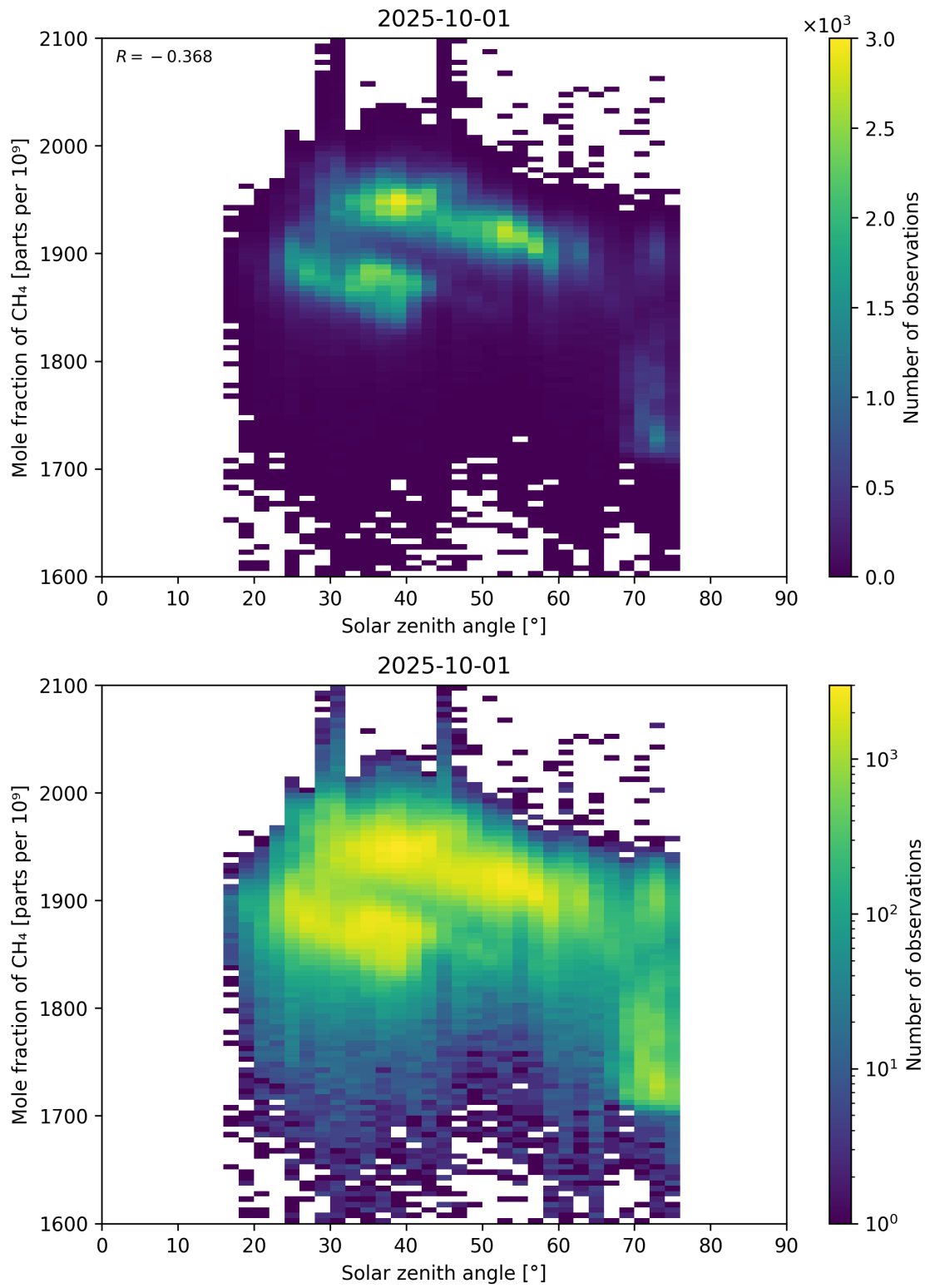
Figure 99: Scatter density plot of “Solar zenith angle” against “Mole fraction of CH 4 ” for 2025-10-01 to 2025-10-02.
