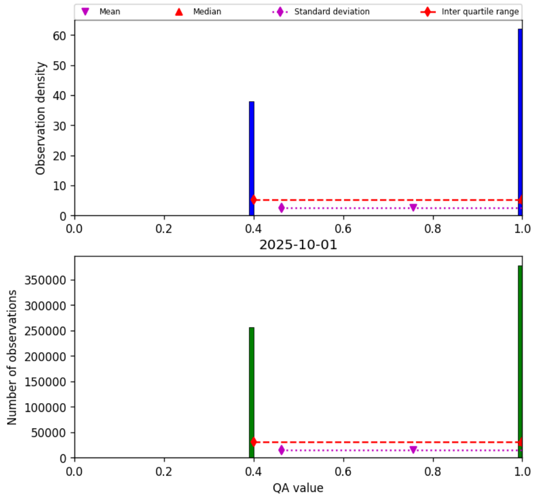
Figure 22: Histogram of “QA value” for 2025-10-01 to 2025-10-02
