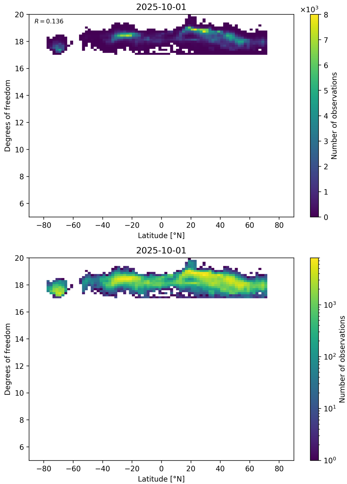
Figure 55: Scatter density plot of “Latitude” against “Degrees of freedom” for 2025-10-01 to 2025-10-02.
