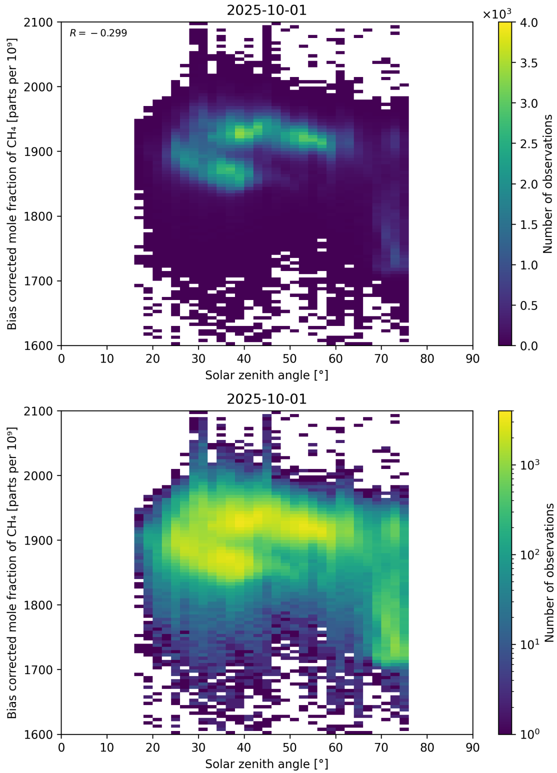
Figure 100: Scatter density plot of “Solar zenith angle” against “Bias corrected mole fraction of CH 4 ” for 2025-10-01 to 2025-10-02.
