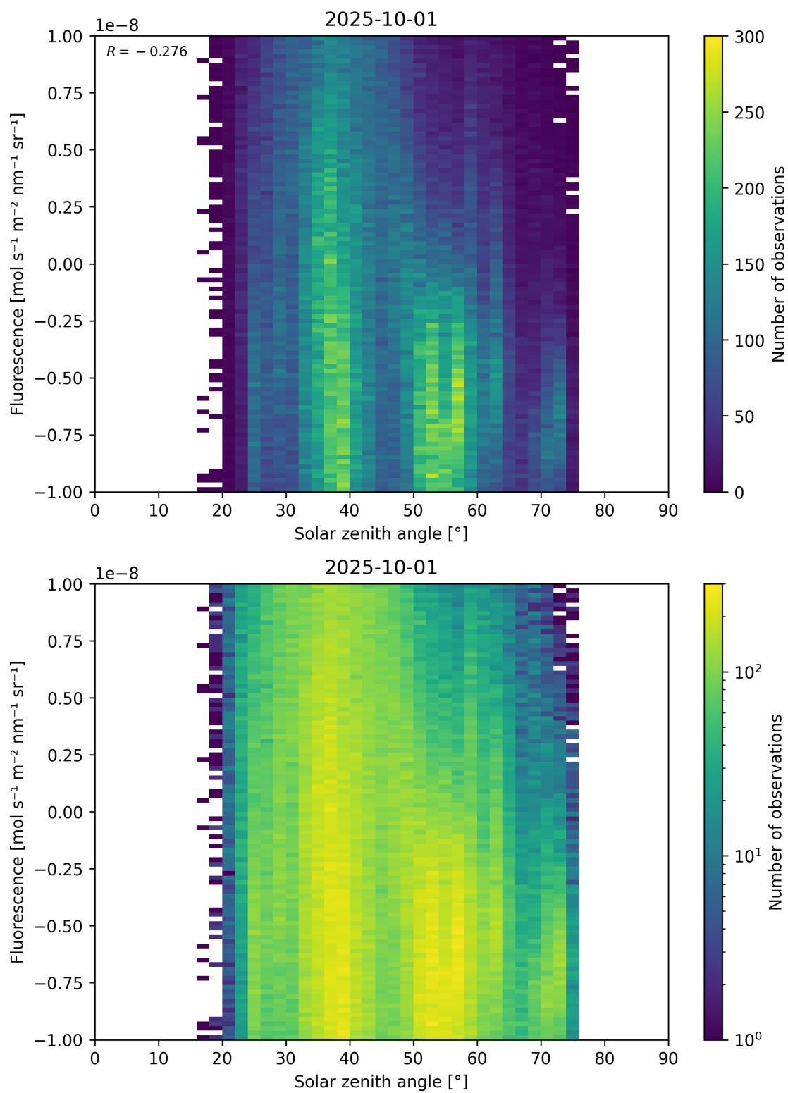
Figure 97: Scatter density plot of “Solar zenith angle” against “Fluorescence” for 2025-10-01 to 2025-10-02.
