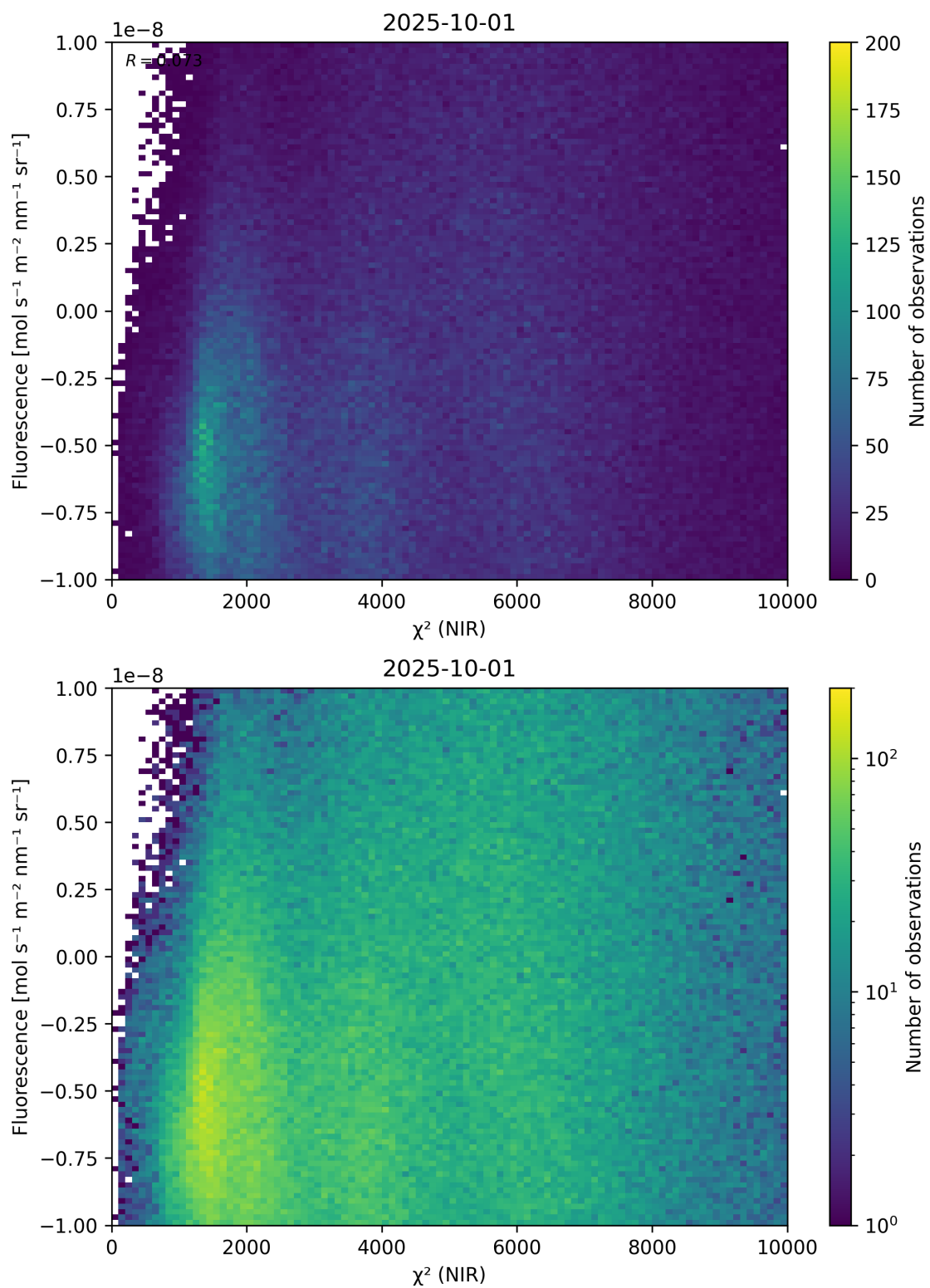
Figure 45: Scatter density plot of “ \chi^2 (NIR)” against “Fluorescence” for 2025-10-01 to 2025-10-02.
