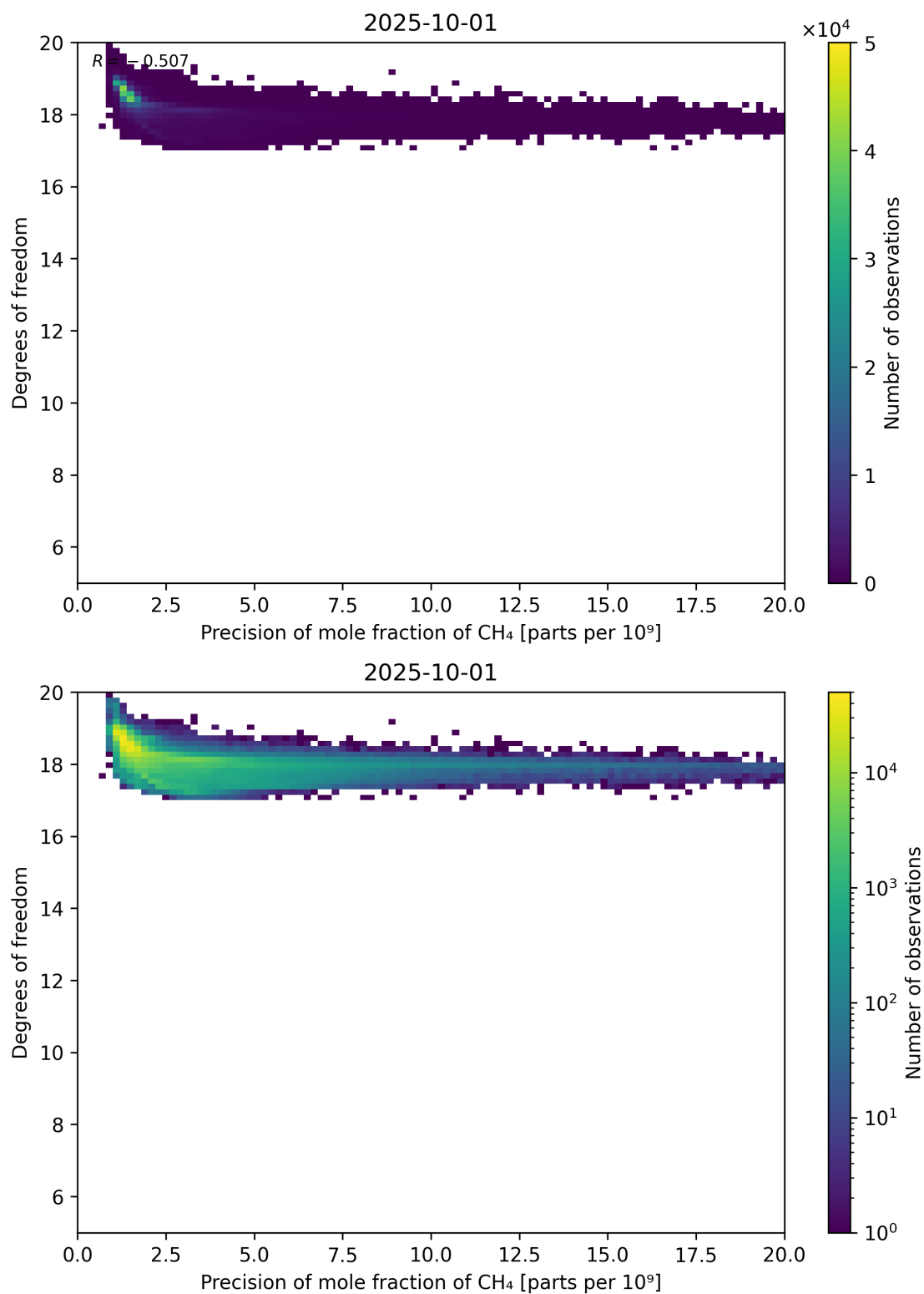
Figure 80: Scatter density plot of “Precision of mole fraction of CH 4 ” against “Degrees of freedom” for 2025-10-01 to 2025-10-02.
