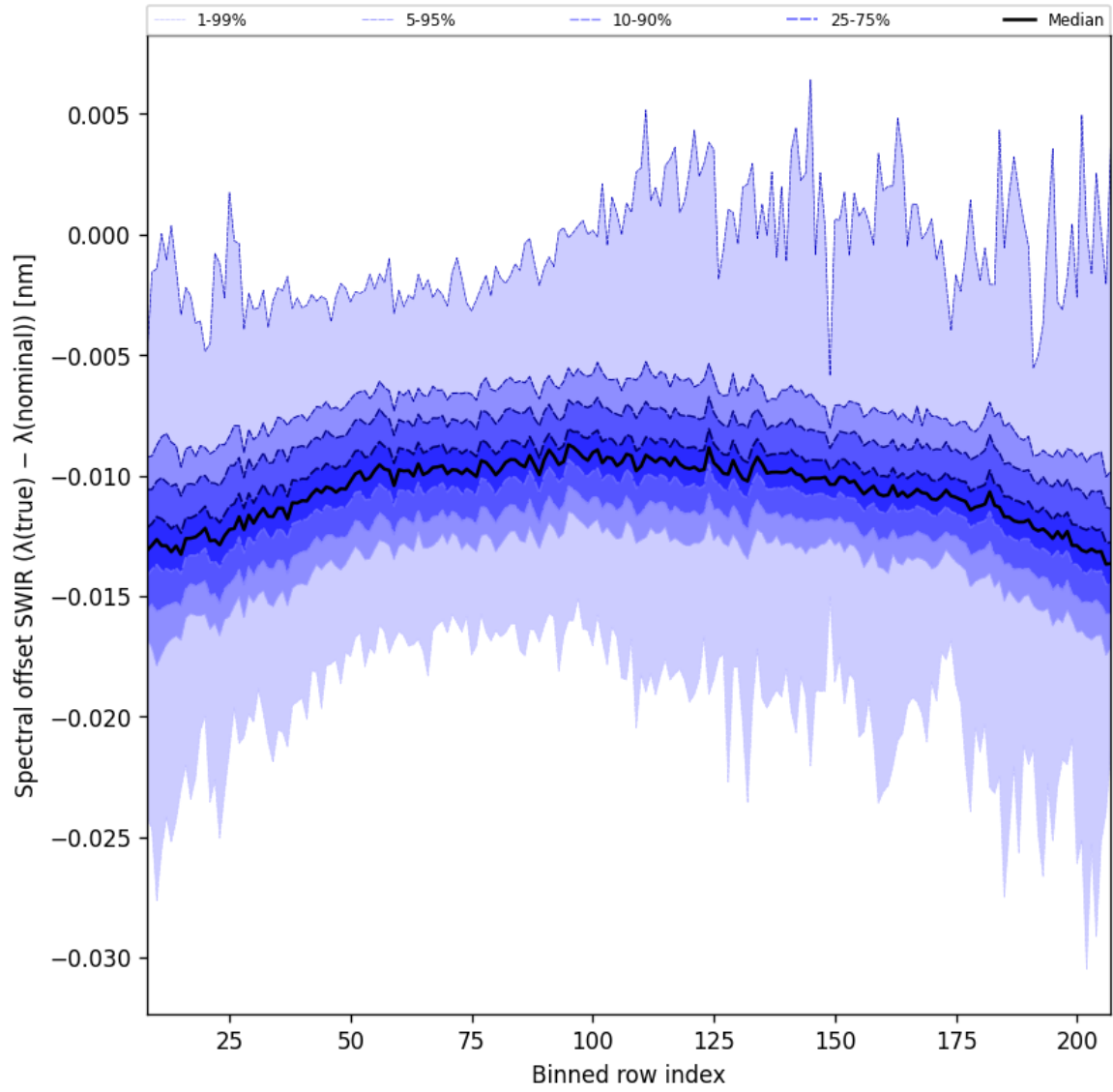
Figure 38: Along track statistics of “Spectral offset SWIR ( \lambda_{\text{true}} - \lambda_{\text{nominal}} )” for 2025-10-01 to 2025-10-02
