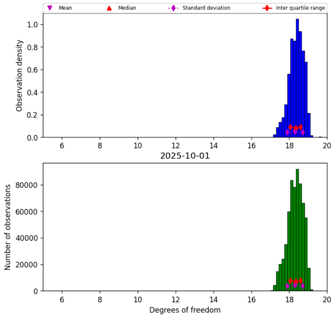
Figure 30: Histogram of “Degrees of freedom” for 2025-10-01 to 2025-10-02
