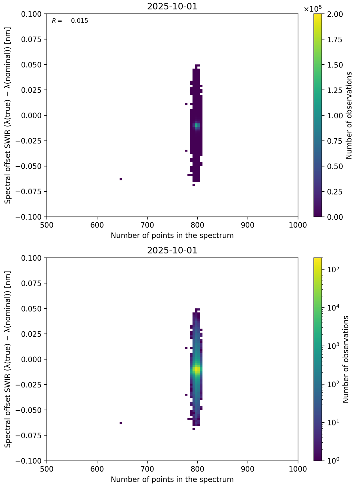
Figure 93: Scatter density plot of “Number of points in the spectrum” against “Spectral offset SWIR ( \lambda_{\text{true}} - \lambda_{\text{nominal}} )” for 2025-10-01 to 2025-10-02.
