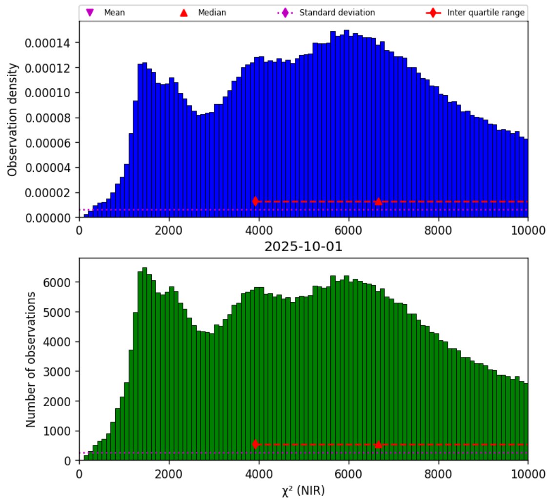
Figure 29: Histogram of " \chi^2 (NIR)" for 2025-10-01 to 2025-10-02
