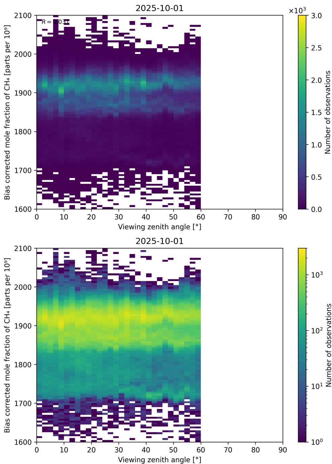
Figure 111: Scatter density plot of “Viewing zenith angle” against “Bias corrected mole fraction of CH 4 ” for 2025-10-01 to 2025-10-02.
