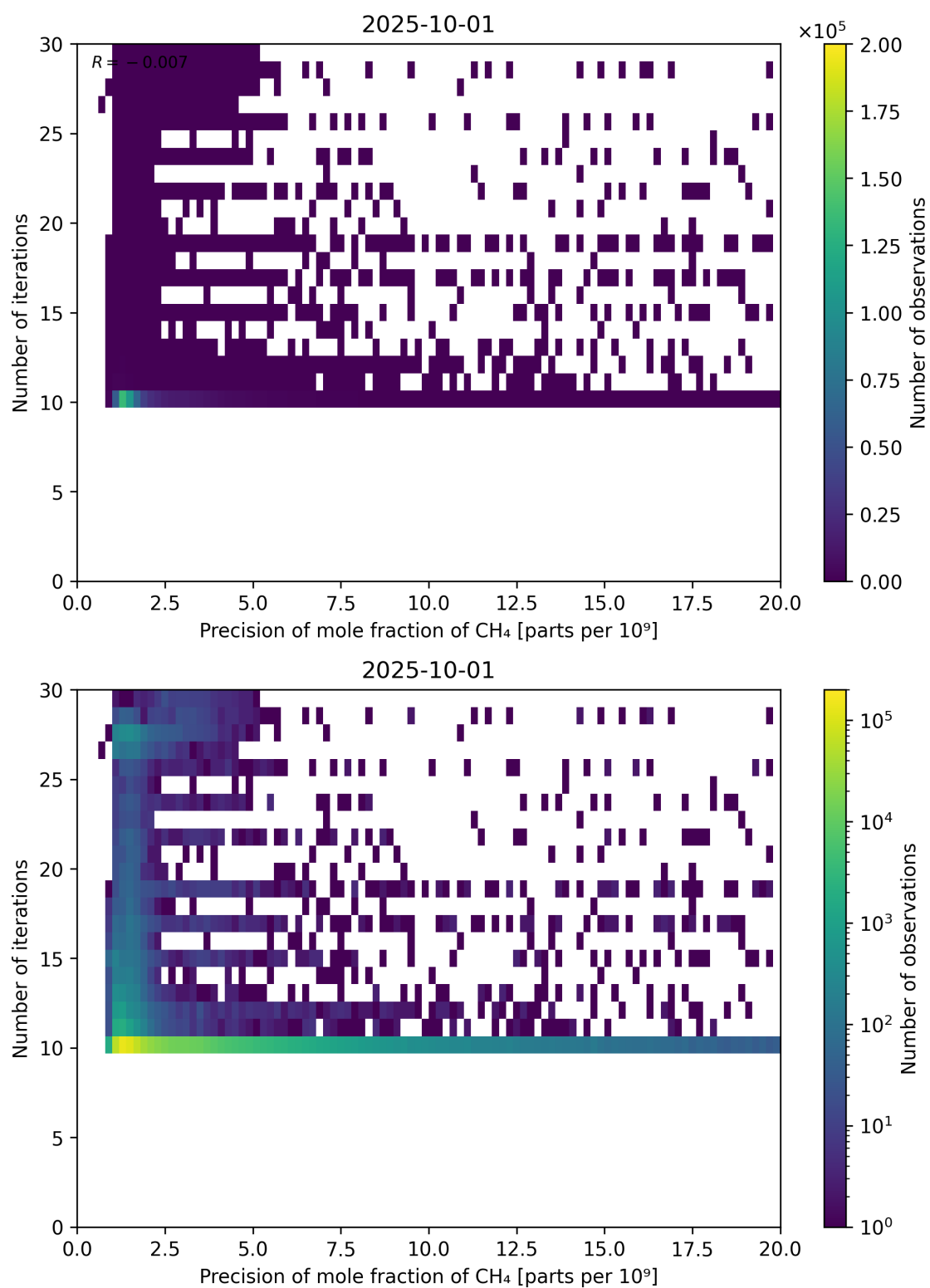
Figure 83: Scatter density plot of “Precision of mole fraction of CH 4 ” against “Number of iterations” for 2025-10-01 to 2025-10-02.
