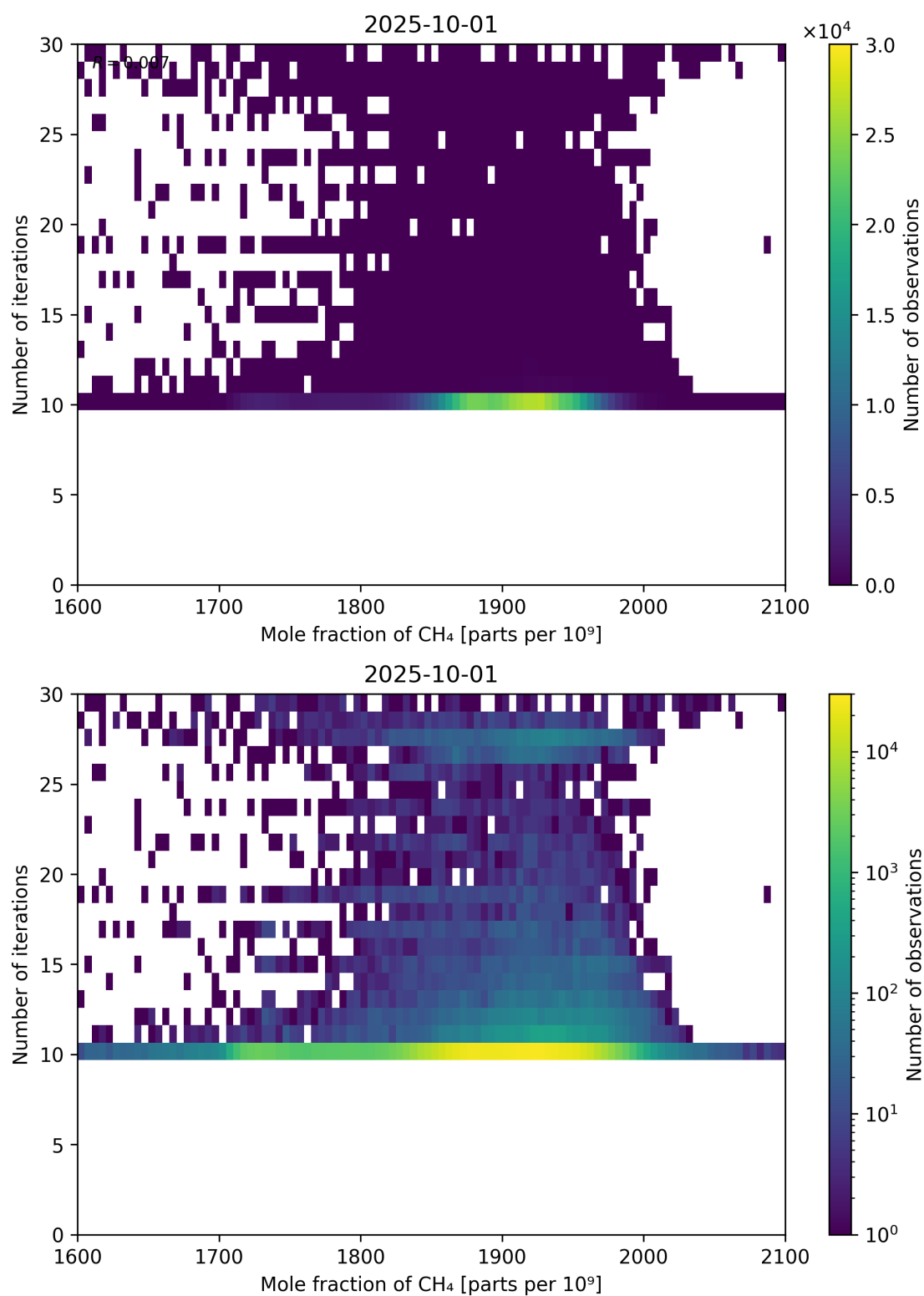
Figure 76: Scatter density plot of “Mole fraction of CH 4 ” against “Number of iterations” for 2025-10-01 to 2025-10-02.
