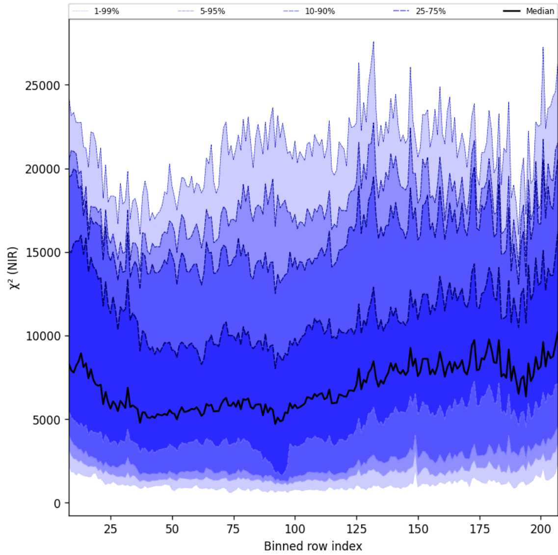
Figure 40: Along track statistics of “ \chi^2 (NIR)” for 2025-10-01 to 2025-10-02
