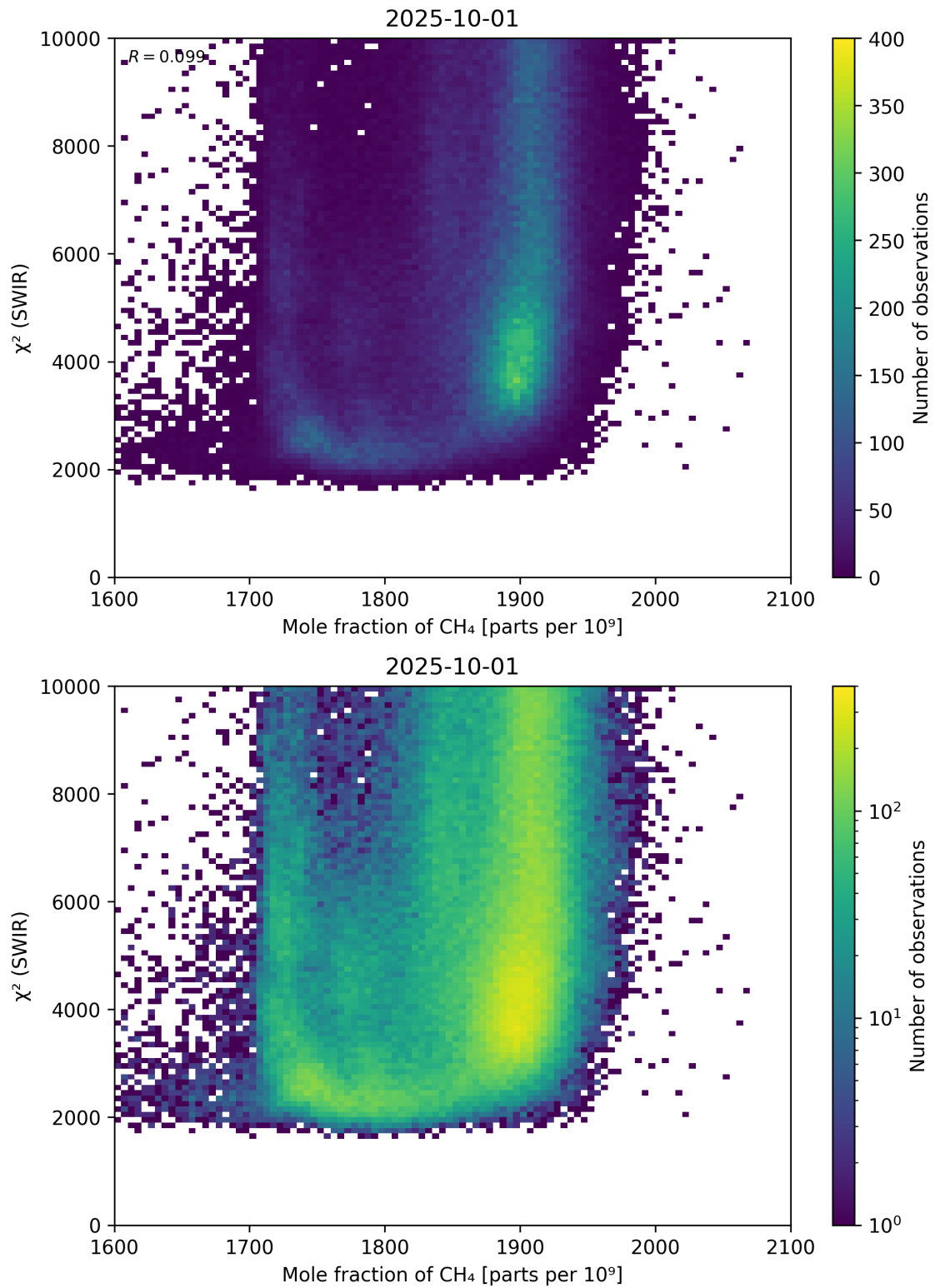
Figure 71: Scatter density plot of “Mole fraction of \text{CH}_4 ” against “ \chi^2 (SWIR)” for 2025-10-01 to 2025-10-02.
