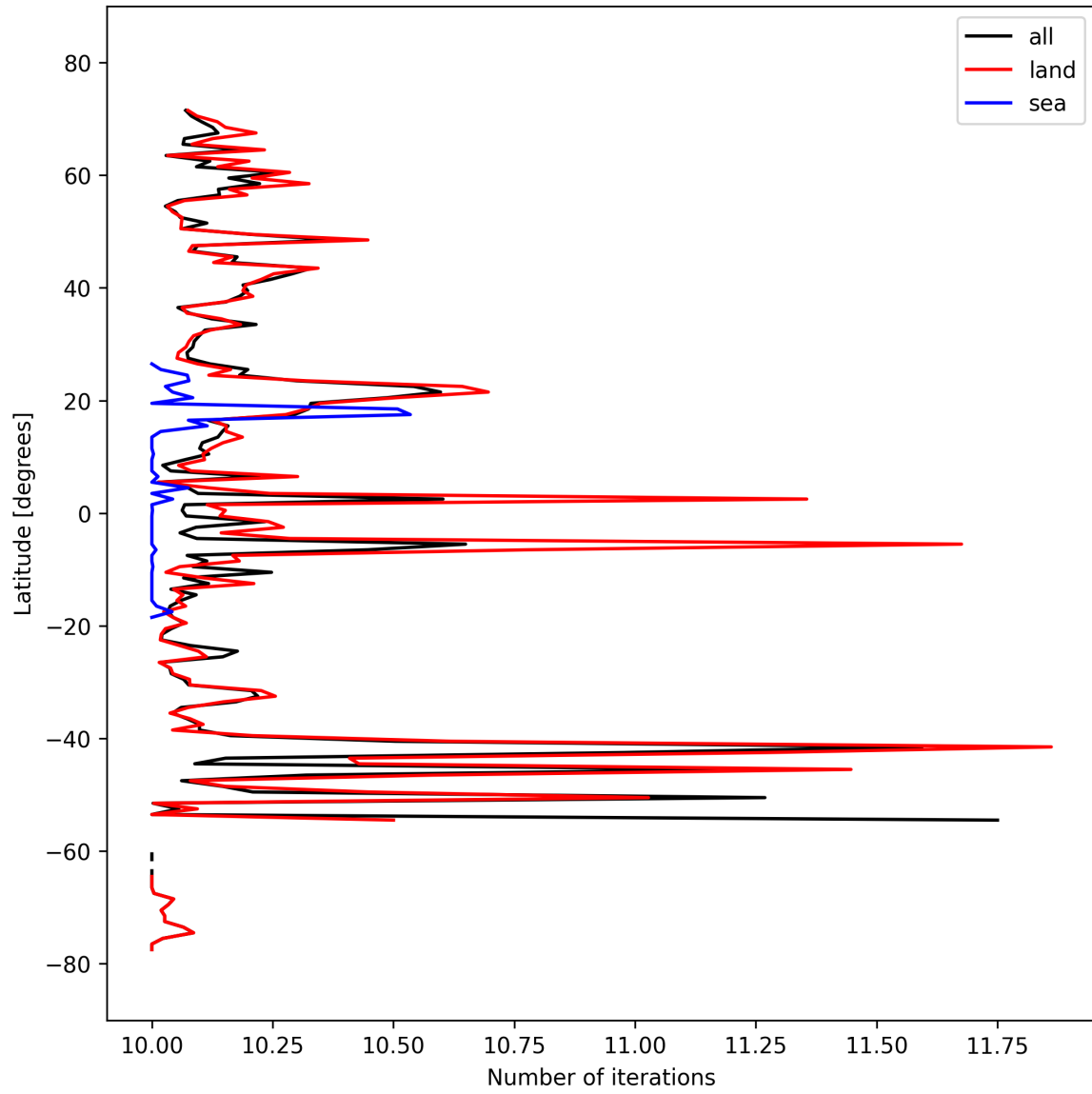
Figure 20: Zonal average of “Number of iterations” for 2025-10-01 to 2025-10-02.
