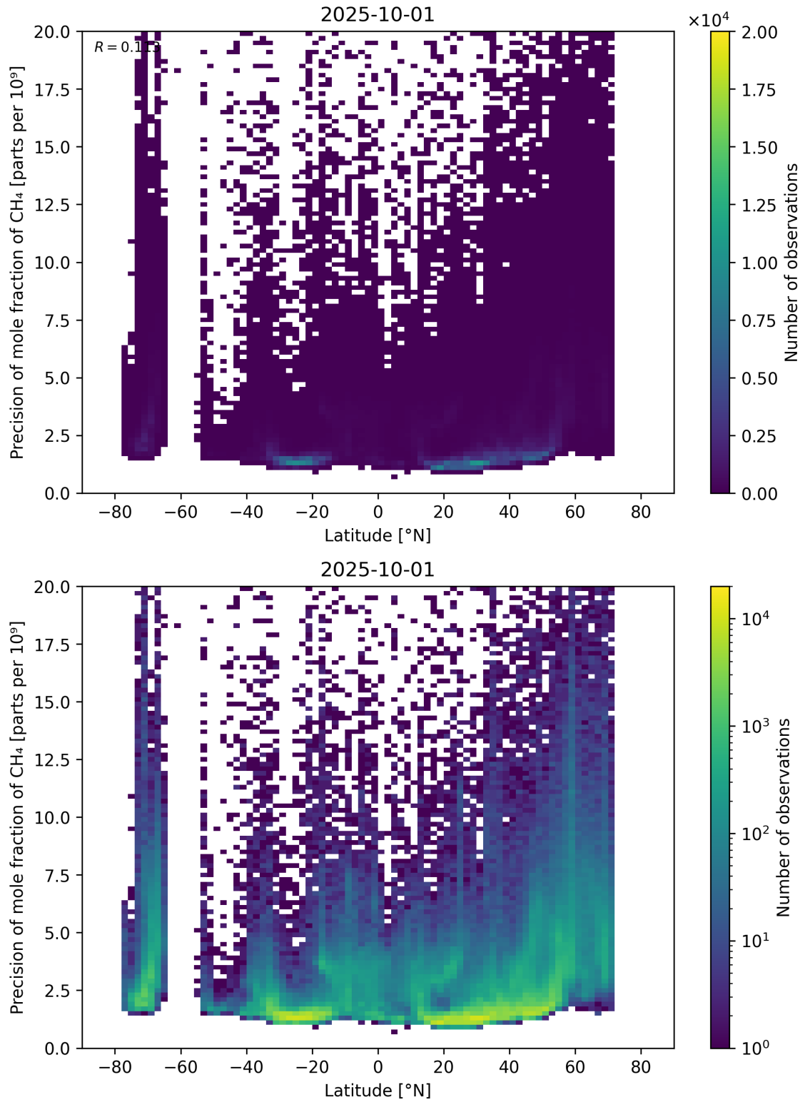
Figure 59: Scatter density plot of “Latitude” against “Precision of mole fraction of CH 4 ” for 2025-10-01 to 2025-10-02.
