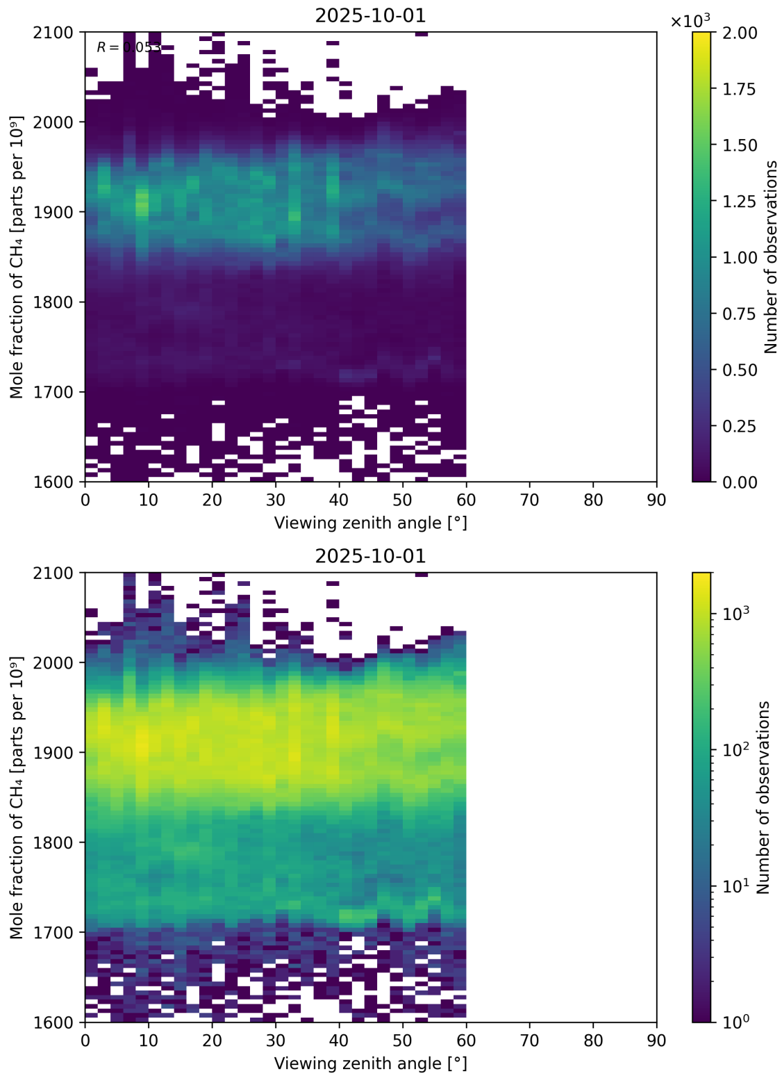
Figure 110: Scatter density plot of “Viewing zenith angle” against “Mole fraction of CH 4 ” for 2025-10-01 to 2025-10-02.
