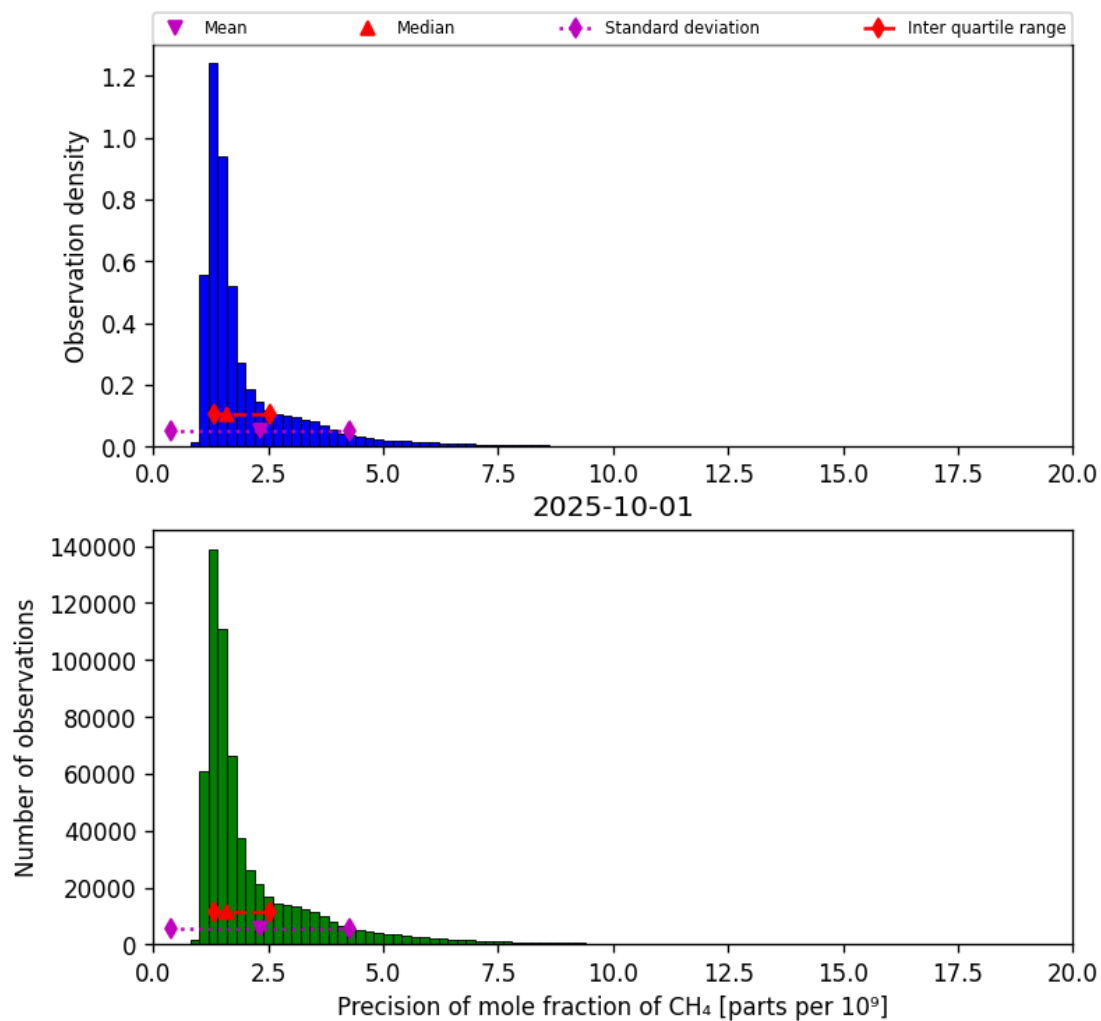
Figure 24: Histogram of “Precision of mole fraction of CH 4 ” for 2025-10-01 to 2025-10-02
