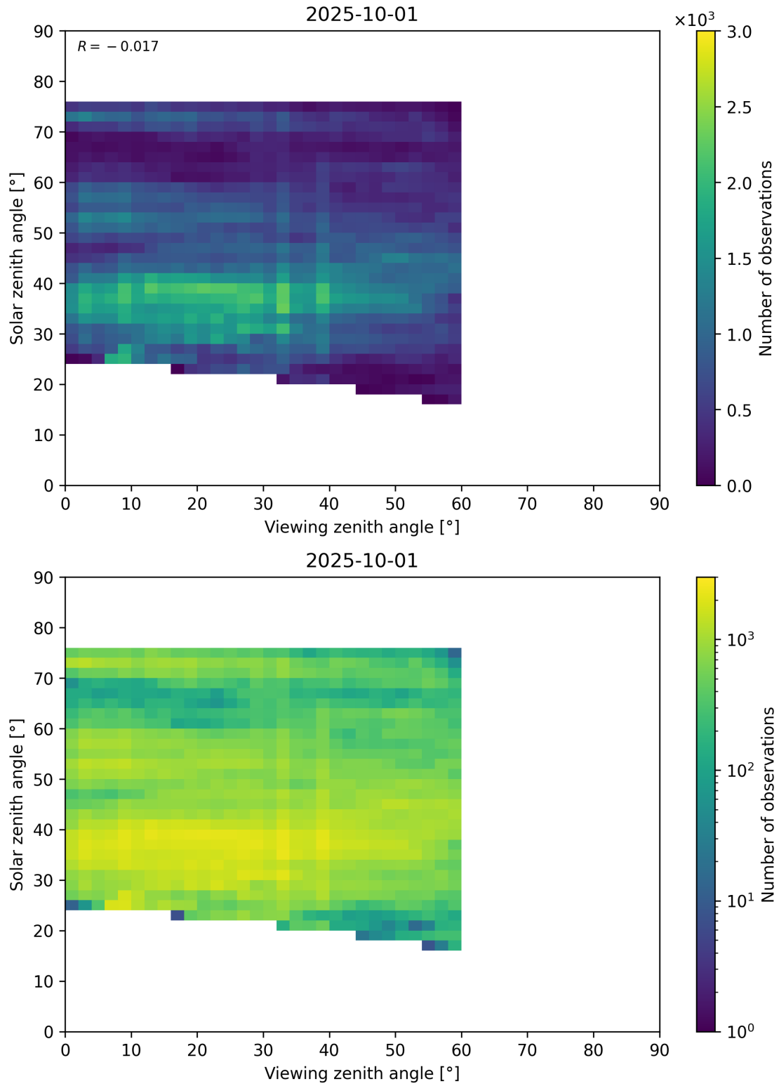
Figure 115: Scatter density plot of “Viewing zenith angle” against “Solar zenith angle” for 2025-10-01 to 2025-10-02.
