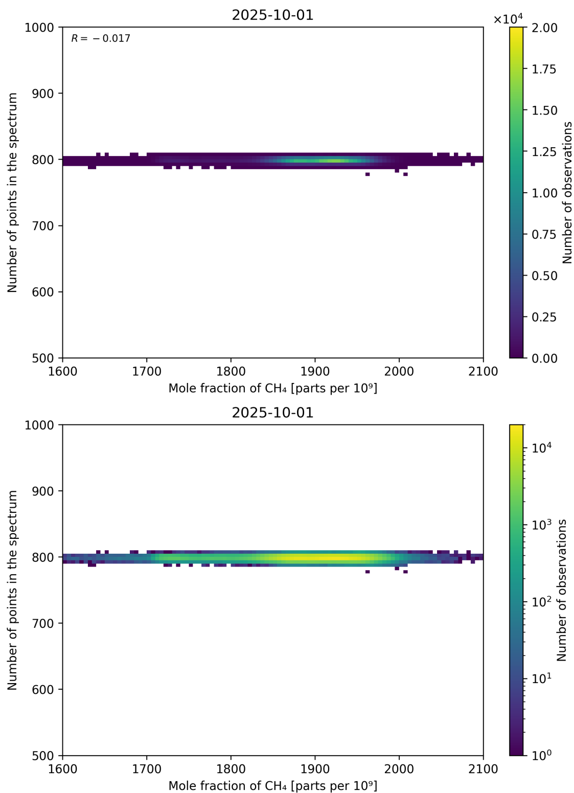
Figure 77: Scatter density plot of “Mole fraction of CH 4 ” against “Number of points in the spectrum” for 2025-10-01 to 2025-10-02.
