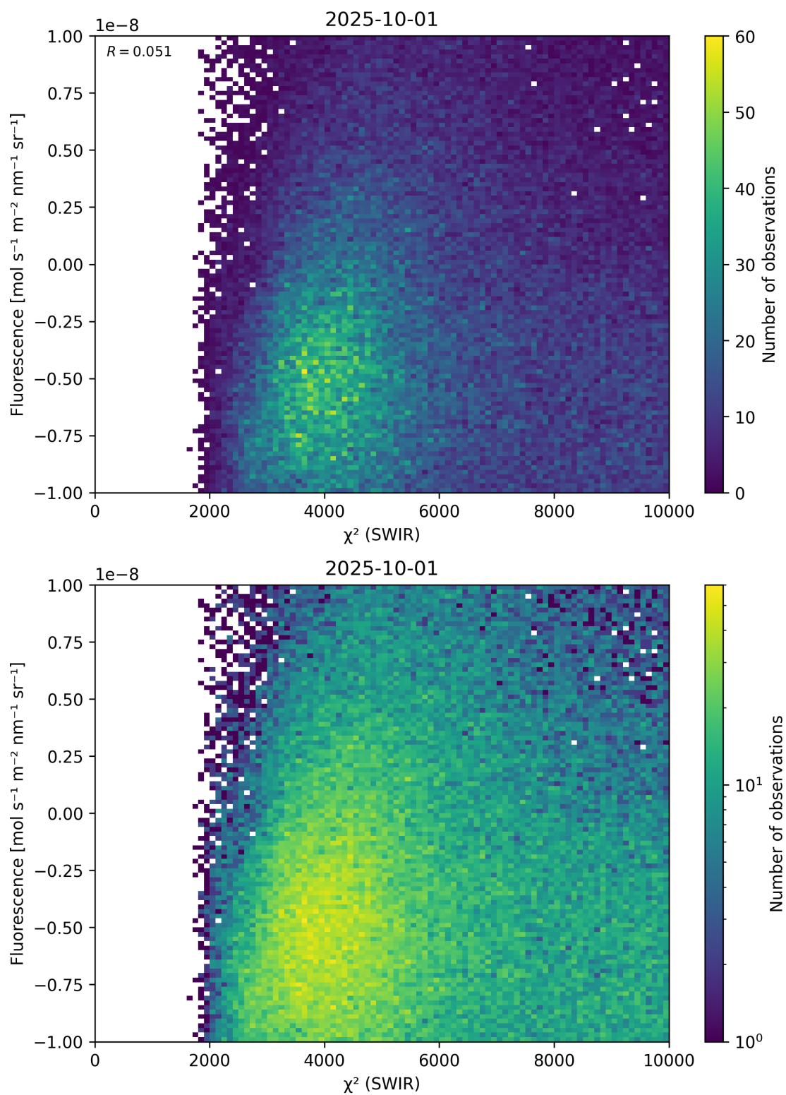
Figure 49: Scatter density plot of “ \chi^2 (SWIR)” against “Fluorescence” for 2025-10-01 to 2025-10-02.
