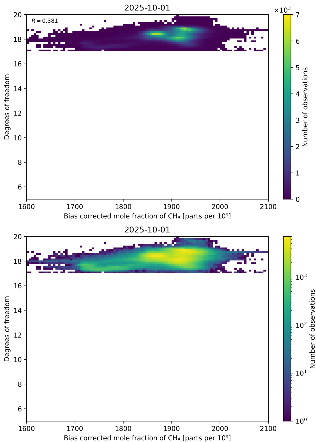
Figure 65: Scatter density plot of “Bias corrected mole fraction of CH 4 ” against “Degrees of freedom” for 2025-10-01 to 2025-10-02.
