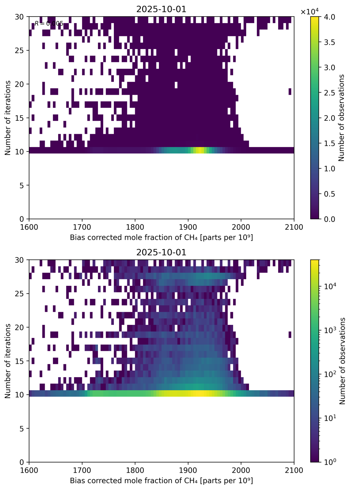
Figure 67: Scatter density plot of “Bias corrected mole fraction of \text{CH}_4 ” against “Number of iterations” for 2025-10-01 to 2025-10-02.
