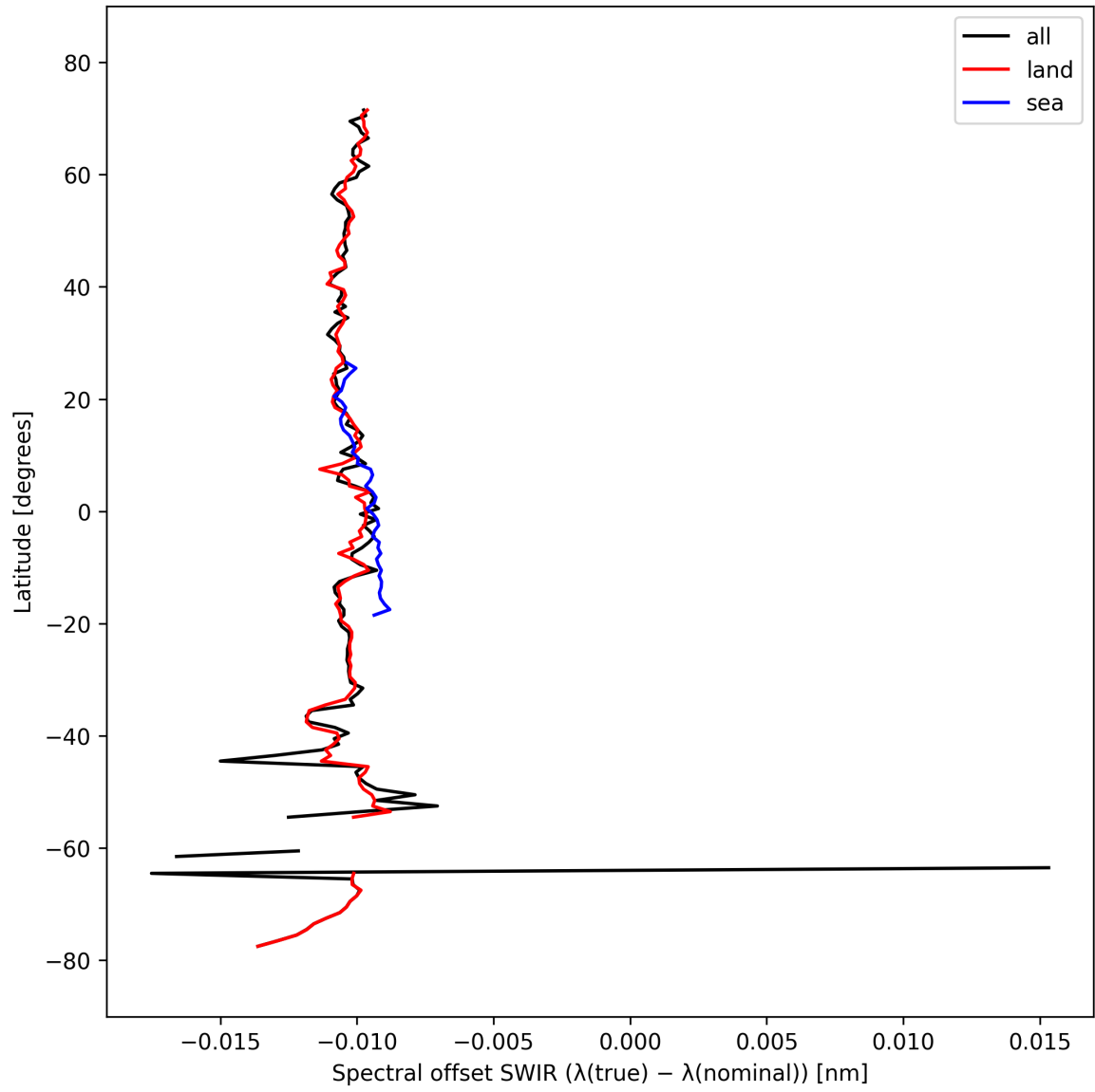
Figure 16: Zonal average of “Spectral offset SWIR ( \lambda_{\text{true}} - \lambda_{\text{nominal}} )” for 2025-10-01 to 2025-10-02.
