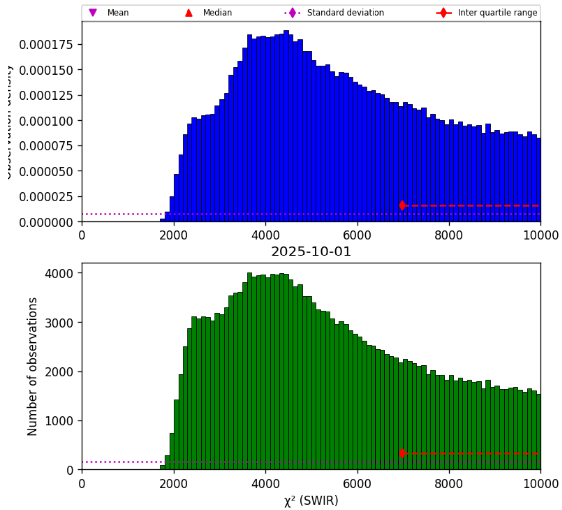
Figure 28: Histogram of “ \chi^2 (SWIR)” for 2025-10-01 to 2025-10-02
