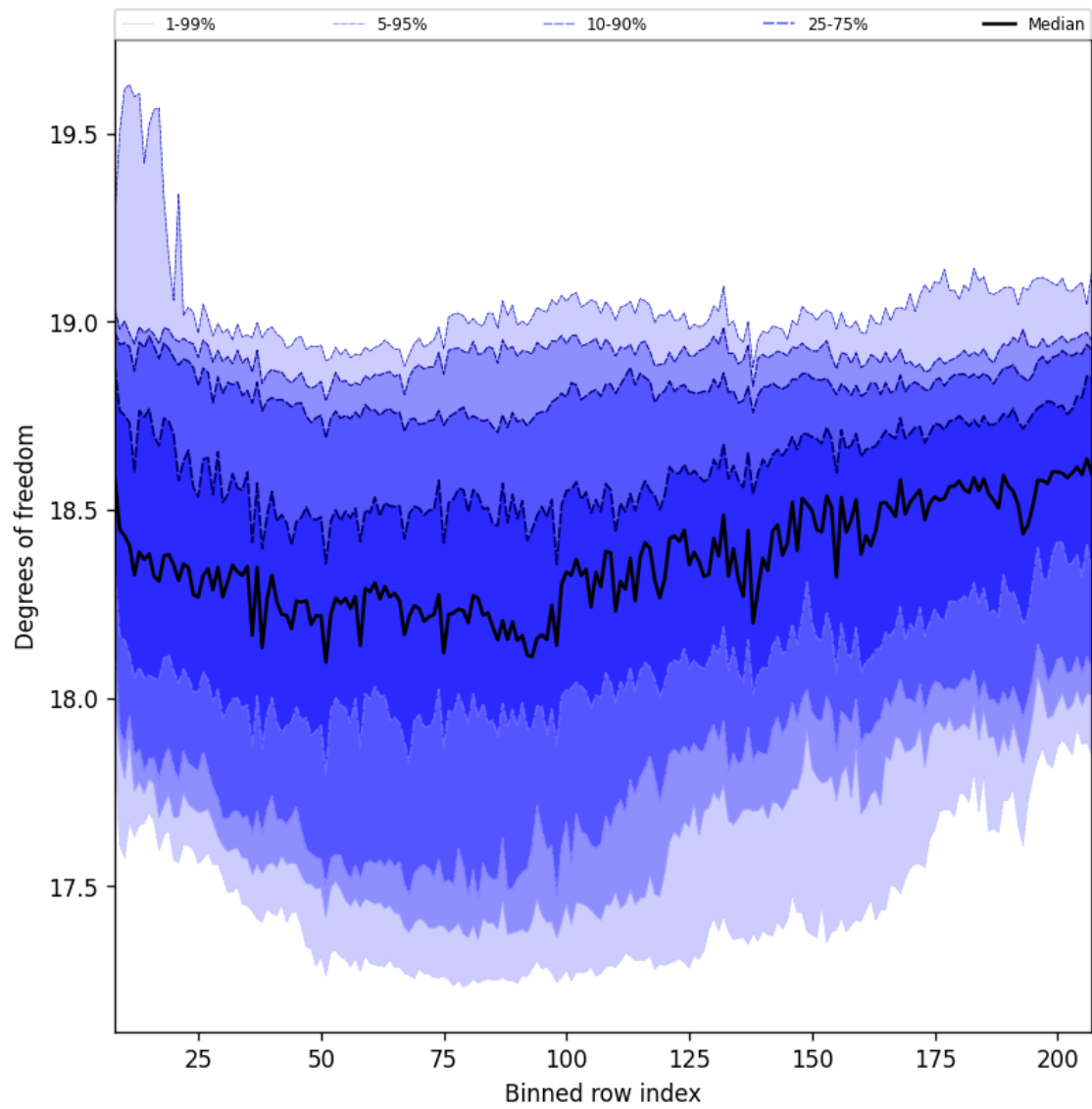
Figure 41: Along track statistics of “Degrees of freedom” for 2025-10-01 to 2025-10-02
