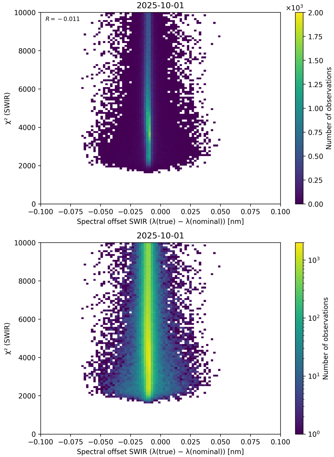
Figure 118: Scatter density plot of “Spectral offset SWIR ( \lambda_{\text{true}} - \lambda_{\text{nominal}} )” against “ \chi^2 (SWIR)” for 2025-10-01 to 2025-10-02.
