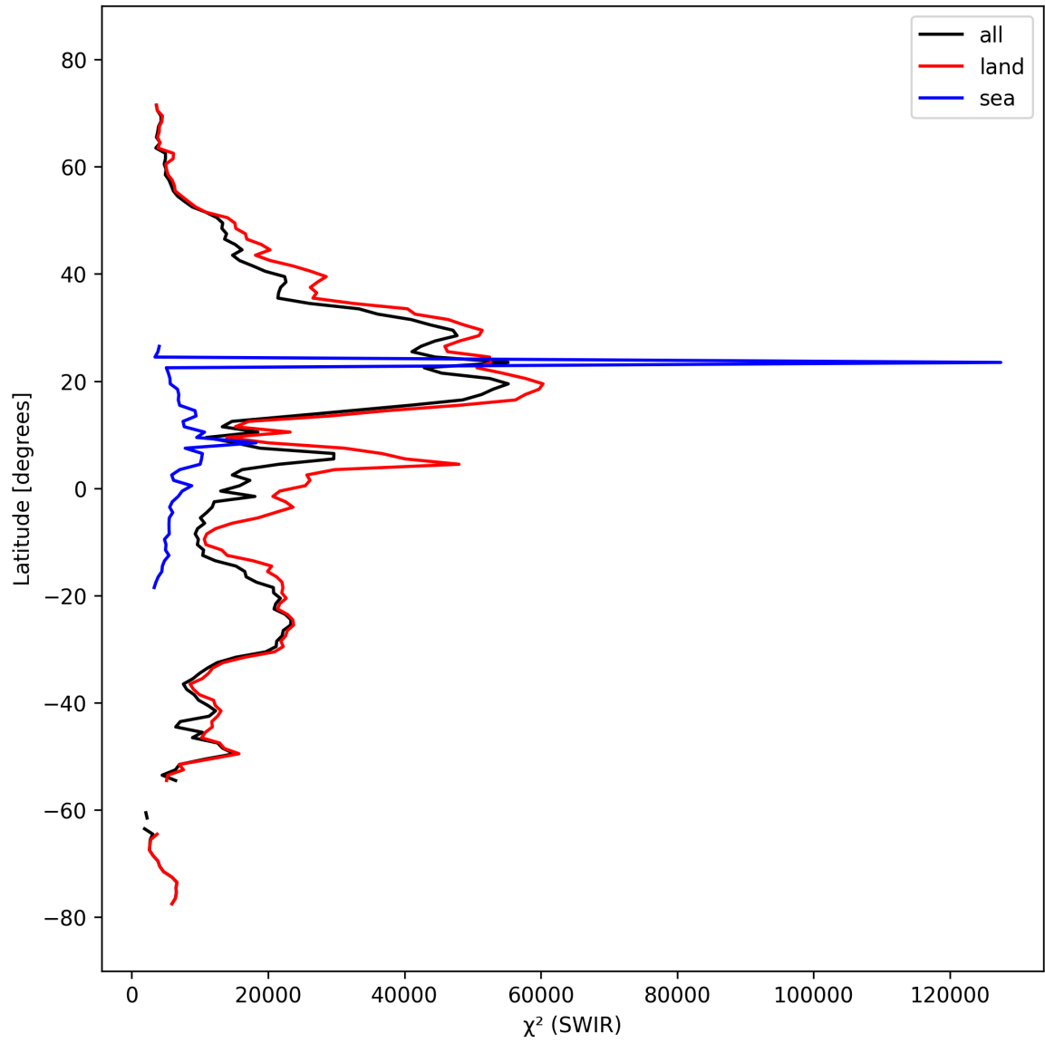
Figure 17: Zonal average of “ \chi^2 (SWIR)” for 2025-10-01 to 2025-10-02.
