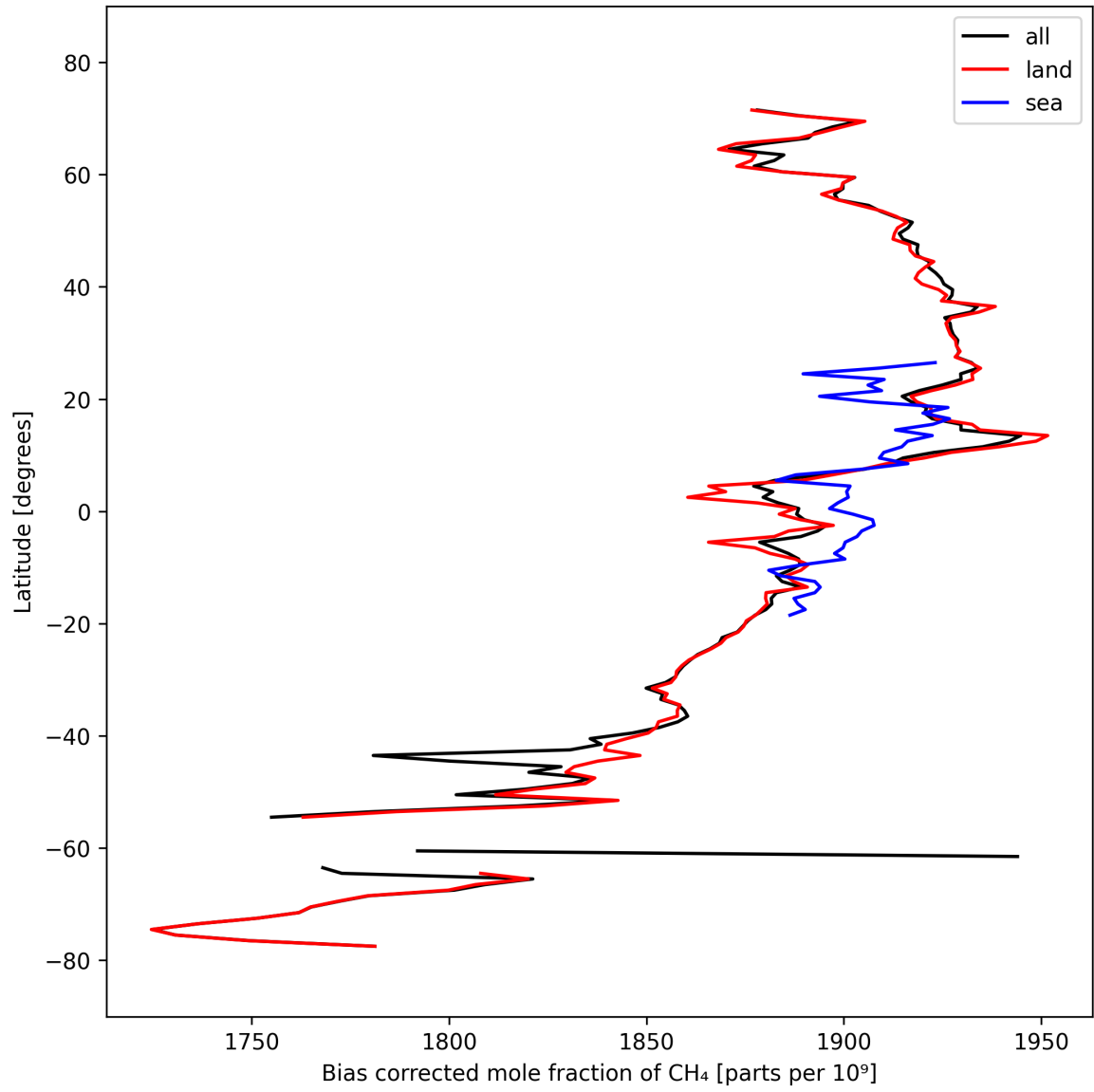
Figure 14: Zonal average of “Bias corrected mole fraction of CH 4 ” for 2025-10-01 to 2025-10-02.
