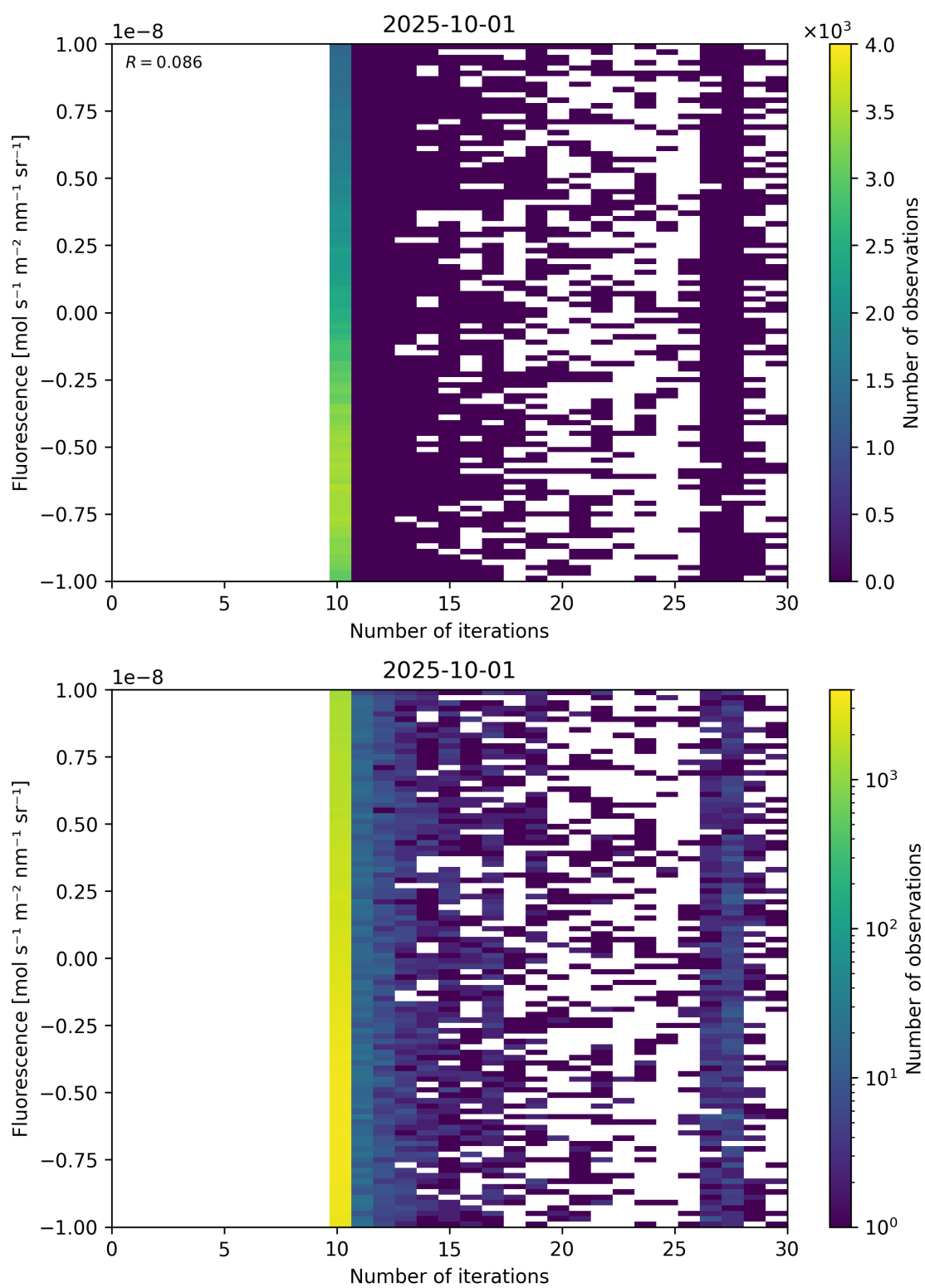
Figure 87: Scatter density plot of “Number of iterations” against “Fluorescence” for 2025-10-01 to 2025-10-02.
