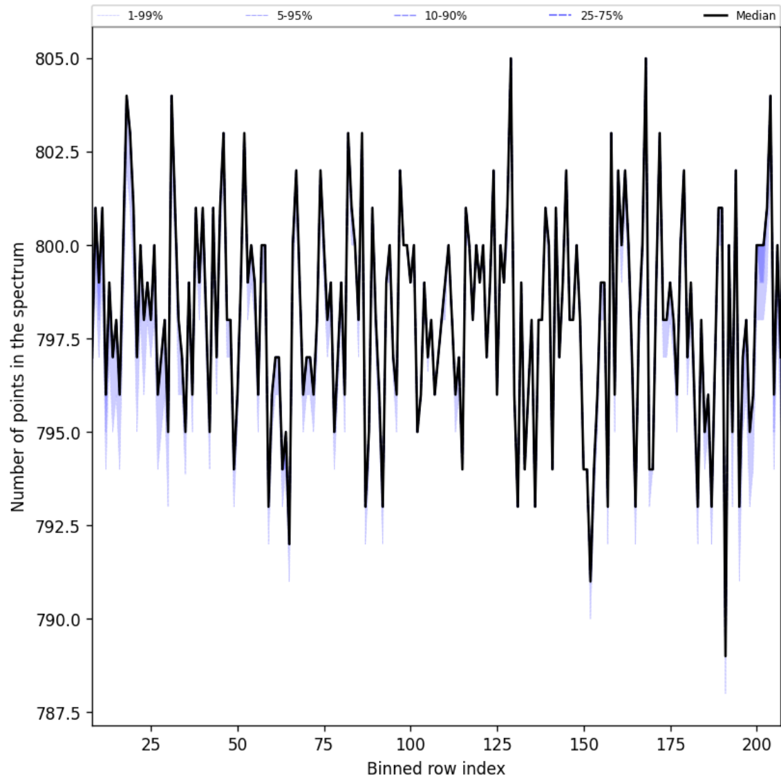
Figure 37: Along track statistics of “Number of points in the spectrum” for 2025-10-01 to 2025-10-02
