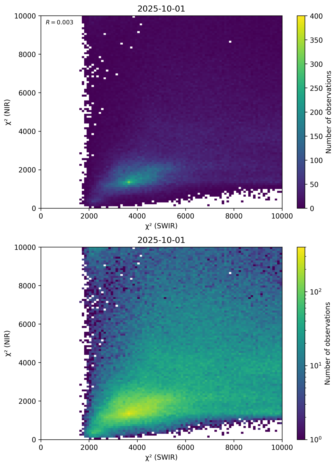
Figure 47: Scatter density plot of “ \chi^2 (SWIR)” against “ \chi^2 (NIR)” for 2025-10-01 to 2025-10-02.
