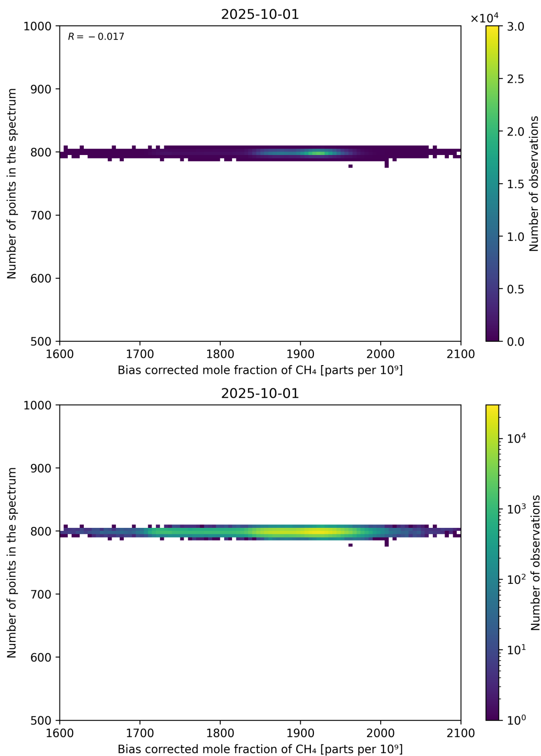
Figure 68: Scatter density plot of “Bias corrected mole fraction of CH 4 ” against “Number of points in the spectrum” for 2025-10-01 to 2025-10-02.
