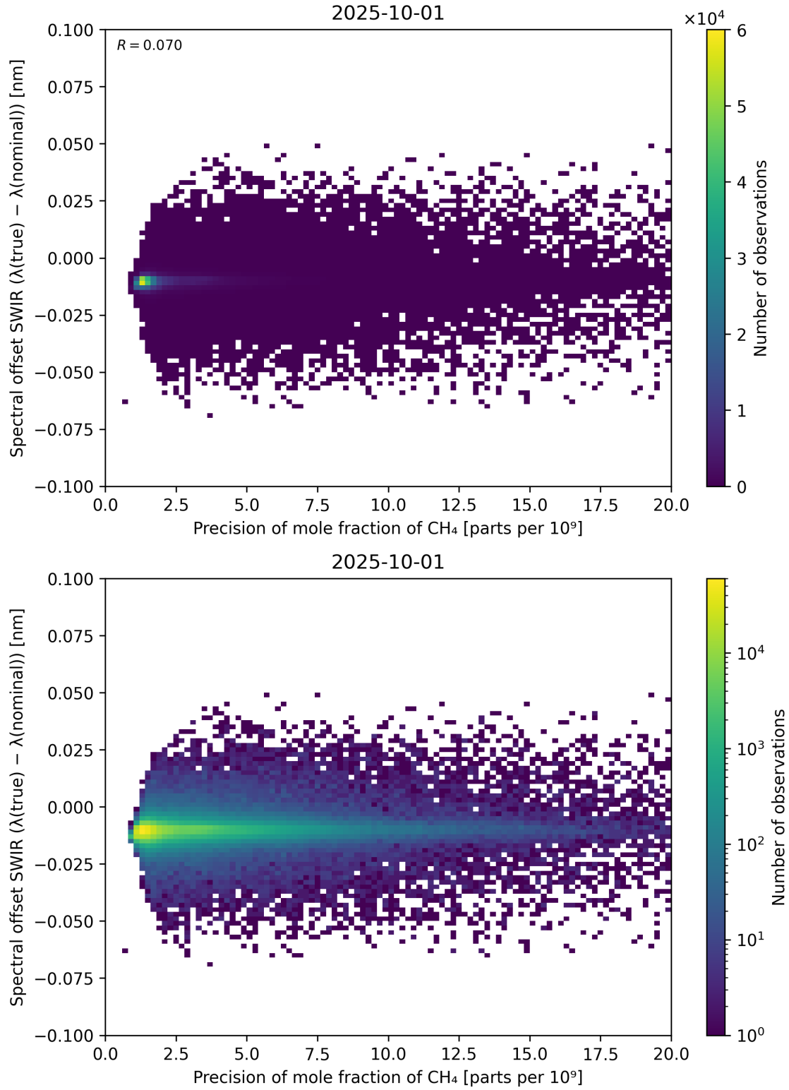
Figure 85: Scatter density plot of “Precision of mole fraction of \text{CH}_4 ” against “Spectral offset SWIR ( \lambda_{\text{true}} - \lambda_{\text{nominal}} )” for 2025-10-01 to 2025-10-02.
