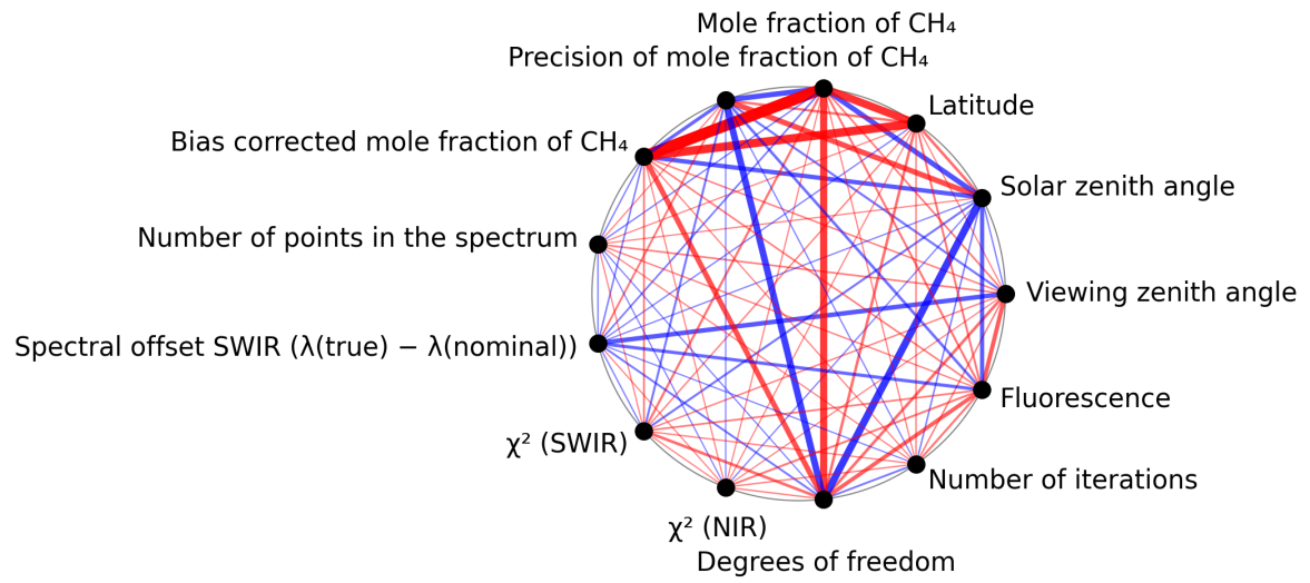
Figure 1: Map of correlation graph for 2025-10-01 to 2025-10-02.
