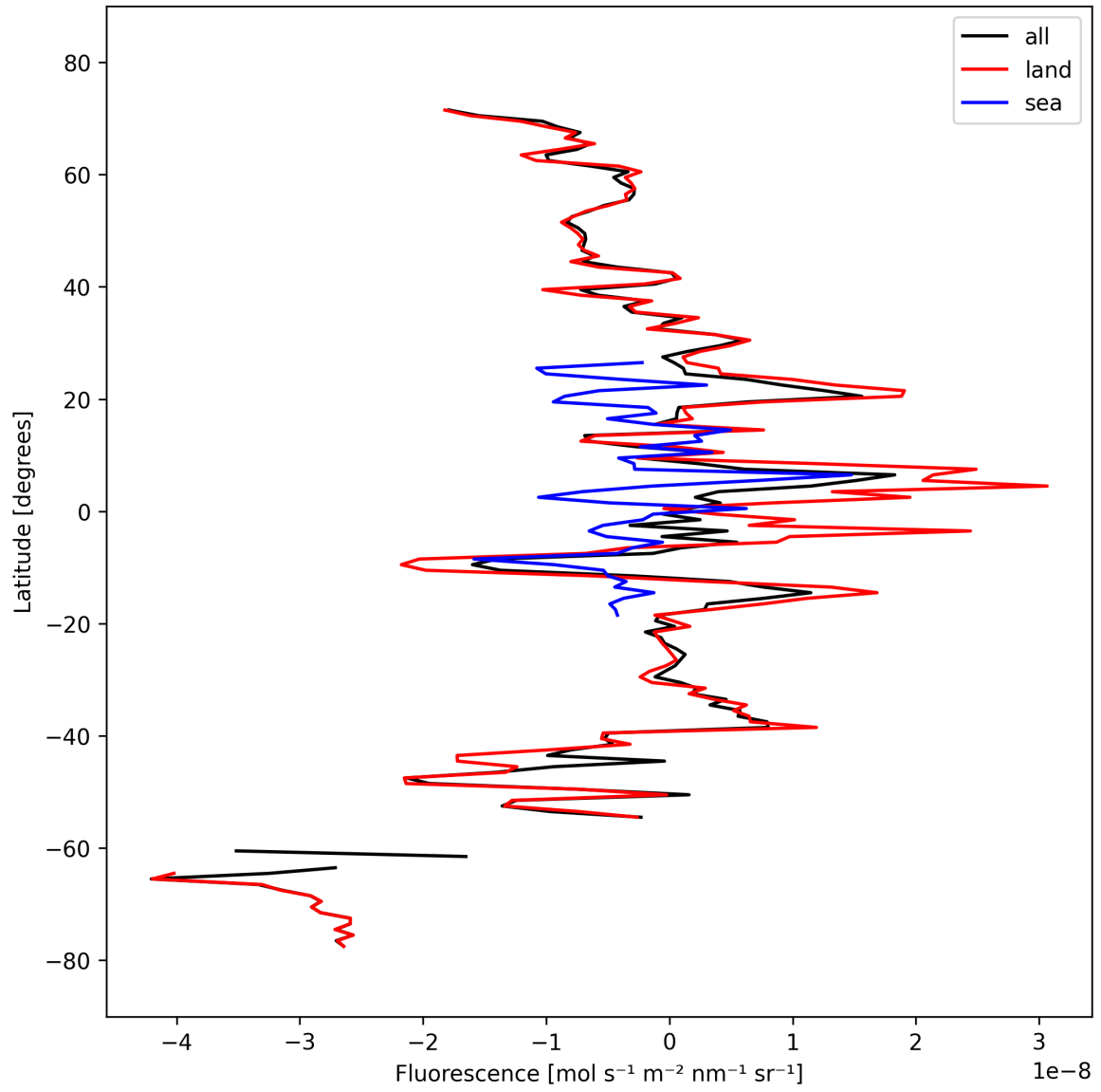
Figure 21: Zonal average of “Fluorescence” for 2025-10-01 to 2025-10-02.
