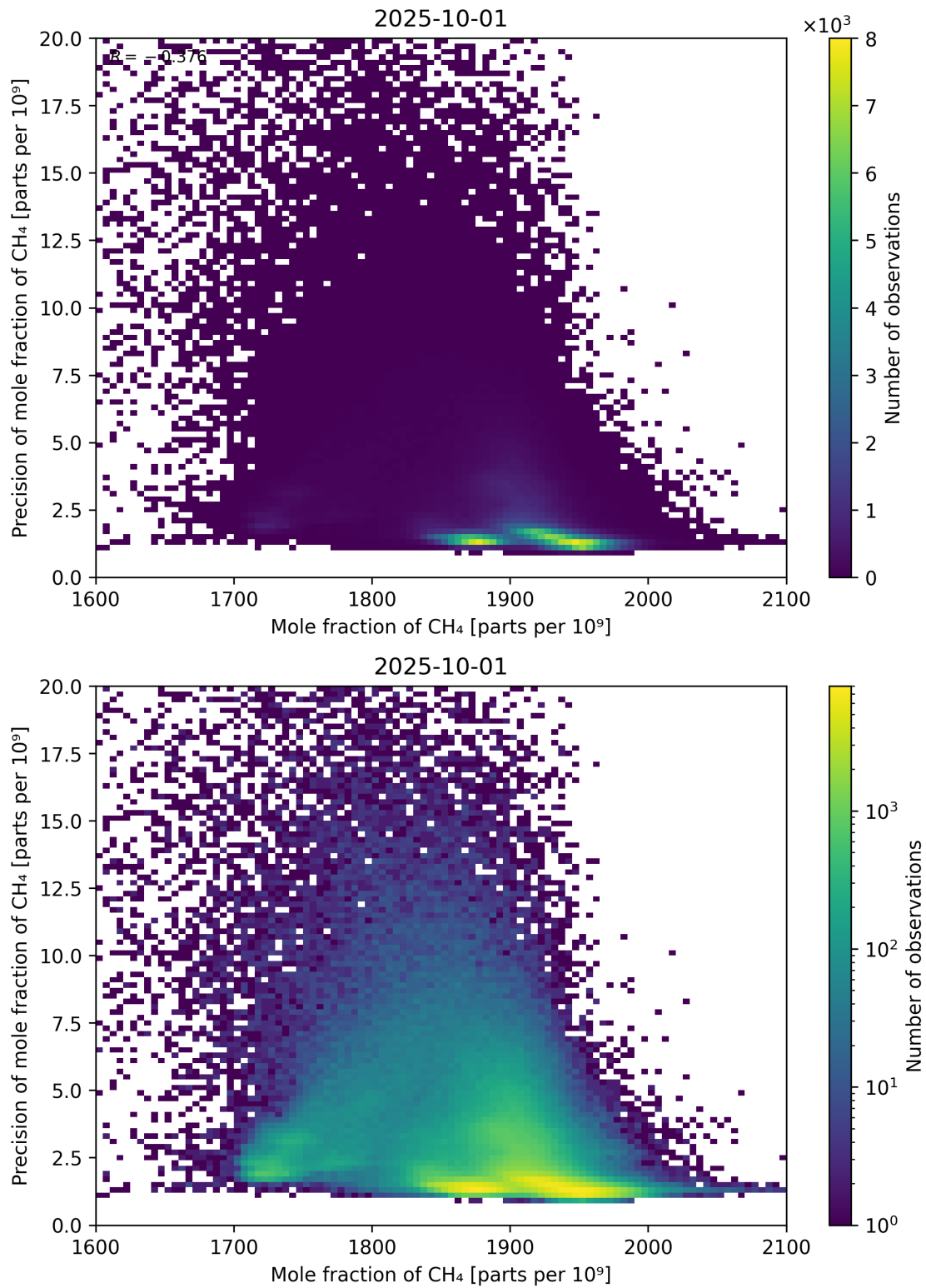
Figure 75: Scatter density plot of “Mole fraction of CH 4 ” against “Precision of mole fraction of CH 4 ” for 2025-10-01 to 2025-10-02.
