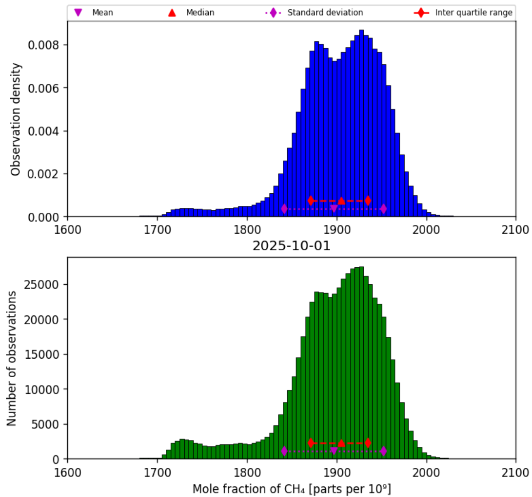
Figure 23: Histogram of “Mole fraction of CH 4 ” for 2025-10-01 to 2025-10-02
