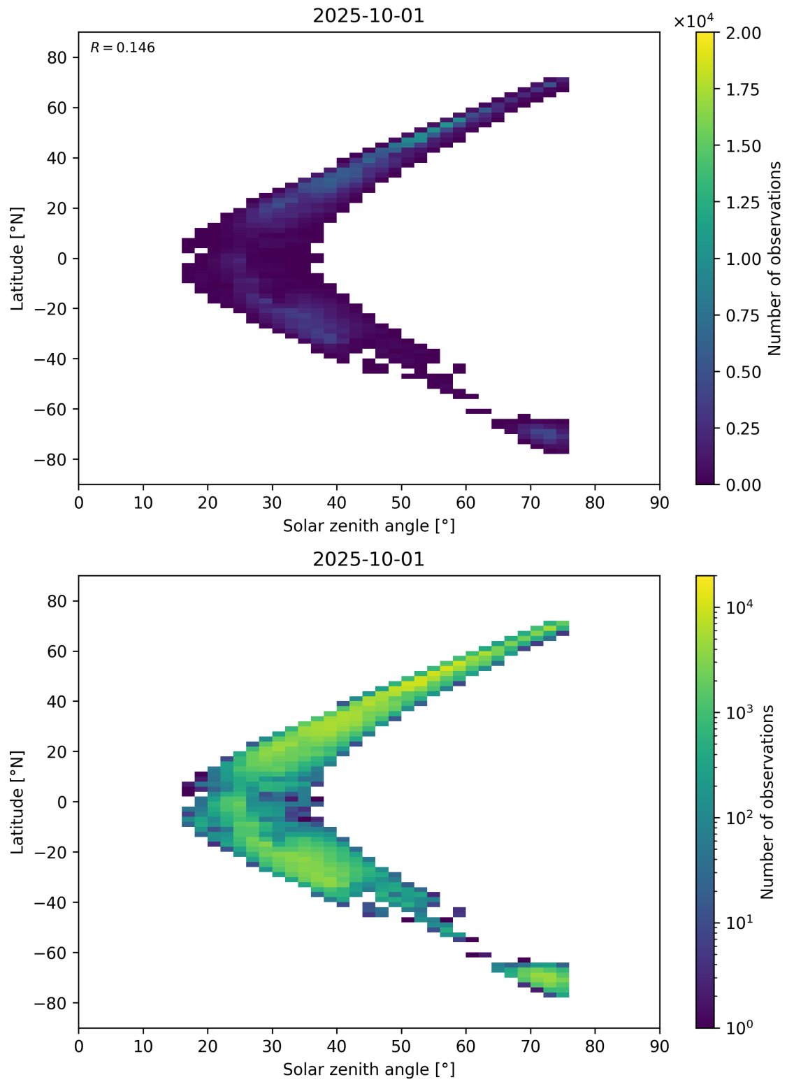
Figure 98: Scatter density plot of “Solar zenith angle” against “Latitude” for 2025-10-01 to 2025-10-02.
