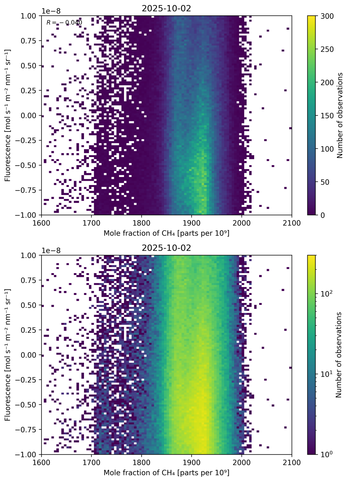
Figure 73: Scatter density plot of “Mole fraction of \text{CH}_4 ” against “Fluorescence” for 2025-10-01 to 2025-10-03.
