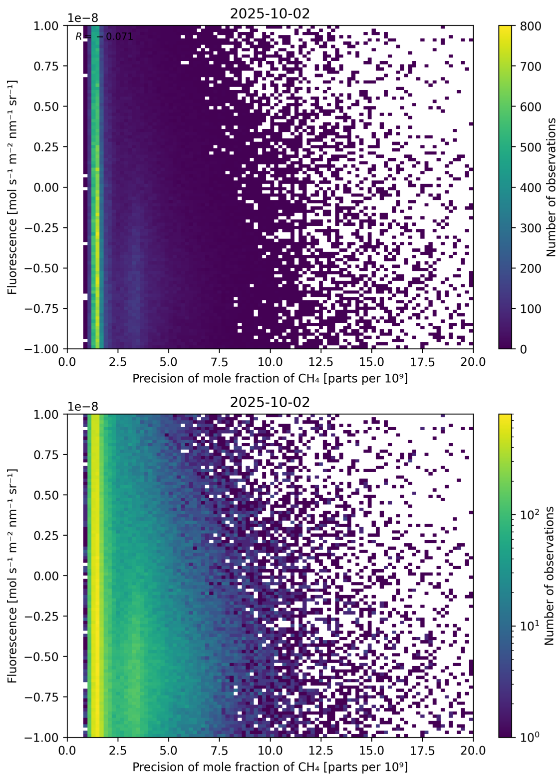
Figure 81: Scatter density plot of “Precision of mole fraction of \text{CH}_4 ” against “Fluorescence” for 2025-10-01 to 2025-10-03.
