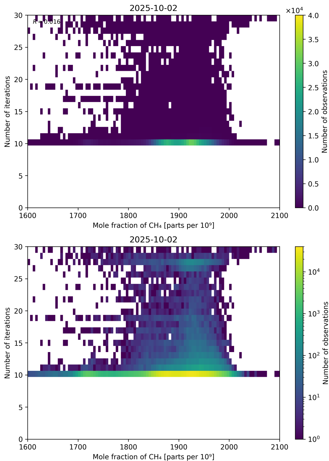
Figure 76: Scatter density plot of “Mole fraction of CH 4 ” against “Number of iterations” for 2025-10-01 to 2025-10-03.
