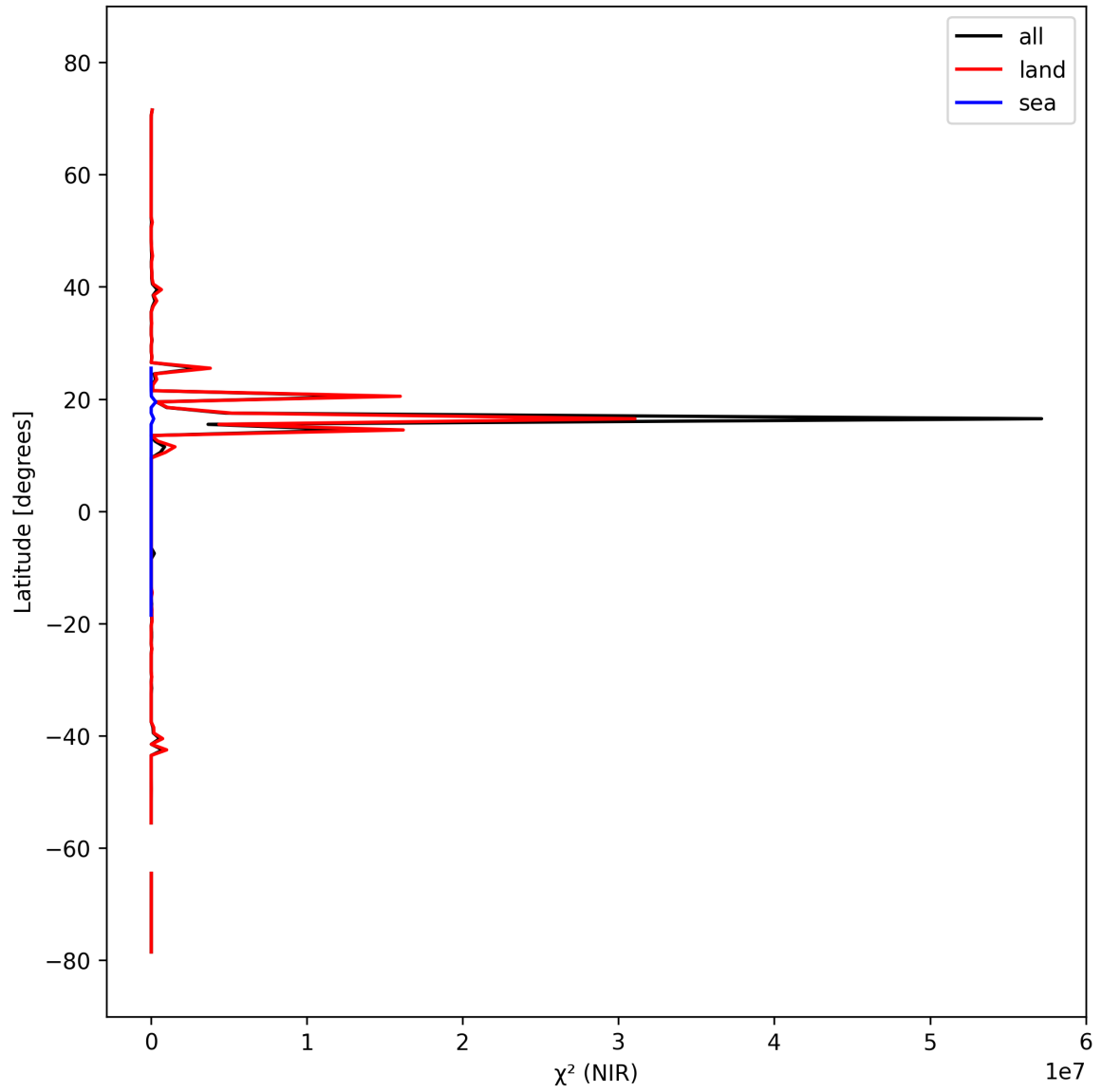
Figure 18: Zonal average of “ \chi^2 (NIR)” for 2025-10-01 to 2025-10-03.
