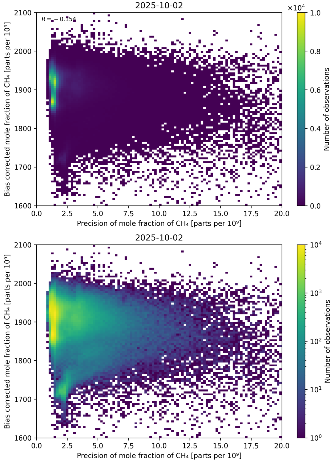
Figure 82: Scatter density plot of “Precision of mole fraction of \text{CH}_4 ” against “Bias corrected mole fraction of \text{CH}_4 ” for 2025-10-01 to 2025-10-03.
