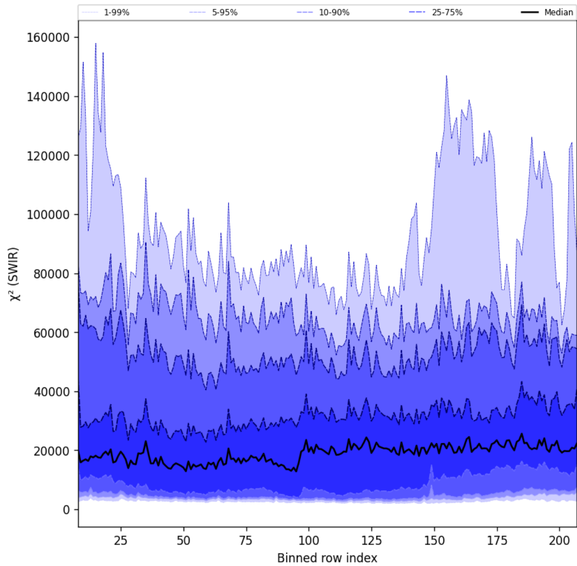
Figure 39: Along track statistics of “ \chi^2 (SWIR)” for 2025-10-01 to 2025-10-03
