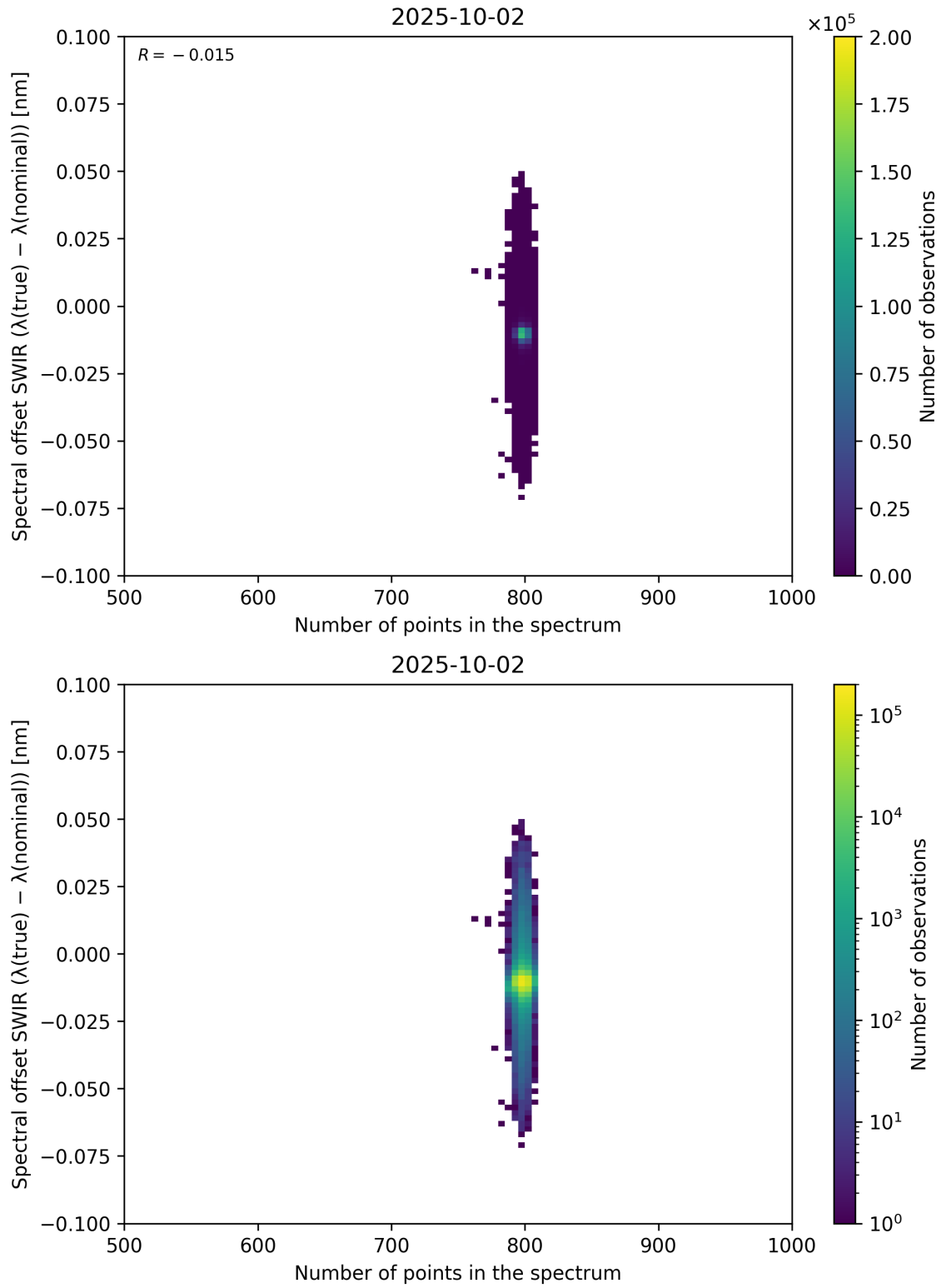
Figure 93: Scatter density plot of “Number of points in the spectrum” against “Spectral offset SWIR ( \lambda_{\text{true}} - \lambda_{\text{nominal}} )” for 2025-10-01 to 2025-10-03.
