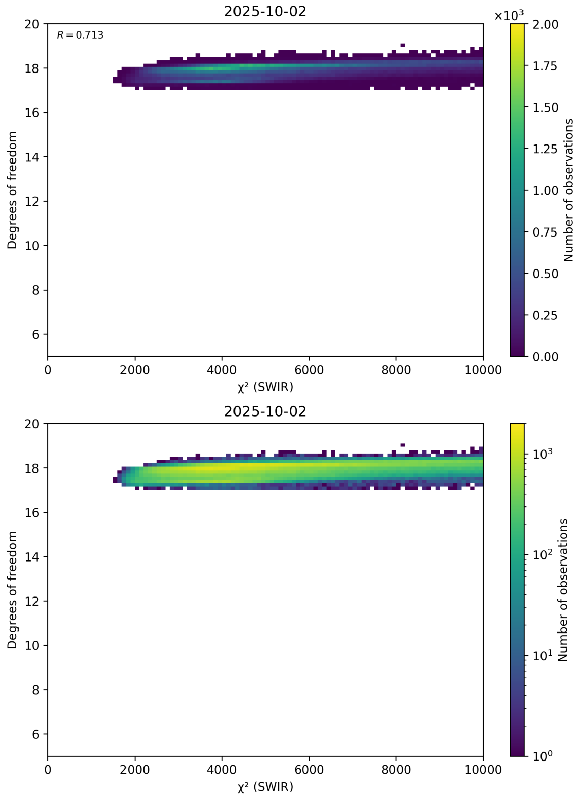
Figure 48: Scatter density plot of “ \chi^2 (SWIR)” against “Degrees of freedom” for 2025-10-01 to 2025-10-03.
