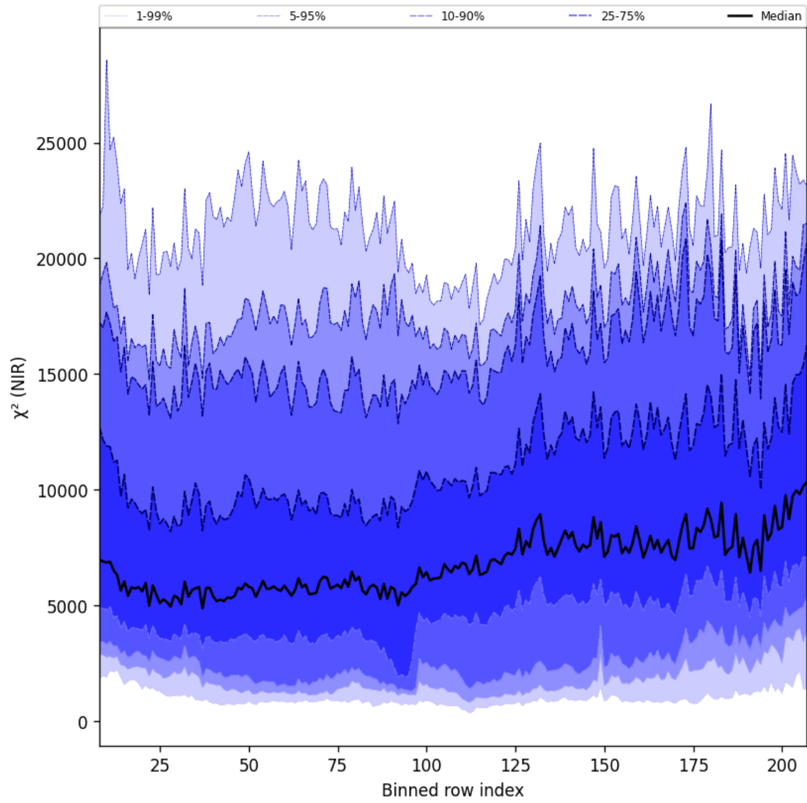
Figure 40: Along track statistics of “ \chi^2 (NIR)” for 2025-10-01 to 2025-10-03
