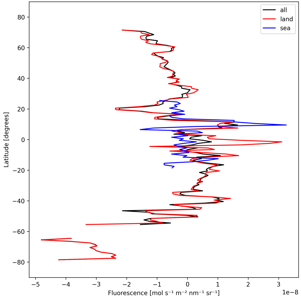
Figure 21: Zonal average of “Fluorescence” for 2025-10-01 to 2025-10-03.
