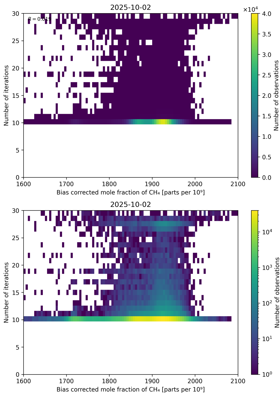
Figure 67: Scatter density plot of “Bias corrected mole fraction of \text{CH}_4 ” against “Number of iterations” for 2025-10-01 to 2025-10-03.
