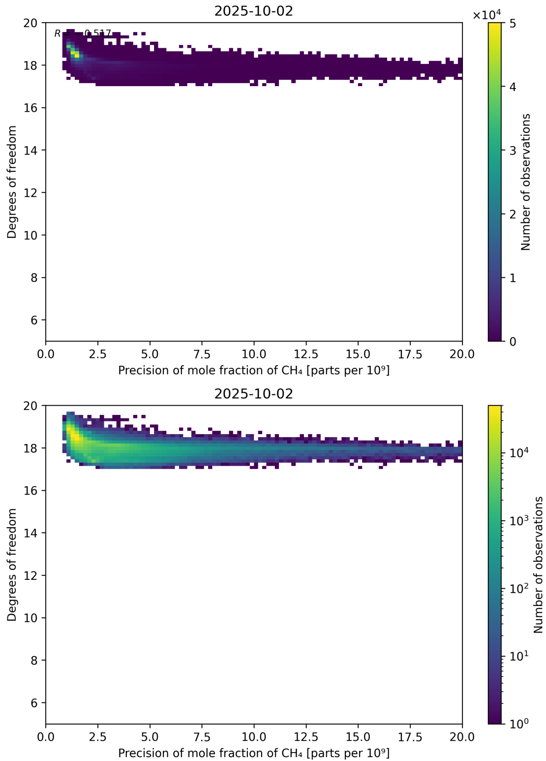
Figure 80: Scatter density plot of “Precision of mole fraction of CH 4 ” against “Degrees of freedom” for 2025-10-01 to 2025-10-03.
