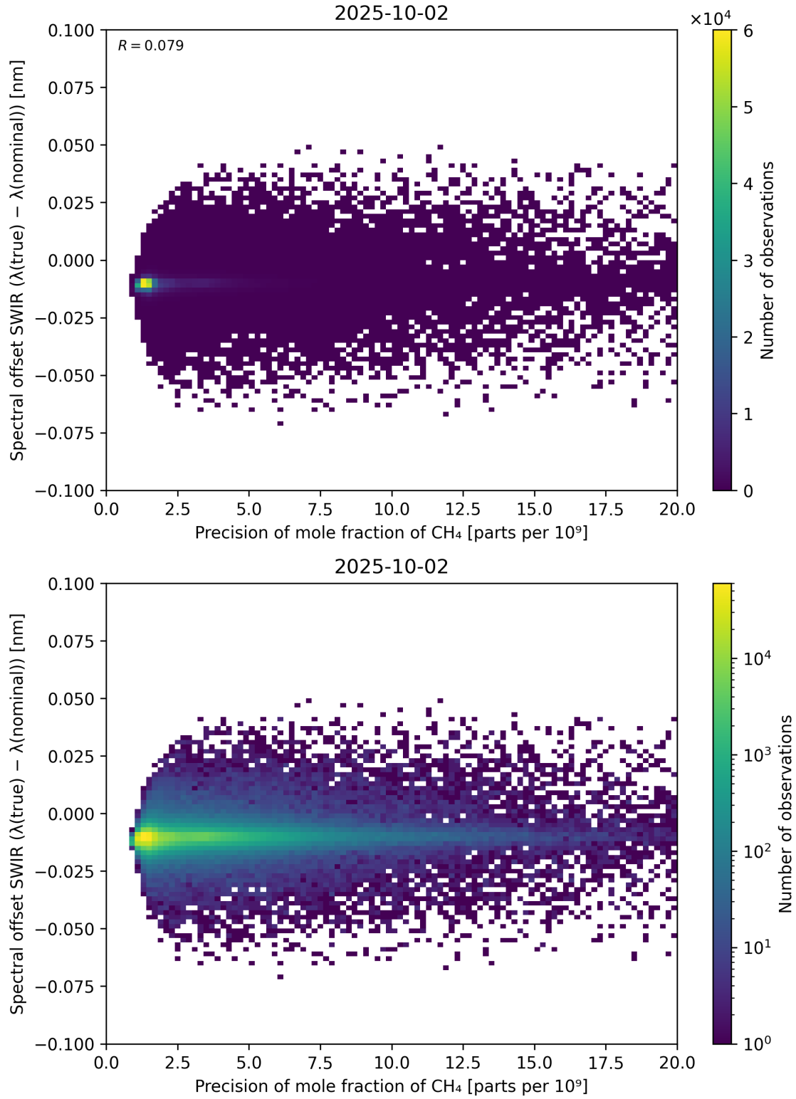
Figure 85: Scatter density plot of “Precision of mole fraction of \text{CH}_4 ” against “Spectral offset SWIR ( \lambda_{\text{true}} - \lambda_{\text{nominal}} )” for 2025-10-01 to 2025-10-03.
