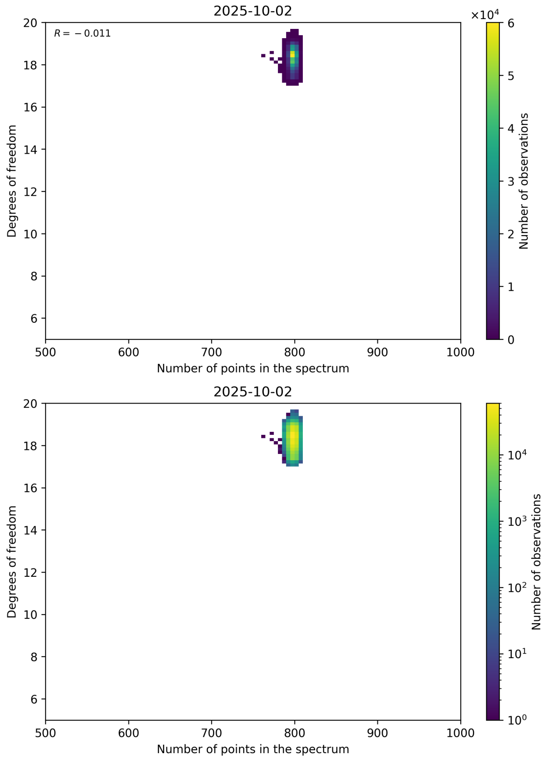
Figure 90: Scatter density plot of “Number of points in the spectrum” against “Degrees of freedom” for 2025-10-01 to 2025-10-03.
