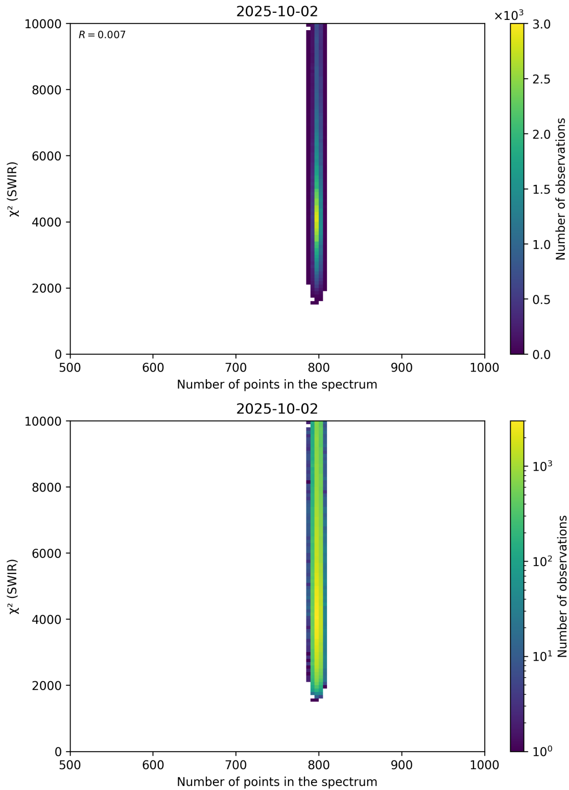
Figure 89: Scatter density plot of “Number of points in the spectrum” against “ \chi^2 (SWIR)” for 2025-10-01 to 2025-10-03.
