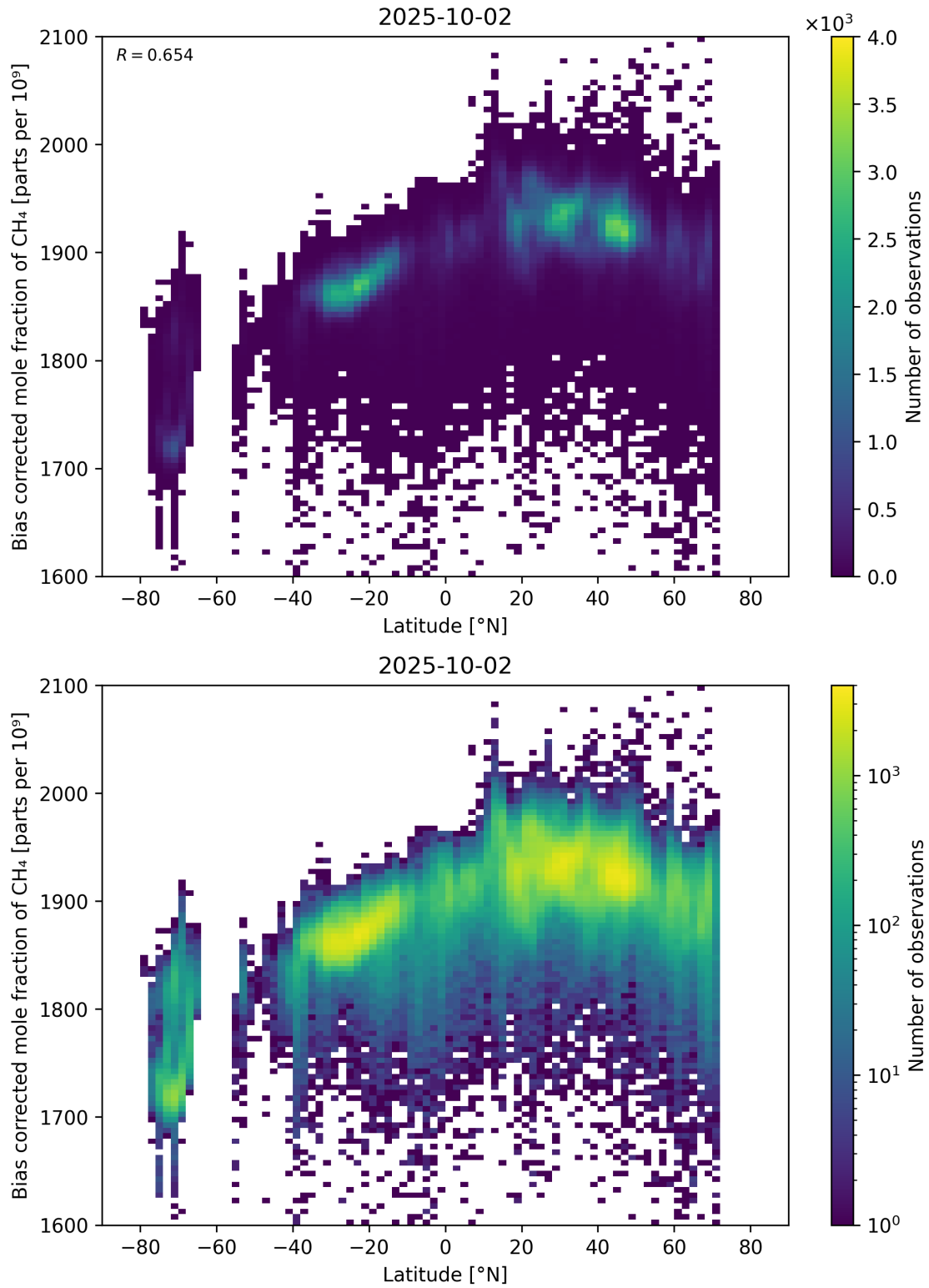
Figure 58: Scatter density plot of “Latitude” against “Bias corrected mole fraction of CH 4 ” for 2025-10-01 to 2025-10-03.
