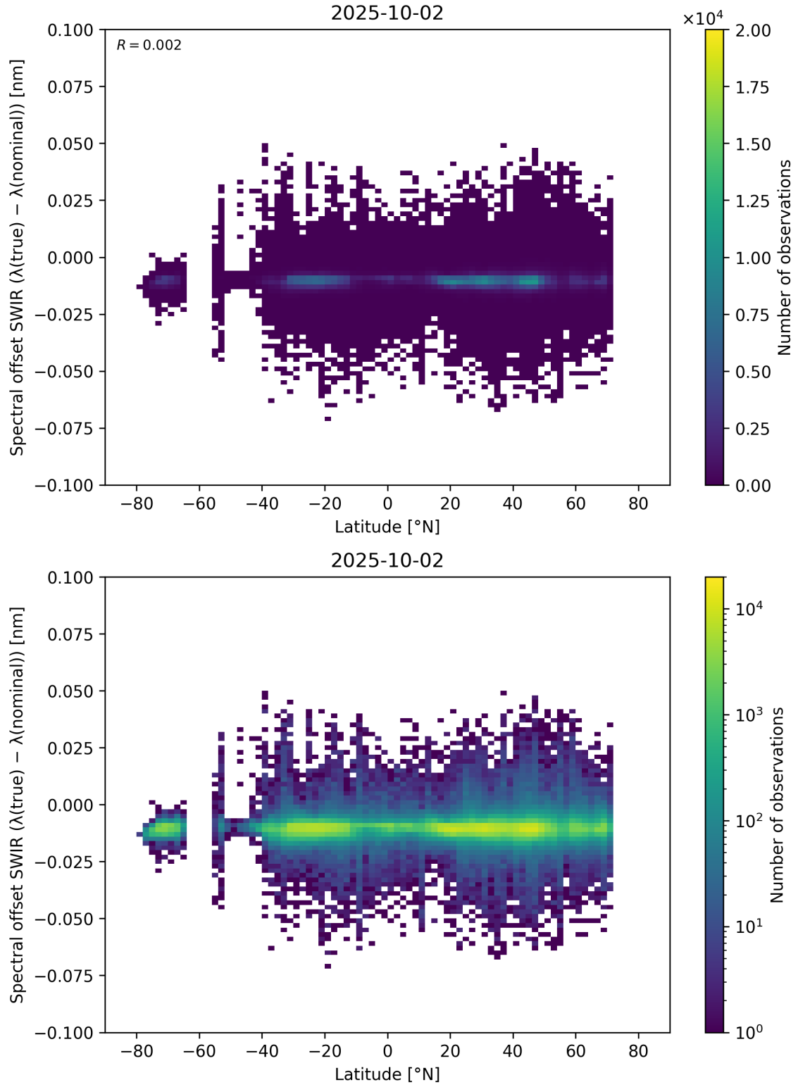
Figure 62: Scatter density plot of “Latitude” against “Spectral offset SWIR ( \lambda_{\text{true}} - \lambda_{\text{nominal}} )” for 2025-10-01 to 2025-10-03.
