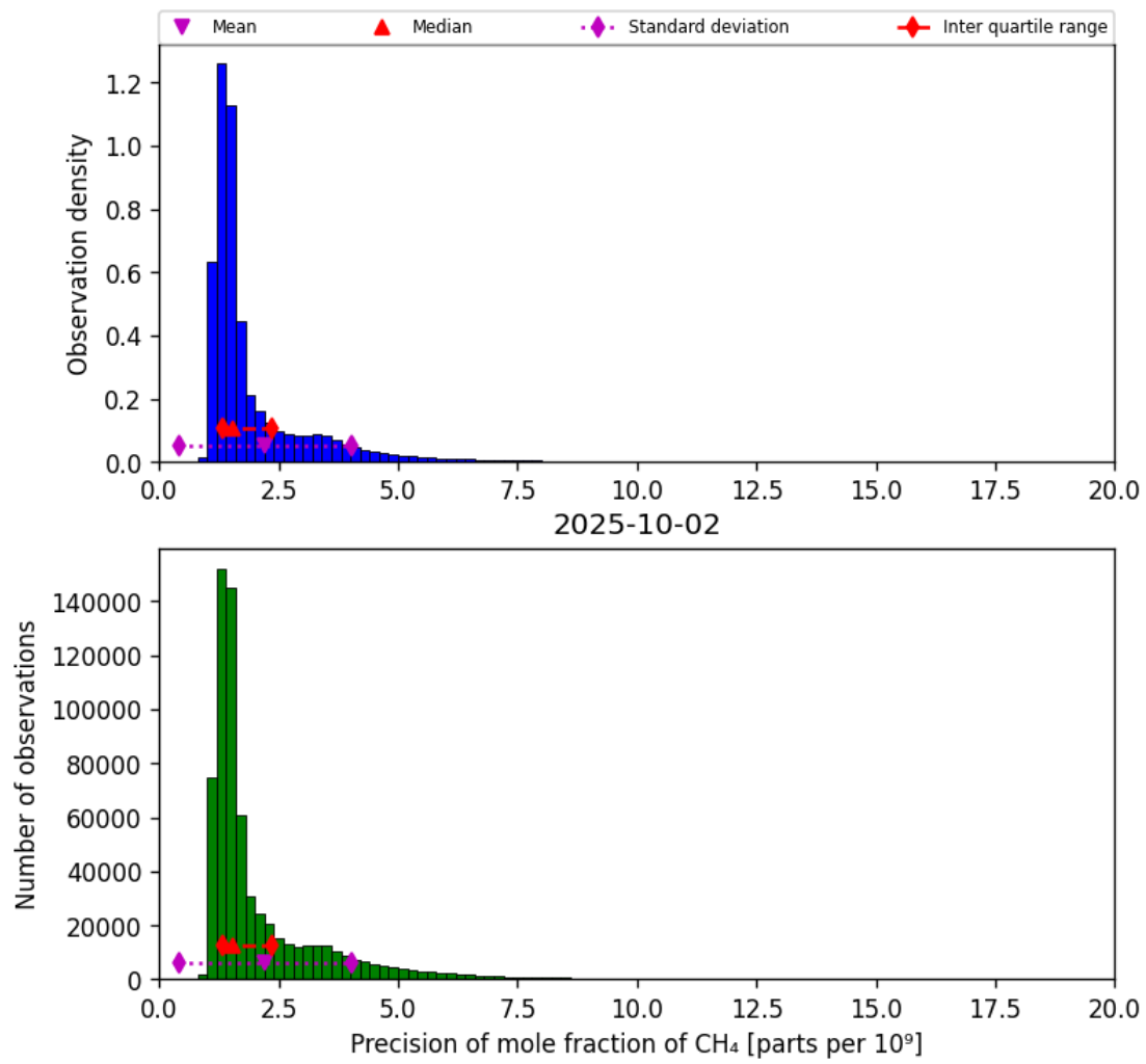
Figure 24: Histogram of “Precision of mole fraction of CH 4 ” for 2025-10-01 to 2025-10-03
