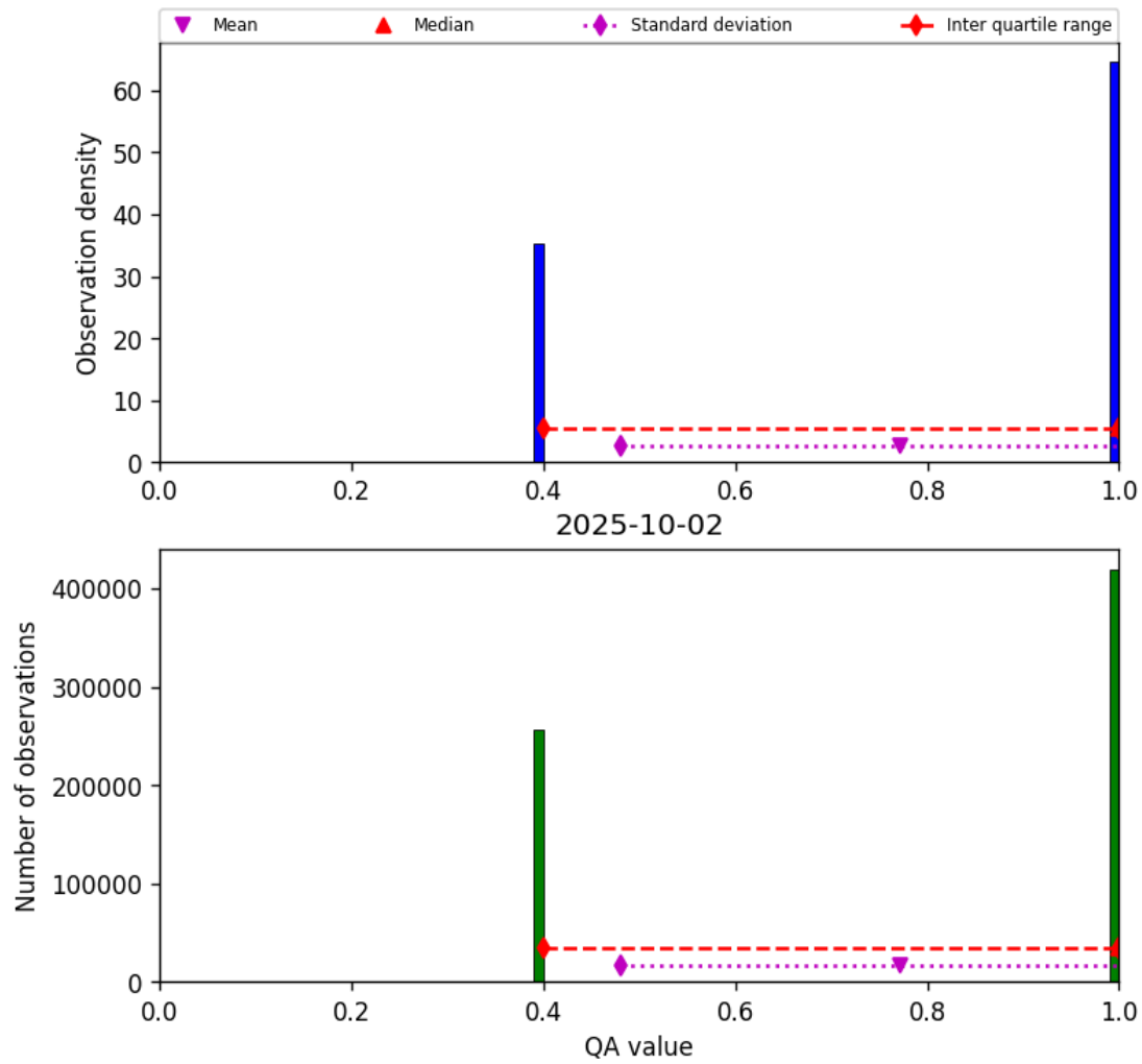
Figure 22: Histogram of “QA value” for 2025-10-01 to 2025-10-03
