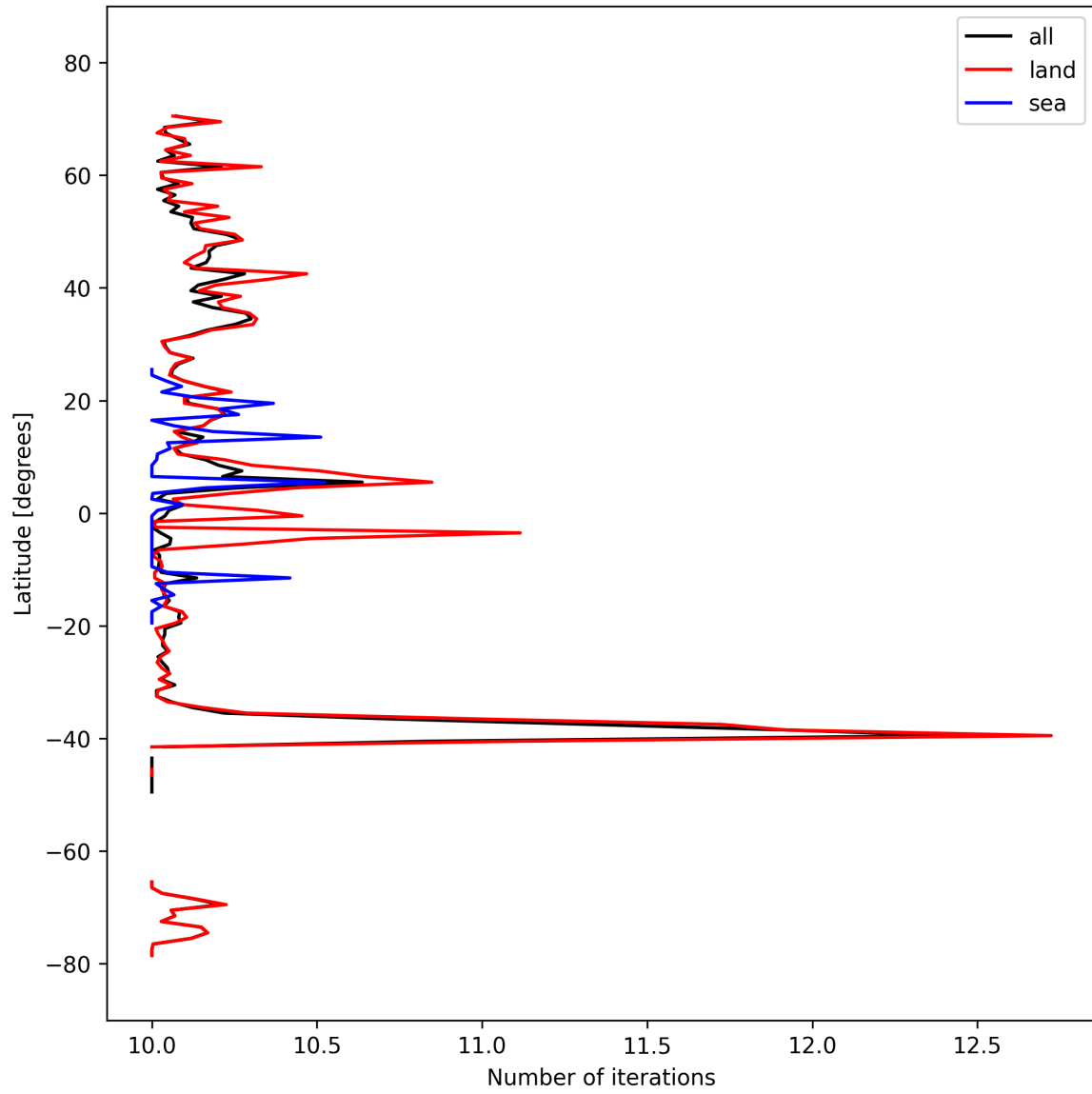
Figure 20: Zonal average of “Number of iterations” for 2025-10-02 to 2025-10-04.
