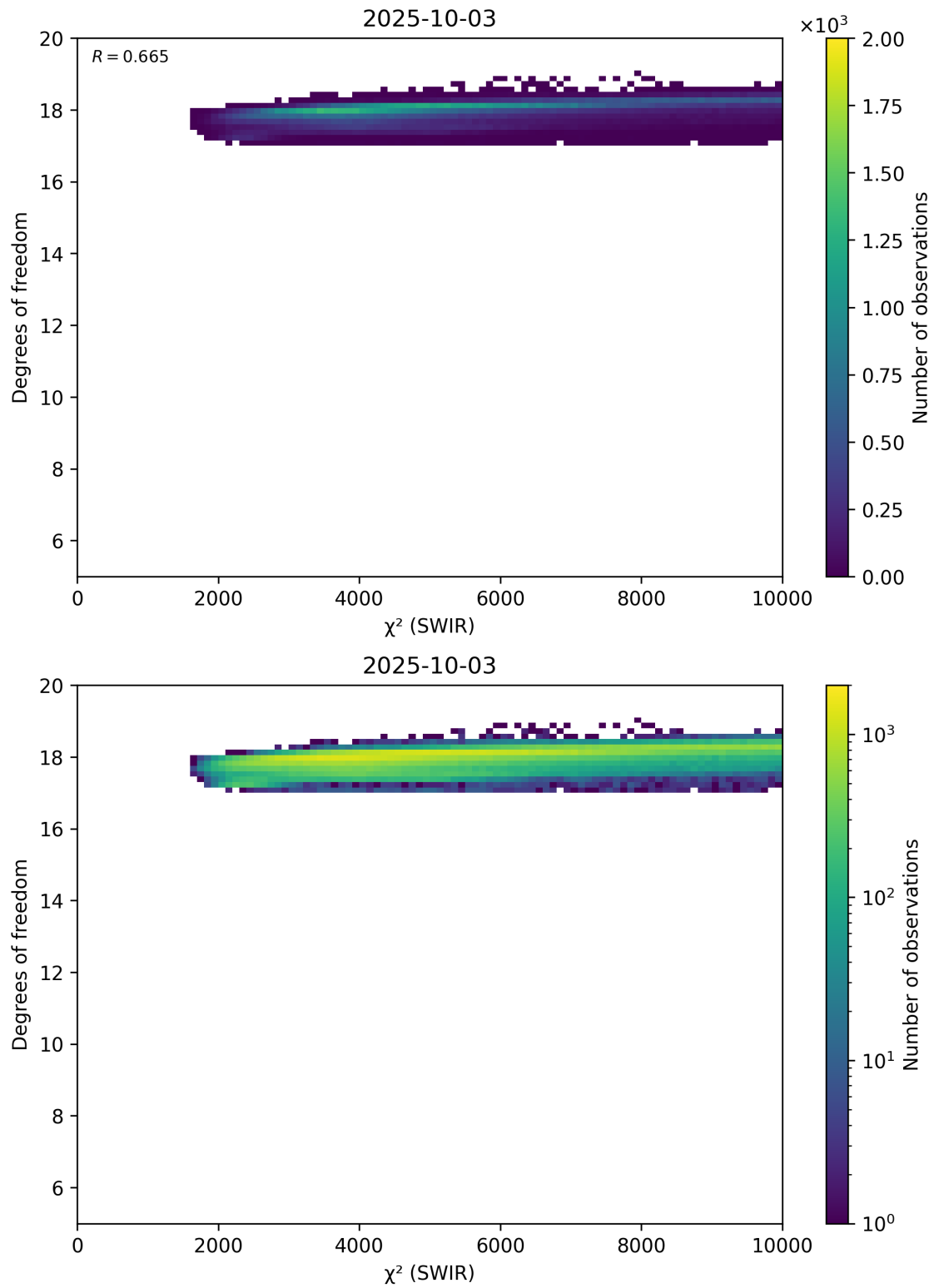
Figure 48: Scatter density plot of “ \chi^2 (SWIR)” against “Degrees of freedom” for 2025-10-02 to 2025-10-04.
