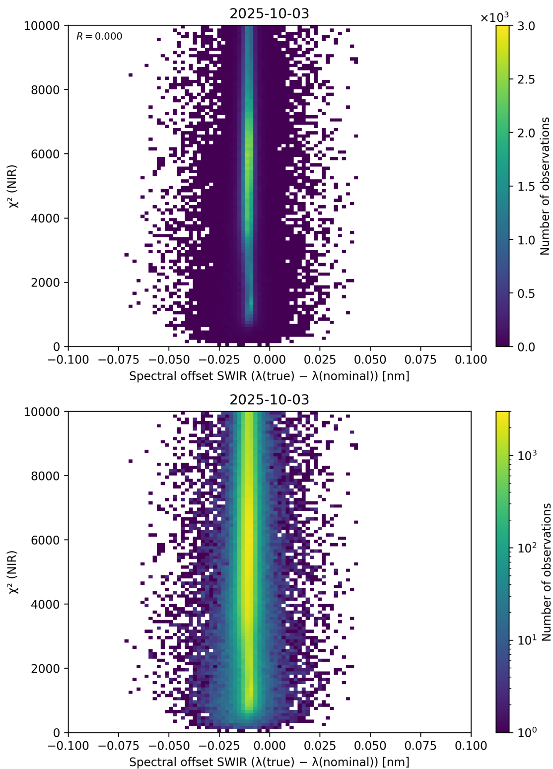
Figure 117: Scatter density plot of “Spectral offset SWIR ( \lambda_{\text{true}} - \lambda_{\text{nominal}} )” against “ \chi^2 (NIR)” for 2025-10-02 to 2025-10-04.
