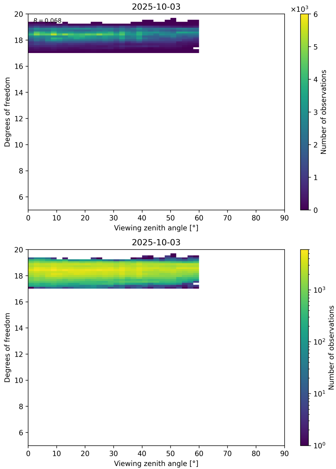
Figure 107: Scatter density plot of “Viewing zenith angle” against “Degrees of freedom” for 2025-10-02 to 2025-10-04.
