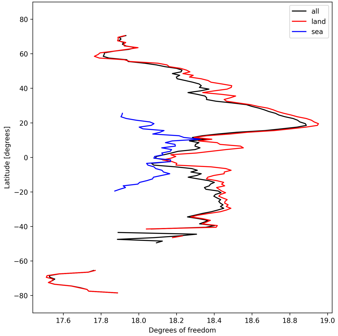
Figure 19: Zonal average of “Degrees of freedom” for 2025-10-02 to 2025-10-04.
