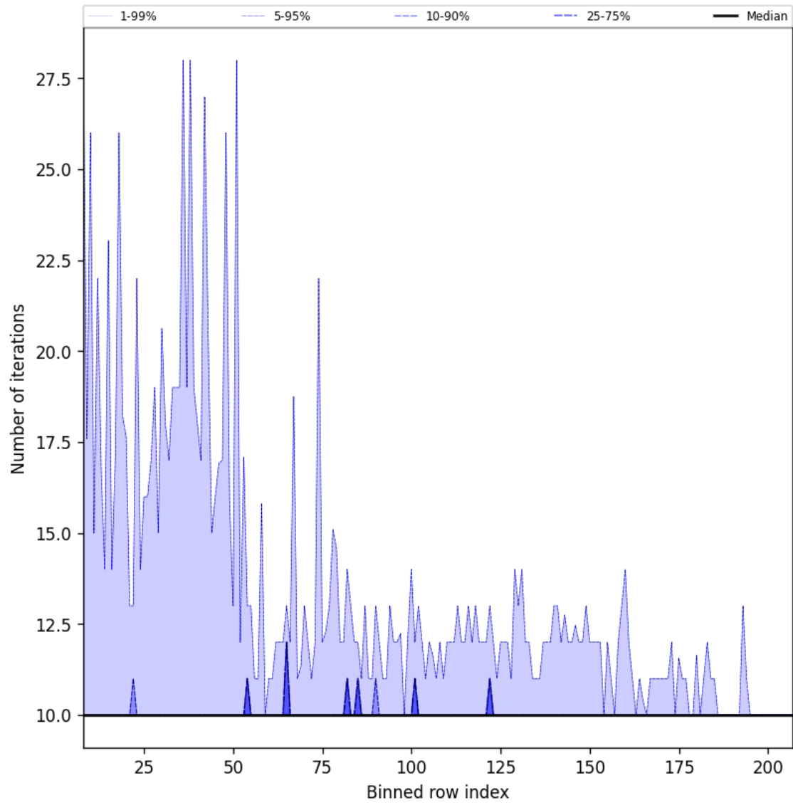
Figure 42: Along track statistics of “Number of iterations” for 2025-10-02 to 2025-10-04
