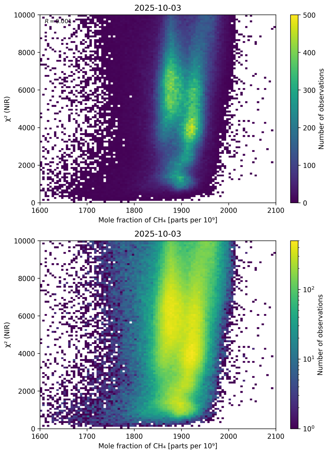
Figure 70: Scatter density plot of “Mole fraction of CH 4 ” against “ \chi^2 (NIR)” for 2025-10-02 to 2025-10-04.
