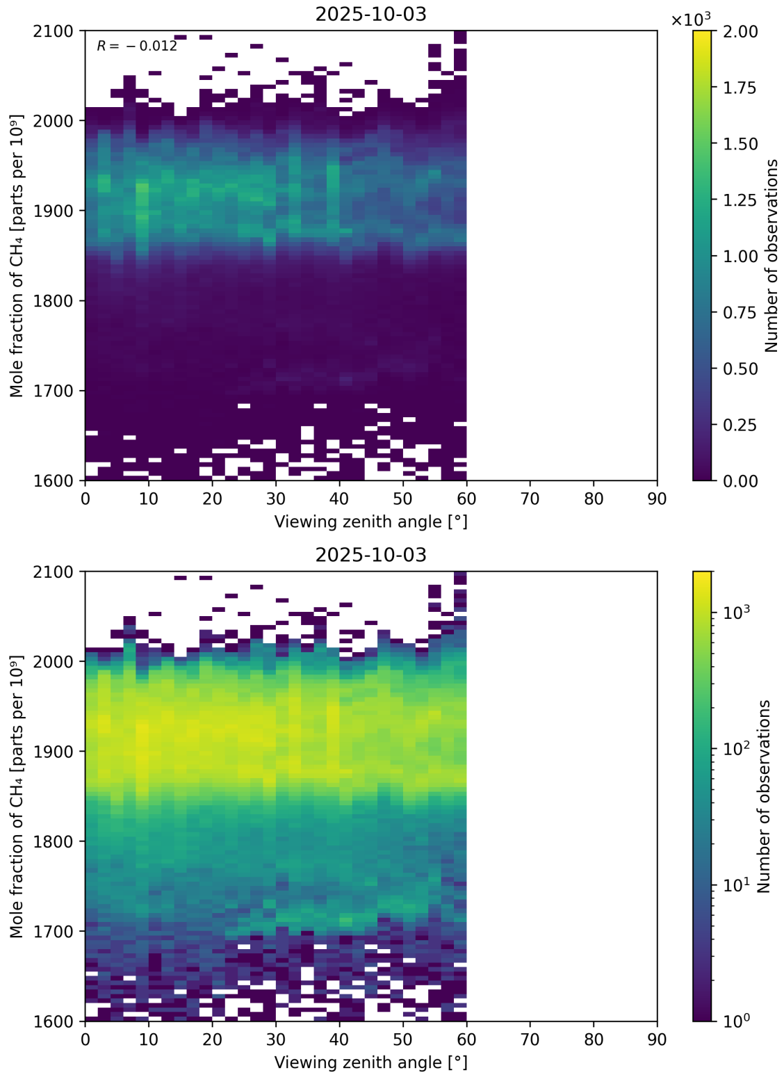
Figure 110: Scatter density plot of “Viewing zenith angle” against “Mole fraction of CH 4 ” for 2025-10-02 to 2025-10-04.
