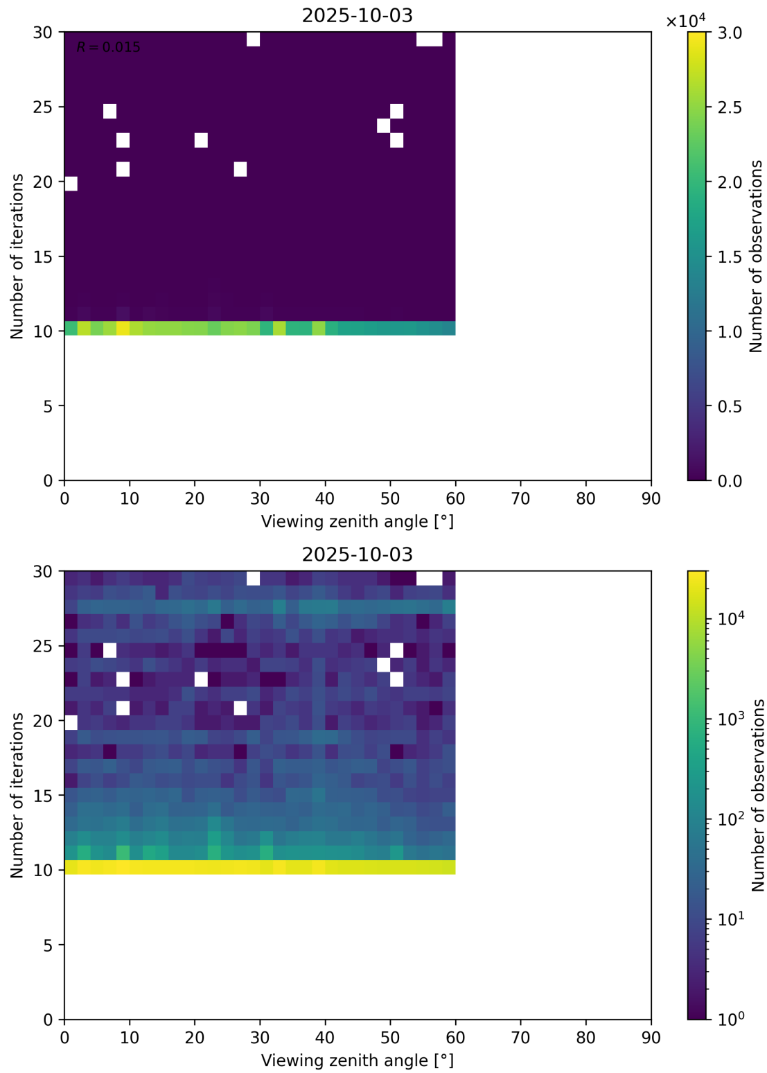
Figure 113: Scatter density plot of “Viewing zenith angle” against “Number of iterations” for 2025-10-02 to 2025-10-04.
