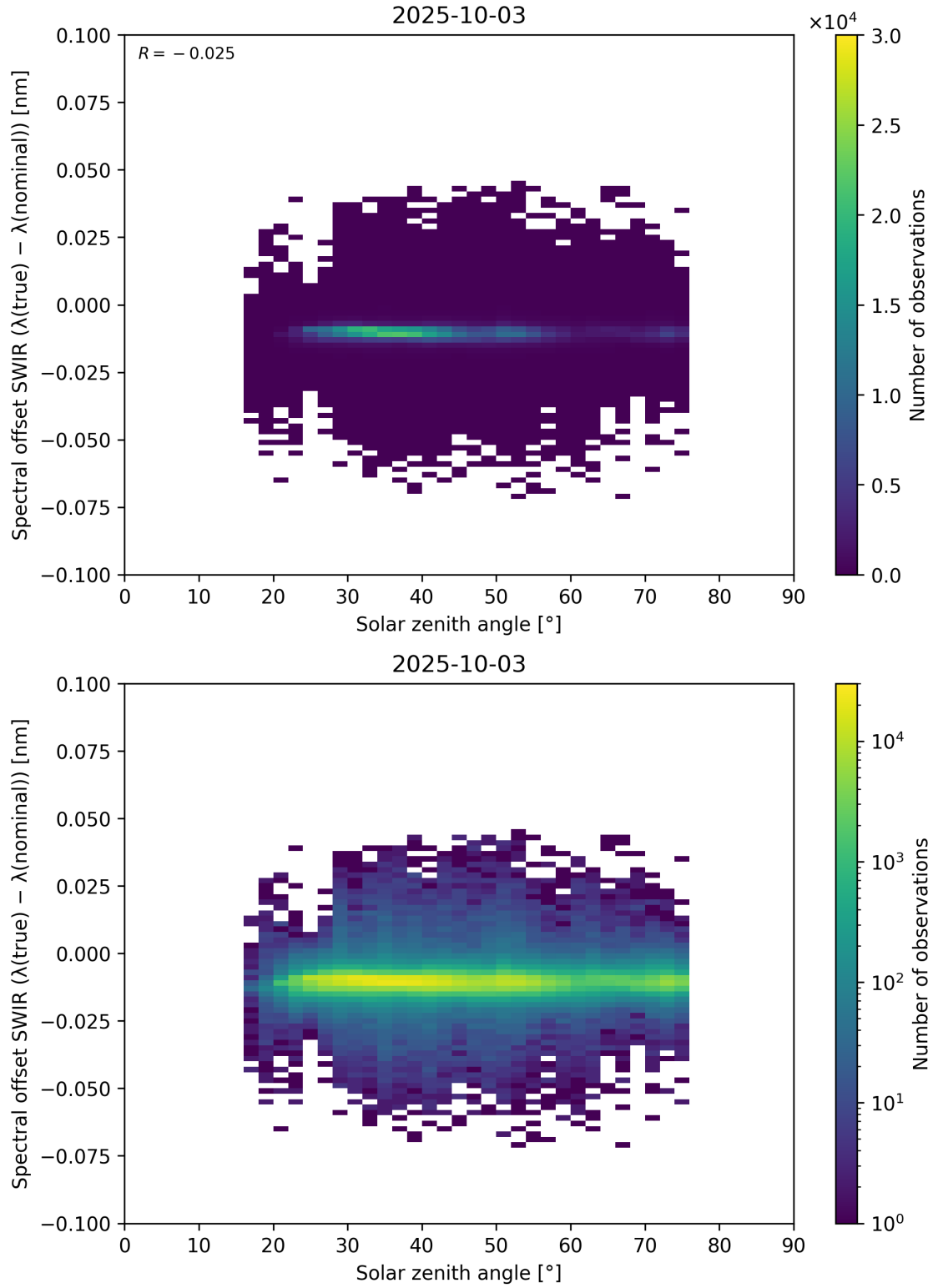
Figure 104: Scatter density plot of “Solar zenith angle” against “Spectral offset SWIR ( \lambda_{\text{true}} - \lambda_{\text{nominal}} )” for 2025-10-02 to 2025-10-04.
