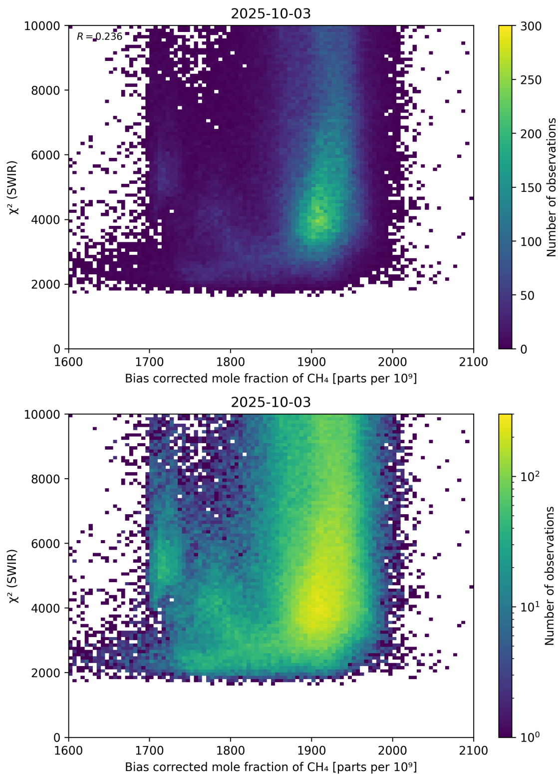
Figure 64: Scatter density plot of “Bias corrected mole fraction of \text{CH}_4 ” against “ \chi^2 (SWIR)” for 2025-10-02 to 2025-10-04.
