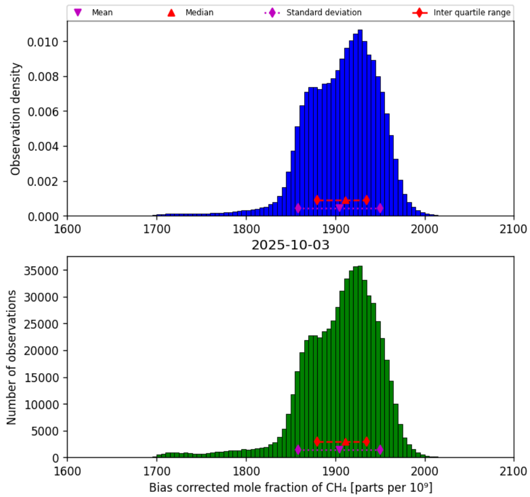
Figure 25: Histogram of “Bias corrected mole fraction of CH 4 ” for 2025-10-02 to 2025-10-04
