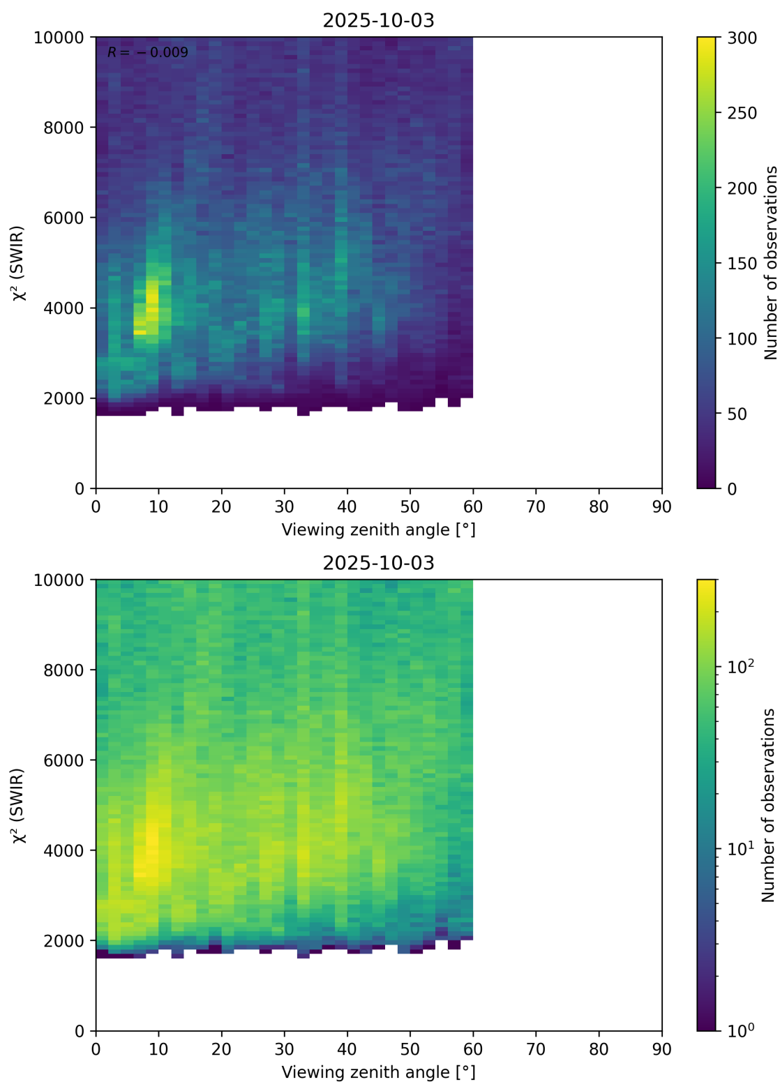
Figure 106: Scatter density plot of “Viewing zenith angle” against “ \chi^2 (SWIR)” for 2025-10-02 to 2025-10-04.
