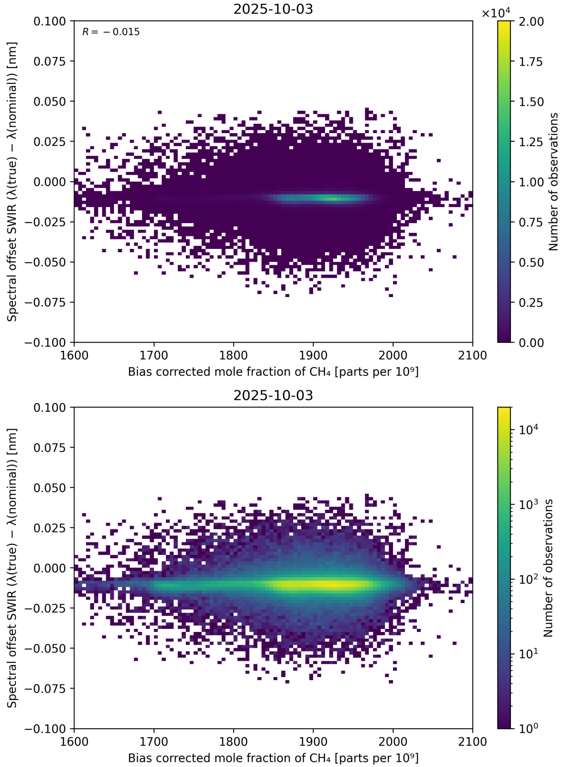
Figure 69: Scatter density plot of “Bias corrected mole fraction of \text{CH}_4 ” against “Spectral offset SWIR ( \lambda_{\text{true}} - \lambda_{\text{nominal}} )” for 2025-10-02 to 2025-10-04.
