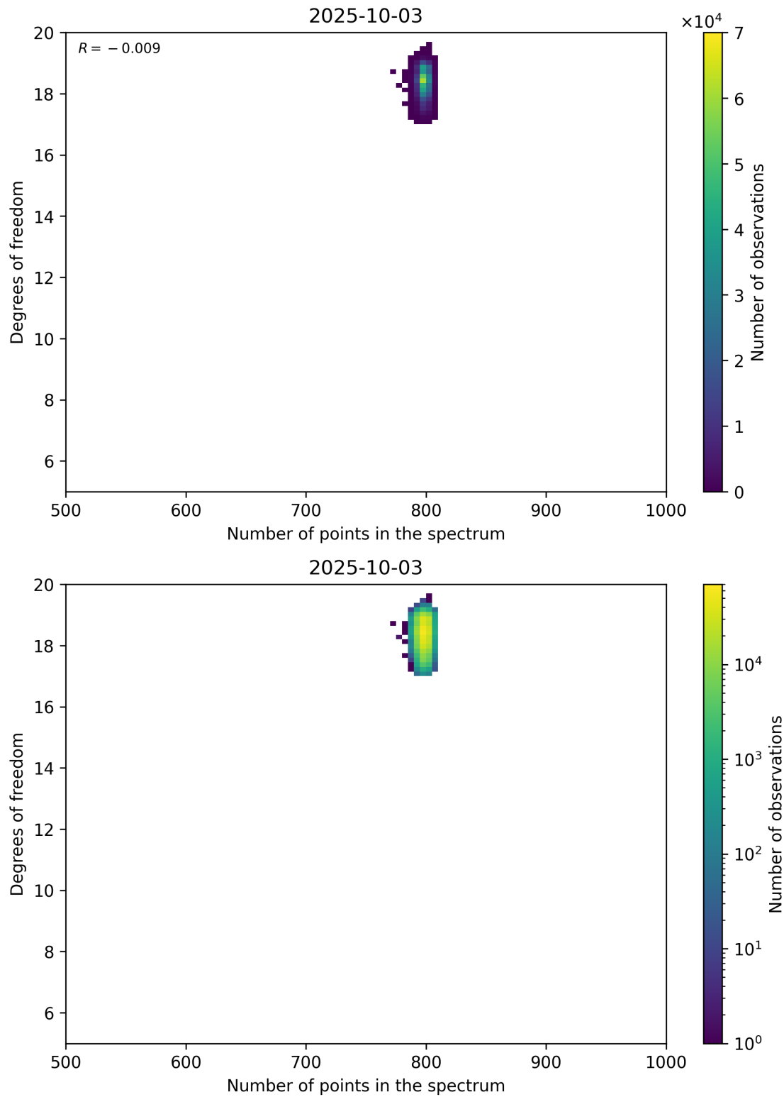
Figure 90: Scatter density plot of “Number of points in the spectrum” against “Degrees of freedom” for 2025-10-02 to 2025-10-04.
