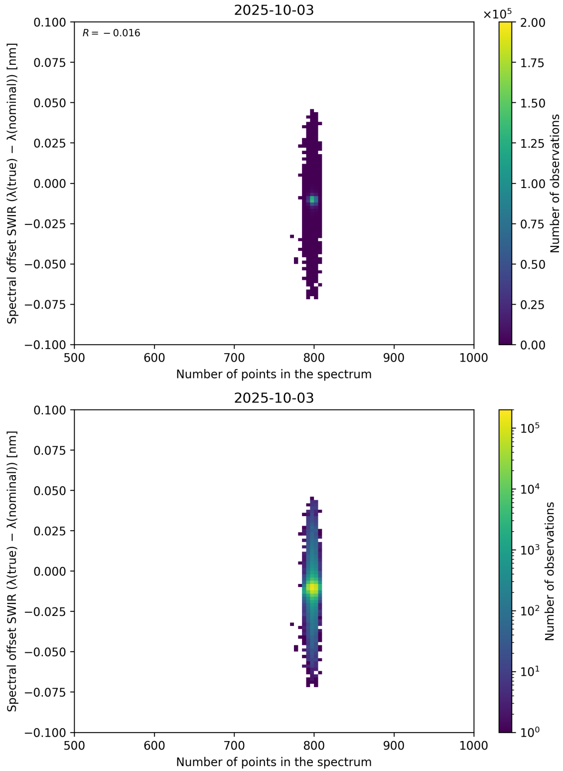
Figure 93: Scatter density plot of “Number of points in the spectrum” against “Spectral offset SWIR ( \lambda_{\text{true}} - \lambda_{\text{nominal}} )” for 2025-10-02 to 2025-10-04.
