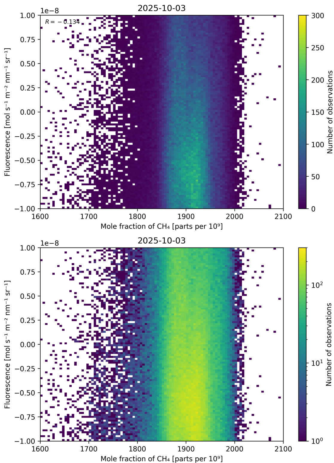
Figure 73: Scatter density plot of “Mole fraction of \text{CH}_4 ” against “Fluorescence” for 2025-10-02 to 2025-10-04.
