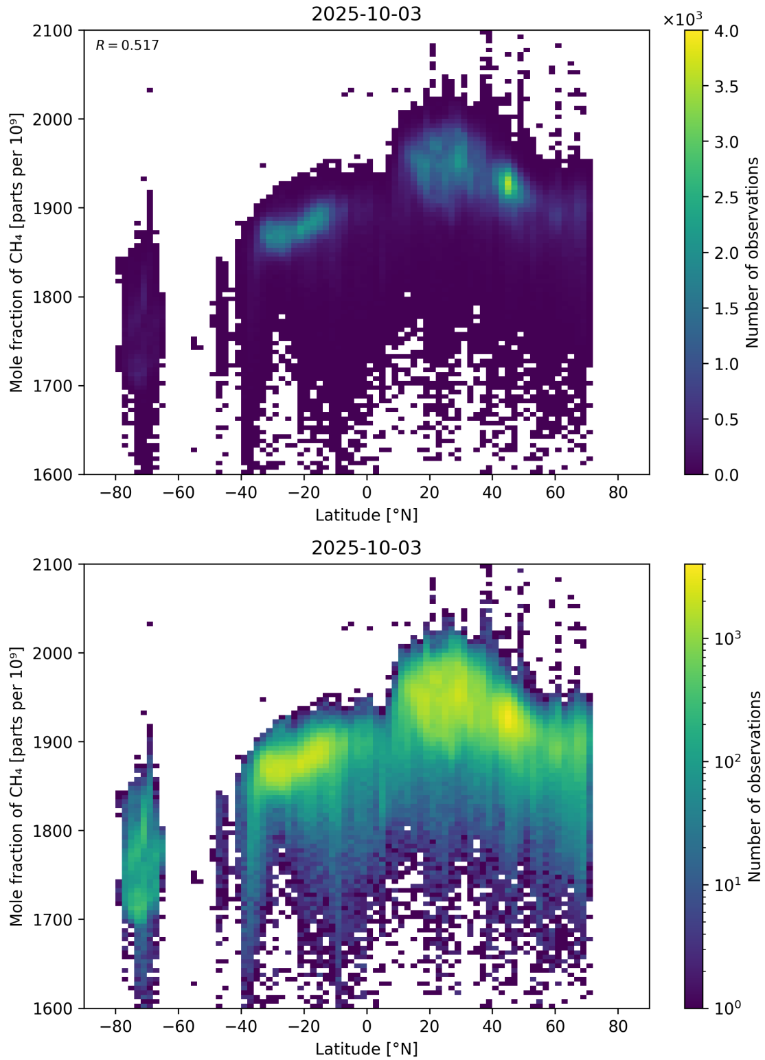
Figure 57: Scatter density plot of “Latitude” against “Mole fraction of CH 4 ” for 2025-10-02 to 2025-10-04.
