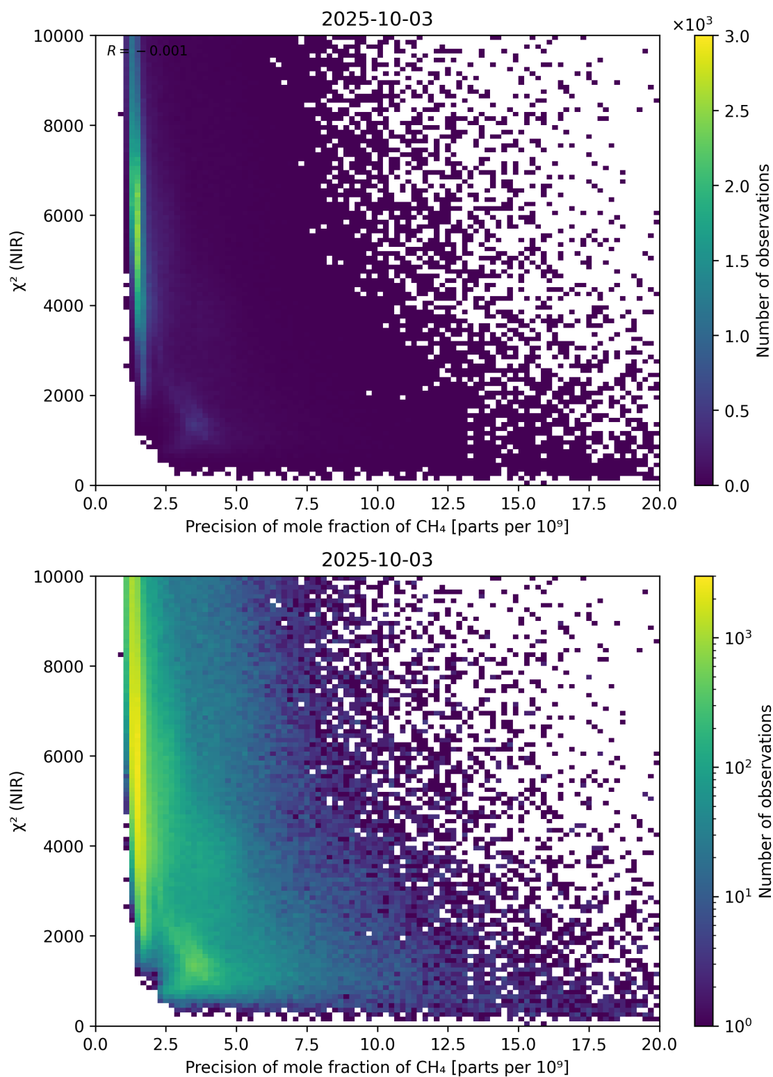
Figure 78: Scatter density plot of “Precision of mole fraction of CH 4 ” against “ \chi^2 (NIR)” for 2025-10-02 to 2025-10-04.
