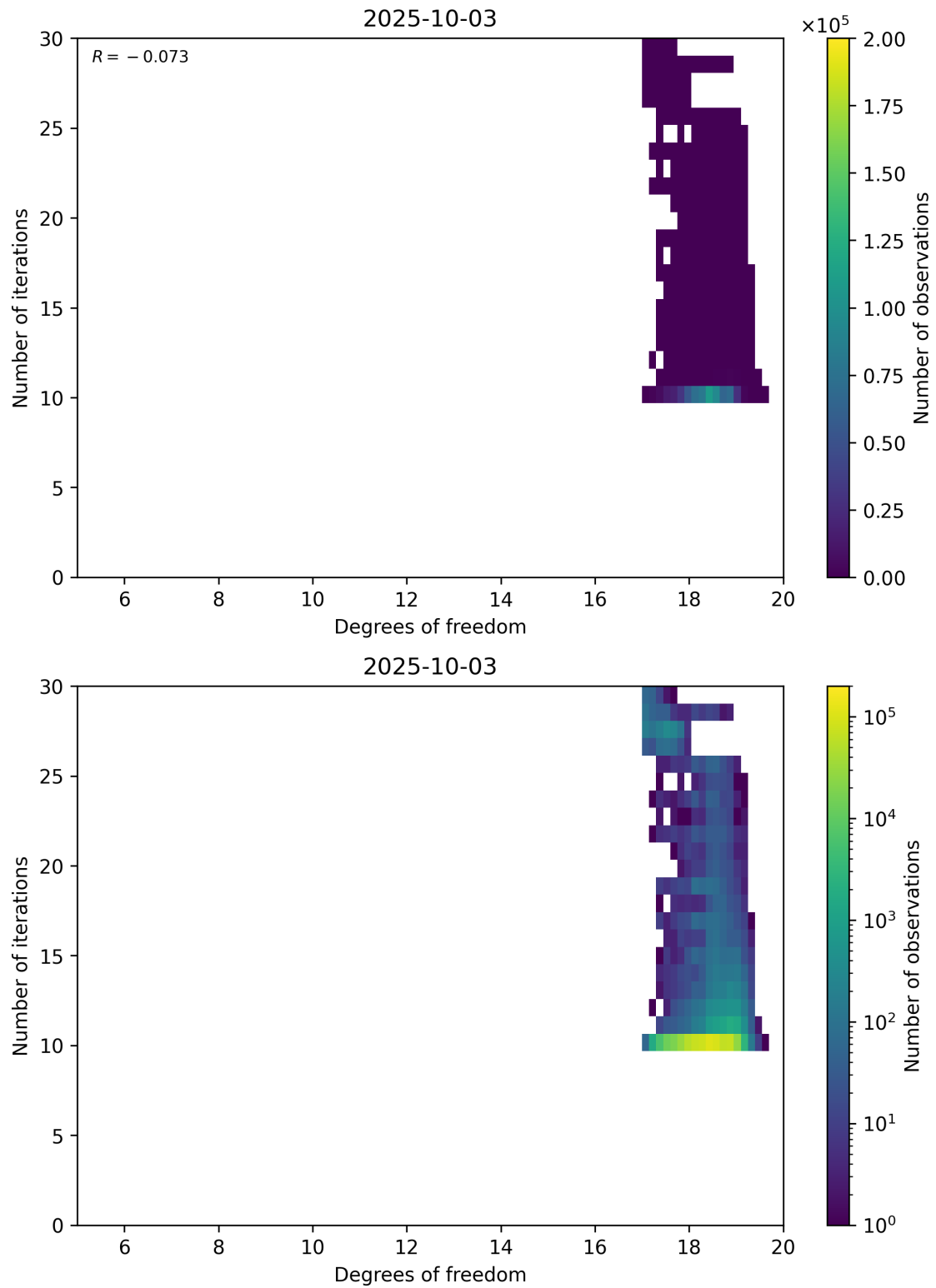
Figure 52: Scatter density plot of “Degrees of freedom” against “Number of iterations” for 2025-10-02 to 2025-10-04.
