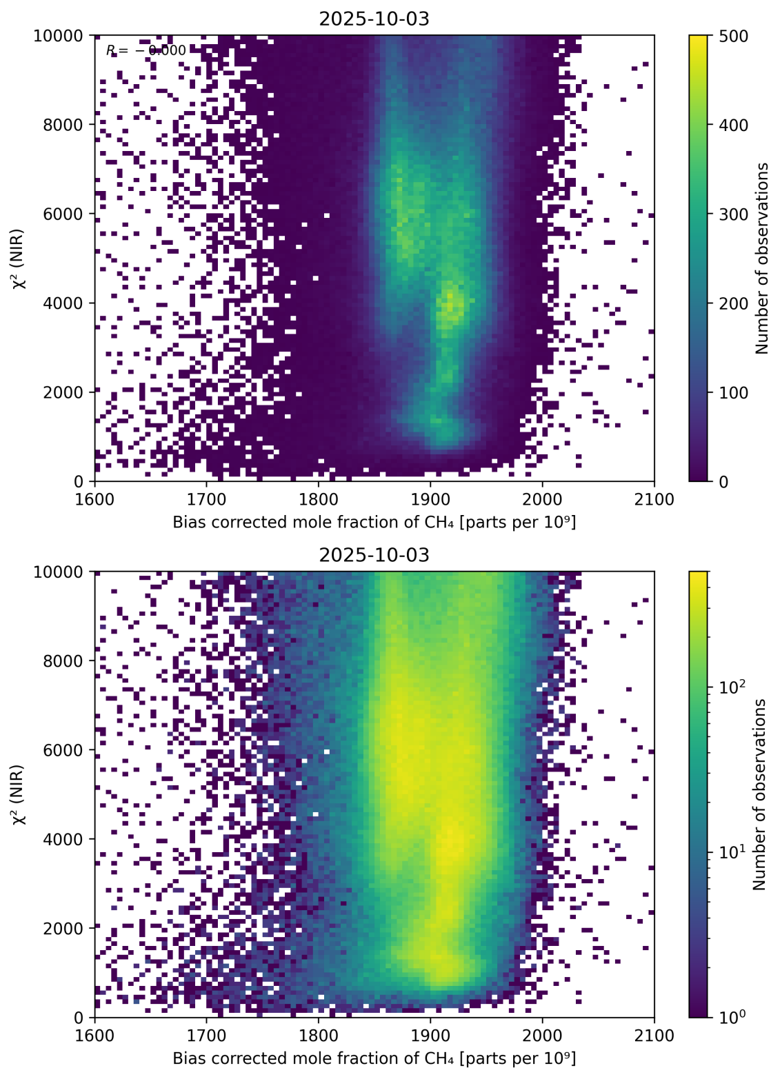
Figure 63: Scatter density plot of “Bias corrected mole fraction of \text{CH}_4 ” against “ \chi^2 (NIR)” for 2025-10-02 to 2025-10-04.
