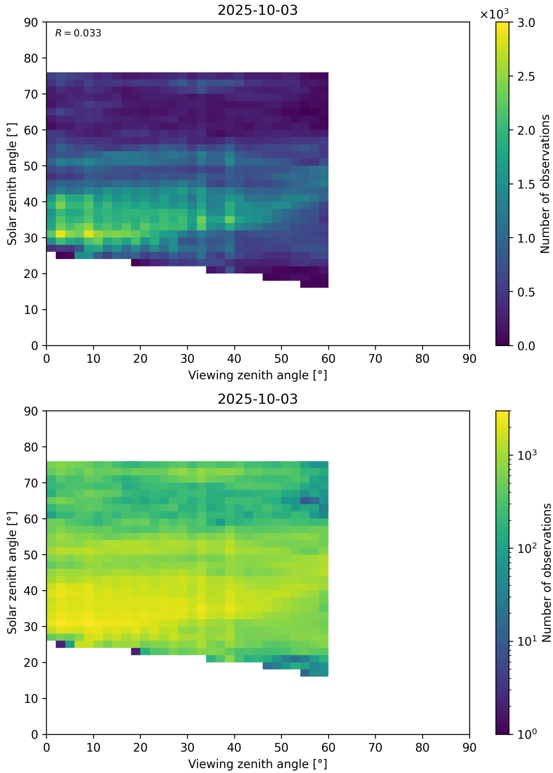
Figure 115: Scatter density plot of “Viewing zenith angle” against “Solar zenith angle” for 2025-10-02 to 2025-10-04.
