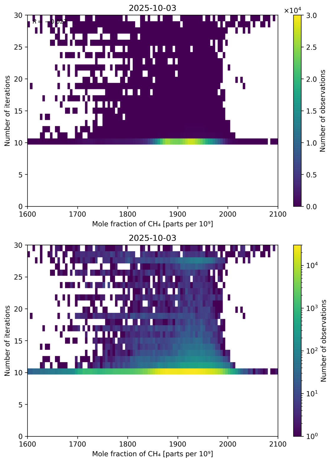
Figure 76: Scatter density plot of “Mole fraction of CH 4 ” against “Number of iterations” for 2025-10-02 to 2025-10-04.
