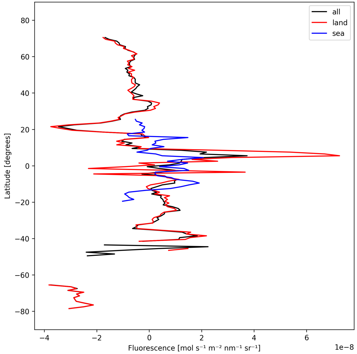
Figure 21: Zonal average of “Fluorescence” for 2025-10-02 to 2025-10-04.
