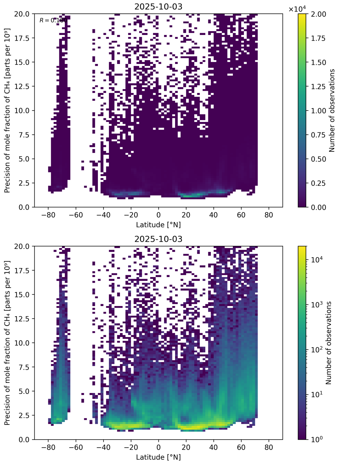
Figure 59: Scatter density plot of “Latitude” against “Precision of mole fraction of CH 4 ” for 2025-10-02 to 2025-10-04.
