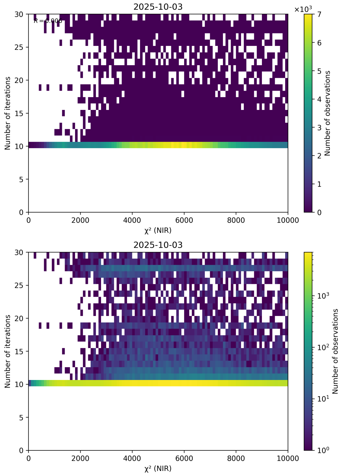
Figure 46: Scatter density plot of “ \chi^2 (NIR)” against “Number of iterations” for 2025-10-02 to 2025-10-04.
