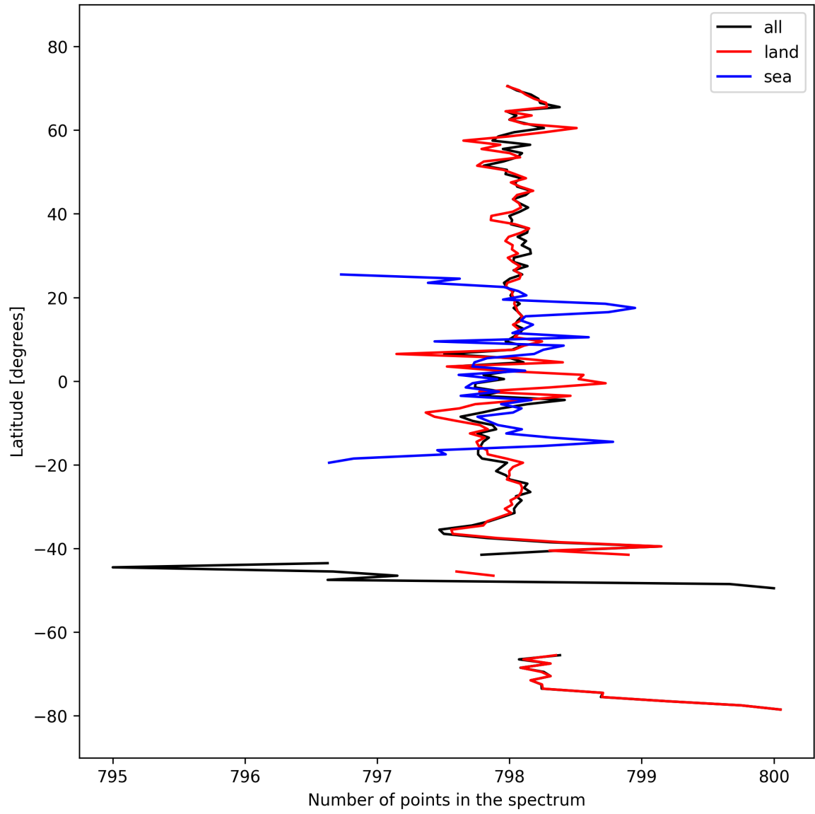
Figure 15: Zonal average of “Number of points in the spectrum” for 2025-10-02 to 2025-10-04.
