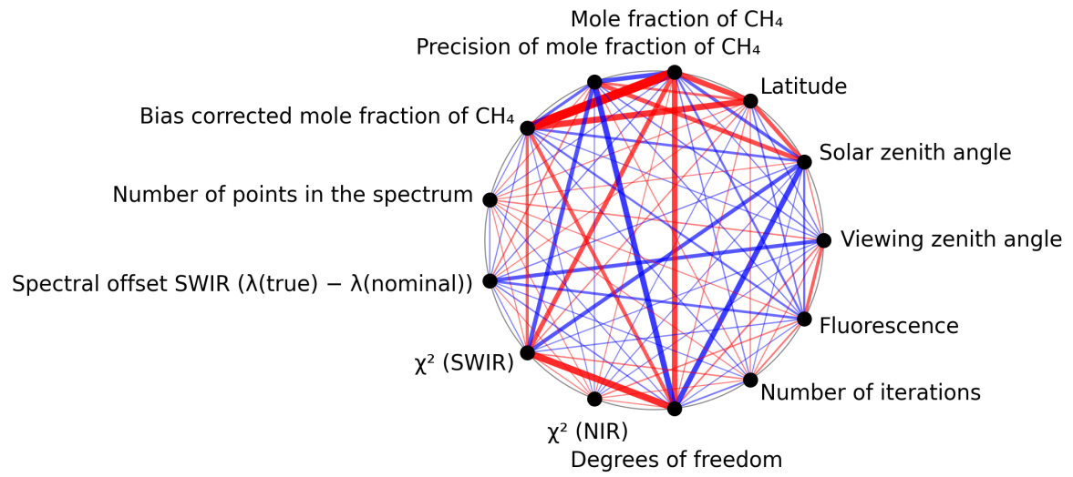
Figure 1: Map of correlation graph for 2025-10-02 to 2025-10-04.
