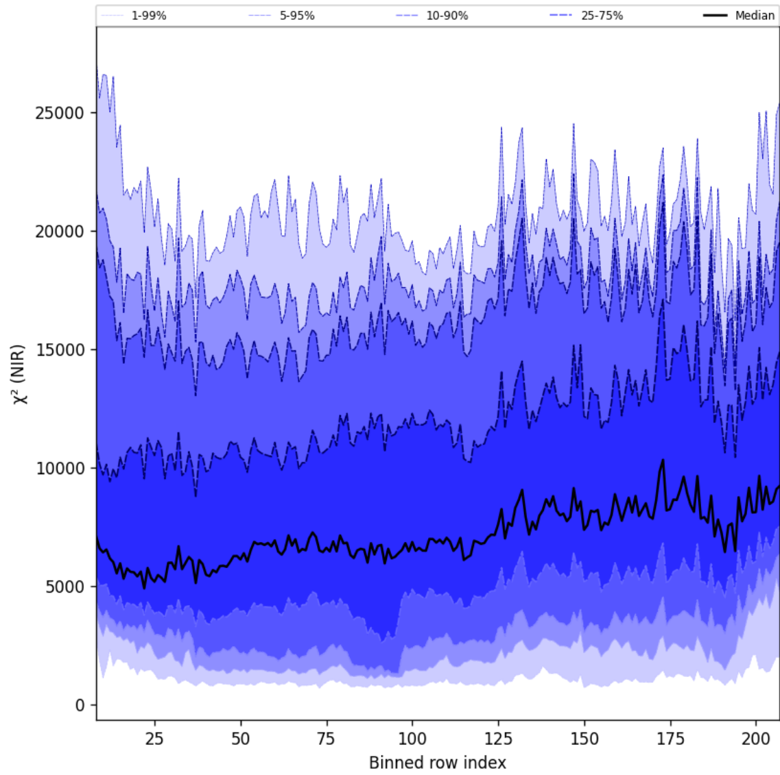
Figure 40: Along track statistics of “ \chi^2 (NIR)” for 2025-10-02 to 2025-10-04
