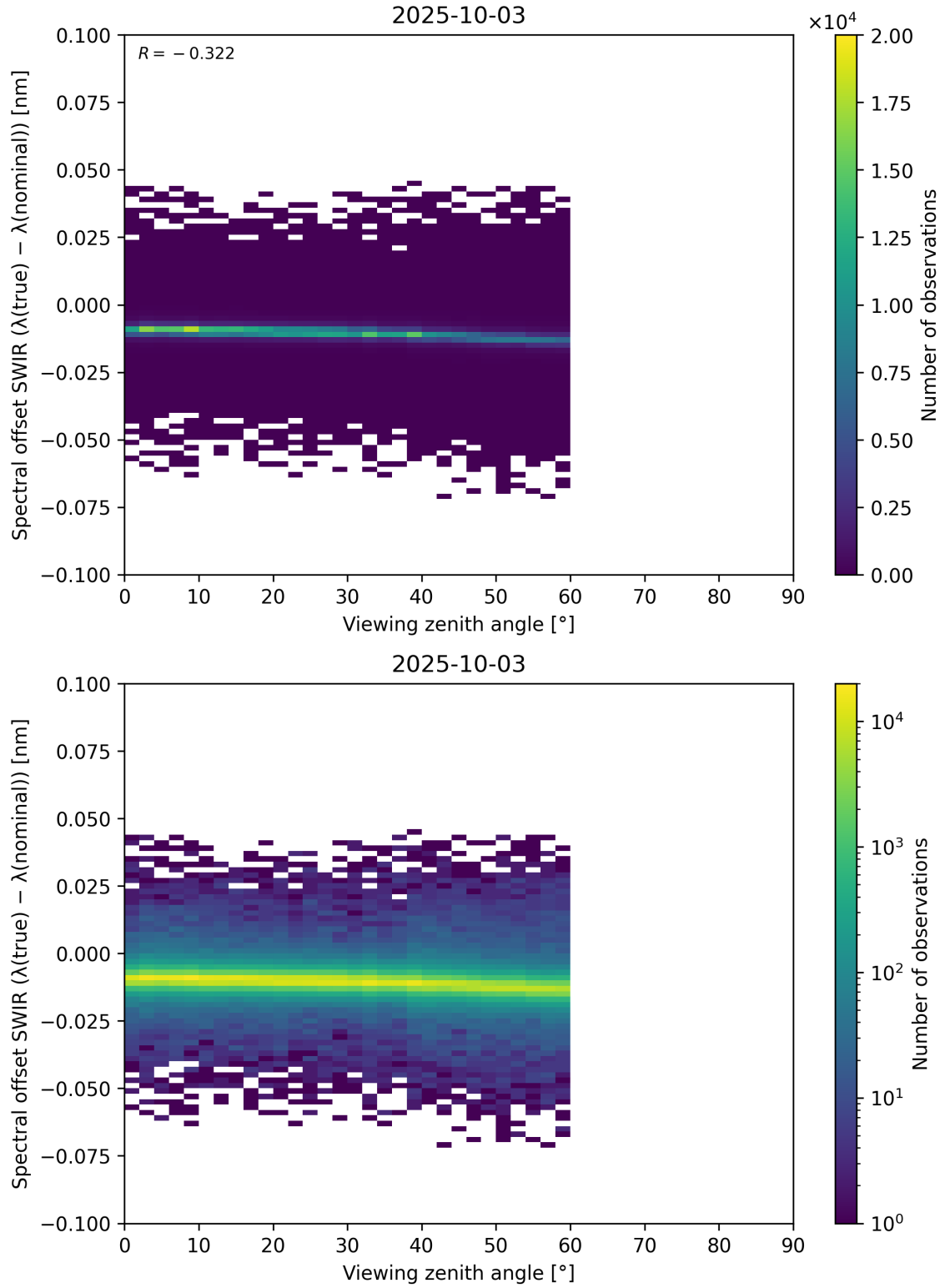
Figure 116: Scatter density plot of “Viewing zenith angle” against “Spectral offset SWIR ( \lambda_{\text{true}} - \lambda_{\text{nominal}} )” for 2025-10-02 to 2025-10-04.
