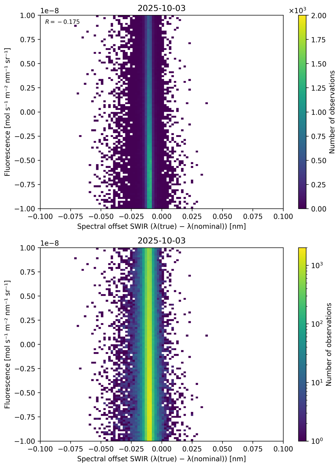
Figure 120: Scatter density plot of “Spectral offset SWIR ( \lambda_{\text{true}} - \lambda_{\text{nominal}} )” against “Fluorescence” for 2025-10-02 to 2025-10-04.
