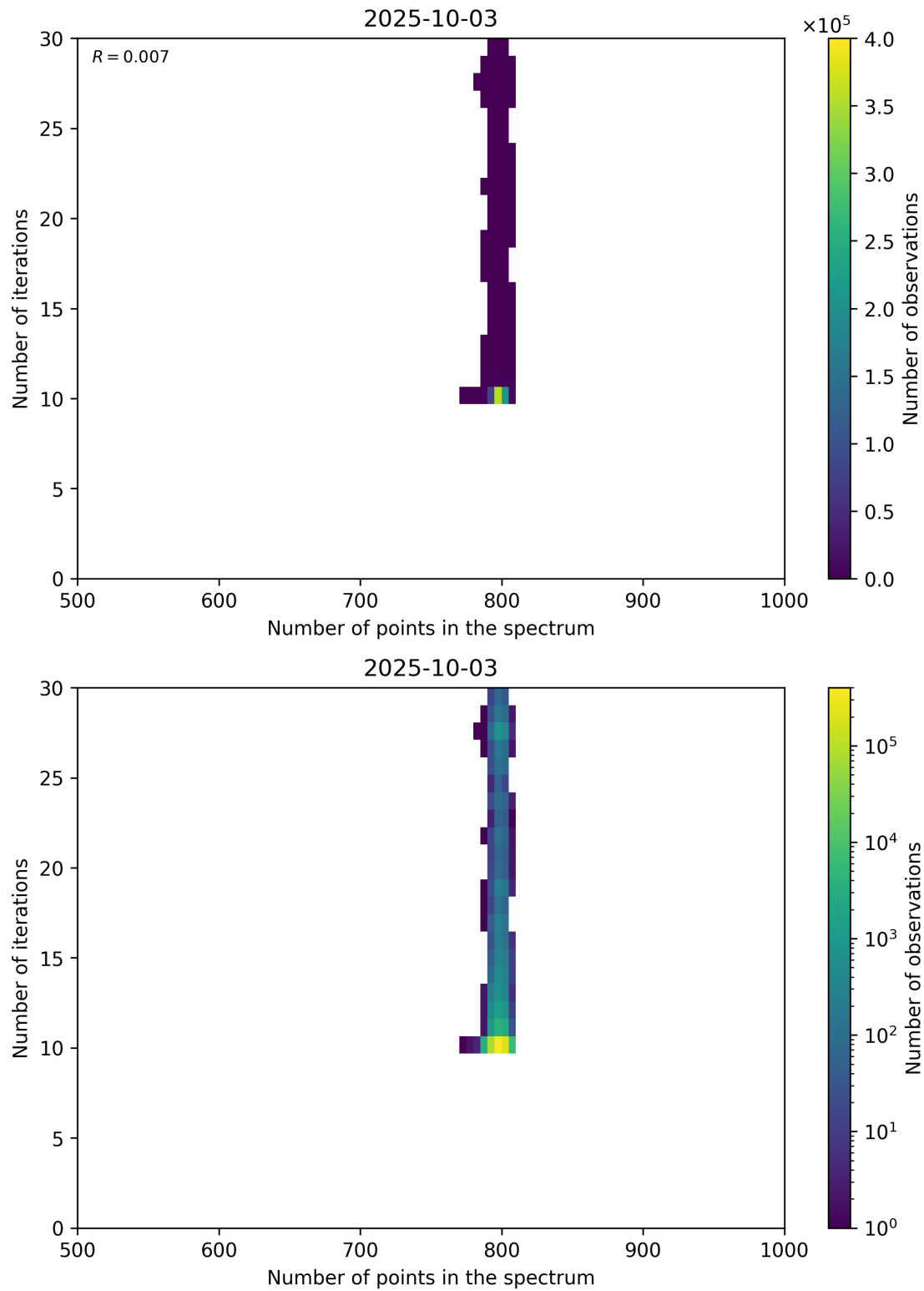
Figure 92: Scatter density plot of “Number of points in the spectrum” against “Number of iterations” for 2025-10-02 to 2025-10-04.
