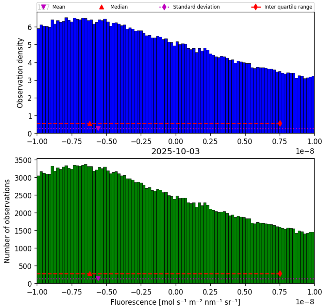
Figure 32: Histogram of “Fluorescence” for 2025-10-02 to 2025-10-04
