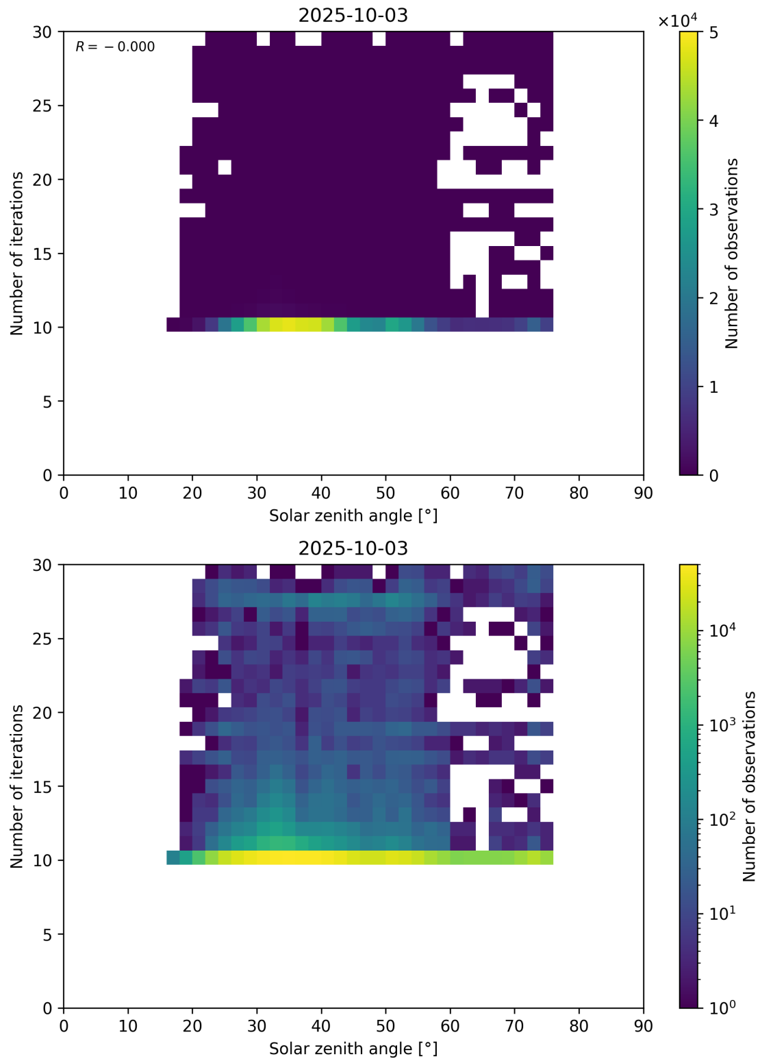
Figure 102: Scatter density plot of “Solar zenith angle” against “Number of iterations” for 2025-10-02 to 2025-10-04.
