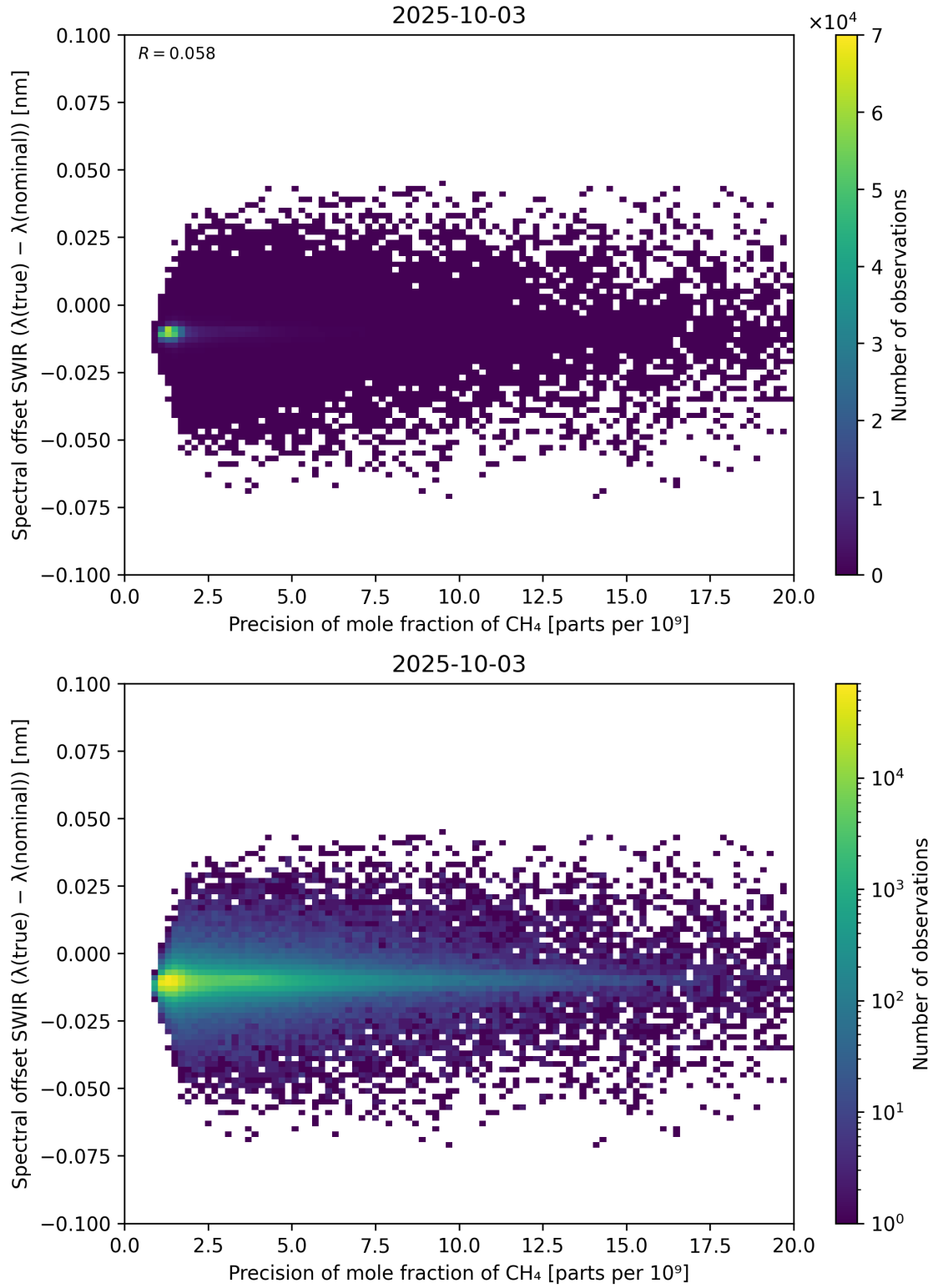
Figure 85: Scatter density plot of “Precision of mole fraction of \text{CH}_4 ” against “Spectral offset SWIR ( \lambda_{\text{true}} - \lambda_{\text{nominal}} )” for 2025-10-02 to 2025-10-04.
