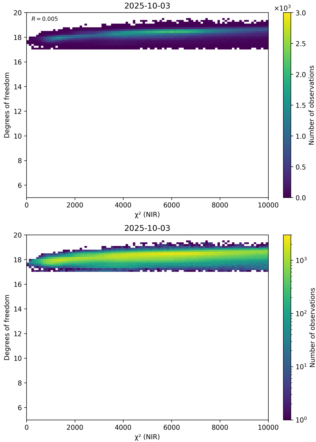
Figure 44: Scatter density plot of “ \chi^2 (NIR)” against “Degrees of freedom” for 2025-10-02 to 2025-10-04.
