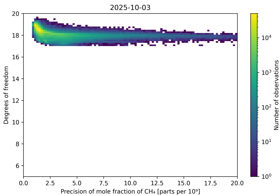
Figure 80: Scatter density plot of “Precision of mole fraction of CH 4 ” against “Degrees of freedom” for 2025-10-02 to 2025-10-04.
