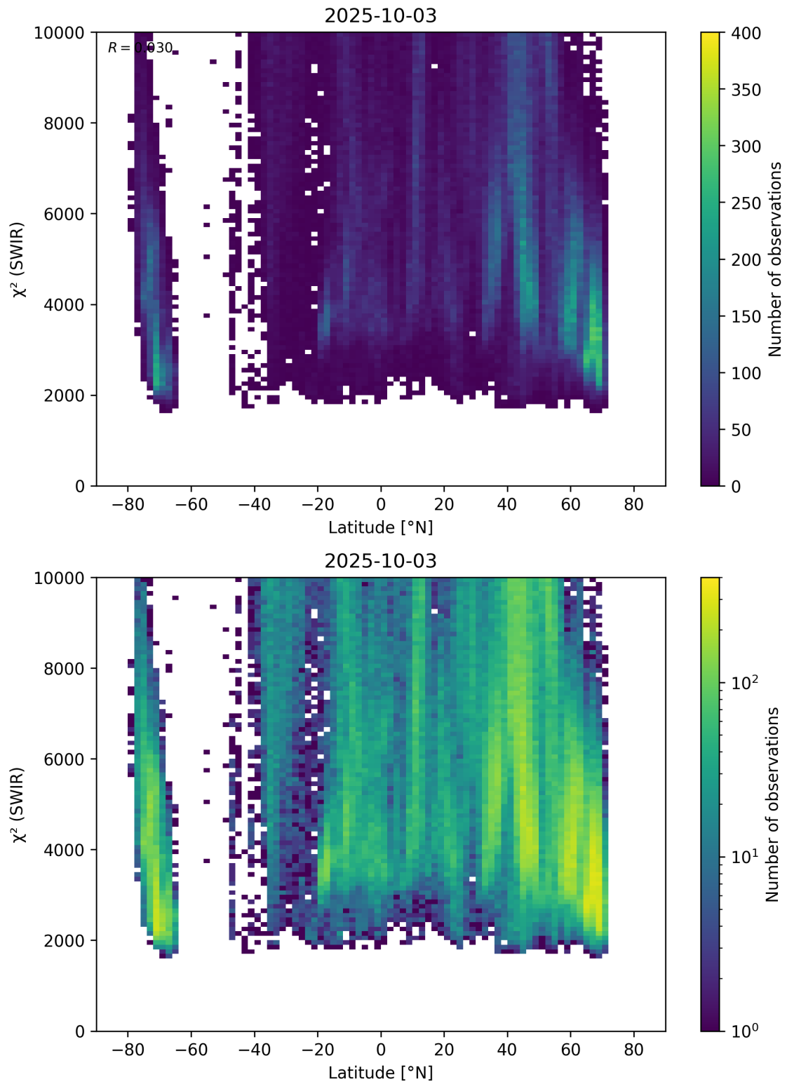
Figure 54: Scatter density plot of “Latitude” against “ \chi^2 (SWIR)” for 2025-10-02 to 2025-10-04.
