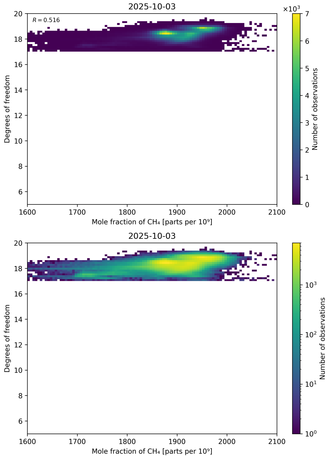
Figure 72: Scatter density plot of “Mole fraction of CH 4 ” against “Degrees of freedom” for 2025-10-02 to 2025-10-04.
