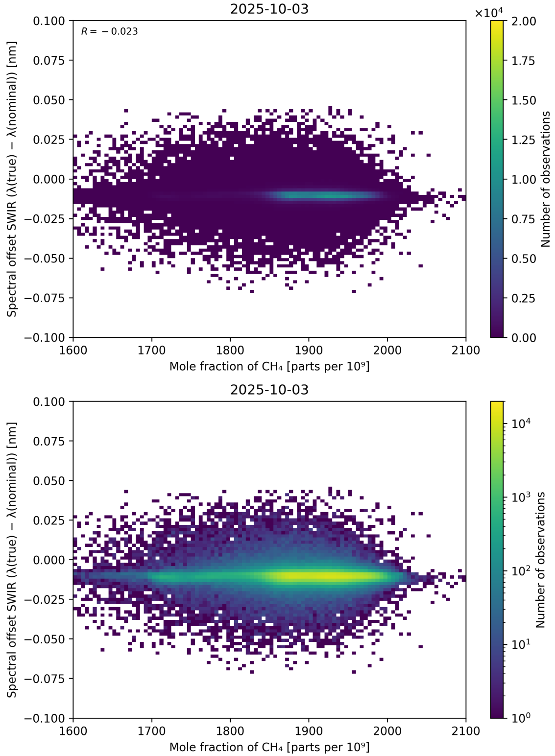
Figure 86: Scatter density plot of “Mole fraction of CH 4 ” against “Spectral offset SWIR ( \lambda_{\text{true}} - \lambda_{\text{nominal}} )” for 2025-10-02 to 2025-10-04.
