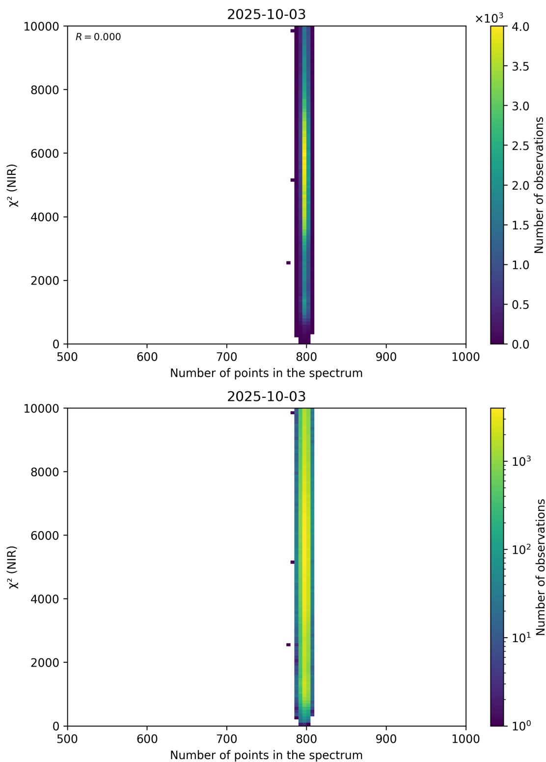
Figure 88: Scatter density plot of “Number of points in the spectrum” against “ \chi^2 (NIR)” for 2025-10-02 to 2025-10-04.
