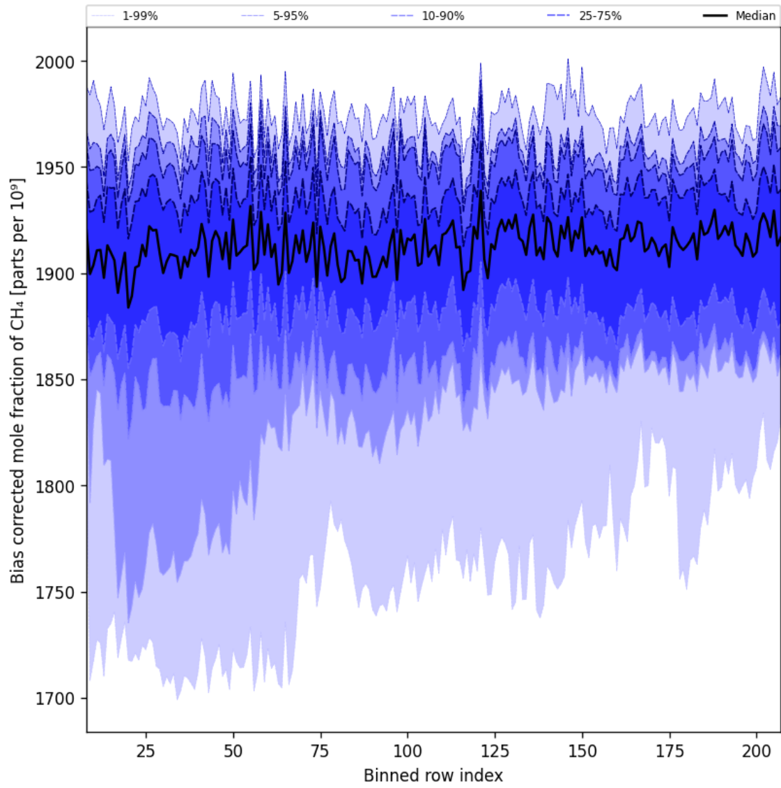
Figure 36: Along track statistics of “Bias corrected mole fraction of CH 4 ” for 2025-10-02 to 2025-10-04
