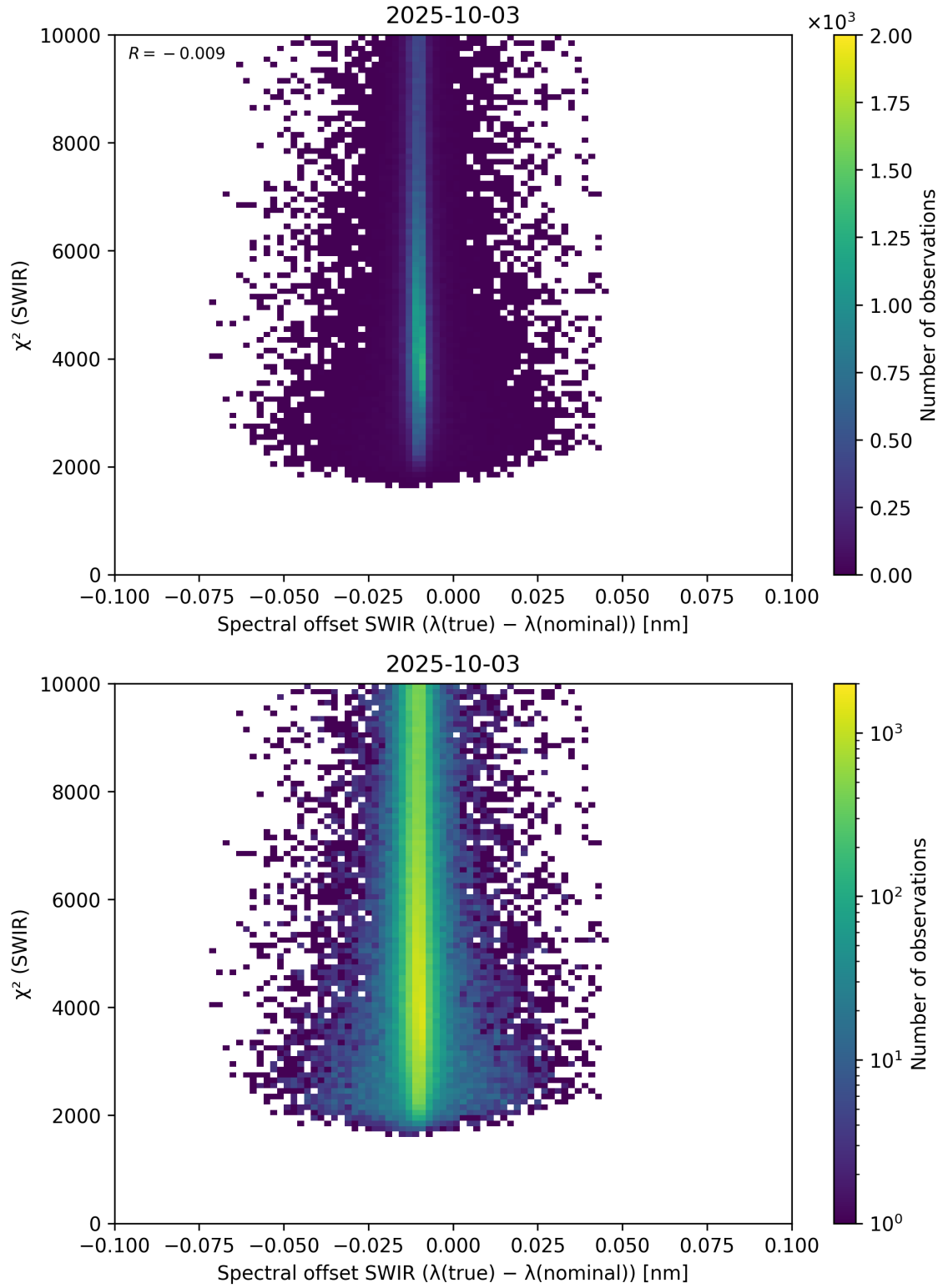
Figure 118: Scatter density plot of “Spectral offset SWIR ( \lambda_{\text{true}} - \lambda_{\text{nominal}} )” against “ \chi^2 (SWIR)” for 2025-10-02 to 2025-10-04.
