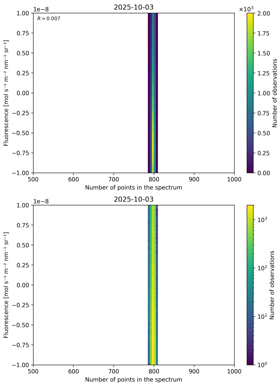
Figure 91: Scatter density plot of “Number of points in the spectrum” against “Fluorescence” for 2025-10-02 to 2025-10-04.
