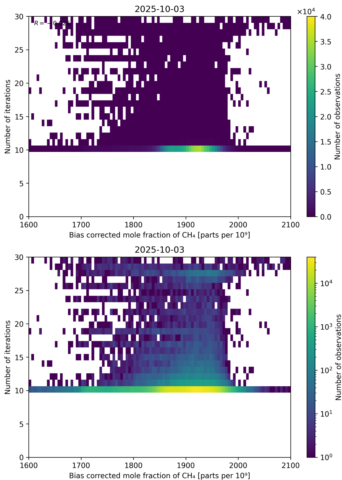
Figure 67: Scatter density plot of “Bias corrected mole fraction of CH 4 ” against “Number of iterations” for 2025-10-02 to 2025-10-04.
