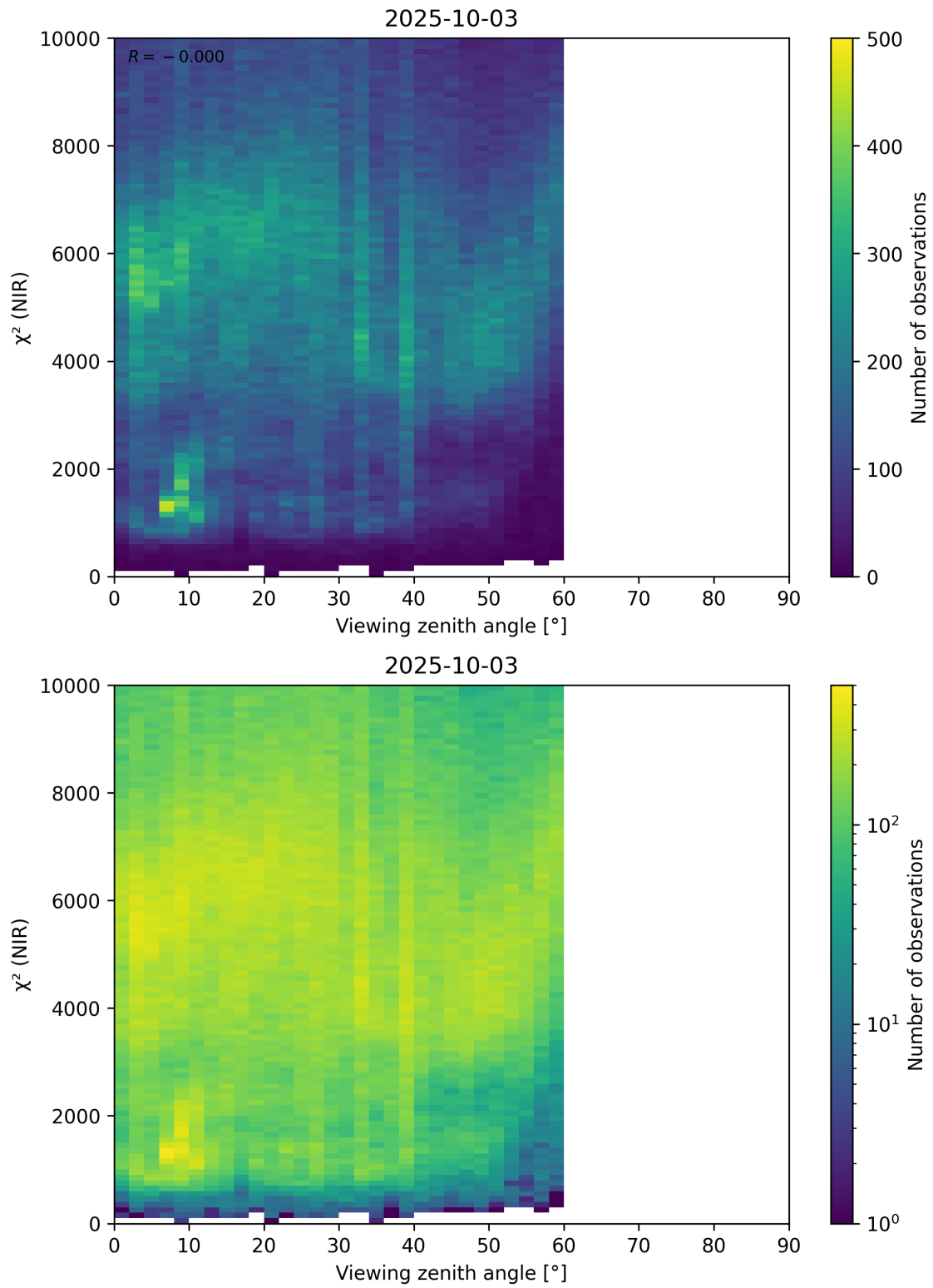
Figure 105: Scatter density plot of “Viewing zenith angle” against “ \chi^2 (NIR)” for 2025-10-02 to 2025-10-04.
