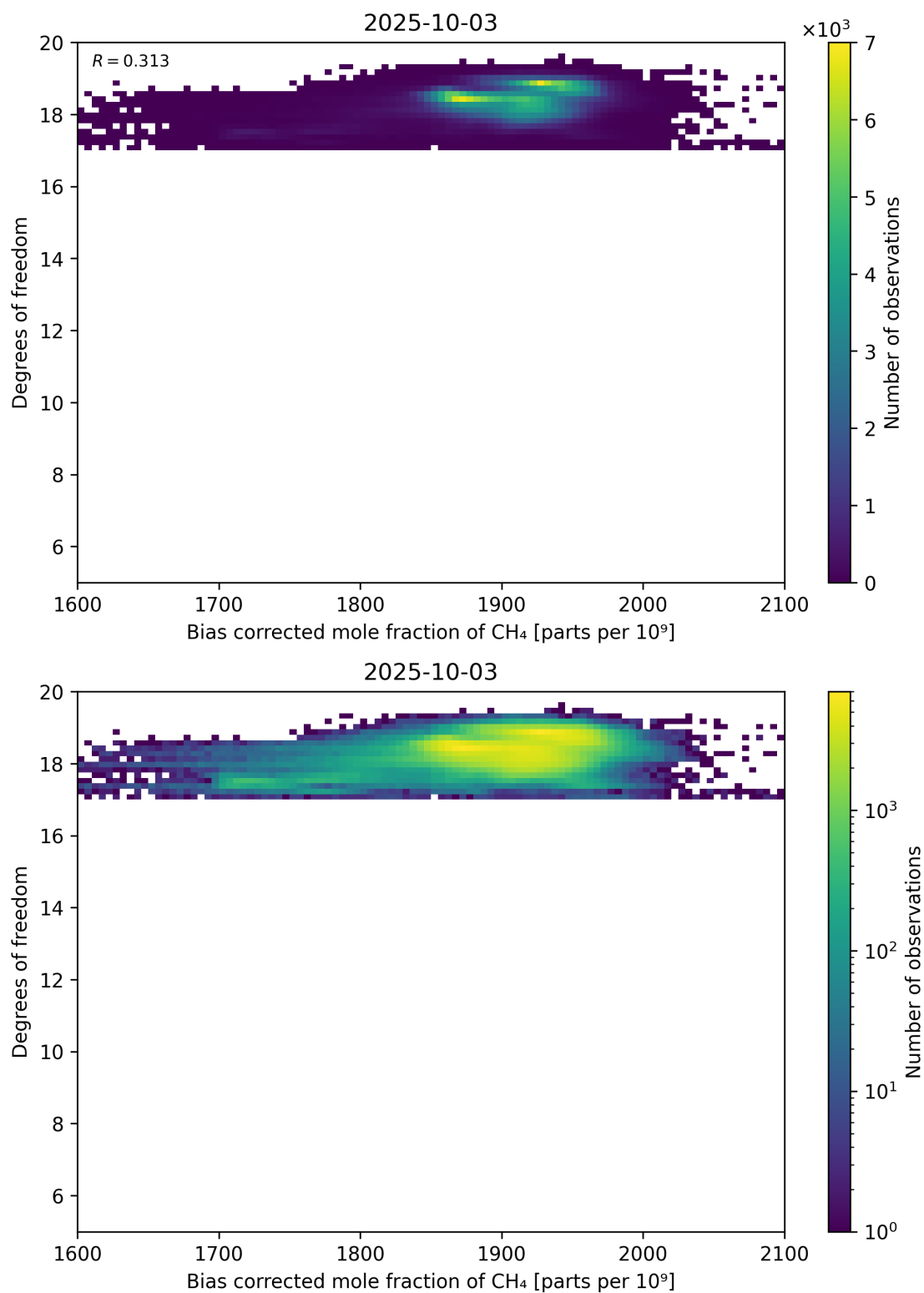
Figure 65: Scatter density plot of “Bias corrected mole fraction of CH 4 ” against “Degrees of freedom” for 2025-10-02 to 2025-10-04.
