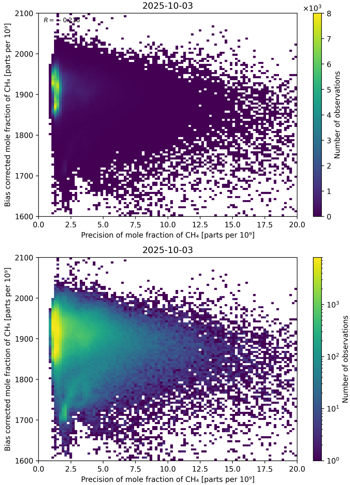
Figure 82: Scatter density plot of “Precision of mole fraction of CH 4 ” against “Bias corrected mole fraction of CH 4 ” for 2025-10-02 to 2025-10-04.
