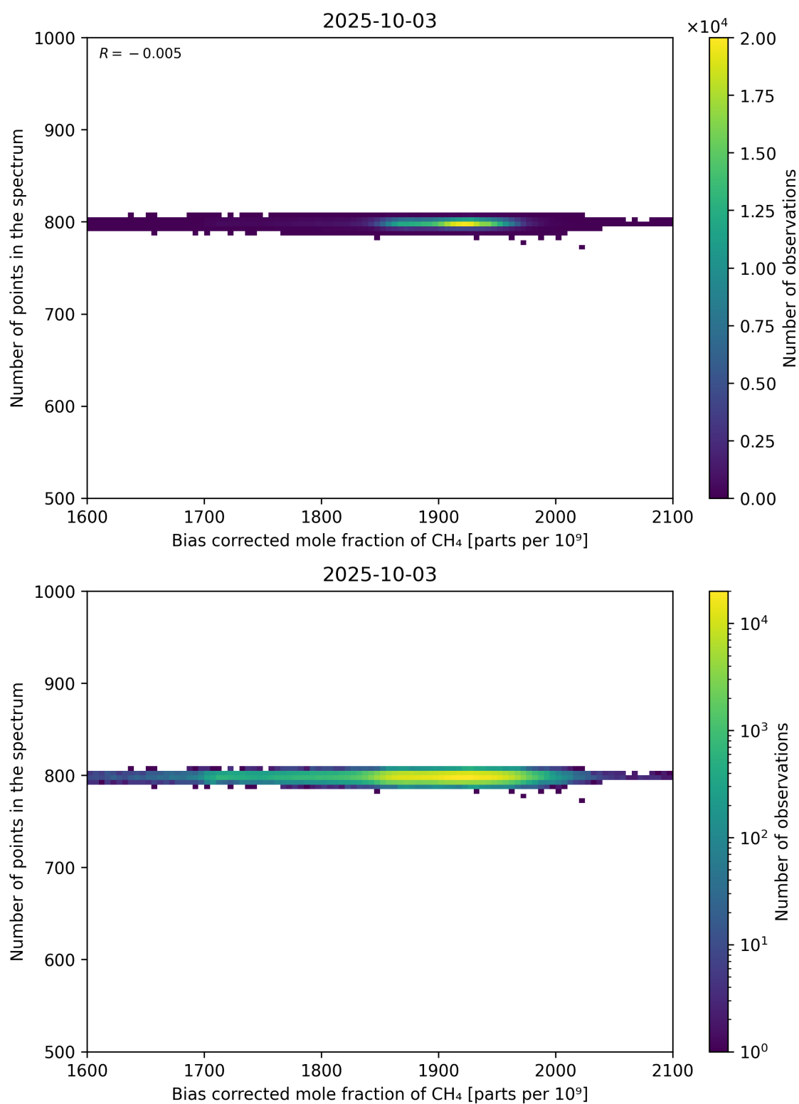
Figure 68: Scatter density plot of “Bias corrected mole fraction of CH 4 ” against “Number of points in the spectrum” for 2025-10-02 to 2025-10-04.
