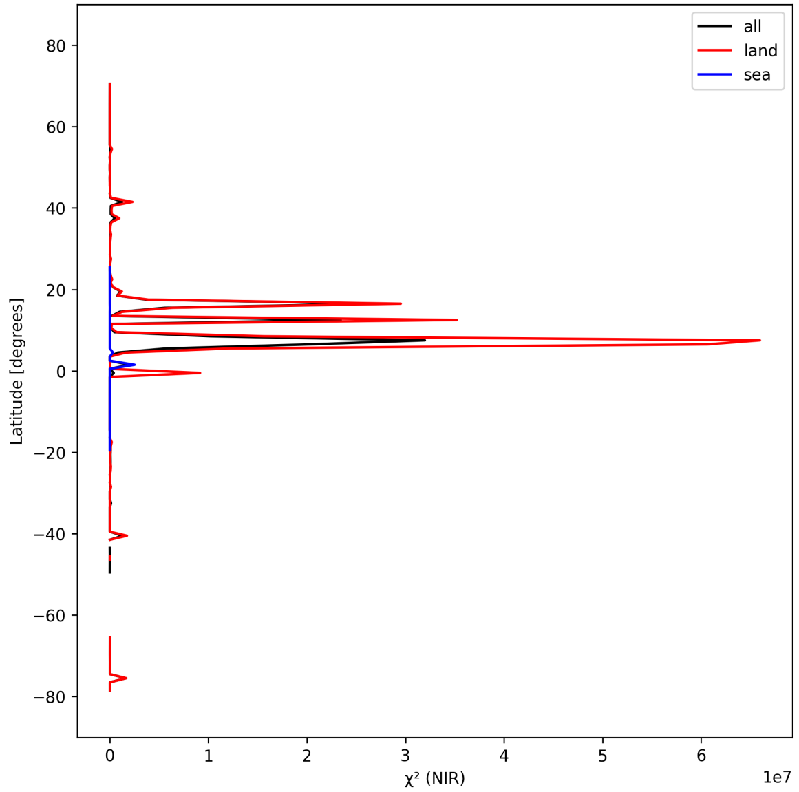
Figure 18: Zonal average of “ \chi^2 (NIR)” for 2025-10-02 to 2025-10-04.
