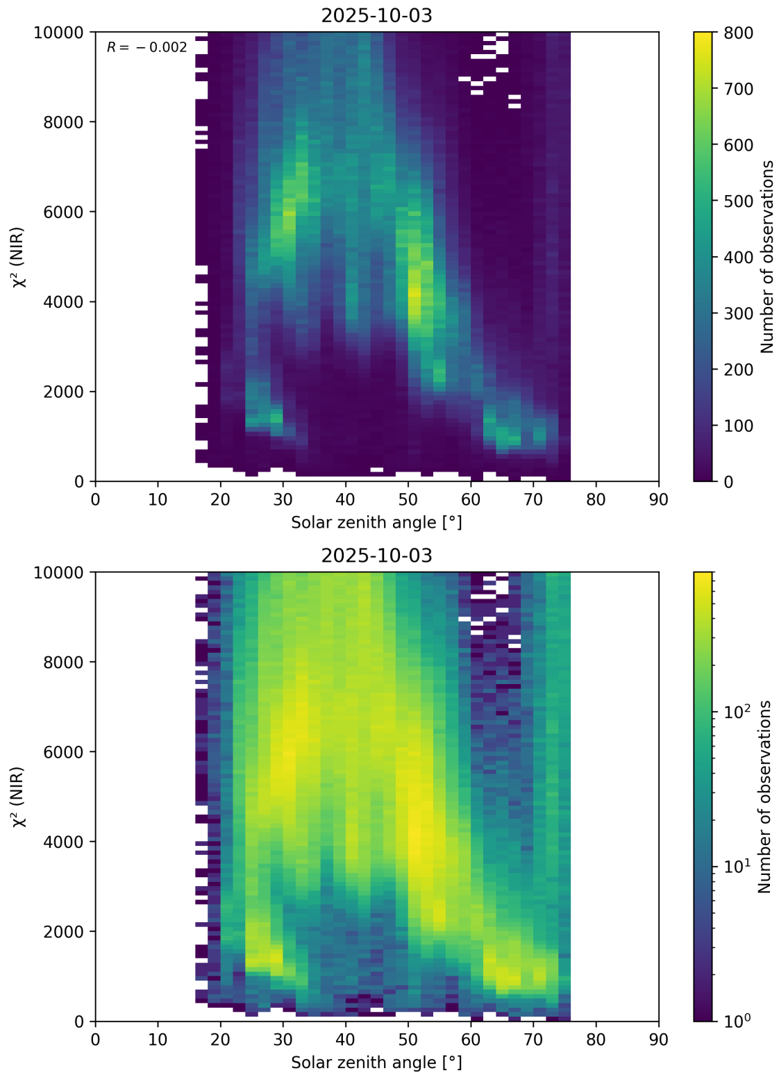
Figure 94: Scatter density plot of “Solar zenith angle” against “ \chi^2 (NIR)” for 2025-10-02 to 2025-10-04.
