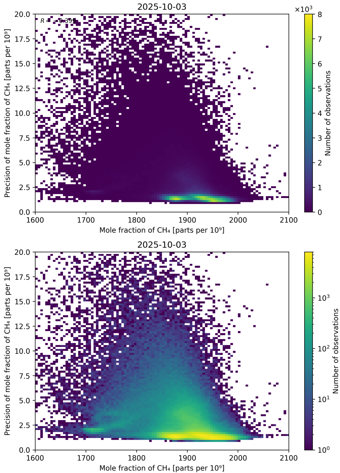
Figure 75: Scatter density plot of “Mole fraction of CH 4 ” against “Precision of mole fraction of CH 4 ” for 2025-10-02 to 2025-10-04.
