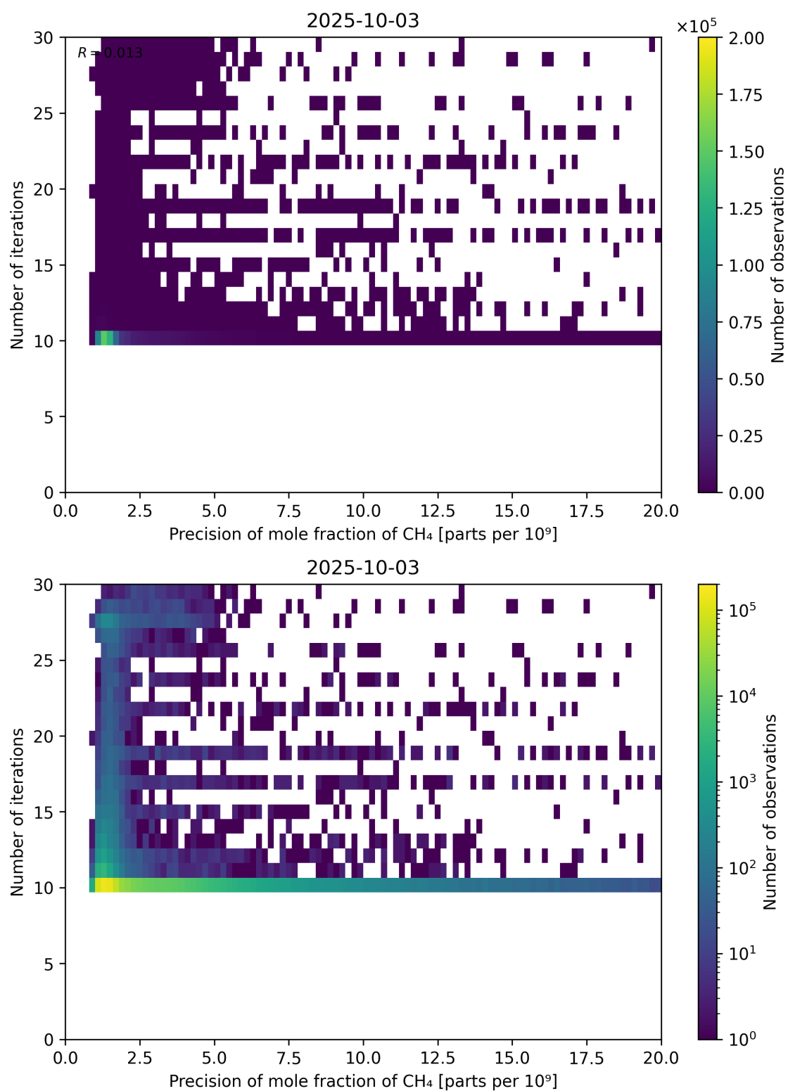
Figure 83: Scatter density plot of “Precision of mole fraction of CH 4 ” against “Number of iterations” for 2025-10-02 to 2025-10-04.
