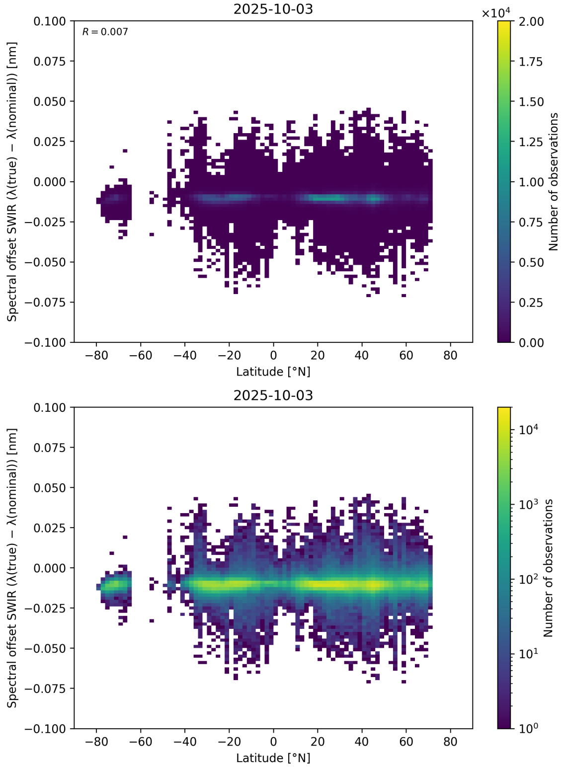
Figure 62: Scatter density plot of “Latitude” against “Spectral offset SWIR ( \lambda_{\text{true}} - \lambda_{\text{nominal}} )” for 2025-10-02 to 2025-10-04.
