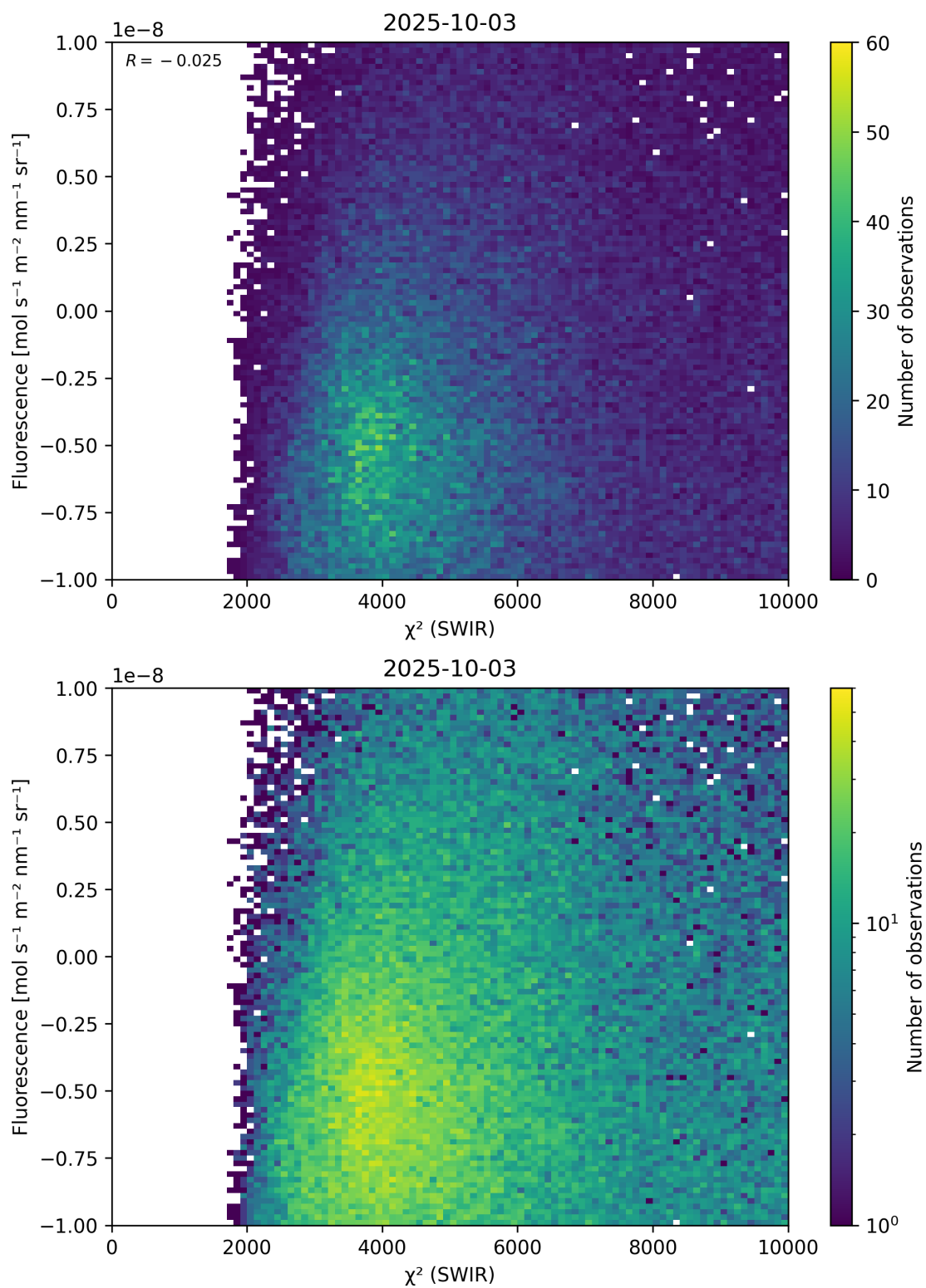
Figure 49: Scatter density plot of “ \chi^2 (SWIR)” against “Fluorescence” for 2025-10-02 to 2025-10-04.
