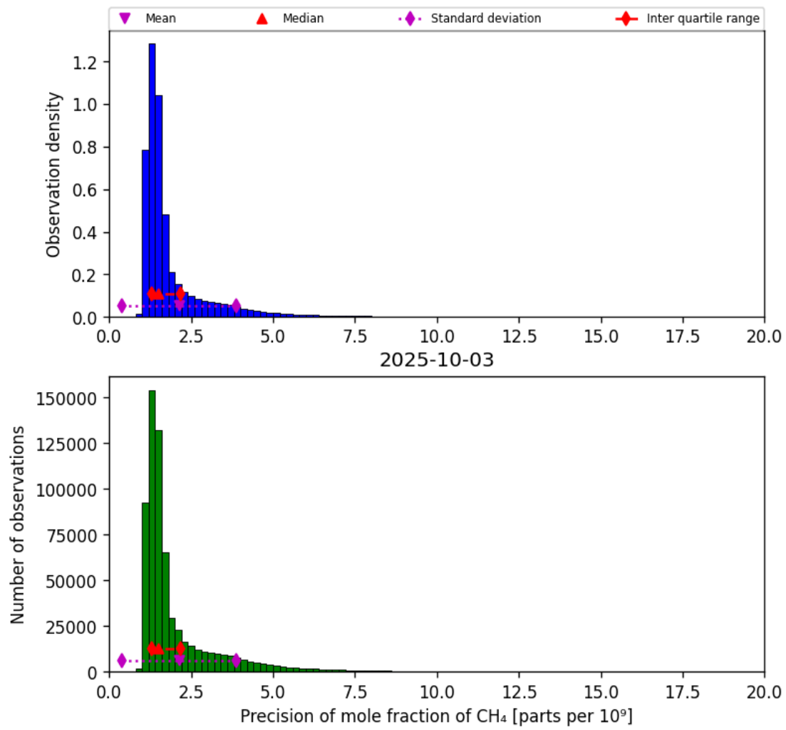
Figure 24: Histogram of “Precision of mole fraction of CH 4 ” for 2025-10-02 to 2025-10-04
