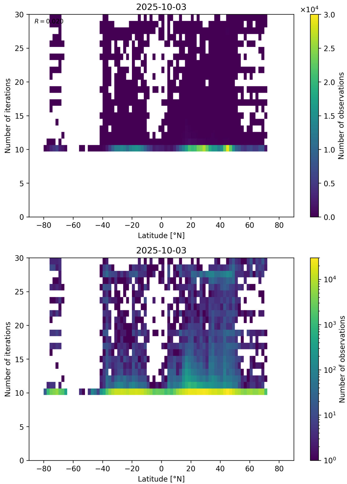
Figure 60: Scatter density plot of “Latitude” against “Number of iterations” for 2025-10-02 to 2025-10-04.
