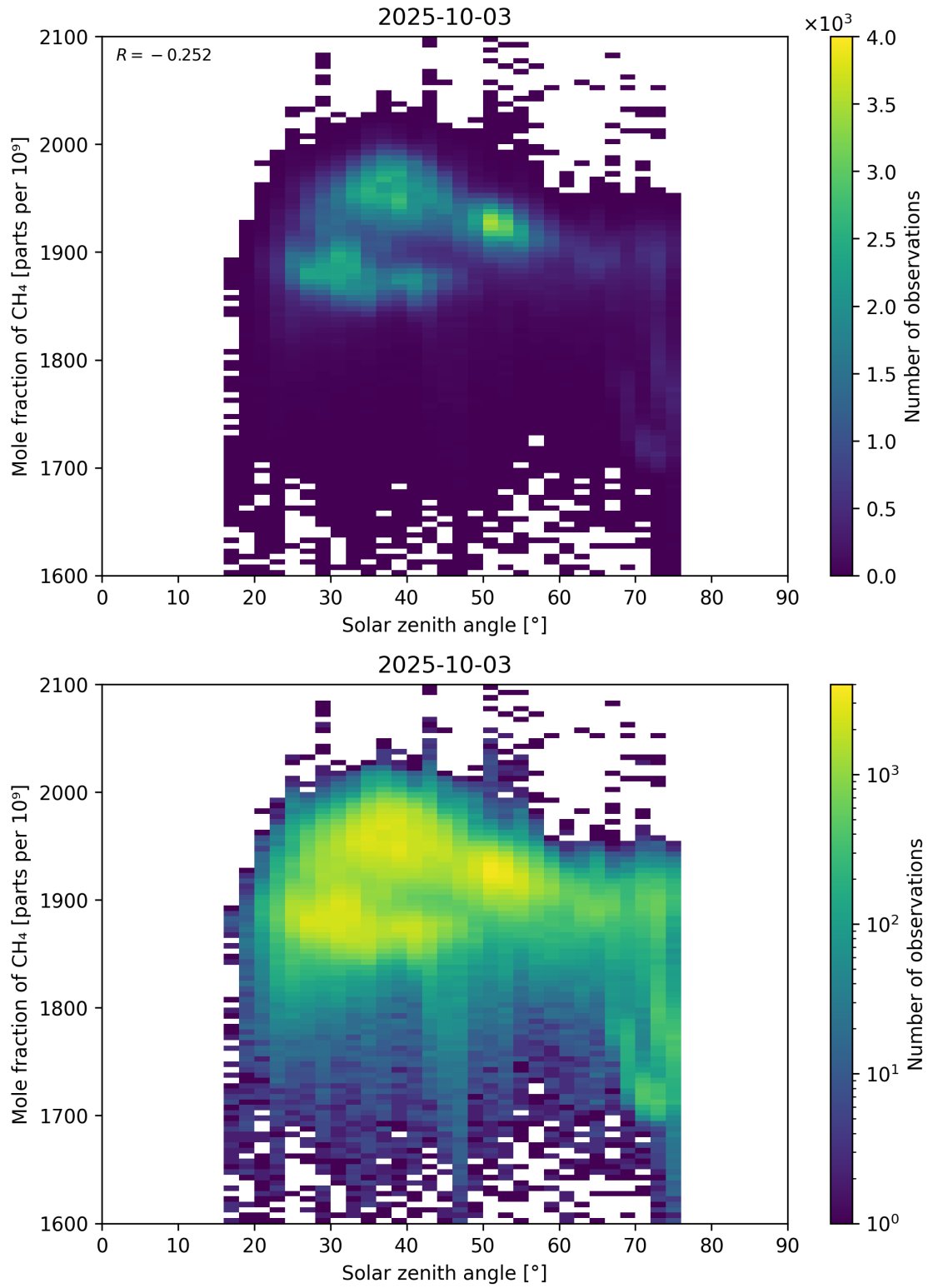
Figure 99: Scatter density plot of “Solar zenith angle” against “Mole fraction of CH 4 ” for 2025-10-02 to 2025-10-04.
