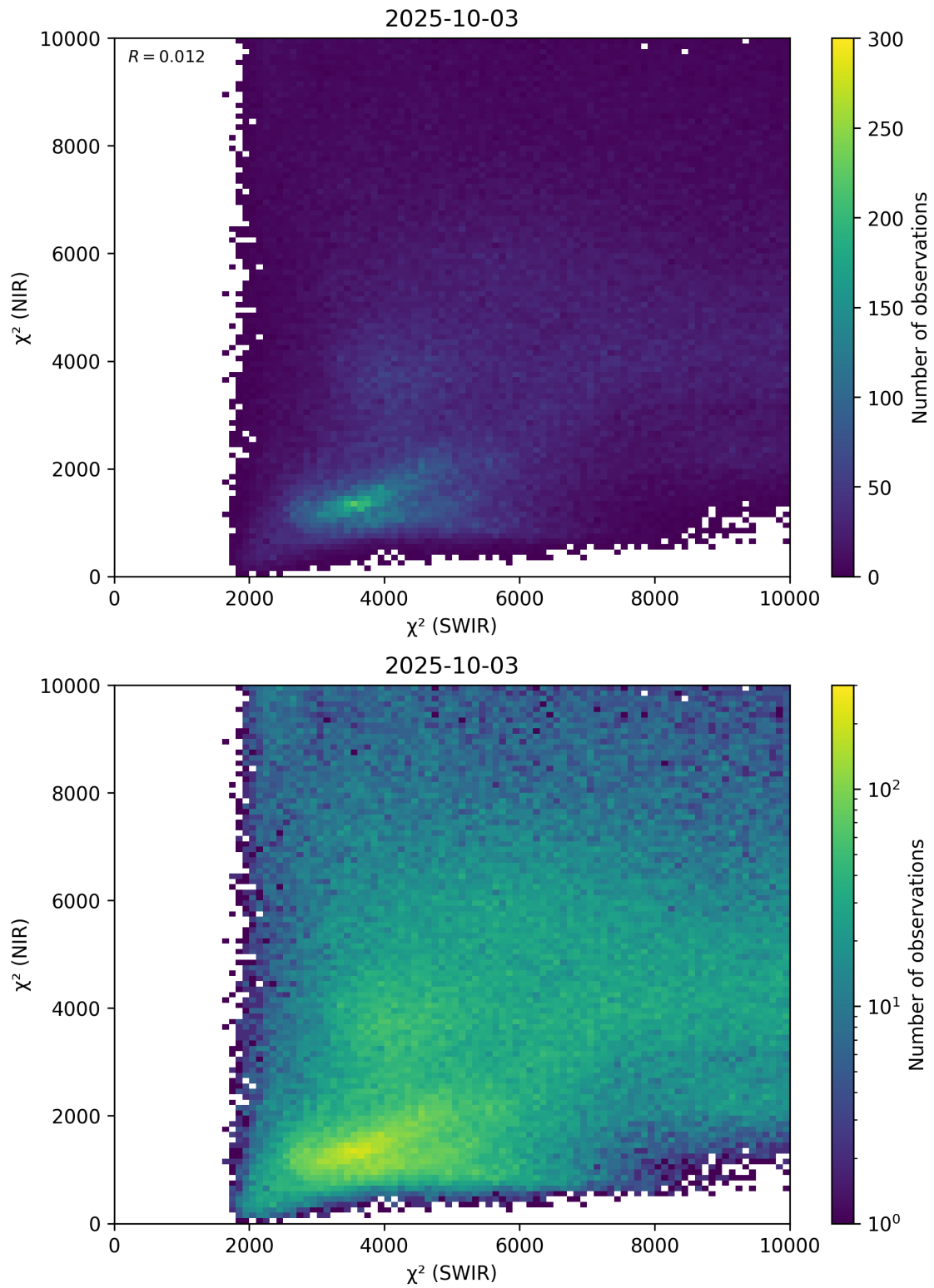
Figure 47: Scatter density plot of “ \chi^2 (SWIR)” against “ \chi^2 (NIR)” for 2025-10-02 to 2025-10-04.
