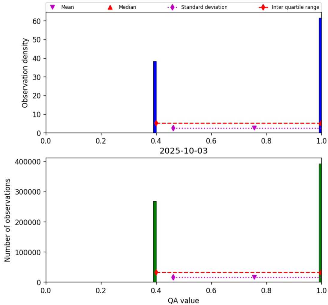
Figure 22: Histogram of “QA value” for 2025-10-02 to 2025-10-04
