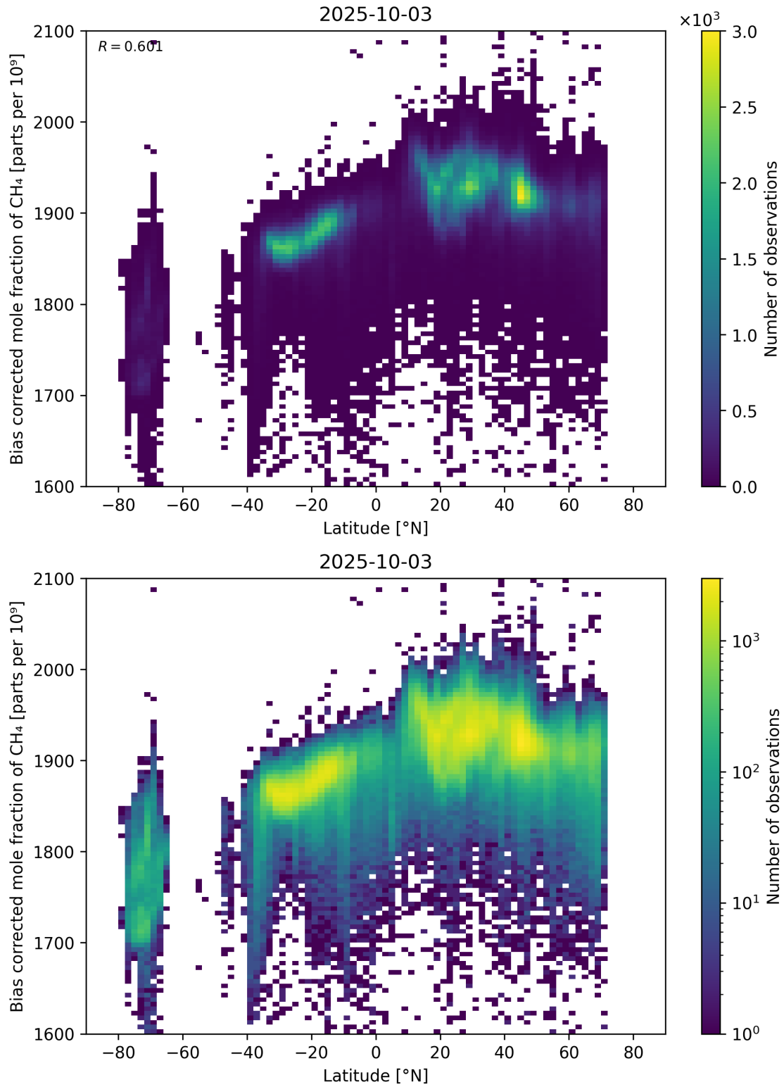
Figure 58: Scatter density plot of “Latitude” against “Bias corrected mole fraction of CH 4 ” for 2025-10-02 to 2025-10-04.
