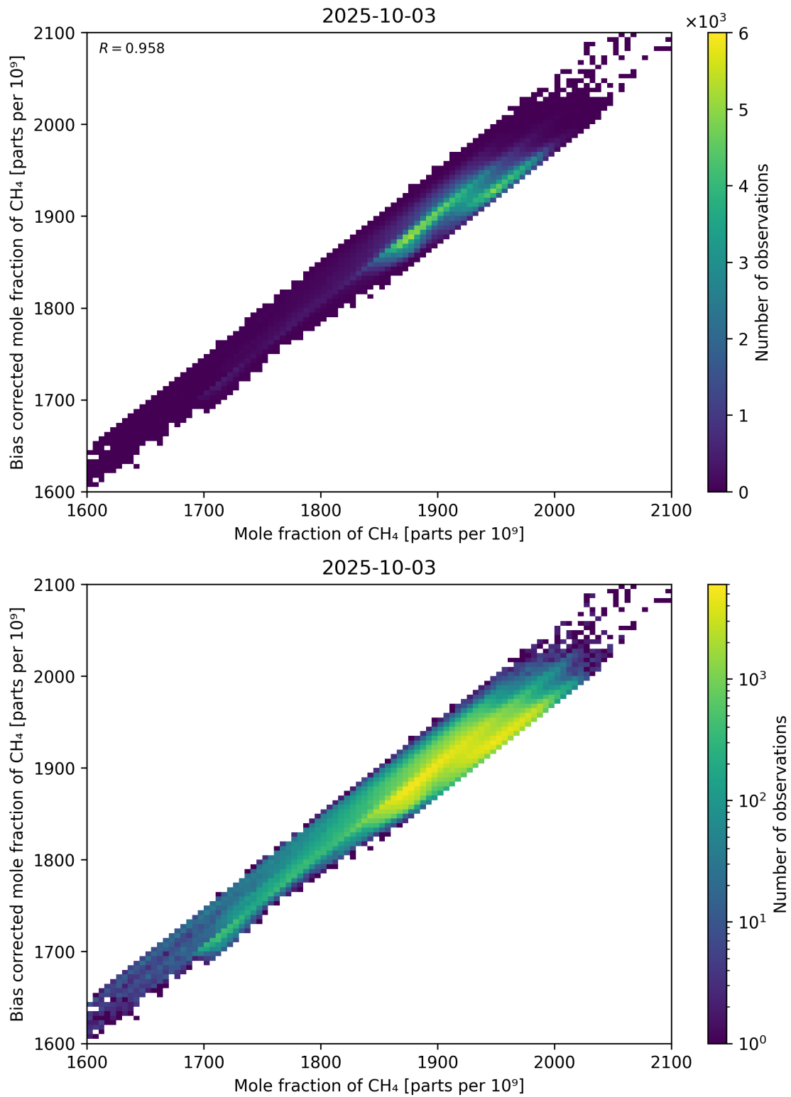
Figure 74: Scatter density plot of “Mole fraction of CH 4 ” against “Bias corrected mole fraction of CH 4 ” for 2025-10-02 to 2025-10-04.
