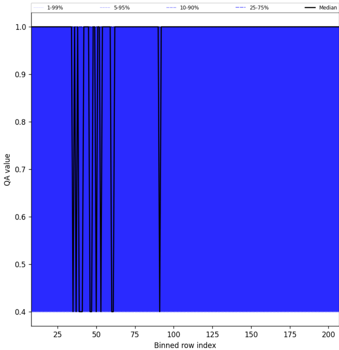
Figure 33: Along track statistics of “QA value” for 2025-10-02 to 2025-10-04
