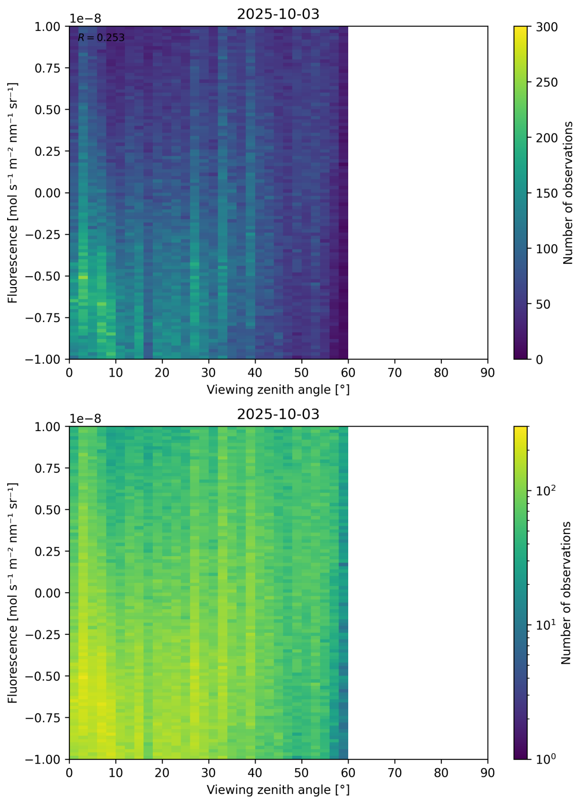
Figure 108: Scatter density plot of “Viewing zenith angle” against “Fluorescence” for 2025-10-02 to 2025-10-04.
