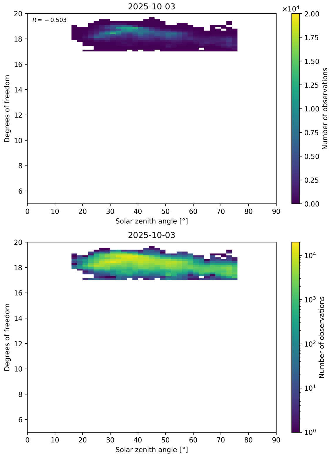
Figure 96: Scatter density plot of “Solar zenith angle” against “Degrees of freedom” for 2025-10-02 to 2025-10-04.
