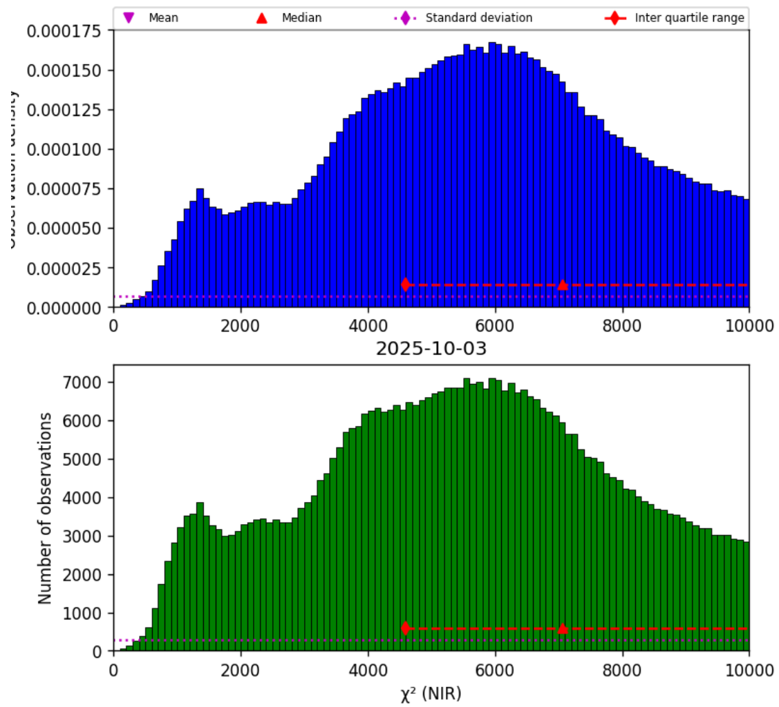
Figure 29: Histogram of “ \chi^2 (NIR)” for 2025-10-02 to 2025-10-04
