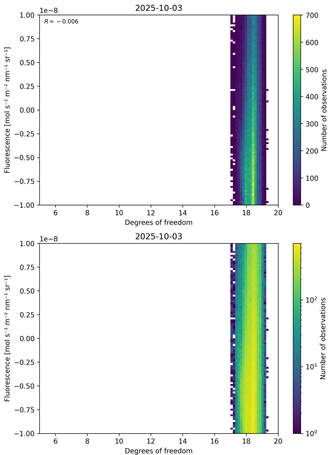
Figure 51: Scatter density plot of “Degrees of freedom” against “Fluorescence” for 2025-10-02 to 2025-10-04.
