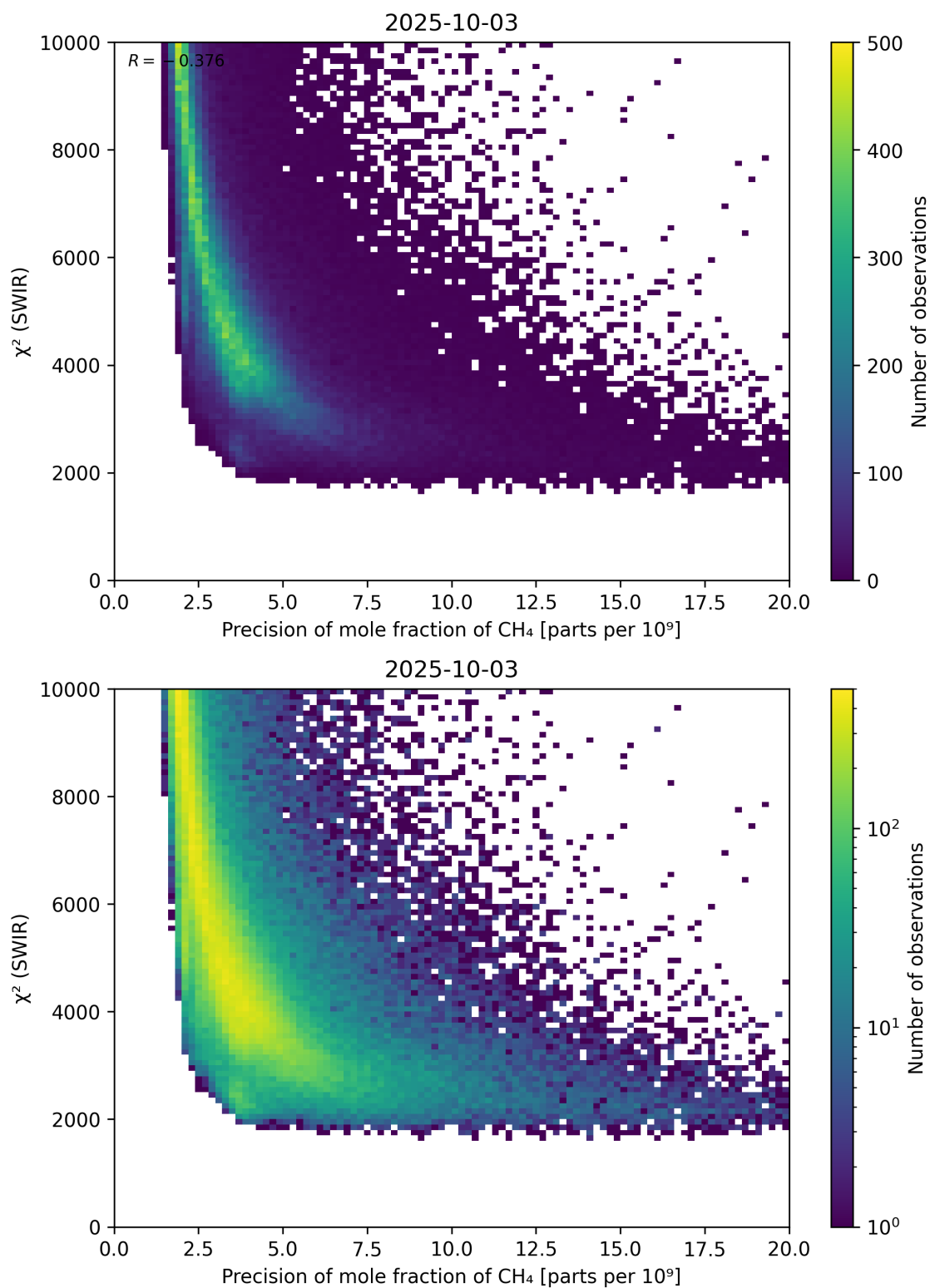
Figure 79: Scatter density plot of “Precision of mole fraction of CH 4 ” against “ \chi^2 (SWIR)” for 2025-10-02 to 2025-10-04.
