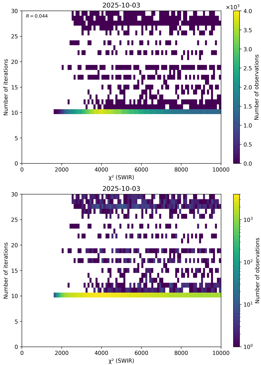
Figure 50: Scatter density plot of “ \chi^2 (SWIR)” against “Number of iterations” for 2025-10-02 to 2025-10-04.
