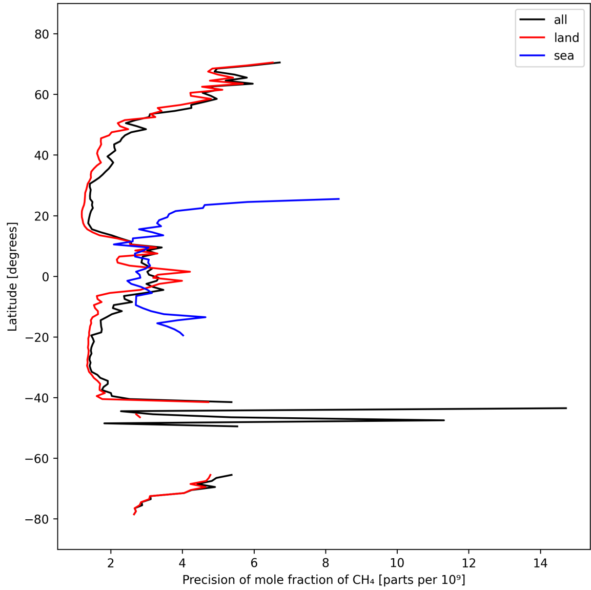
Figure 13: Zonal average of “Precision of mole fraction of CH 4 ” for 2025-10-02 to 2025-10-04.
