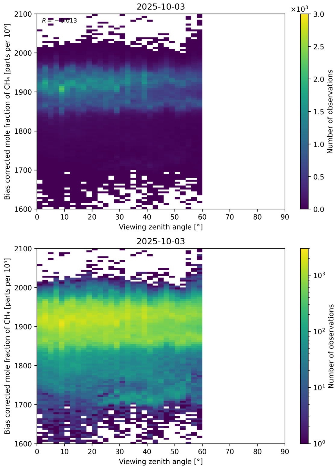
Figure 111: Scatter density plot of “Viewing zenith angle” against “Bias corrected mole fraction of CH 4 ” for 2025-10-02 to 2025-10-04.
