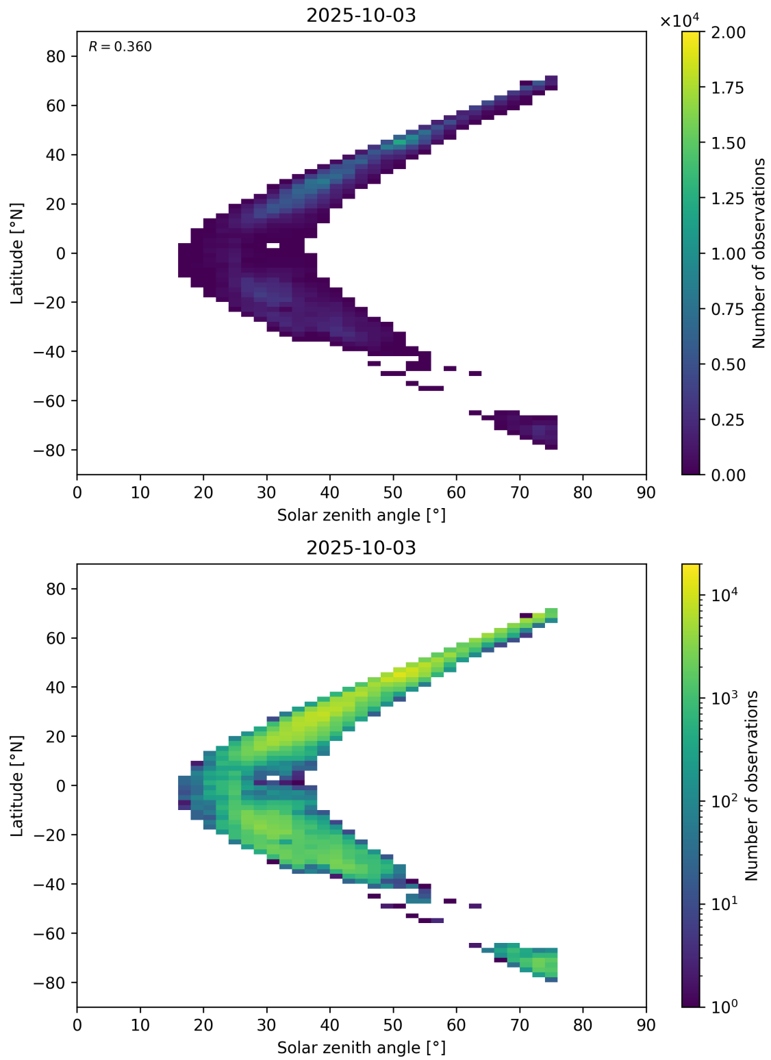
Figure 98: Scatter density plot of “Solar zenith angle” against “Latitude” for 2025-10-02 to 2025-10-04.
