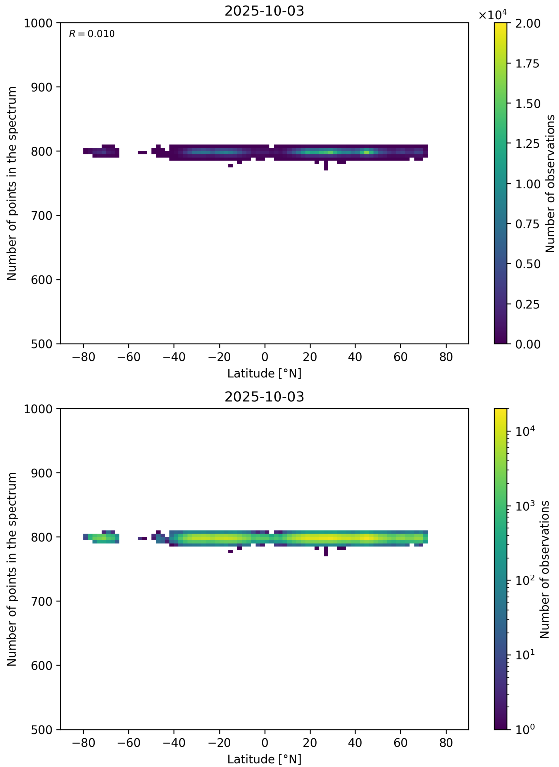
Figure 61: Scatter density plot of “Latitude” against “Number of points in the spectrum” for 2025-10-02 to 2025-10-04.
