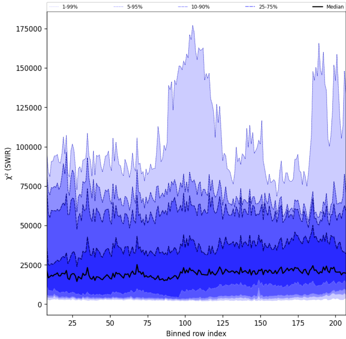
Figure 39: Along track statistics of " \chi^2 (SWIR)" for 2025-10-02 to 2025-10-04
