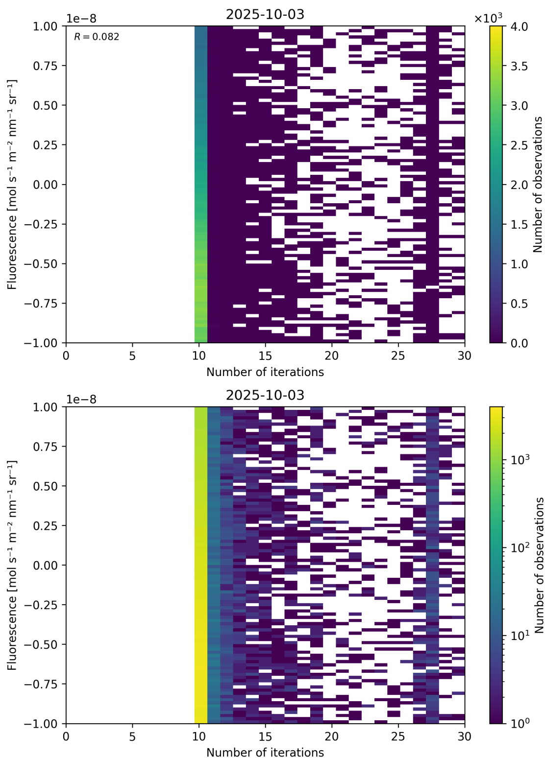
Figure 87: Scatter density plot of “Number of iterations” against “Fluorescence” for 2025-10-02 to 2025-10-04.
