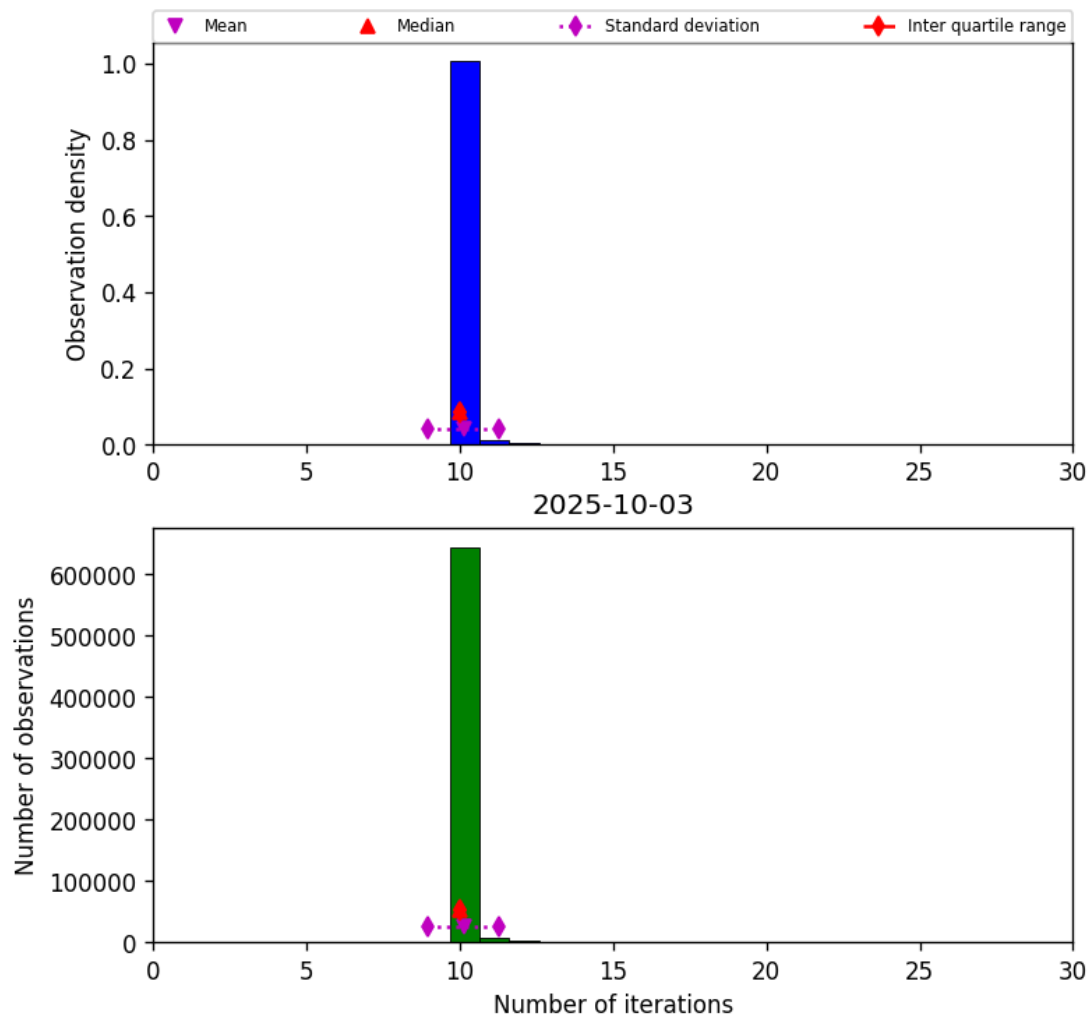
Figure 31: Histogram of “Number of iterations” for 2025-10-02 to 2025-10-04
