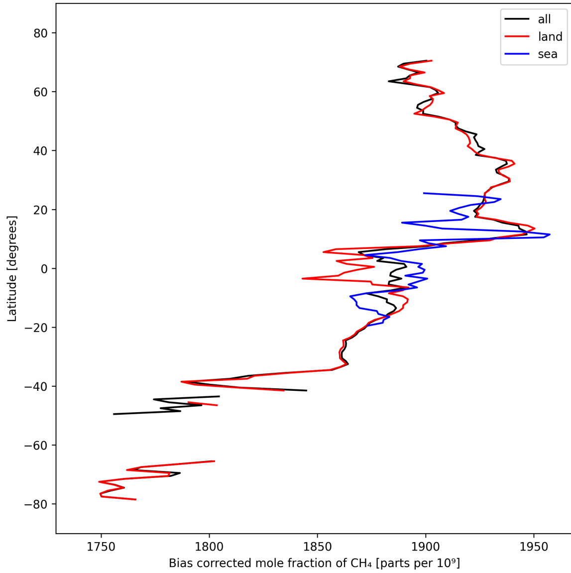
Figure 14: Zonal average of “Bias corrected mole fraction of CH 4 ” for 2025-10-02 to 2025-10-04.
