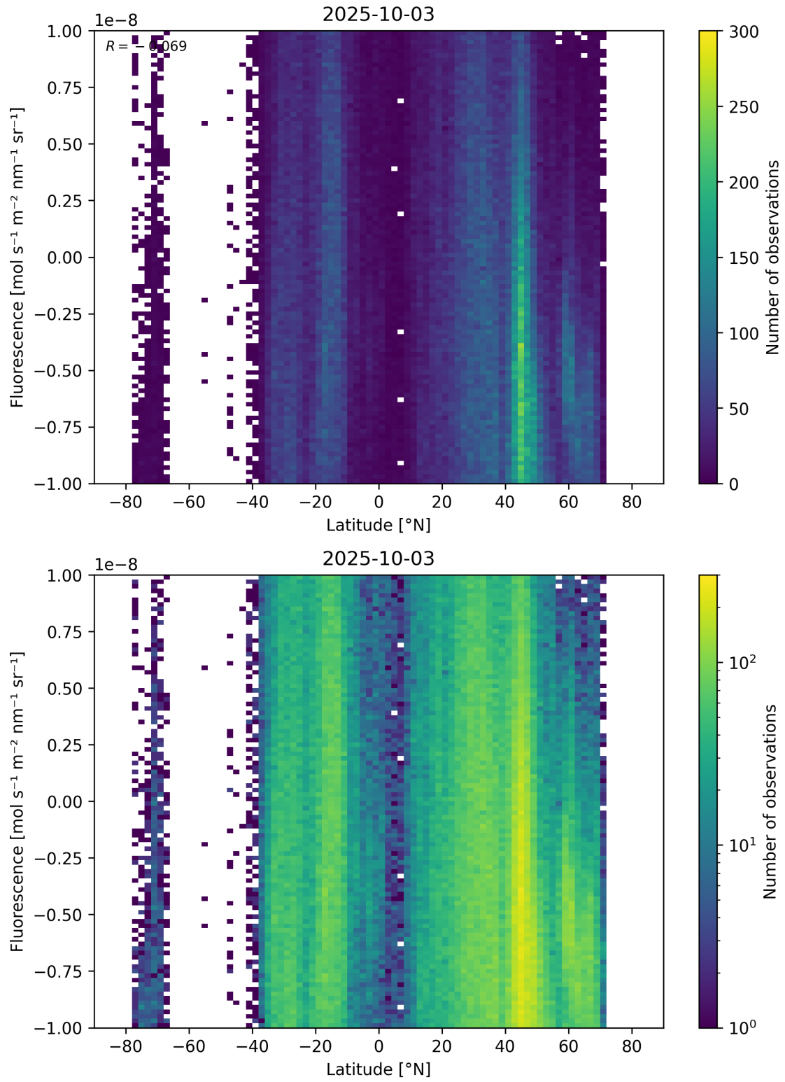
Figure 56: Scatter density plot of “Latitude” against “Fluorescence” for 2025-10-02 to 2025-10-04.
