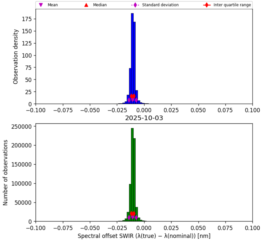
Figure 27: Histogram of “Spectral offset SWIR ( \lambda_{\text{true}} - \lambda_{\text{nominal}} )” for 2025-10-02 to 2025-10-04
