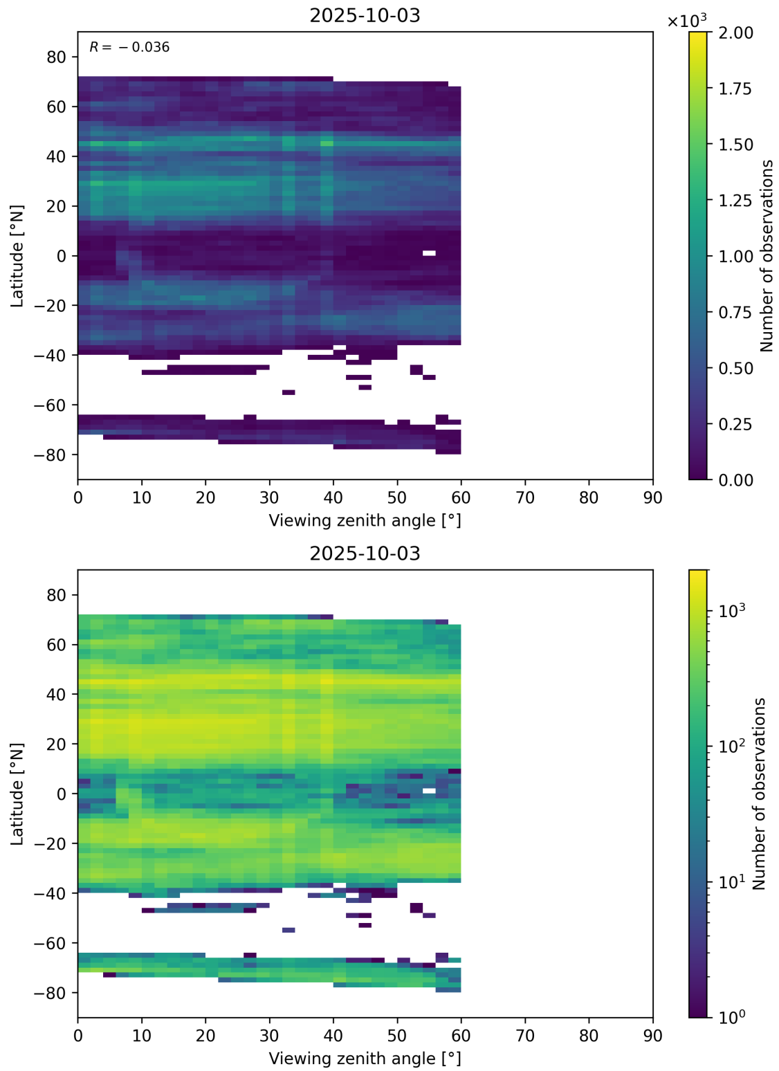
Figure 109: Scatter density plot of “Viewing zenith angle” against “Latitude” for 2025-10-02 to 2025-10-04.
