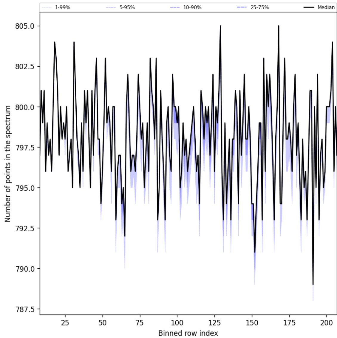
Figure 37: Along track statistics of “Number of points in the spectrum” for 2025-10-02 to 2025-10-04
