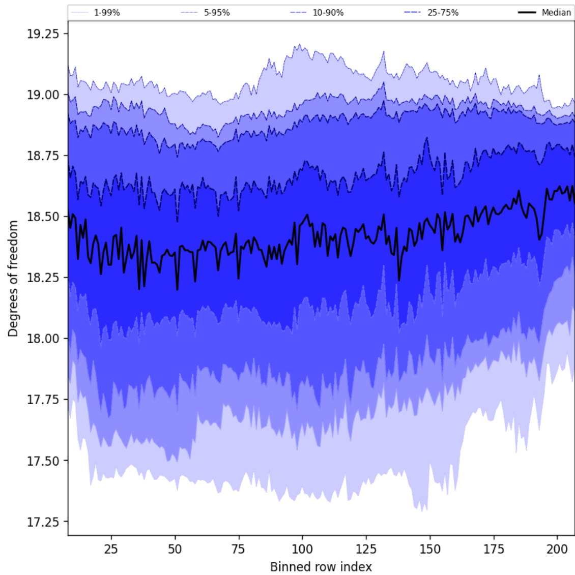
Figure 41: Along track statistics of “Degrees of freedom” for 2025-10-02 to 2025-10-04
