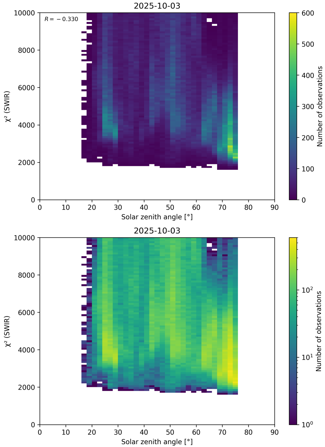
Figure 95: Scatter density plot of “Solar zenith angle” against “ \chi^2 (SWIR)” for 2025-10-02 to 2025-10-04.
