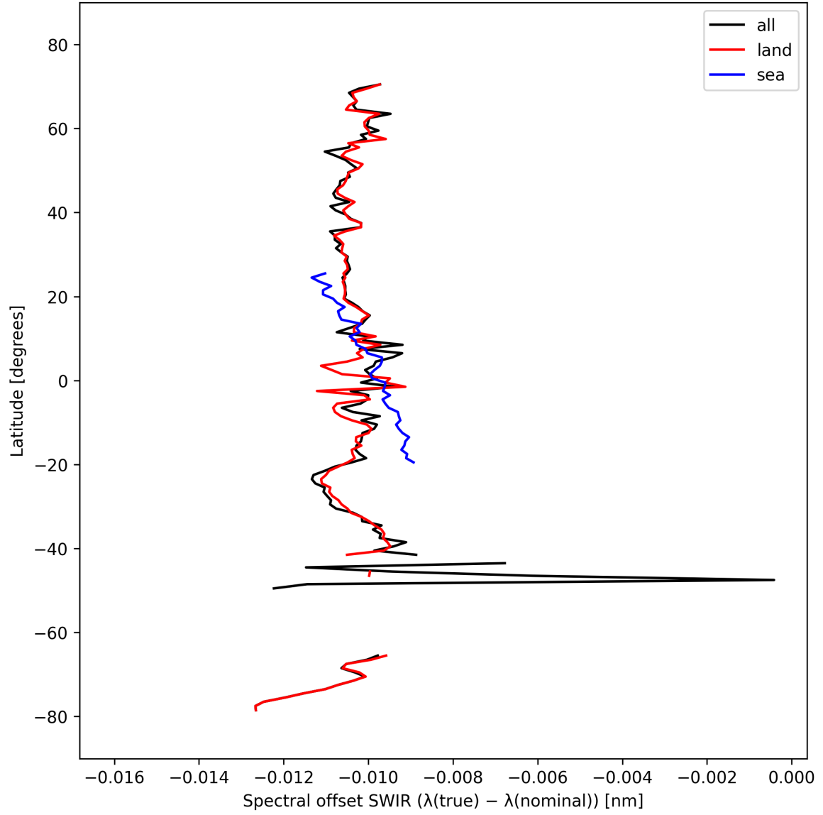
Figure 16: Zonal average of “Spectral offset SWIR ( \lambda_{\text{true}} - \lambda_{\text{nominal}} )” for 2025-10-02 to 2025-10-04.
