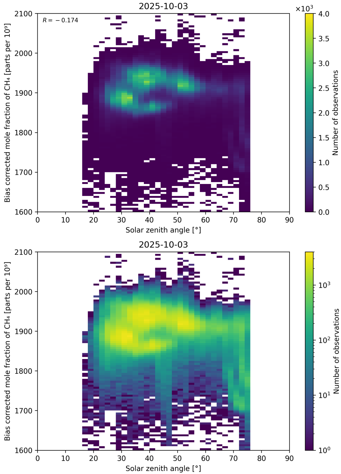
Figure 100: Scatter density plot of “Solar zenith angle” against “Bias corrected mole fraction of \text{CH}_4 ” for 2025-10-02 to 2025-10-04.
