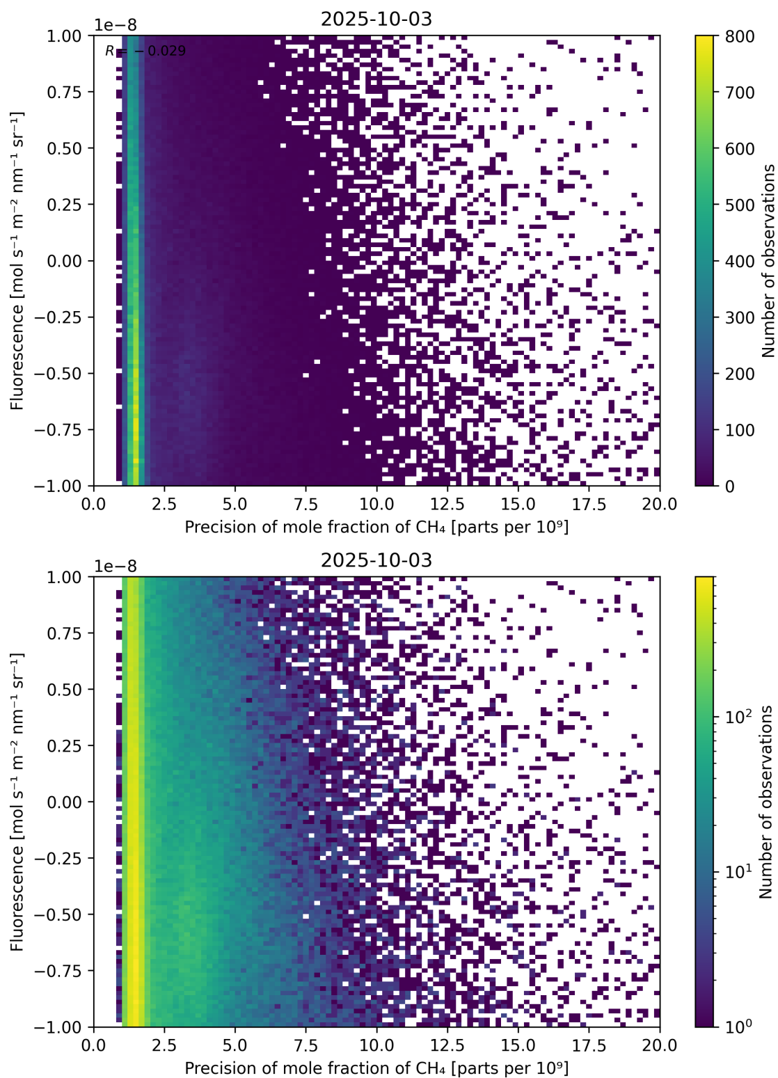
Figure 81: Scatter density plot of “Precision of mole fraction of \text{CH}_4 ” against “Fluorescence” for 2025-10-02 to 2025-10-04.
