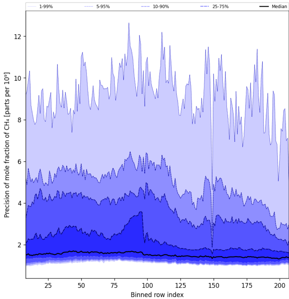
Figure 35: Along track statistics of “Precision of mole fraction of CH 4 ” for 2025-10-02 to 2025-10-04
