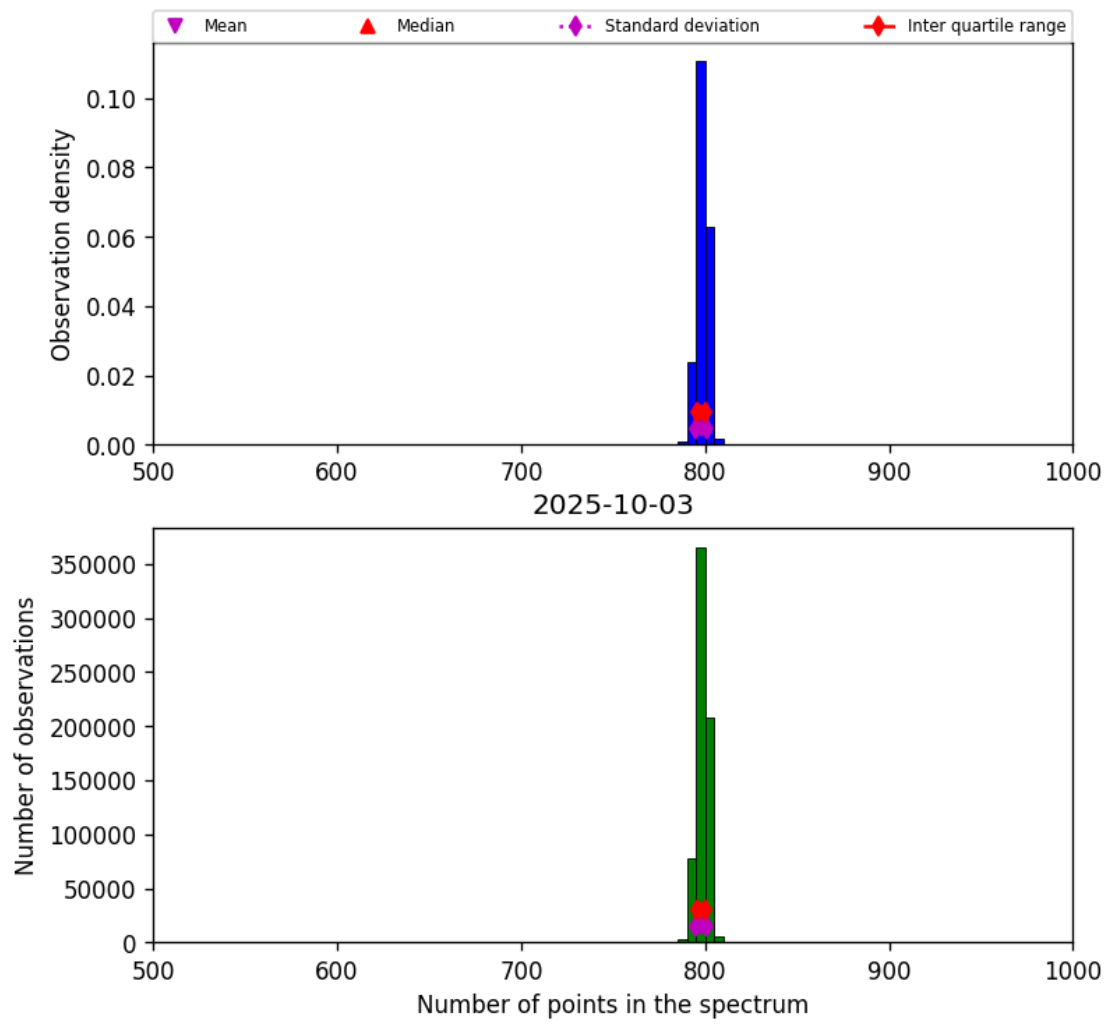
Figure 26: Histogram of “Number of points in the spectrum” for 2025-10-02 to 2025-10-04
