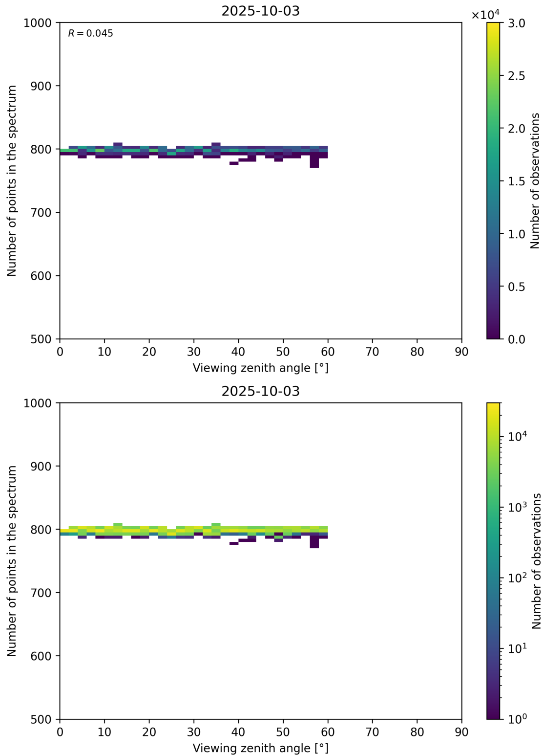
Figure 114: Scatter density plot of “Viewing zenith angle” against “Number of points in the spectrum” for 2025-10-02 to 2025-10-04.
