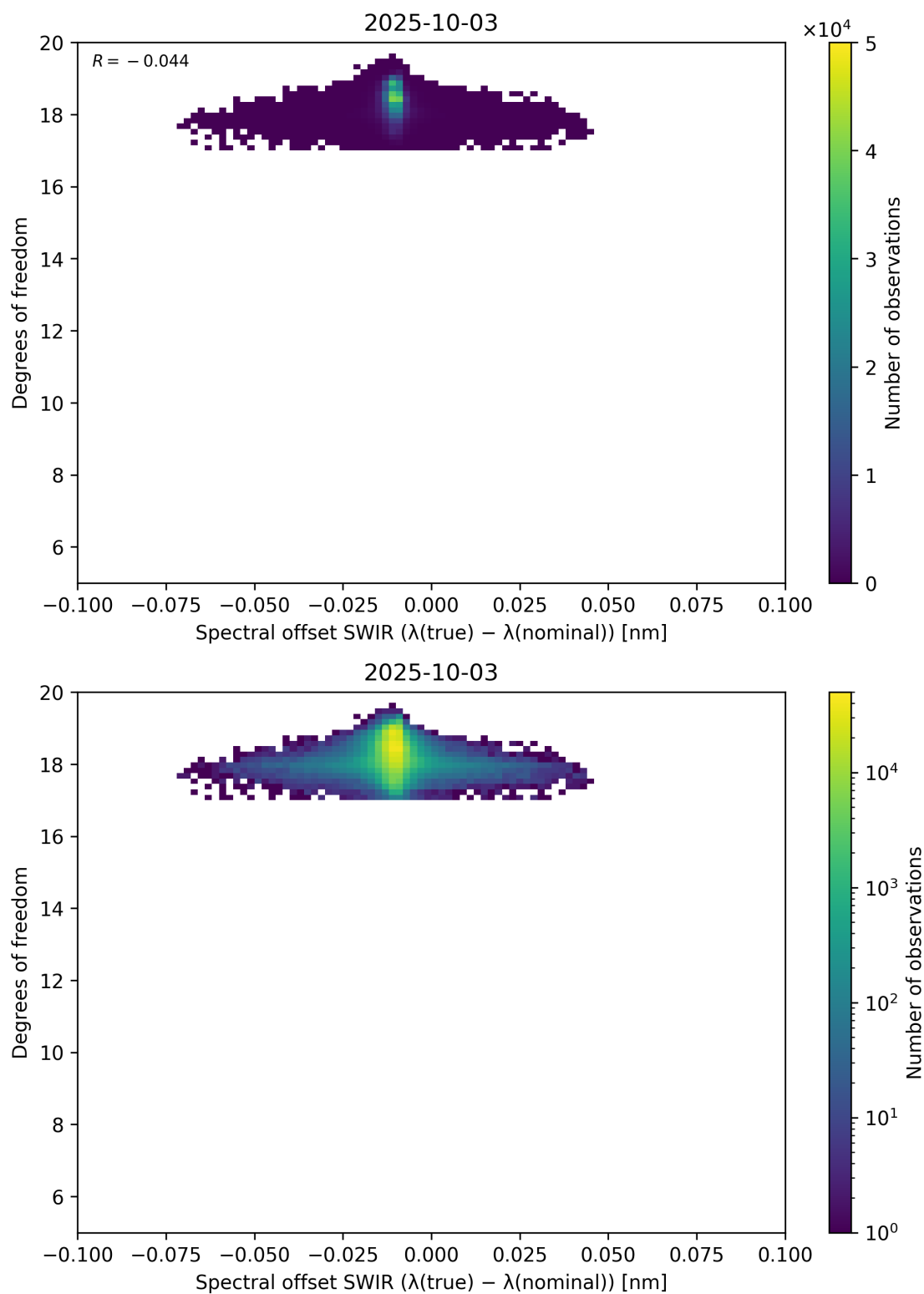
Figure 119: Scatter density plot of “Spectral offset SWIR ( \lambda_{\text{true}} - \lambda_{\text{nominal}} )” against “Degrees of freedom” for 2025-10-02 to 2025-10-04.
