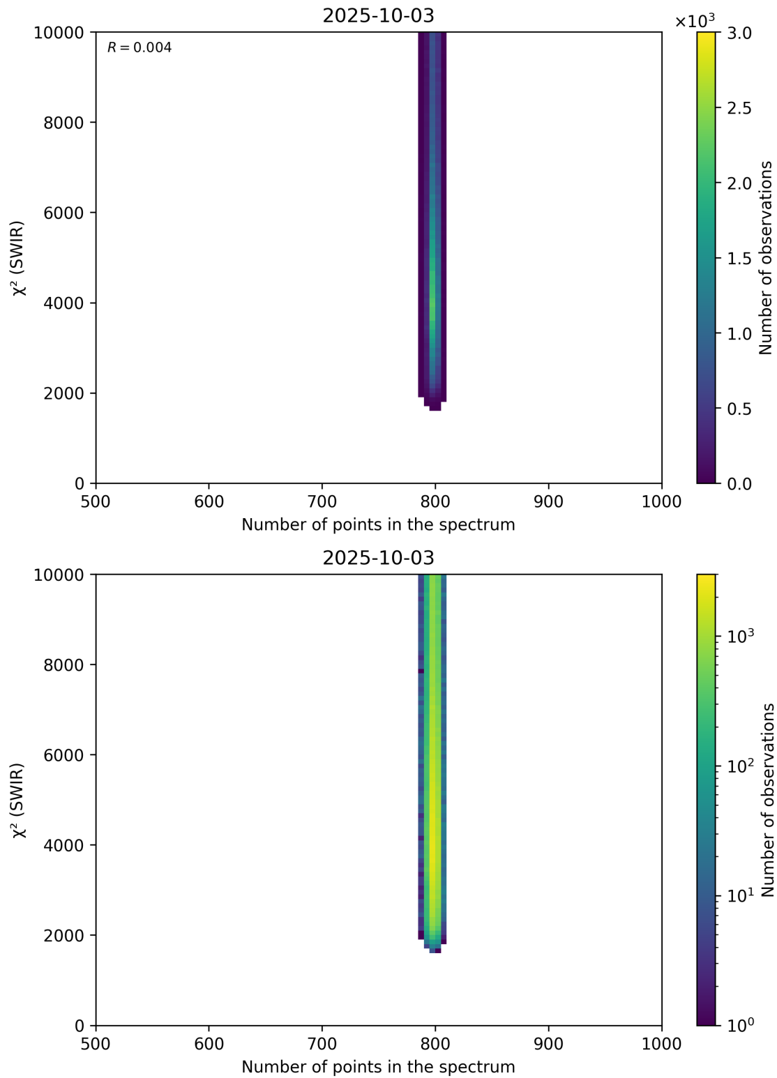
Figure 89: Scatter density plot of “Number of points in the spectrum” against “ \chi^2 (SWIR)” for 2025-10-02 to 2025-10-04.
