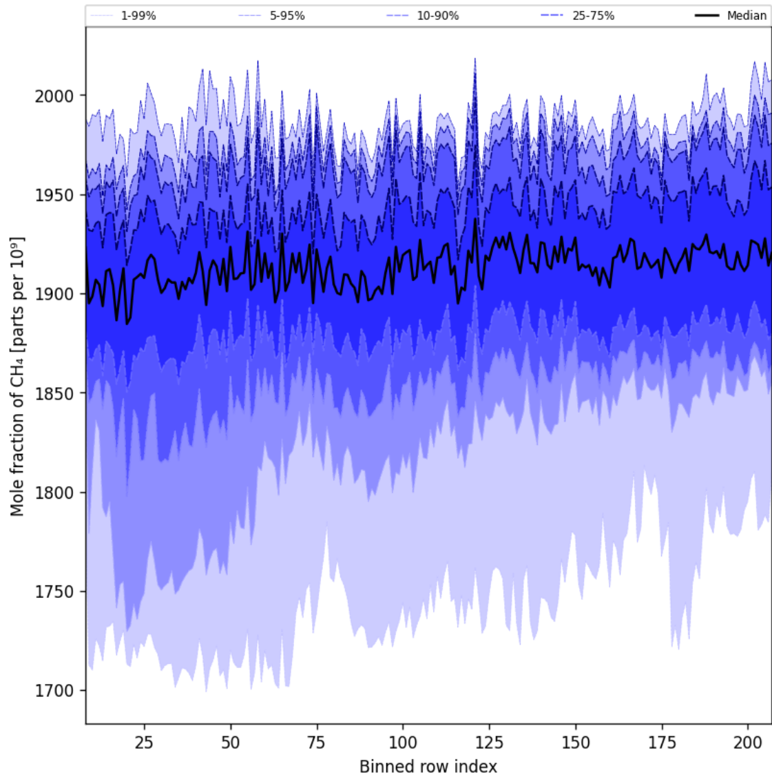
Figure 34: Along track statistics of “Mole fraction of CH 4 ” for 2025-10-02 to 2025-10-04
