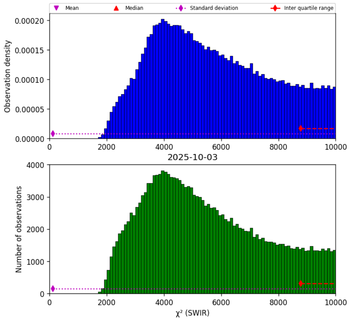
Figure 28: Histogram of “ \chi^2 (SWIR)” for 2025-10-02 to 2025-10-04
