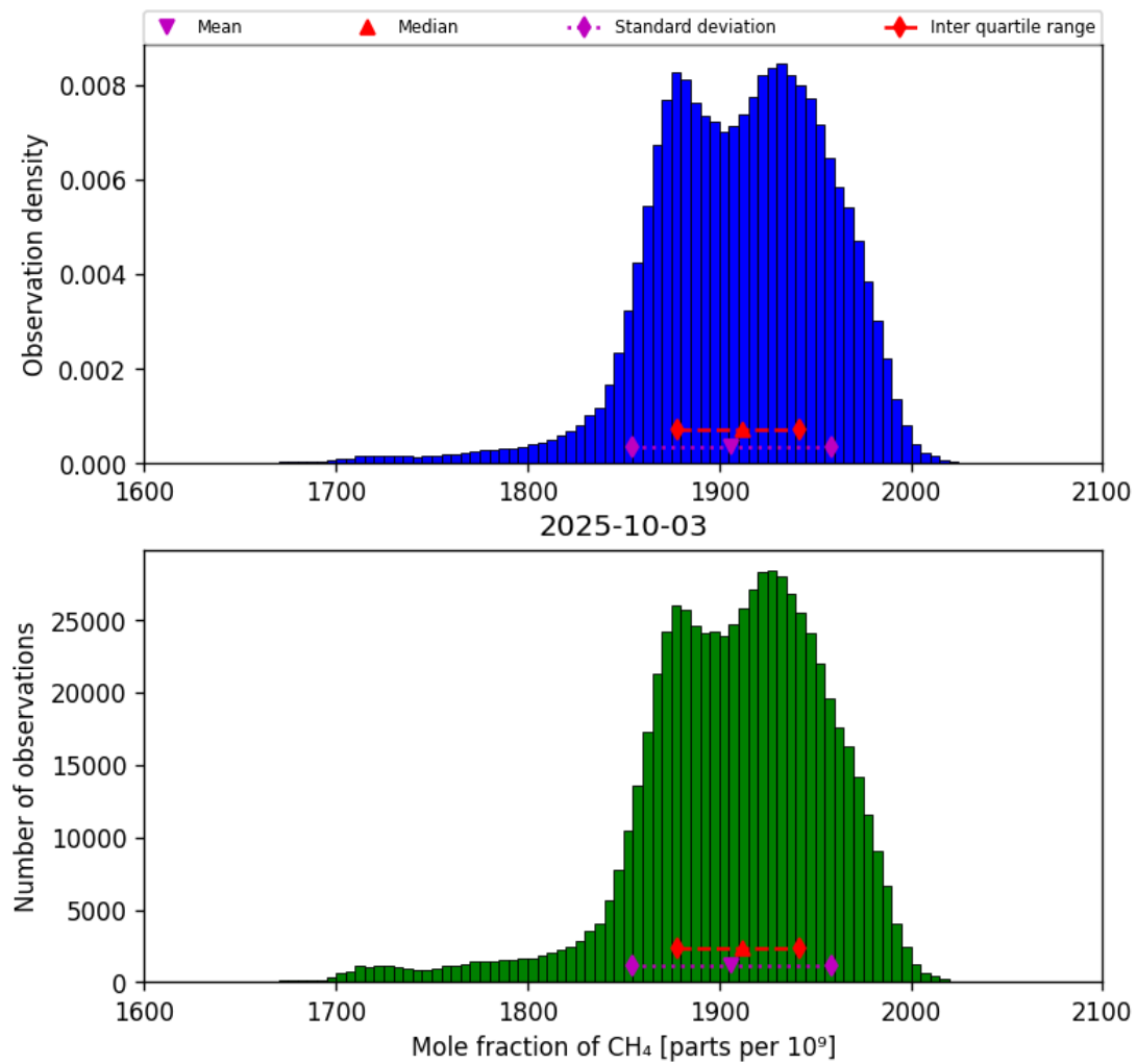
Figure 23: Histogram of “Mole fraction of CH 4 ” for 2025-10-02 to 2025-10-04
