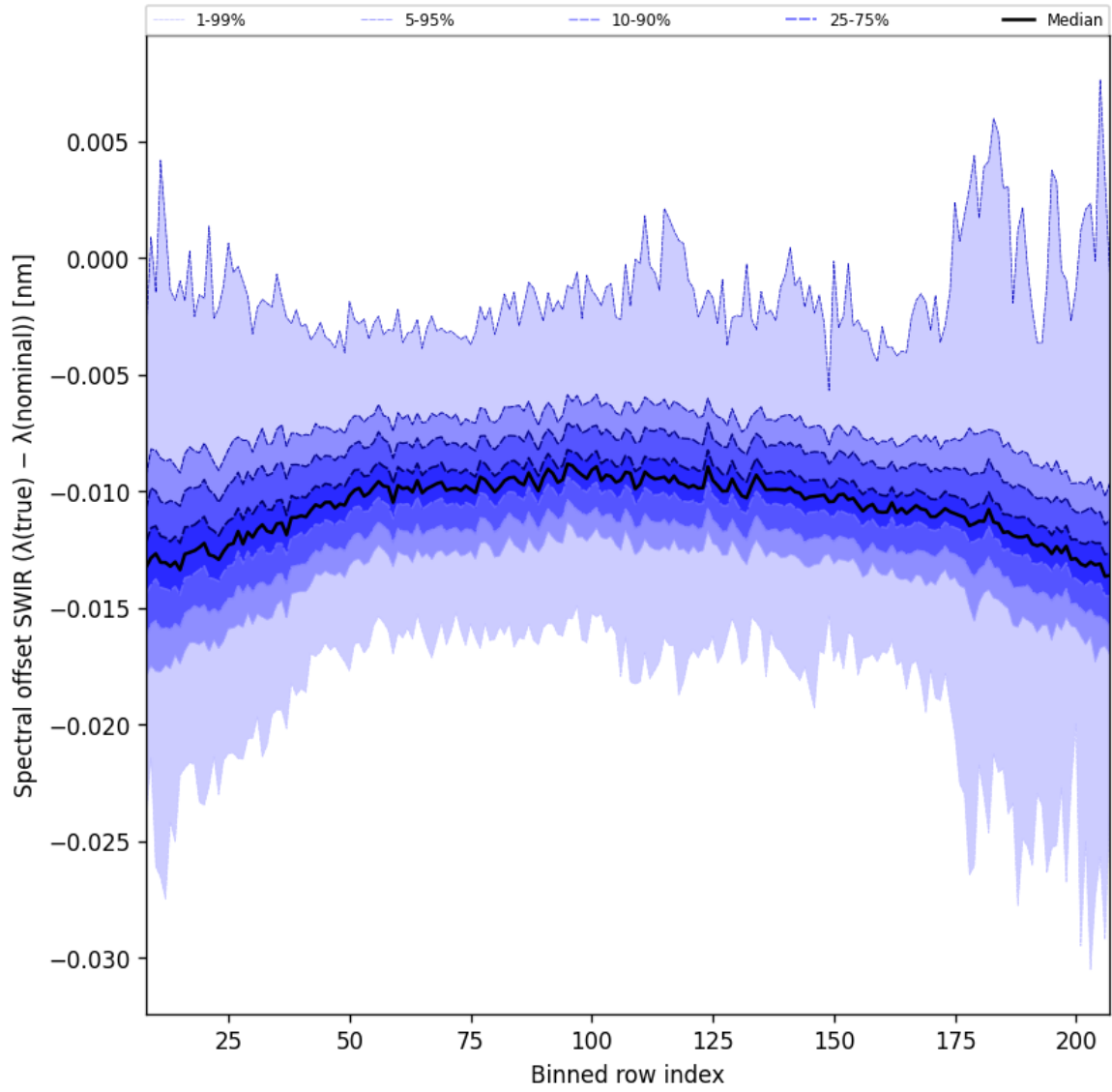
Figure 38: Along track statistics of “Spectral offset SWIR ( \lambda_{\text{true}} - \lambda_{\text{nominal}} )” for 2025-10-02 to 2025-10-04
