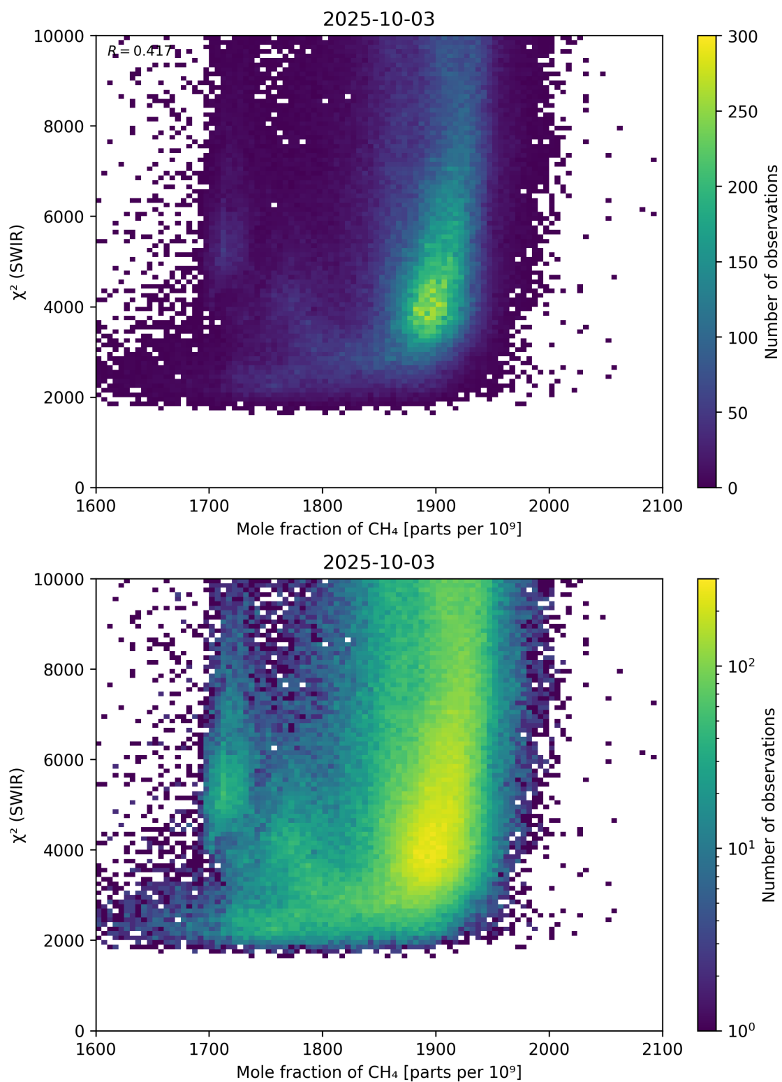
Figure 71: Scatter density plot of “Mole fraction of CH 4 ” against “ \chi^2 (SWIR)” for 2025-10-02 to 2025-10-04.
