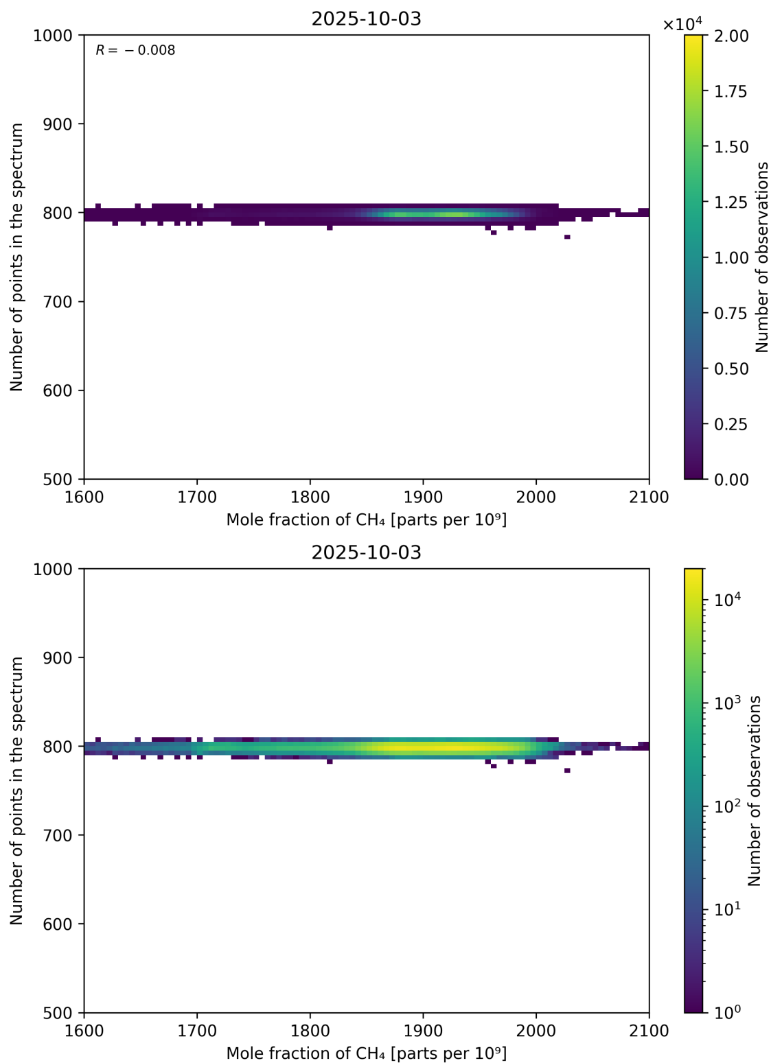
Figure 77: Scatter density plot of “Mole fraction of CH 4 ” against “Number of points in the spectrum” for 2025-10-02 to 2025-10-04.
