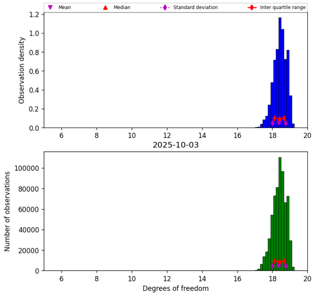
Figure 30: Histogram of “Degrees of freedom” for 2025-10-02 to 2025-10-04
