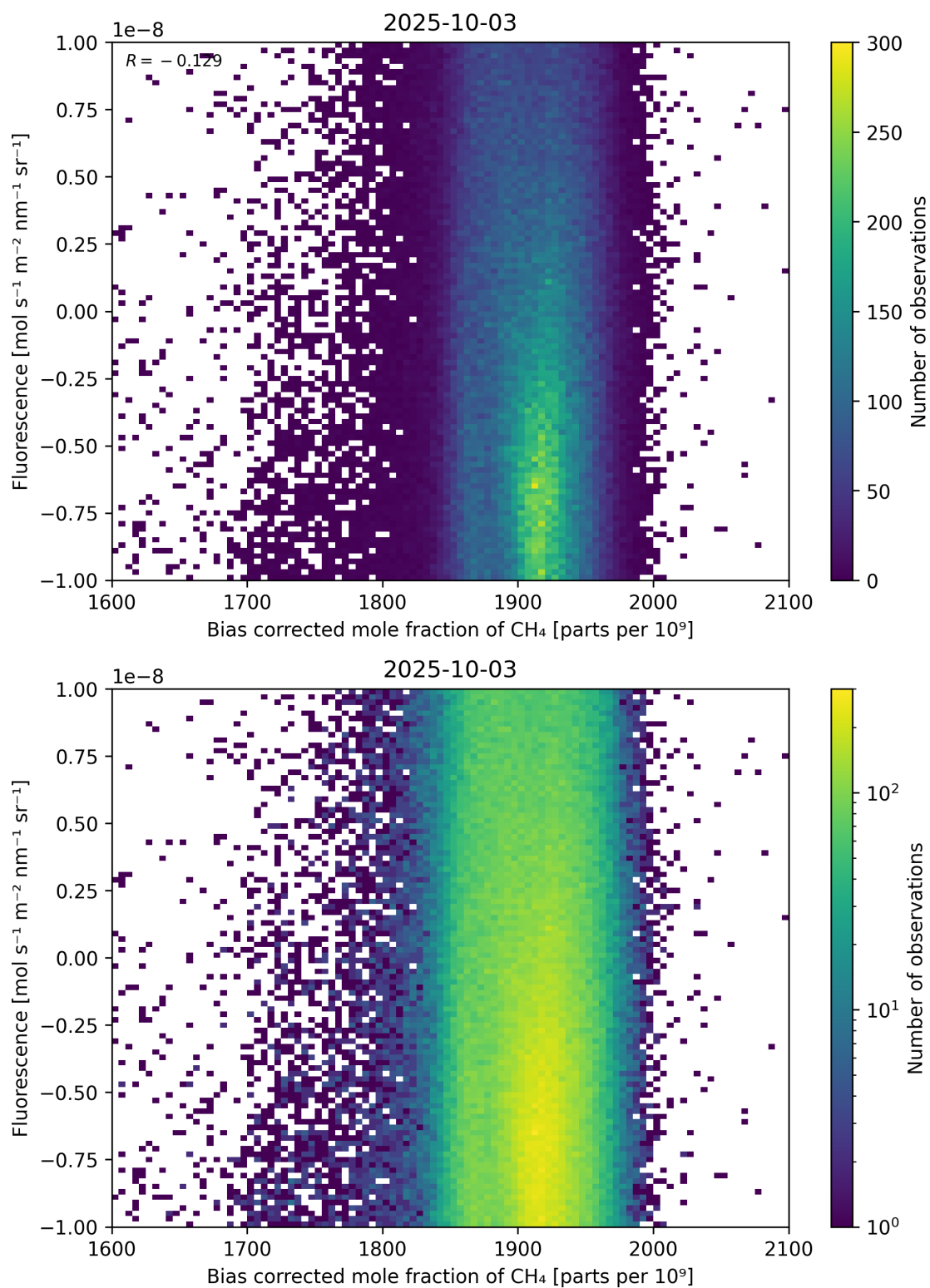
Figure 66: Scatter density plot of “Bias corrected mole fraction of \text{CH}_4 ” against “Fluorescence” for 2025-10-02 to 2025-10-04.
