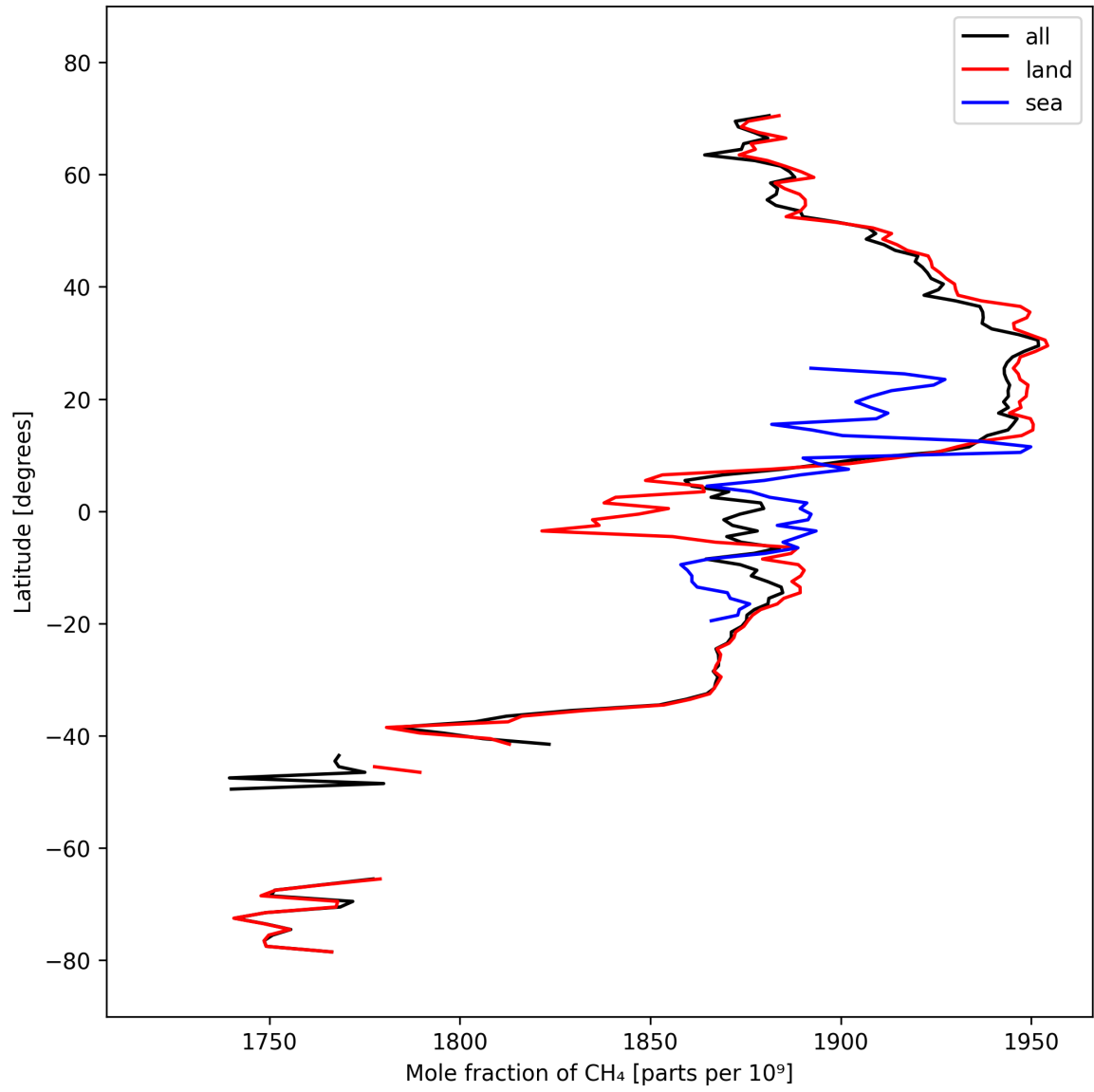
Figure 12: Zonal average of “Mole fraction of \text{CH}_4 ” for 2025-10-02 to 2025-10-04.
