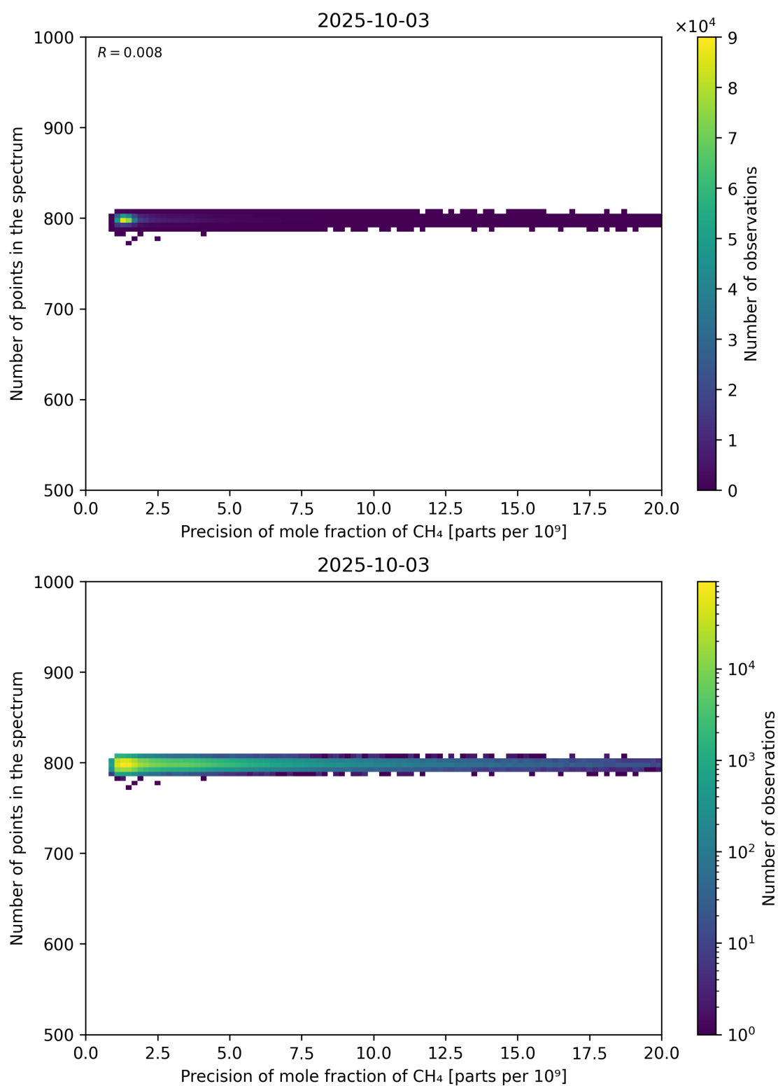
Figure 84: Scatter density plot of “Precision of mole fraction of CH 4 ” against “Number of points in the spectrum” for 2025-10-02 to 2025-10-04.
