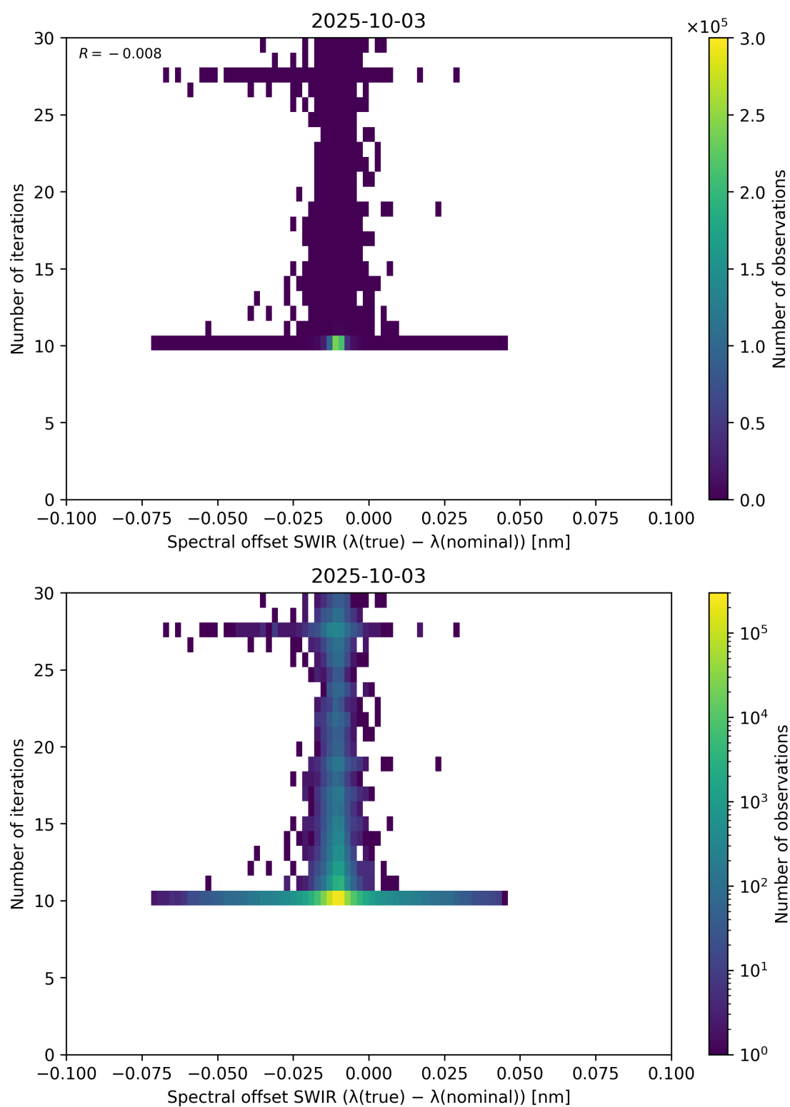
Figure 121: Scatter density plot of “Spectral offset SWIR ( \lambda_{\text{true}} - \lambda_{\text{nominal}} )” against “Number of iterations” for 2025-10-02 to 2025-10-04.
