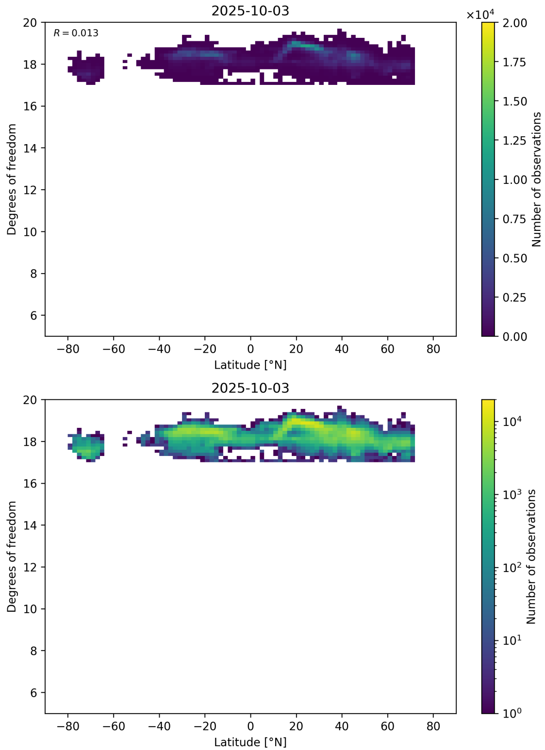
Figure 55: Scatter density plot of “Latitude” against “Degrees of freedom” for 2025-10-02 to 2025-10-04.
