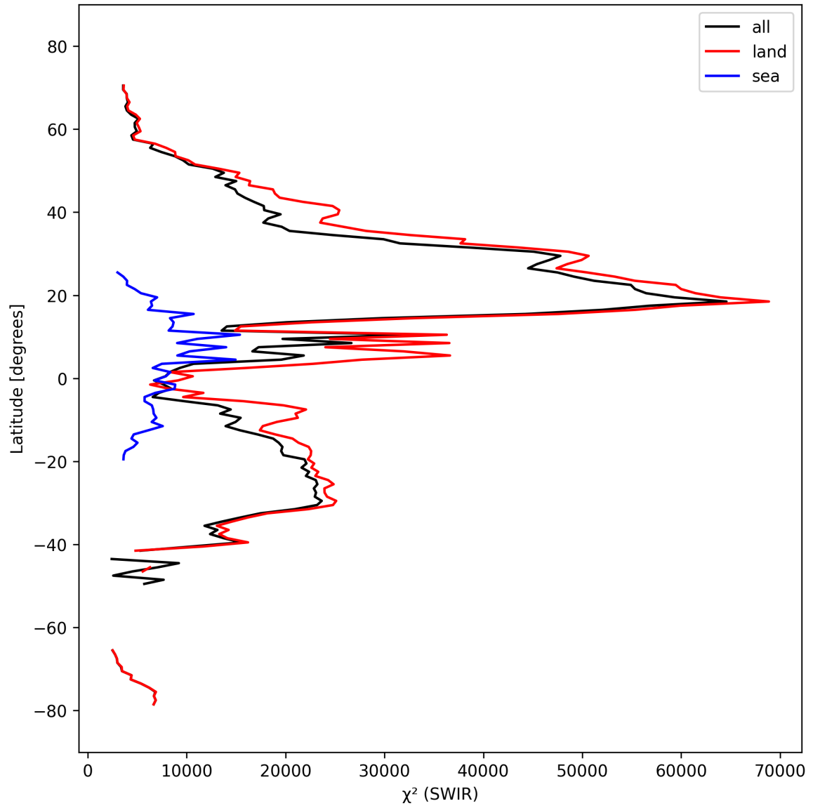
Figure 17: Zonal average of “ \chi^2 (SWIR)” for 2025-10-02 to 2025-10-04.
