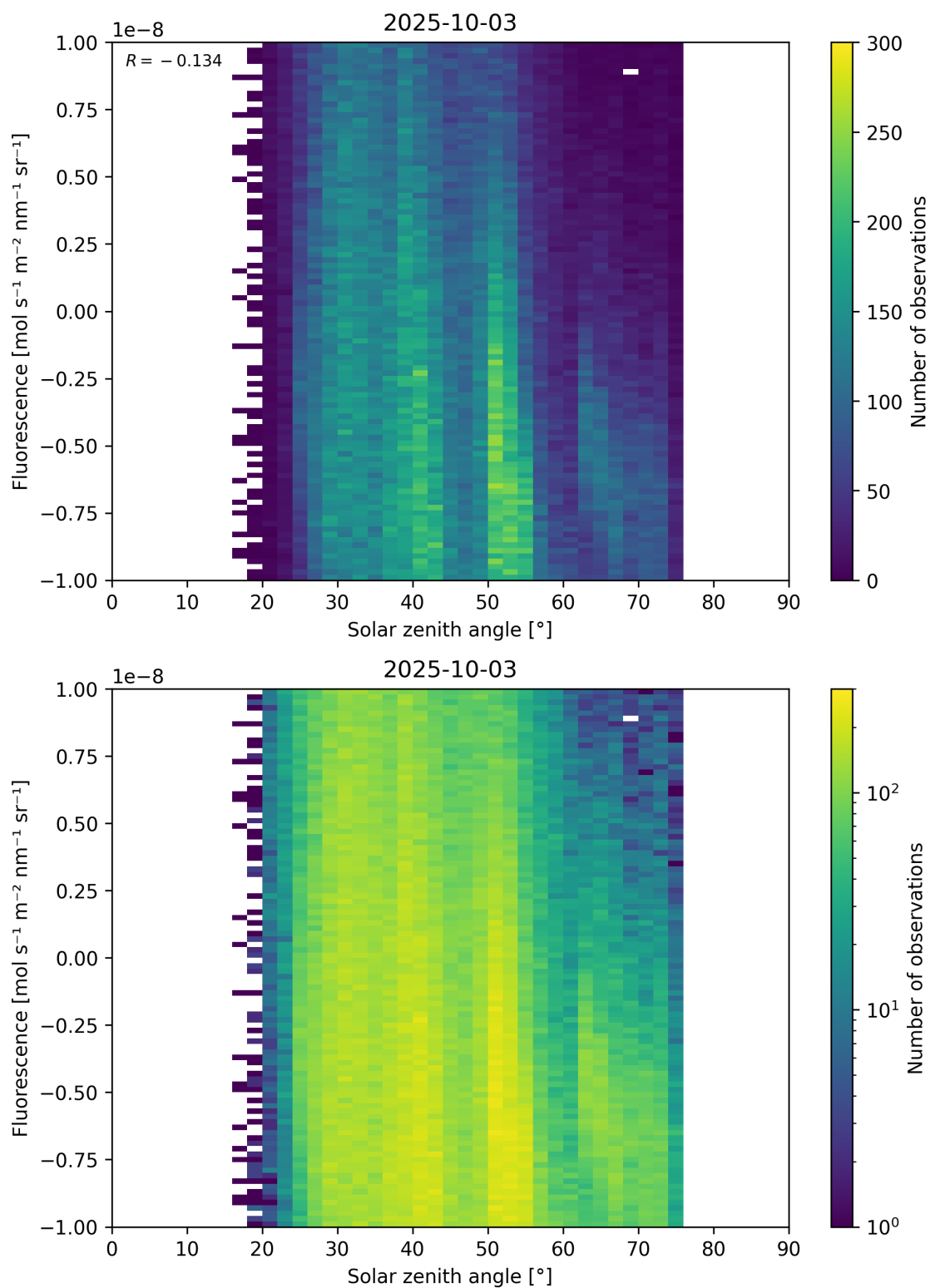
Figure 97: Scatter density plot of “Solar zenith angle” against “Fluorescence” for 2025-10-02 to 2025-10-04.
