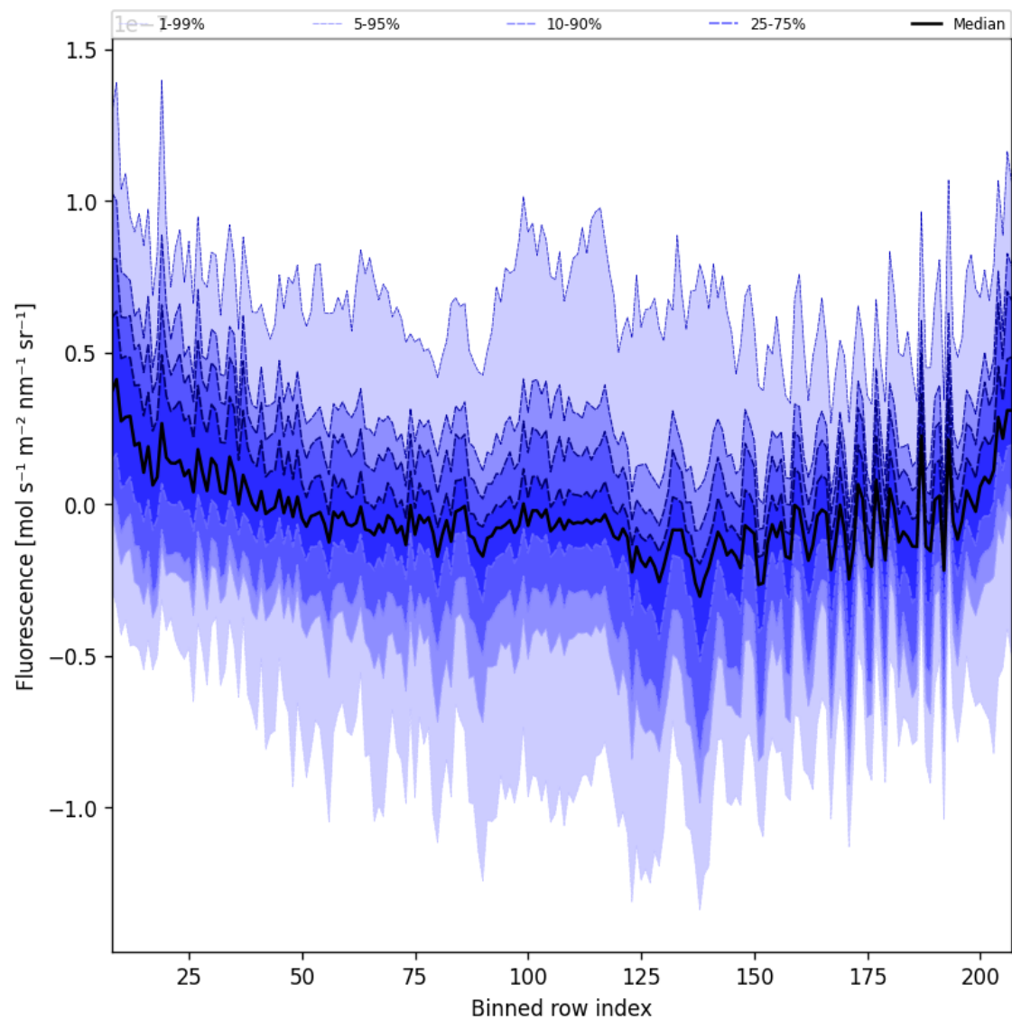
Figure 43: Along track statistics of “Fluorescence” for 2025-10-02 to 2025-10-04
