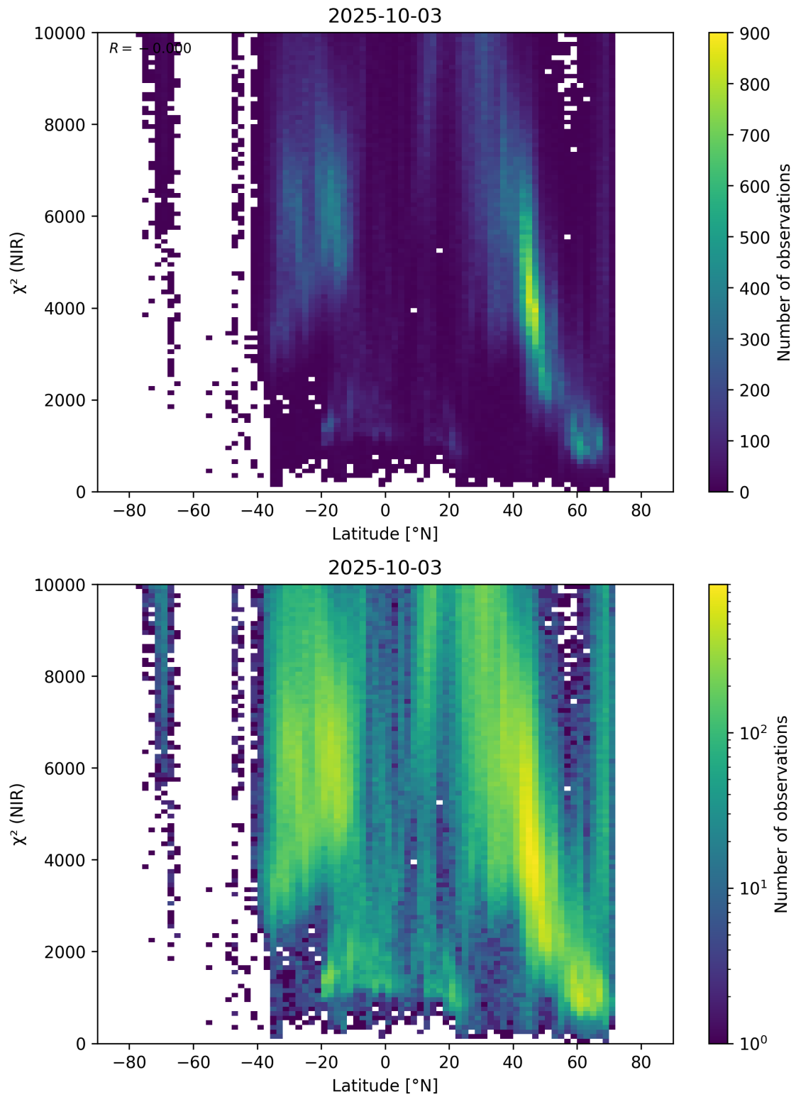
Figure 53: Scatter density plot of “Latitude” against “ \chi^2 (NIR)” for 2025-10-02 to 2025-10-04.
