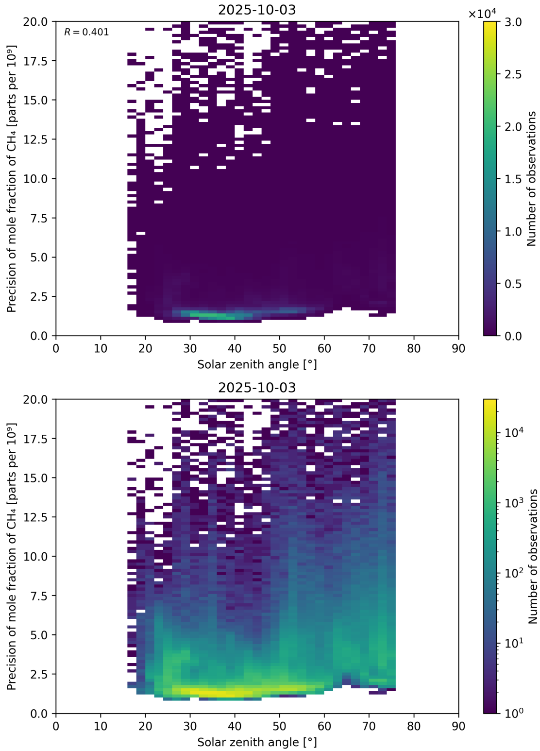
Figure 101: Scatter density plot of “Solar zenith angle” against “Precision of mole fraction of CH 4 ” for 2025-10-02 to 2025-10-04.
