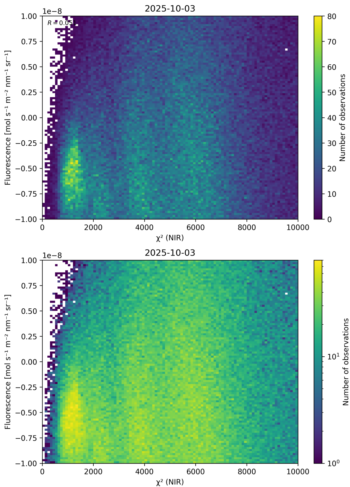
Figure 45: Scatter density plot of “ \chi^2 (NIR)” against “Fluorescence” for 2025-10-02 to 2025-10-04.
