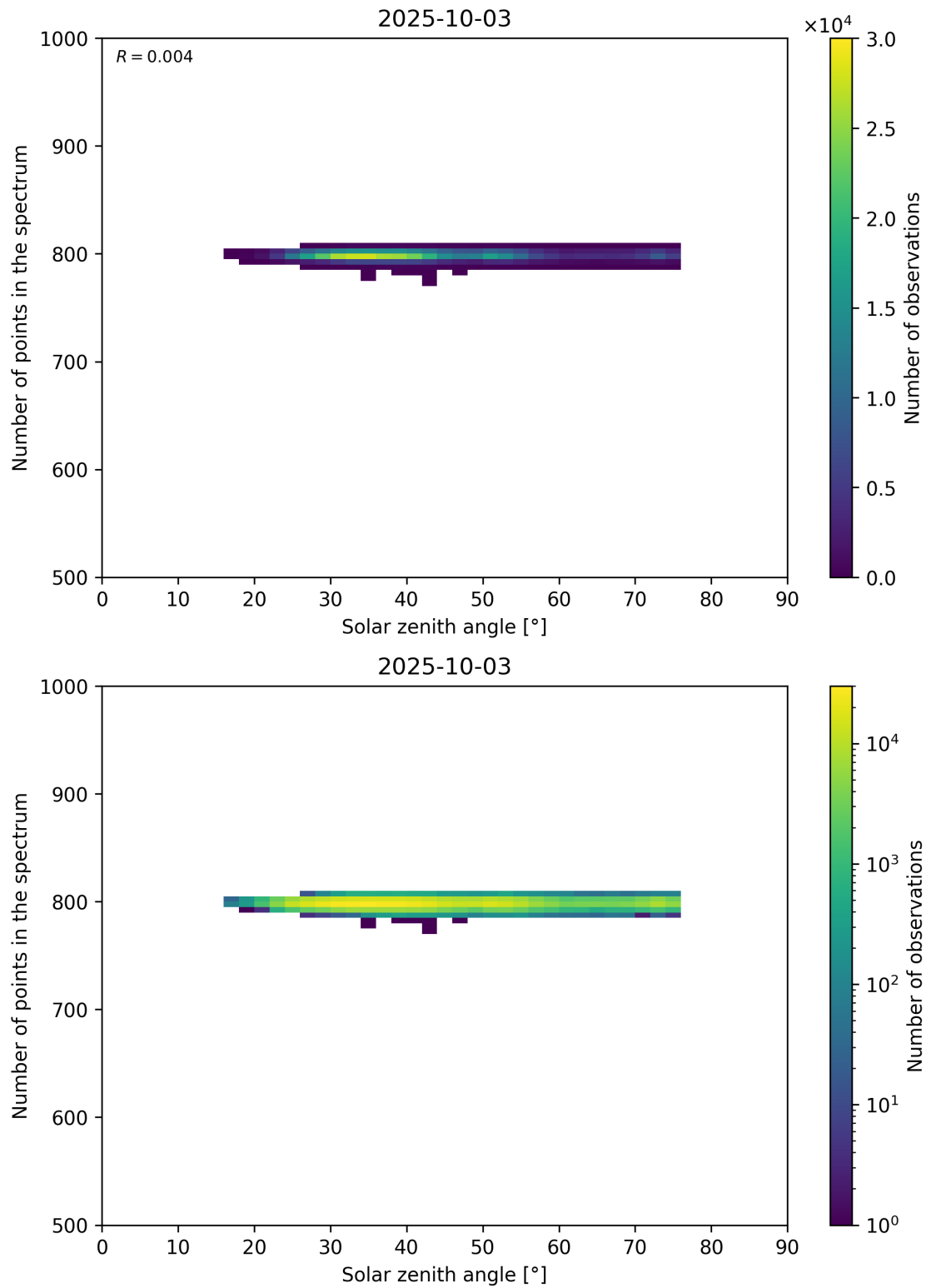
Figure 103: Scatter density plot of “Solar zenith angle” against “Number of points in the spectrum” for 2025-10-02 to 2025-10-04.
