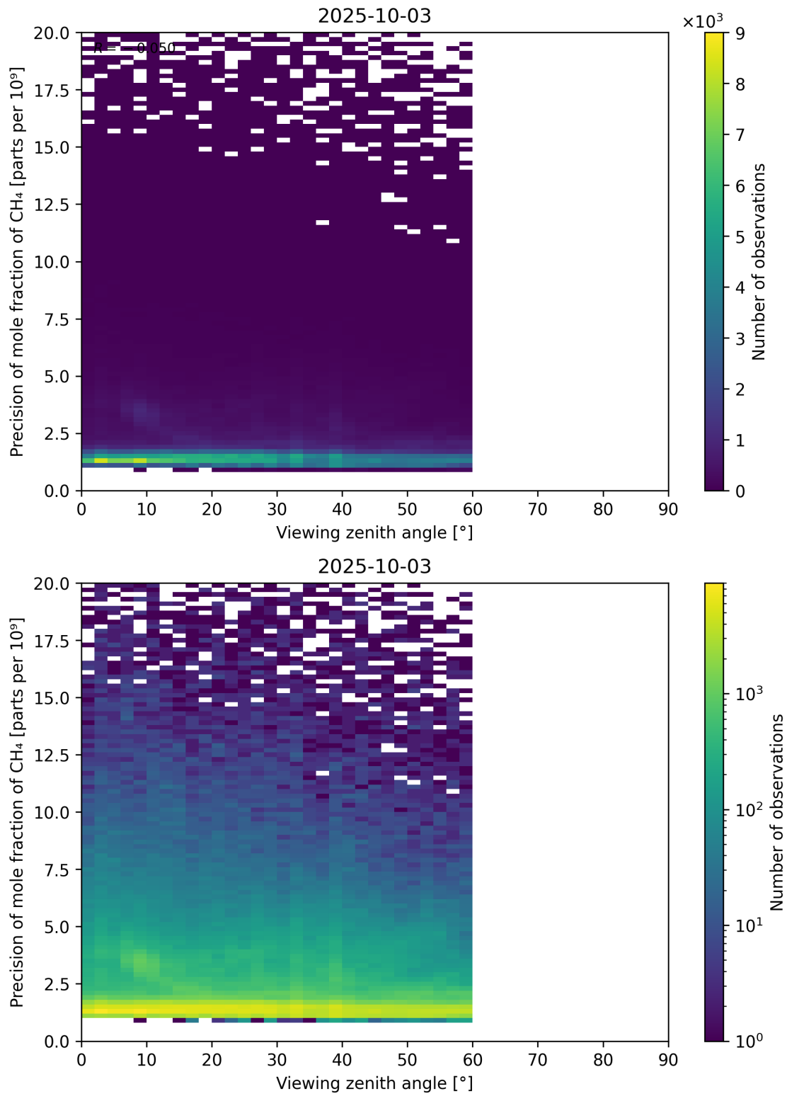
Figure 112: Scatter density plot of “Viewing zenith angle” against “Precision of mole fraction of CH 4 ” for 2025-10-02 to 2025-10-04.
