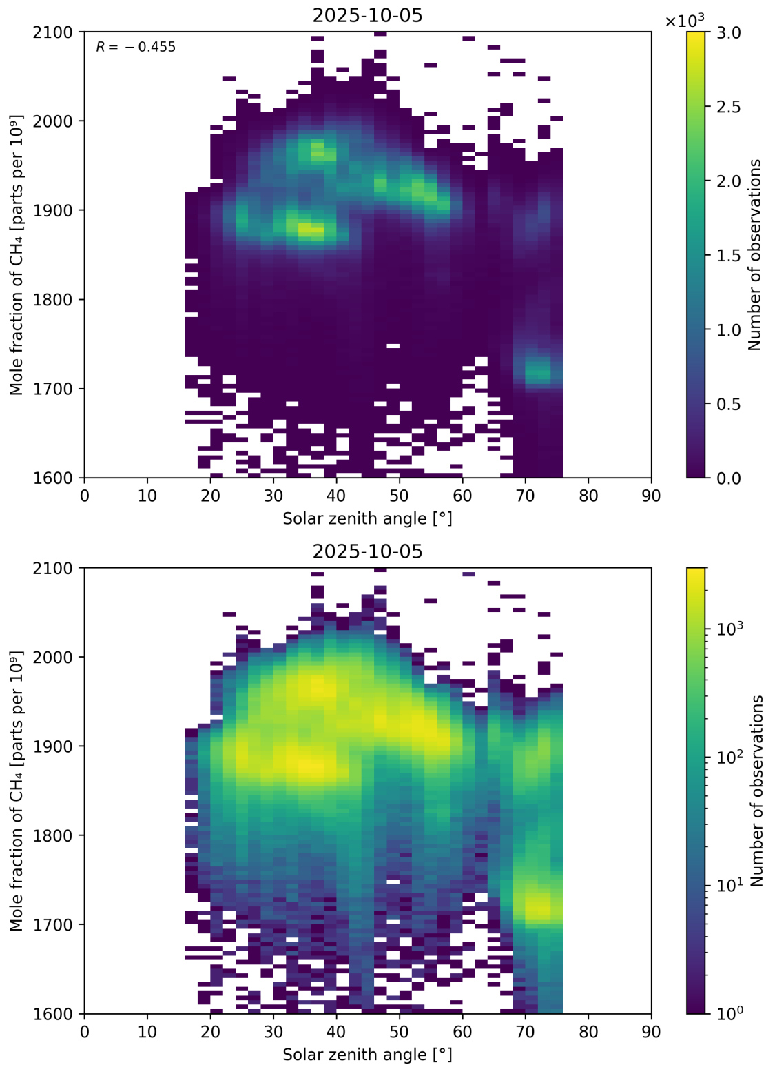
Figure 99: Scatter density plot of “Solar zenith angle” against “Mole fraction of CH 4 ” for 2025-10-04 to 2025-10-06.
