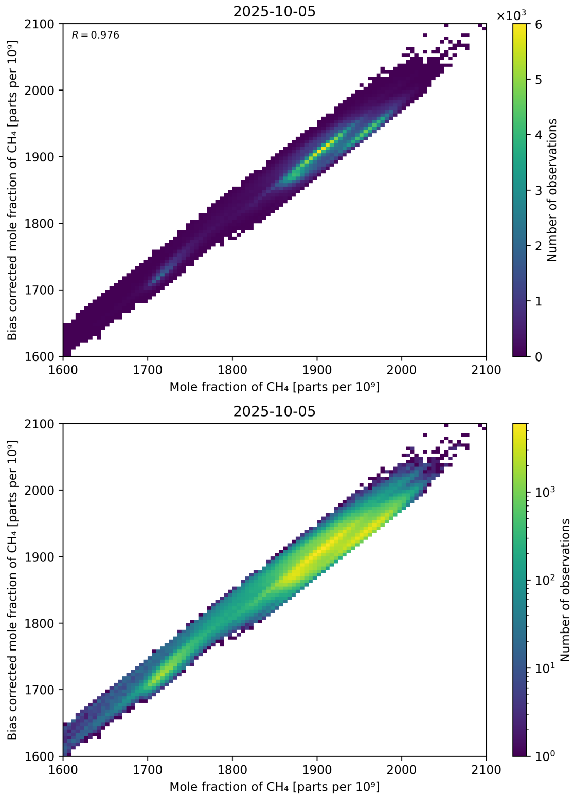
Figure 74: Scatter density plot of “Mole fraction of CH 4 ” against “Bias corrected mole fraction of CH 4 ” for 2025-10-04 to 2025-10-06.
