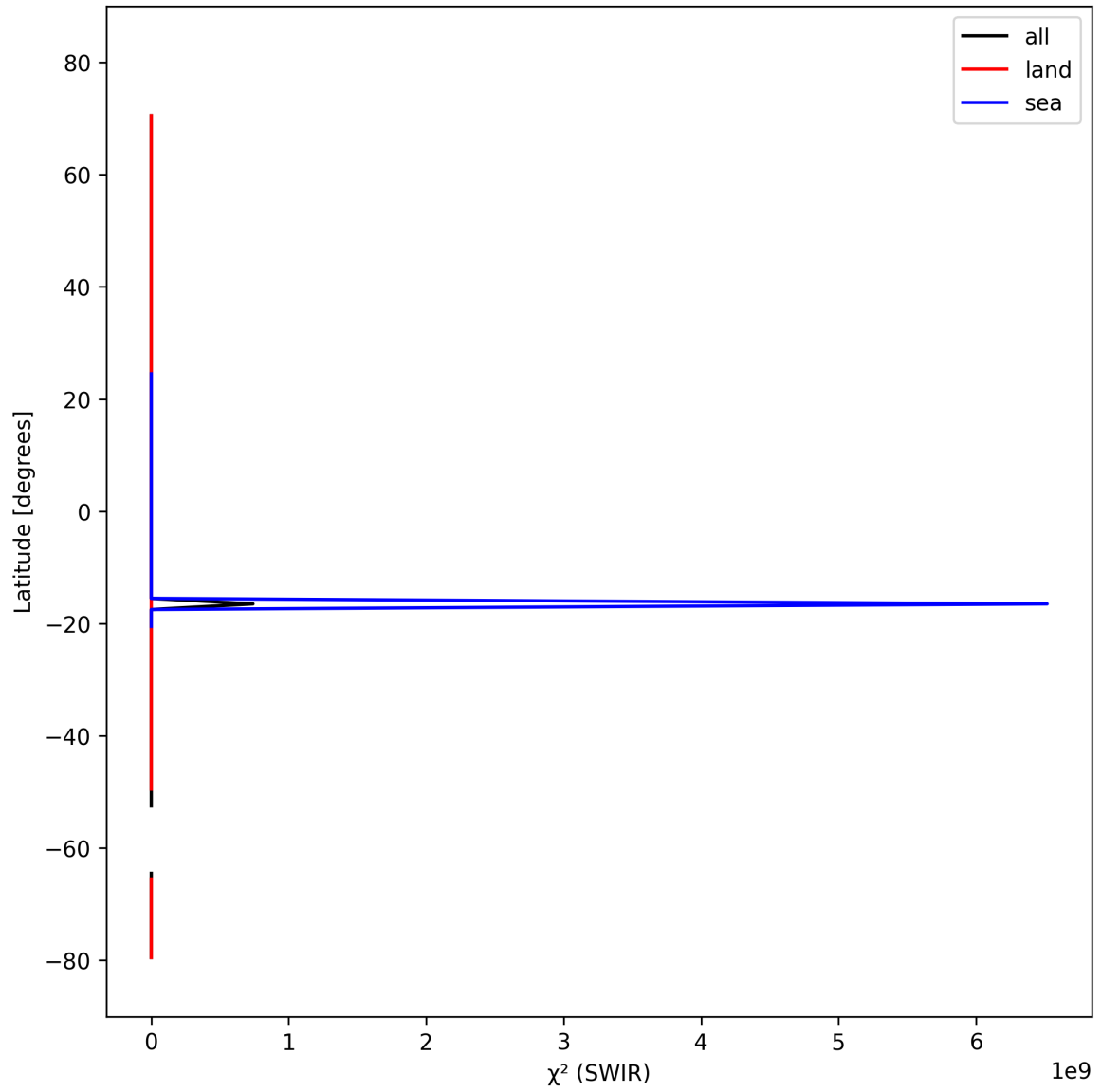
Figure 17: Zonal average of “ \chi^2 (SWIR)” for 2025-10-04 to 2025-10-06.
