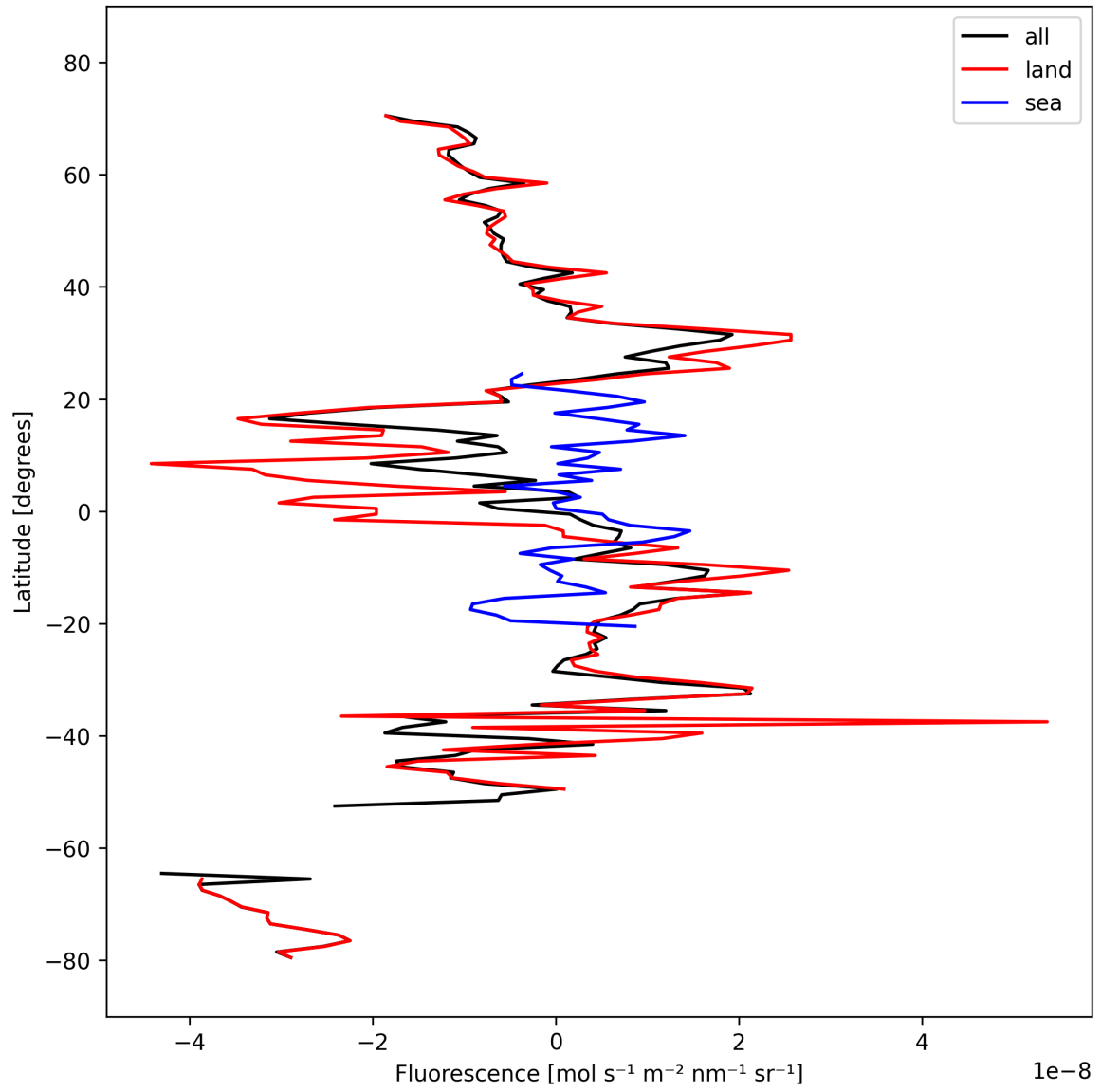
Figure 21: Zonal average of “Fluorescence” for 2025-10-04 to 2025-10-06.
