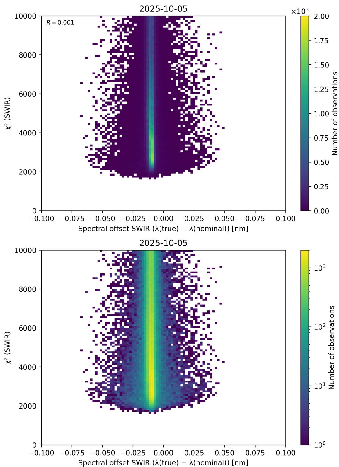
Figure 118: Scatter density plot of “Spectral offset SWIR ( \lambda_{\text{true}} - \lambda_{\text{nominal}} )” against “ \chi^2 (SWIR)” for 2025-10-04 to 2025-10-06.
