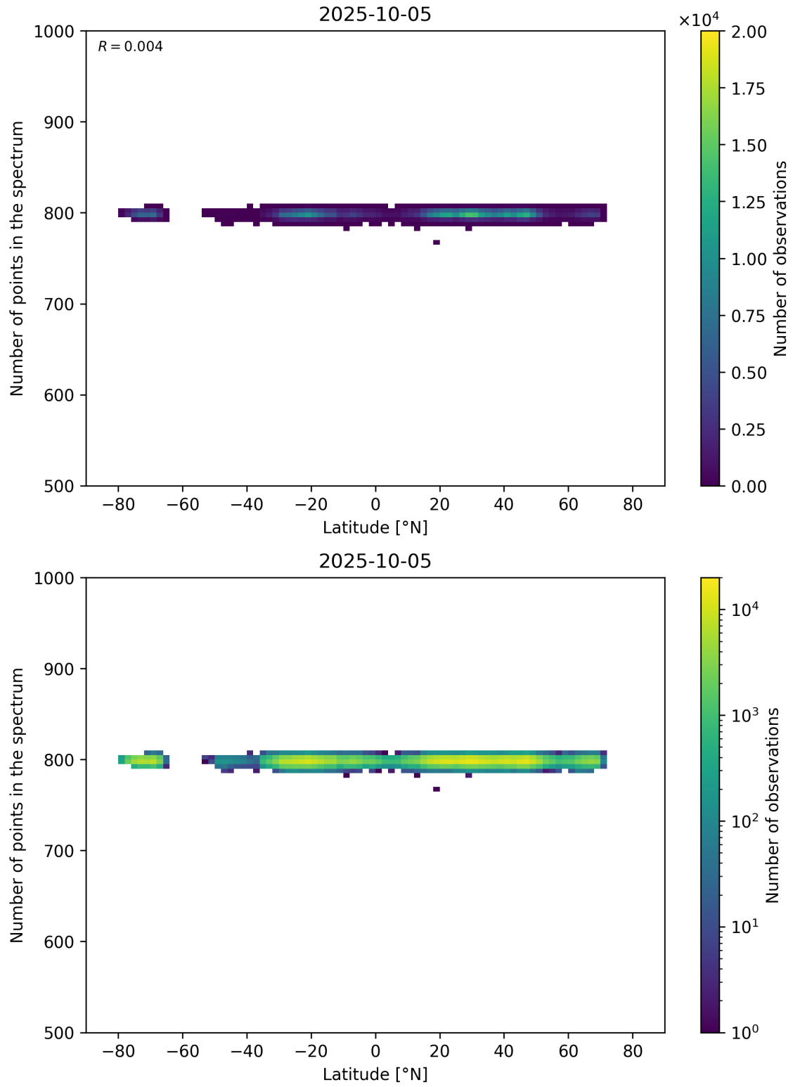
Figure 61: Scatter density plot of “Latitude” against “Number of points in the spectrum” for 2025-10-04 to 2025-10-06.
