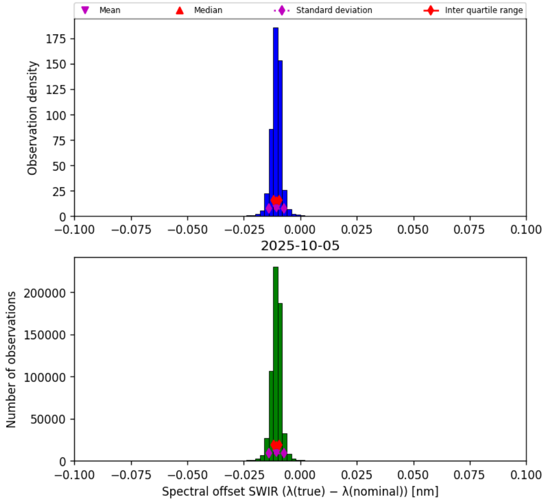
Figure 27: Histogram of “Spectral offset SWIR ( \lambda_{\text{true}} - \lambda_{\text{nominal}} )” for 2025-10-04 to 2025-10-06
