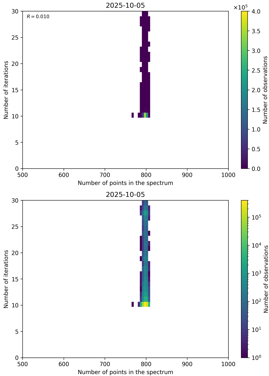
Figure 92: Scatter density plot of “Number of points in the spectrum” against “Number of iterations” for 2025-10-04 to 2025-10-06.
