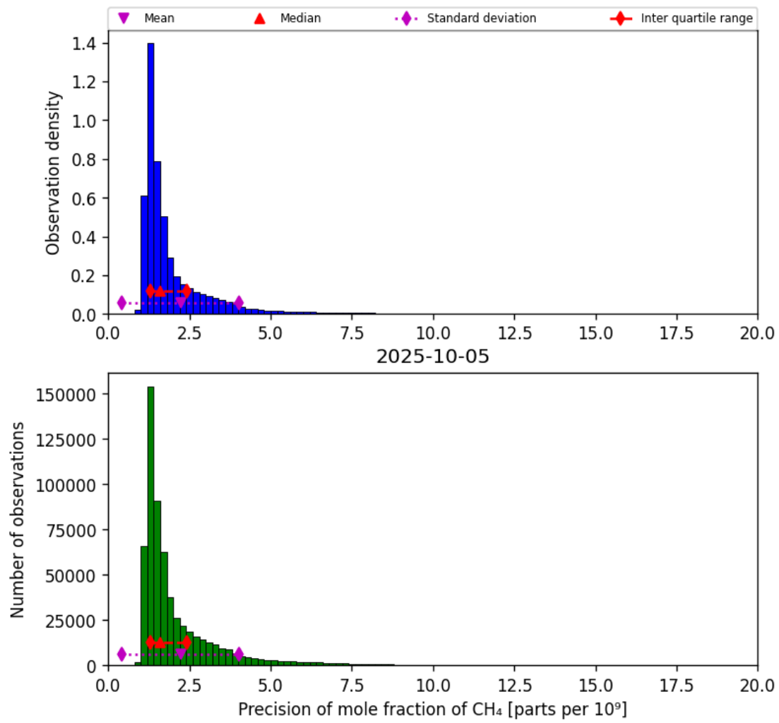
Figure 24: Histogram of “Precision of mole fraction of CH 4 ” for 2025-10-04 to 2025-10-06
