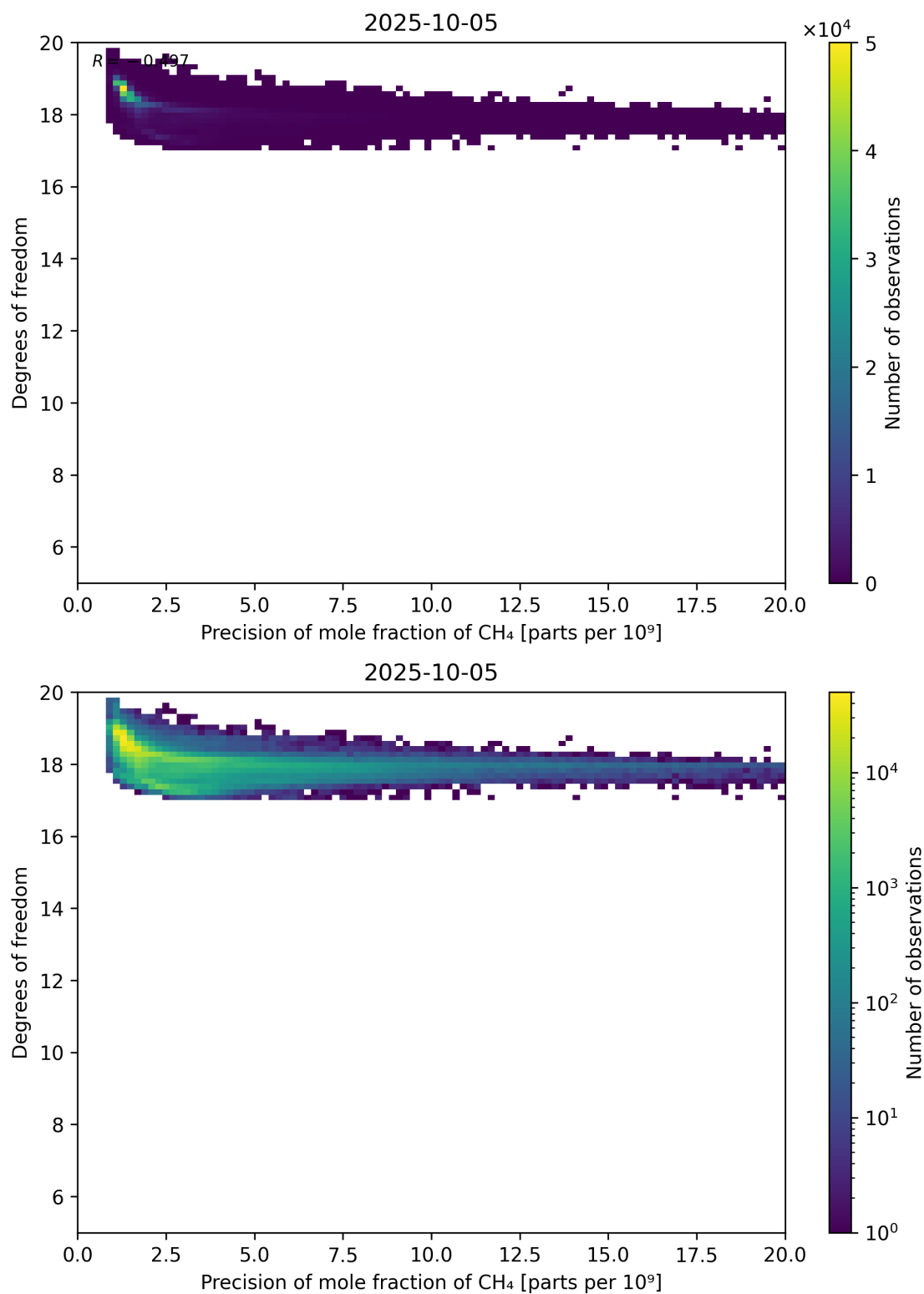
Figure 80: Scatter density plot of “Precision of mole fraction of CH 4 ” against “Degrees of freedom” for 2025-10-04 to 2025-10-06.
