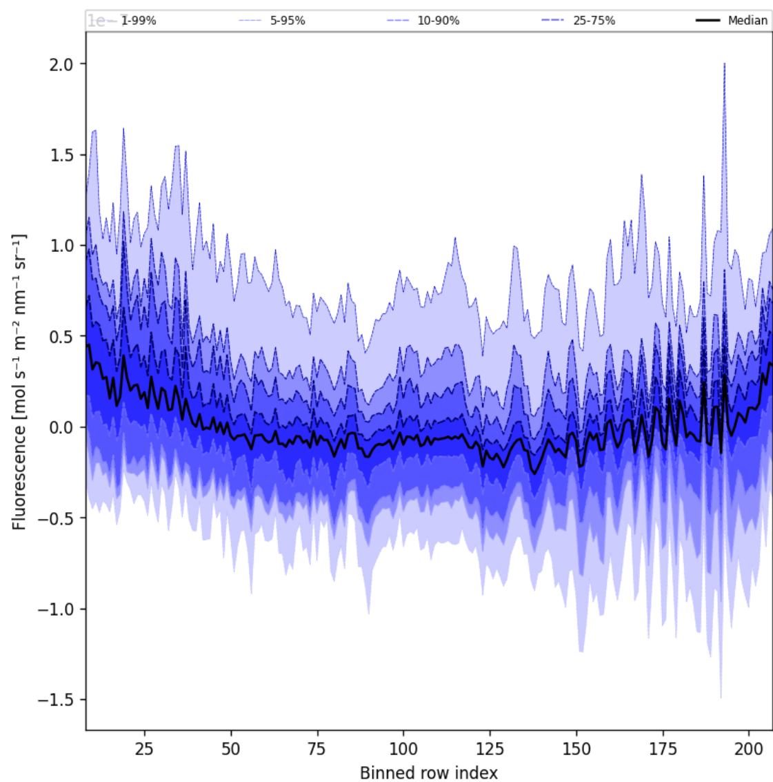
Figure 43: Along track statistics of “Fluorescence” for 2025-10-04 to 2025-10-06
