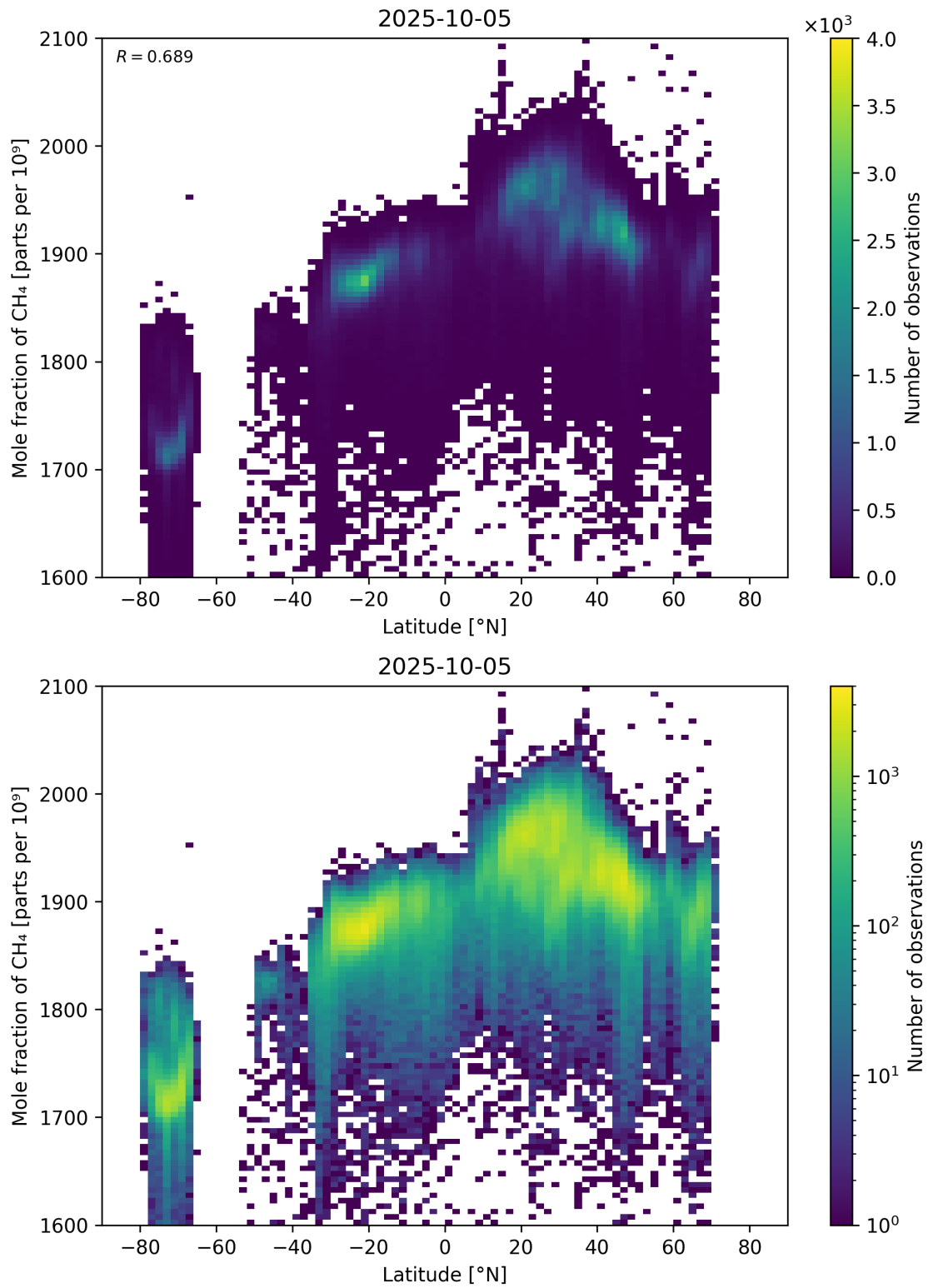
Figure 57: Scatter density plot of “Latitude” against “Mole fraction of CH 4 ” for 2025-10-04 to 2025-10-06.
