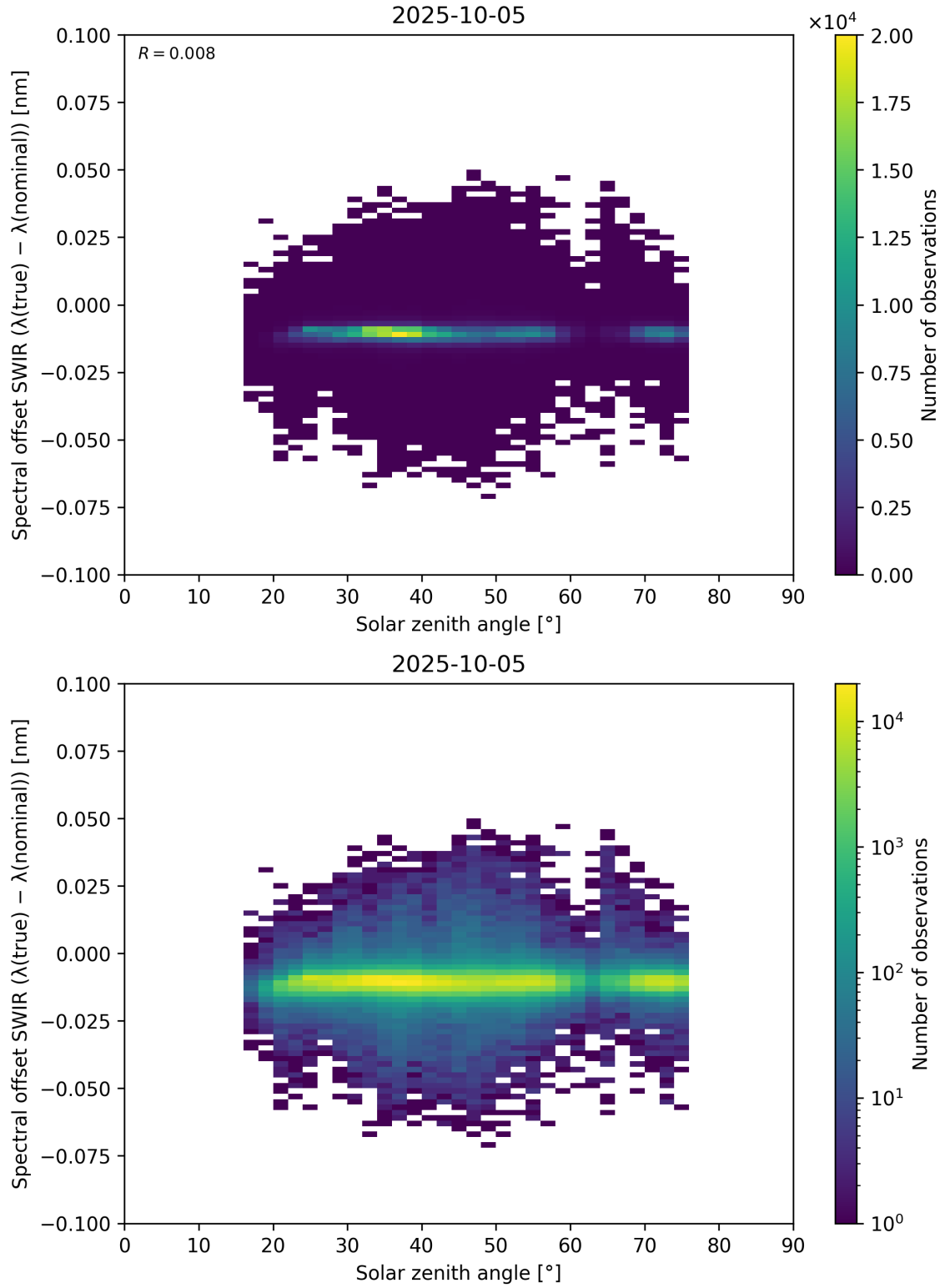
Figure 104: Scatter density plot of “Solar zenith angle” against “Spectral offset SWIR ( \lambda_{\text{true}} - \lambda_{\text{nominal}} )” for 2025-10-04 to 2025-10-06.
