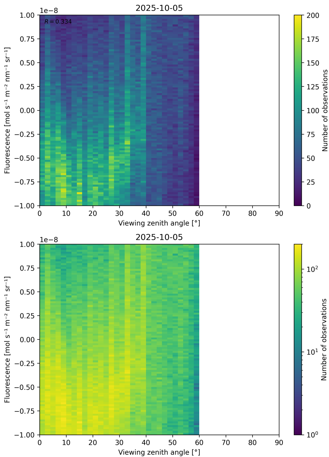
Figure 108: Scatter density plot of “Viewing zenith angle” against “Fluorescence” for 2025-10-04 to 2025-10-06.
