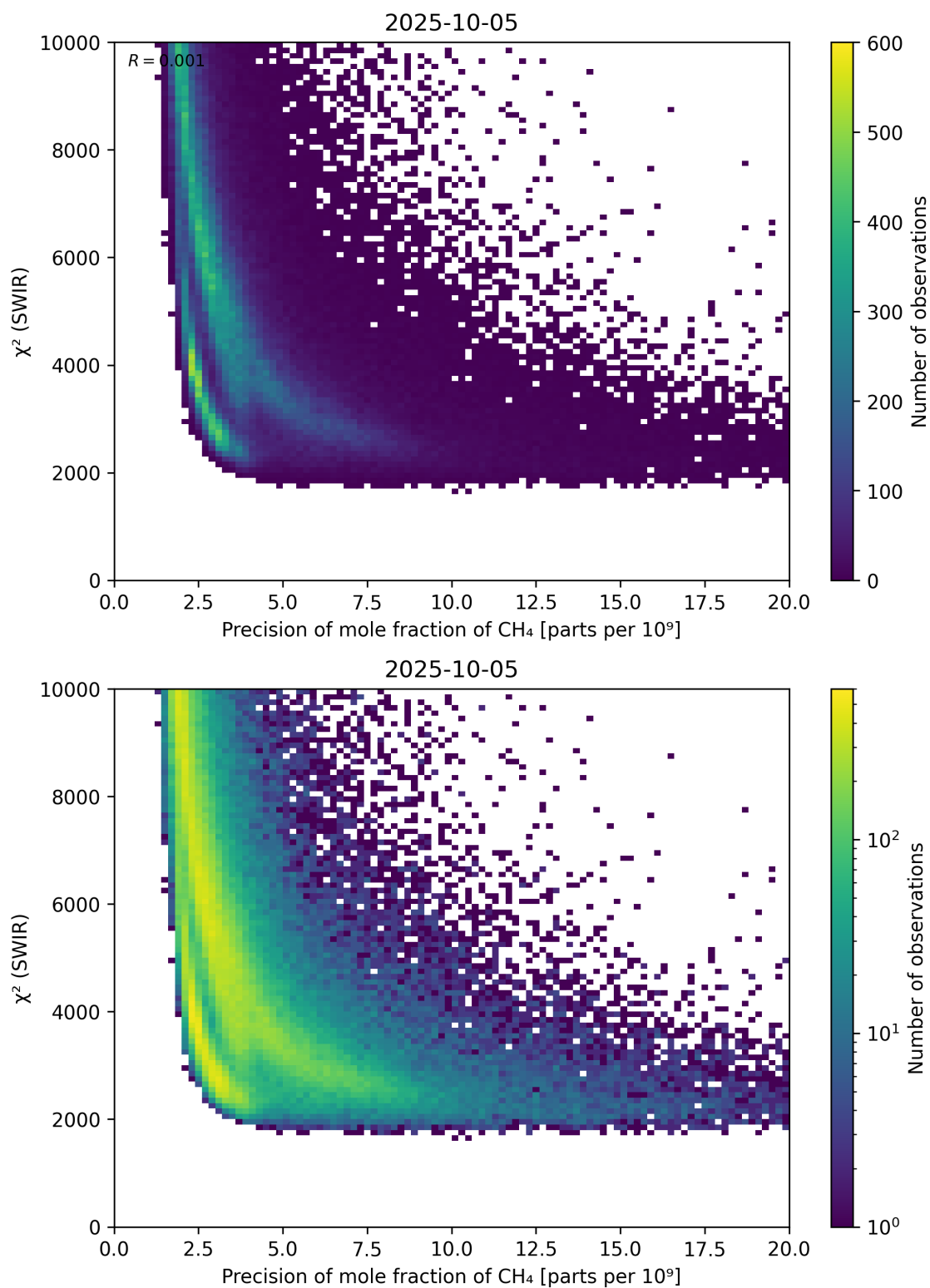
Figure 79: Scatter density plot of “Precision of mole fraction of CH 4 ” against “ \chi^2 (SWIR)” for 2025-10-04 to 2025-10-06.
