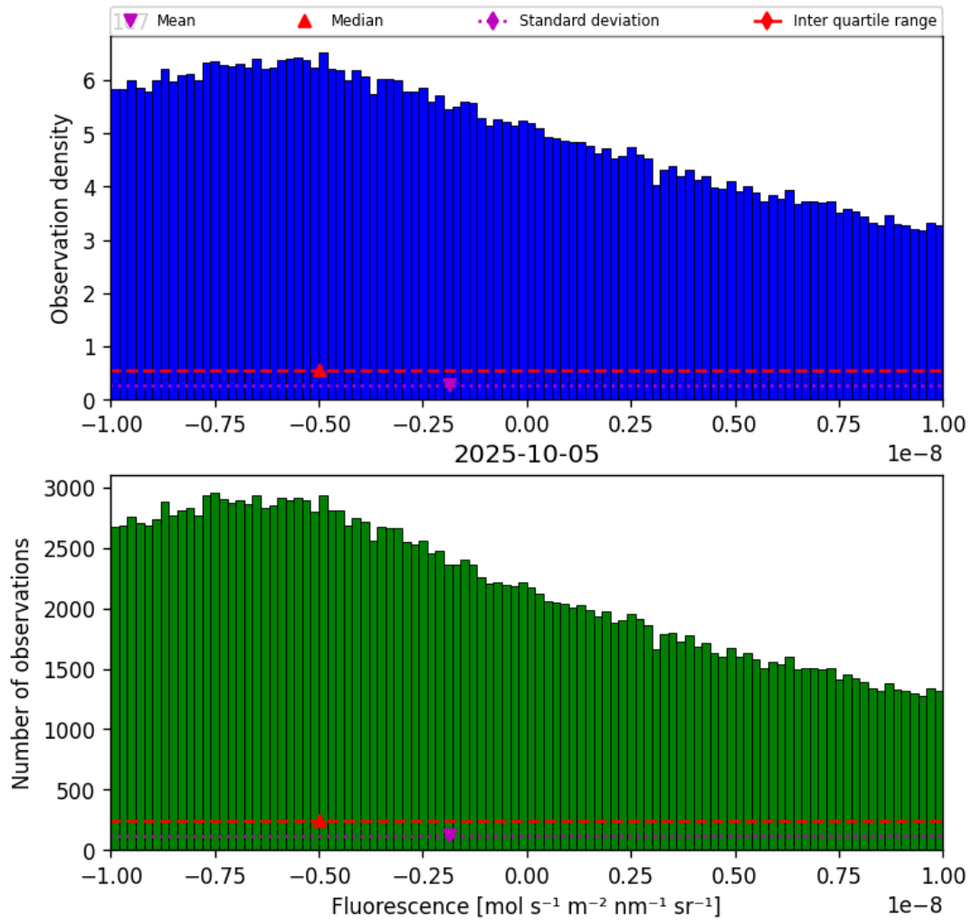
Figure 32: Histogram of “Fluorescence” for 2025-10-04 to 2025-10-06
