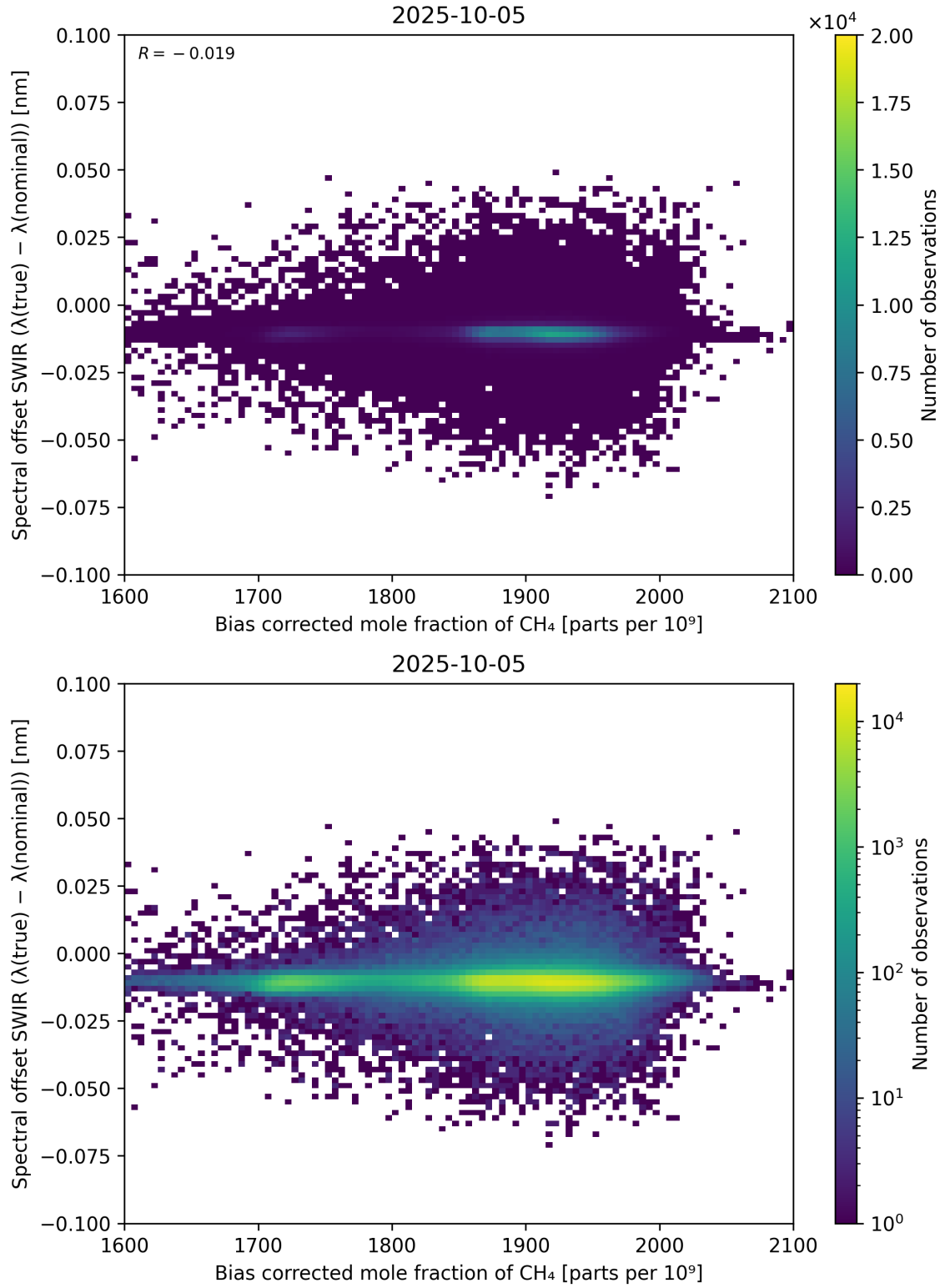
Figure 69: Scatter density plot of “Bias corrected mole fraction of \text{CH}_4 ” against “Spectral offset SWIR ( \lambda_{\text{true}} - \lambda_{\text{nominal}} )” for 2025-10-04 to 2025-10-06.
