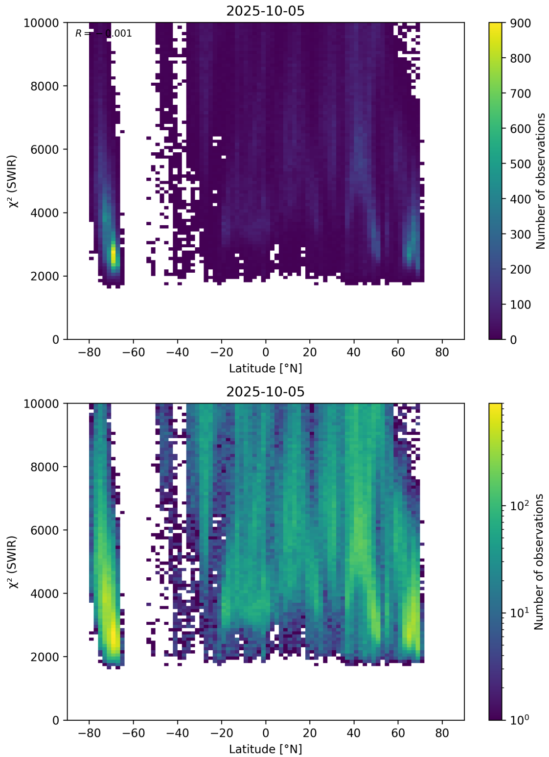
Figure 54: Scatter density plot of “Latitude” against “ \chi^2 (SWIR)” for 2025-10-04 to 2025-10-06.
