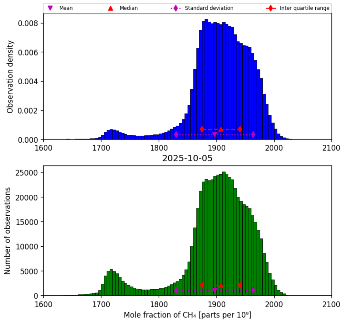
Figure 23: Histogram of “Mole fraction of CH 4 ” for 2025-10-04 to 2025-10-06
