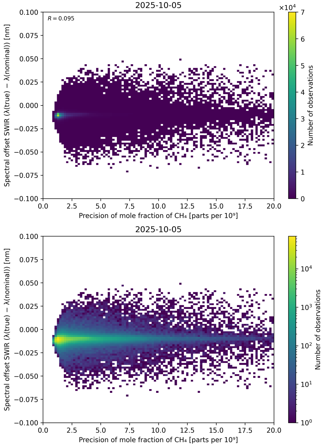
Figure 85: Scatter density plot of “Precision of mole fraction of \text{CH}_4 ” against “Spectral offset SWIR ( \lambda_{\text{true}} - \lambda_{\text{nominal}} )” for 2025-10-04 to 2025-10-06.
