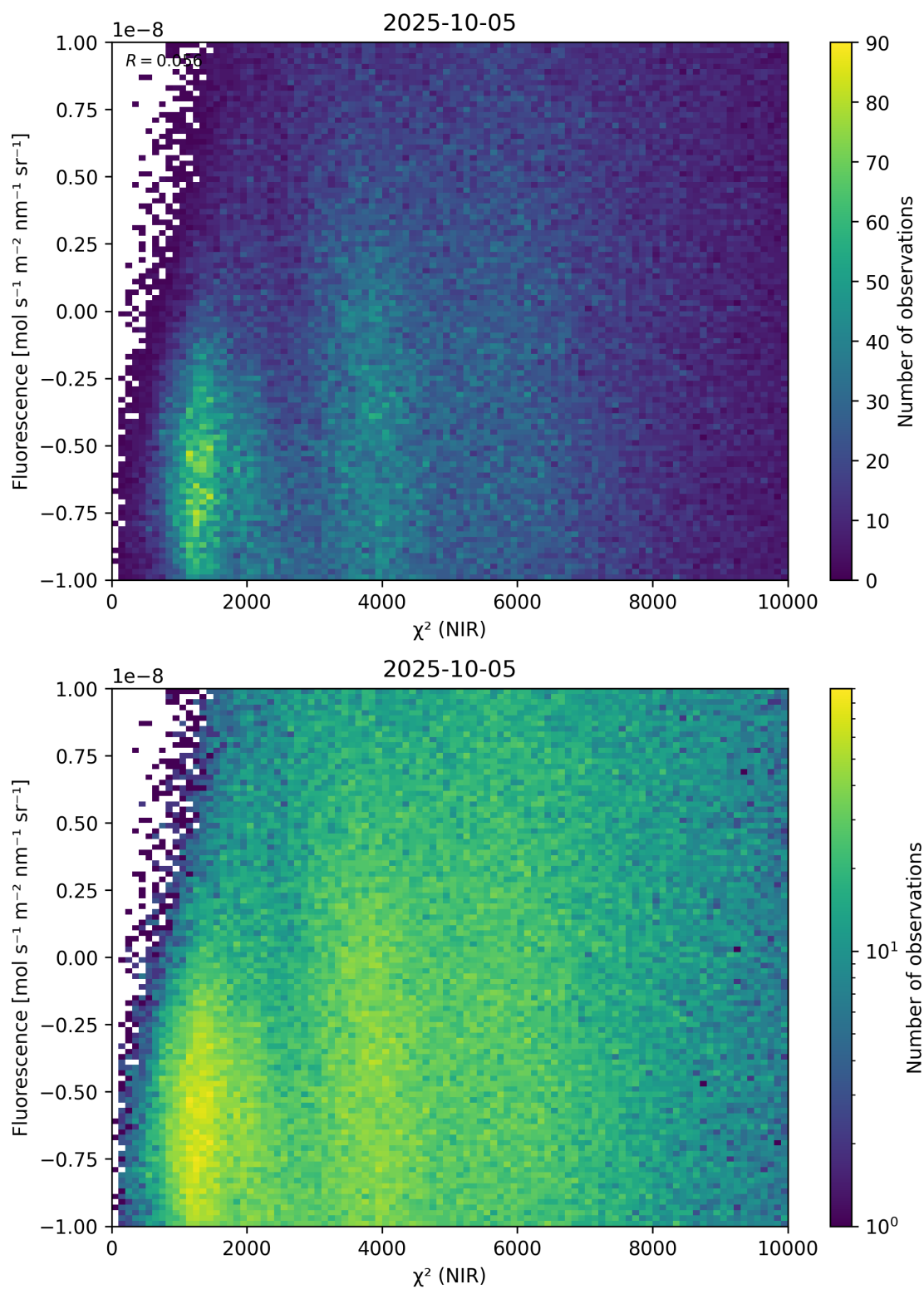
Figure 45: Scatter density plot of “ \chi^2 (NIR)” against “Fluorescence” for 2025-10-04 to 2025-10-06.
