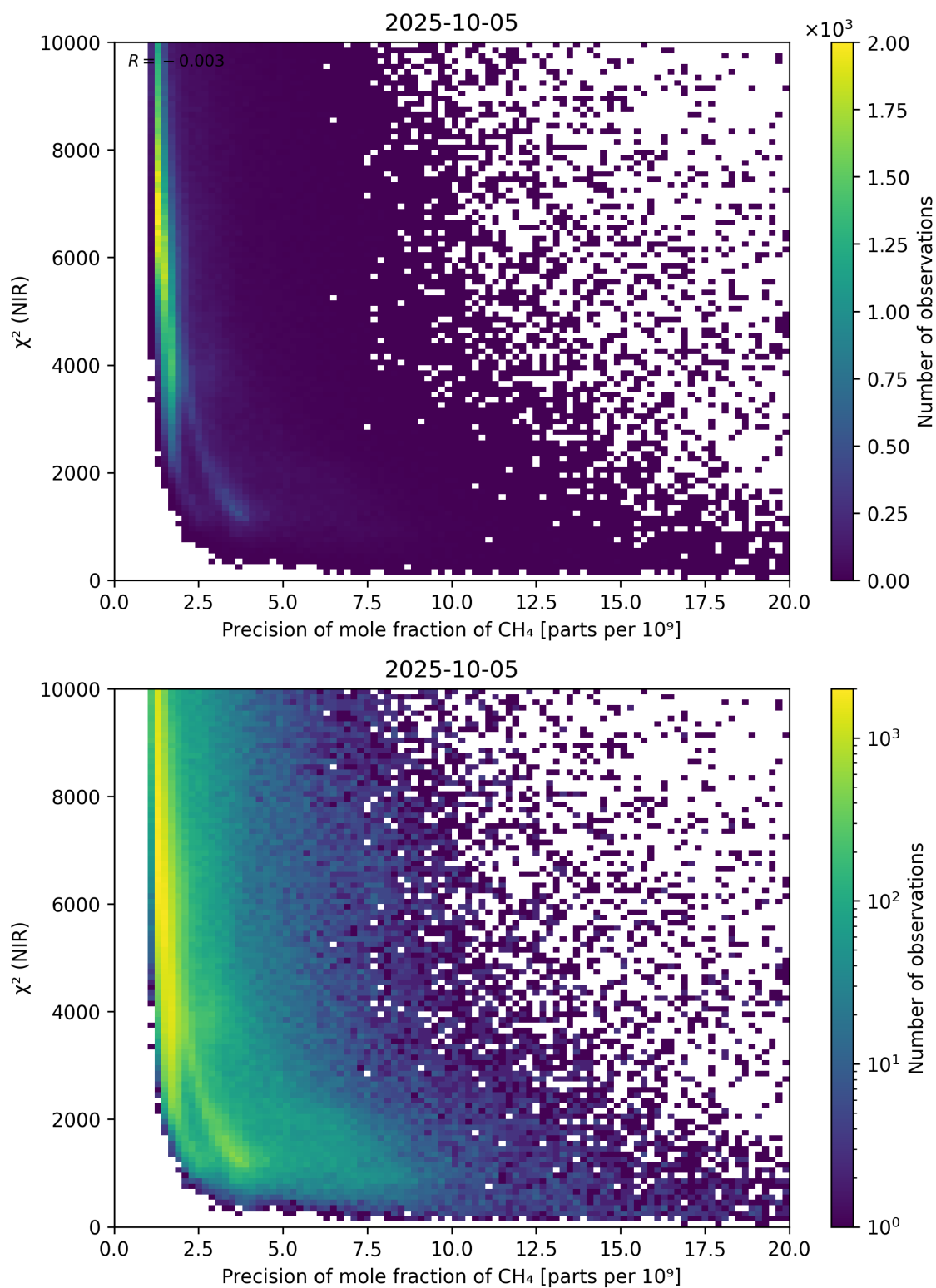
Figure 78: Scatter density plot of “Precision of mole fraction of CH 4 ” against “ \chi^2 (NIR)” for 2025-10-04 to 2025-10-06.
