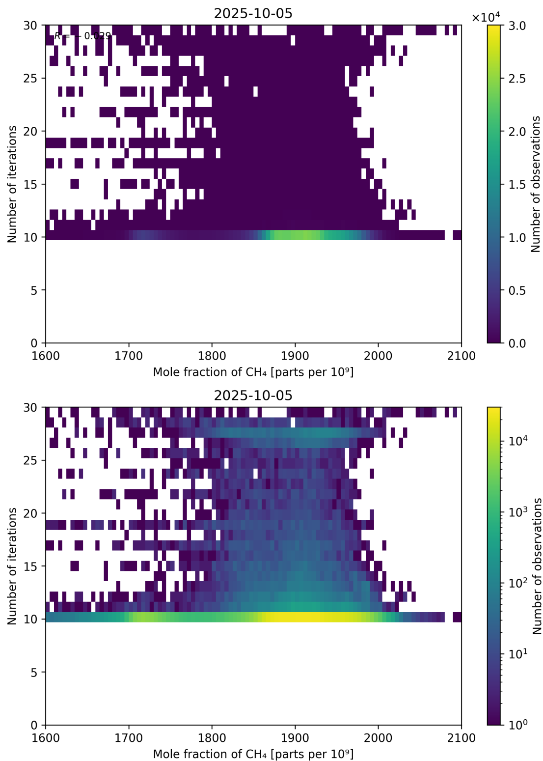
Figure 76: Scatter density plot of “Mole fraction of CH 4 ” against “Number of iterations” for 2025-10-04 to 2025-10-06.
