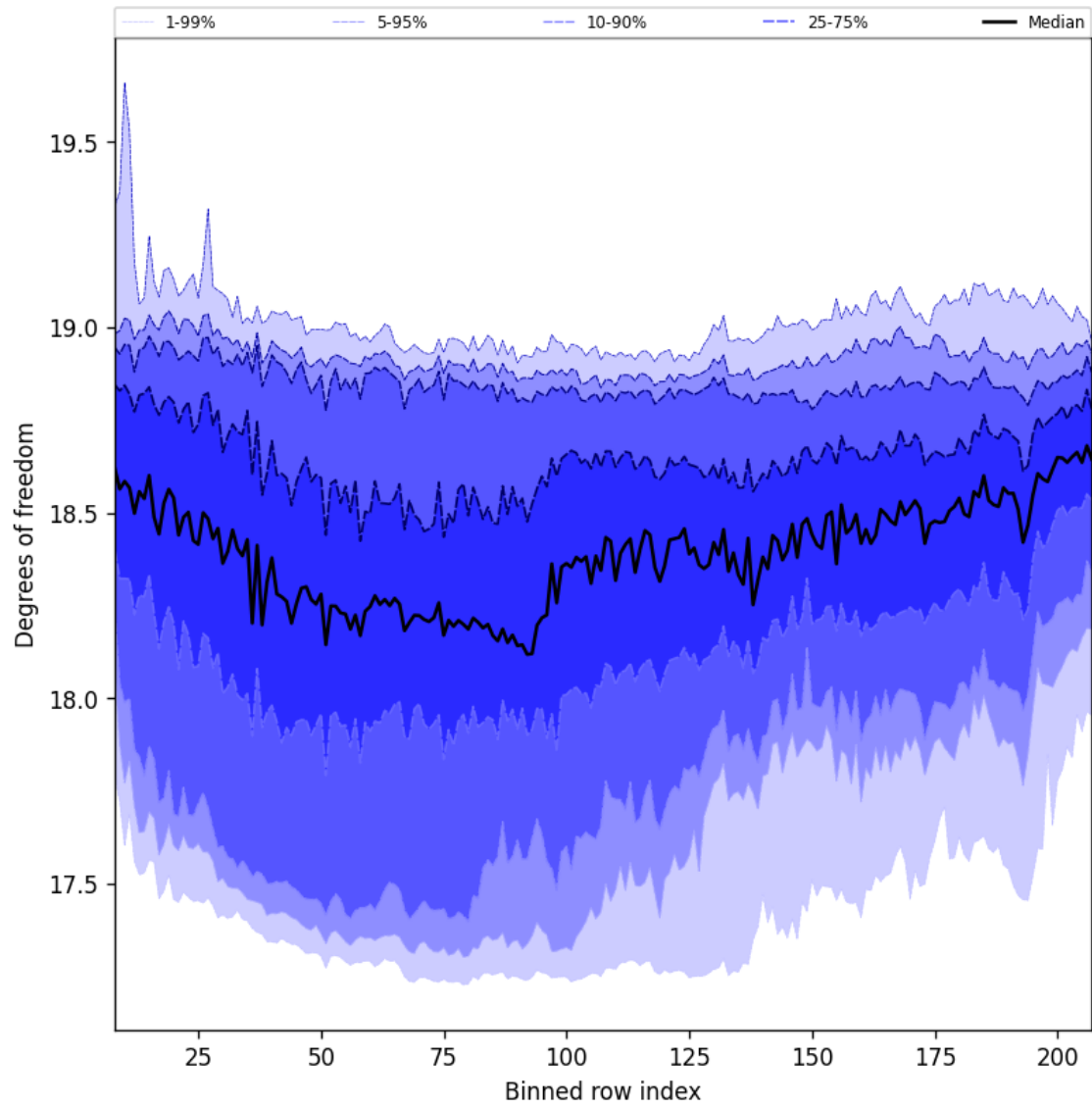
Figure 41: Along track statistics of “Degrees of freedom” for 2025-10-04 to 2025-10-06
