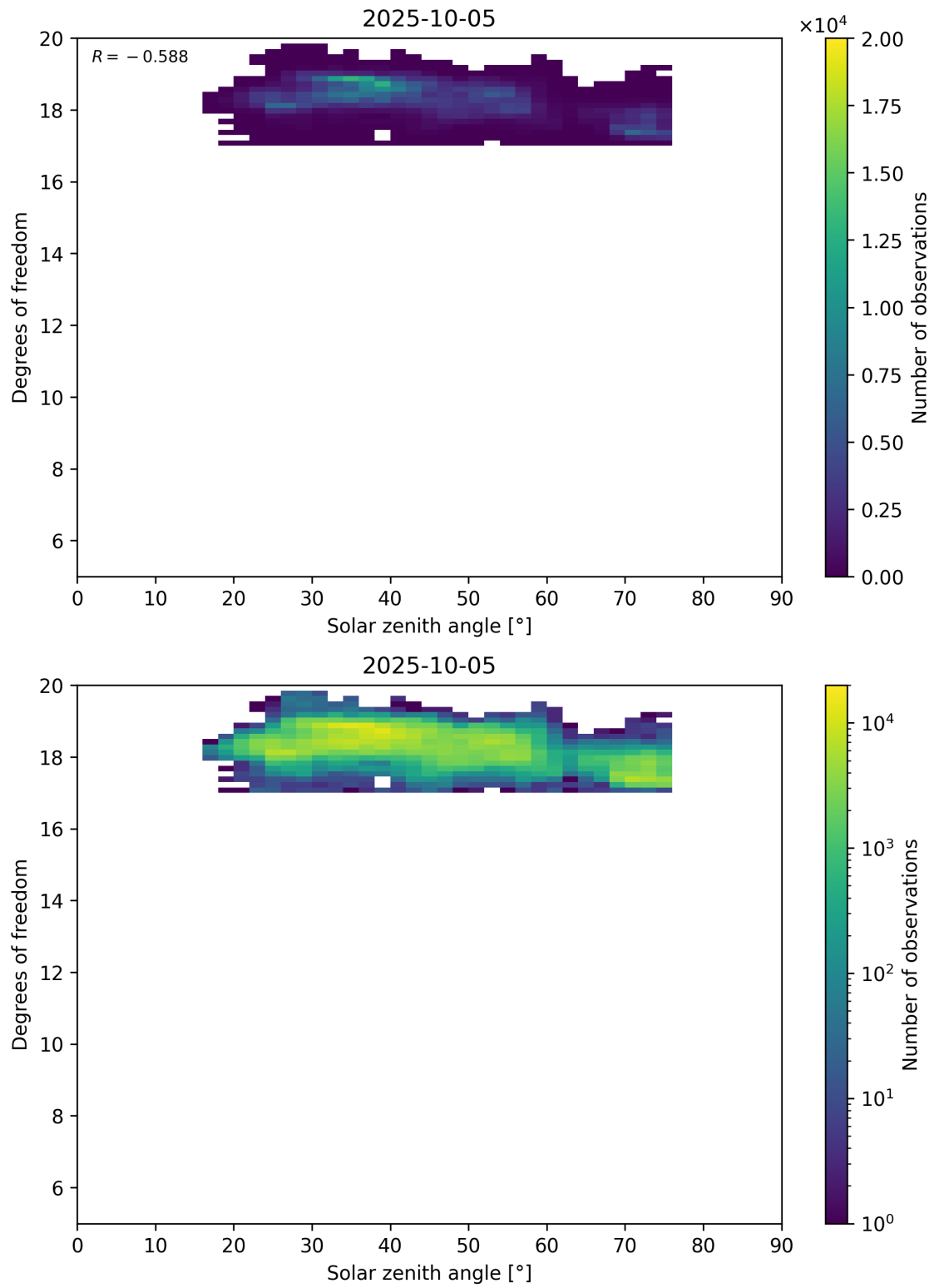
Figure 96: Scatter density plot of “Solar zenith angle” against “Degrees of freedom” for 2025-10-04 to 2025-10-06.
