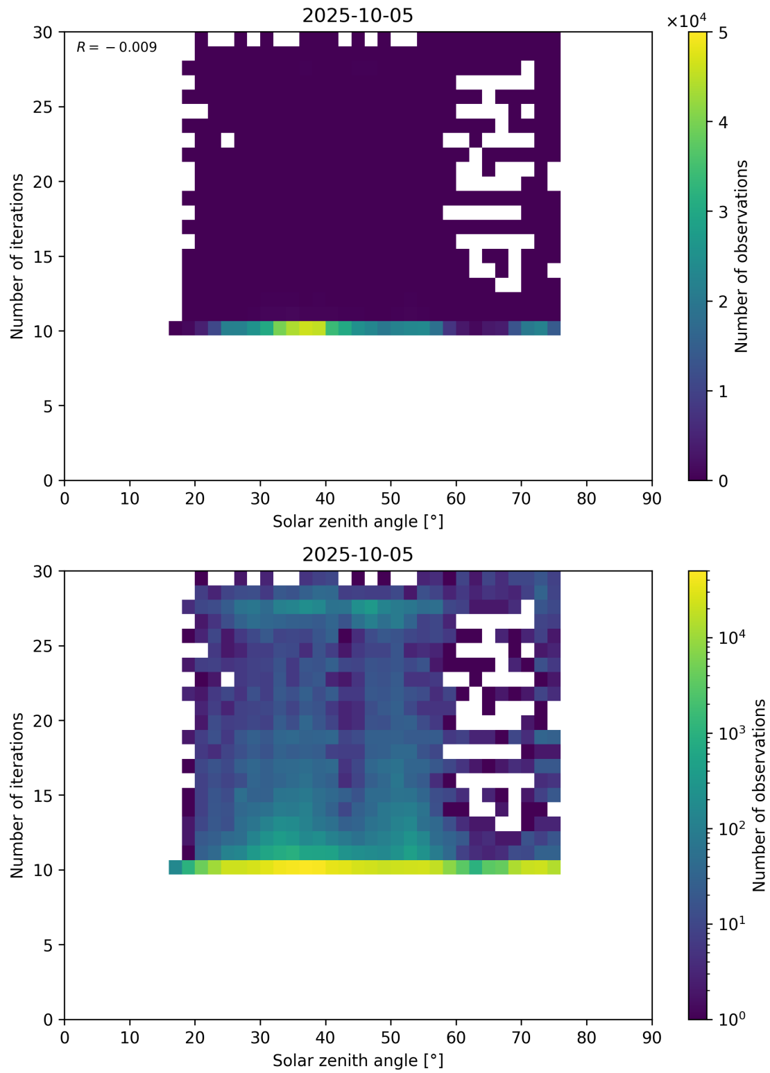
Figure 102: Scatter density plot of “Solar zenith angle” against “Number of iterations” for 2025-10-04 to 2025-10-06.
