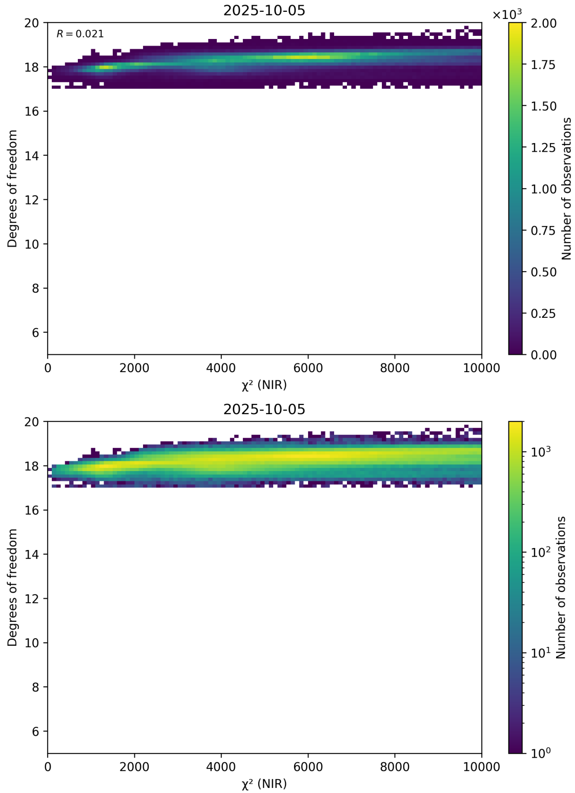
Figure 44: Scatter density plot of “ \chi^2 (NIR)” against “Degrees of freedom” for 2025-10-04 to 2025-10-06.
