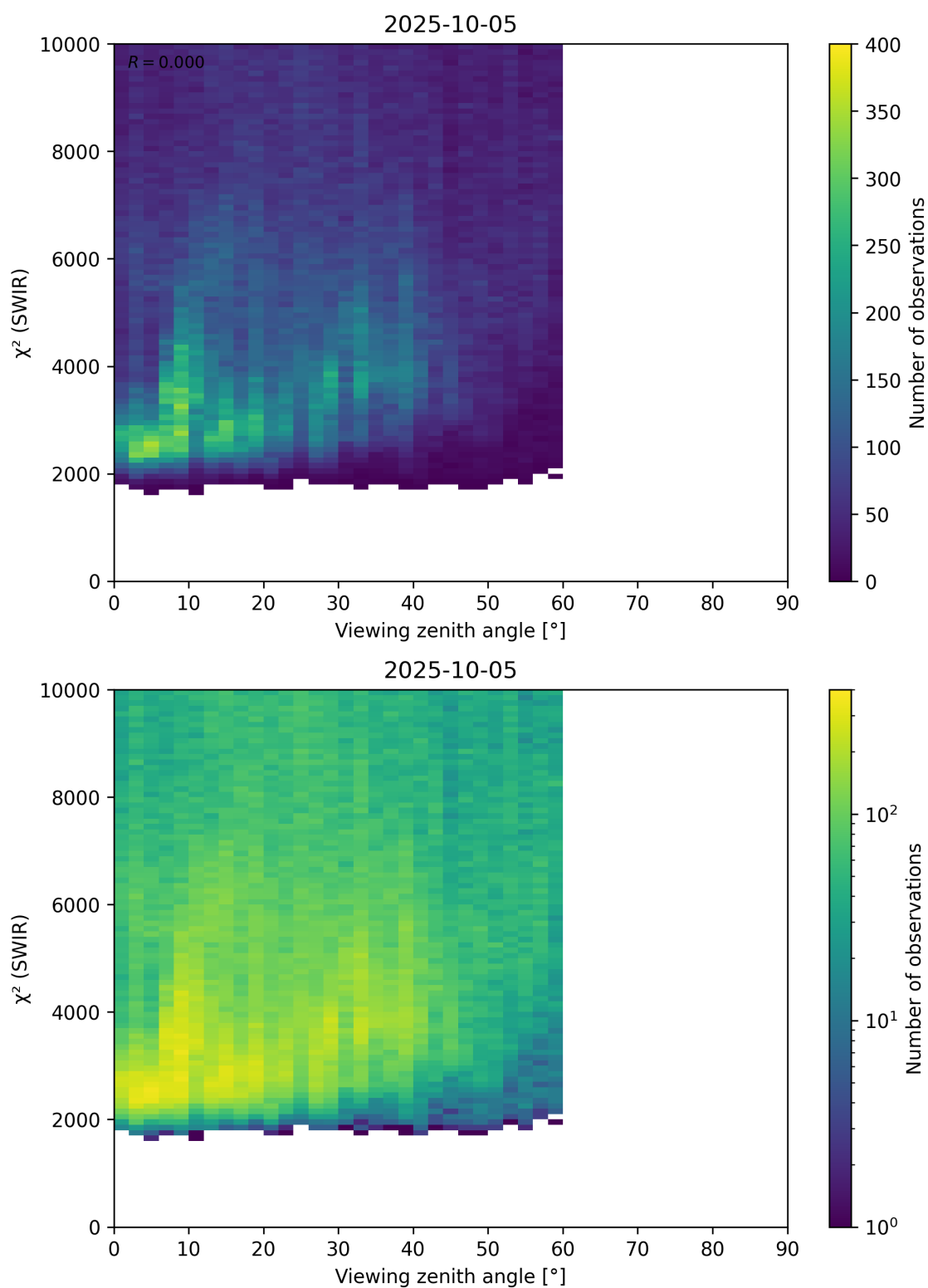
Figure 106: Scatter density plot of “Viewing zenith angle” against “ \chi^2 (SWIR)” for 2025-10-04 to 2025-10-06.
