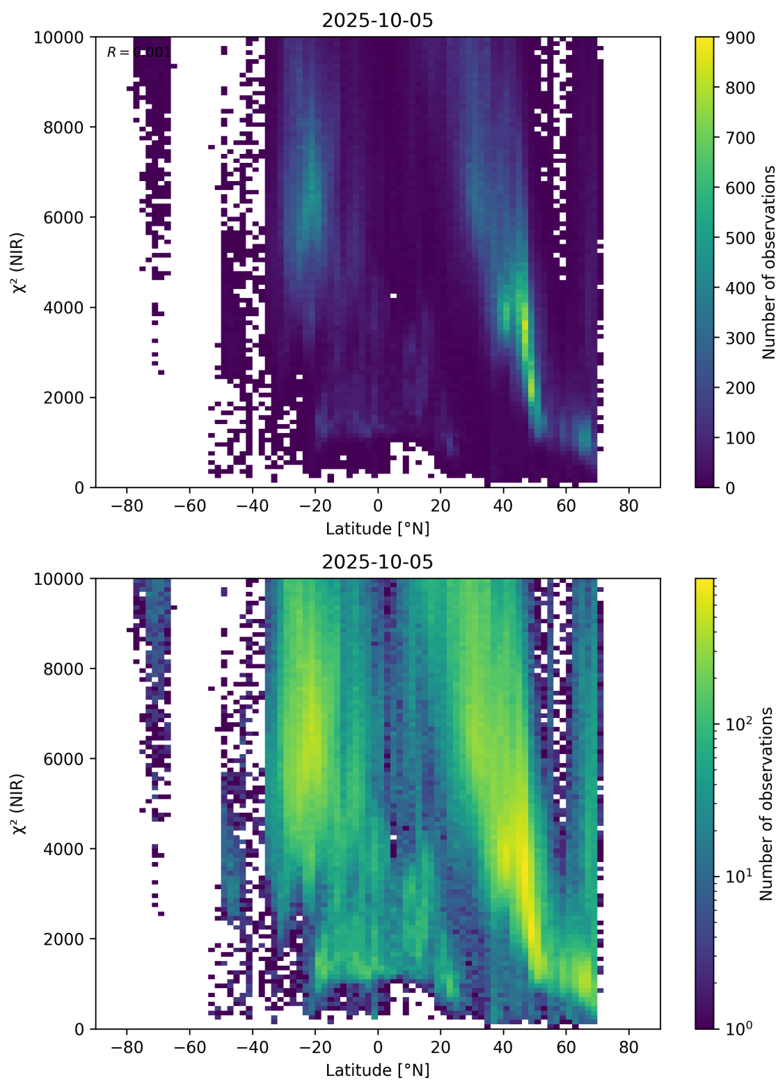
Figure 53: Scatter density plot of “Latitude” against “ \chi^2 (NIR)” for 2025-10-04 to 2025-10-06.
