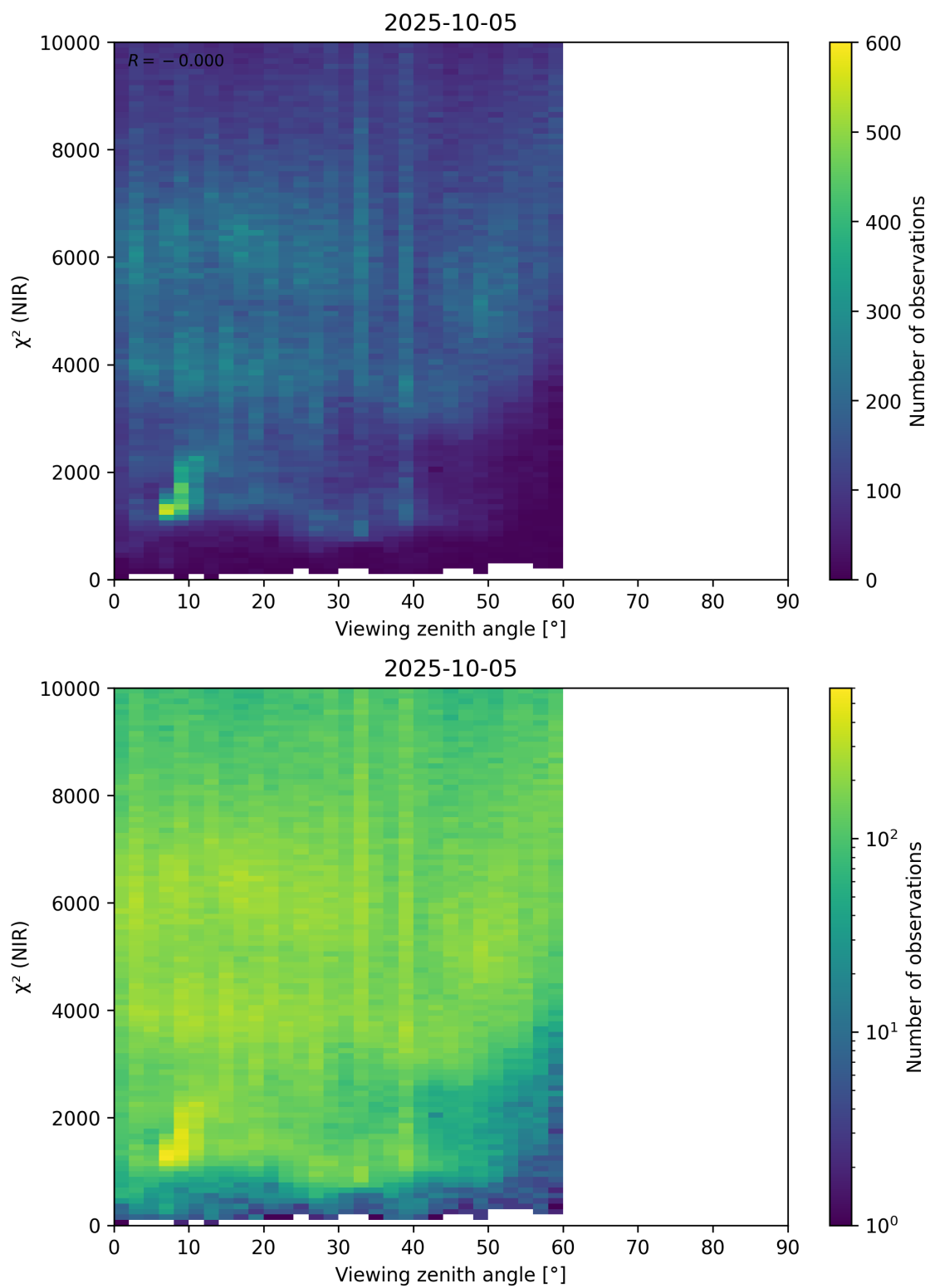
Figure 105: Scatter density plot of “Viewing zenith angle” against “ \chi^2 (NIR)” for 2025-10-04 to 2025-10-06.
