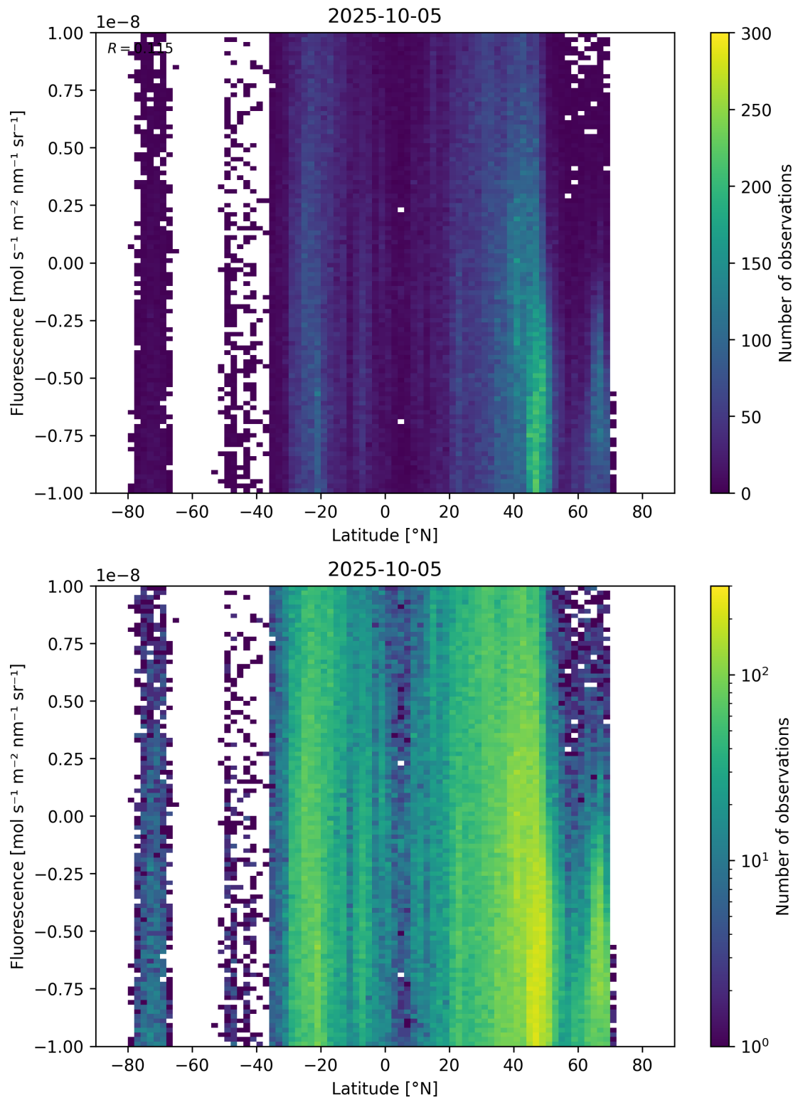
Figure 56: Scatter density plot of “Latitude” against “Fluorescence” for 2025-10-04 to 2025-10-06.
