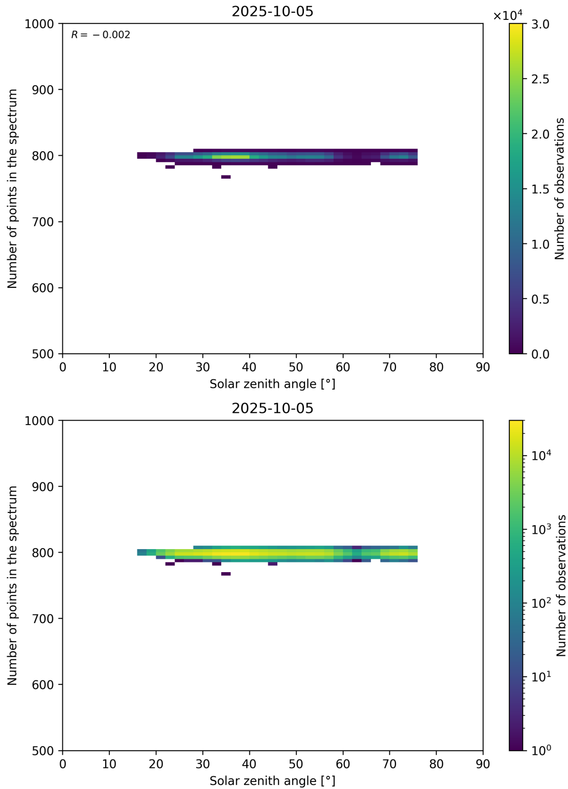
Figure 103: Scatter density plot of “Solar zenith angle” against “Number of points in the spectrum” for 2025-10-04 to 2025-10-06.
