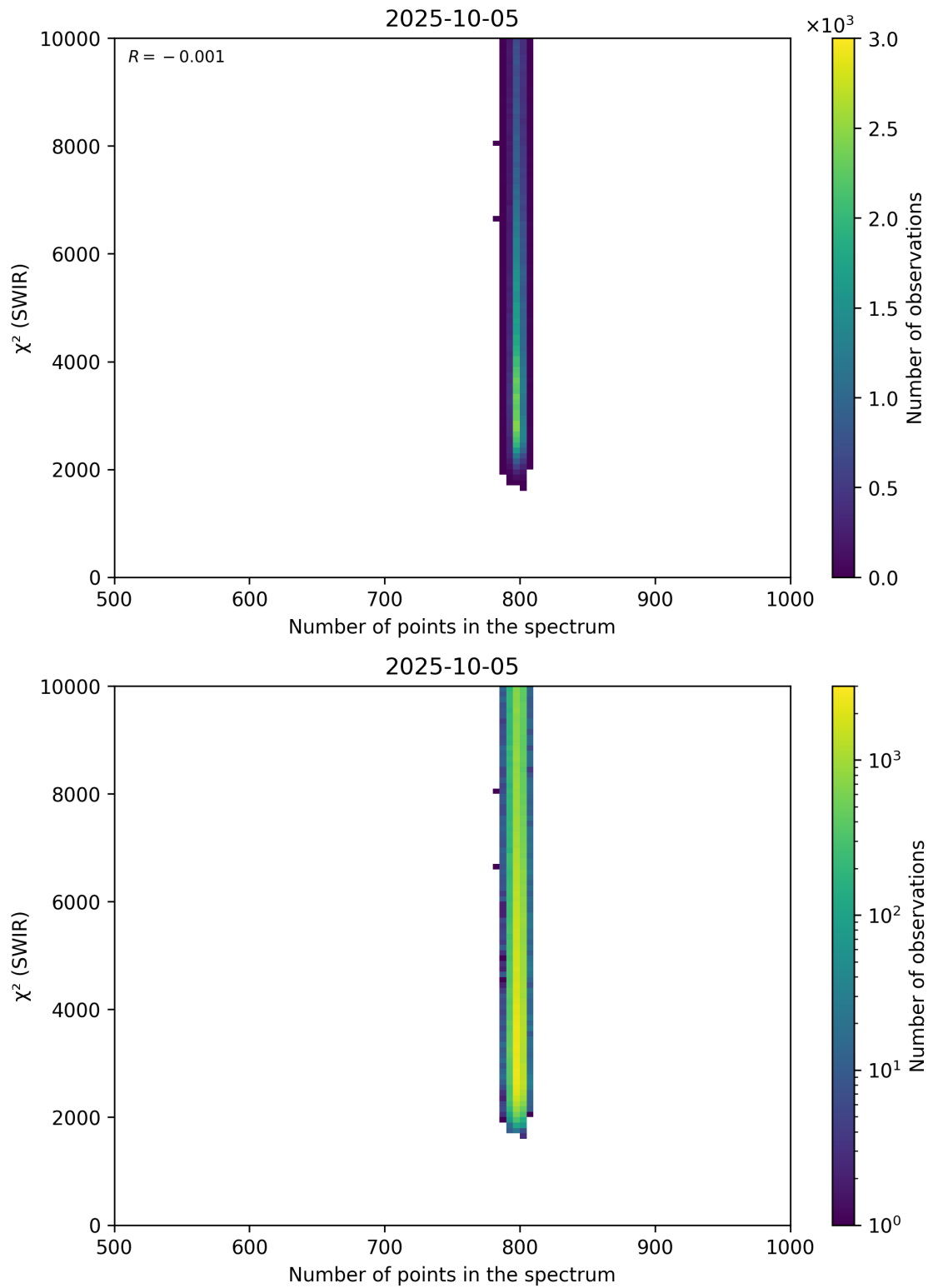
Figure 89: Scatter density plot of “Number of points in the spectrum” against “ \chi^2 (SWIR)” for 2025-10-04 to 2025-10-06.
