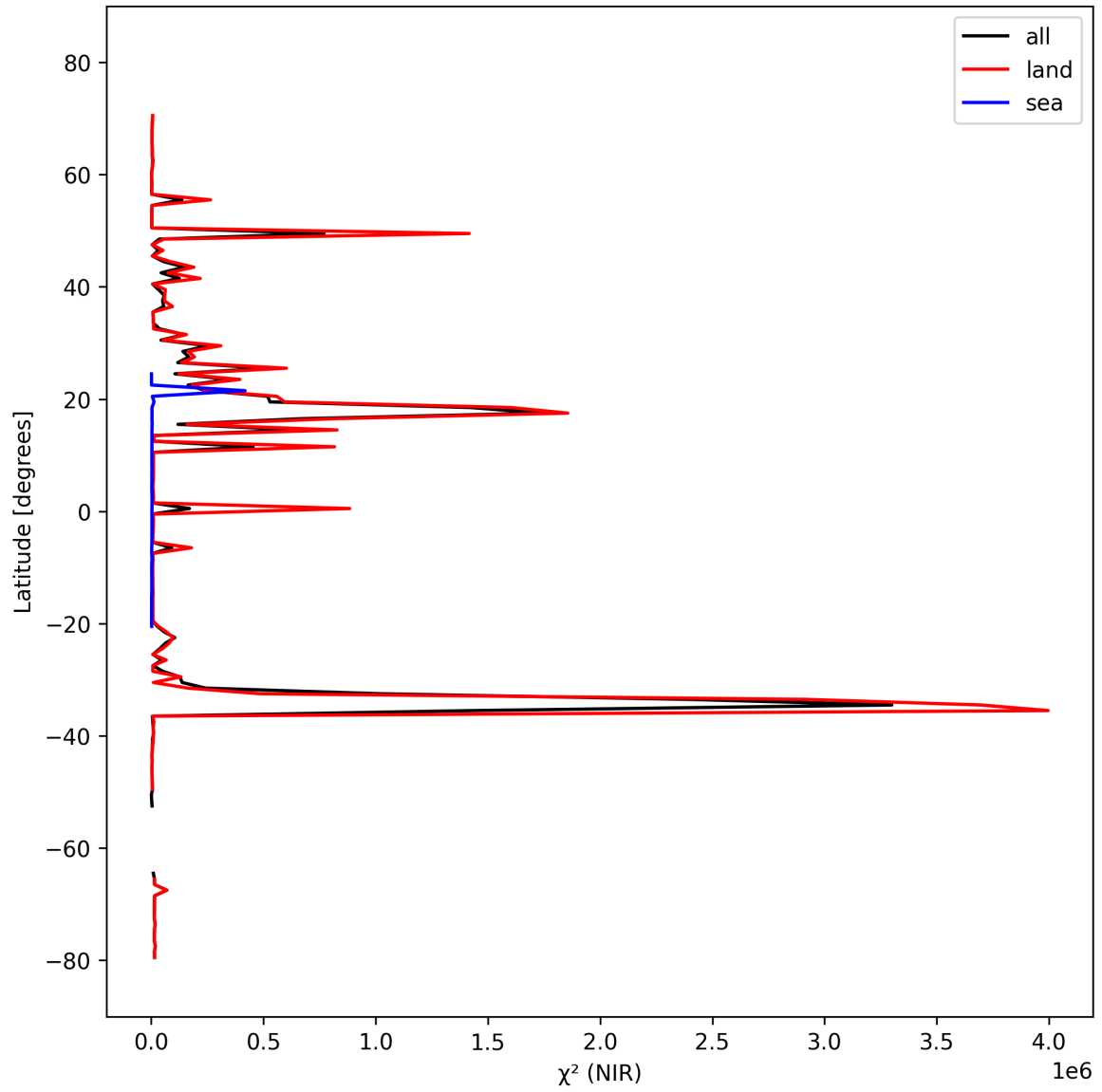
Figure 18: Zonal average of “ \chi^2 (NIR)” for 2025-10-04 to 2025-10-06.
