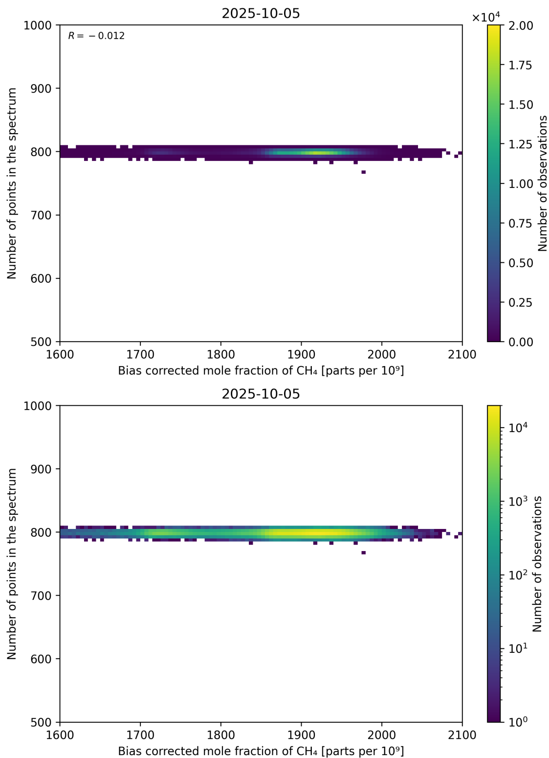
Figure 68: Scatter density plot of “Bias corrected mole fraction of CH 4 ” against “Number of points in the spectrum” for 2025-10-04 to 2025-10-06.
