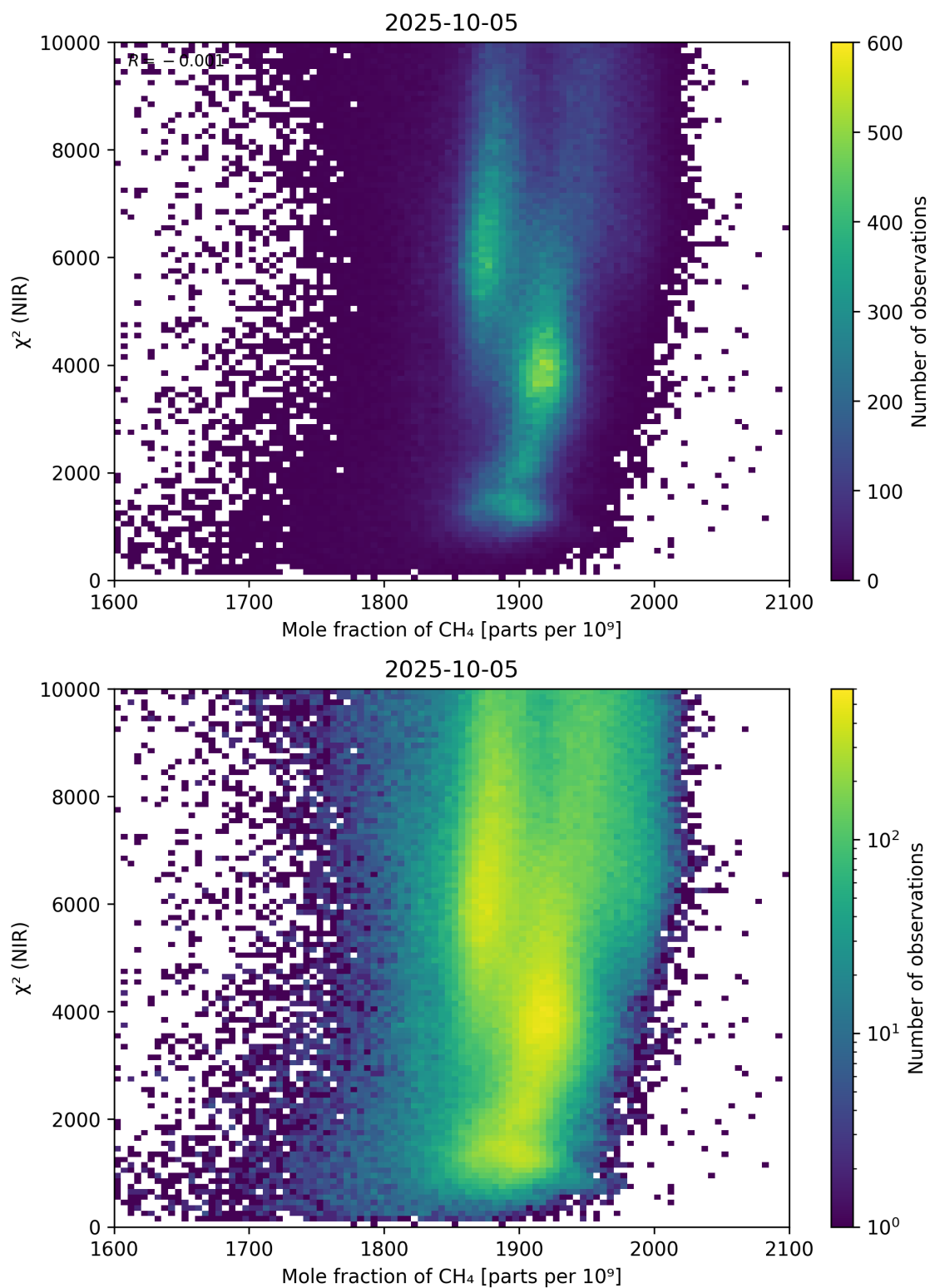
Figure 70: Scatter density plot of “Mole fraction of \text{CH}_4 ” against “ \chi^2 (NIR)” for 2025-10-04 to 2025-10-06.
