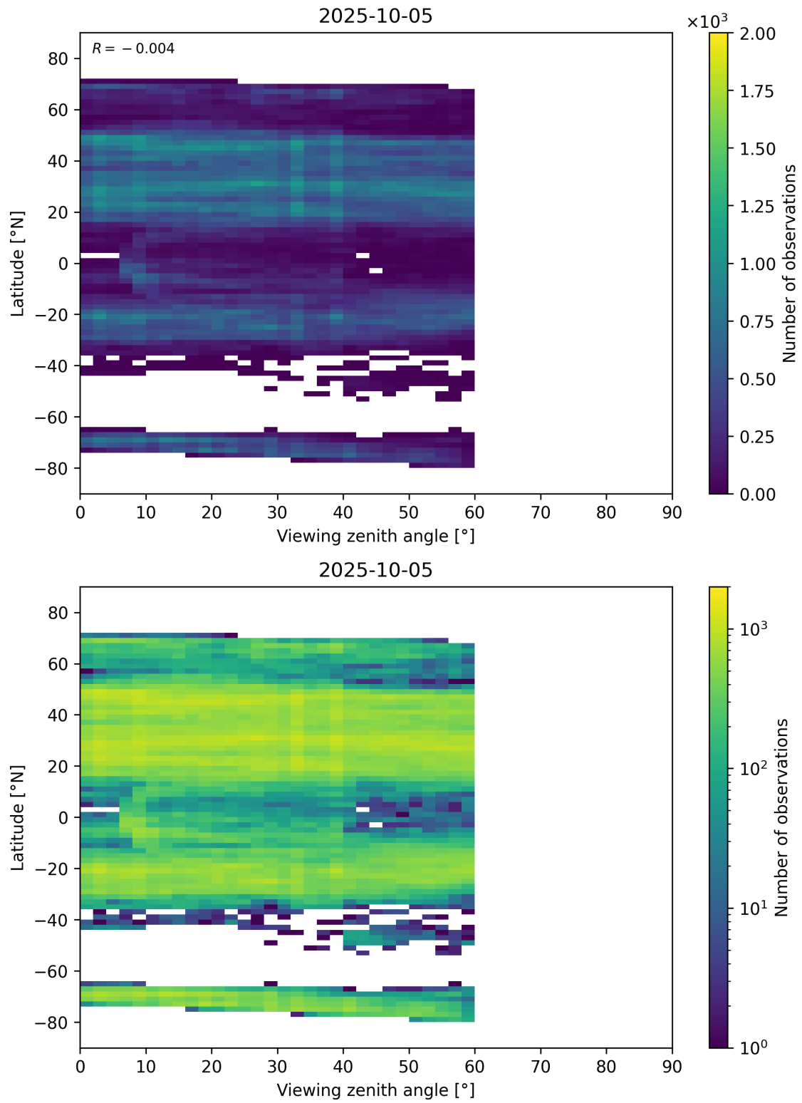
Figure 109: Scatter density plot of “Viewing zenith angle” against “Latitude” for 2025-10-04 to 2025-10-06.
