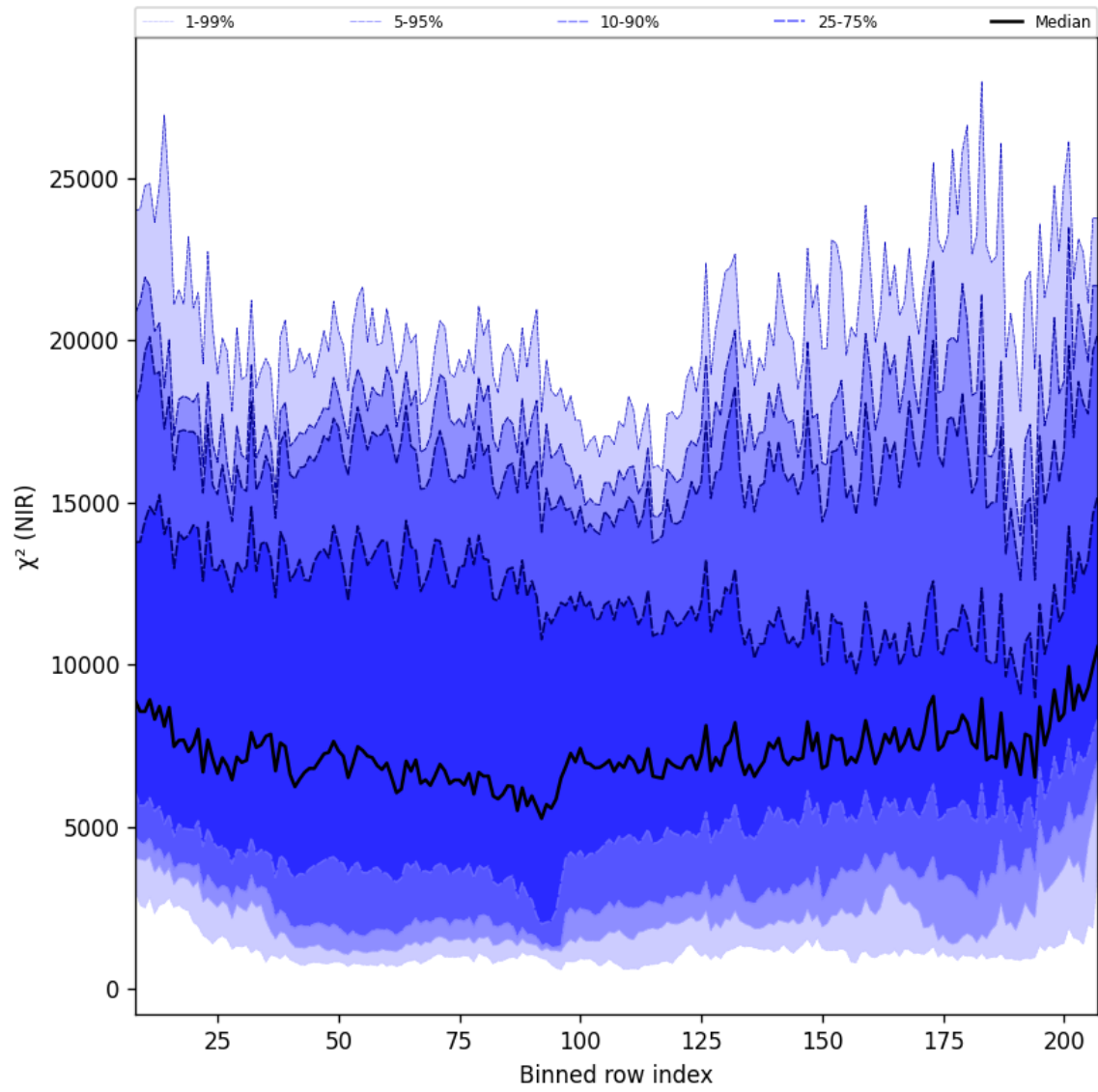
Figure 40: Along track statistics of “ \chi^2 (NIR)” for 2025-10-04 to 2025-10-06
