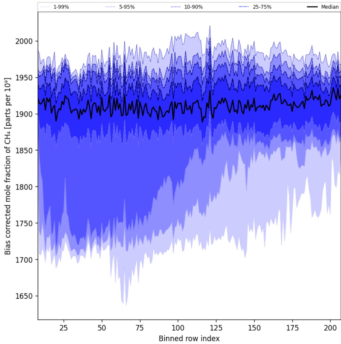
Figure 36: Along track statistics of “Bias corrected mole fraction of CH 4 ” for 2025-10-04 to 2025-10-06
