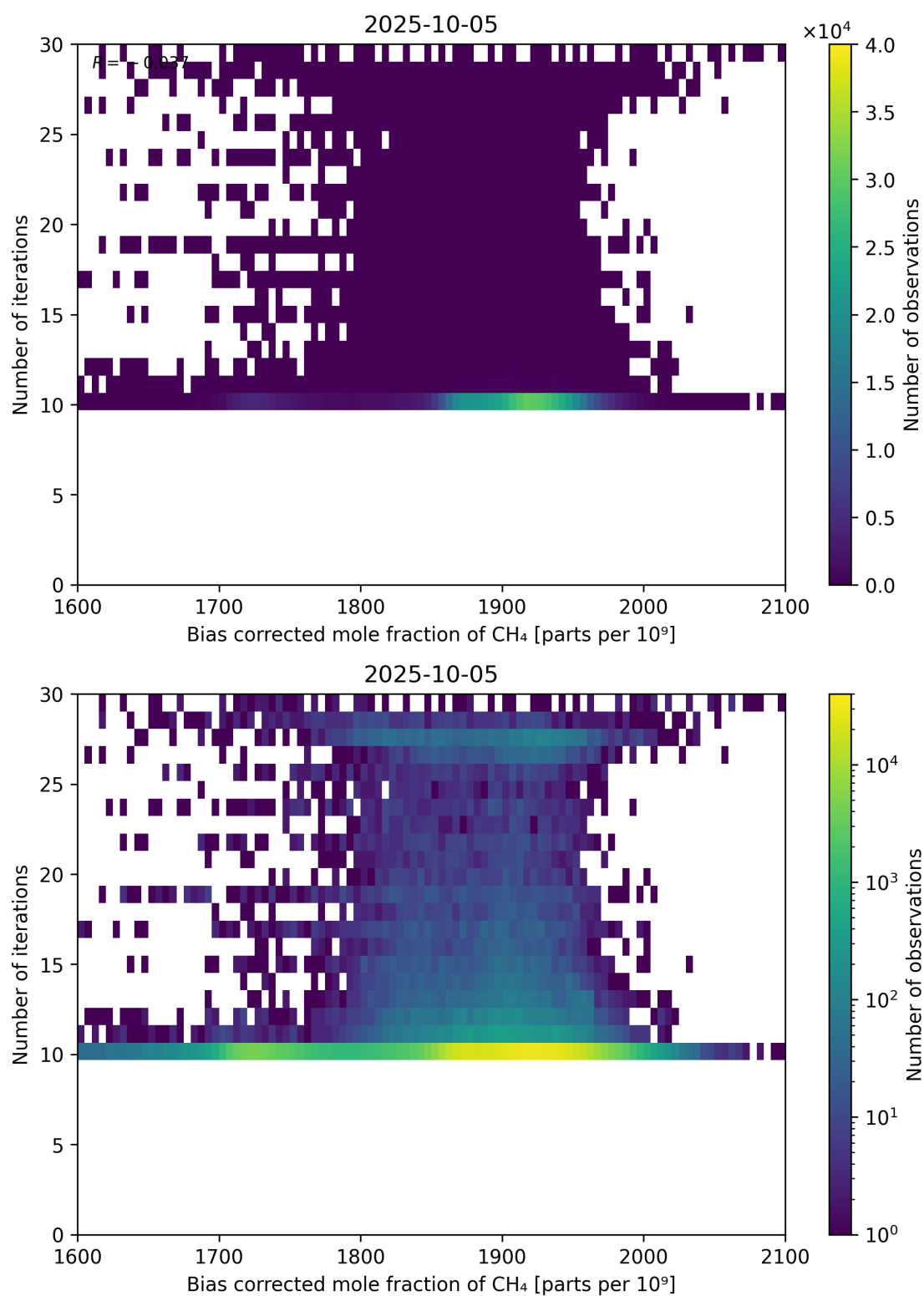
Figure 67: Scatter density plot of “Bias corrected mole fraction of CH 4 ” against “Number of iterations” for 2025-10-04 to 2025-10-06.
