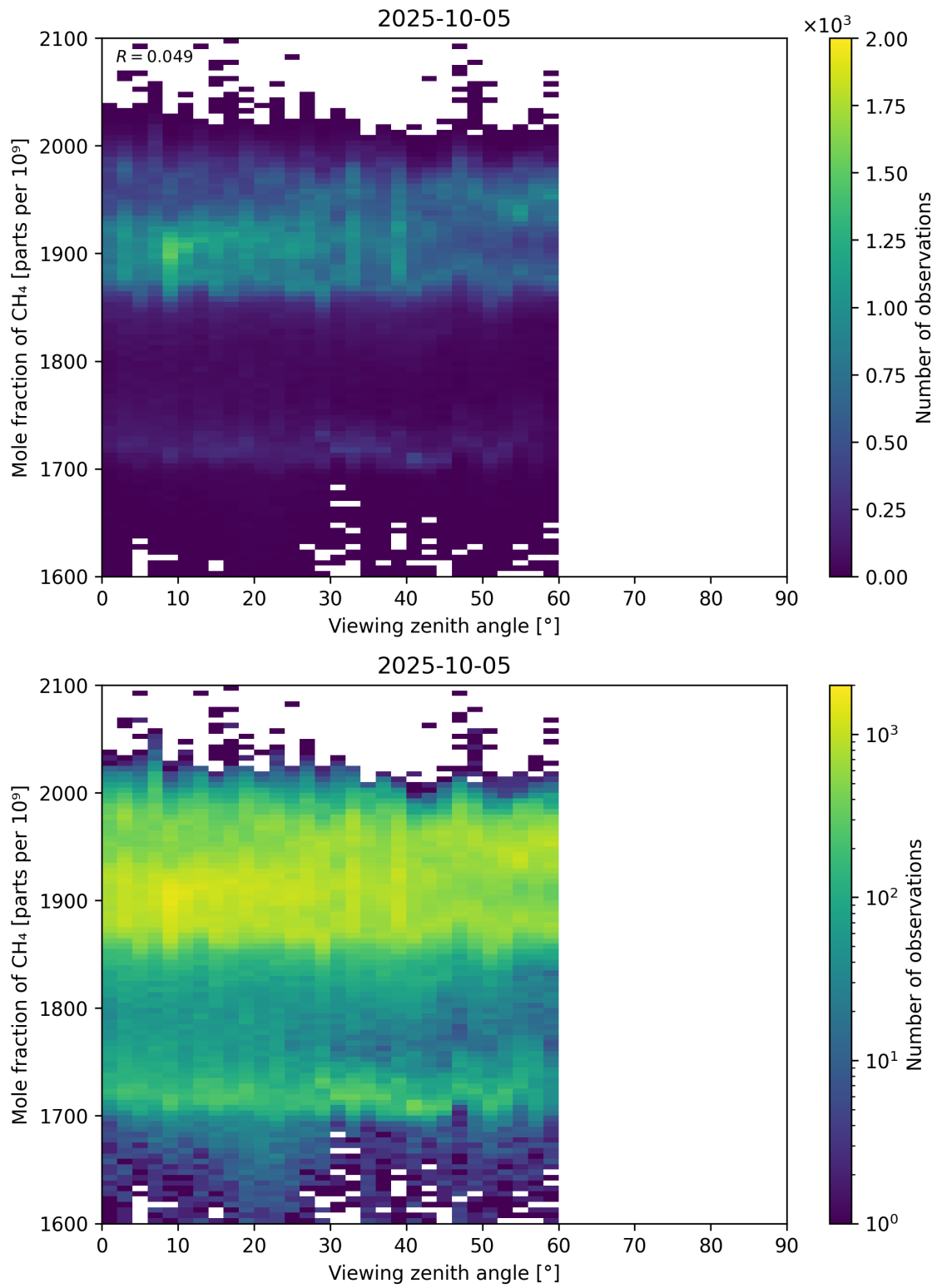
Figure 110: Scatter density plot of “Viewing zenith angle” against “Mole fraction of CH 4 ” for 2025-10-04 to 2025-10-06.
