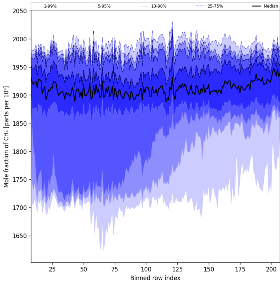
Figure 34: Along track statistics of “Mole fraction of CH 4 ” for 2025-10-04 to 2025-10-06
