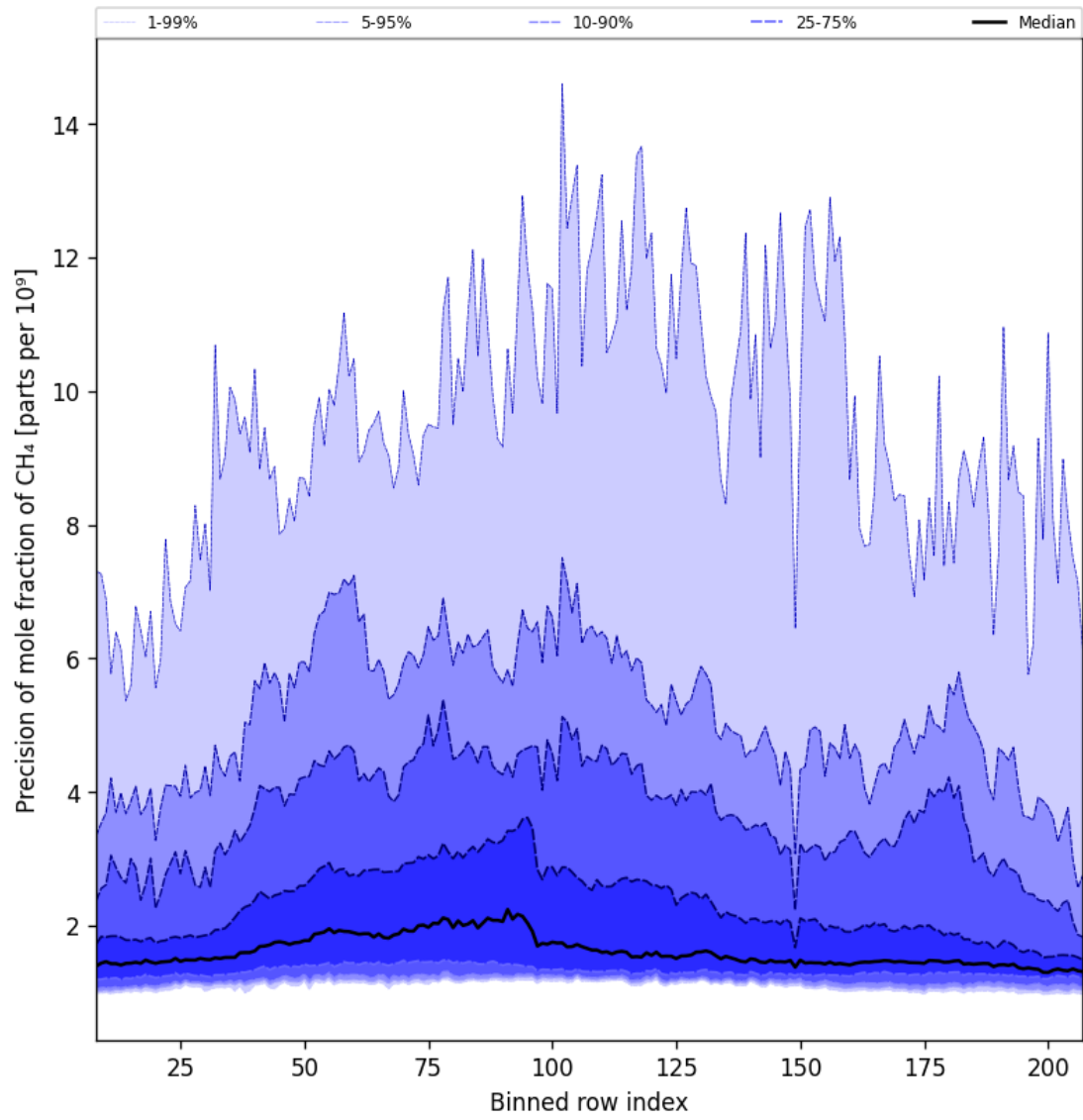
Figure 35: Along track statistics of “Precision of mole fraction of CH 4 ” for 2025-10-04 to 2025-10-06
