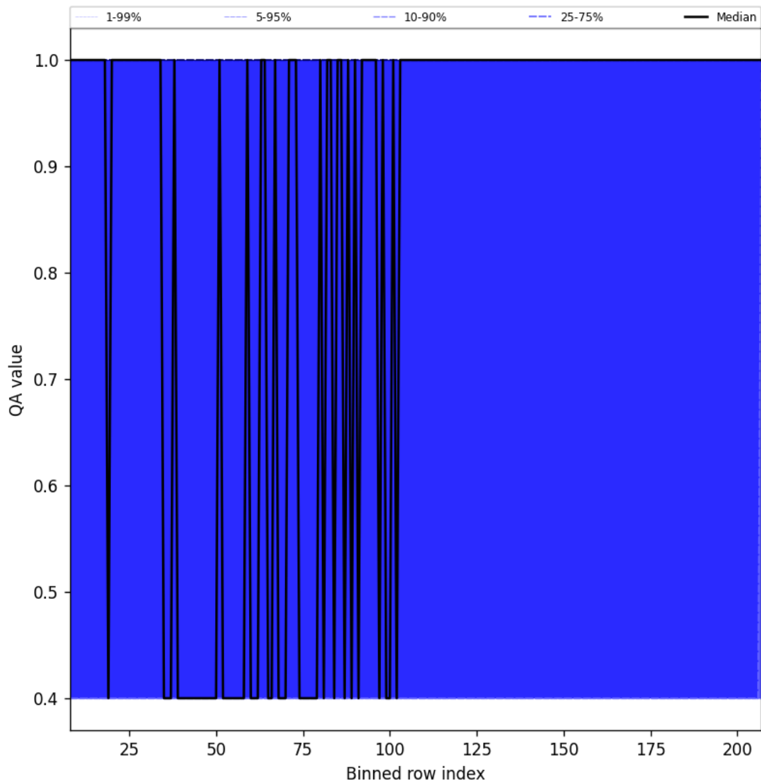
Figure 33: Along track statistics of “QA value” for 2025-10-04 to 2025-10-06
