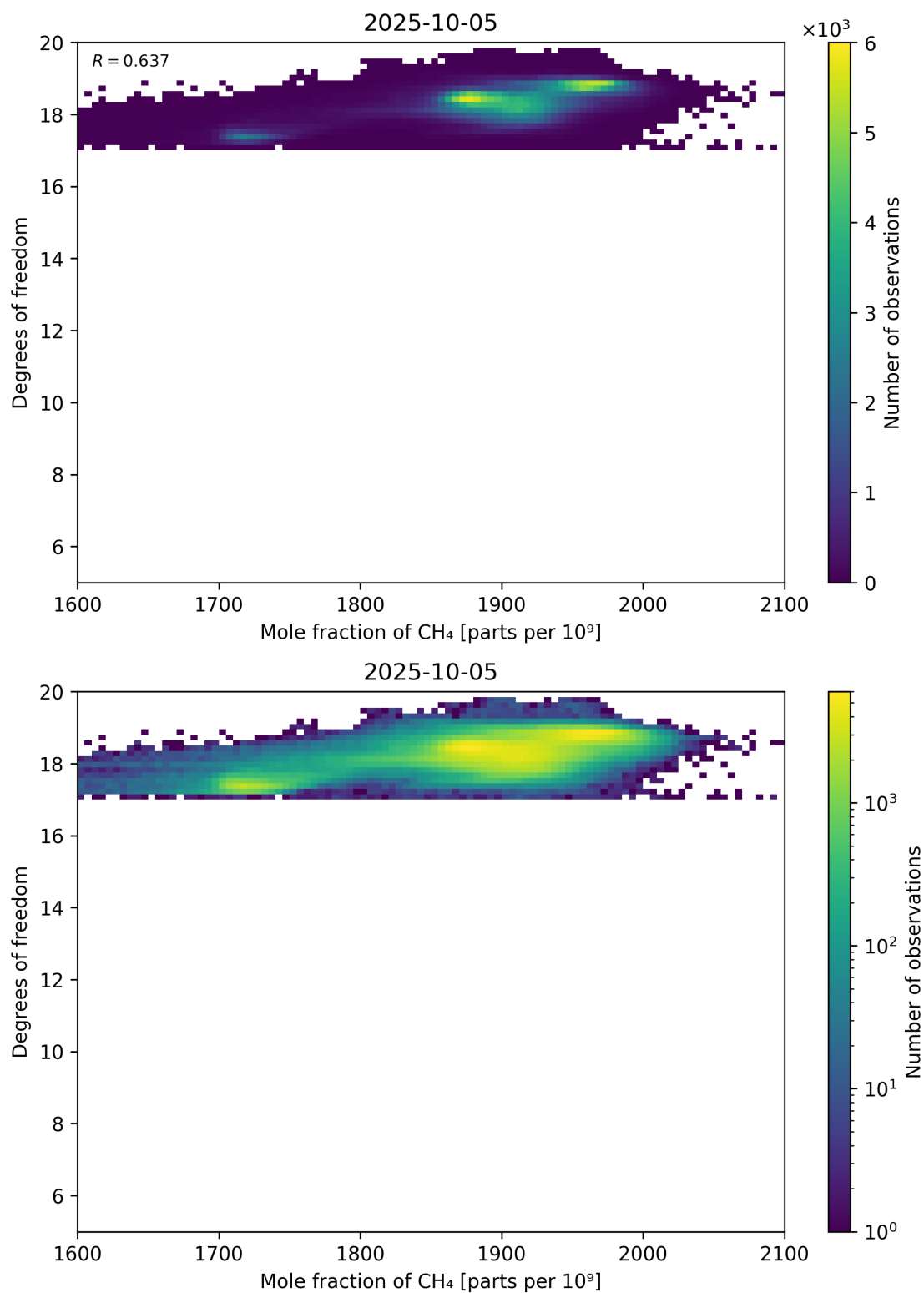
Figure 72: Scatter density plot of “Mole fraction of CH 4 ” against “Degrees of freedom” for 2025-10-04 to 2025-10-06.
