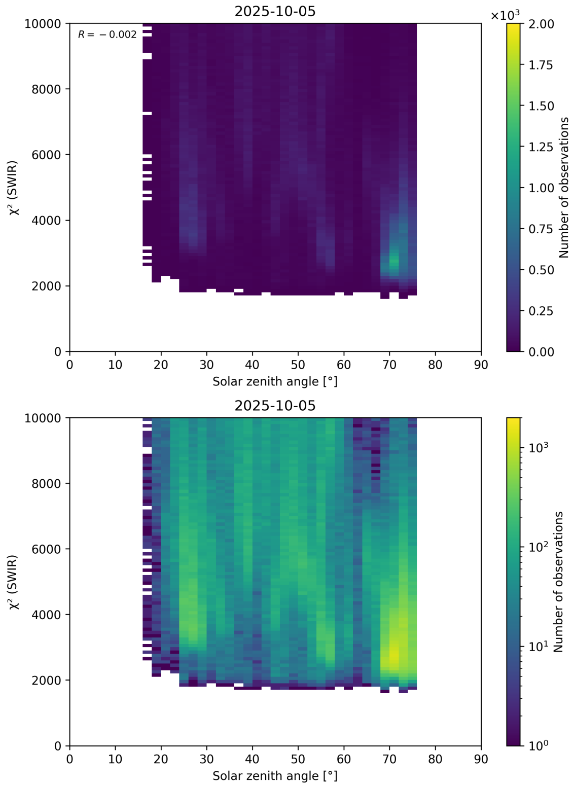
Figure 95: Scatter density plot of “Solar zenith angle” against “ \chi^2 (SWIR)” for 2025-10-04 to 2025-10-06.
