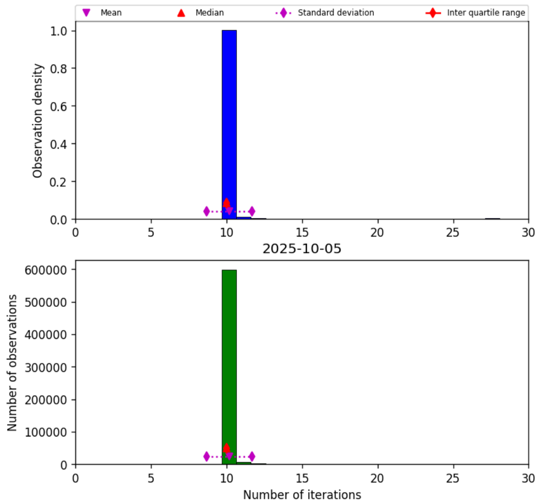
Figure 31: Histogram of “Number of iterations” for 2025-10-04 to 2025-10-06
