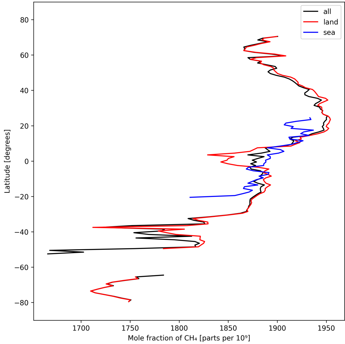
Figure 12: Zonal average of “Mole fraction of \text{CH}_4 ” for 2025-10-04 to 2025-10-06.
