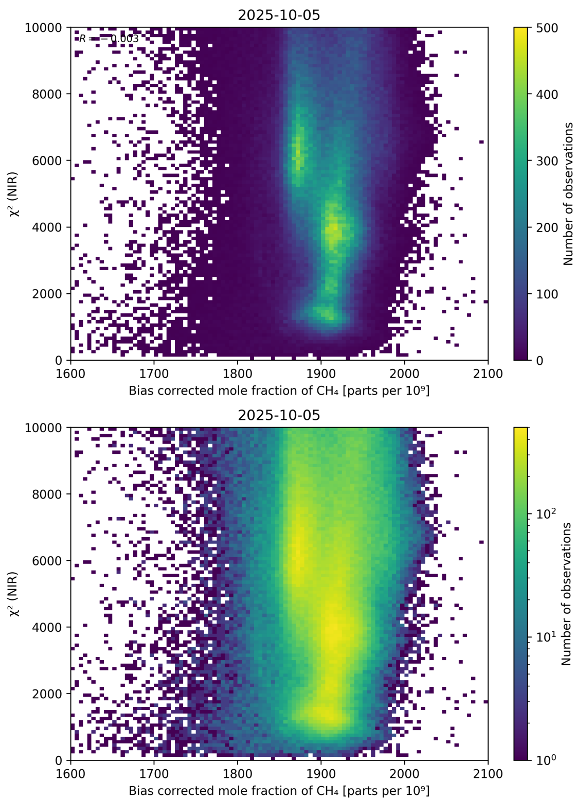
Figure 63: Scatter density plot of “Bias corrected mole fraction of \text{CH}_4 ” against “ \chi^2 (NIR)” for 2025-10-04 to 2025-10-06.
