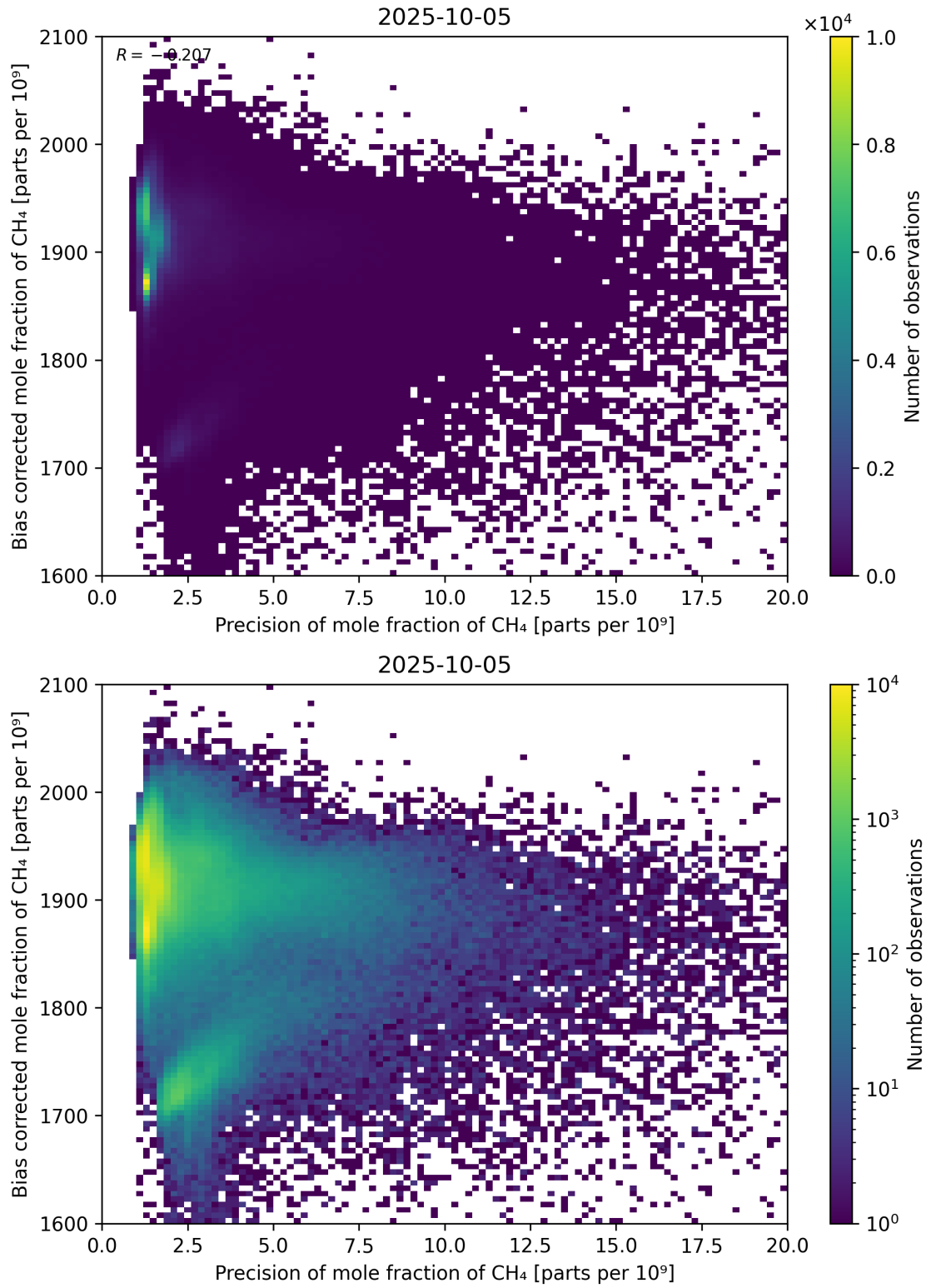
Figure 82: Scatter density plot of “Precision of mole fraction of CH 4 ” against “Bias corrected mole fraction of CH 4 ” for 2025-10-04 to 2025-10-06.
