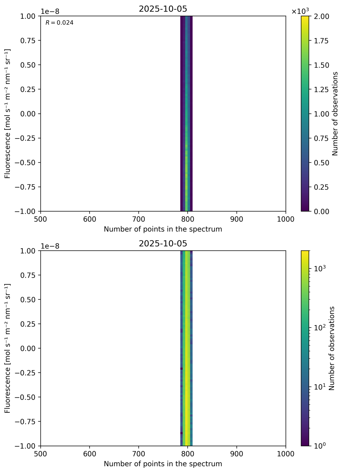
Figure 91: Scatter density plot of “Number of points in the spectrum” against “Fluorescence” for 2025-10-04 to 2025-10-06.
