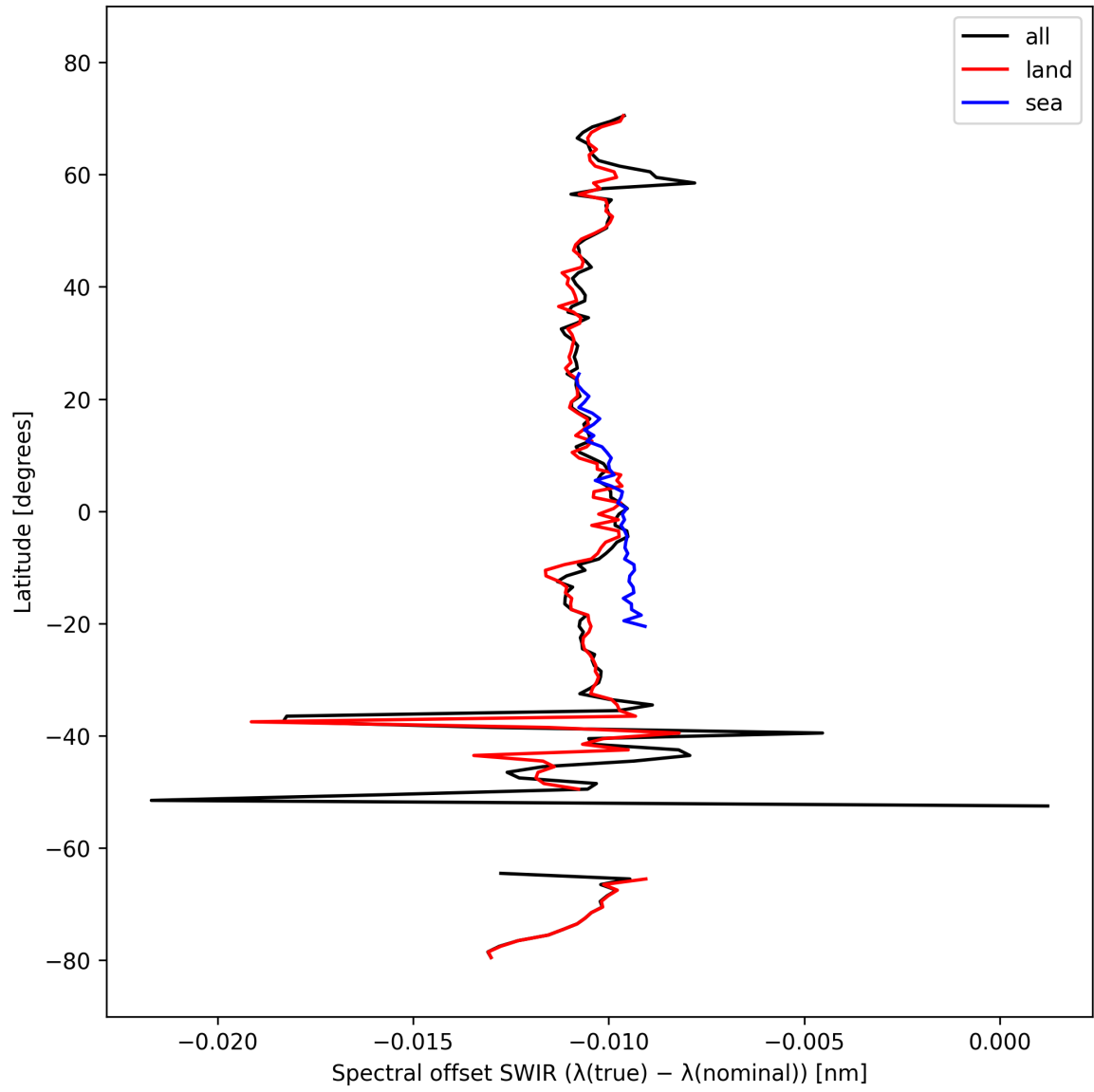
Figure 16: Zonal average of “Spectral offset SWIR ( \lambda_{\text{true}} - \lambda_{\text{nominal}} )” for 2025-10-04 to 2025-10-06.
