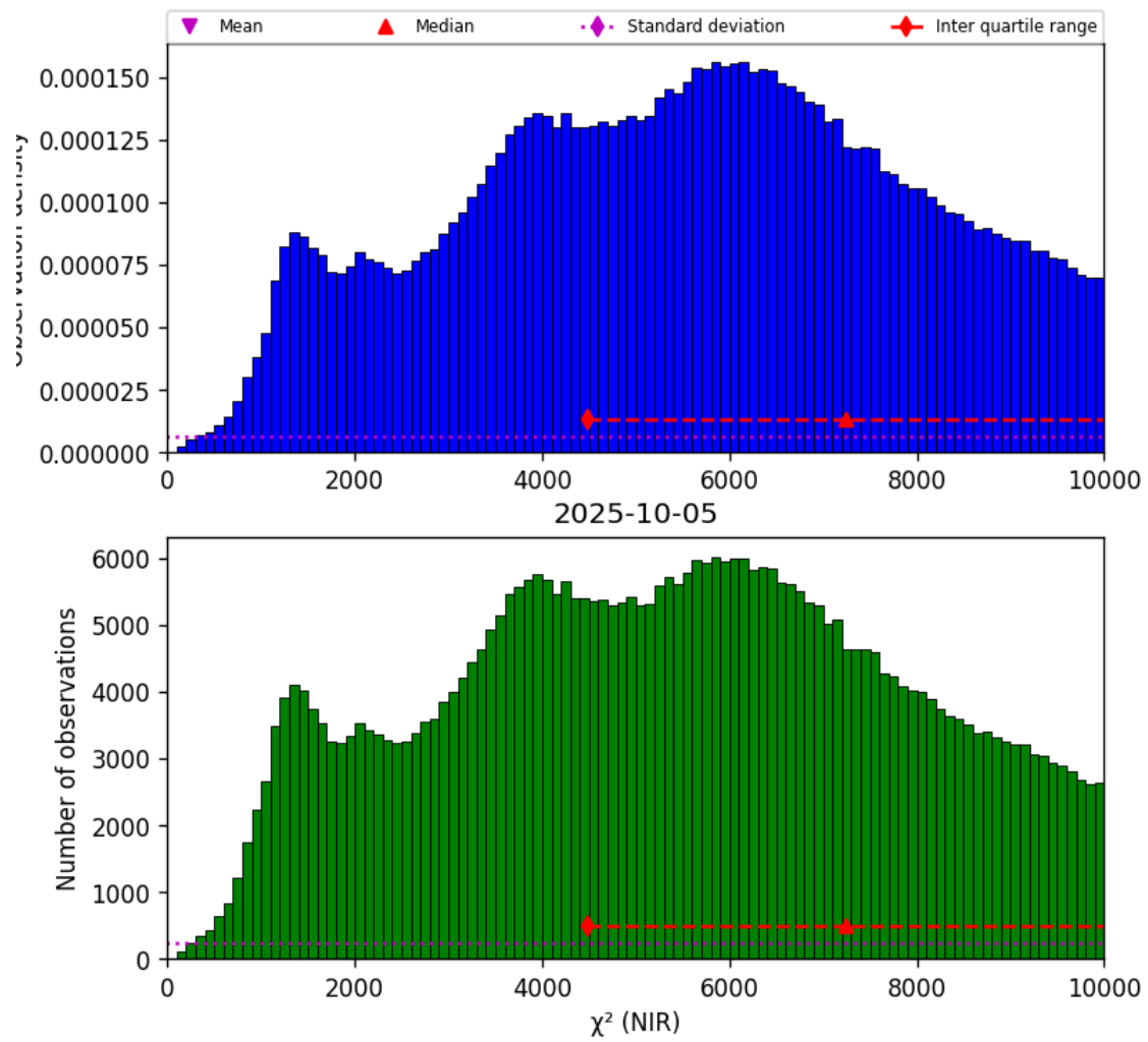
Figure 29: Histogram of “ \chi^2 (NIR)” for 2025-10-04 to 2025-10-06
