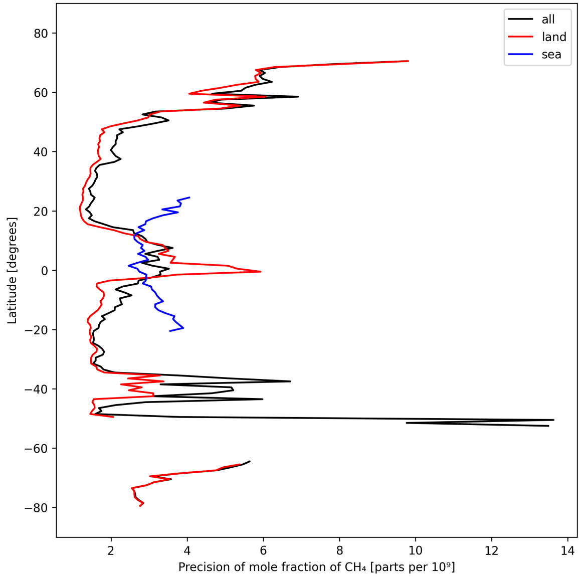
Figure 13: Zonal average of “Precision of mole fraction of CH 4 ” for 2025-10-04 to 2025-10-06.
