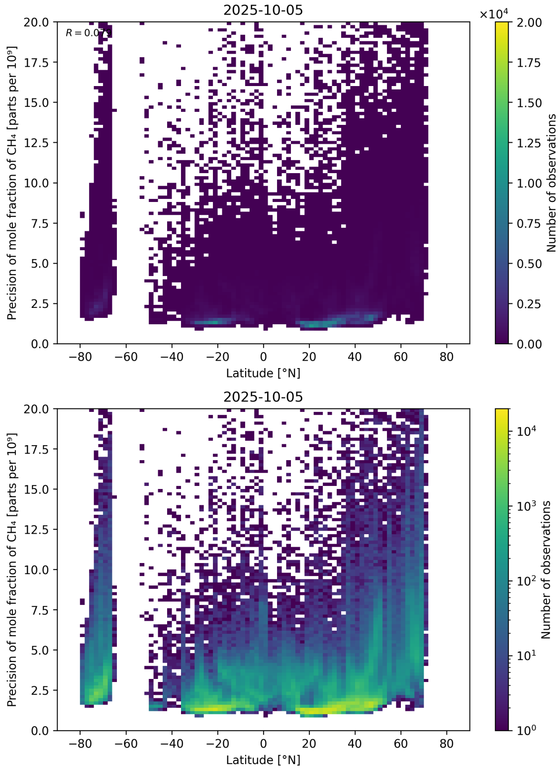
Figure 59: Scatter density plot of “Latitude” against “Precision of mole fraction of CH 4 ” for 2025-10-04 to 2025-10-06.
