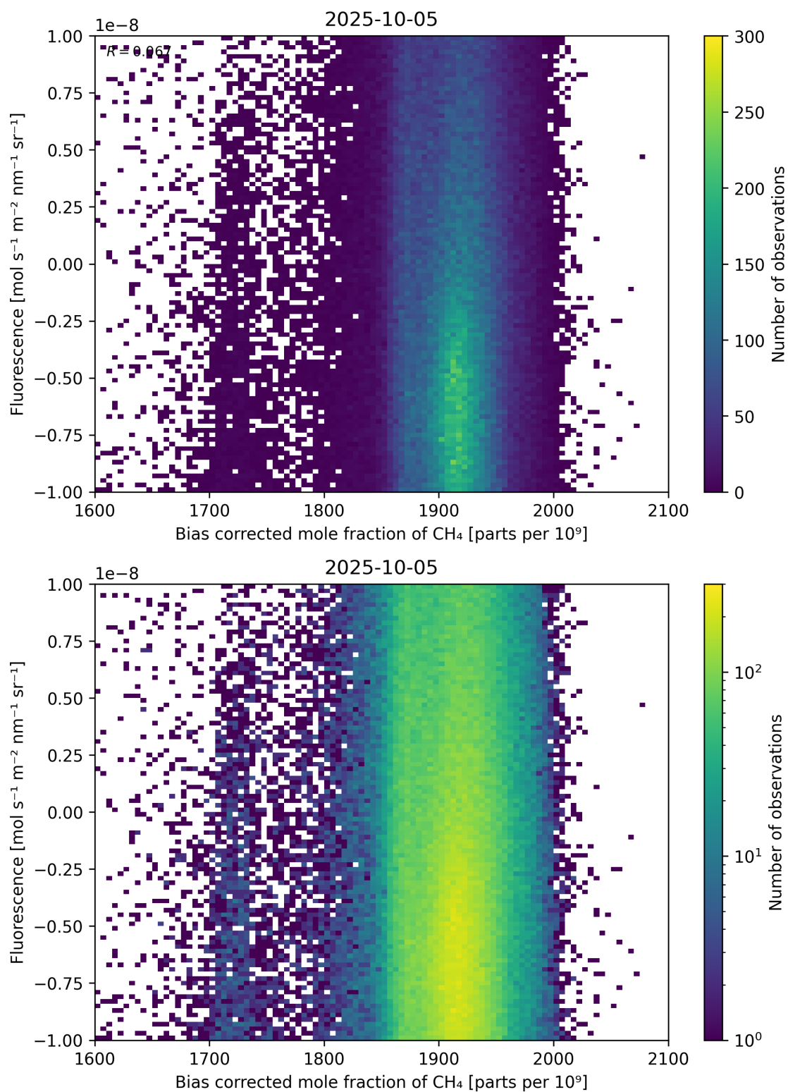
Figure 66: Scatter density plot of “Bias corrected mole fraction of \text{CH}_4 ” against “Fluorescence” for 2025-10-04 to 2025-10-06.
