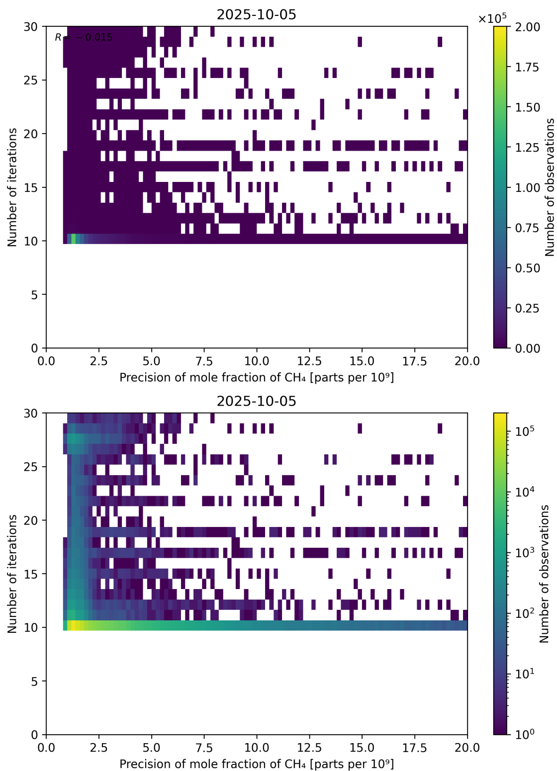
Figure 83: Scatter density plot of “Precision of mole fraction of CH 4 ” against “Number of iterations” for 2025-10-04 to 2025-10-06.
