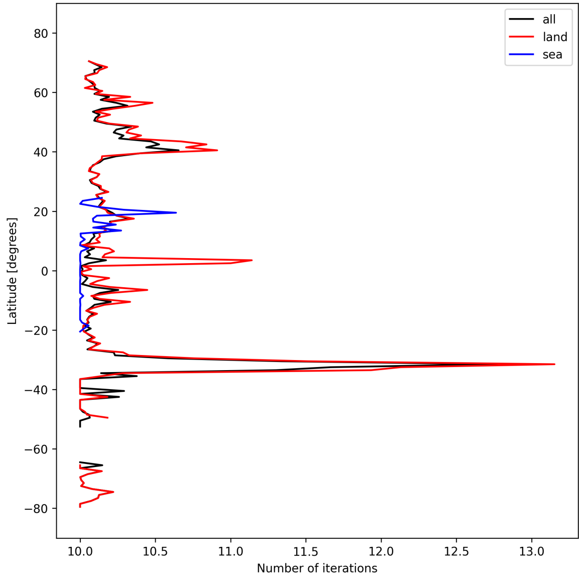
Figure 20: Zonal average of “Number of iterations” for 2025-10-04 to 2025-10-06.
