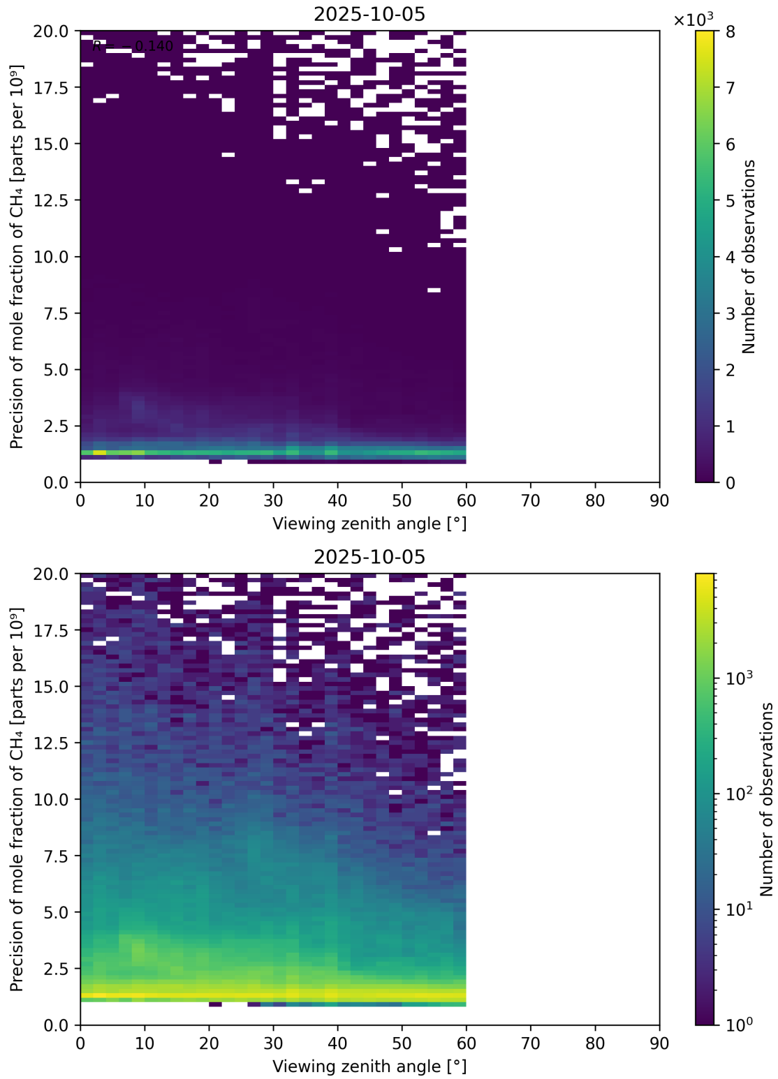
Figure 112: Scatter density plot of “Viewing zenith angle” against “Precision of mole fraction of CH 4 ” for 2025-10-04 to 2025-10-06.
