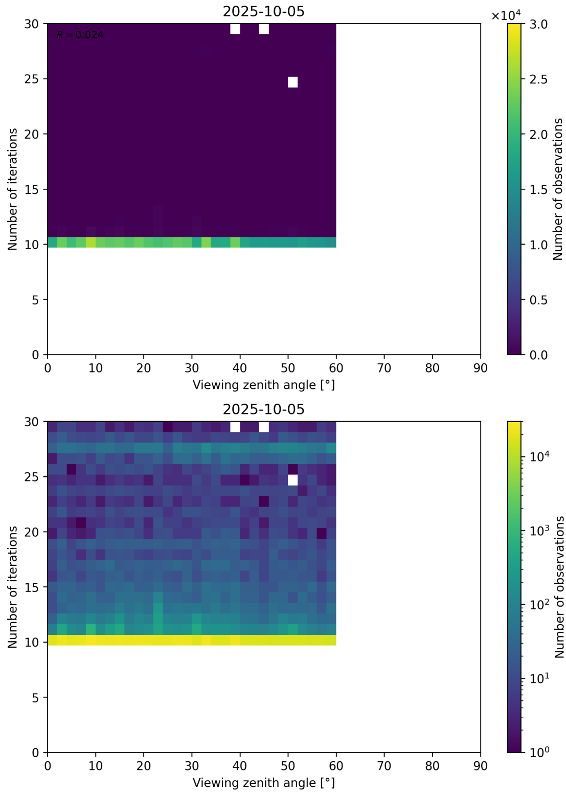
Figure 113: Scatter density plot of “Viewing zenith angle” against “Number of iterations” for 2025-10-04 to 2025-10-06.
