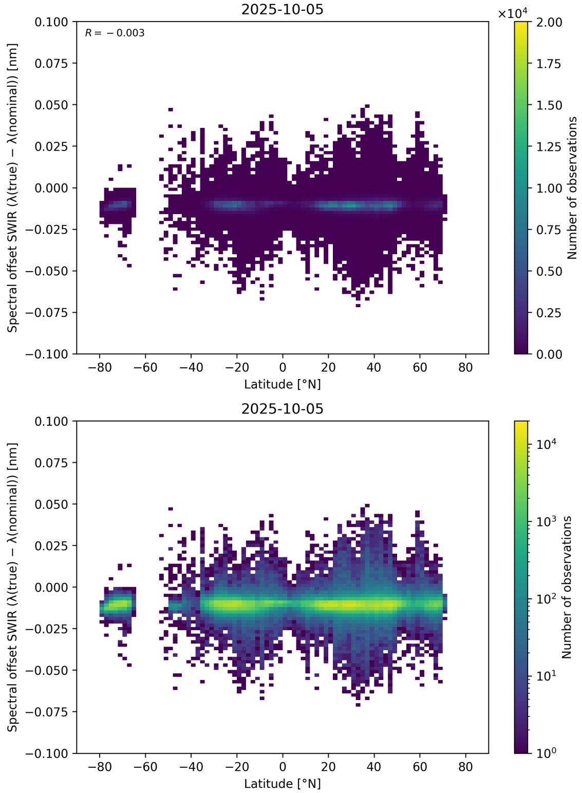
Figure 62: Scatter density plot of “Latitude” against “Spectral offset SWIR ( \lambda_{\text{true}} - \lambda_{\text{nominal}} )” for 2025-10-04 to 2025-10-06.
