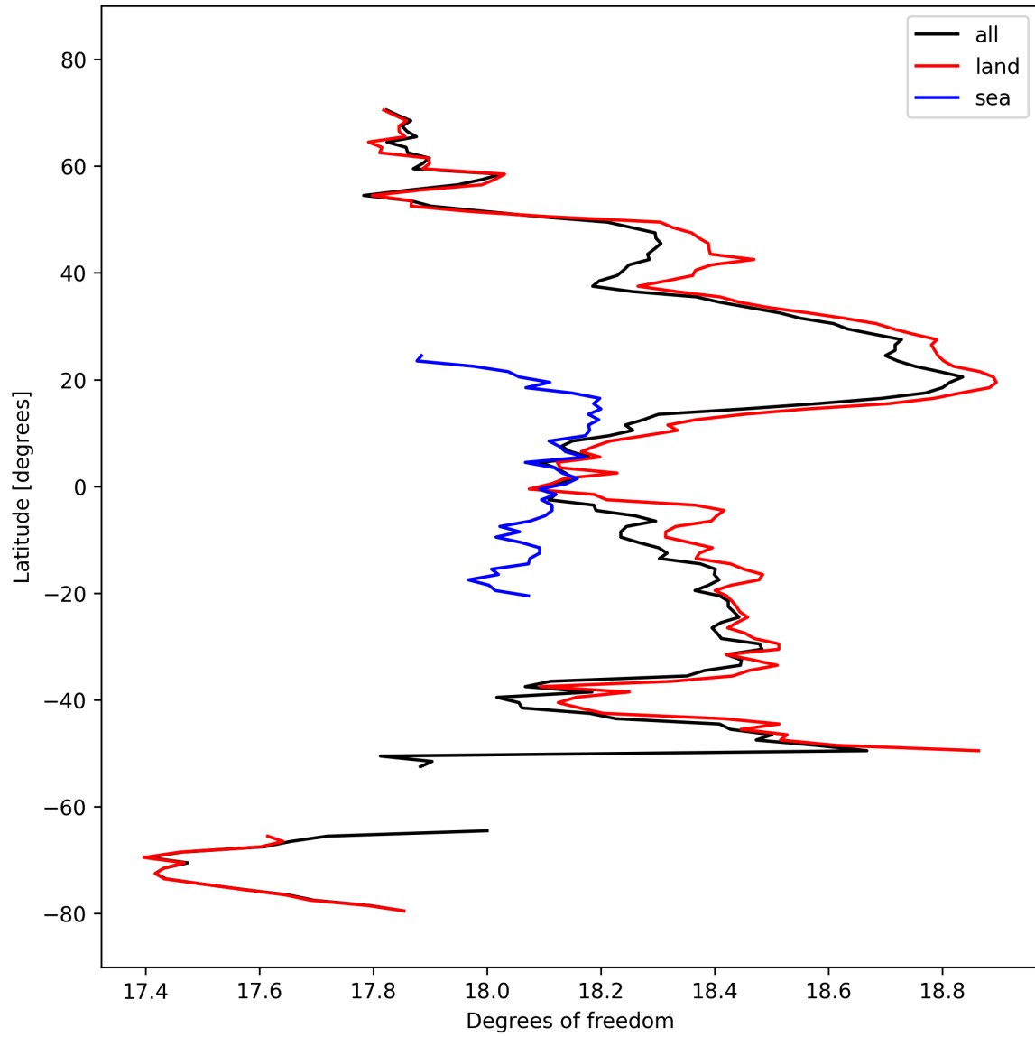
Figure 19: Zonal average of “Degrees of freedom” for 2025-10-04 to 2025-10-06.
