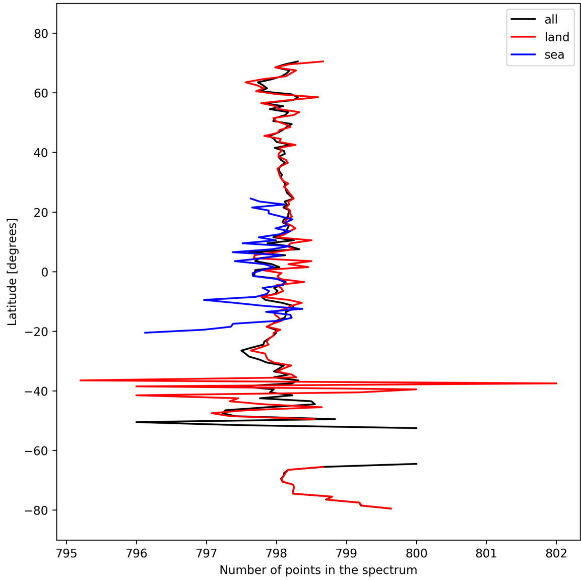
Figure 15: Zonal average of “Number of points in the spectrum” for 2025-10-04 to 2025-10-06.
