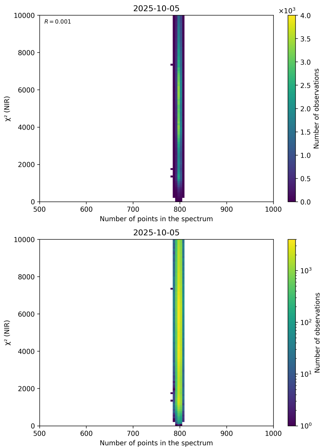
Figure 88: Scatter density plot of “Number of points in the spectrum” against “ \chi^2 (NIR)” for 2025-10-04 to 2025-10-06.
