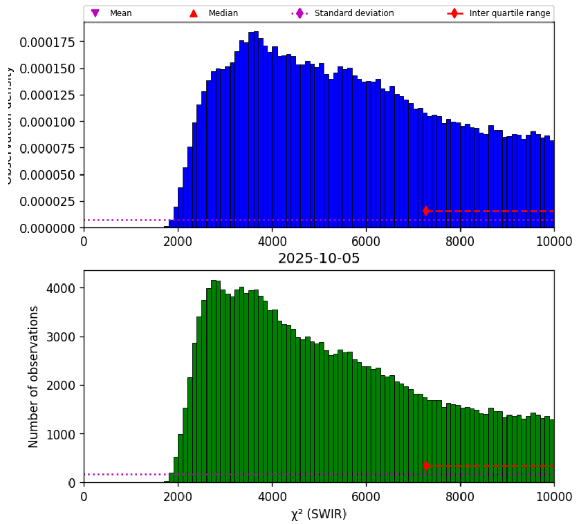
Figure 28: Histogram of “ \chi^2 (SWIR)” for 2025-10-04 to 2025-10-06
