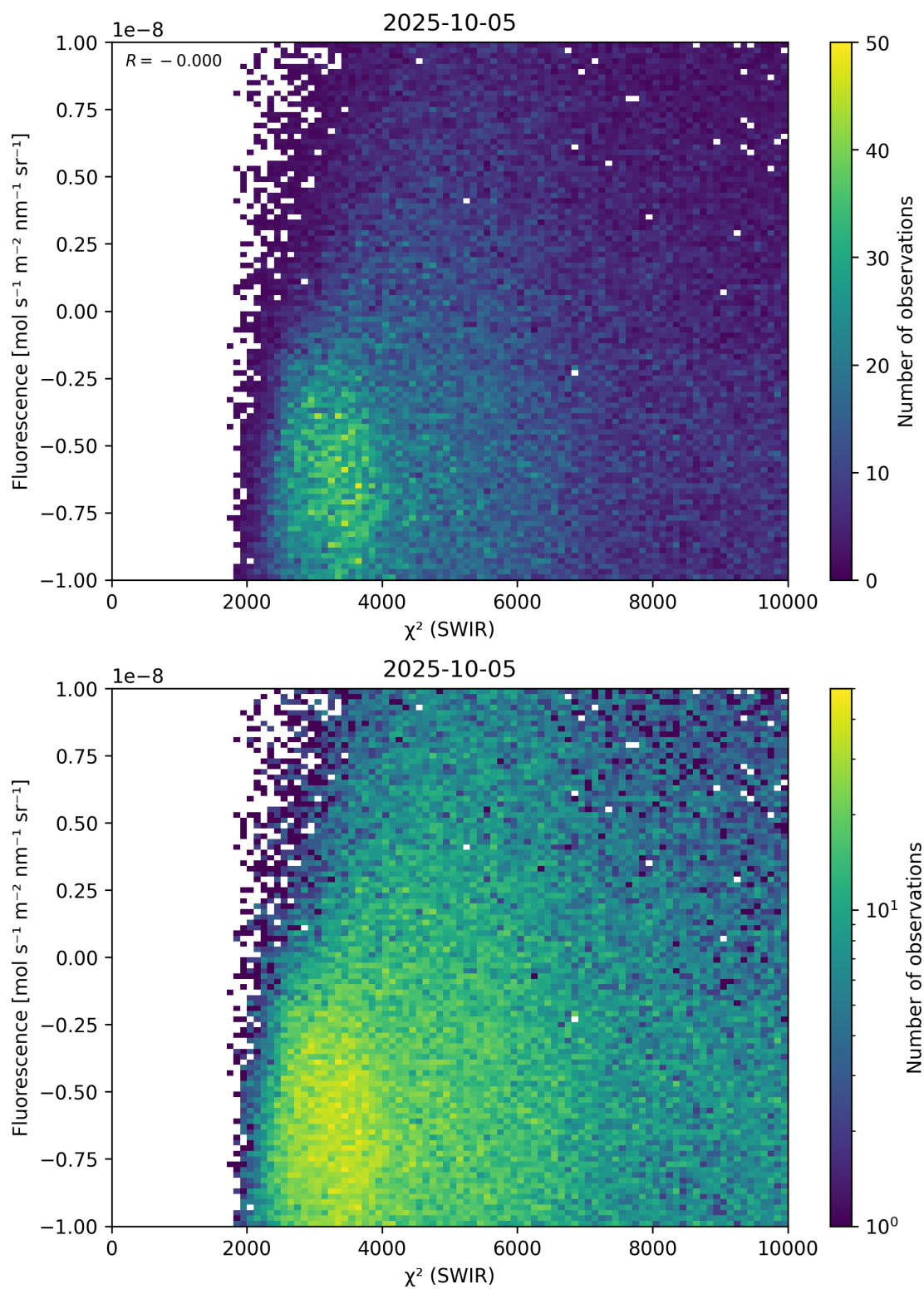
Figure 49: Scatter density plot of “ \chi^2 (SWIR)” against “Fluorescence” for 2025-10-04 to 2025-10-06.
