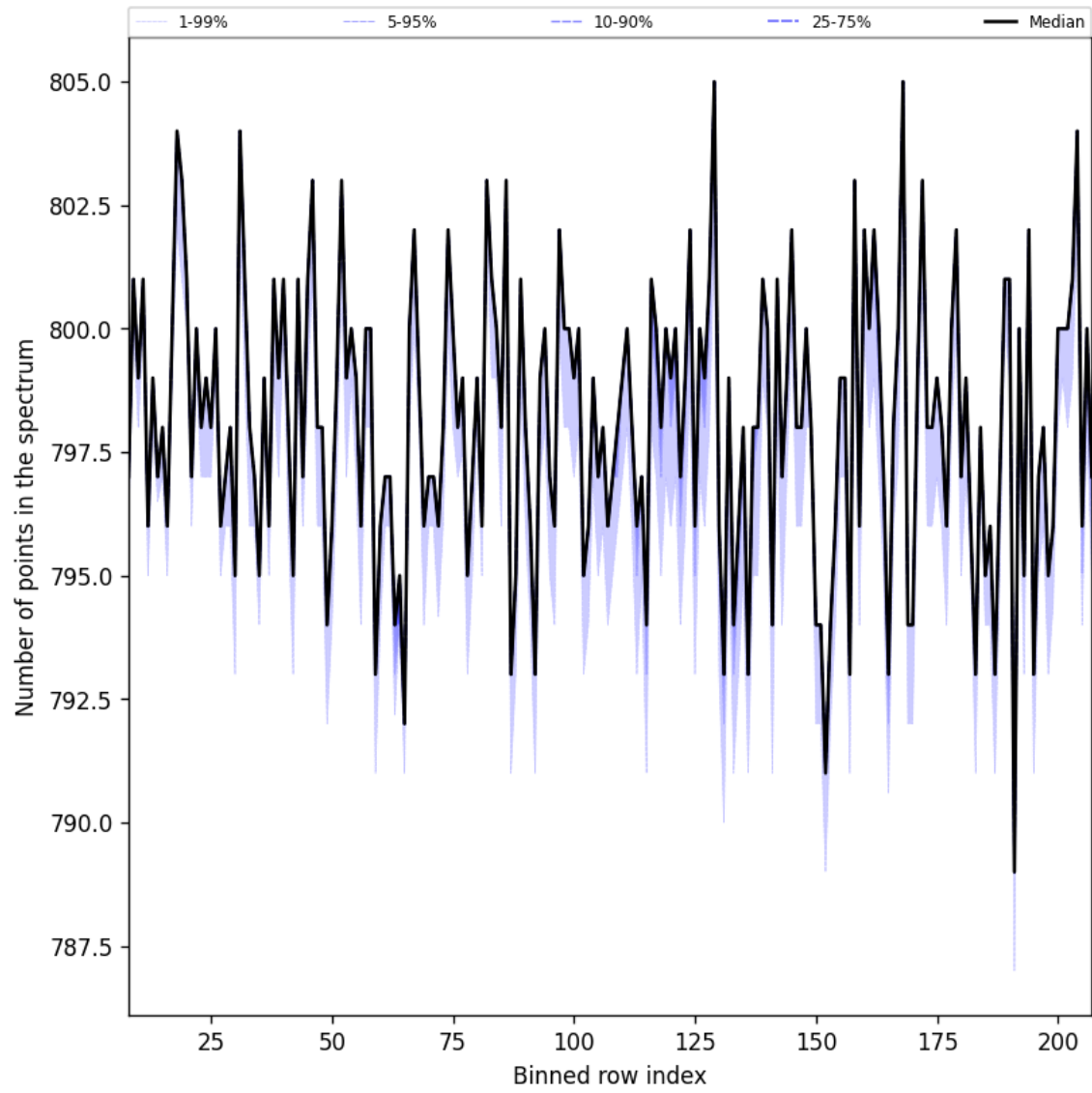
Figure 37: Along track statistics of “Number of points in the spectrum” for 2025-10-04 to 2025-10-06
