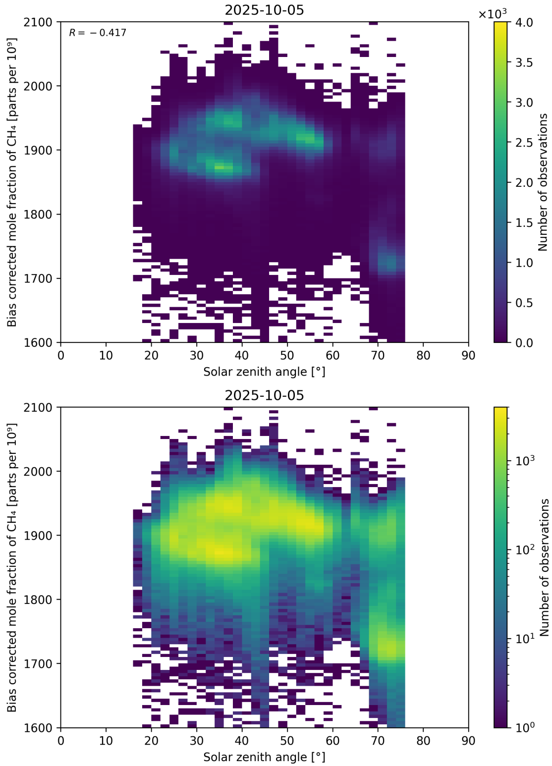
Figure 100: Scatter density plot of “Solar zenith angle” against “Bias corrected mole fraction of CH 4 ” for 2025-10-04 to 2025-10-06.
