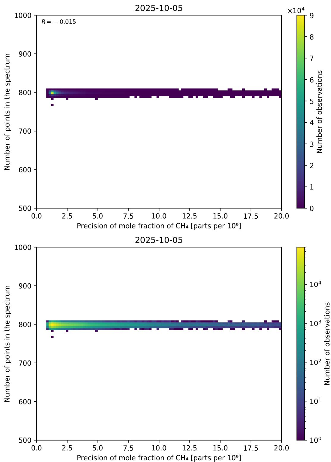
Figure 84: Scatter density plot of “Precision of mole fraction of CH 4 ” against “Number of points in the spectrum” for 2025-10-04 to 2025-10-06.
