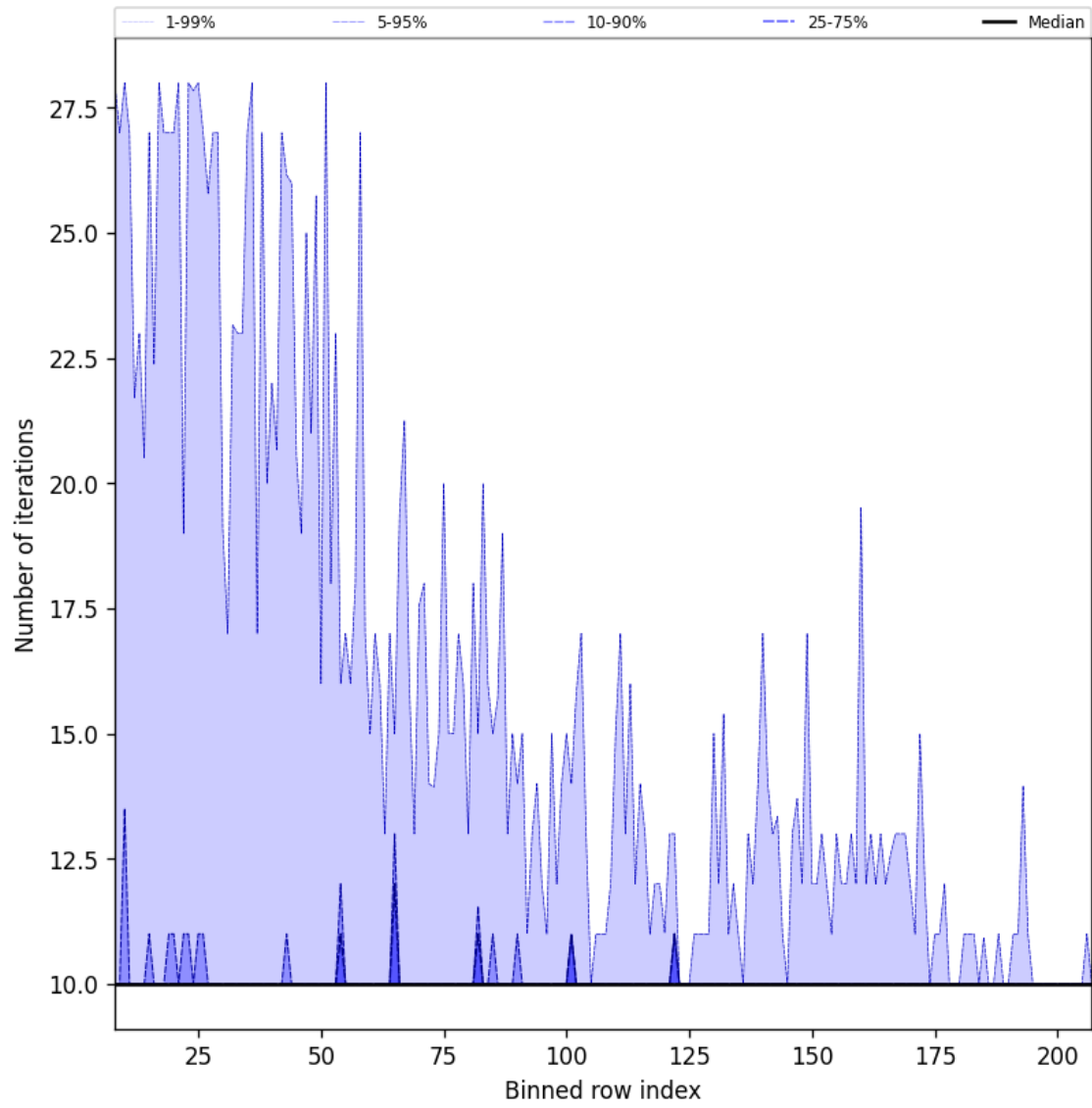
Figure 42: Along track statistics of “Number of iterations” for 2025-10-04 to 2025-10-06
