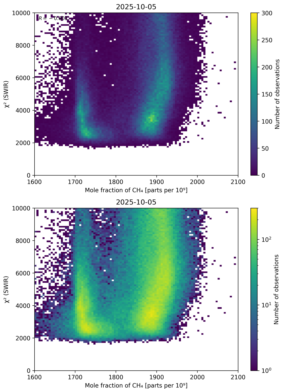
Figure 71: Scatter density plot of “Mole fraction of \text{CH}_4 ” against “ \chi^2 (SWIR)” for 2025-10-04 to 2025-10-06.
