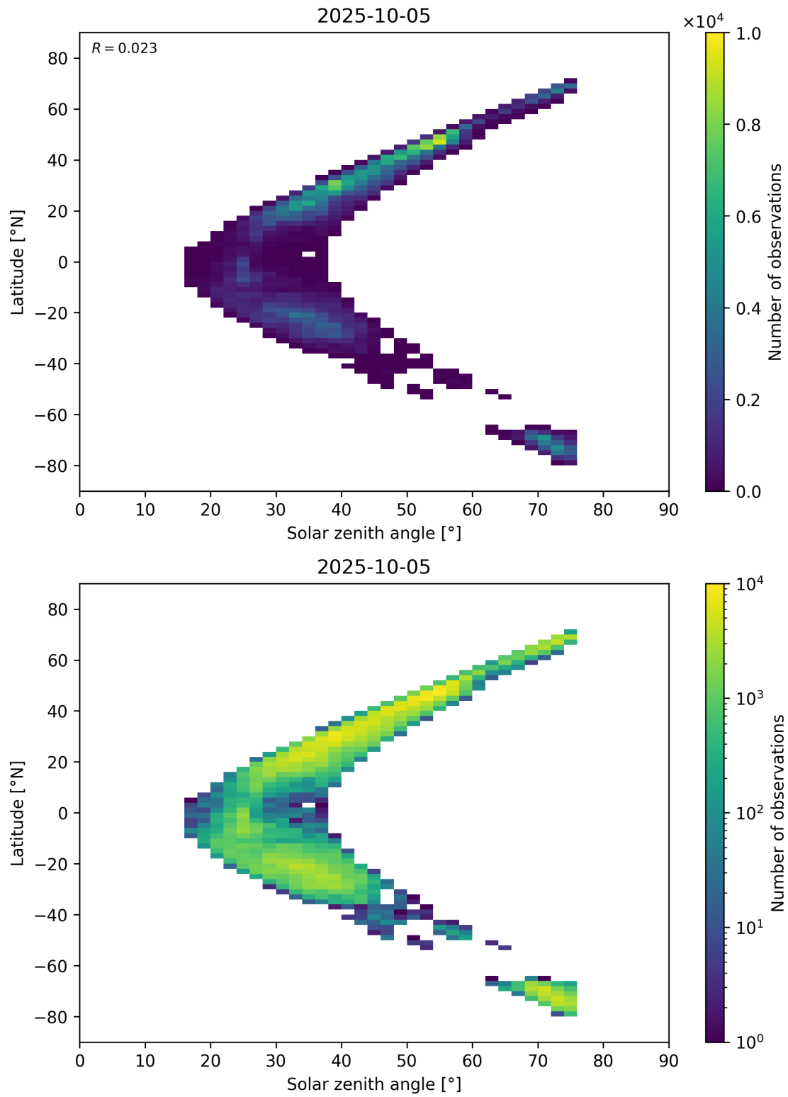
Figure 98: Scatter density plot of “Solar zenith angle” against “Latitude” for 2025-10-04 to 2025-10-06.
