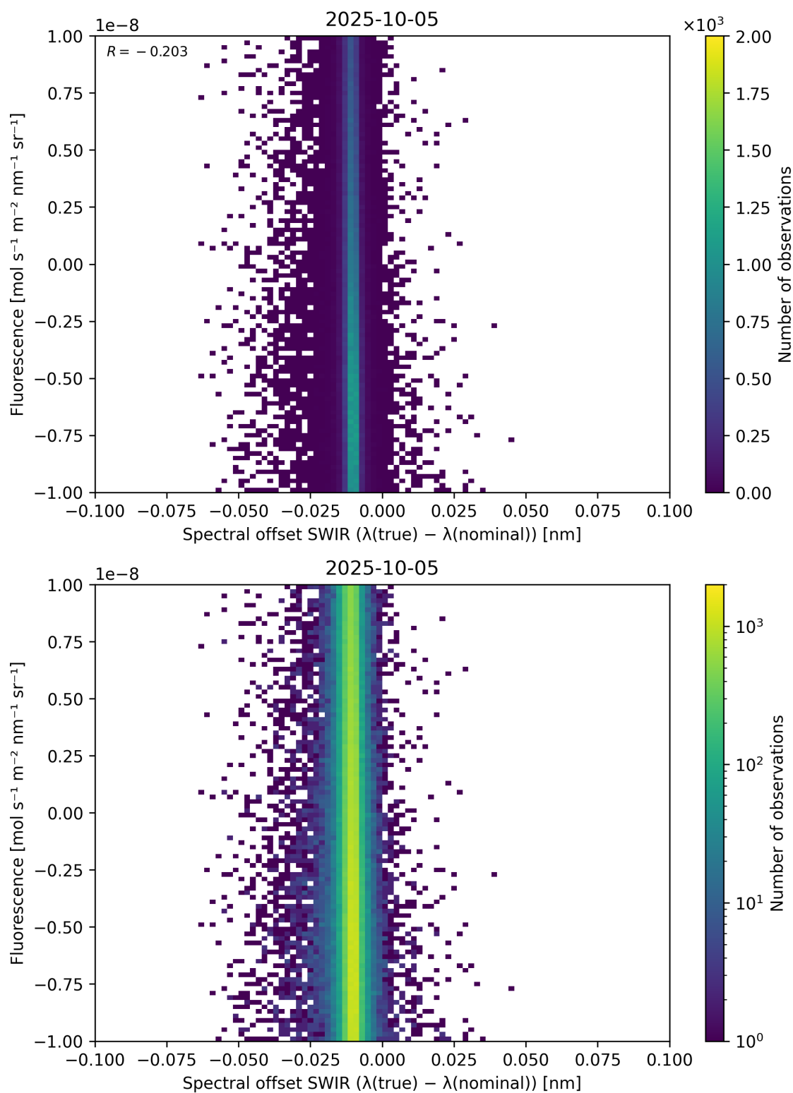
Figure 120: Scatter density plot of “Spectral offset SWIR ( \lambda_{\text{true}} - \lambda_{\text{nominal}} )” against “Fluorescence” for 2025-10-04 to 2025-10-06.
