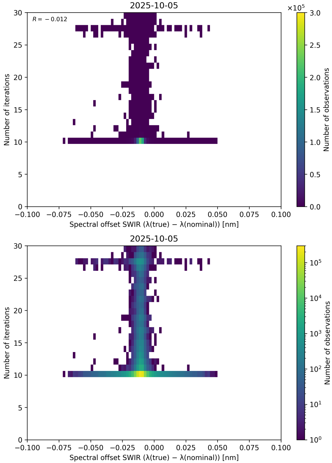
Figure 121: Scatter density plot of “Spectral offset SWIR ( \lambda_{\text{true}} - \lambda_{\text{nominal}} )” against “Number of iterations” for 2025-10-04 to 2025-10-06.
