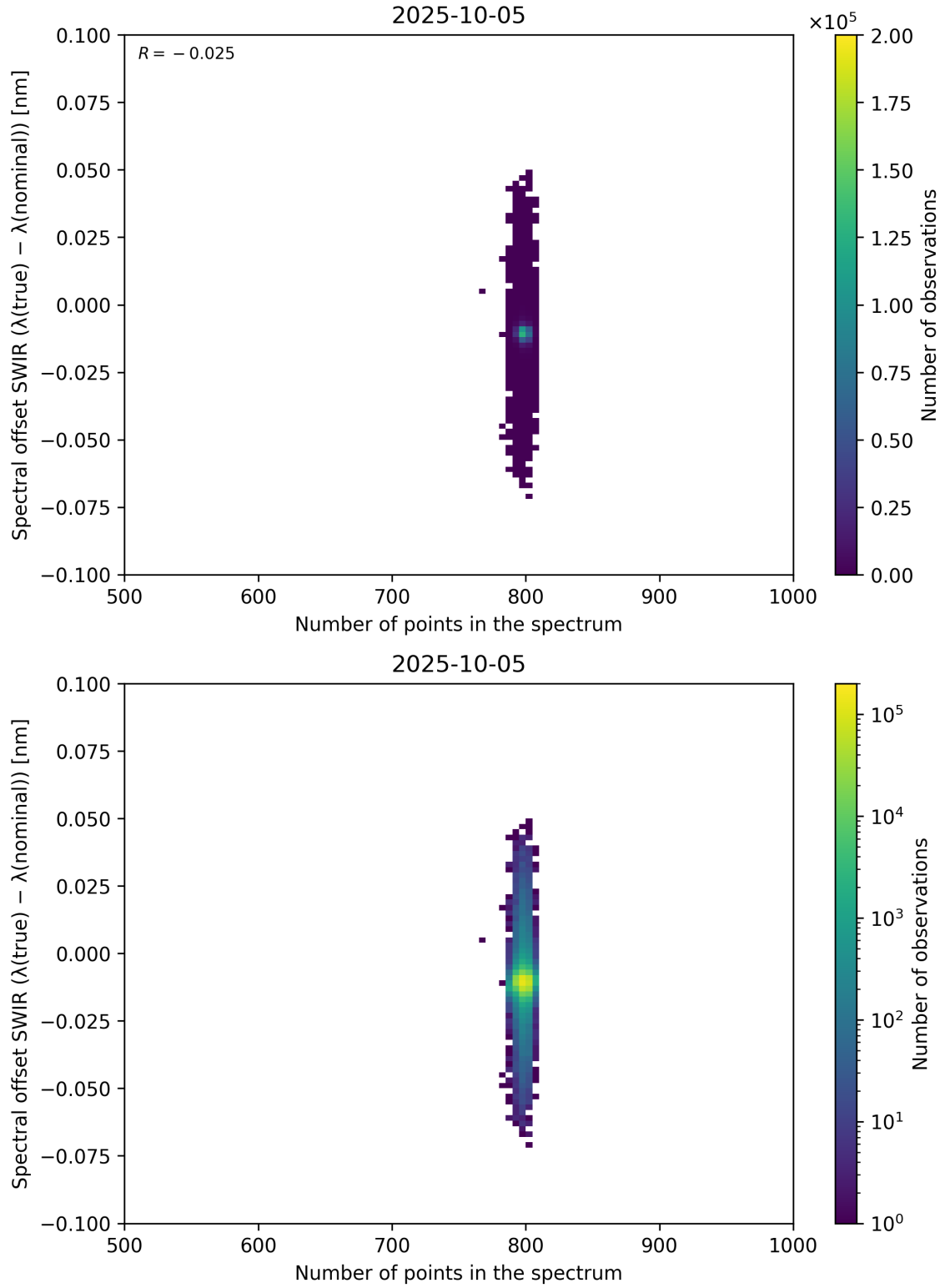
Figure 93: Scatter density plot of “Number of points in the spectrum” against “Spectral offset SWIR ( \lambda_{\text{true}} - \lambda_{\text{nominal}} )” for 2025-10-04 to 2025-10-06.
