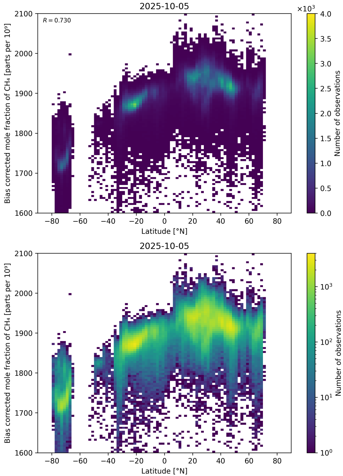
Figure 58: Scatter density plot of “Latitude” against “Bias corrected mole fraction of \text{CH}_4 ” for 2025-10-04 to 2025-10-06.
