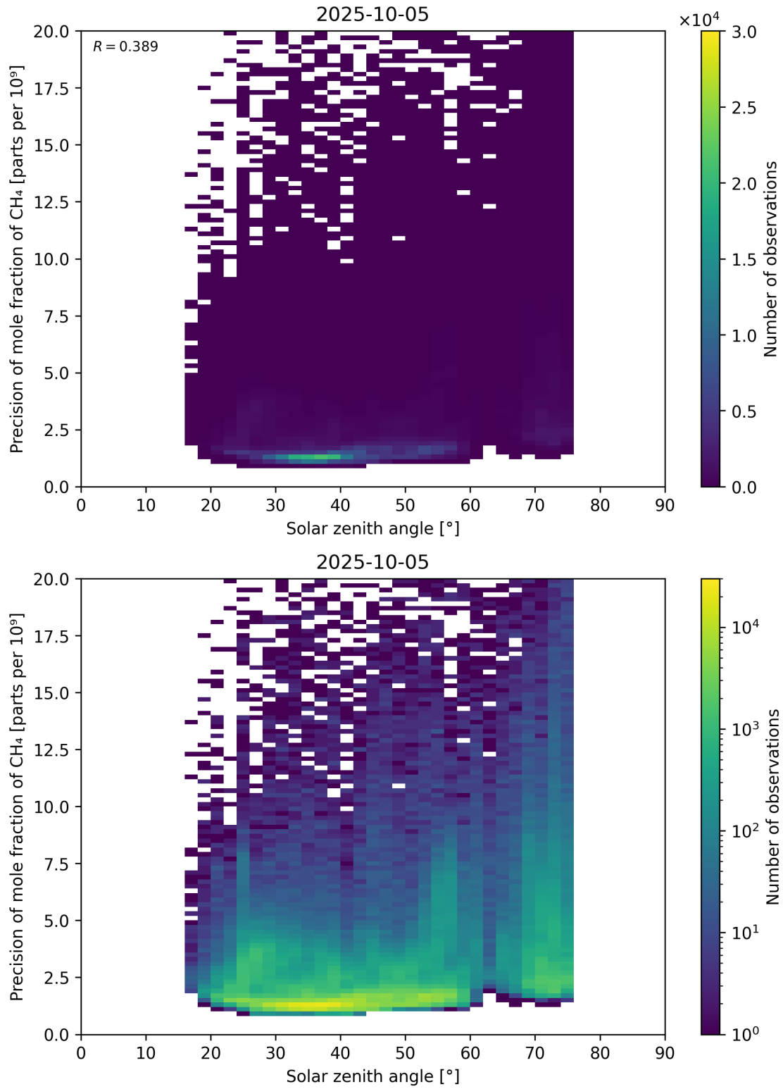
Figure 101: Scatter density plot of “Solar zenith angle” against “Precision of mole fraction of \text{CH}_4 ” for 2025-10-04 to 2025-10-06.
