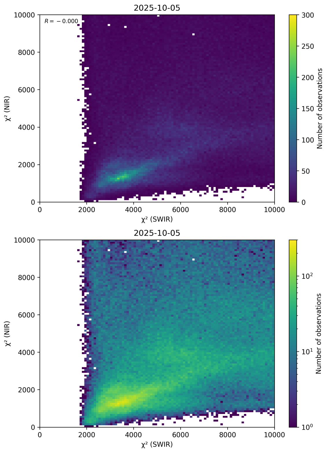
Figure 47: Scatter density plot of “ \chi^2 (SWIR)” against “ \chi^2 (NIR)” for 2025-10-04 to 2025-10-06.
