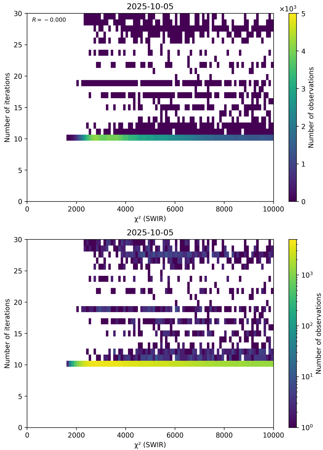
Figure 50: Scatter density plot of “ \chi^2 (SWIR)” against “Number of iterations” for 2025-10-04 to 2025-10-06.
