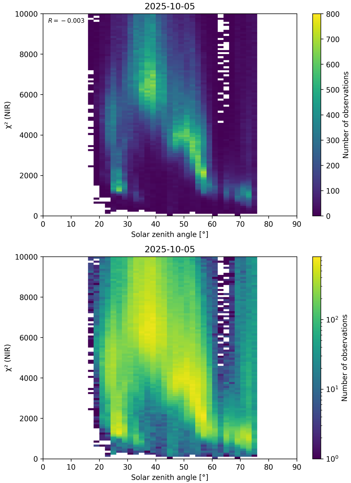
Figure 94: Scatter density plot of “Solar zenith angle” against “ \chi^2 (NIR)” for 2025-10-04 to 2025-10-06.
