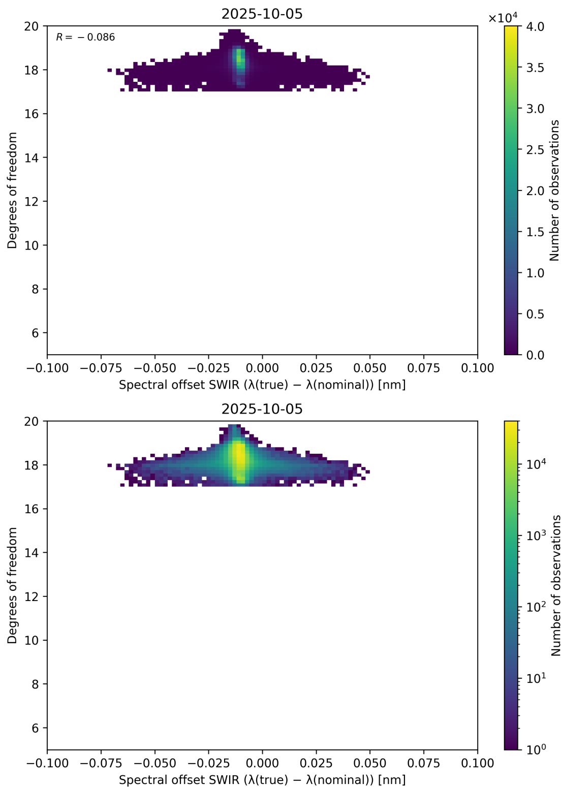
Figure 119: Scatter density plot of “Spectral offset SWIR ( \lambda_{\text{true}} - \lambda_{\text{nominal}} )” against “Degrees of freedom” for 2025-10-04 to 2025-10-06.
