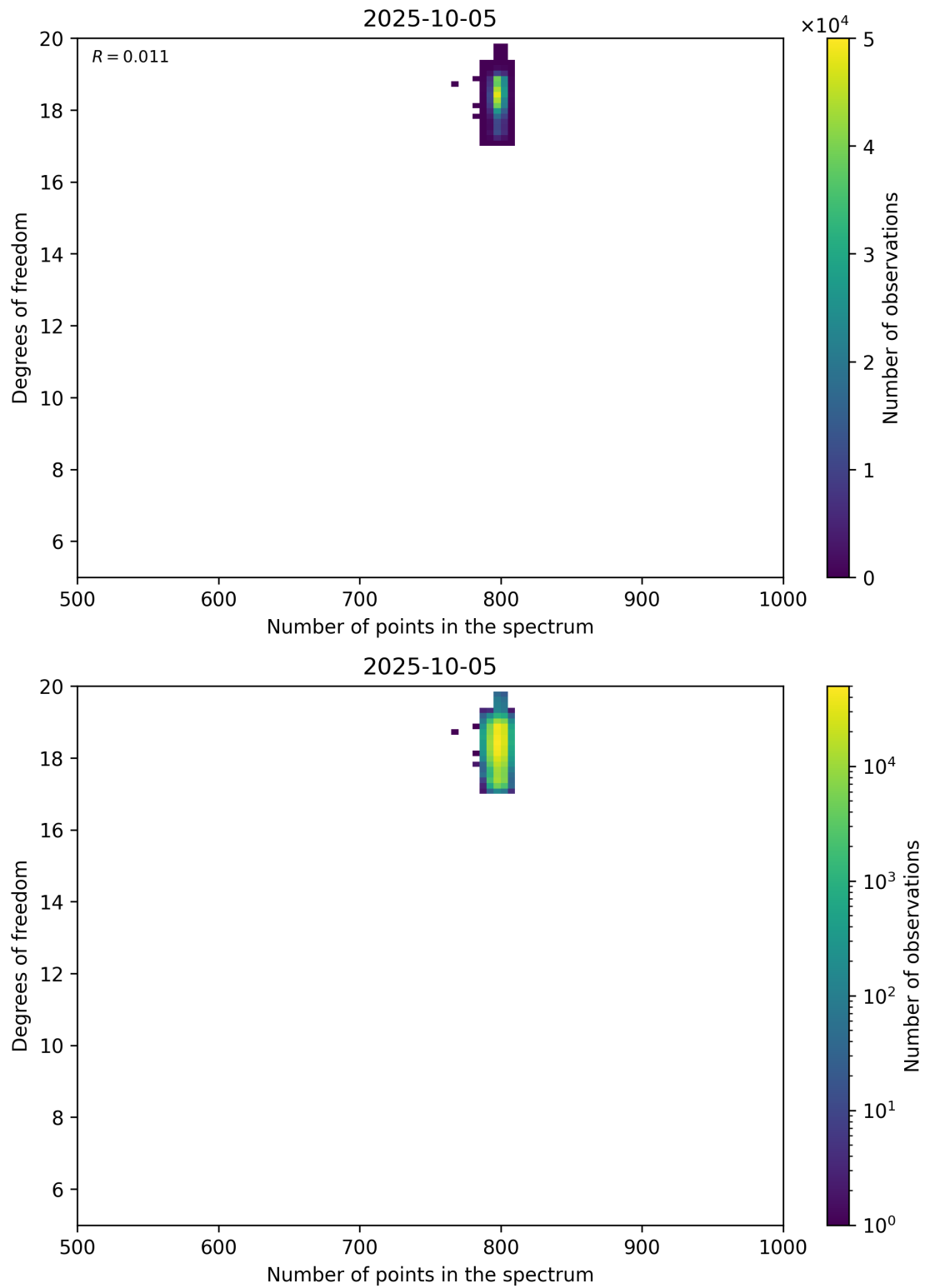
Figure 90: Scatter density plot of “Number of points in the spectrum” against “Degrees of freedom” for 2025-10-04 to 2025-10-06.
