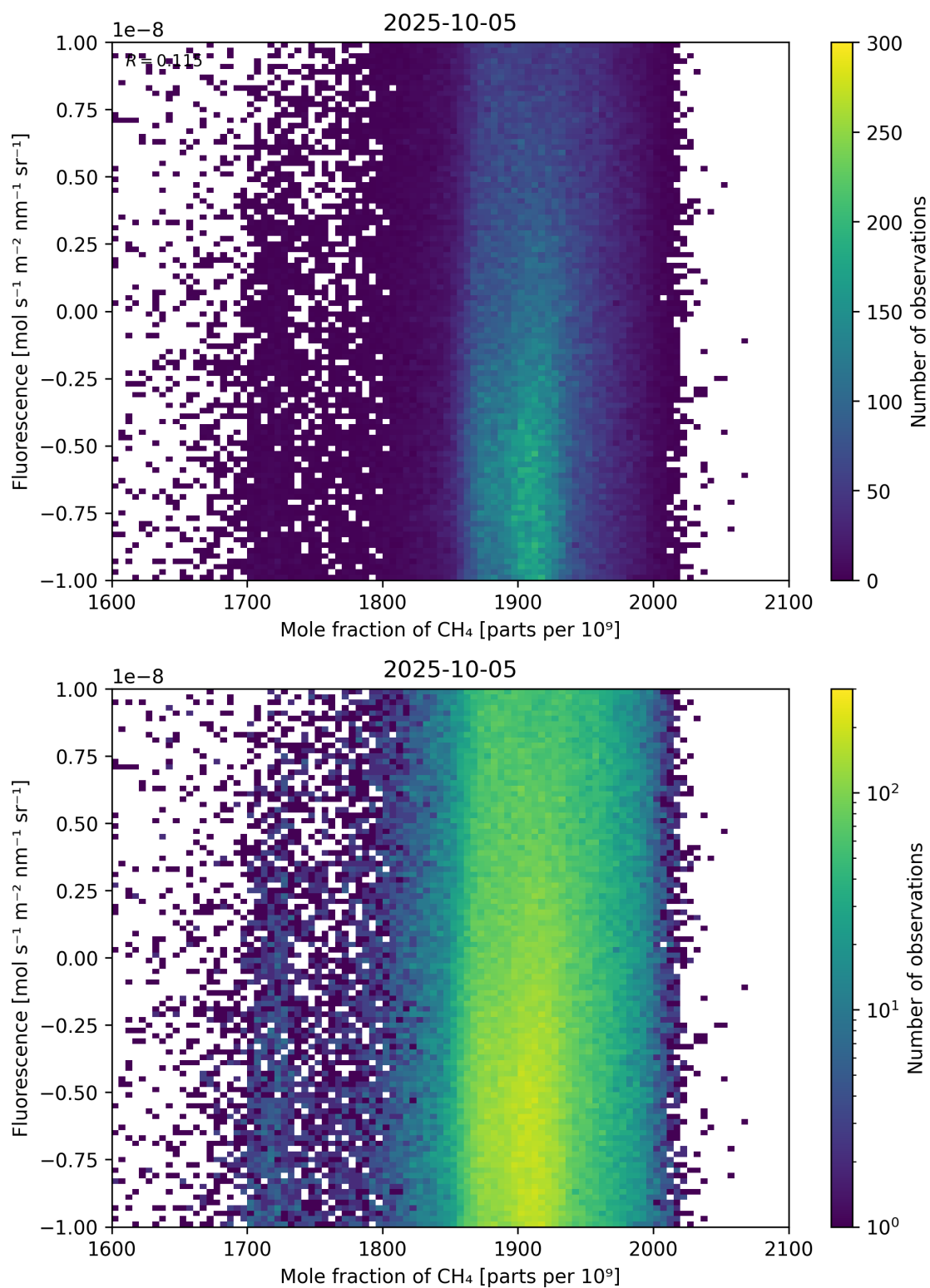
Figure 73: Scatter density plot of “Mole fraction of \text{CH}_4 ” against “Fluorescence” for 2025-10-04 to 2025-10-06.
