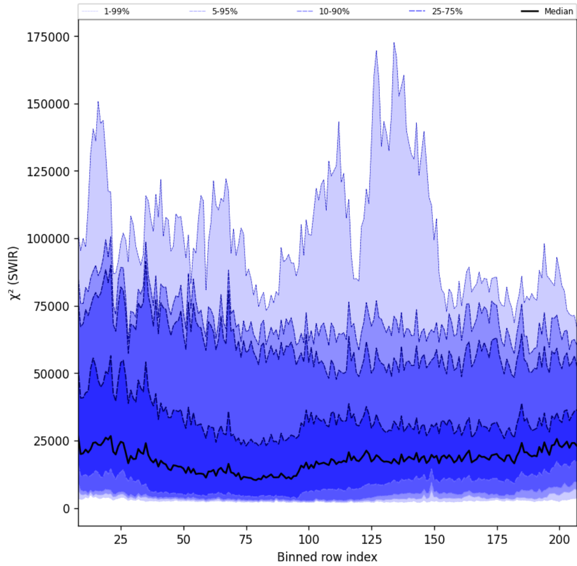
Figure 39: Along track statistics of " \chi^2 (SWIR)" for 2025-10-04 to 2025-10-06
