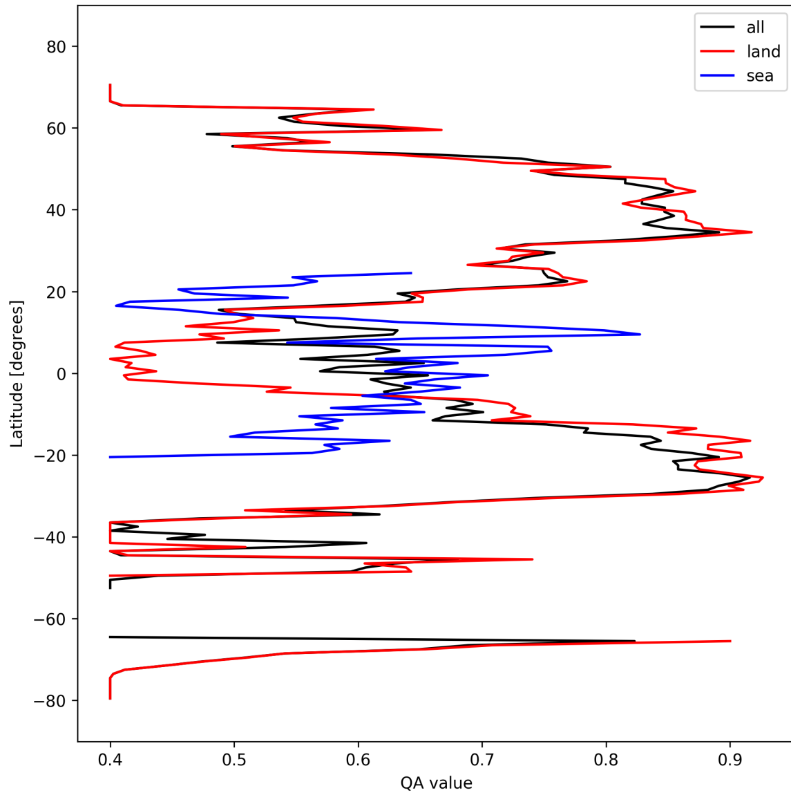
Figure 11: Zonal average of “QA value” for 2025-10-04 to 2025-10-06.
