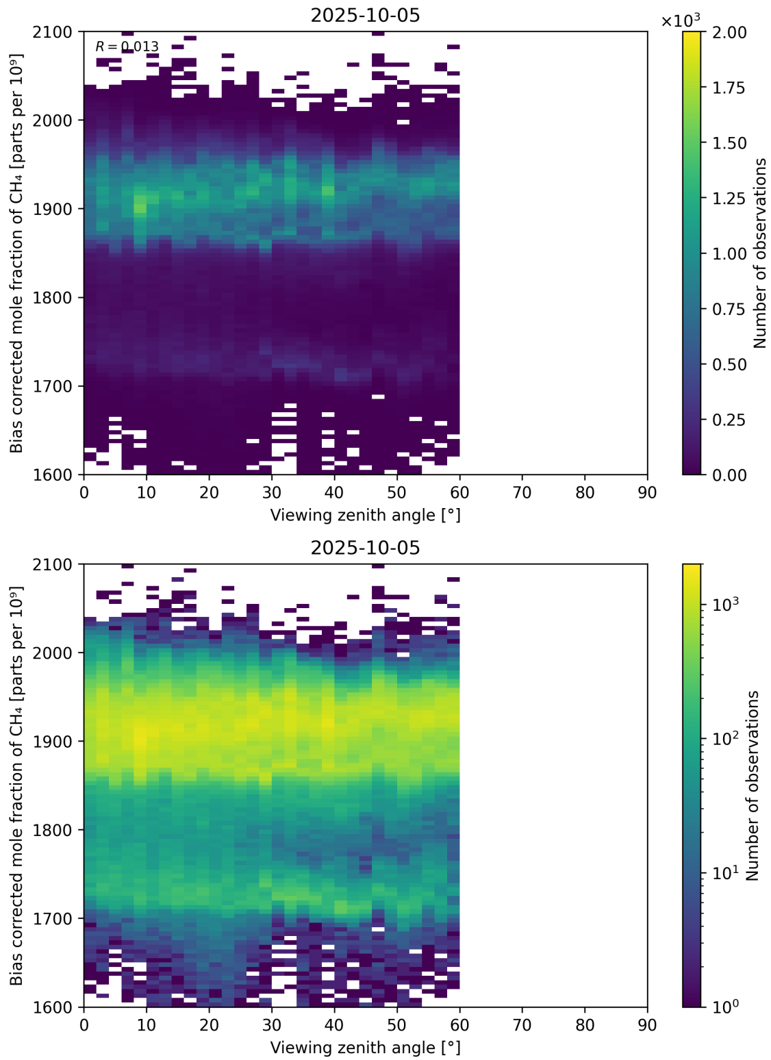
Figure 111: Scatter density plot of “Viewing zenith angle” against “Bias corrected mole fraction of CH 4 ” for 2025-10-04 to 2025-10-06.
