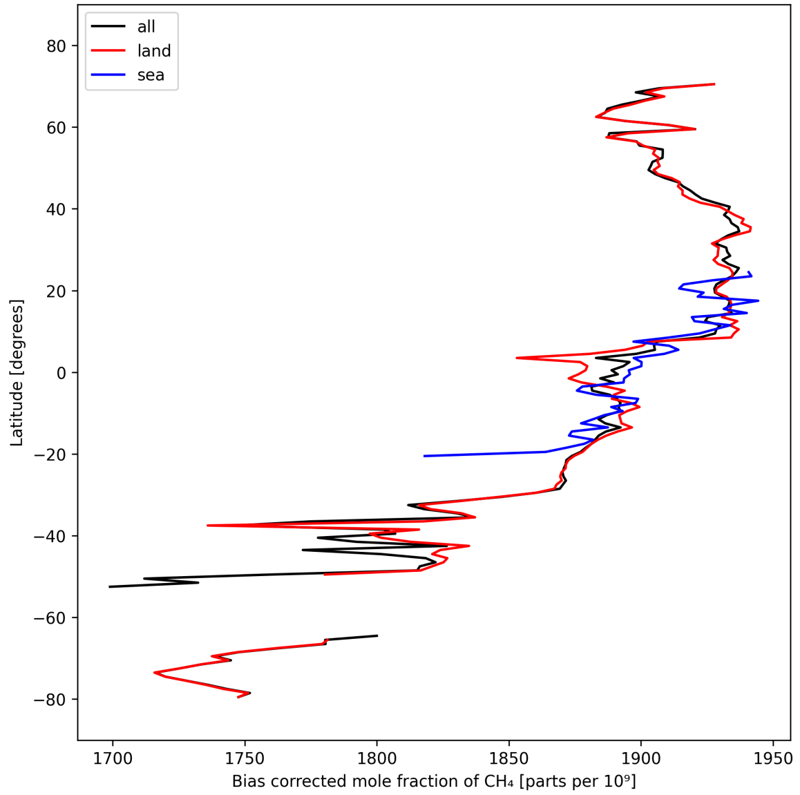
Figure 14: Zonal average of “Bias corrected mole fraction of CH 4 ” for 2025-10-04 to 2025-10-06.
