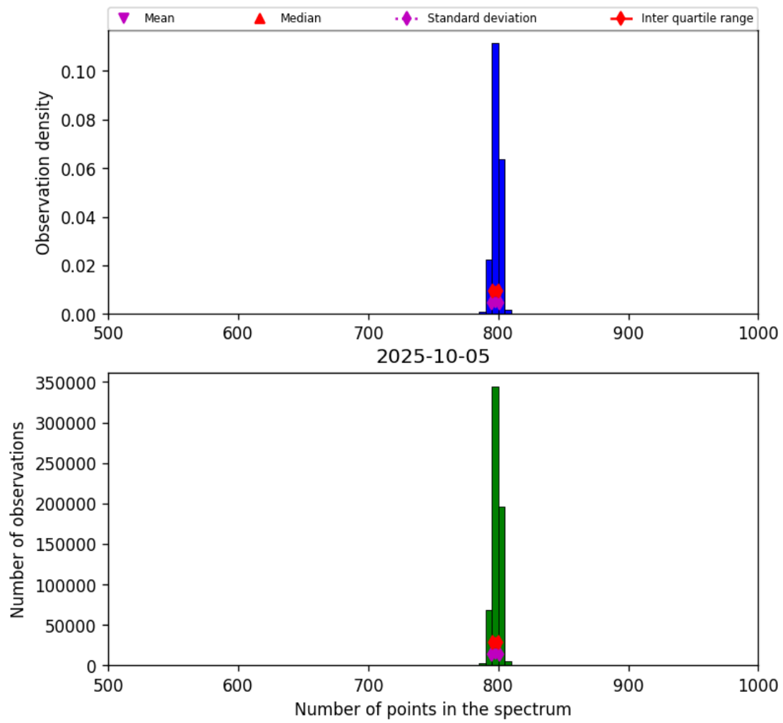
Figure 26: Histogram of “Number of points in the spectrum” for 2025-10-04 to 2025-10-06
