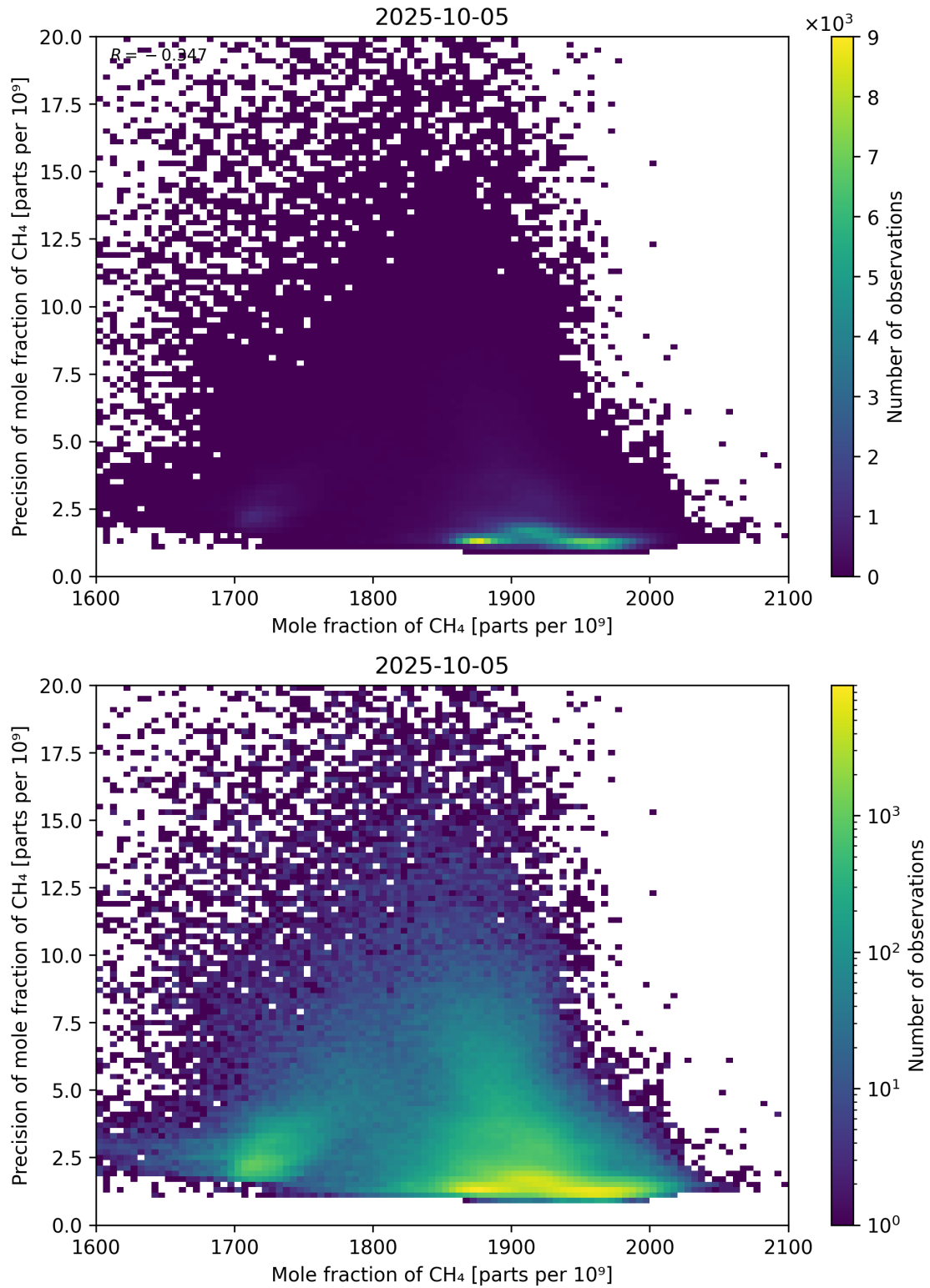
Figure 75: Scatter density plot of “Mole fraction of CH 4 ” against “Precision of mole fraction of CH 4 ” for 2025-10-04 to 2025-10-06.
