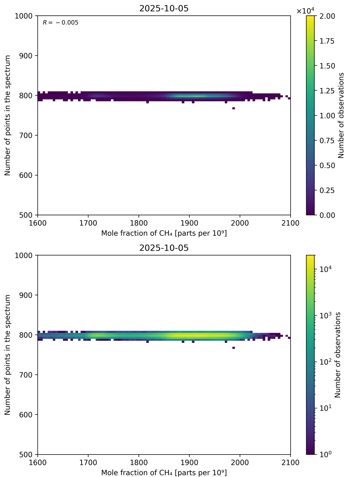
Figure 77: Scatter density plot of “Mole fraction of CH 4 ” against “Number of points in the spectrum” for 2025-10-04 to 2025-10-06.
