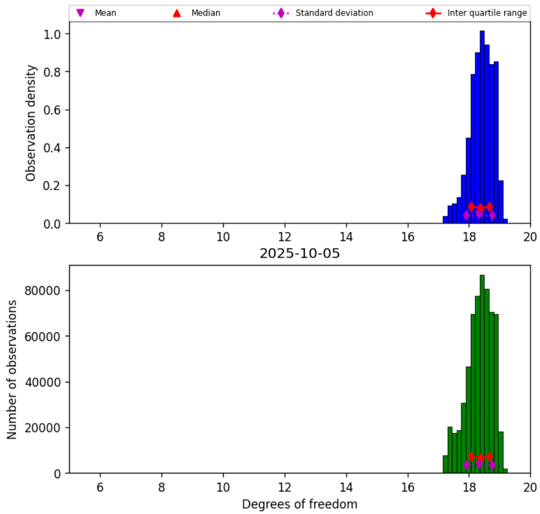
Figure 30: Histogram of “Degrees of freedom” for 2025-10-04 to 2025-10-06
