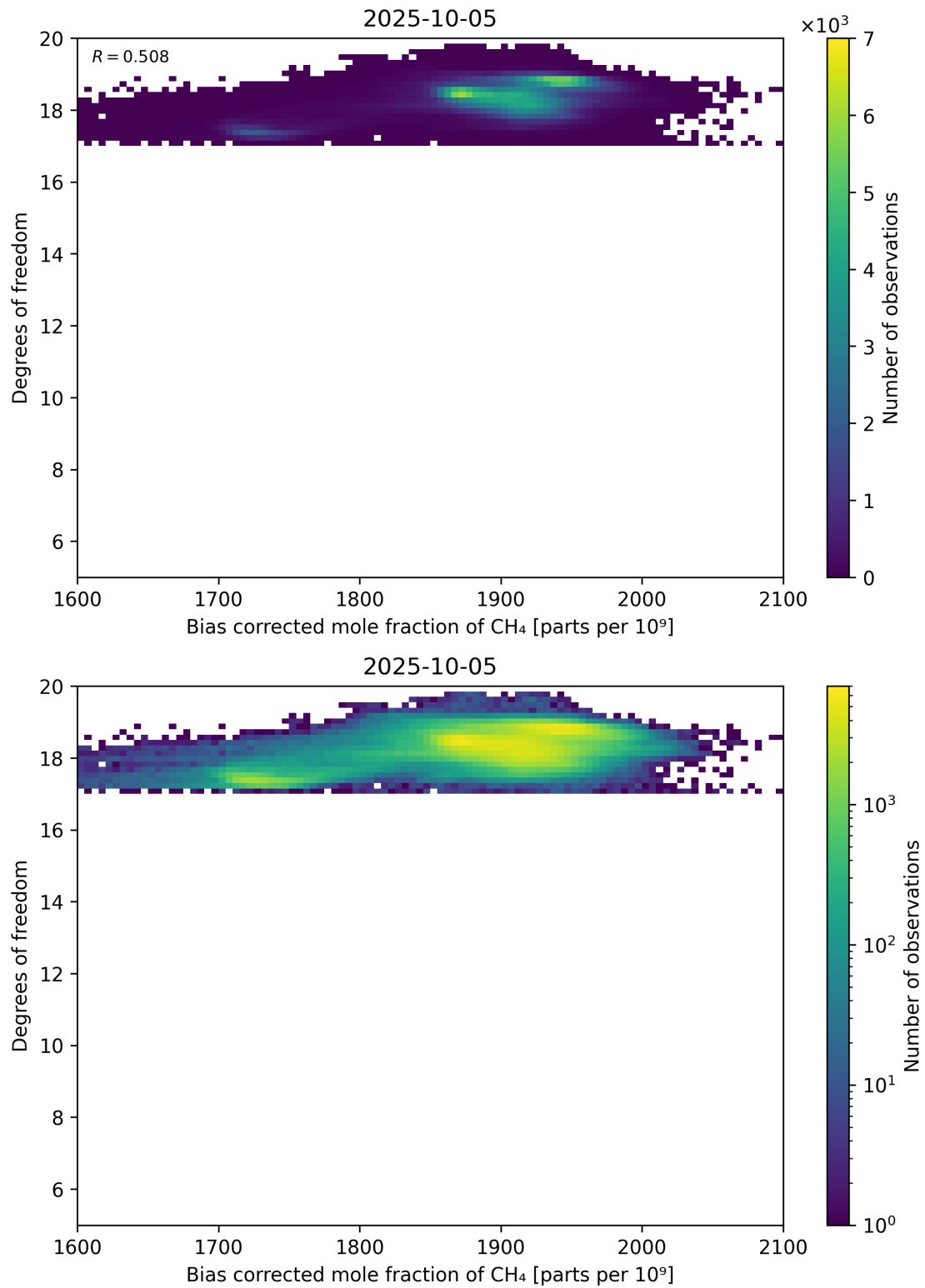
Figure 65: Scatter density plot of “Bias corrected mole fraction of CH 4 ” against “Degrees of freedom” for 2025-10-04 to 2025-10-06.
