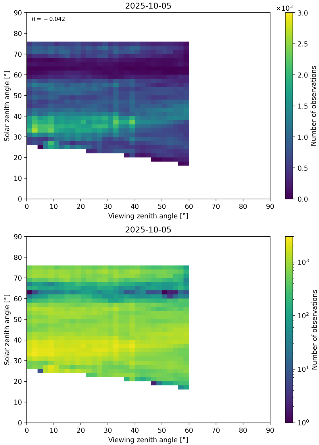
Figure 115: Scatter density plot of “Viewing zenith angle” against “Solar zenith angle” for 2025-10-04 to 2025-10-06.
