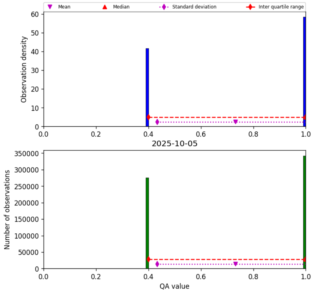
Figure 22: Histogram of “QA value” for 2025-10-04 to 2025-10-06
