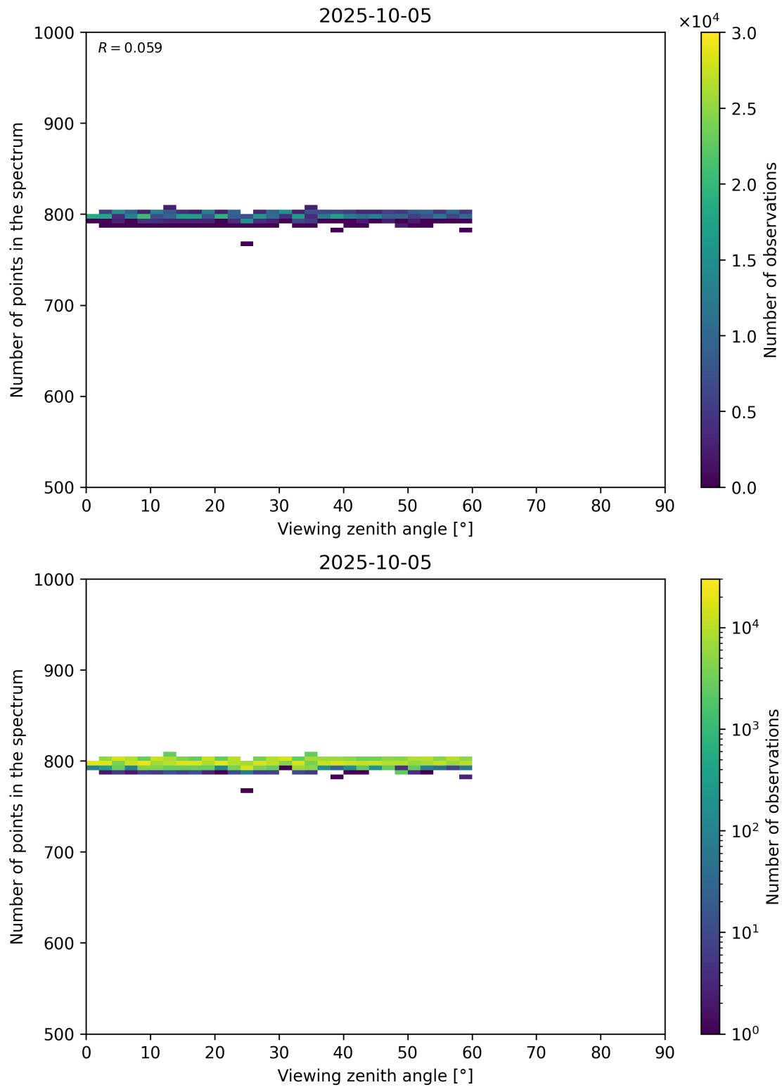
Figure 114: Scatter density plot of “Viewing zenith angle” against “Number of points in the spectrum” for 2025-10-04 to 2025-10-06.
