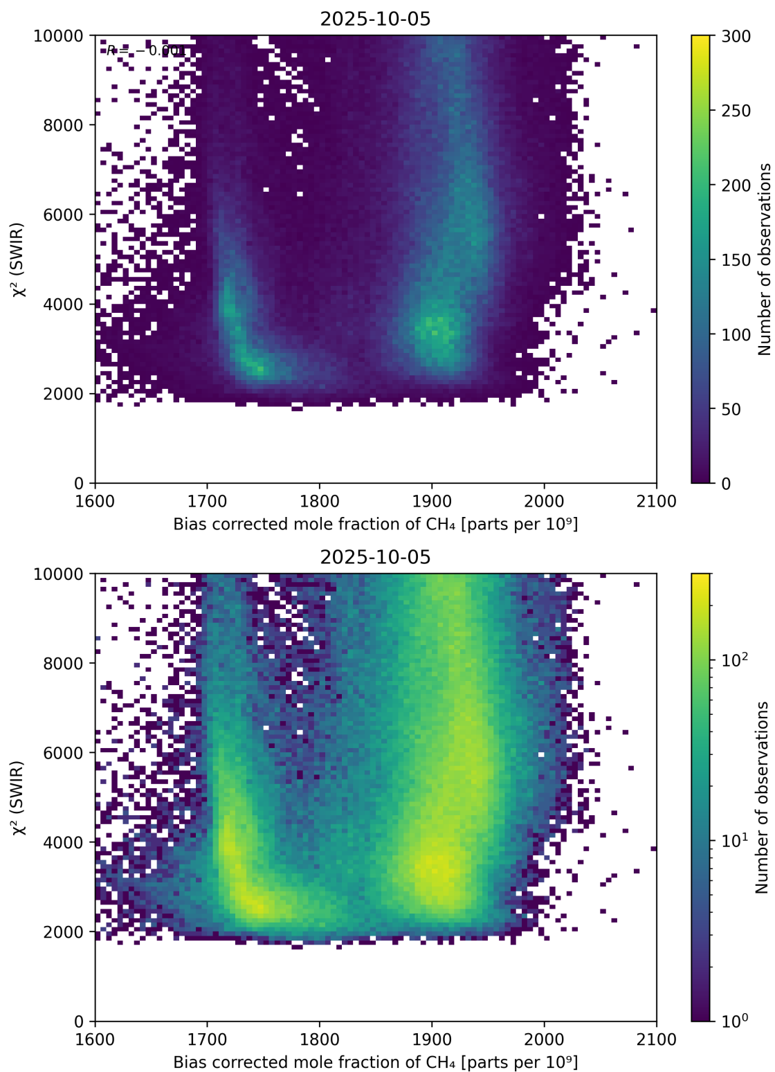
Figure 64: Scatter density plot of “Bias corrected mole fraction of \text{CH}_4 ” against “ \chi^2 (SWIR)” for 2025-10-04 to 2025-10-06.
