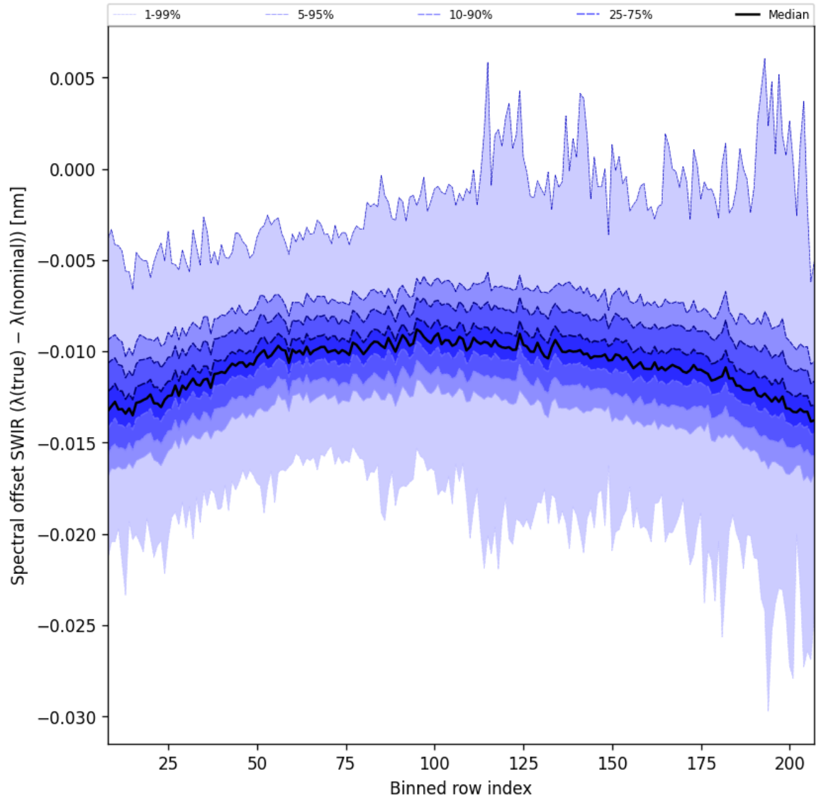
Figure 38: Along track statistics of “Spectral offset SWIR ( \lambda_{\text{true}} - \lambda_{\text{nominal}} )” for 2025-10-04 to 2025-10-06
