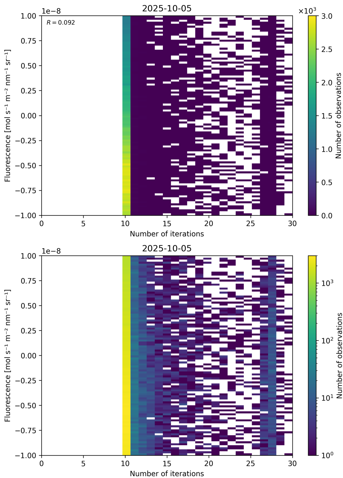
Figure 87: Scatter density plot of “Number of iterations” against “Fluorescence” for 2025-10-04 to 2025-10-06.
