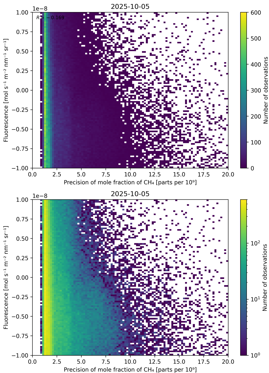
Figure 81: Scatter density plot of “Precision of mole fraction of CH 4 ” against “Fluorescence” for 2025-10-04 to 2025-10-06.
