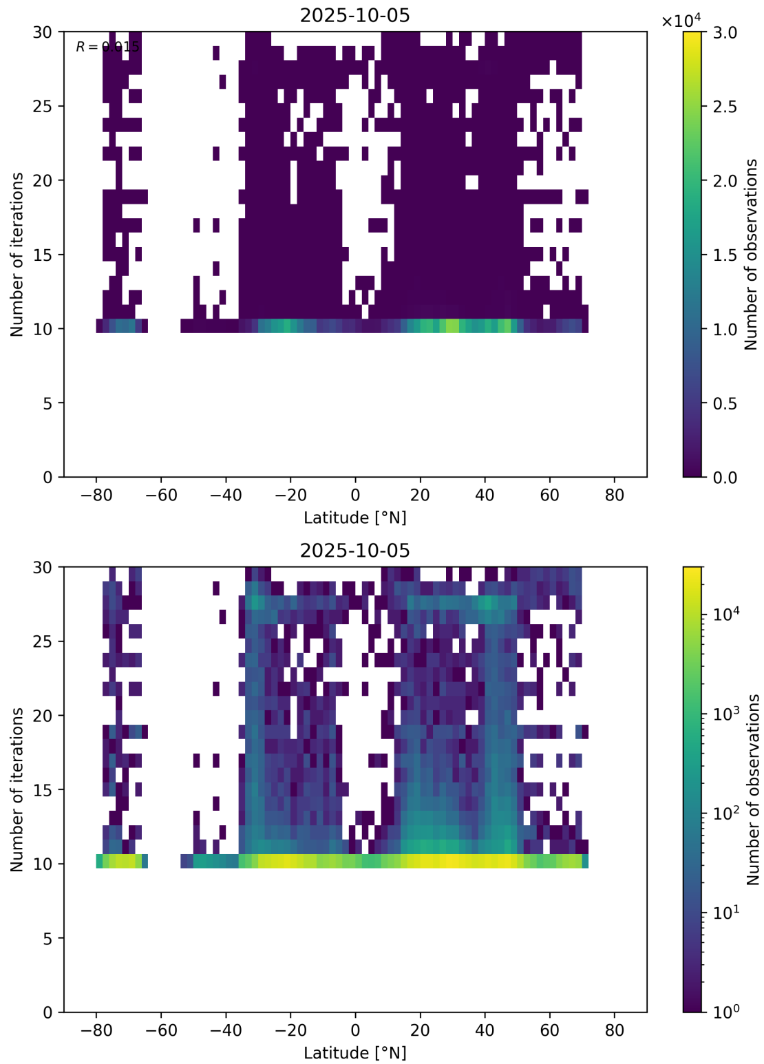
Figure 60: Scatter density plot of “Latitude” against “Number of iterations” for 2025-10-04 to 2025-10-06.
