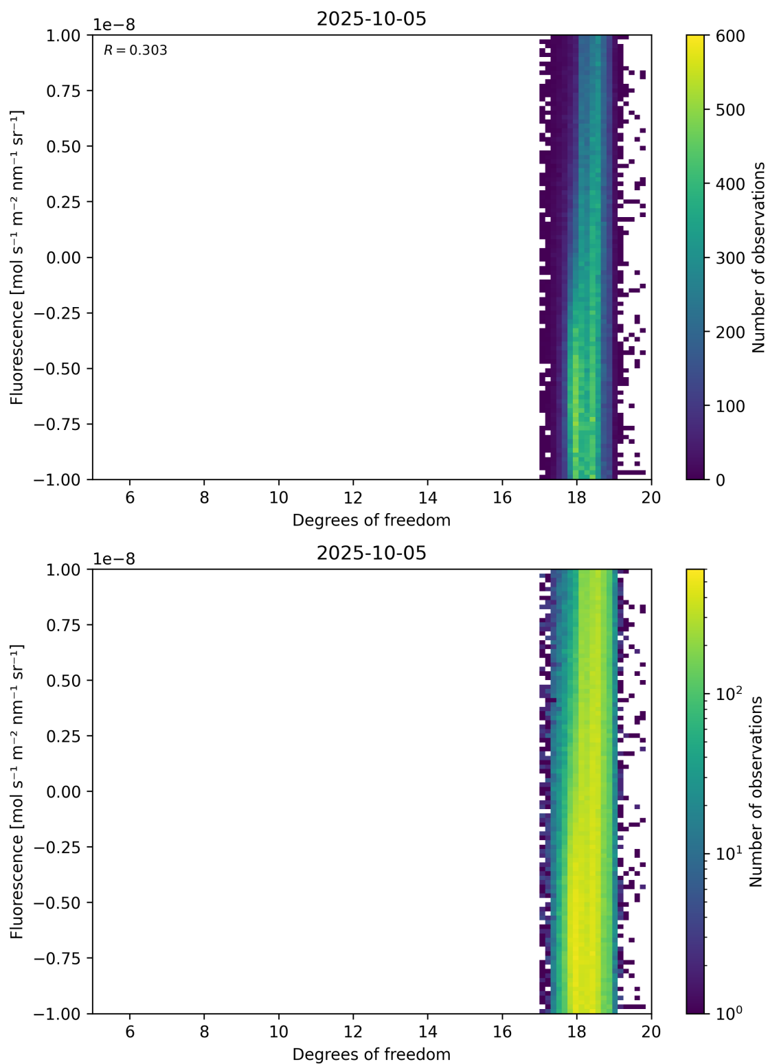
Figure 51: Scatter density plot of “Degrees of freedom” against “Fluorescence” for 2025-10-04 to 2025-10-06.
