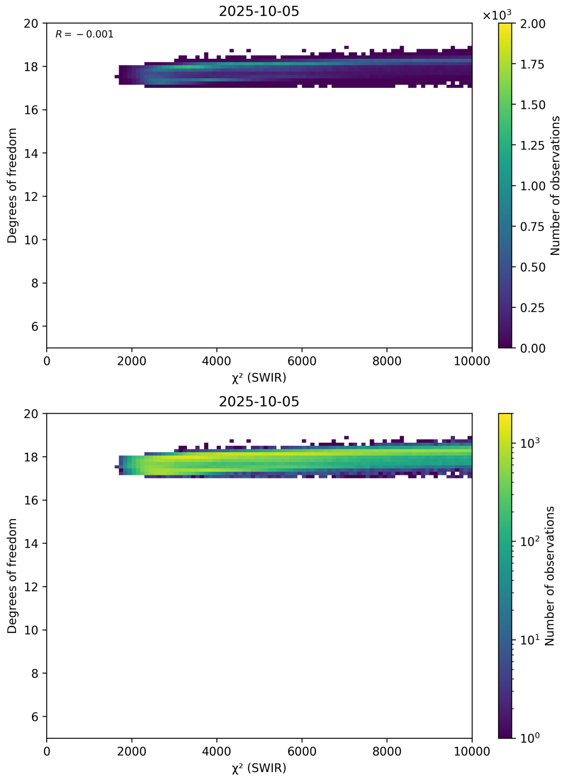
Figure 48: Scatter density plot of “ \chi^2 (SWIR)” against “Degrees of freedom” for 2025-10-04 to 2025-10-06.
