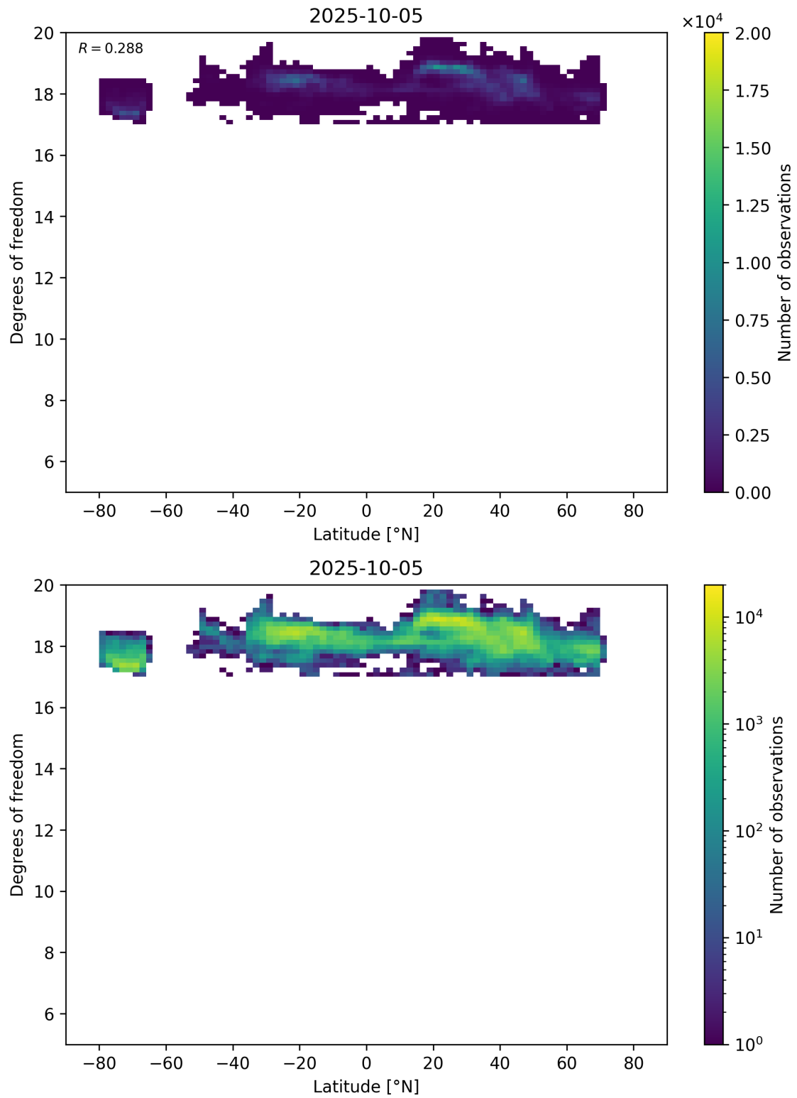
Figure 55: Scatter density plot of “Latitude” against “Degrees of freedom” for 2025-10-04 to 2025-10-06.
