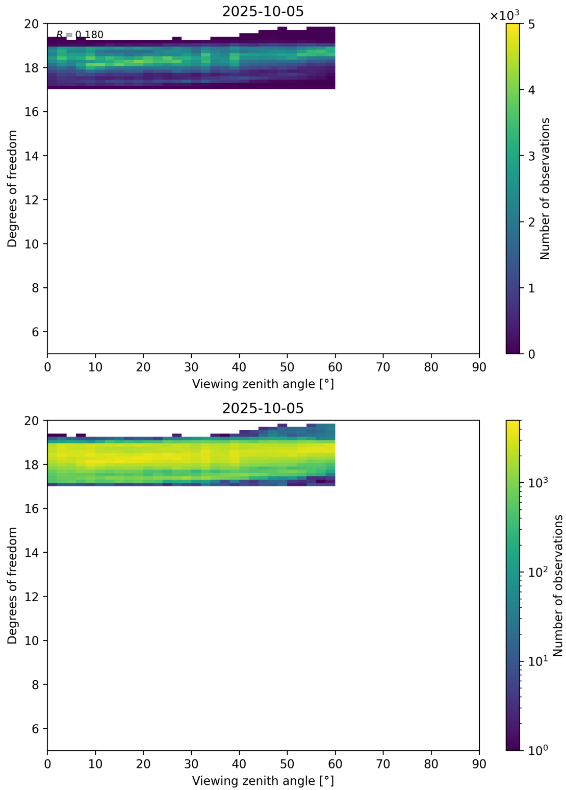
Figure 107: Scatter density plot of “Viewing zenith angle” against “Degrees of freedom” for 2025-10-04 to 2025-10-06.
