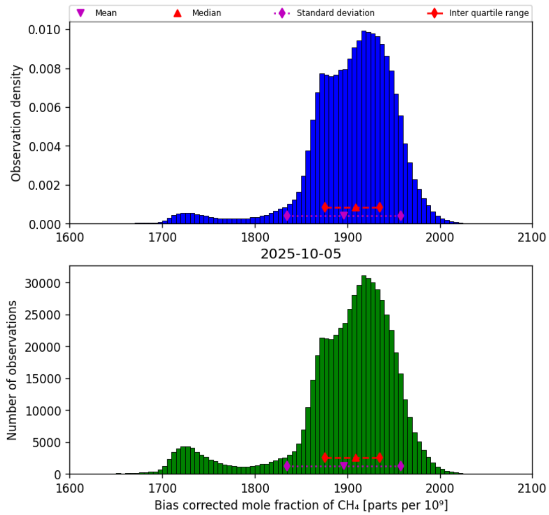
Figure 25: Histogram of “Bias corrected mole fraction of CH 4 ” for 2025-10-04 to 2025-10-06
