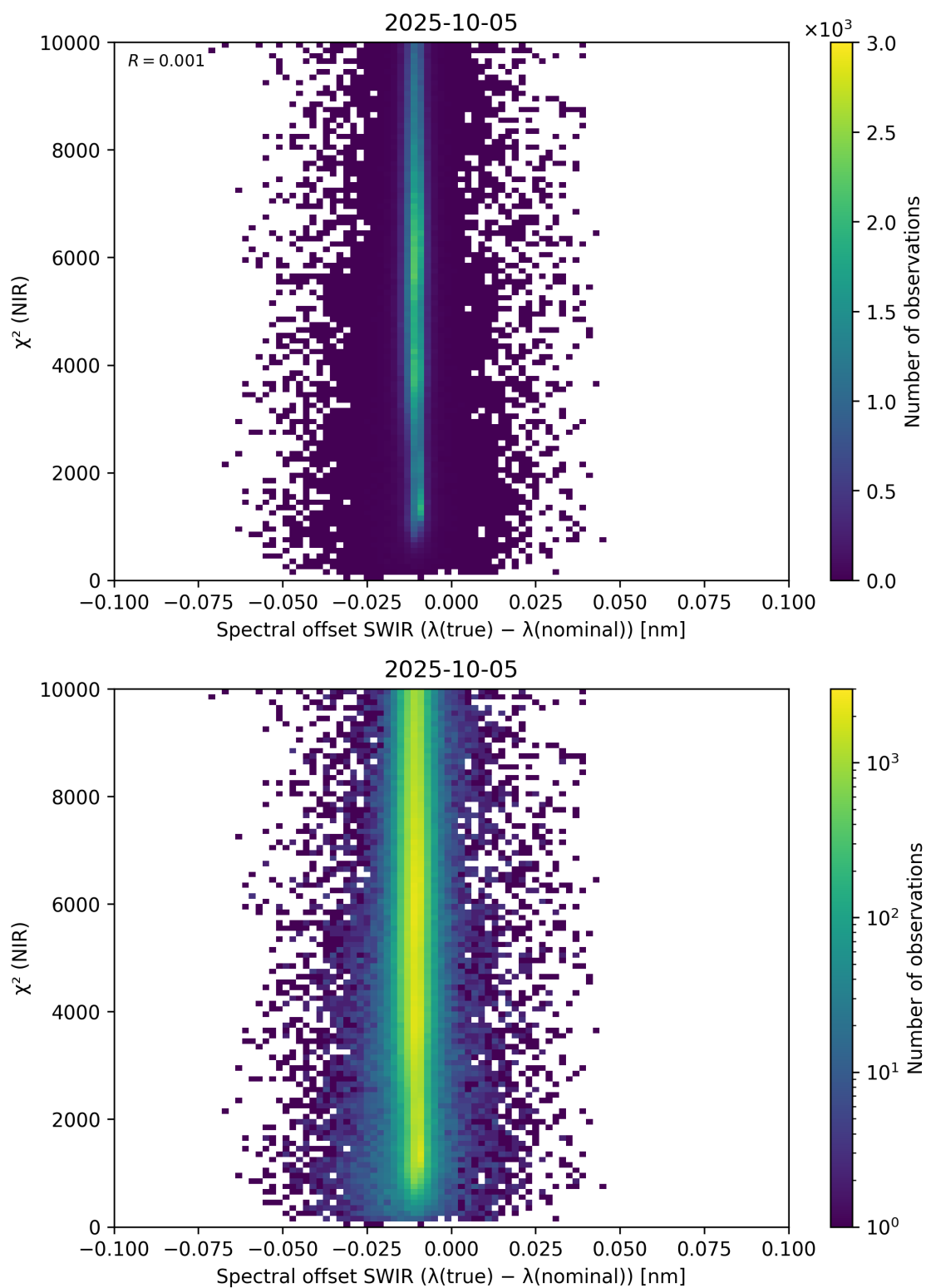
Figure 117: Scatter density plot of “Spectral offset SWIR ( \lambda_{\text{true}} - \lambda_{\text{nominal}} )” against “ \chi^2 (NIR)” for 2025-10-04 to 2025-10-06.
