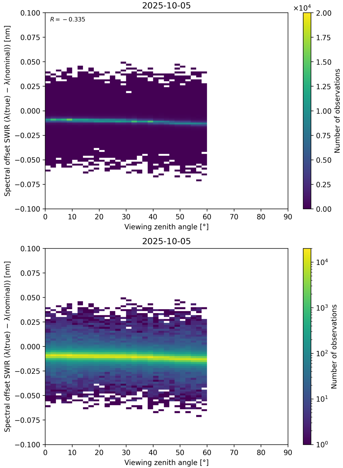
Figure 116: Scatter density plot of “Viewing zenith angle” against “Spectral offset SWIR ( \lambda_{\text{true}} - \lambda_{\text{nominal}} )” for 2025-10-04 to 2025-10-06.
