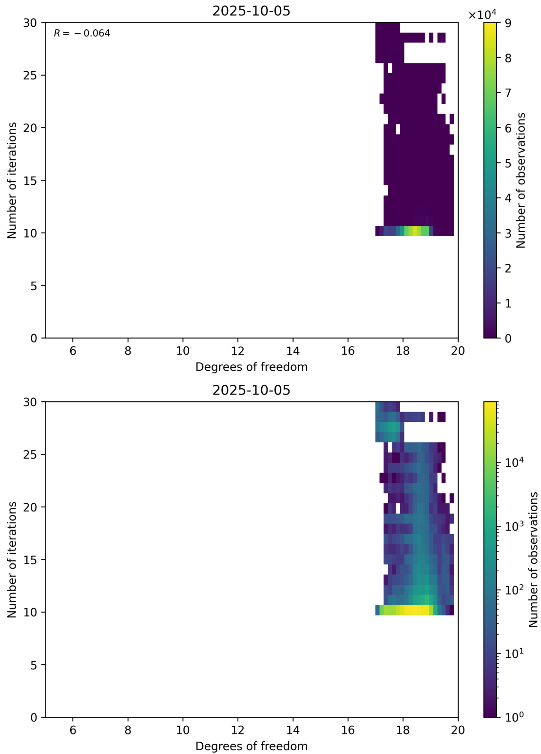
Figure 52: Scatter density plot of “Degrees of freedom” against “Number of iterations” for 2025-10-04 to 2025-10-06.
