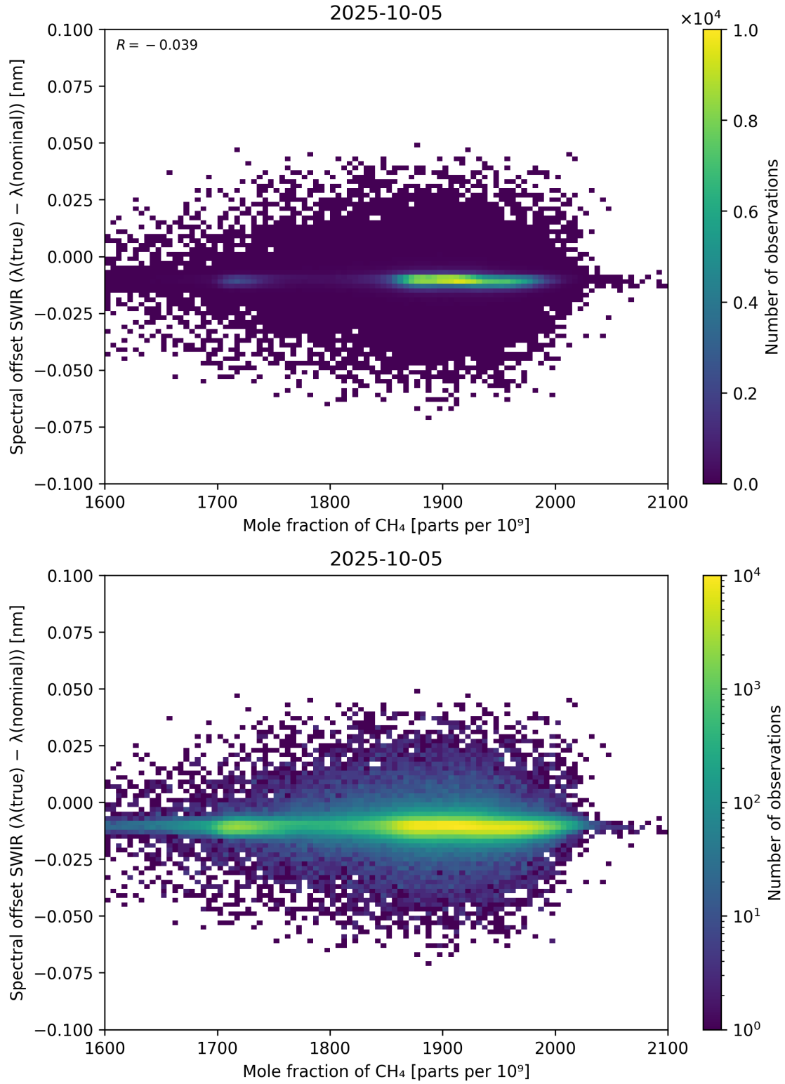
Figure 86: Scatter density plot of “Mole fraction of CH 4 ” against “Spectral offset SWIR ( \lambda_{\text{true}} - \lambda_{\text{nominal}} )” for 2025-10-04 to 2025-10-06.
