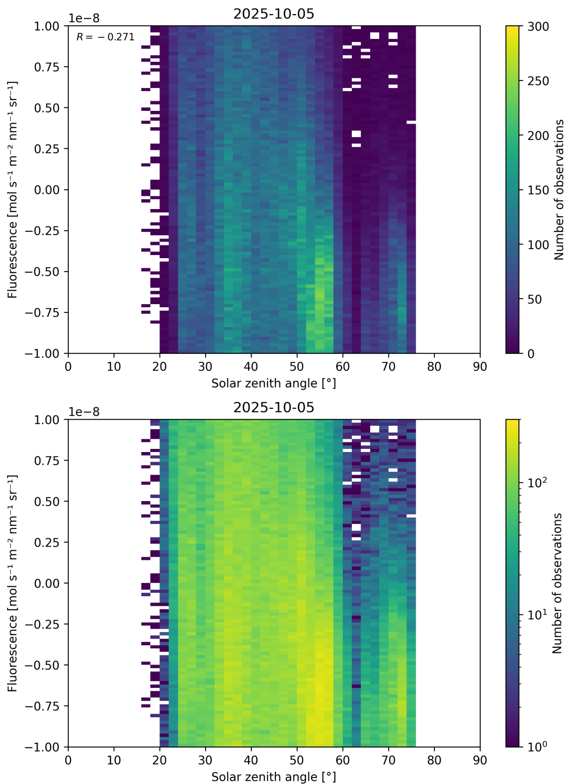
Figure 97: Scatter density plot of “Solar zenith angle” against “Fluorescence” for 2025-10-04 to 2025-10-06.
