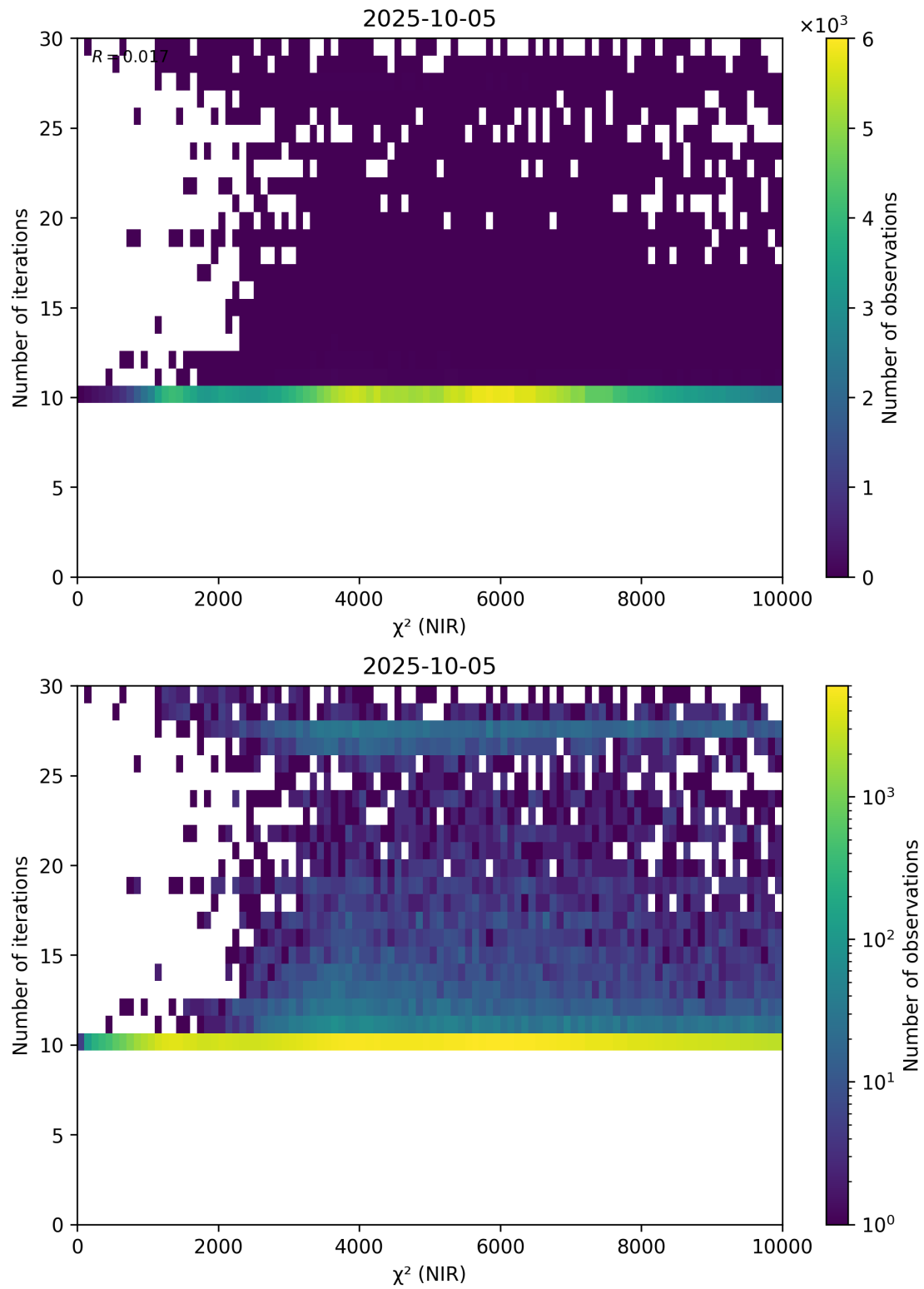
Figure 46: Scatter density plot of “ \chi^2 (NIR)” against “Number of iterations” for 2025-10-04 to 2025-10-06.
