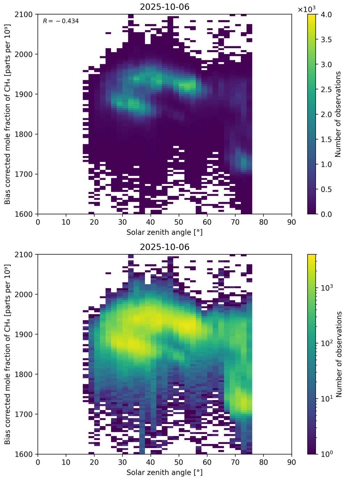
Figure 100: Scatter density plot of “Solar zenith angle” against “Bias corrected mole fraction of CH 4 ” for 2025-10-06 to 2025-10-07.
