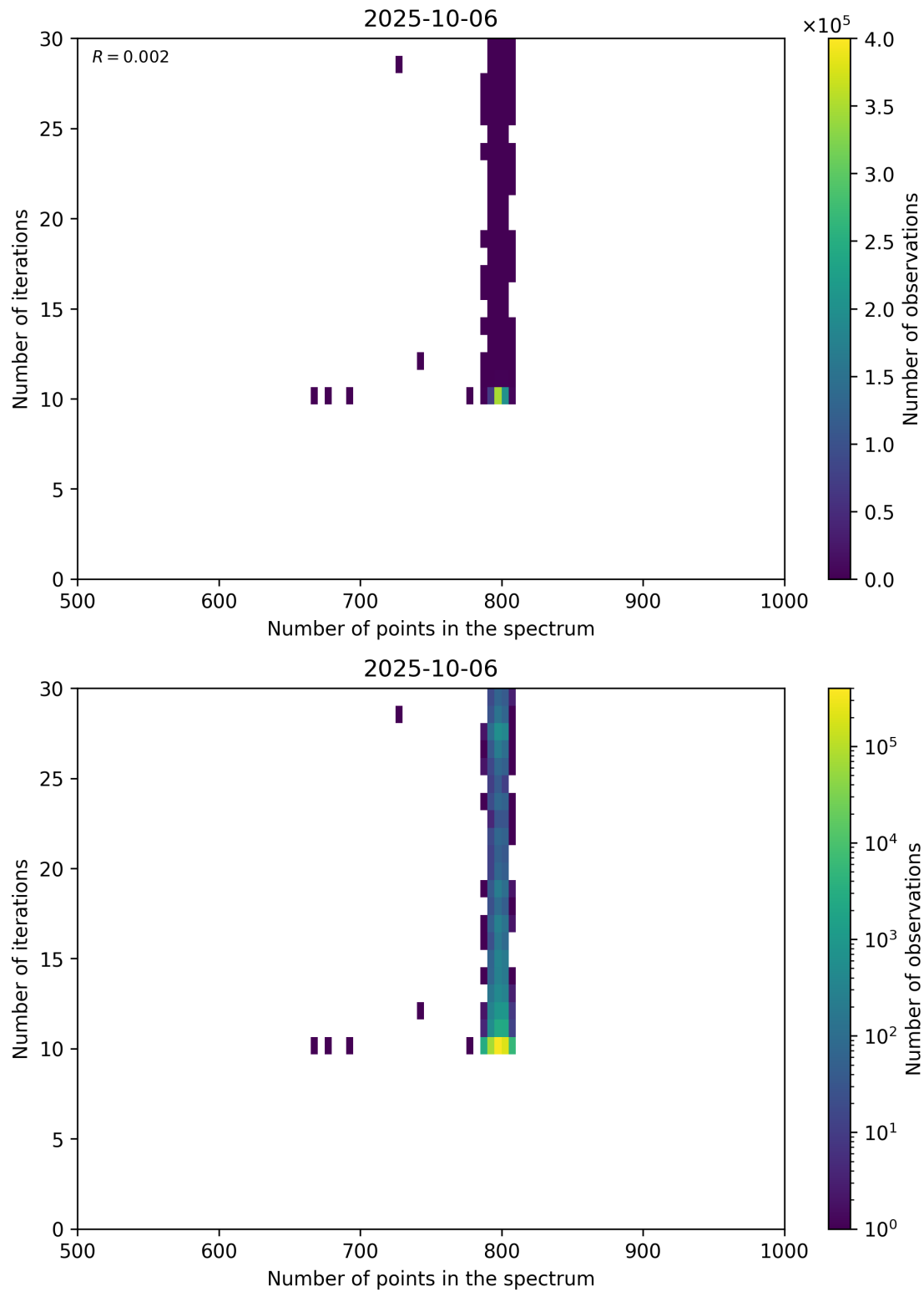
Figure 92: Scatter density plot of “Number of points in the spectrum” against “Number of iterations” for 2025-10-06 to 2025-10-07.
