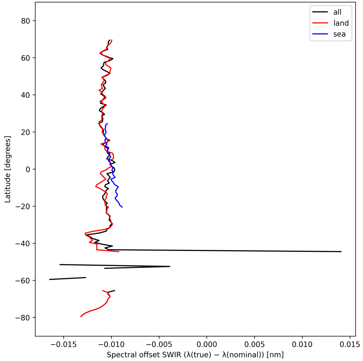
Figure 16: Zonal average of “Spectral offset SWIR ( \lambda_{\text{true}} - \lambda_{\text{nominal}} )” for 2025-10-06 to 2025-10-07.
