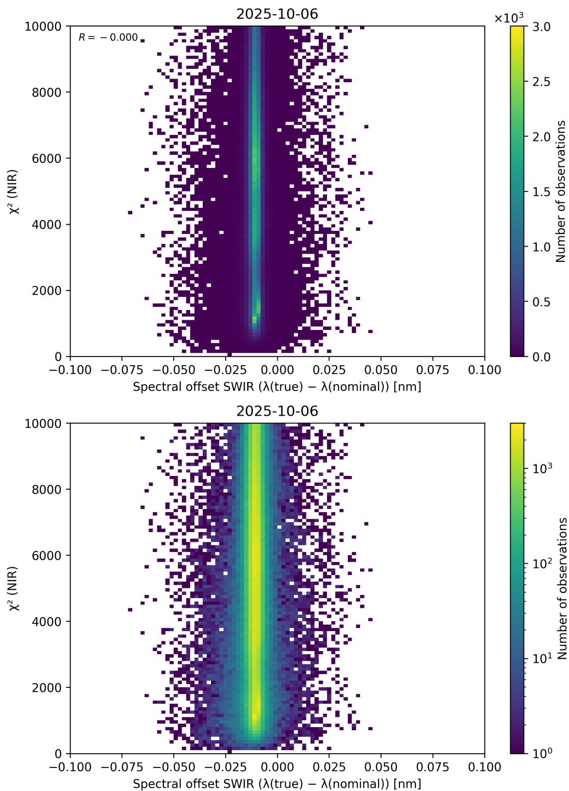
Figure 117: Scatter density plot of “Spectral offset SWIR ( \lambda_{\text{true}} - \lambda_{\text{nominal}} )” against “ \chi^2 (NIR)” for 2025-10-06 to 2025-10-07.
