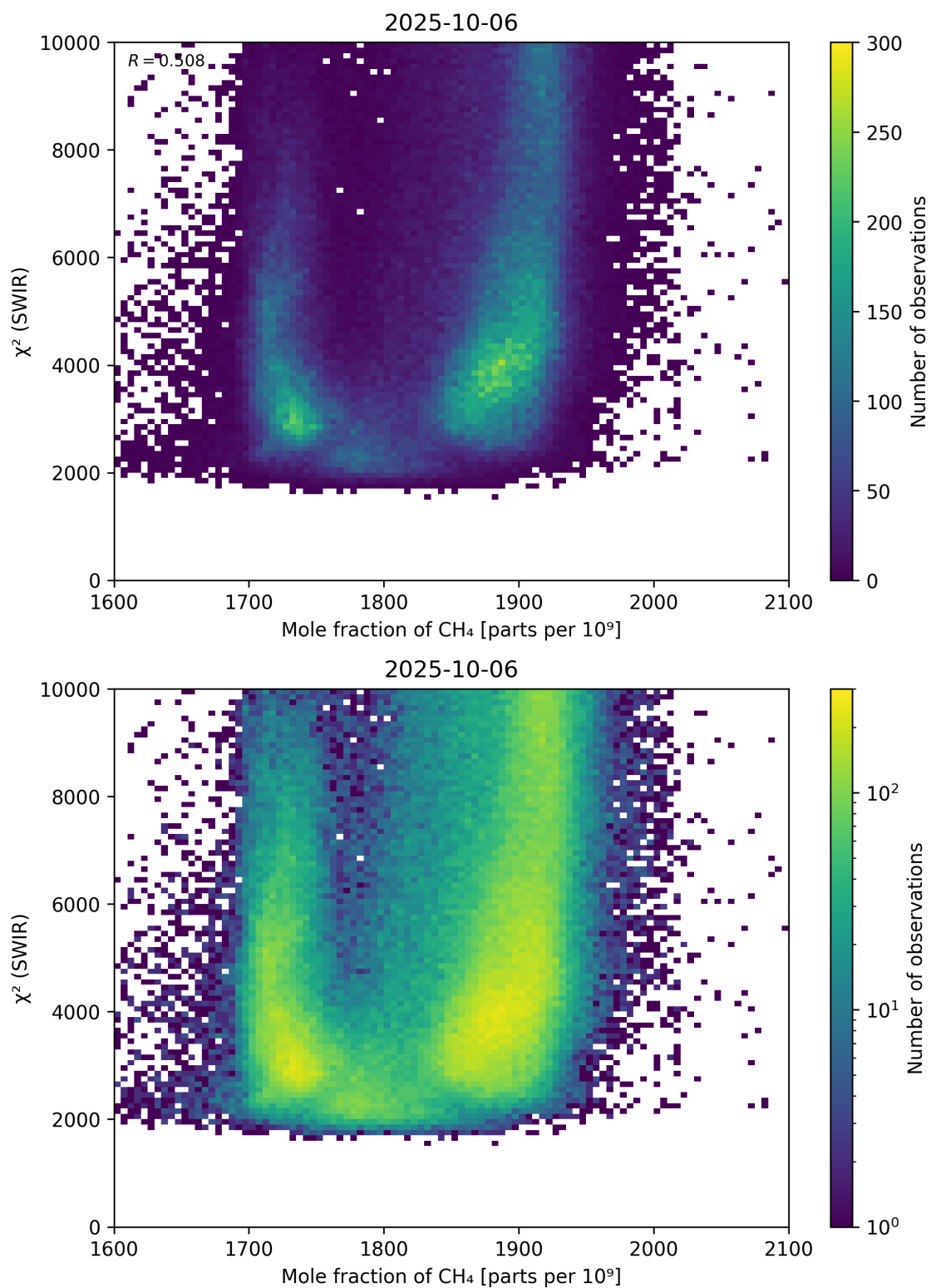
Figure 71: Scatter density plot of “Mole fraction of \text{CH}_4 ” against “ \chi^2 (SWIR)” for 2025-10-06 to 2025-10-07.
