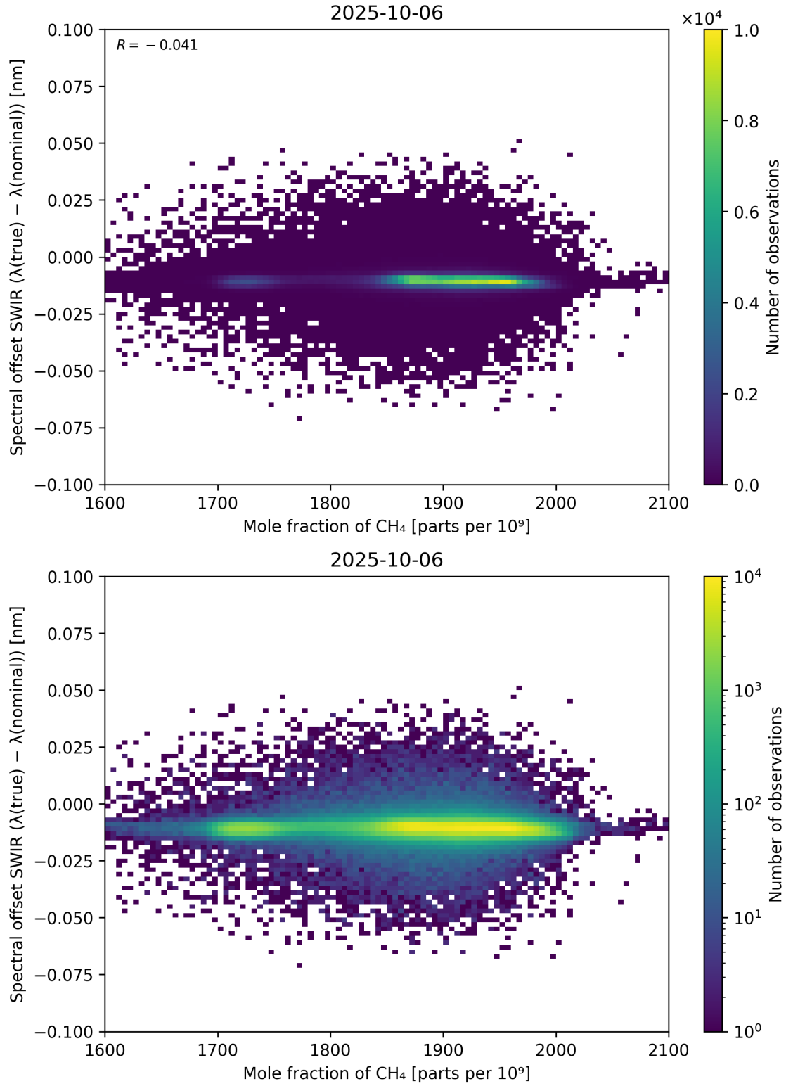
Figure 86: Scatter density plot of “Mole fraction of CH 4 ” against “Spectral offset SWIR ( \lambda_{\text{true}} - \lambda_{\text{nominal}} )” for 2025-10-06 to 2025-10-07.
