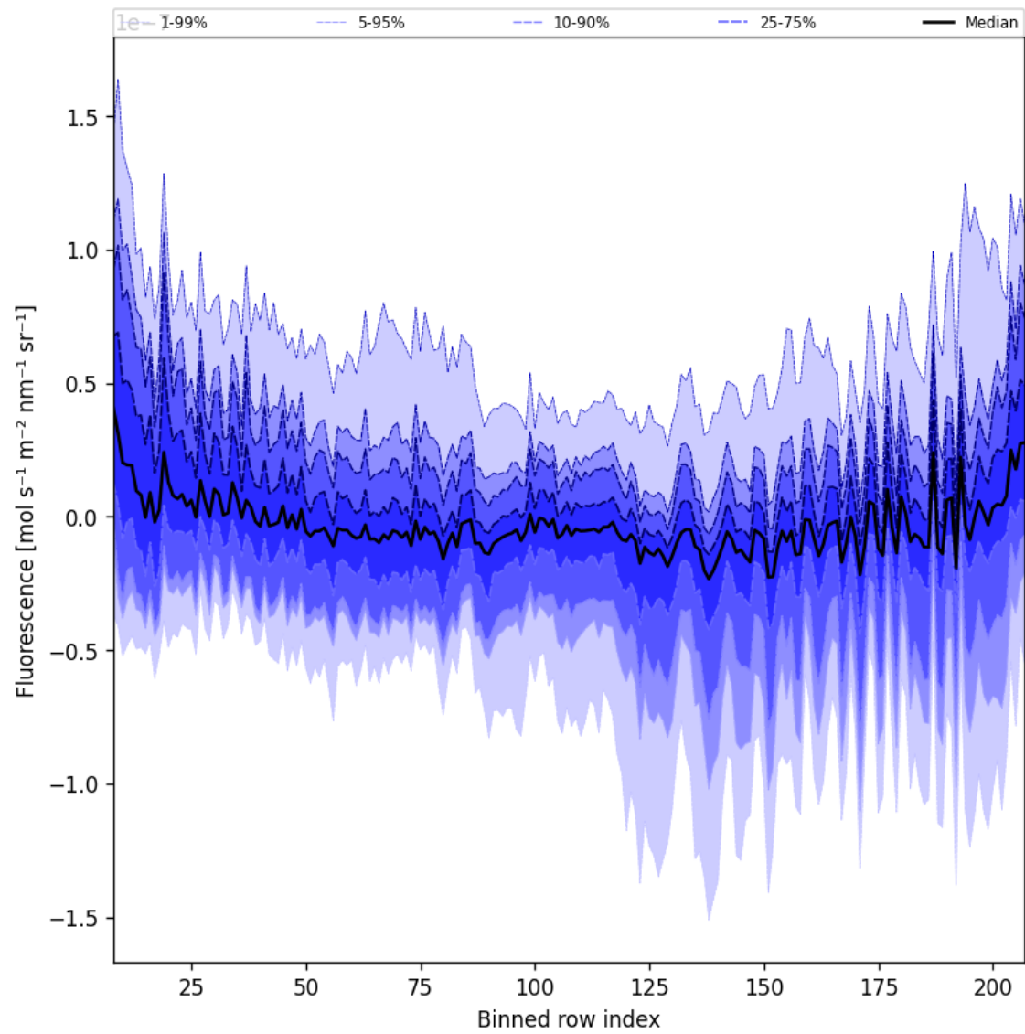
Figure 43: Along track statistics of “Fluorescence” for 2025-10-06 to 2025-10-07
