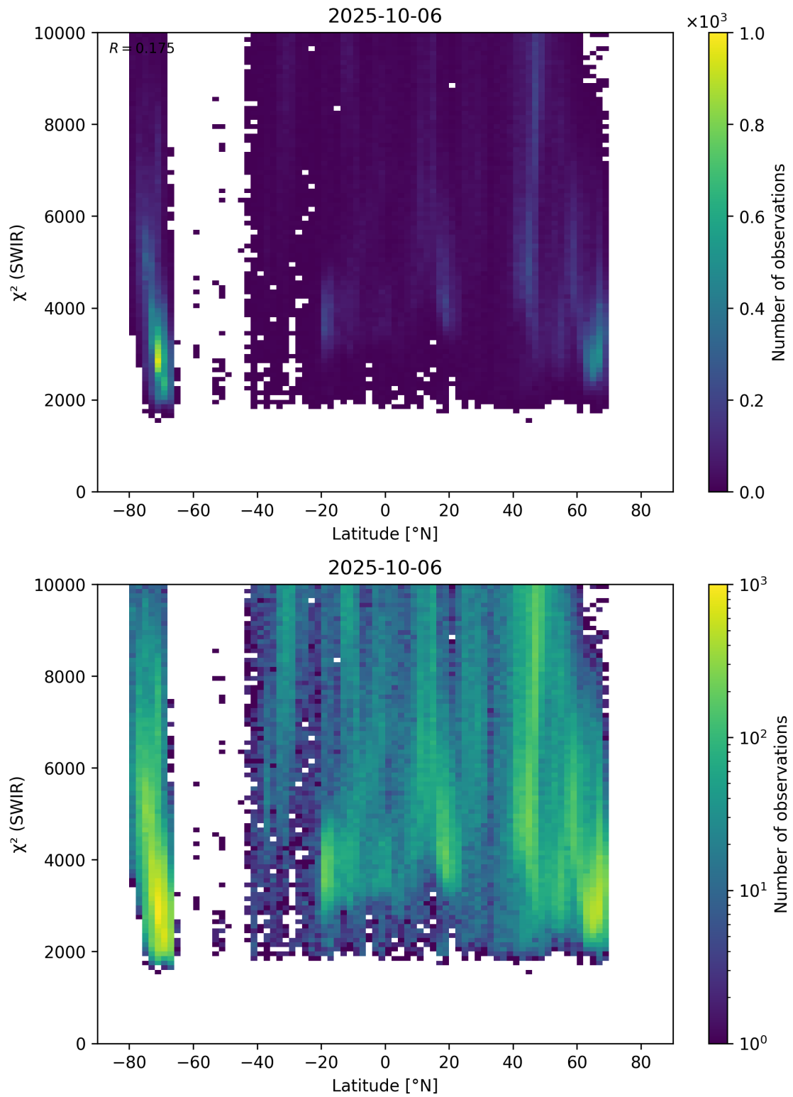
Figure 54: Scatter density plot of “Latitude” against “ \chi^2 (SWIR)” for 2025-10-06 to 2025-10-07.
