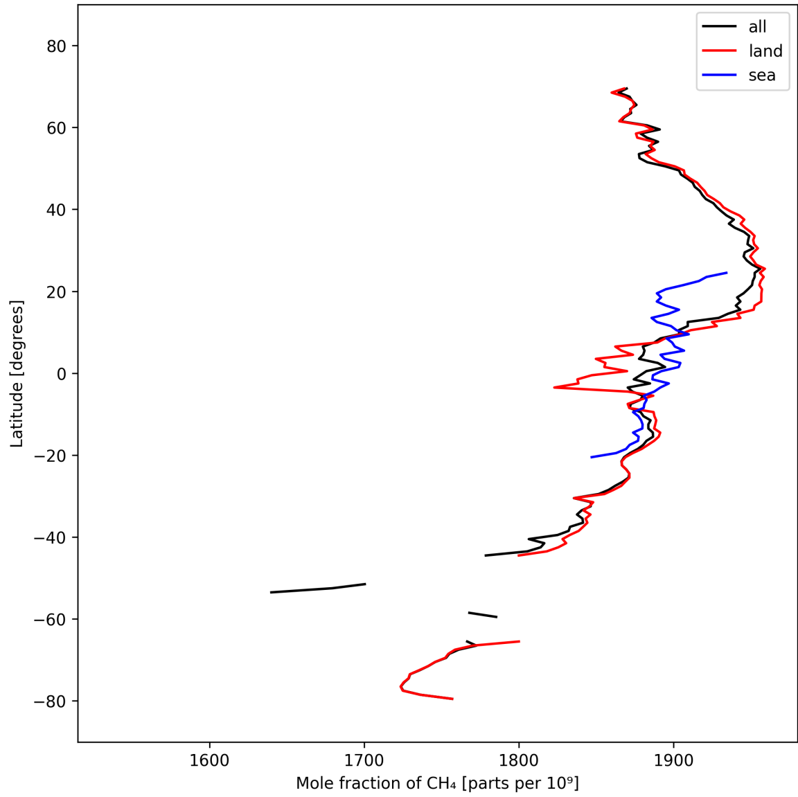
Figure 12: Zonal average of “Mole fraction of CH 4 ” for 2025-10-06 to 2025-10-07.
