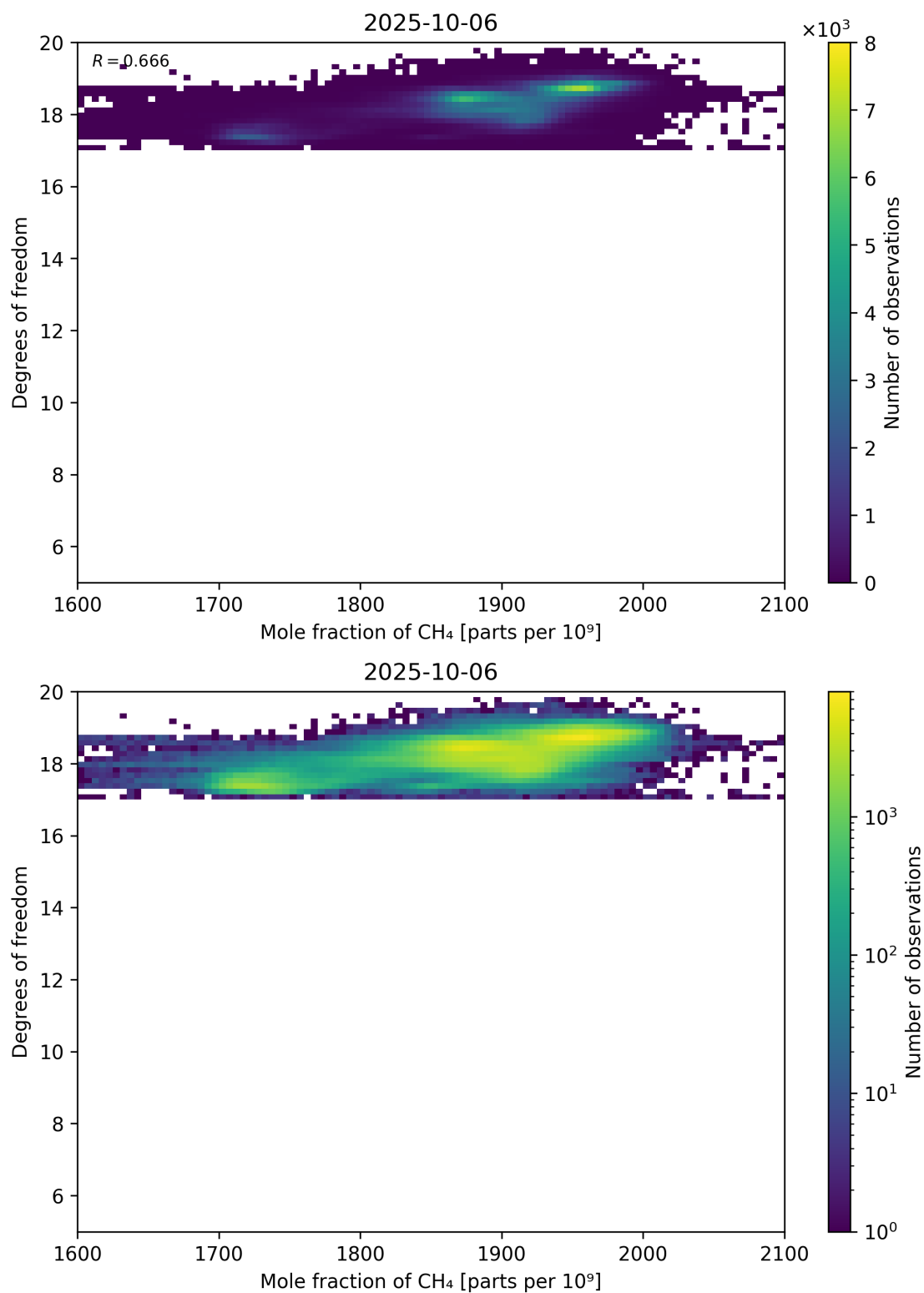
Figure 72: Scatter density plot of “Mole fraction of CH 4 ” against “Degrees of freedom” for 2025-10-06 to 2025-10-07.
