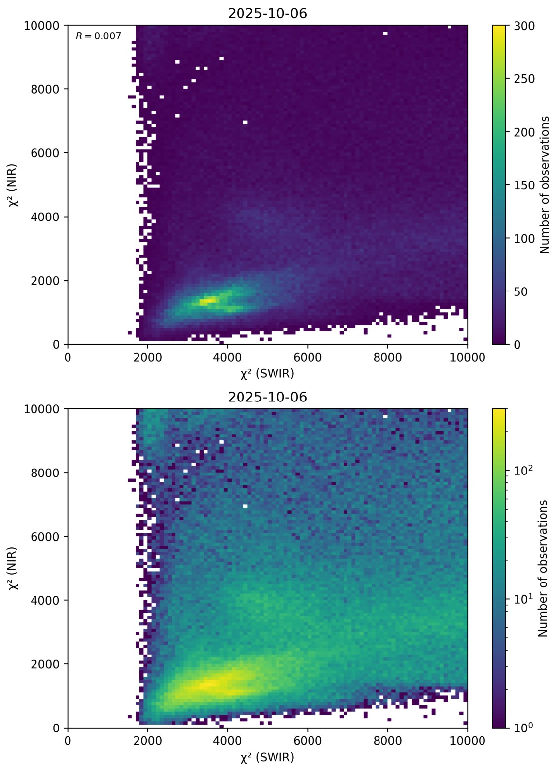
Figure 47: Scatter density plot of “ \chi^2 (SWIR)” against “ \chi^2 (NIR)” for 2025-10-06 to 2025-10-07.
