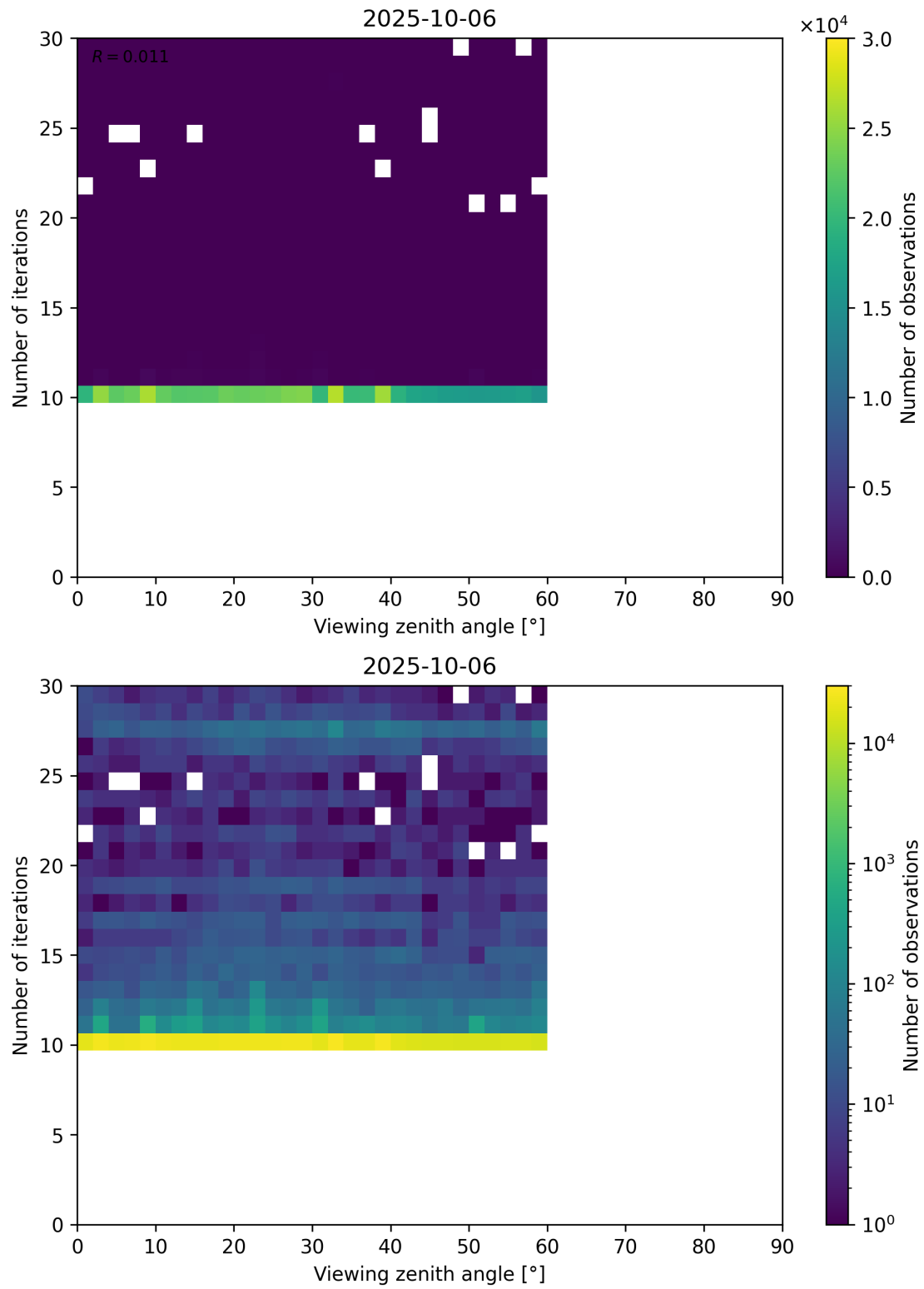
Figure 113: Scatter density plot of “Viewing zenith angle” against “Number of iterations” for 2025-10-06 to 2025-10-07.
