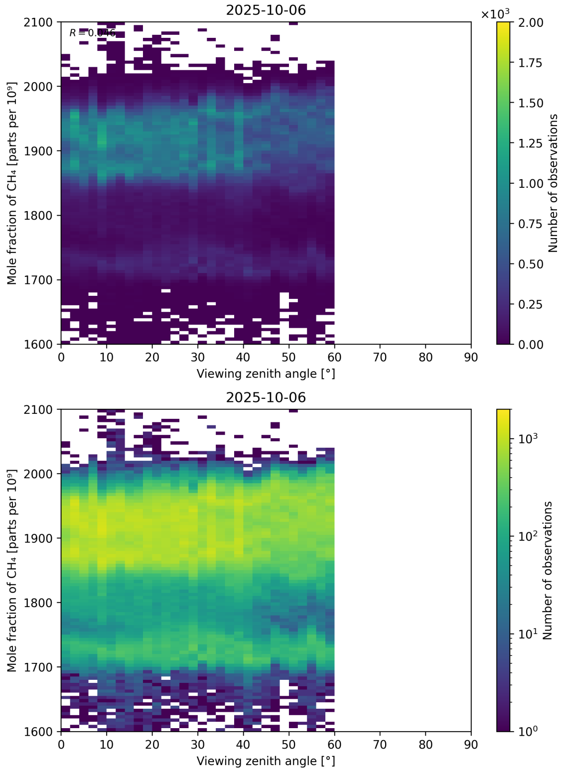
Figure 110: Scatter density plot of “Viewing zenith angle” against “Mole fraction of CH 4 ” for 2025-10-06 to 2025-10-07.
