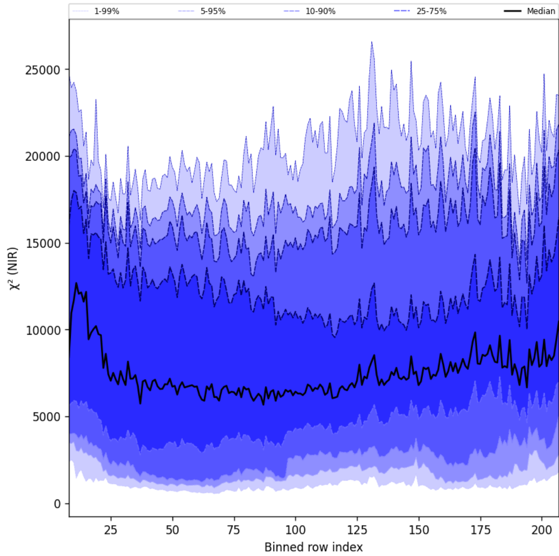
Figure 40: Along track statistics of “ \chi^2 (NIR)” for 2025-10-06 to 2025-10-07
