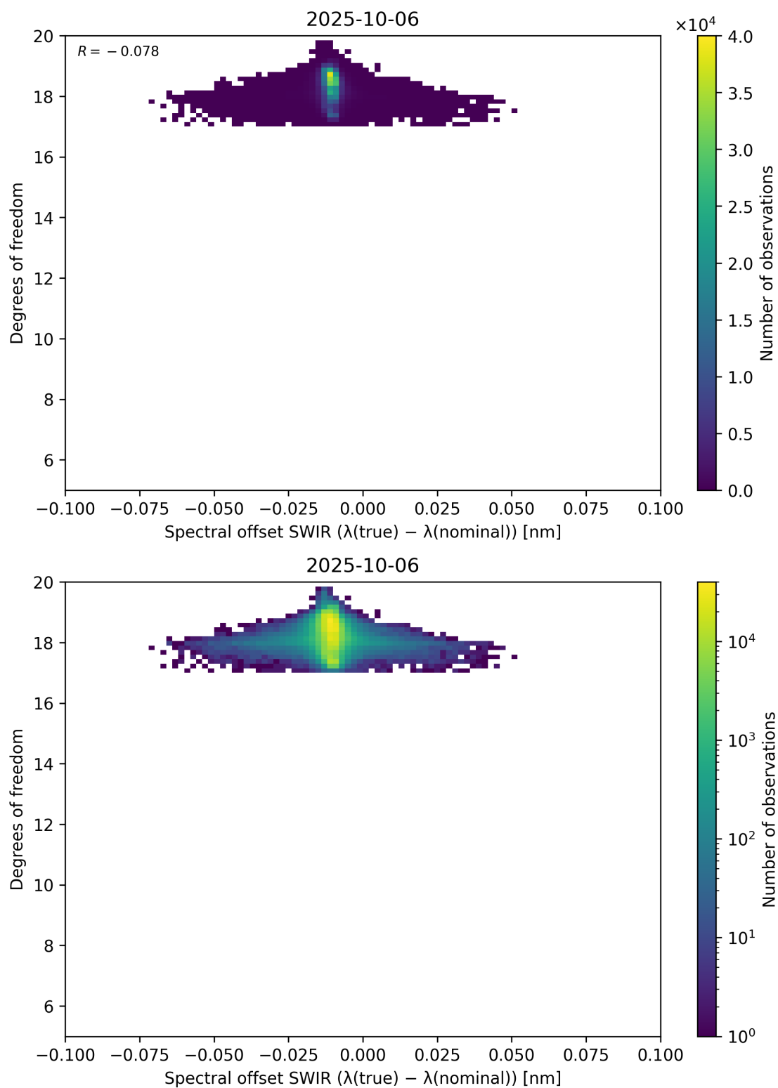
Figure 119: Scatter density plot of “Spectral offset SWIR ( \lambda_{\text{true}} - \lambda_{\text{nominal}} )” against “Degrees of freedom” for 2025-10-06 to 2025-10-07.
