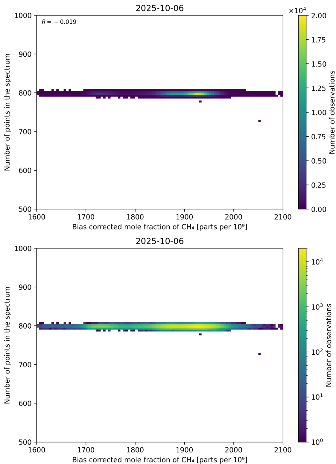
Figure 68: Scatter density plot of “Bias corrected mole fraction of CH 4 ” against “Number of points in the spectrum” for 2025-10-06 to 2025-10-07.
