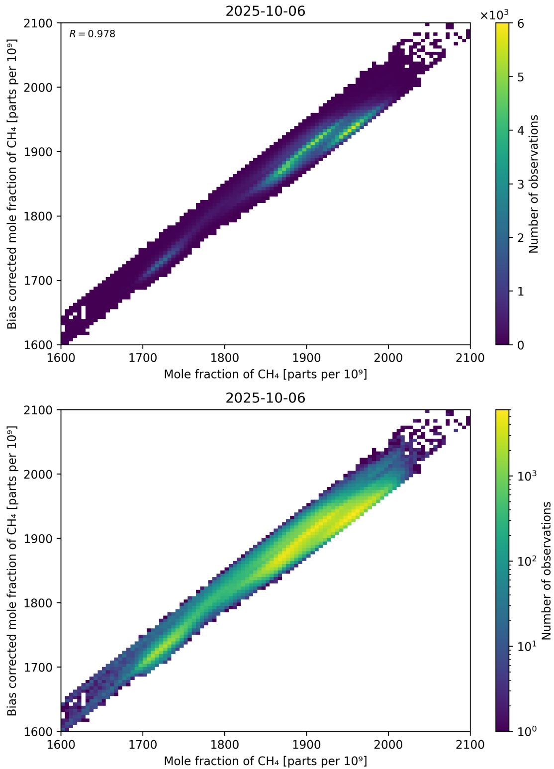
Figure 74: Scatter density plot of “Mole fraction of CH 4 ” against “Bias corrected mole fraction of CH 4 ” for 2025-10-06 to 2025-10-07.
