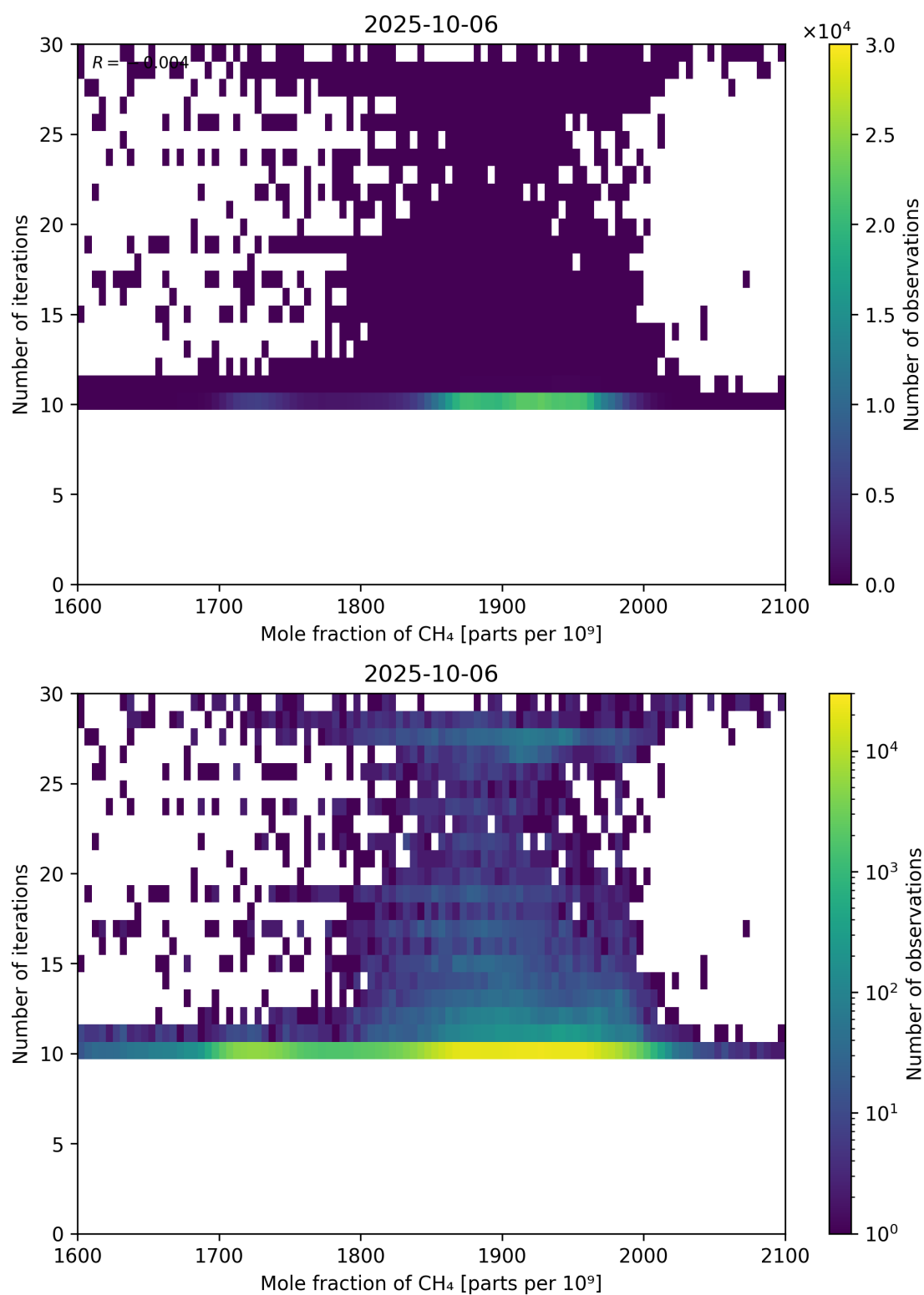
Figure 76: Scatter density plot of “Mole fraction of CH 4 ” against “Number of iterations” for 2025-10-06 to 2025-10-07.
