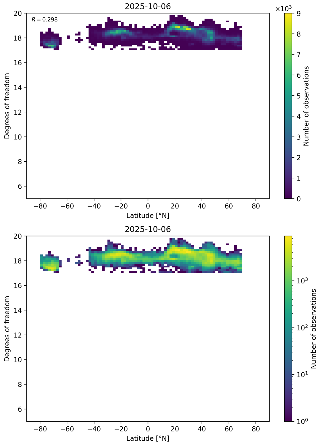
Figure 55: Scatter density plot of “Latitude” against “Degrees of freedom” for 2025-10-06 to 2025-10-07.
