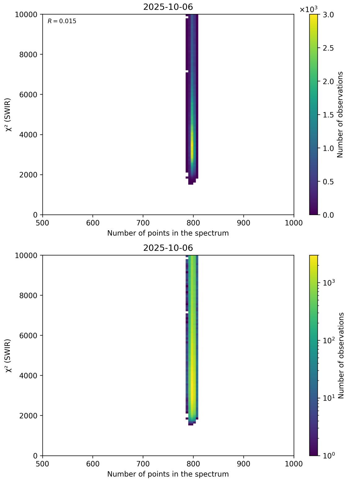
Figure 89: Scatter density plot of “Number of points in the spectrum” against “ \chi^2 (SWIR)” for 2025-10-06 to 2025-10-07.
