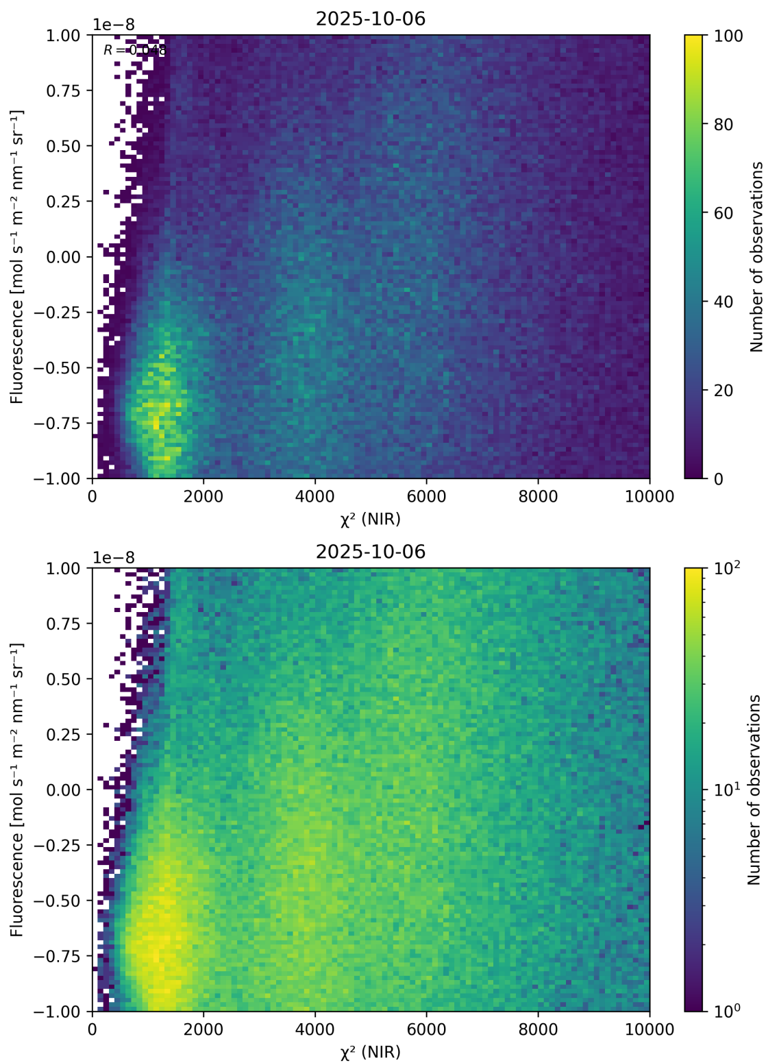
Figure 45: Scatter density plot of “ \chi^2 (NIR)” against “Fluorescence” for 2025-10-06 to 2025-10-07.
