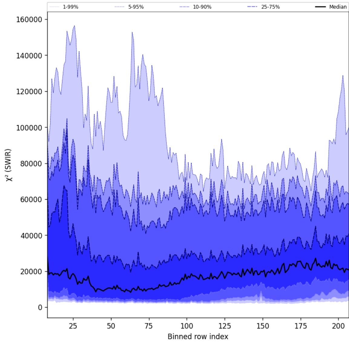
Figure 39: Along track statistics of “ \chi^2 (SWIR)” for 2025-10-06 to 2025-10-07
