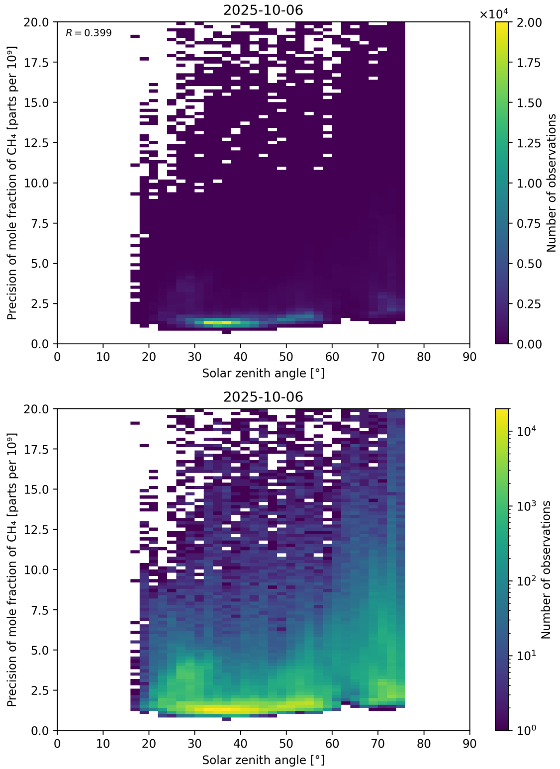
Figure 101: Scatter density plot of “Solar zenith angle” against “Precision of mole fraction of CH 4 ” for 2025-10-06 to 2025-10-07.
