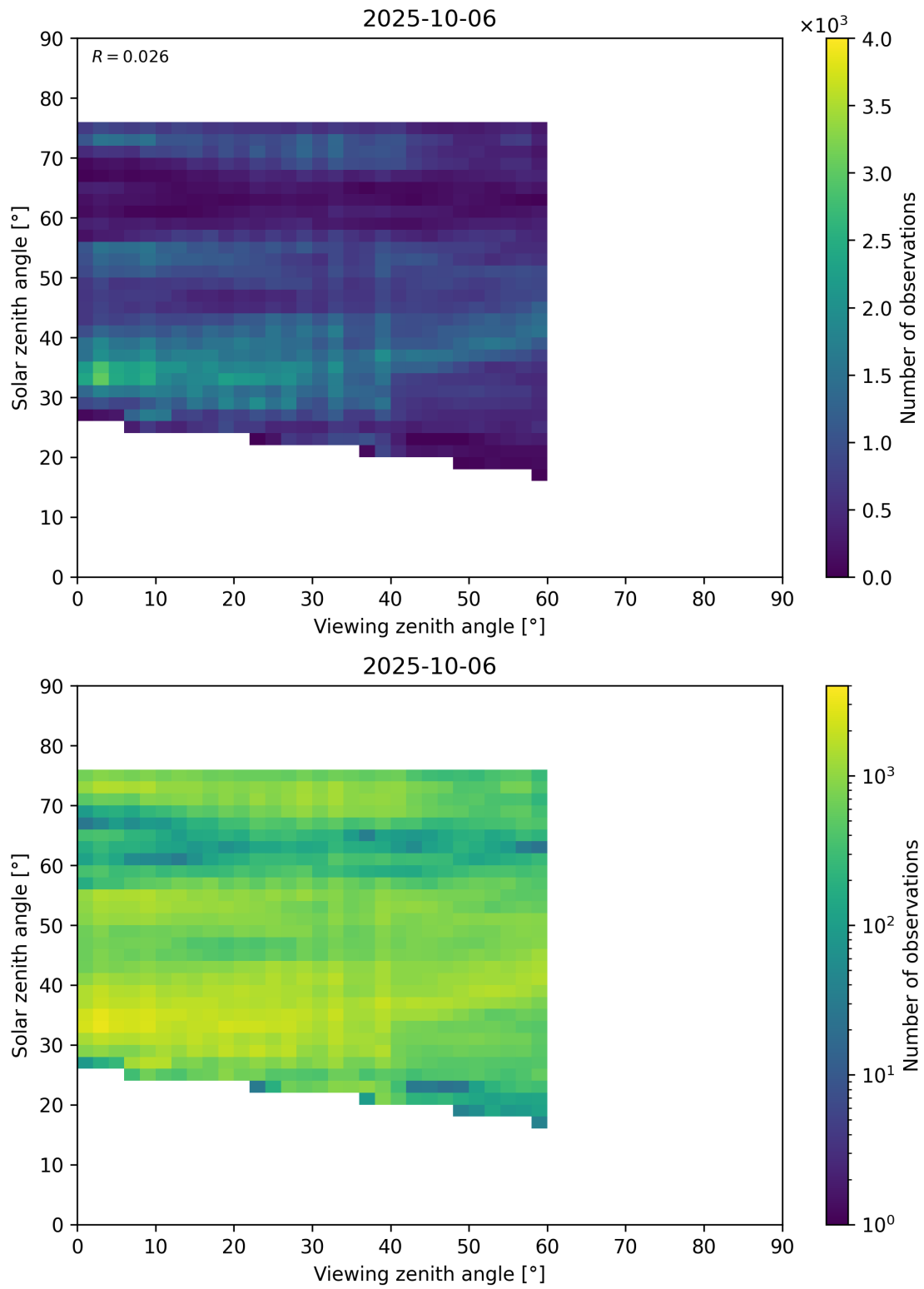
Figure 115: Scatter density plot of “Viewing zenith angle” against “Solar zenith angle” for 2025-10-06 to 2025-10-07.
