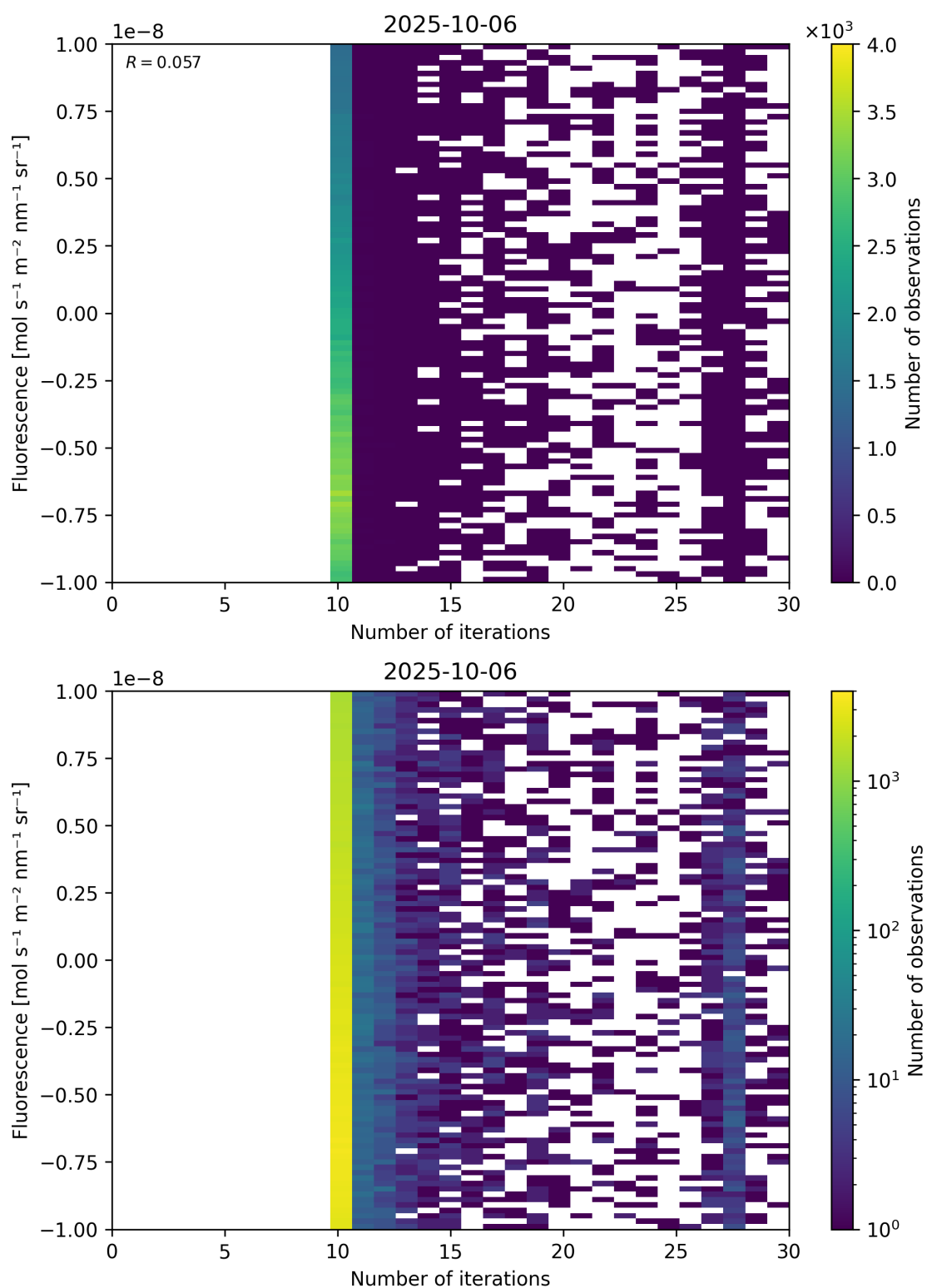
Figure 87: Scatter density plot of “Number of iterations” against “Fluorescence” for 2025-10-06 to 2025-10-07.
