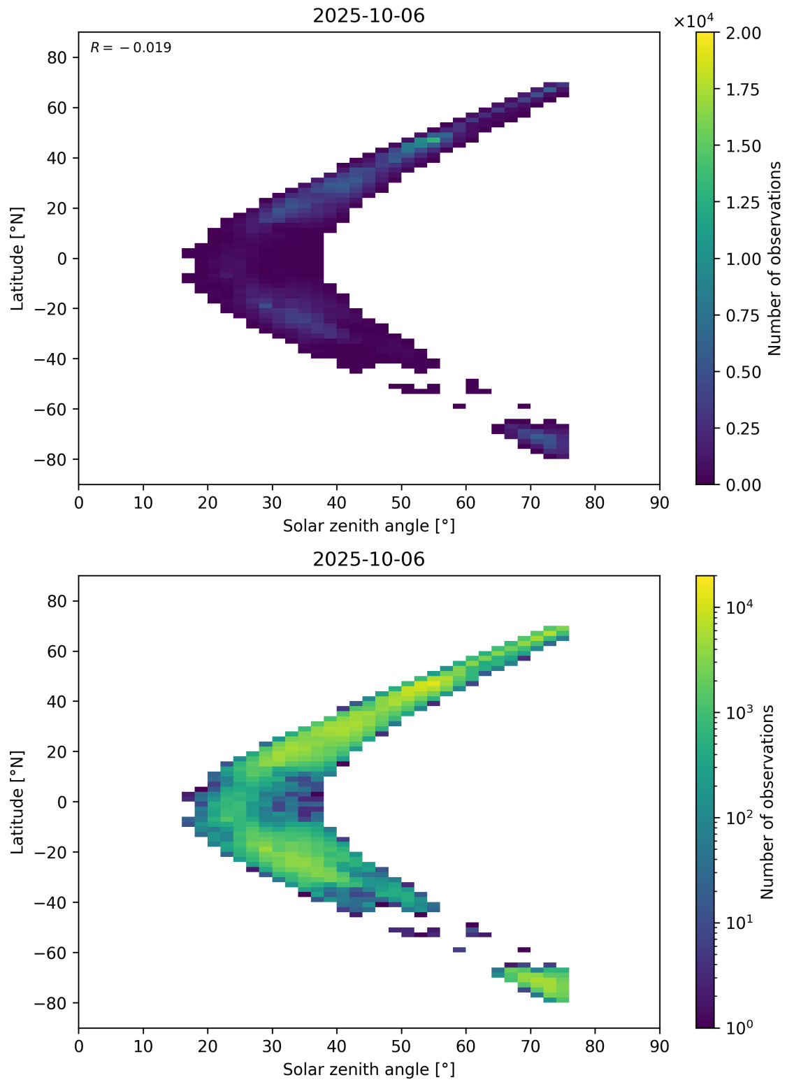
Figure 98: Scatter density plot of “Solar zenith angle” against “Latitude” for 2025-10-06 to 2025-10-07.
