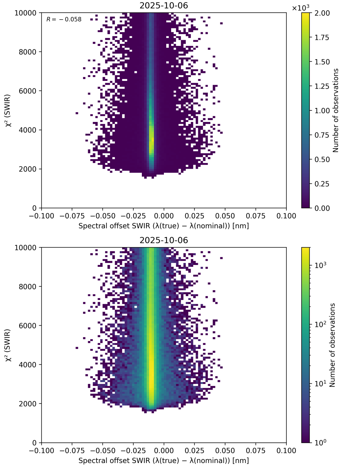
Figure 118: Scatter density plot of “Spectral offset SWIR ( \lambda_{\text{true}} - \lambda_{\text{nominal}} )” against “ \chi^2 (SWIR)” for 2025-10-06 to 2025-10-07.
