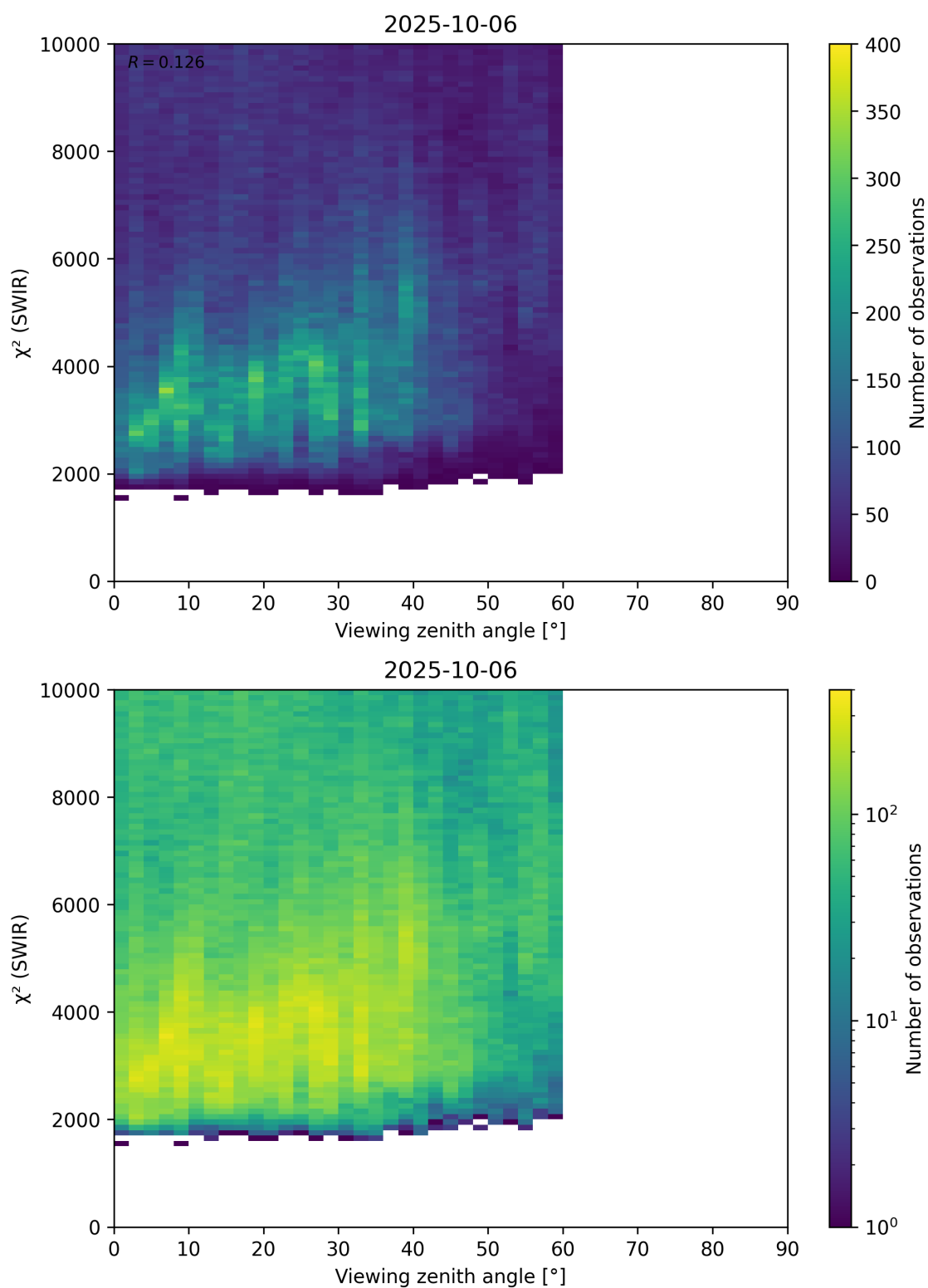
Figure 106: Scatter density plot of “Viewing zenith angle” against “ \chi^2 (SWIR)” for 2025-10-06 to 2025-10-07.
