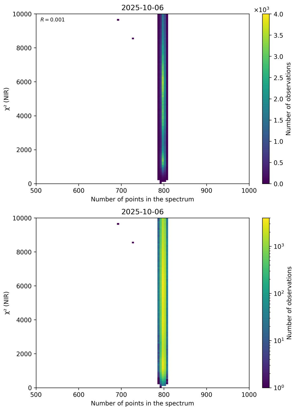
Figure 88: Scatter density plot of “Number of points in the spectrum” against “ \chi^2 (NIR)” for 2025-10-06 to 2025-10-07.
