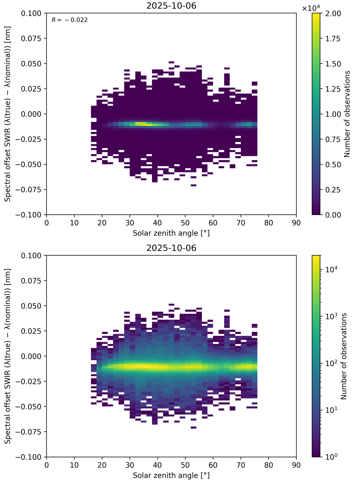
Figure 104: Scatter density plot of “Solar zenith angle” against “Spectral offset SWIR ( \lambda_{\text{true}} - \lambda_{\text{nominal}} )” for 2025-10-06 to 2025-10-07.
