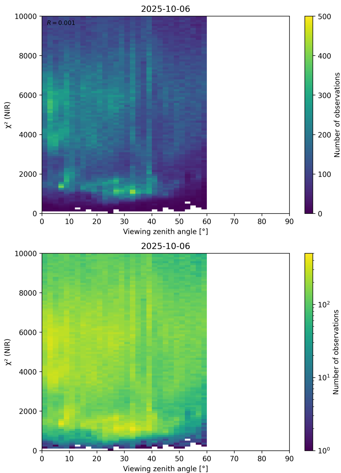
Figure 105: Scatter density plot of “Viewing zenith angle” against “ \chi^2 (NIR)” for 2025-10-06 to 2025-10-07.
