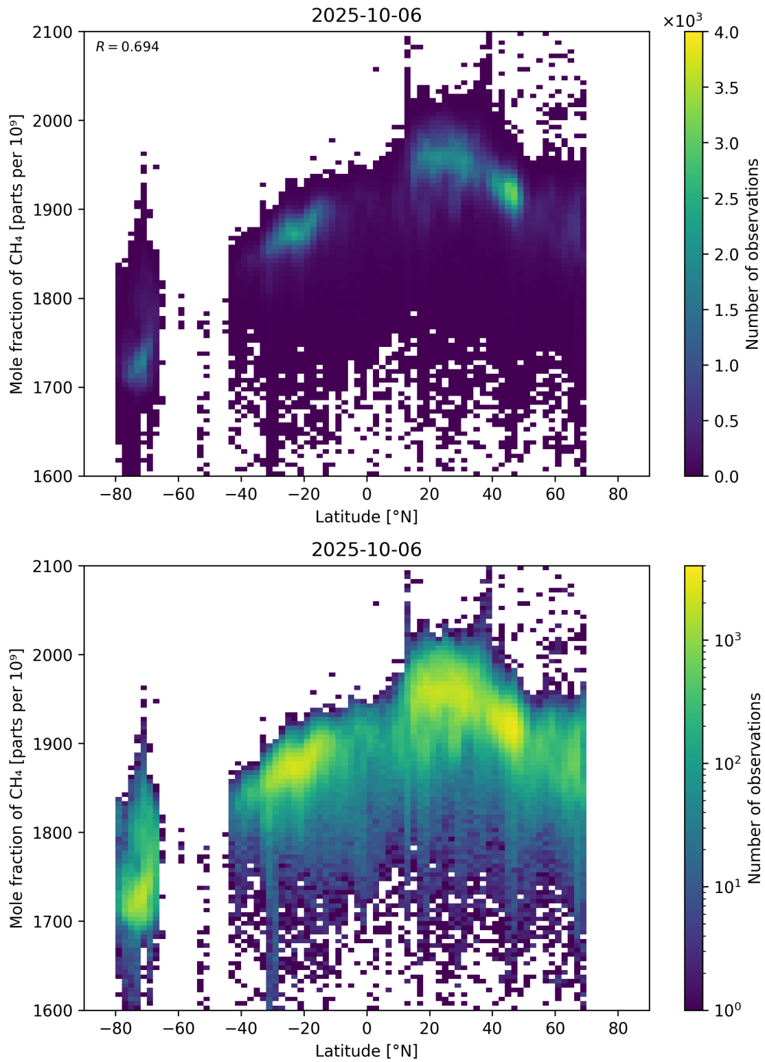
Figure 57: Scatter density plot of “Latitude” against “Mole fraction of CH 4 ” for 2025-10-06 to 2025-10-07.
