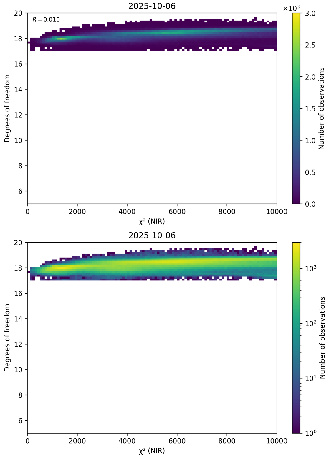
Figure 44: Scatter density plot of “ \chi^2 (NIR)” against “Degrees of freedom” for 2025-10-06 to 2025-10-07.
