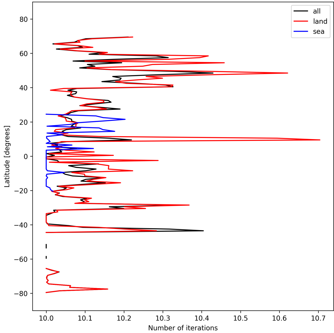
Figure 20: Zonal average of “Number of iterations” for 2025-10-06 to 2025-10-07.
