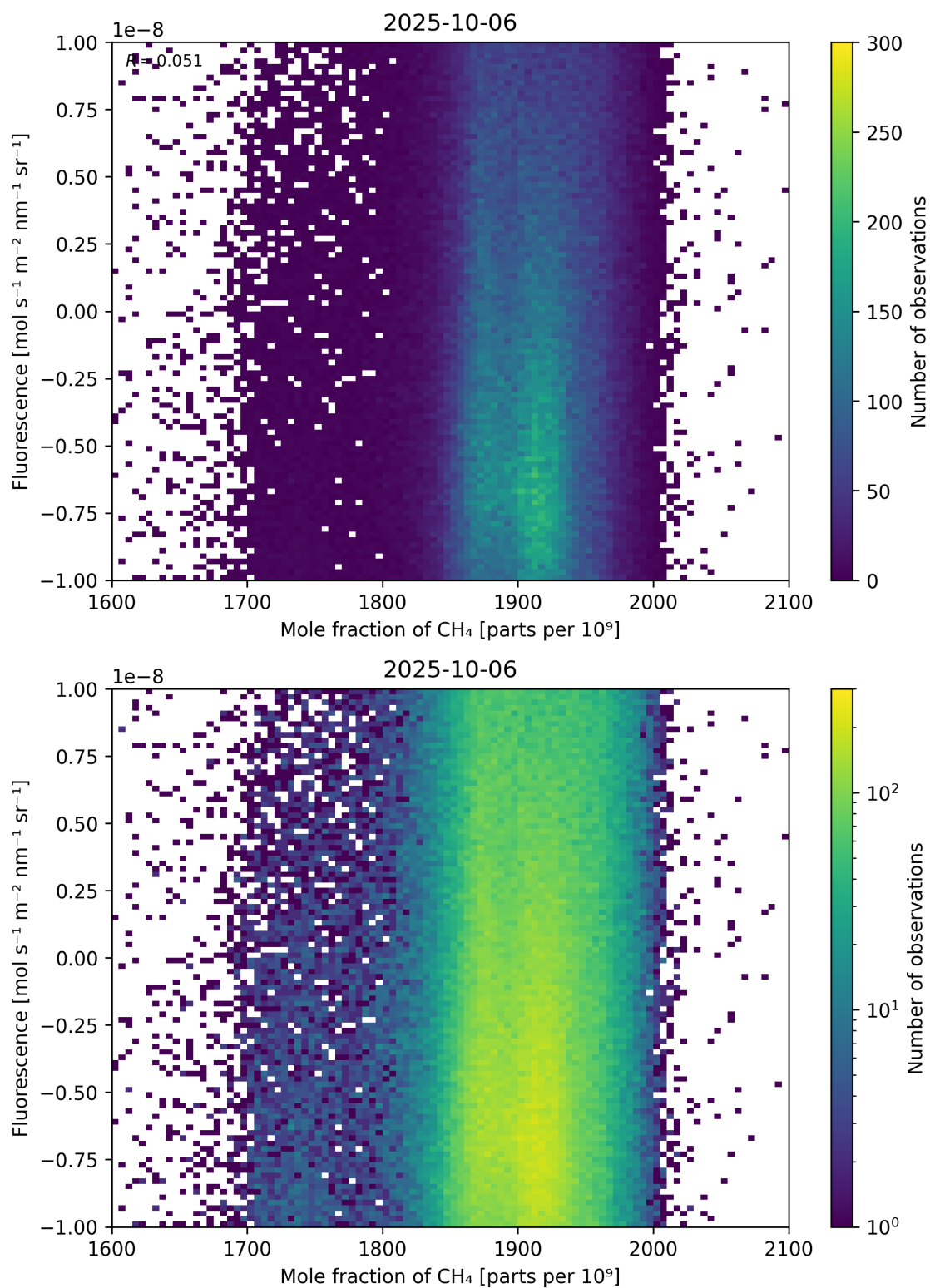
Figure 73: Scatter density plot of “Mole fraction of \text{CH}_4 ” against “Fluorescence” for 2025-10-06 to 2025-10-07.
