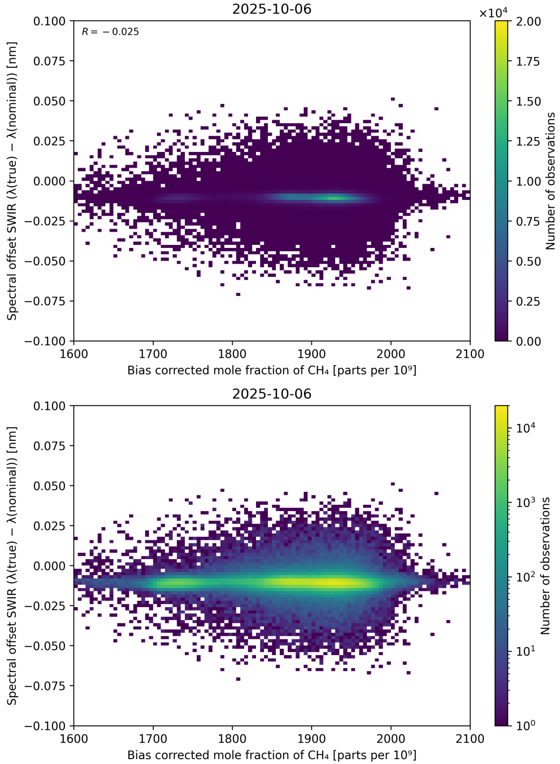
Figure 69: Scatter density plot of “Bias corrected mole fraction of \text{CH}_4 ” against “Spectral offset SWIR ( \lambda_{\text{true}} - \lambda_{\text{nominal}} )” for 2025-10-06 to 2025-10-07.
