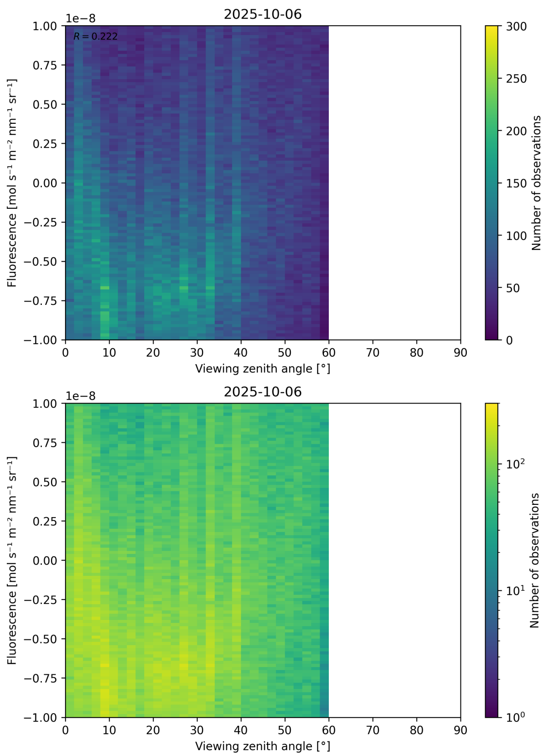
Figure 108: Scatter density plot of “Viewing zenith angle” against “Fluorescence” for 2025-10-06 to 2025-10-07.
