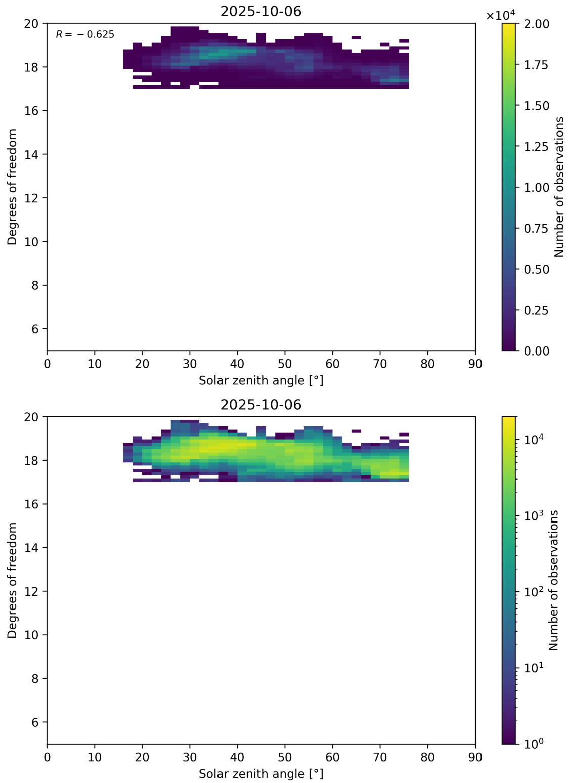
Figure 96: Scatter density plot of “Solar zenith angle” against “Degrees of freedom” for 2025-10-06 to 2025-10-07.
