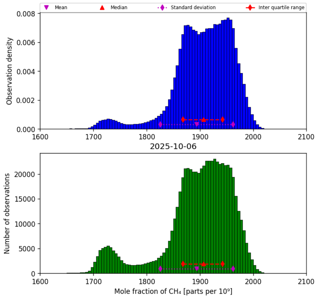
Figure 23: Histogram of “Mole fraction of CH 4 ” for 2025-10-06 to 2025-10-07
