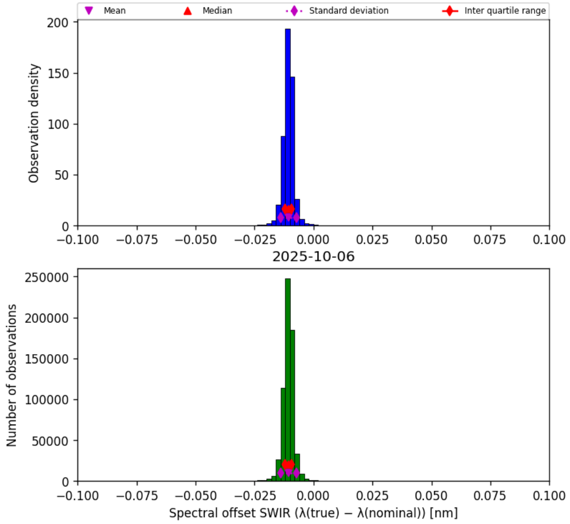
Figure 27: Histogram of “Spectral offset SWIR ( \lambda_{\text{true}} - \lambda_{\text{nominal}} )” for 2025-10-06 to 2025-10-07
