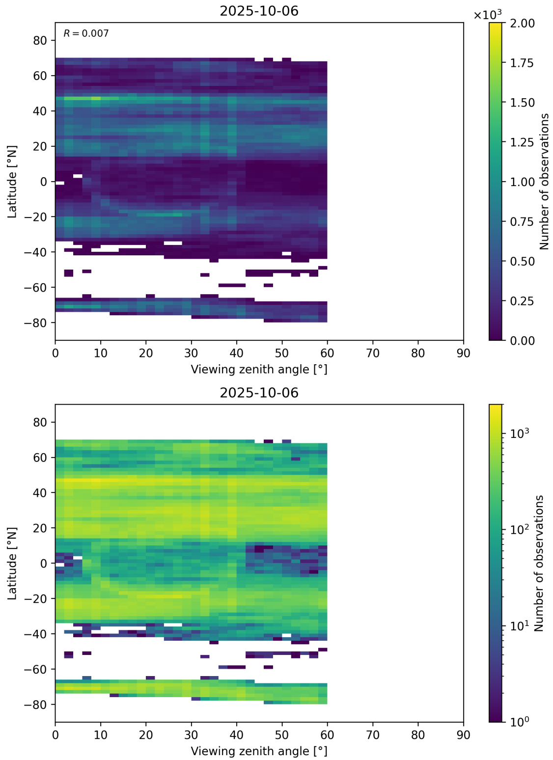
Figure 109: Scatter density plot of “Viewing zenith angle” against “Latitude” for 2025-10-06 to 2025-10-07.
