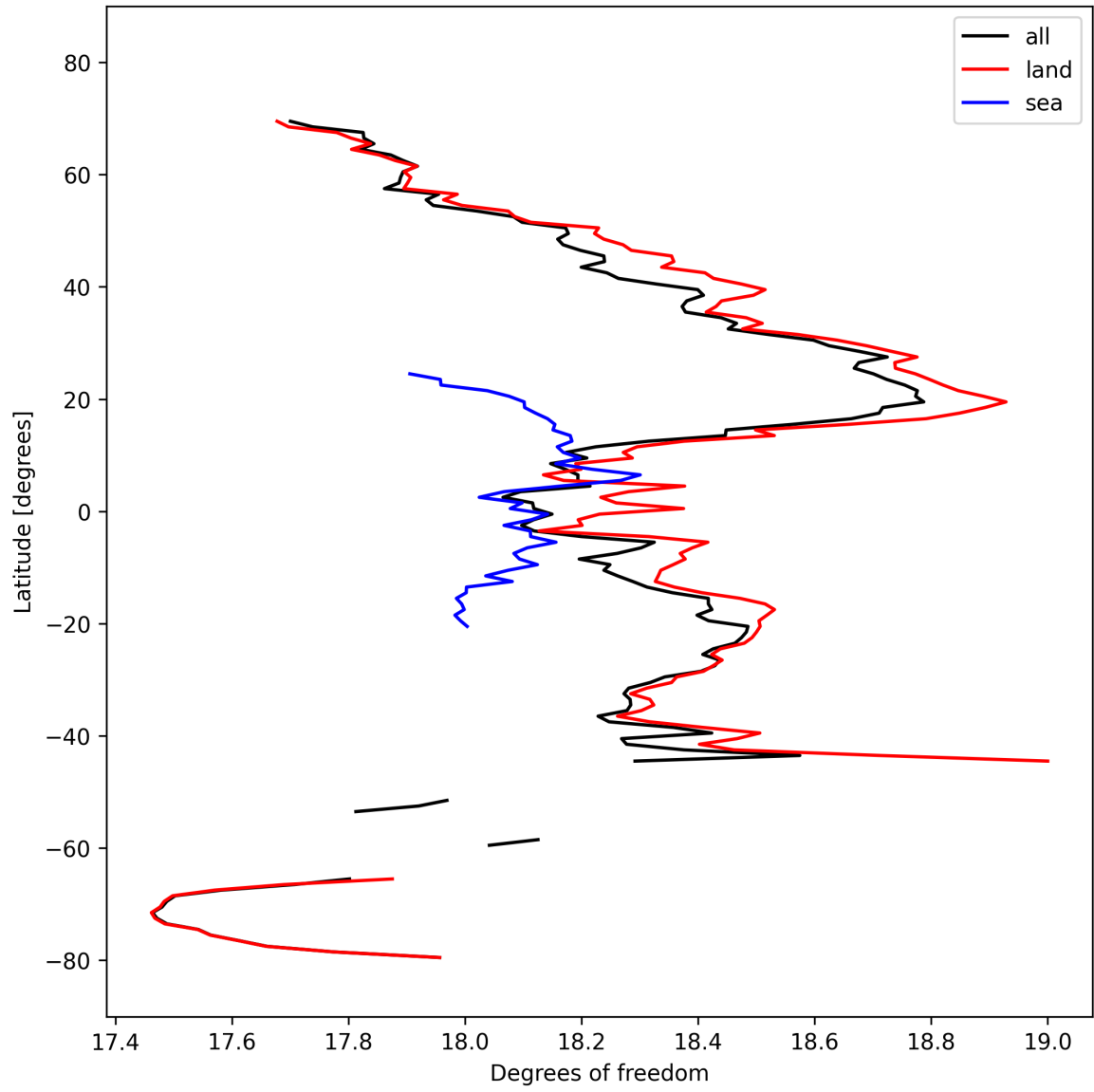
Figure 19: Zonal average of “Degrees of freedom” for 2025-10-06 to 2025-10-07.
