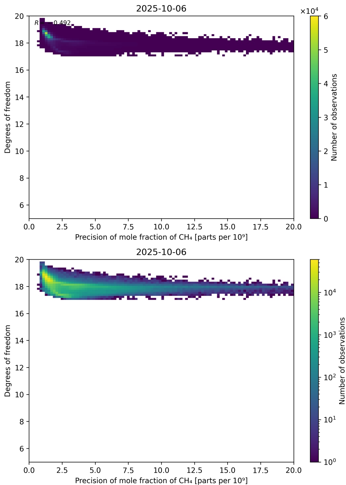
Figure 80: Scatter density plot of “Precision of mole fraction of CH 4 ” against “Degrees of freedom” for 2025-10-06 to 2025-10-07.
