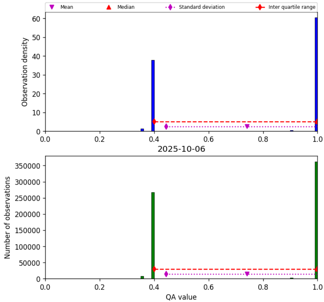
Figure 22: Histogram of “QA value” for 2025-10-06 to 2025-10-07
