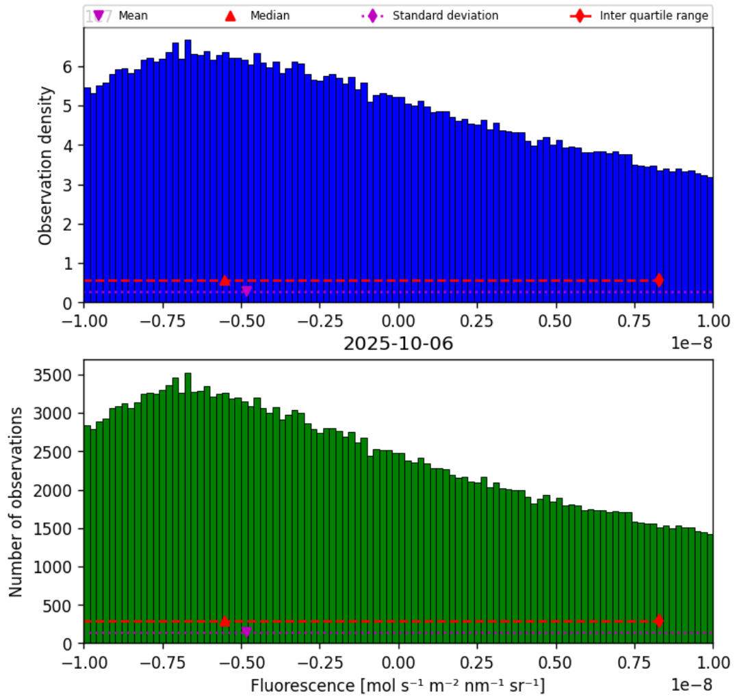
Figure 32: Histogram of “Fluorescence” for 2025-10-06 to 2025-10-07
