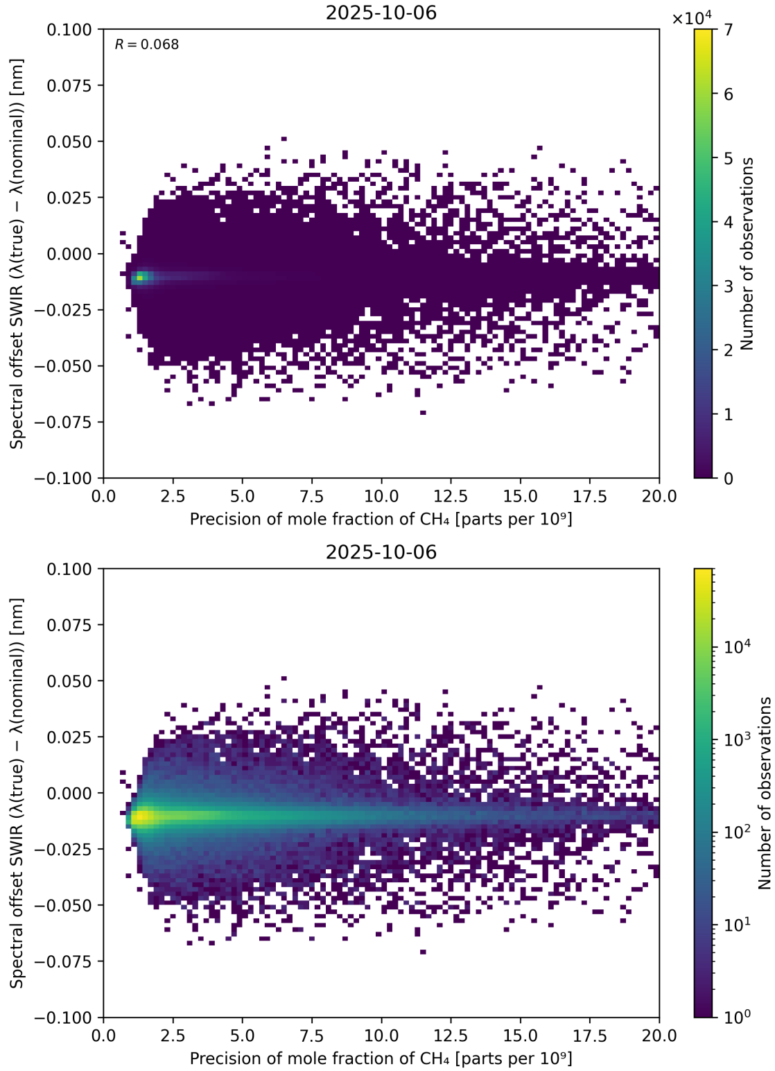
Figure 85: Scatter density plot of “Precision of mole fraction of \text{CH}_4 ” against “Spectral offset SWIR ( \lambda_{\text{true}} - \lambda_{\text{nominal}} )” for 2025-10-06 to 2025-10-07.
