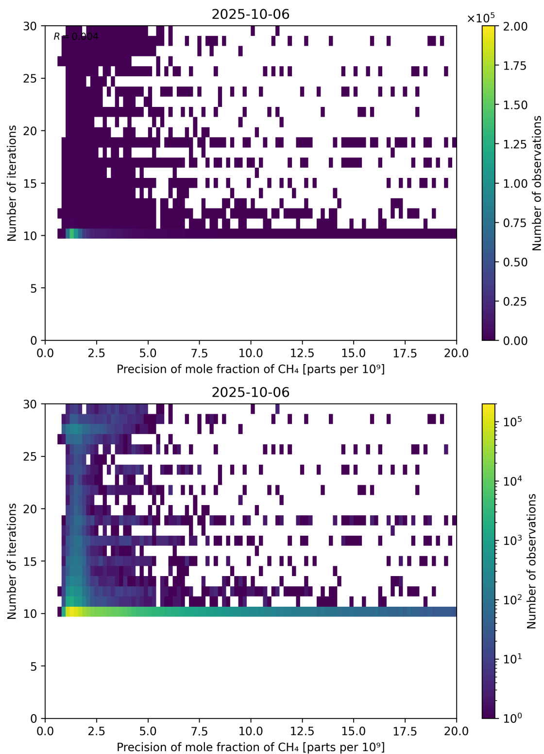
Figure 83: Scatter density plot of “Precision of mole fraction of \text{CH}_4 ” against “Number of iterations” for 2025-10-06 to 2025-10-07.
