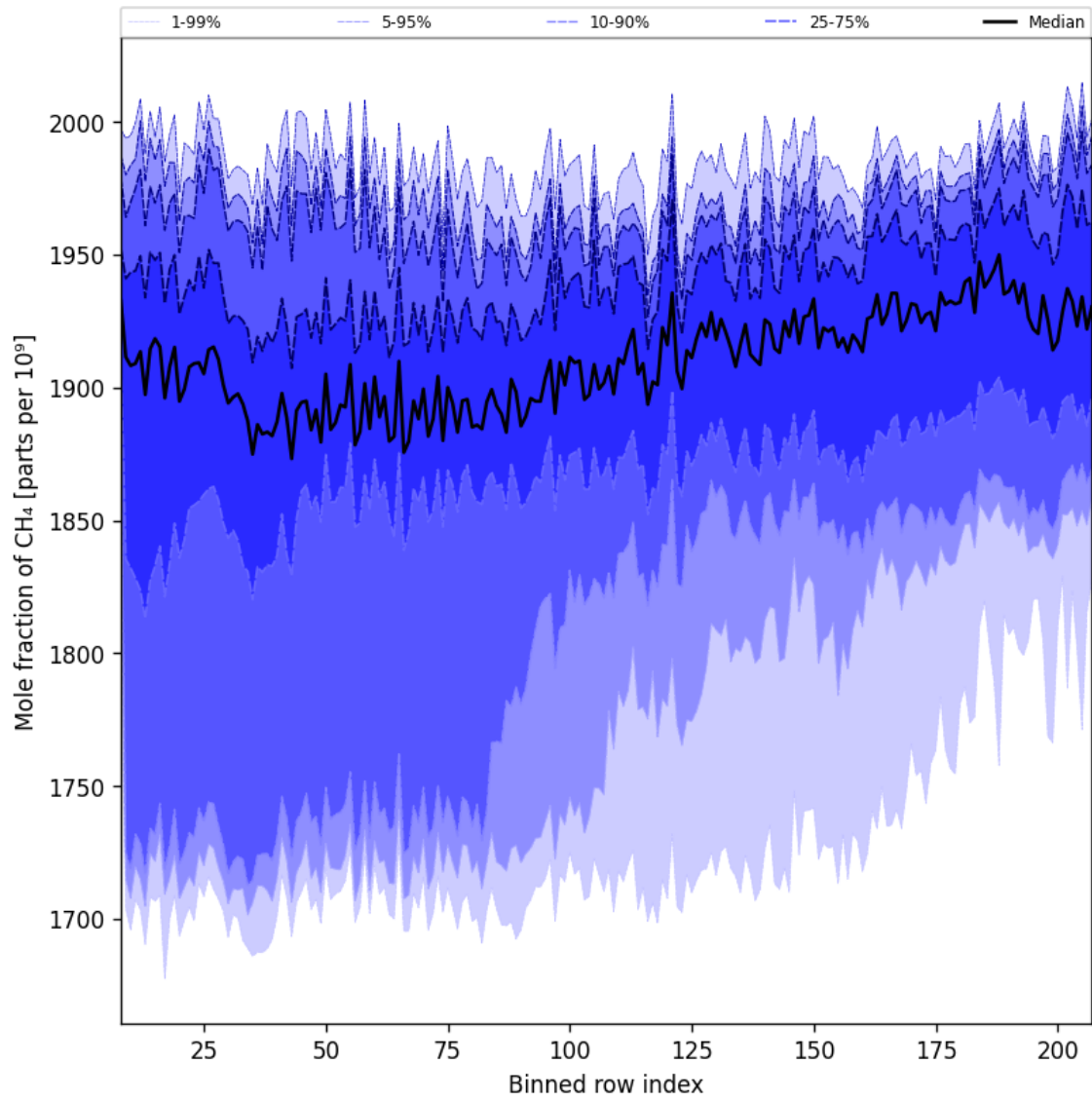
Figure 34: Along track statistics of “Mole fraction of CH 4 ” for 2025-10-06 to 2025-10-07
