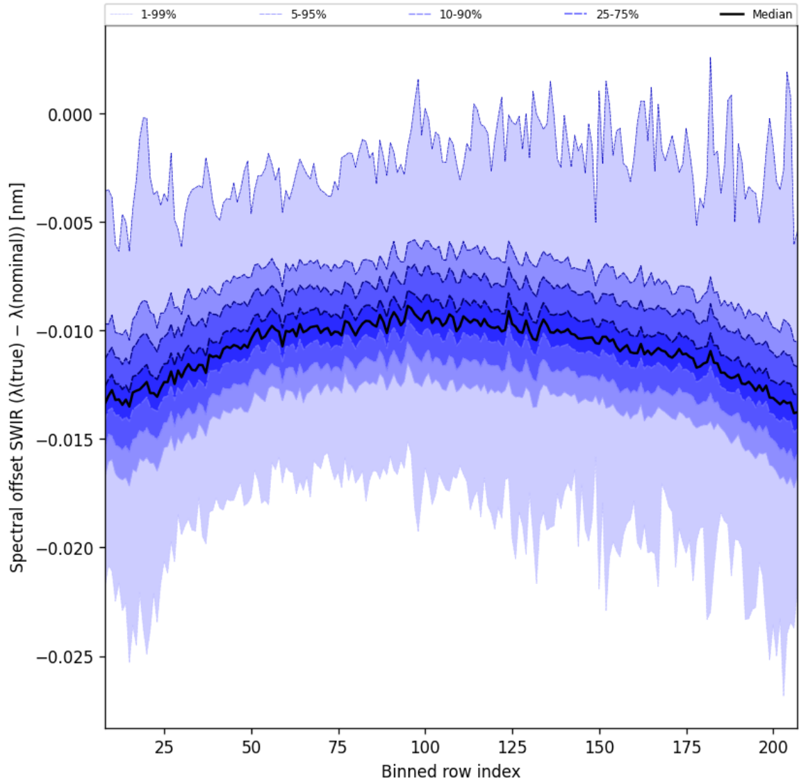
Figure 38: Along track statistics of “Spectral offset SWIR ( \lambda_{\text{true}} - \lambda_{\text{nominal}} )” for 2025-10-06 to 2025-10-07
