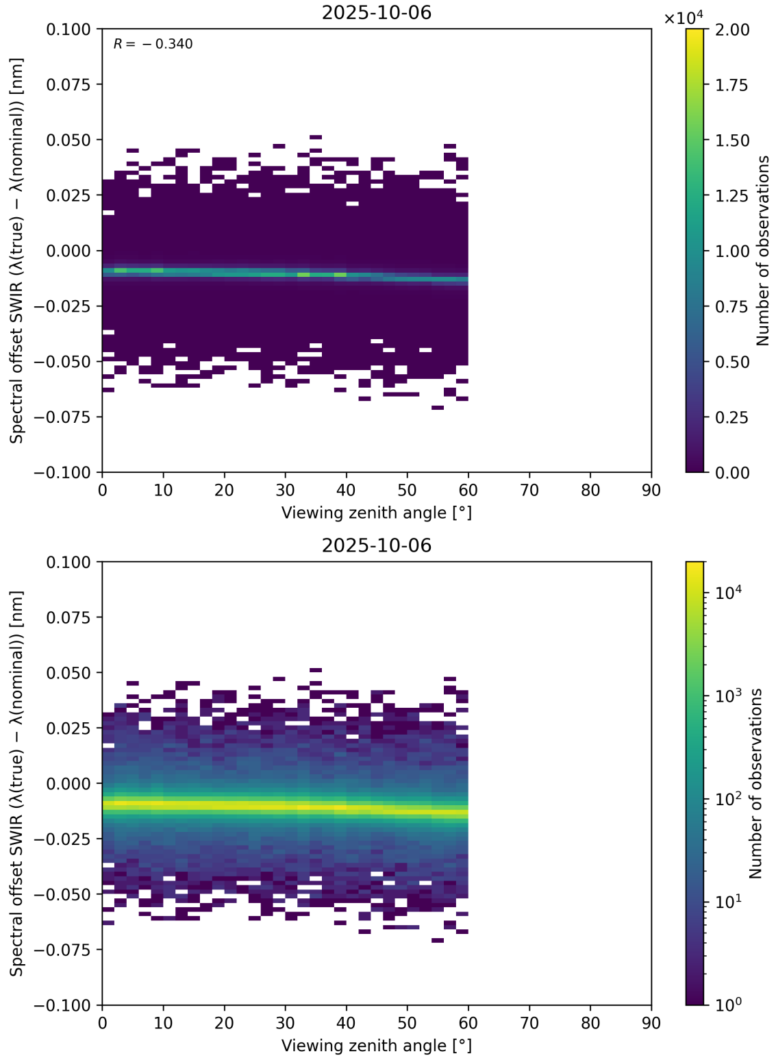
Figure 116: Scatter density plot of “Viewing zenith angle” against “Spectral offset SWIR ( \lambda_{\text{true}} - \lambda_{\text{nominal}} )” for 2025-10-06 to 2025-10-07.
