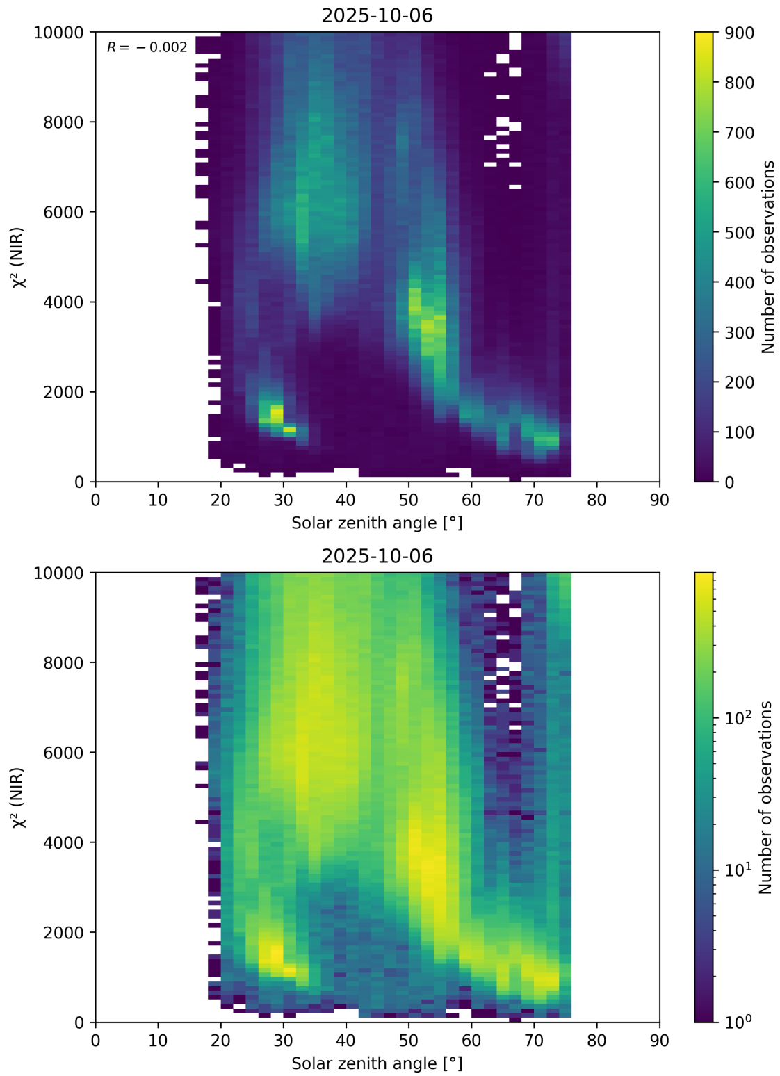
Figure 94: Scatter density plot of “Solar zenith angle” against “ \chi^2 (NIR)” for 2025-10-06 to 2025-10-07.
