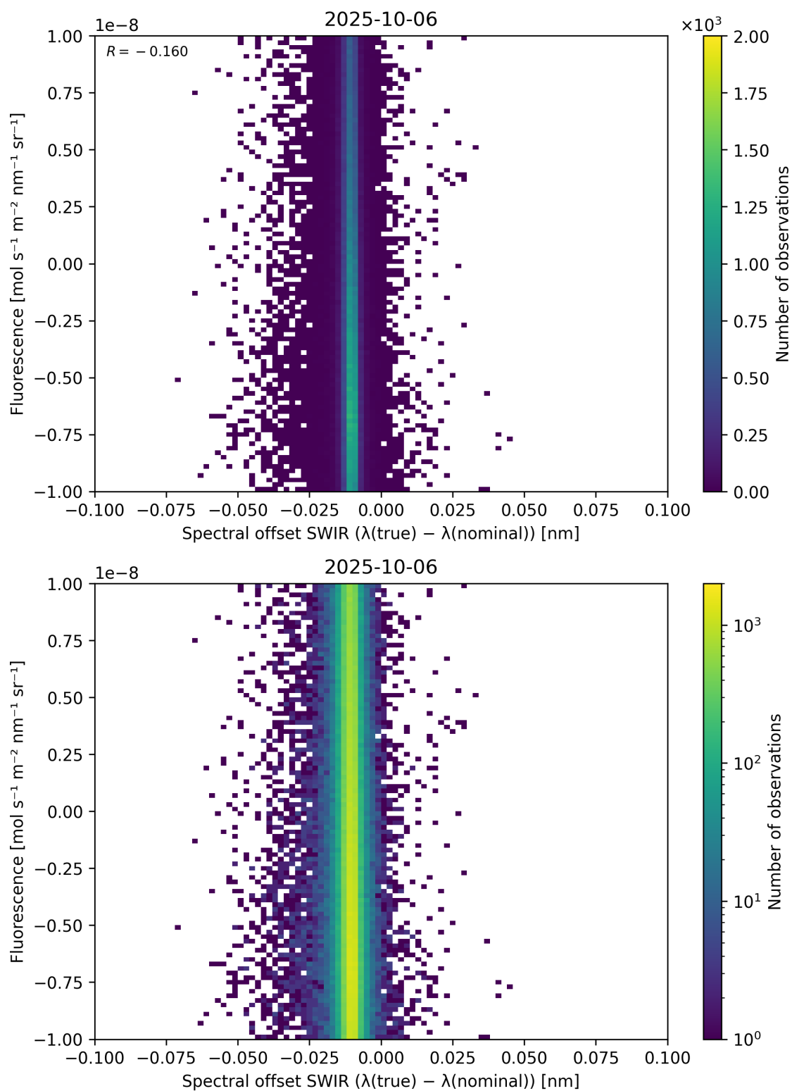
Figure 120: Scatter density plot of “Spectral offset SWIR ( \lambda_{\text{true}} - \lambda_{\text{nominal}} )” against “Fluorescence” for 2025-10-06 to 2025-10-07.
