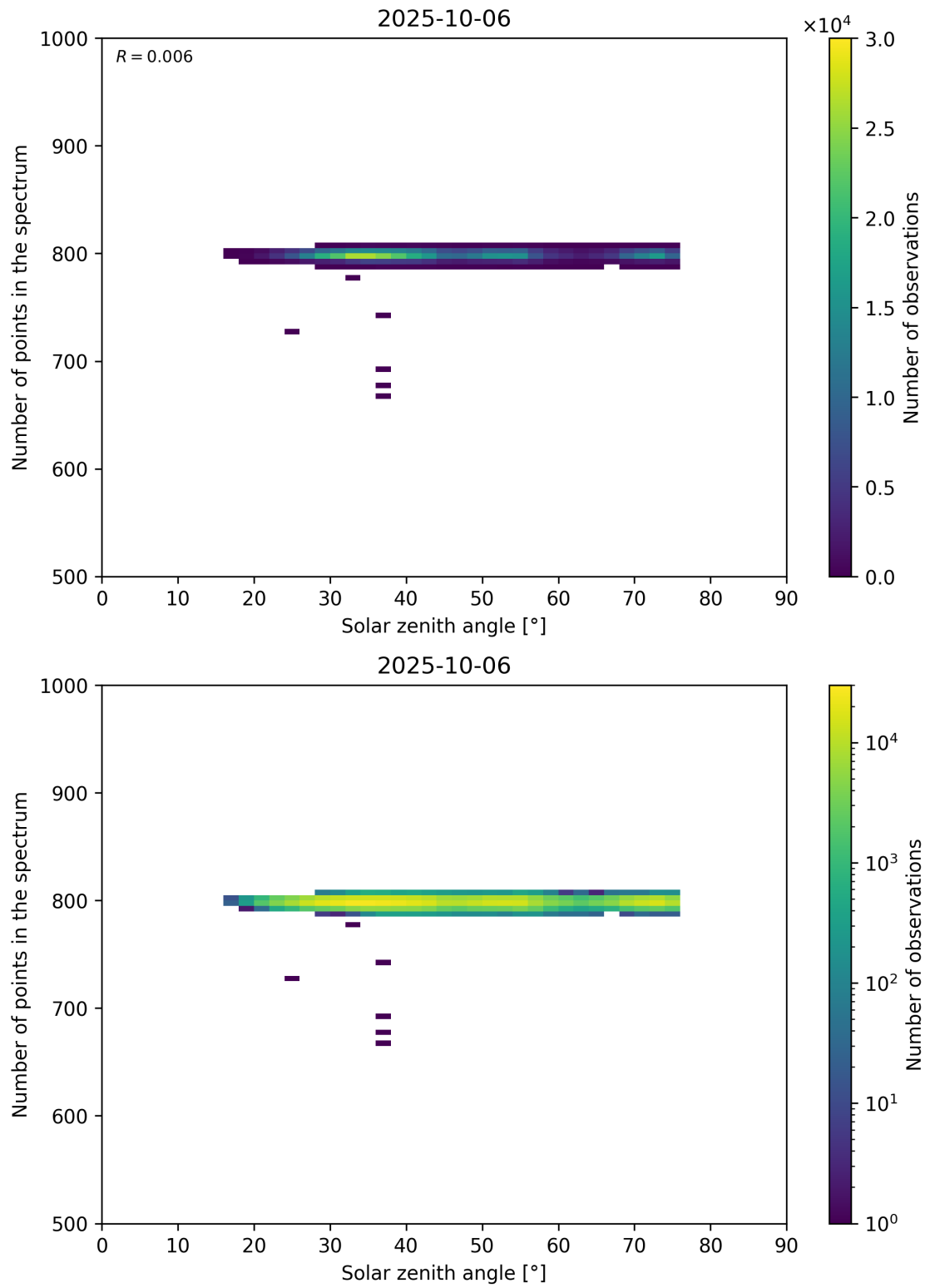
Figure 103: Scatter density plot of “Solar zenith angle” against “Number of points in the spectrum” for 2025-10-06 to 2025-10-07.
