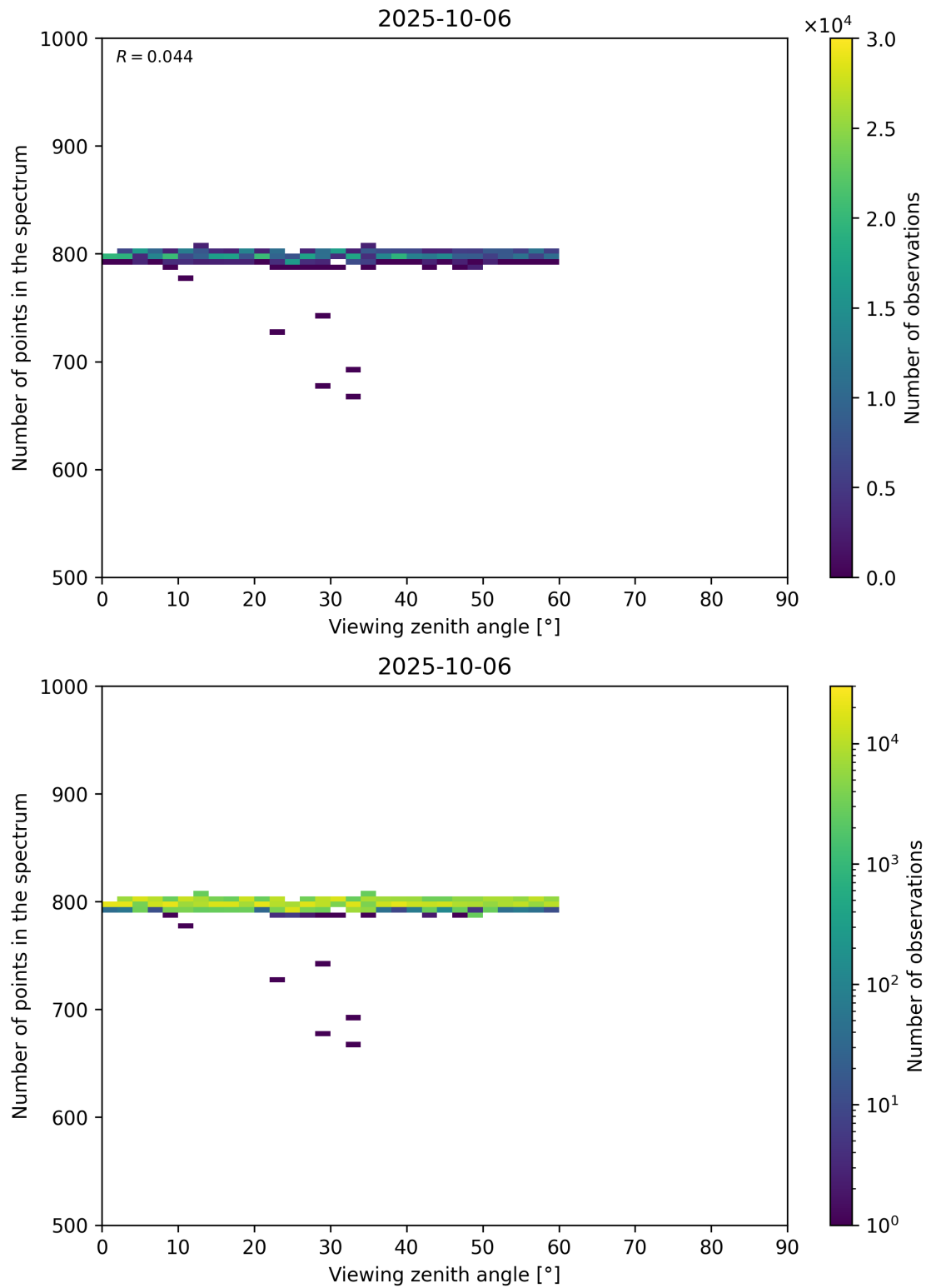
Figure 114: Scatter density plot of “Viewing zenith angle” against “Number of points in the spectrum” for 2025-10-06 to 2025-10-07.
