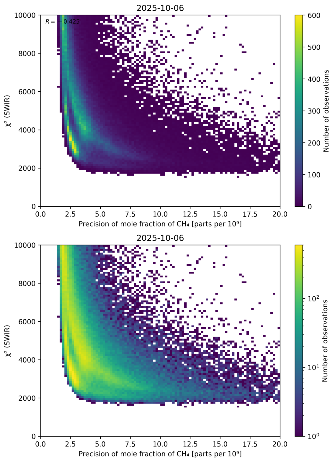
Figure 79: Scatter density plot of “Precision of mole fraction of CH 4 ” against “ \chi^2 (SWIR)” for 2025-10-06 to 2025-10-07.
