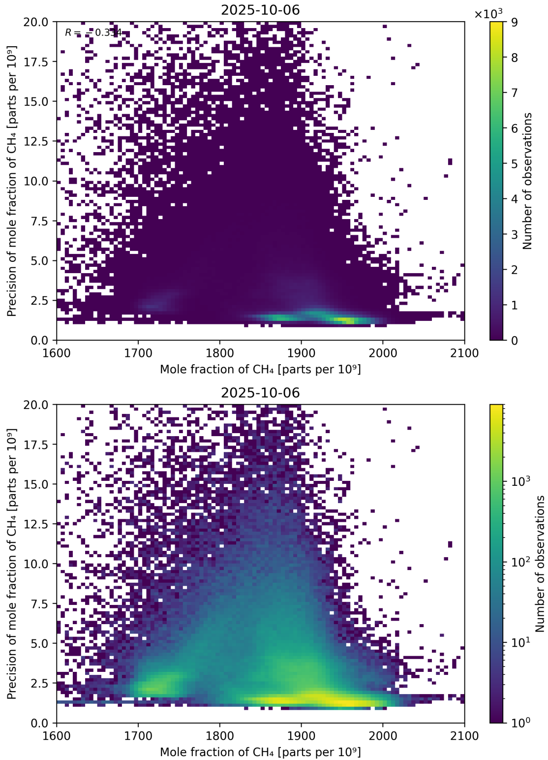
Figure 75: Scatter density plot of “Mole fraction of CH 4 ” against “Precision of mole fraction of CH 4 ” for 2025-10-06 to 2025-10-07.
