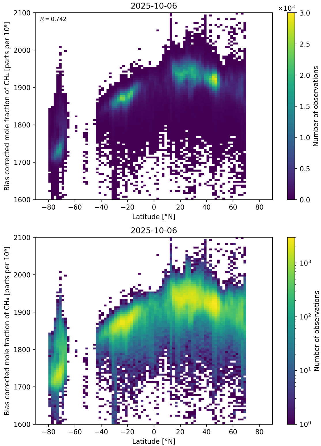
Figure 58: Scatter density plot of “Latitude” against “Bias corrected mole fraction of CH 4 ” for 2025-10-06 to 2025-10-07.
