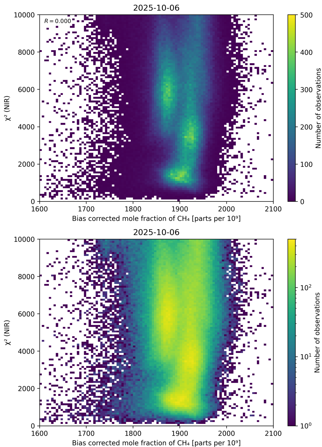
Figure 63: Scatter density plot of “Bias corrected mole fraction of CH 4 ” against “ \chi^2 (NIR)” for 2025-10-06 to 2025-10-07.
