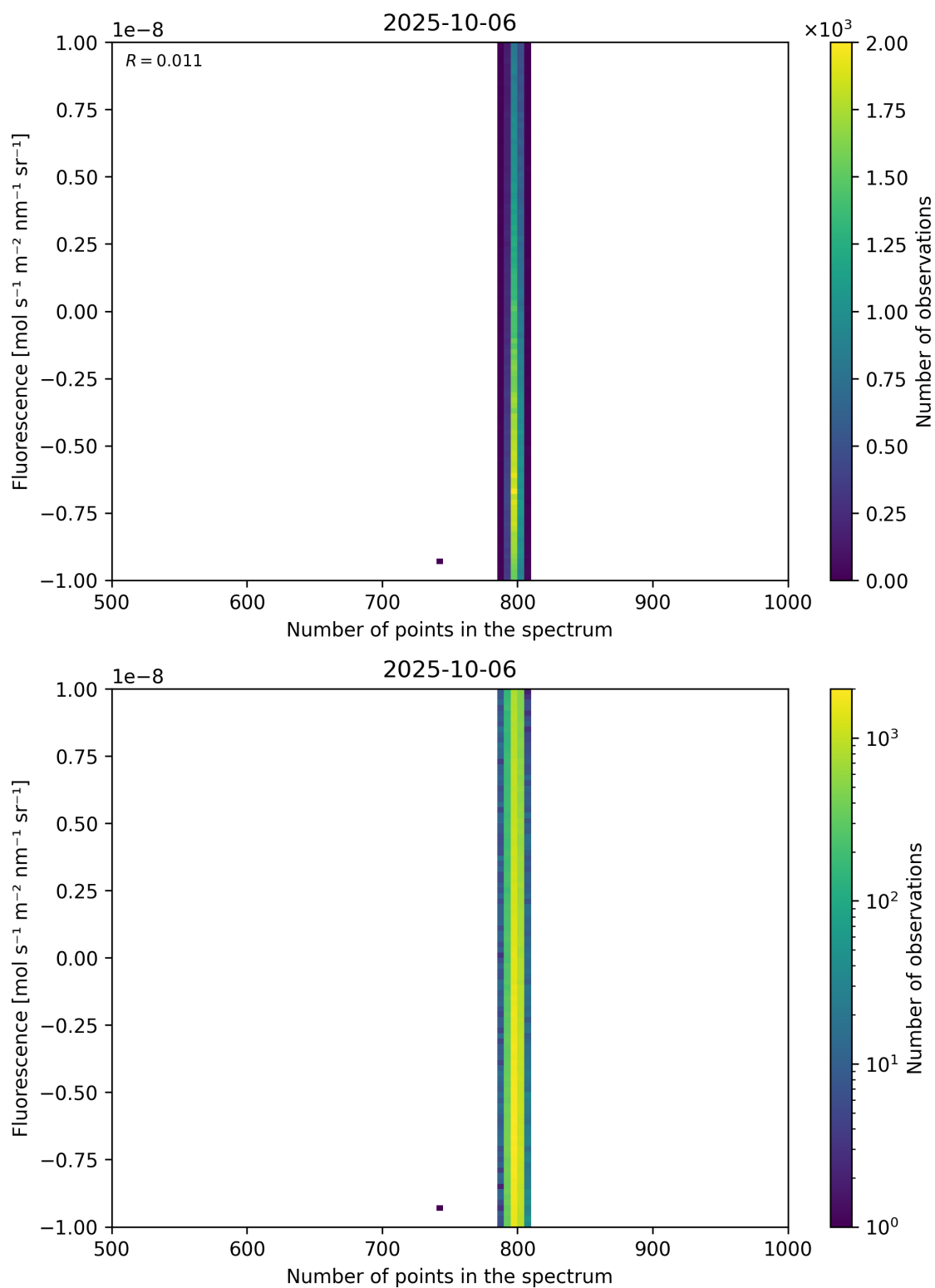
Figure 91: Scatter density plot of “Number of points in the spectrum” against “Fluorescence” for 2025-10-06 to 2025-10-07.
