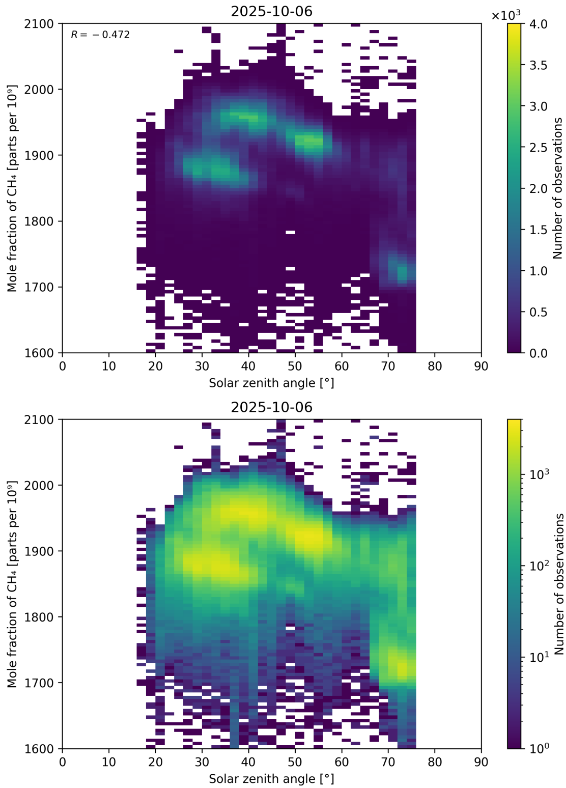
Figure 99: Scatter density plot of “Solar zenith angle” against “Mole fraction of CH 4 ” for 2025-10-06 to 2025-10-07.
