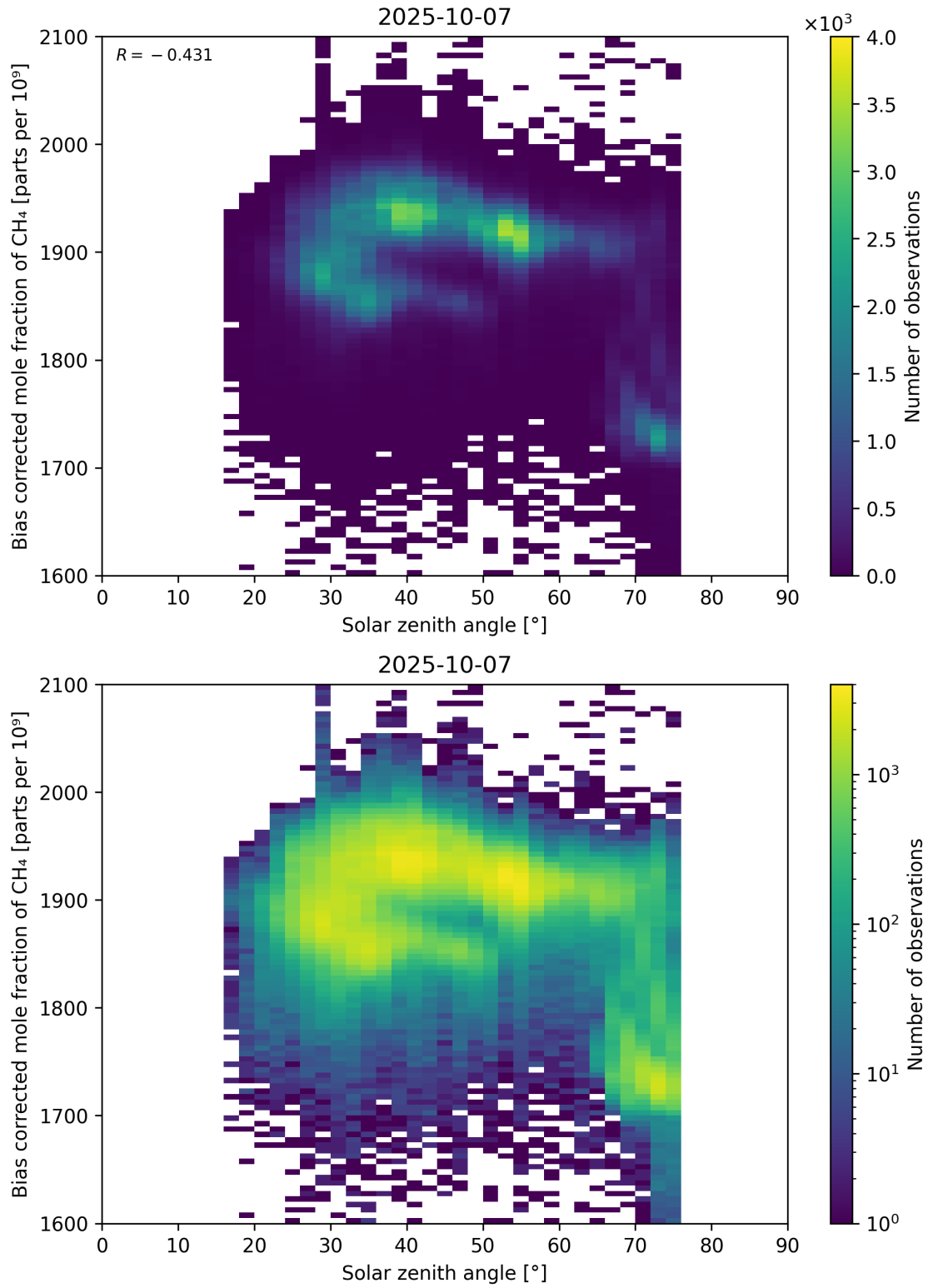
Figure 100: Scatter density plot of “Solar zenith angle” against “Bias corrected mole fraction of CH 4 ” for 2025-10-06 to 2025-10-08.
