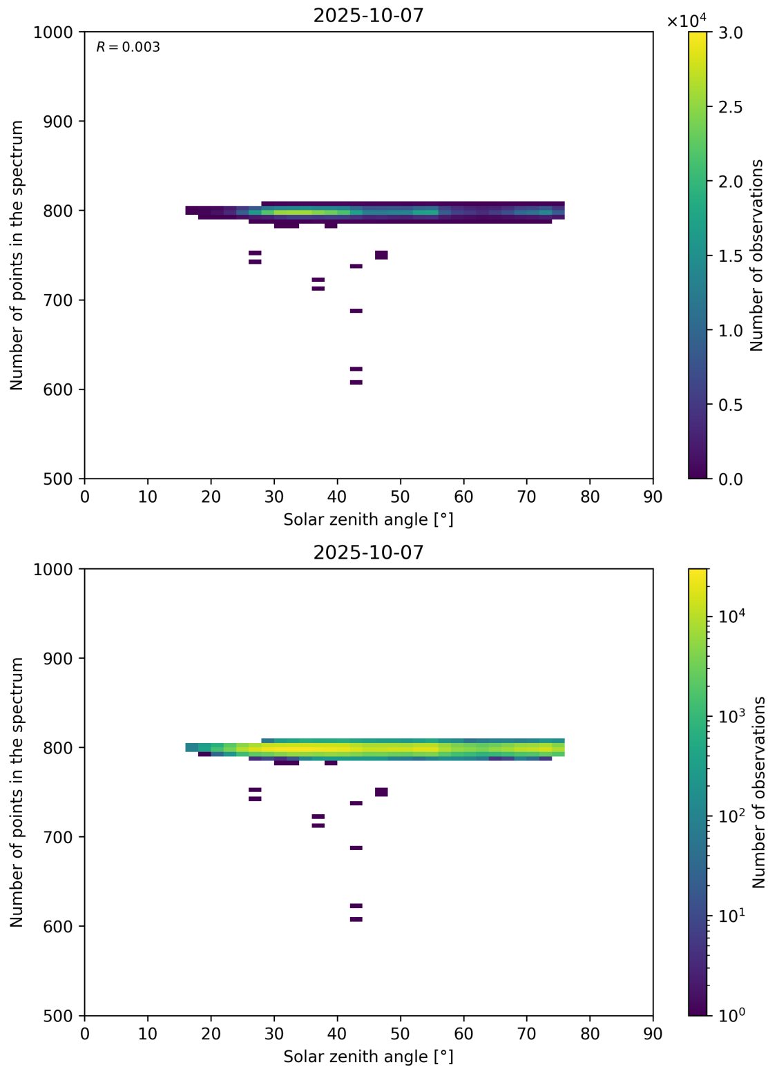
Figure 103: Scatter density plot of “Solar zenith angle” against “Number of points in the spectrum” for 2025-10-06 to 2025-10-08.
