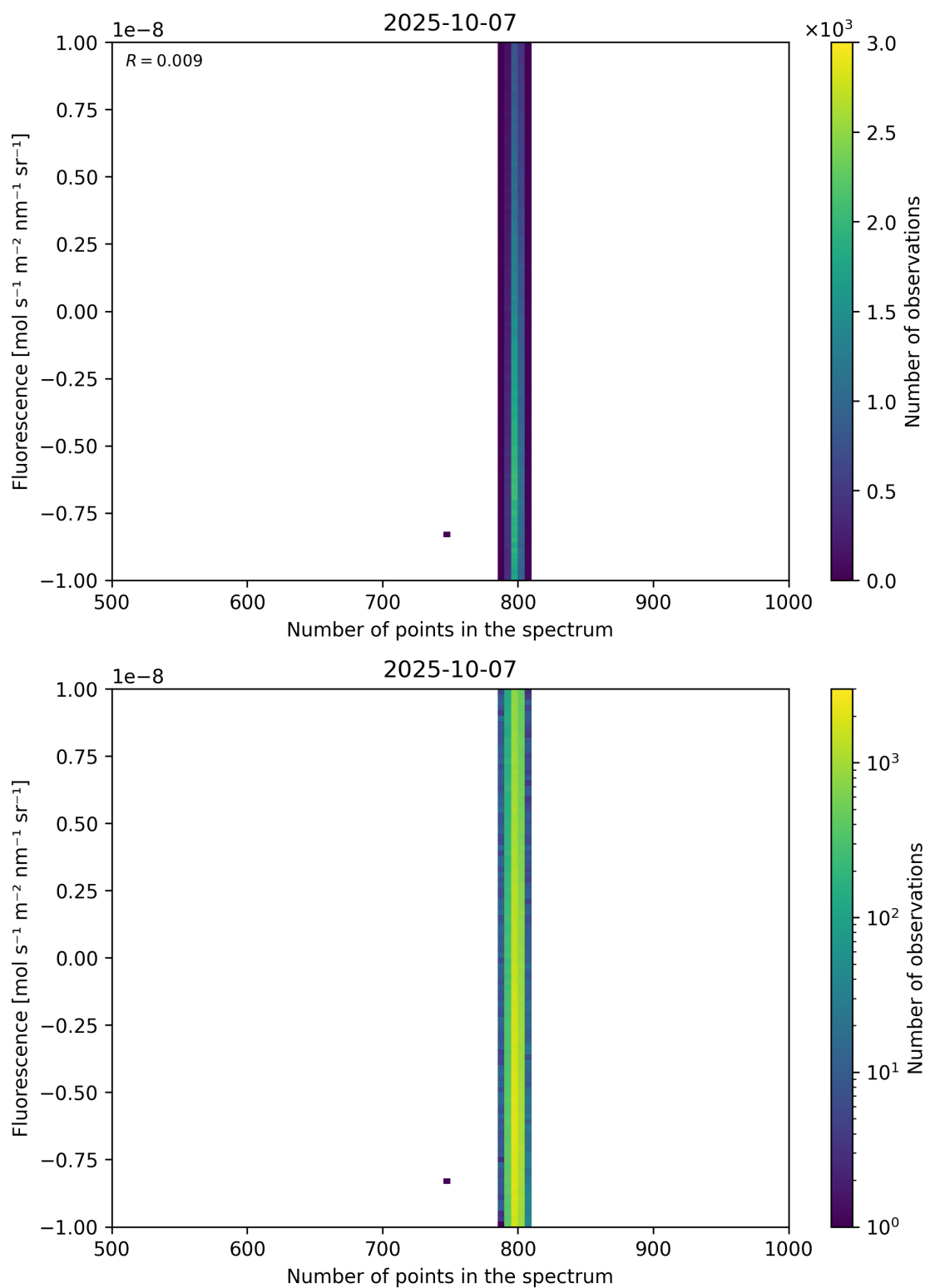
Figure 91: Scatter density plot of “Number of points in the spectrum” against “Fluorescence” for 2025-10-06 to 2025-10-08.
