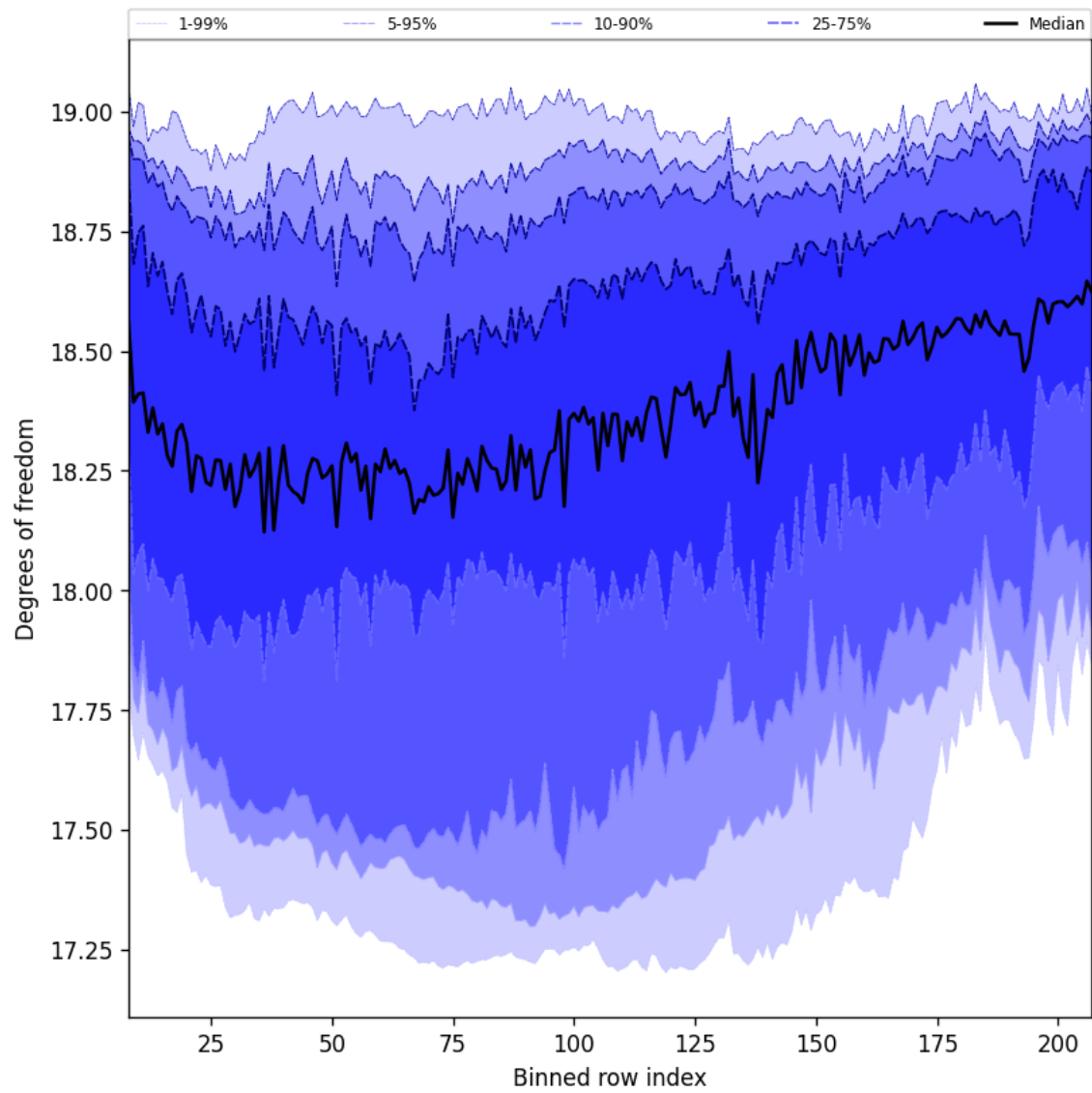
Figure 41: Along track statistics of “Degrees of freedom” for 2025-10-06 to 2025-10-08
