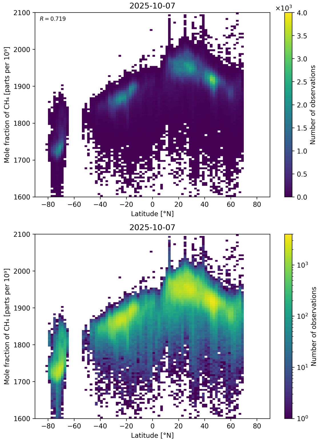
Figure 57: Scatter density plot of “Latitude” against “Mole fraction of CH 4 ” for 2025-10-06 to 2025-10-08.
