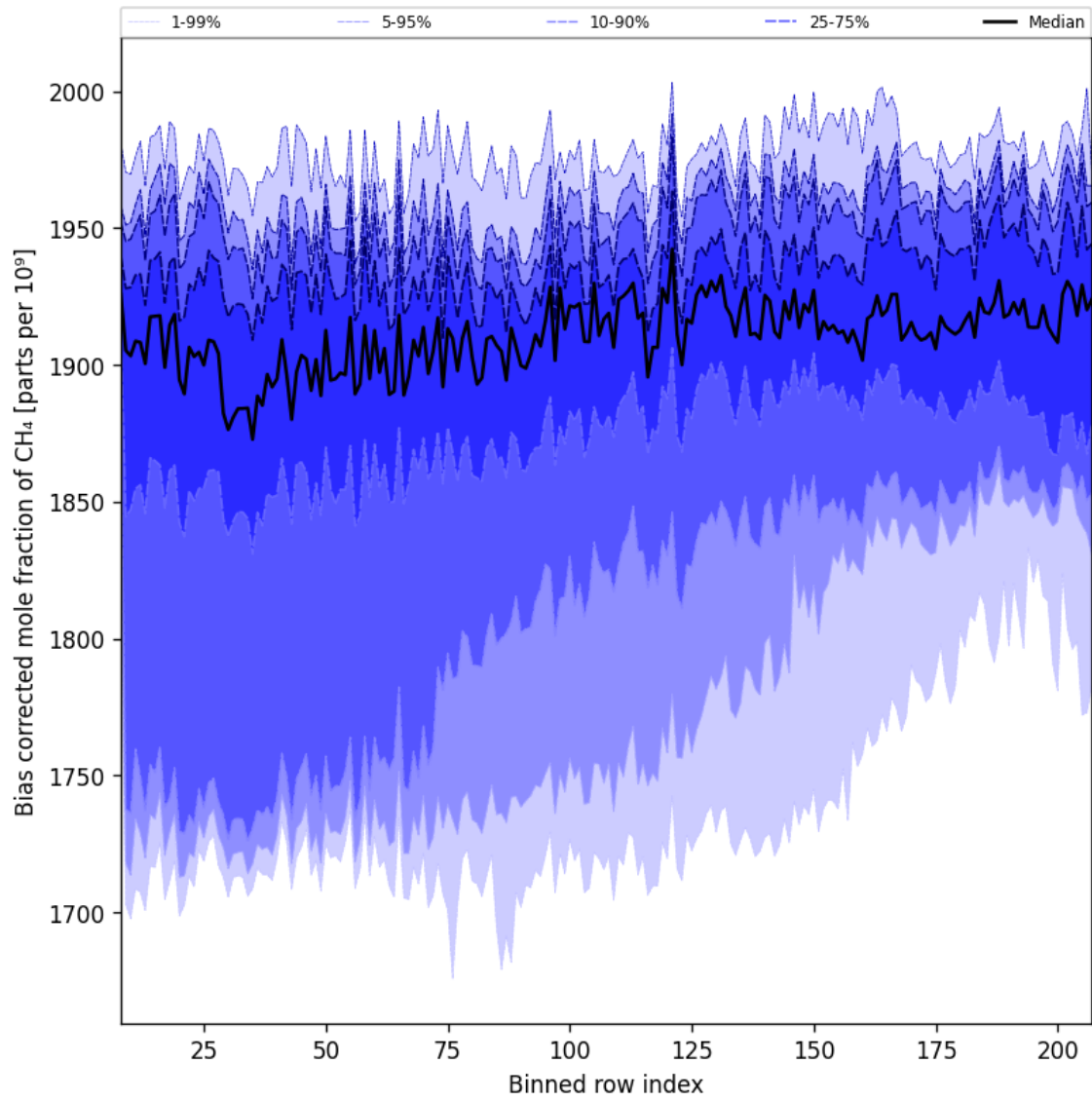
Figure 36: Along track statistics of “Bias corrected mole fraction of CH 4 ” for 2025-10-06 to 2025-10-08
