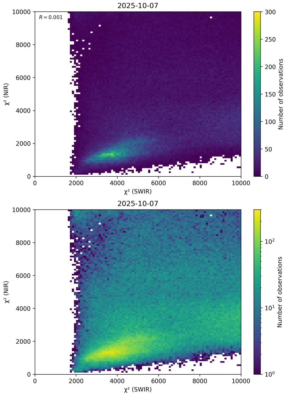
Figure 47: Scatter density plot of “ \chi^2 (SWIR)” against “ \chi^2 (NIR)” for 2025-10-06 to 2025-10-08.
