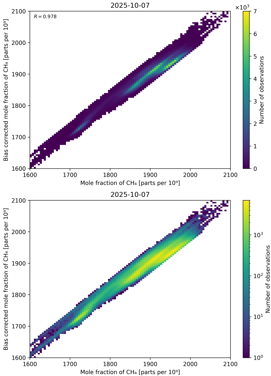
Figure 74: Scatter density plot of “Mole fraction of CH 4 ” against “Bias corrected mole fraction of CH 4 ” for 2025-10-06 to 2025-10-08.
