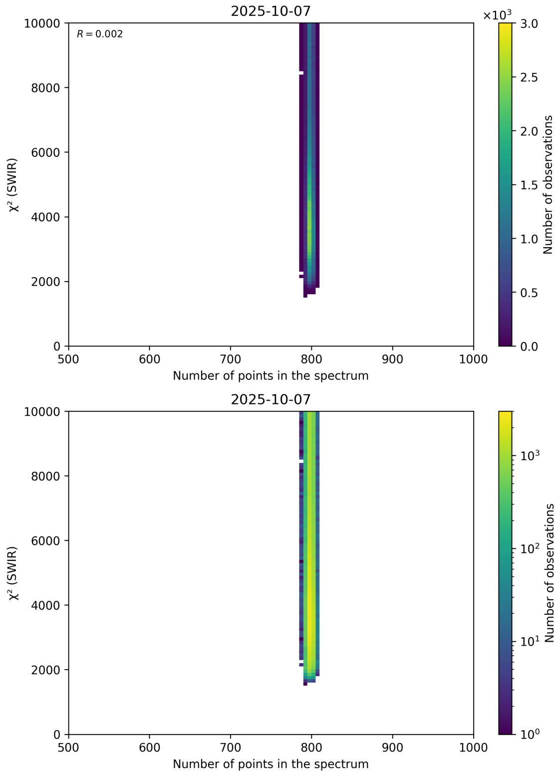
Figure 89: Scatter density plot of “Number of points in the spectrum” against “ \chi^2 (SWIR)” for 2025-10-06 to 2025-10-08.
