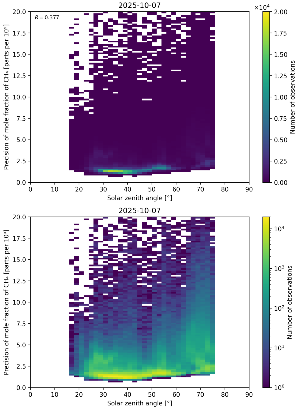
Figure 101: Scatter density plot of “Solar zenith angle” against “Precision of mole fraction of \text{CH}_4 ” for 2025-10-06 to 2025-10-08.
