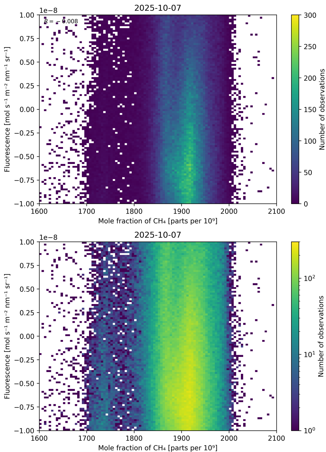
Figure 73: Scatter density plot of “Mole fraction of \text{CH}_4 ” against “Fluorescence” for 2025-10-06 to 2025-10-08.
