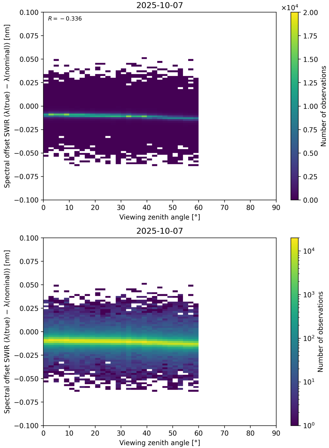
Figure 116: Scatter density plot of “Viewing zenith angle” against “Spectral offset SWIR ( \lambda_{\text{true}} - \lambda_{\text{nominal}} )” for 2025-10-06 to 2025-10-08.
