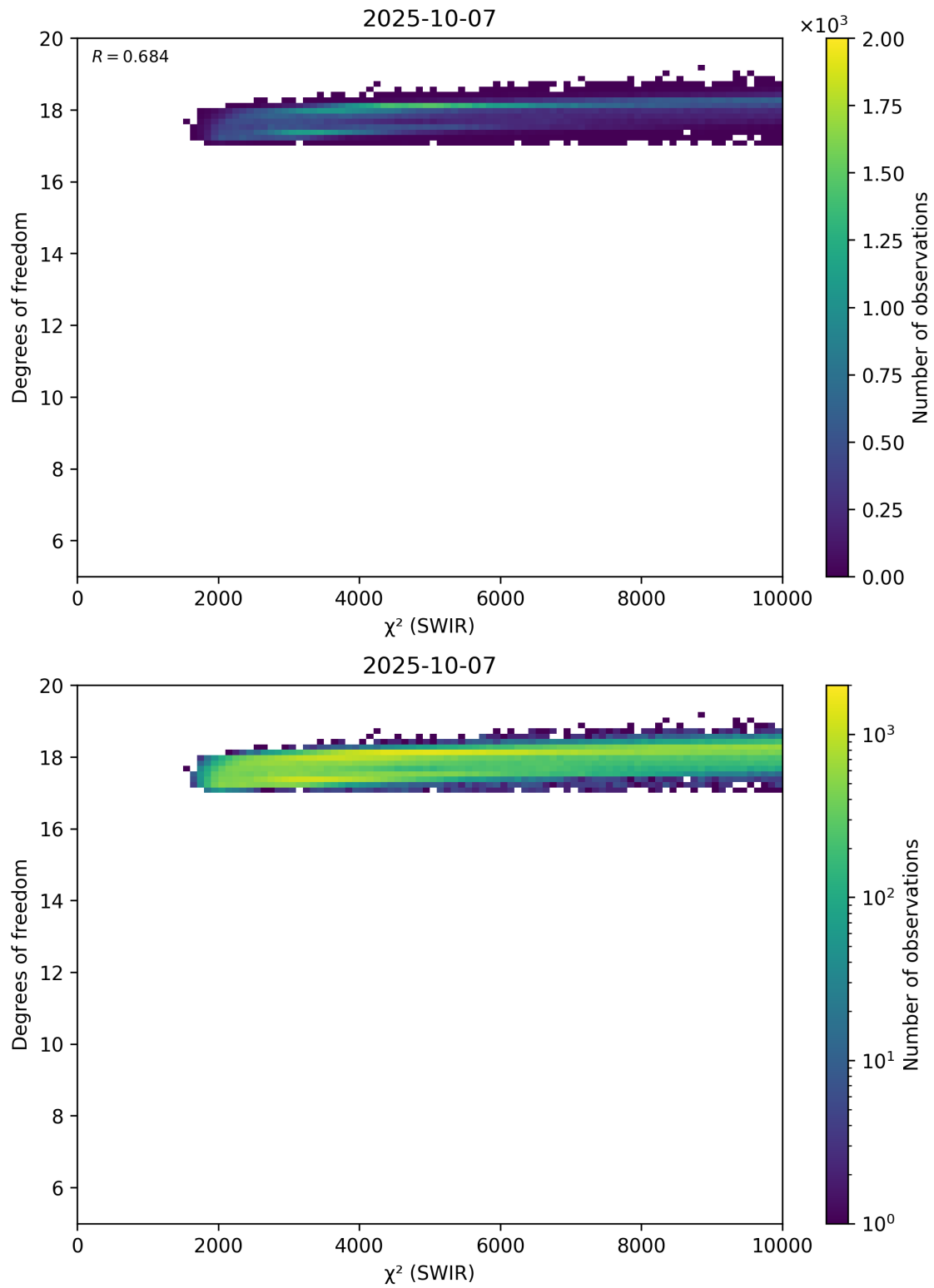
Figure 48: Scatter density plot of “ \chi^2 (SWIR)” against “Degrees of freedom” for 2025-10-06 to 2025-10-08.
