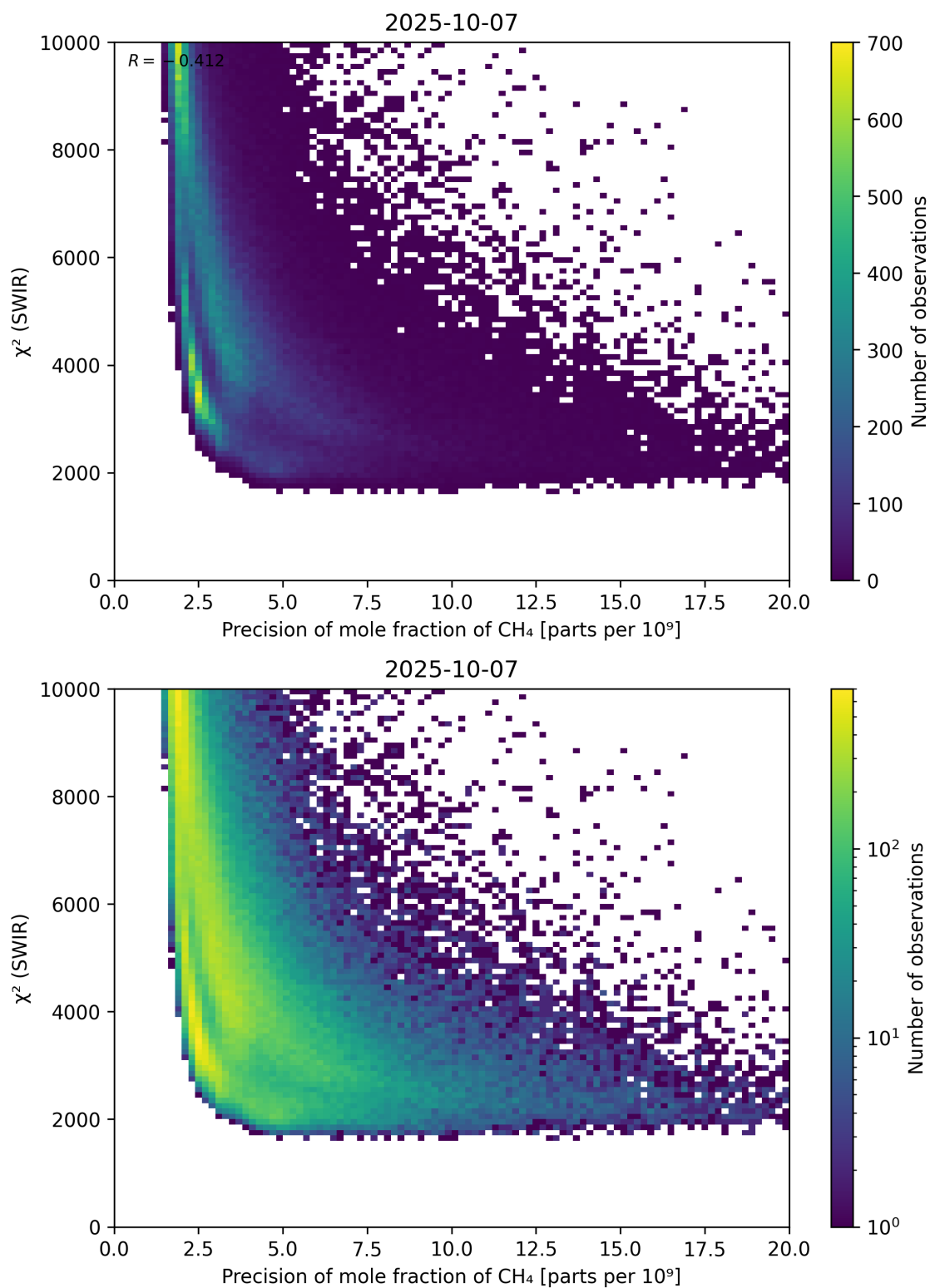
Figure 79: Scatter density plot of “Precision of mole fraction of CH 4 ” against “ \chi^2 (SWIR)” for 2025-10-06 to 2025-10-08.
