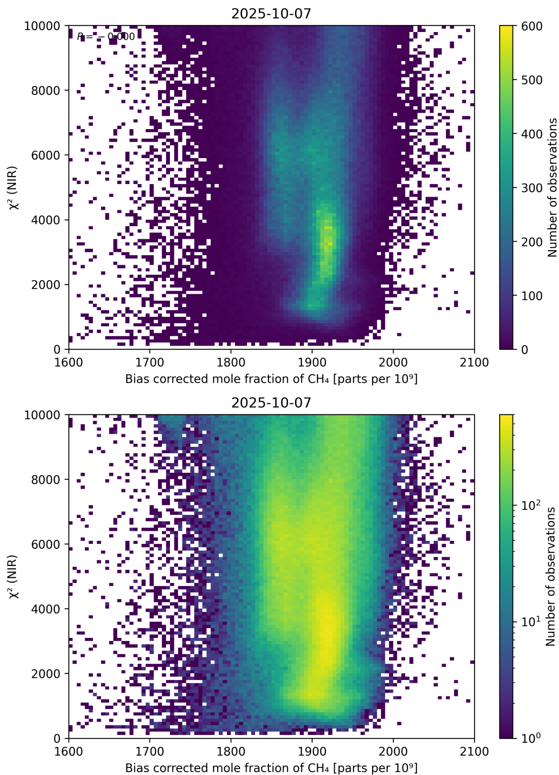
Figure 63: Scatter density plot of “Bias corrected mole fraction of CH 4 ” against “ \chi^2 (NIR)” for 2025-10-06 to 2025-10-08.
