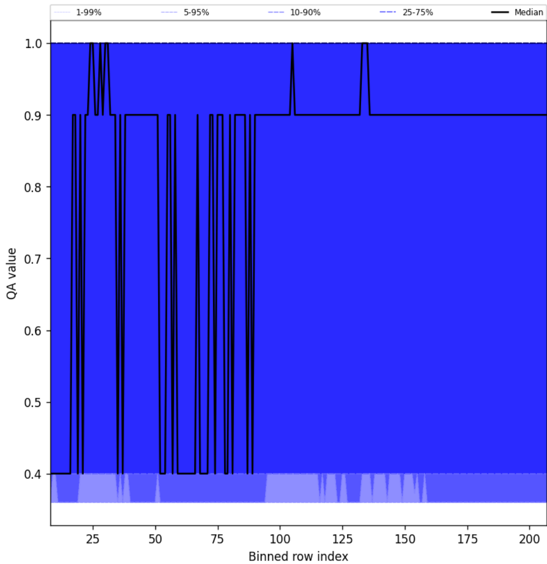
Figure 33: Along track statistics of “QA value” for 2025-10-06 to 2025-10-08
