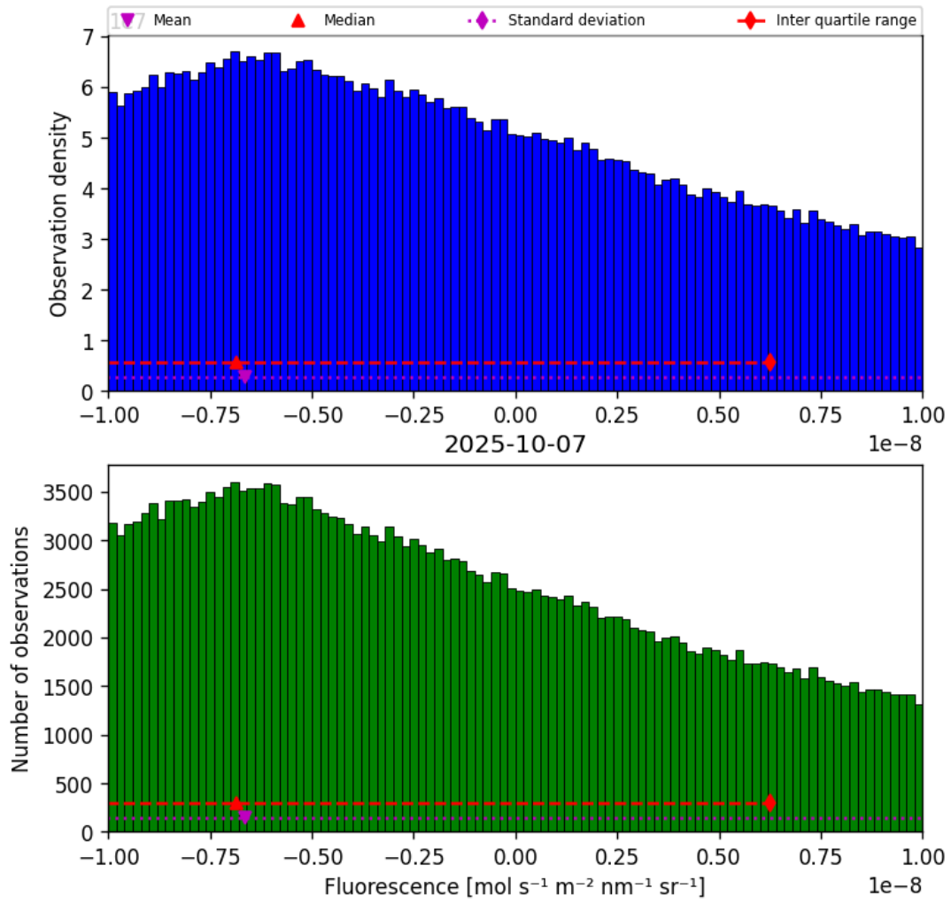
Figure 32: Histogram of “Fluorescence” for 2025-10-06 to 2025-10-08
