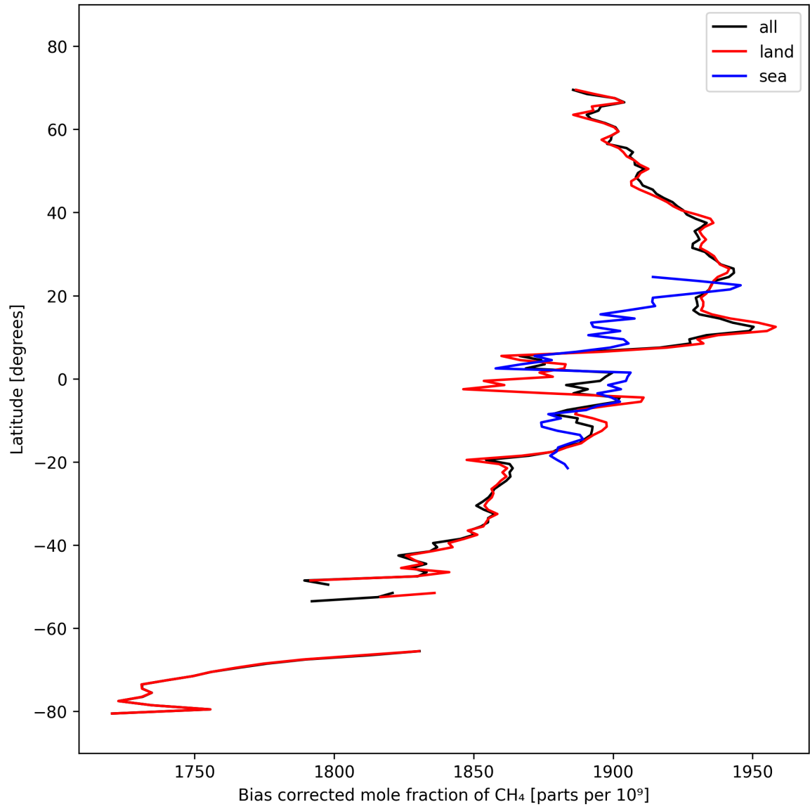
Figure 14: Zonal average of “Bias corrected mole fraction of CH 4 ” for 2025-10-06 to 2025-10-08.
