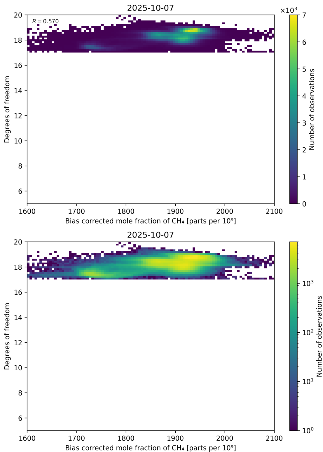
Figure 65: Scatter density plot of “Bias corrected mole fraction of CH 4 ” against “Degrees of freedom” for 2025-10-06 to 2025-10-08.
