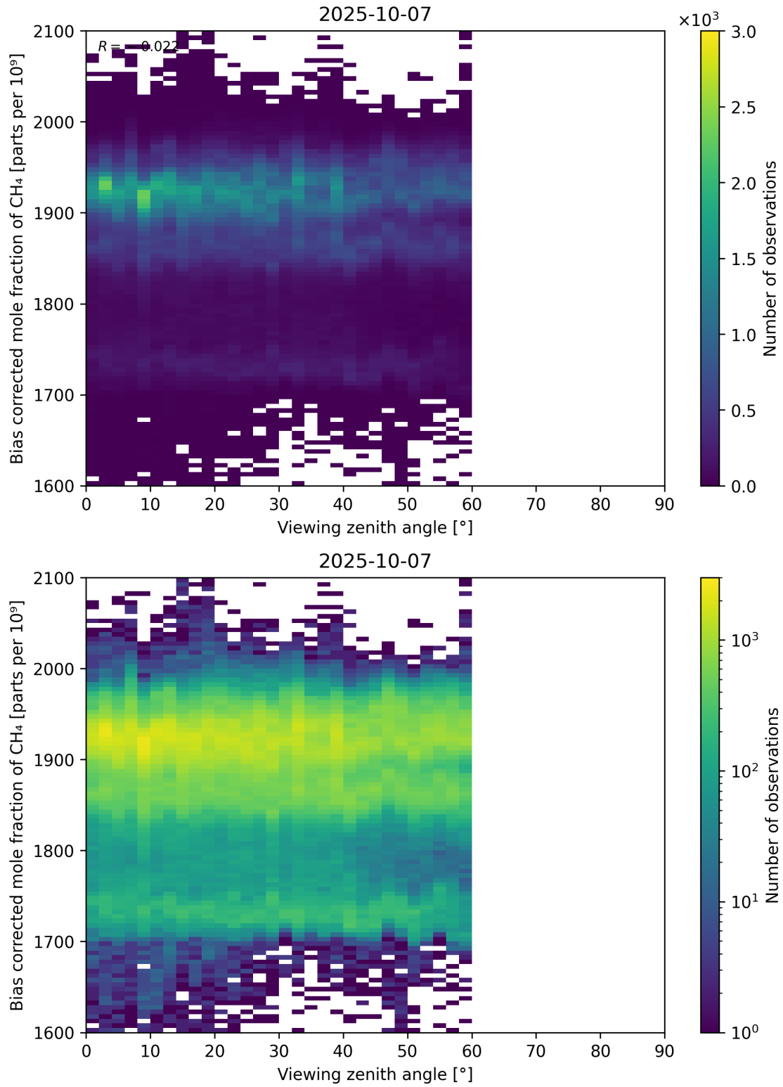
Figure 111: Scatter density plot of “Viewing zenith angle” against “Bias corrected mole fraction of CH 4 ” for 2025-10-06 to 2025-10-08.
