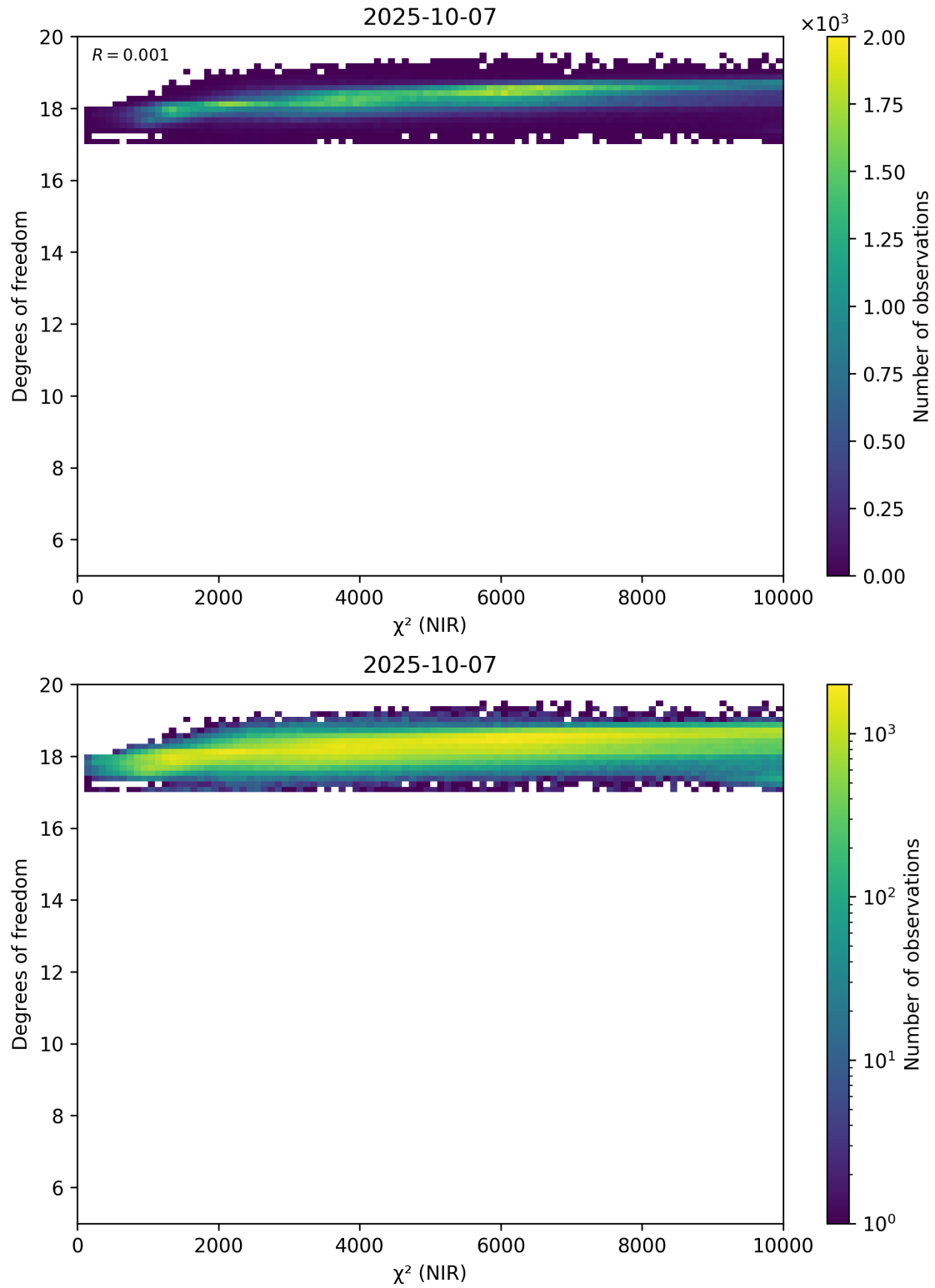
Figure 44: Scatter density plot of “ \chi^2 (NIR)” against “Degrees of freedom” for 2025-10-06 to 2025-10-08.
