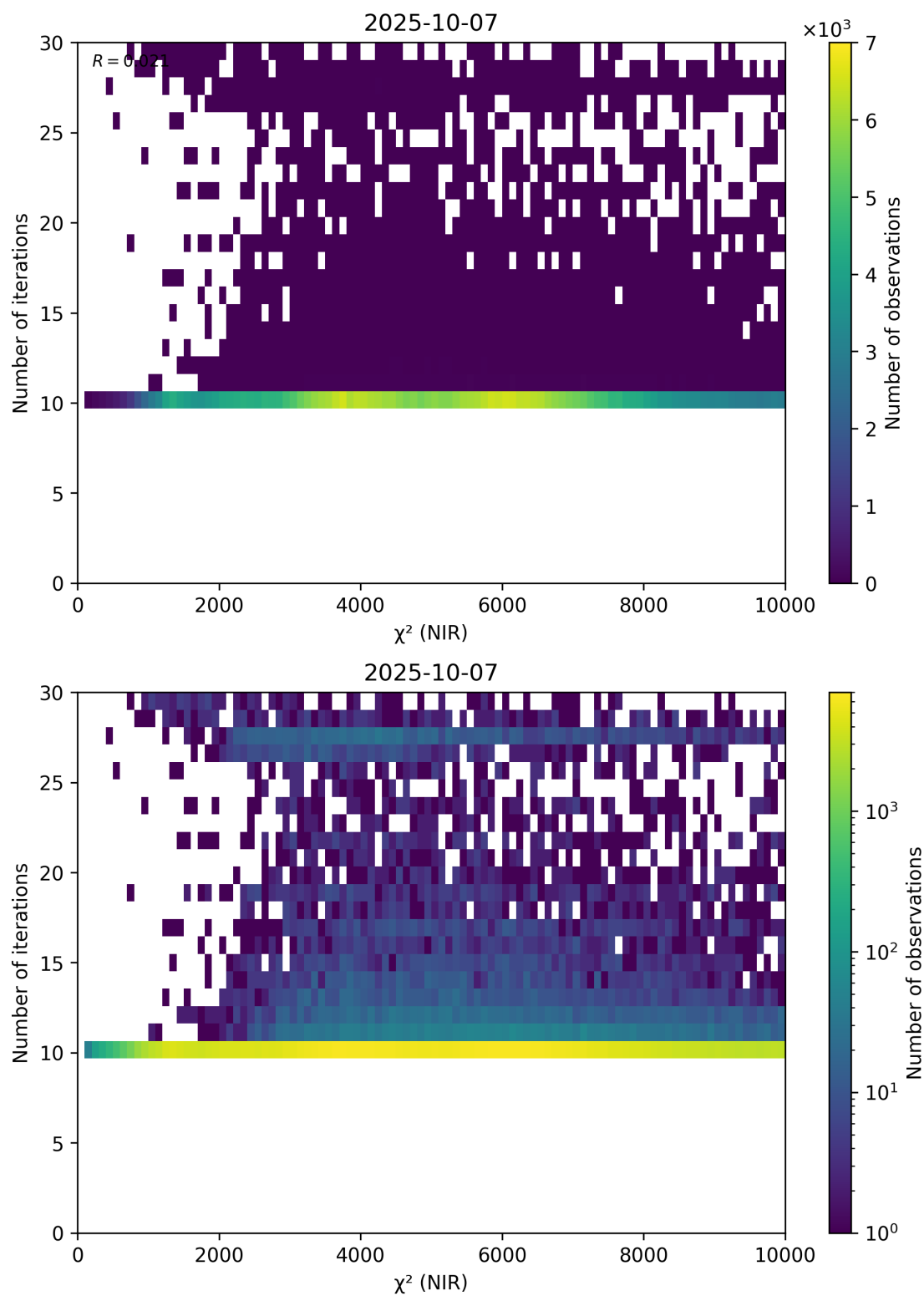
Figure 46: Scatter density plot of “ \chi^2 (NIR)” against “Number of iterations” for 2025-10-06 to 2025-10-08.
