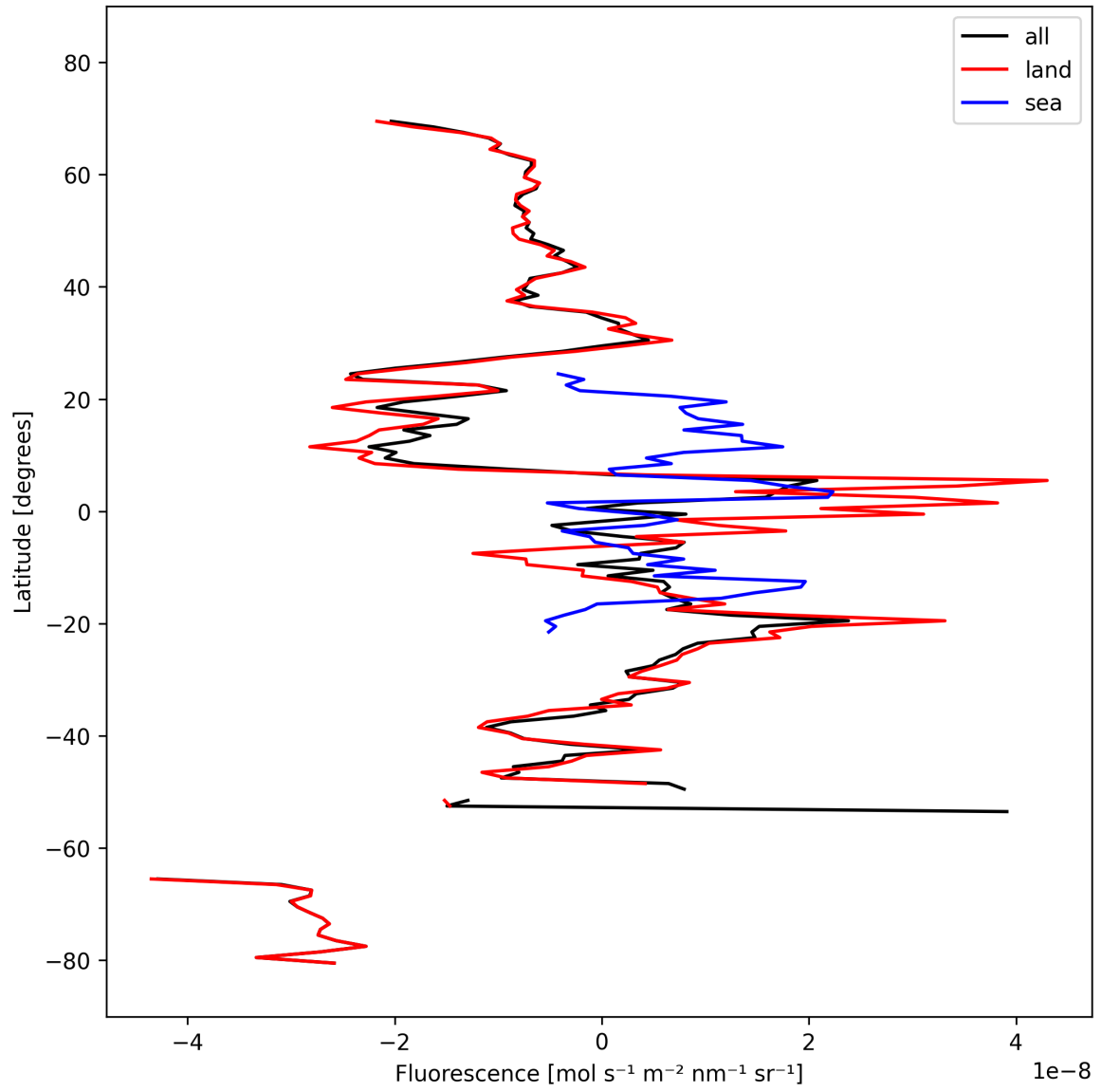
Figure 21: Zonal average of “Fluorescence” for 2025-10-06 to 2025-10-08.
