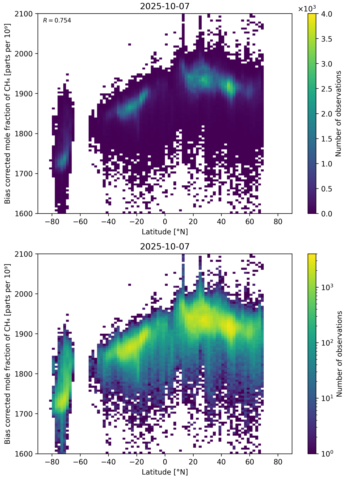
Figure 58: Scatter density plot of “Latitude” against “Bias corrected mole fraction of CH 4 ” for 2025-10-06 to 2025-10-08.
