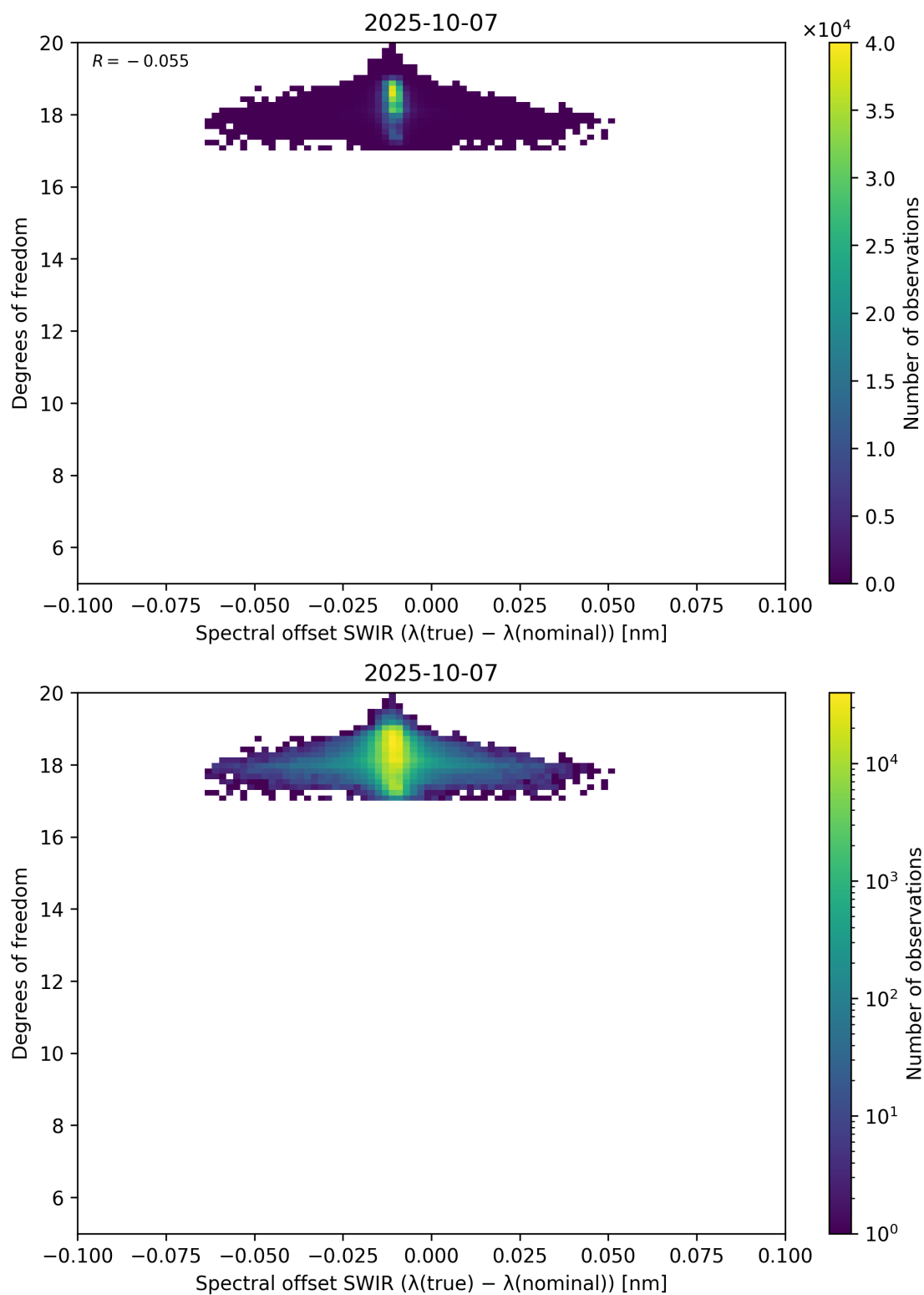
Figure 119: Scatter density plot of “Spectral offset SWIR ( \lambda_{\text{true}} - \lambda_{\text{nominal}} )” against “Degrees of freedom” for 2025-10-06 to 2025-10-08.
