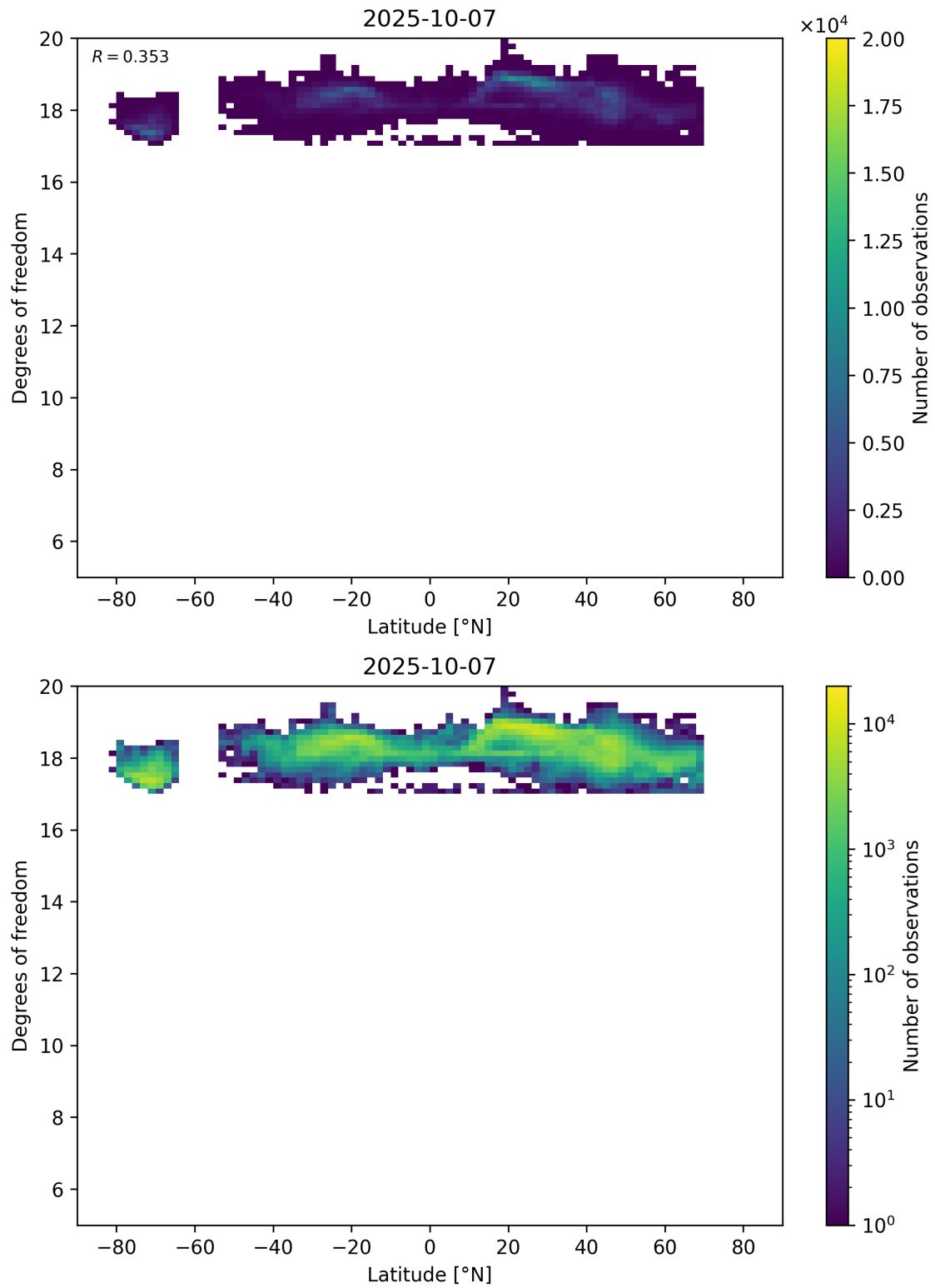
Figure 55: Scatter density plot of “Latitude” against “Degrees of freedom” for 2025-10-06 to 2025-10-08.
