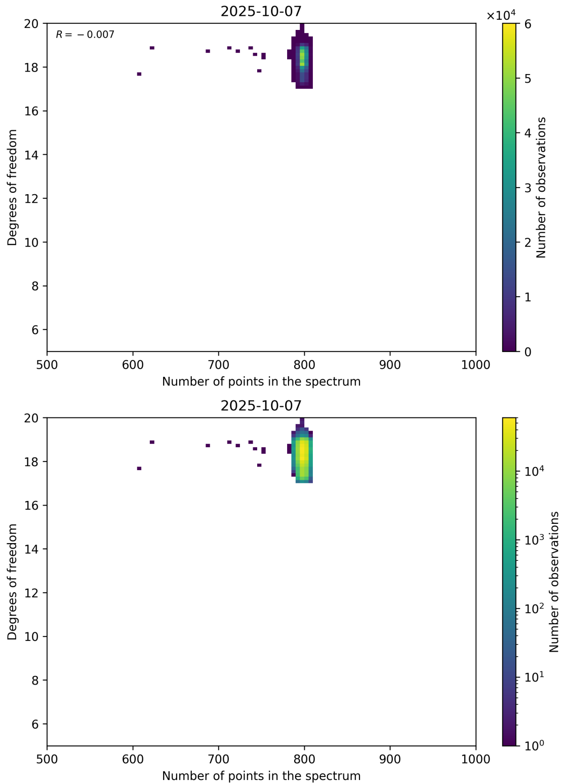
Figure 90: Scatter density plot of “Number of points in the spectrum” against “Degrees of freedom” for 2025-10-06 to 2025-10-08.
