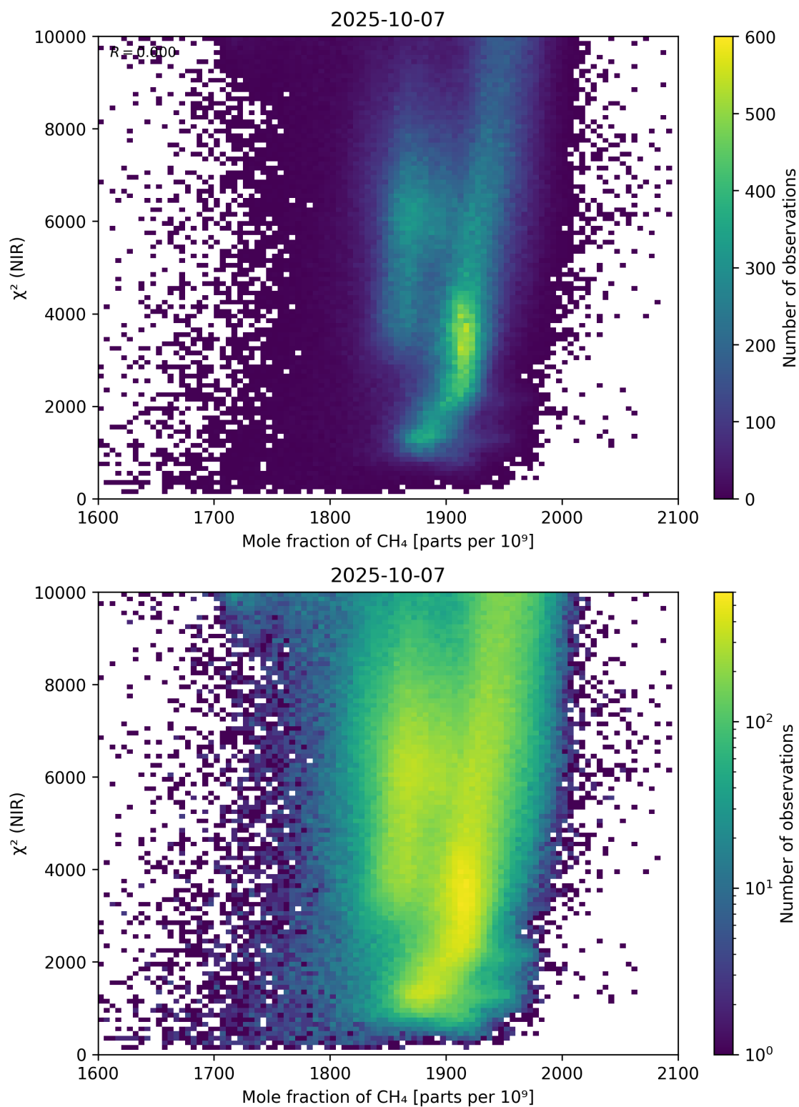
Figure 70: Scatter density plot of “Mole fraction of \text{CH}_4 ” against “ \chi^2 (NIR)” for 2025-10-06 to 2025-10-08.
