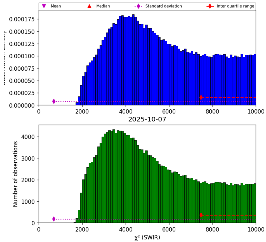
Figure 28: Histogram of “ \chi^2 (SWIR)” for 2025-10-06 to 2025-10-08
