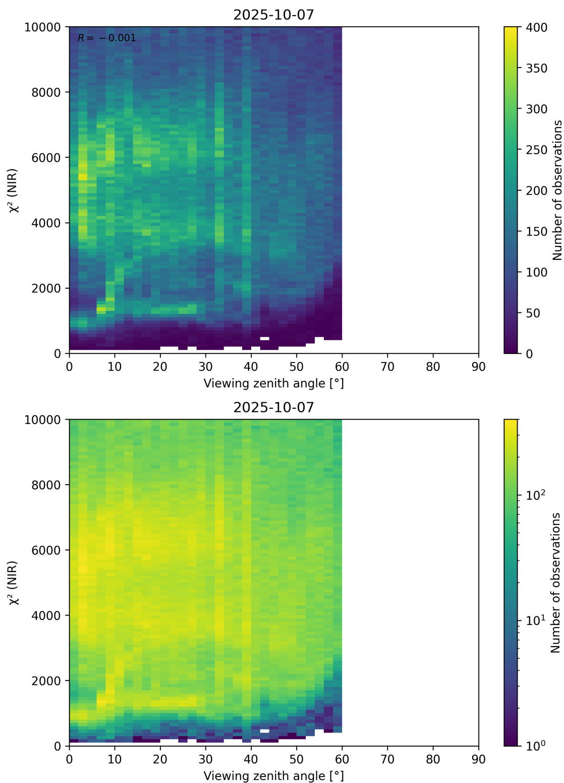
Figure 105: Scatter density plot of “Viewing zenith angle” against “ \chi^2 (NIR)” for 2025-10-06 to 2025-10-08.
