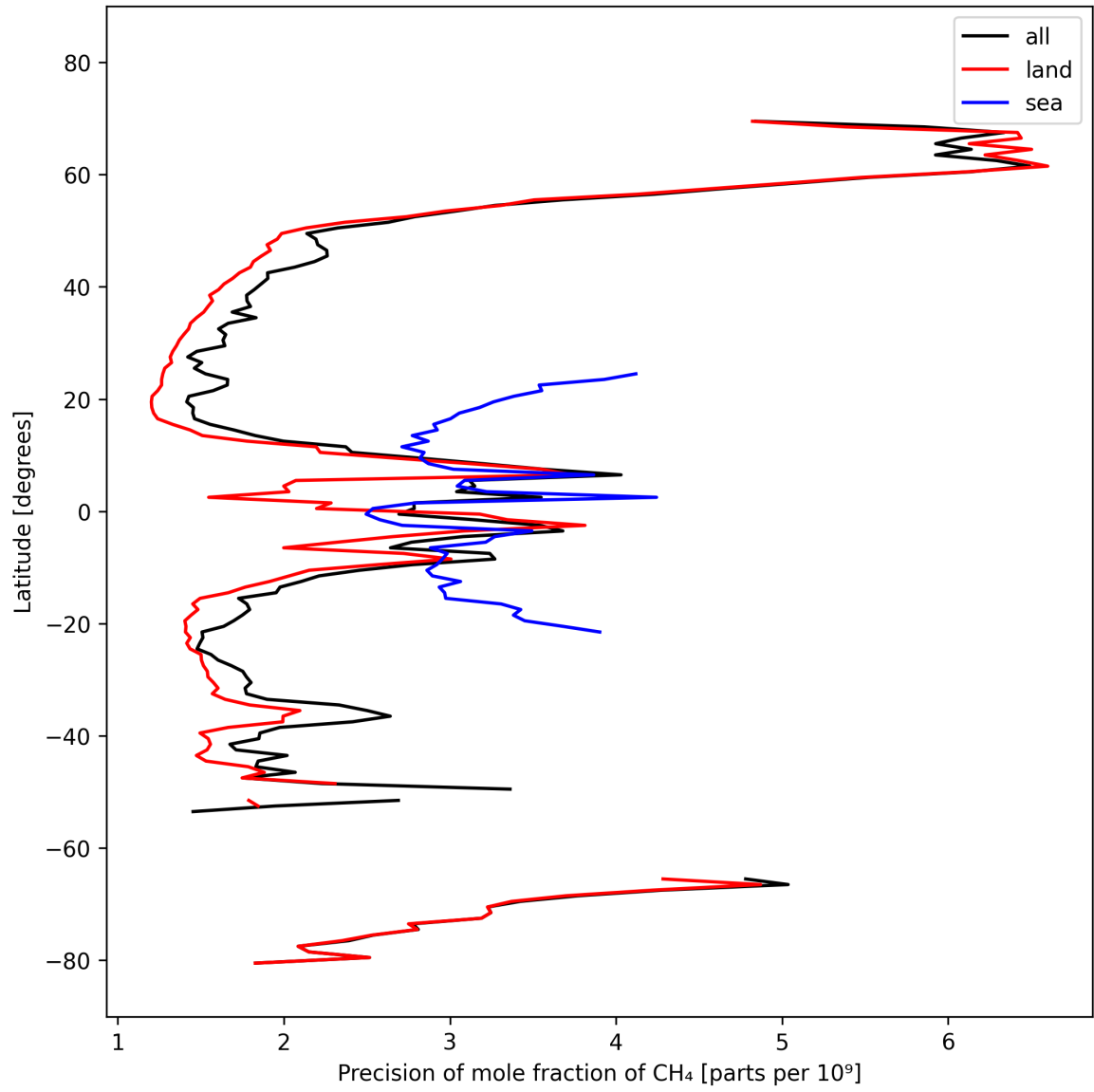
Figure 13: Zonal average of “Precision of mole fraction of CH 4 ” for 2025-10-06 to 2025-10-08.
