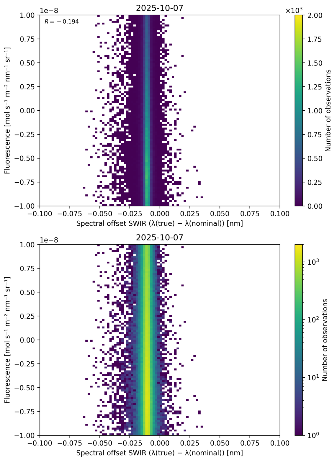
Figure 120: Scatter density plot of “Spectral offset SWIR ( \lambda_{\text{true}} - \lambda_{\text{nominal}} )” against “Fluorescence” for 2025-10-06 to 2025-10-08.
