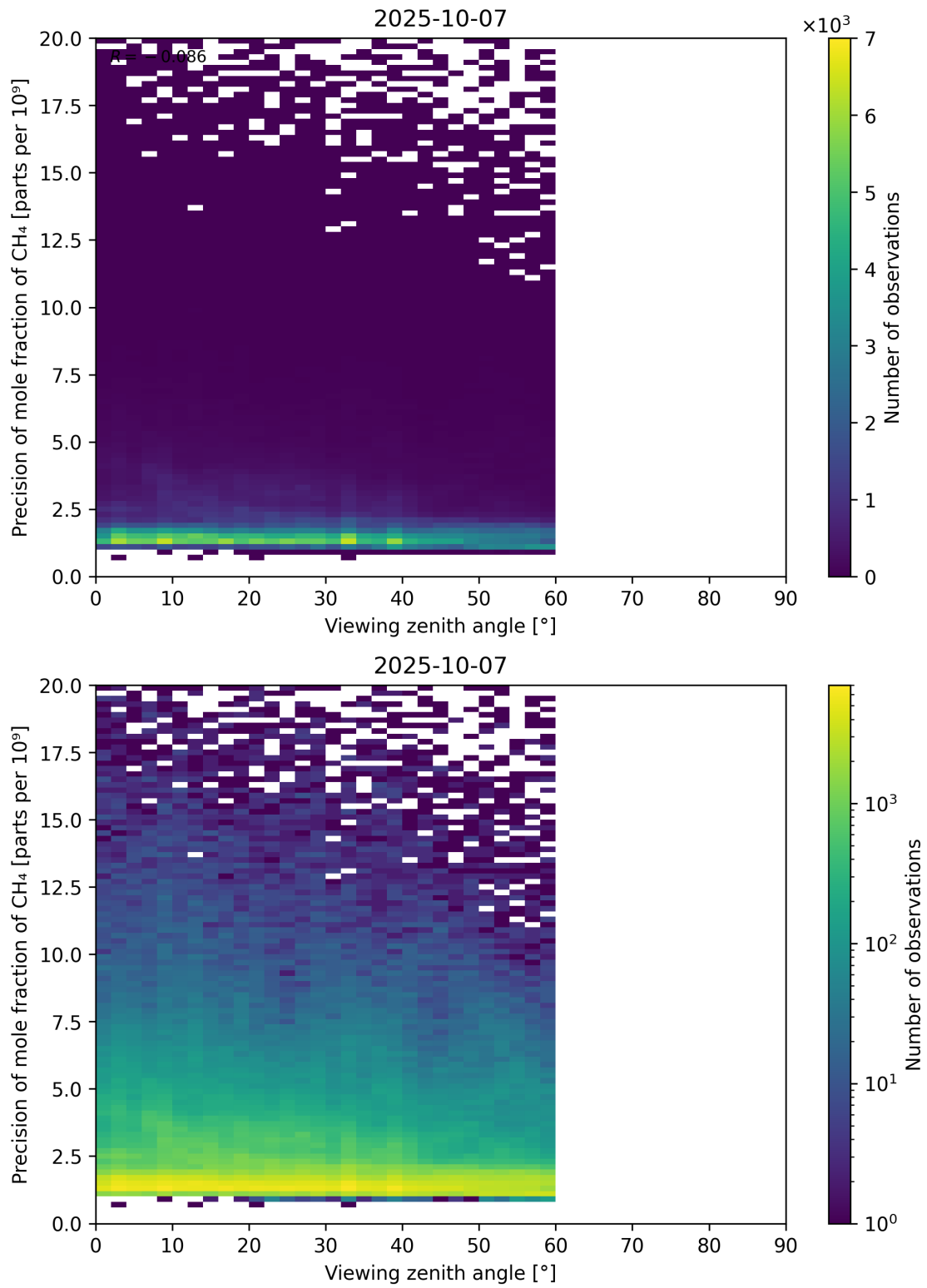
Figure 112: Scatter density plot of “Viewing zenith angle” against “Precision of mole fraction of CH 4 ” for 2025-10-06 to 2025-10-08.
