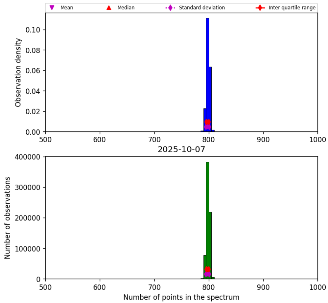
Figure 26: Histogram of “Number of points in the spectrum” for 2025-10-06 to 2025-10-08
