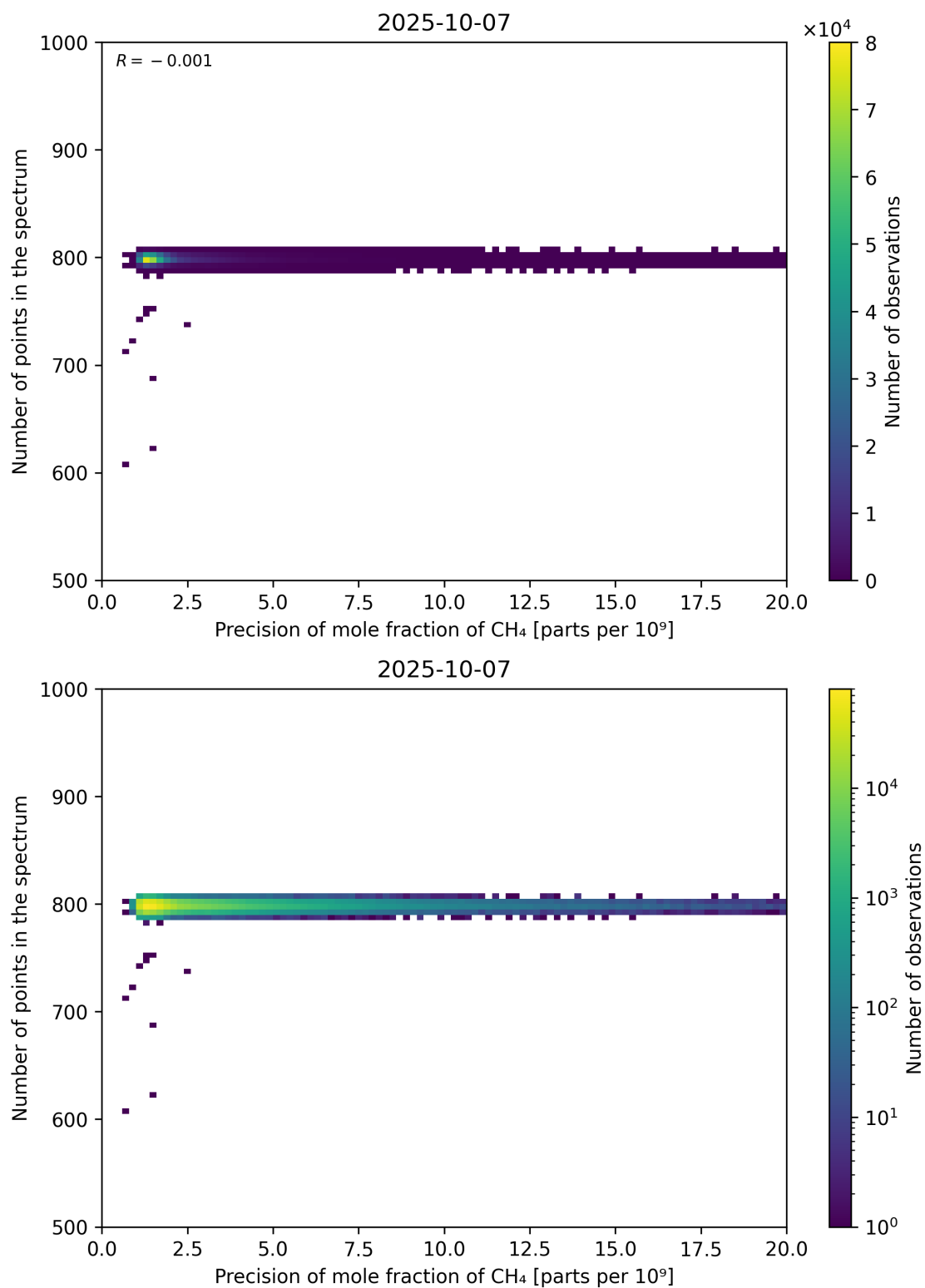
Figure 84: Scatter density plot of “Precision of mole fraction of CH 4 ” against “Number of points in the spectrum” for 2025-10-06 to 2025-10-08.
