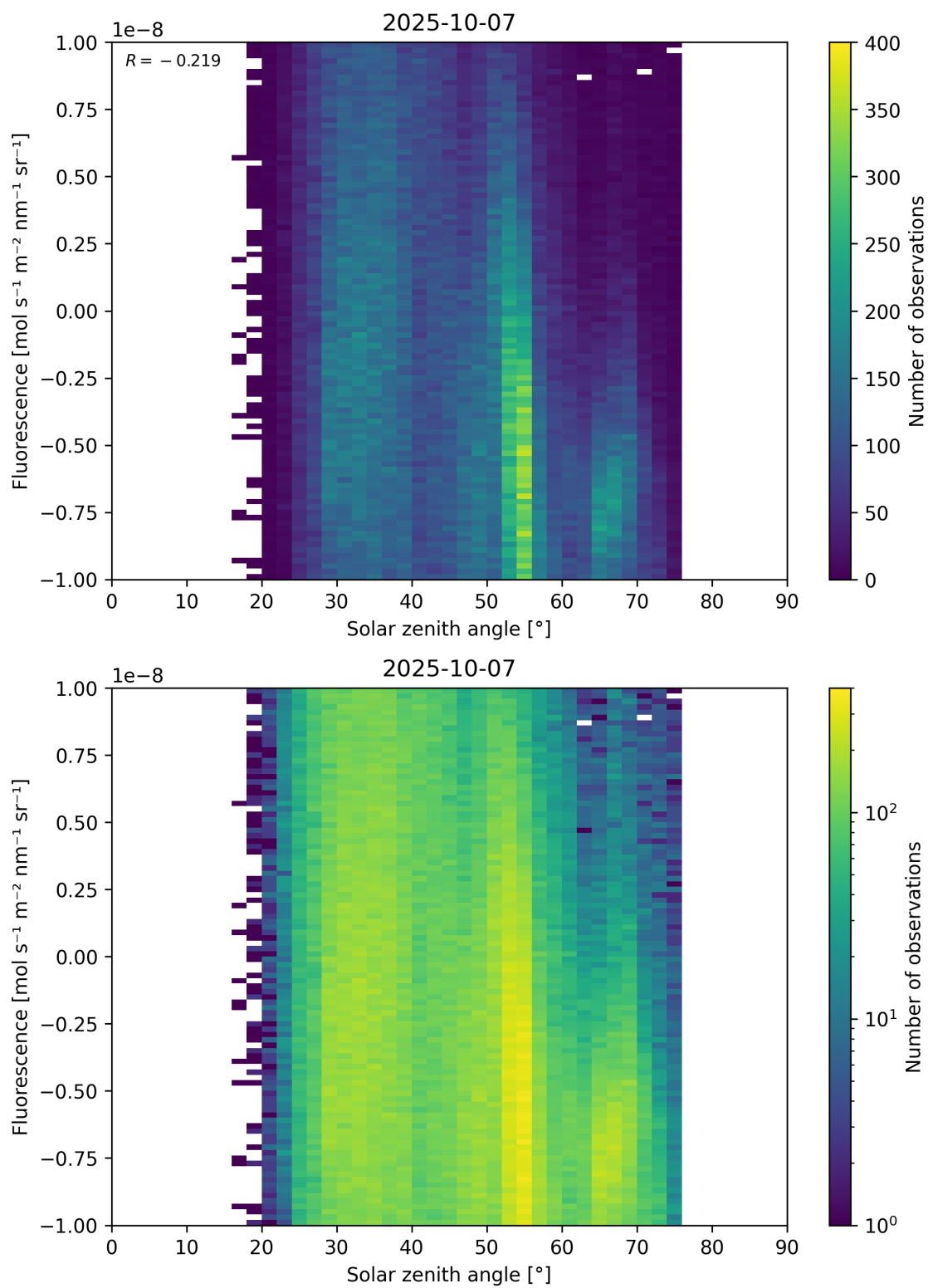
Figure 97: Scatter density plot of “Solar zenith angle” against “Fluorescence” for 2025-10-06 to 2025-10-08.
