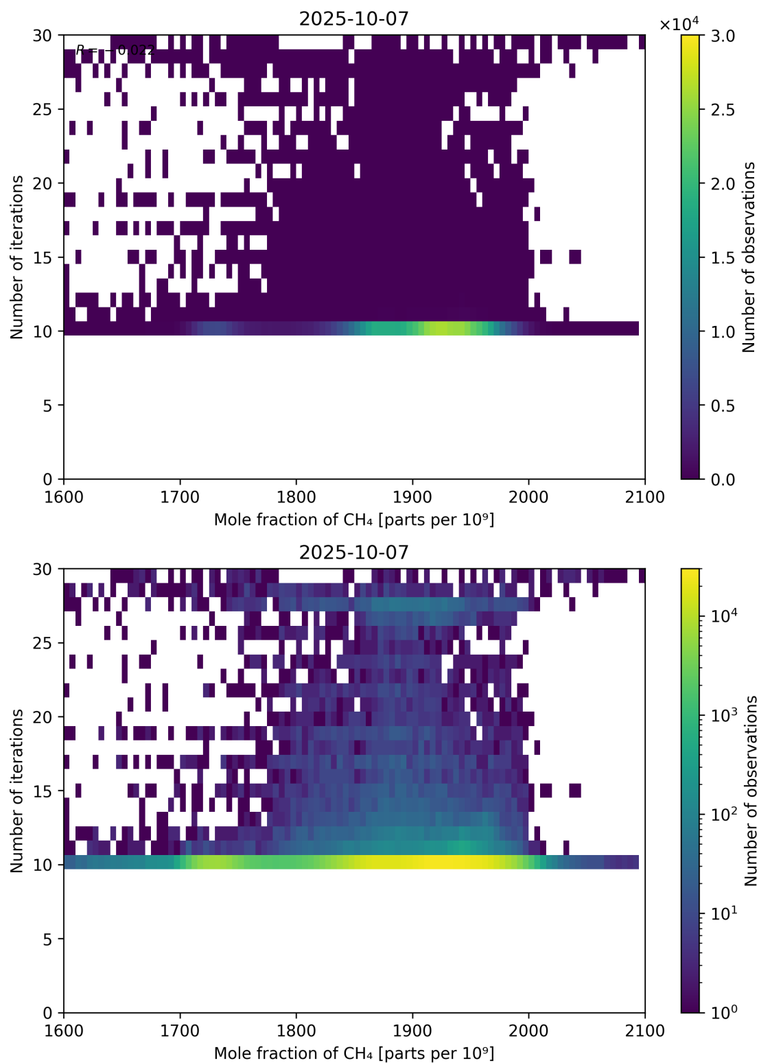
Figure 76: Scatter density plot of “Mole fraction of CH 4 ” against “Number of iterations” for 2025-10-06 to 2025-10-08.
