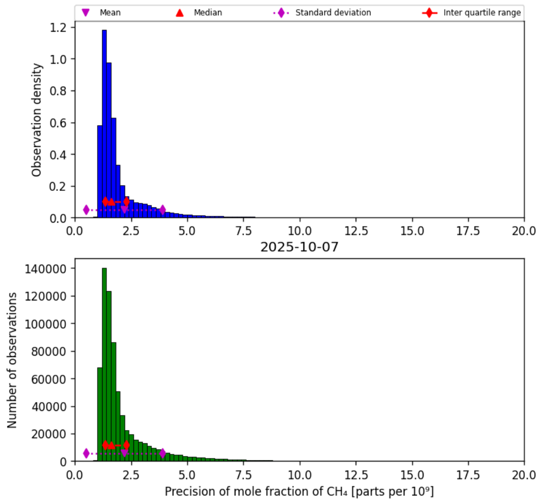
Figure 24: Histogram of “Precision of mole fraction of CH 4 ” for 2025-10-06 to 2025-10-08
