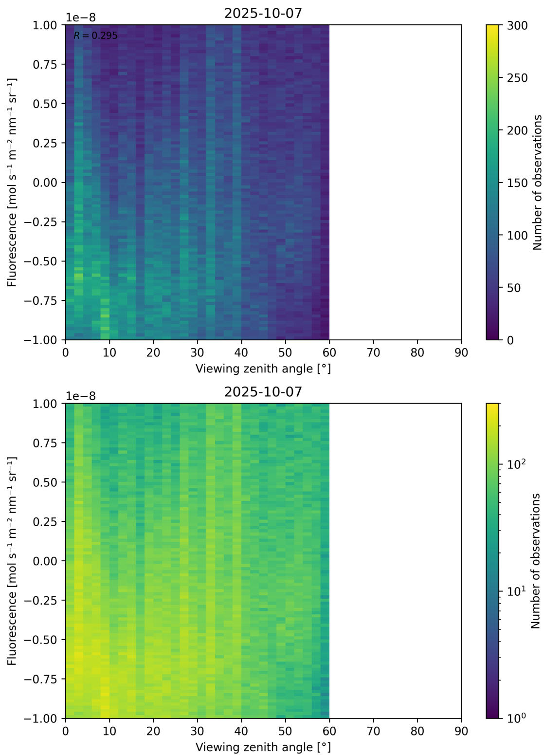
Figure 108: Scatter density plot of “Viewing zenith angle” against “Fluorescence” for 2025-10-06 to 2025-10-08.
