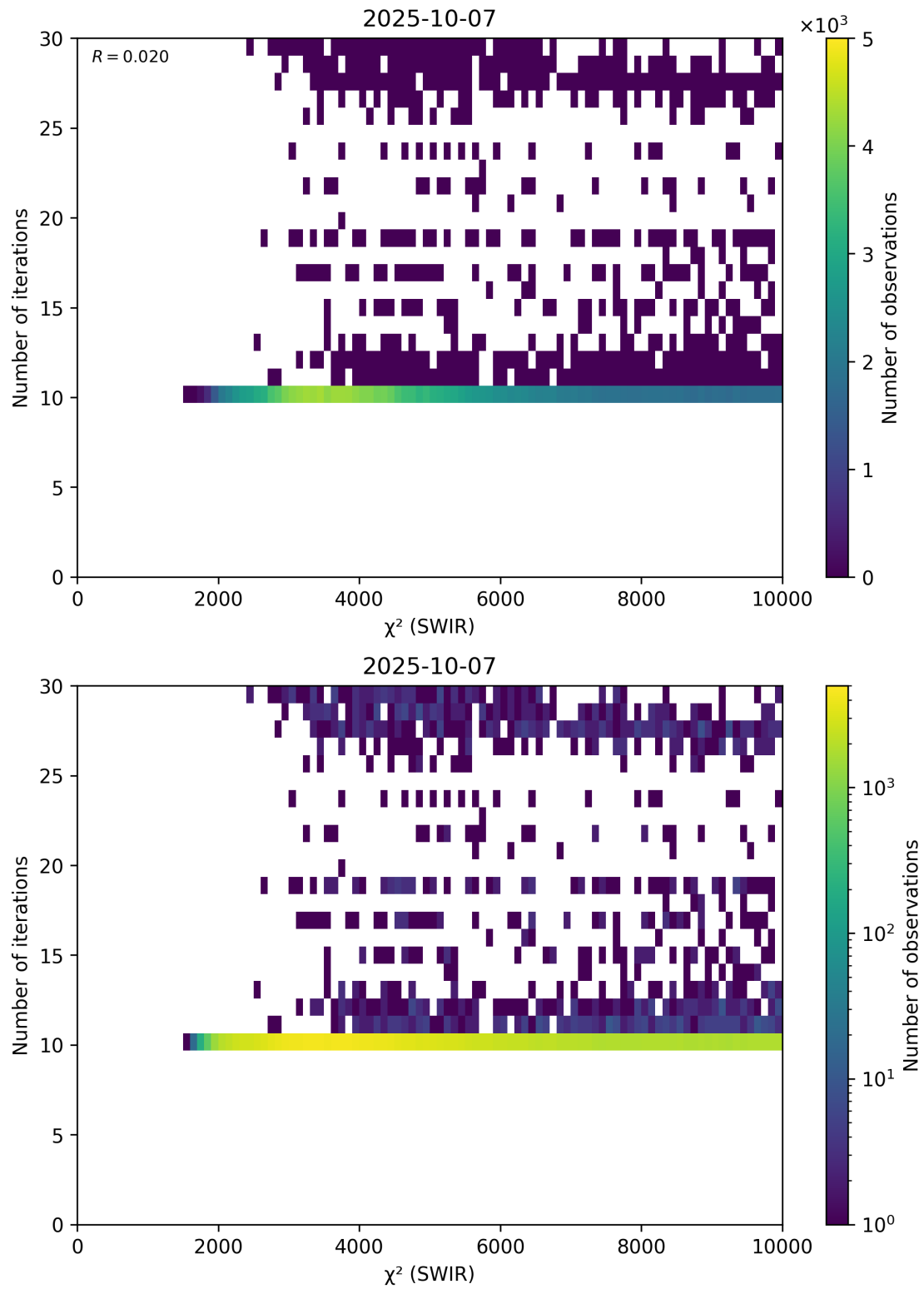
Figure 50: Scatter density plot of “ \chi^2 (SWIR)” against “Number of iterations” for 2025-10-06 to 2025-10-08.
