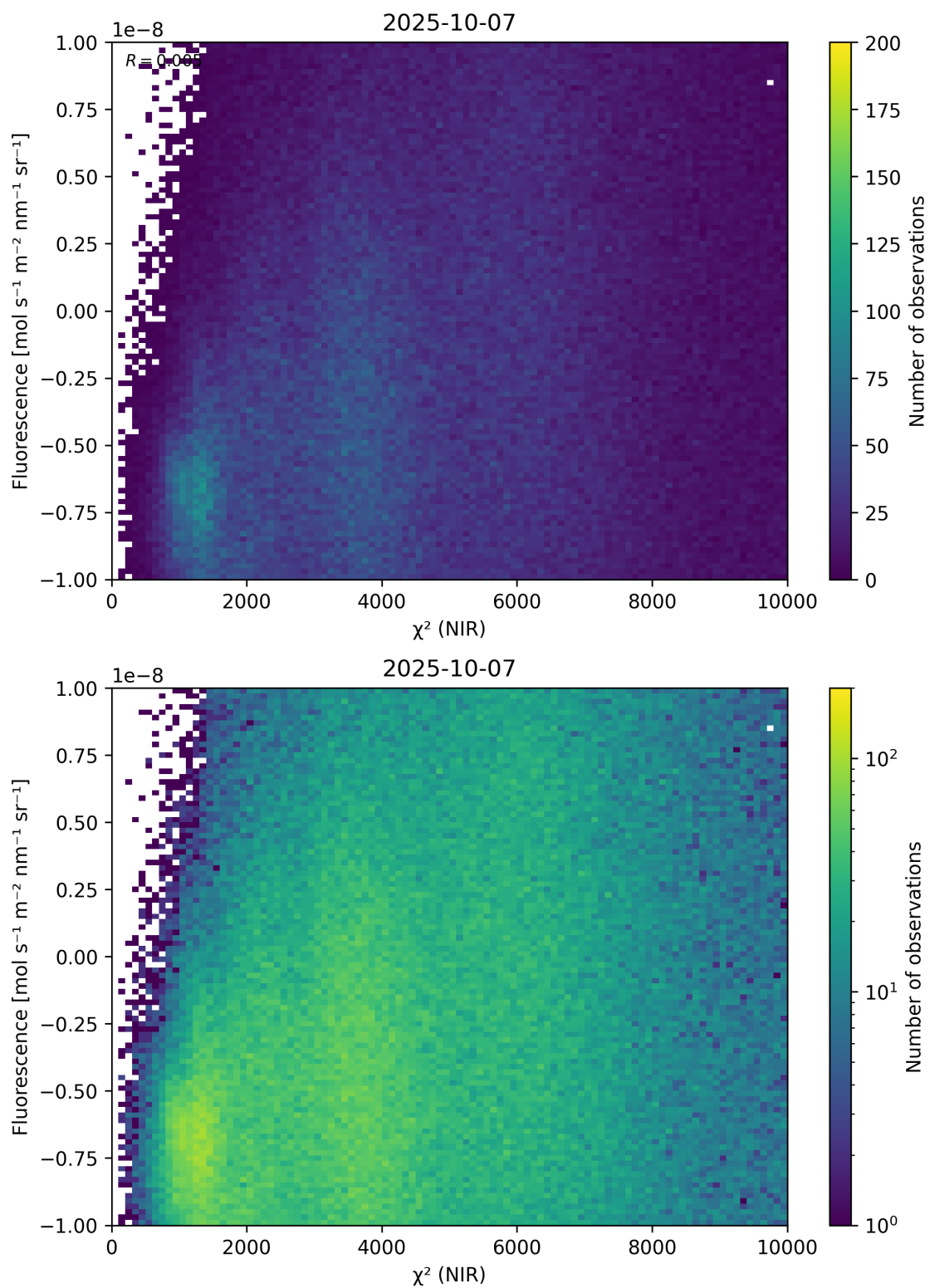
Figure 45: Scatter density plot of “ \chi^2 (NIR)” against “Fluorescence” for 2025-10-06 to 2025-10-08.
