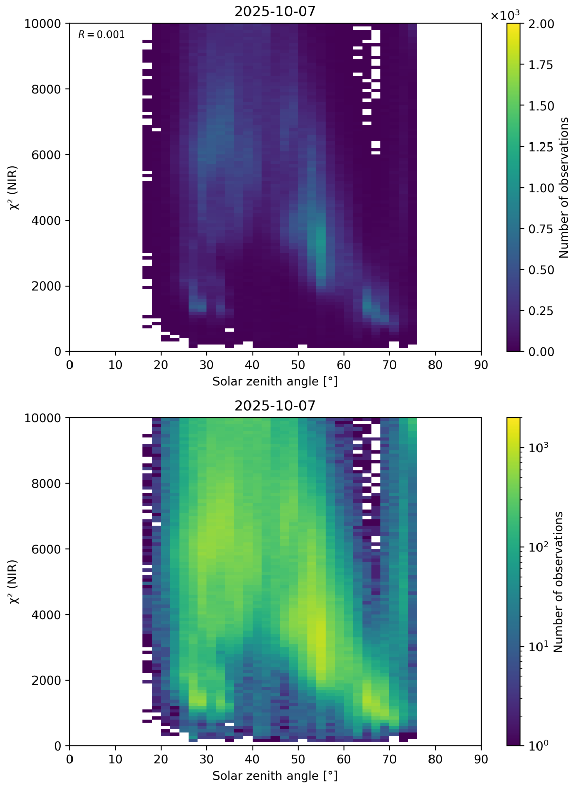
Figure 94: Scatter density plot of “Solar zenith angle” against “ \chi^2 (NIR)” for 2025-10-06 to 2025-10-08.
