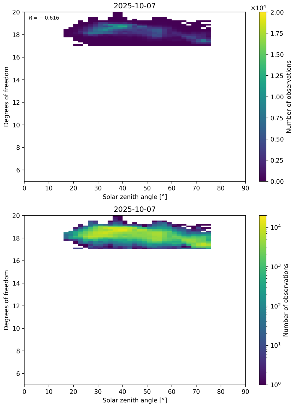
Figure 96: Scatter density plot of “Solar zenith angle” against “Degrees of freedom” for 2025-10-06 to 2025-10-08.
