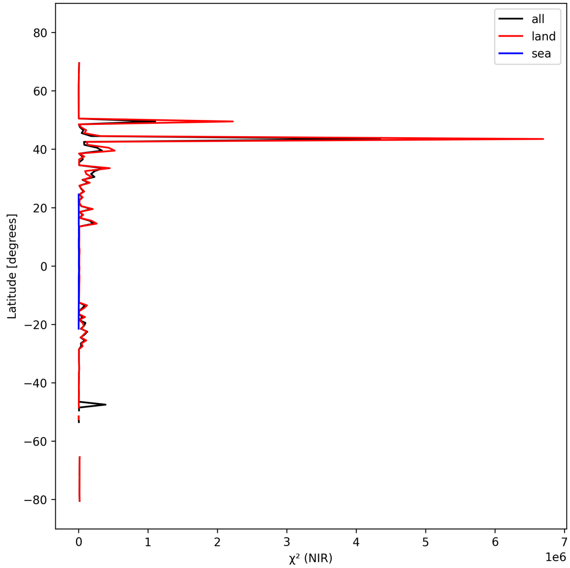
Figure 18: Zonal average of “ \chi^2 (NIR)” for 2025-10-06 to 2025-10-08.
