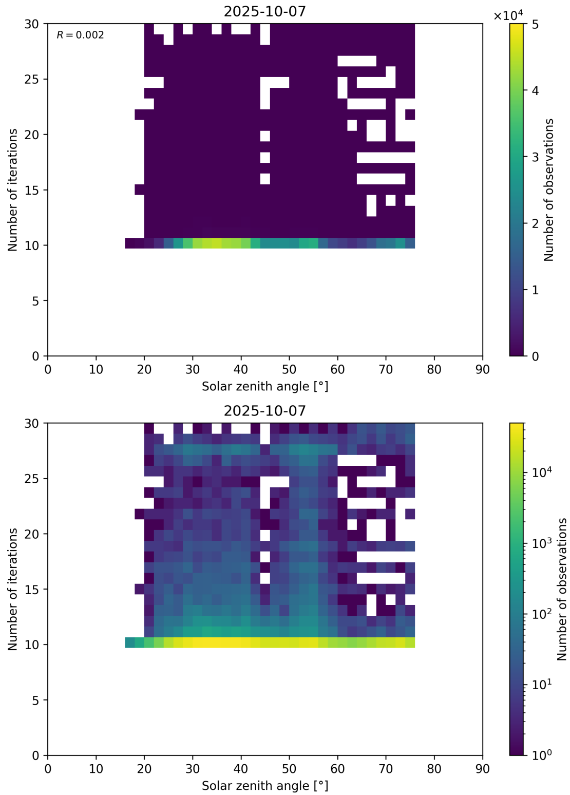
Figure 102: Scatter density plot of “Solar zenith angle” against “Number of iterations” for 2025-10-06 to 2025-10-08.
