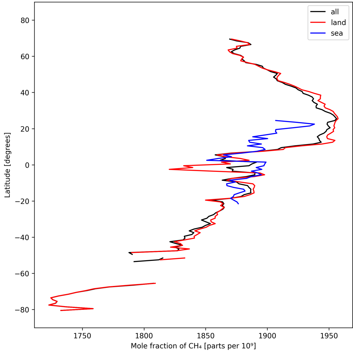
Figure 12: Zonal average of “Mole fraction of \text{CH}_4 ” for 2025-10-06 to 2025-10-08.
