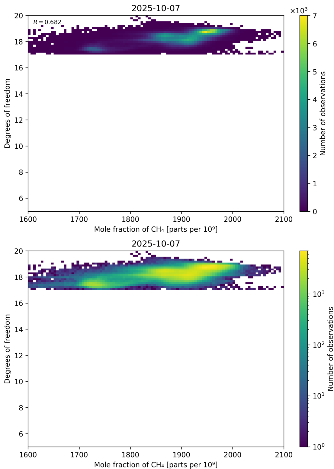
Figure 72: Scatter density plot of “Mole fraction of CH 4 ” against “Degrees of freedom” for 2025-10-06 to 2025-10-08.
