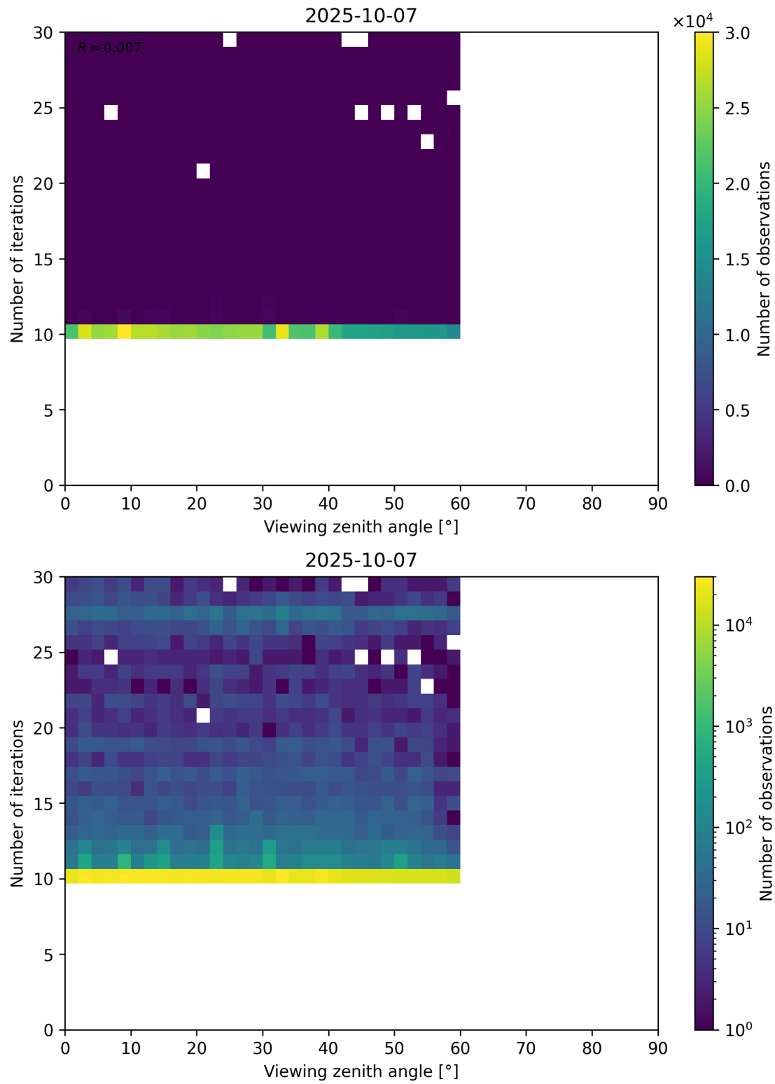
Figure 113: Scatter density plot of “Viewing zenith angle” against “Number of iterations” for 2025-10-06 to 2025-10-08.
