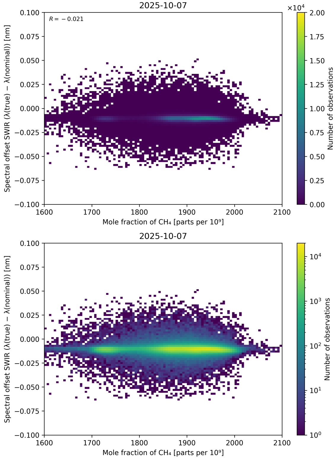
Figure 86: Scatter density plot of “Mole fraction of CH 4 ” against “Spectral offset SWIR ( \lambda_{\text{true}} - \lambda_{\text{nominal}} )” for 2025-10-06 to 2025-10-08.
