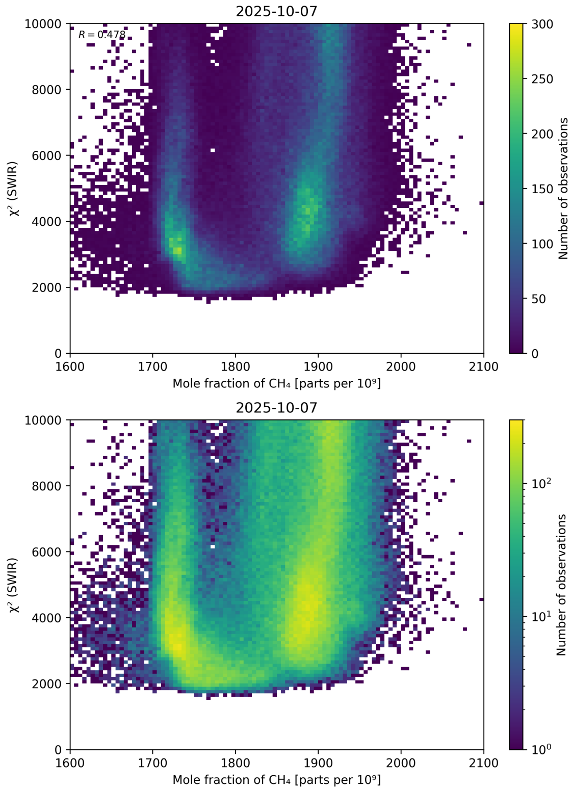
Figure 71: Scatter density plot of “Mole fraction of \text{CH}_4 ” against “ \chi^2 (SWIR)” for 2025-10-06 to 2025-10-08.
