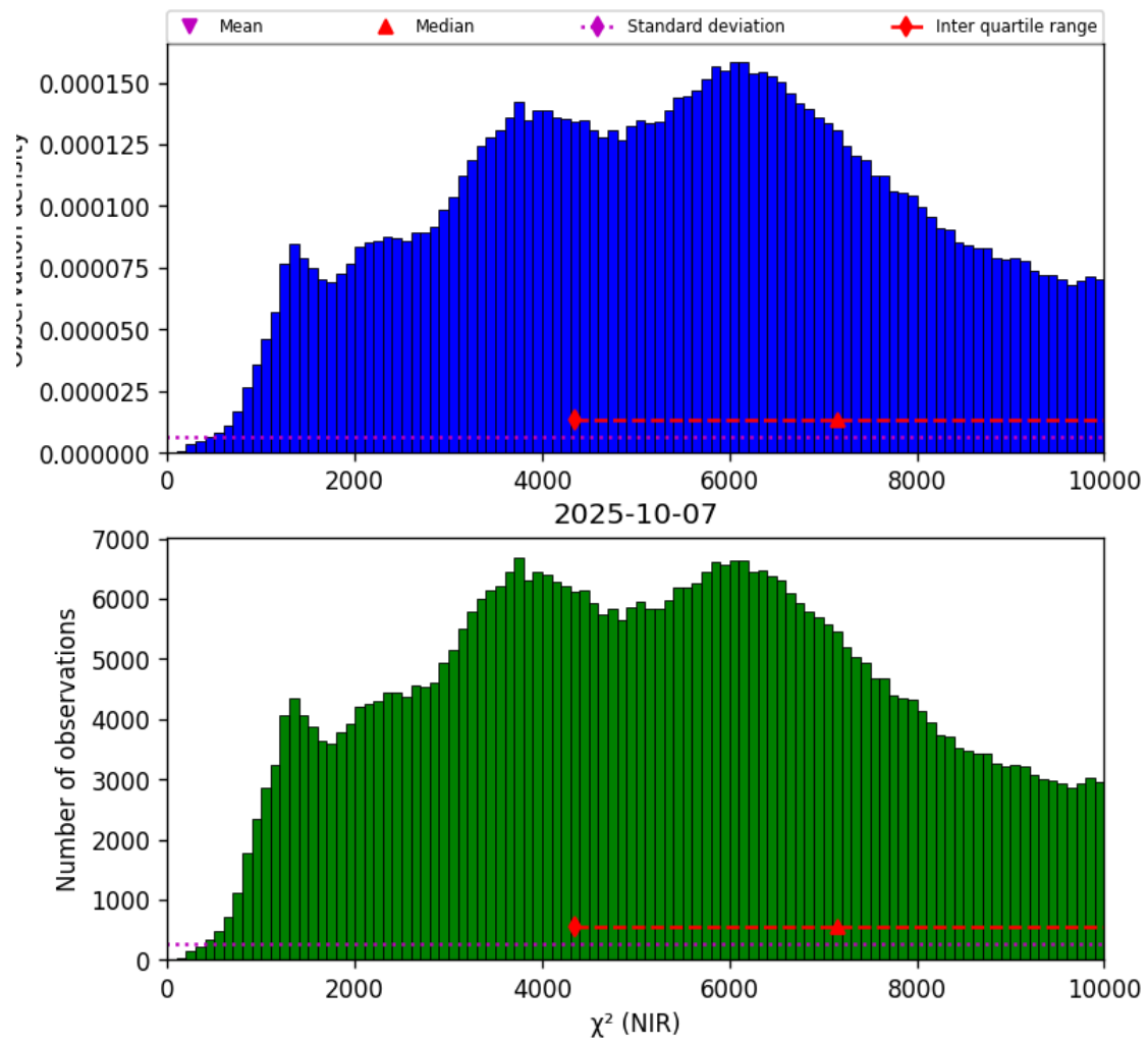
Figure 29: Histogram of “ \chi^2 (NIR)” for 2025-10-06 to 2025-10-08
