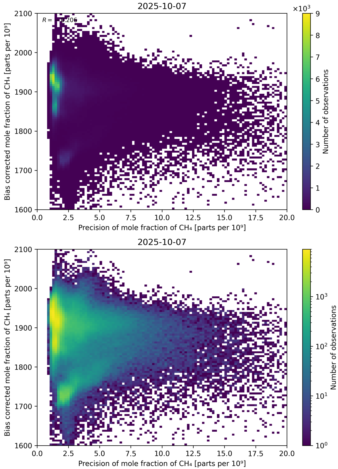
Figure 82: Scatter density plot of “Precision of mole fraction of CH 4 ” against “Bias corrected mole fraction of CH 4 ” for 2025-10-06 to 2025-10-08.
