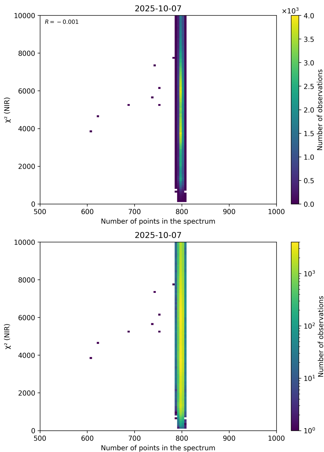
Figure 88: Scatter density plot of “Number of points in the spectrum” against “ \chi^2 (NIR)” for 2025-10-06 to 2025-10-08.
