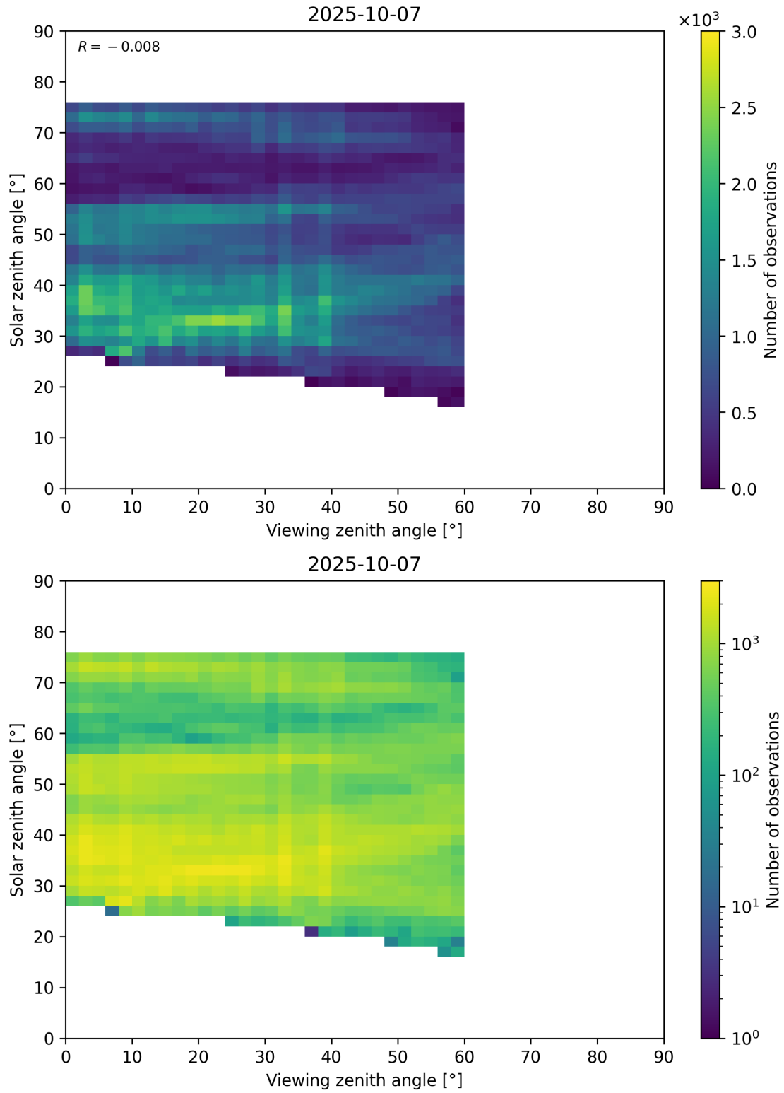
Figure 115: Scatter density plot of “Viewing zenith angle” against “Solar zenith angle” for 2025-10-06 to 2025-10-08.
