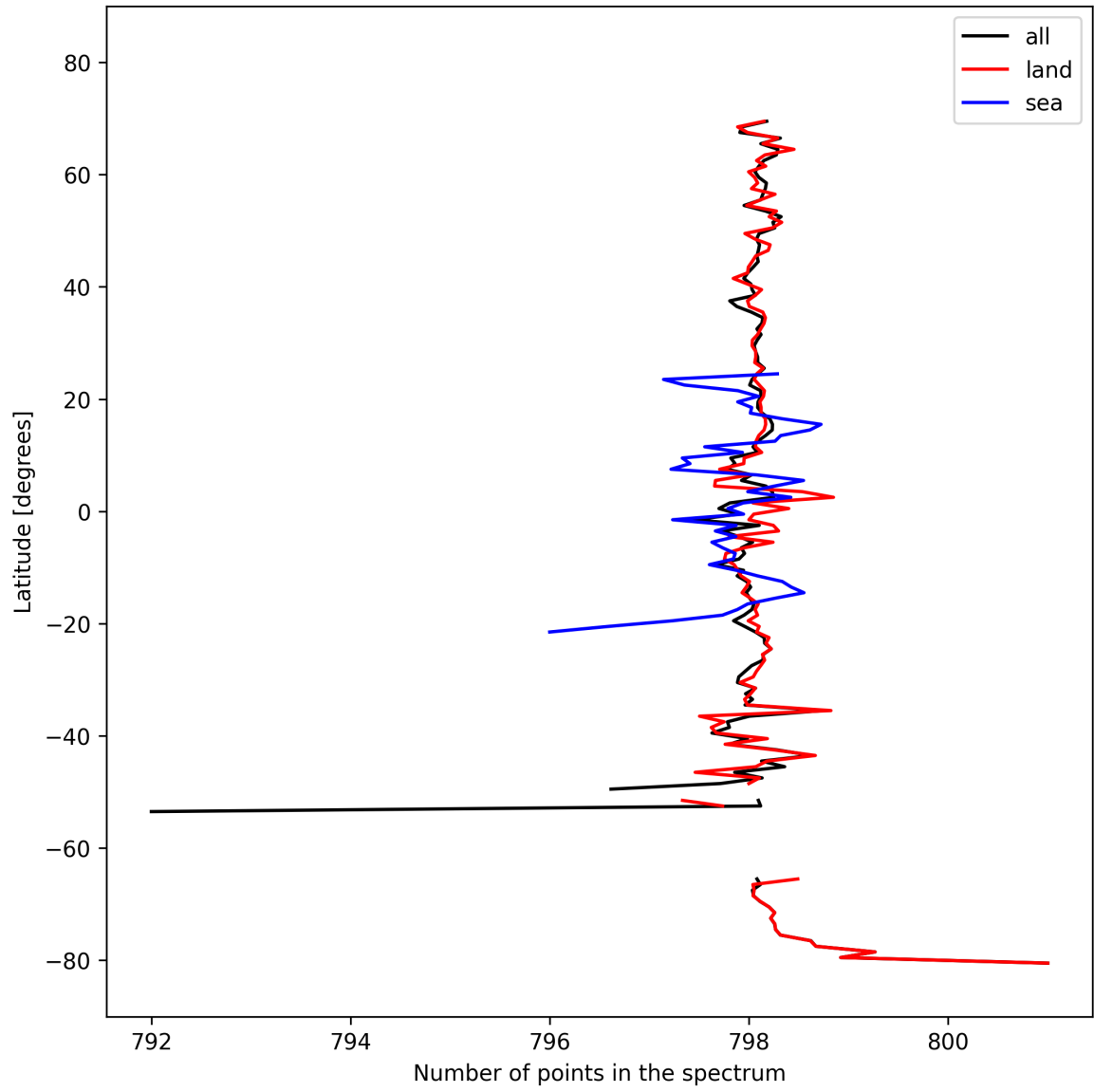
Figure 15: Zonal average of “Number of points in the spectrum” for 2025-10-06 to 2025-10-08.
