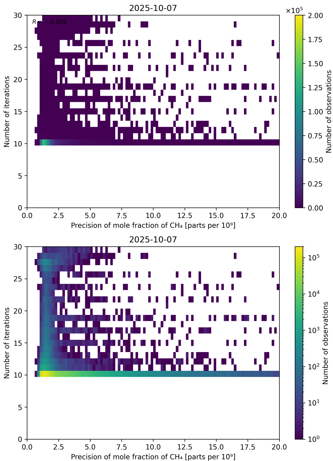
Figure 83: Scatter density plot of “Precision of mole fraction of CH 4 ” against “Number of iterations” for 2025-10-06 to 2025-10-08.
