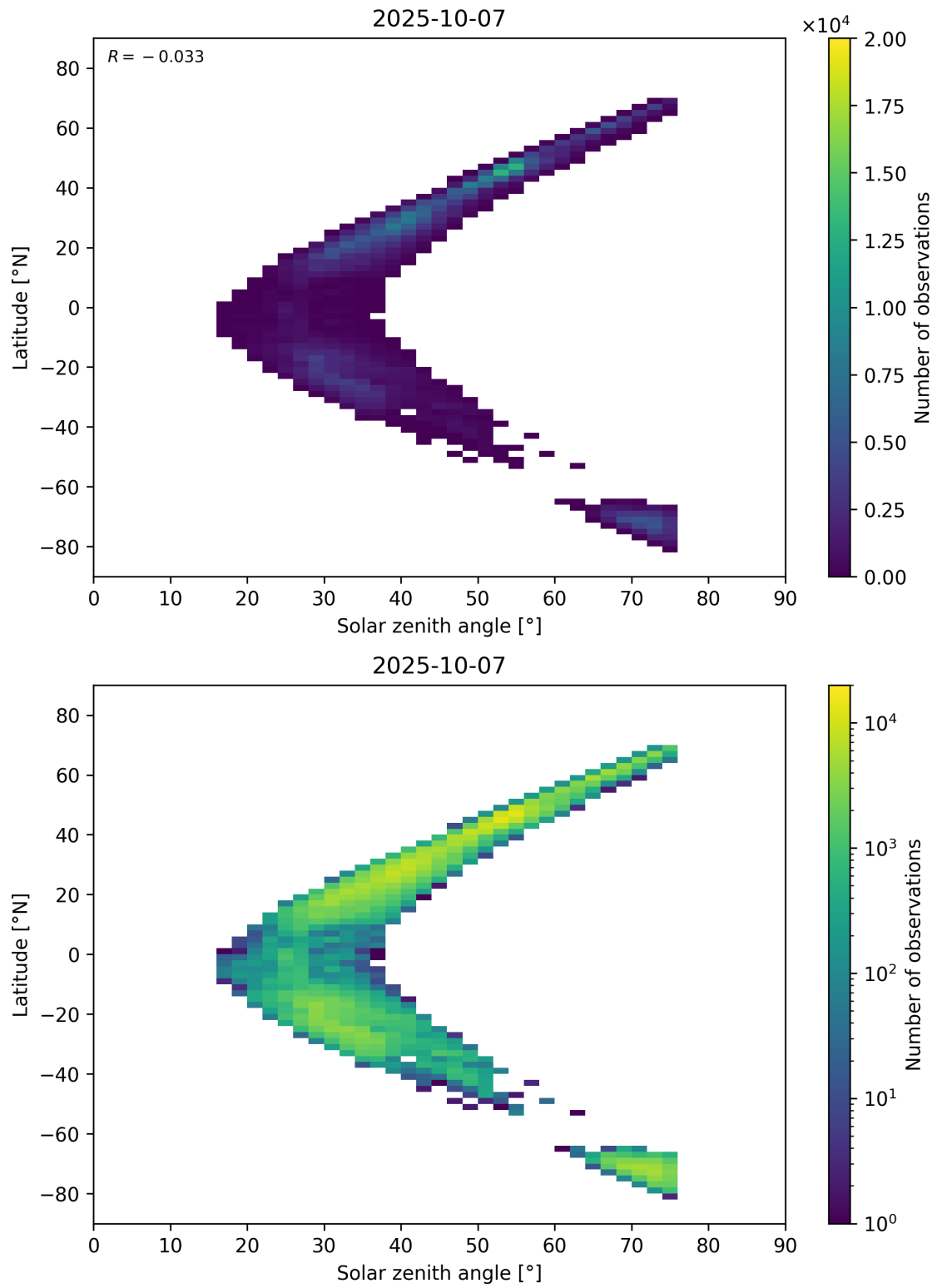
Figure 98: Scatter density plot of “Solar zenith angle” against “Latitude” for 2025-10-06 to 2025-10-08.
