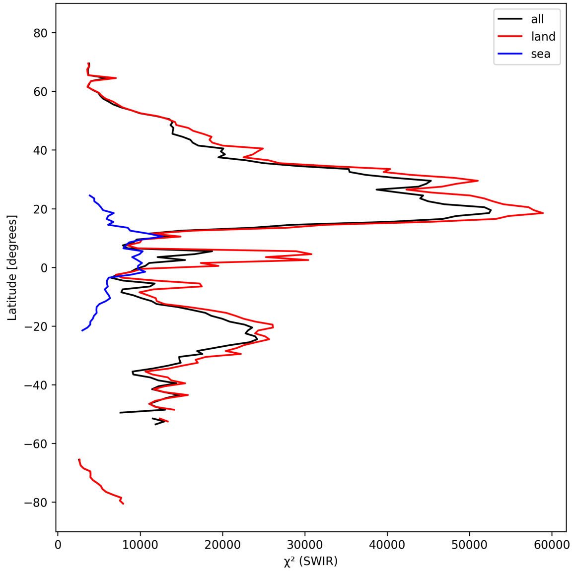
Figure 17: Zonal average of “ \chi^2 (SWIR)” for 2025-10-06 to 2025-10-08.
