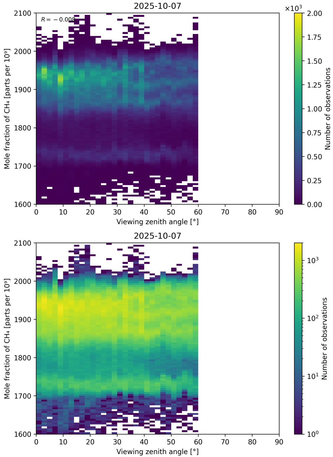
Figure 110: Scatter density plot of “Viewing zenith angle” against “Mole fraction of CH 4 ” for 2025-10-06 to 2025-10-08.
