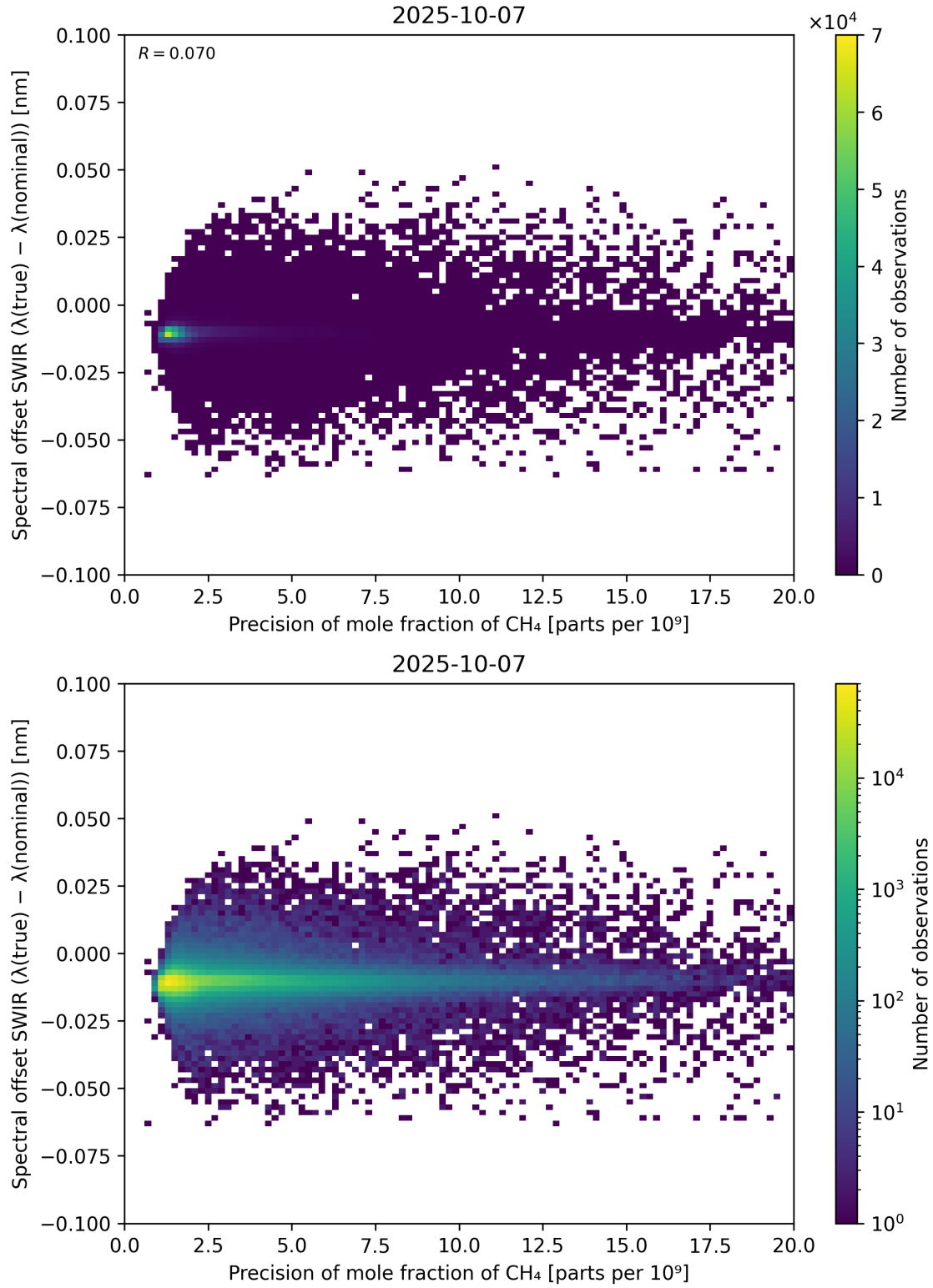
Figure 85: Scatter density plot of “Precision of mole fraction of CH 4 ” against “Spectral offset SWIR ( \lambda_{\text{true}} - \lambda_{\text{nominal}} )” for 2025-10-06 to 2025-10-08.
