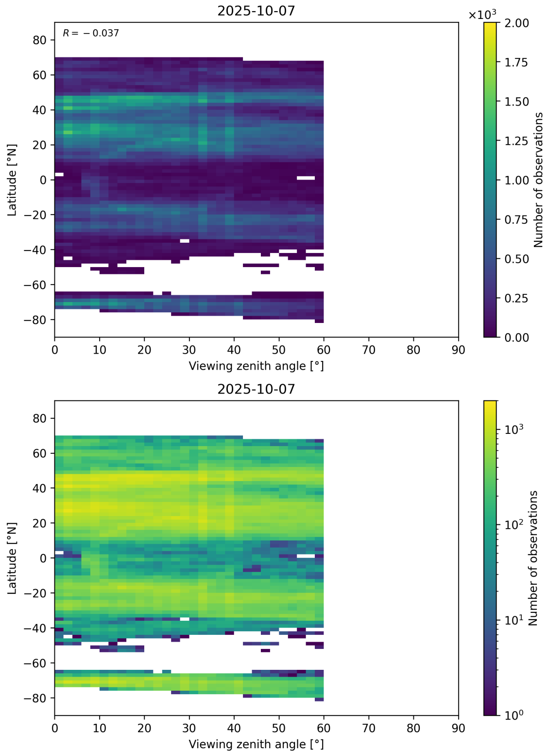
Figure 109: Scatter density plot of “Viewing zenith angle” against “Latitude” for 2025-10-06 to 2025-10-08.
