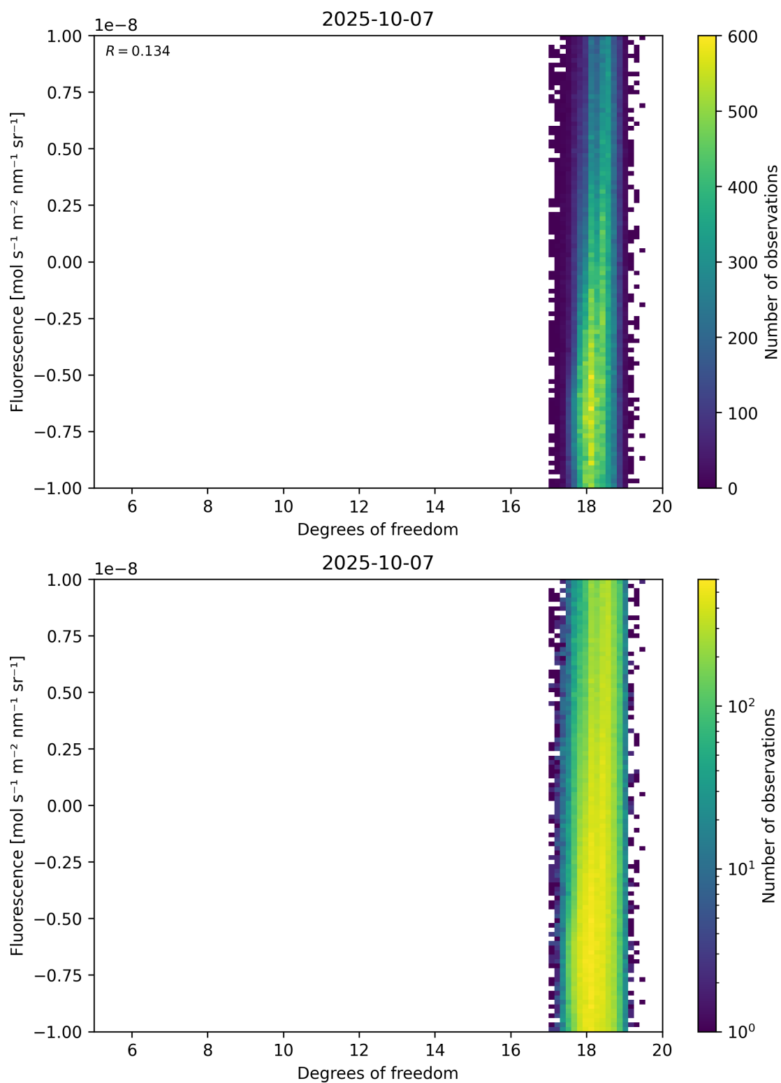
Figure 51: Scatter density plot of “Degrees of freedom” against “Fluorescence” for 2025-10-06 to 2025-10-08.
