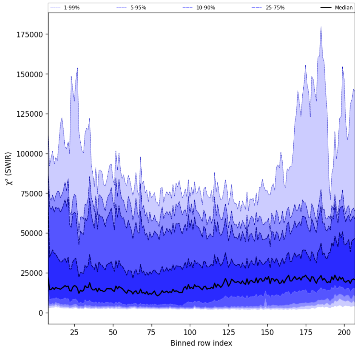
Figure 39: Along track statistics of “ \chi^2 (SWIR)” for 2025-10-06 to 2025-10-08
