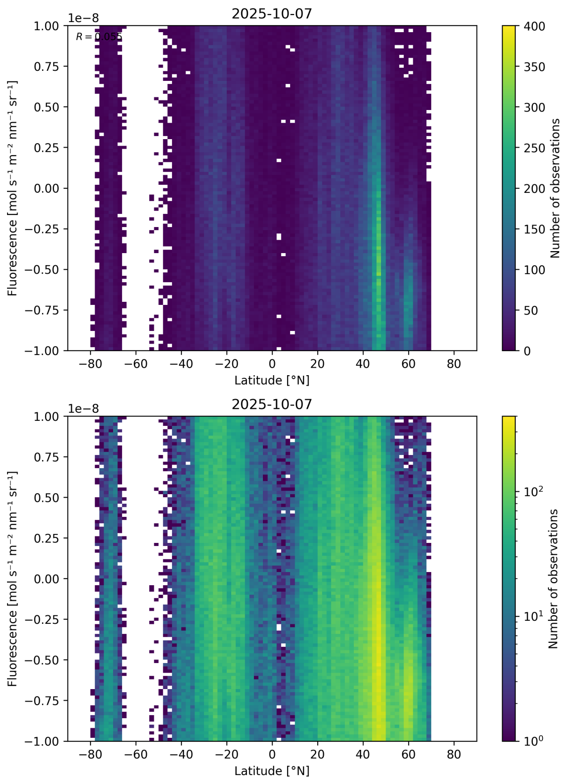
Figure 56: Scatter density plot of “Latitude” against “Fluorescence” for 2025-10-06 to 2025-10-08.
