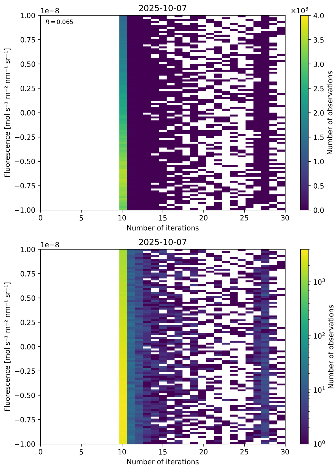
Figure 87: Scatter density plot of “Number of iterations” against “Fluorescence” for 2025-10-06 to 2025-10-08.
