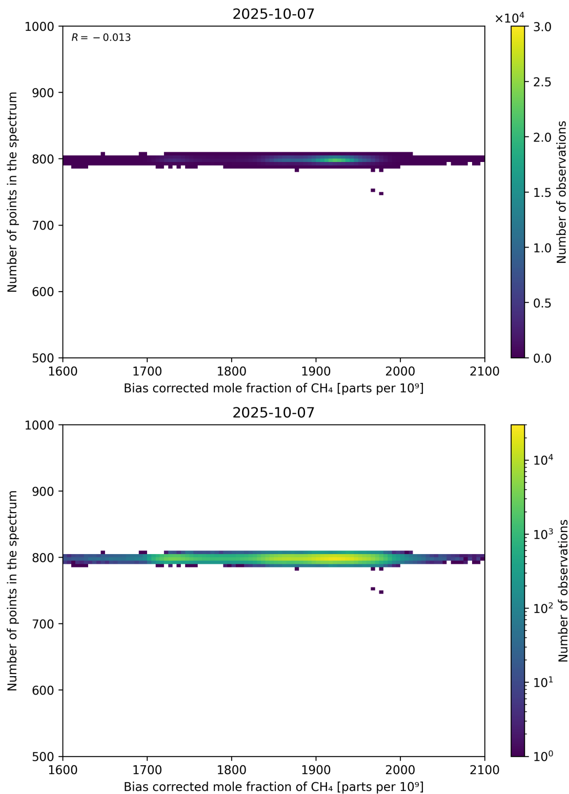
Figure 68: Scatter density plot of “Bias corrected mole fraction of CH 4 ” against “Number of points in the spectrum” for 2025-10-06 to 2025-10-08.
