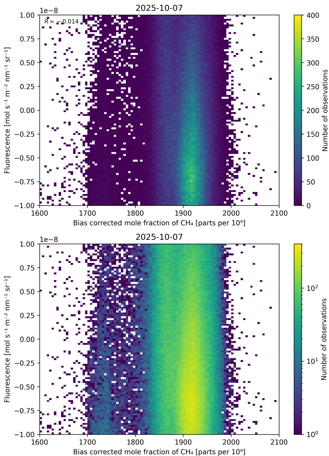
Figure 66: Scatter density plot of “Bias corrected mole fraction of \text{CH}_4 ” against “Fluorescence” for 2025-10-06 to 2025-10-08.
