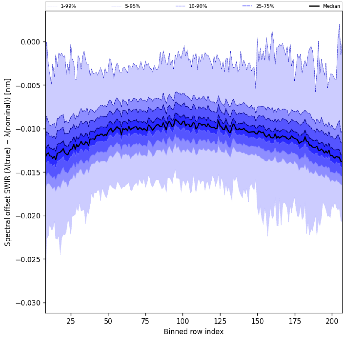
Figure 38: Along track statistics of “Spectral offset SWIR ( \lambda_{\text{true}} - \lambda_{\text{nominal}} )” for 2025-10-06 to 2025-10-08
