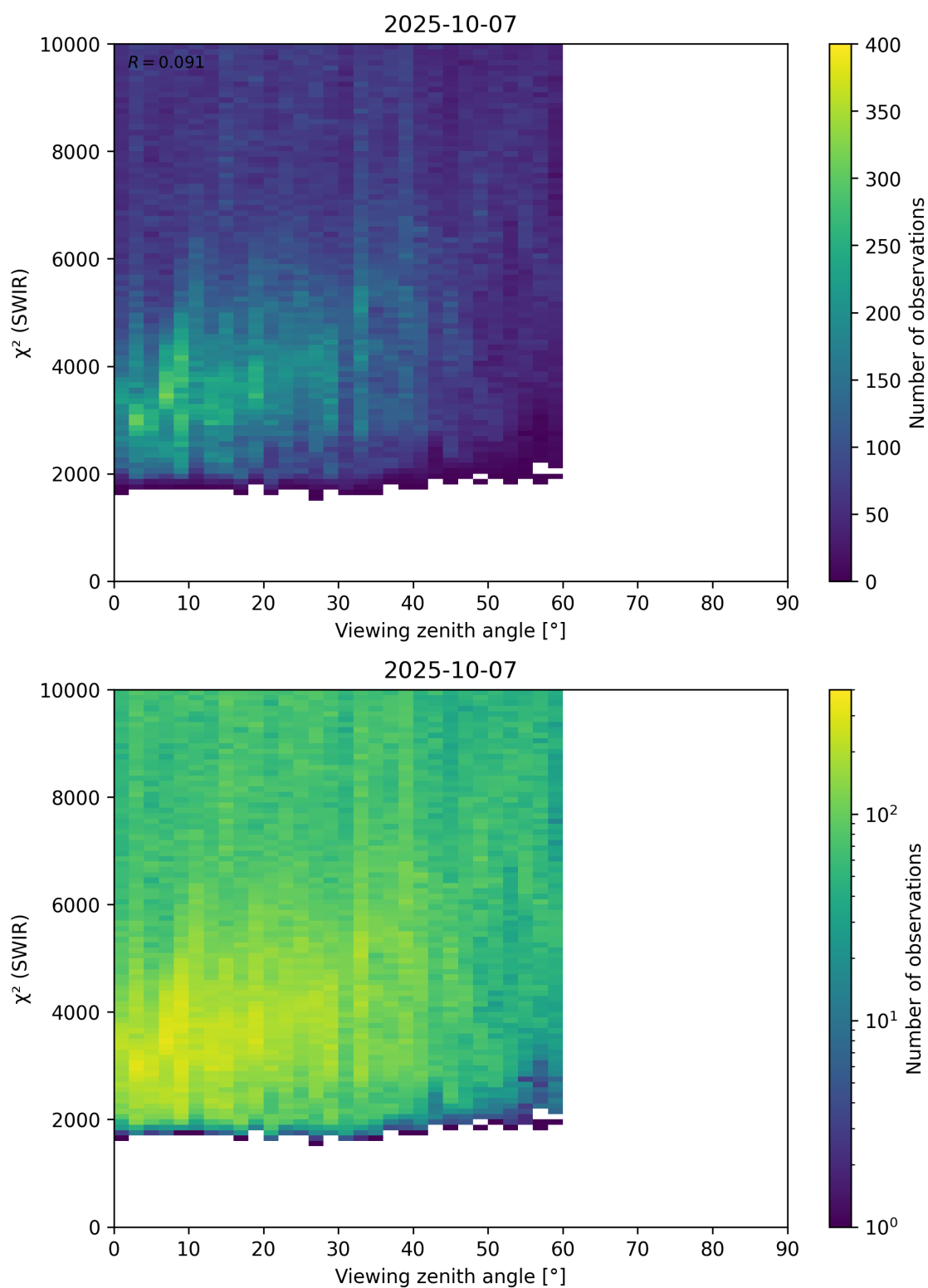
Figure 106: Scatter density plot of “Viewing zenith angle” against “ \chi^2 (SWIR)” for 2025-10-06 to 2025-10-08.
