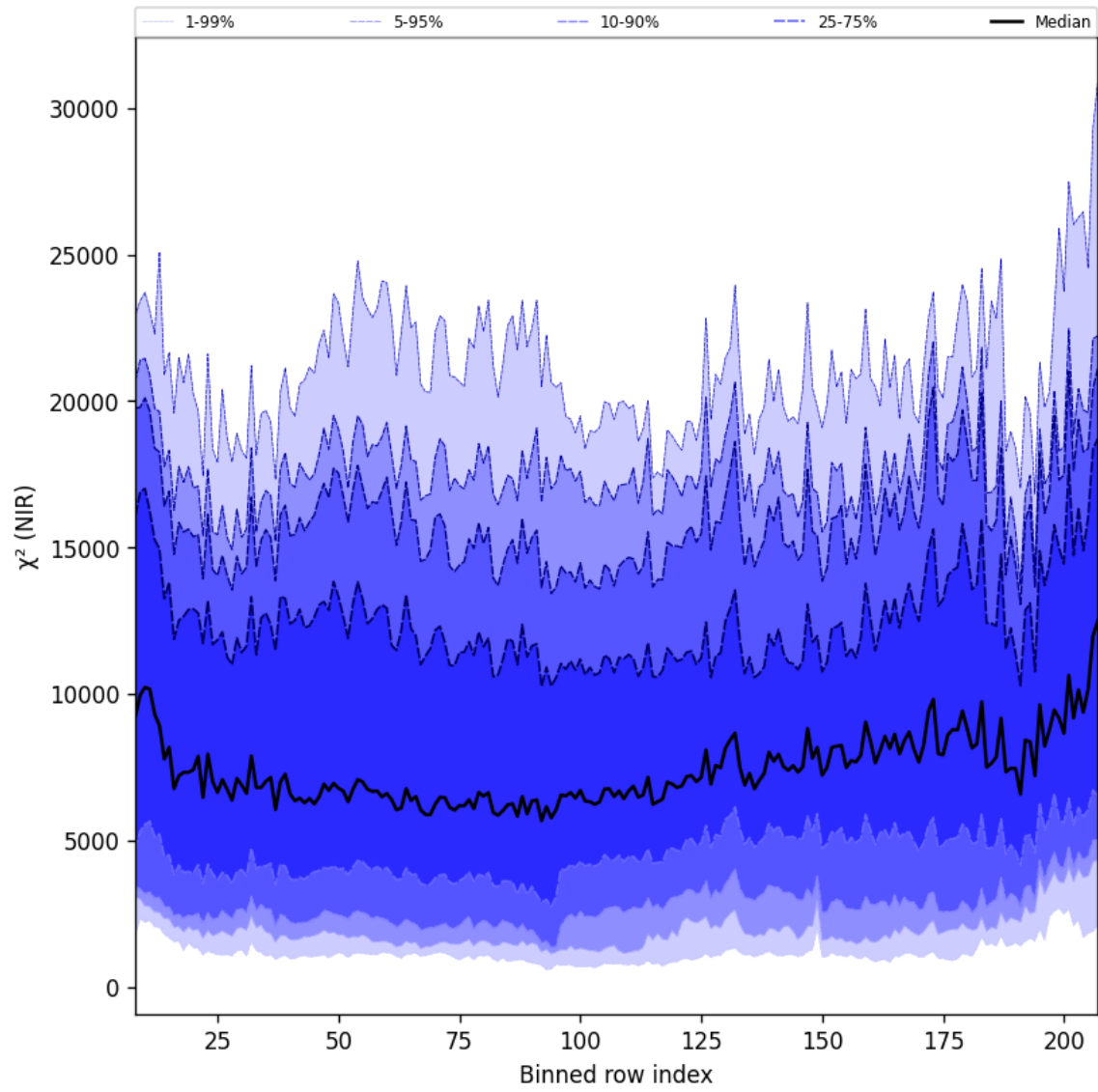
Figure 40: Along track statistics of “ \chi^2 (NIR)” for 2025-10-06 to 2025-10-08
