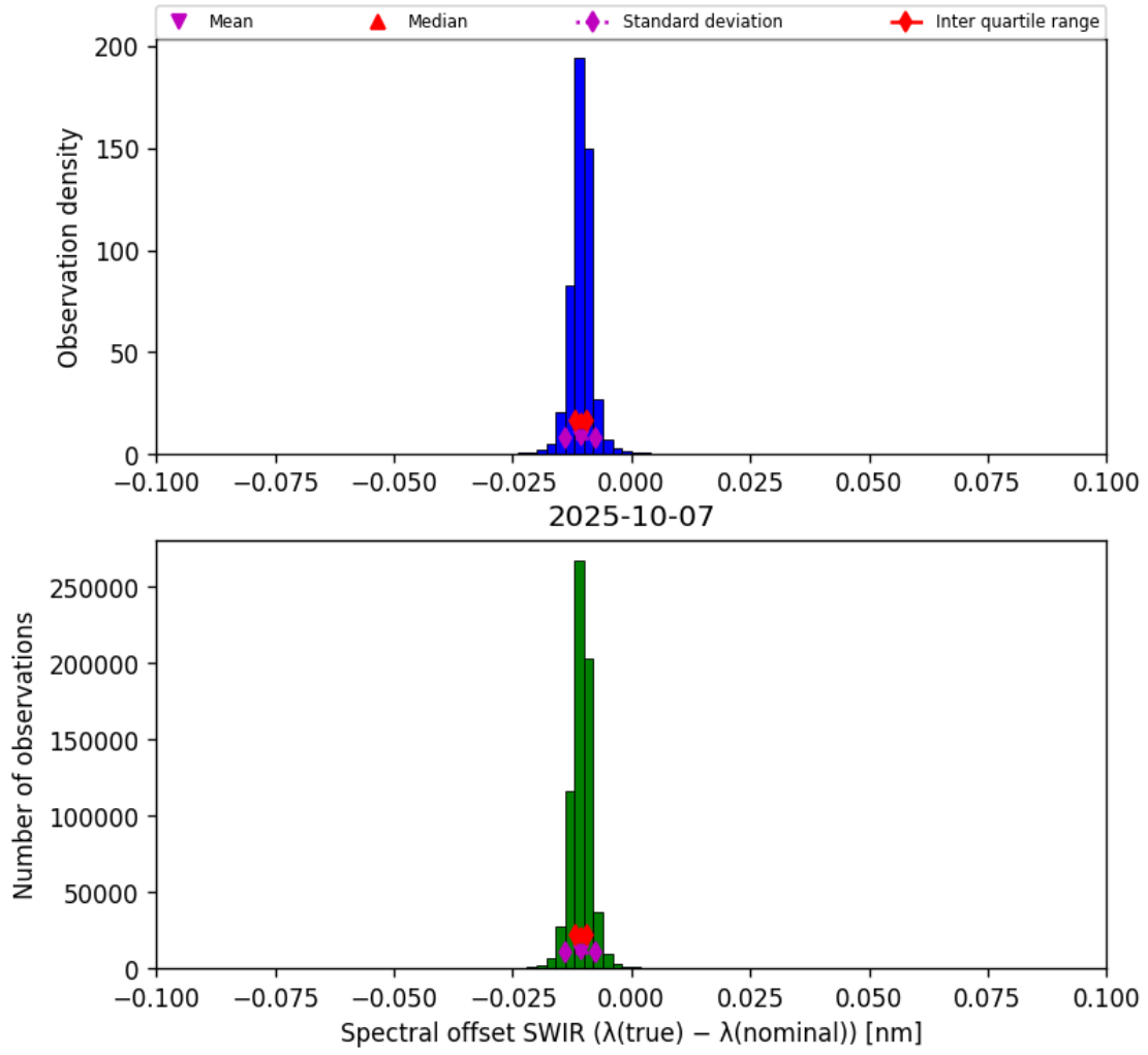
Figure 27: Histogram of “Spectral offset SWIR ( \lambda_{\text{true}} - \lambda_{\text{nominal}} )” for 2025-10-06 to 2025-10-08
