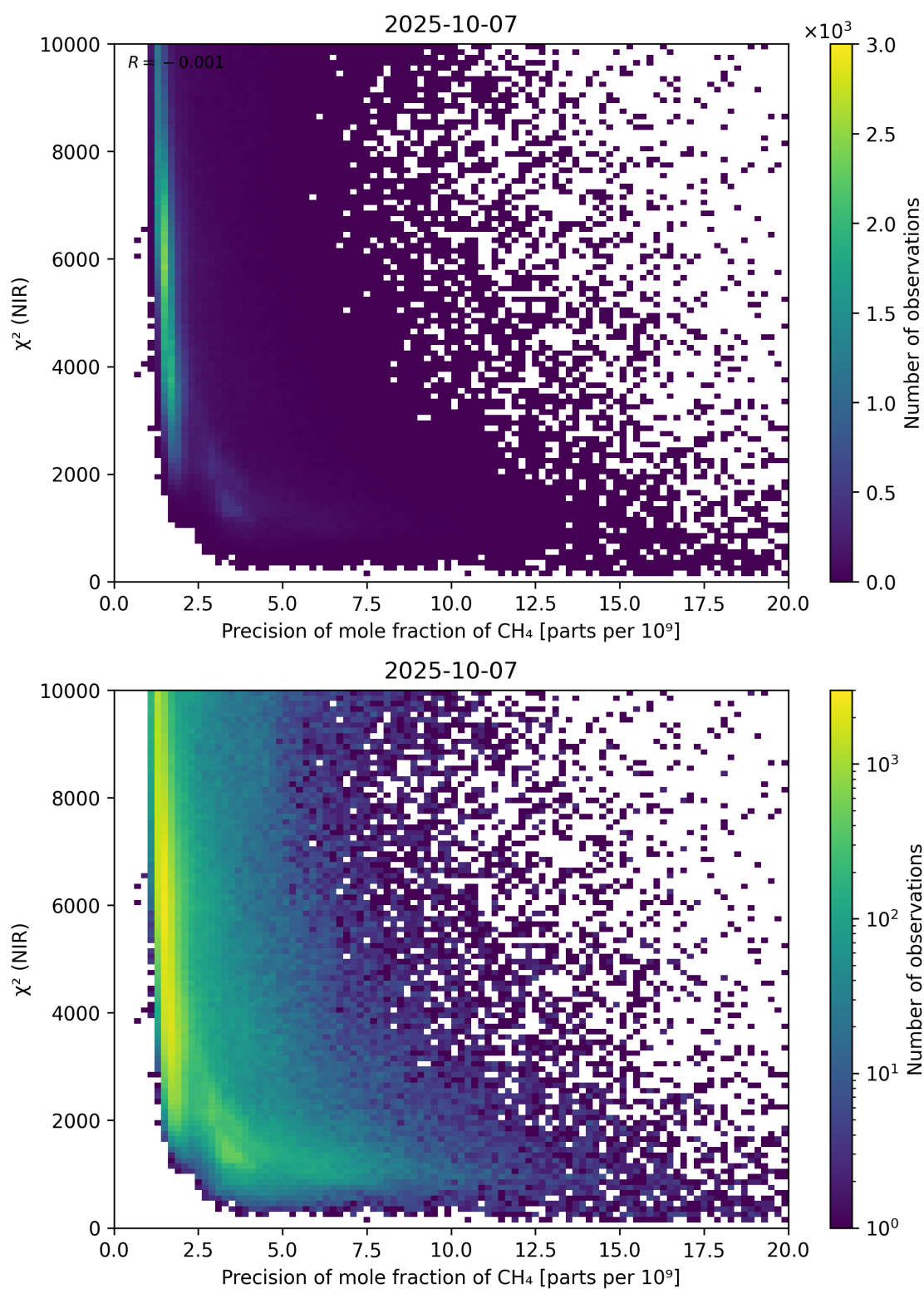
Figure 78: Scatter density plot of “Precision of mole fraction of CH 4 ” against “ \chi^2 (NIR)” for 2025-10-06 to 2025-10-08.
