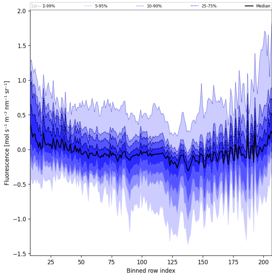
Figure 43: Along track statistics of “Fluorescence” for 2025-10-06 to 2025-10-08
