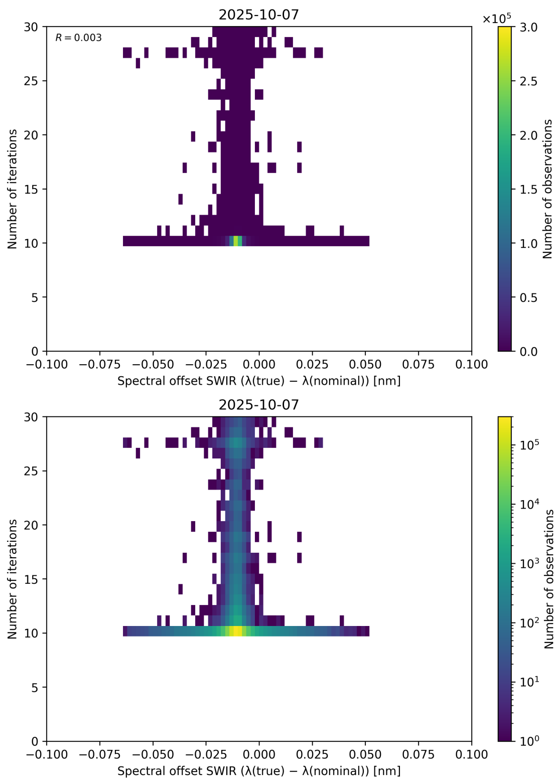
Figure 121: Scatter density plot of “Spectral offset SWIR ( \lambda_{\text{true}} - \lambda_{\text{nominal}} )” against “Number of iterations” for 2025-10-06 to 2025-10-08.
