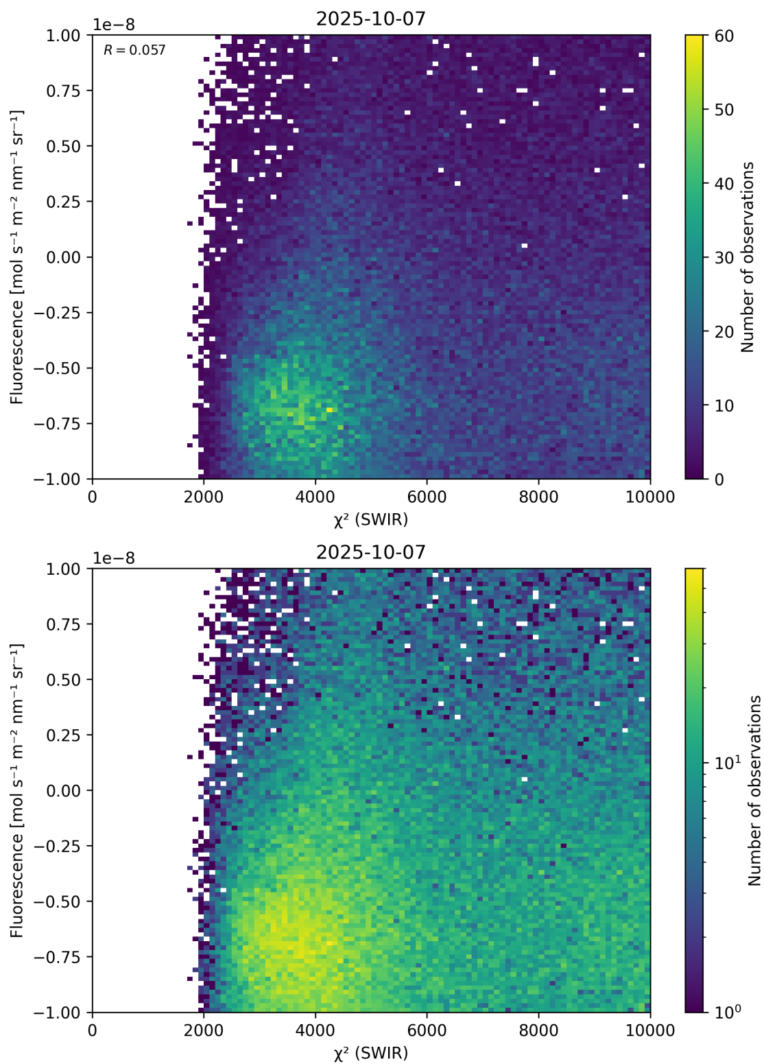
Figure 49: Scatter density plot of “ \chi^2 (SWIR)” against “Fluorescence” for 2025-10-06 to 2025-10-08.
