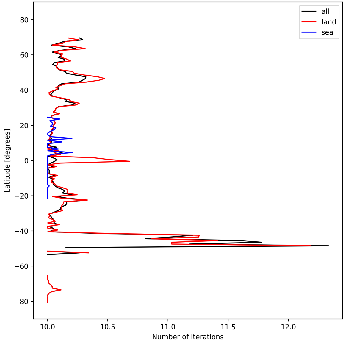
Figure 20: Zonal average of “Number of iterations” for 2025-10-06 to 2025-10-08.
