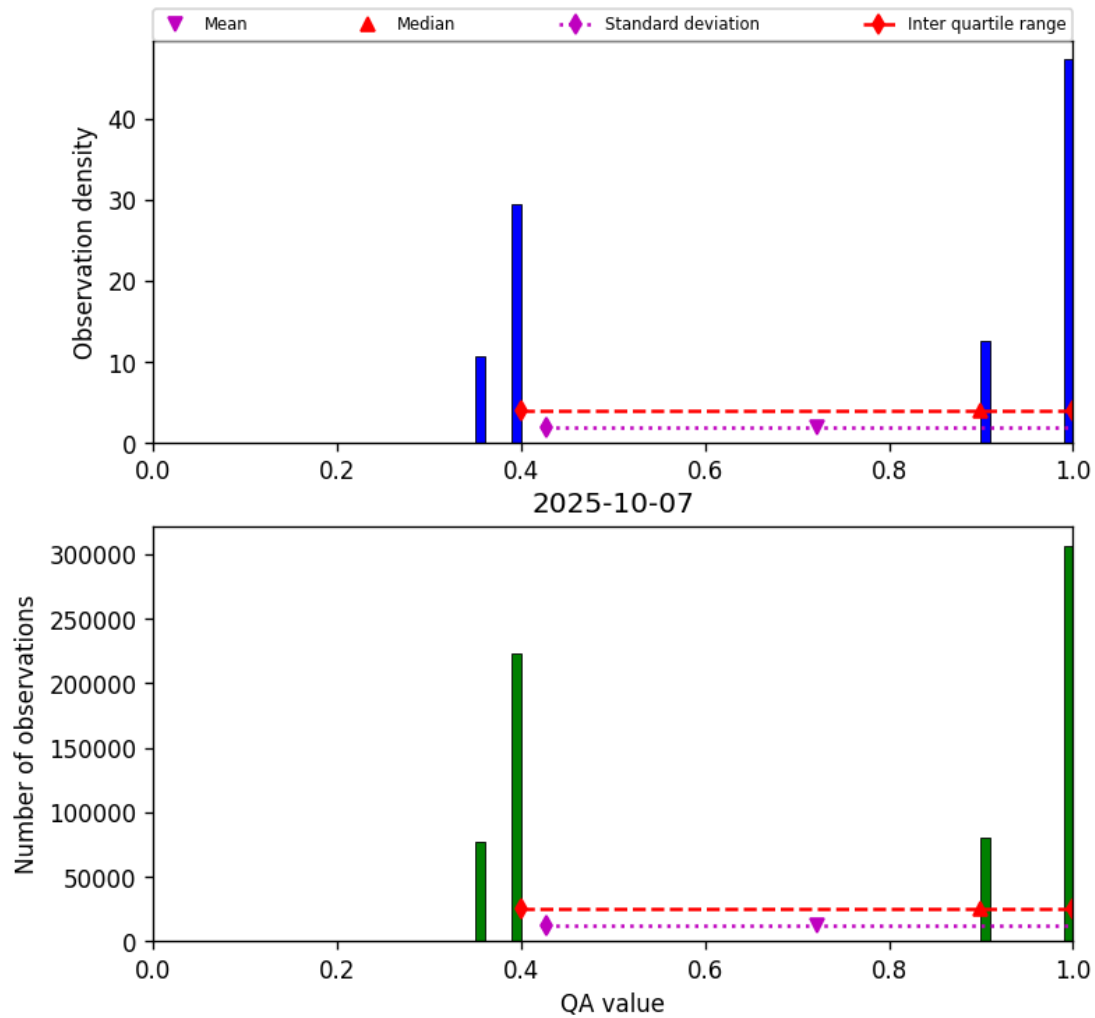
Figure 22: Histogram of “QA value” for 2025-10-06 to 2025-10-08
