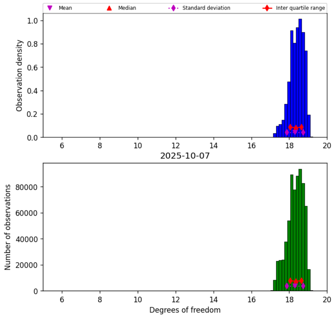
Figure 30: Histogram of “Degrees of freedom” for 2025-10-06 to 2025-10-08
