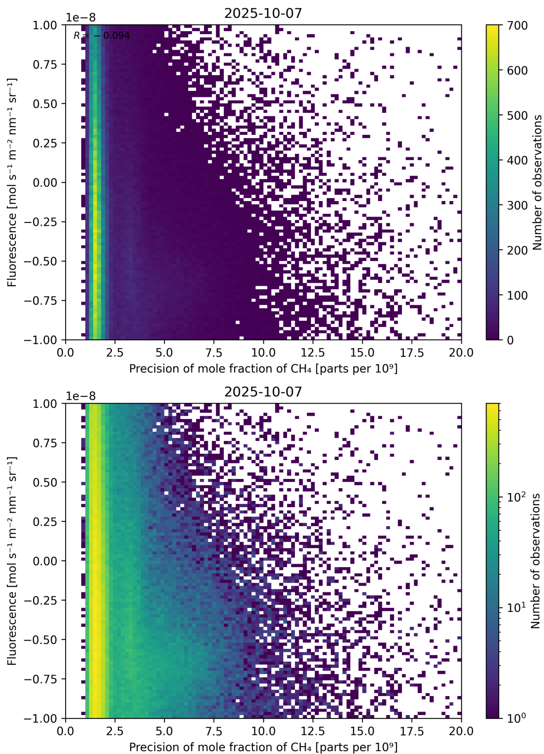
Figure 81: Scatter density plot of “Precision of mole fraction of CH 4 ” against “Fluorescence” for 2025-10-06 to 2025-10-08.
