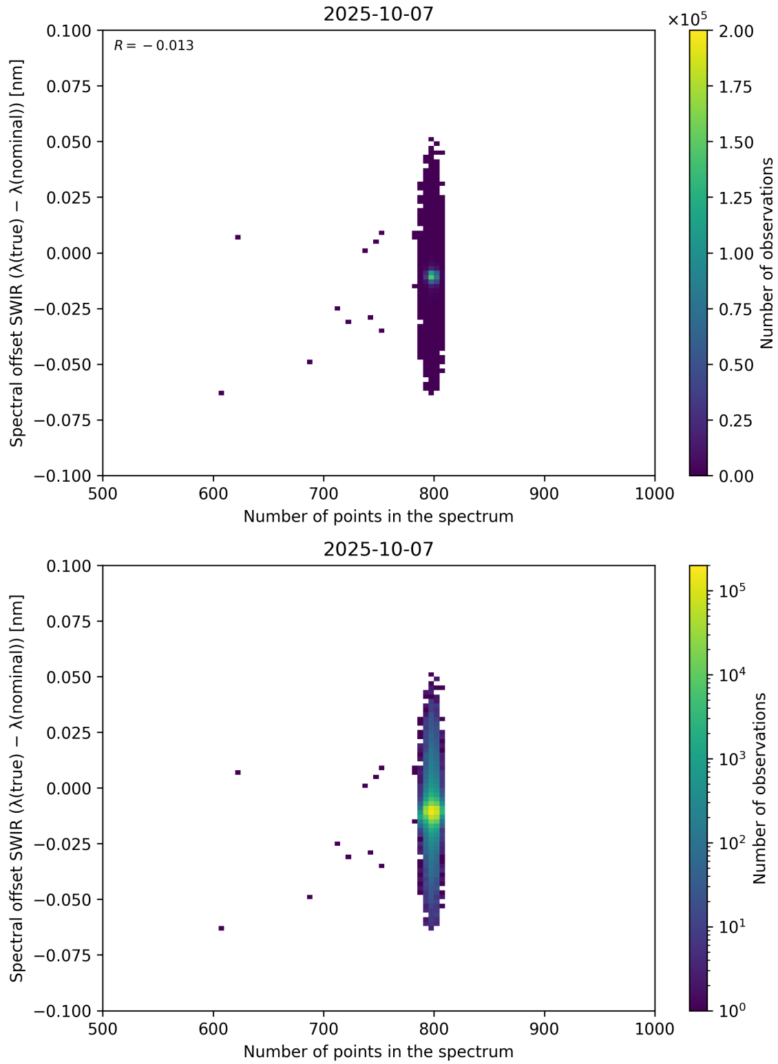
Figure 93: Scatter density plot of “Number of points in the spectrum” against “Spectral offset SWIR ( \lambda_{\text{true}} - \lambda_{\text{nominal}} )” for 2025-10-06 to 2025-10-08.
