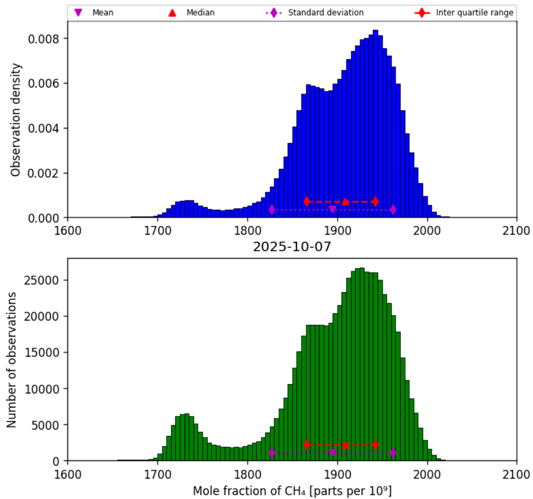
Figure 23: Histogram of “Mole fraction of CH 4 ” for 2025-10-06 to 2025-10-08
