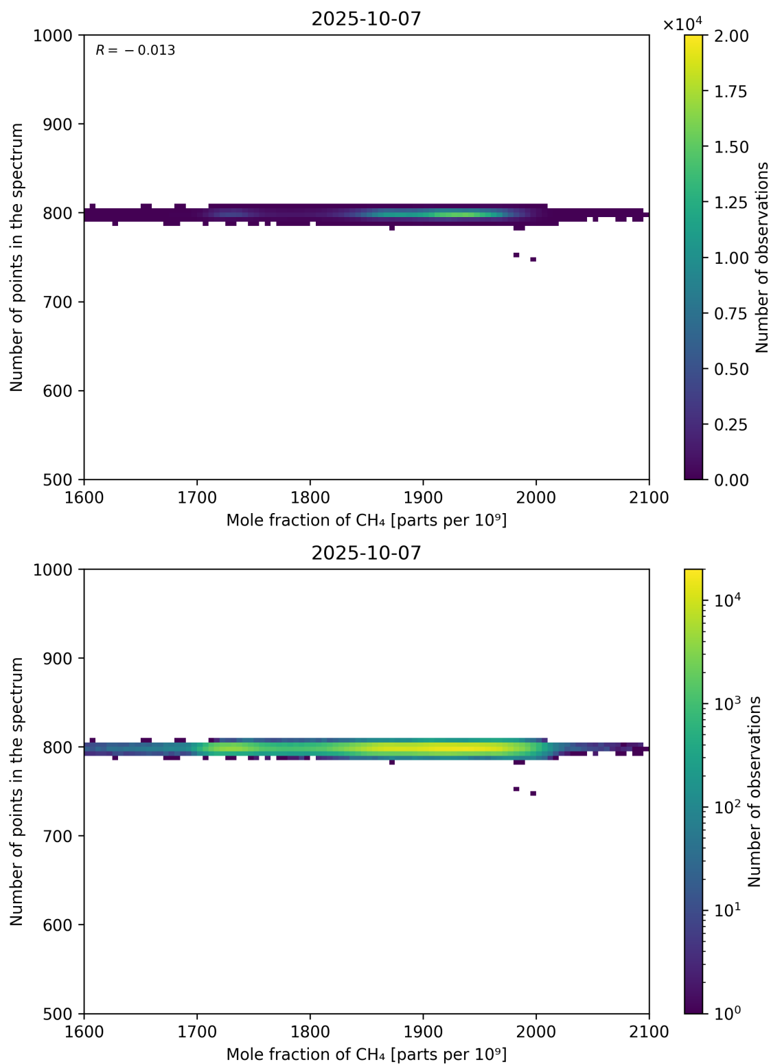
Figure 77: Scatter density plot of “Mole fraction of CH 4 ” against “Number of points in the spectrum” for 2025-10-06 to 2025-10-08.
