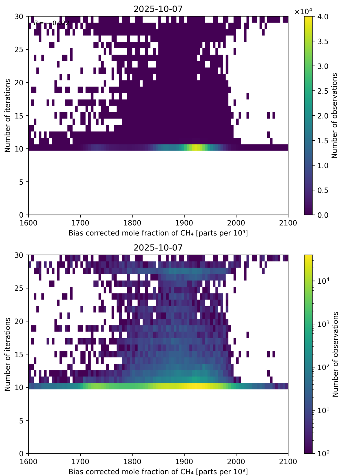
Figure 67: Scatter density plot of “Bias corrected mole fraction of CH 4 ” against “Number of iterations” for 2025-10-06 to 2025-10-08.
