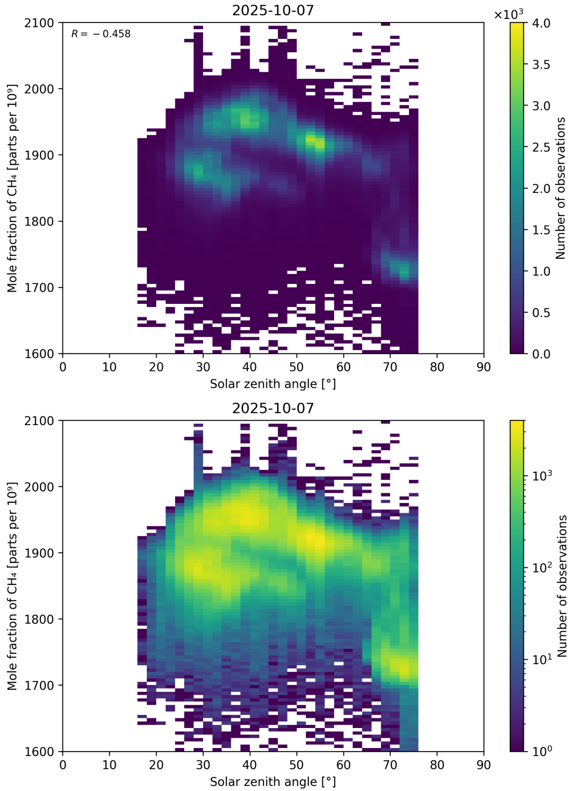
Figure 99: Scatter density plot of “Solar zenith angle” against “Mole fraction of CH 4 ” for 2025-10-06 to 2025-10-08.
