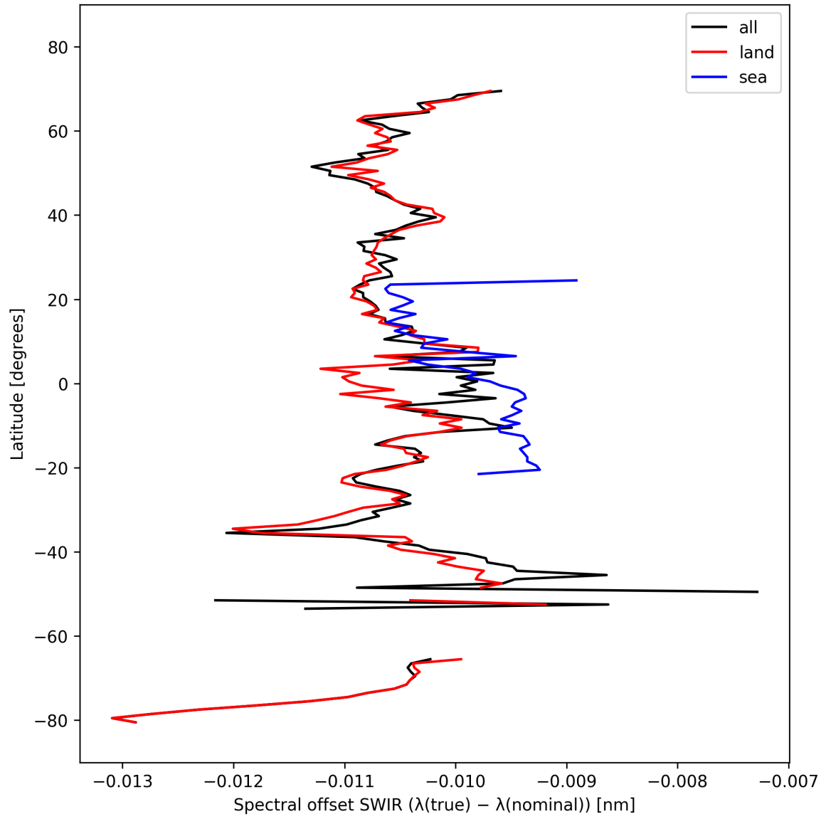
Figure 16: Zonal average of “Spectral offset SWIR ( \lambda_{\text{true}} - \lambda_{\text{nominal}} )” for 2025-10-06 to 2025-10-08.
