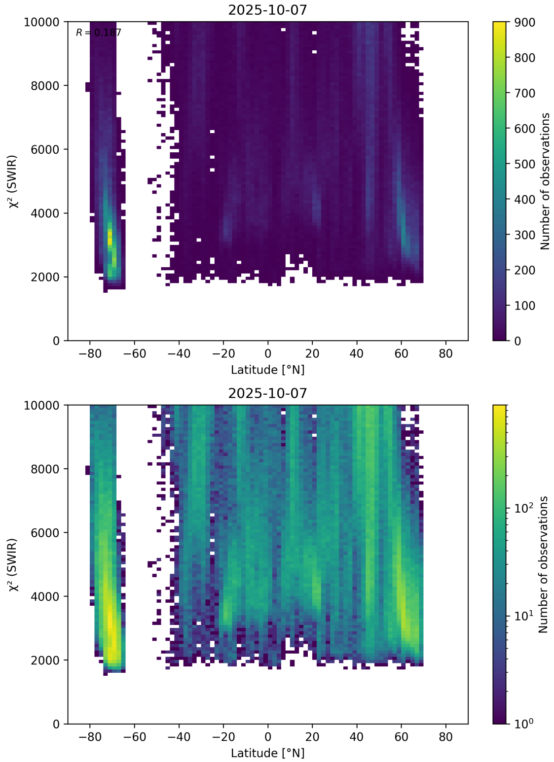
Figure 54: Scatter density plot of “Latitude” against “ \chi^2 (SWIR)” for 2025-10-06 to 2025-10-08.
