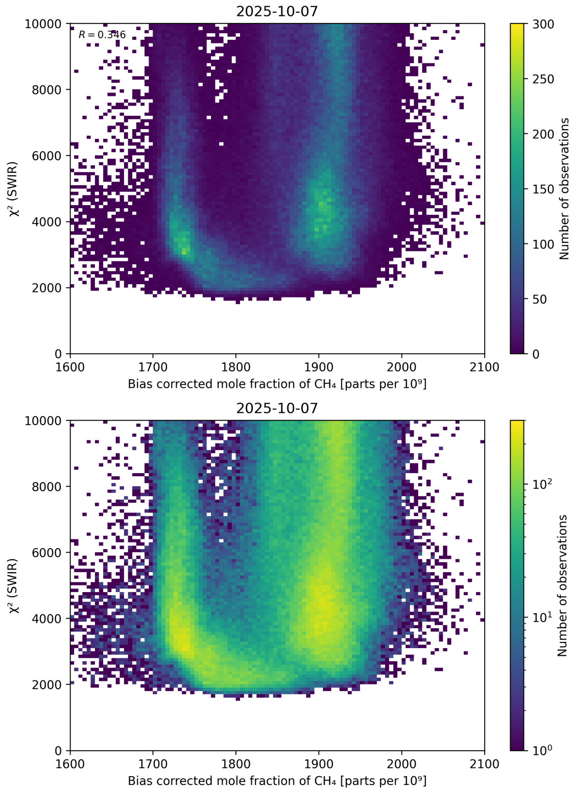
Figure 64: Scatter density plot of “Bias corrected mole fraction of \text{CH}_4 ” against “ \chi^2 (SWIR)” for 2025-10-06 to 2025-10-08.
