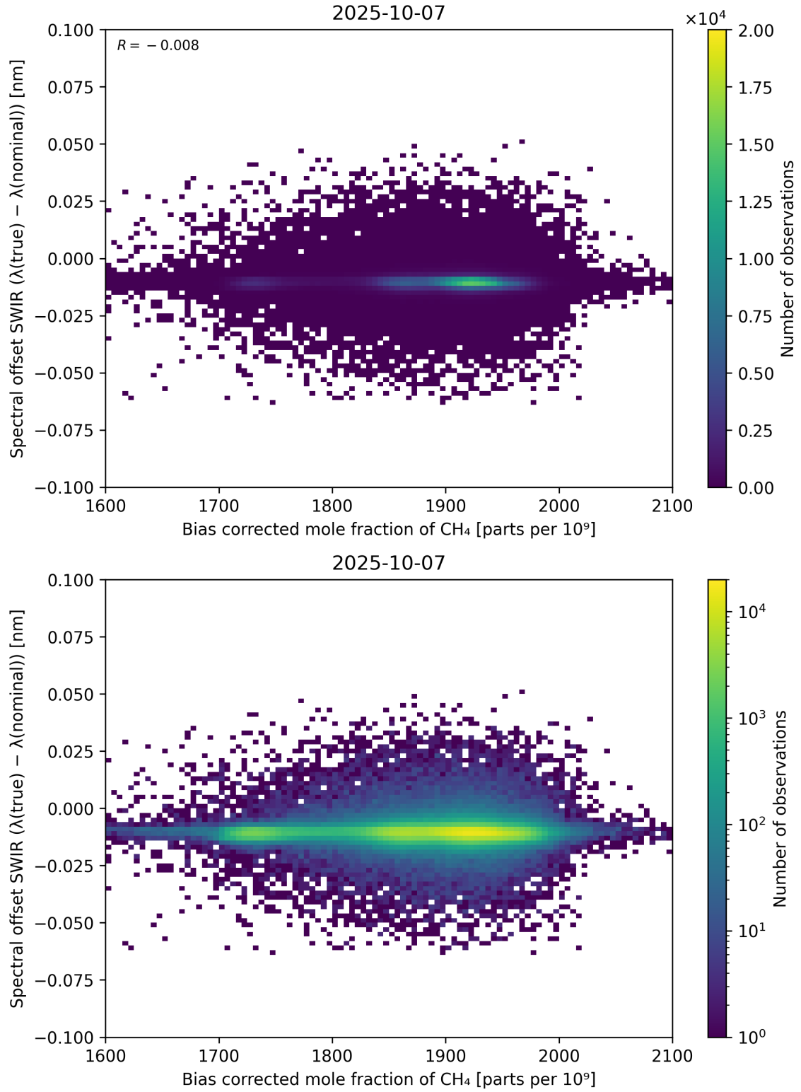
Figure 69: Scatter density plot of “Bias corrected mole fraction of \text{CH}_4 ” against “Spectral offset SWIR ( \lambda_{\text{true}} - \lambda_{\text{nominal}} )” for 2025-10-06 to 2025-10-08.
