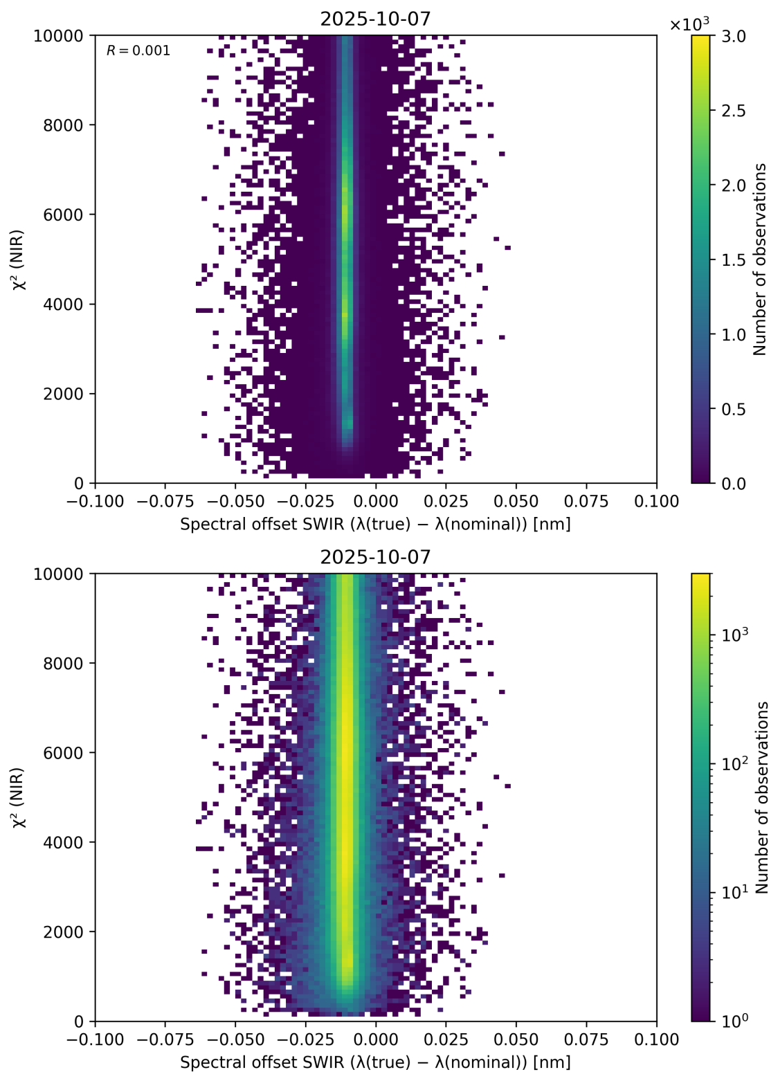
Figure 117: Scatter density plot of “Spectral offset SWIR ( \lambda_{\text{true}} - \lambda_{\text{nominal}} )” against “ \chi^2 (NIR)” for 2025-10-06 to 2025-10-08.
