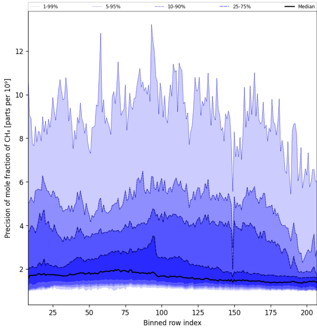
Figure 35: Along track statistics of “Precision of mole fraction of CH 4 ” for 2025-10-06 to 2025-10-08
