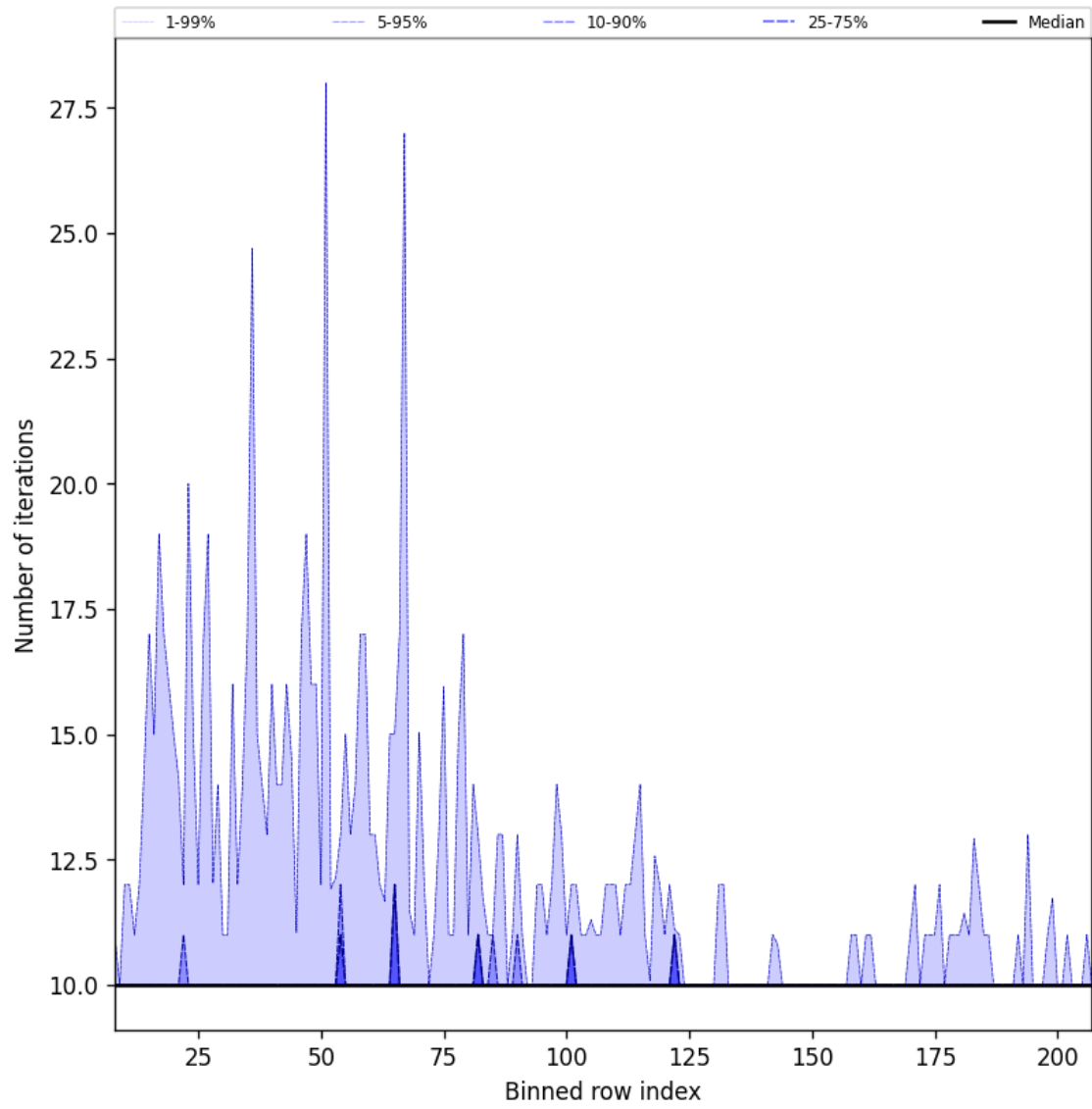
Figure 42: Along track statistics of “Number of iterations” for 2025-10-06 to 2025-10-08
