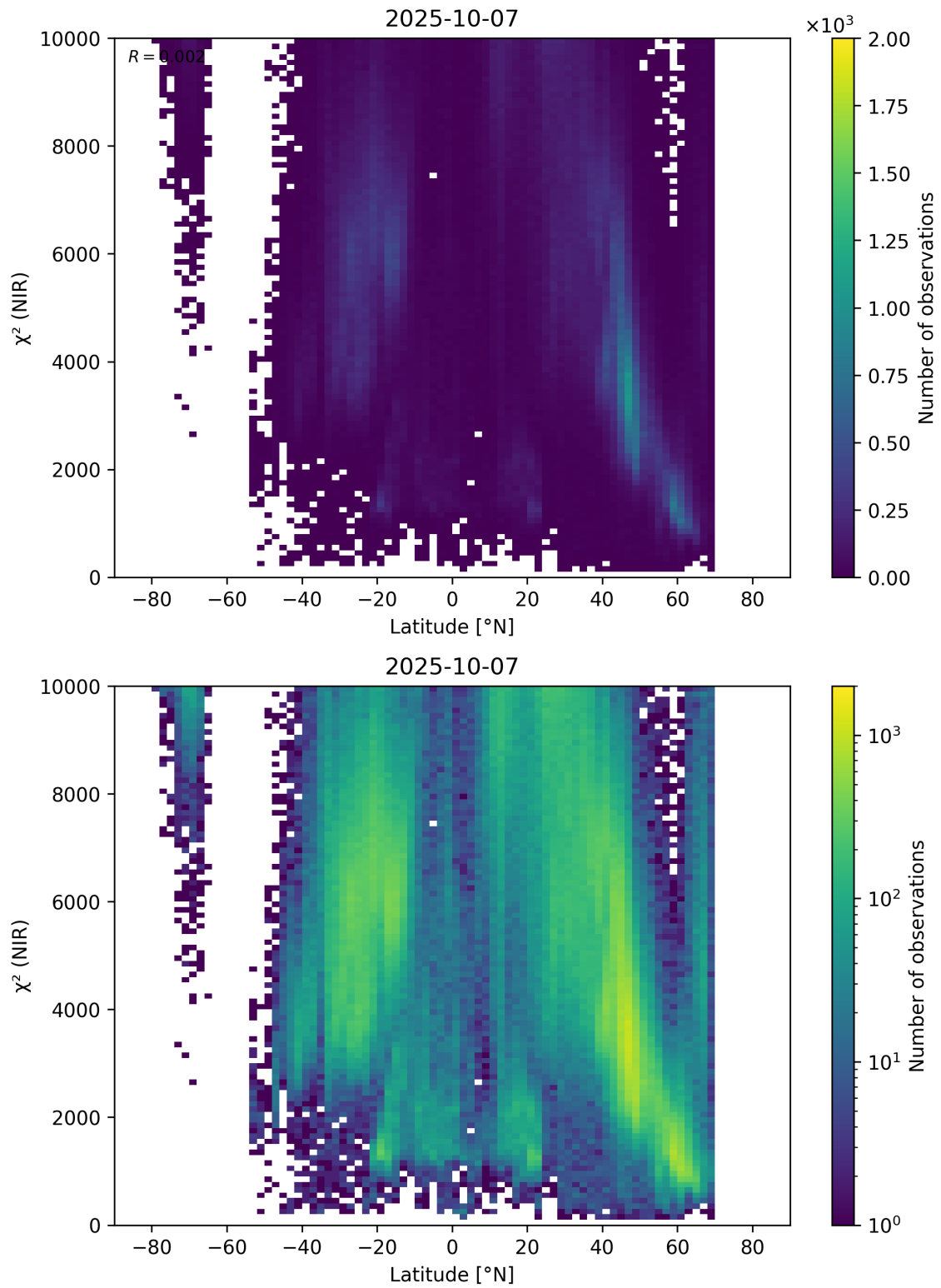
Figure 53: Scatter density plot of “Latitude” against “ \chi^2 (NIR)” for 2025-10-06 to 2025-10-08.
