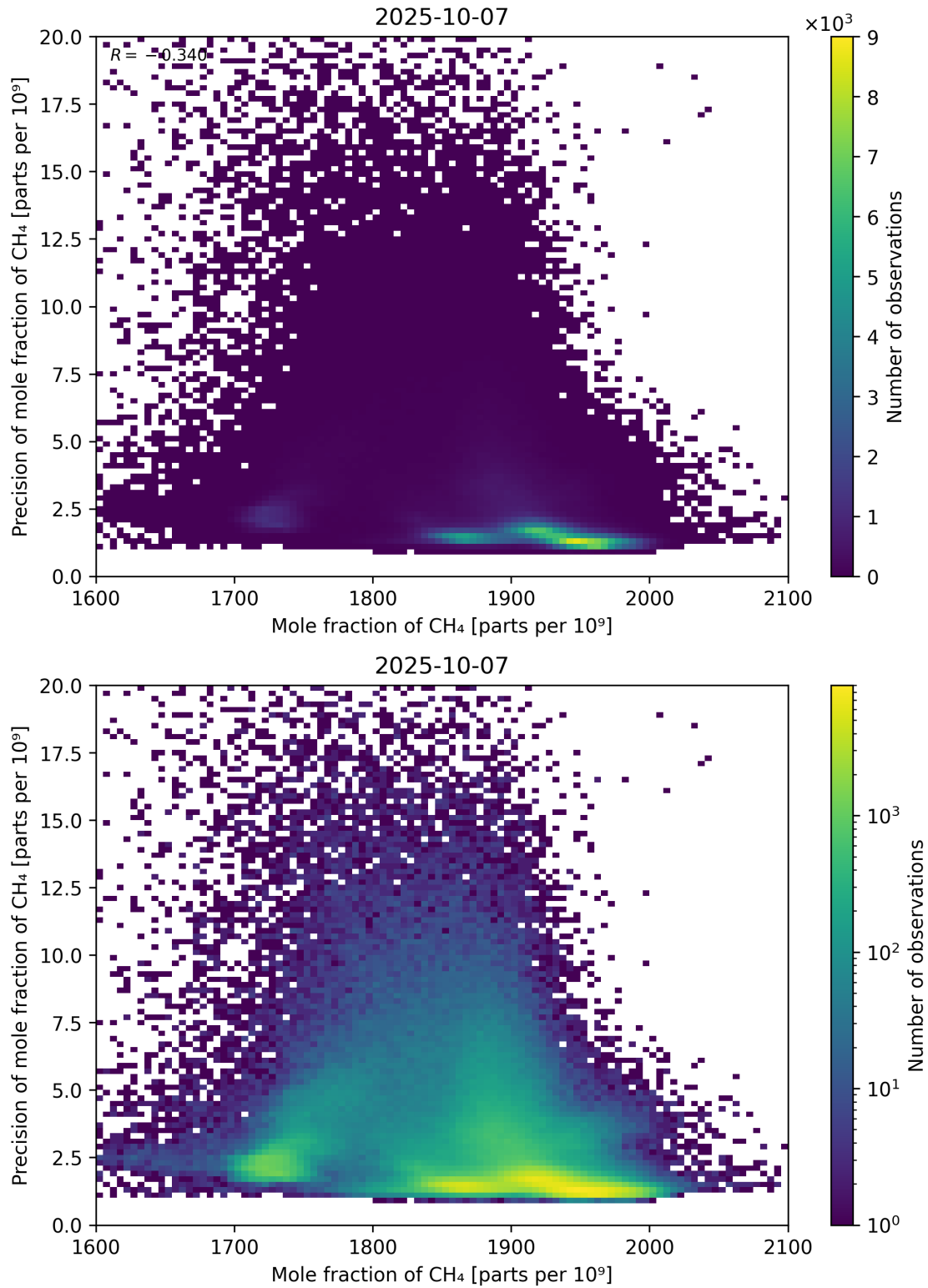
Figure 75: Scatter density plot of “Mole fraction of CH 4 ” against “Precision of mole fraction of CH 4 ” for 2025-10-06 to 2025-10-08.
