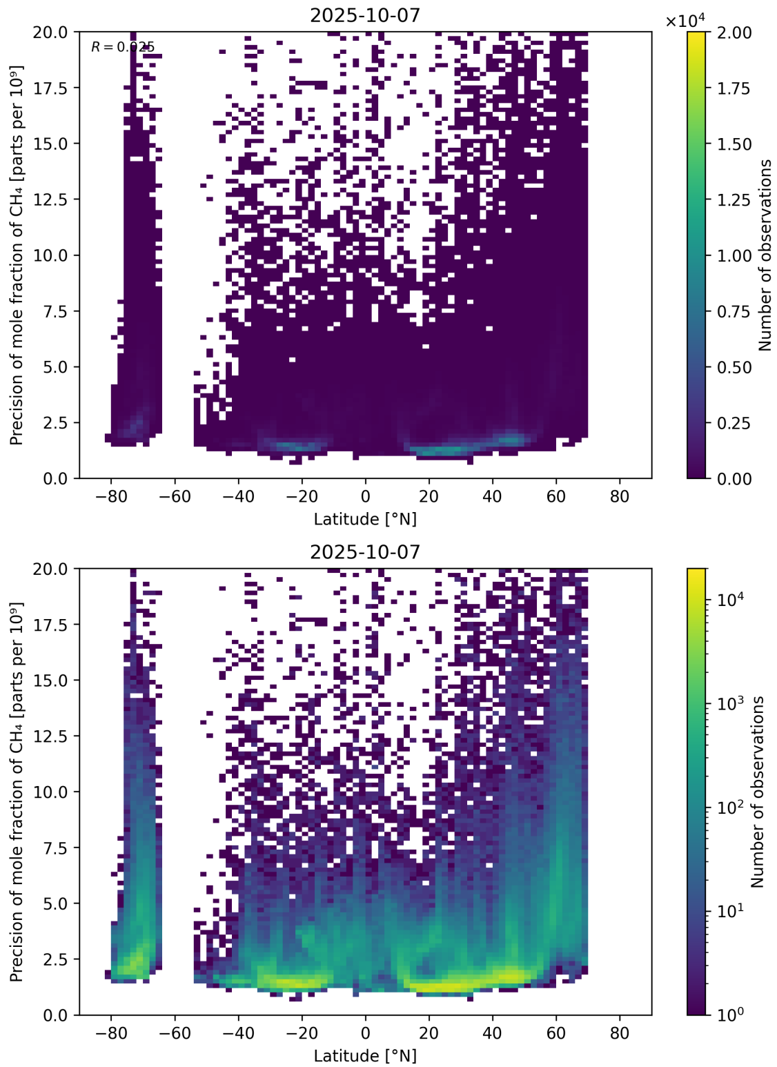
Figure 59: Scatter density plot of “Latitude” against “Precision of mole fraction of CH 4 ” for 2025-10-06 to 2025-10-08.
