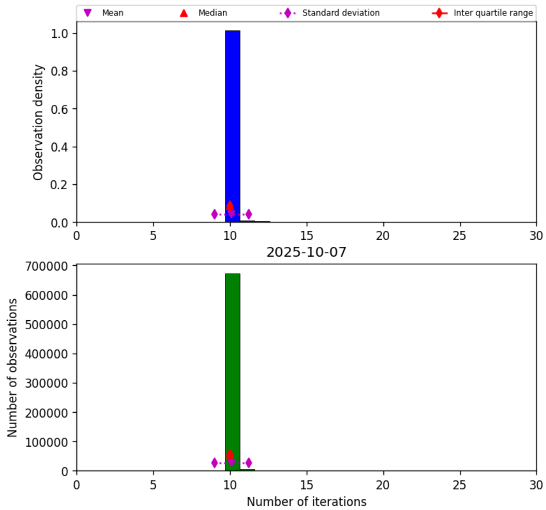
Figure 31: Histogram of “Number of iterations” for 2025-10-06 to 2025-10-08
