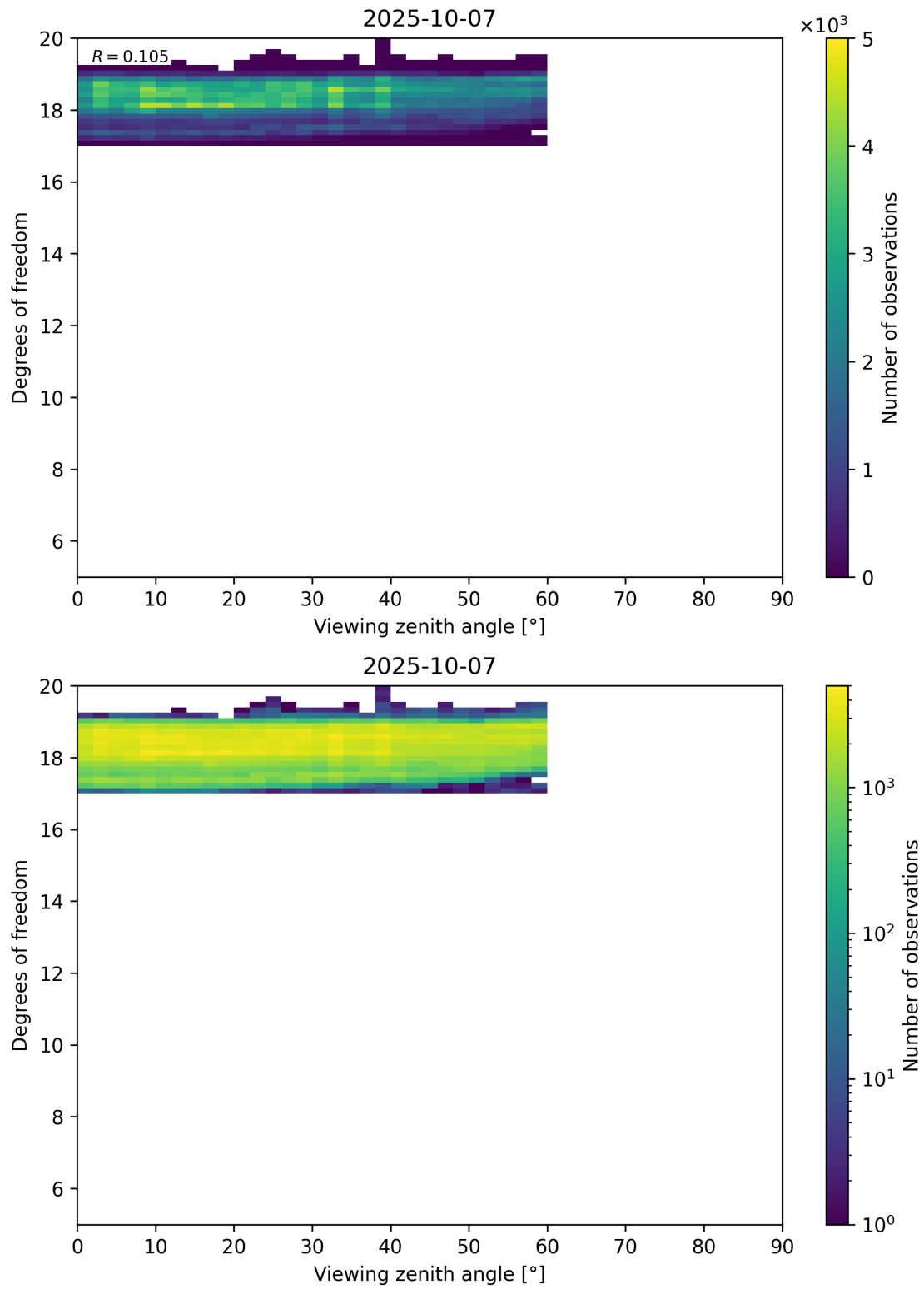
Figure 107: Scatter density plot of “Viewing zenith angle” against “Degrees of freedom” for 2025-10-06 to 2025-10-08.
