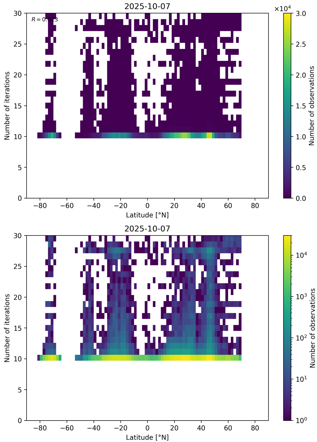
Figure 60: Scatter density plot of “Latitude” against “Number of iterations” for 2025-10-06 to 2025-10-08.
