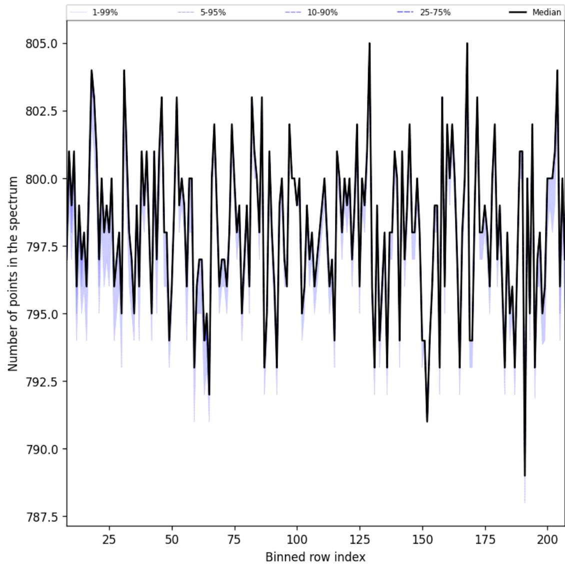
Figure 37: Along track statistics of “Number of points in the spectrum” for 2025-10-06 to 2025-10-08
