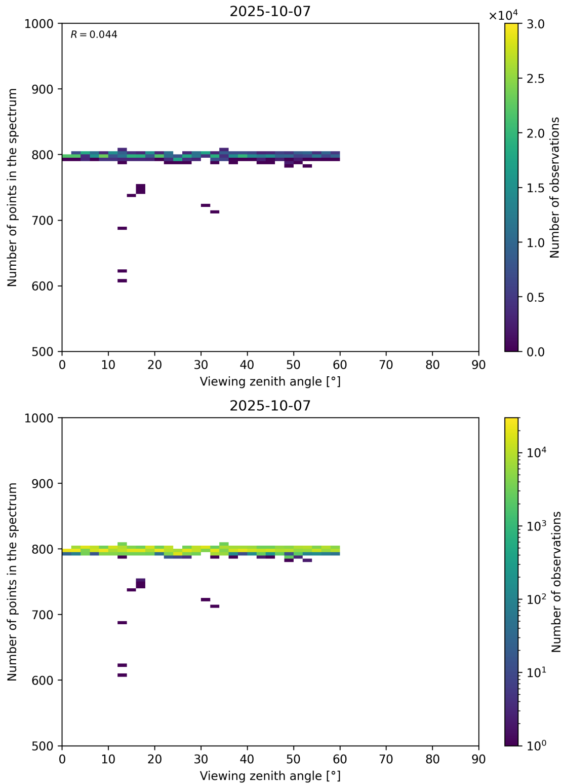
Figure 114: Scatter density plot of “Viewing zenith angle” against “Number of points in the spectrum” for 2025-10-06 to 2025-10-08.
