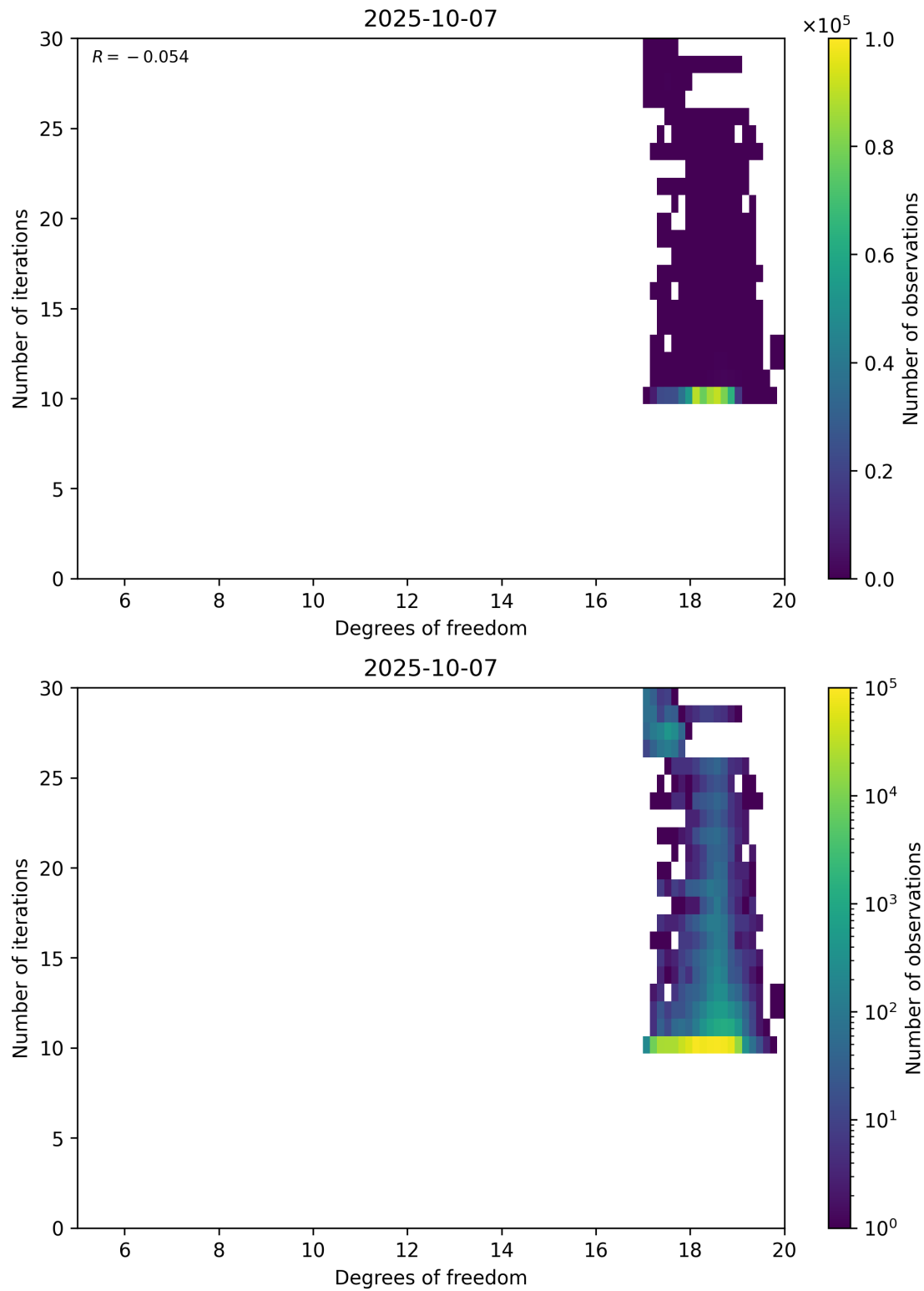
Figure 52: Scatter density plot of “Degrees of freedom” against “Number of iterations” for 2025-10-06 to 2025-10-08.
