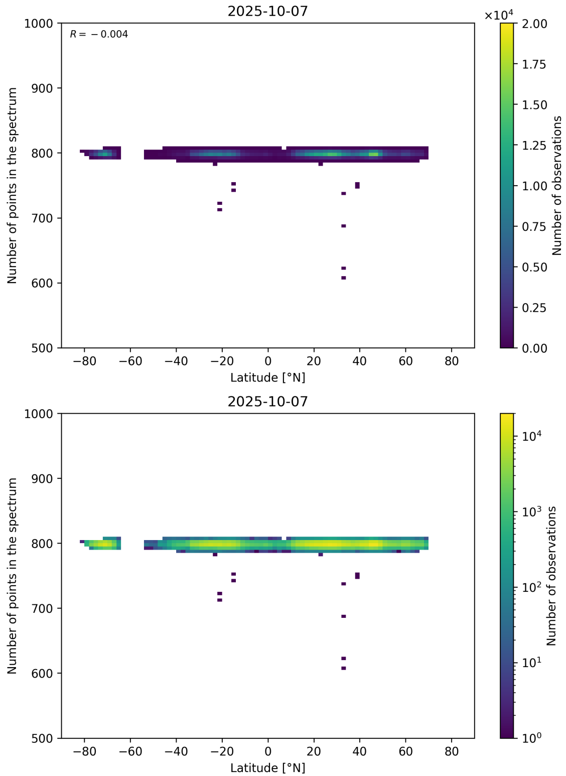
Figure 61: Scatter density plot of “Latitude” against “Number of points in the spectrum” for 2025-10-06 to 2025-10-08.
