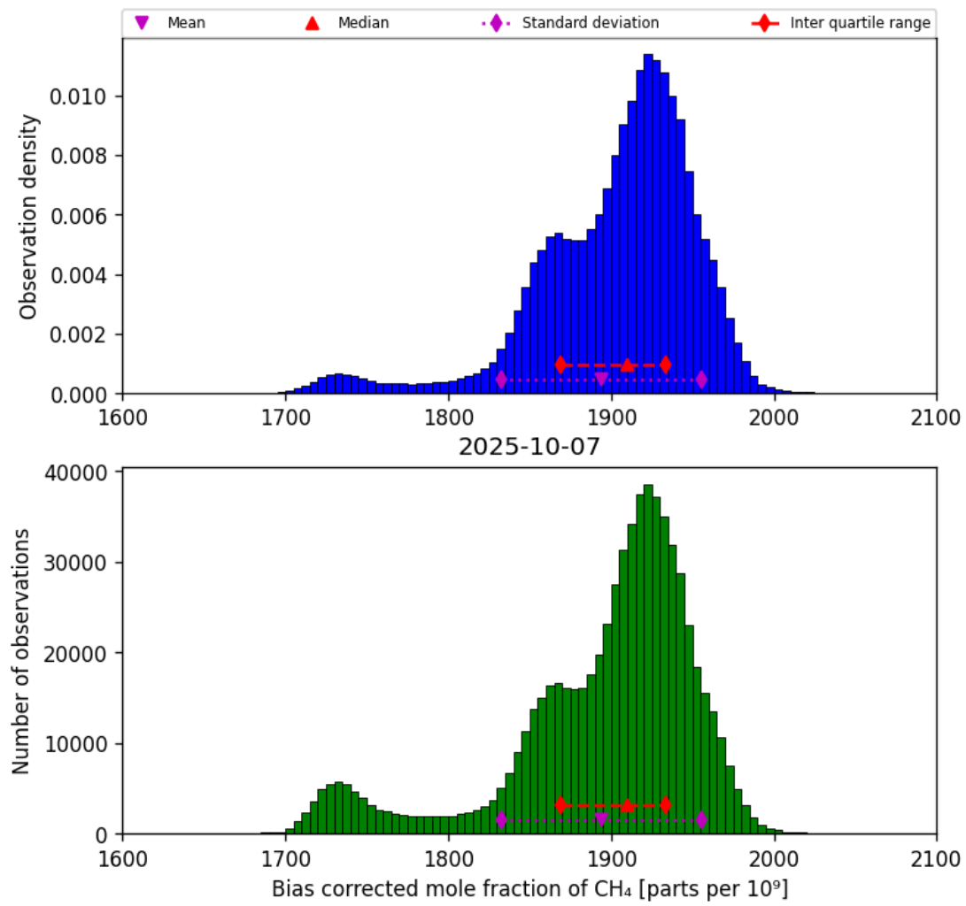
Figure 25: Histogram of “Bias corrected mole fraction of CH 4 ” for 2025-10-06 to 2025-10-08
