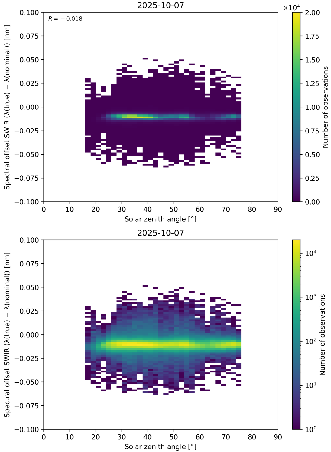
Figure 104: Scatter density plot of “Solar zenith angle” against “Spectral offset SWIR ( \lambda_{\text{true}} - \lambda_{\text{nominal}} )” for 2025-10-06 to 2025-10-08.
