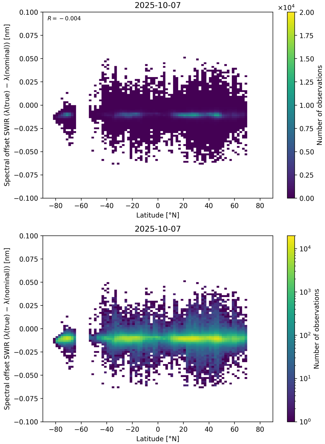
Figure 62: Scatter density plot of “Latitude” against “Spectral offset SWIR ( \lambda_{\text{true}} - \lambda_{\text{nominal}} )” for 2025-10-06 to 2025-10-08.
