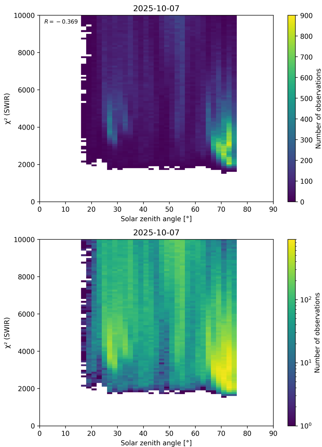
Figure 95: Scatter density plot of “Solar zenith angle” against “ \chi^2 (SWIR)” for 2025-10-06 to 2025-10-08.
