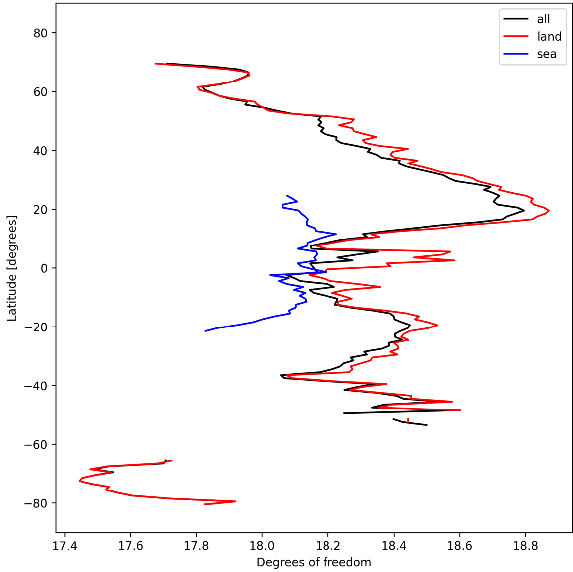
Figure 19: Zonal average of “Degrees of freedom” for 2025-10-06 to 2025-10-08.
