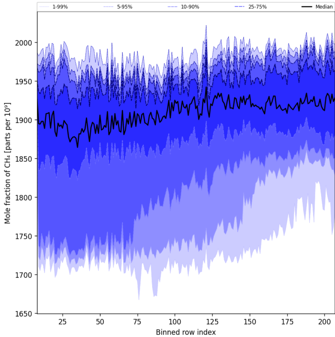
Figure 34: Along track statistics of “Mole fraction of CH 4 ” for 2025-10-06 to 2025-10-08
