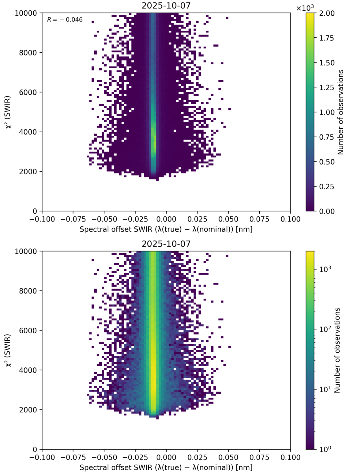
Figure 118: Scatter density plot of “Spectral offset SWIR ( \lambda_{\text{true}} - \lambda_{\text{nominal}} )” against “ \chi^2 (SWIR)” for 2025-10-06 to 2025-10-08.
