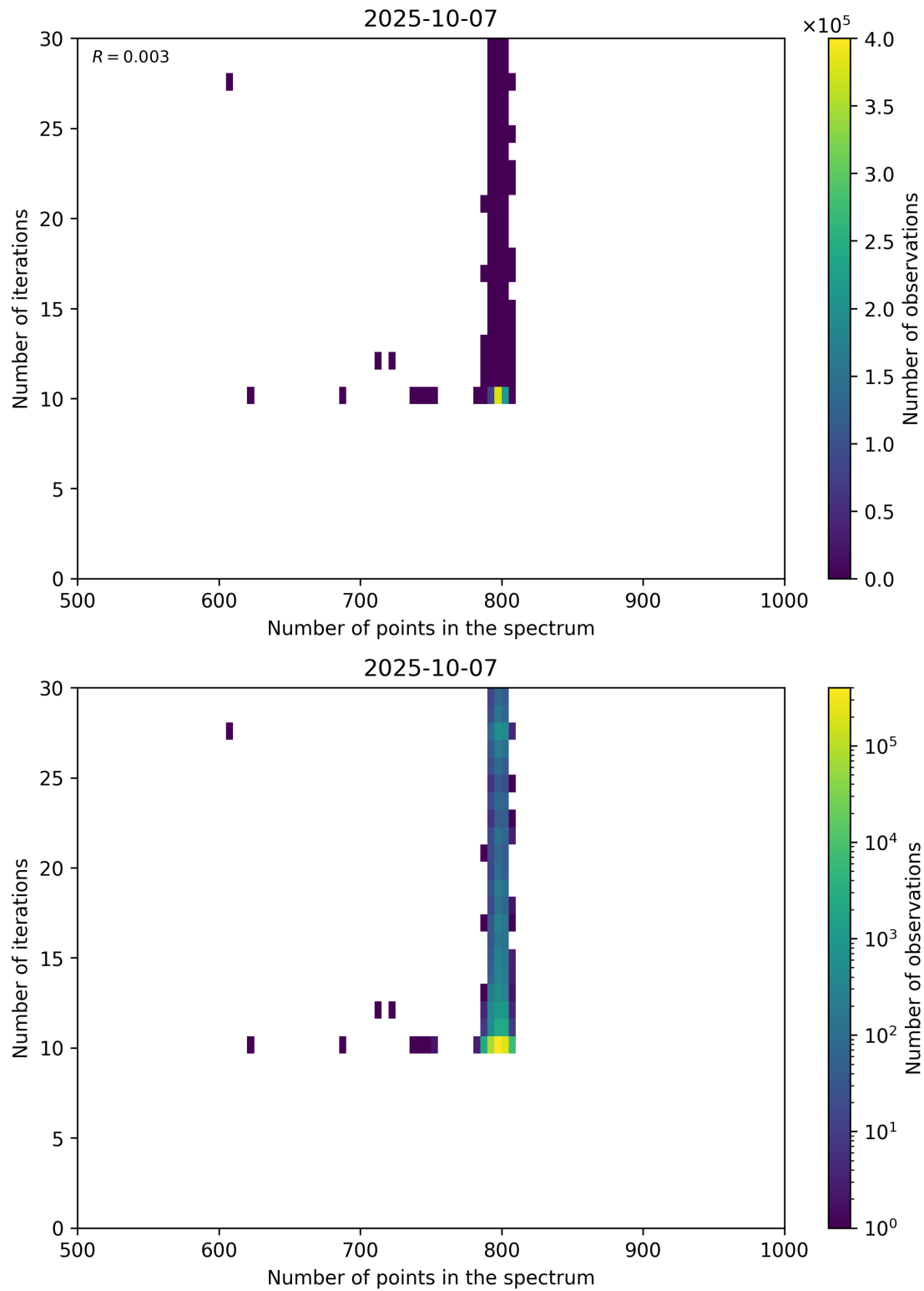
Figure 92: Scatter density plot of “Number of points in the spectrum” against “Number of iterations” for 2025-10-06 to 2025-10-08.
