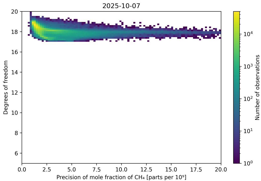
Figure 80: Scatter density plot of “Precision of mole fraction of CH 4 ” against “Degrees of freedom” for 2025-10-06 to 2025-10-08.
