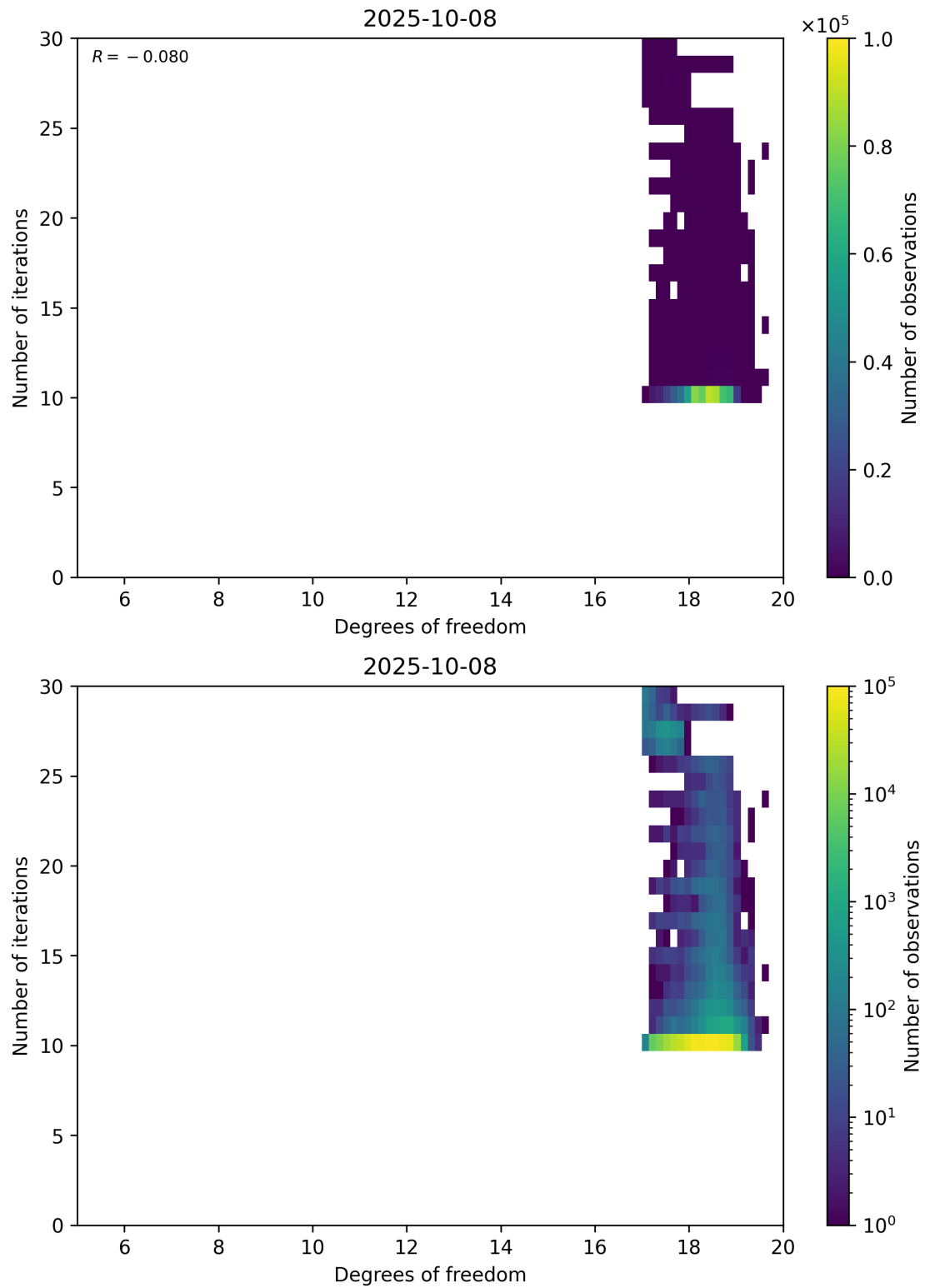
Figure 52: Scatter density plot of “Degrees of freedom” against “Number of iterations” for 2025-10-07 to 2025-10-09.
