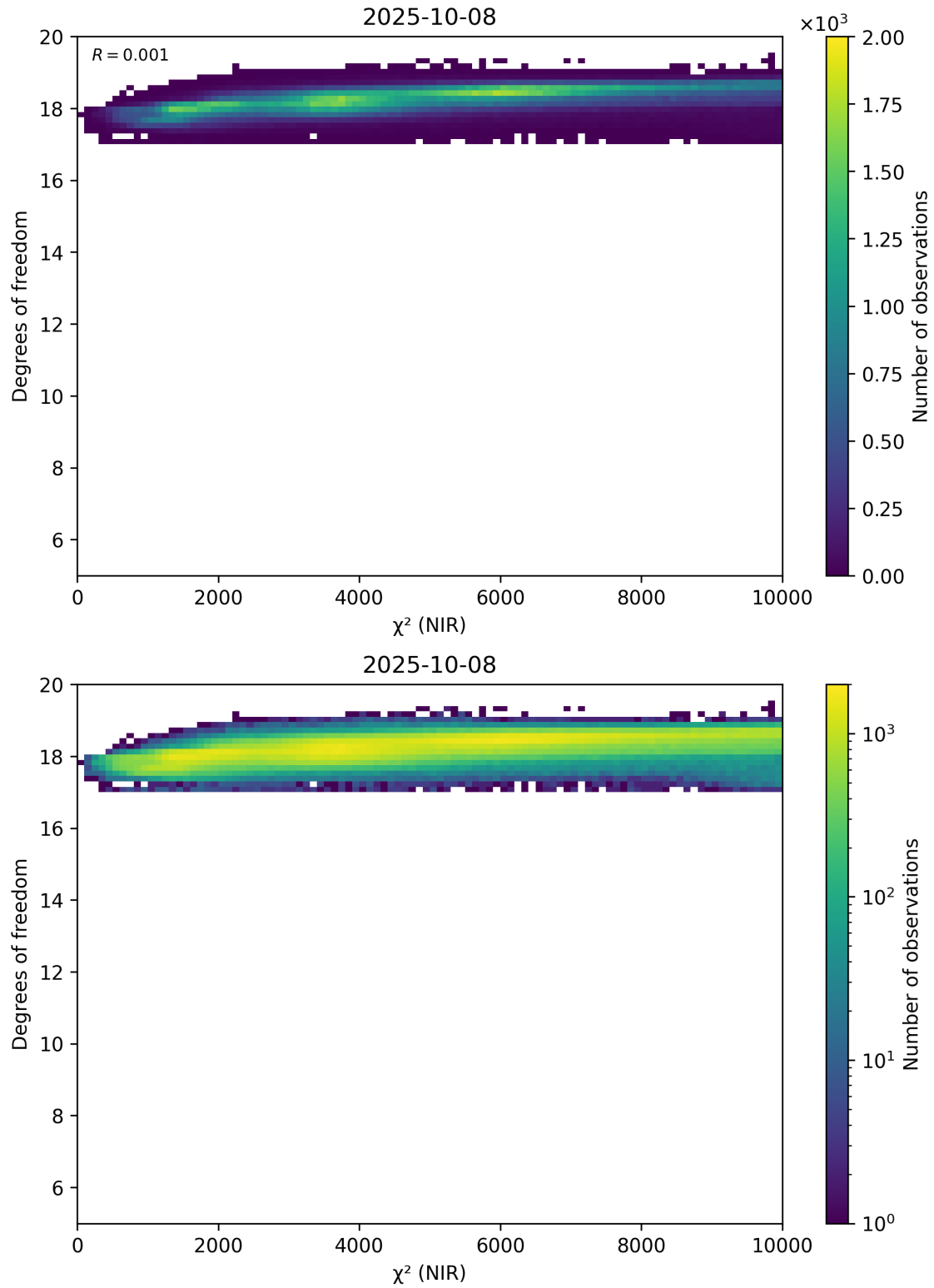
Figure 44: Scatter density plot of “ \chi^2 (NIR)” against “Degrees of freedom” for 2025-10-07 to 2025-10-09.
