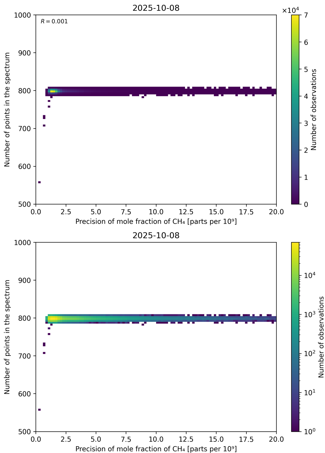
Figure 84: Scatter density plot of “Precision of mole fraction of CH 4 ” against “Number of points in the spectrum” for 2025-10-07 to 2025-10-09.
