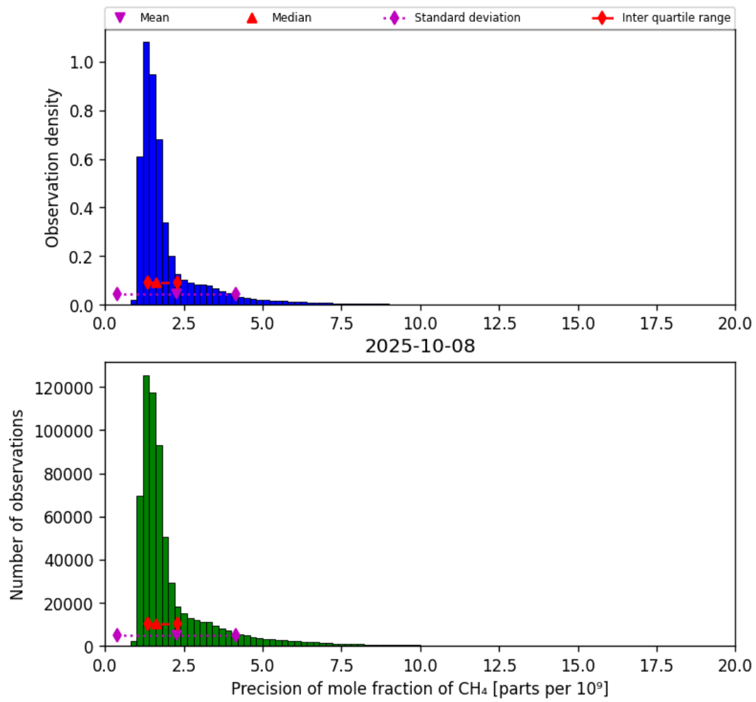
Figure 24: Histogram of “Precision of mole fraction of CH 4 ” for 2025-10-07 to 2025-10-09
