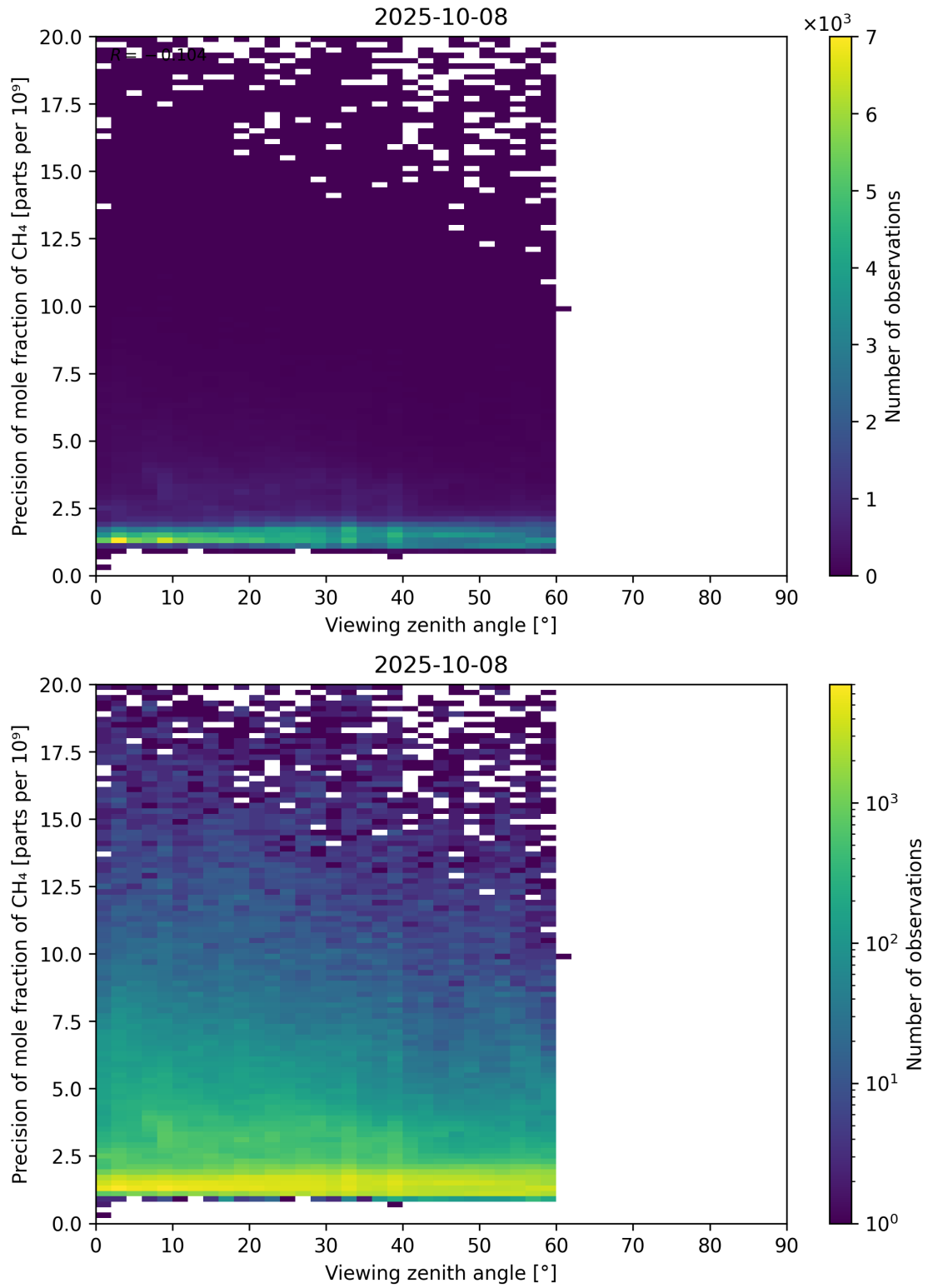
Figure 112: Scatter density plot of “Viewing zenith angle” against “Precision of mole fraction of CH 4 ” for 2025-10-07 to 2025-10-09.
