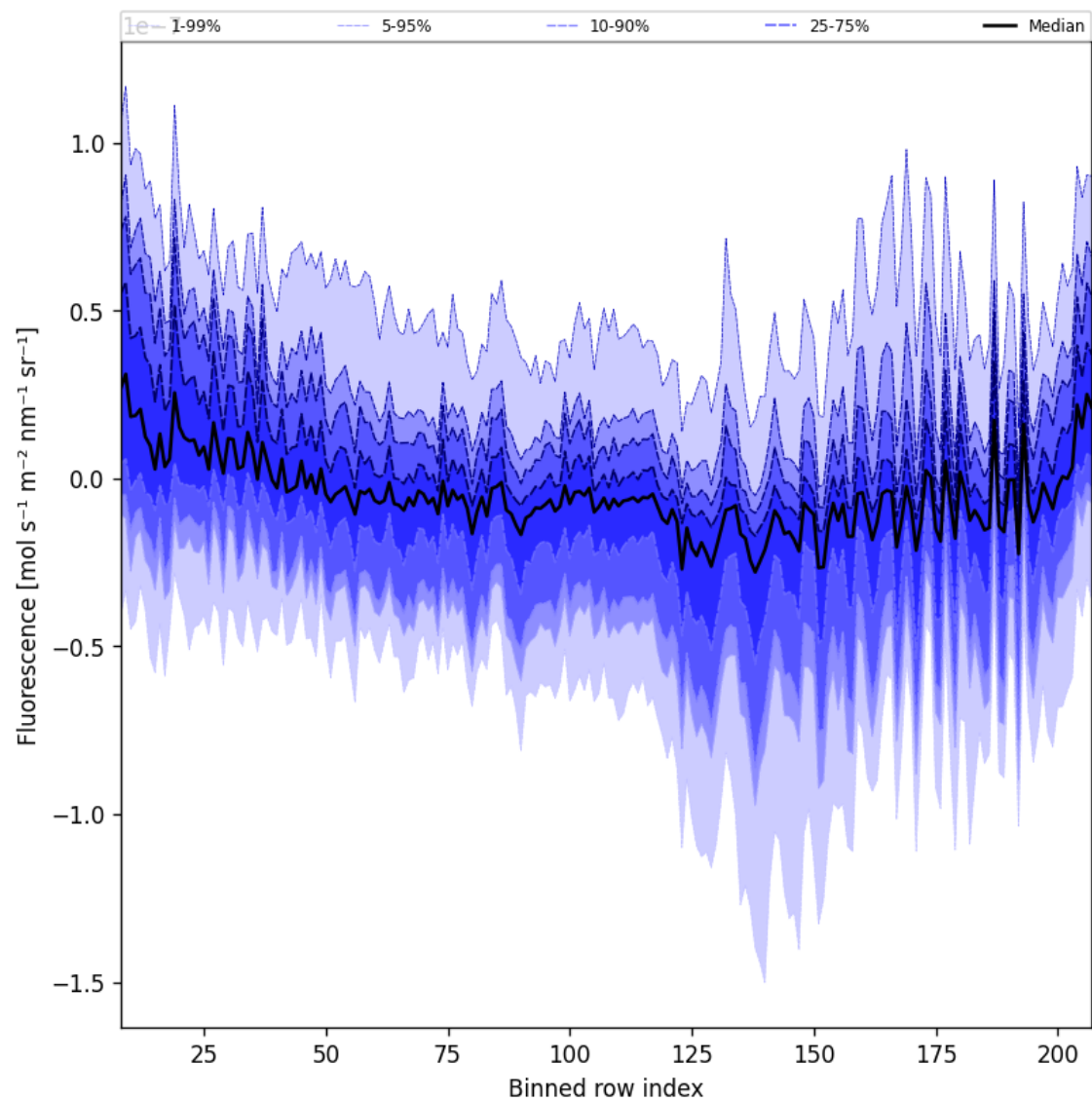
Figure 43: Along track statistics of “Fluorescence” for 2025-10-07 to 2025-10-09
