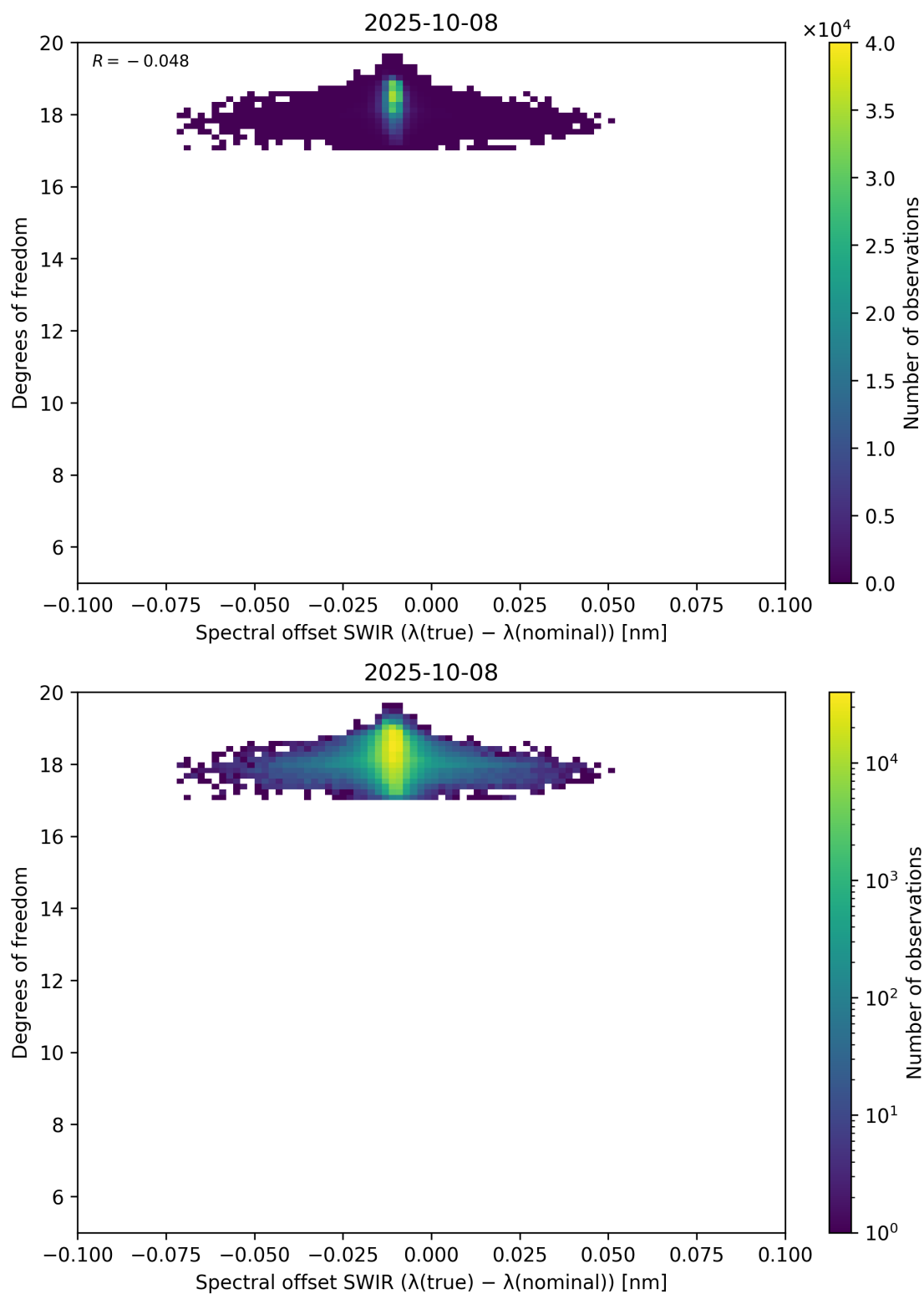
Figure 119: Scatter density plot of “Spectral offset SWIR ( \lambda_{\text{true}} - \lambda_{\text{nominal}} )” against “Degrees of freedom” for 2025-10-07 to 2025-10-09.
