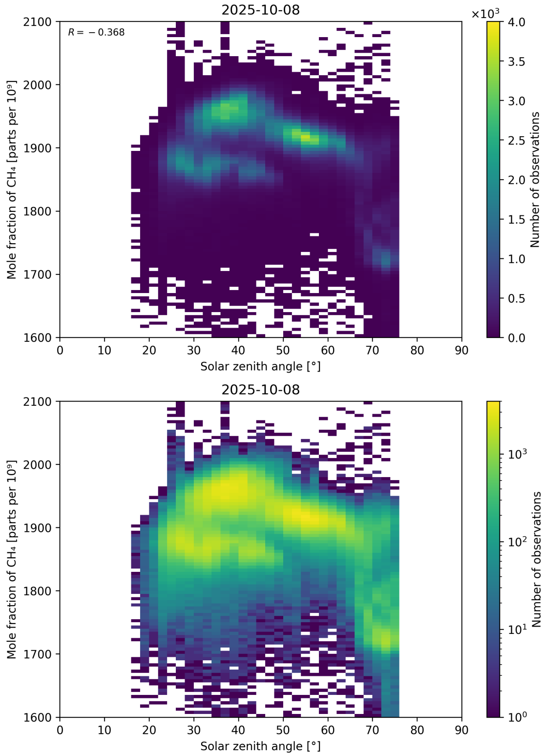
Figure 99: Scatter density plot of “Solar zenith angle” against “Mole fraction of CH 4 ” for 2025-10-07 to 2025-10-09.
