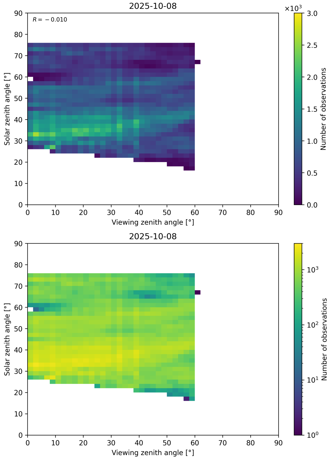
Figure 115: Scatter density plot of “Viewing zenith angle” against “Solar zenith angle” for 2025-10-07 to 2025-10-09.
