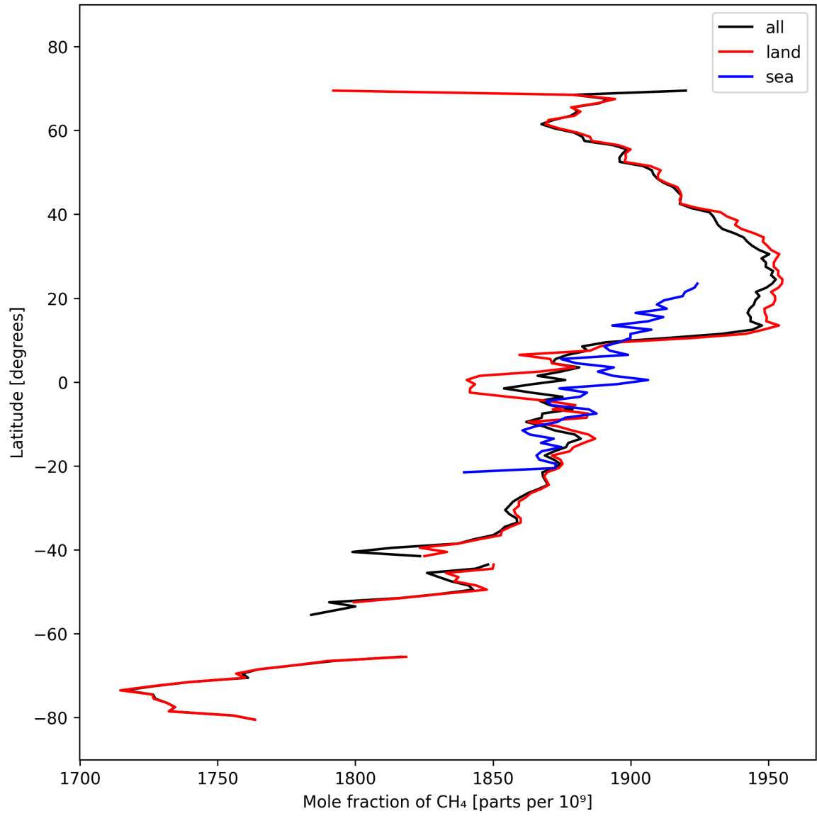
Figure 12: Zonal average of “Mole fraction of \text{CH}_4 ” for 2025-10-07 to 2025-10-09.
