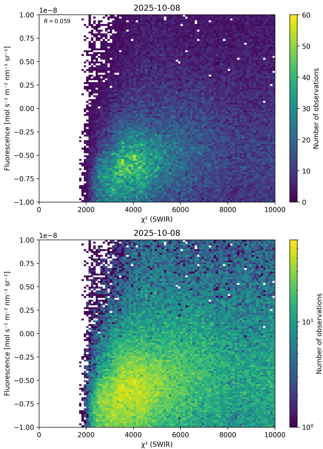
Figure 49: Scatter density plot of “ \chi^2 (SWIR)” against “Fluorescence” for 2025-10-07 to 2025-10-09.
