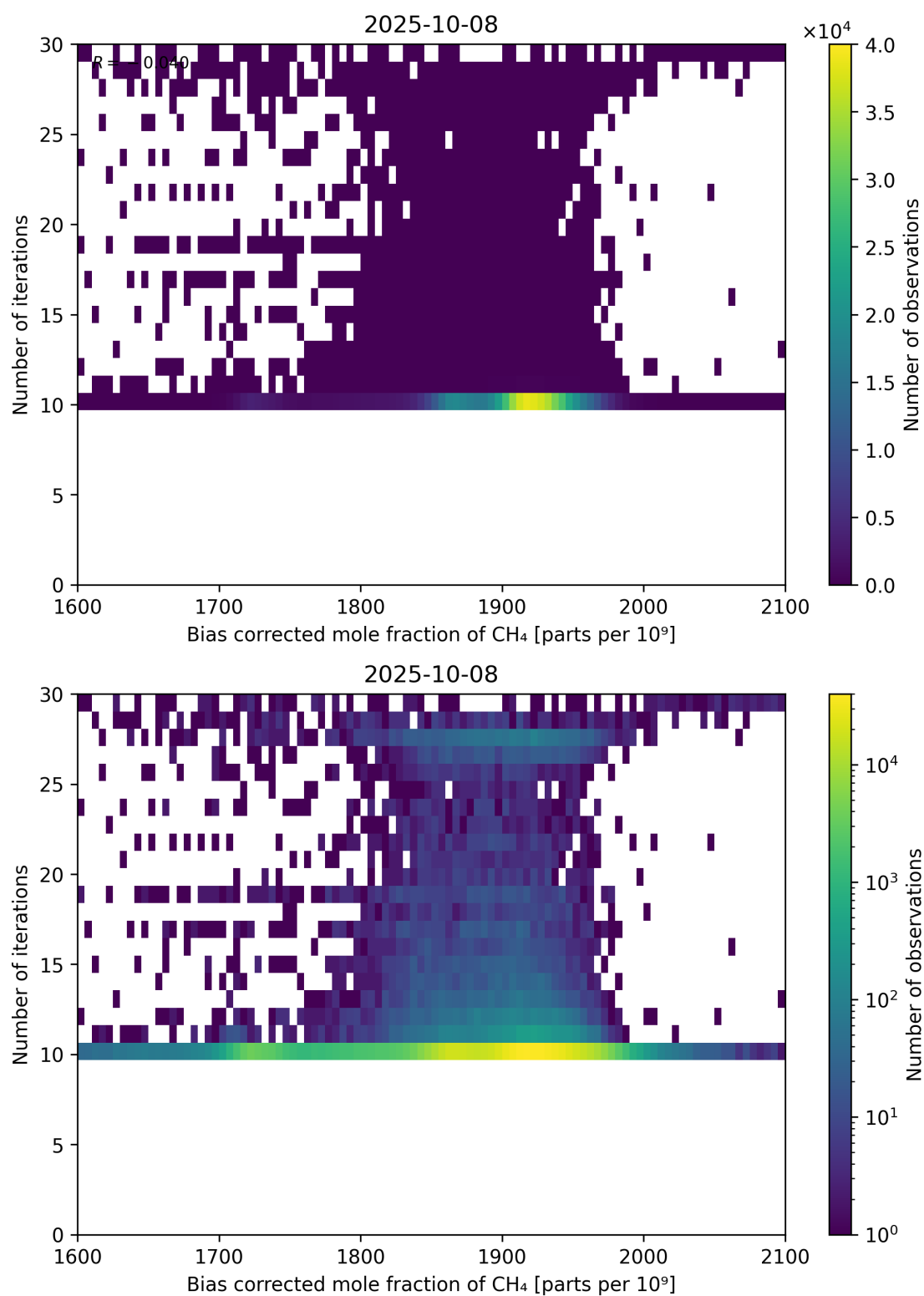
Figure 67: Scatter density plot of “Bias corrected mole fraction of \text{CH}_4 ” against “Number of iterations” for 2025-10-07 to 2025-10-09.
