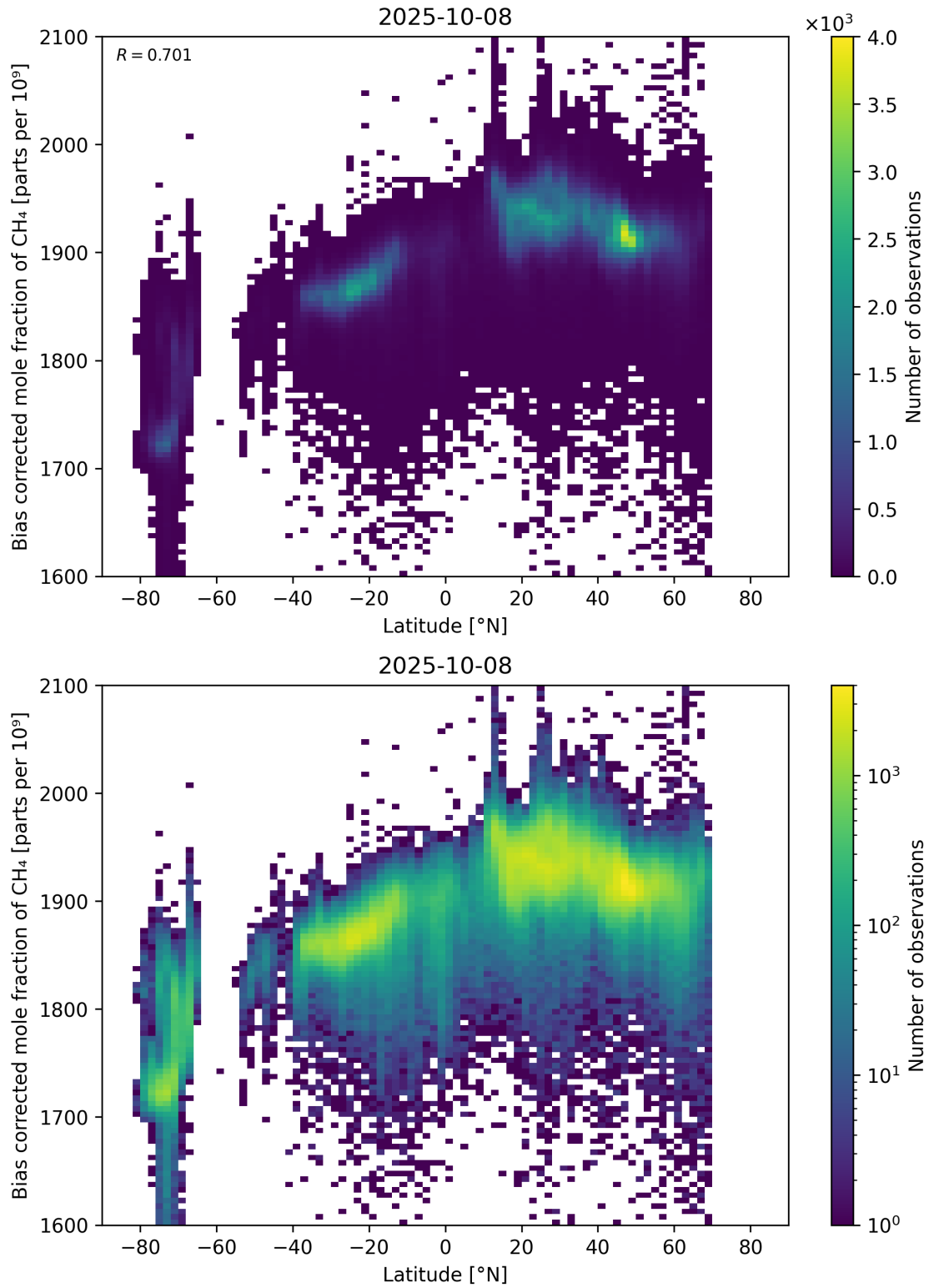
Figure 58: Scatter density plot of “Latitude” against “Bias corrected mole fraction of \text{CH}_4 ” for 2025-10-07 to 2025-10-09.
