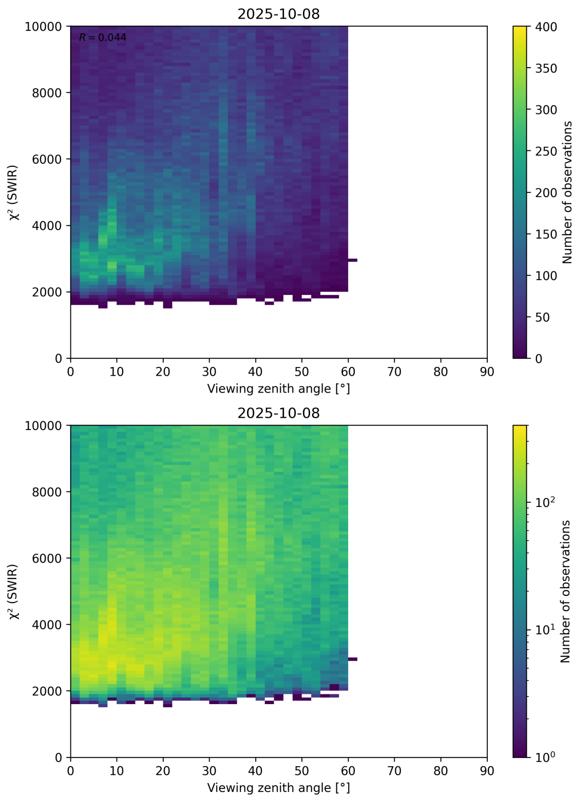
Figure 106: Scatter density plot of “Viewing zenith angle” against “ \chi^2 (SWIR)” for 2025-10-07 to 2025-10-09.
