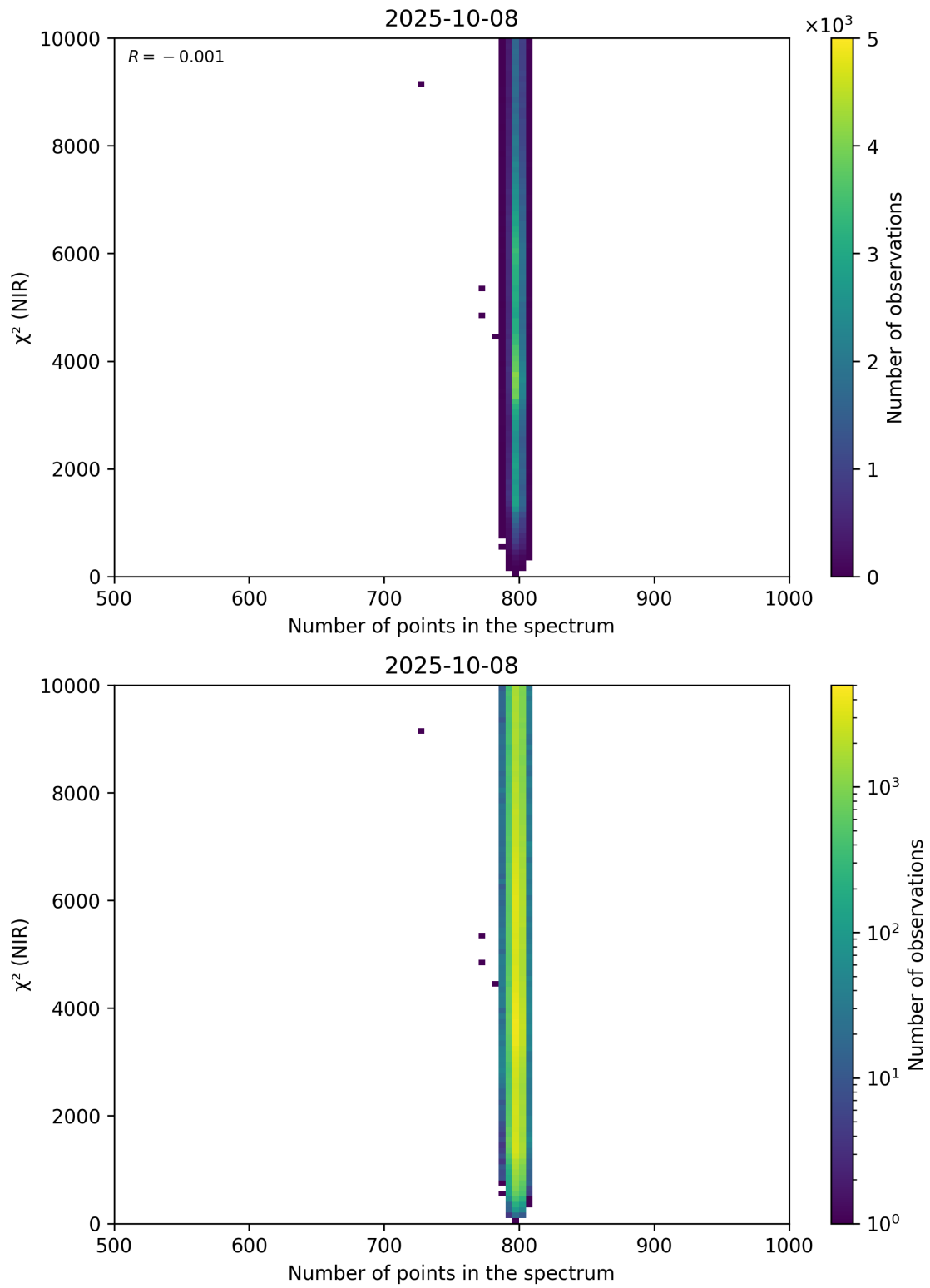
Figure 88: Scatter density plot of “Number of points in the spectrum” against “ \chi^2 (NIR)” for 2025-10-07 to 2025-10-09.
