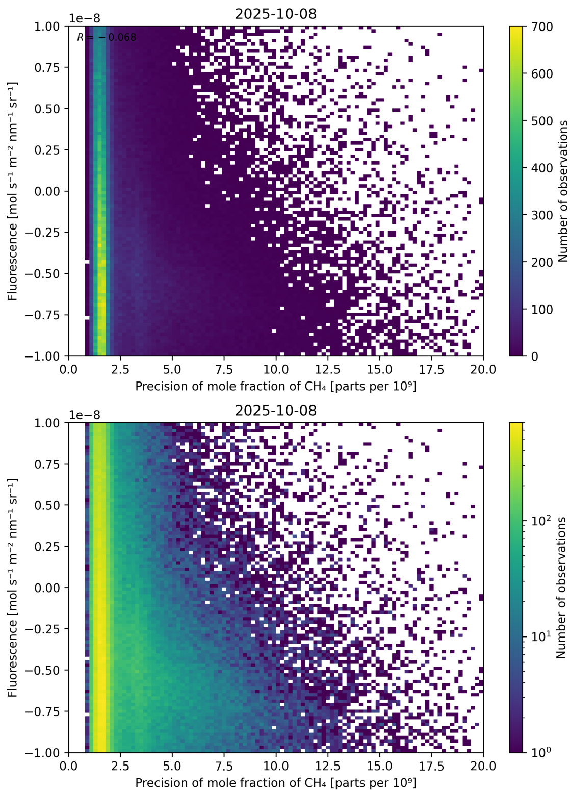
Figure 81: Scatter density plot of “Precision of mole fraction of CH 4 ” against “Fluorescence” for 2025-10-07 to 2025-10-09.
