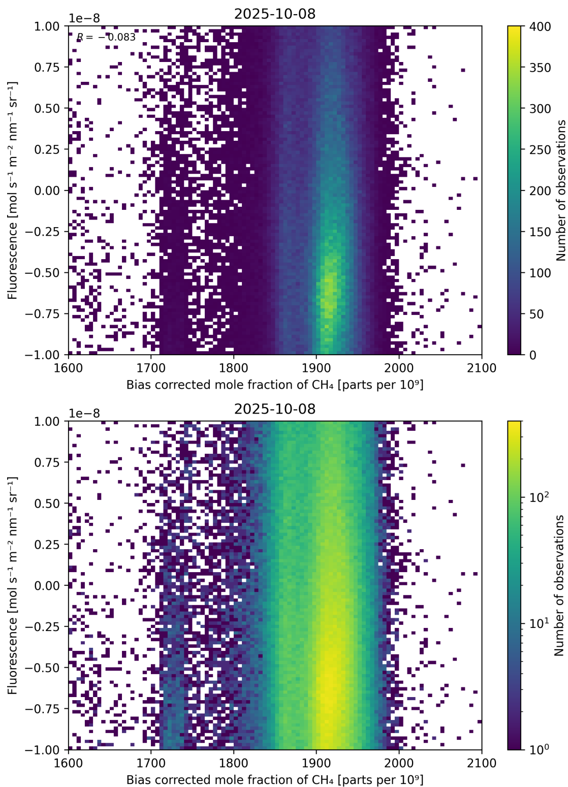
Figure 66: Scatter density plot of “Bias corrected mole fraction of \text{CH}_4 ” against “Fluorescence” for 2025-10-07 to 2025-10-09.
