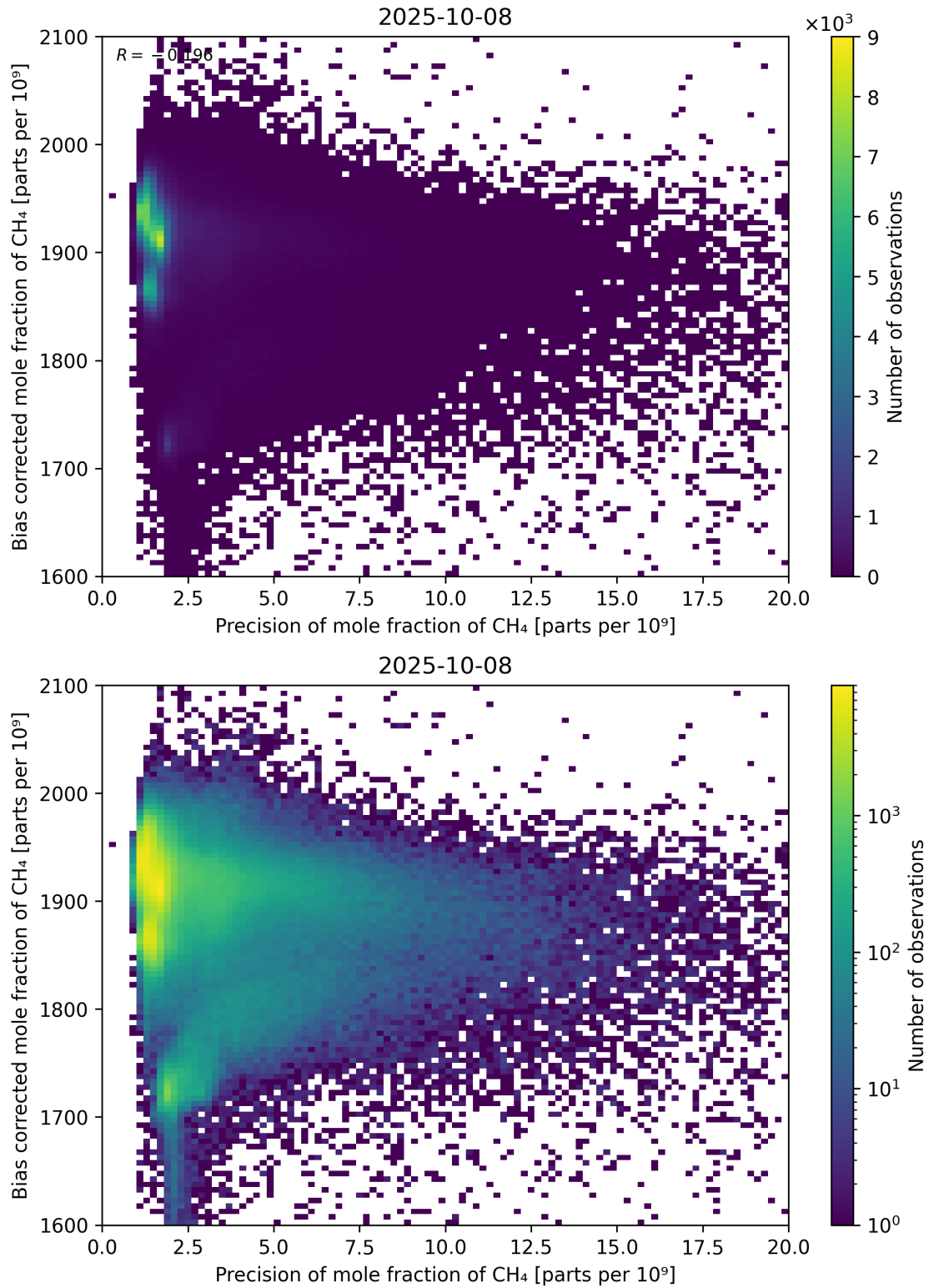
Figure 82: Scatter density plot of “Precision of mole fraction of CH 4 ” against “Bias corrected mole fraction of CH 4 ” for 2025-10-07 to 2025-10-09.
