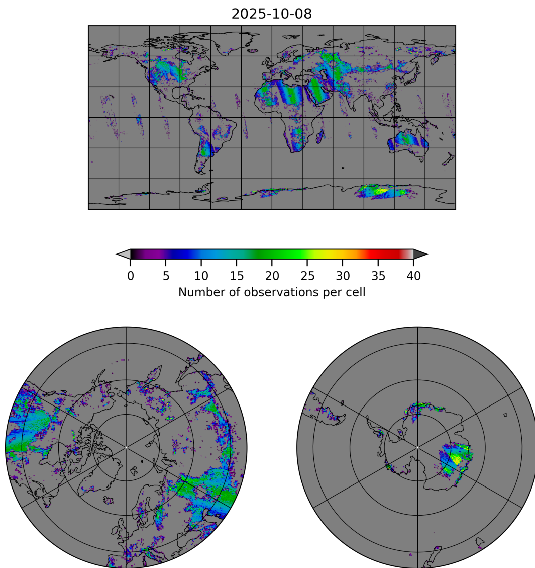
Figure 10: Map of the number of observations for 2025-10-07 to 2025-10-09
