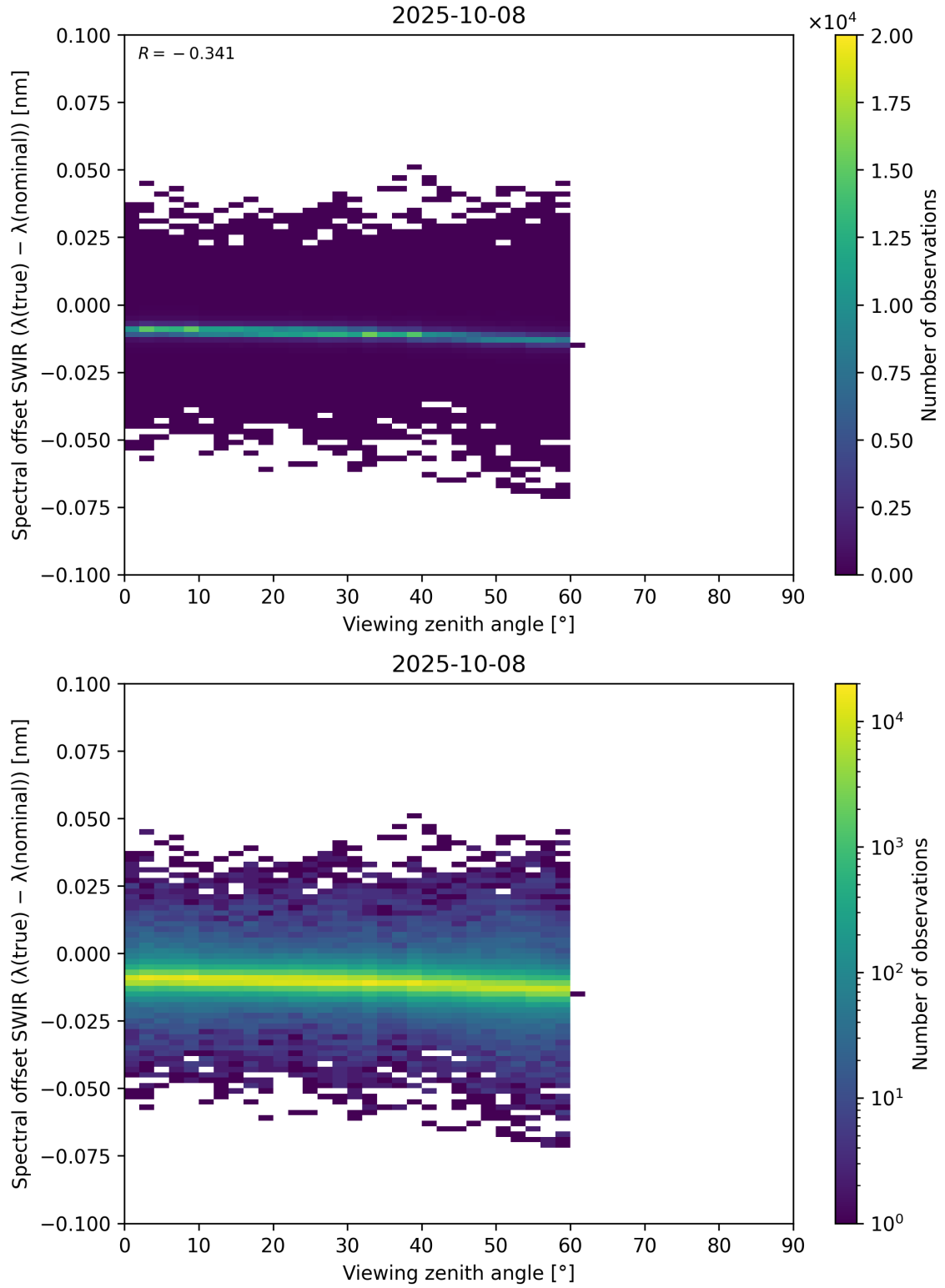
Figure 116: Scatter density plot of “Viewing zenith angle” against “Spectral offset SWIR ( \lambda_{\text{true}} - \lambda_{\text{nominal}} )” for 2025-10-07 to 2025-10-09.
