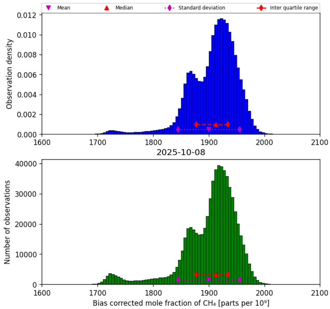
Figure 25: Histogram of “Bias corrected mole fraction of CH 4 ” for 2025-10-07 to 2025-10-09
