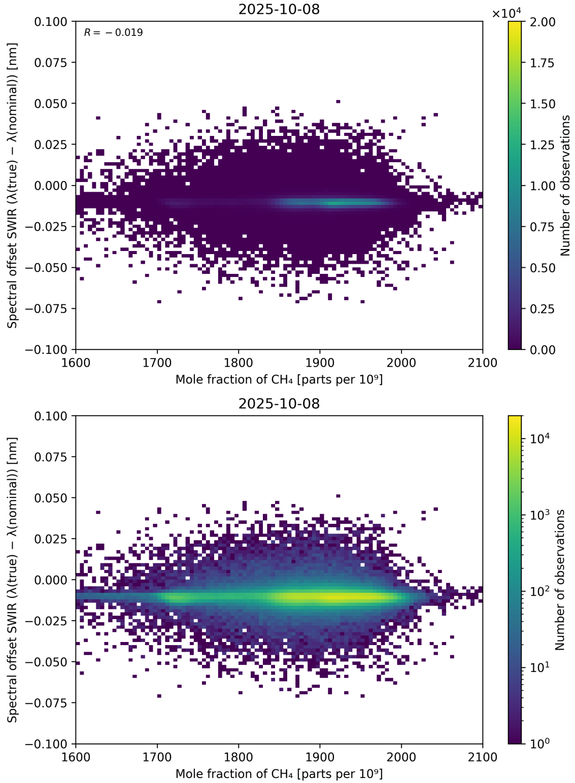
Figure 86: Scatter density plot of “Mole fraction of CH 4 ” against “Spectral offset SWIR ( \lambda_{\text{true}} - \lambda_{\text{nominal}} )” for 2025-10-07 to 2025-10-09.
