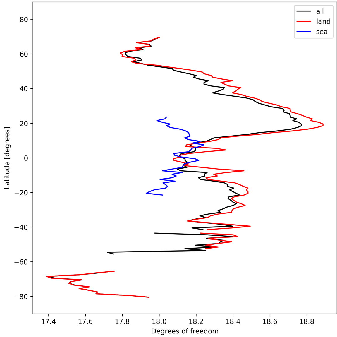
Figure 19: Zonal average of “Degrees of freedom” for 2025-10-07 to 2025-10-09.
