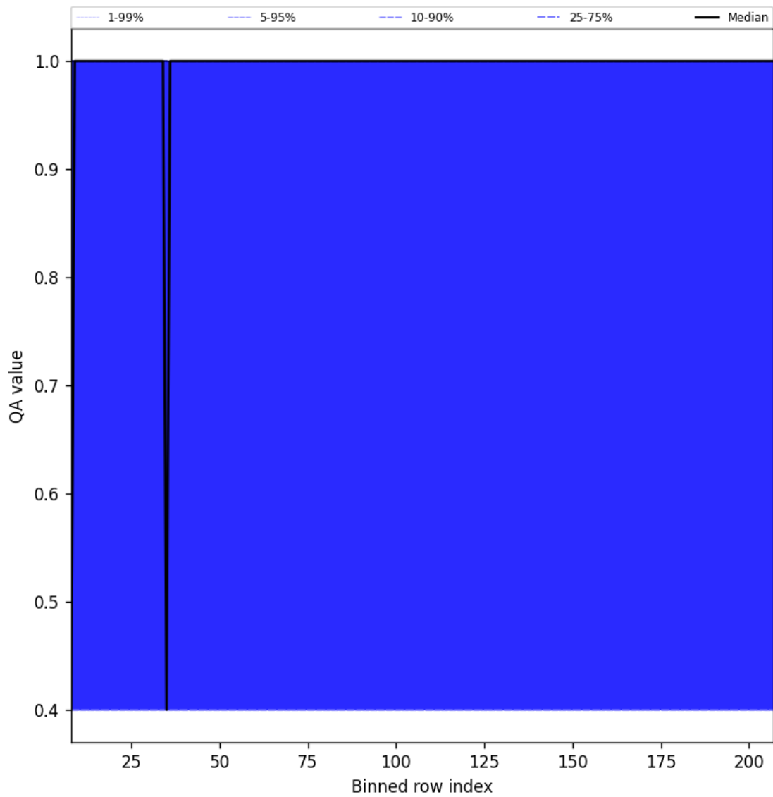
Figure 33: Along track statistics of “QA value” for 2025-10-07 to 2025-10-09
