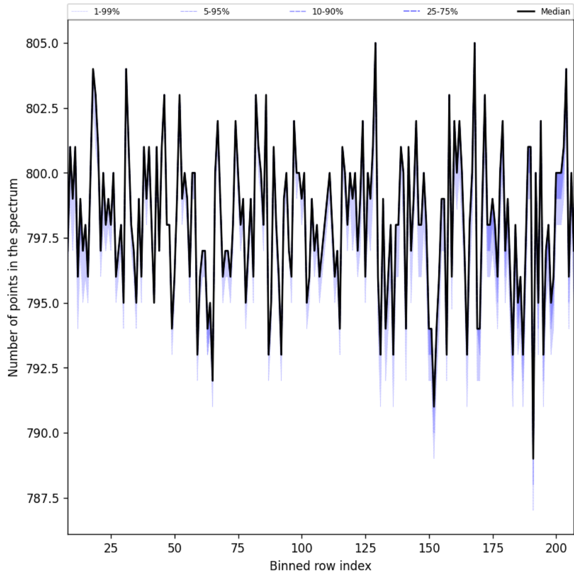
Figure 37: Along track statistics of “Number of points in the spectrum” for 2025-10-07 to 2025-10-09
