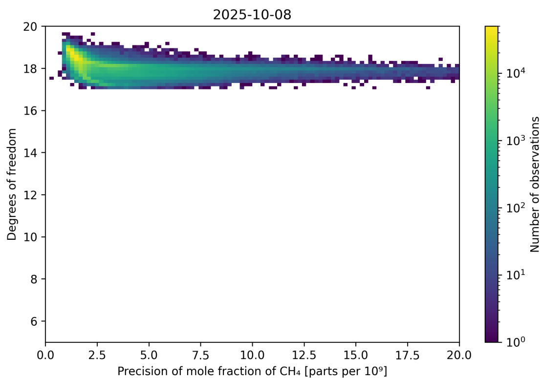
Figure 80: Scatter density plot of “Precision of mole fraction of CH 4 ” against “Degrees of freedom” for 2025-10-07 to 2025-10-09.
