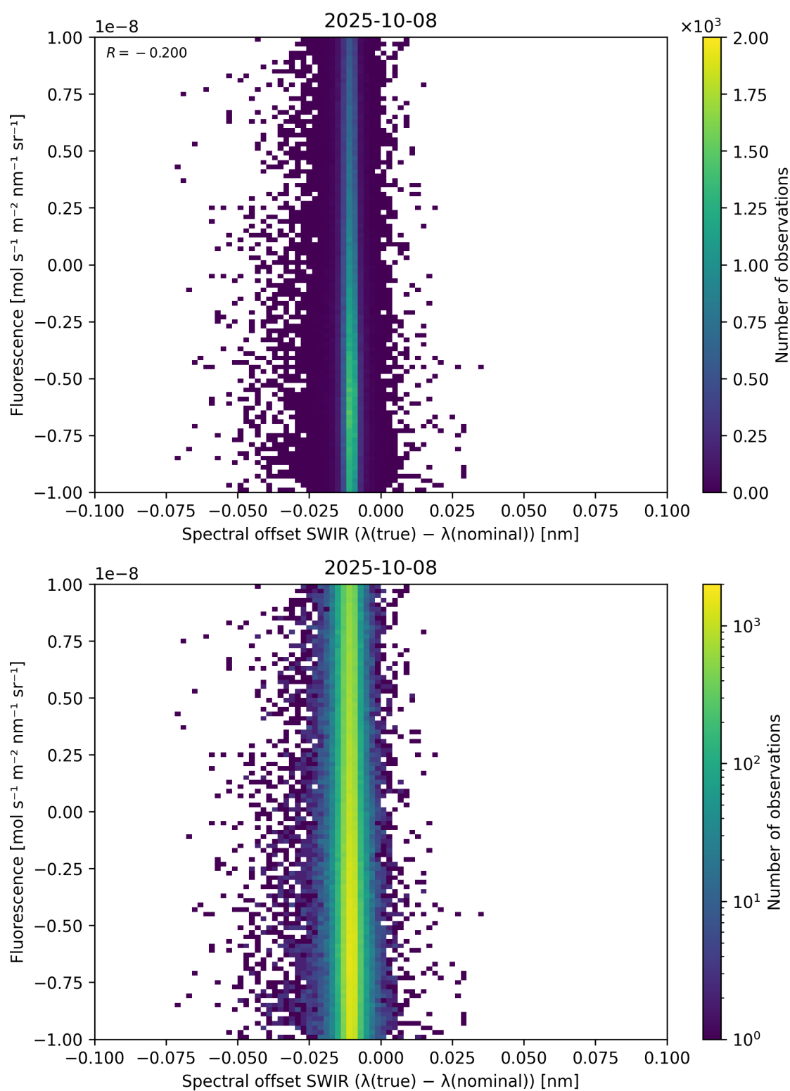
Figure 120: Scatter density plot of “Spectral offset SWIR ( \lambda_{\text{true}} - \lambda_{\text{nominal}} )” against “Fluorescence” for 2025-10-07 to 2025-10-09.
