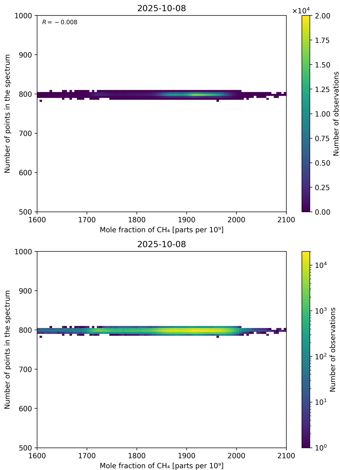
Figure 77: Scatter density plot of “Mole fraction of CH 4 ” against “Number of points in the spectrum” for 2025-10-07 to 2025-10-09.
