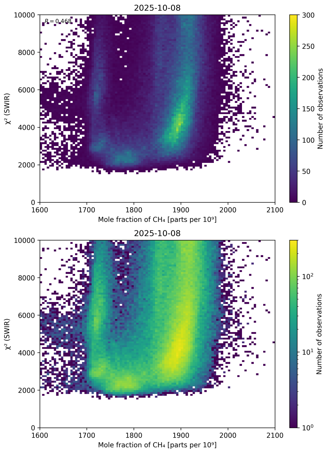
Figure 71: Scatter density plot of “Mole fraction of CH 4 ” against “ \chi^2 (SWIR)” for 2025-10-07 to 2025-10-09.
