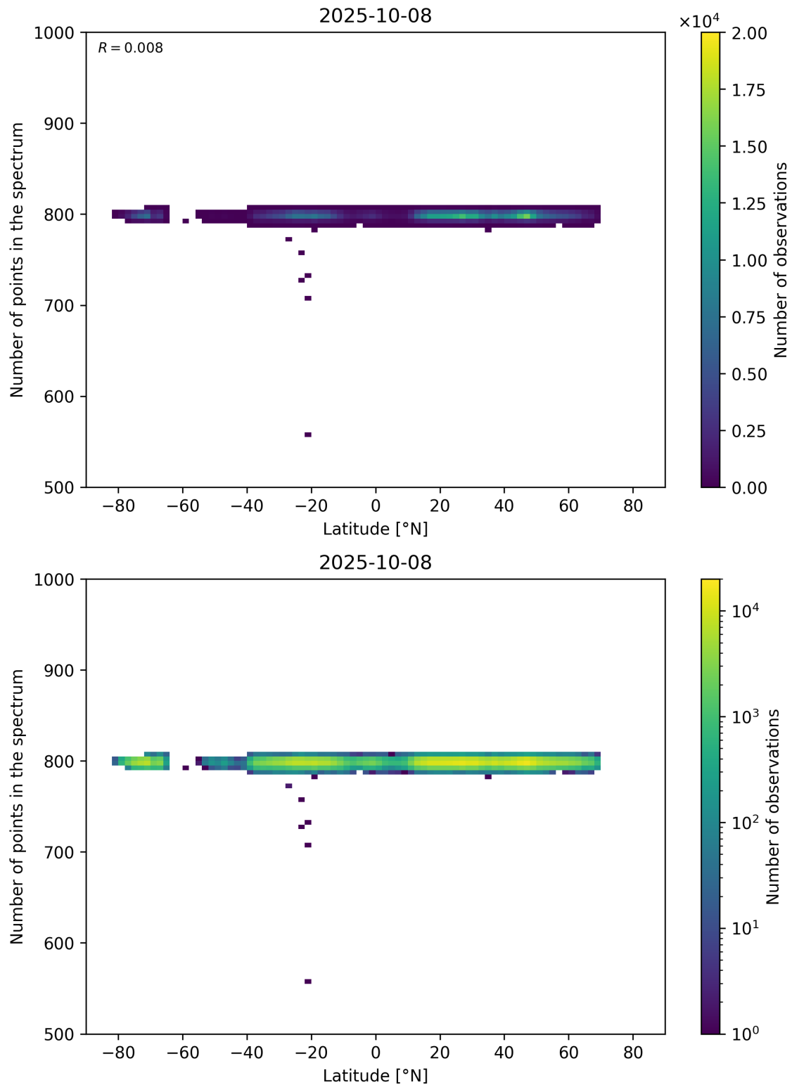
Figure 61: Scatter density plot of “Latitude” against “Number of points in the spectrum” for 2025-10-07 to 2025-10-09.
