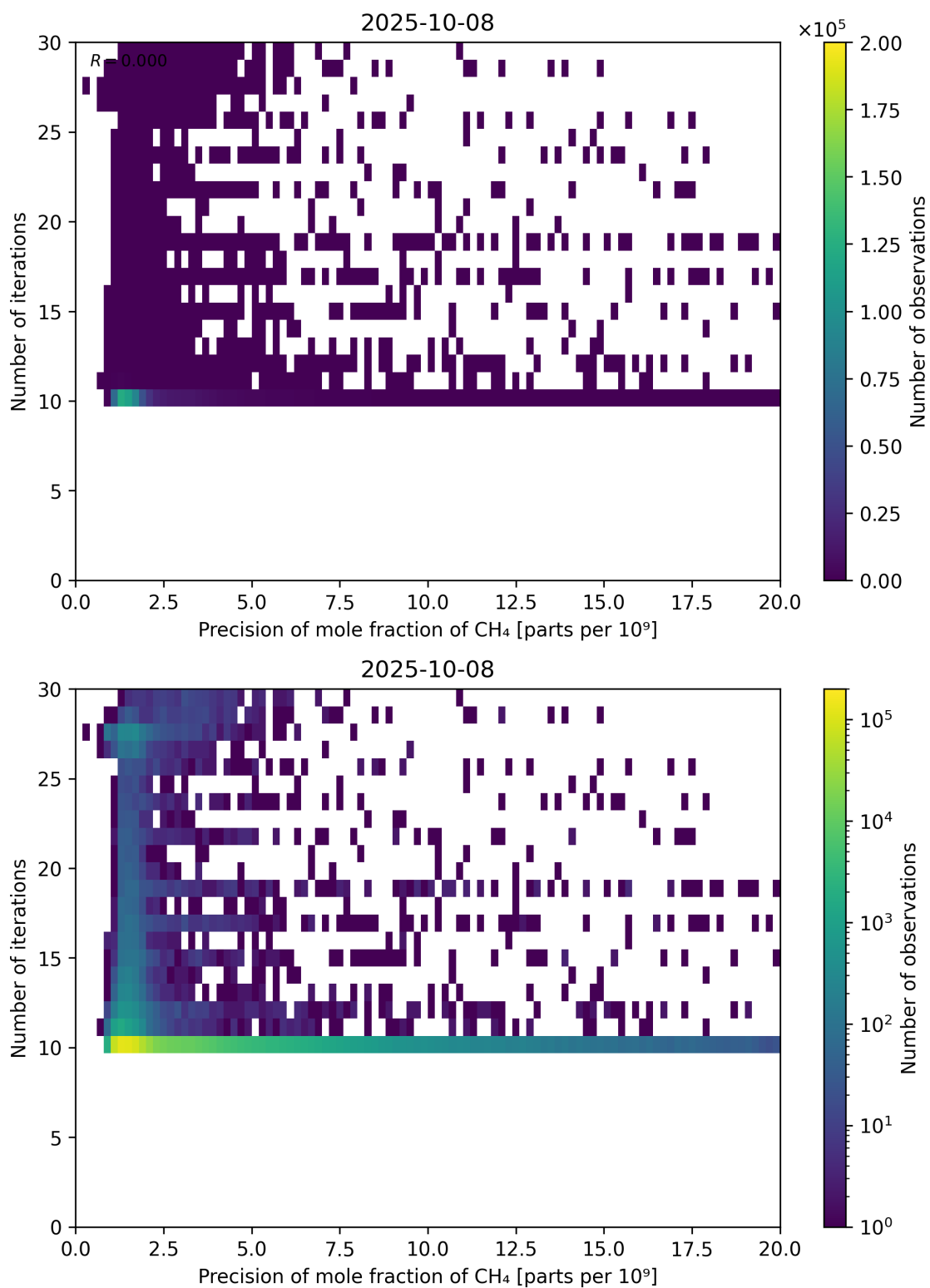
Figure 83: Scatter density plot of “Precision of mole fraction of CH 4 ” against “Number of iterations” for 2025-10-07 to 2025-10-09.
