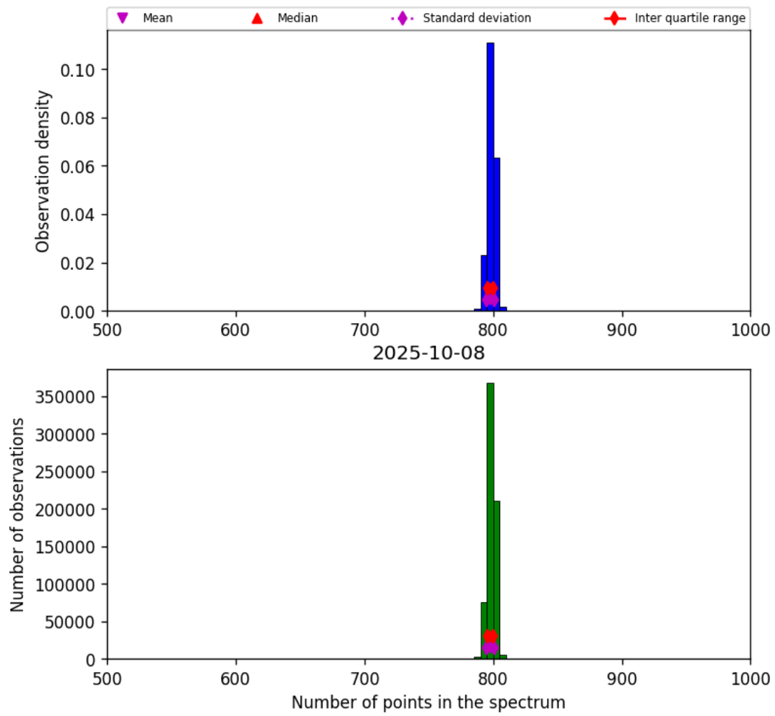
Figure 26: Histogram of “Number of points in the spectrum” for 2025-10-07 to 2025-10-09
