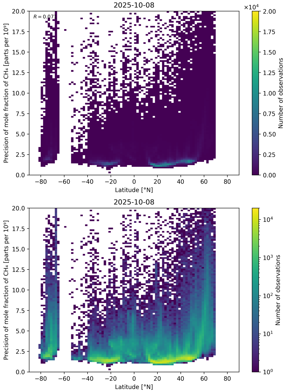
Figure 59: Scatter density plot of “Latitude” against “Precision of mole fraction of CH 4 ” for 2025-10-07 to 2025-10-09.
