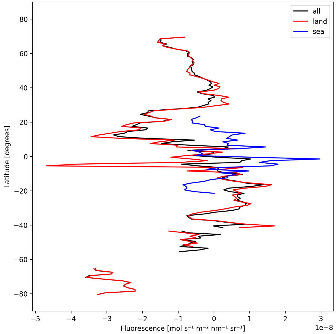
Figure 21: Zonal average of “Fluorescence” for 2025-10-07 to 2025-10-09.
