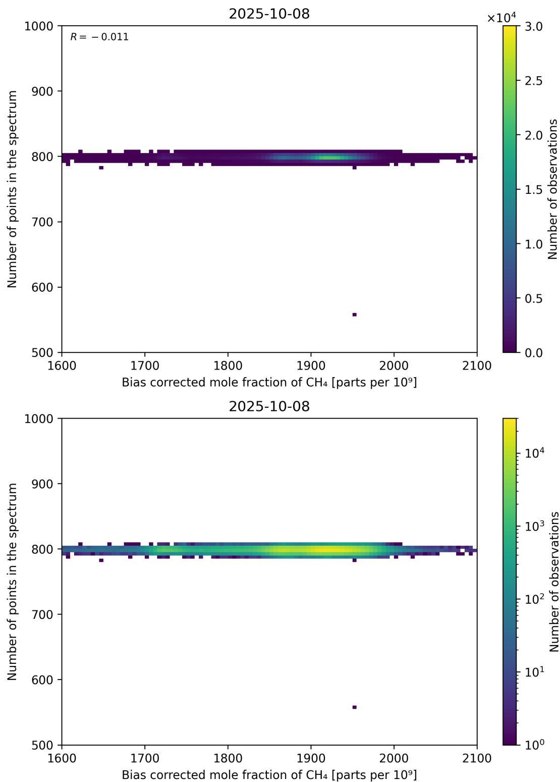
Figure 68: Scatter density plot of “Bias corrected mole fraction of CH 4 ” against “Number of points in the spectrum” for 2025-10-07 to 2025-10-09.
