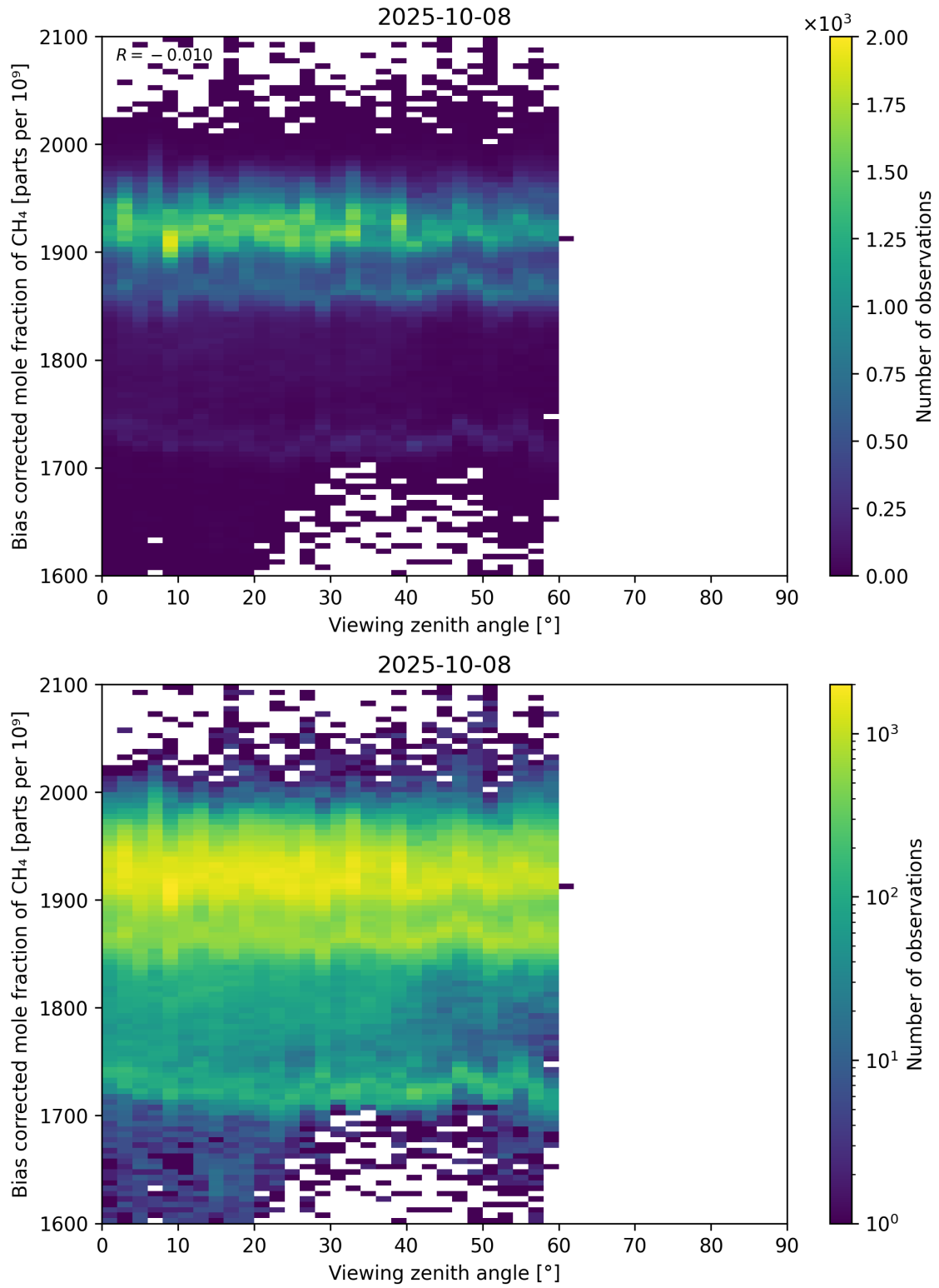
Figure 111: Scatter density plot of “Viewing zenith angle” against “Bias corrected mole fraction of CH 4 ” for 2025-10-07 to 2025-10-09.
