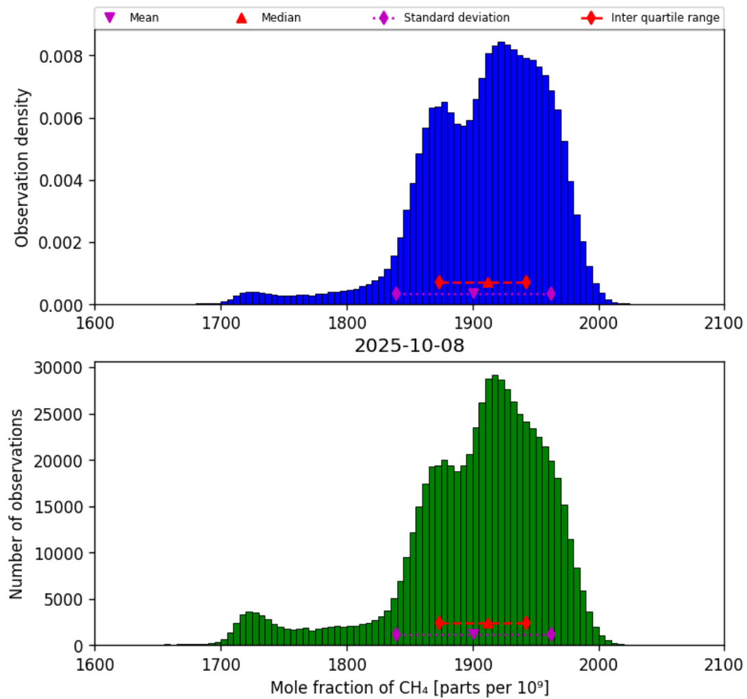
Figure 23: Histogram of “Mole fraction of CH 4 ” for 2025-10-07 to 2025-10-09
