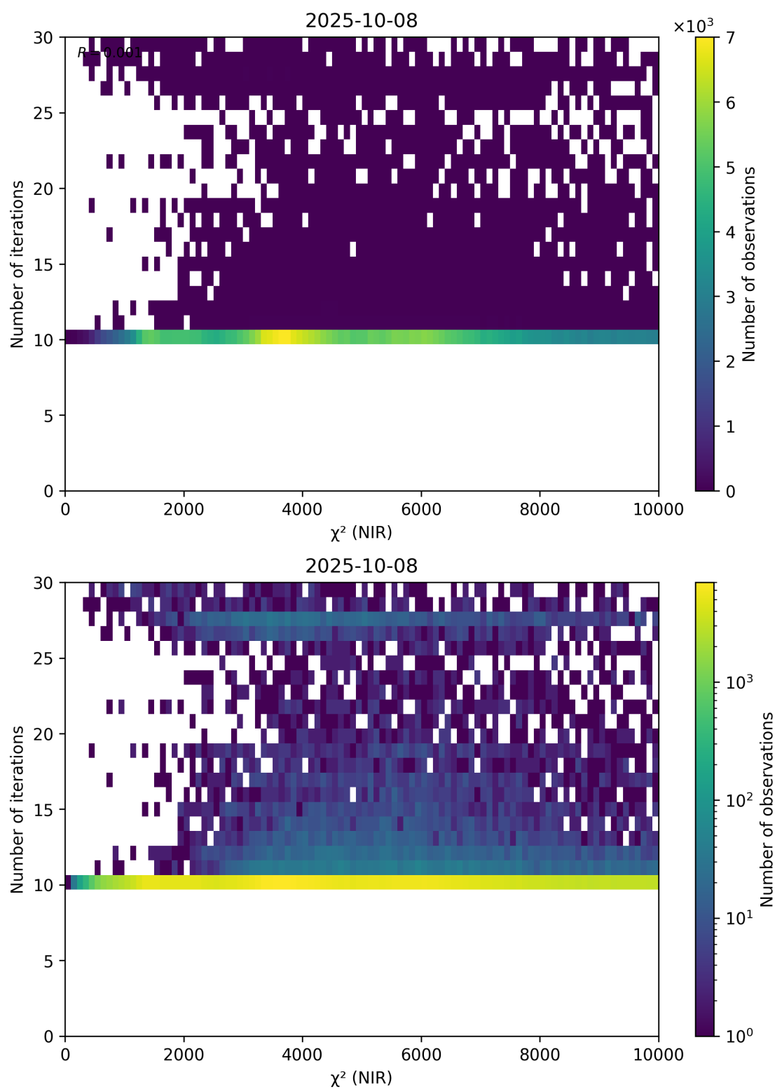
Figure 46: Scatter density plot of “ \chi^2 (NIR)” against “Number of iterations” for 2025-10-07 to 2025-10-09.
