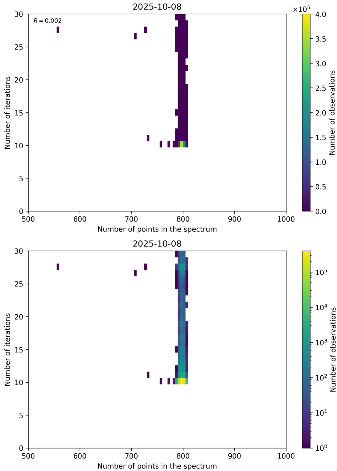
Figure 92: Scatter density plot of “Number of points in the spectrum” against “Number of iterations” for 2025-10-07 to 2025-10-09.
