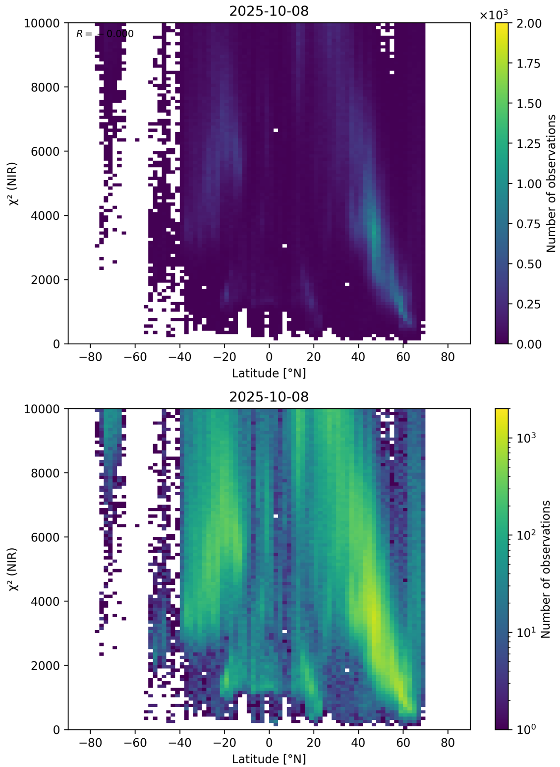
Figure 53: Scatter density plot of “Latitude” against “ \chi^2 (NIR)” for 2025-10-07 to 2025-10-09.
