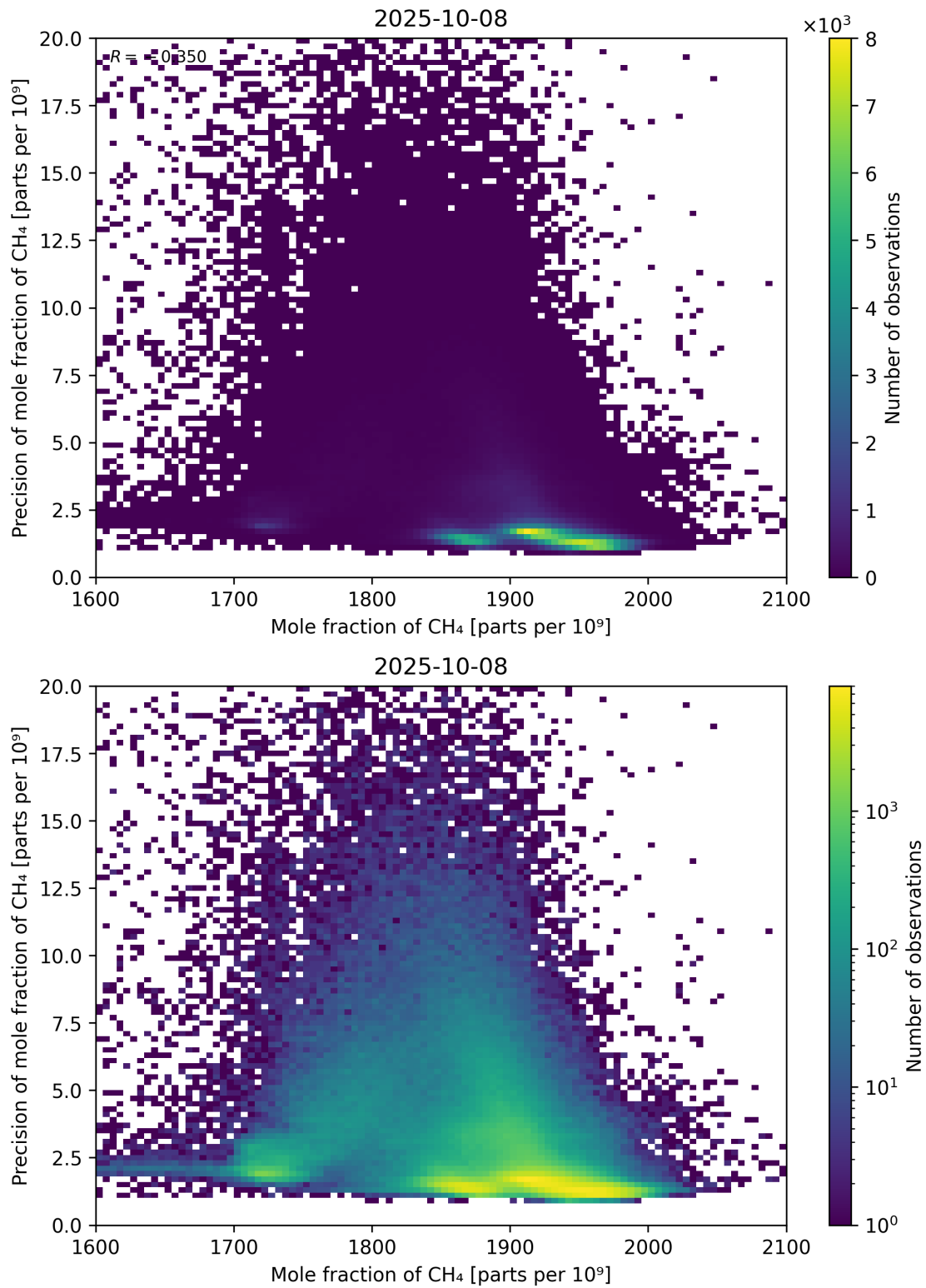
Figure 75: Scatter density plot of “Mole fraction of CH 4 ” against “Precision of mole fraction of CH 4 ” for 2025-10-07 to 2025-10-09.
