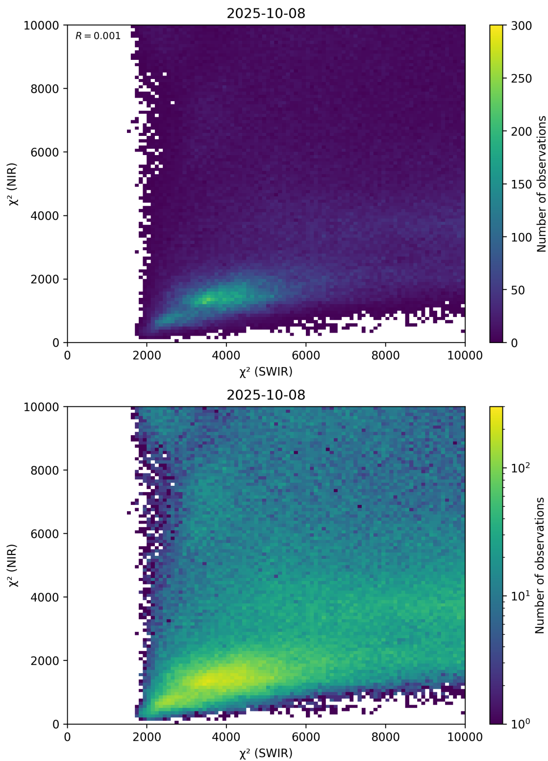
Figure 47: Scatter density plot of “ \chi^2 (SWIR)” against “ \chi^2 (NIR)” for 2025-10-07 to 2025-10-09.
