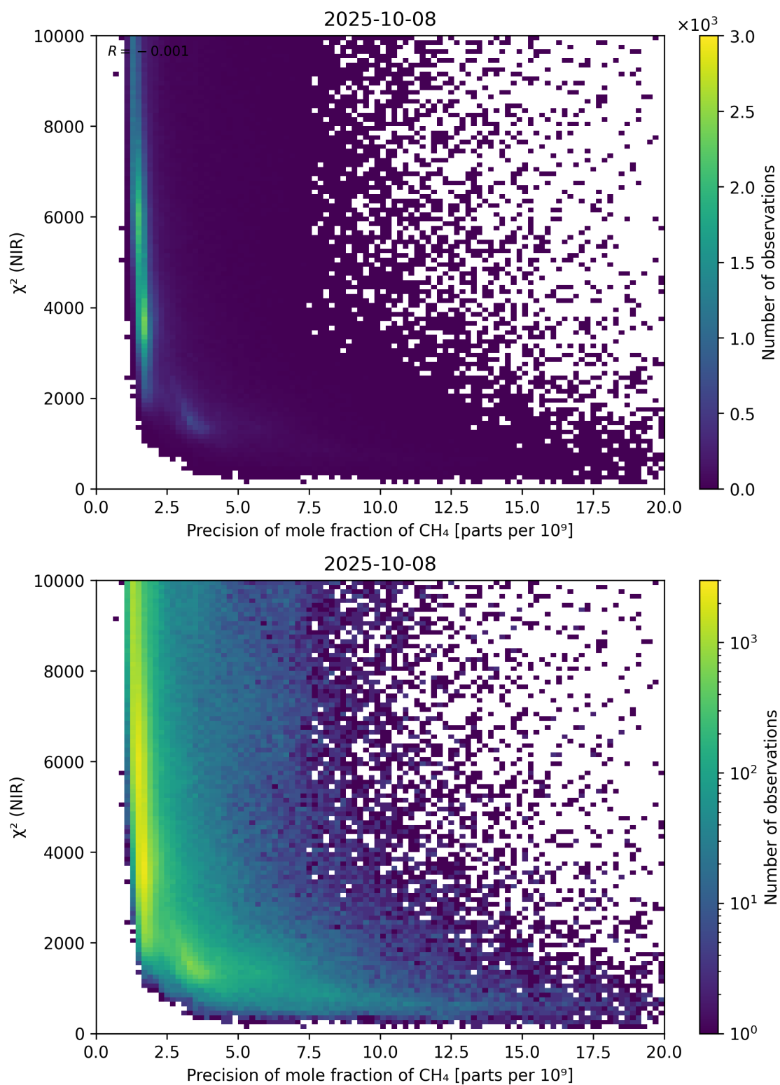
Figure 78: Scatter density plot of “Precision of mole fraction of CH 4 ” against “ \chi^2 (NIR)” for 2025-10-07 to 2025-10-09.
