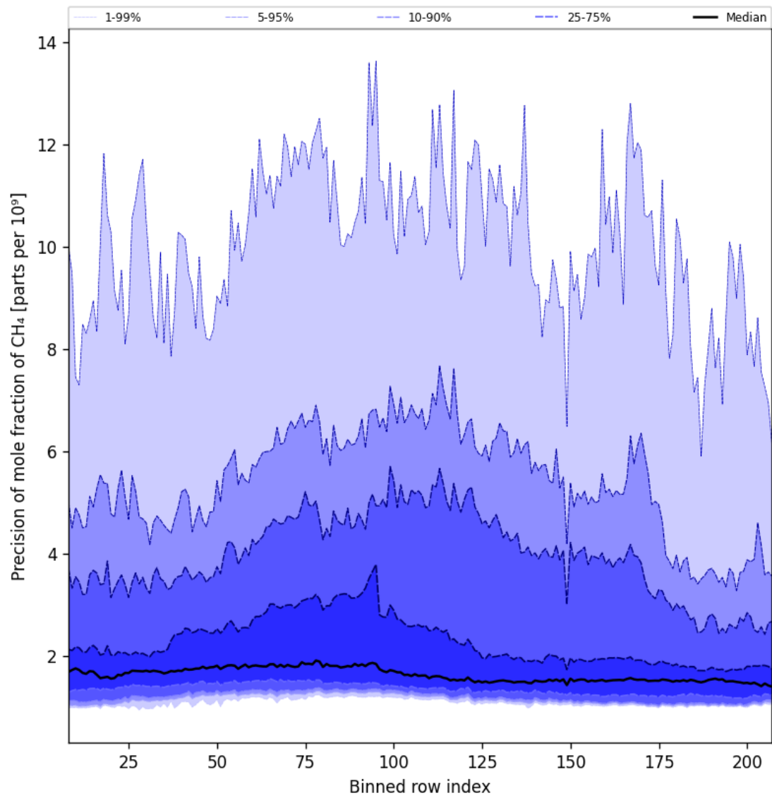
Figure 35: Along track statistics of “Precision of mole fraction of CH 4 ” for 2025-10-07 to 2025-10-09
