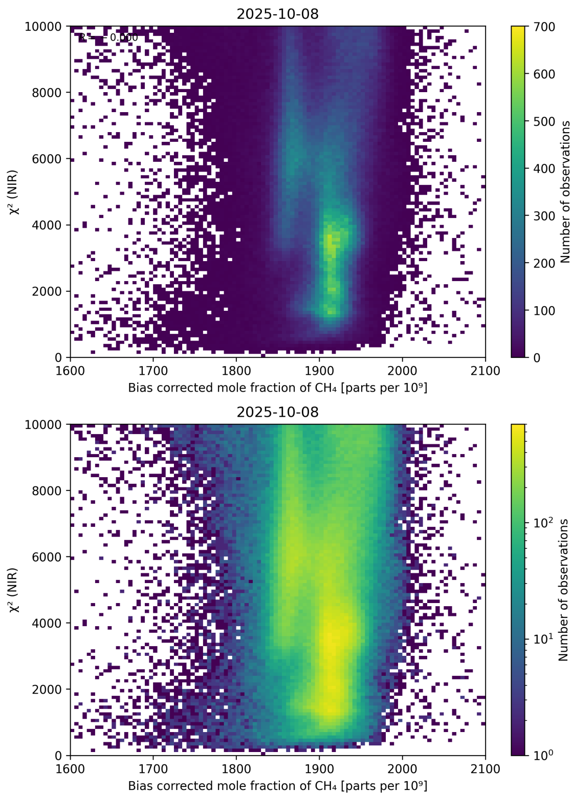
Figure 63: Scatter density plot of “Bias corrected mole fraction of \text{CH}_4 ” against “ \chi^2 (NIR)” for 2025-10-07 to 2025-10-09.
