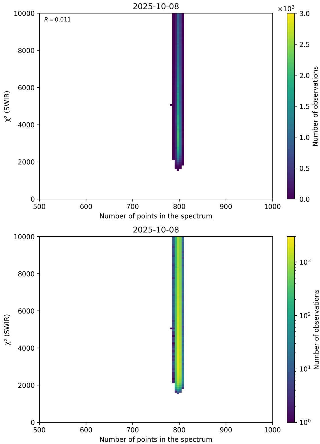
Figure 89: Scatter density plot of “Number of points in the spectrum” against “ \chi^2 (SWIR)” for 2025-10-07 to 2025-10-09.
