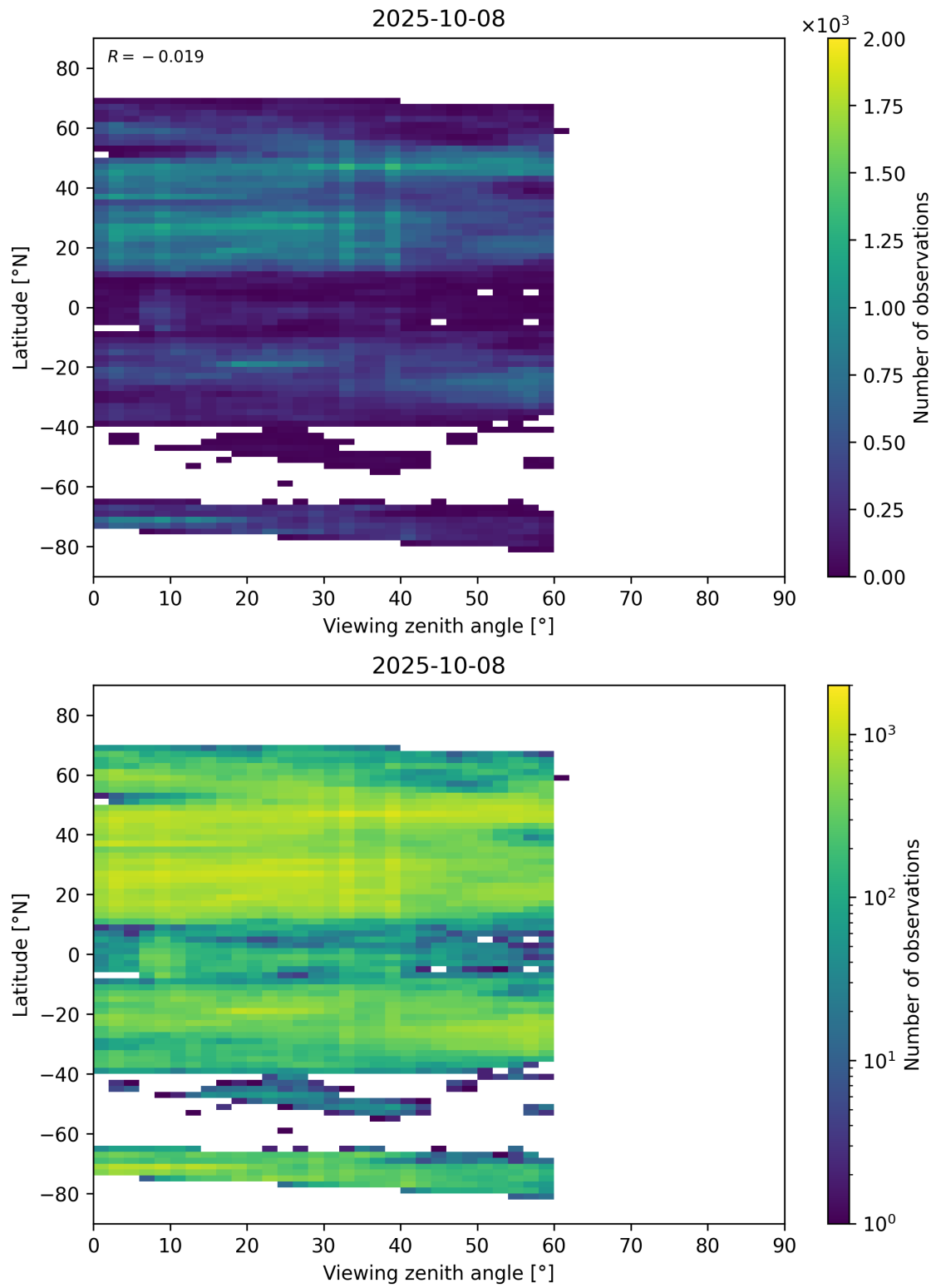
Figure 109: Scatter density plot of “Viewing zenith angle” against “Latitude” for 2025-10-07 to 2025-10-09.
