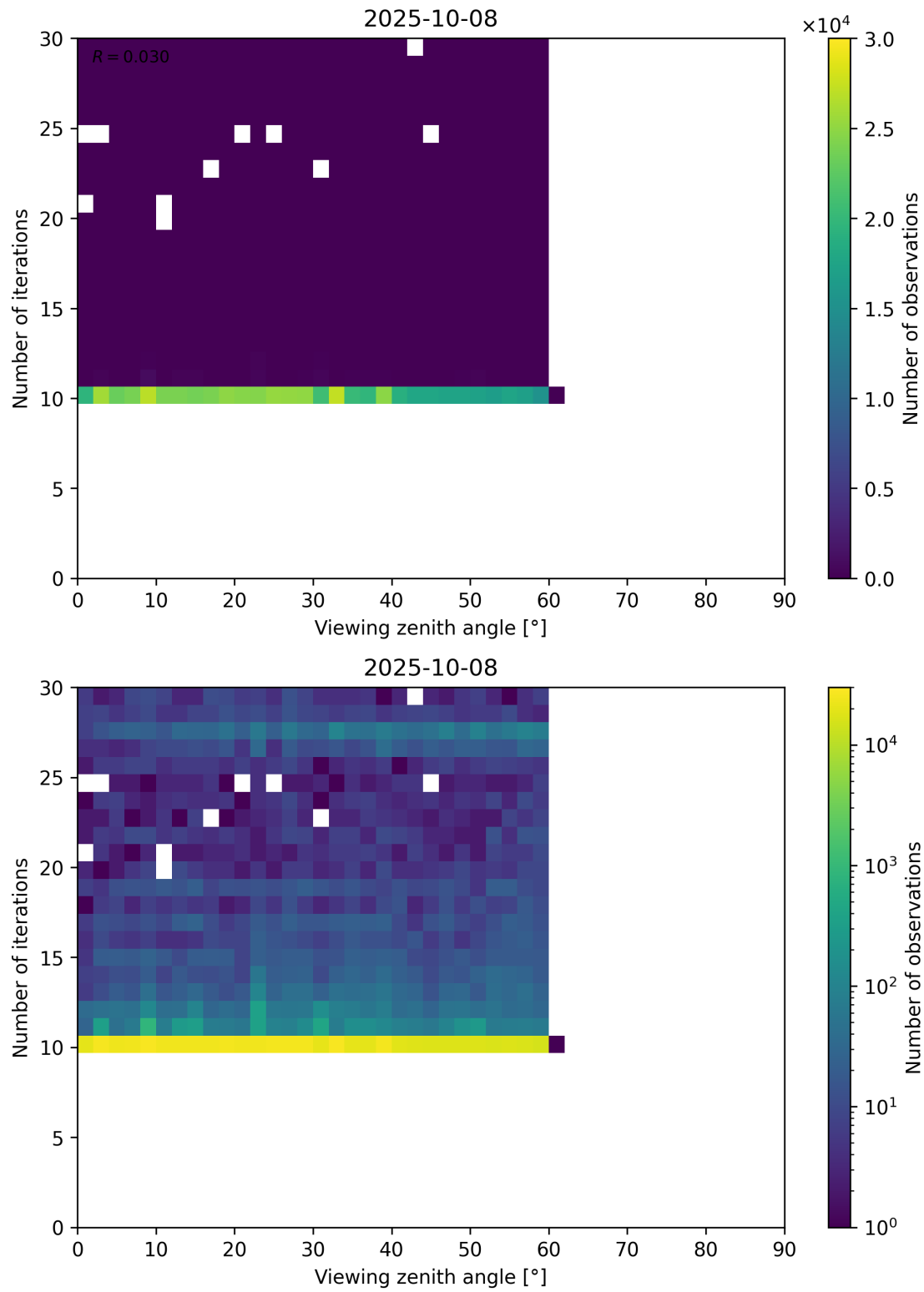
Figure 113: Scatter density plot of “Viewing zenith angle” against “Number of iterations” for 2025-10-07 to 2025-10-09.
