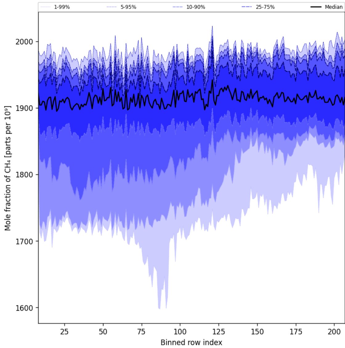
Figure 34: Along track statistics of “Mole fraction of CH 4 ” for 2025-10-07 to 2025-10-09
