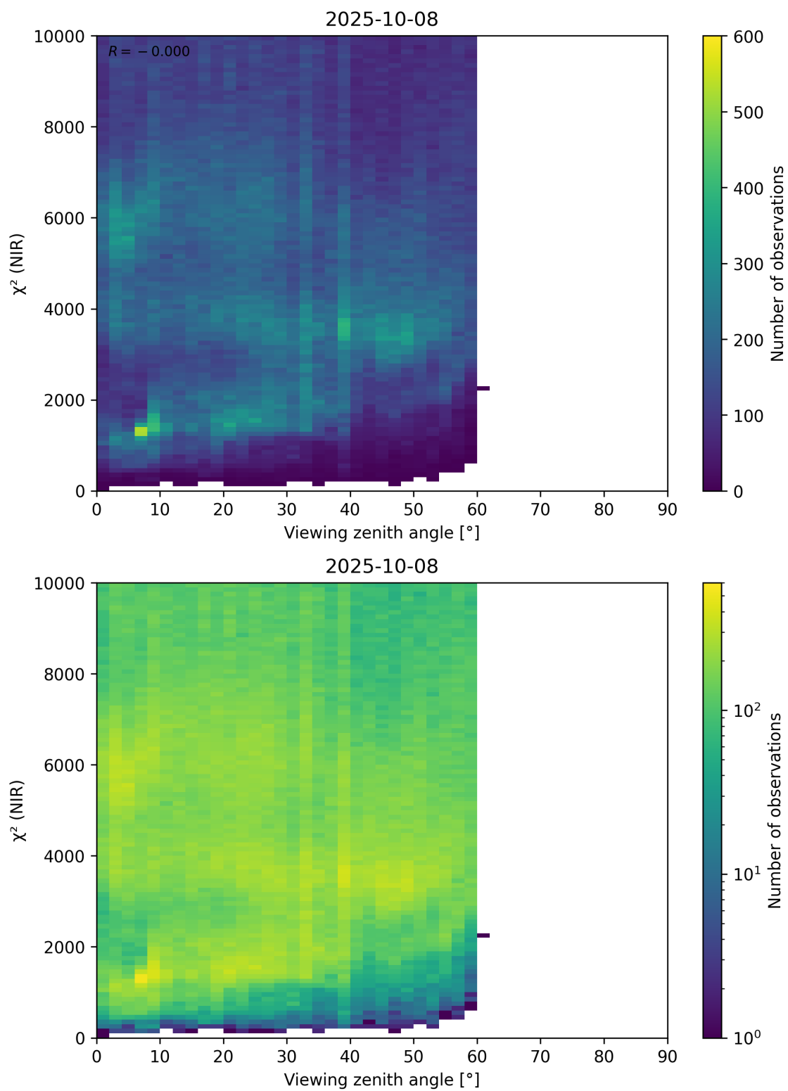
Figure 105: Scatter density plot of “Viewing zenith angle” against “ \chi^2 (NIR)” for 2025-10-07 to 2025-10-09.
