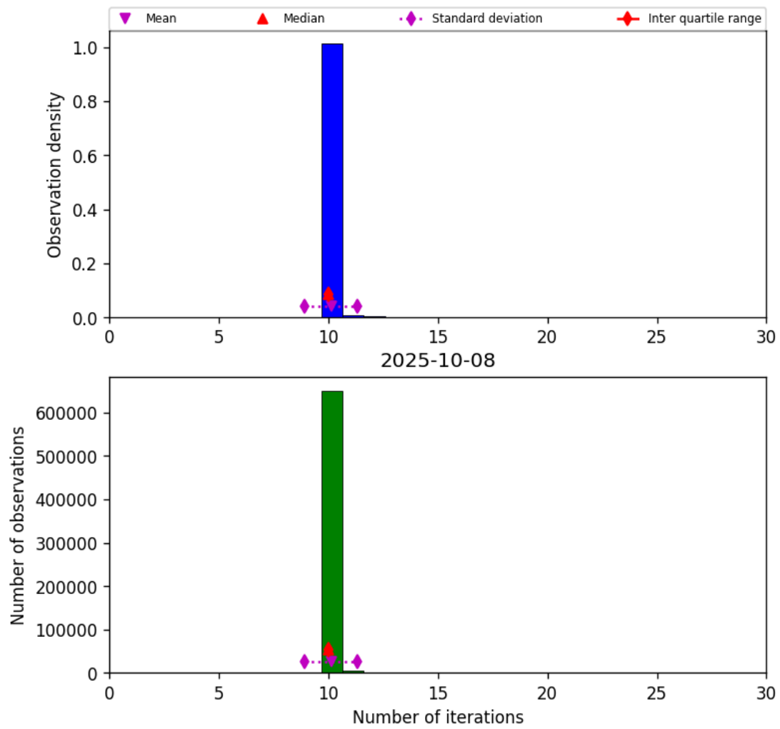
Figure 31: Histogram of “Number of iterations” for 2025-10-07 to 2025-10-09
