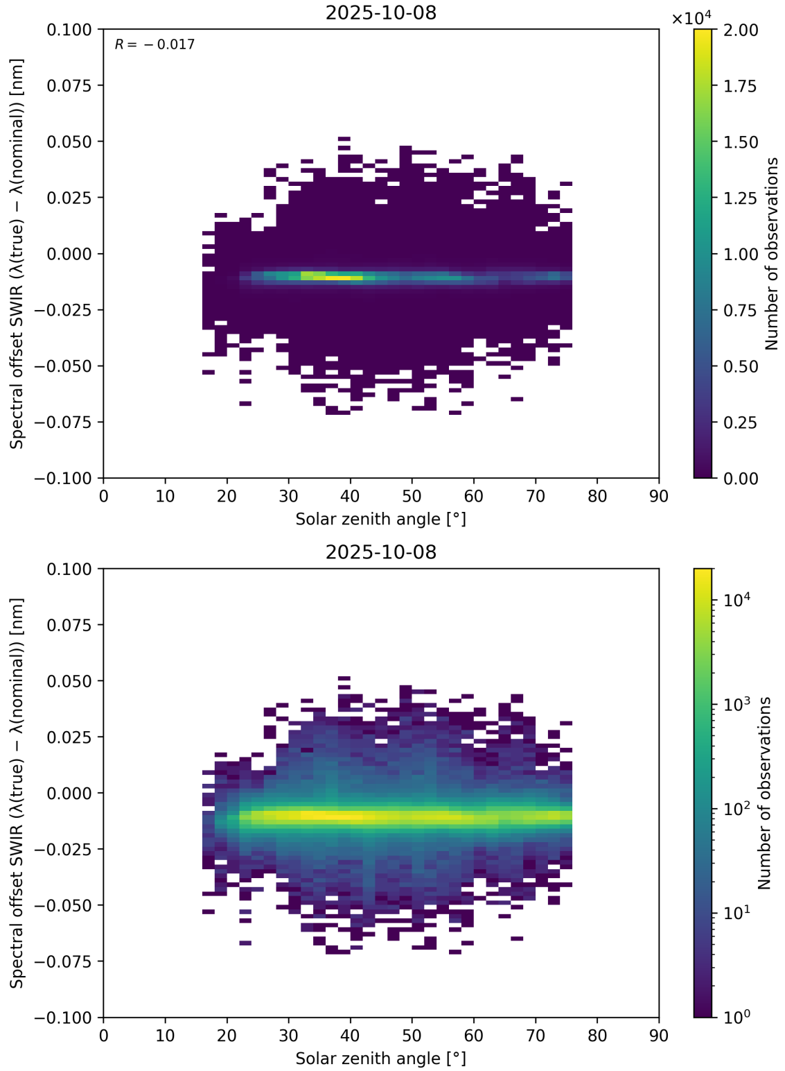
Figure 104: Scatter density plot of “Solar zenith angle” against “Spectral offset SWIR ( \lambda_{\text{true}} - \lambda_{\text{nominal}} )” for 2025-10-07 to 2025-10-09.
