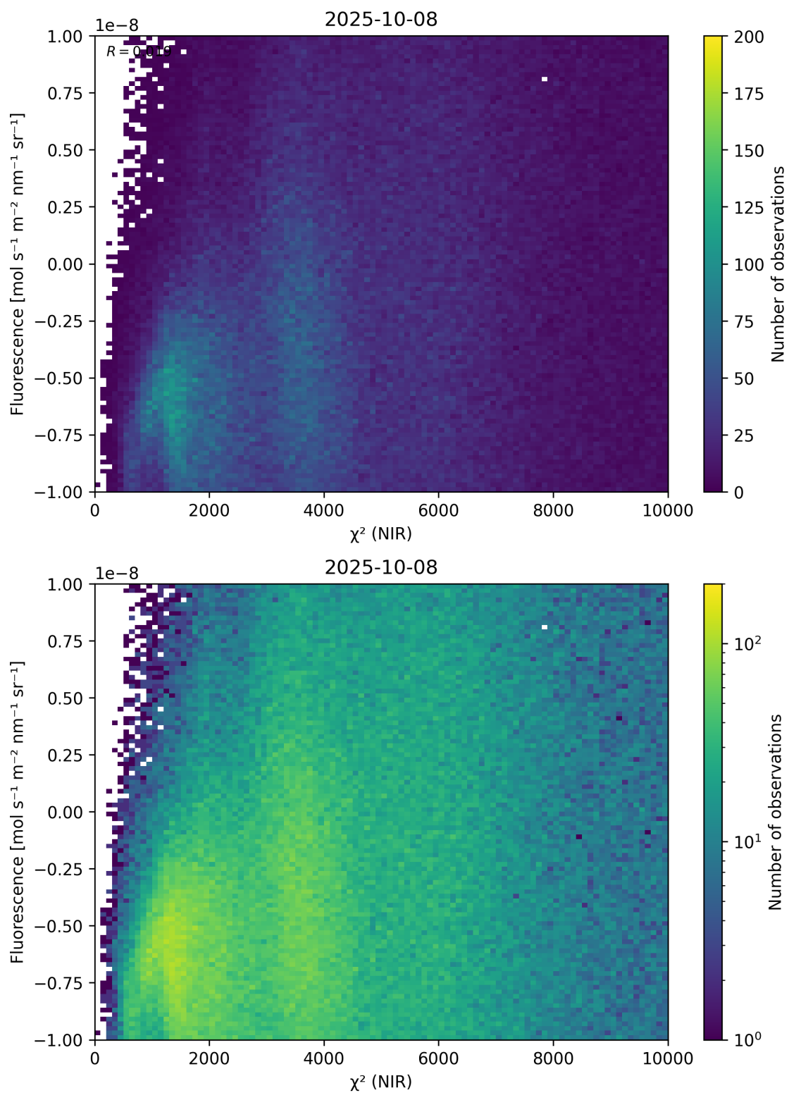
Figure 45: Scatter density plot of “ \chi^2 (NIR)” against “Fluorescence” for 2025-10-07 to 2025-10-09.
