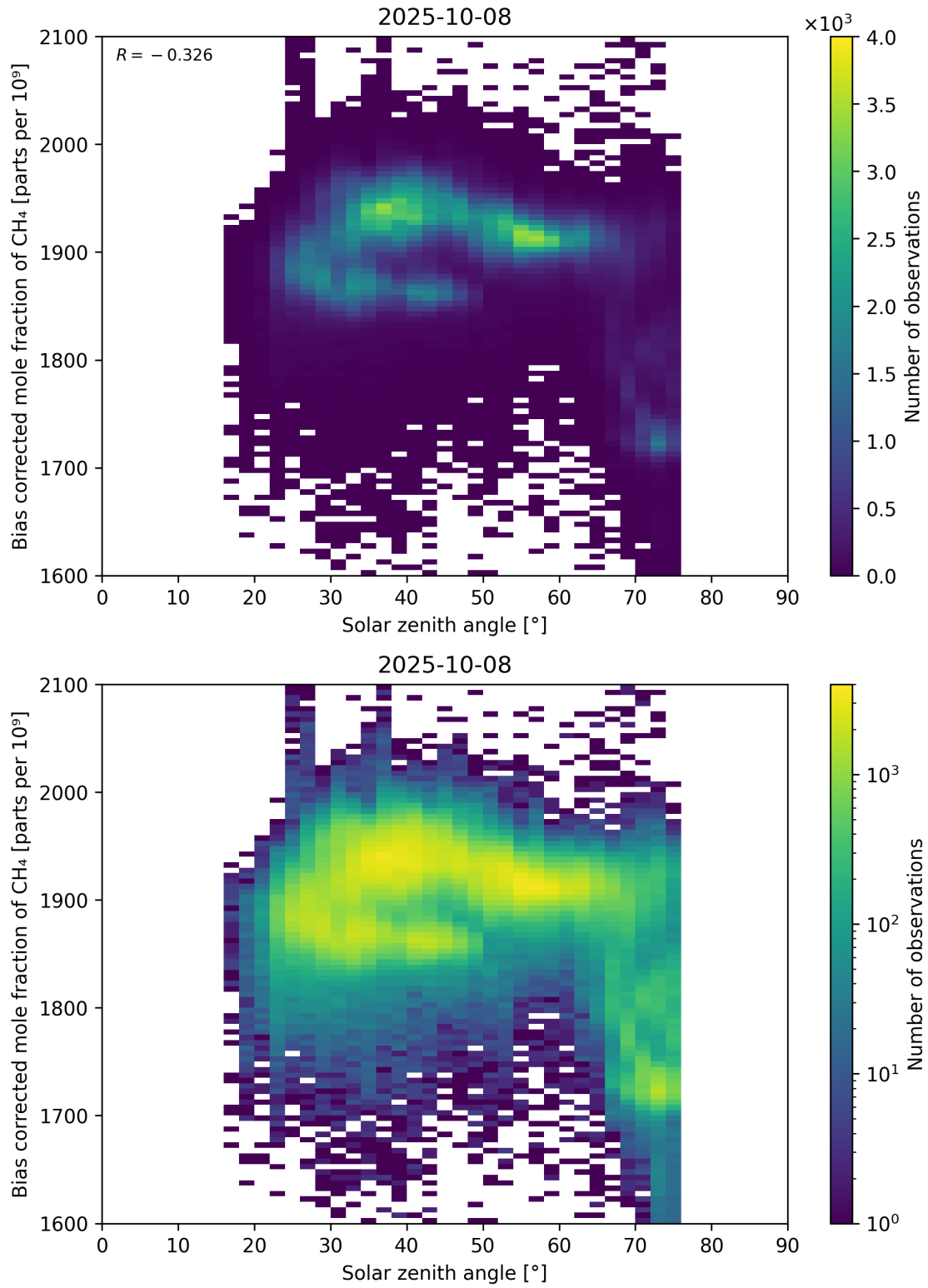
Figure 100: Scatter density plot of “Solar zenith angle” against “Bias corrected mole fraction of CH 4 ” for 2025-10-07 to 2025-10-09.
