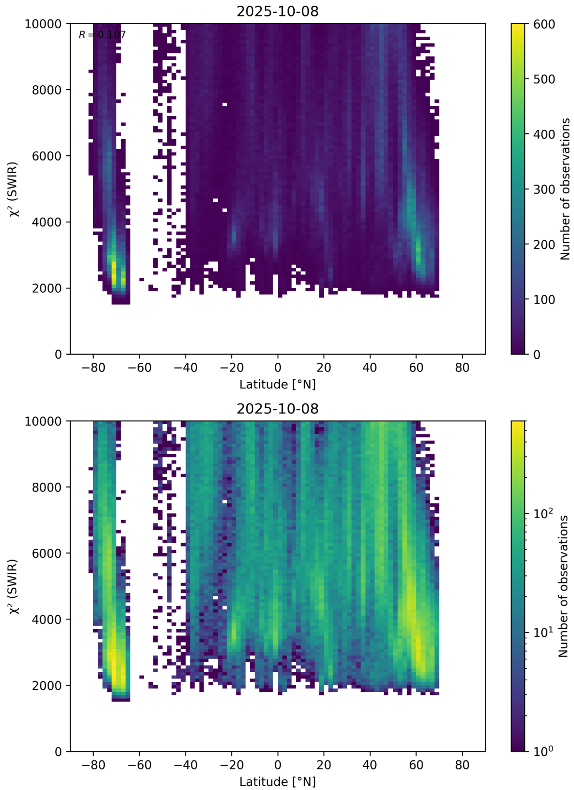
Figure 54: Scatter density plot of “Latitude” against “ \chi^2 (SWIR)” for 2025-10-07 to 2025-10-09.
