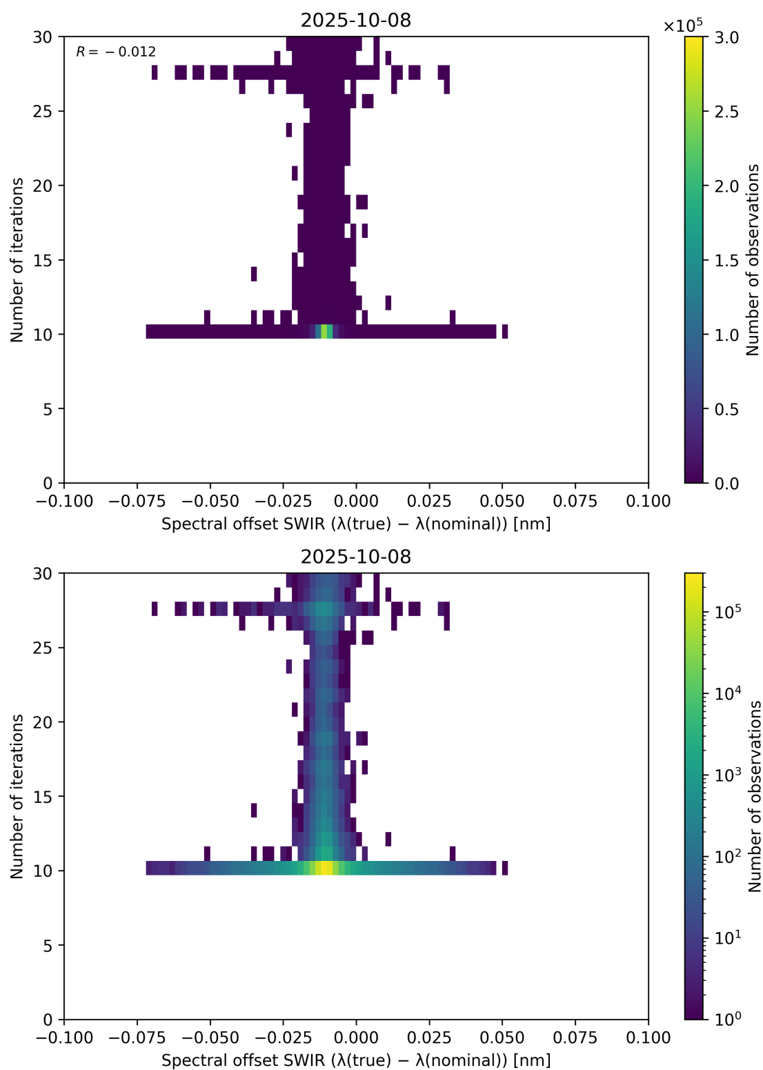
Figure 121: Scatter density plot of “Spectral offset SWIR ( \lambda_{\text{true}} - \lambda_{\text{nominal}} )” against “Number of iterations” for 2025-10-07 to 2025-10-09.
