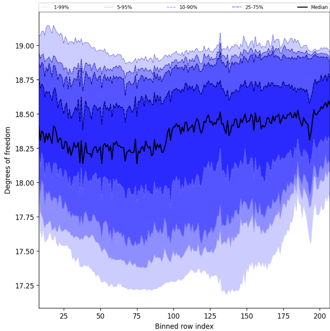
Figure 41: Along track statistics of “Degrees of freedom” for 2025-10-07 to 2025-10-09
