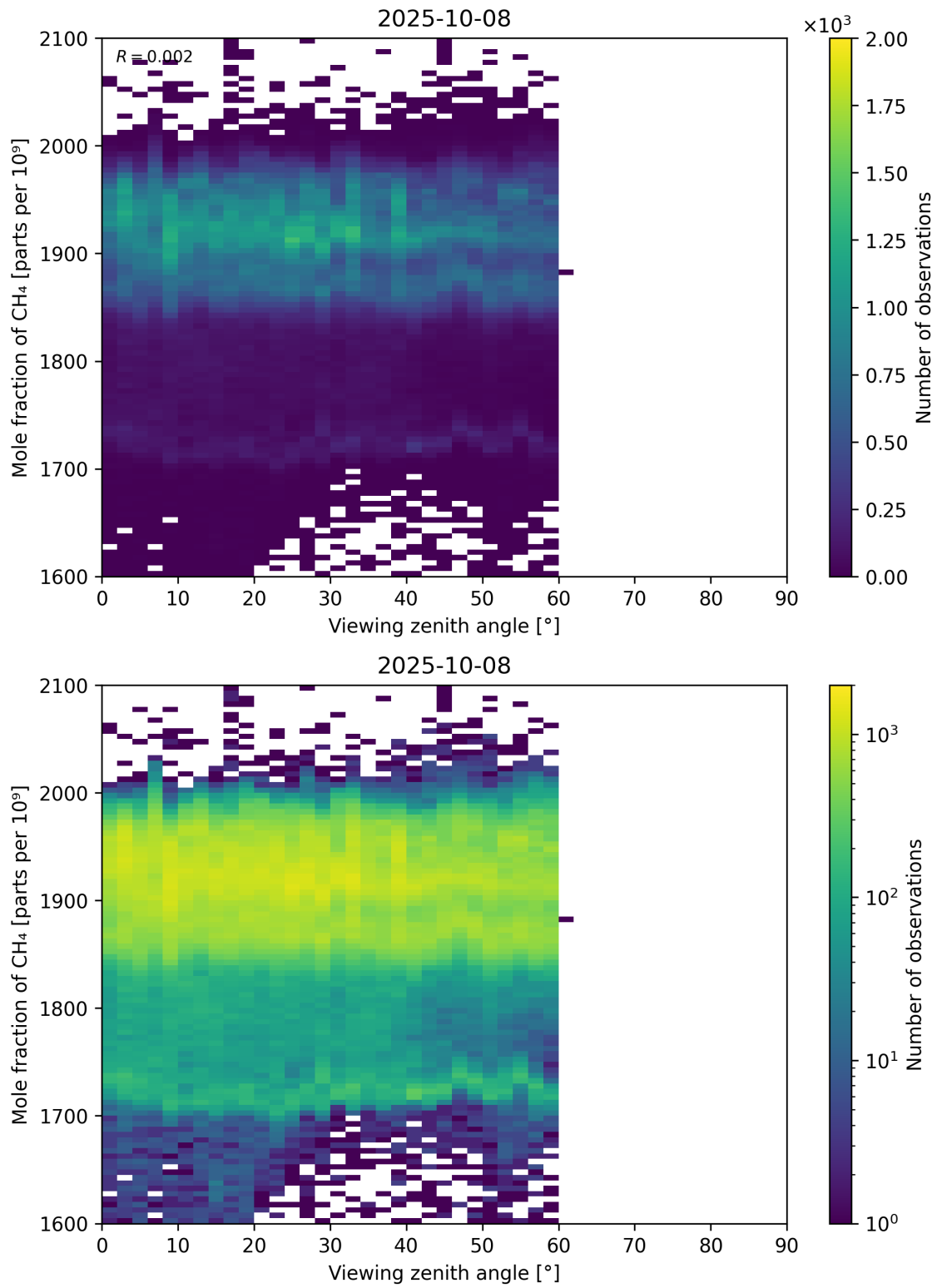
Figure 110: Scatter density plot of “Viewing zenith angle” against “Mole fraction of CH 4 ” for 2025-10-07 to 2025-10-09.
