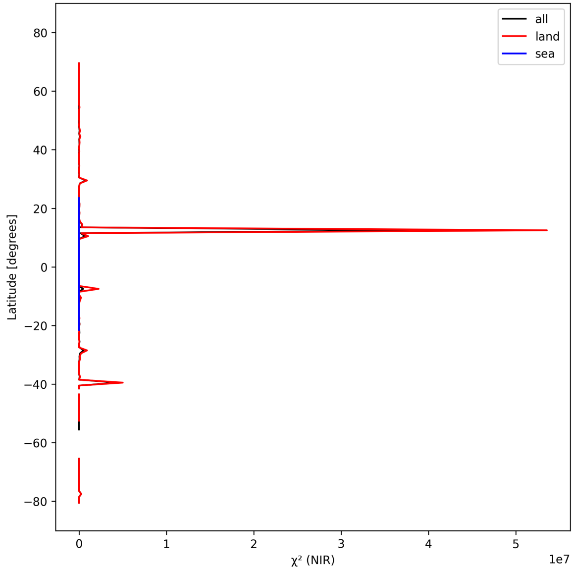
Figure 18: Zonal average of “ \chi^2 (NIR)” for 2025-10-07 to 2025-10-09.
