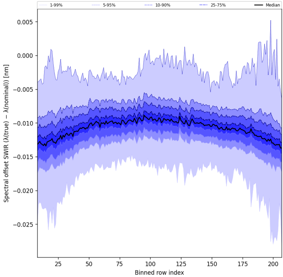
Figure 38: Along track statistics of “Spectral offset SWIR ( \lambda_{\text{true}} - \lambda_{\text{nominal}} )” for 2025-10-07 to 2025-10-09
