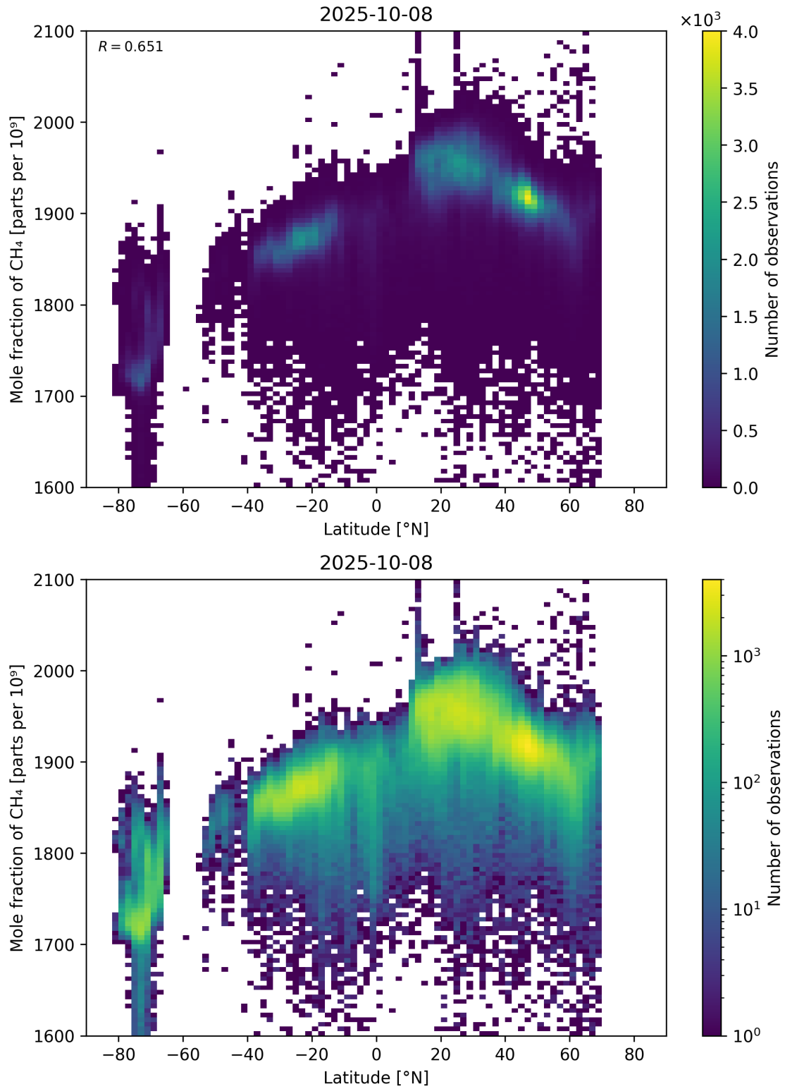
Figure 57: Scatter density plot of “Latitude” against “Mole fraction of CH 4 ” for 2025-10-07 to 2025-10-09.
