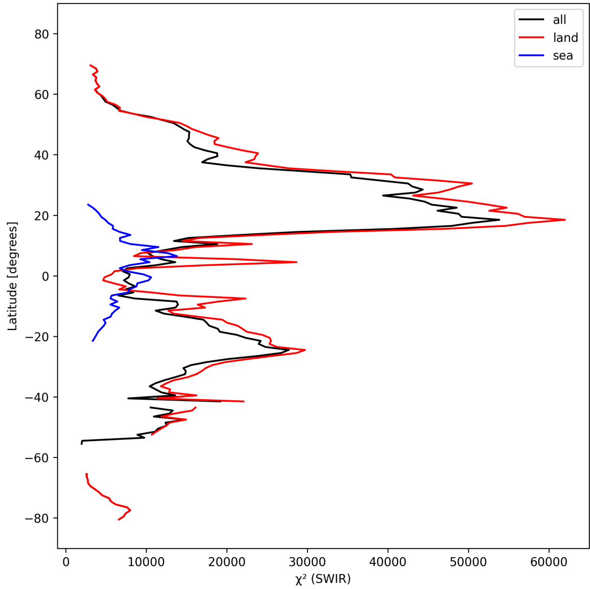
Figure 17: Zonal average of “ \chi^2 (SWIR)” for 2025-10-07 to 2025-10-09.
