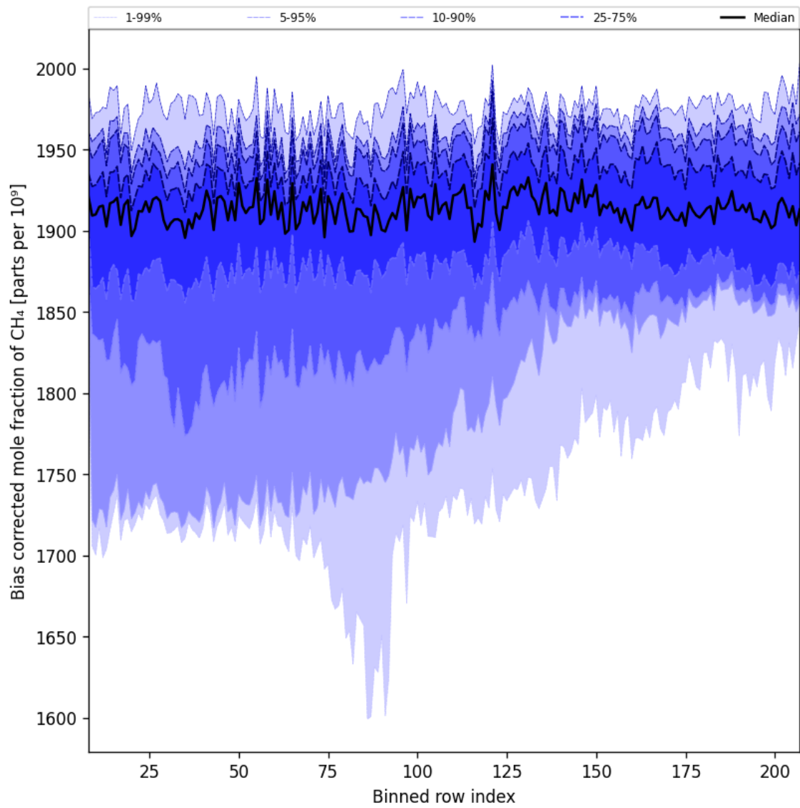
Figure 36: Along track statistics of “Bias corrected mole fraction of CH 4 ” for 2025-10-07 to 2025-10-09
