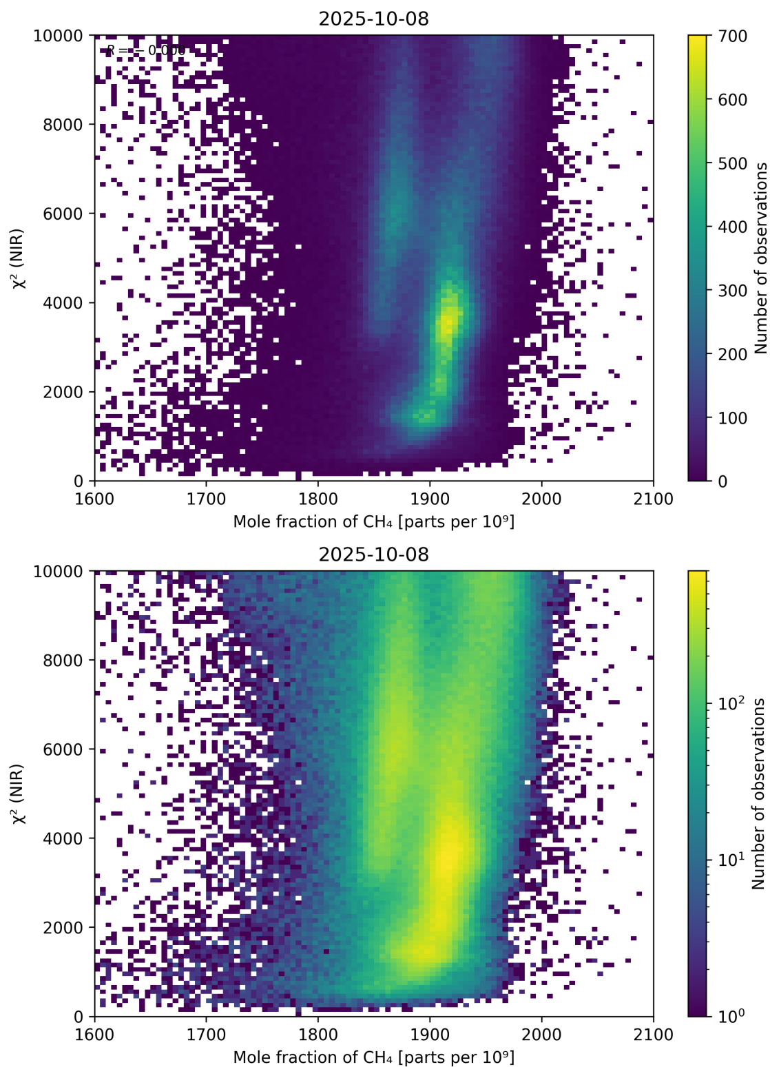
Figure 70: Scatter density plot of “Mole fraction of \text{CH}_4 ” against “ \chi^2 (NIR)” for 2025-10-07 to 2025-10-09.
