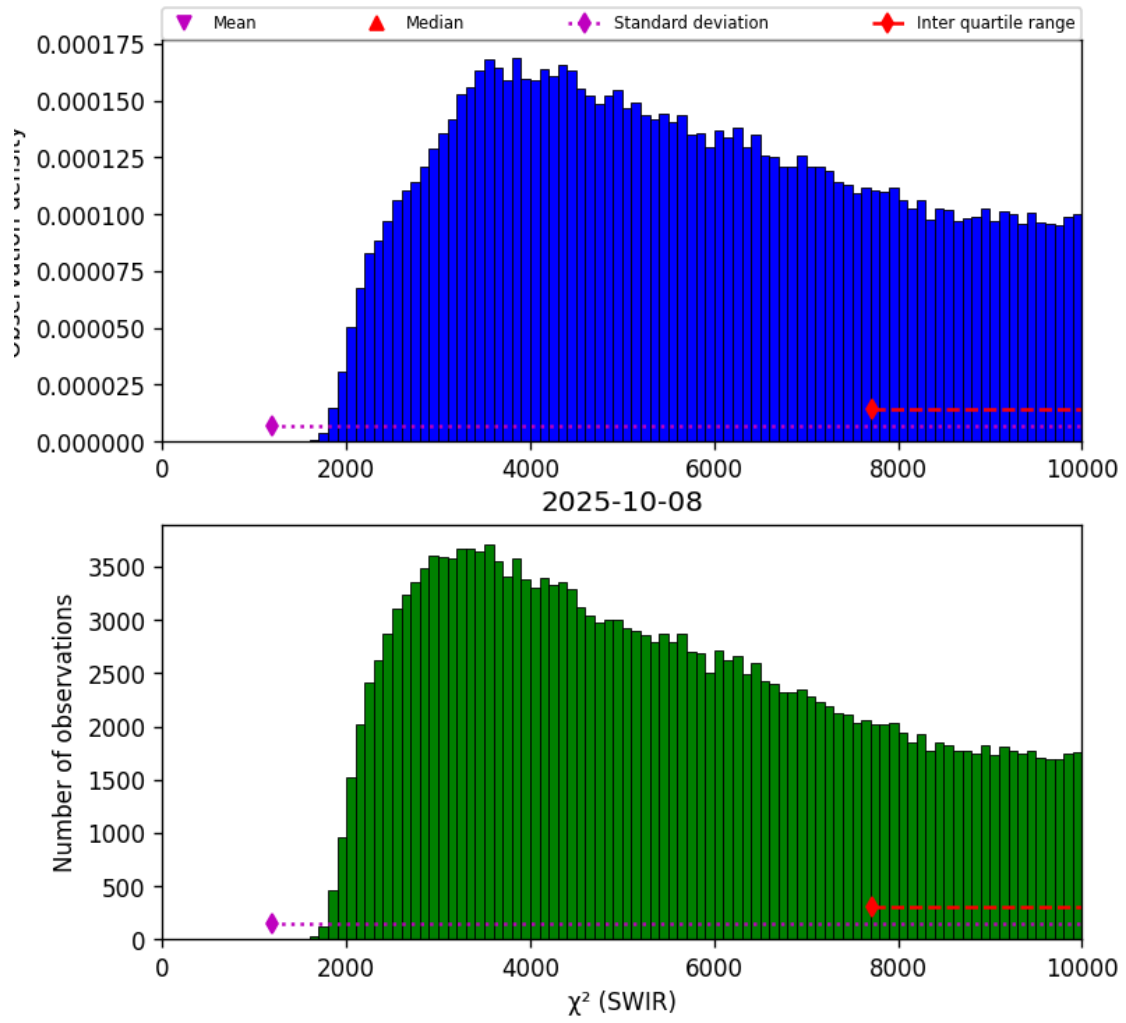
Figure 28: Histogram of “ \chi^2 (SWIR)” for 2025-10-07 to 2025-10-09
