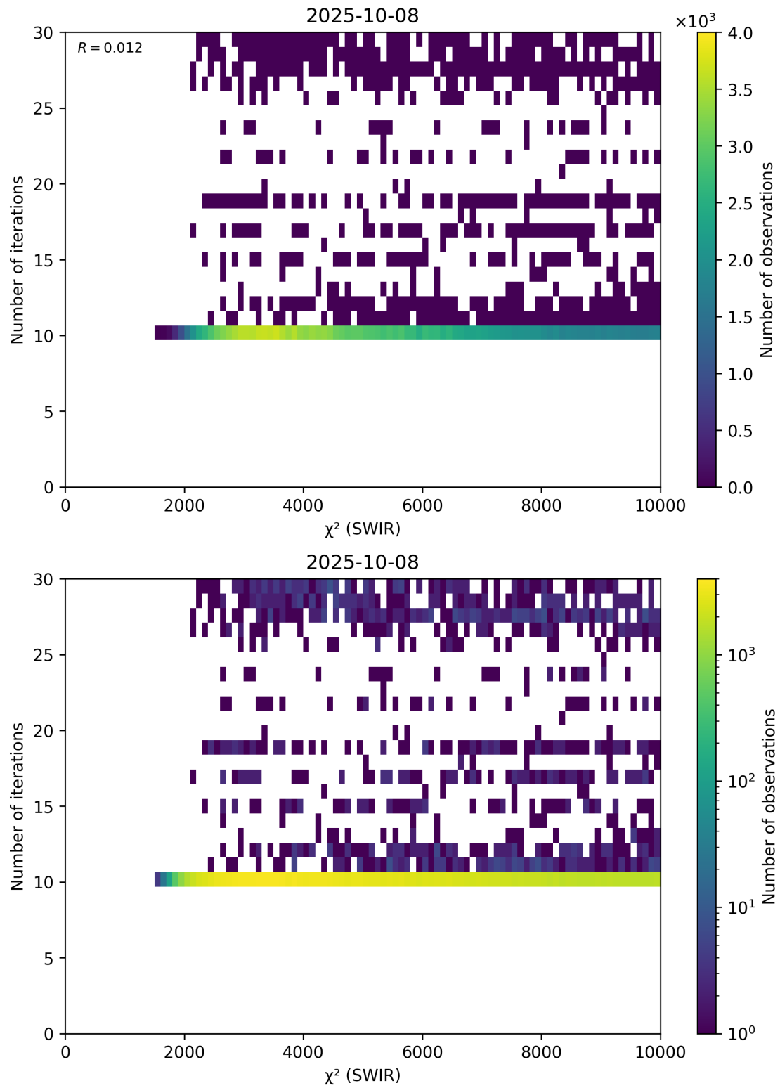
Figure 50: Scatter density plot of “ \chi^2 (SWIR)” against “Number of iterations” for 2025-10-07 to 2025-10-09.
