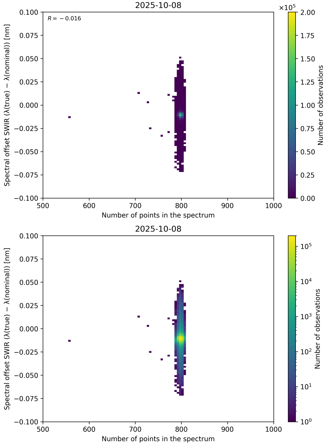
Figure 93: Scatter density plot of “Number of points in the spectrum” against “Spectral offset SWIR ( \lambda_{\text{true}} - \lambda_{\text{nominal}} )” for 2025-10-07 to 2025-10-09.
