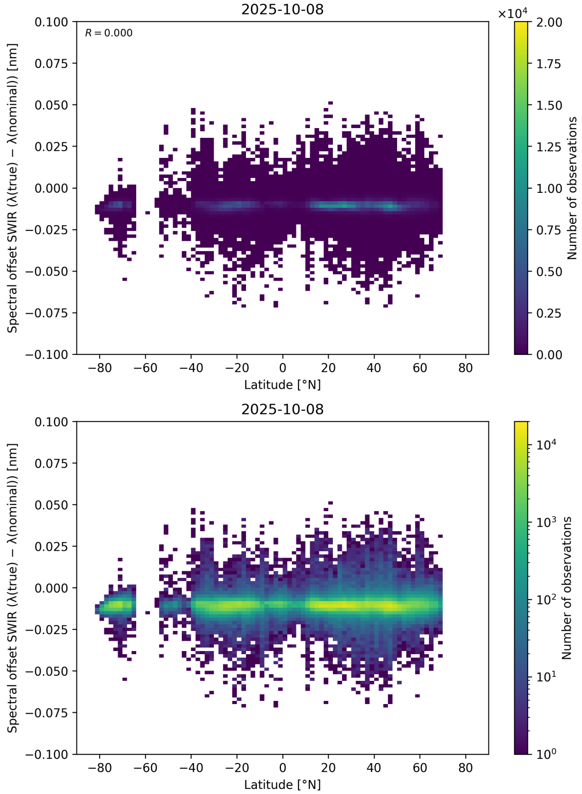
Figure 62: Scatter density plot of “Latitude” against “Spectral offset SWIR ( \lambda_{\text{true}} - \lambda_{\text{nominal}} )” for 2025-10-07 to 2025-10-09.
