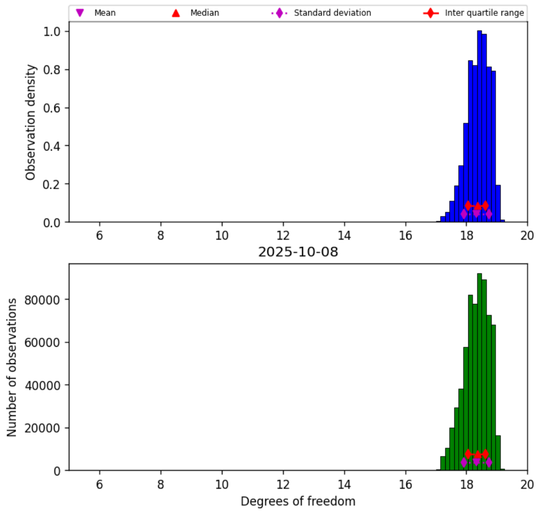
Figure 30: Histogram of “Degrees of freedom” for 2025-10-07 to 2025-10-09
