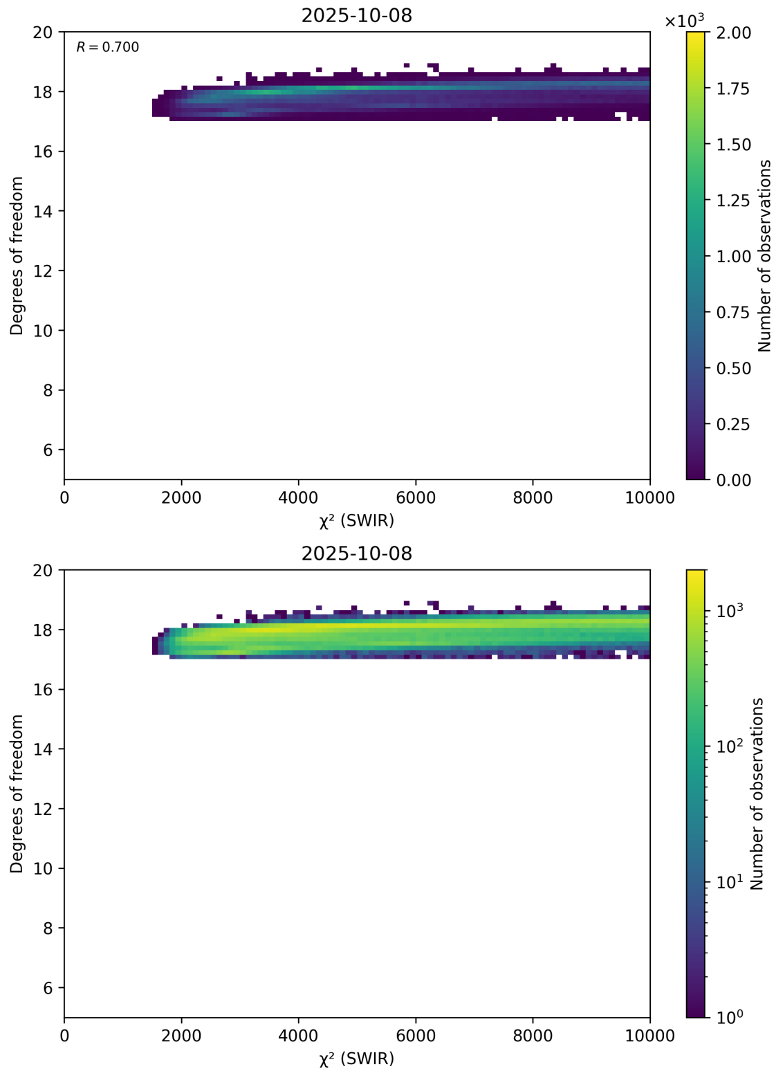
Figure 48: Scatter density plot of “ \chi^2 (SWIR)” against “Degrees of freedom” for 2025-10-07 to 2025-10-09.
