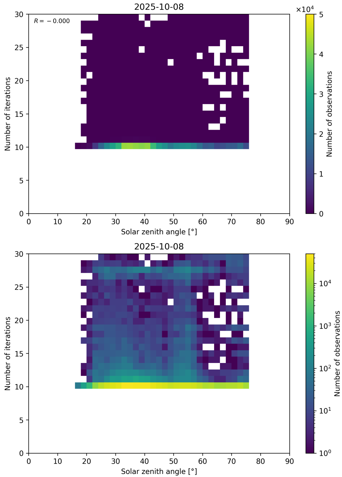
Figure 102: Scatter density plot of “Solar zenith angle” against “Number of iterations” for 2025-10-07 to 2025-10-09.
