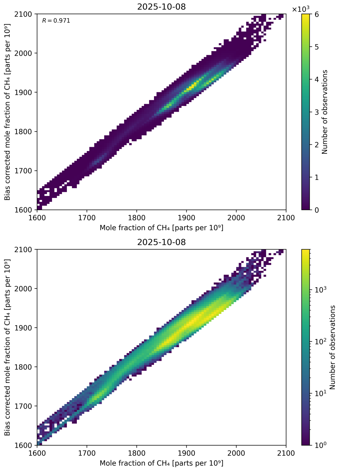
Figure 74: Scatter density plot of “Mole fraction of CH 4 ” against “Bias corrected mole fraction of CH 4 ” for 2025-10-07 to 2025-10-09.
