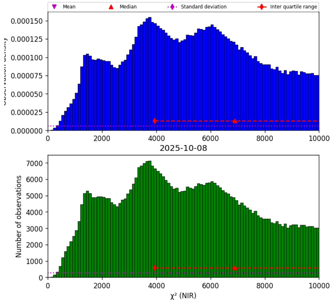
Figure 29: Histogram of “ \chi^2 (NIR)” for 2025-10-07 to 2025-10-09
