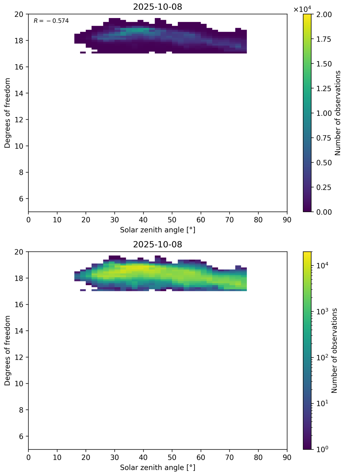
Figure 96: Scatter density plot of “Solar zenith angle” against “Degrees of freedom” for 2025-10-07 to 2025-10-09.
