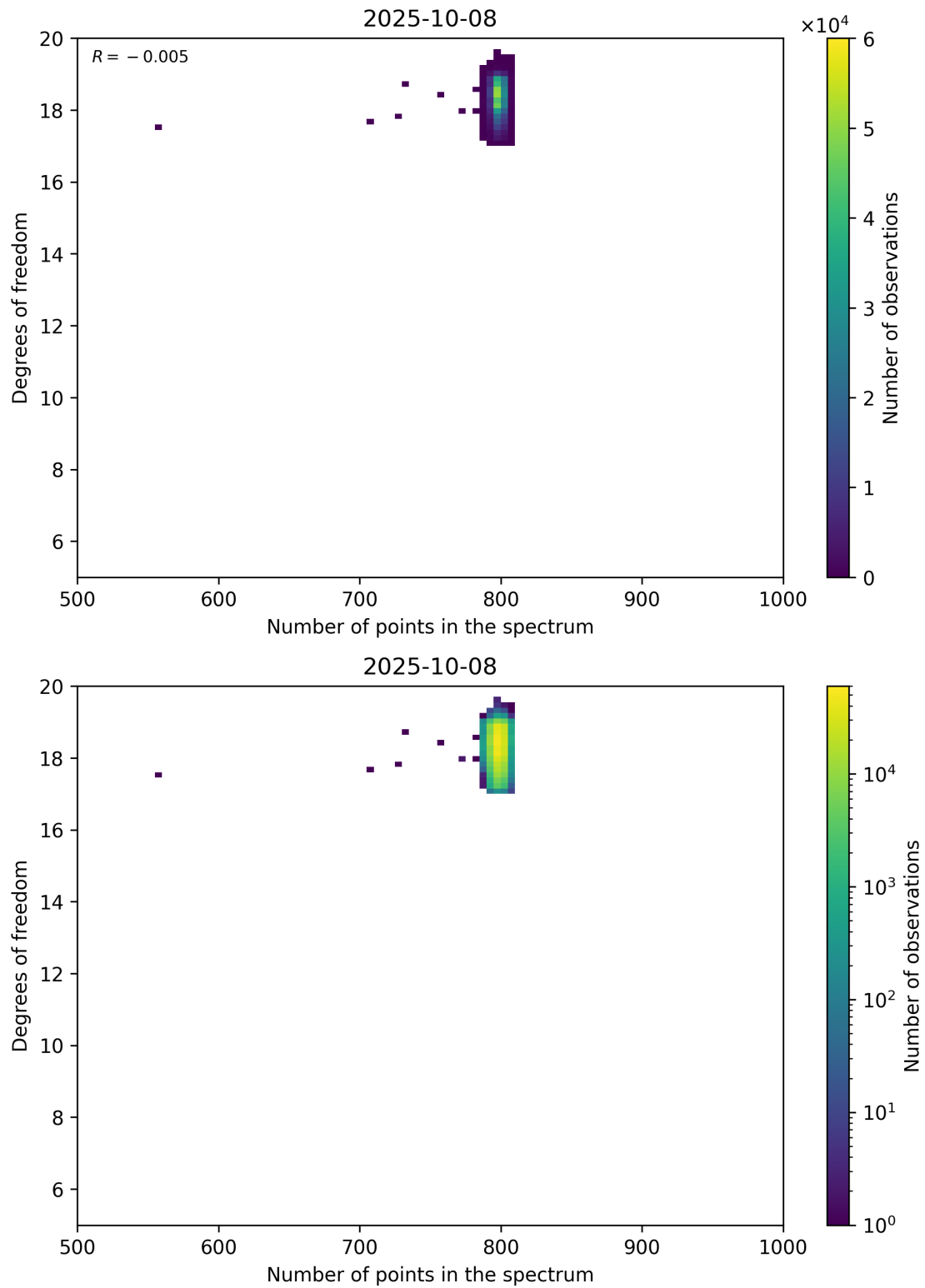
Figure 90: Scatter density plot of “Number of points in the spectrum” against “Degrees of freedom” for 2025-10-07 to 2025-10-09.
