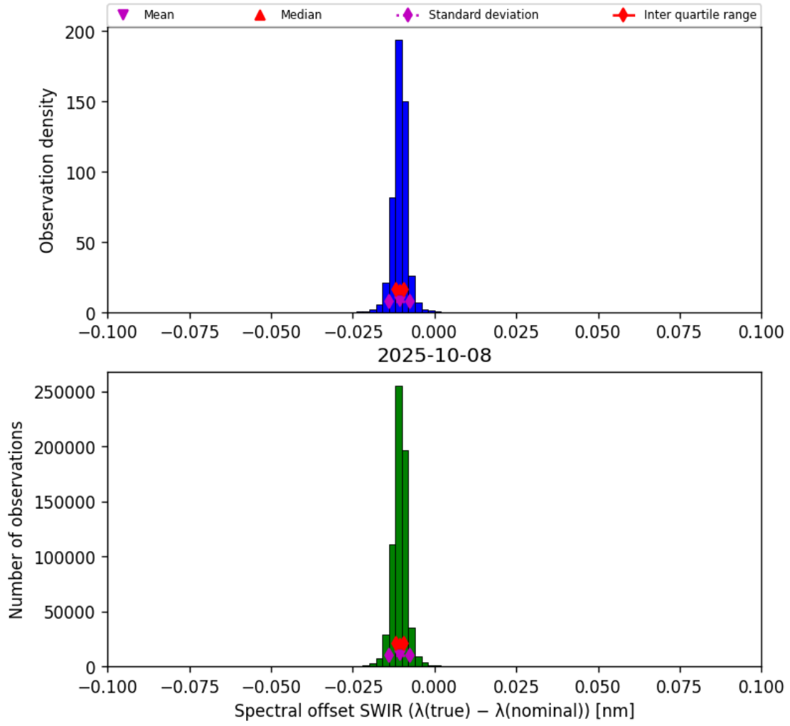
Figure 27: Histogram of “Spectral offset SWIR ( \lambda_{\text{true}} - \lambda_{\text{nominal}} )” for 2025-10-07 to 2025-10-09
