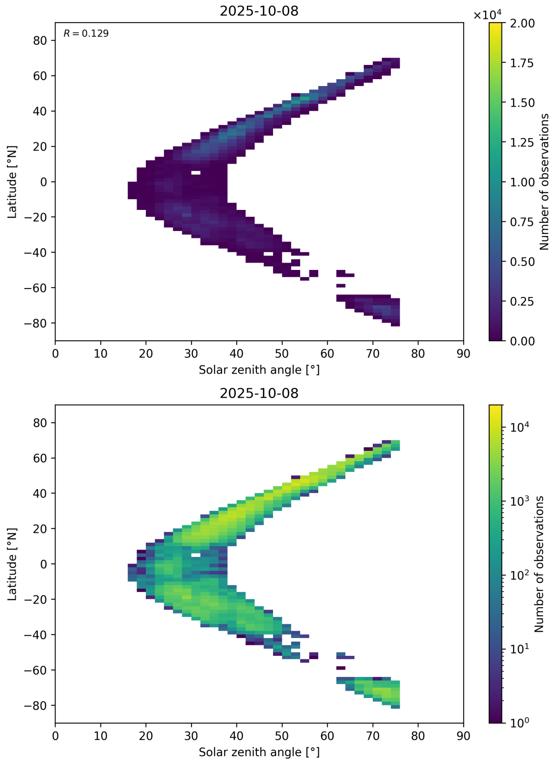
Figure 98: Scatter density plot of “Solar zenith angle” against “Latitude” for 2025-10-07 to 2025-10-09.
