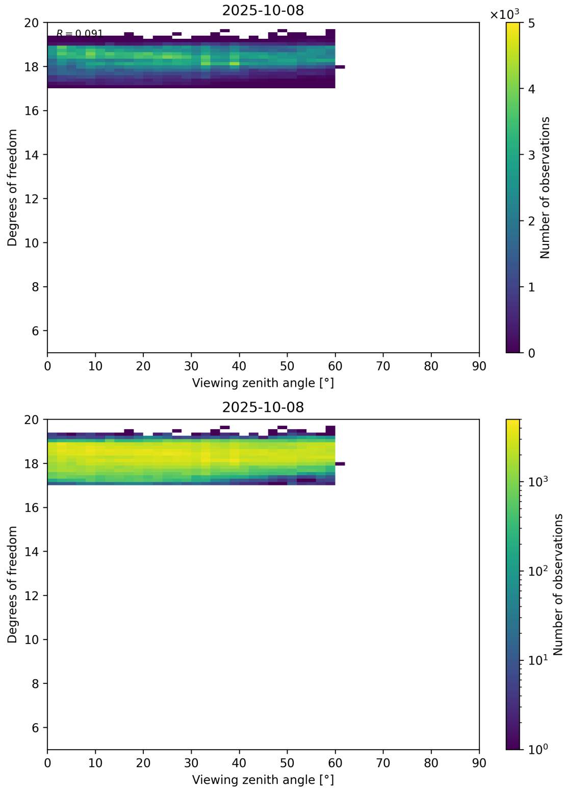
Figure 107: Scatter density plot of “Viewing zenith angle” against “Degrees of freedom” for 2025-10-07 to 2025-10-09.
