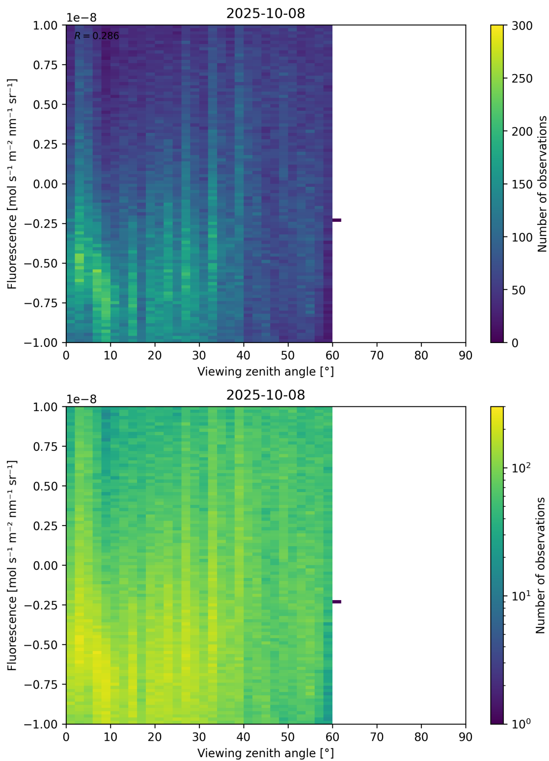
Figure 108: Scatter density plot of “Viewing zenith angle” against “Fluorescence” for 2025-10-07 to 2025-10-09.
