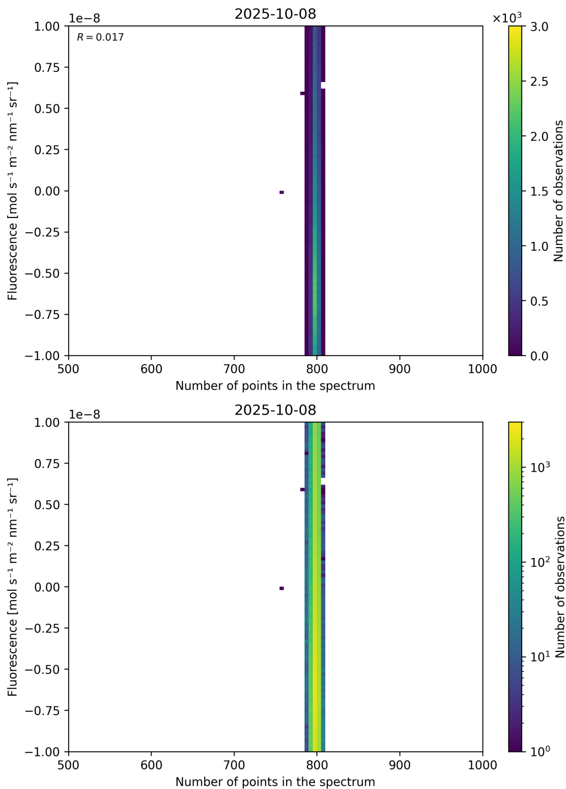
Figure 91: Scatter density plot of “Number of points in the spectrum” against “Fluorescence” for 2025-10-07 to 2025-10-09.
