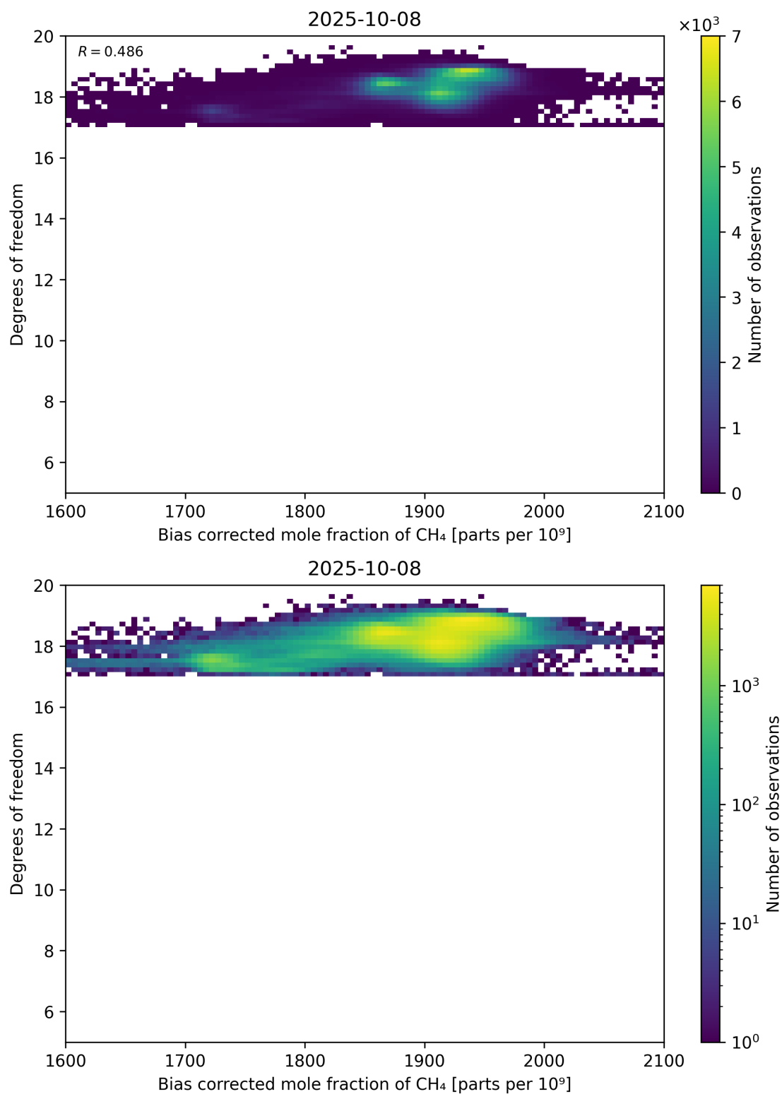
Figure 65: Scatter density plot of “Bias corrected mole fraction of CH 4 ” against “Degrees of freedom” for 2025-10-07 to 2025-10-09.
