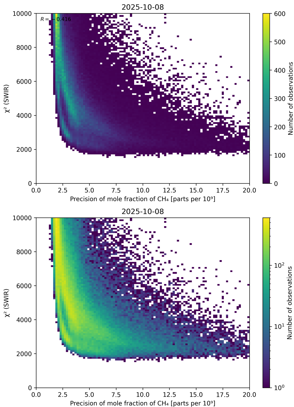
Figure 79: Scatter density plot of “Precision of mole fraction of \text{CH}_4 ” against “ \chi^2 (SWIR)” for 2025-10-07 to 2025-10-09.
