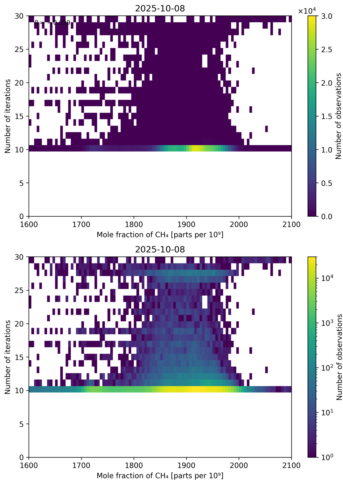
Figure 76: Scatter density plot of “Mole fraction of CH 4 ” against “Number of iterations” for 2025-10-07 to 2025-10-09.
