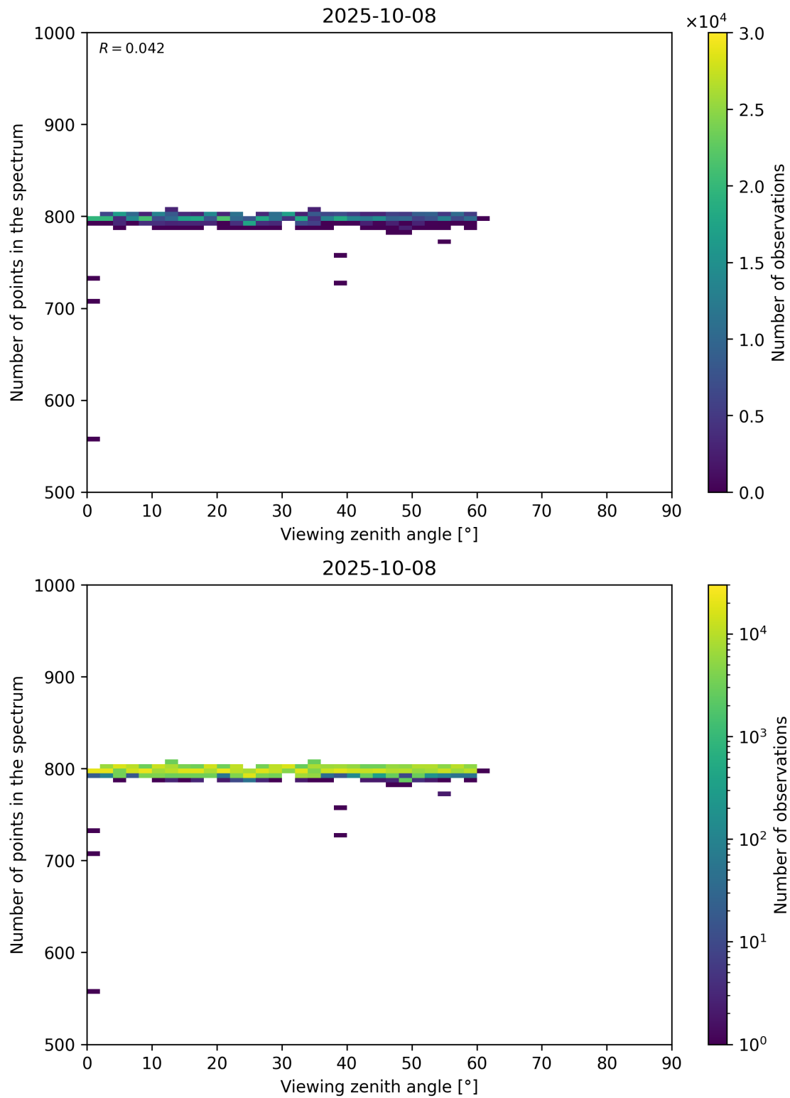
Figure 114: Scatter density plot of “Viewing zenith angle” against “Number of points in the spectrum” for 2025-10-07 to 2025-10-09.
