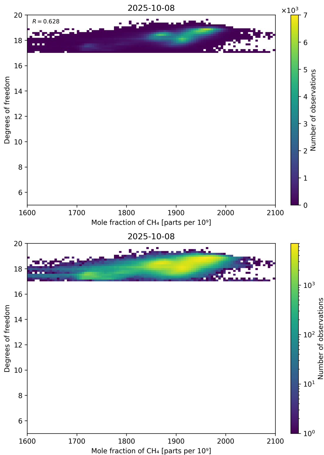
Figure 72: Scatter density plot of “Mole fraction of CH 4 ” against “Degrees of freedom” for 2025-10-07 to 2025-10-09.
