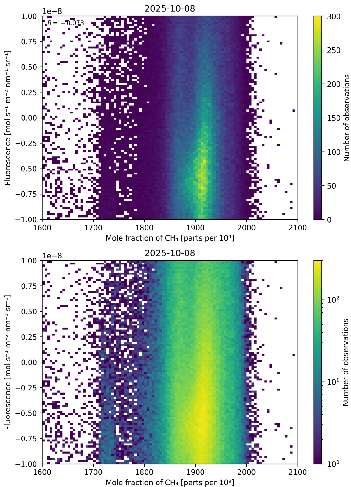
Figure 73: Scatter density plot of “Mole fraction of \text{CH}_4 ” against “Fluorescence” for 2025-10-07 to 2025-10-09.
