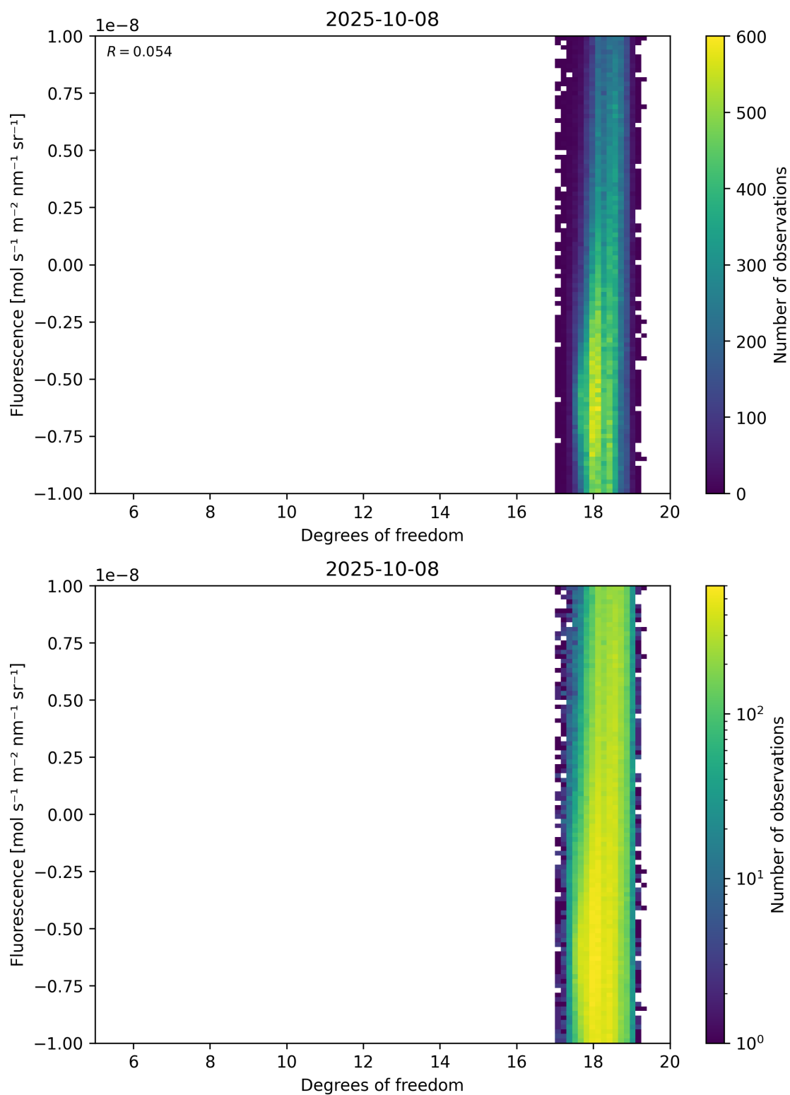
Figure 51: Scatter density plot of “Degrees of freedom” against “Fluorescence” for 2025-10-07 to 2025-10-09.
