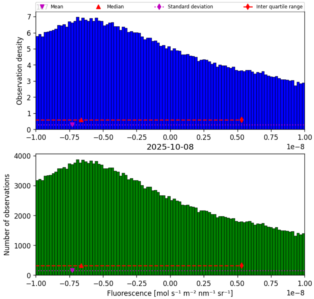
Figure 32: Histogram of “Fluorescence” for 2025-10-07 to 2025-10-09
