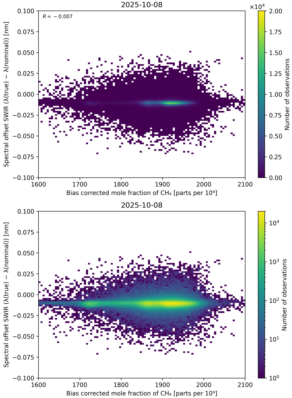
Figure 69: Scatter density plot of “Bias corrected mole fraction of CH 4 ” against “Spectral offset SWIR ( \lambda_{\text{true}} - \lambda_{\text{nominal}} )” for 2025-10-07 to 2025-10-09.
