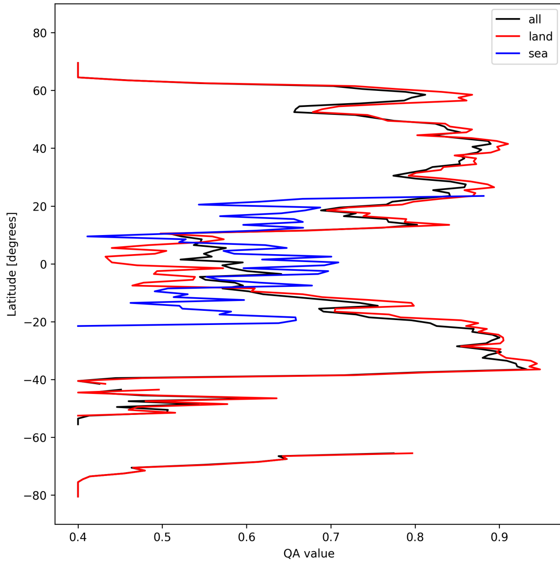
Figure 11: Zonal average of “QA value” for 2025-10-07 to 2025-10-09.
