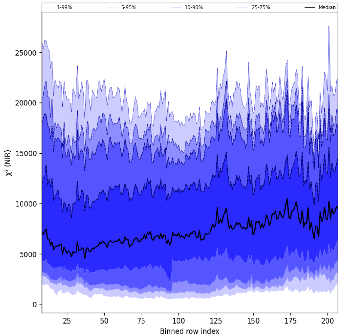
Figure 40: Along track statistics of “ \chi^2 (NIR)” for 2025-10-07 to 2025-10-09
