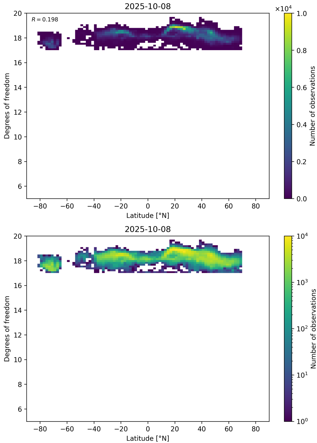
Figure 55: Scatter density plot of “Latitude” against “Degrees of freedom” for 2025-10-07 to 2025-10-09.
