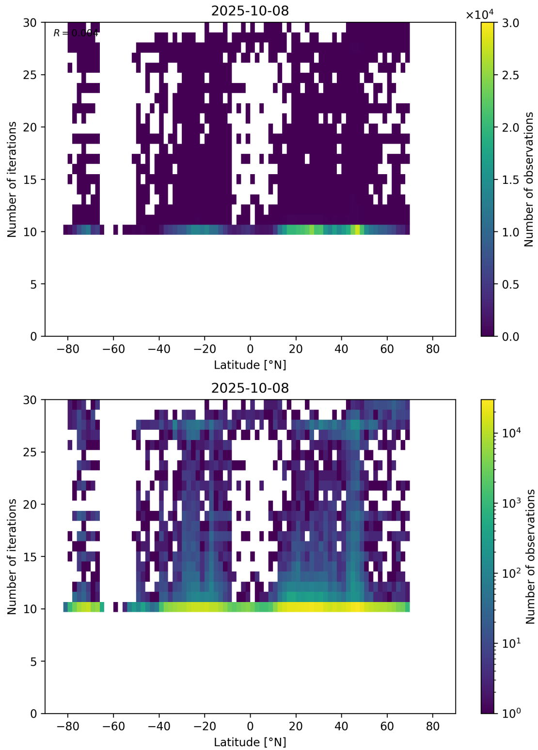
Figure 60: Scatter density plot of “Latitude” against “Number of iterations” for 2025-10-07 to 2025-10-09.
