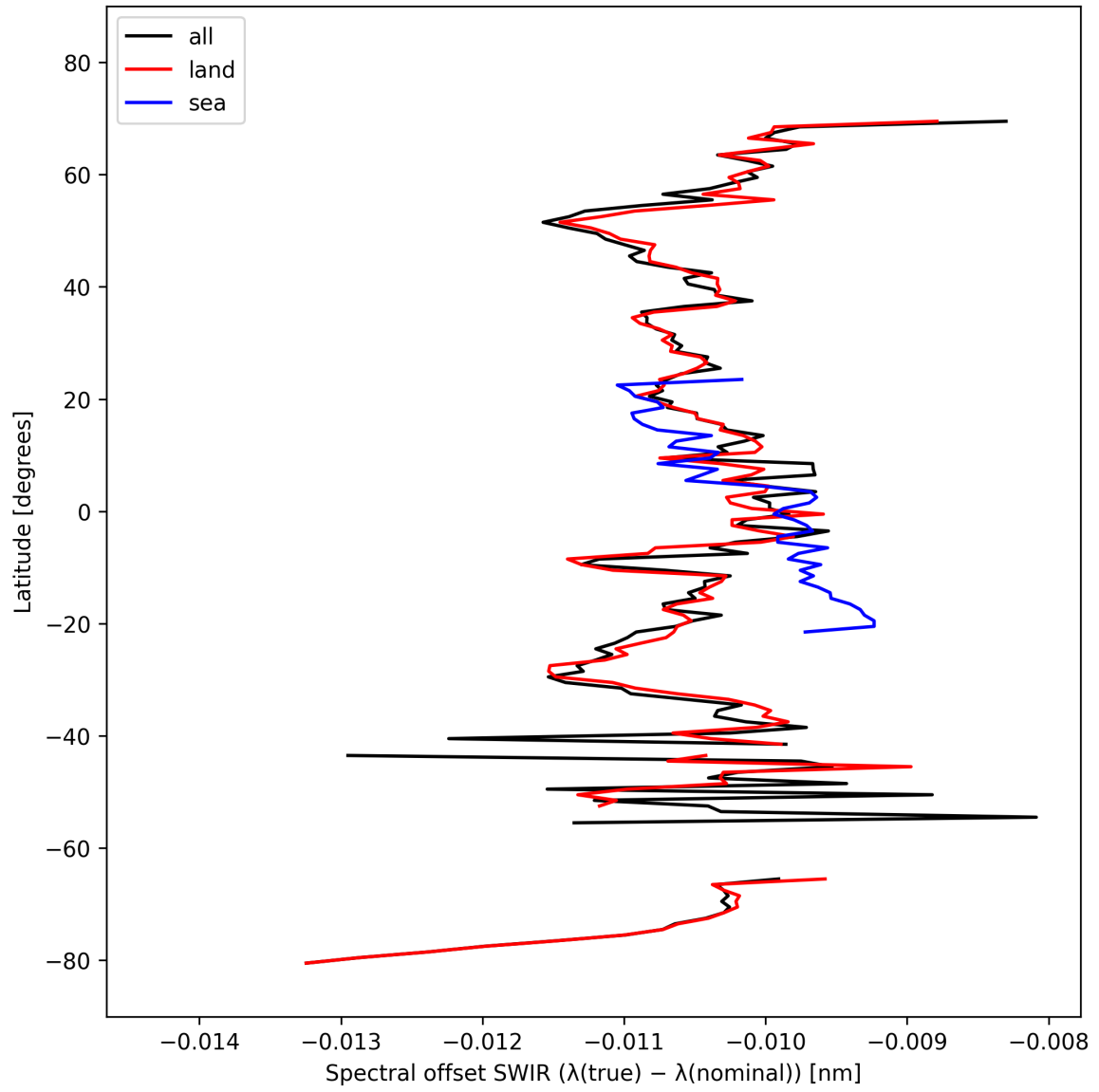
Figure 16: Zonal average of “Spectral offset SWIR ( \lambda_{\text{true}} - \lambda_{\text{nominal}} )” for 2025-10-07 to 2025-10-09.
