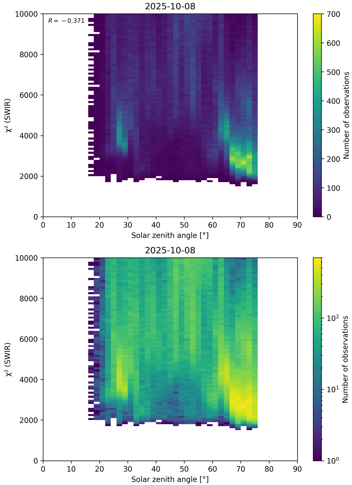
Figure 95: Scatter density plot of “Solar zenith angle” against “ \chi^2 (SWIR)” for 2025-10-07 to 2025-10-09.
