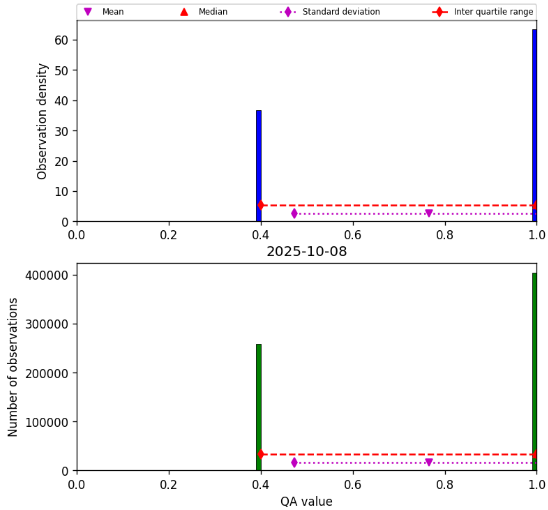
Figure 22: Histogram of “QA value” for 2025-10-07 to 2025-10-09
