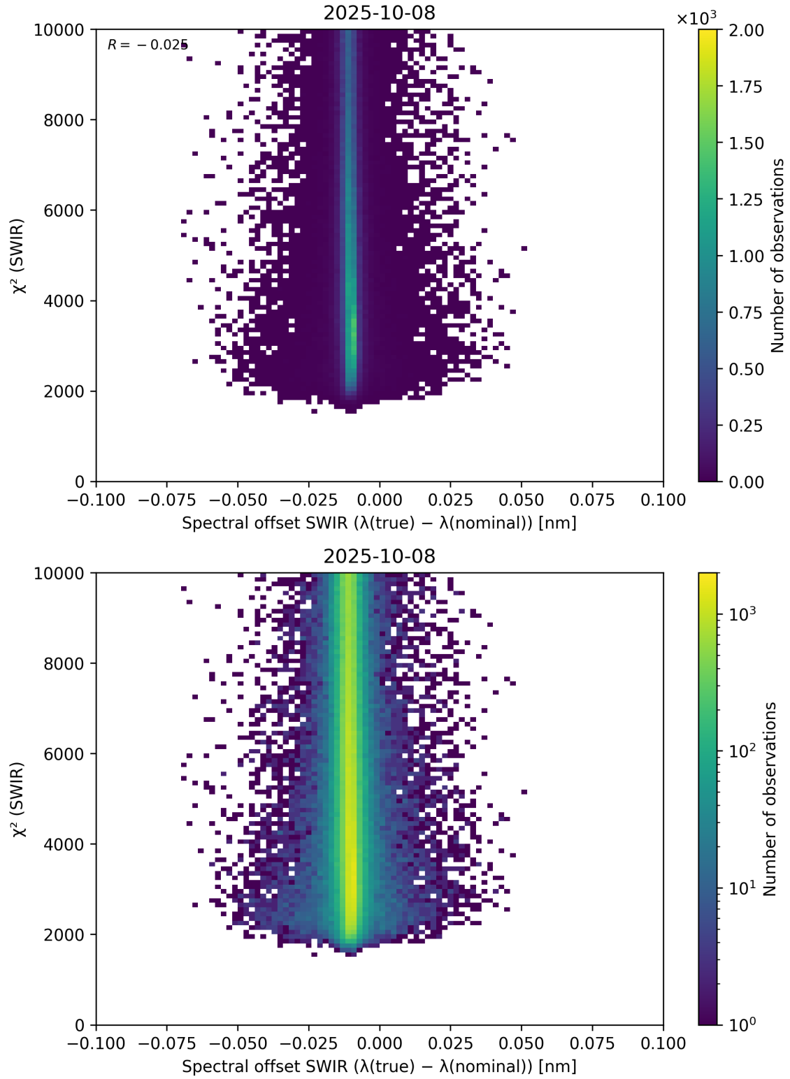
Figure 118: Scatter density plot of “Spectral offset SWIR ( \lambda_{\text{true}} - \lambda_{\text{nominal}} )” against “ \chi^2 (SWIR)” for 2025-10-07 to 2025-10-09.
