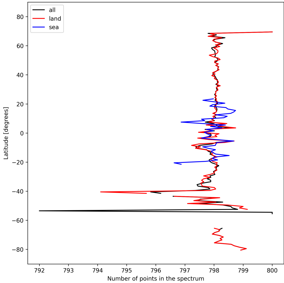
Figure 15: Zonal average of “Number of points in the spectrum” for 2025-10-07 to 2025-10-09.
