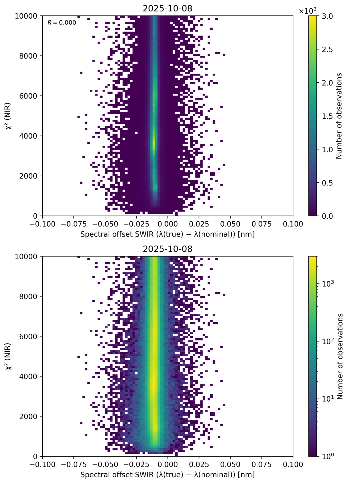
Figure 117: Scatter density plot of “Spectral offset SWIR ( \lambda_{\text{true}} - \lambda_{\text{nominal}} )” against “ \chi^2 (NIR)” for 2025-10-07 to 2025-10-09.
