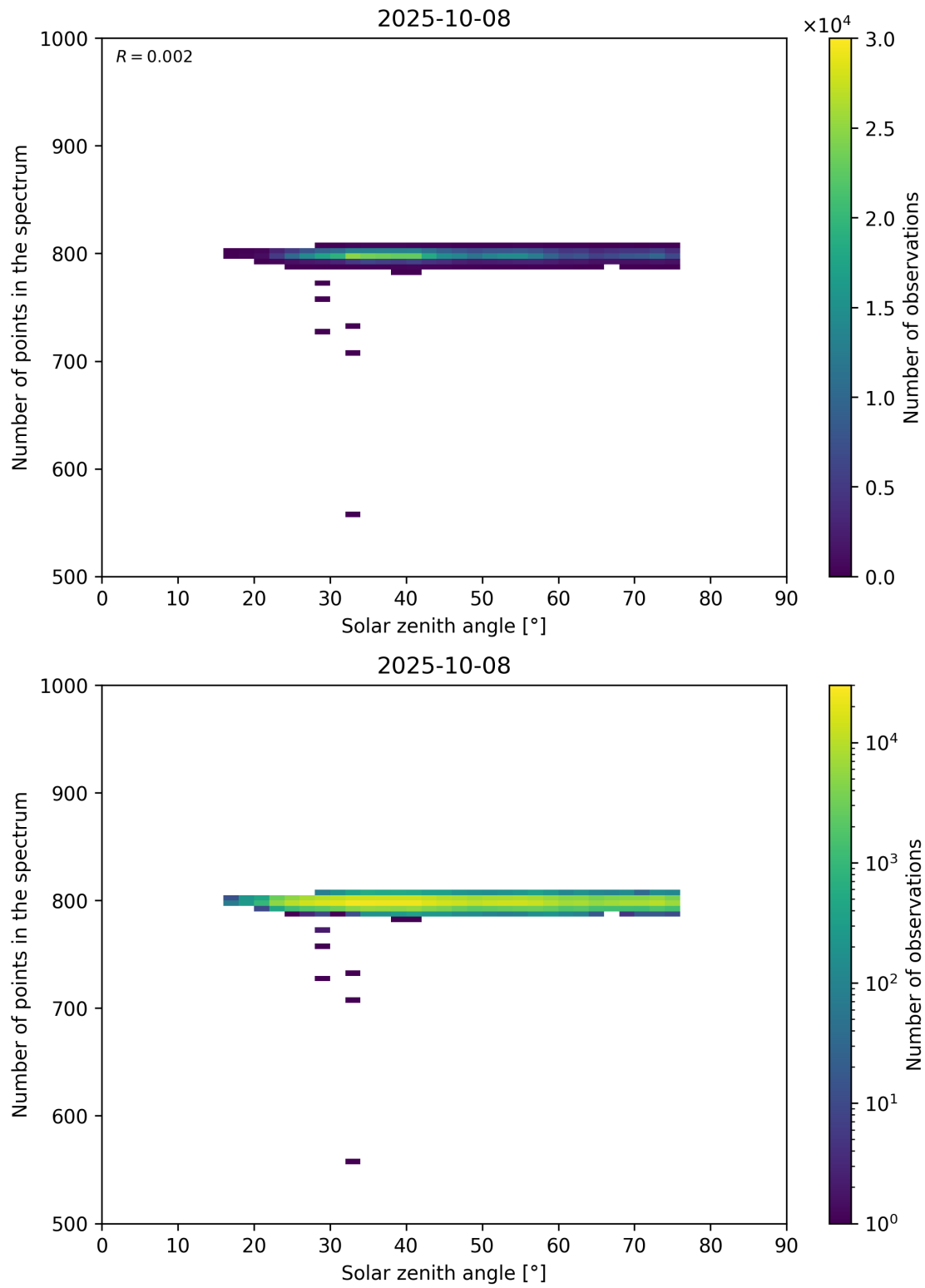
Figure 103: Scatter density plot of “Solar zenith angle” against “Number of points in the spectrum” for 2025-10-07 to 2025-10-09.
