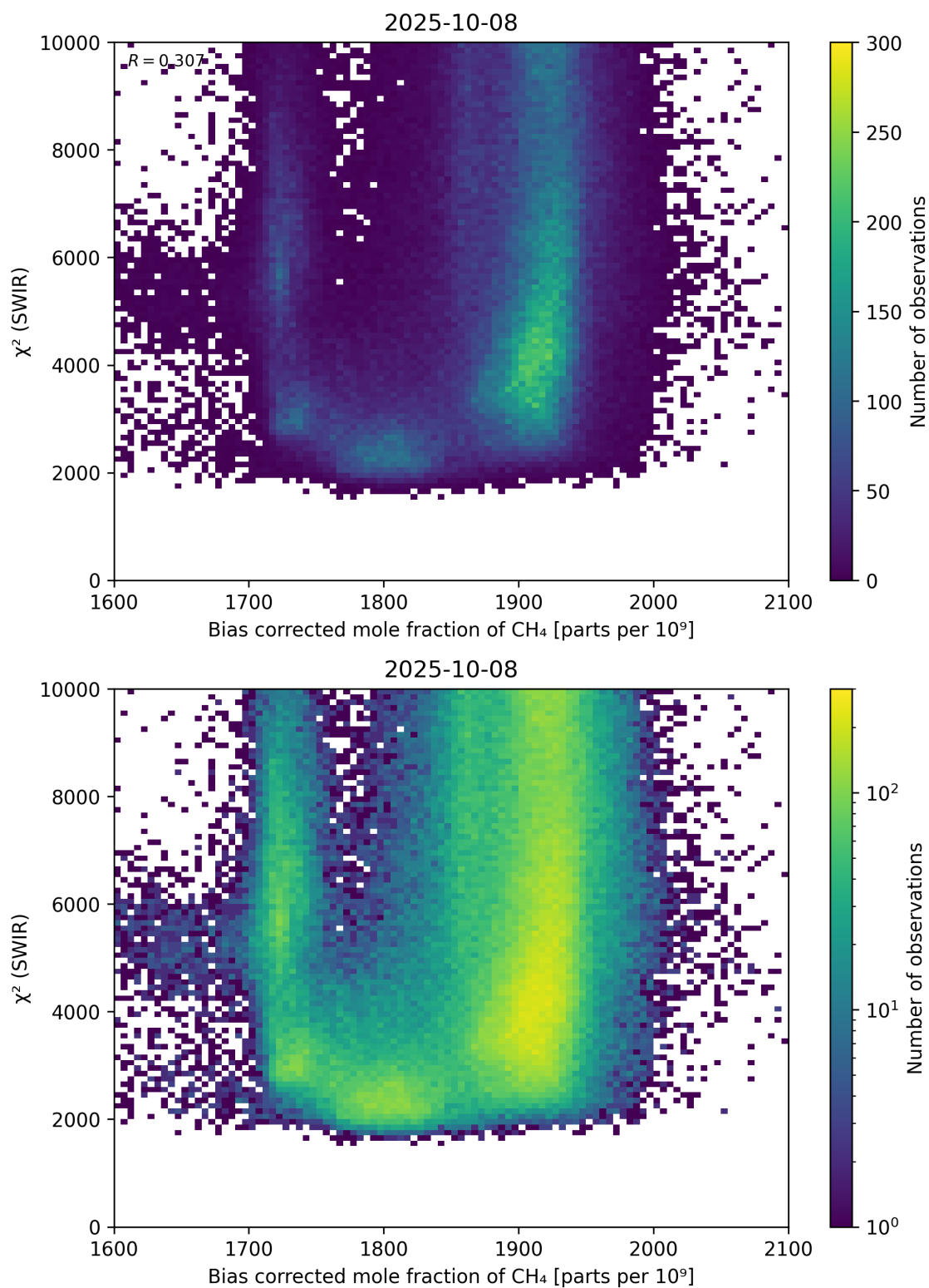
Figure 64: Scatter density plot of “Bias corrected mole fraction of \text{CH}_4 ” against “ \chi^2 (SWIR)” for 2025-10-07 to 2025-10-09.
