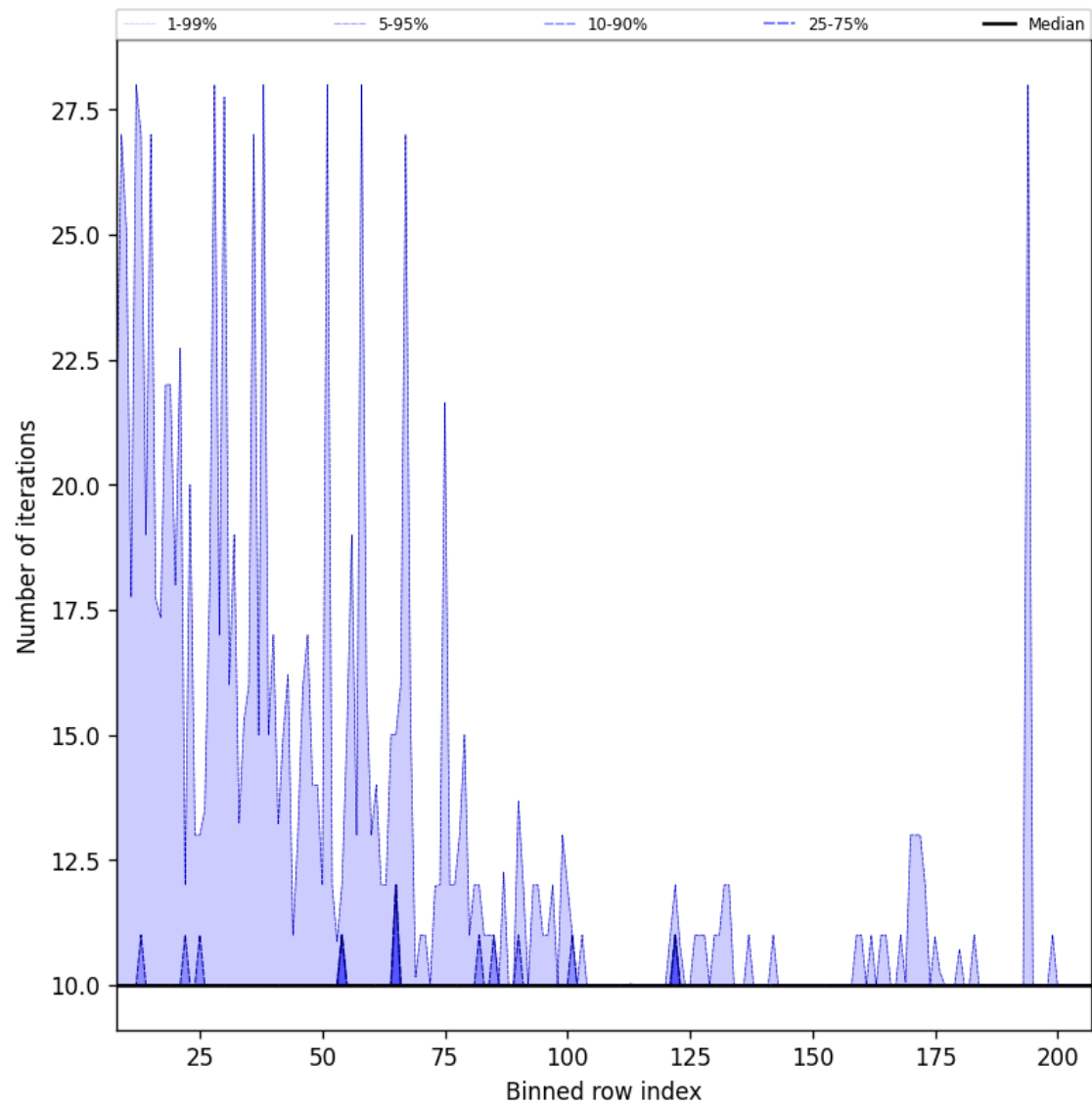
Figure 42: Along track statistics of “Number of iterations” for 2025-10-07 to 2025-10-09
