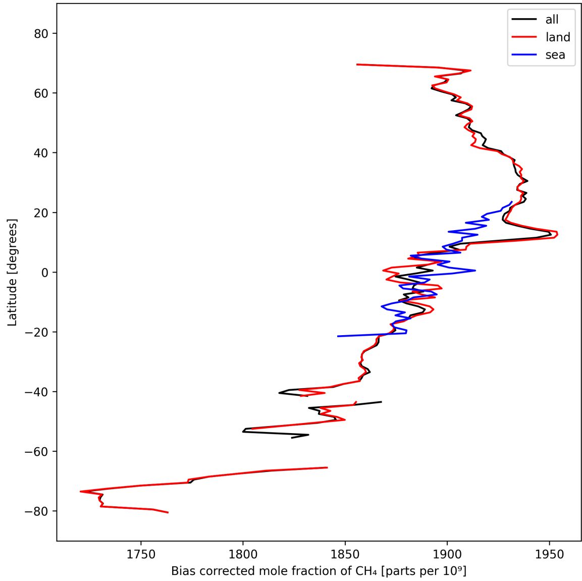
Figure 14: Zonal average of “Bias corrected mole fraction of \text{CH}_4 ” for 2025-10-07 to 2025-10-09.
