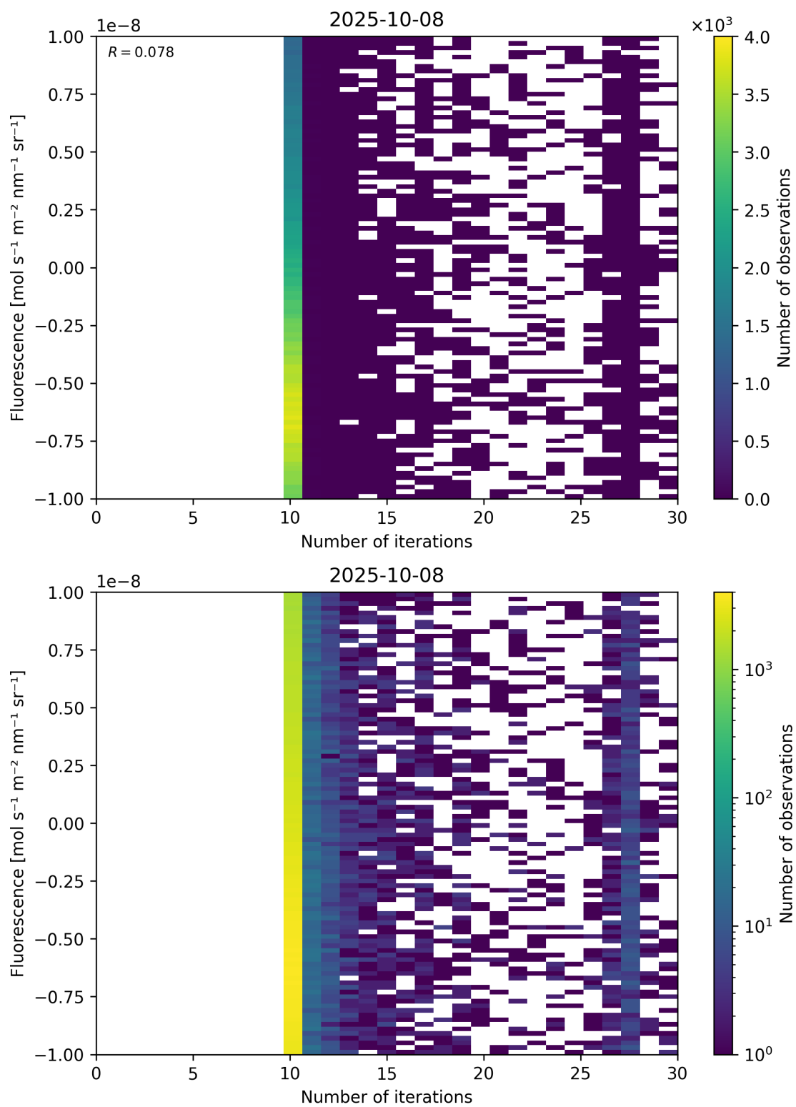
Figure 87: Scatter density plot of “Number of iterations” against “Fluorescence” for 2025-10-07 to 2025-10-09.
