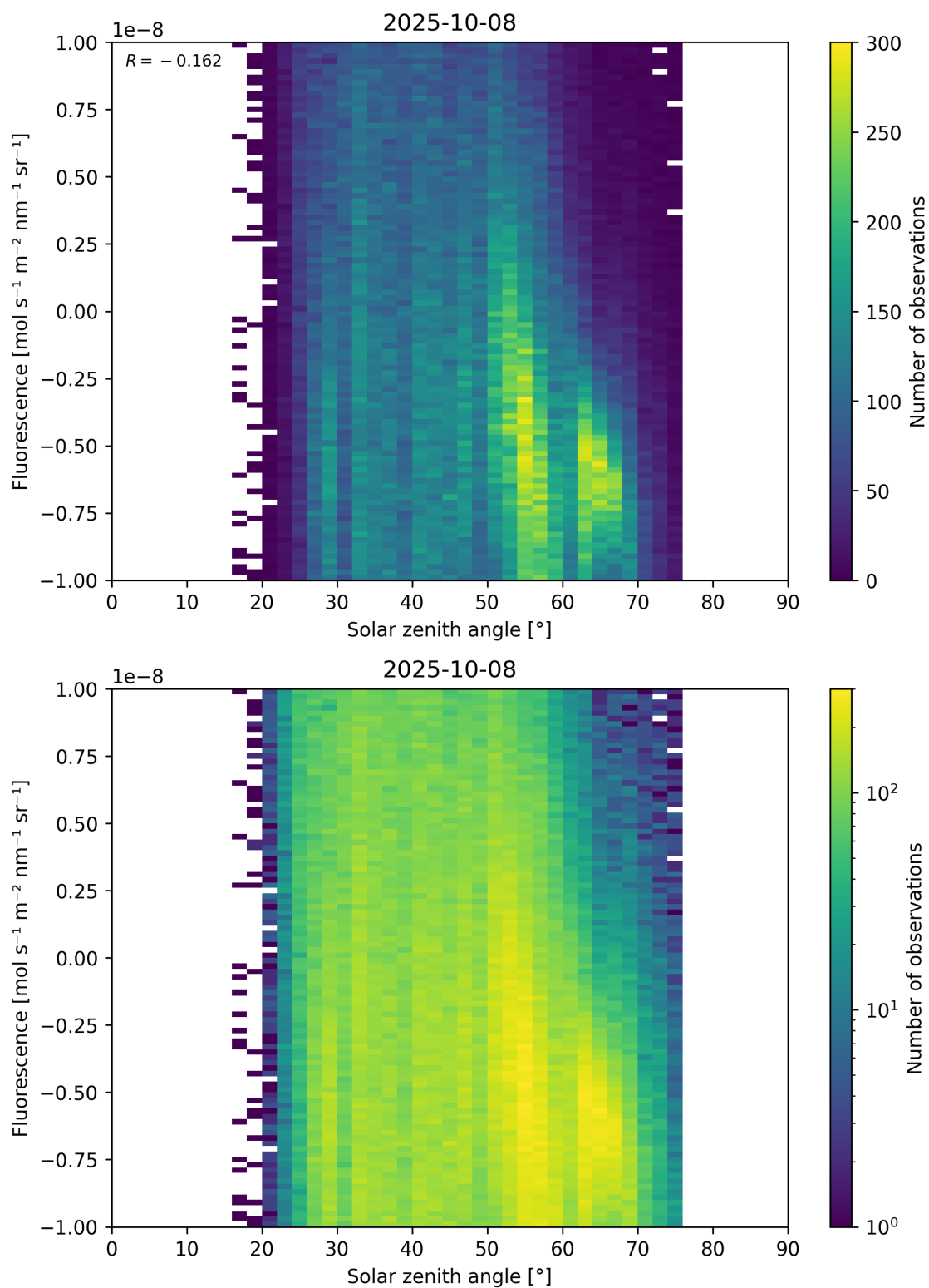
Figure 97: Scatter density plot of “Solar zenith angle” against “Fluorescence” for 2025-10-07 to 2025-10-09.
