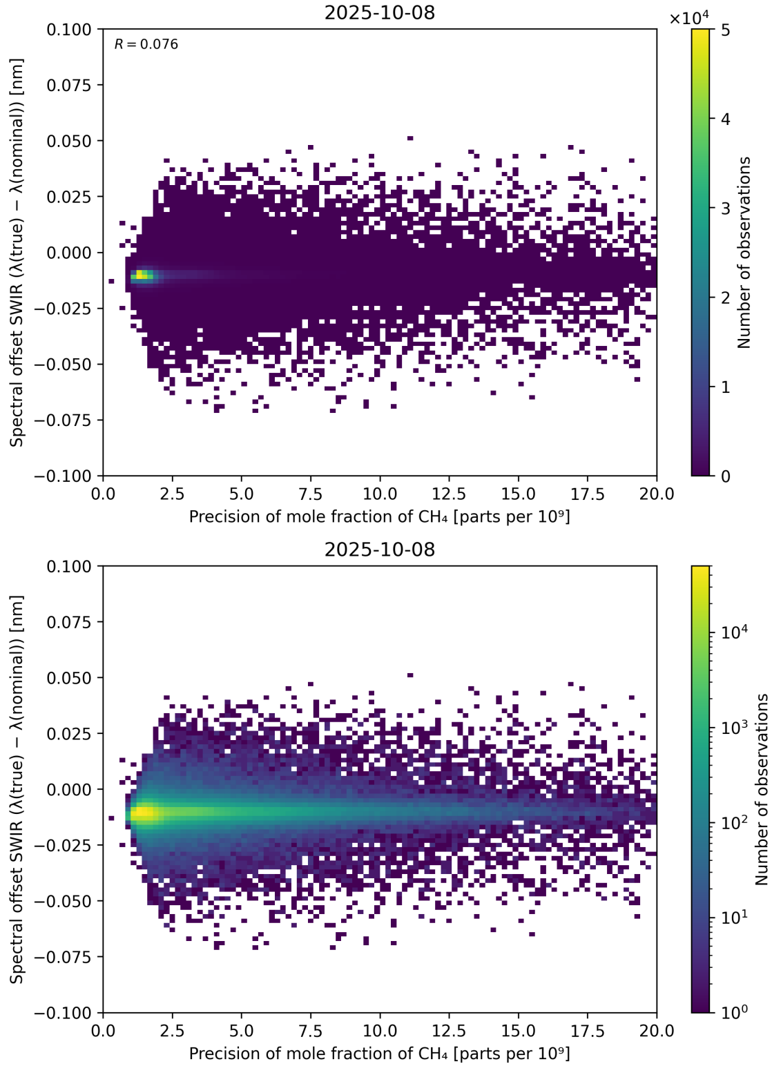
Figure 85: Scatter density plot of “Precision of mole fraction of CH 4 ” against “Spectral offset SWIR ( \lambda_{\text{true}} - \lambda_{\text{nominal}} )” for 2025-10-07 to 2025-10-09.
