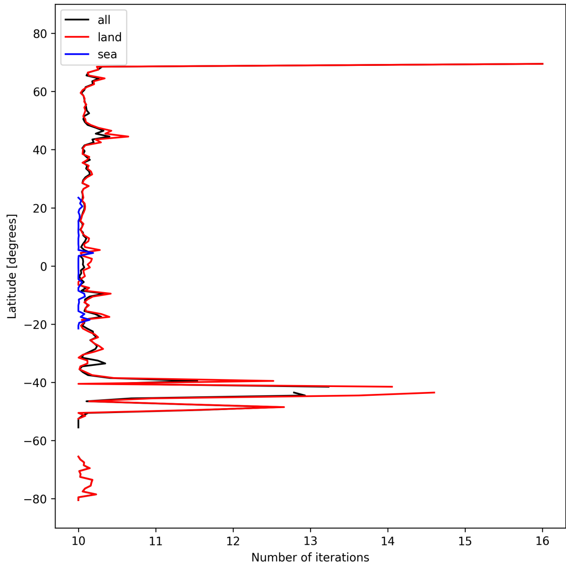
Figure 20: Zonal average of “Number of iterations” for 2025-10-07 to 2025-10-09.
