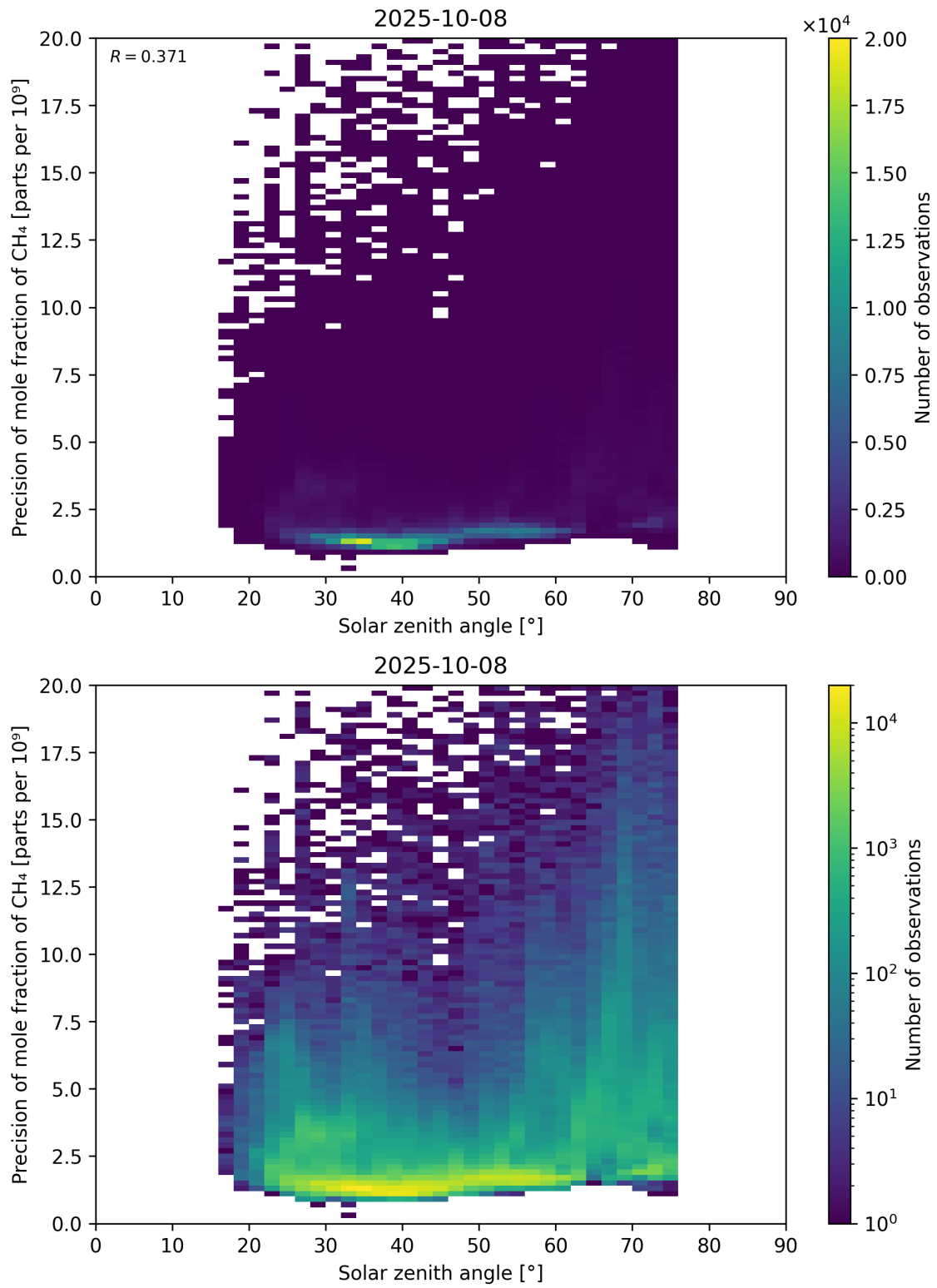
Figure 101: Scatter density plot of “Solar zenith angle” against “Precision of mole fraction of CH 4 ” for 2025-10-07 to 2025-10-09.
