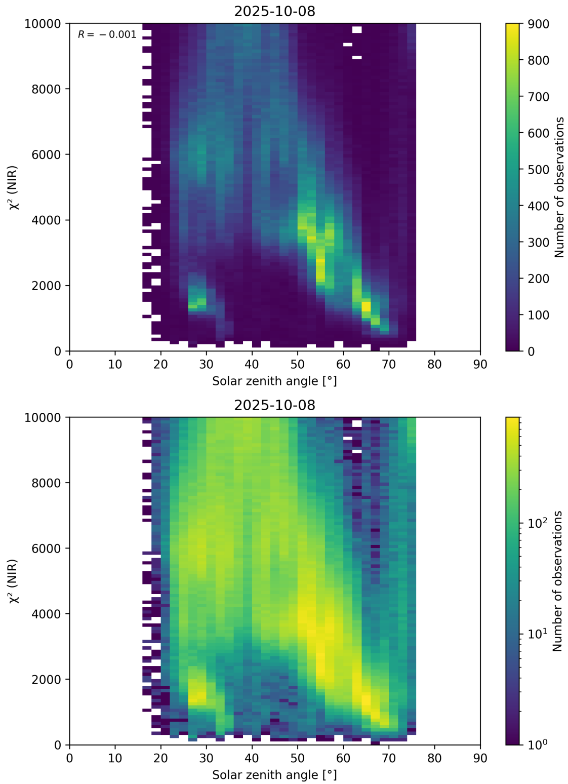
Figure 94: Scatter density plot of “Solar zenith angle” against “ \chi^2 (NIR)” for 2025-10-07 to 2025-10-09.
