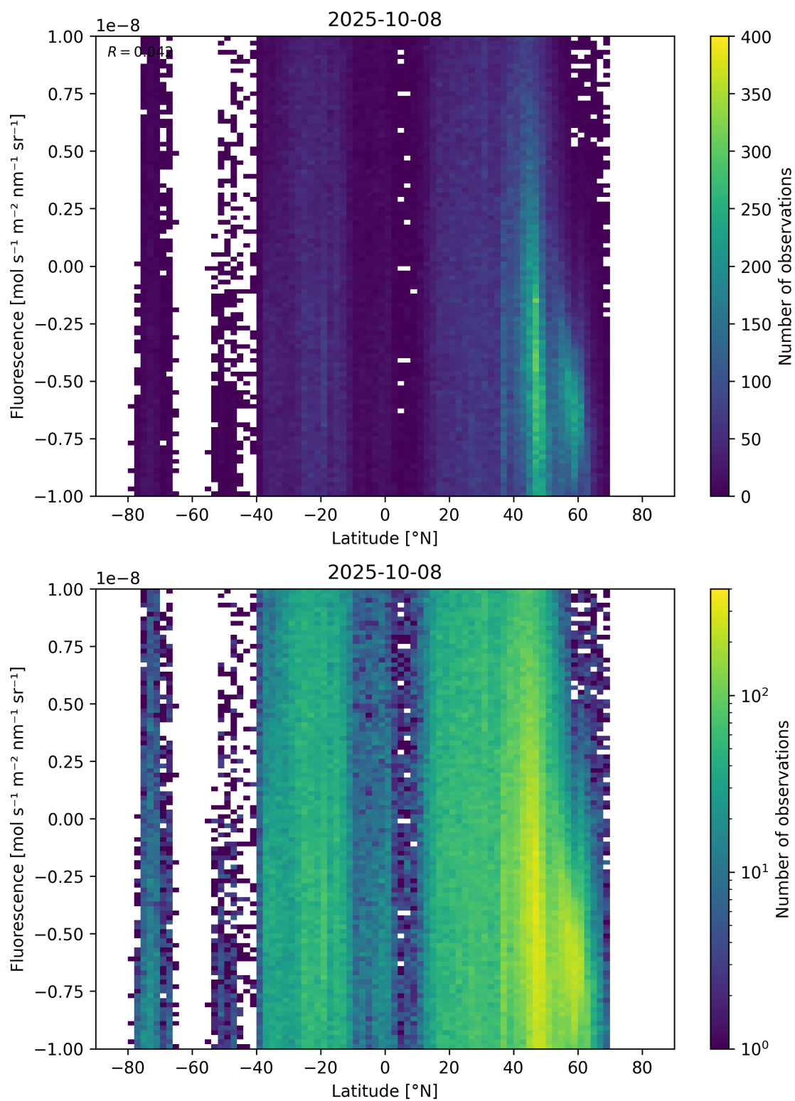
Figure 56: Scatter density plot of “Latitude” against “Fluorescence” for 2025-10-07 to 2025-10-09.
