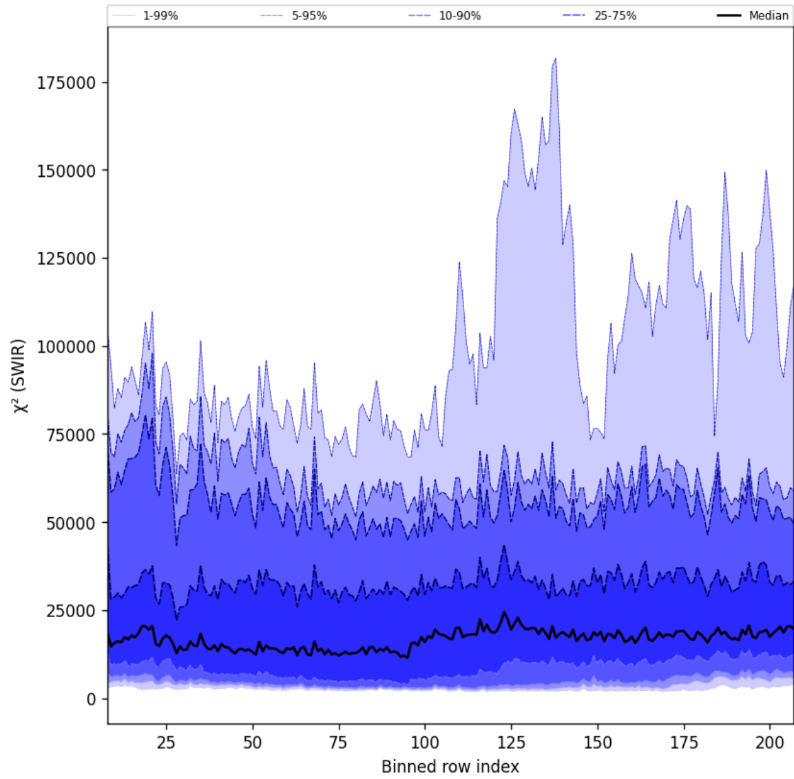
Figure 39: Along track statistics of “ \chi^2 (SWIR)” for 2025-10-07 to 2025-10-09
