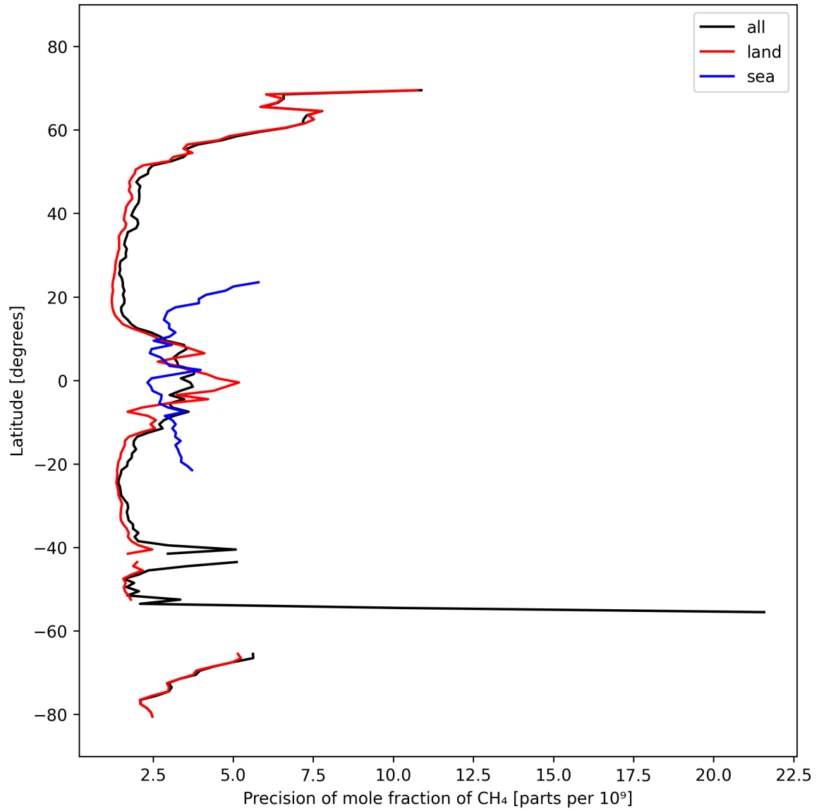
Figure 13: Zonal average of “Precision of mole fraction of CH 4 ” for 2025-10-07 to 2025-10-09.
