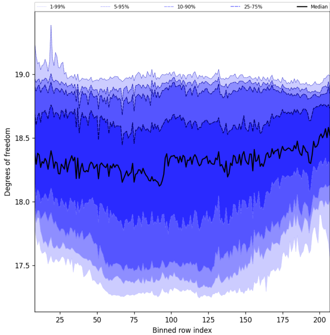
Figure 41: Along track statistics of “Degrees of freedom” for 2025-10-08 to 2025-10-10
