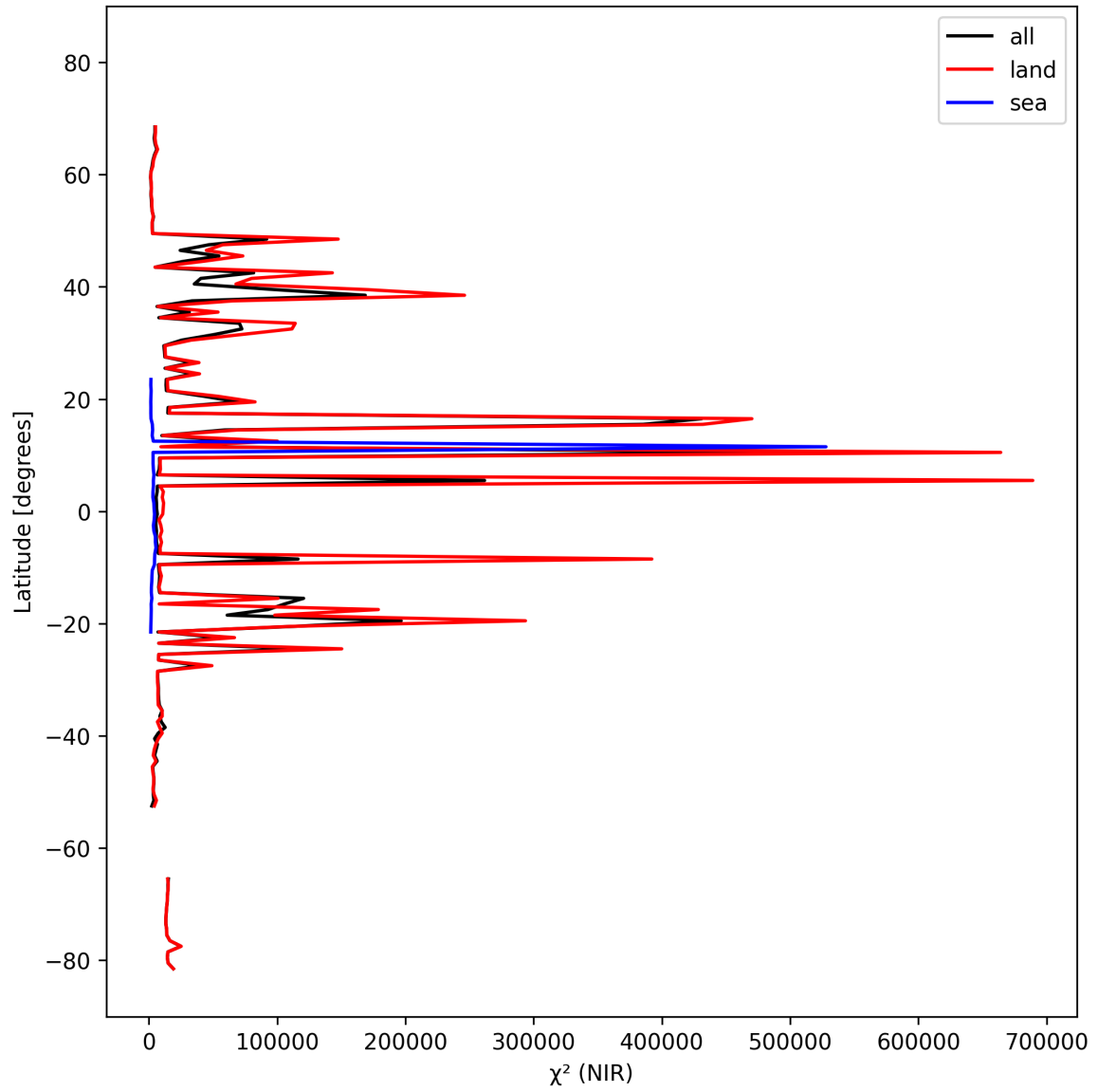
Figure 18: Zonal average of “ \chi^2 (NIR)” for 2025-10-08 to 2025-10-10.
