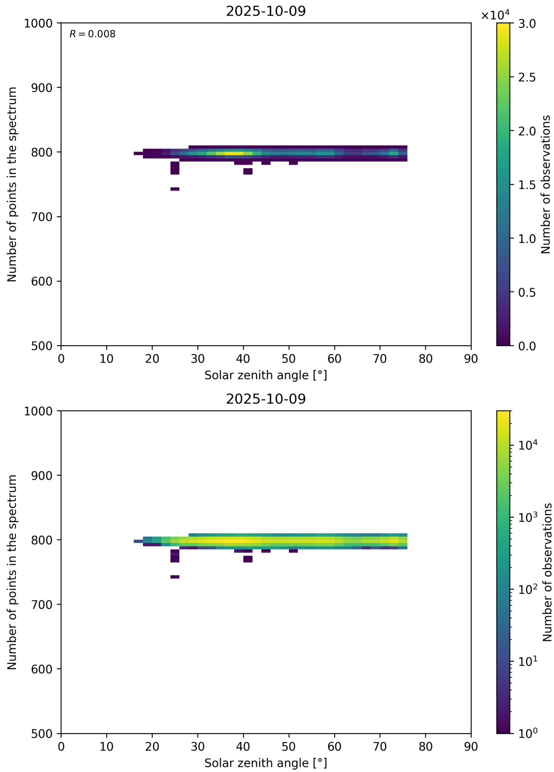
Figure 103: Scatter density plot of “Solar zenith angle” against “Number of points in the spectrum” for 2025-10-08 to 2025-10-10.
