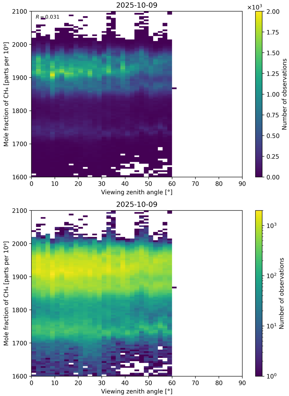
Figure 110: Scatter density plot of “Viewing zenith angle” against “Mole fraction of CH 4 ” for 2025-10-08 to 2025-10-10.
