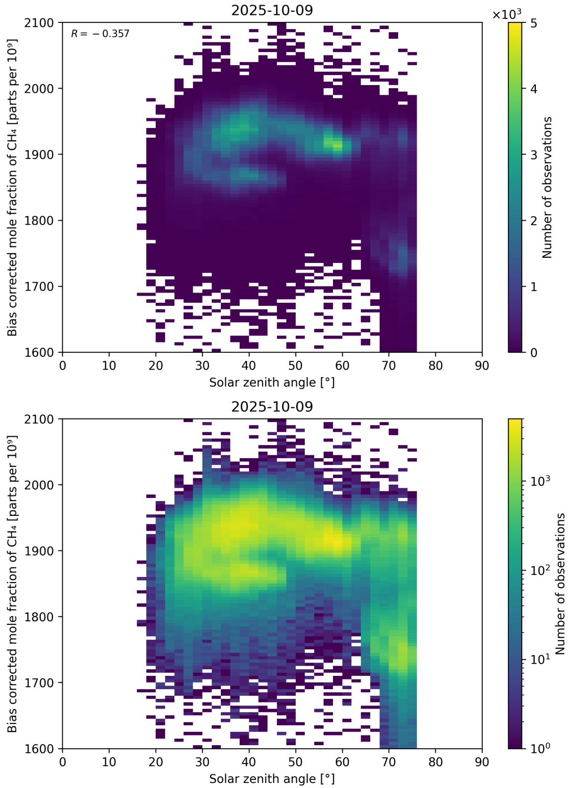
Figure 100: Scatter density plot of “Solar zenith angle” against “Bias corrected mole fraction of CH 4 ” for 2025-10-08 to 2025-10-10.
