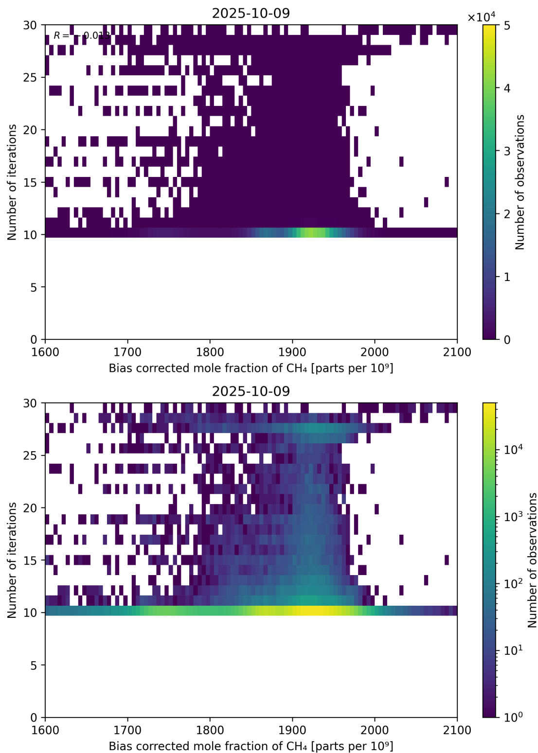
Figure 67: Scatter density plot of “Bias corrected mole fraction of CH 4 ” against “Number of iterations” for 2025-10-08 to 2025-10-10.
