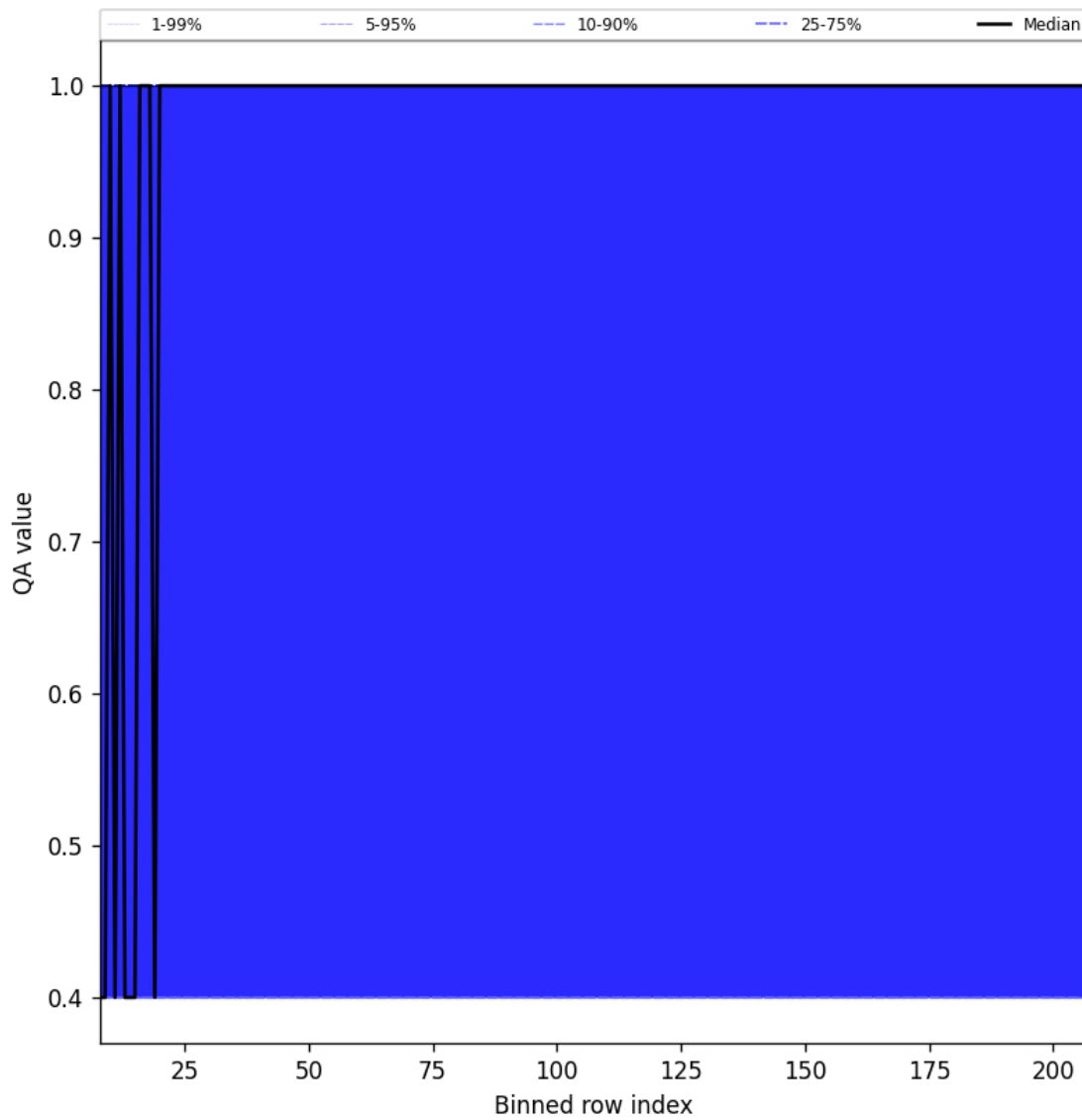
Figure 33: Along track statistics of “QA value” for 2025-10-08 to 2025-10-10
