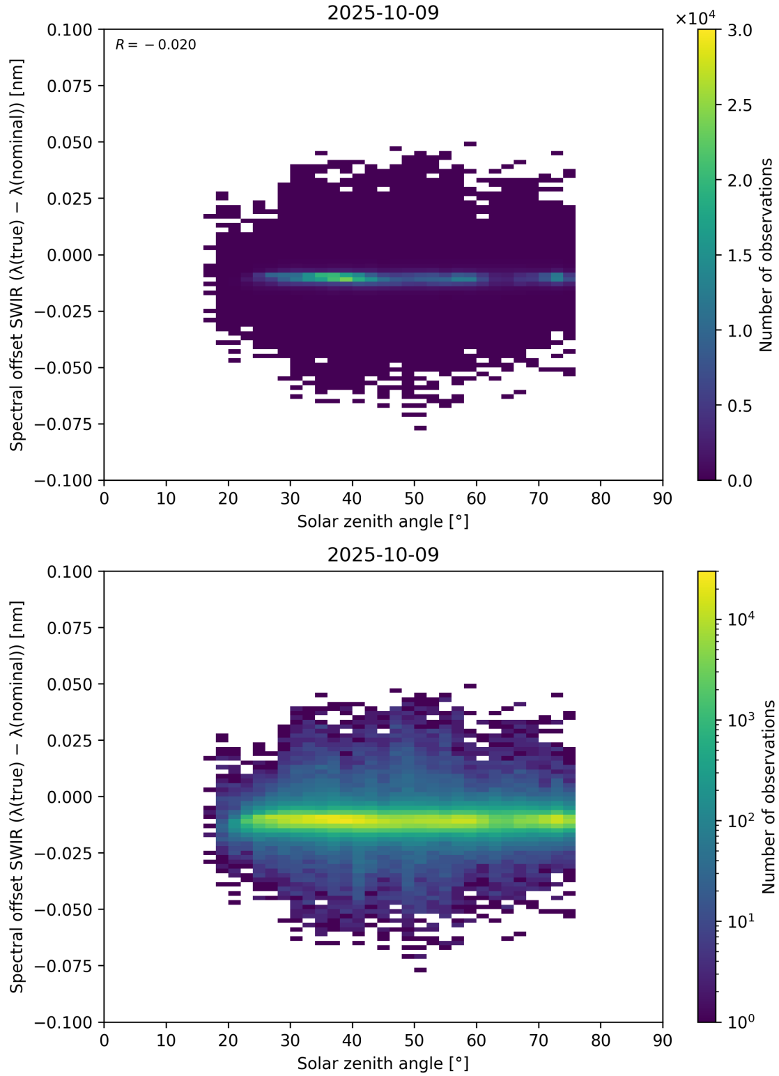
Figure 104: Scatter density plot of “Solar zenith angle” against “Spectral offset SWIR ( \lambda_{\text{true}} - \lambda_{\text{nominal}} )” for 2025-10-08 to 2025-10-10.
