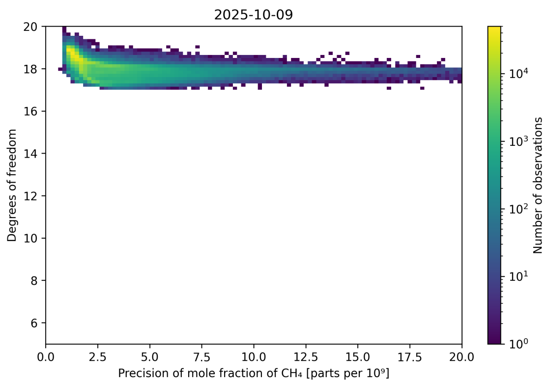
Figure 80: Scatter density plot of “Precision of mole fraction of CH 4 ” against “Degrees of freedom” for 2025-10-08 to 2025-10-10.
