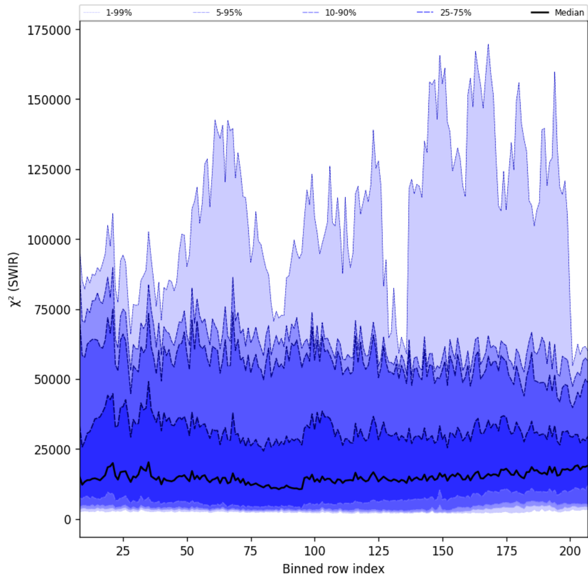
Figure 39: Along track statistics of “ \chi^2 (SWIR)” for 2025-10-08 to 2025-10-10
