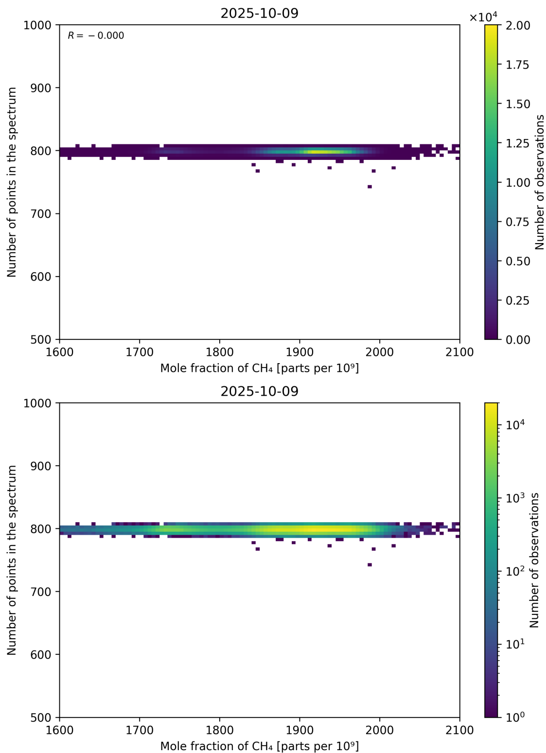
Figure 77: Scatter density plot of “Mole fraction of CH 4 ” against “Number of points in the spectrum” for 2025-10-08 to 2025-10-10.
