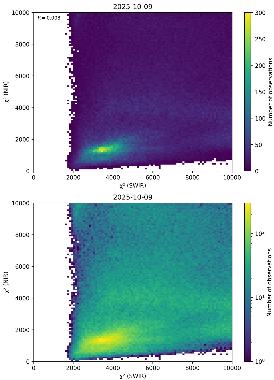
Figure 47: Scatter density plot of “ \chi^2 (SWIR)” against “ \chi^2 (NIR)” for 2025-10-08 to 2025-10-10.
