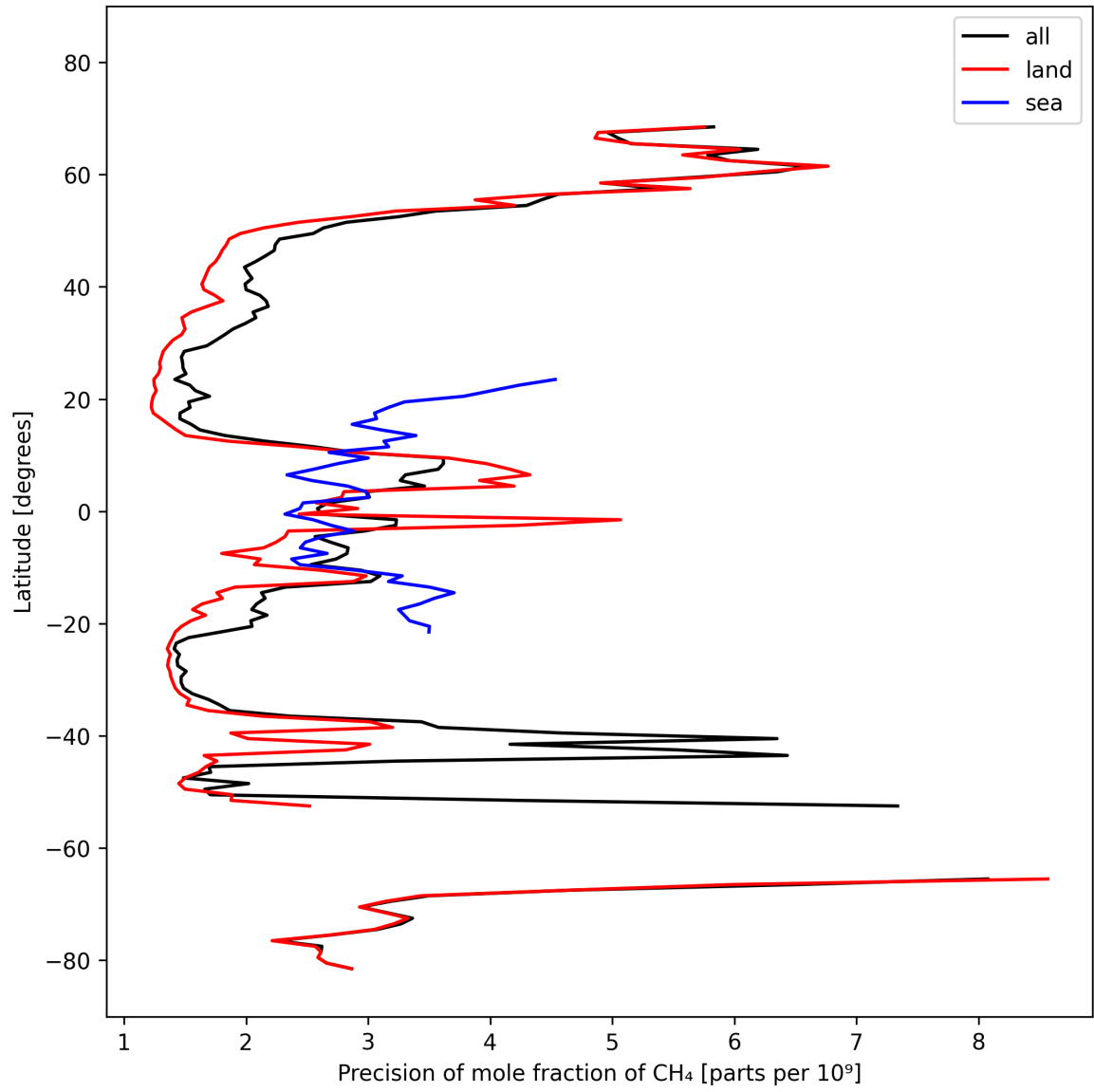
Figure 13: Zonal average of “Precision of mole fraction of CH 4 ” for 2025-10-08 to 2025-10-10.
