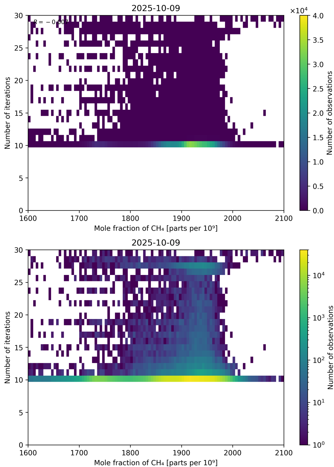
Figure 76: Scatter density plot of “Mole fraction of CH 4 ” against “Number of iterations” for 2025-10-08 to 2025-10-10.
