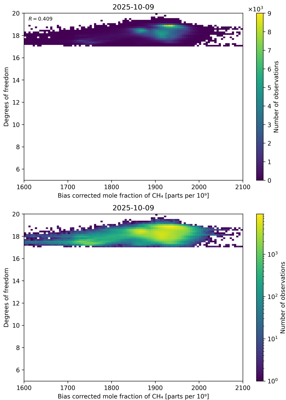
Figure 65: Scatter density plot of “Bias corrected mole fraction of CH 4 ” against “Degrees of freedom” for 2025-10-08 to 2025-10-10.
