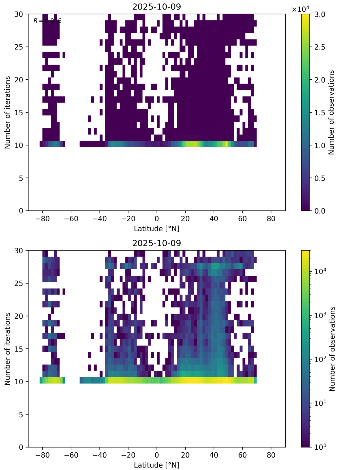
Figure 60: Scatter density plot of “Latitude” against “Number of iterations” for 2025-10-08 to 2025-10-10.
