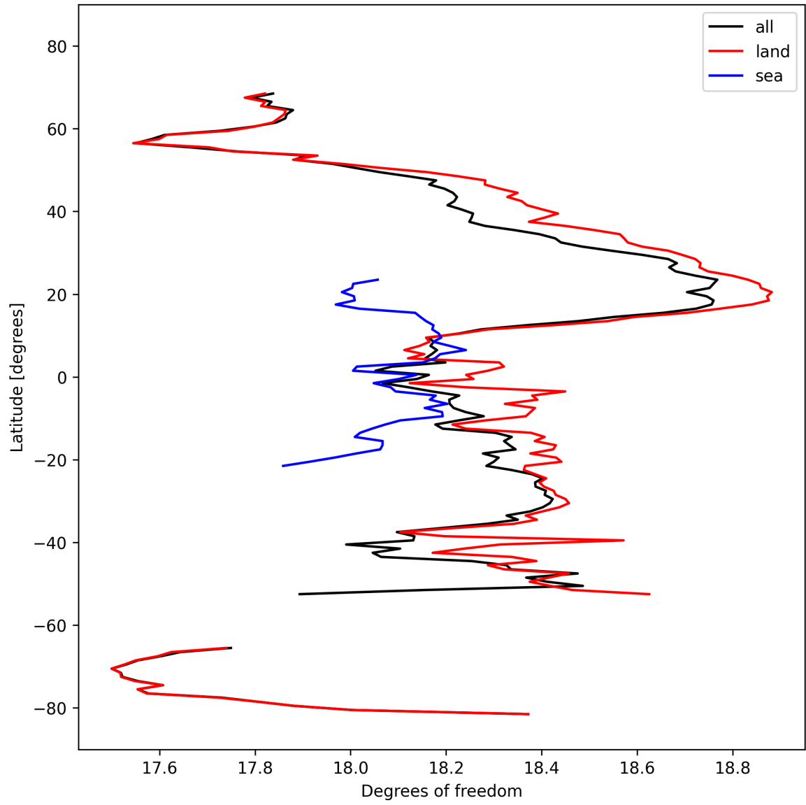
Figure 19: Zonal average of “Degrees of freedom” for 2025-10-08 to 2025-10-10.
