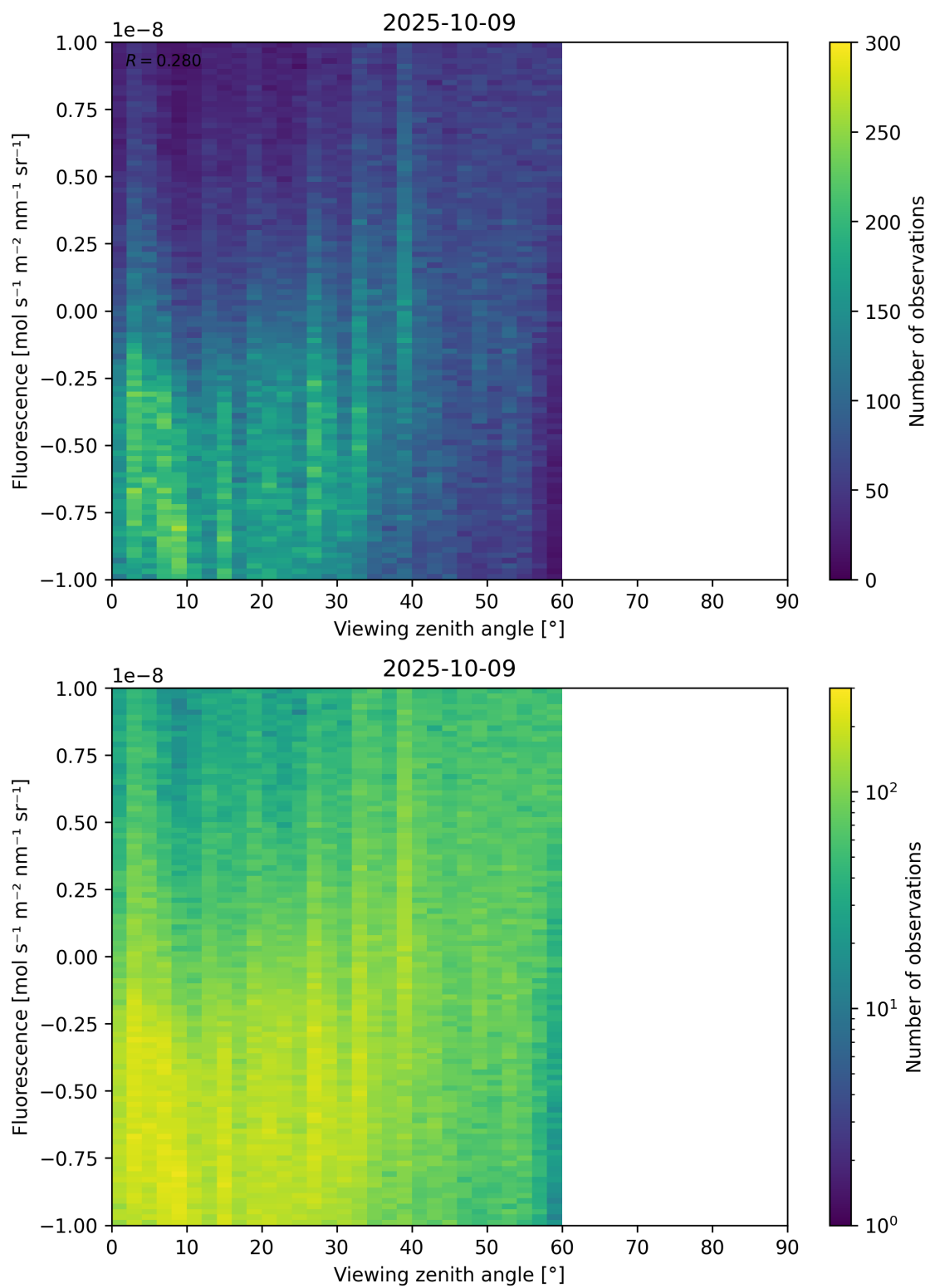
Figure 108: Scatter density plot of “Viewing zenith angle” against “Fluorescence” for 2025-10-08 to 2025-10-10.
