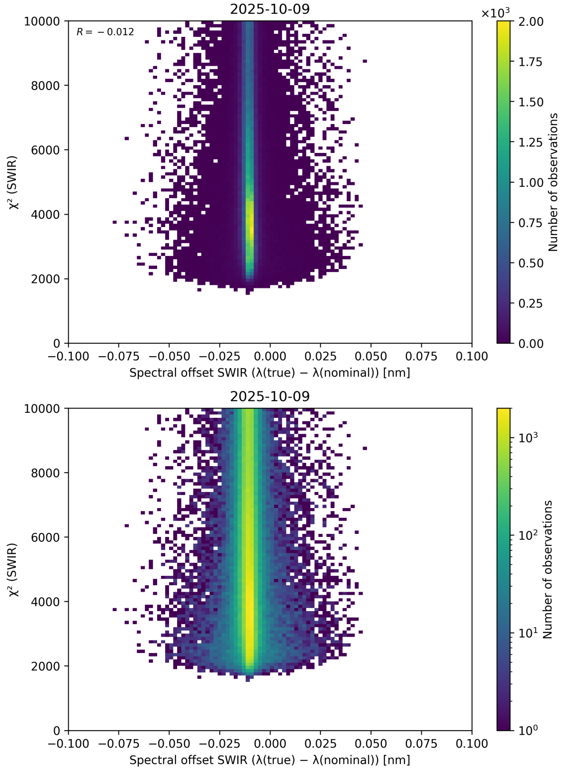
Figure 118: Scatter density plot of “Spectral offset SWIR ( \lambda_{\text{true}} - \lambda_{\text{nominal}} )” against “ \chi^2 (SWIR)” for 2025-10-08 to 2025-10-10.
