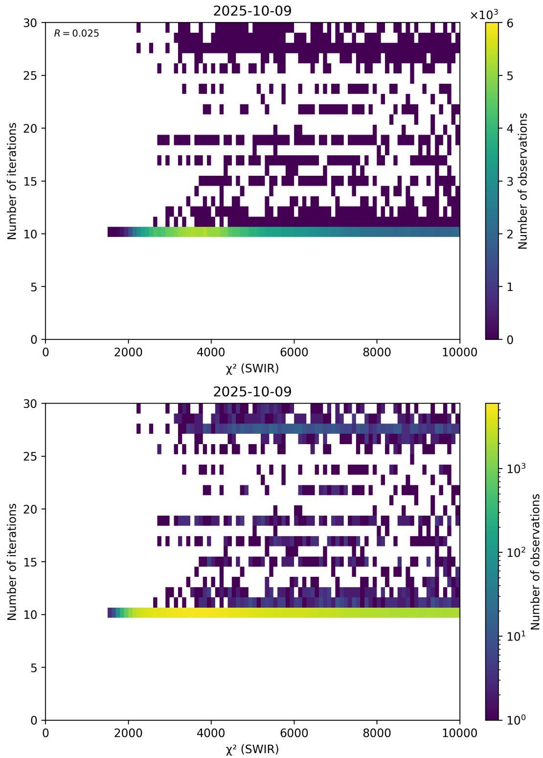
Figure 50: Scatter density plot of “ \chi^2 (SWIR)” against “Number of iterations” for 2025-10-08 to 2025-10-10.
