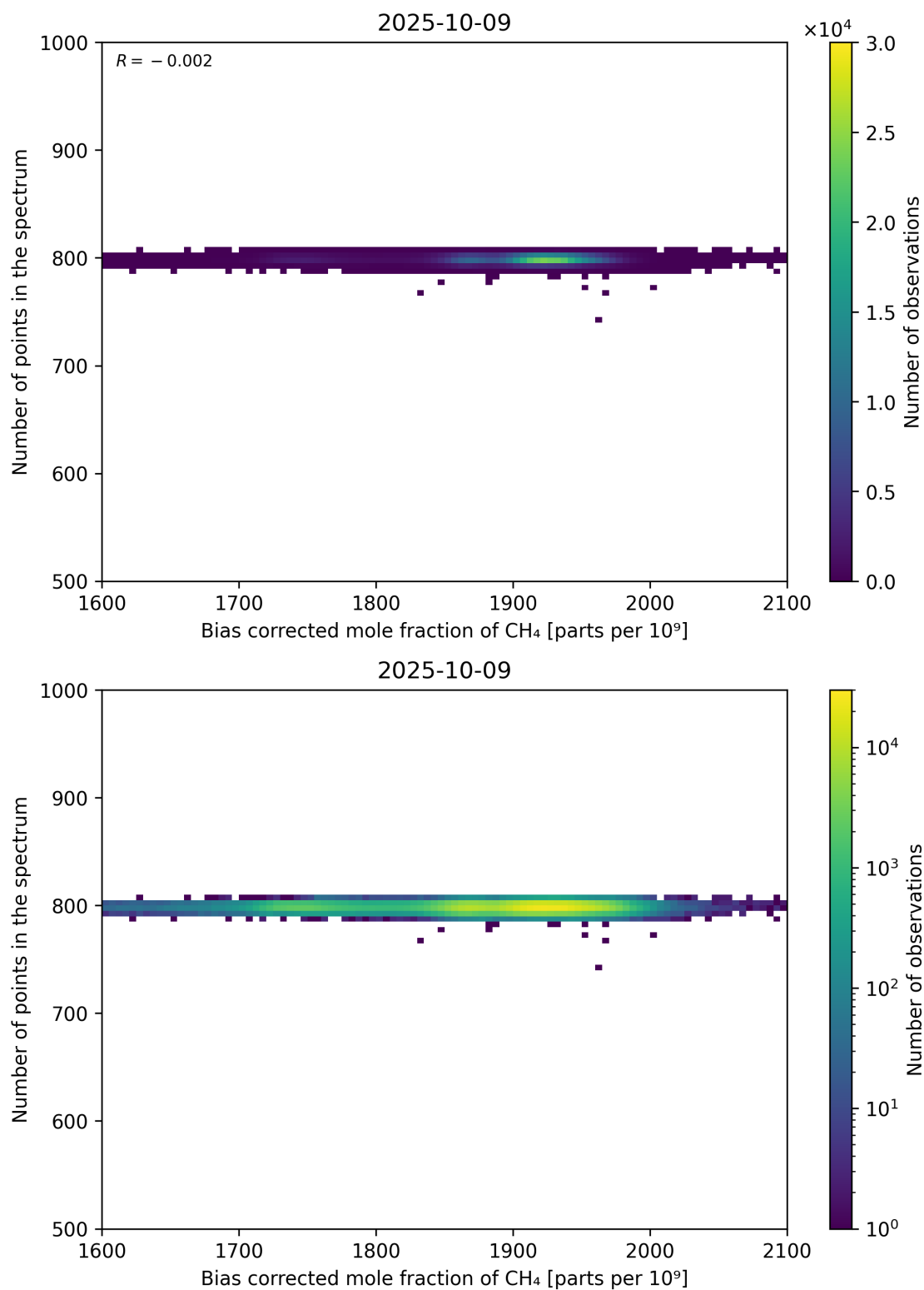
Figure 68: Scatter density plot of “Bias corrected mole fraction of CH 4 ” against “Number of points in the spectrum” for 2025-10-08 to 2025-10-10.
