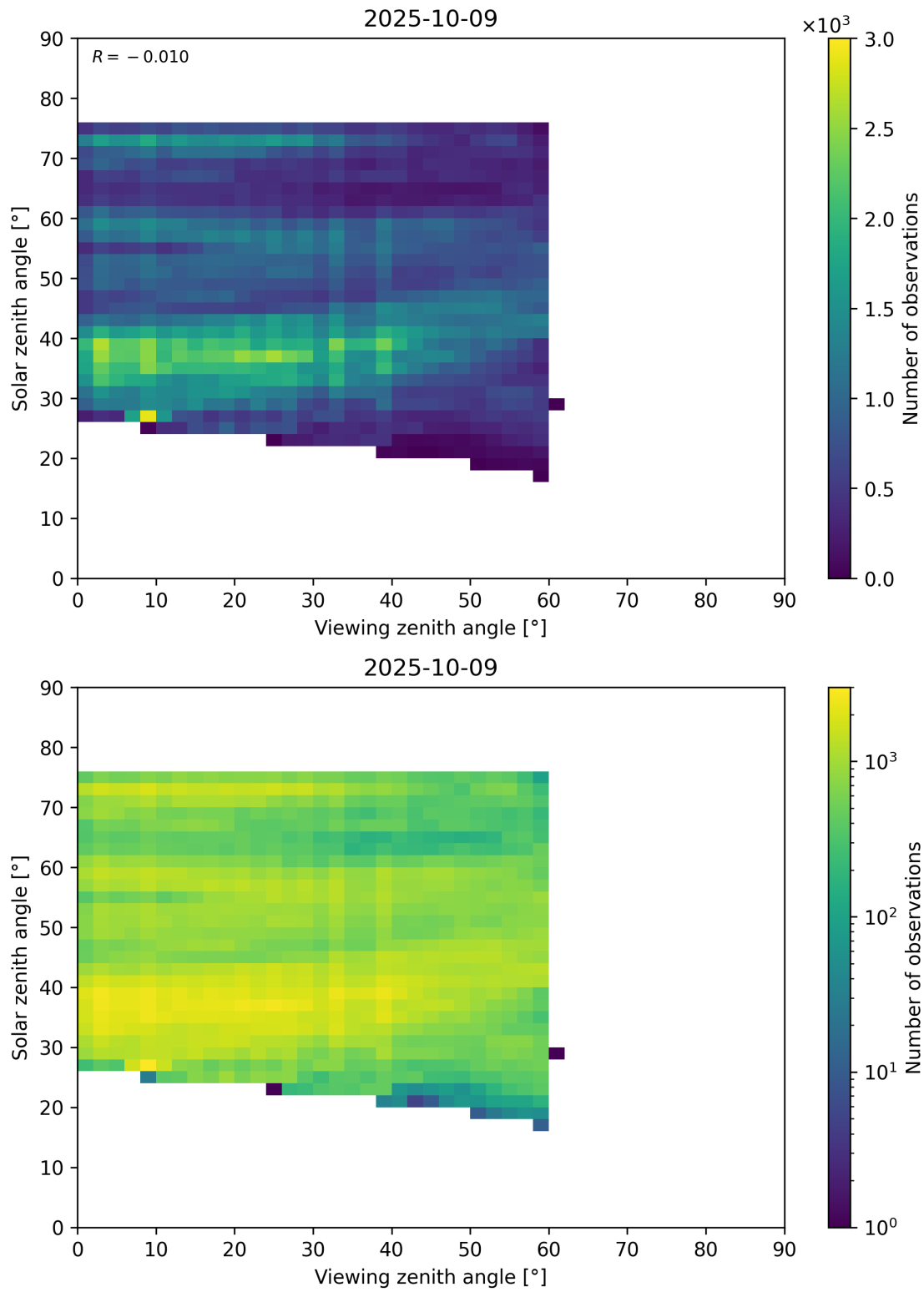
Figure 115: Scatter density plot of “Viewing zenith angle” against “Solar zenith angle” for 2025-10-08 to 2025-10-10.
