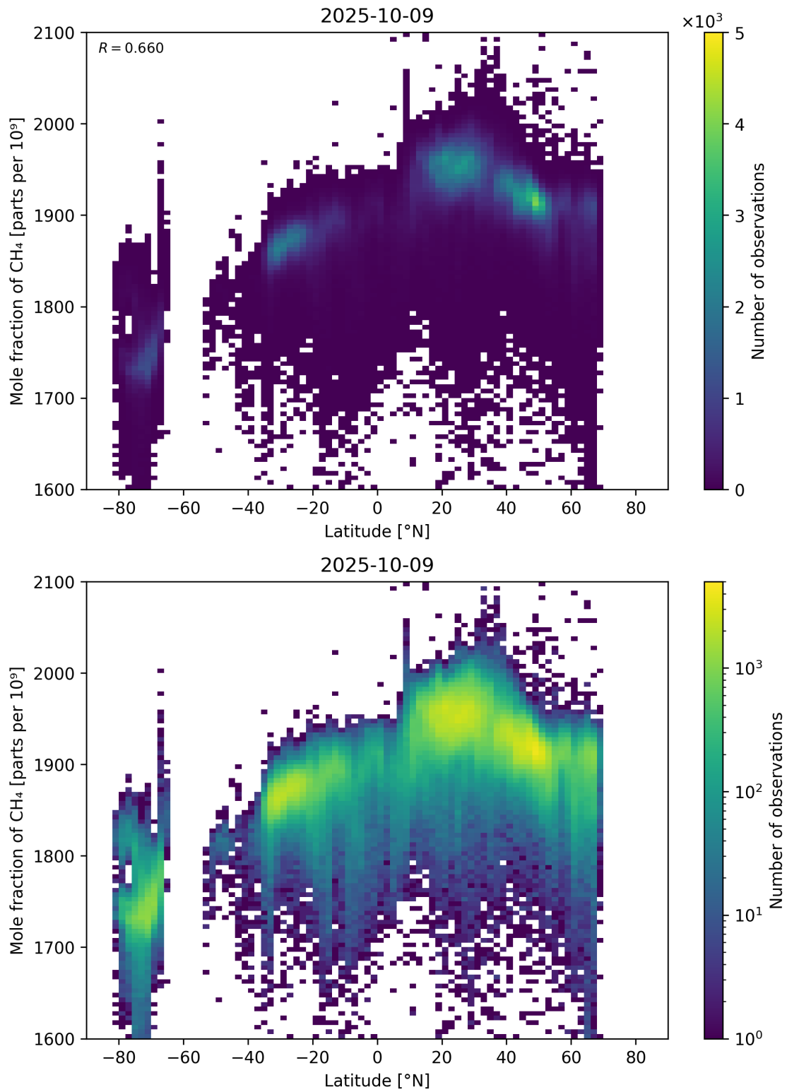
Figure 57: Scatter density plot of “Latitude” against “Mole fraction of CH 4 ” for 2025-10-08 to 2025-10-10.
