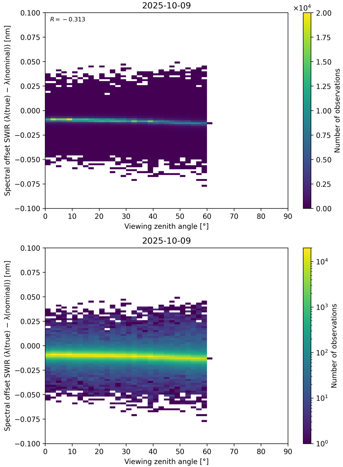
Figure 116: Scatter density plot of “Viewing zenith angle” against “Spectral offset SWIR ( \lambda_{\text{true}} - \lambda_{\text{nominal}} )” for 2025-10-08 to 2025-10-10.
