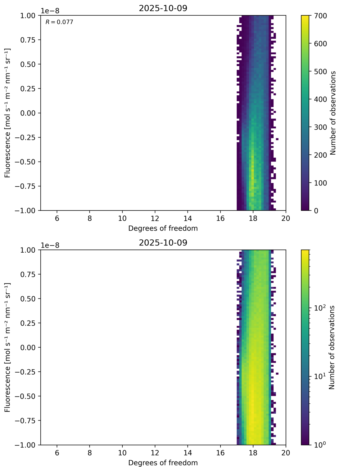
Figure 51: Scatter density plot of “Degrees of freedom” against “Fluorescence” for 2025-10-08 to 2025-10-10.
