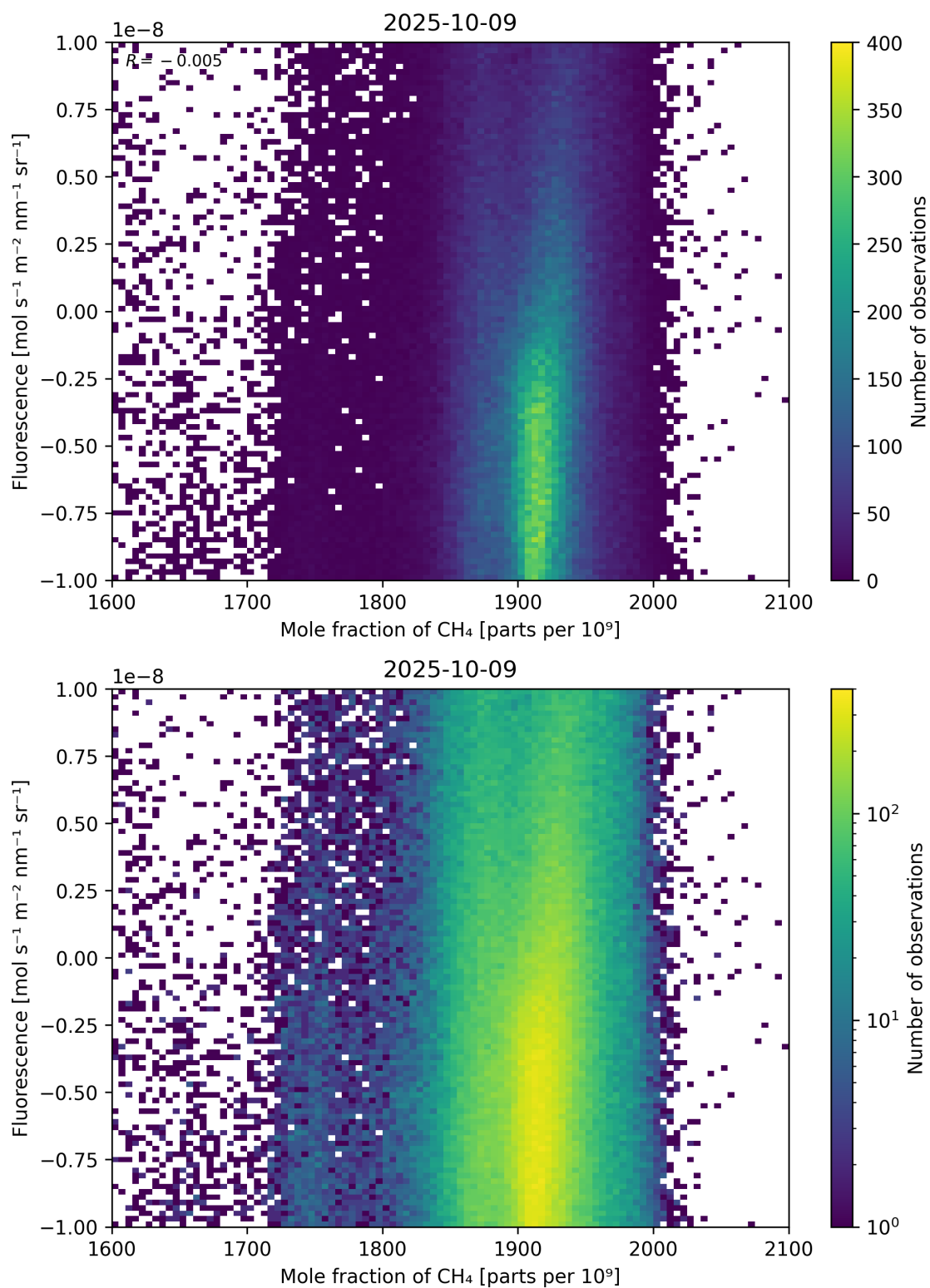
Figure 73: Scatter density plot of “Mole fraction of \text{CH}_4 ” against “Fluorescence” for 2025-10-08 to 2025-10-10.
