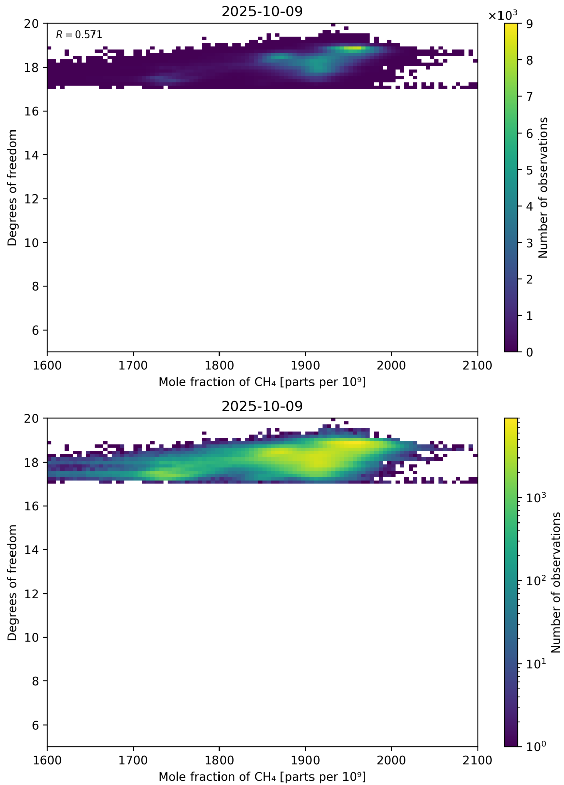
Figure 72: Scatter density plot of “Mole fraction of CH 4 ” against “Degrees of freedom” for 2025-10-08 to 2025-10-10.
