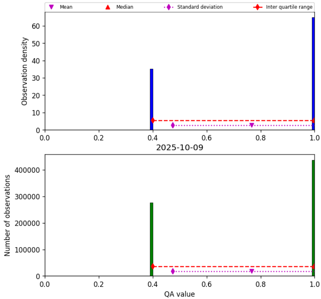
Figure 22: Histogram of “QA value” for 2025-10-08 to 2025-10-10
