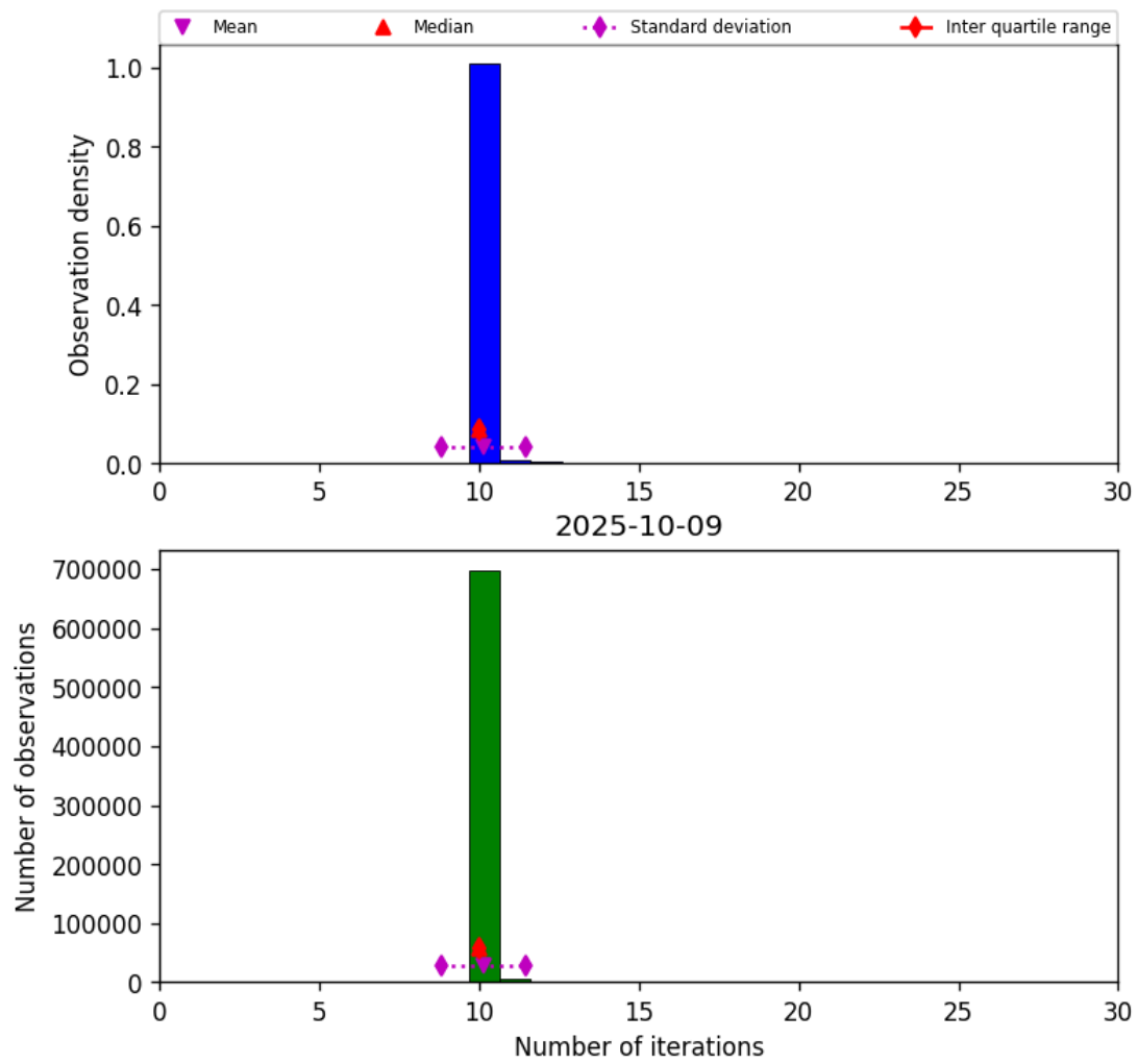
Figure 31: Histogram of “Number of iterations” for 2025-10-08 to 2025-10-10
