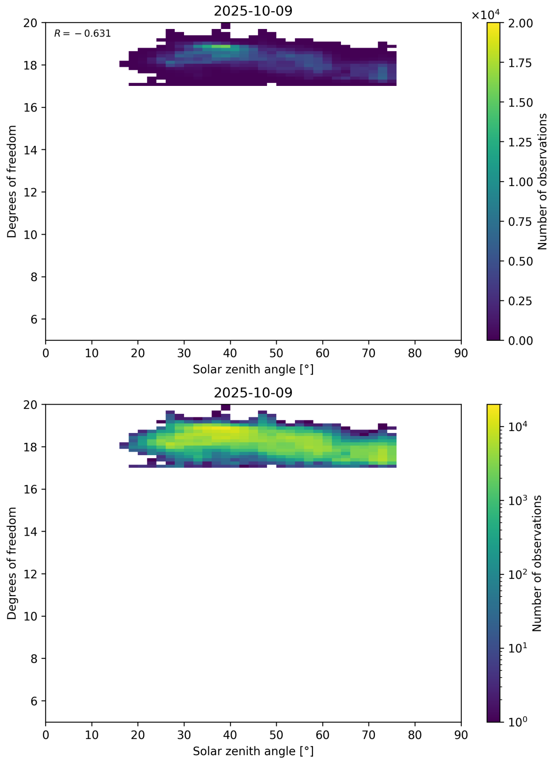
Figure 96: Scatter density plot of “Solar zenith angle” against “Degrees of freedom” for 2025-10-08 to 2025-10-10.
