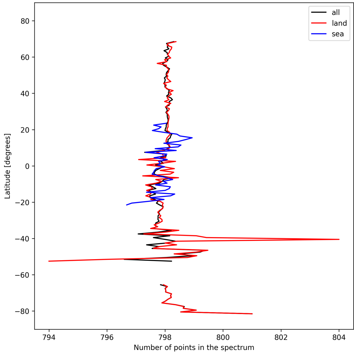
Figure 15: Zonal average of “Number of points in the spectrum” for 2025-10-08 to 2025-10-10.
