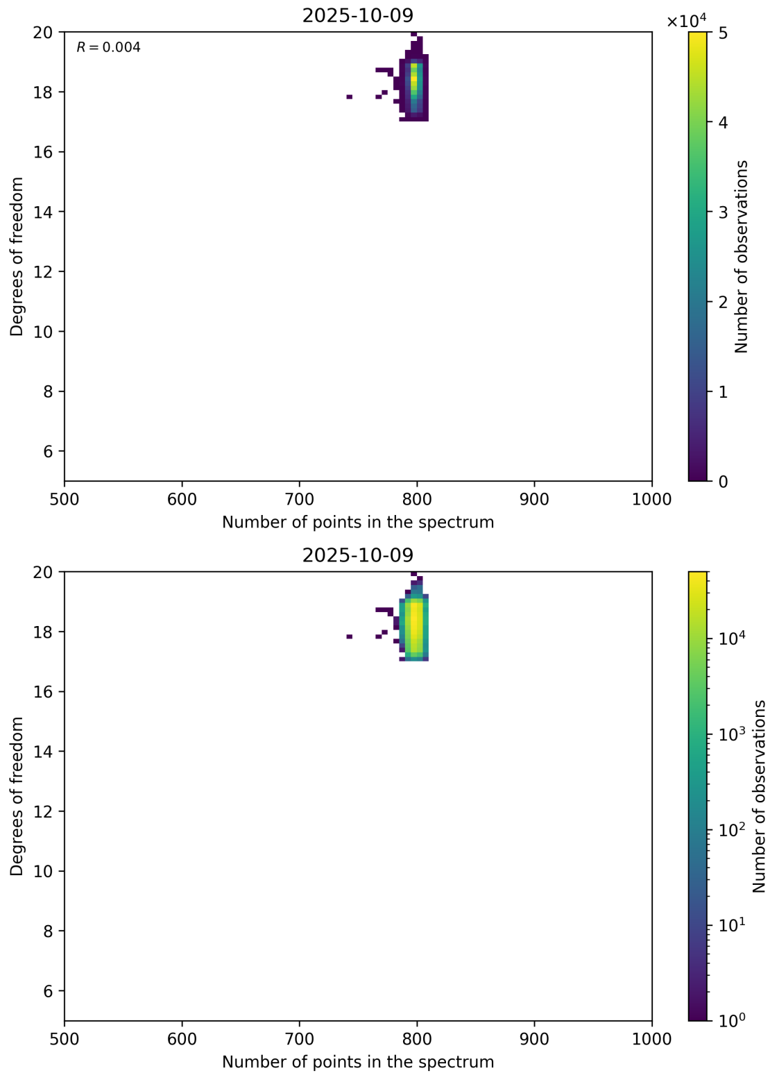
Figure 90: Scatter density plot of “Number of points in the spectrum” against “Degrees of freedom” for 2025-10-08 to 2025-10-10.
