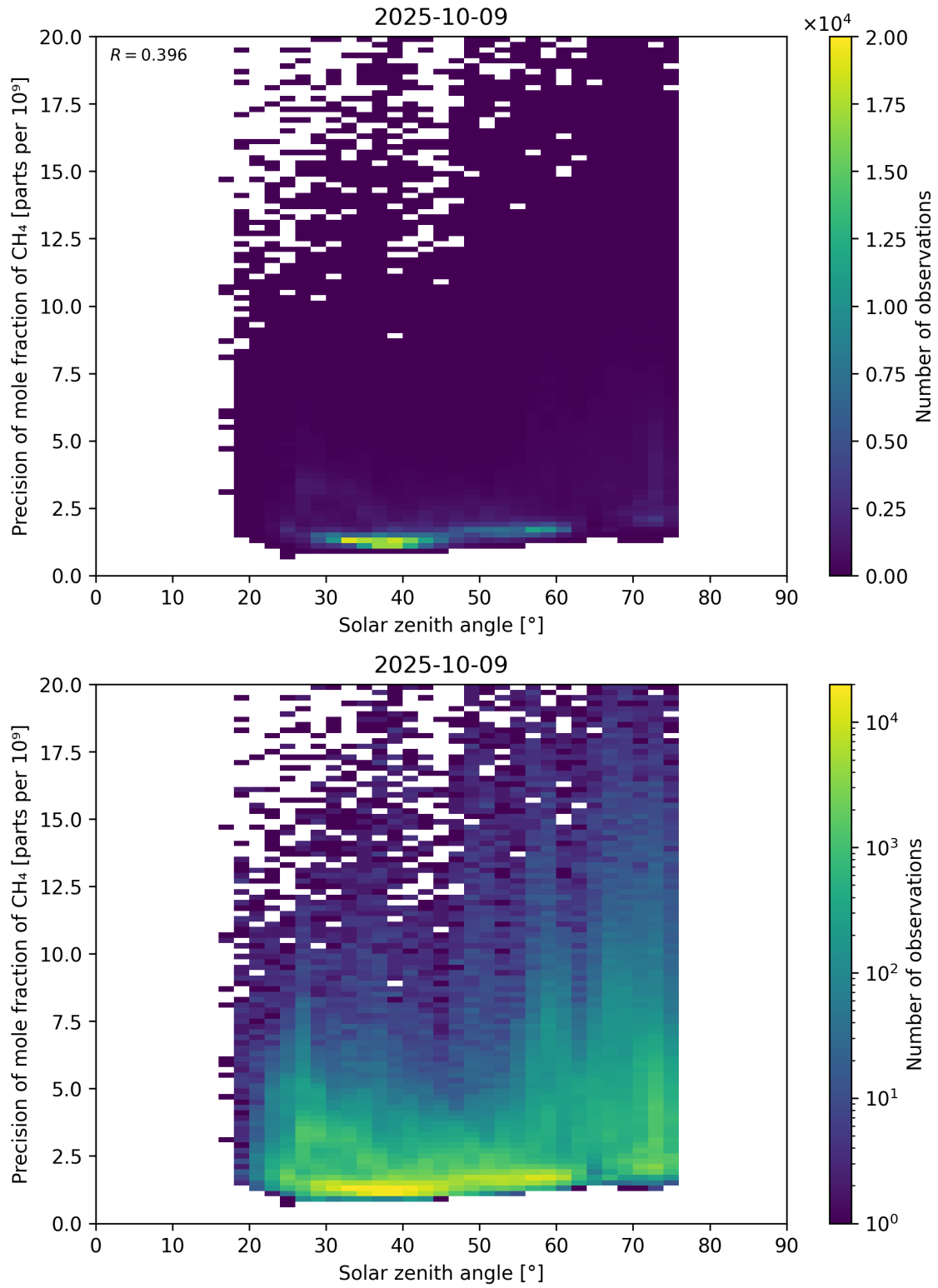
Figure 101: Scatter density plot of “Solar zenith angle” against “Precision of mole fraction of CH 4 ” for 2025-10-08 to 2025-10-10.
