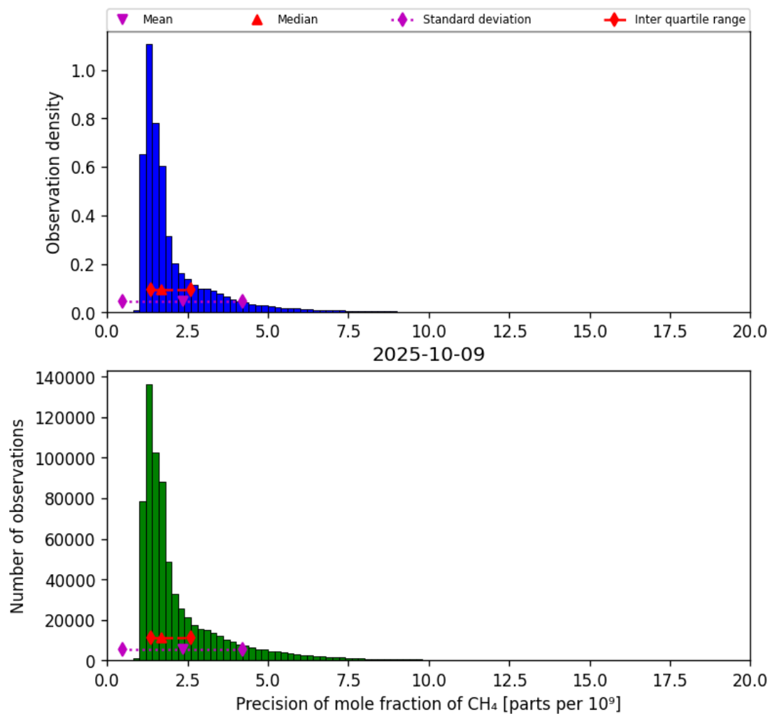
Figure 24: Histogram of “Precision of mole fraction of CH 4 ” for 2025-10-08 to 2025-10-10
