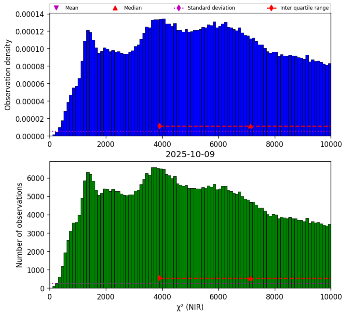
Figure 29: Histogram of “ \chi^2 (NIR)” for 2025-10-08 to 2025-10-10
