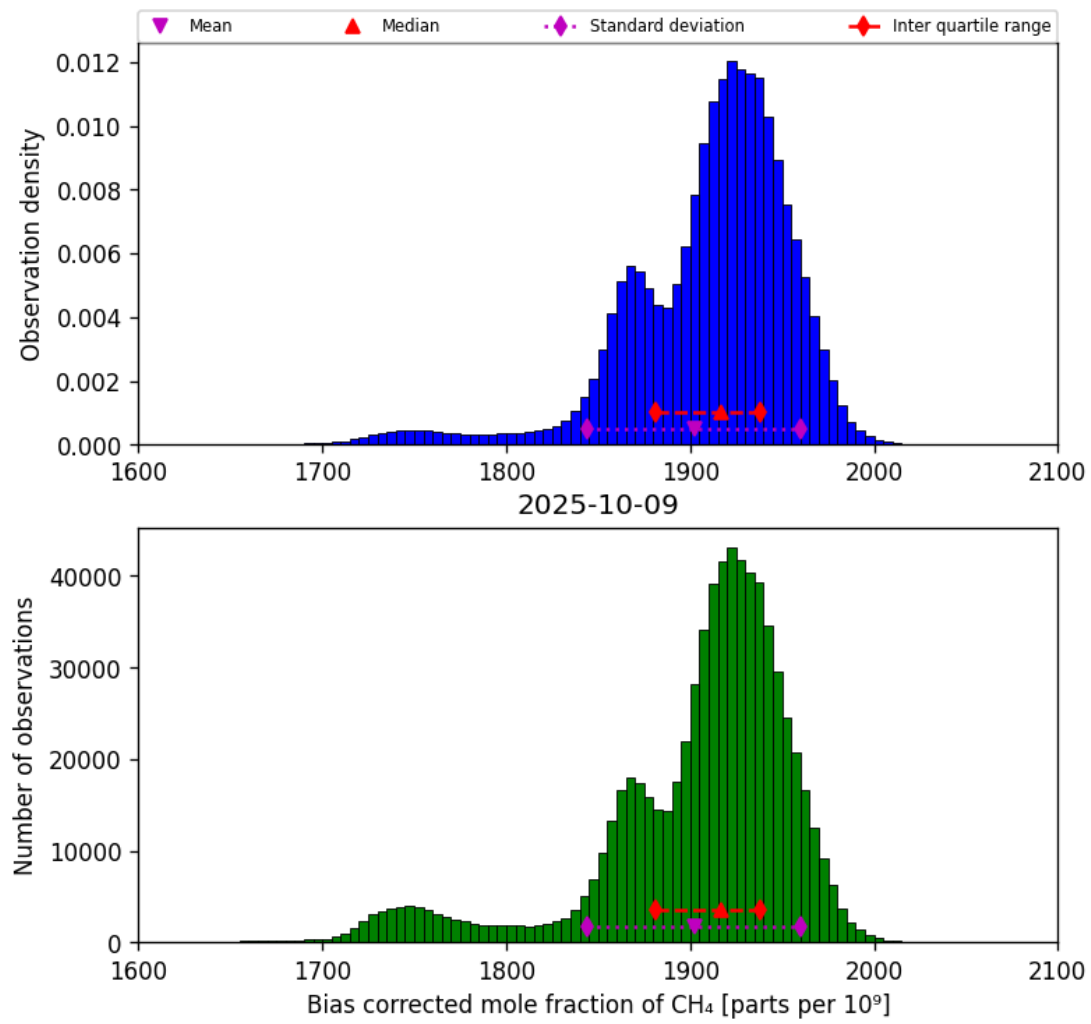
Figure 25: Histogram of “Bias corrected mole fraction of CH 4 ” for 2025-10-08 to 2025-10-10
