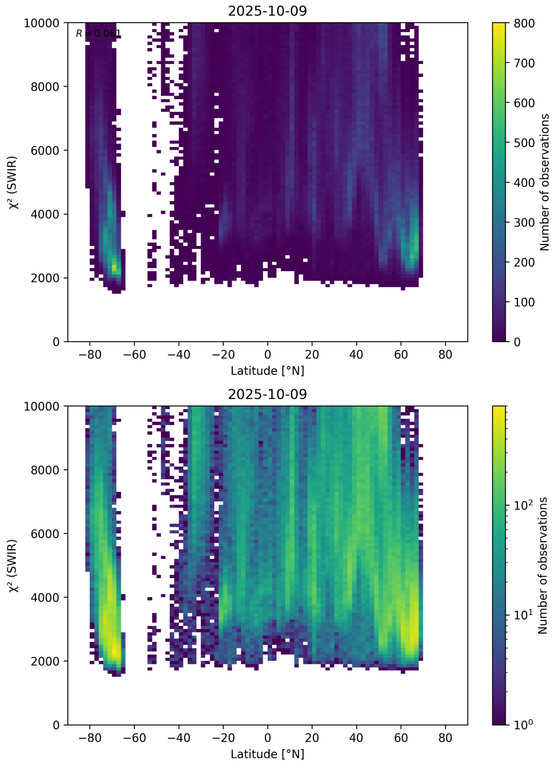
Figure 54: Scatter density plot of “Latitude” against “ \chi^2 (SWIR)” for 2025-10-08 to 2025-10-10.
