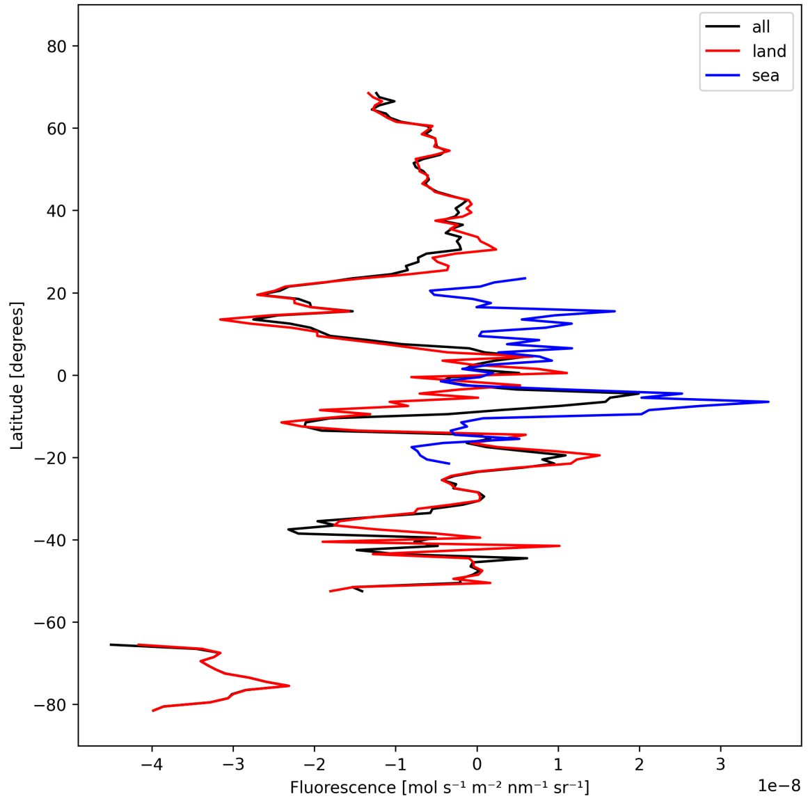
Figure 21: Zonal average of “Fluorescence” for 2025-10-08 to 2025-10-10.
