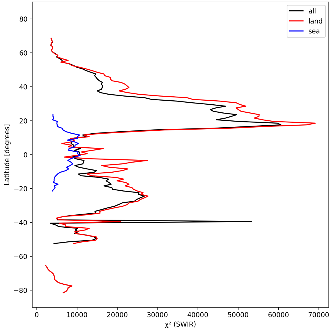
Figure 17: Zonal average of “ \chi^2 (SWIR)” for 2025-10-08 to 2025-10-10.
