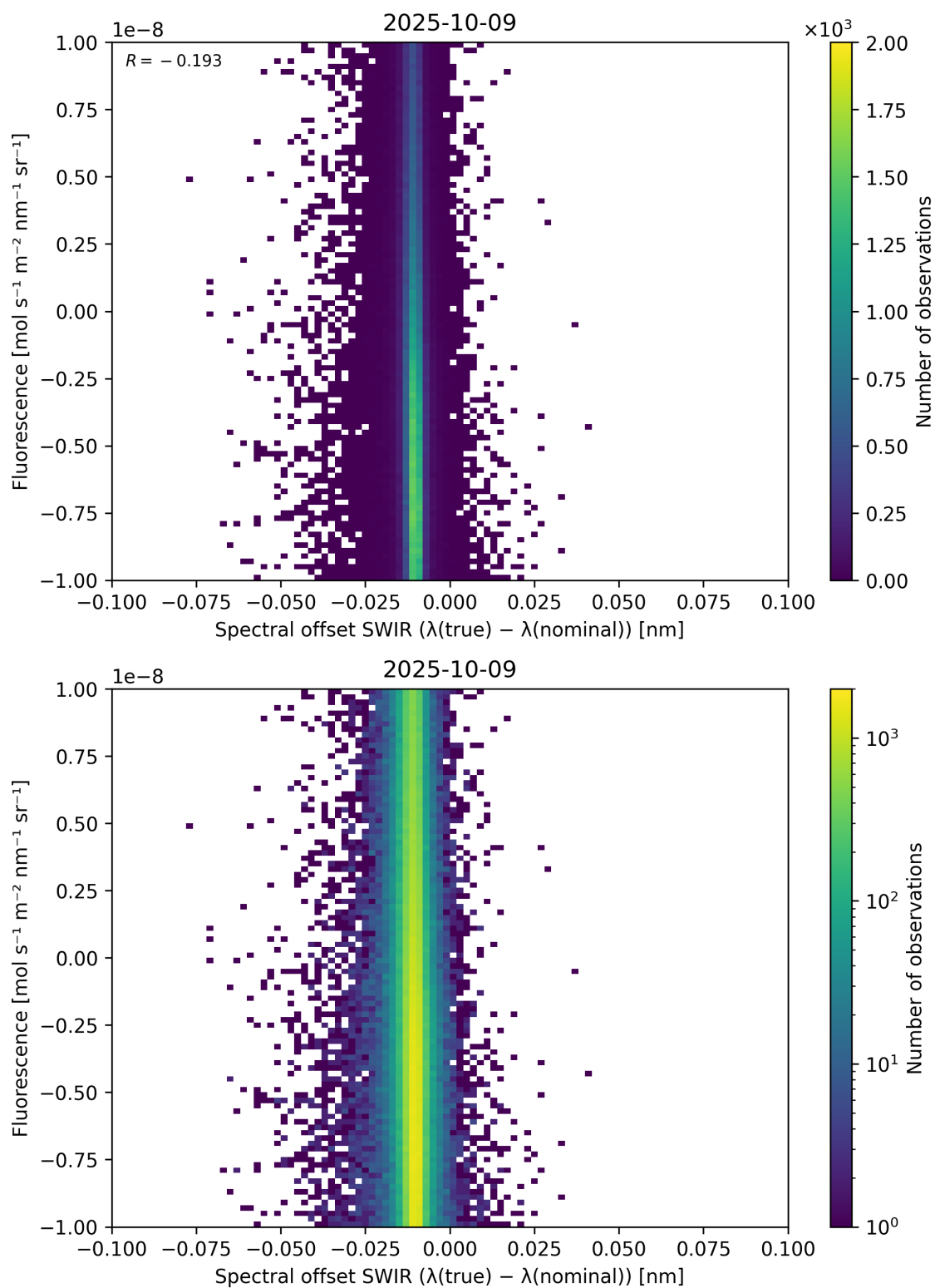
Figure 120: Scatter density plot of “Spectral offset SWIR ( \lambda_{\text{true}} - \lambda_{\text{nominal}} )” against “Fluorescence” for 2025-10-08 to 2025-10-10.
