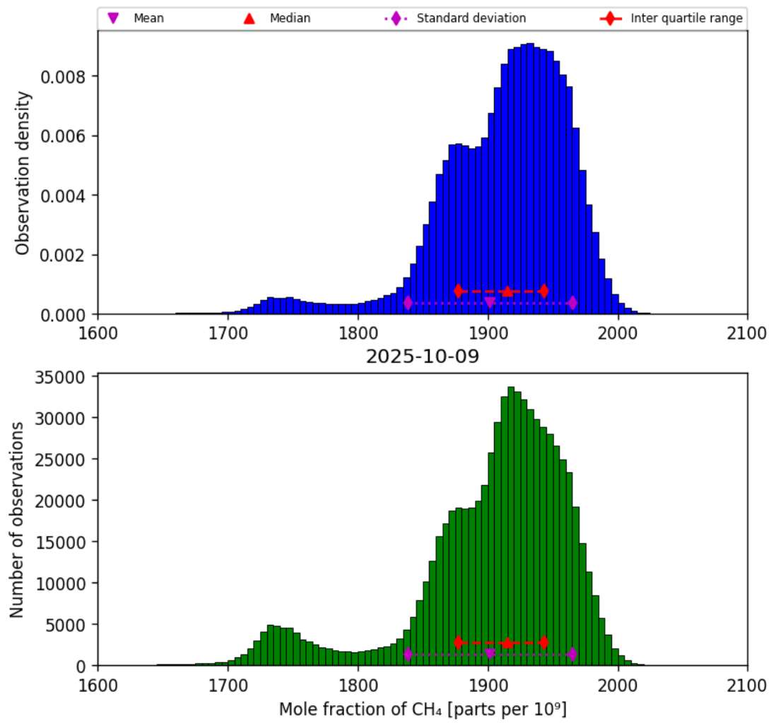
Figure 23: Histogram of “Mole fraction of CH 4 ” for 2025-10-08 to 2025-10-10
