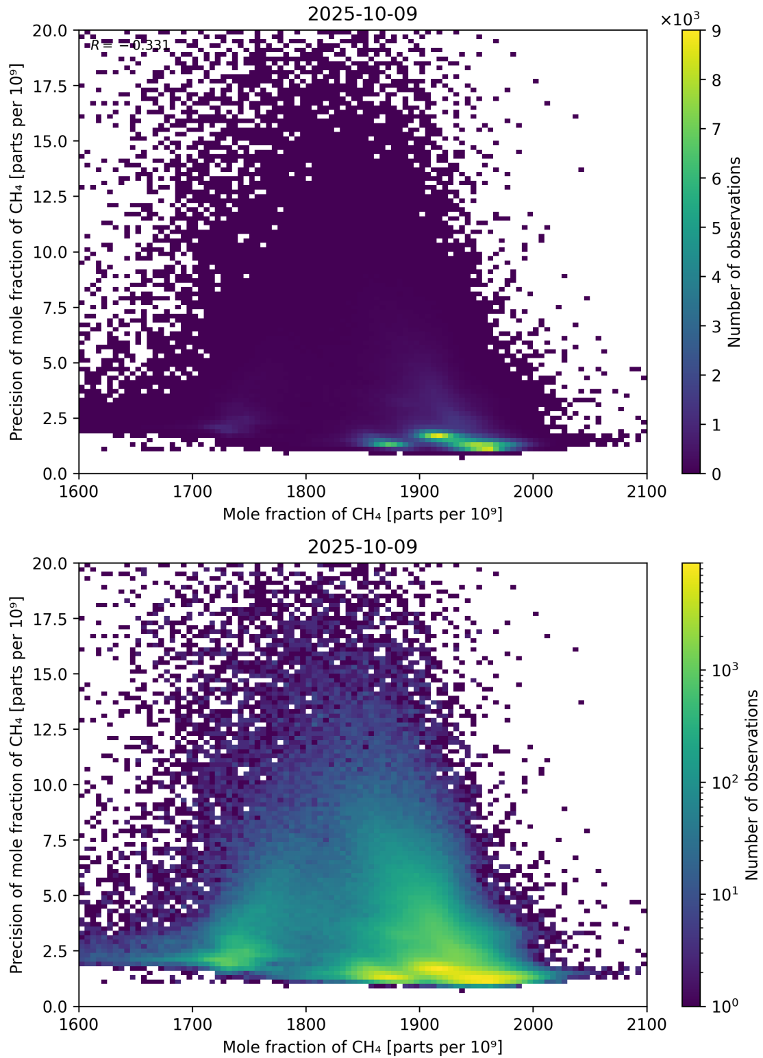
Figure 75: Scatter density plot of “Mole fraction of CH 4 ” against “Precision of mole fraction of CH 4 ” for 2025-10-08 to 2025-10-10.
