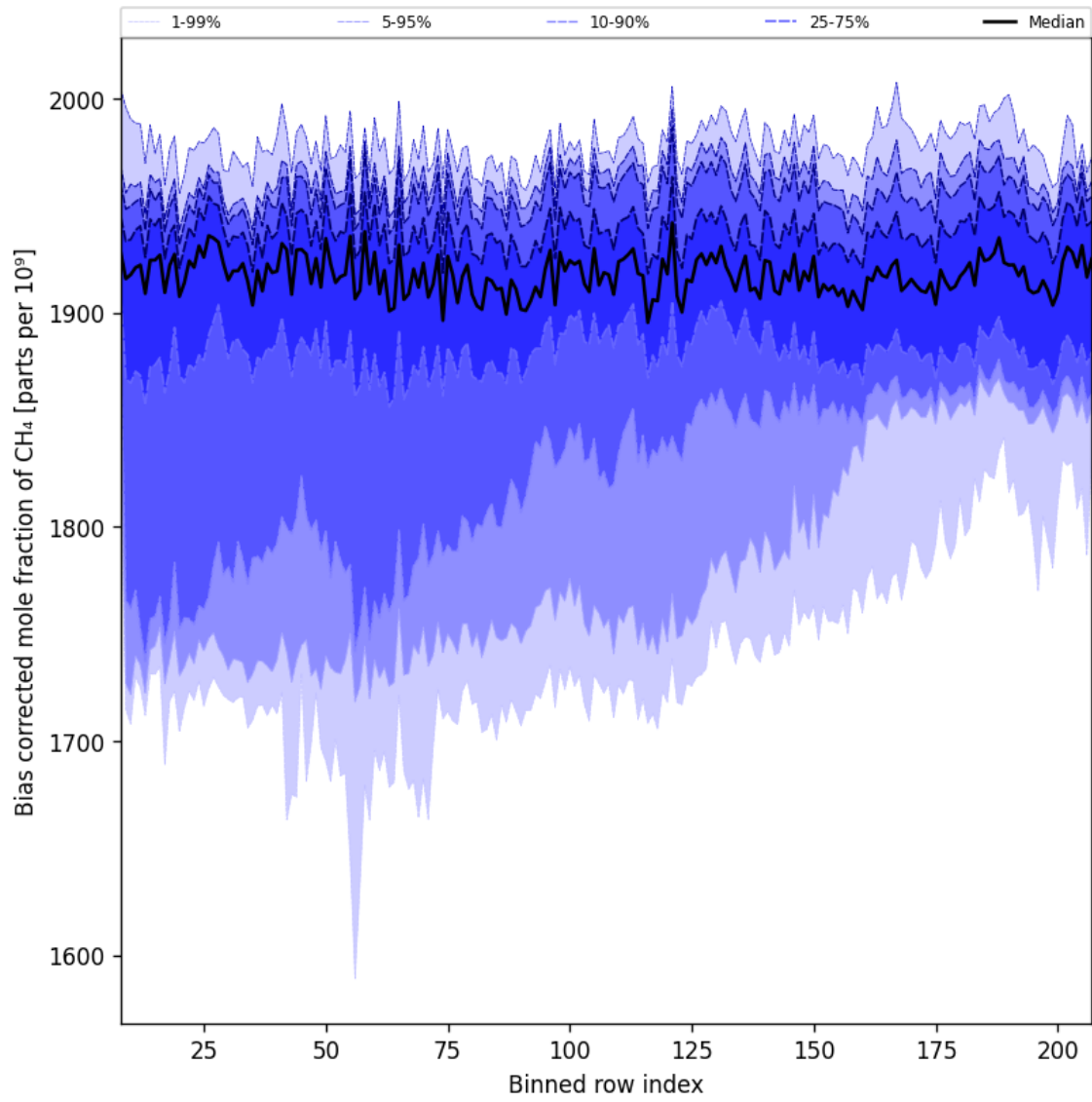
Figure 36: Along track statistics of “Bias corrected mole fraction of CH 4 ” for 2025-10-08 to 2025-10-10
