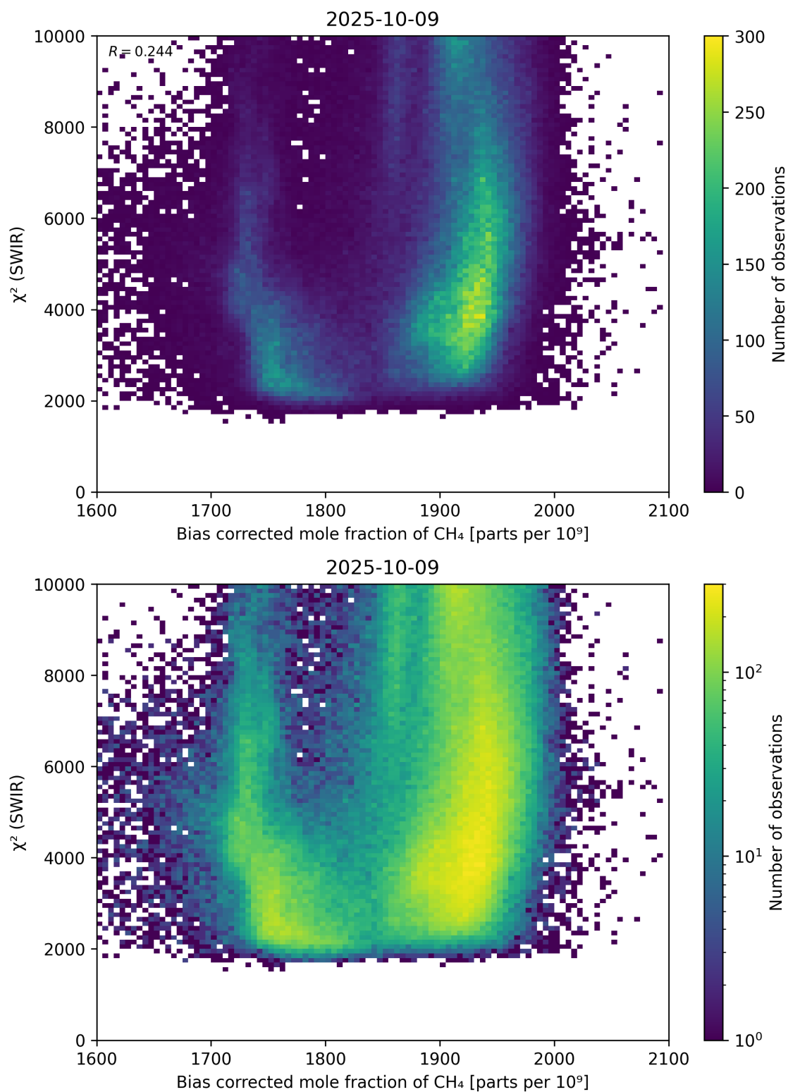
Figure 64: Scatter density plot of “Bias corrected mole fraction of CH 4 ” against “ \chi^2 (SWIR)” for 2025-10-08 to 2025-10-10.
