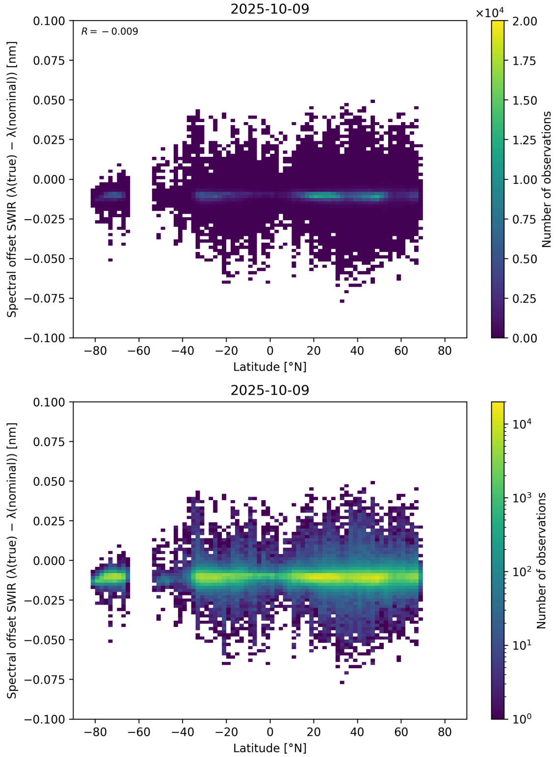
Figure 62: Scatter density plot of “Latitude” against “Spectral offset SWIR ( \lambda_{\text{true}} - \lambda_{\text{nominal}} )” for 2025-10-08 to 2025-10-10.
