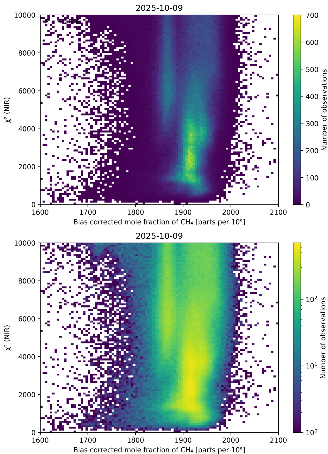
Figure 63: Scatter density plot of “Bias corrected mole fraction of \text{CH}_4 ” against “ \chi^2 (NIR)” for 2025-10-08 to 2025-10-10.
