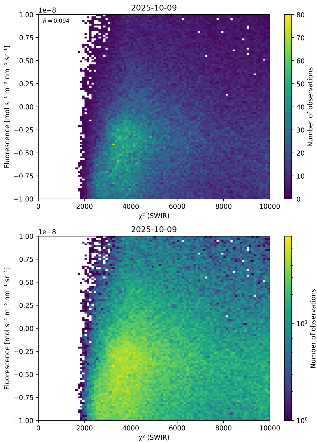
Figure 49: Scatter density plot of “ \chi^2 (SWIR)” against “Fluorescence” for 2025-10-08 to 2025-10-10.
