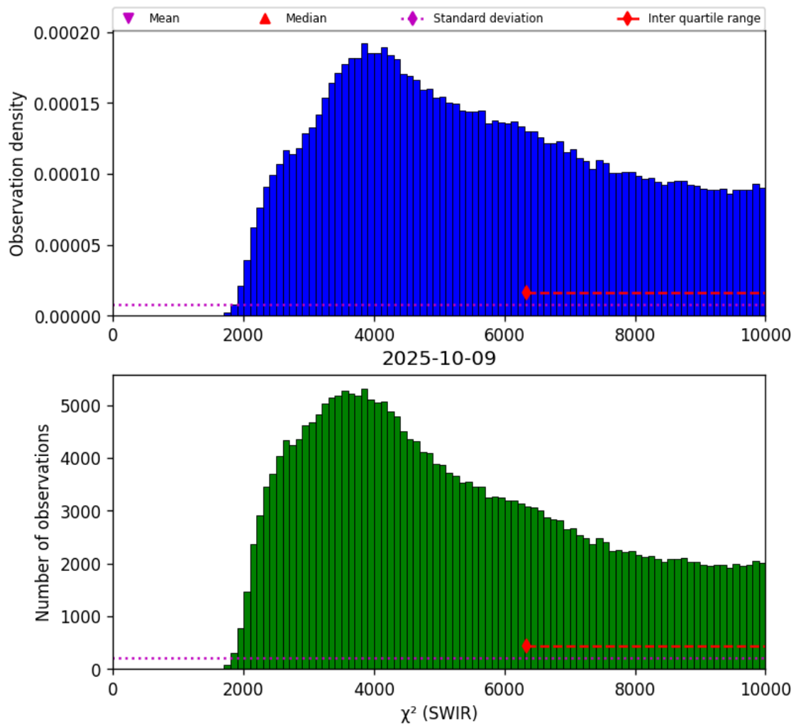
Figure 28: Histogram of " \chi^2 (SWIR)" for 2025-10-08 to 2025-10-10
