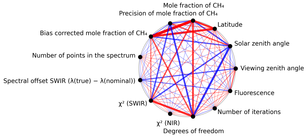
Figure 1: Map of correlation graph for 2025-10-08 to 2025-10-10.
