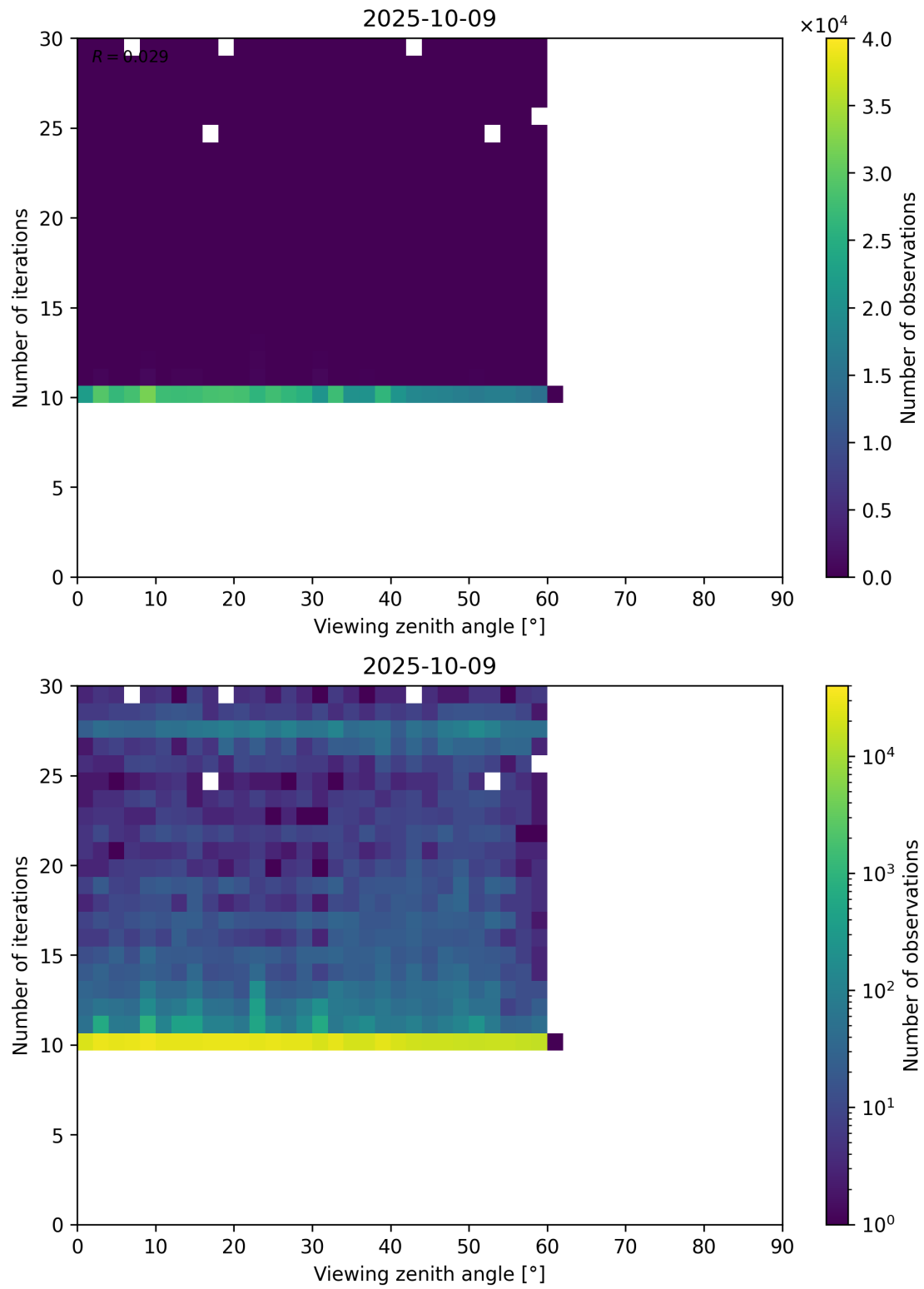
Figure 113: Scatter density plot of “Viewing zenith angle” against “Number of iterations” for 2025-10-08 to 2025-10-10.
