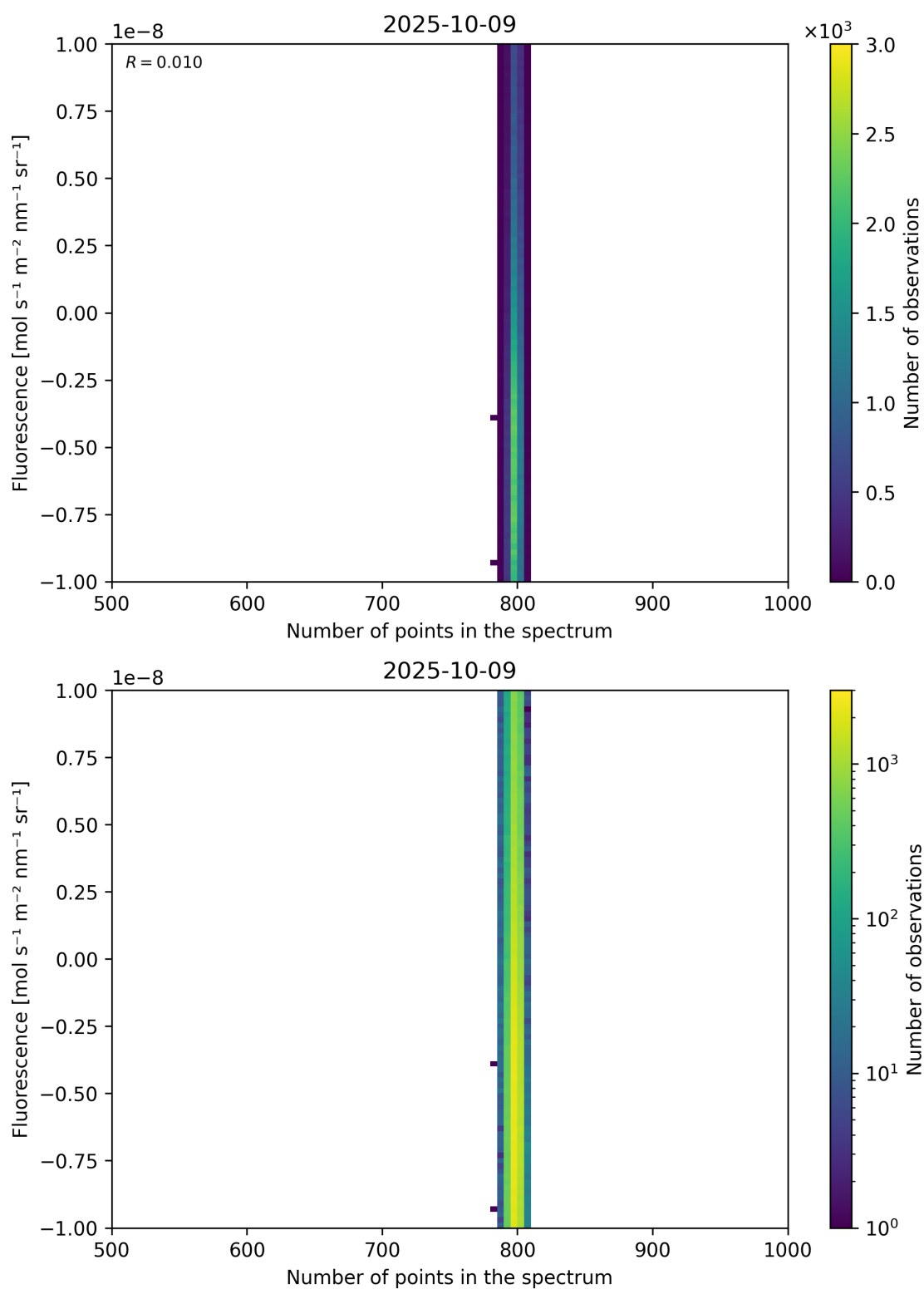
Figure 91: Scatter density plot of “Number of points in the spectrum” against “Fluorescence” for 2025-10-08 to 2025-10-10.
