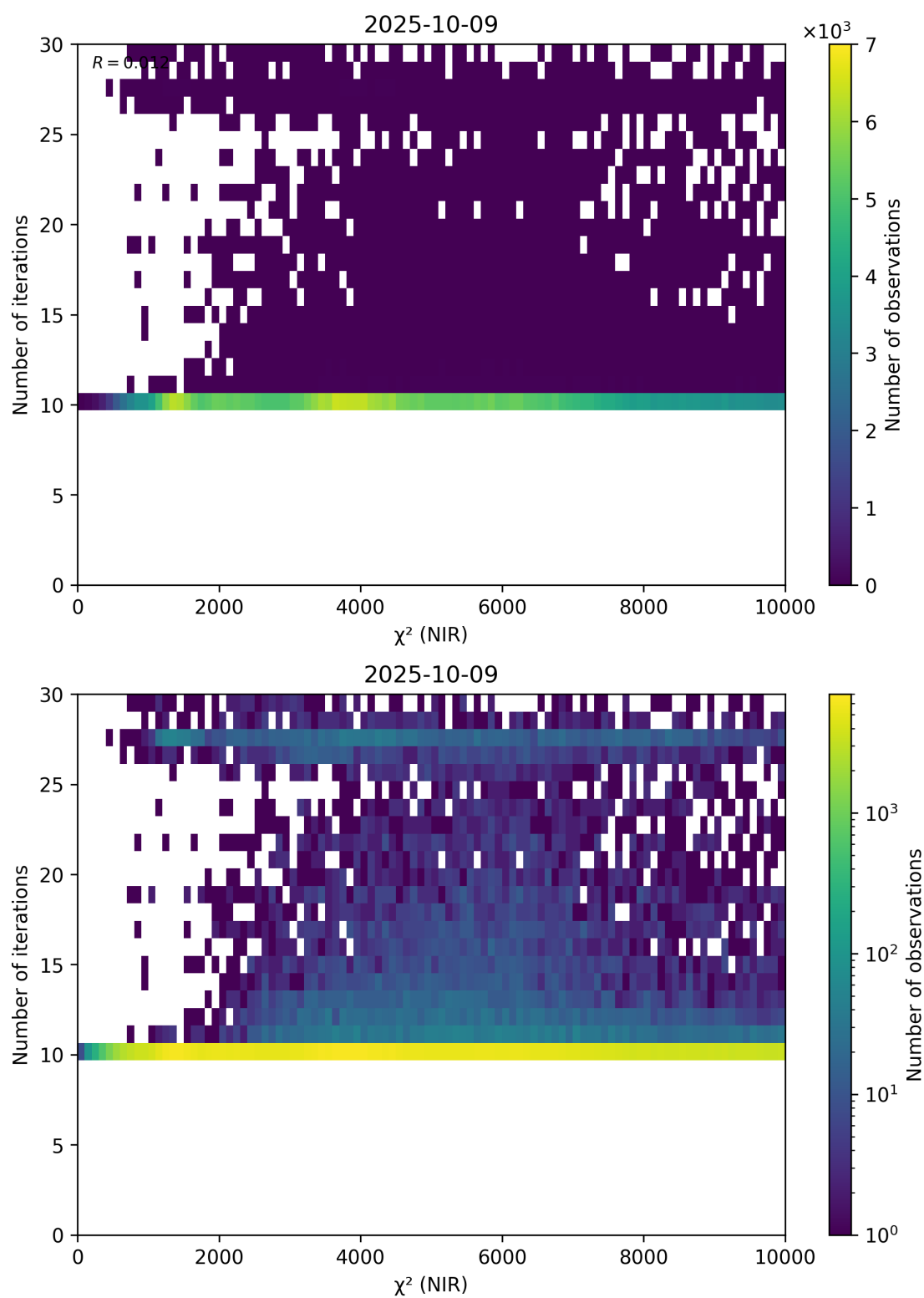
Figure 46: Scatter density plot of “ \chi^2 (NIR)” against “Number of iterations” for 2025-10-08 to 2025-10-10.
