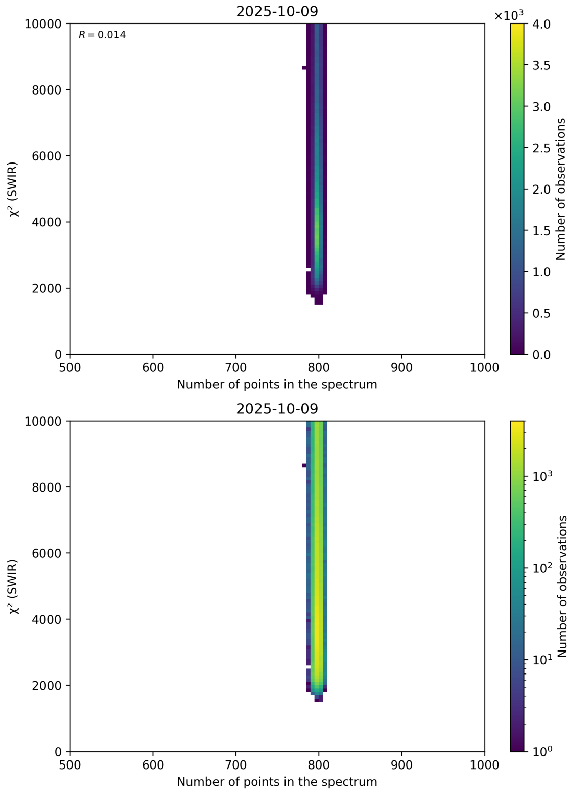
Figure 89: Scatter density plot of “Number of points in the spectrum” against “ \chi^2 (SWIR)” for 2025-10-08 to 2025-10-10.
