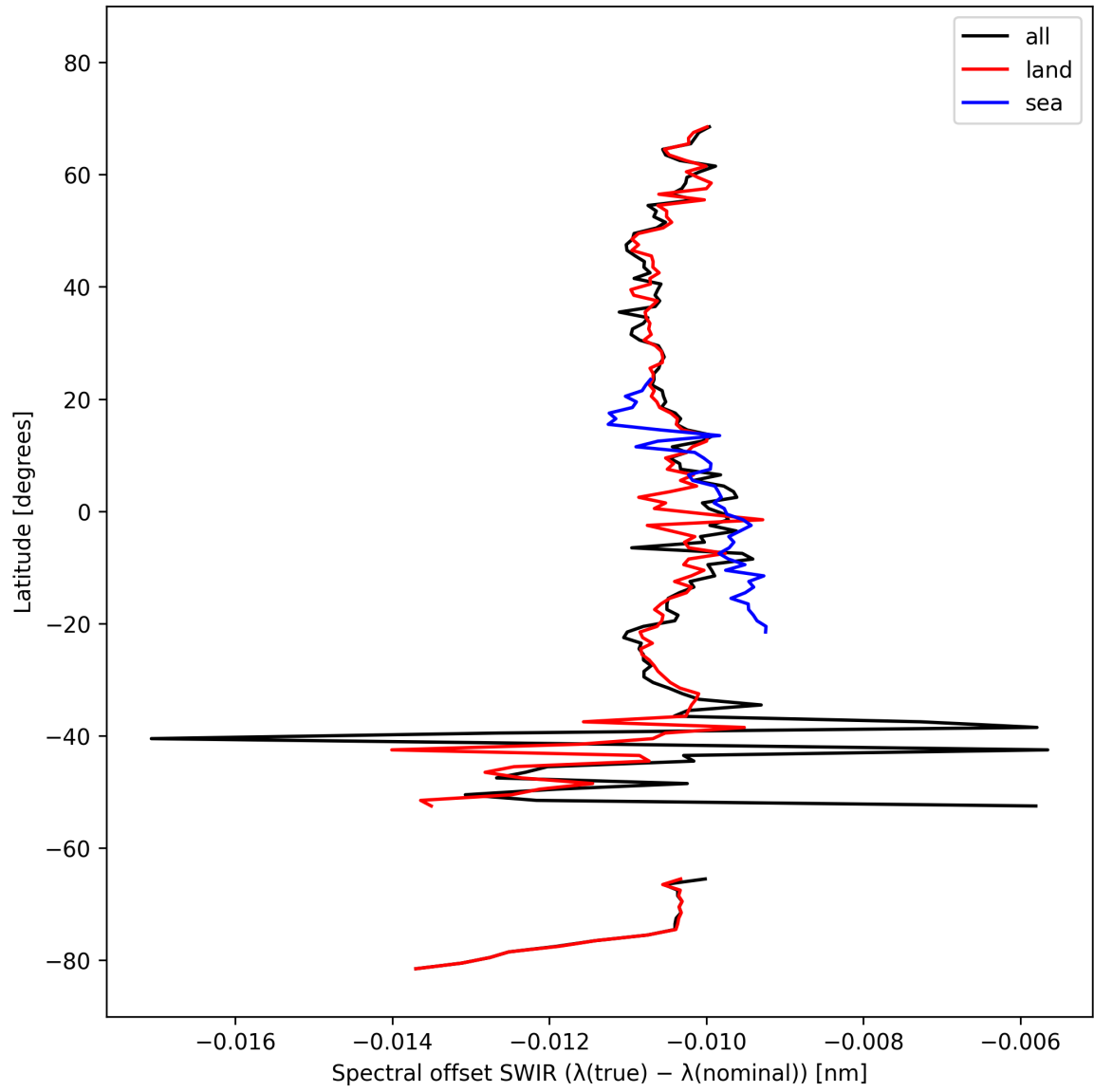
Figure 16: Zonal average of “Spectral offset SWIR ( \lambda_{\text{true}} - \lambda_{\text{nominal}} )” for 2025-10-08 to 2025-10-10.
