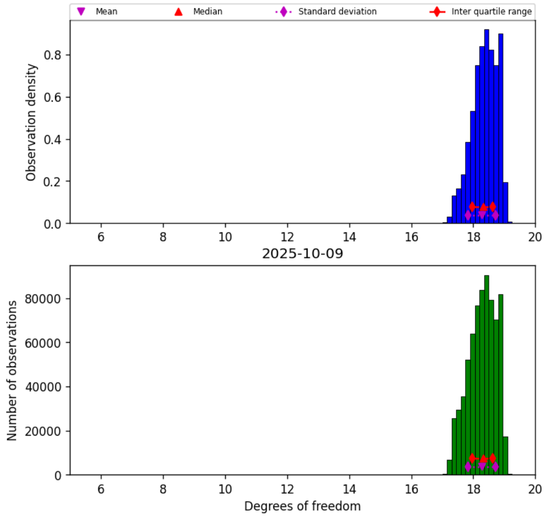
Figure 30: Histogram of “Degrees of freedom” for 2025-10-08 to 2025-10-10
