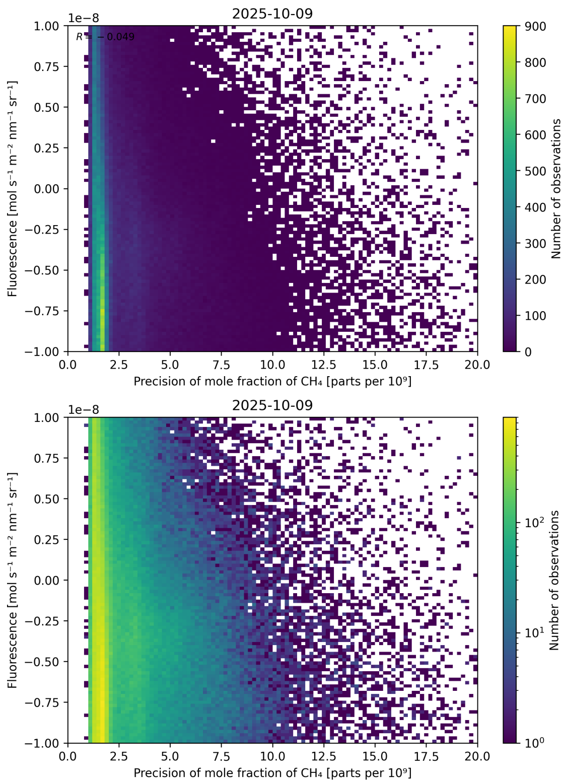
Figure 81: Scatter density plot of “Precision of mole fraction of \text{CH}_4 ” against “Fluorescence” for 2025-10-08 to 2025-10-10.
