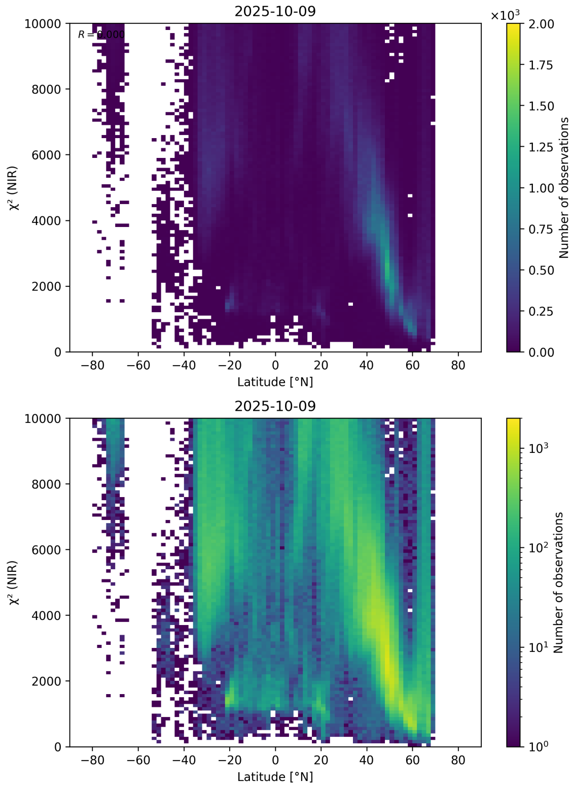
Figure 53: Scatter density plot of “Latitude” against “ \chi^2 (NIR)” for 2025-10-08 to 2025-10-10.
