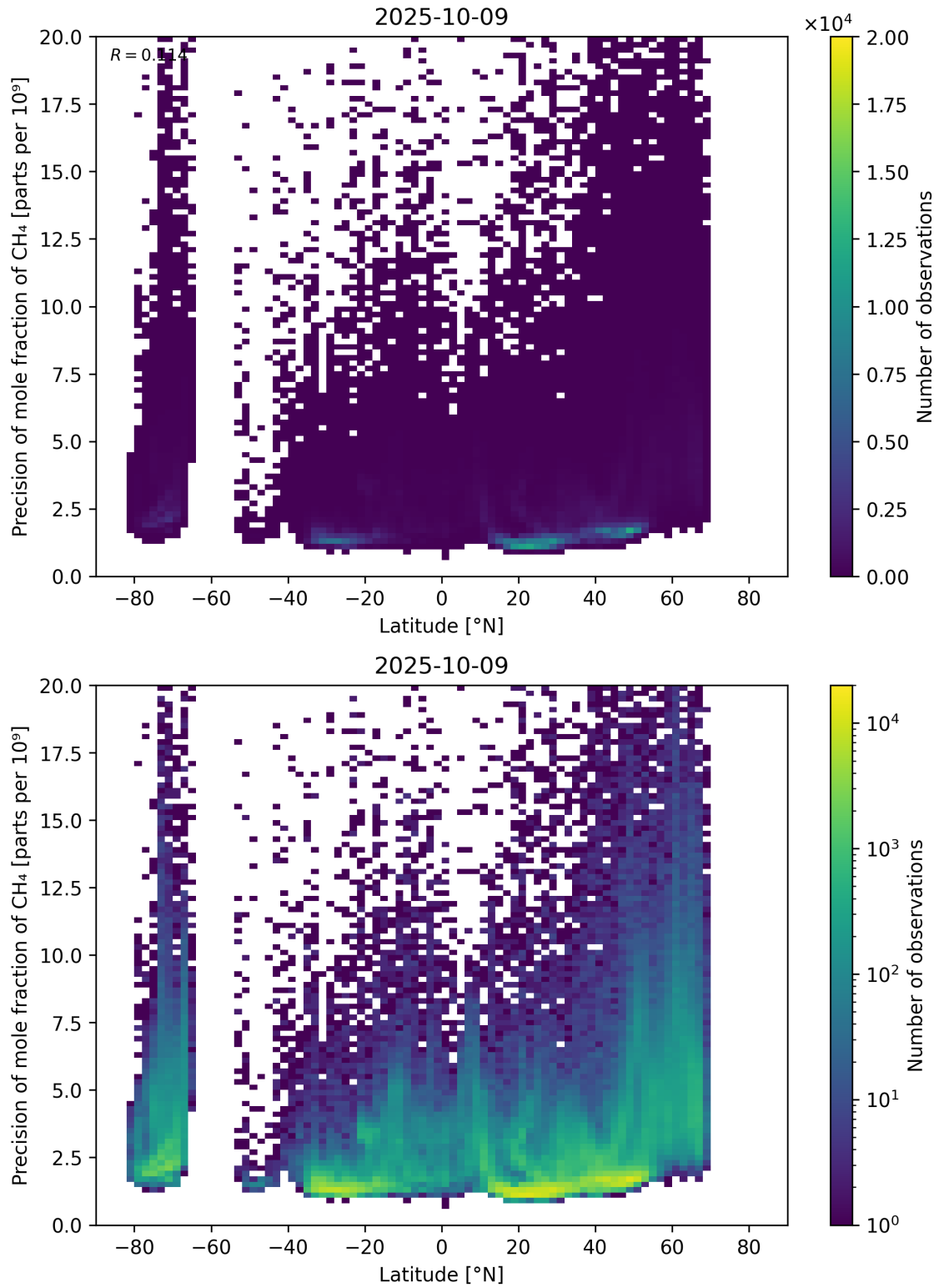
Figure 59: Scatter density plot of “Latitude” against “Precision of mole fraction of CH 4 ” for 2025-10-08 to 2025-10-10.
