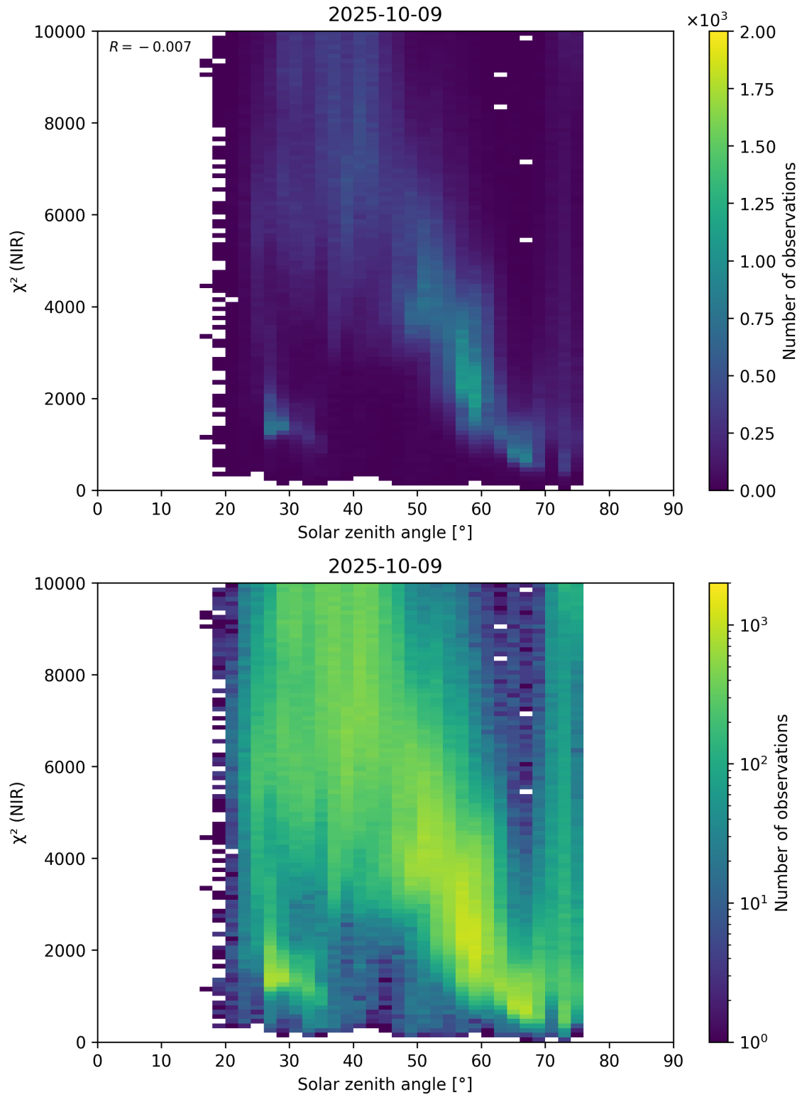
Figure 94: Scatter density plot of “Solar zenith angle” against “ \chi^2 (NIR)” for 2025-10-08 to 2025-10-10.
