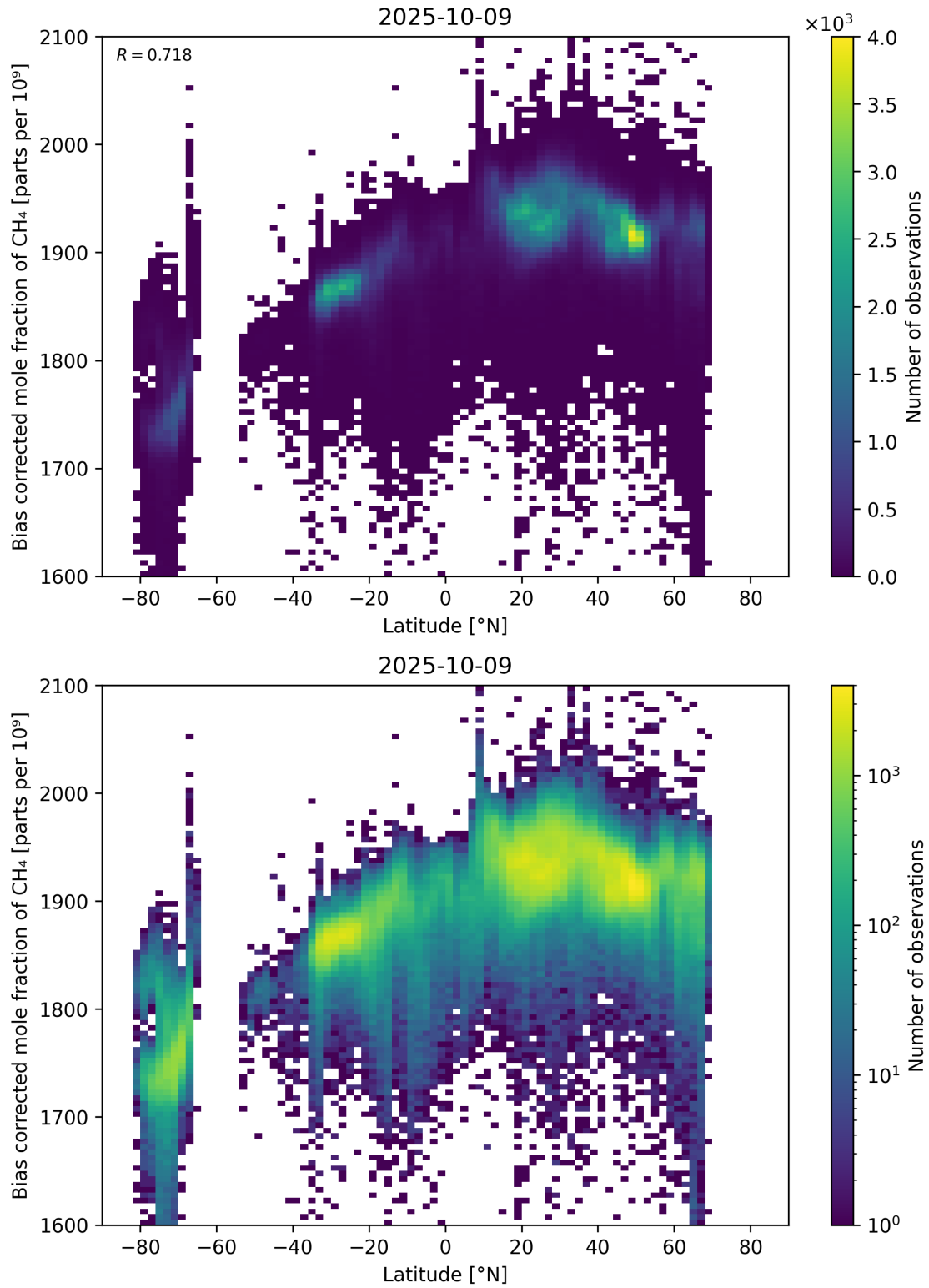
Figure 58: Scatter density plot of “Latitude” against “Bias corrected mole fraction of \text{CH}_4 ” for 2025-10-08 to 2025-10-10.
