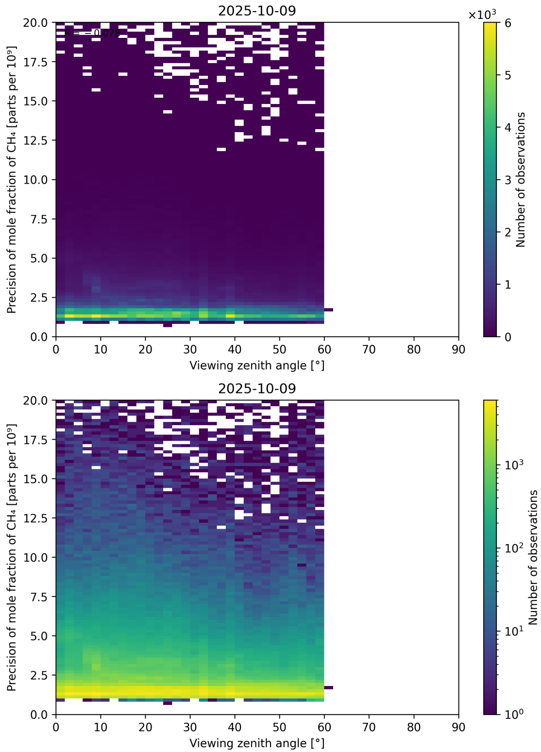
Figure 112: Scatter density plot of “Viewing zenith angle” against “Precision of mole fraction of CH 4 ” for 2025-10-08 to 2025-10-10.
