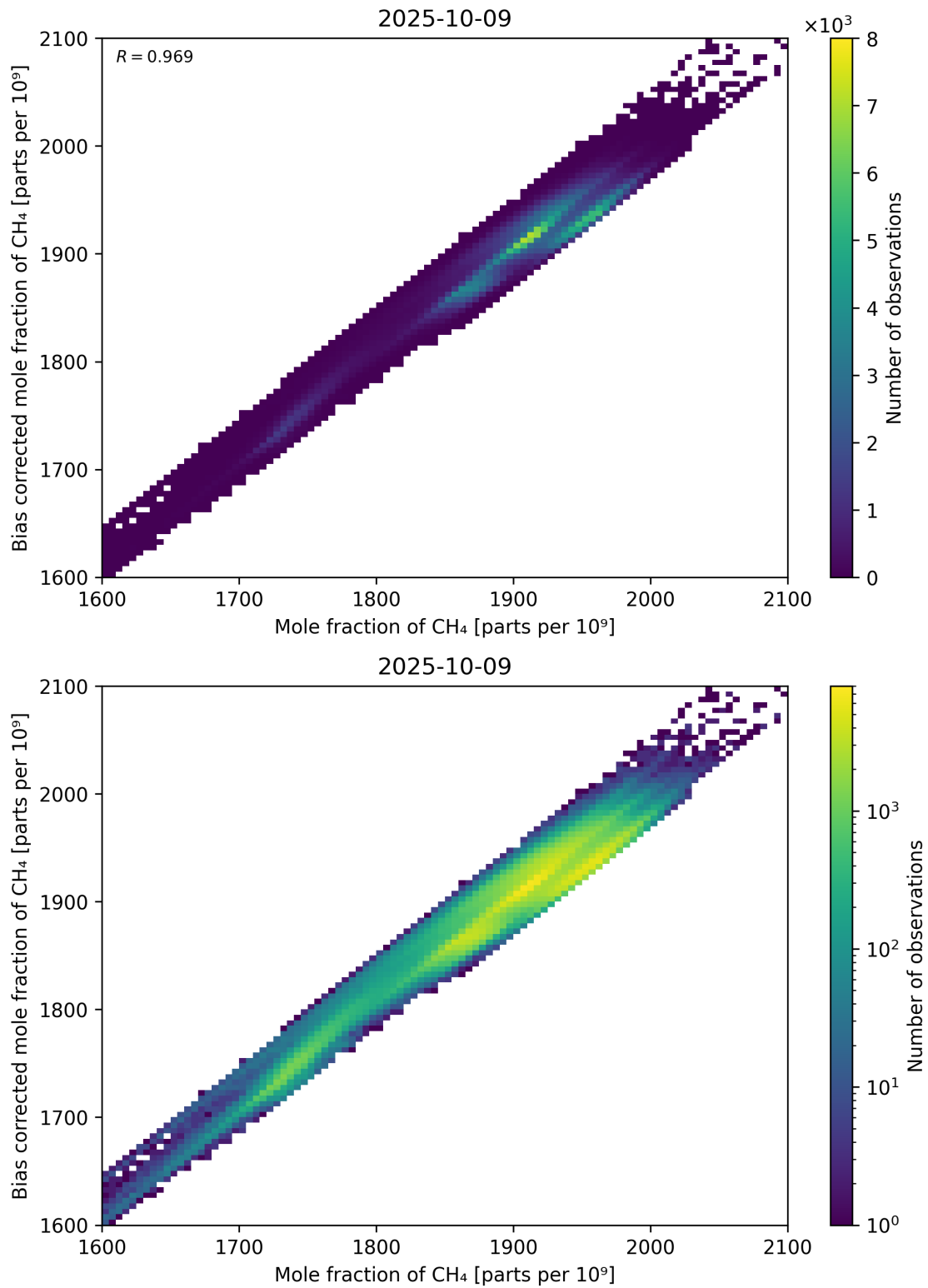
Figure 74: Scatter density plot of “Mole fraction of CH 4 ” against “Bias corrected mole fraction of CH 4 ” for 2025-10-08 to 2025-10-10.
