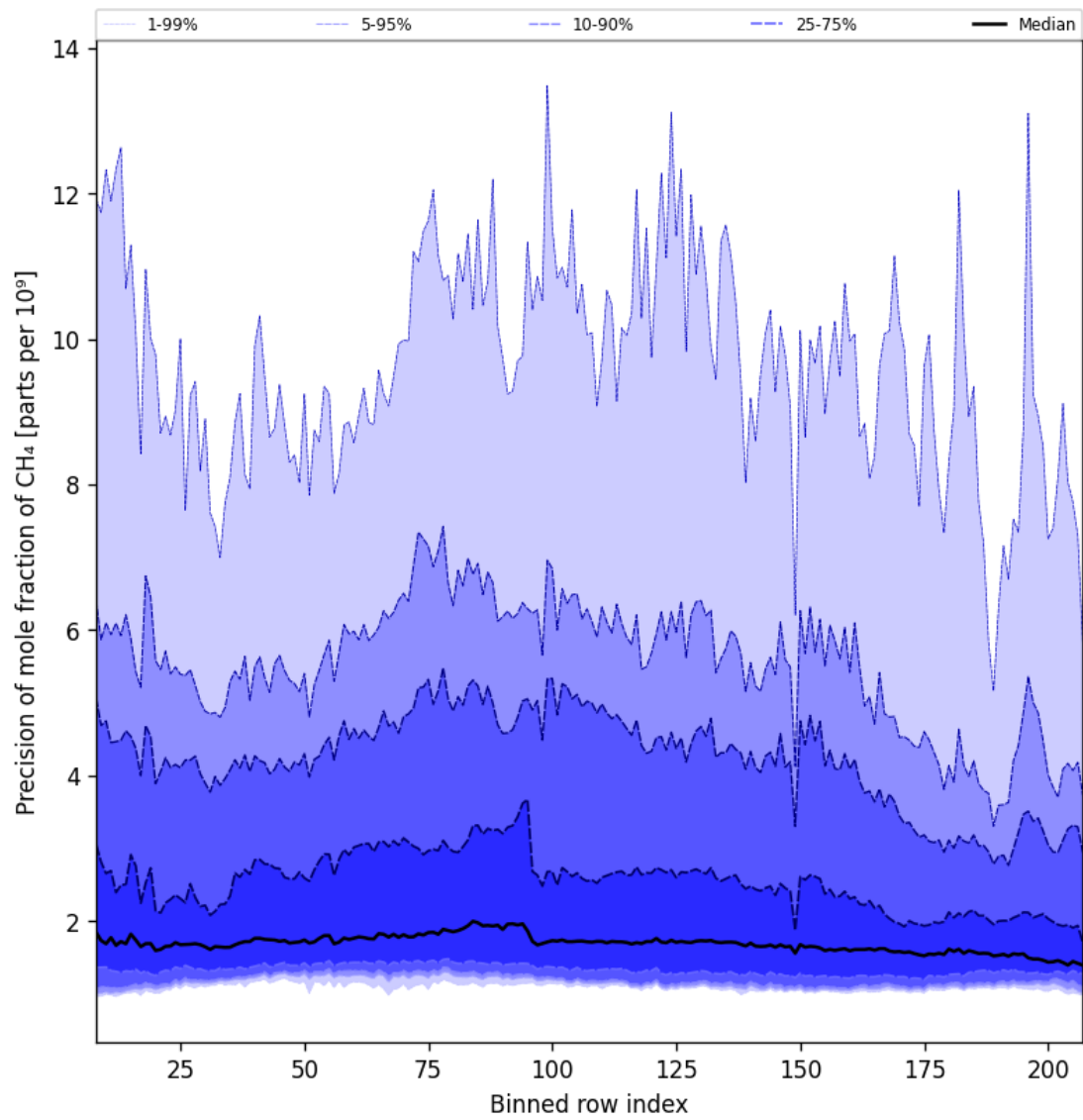
Figure 35: Along track statistics of “Precision of mole fraction of CH 4 ” for 2025-10-08 to 2025-10-10
