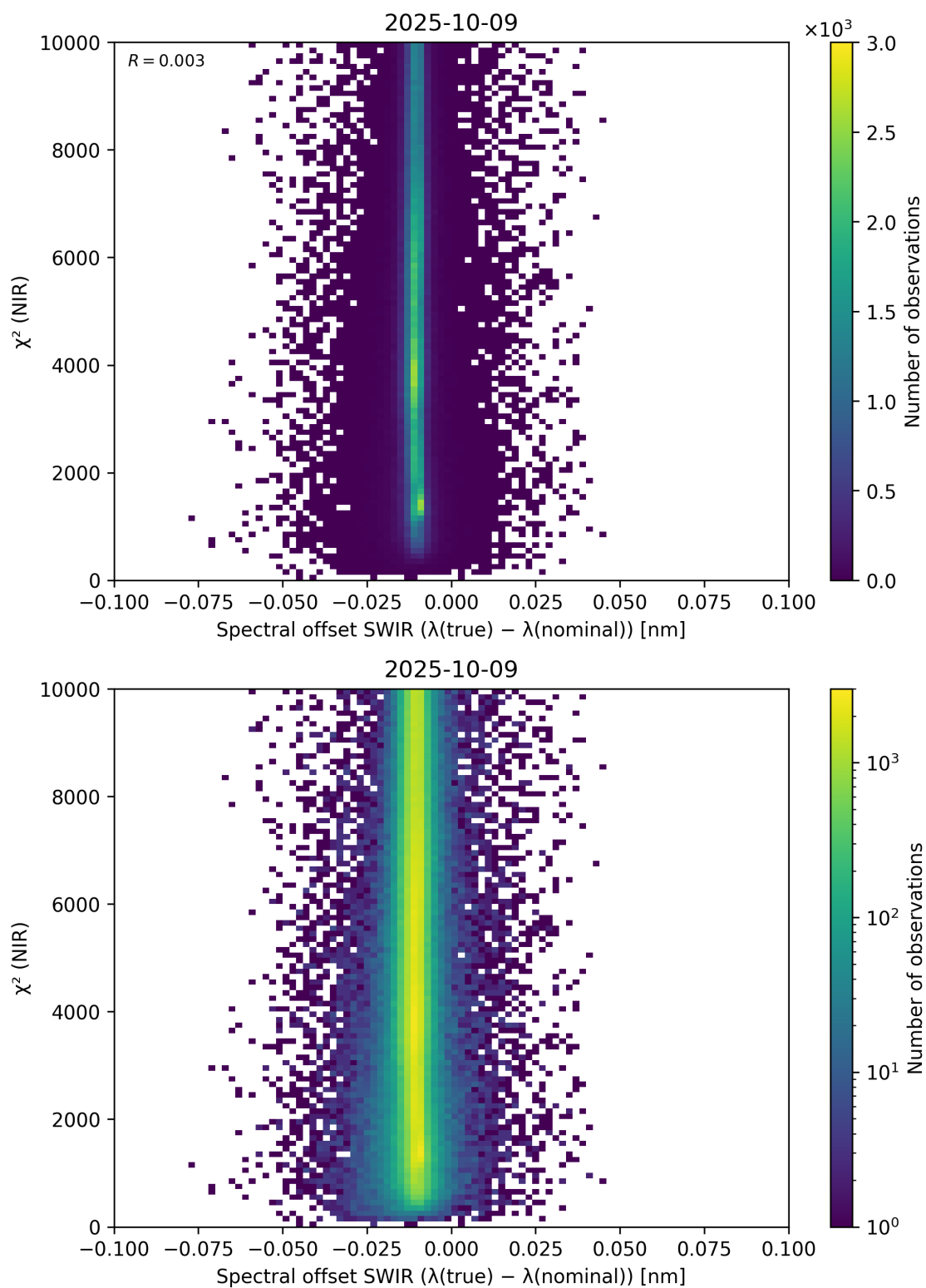
Figure 117: Scatter density plot of “Spectral offset SWIR ( \lambda_{\text{true}} - \lambda_{\text{nominal}} )” against “ \chi^2 (NIR)” for 2025-10-08 to 2025-10-10.
