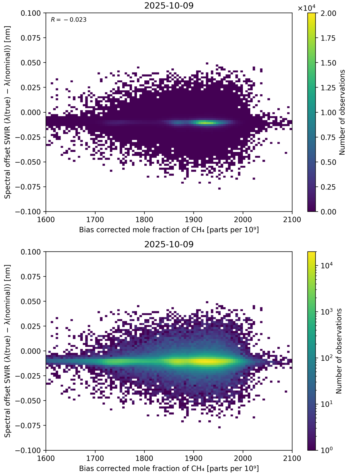
Figure 69: Scatter density plot of “Bias corrected mole fraction of \text{CH}_4 ” against “Spectral offset SWIR ( \lambda_{\text{true}} - \lambda_{\text{nominal}} )” for 2025-10-08 to 2025-10-10.
