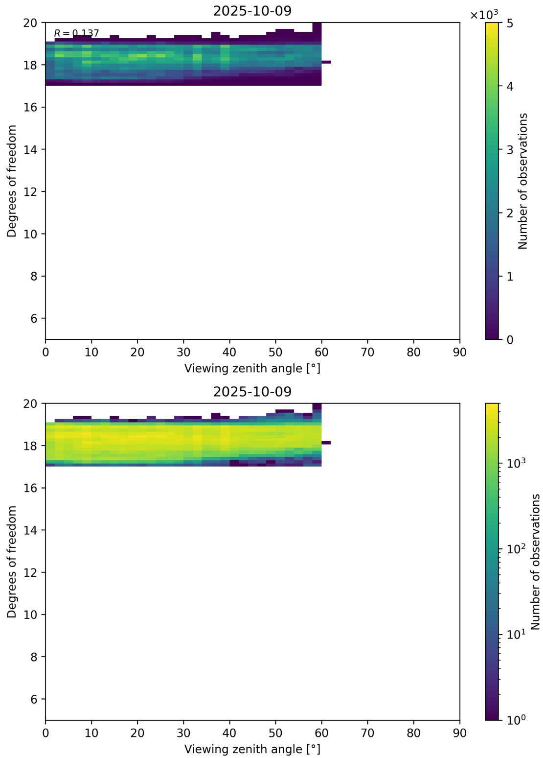
Figure 107: Scatter density plot of “Viewing zenith angle” against “Degrees of freedom” for 2025-10-08 to 2025-10-10.
