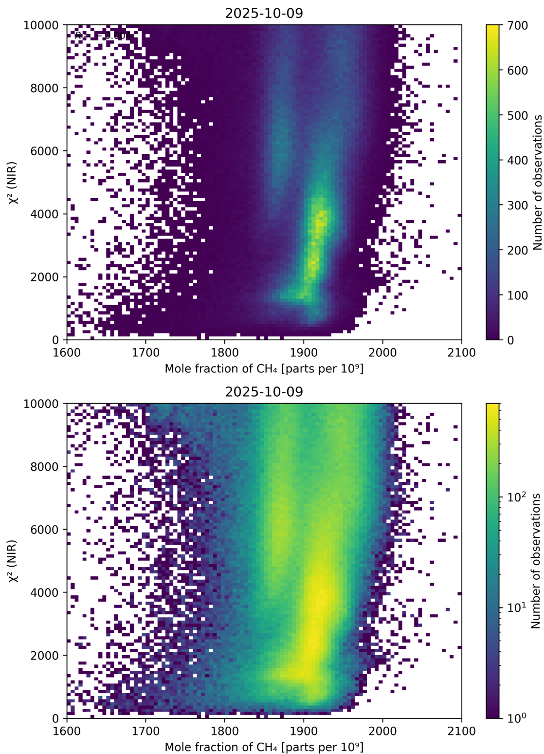
Figure 70: Scatter density plot of “Mole fraction of CH 4 ” against “ \chi^2 (NIR)” for 2025-10-08 to 2025-10-10.
