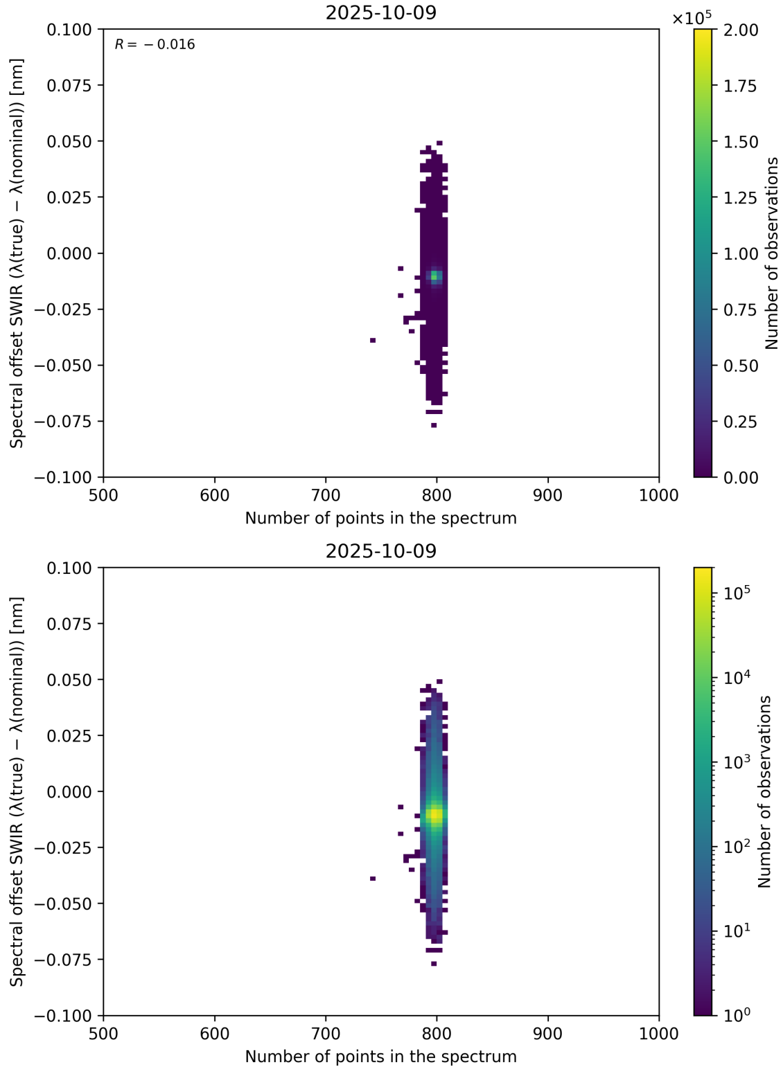
Figure 93: Scatter density plot of “Number of points in the spectrum” against “Spectral offset SWIR ( \lambda_{\text{true}} - \lambda_{\text{nominal}} )” for 2025-10-08 to 2025-10-10.
