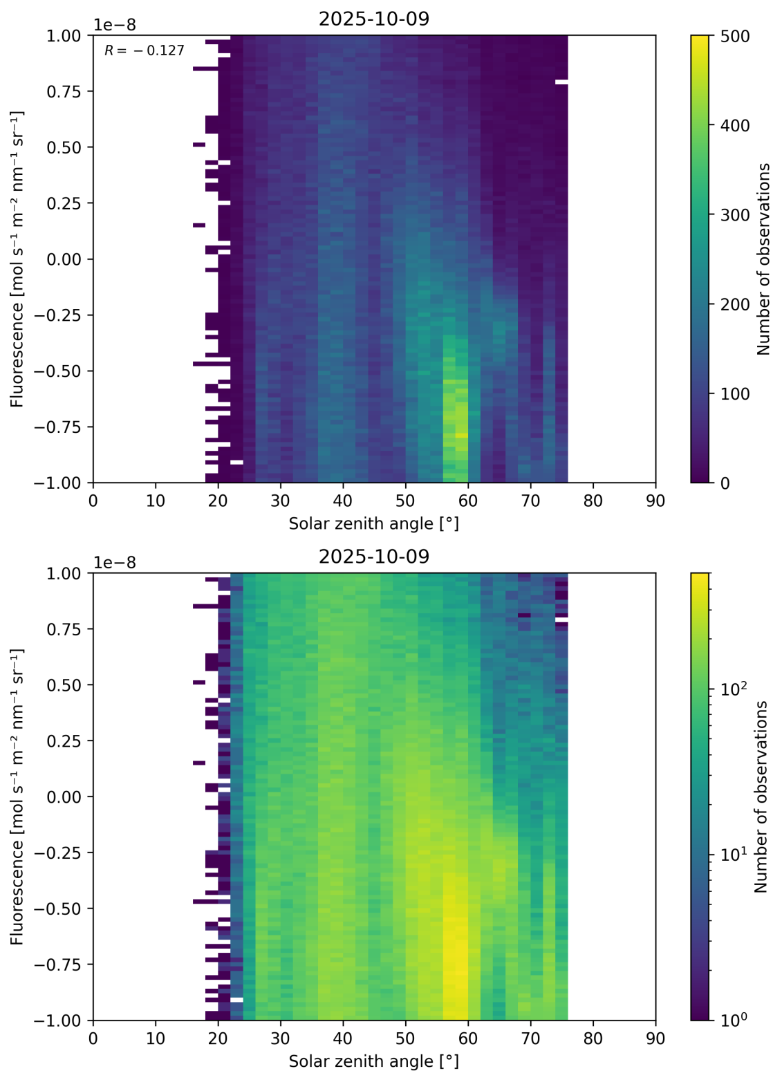
Figure 97: Scatter density plot of “Solar zenith angle” against “Fluorescence” for 2025-10-08 to 2025-10-10.
