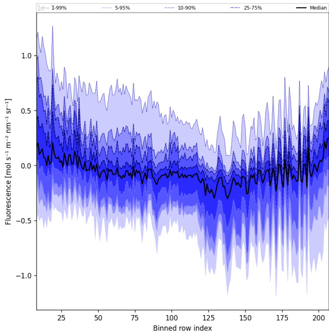
Figure 43: Along track statistics of “Fluorescence” for 2025-10-08 to 2025-10-10
