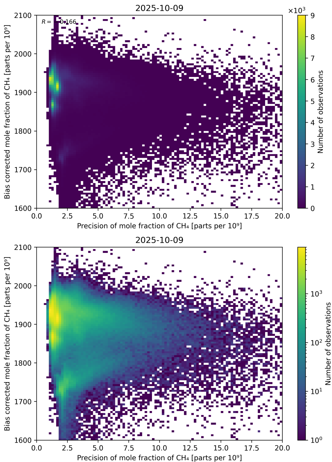
Figure 82: Scatter density plot of “Precision of mole fraction of CH 4 ” against “Bias corrected mole fraction of CH 4 ” for 2025-10-08 to 2025-10-10.
