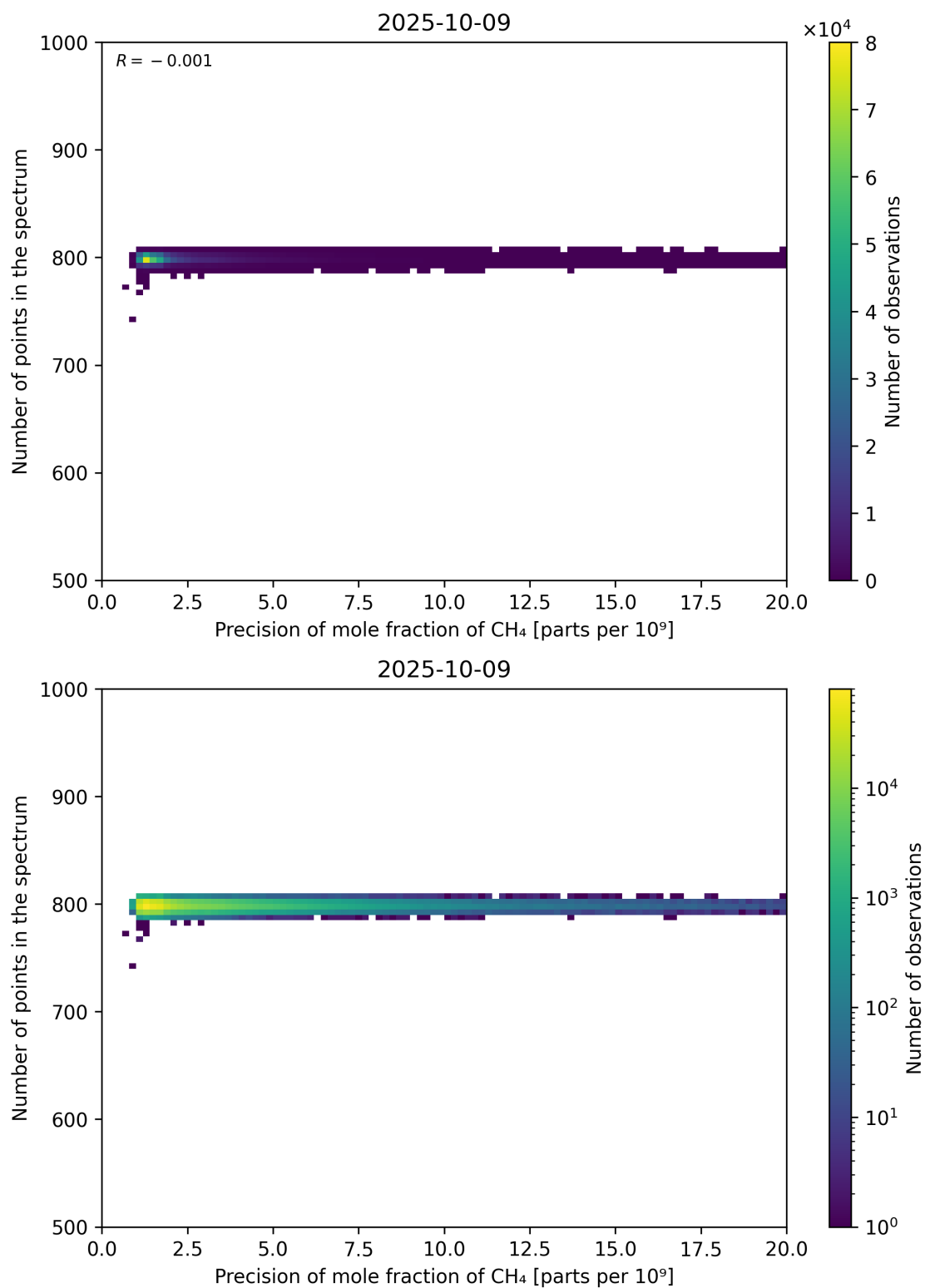
Figure 84: Scatter density plot of “Precision of mole fraction of CH 4 ” against “Number of points in the spectrum” for 2025-10-08 to 2025-10-10.
