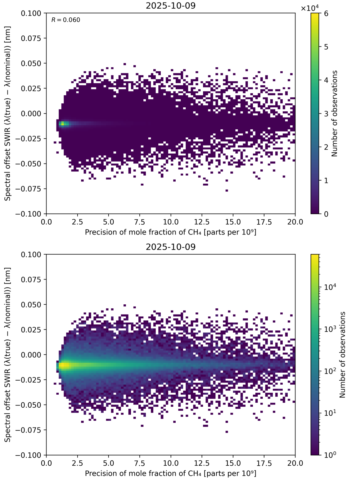
Figure 85: Scatter density plot of “Precision of mole fraction of \text{CH}_4 ” against “Spectral offset SWIR ( \lambda_{\text{true}} - \lambda_{\text{nominal}} )” for 2025-10-08 to 2025-10-10.
