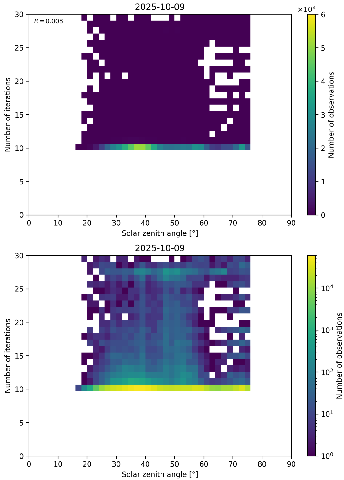
Figure 102: Scatter density plot of “Solar zenith angle” against “Number of iterations” for 2025-10-08 to 2025-10-10.
