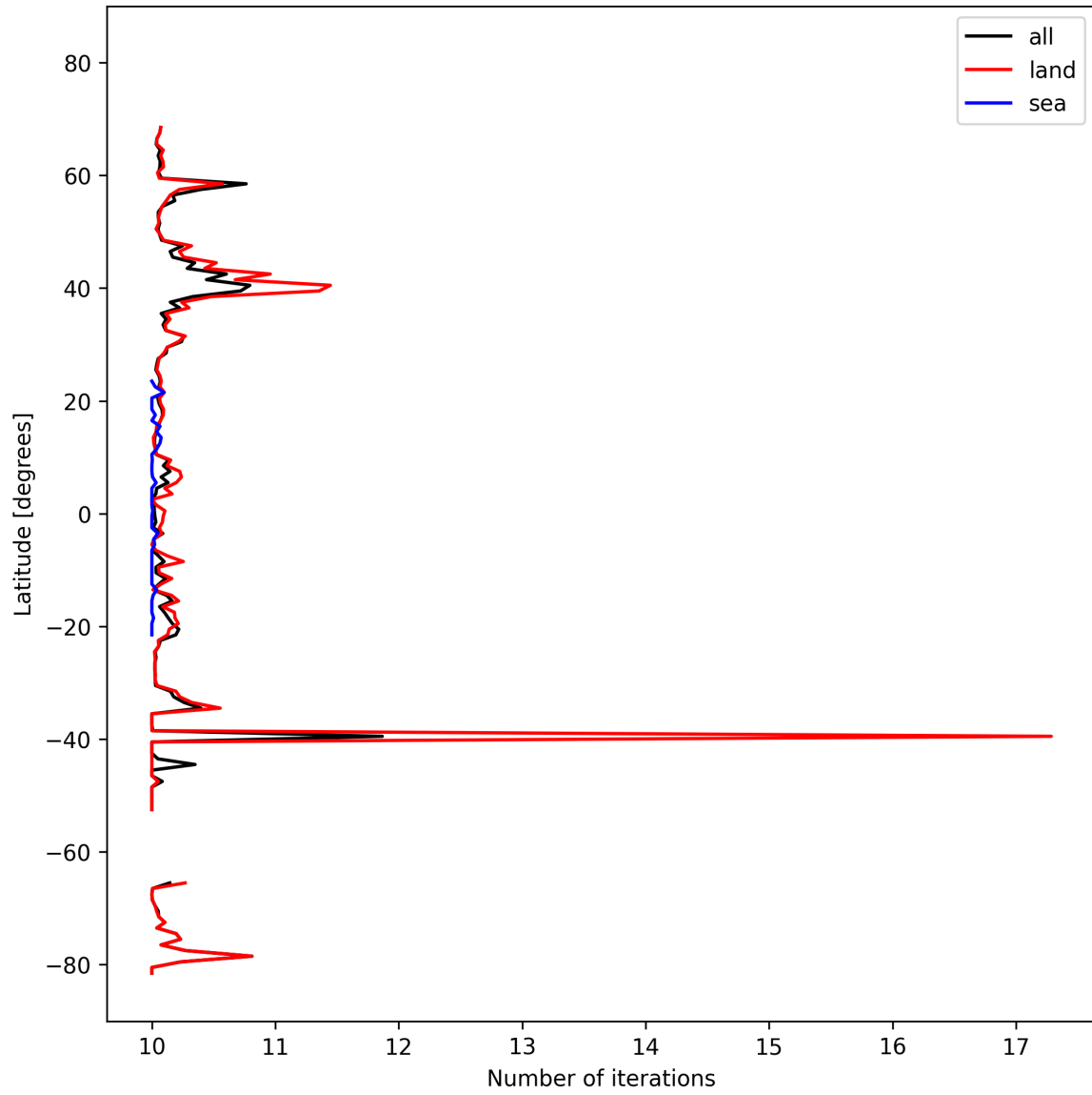
Figure 20: Zonal average of “Number of iterations” for 2025-10-08 to 2025-10-10.
