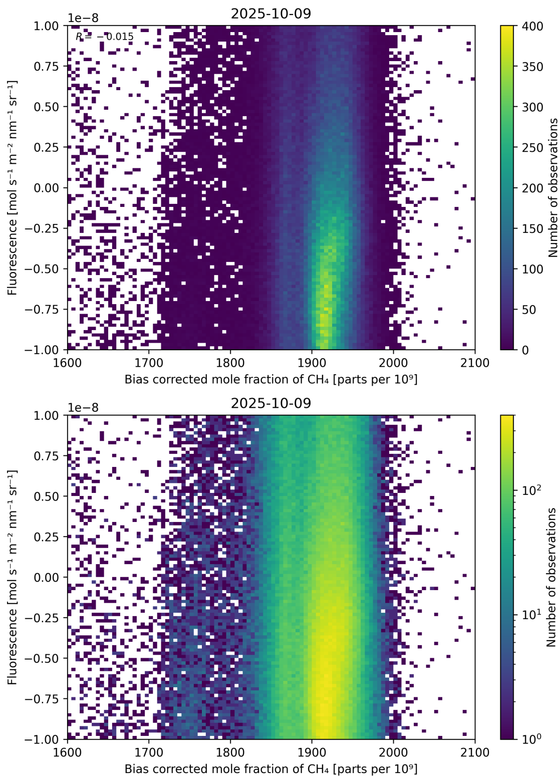
Figure 66: Scatter density plot of “Bias corrected mole fraction of \text{CH}_4 ” against “Fluorescence” for 2025-10-08 to 2025-10-10.
