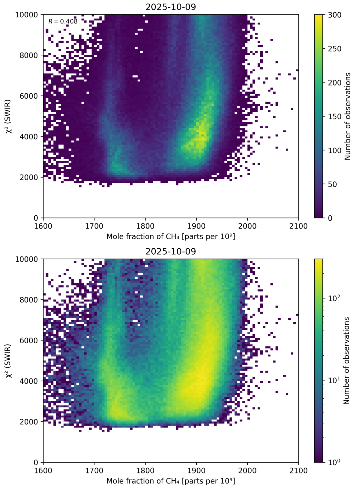
Figure 71: Scatter density plot of “Mole fraction of CH 4 ” against “ \chi^2 (SWIR)” for 2025-10-08 to 2025-10-10.
