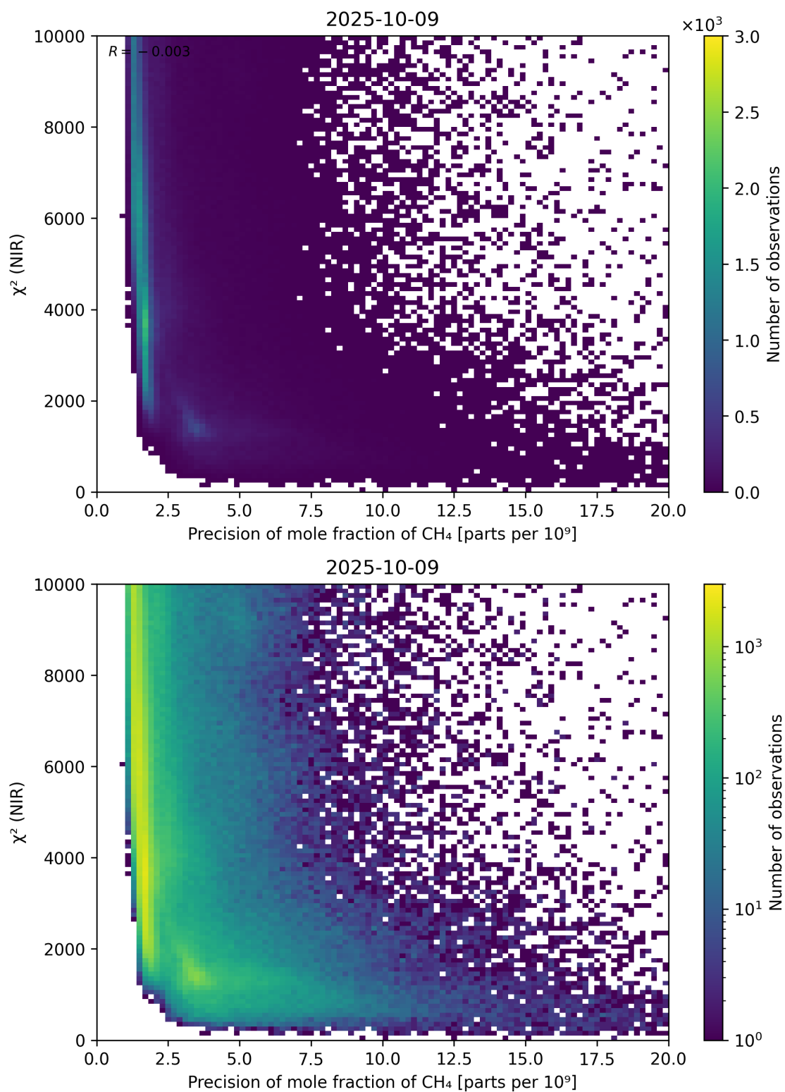
Figure 78: Scatter density plot of “Precision of mole fraction of CH 4 ” against “ \chi^2 (NIR)” for 2025-10-08 to 2025-10-10.
