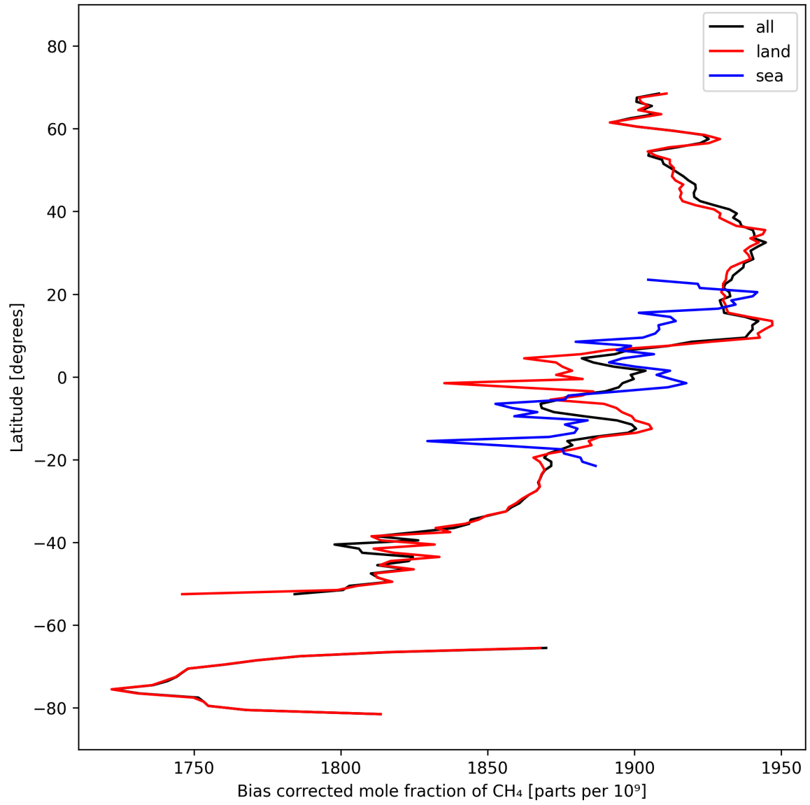
Figure 14: Zonal average of “Bias corrected mole fraction of CH 4 ” for 2025-10-08 to 2025-10-10.
