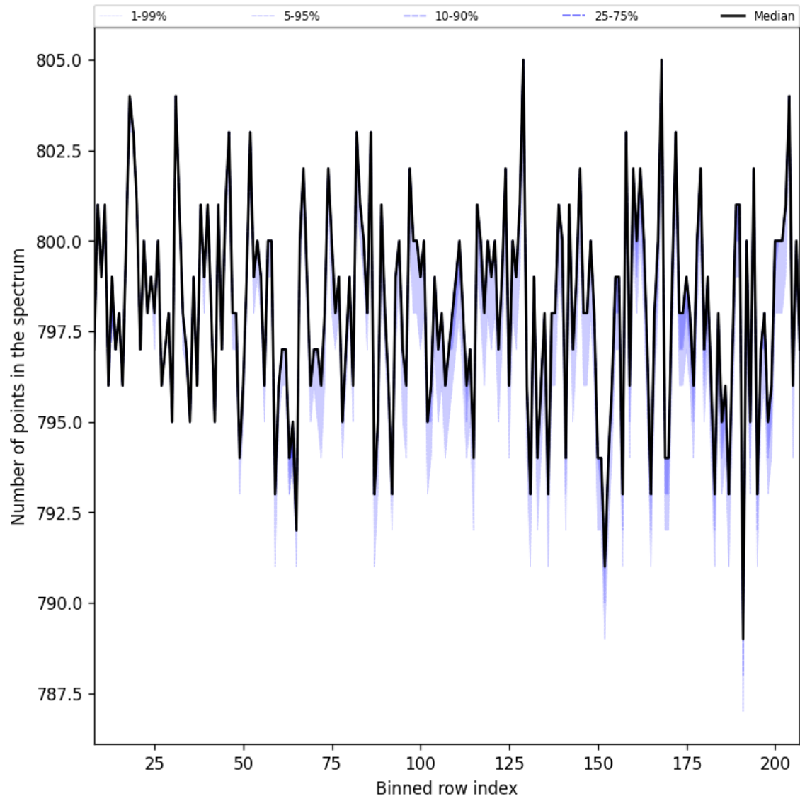
Figure 37: Along track statistics of “Number of points in the spectrum” for 2025-10-08 to 2025-10-10
