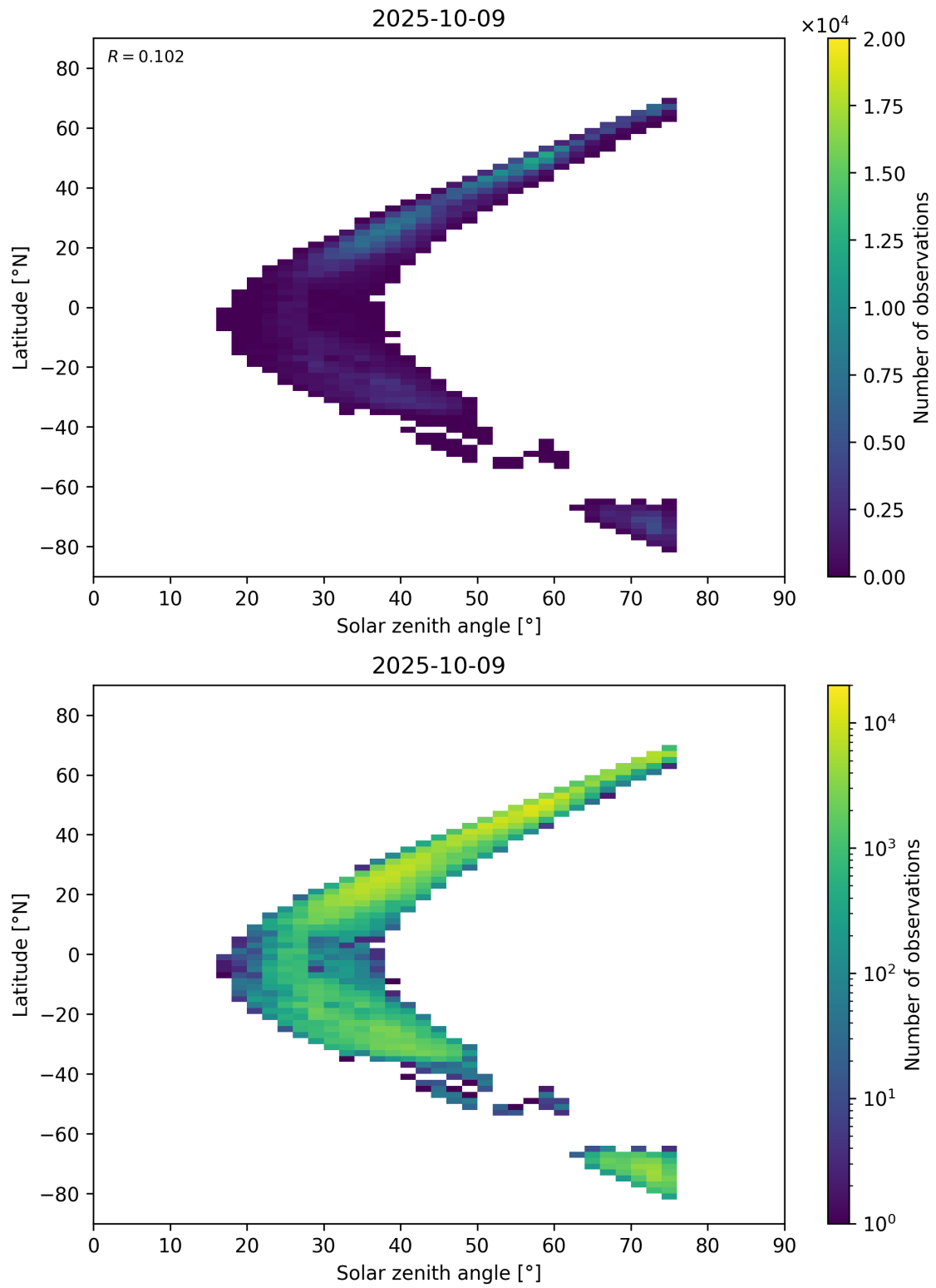
Figure 98: Scatter density plot of “Solar zenith angle” against “Latitude” for 2025-10-08 to 2025-10-10.
