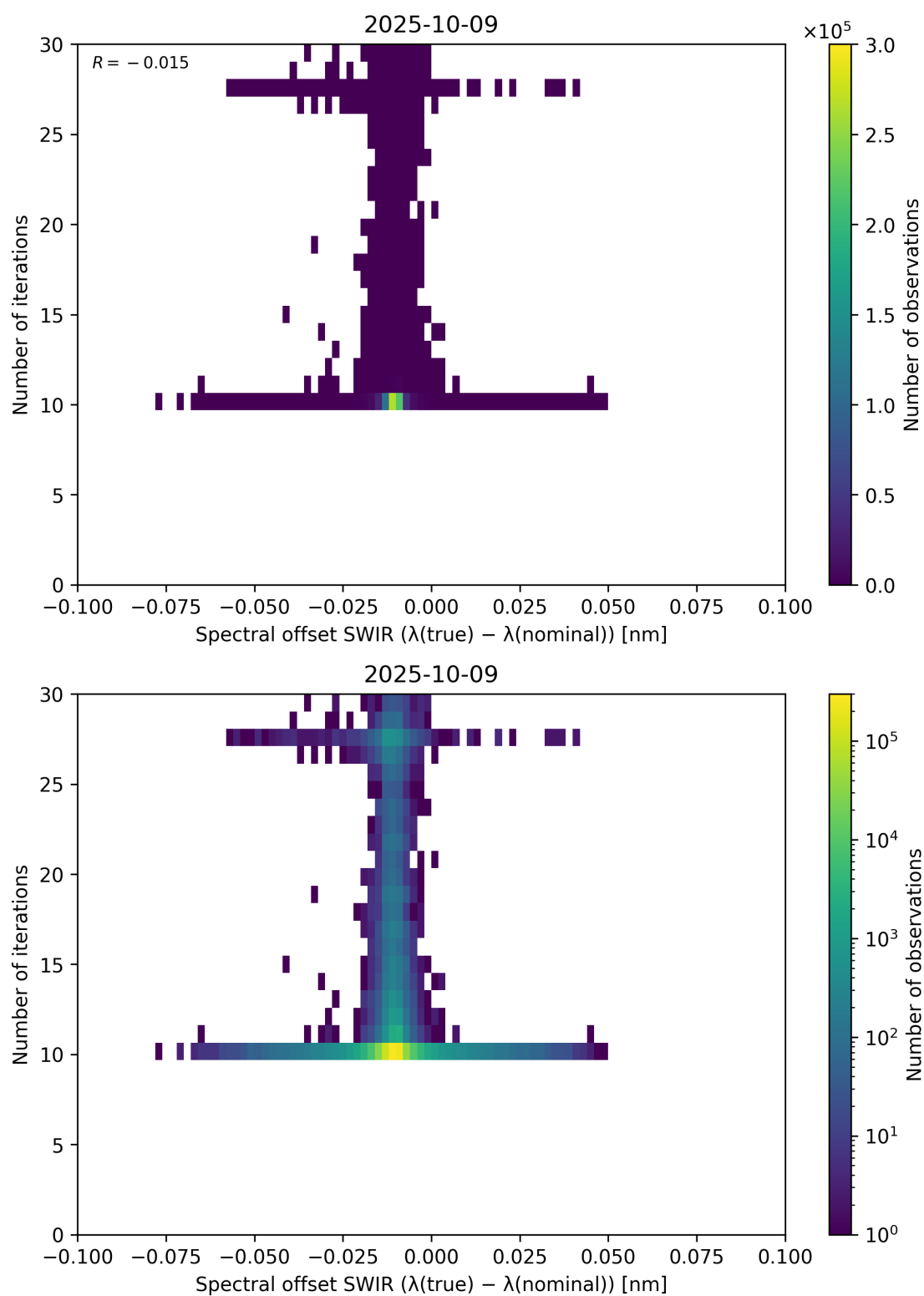
Figure 121: Scatter density plot of “Spectral offset SWIR ( \lambda_{\text{true}} - \lambda_{\text{nominal}} )” against “Number of iterations” for 2025-10-08 to 2025-10-10.
