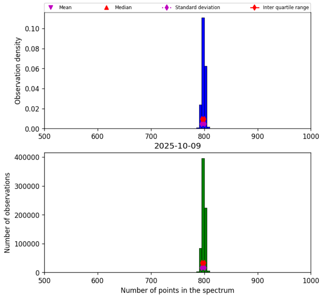
Figure 26: Histogram of “Number of points in the spectrum” for 2025-10-08 to 2025-10-10
