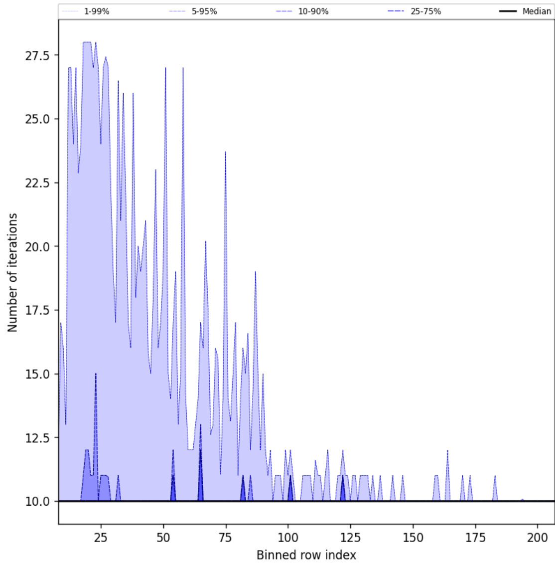
Figure 42: Along track statistics of “Number of iterations” for 2025-10-08 to 2025-10-10
