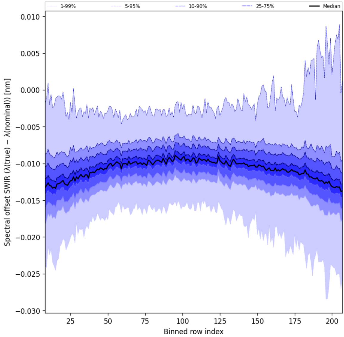
Figure 38: Along track statistics of “Spectral offset SWIR ( \lambda_{\text{true}} - \lambda_{\text{nominal}} )” for 2025-10-08 to 2025-10-10
