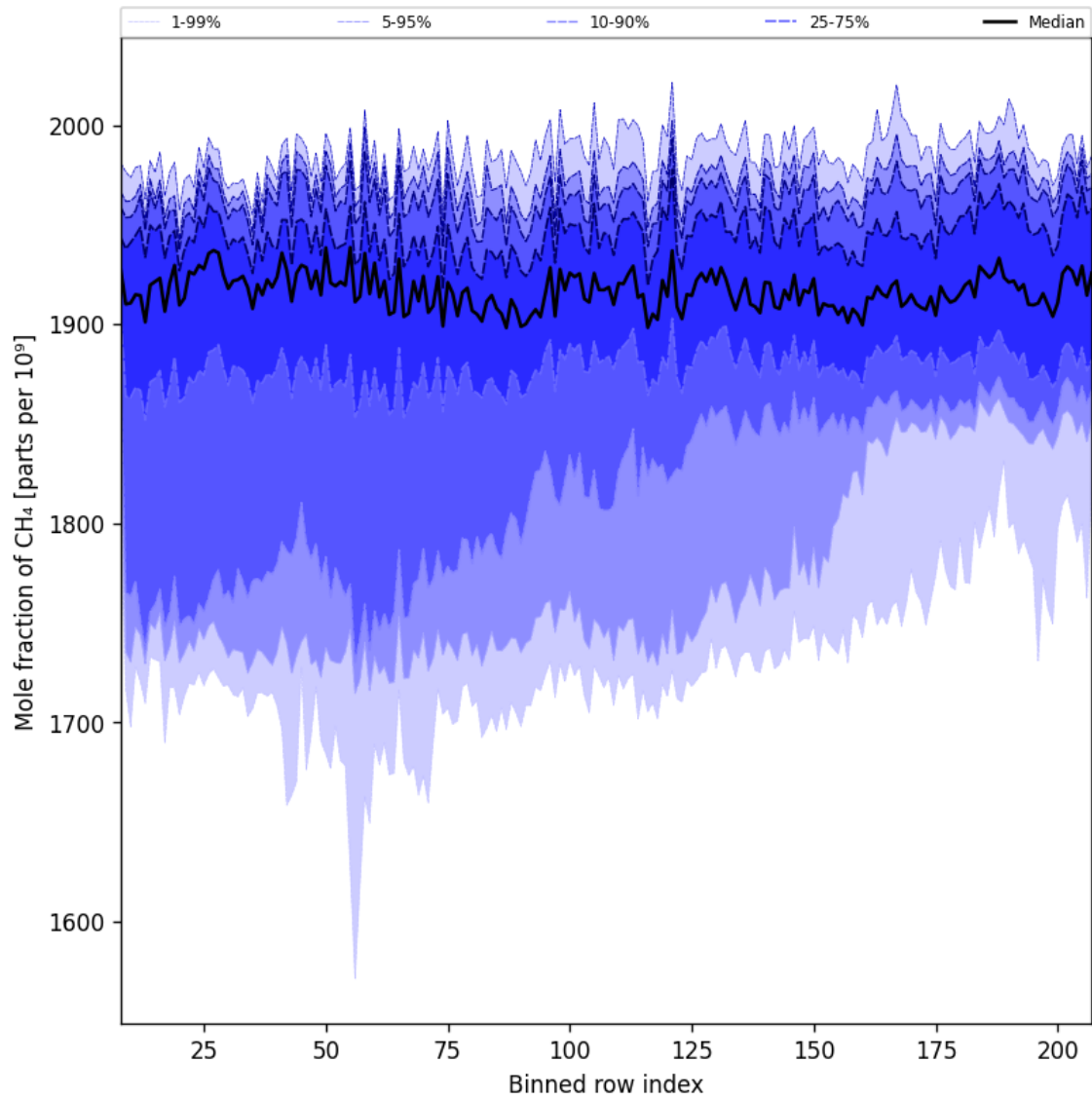
Figure 34: Along track statistics of “Mole fraction of CH 4 ” for 2025-10-08 to 2025-10-10
