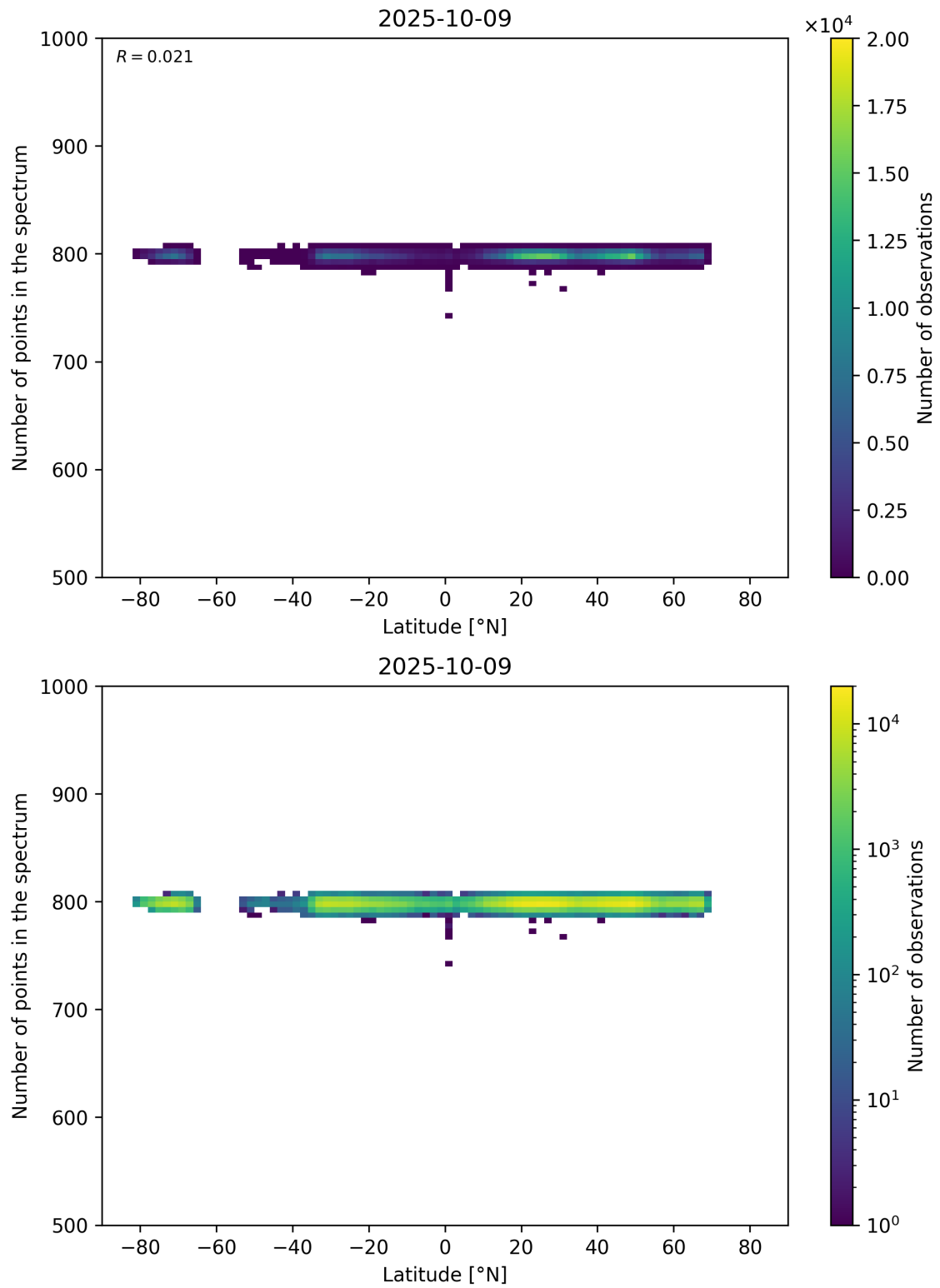
Figure 61: Scatter density plot of “Latitude” against “Number of points in the spectrum” for 2025-10-08 to 2025-10-10.
