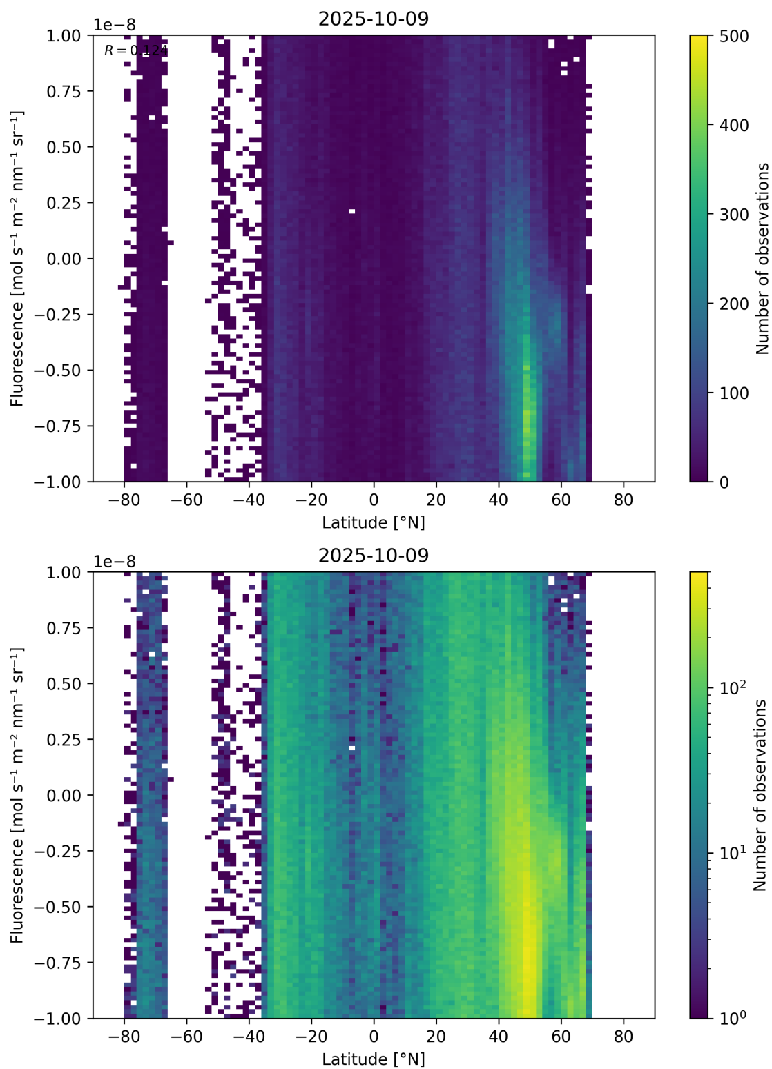
Figure 56: Scatter density plot of “Latitude” against “Fluorescence” for 2025-10-08 to 2025-10-10.
