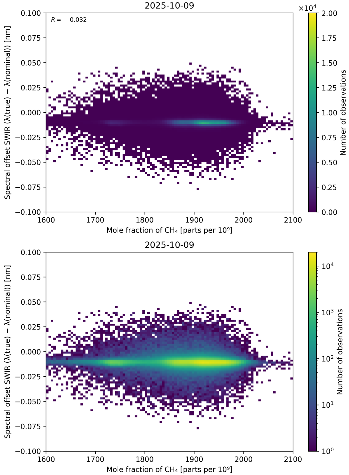
Figure 86: Scatter density plot of “Mole fraction of \text{CH}_4 ” against “Spectral offset SWIR ( \lambda_{\text{true}} - \lambda_{\text{nominal}} )” for 2025-10-08 to 2025-10-10.
