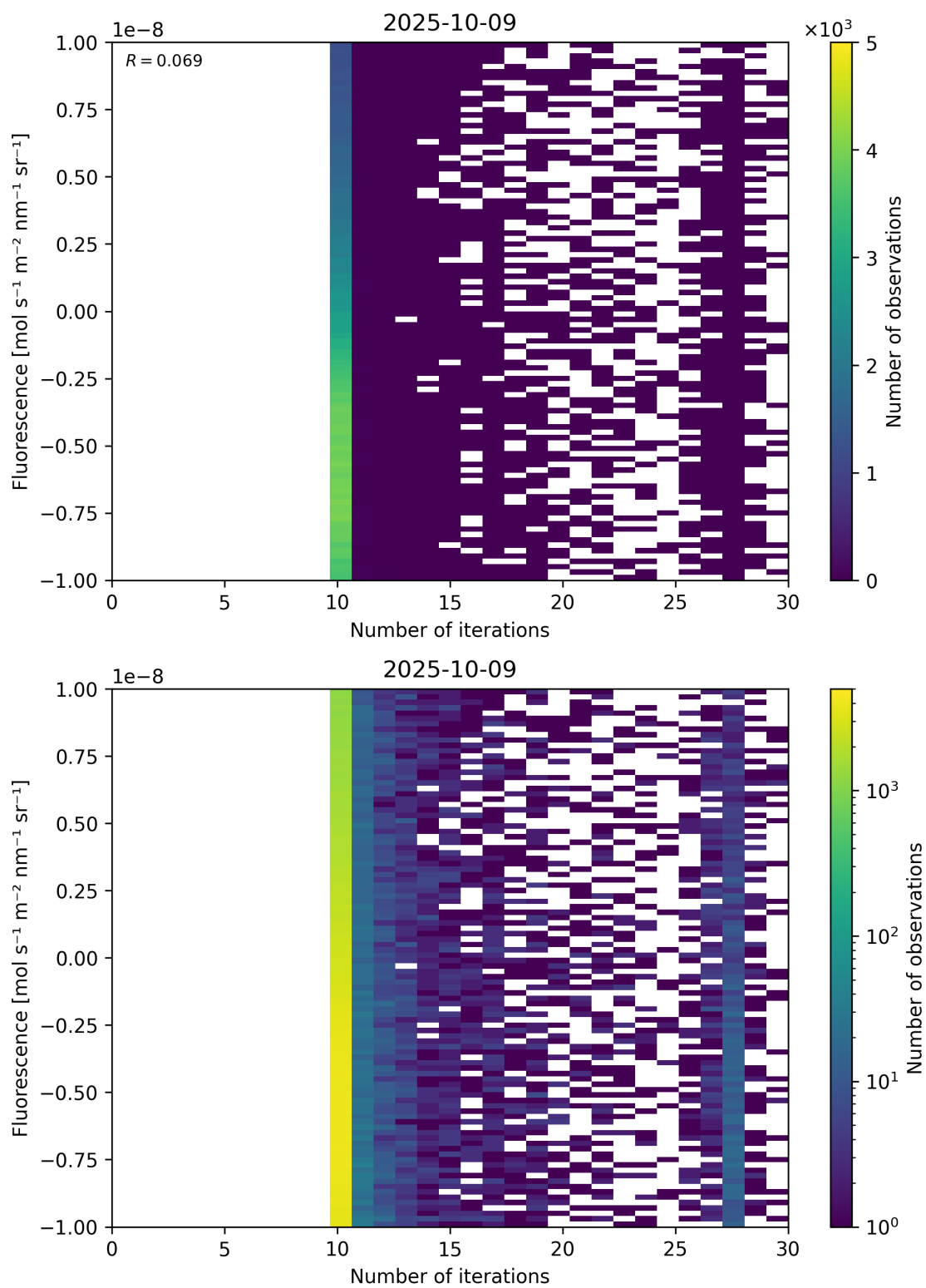
Figure 87: Scatter density plot of “Number of iterations” against “Fluorescence” for 2025-10-08 to 2025-10-10.
