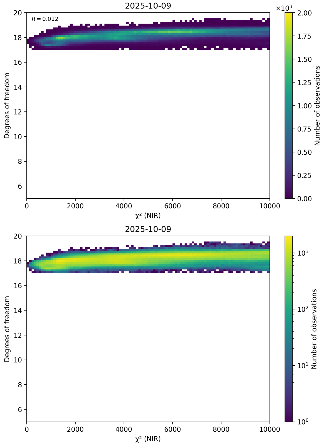
Figure 44: Scatter density plot of “ \chi^2 (NIR)” against “Degrees of freedom” for 2025-10-08 to 2025-10-10.
