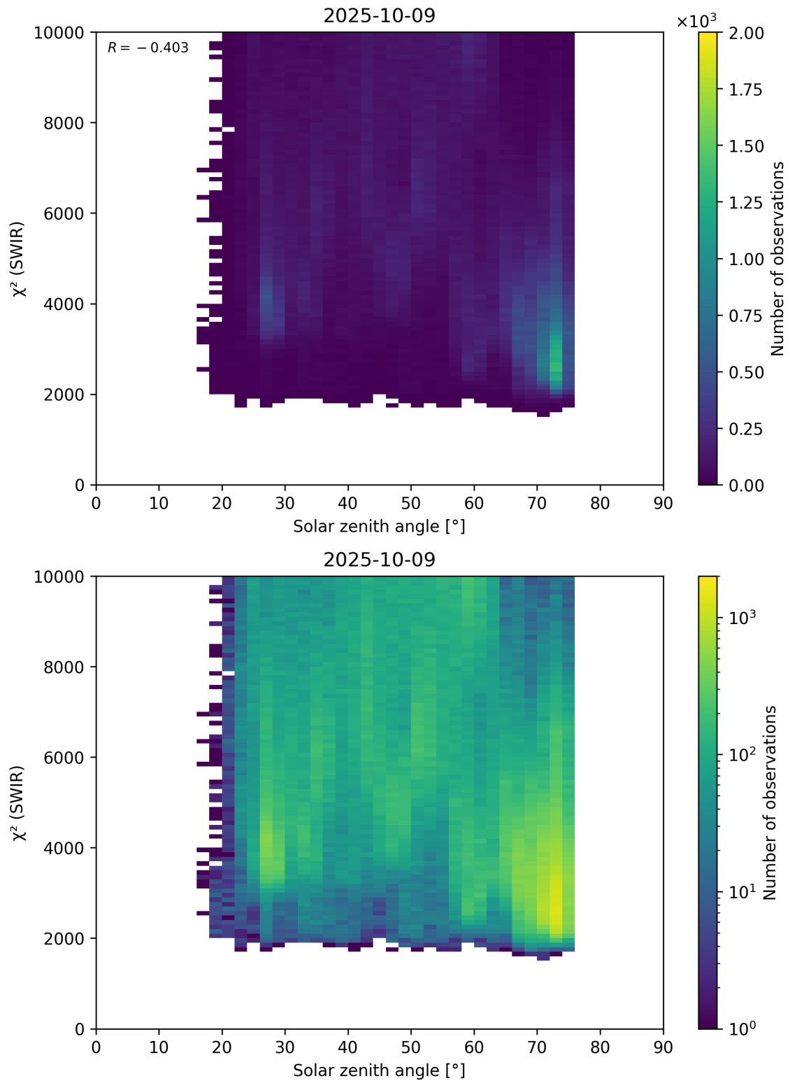
Figure 95: Scatter density plot of “Solar zenith angle” against “ \chi^2 (SWIR)” for 2025-10-08 to 2025-10-10.
