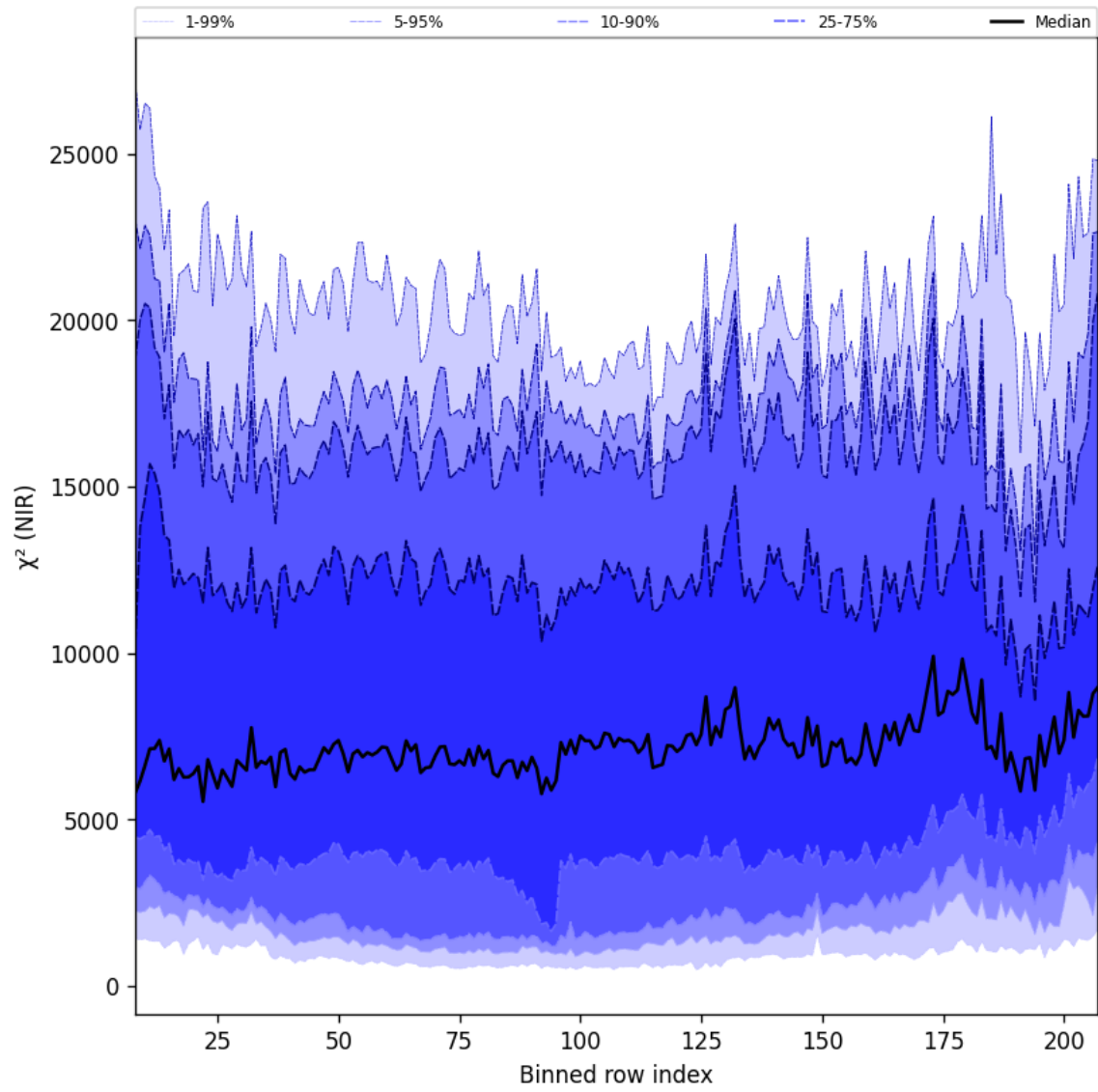
Figure 40: Along track statistics of “ \chi^2 (NIR)” for 2025-10-08 to 2025-10-10
