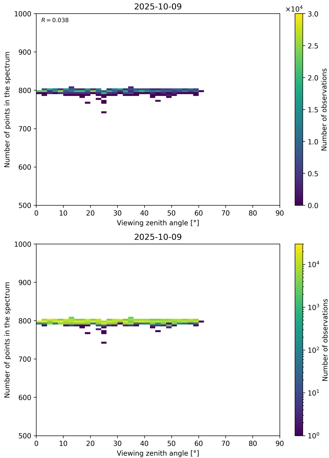
Figure 114: Scatter density plot of “Viewing zenith angle” against “Number of points in the spectrum” for 2025-10-08 to 2025-10-10.
