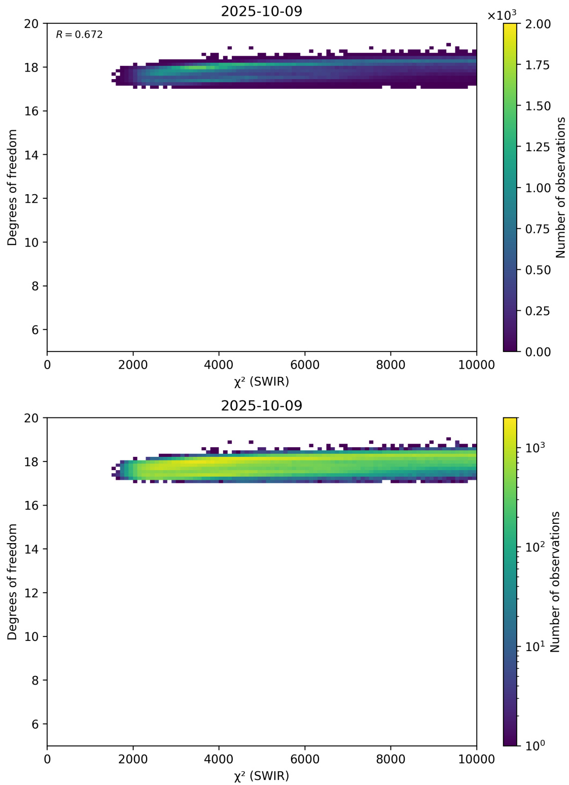
Figure 48: Scatter density plot of “ \chi^2 (SWIR)” against “Degrees of freedom” for 2025-10-08 to 2025-10-10.
