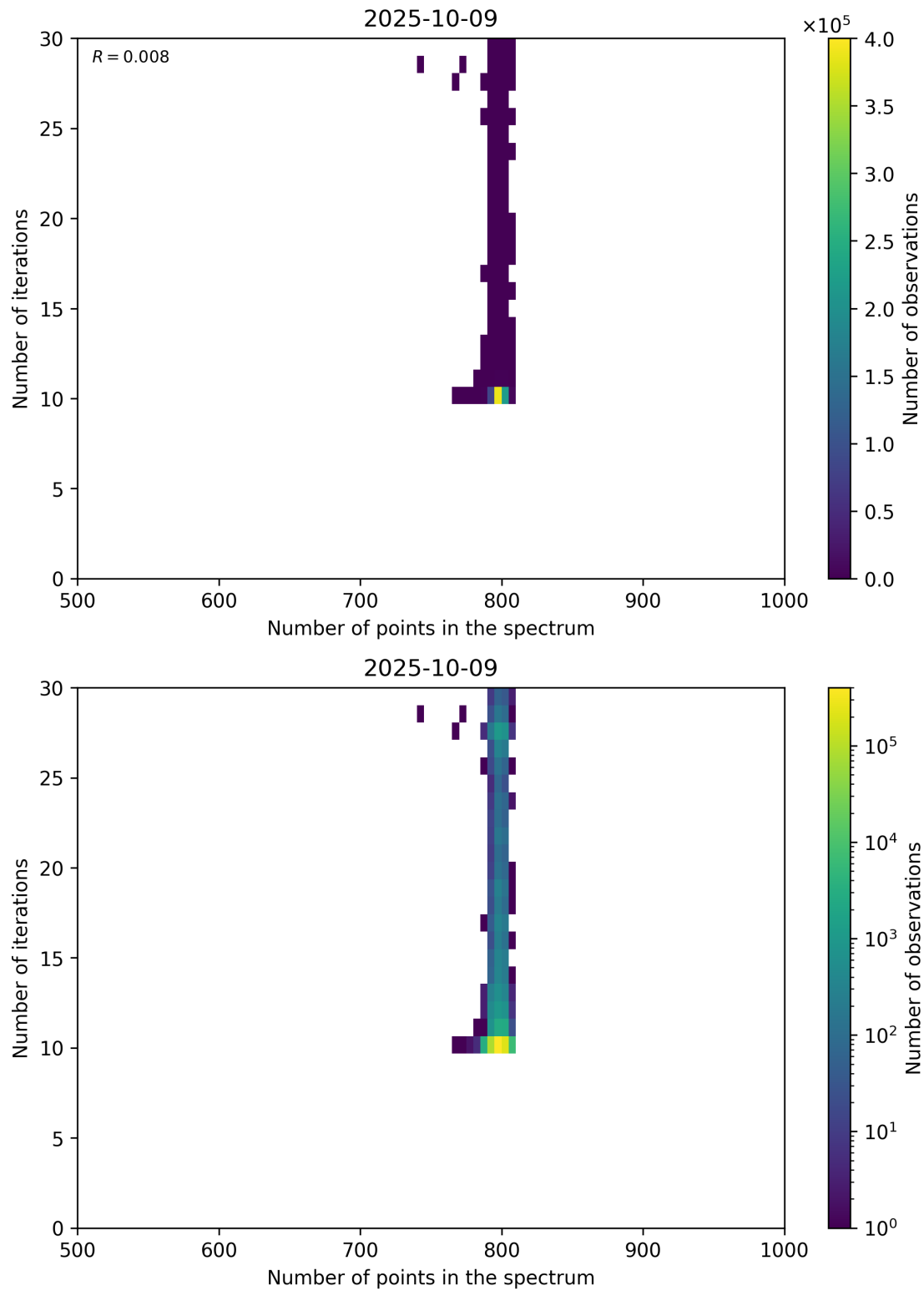
Figure 92: Scatter density plot of “Number of points in the spectrum” against “Number of iterations” for 2025-10-08 to 2025-10-10.
