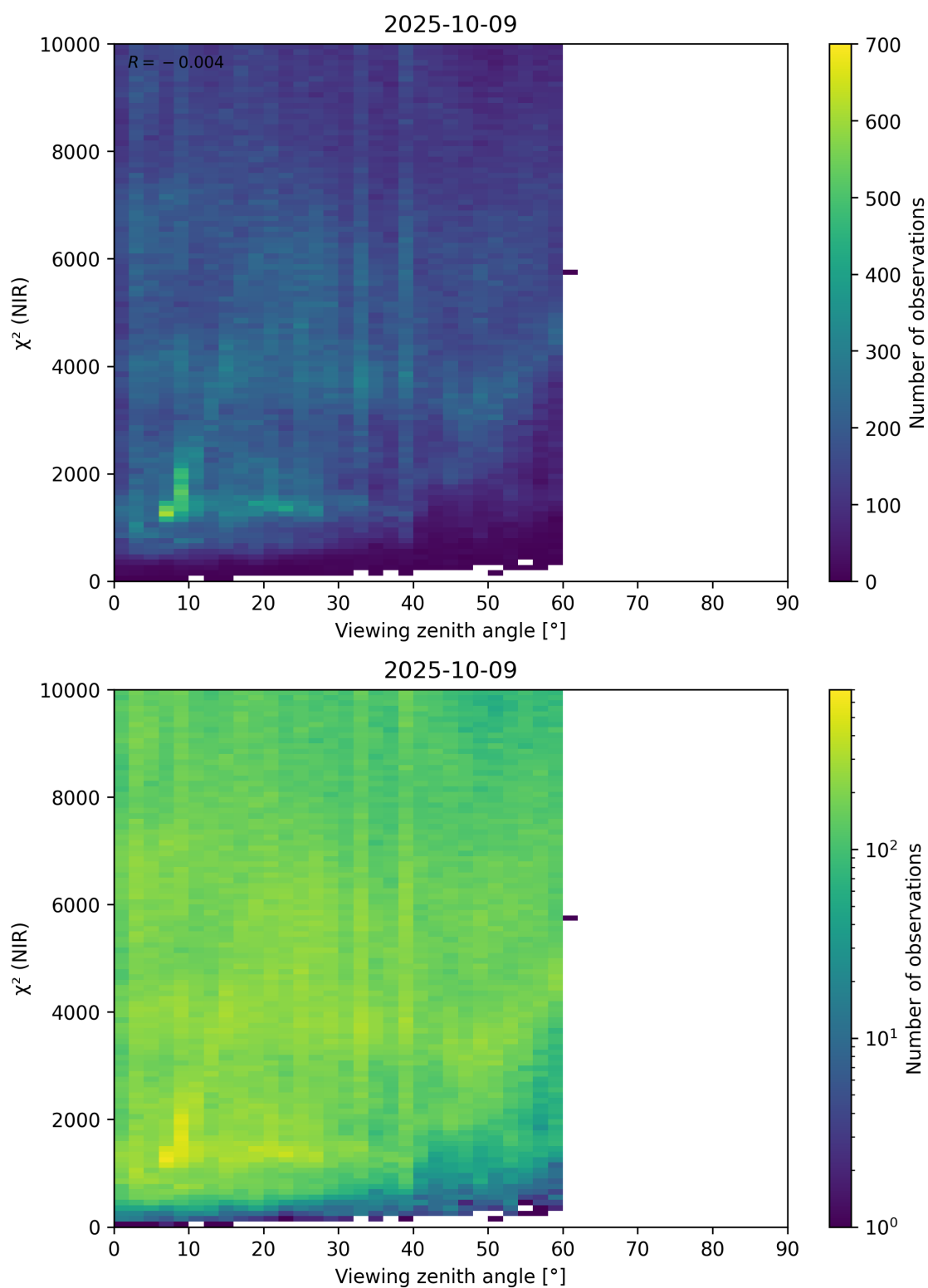
Figure 105: Scatter density plot of “Viewing zenith angle” against “ \chi^2 (NIR)” for 2025-10-08 to 2025-10-10.
