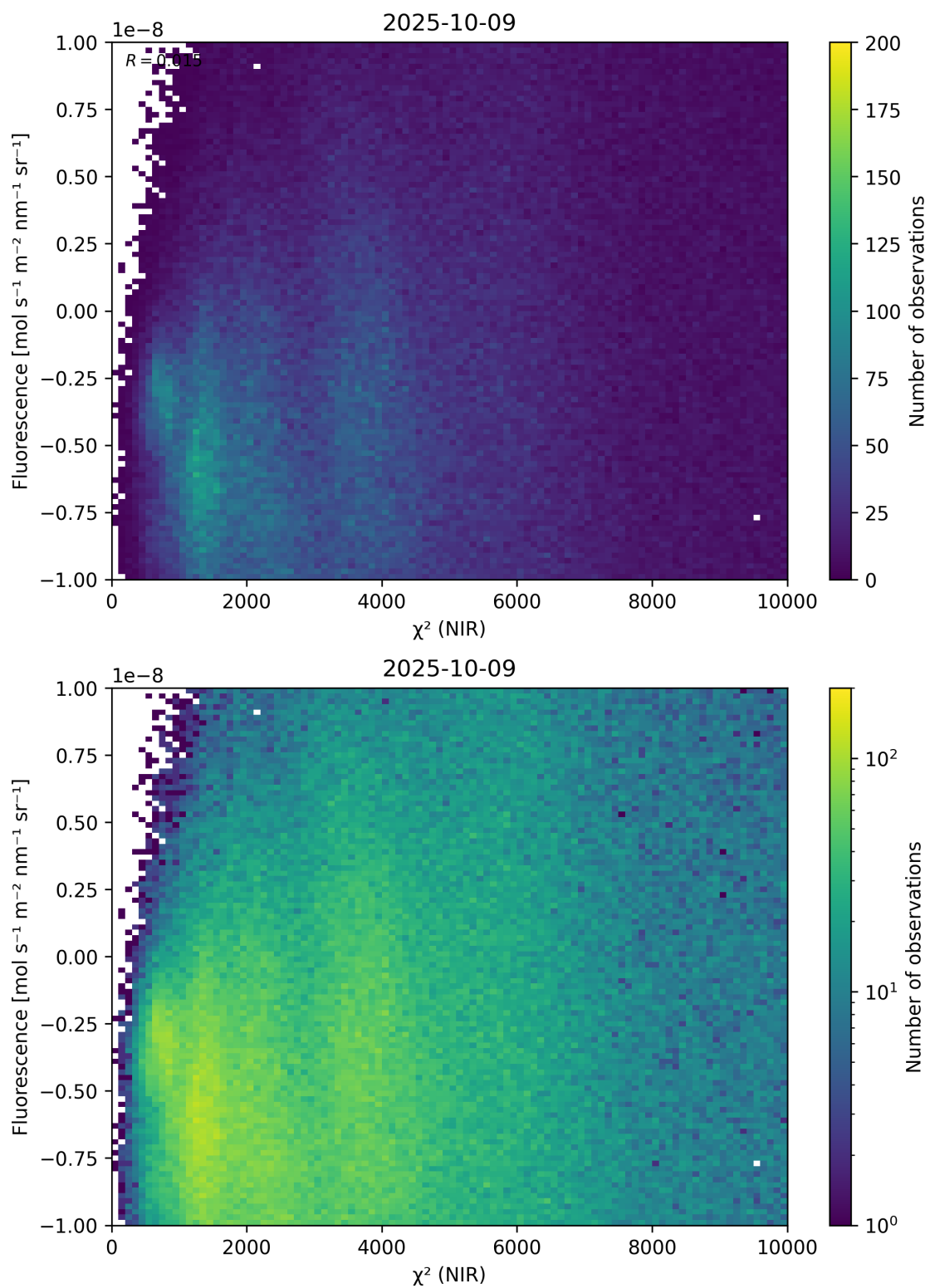
Figure 45: Scatter density plot of “ \chi^2 (NIR)” against “Fluorescence” for 2025-10-08 to 2025-10-10.
