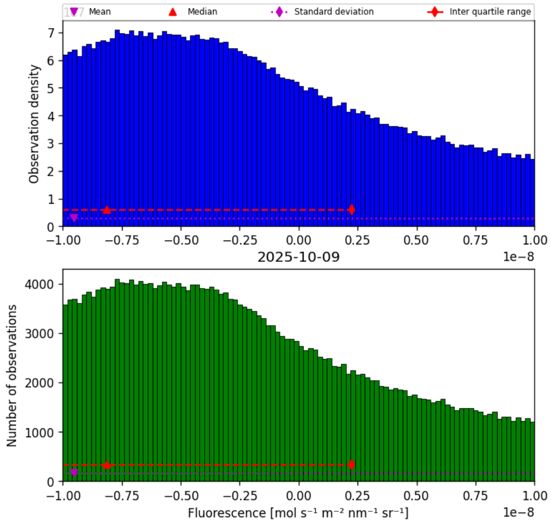
Figure 32: Histogram of “Fluorescence” for 2025-10-08 to 2025-10-10
