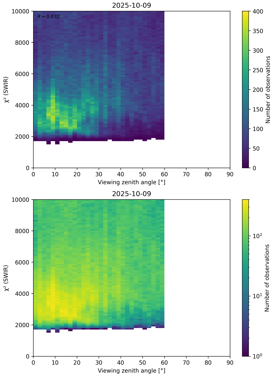
Figure 106: Scatter density plot of “Viewing zenith angle” against “ \chi^2 (SWIR)” for 2025-10-08 to 2025-10-10.
