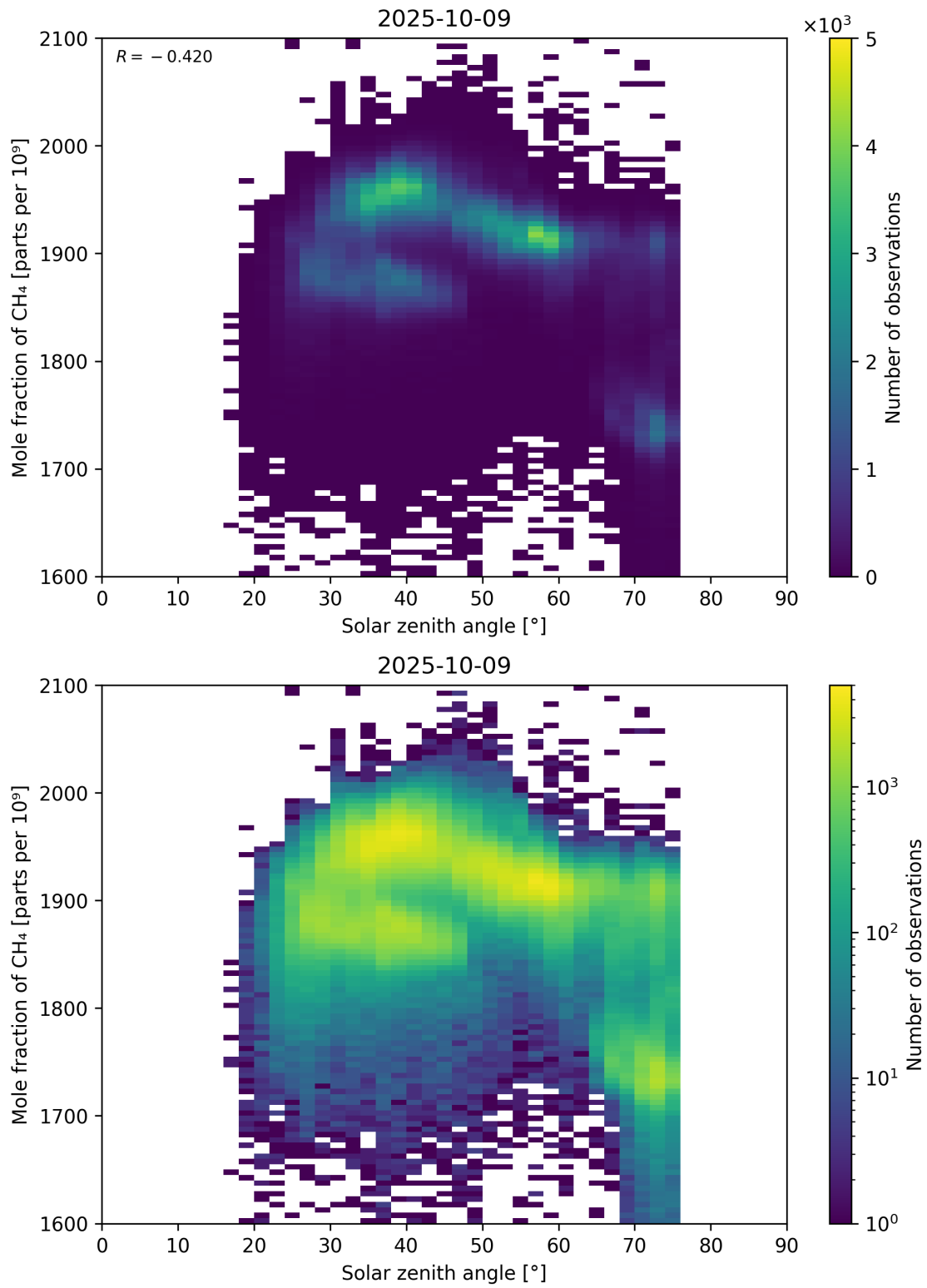
Figure 99: Scatter density plot of “Solar zenith angle” against “Mole fraction of \text{CH}_4 ” for 2025-10-08 to 2025-10-10.
