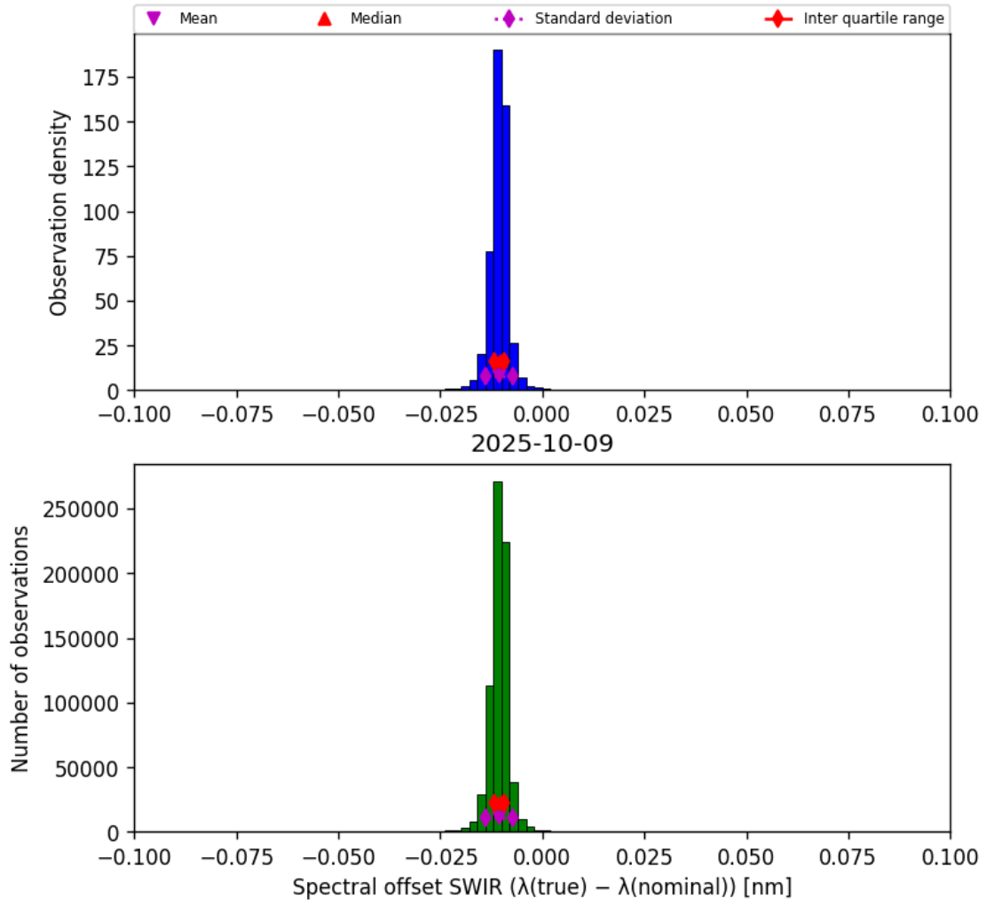
Figure 27: Histogram of “Spectral offset SWIR ( \lambda_{\text{true}} - \lambda_{\text{nominal}} )” for 2025-10-08 to 2025-10-10
