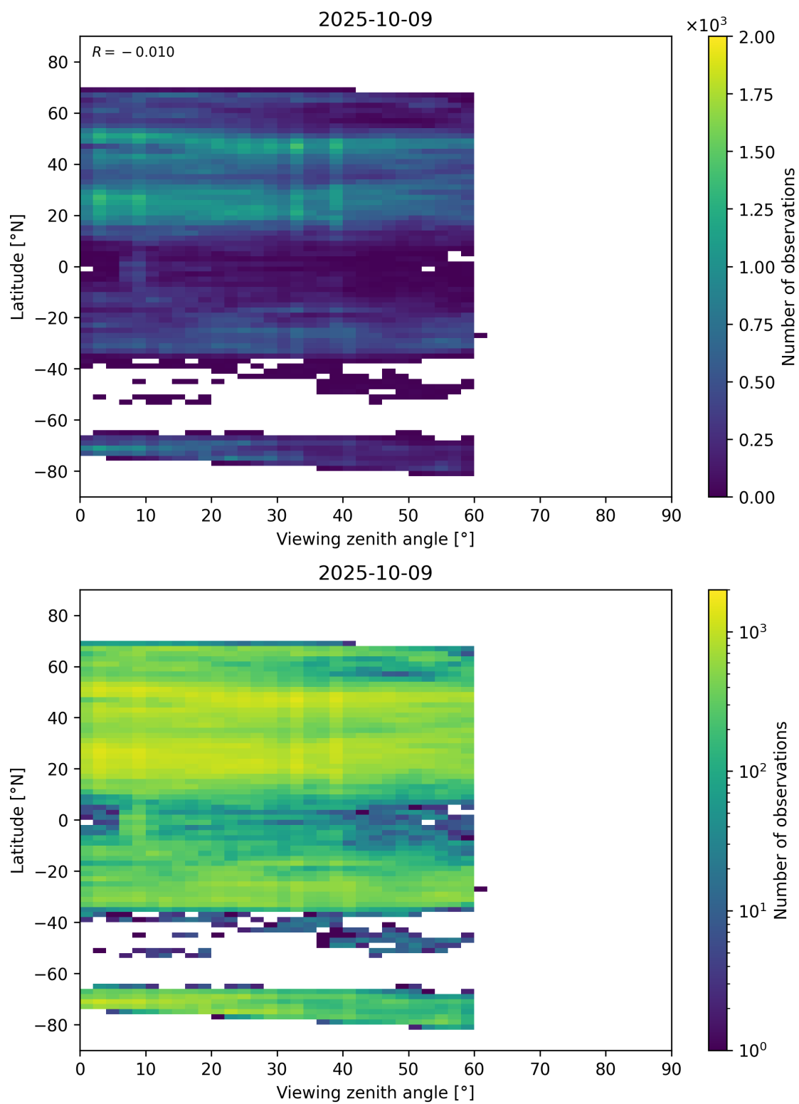
Figure 109: Scatter density plot of “Viewing zenith angle” against “Latitude” for 2025-10-08 to 2025-10-10.
