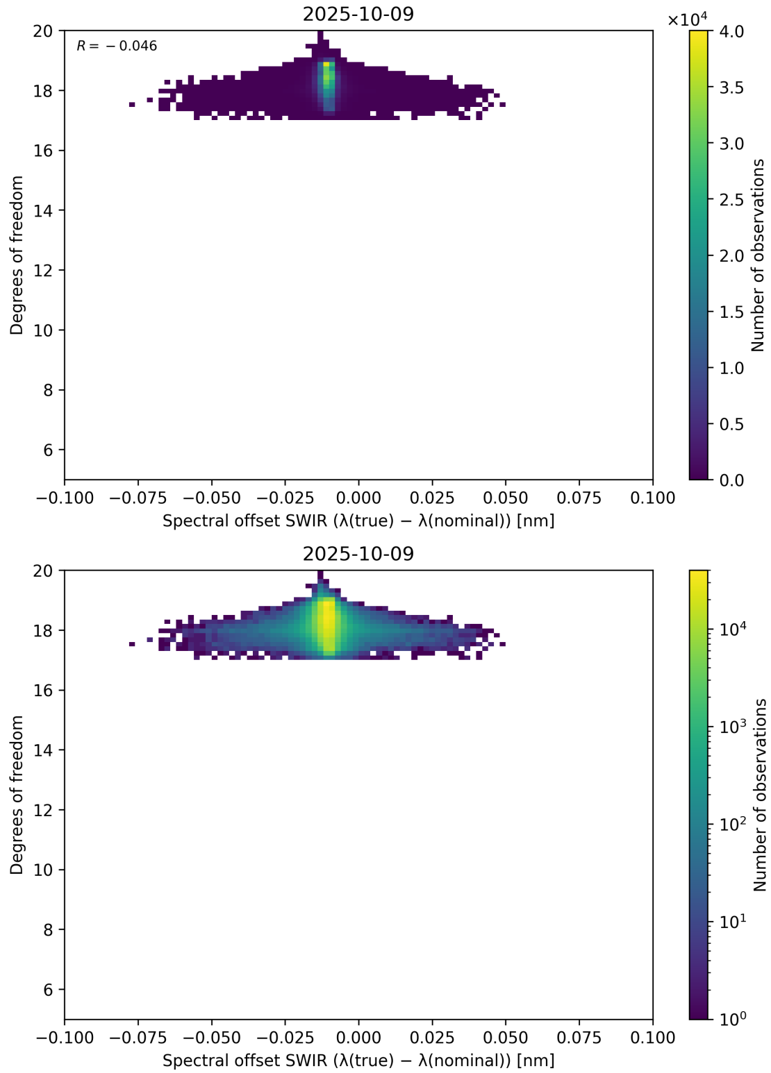
Figure 119: Scatter density plot of “Spectral offset SWIR ( \lambda_{\text{true}} - \lambda_{\text{nominal}} )” against “Degrees of freedom” for 2025-10-08 to 2025-10-10.
