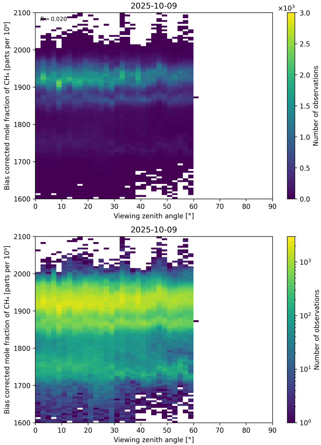
Figure 111: Scatter density plot of “Viewing zenith angle” against “Bias corrected mole fraction of CH 4 ” for 2025-10-08 to 2025-10-10.
