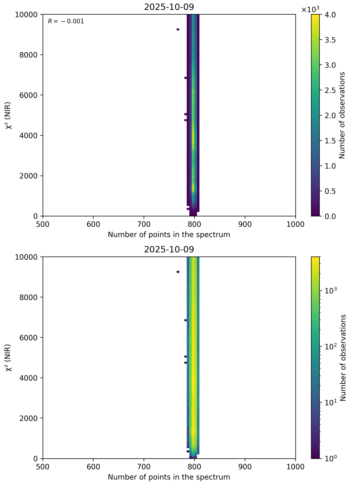
Figure 88: Scatter density plot of “Number of points in the spectrum” against “ \chi^2 (NIR)” for 2025-10-08 to 2025-10-10.
