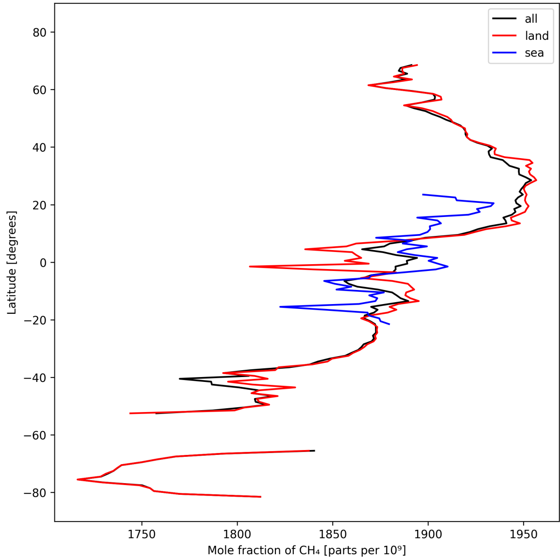
Figure 12: Zonal average of “Mole fraction of \text{CH}_4 ” for 2025-10-08 to 2025-10-10.
