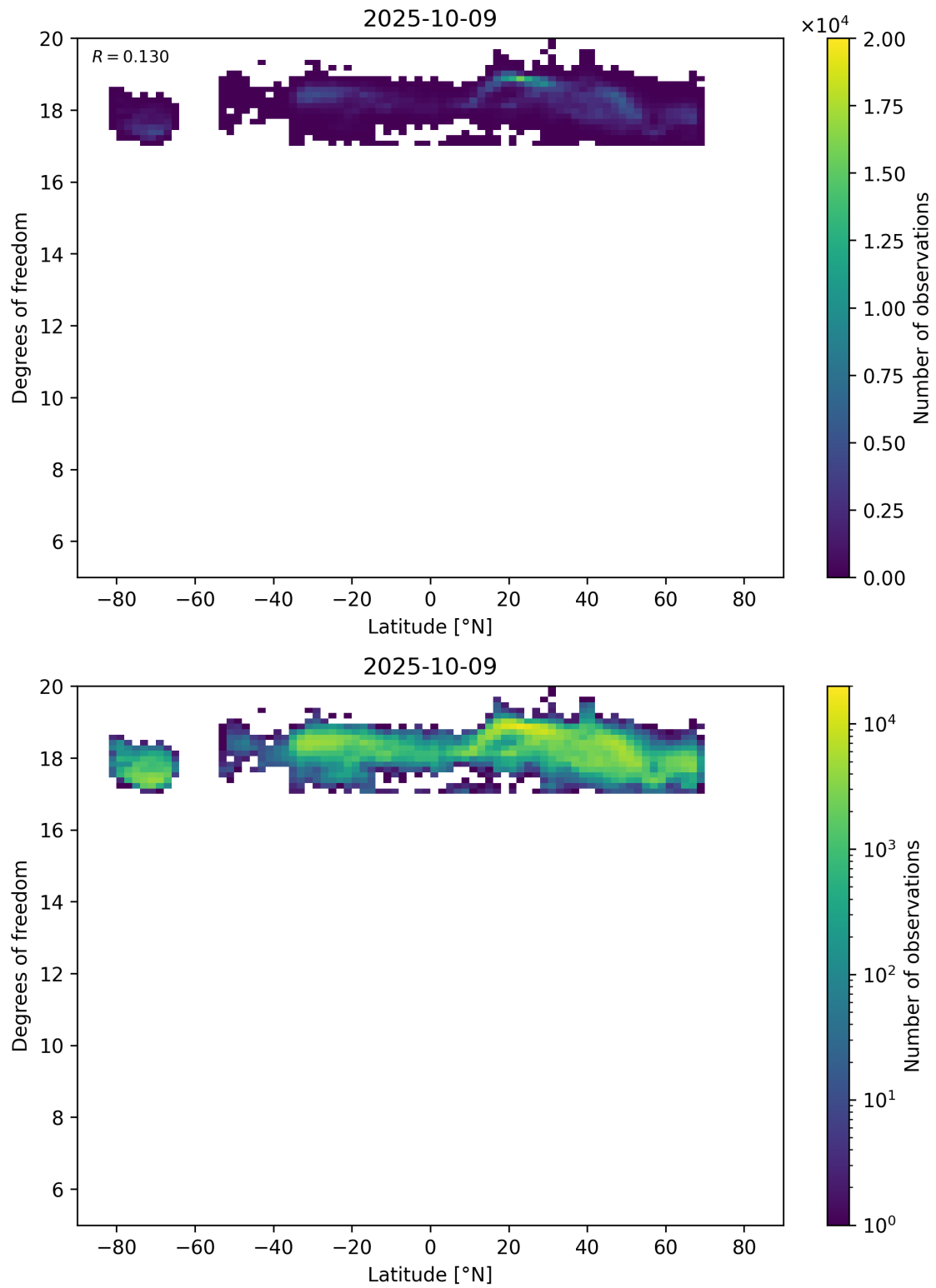
Figure 55: Scatter density plot of “Latitude” against “Degrees of freedom” for 2025-10-08 to 2025-10-10.
