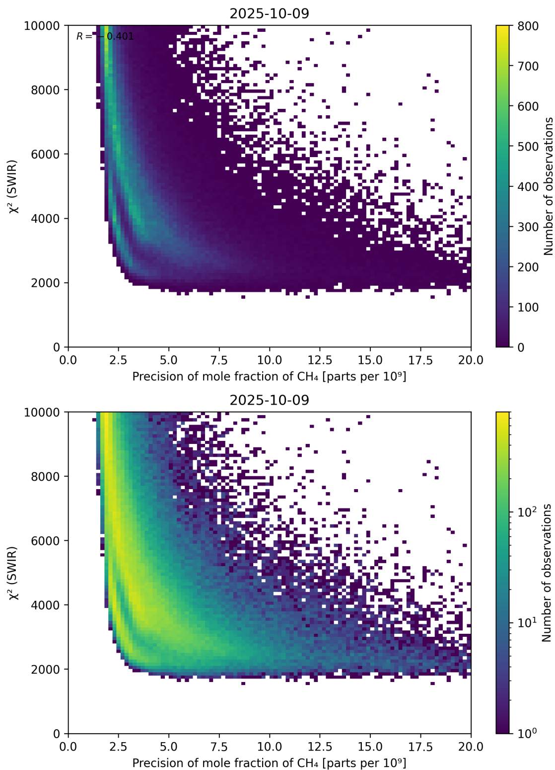
Figure 79: Scatter density plot of “Precision of mole fraction of CH 4 ” against “ \chi^2 (SWIR)” for 2025-10-08 to 2025-10-10.
