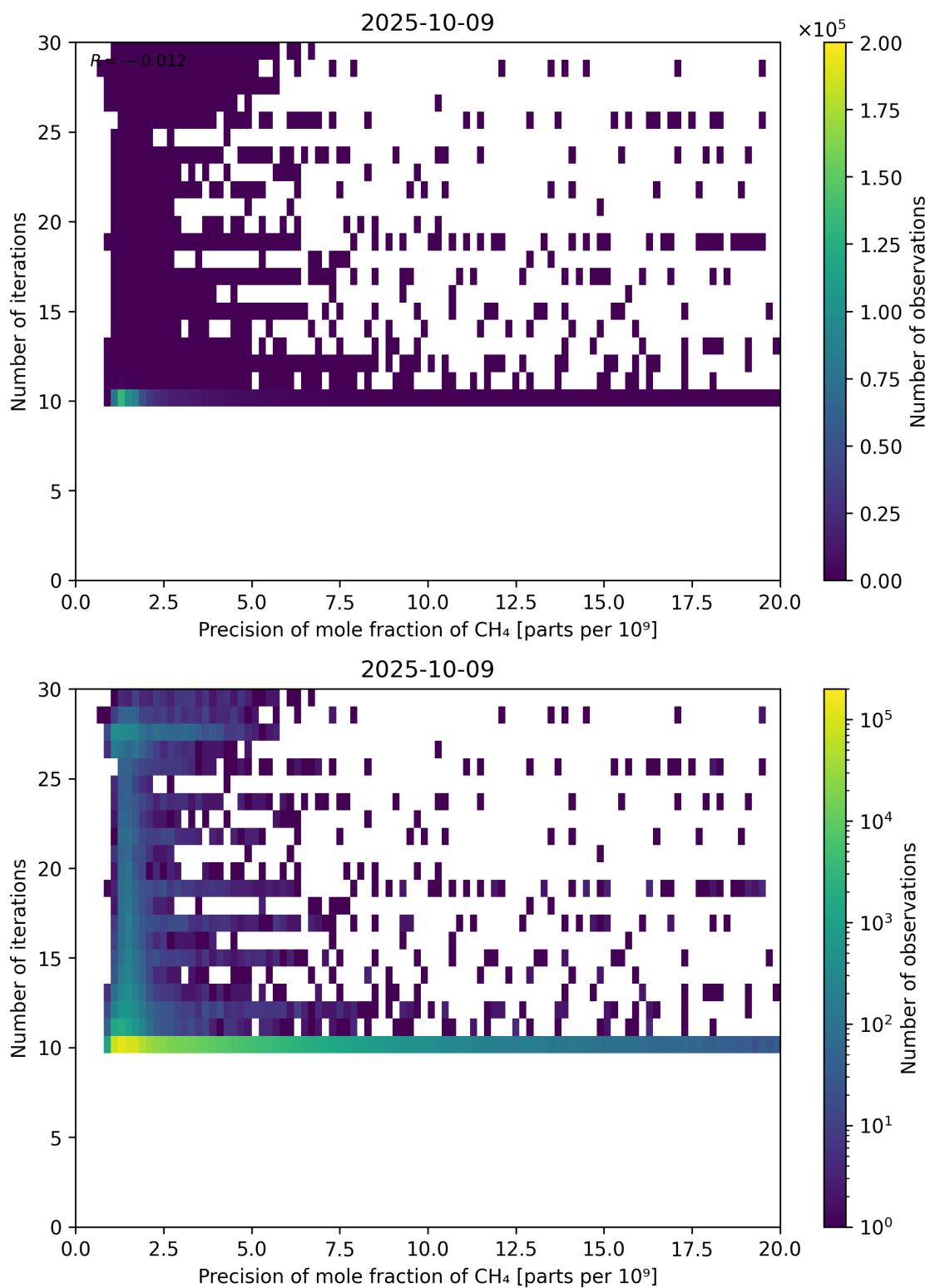
Figure 83: Scatter density plot of “Precision of mole fraction of CH 4 ” against “Number of iterations” for 2025-10-08 to 2025-10-10.
