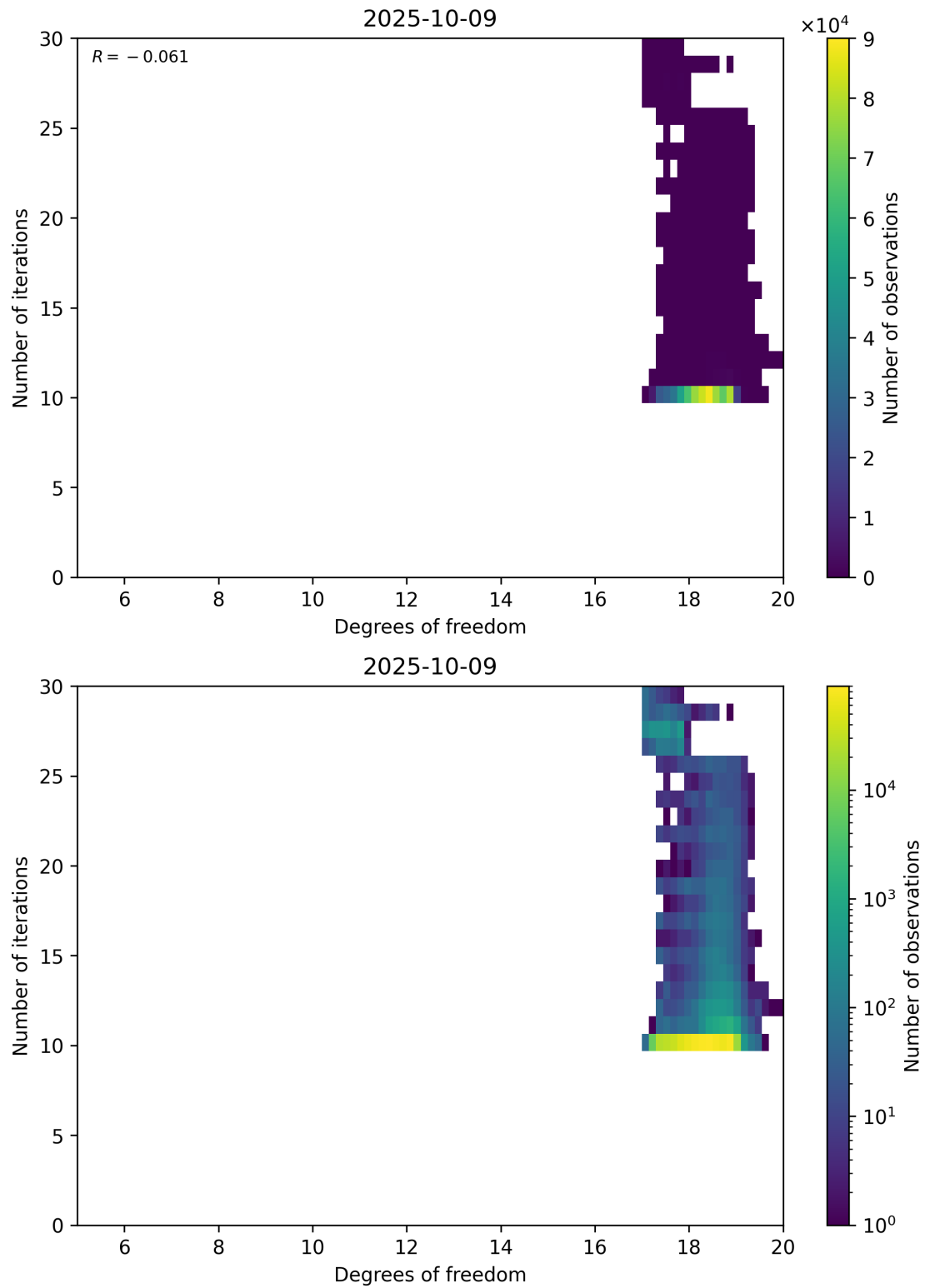
Figure 52: Scatter density plot of “Degrees of freedom” against “Number of iterations” for 2025-10-08 to 2025-10-10.
