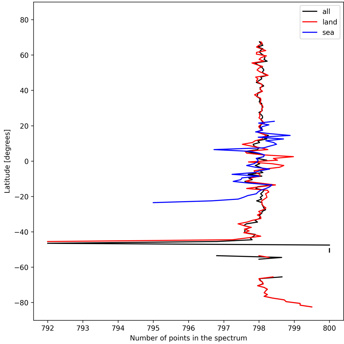
Figure 15: Zonal average of “Number of points in the spectrum” for 2025-10-11 to 2025-10-13.
