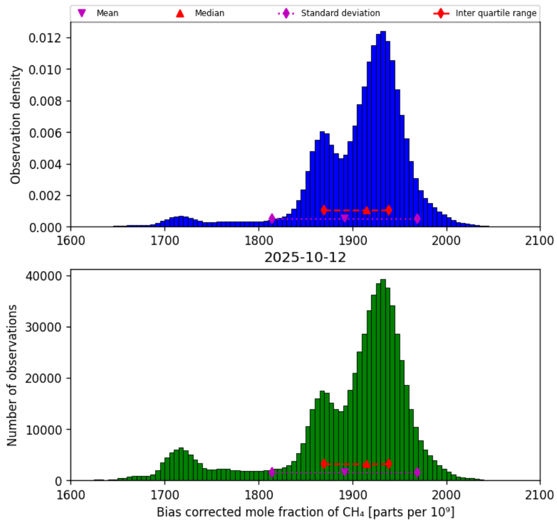
Figure 25: Histogram of “Bias corrected mole fraction of CH 4 ” for 2025-10-11 to 2025-10-13
