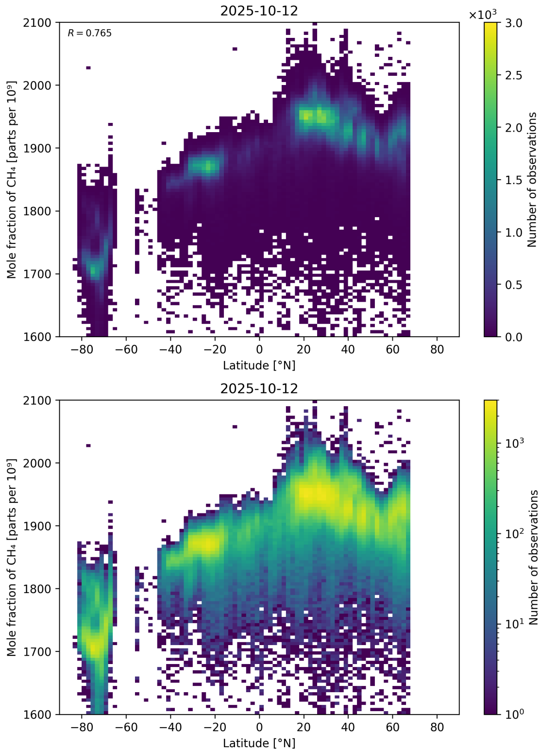
Figure 57: Scatter density plot of “Latitude” against “Mole fraction of \text{CH}_4 ” for 2025-10-11 to 2025-10-13.
