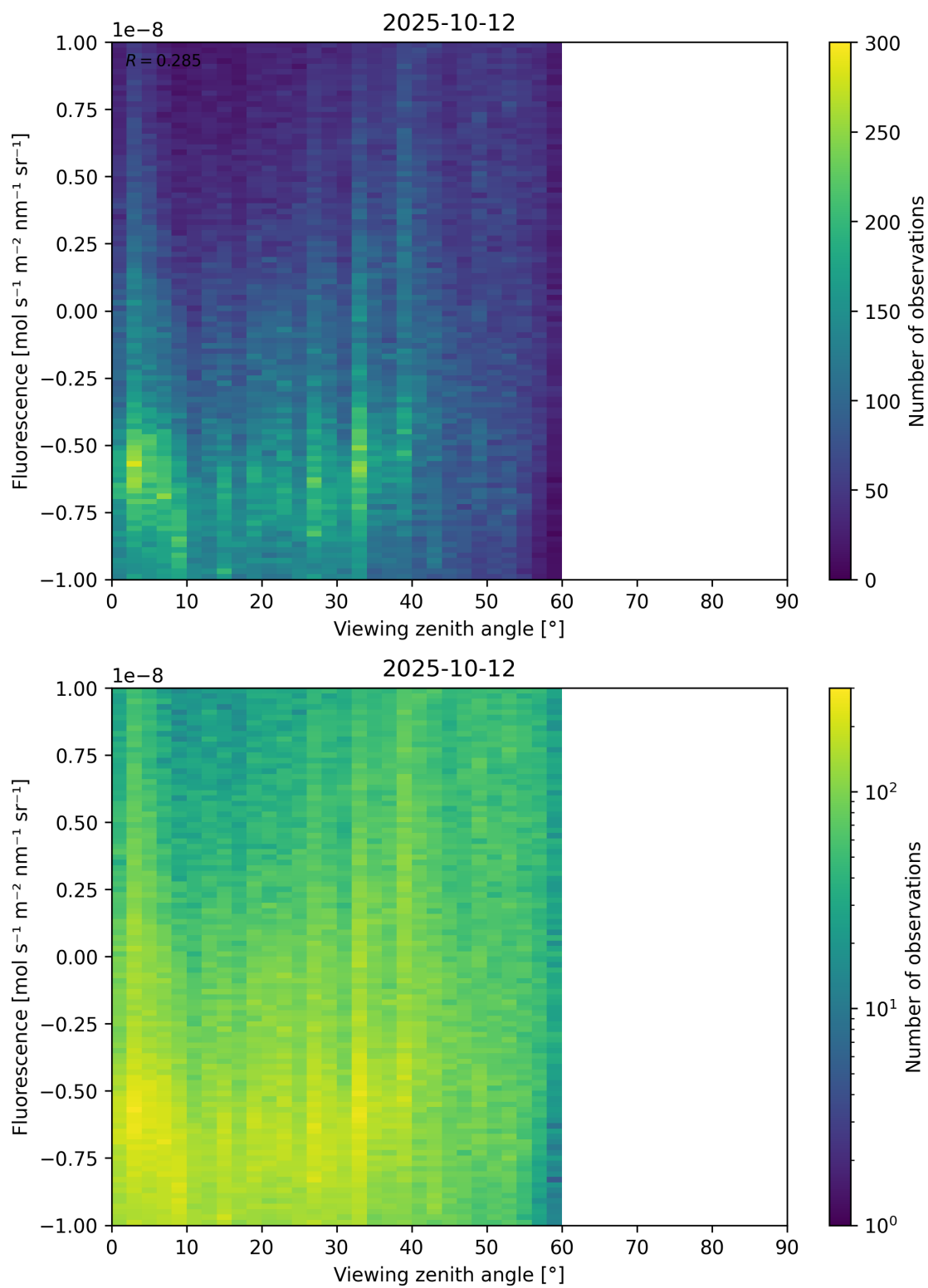
Figure 108: Scatter density plot of “Viewing zenith angle” against “Fluorescence” for 2025-10-11 to 2025-10-13.
