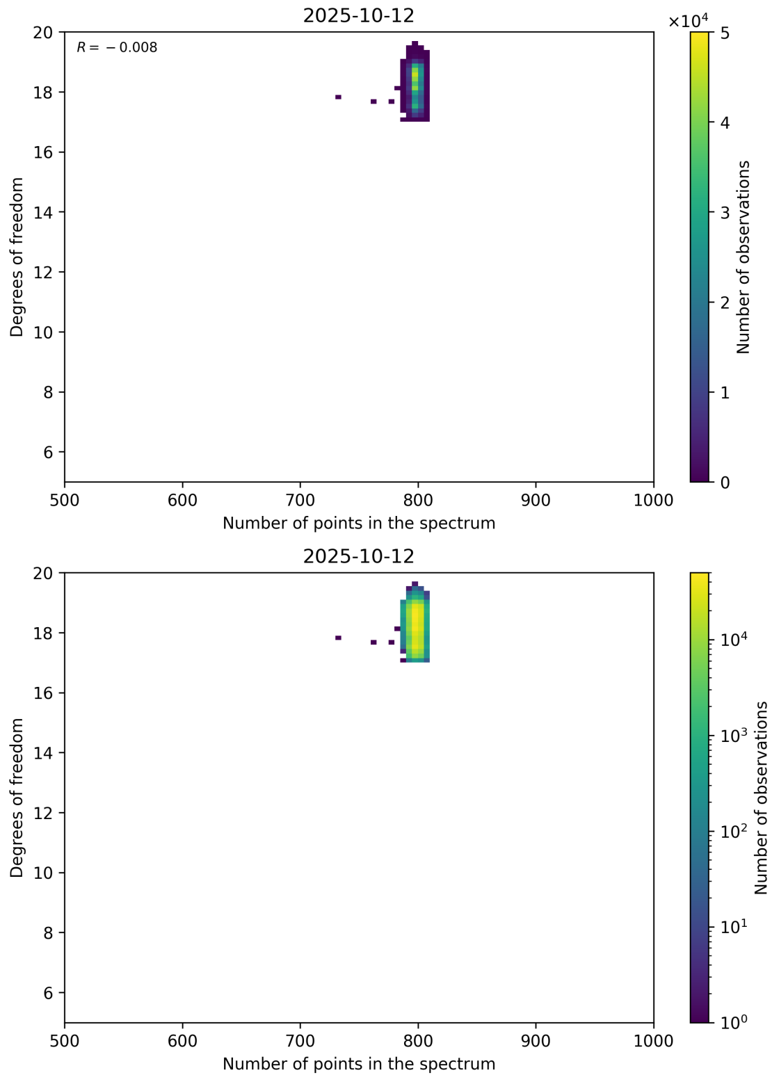
Figure 90: Scatter density plot of “Number of points in the spectrum” against “Degrees of freedom” for 2025-10-11 to 2025-10-13.
