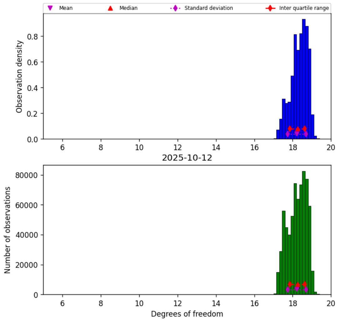
Figure 30: Histogram of “Degrees of freedom” for 2025-10-11 to 2025-10-13
