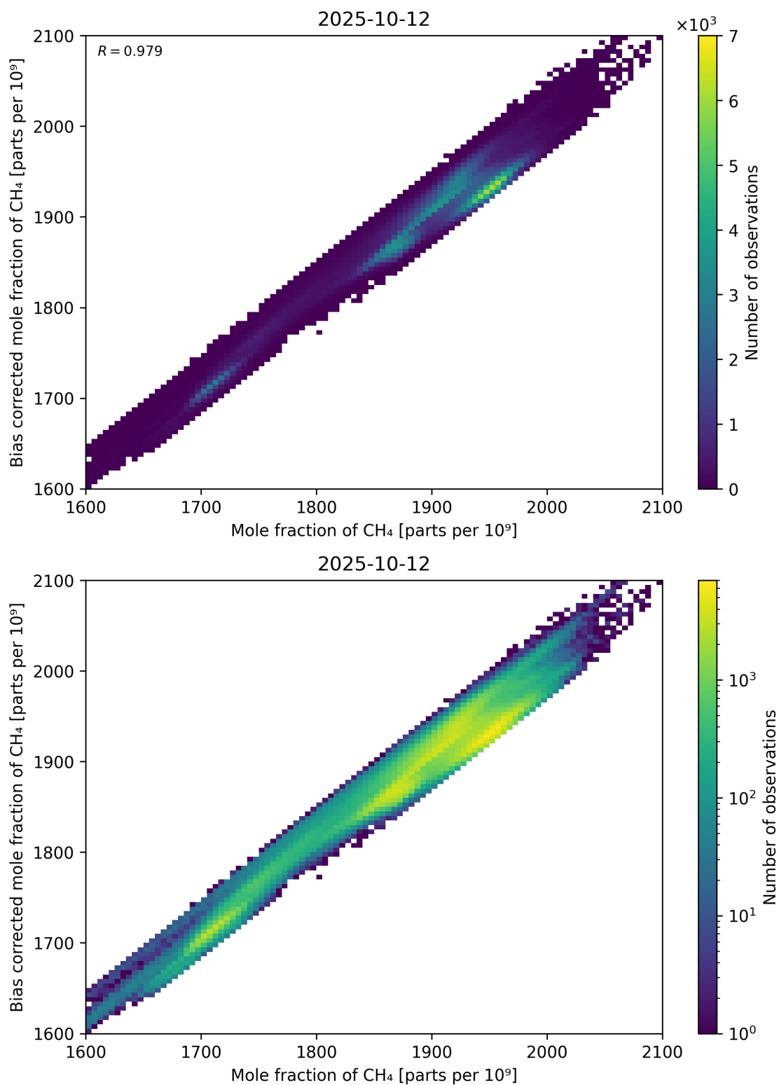
Figure 74: Scatter density plot of “Mole fraction of CH 4 ” against “Bias corrected mole fraction of CH 4 ” for 2025-10-11 to 2025-10-13.
