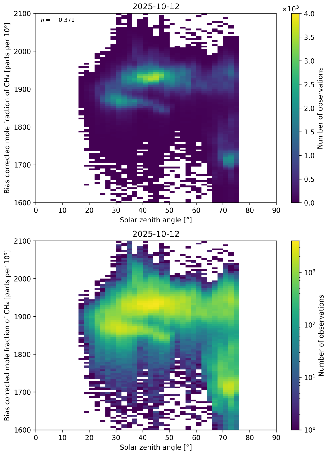
Figure 100: Scatter density plot of “Solar zenith angle” against “Bias corrected mole fraction of CH 4 ” for 2025-10-11 to 2025-10-13.
