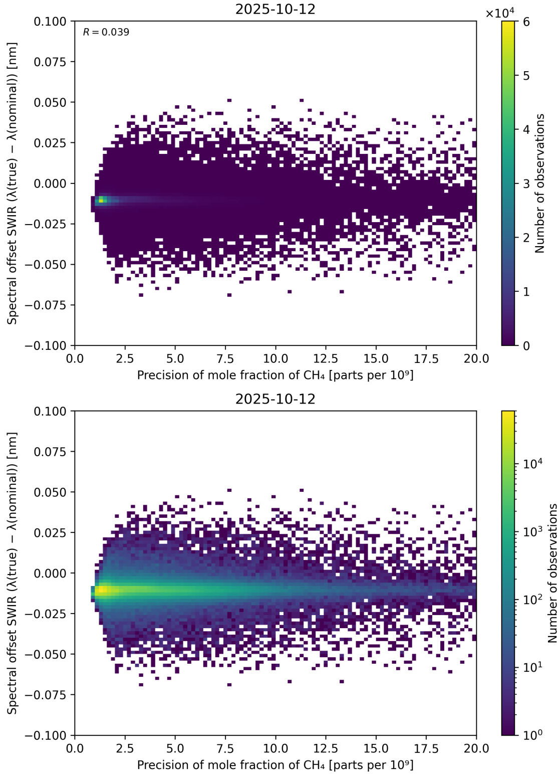
Figure 85: Scatter density plot of “Precision of mole fraction of \text{CH}_4 ” against “Spectral offset SWIR ( \lambda_{\text{true}} - \lambda_{\text{nominal}} )” for 2025-10-11 to 2025-10-13.
