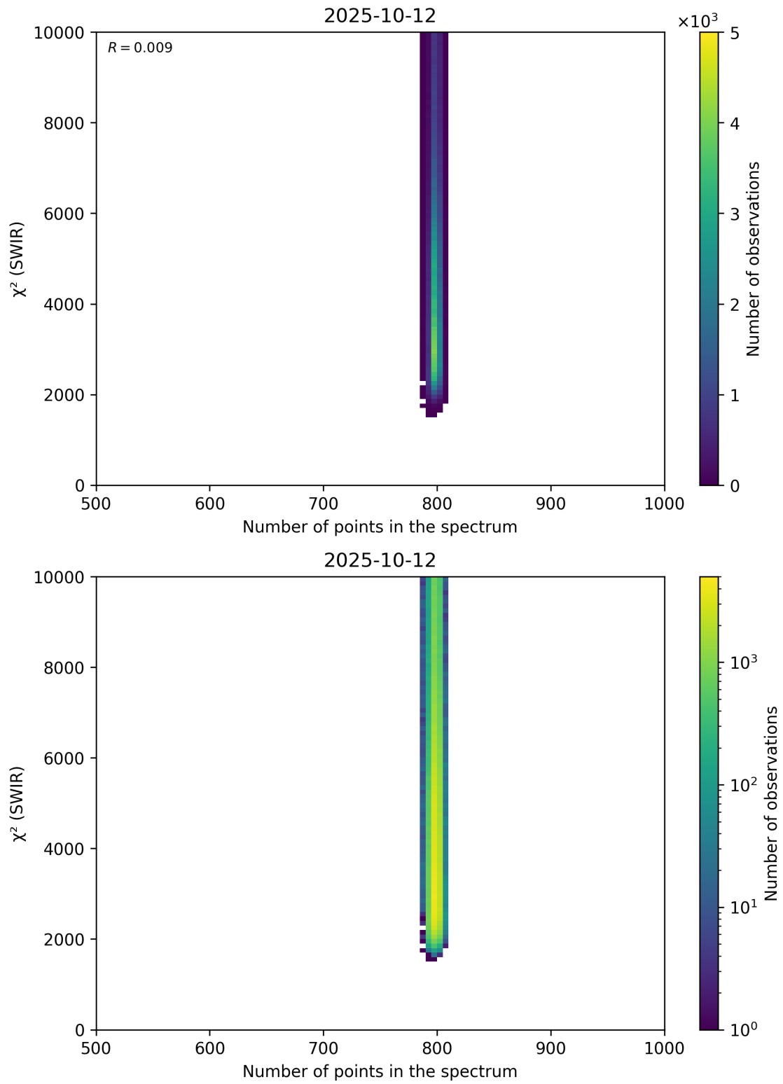
Figure 89: Scatter density plot of “Number of points in the spectrum” against “ \chi^2 (SWIR)” for 2025-10-11 to 2025-10-13.
