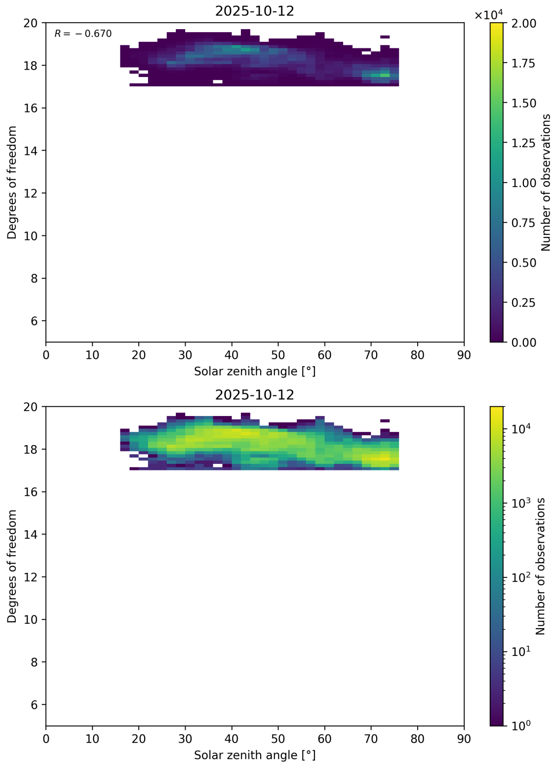
Figure 96: Scatter density plot of “Solar zenith angle” against “Degrees of freedom” for 2025-10-11 to 2025-10-13.
