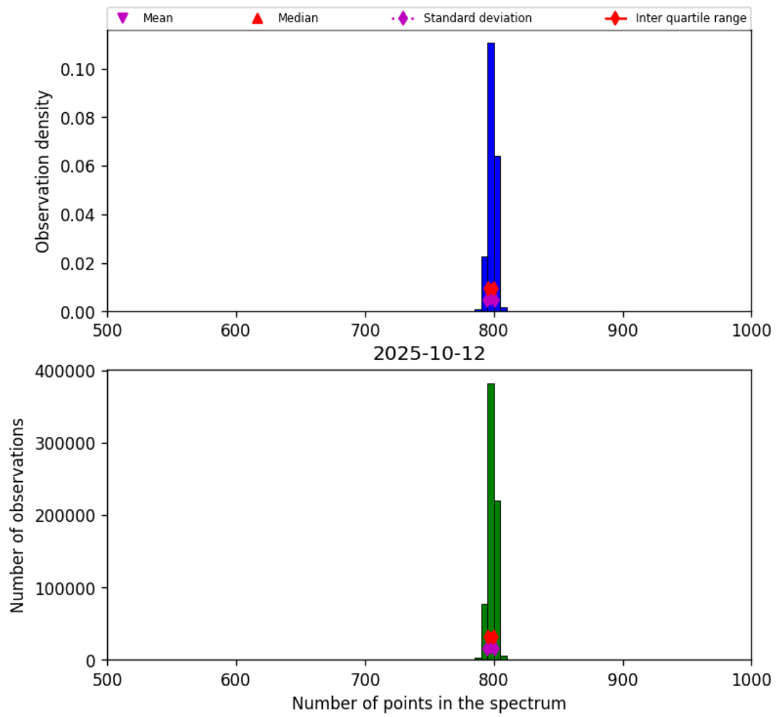
Figure 26: Histogram of “Number of points in the spectrum” for 2025-10-11 to 2025-10-13
