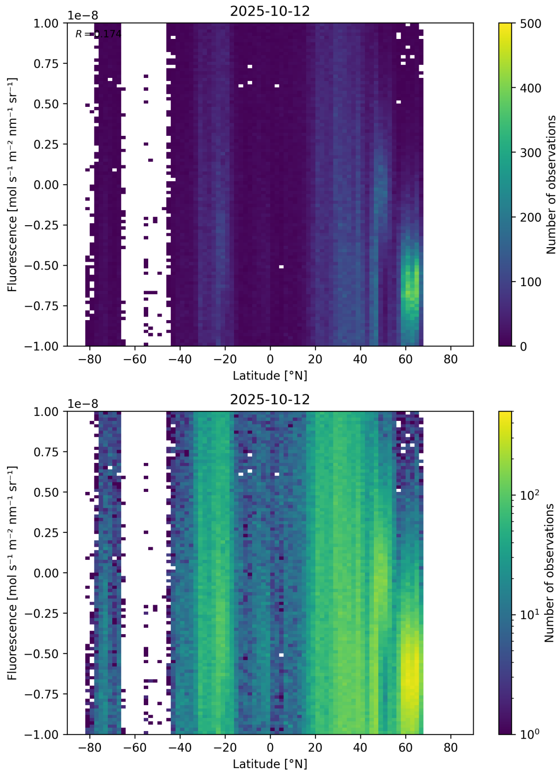
Figure 56: Scatter density plot of “Latitude” against “Fluorescence” for 2025-10-11 to 2025-10-13.
