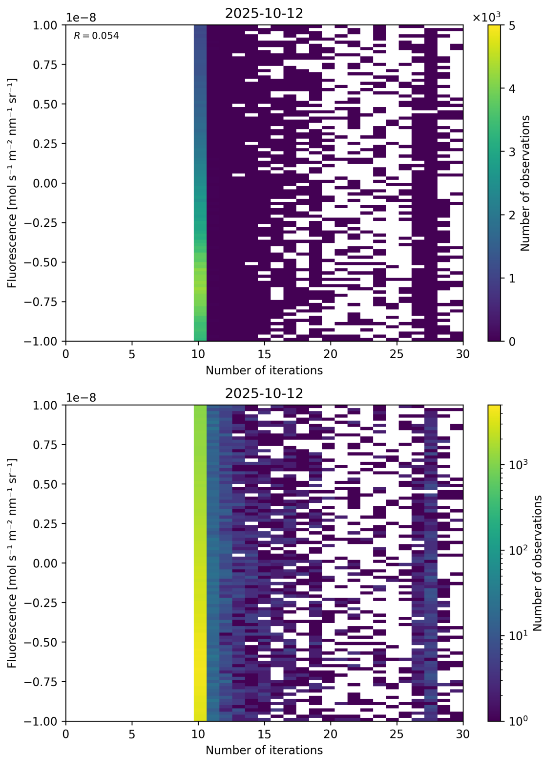
Figure 87: Scatter density plot of “Number of iterations” against “Fluorescence” for 2025-10-11 to 2025-10-13.
