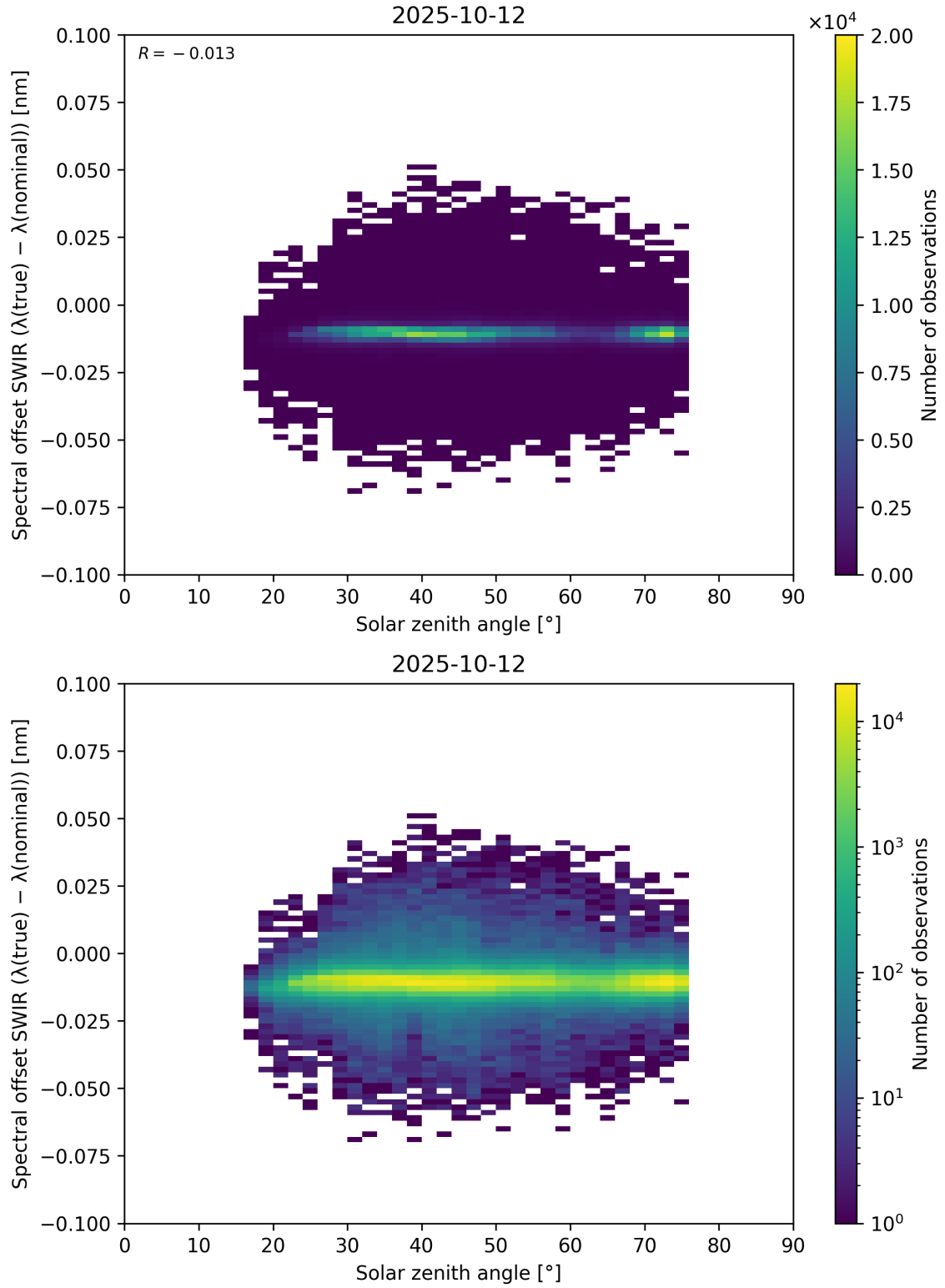
Figure 104: Scatter density plot of “Solar zenith angle” against “Spectral offset SWIR ( \lambda_{\text{true}} - \lambda_{\text{nominal}} )” for 2025-10-11 to 2025-10-13.
