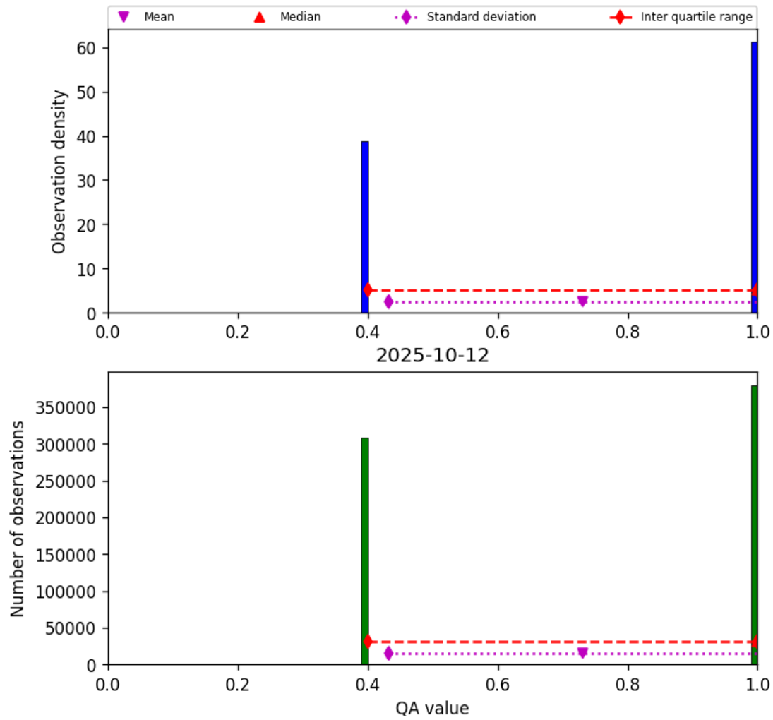
Figure 22: Histogram of “QA value” for 2025-10-11 to 2025-10-13
