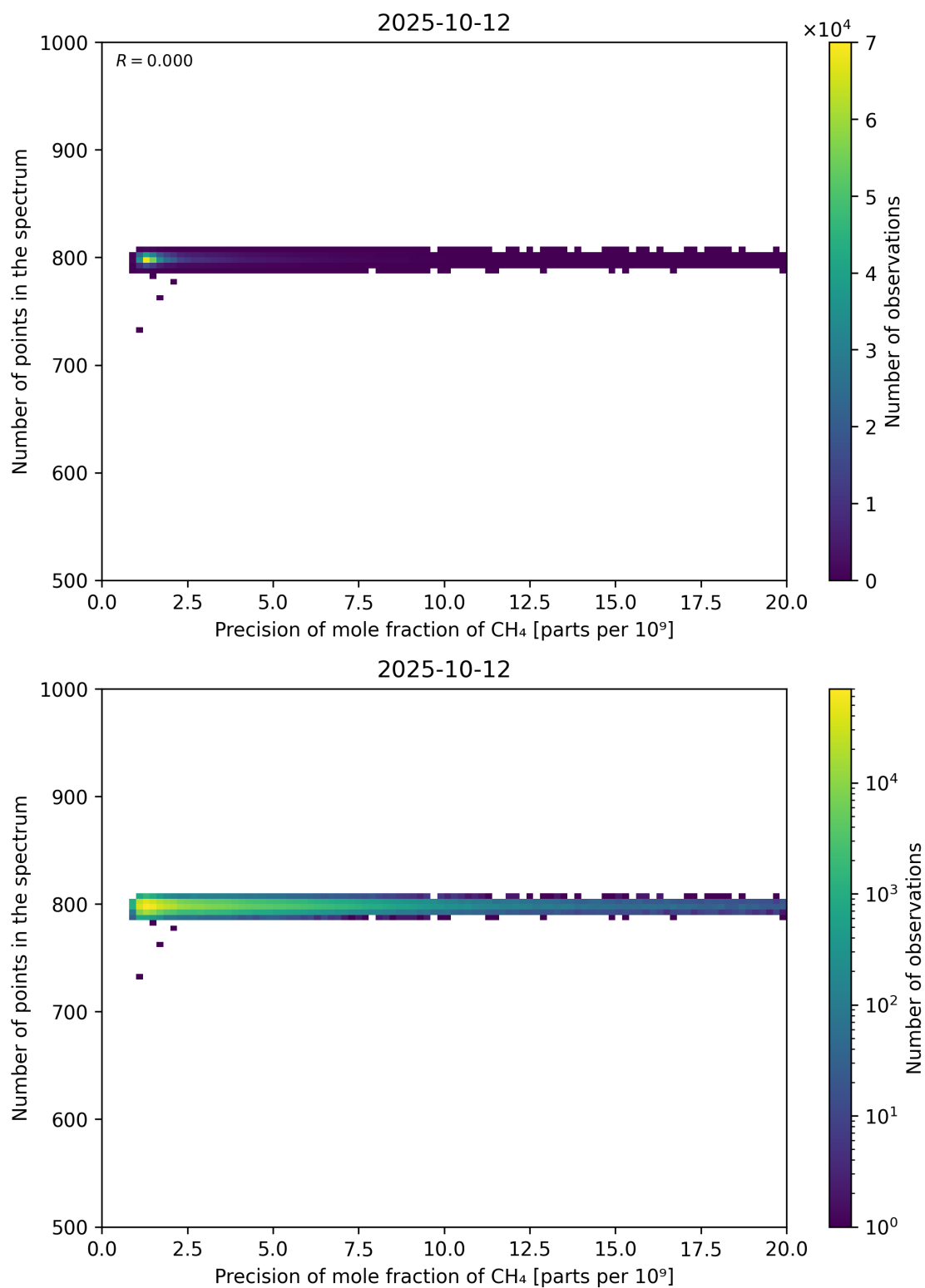
Figure 84: Scatter density plot of “Precision of mole fraction of CH 4 ” against “Number of points in the spectrum” for 2025-10-11 to 2025-10-13.
