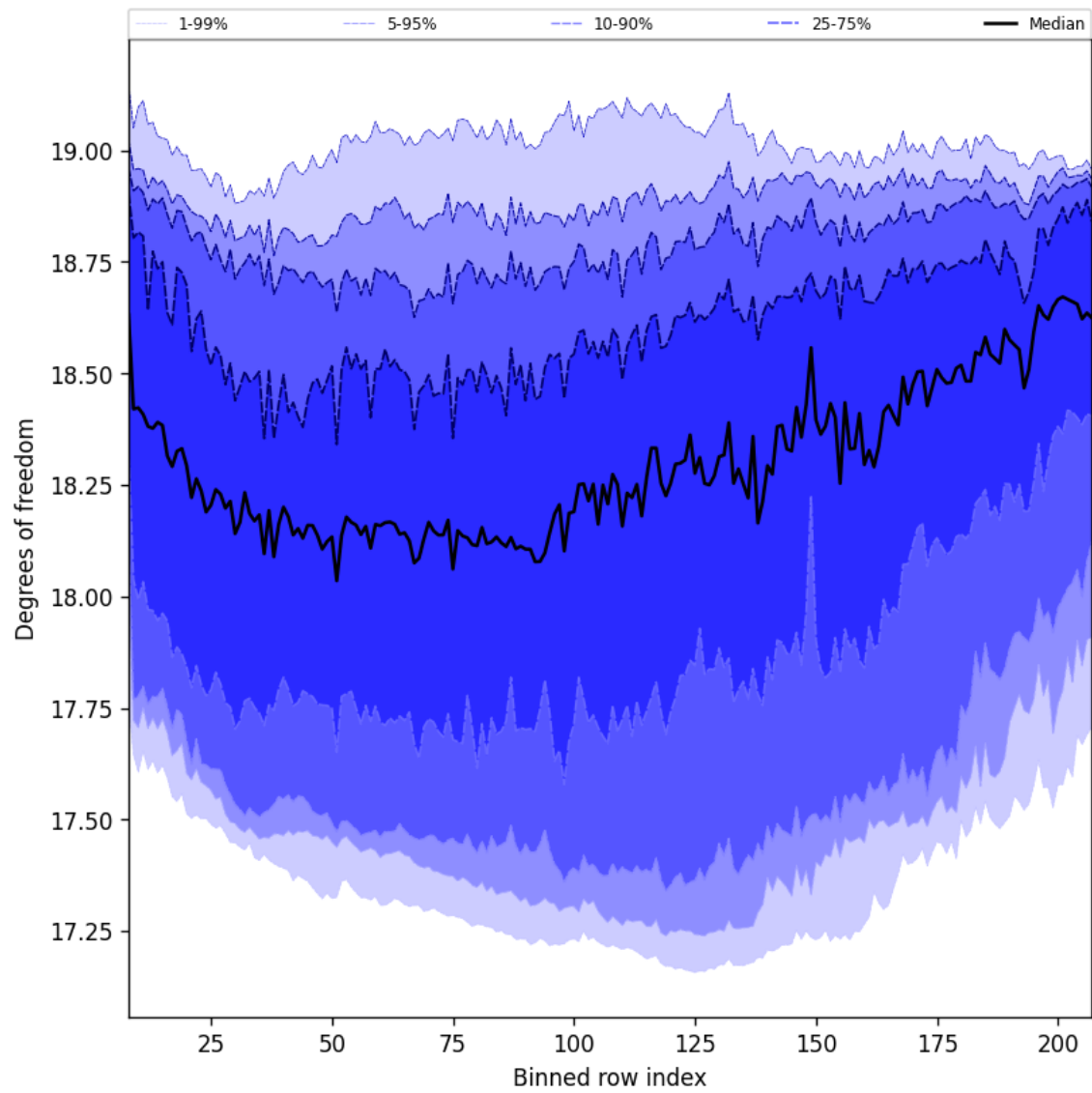
Figure 41: Along track statistics of “Degrees of freedom” for 2025-10-11 to 2025-10-13
