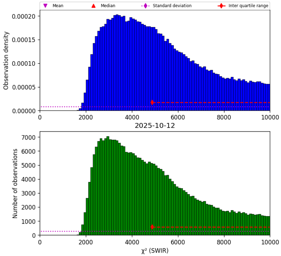
Figure 28: Histogram of “ \chi^2 (SWIR)” for 2025-10-11 to 2025-10-13
