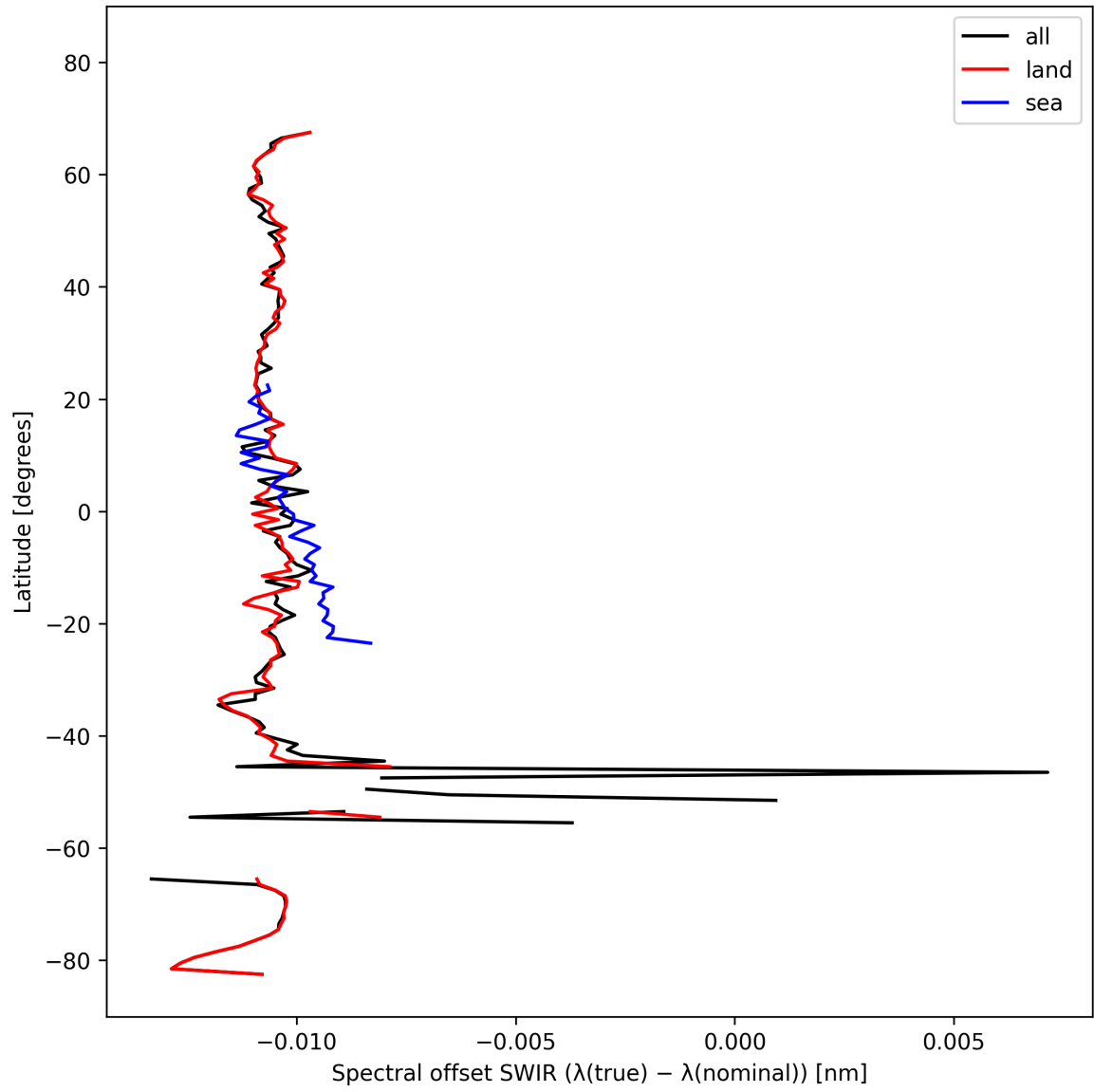
Figure 16: Zonal average of “Spectral offset SWIR ( \lambda_{\text{true}} - \lambda_{\text{nominal}} )” for 2025-10-11 to 2025-10-13.
