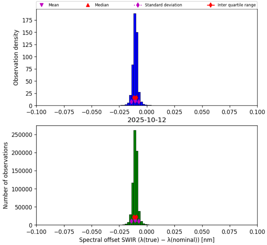
Figure 27: Histogram of “Spectral offset SWIR ( \lambda_{\text{true}} - \lambda_{\text{nominal}} )” for 2025-10-11 to 2025-10-13
