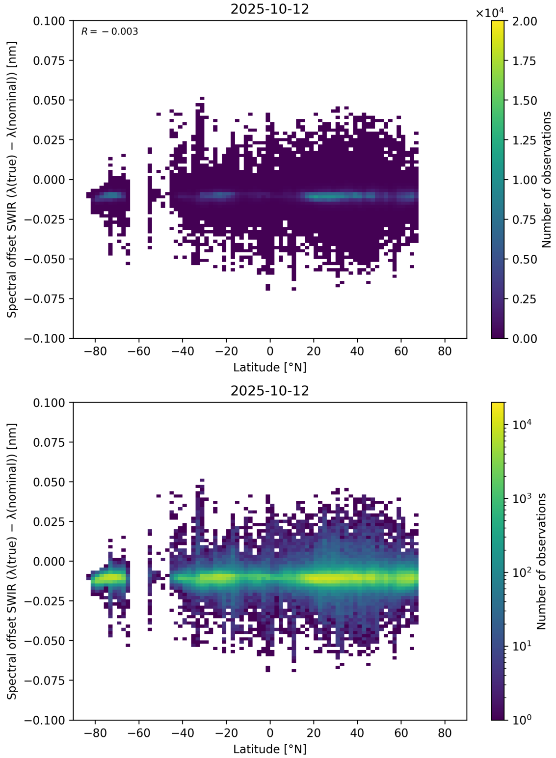
Figure 62: Scatter density plot of “Latitude” against “Spectral offset SWIR ( \lambda_{\text{true}} - \lambda_{\text{nominal}} )” for 2025-10-11 to 2025-10-13.
