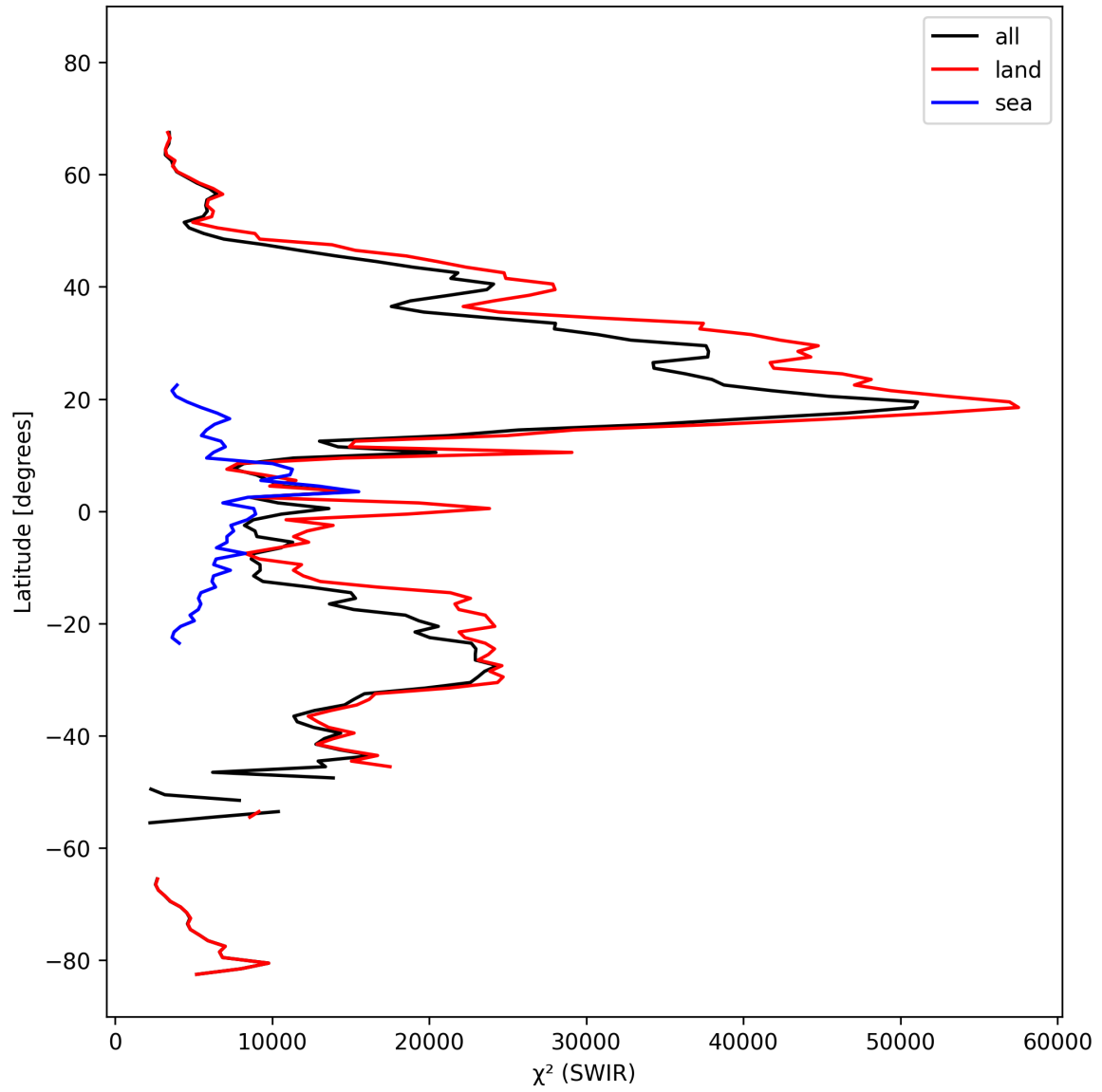
Figure 17: Zonal average of “ \chi^2 (SWIR)” for 2025-10-11 to 2025-10-13.
