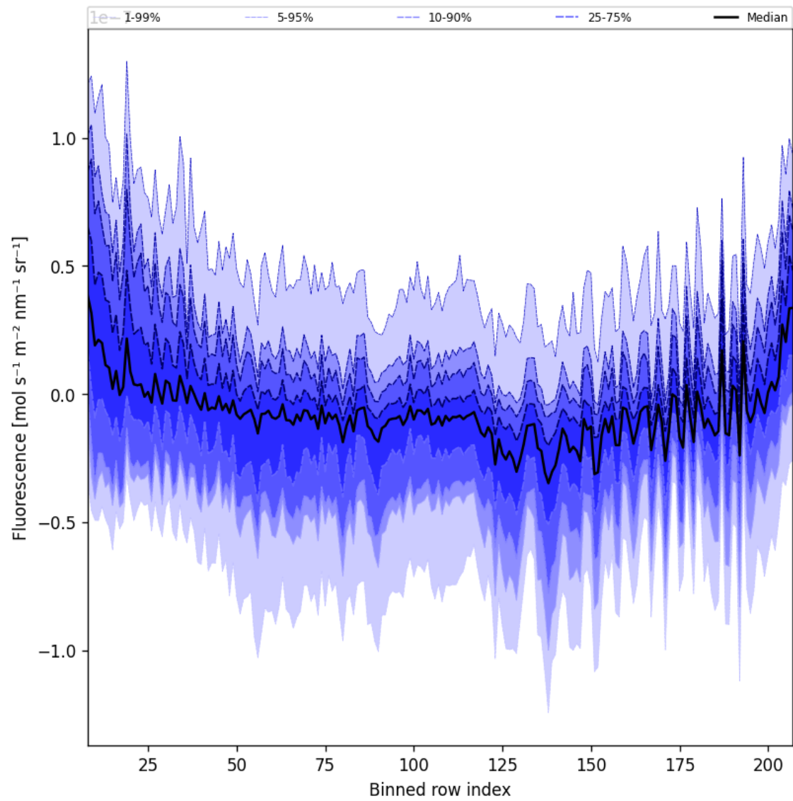
Figure 43: Along track statistics of “Fluorescence” for 2025-10-11 to 2025-10-13
