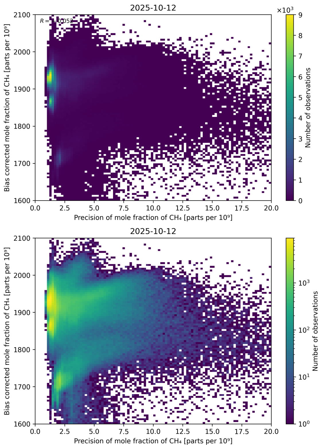
Figure 82: Scatter density plot of “Precision of mole fraction of CH 4 ” against “Bias corrected mole fraction of CH 4 ” for 2025-10-11 to 2025-10-13.
