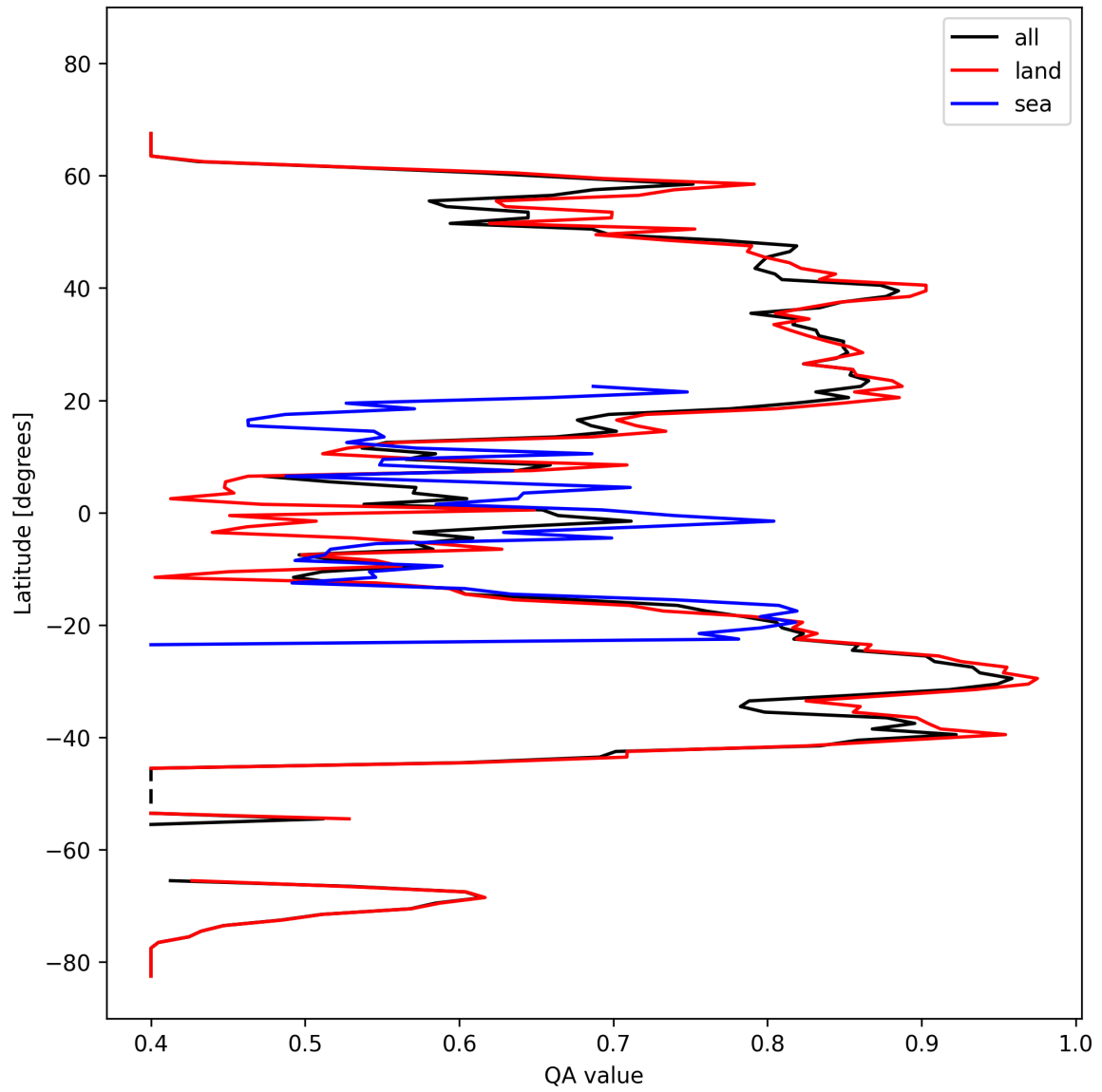
Figure 11: Zonal average of “QA value” for 2025-10-11 to 2025-10-13.
