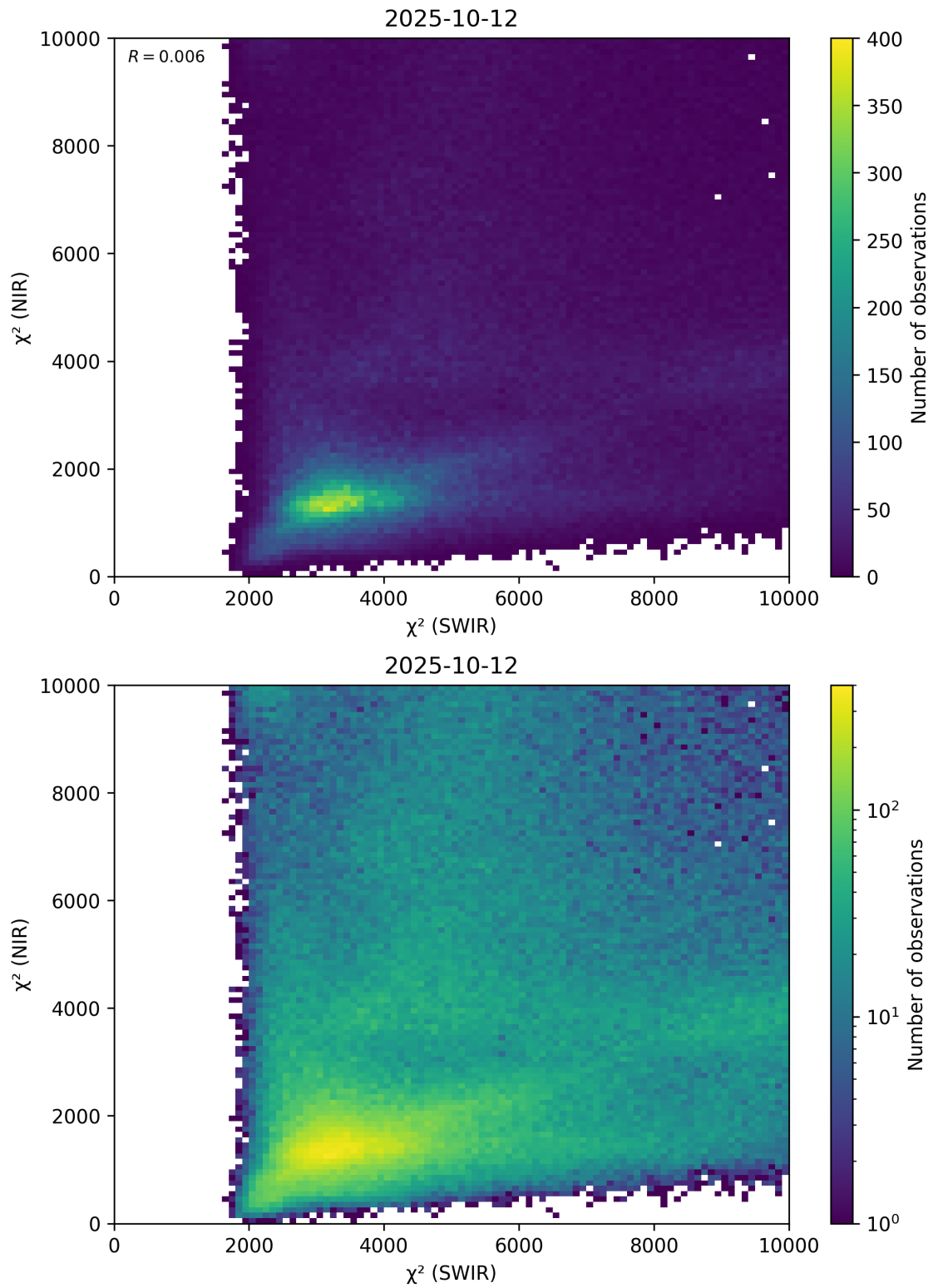
Figure 47: Scatter density plot of “ \chi^2 (SWIR)” against “ \chi^2 (NIR)” for 2025-10-11 to 2025-10-13.
