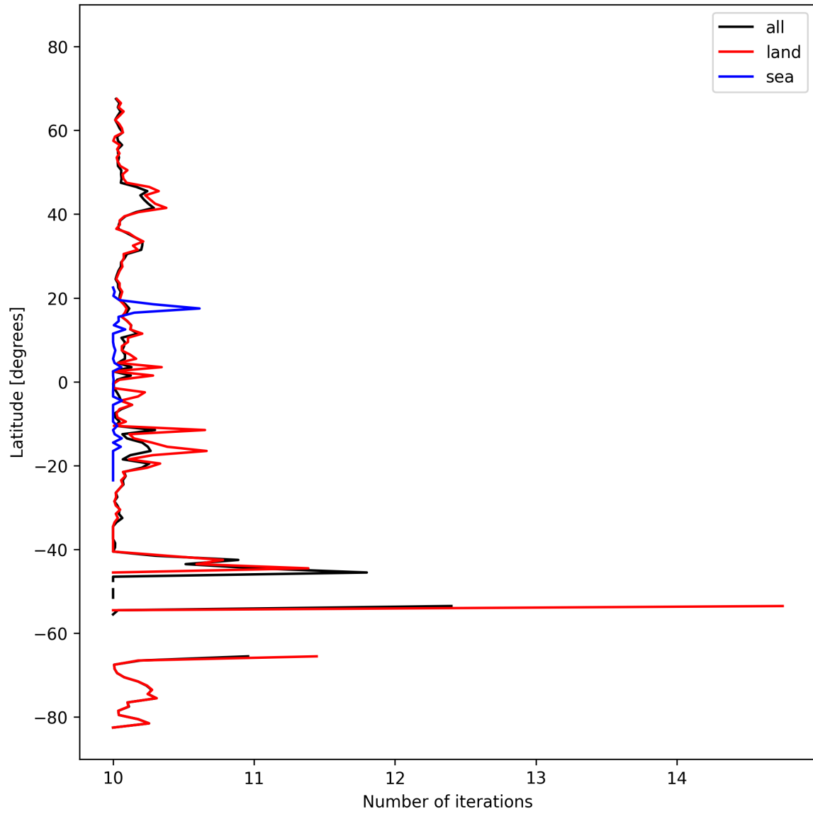
Figure 20: Zonal average of “Number of iterations” for 2025-10-11 to 2025-10-13.
