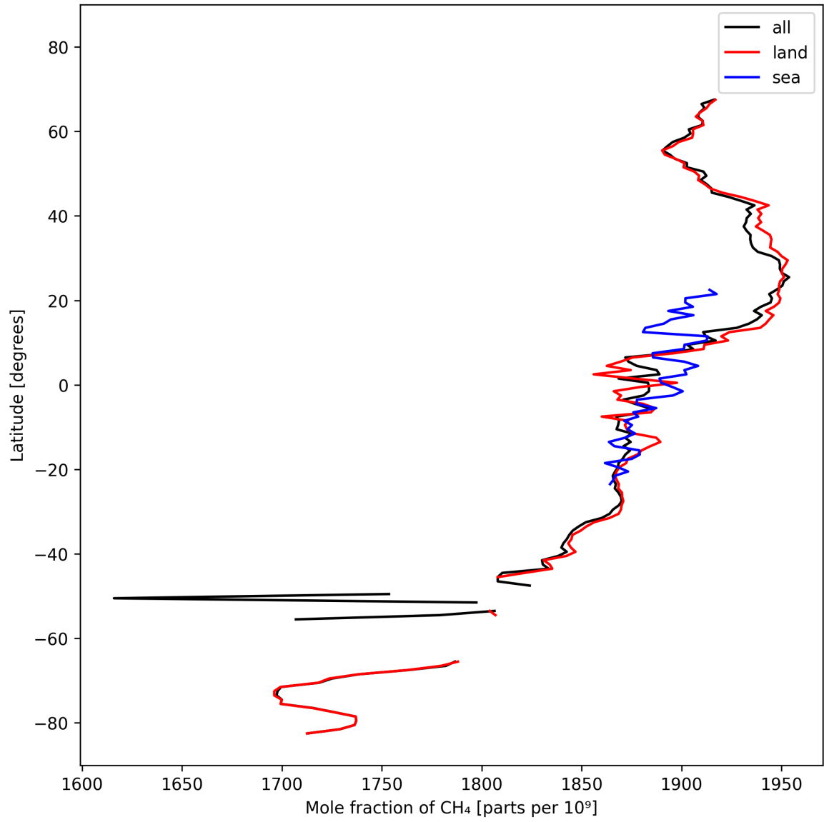
Figure 12: Zonal average of “Mole fraction of CH 4 ” for 2025-10-11 to 2025-10-13.
