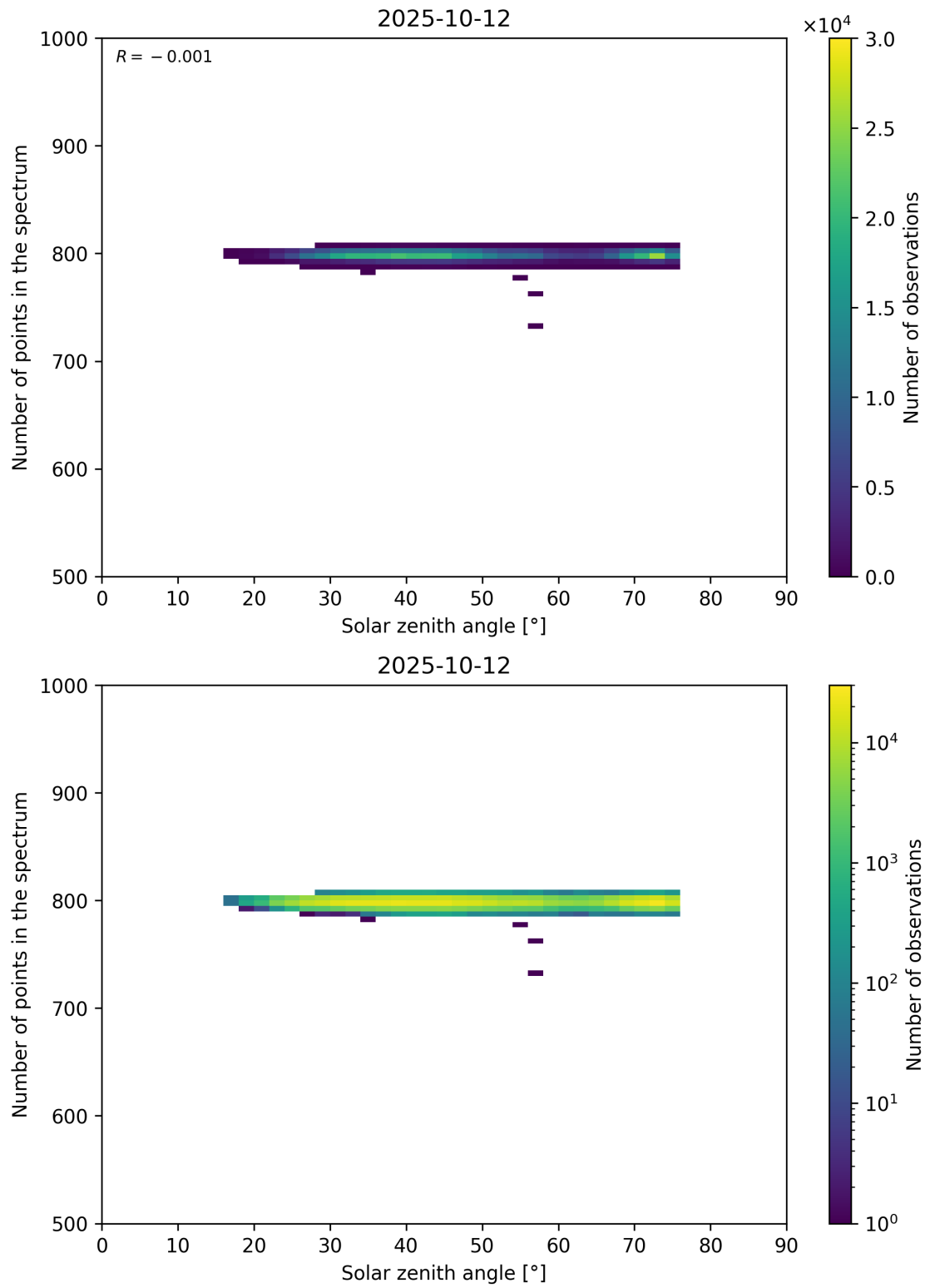
Figure 103: Scatter density plot of “Solar zenith angle” against “Number of points in the spectrum” for 2025-10-11 to 2025-10-13.
