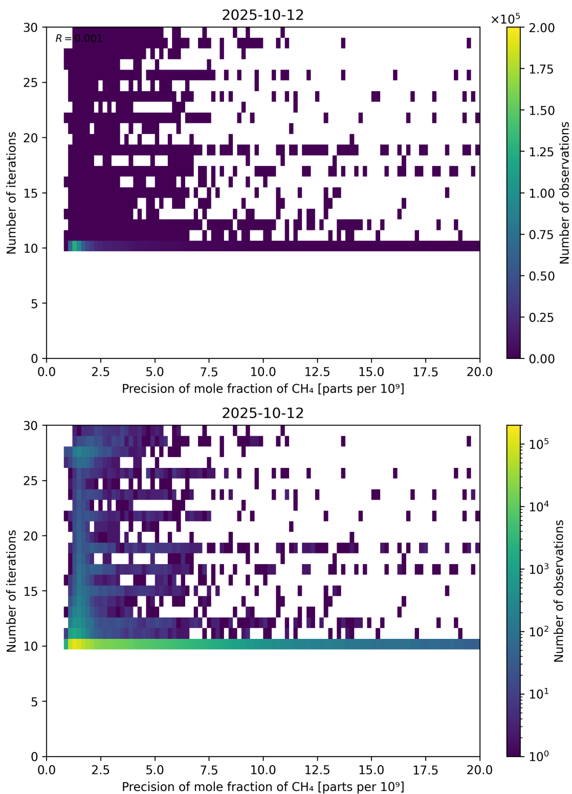
Figure 83: Scatter density plot of “Precision of mole fraction of \text{CH}_4 ” against “Number of iterations” for 2025-10-11 to 2025-10-13.
