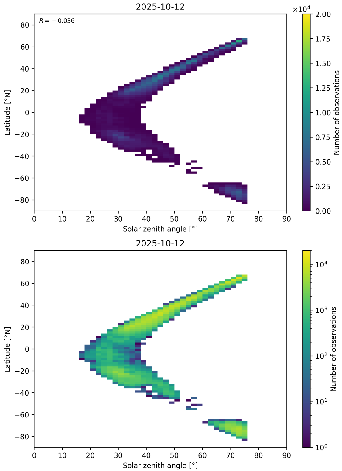
Figure 98: Scatter density plot of “Solar zenith angle” against “Latitude” for 2025-10-11 to 2025-10-13.
