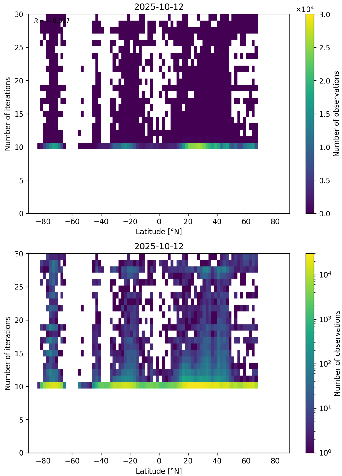
Figure 60: Scatter density plot of “Latitude” against “Number of iterations” for 2025-10-11 to 2025-10-13.
