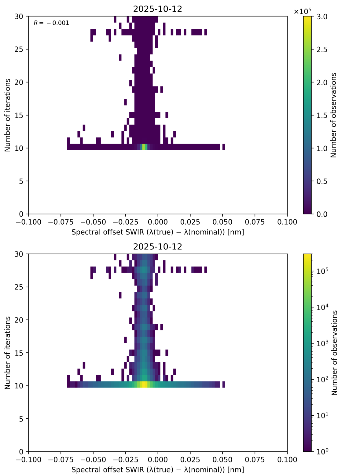
Figure 121: Scatter density plot of “Spectral offset SWIR ( \lambda_{\text{true}} - \lambda_{\text{nominal}} )” against “Number of iterations” for 2025-10-11 to 2025-10-13.
