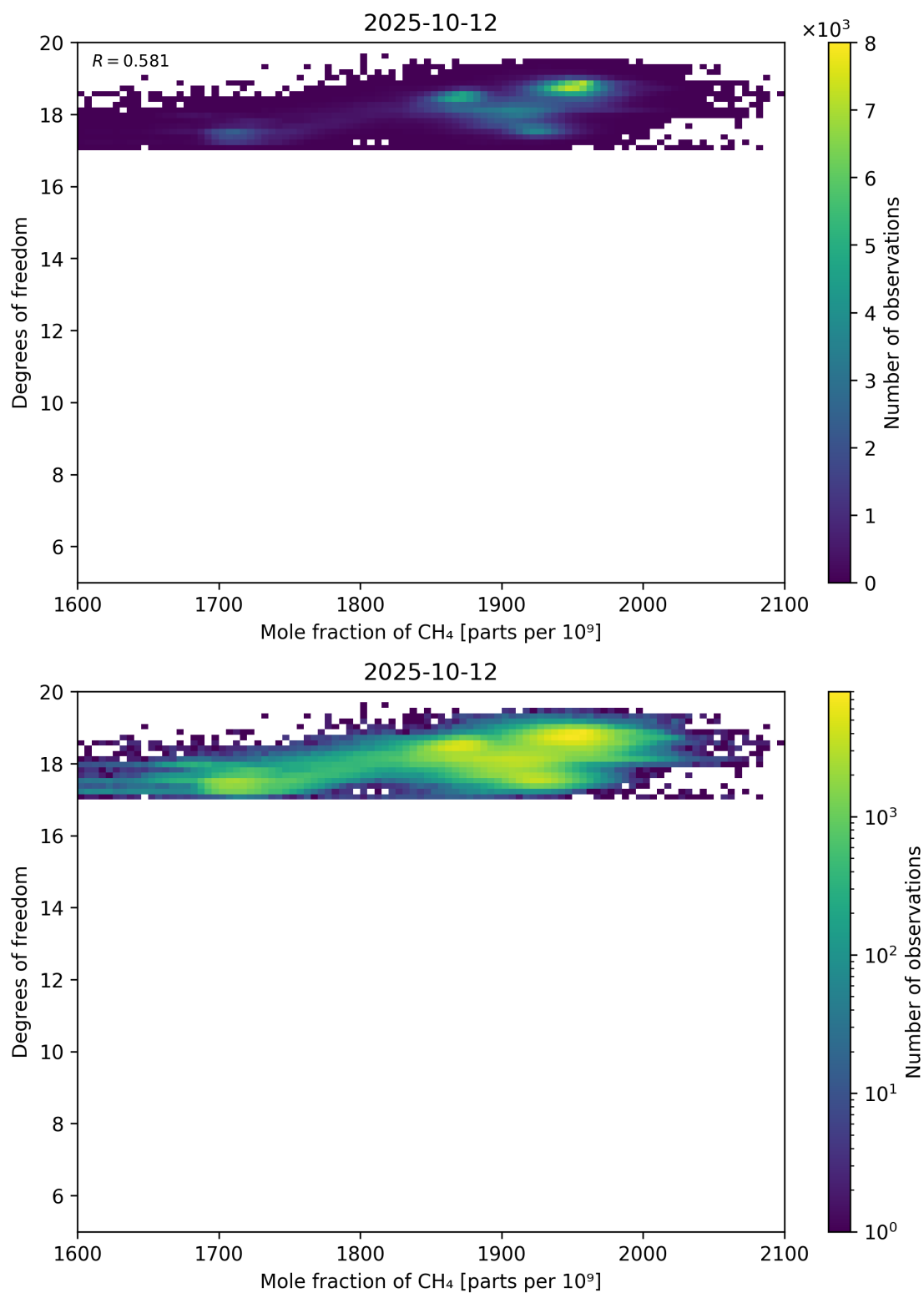
Figure 72: Scatter density plot of “Mole fraction of CH 4 ” against “Degrees of freedom” for 2025-10-11 to 2025-10-13.
