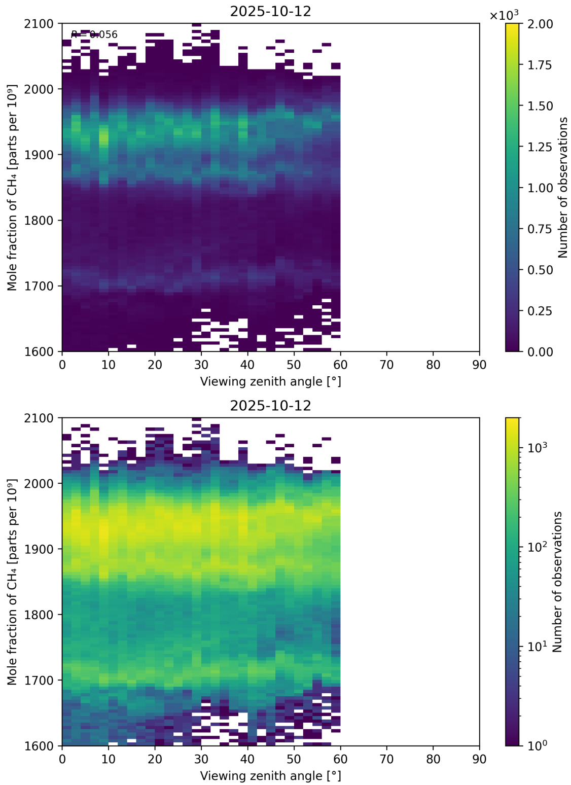
Figure 110: Scatter density plot of “Viewing zenith angle” against “Mole fraction of CH 4 ” for 2025-10-11 to 2025-10-13.
