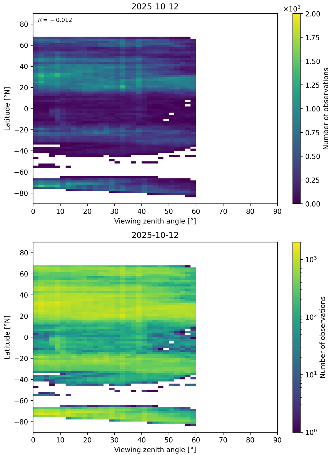
Figure 109: Scatter density plot of “Viewing zenith angle” against “Latitude” for 2025-10-11 to 2025-10-13.
