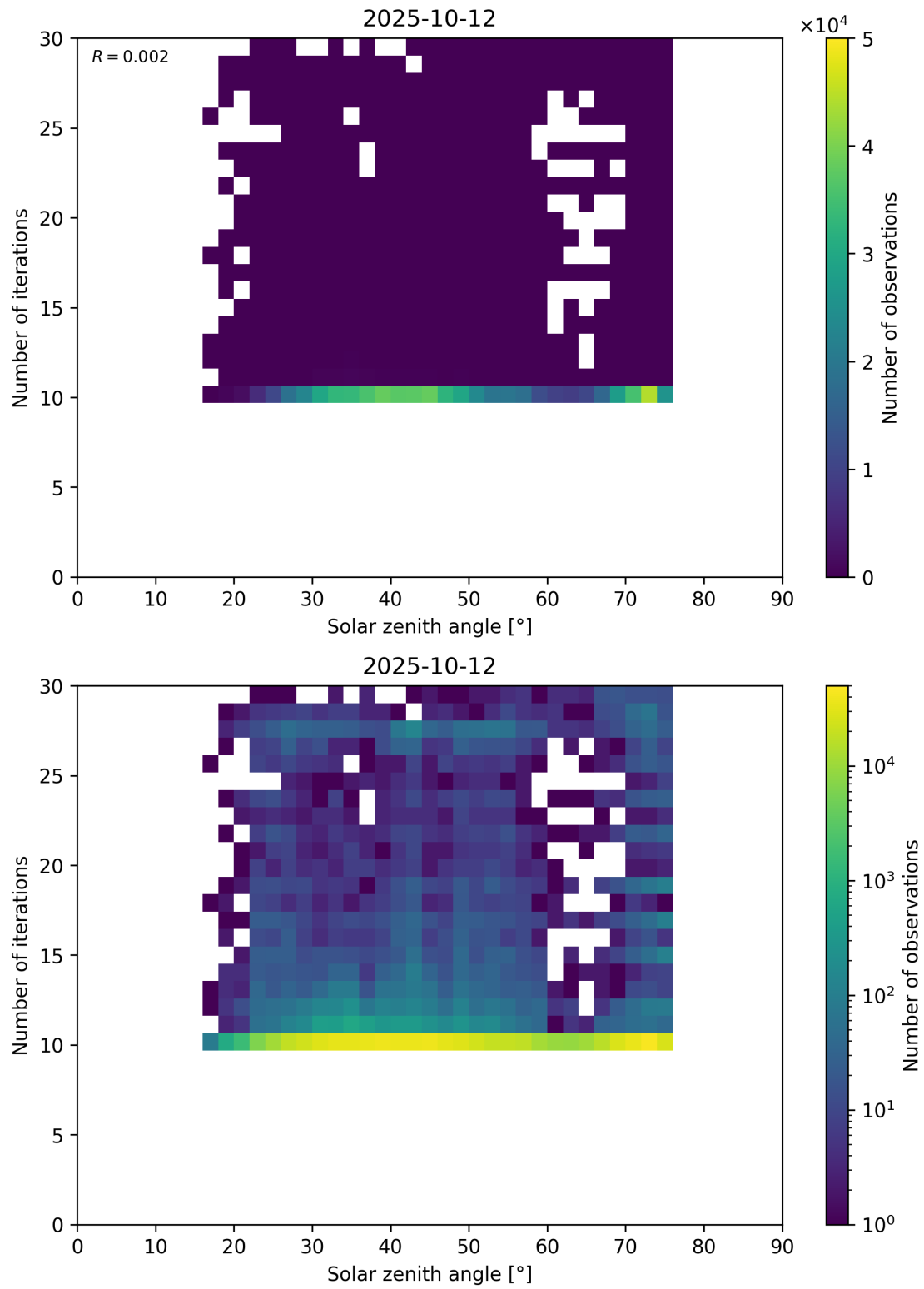
Figure 102: Scatter density plot of “Solar zenith angle” against “Number of iterations” for 2025-10-11 to 2025-10-13.
