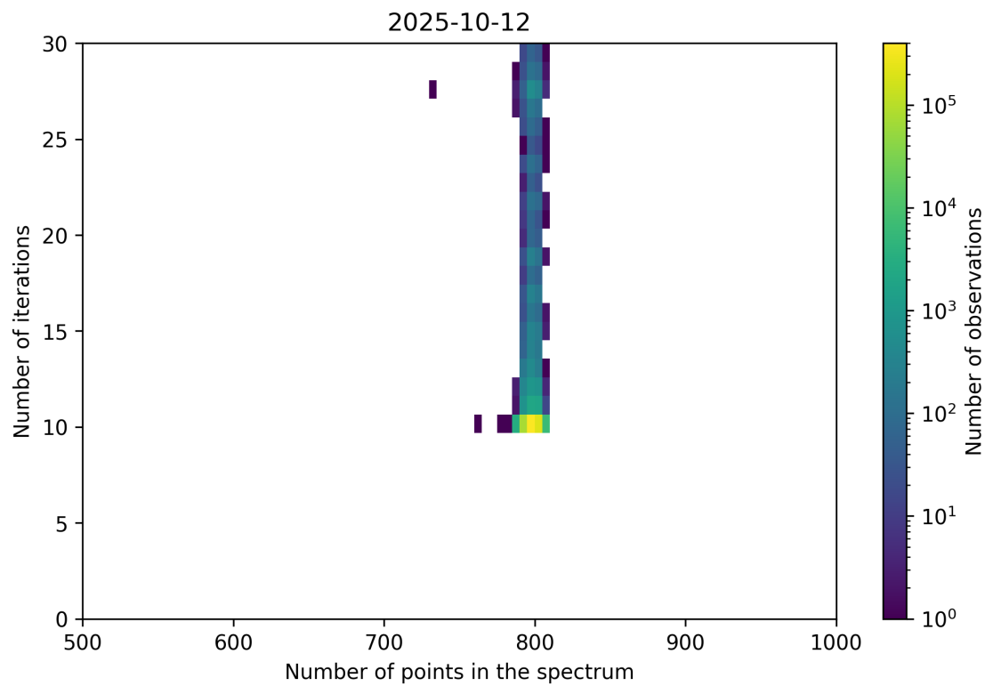
Figure 92: Scatter density plot of “Number of points in the spectrum” against “Number of iterations” for 2025-10-11 to 2025-10-13.
