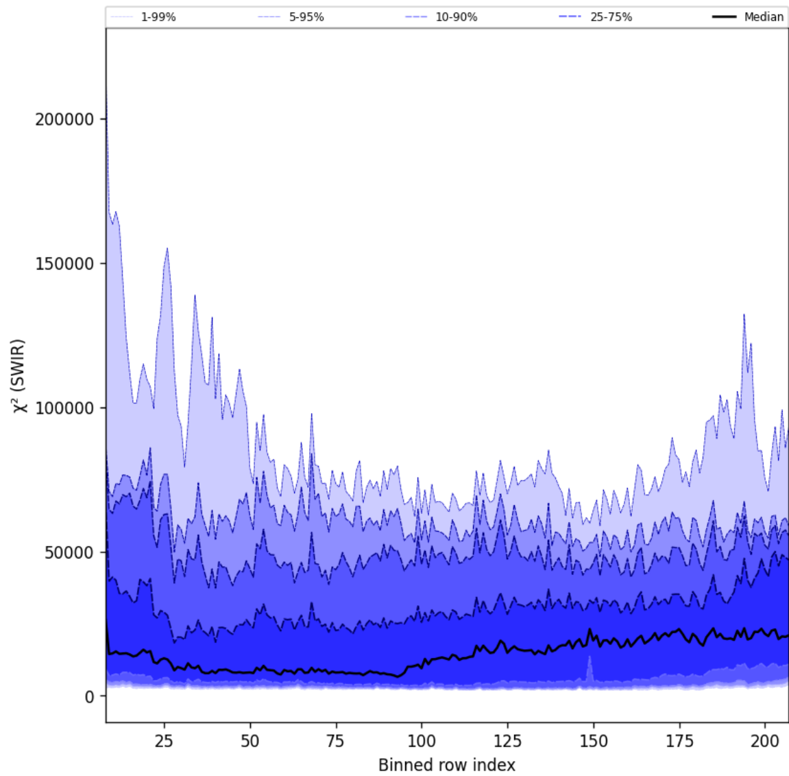
Figure 39: Along track statistics of “ \chi^2 (SWIR)” for 2025-10-11 to 2025-10-13
