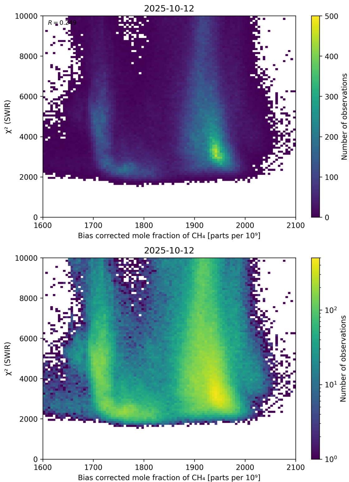
Figure 64: Scatter density plot of “Bias corrected mole fraction of \text{CH}_4 ” against “ \chi^2 (SWIR)” for 2025-10-11 to 2025-10-13.
