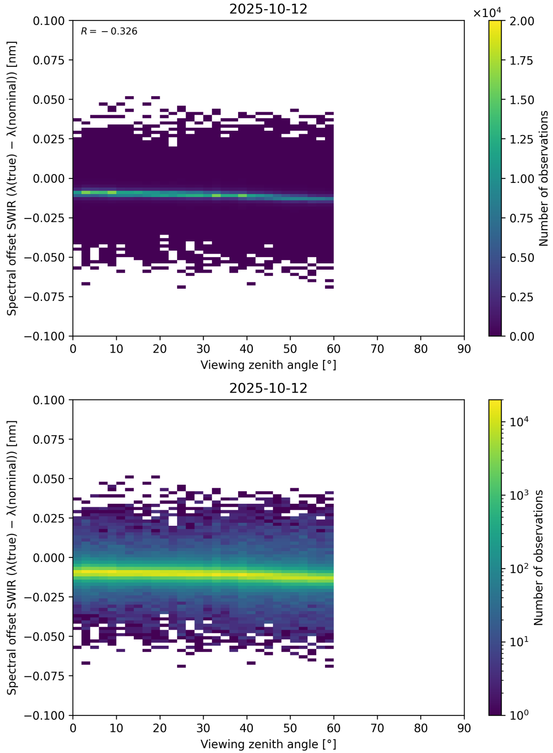
Figure 116: Scatter density plot of “Viewing zenith angle” against “Spectral offset SWIR ( \lambda_{\text{true}} - \lambda_{\text{nominal}} )” for 2025-10-11 to 2025-10-13.
