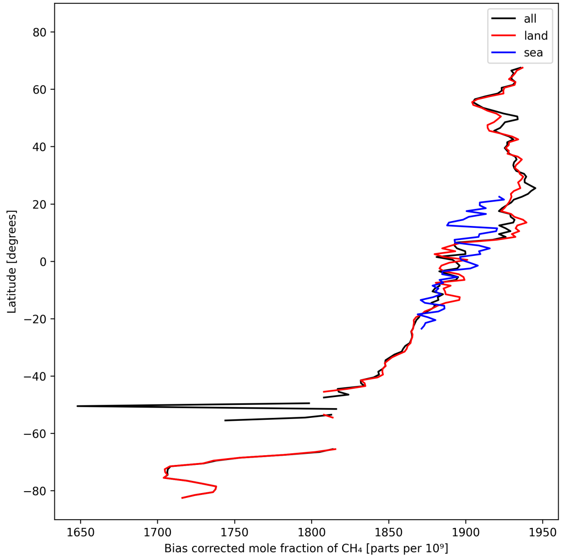
Figure 14: Zonal average of “Bias corrected mole fraction of CH 4 ” for 2025-10-11 to 2025-10-13.
