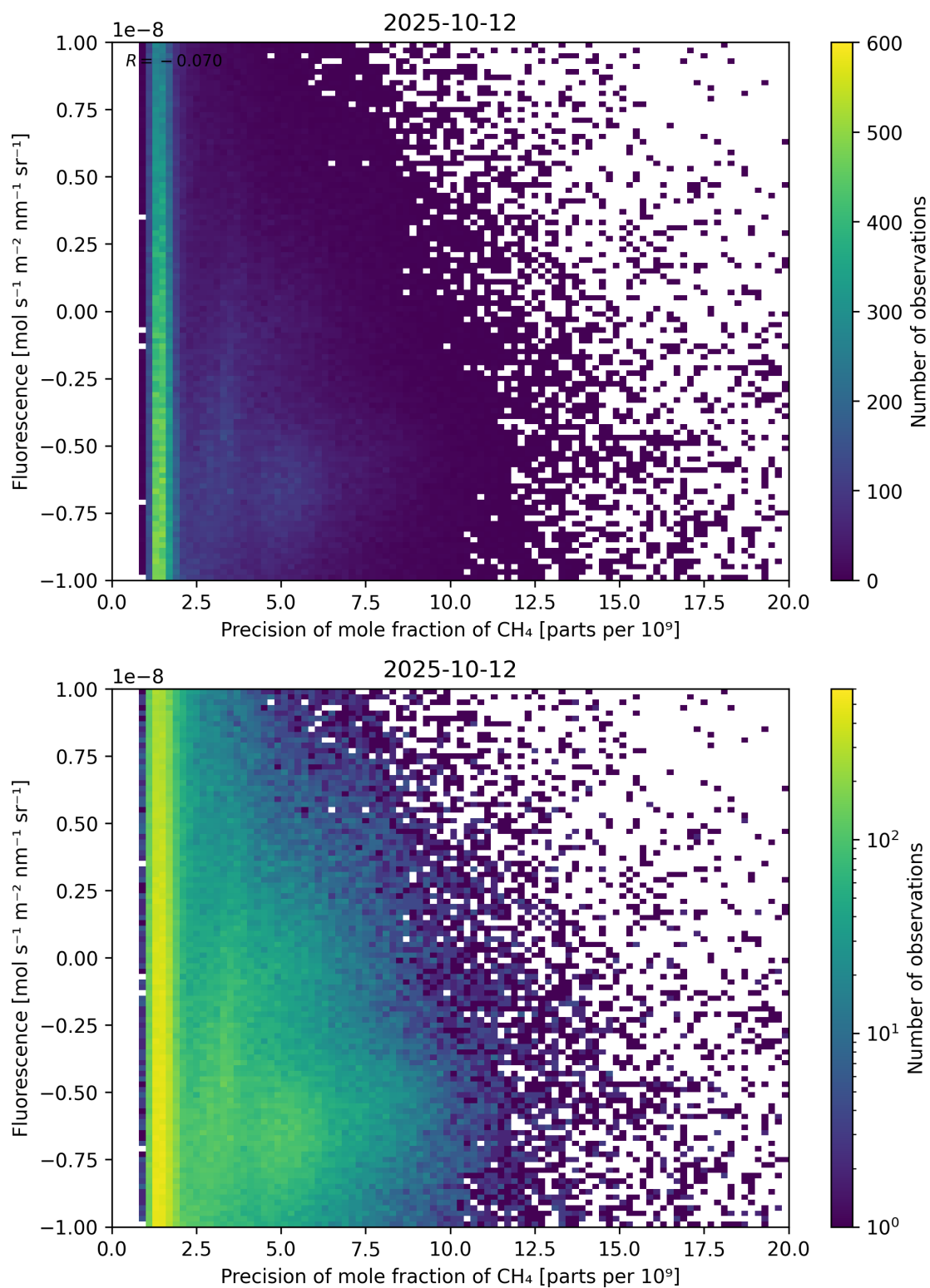
Figure 81: Scatter density plot of “Precision of mole fraction of CH 4 ” against “Fluorescence” for 2025-10-11 to 2025-10-13.
