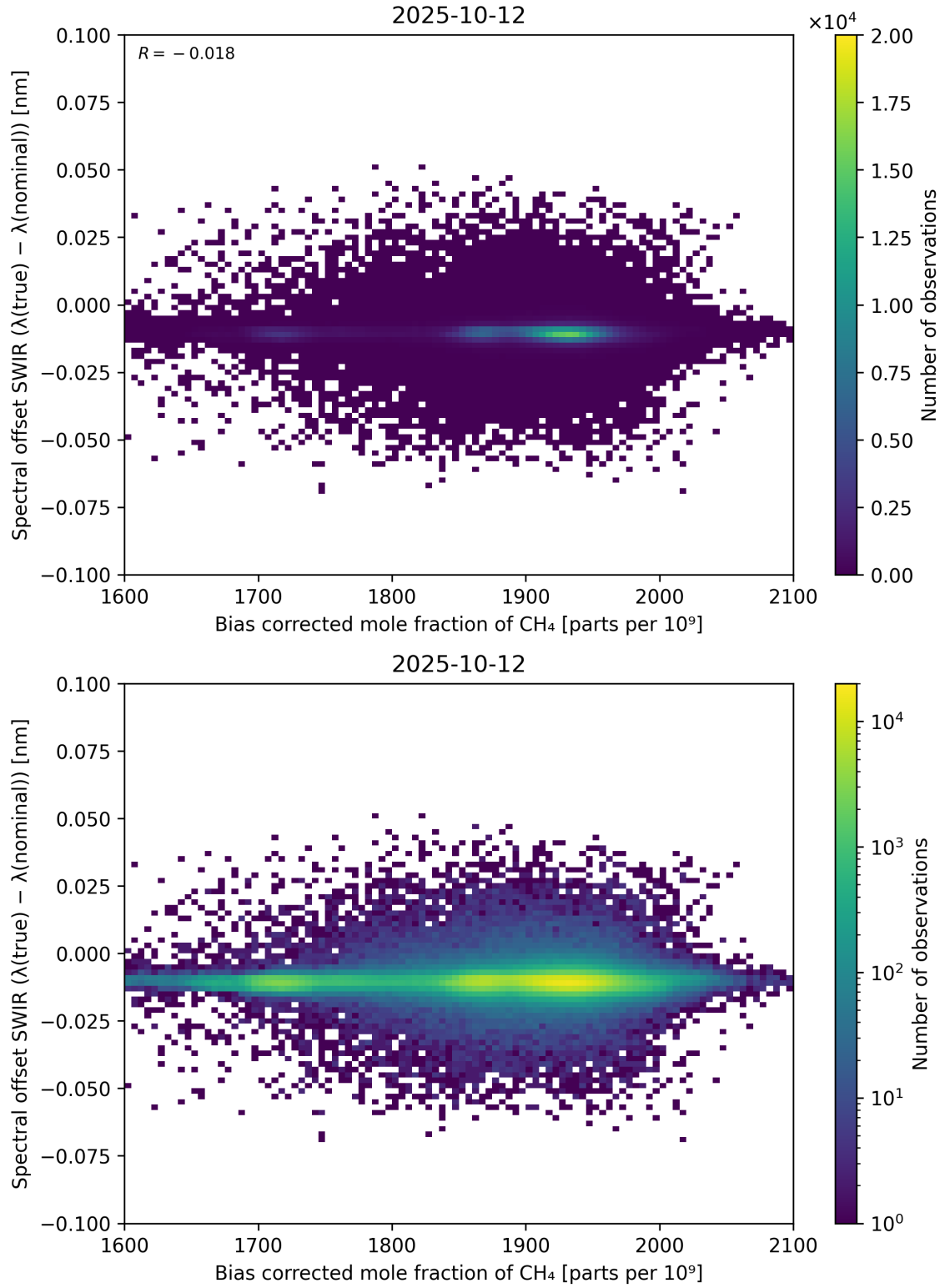
Figure 69: Scatter density plot of “Bias corrected mole fraction of \text{CH}_4 ” against “Spectral offset SWIR ( \lambda_{\text{true}} - \lambda_{\text{nominal}} )” for 2025-10-11 to 2025-10-13.
