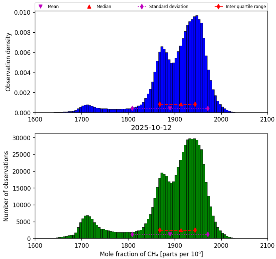
Figure 23: Histogram of “Mole fraction of CH 4 ” for 2025-10-11 to 2025-10-13
