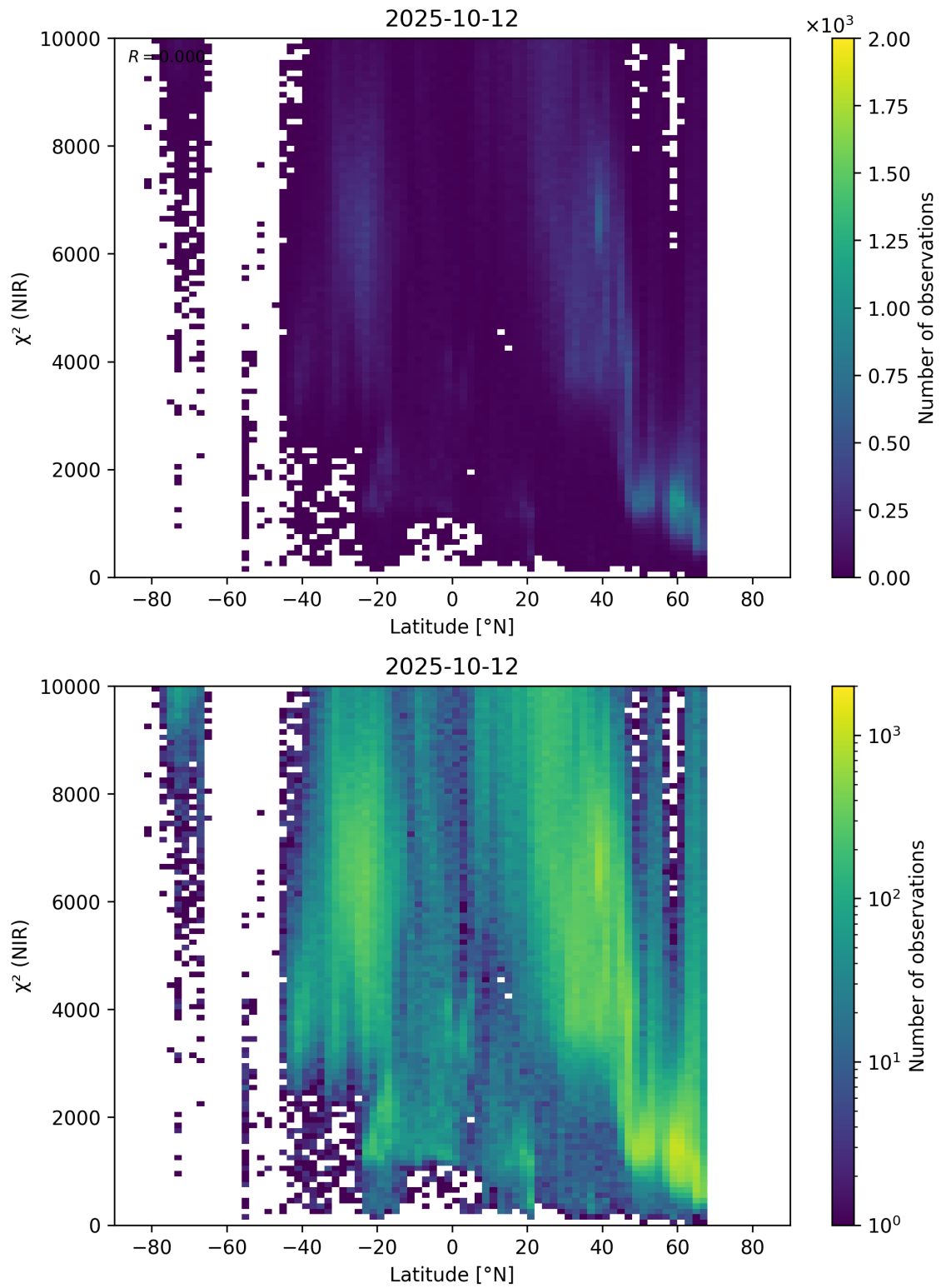
Figure 53: Scatter density plot of “Latitude” against “ \chi^2 (NIR)” for 2025-10-11 to 2025-10-13.
