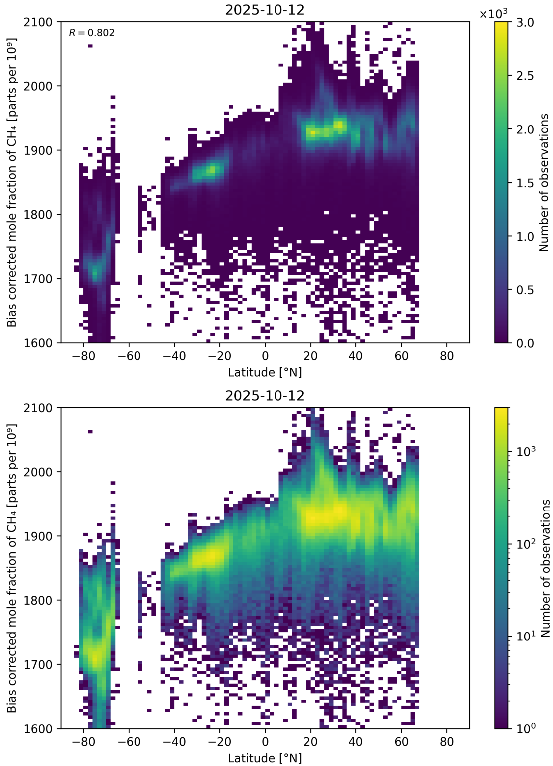
Figure 58: Scatter density plot of “Latitude” against “Bias corrected mole fraction of CH 4 ” for 2025-10-11 to 2025-10-13.
