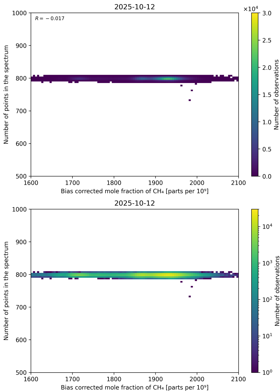
Figure 68: Scatter density plot of “Bias corrected mole fraction of CH 4 ” against “Number of points in the spectrum” for 2025-10-11 to 2025-10-13.
