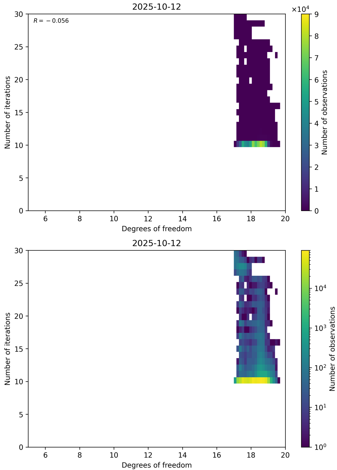
Figure 52: Scatter density plot of “Degrees of freedom” against “Number of iterations” for 2025-10-11 to 2025-10-13.
