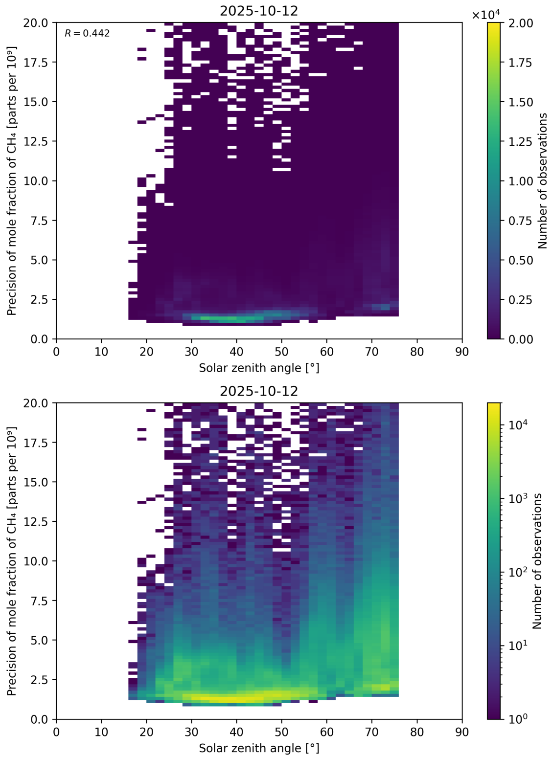
Figure 101: Scatter density plot of “Solar zenith angle” against “Precision of mole fraction of \text{CH}_4 ” for 2025-10-11 to 2025-10-13.
