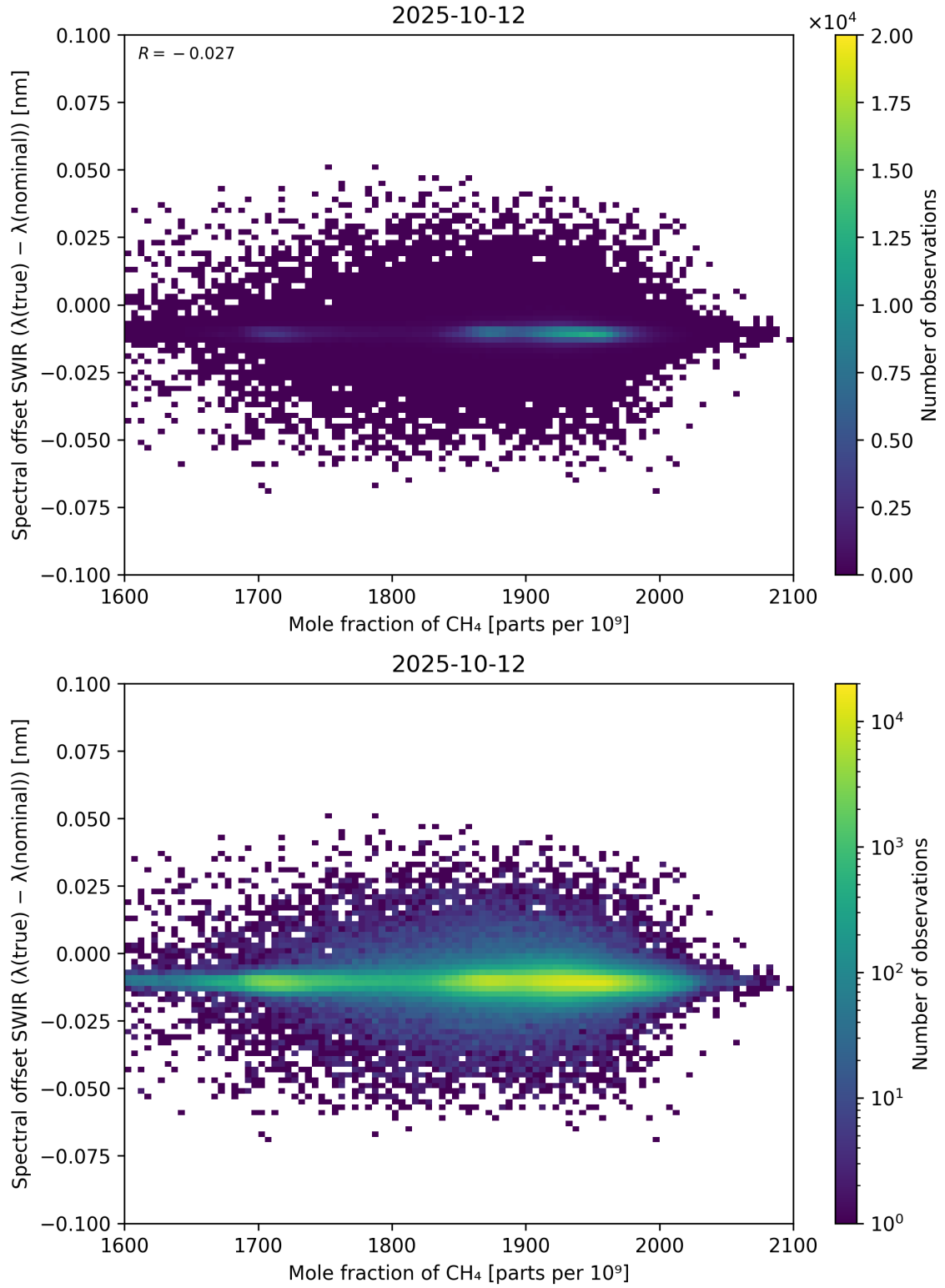
Figure 86: Scatter density plot of “Mole fraction of CH 4 ” against “Spectral offset SWIR ( \lambda_{\text{true}} - \lambda_{\text{nominal}} )” for 2025-10-11 to 2025-10-13.
