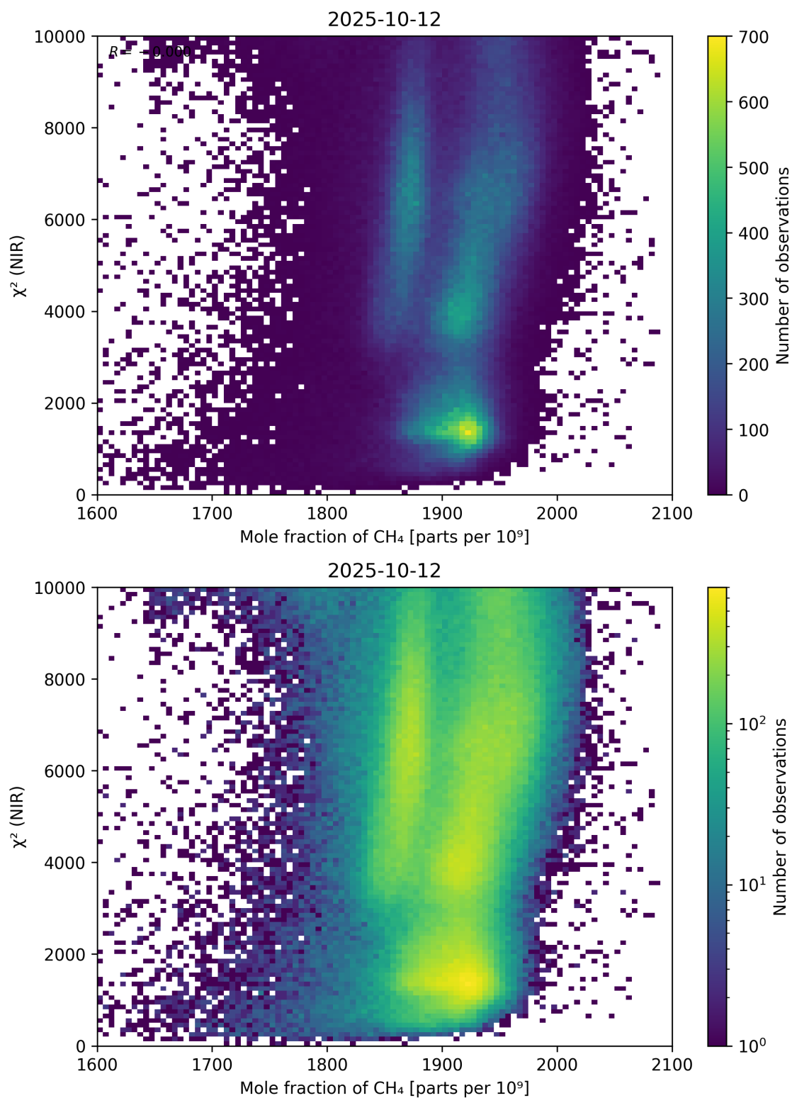
Figure 70: Scatter density plot of “Mole fraction of \text{CH}_4 ” against “ \chi^2 (NIR)” for 2025-10-11 to 2025-10-13.
