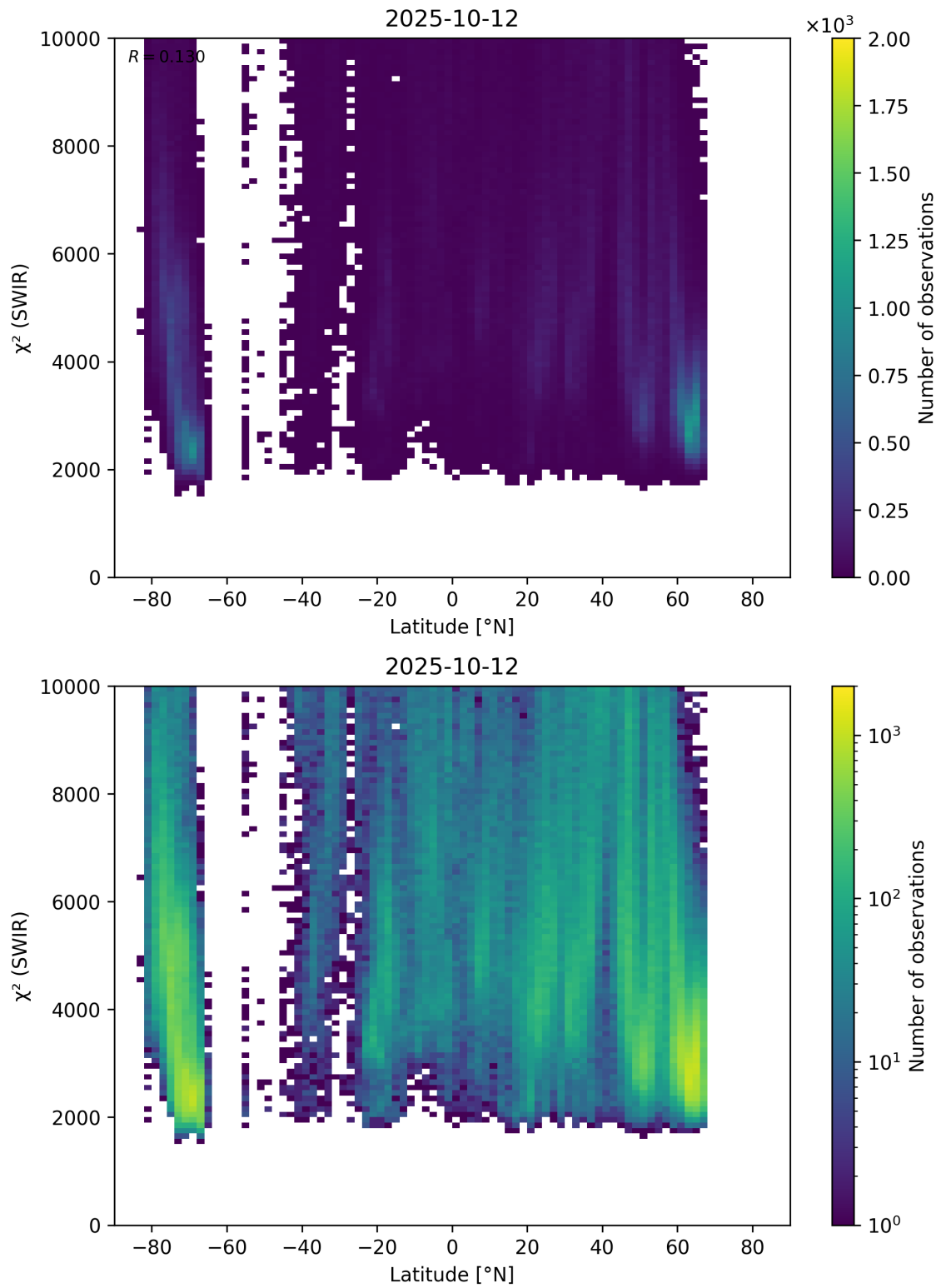
Figure 54: Scatter density plot of “Latitude” against “ \chi^2 (SWIR)” for 2025-10-11 to 2025-10-13.
