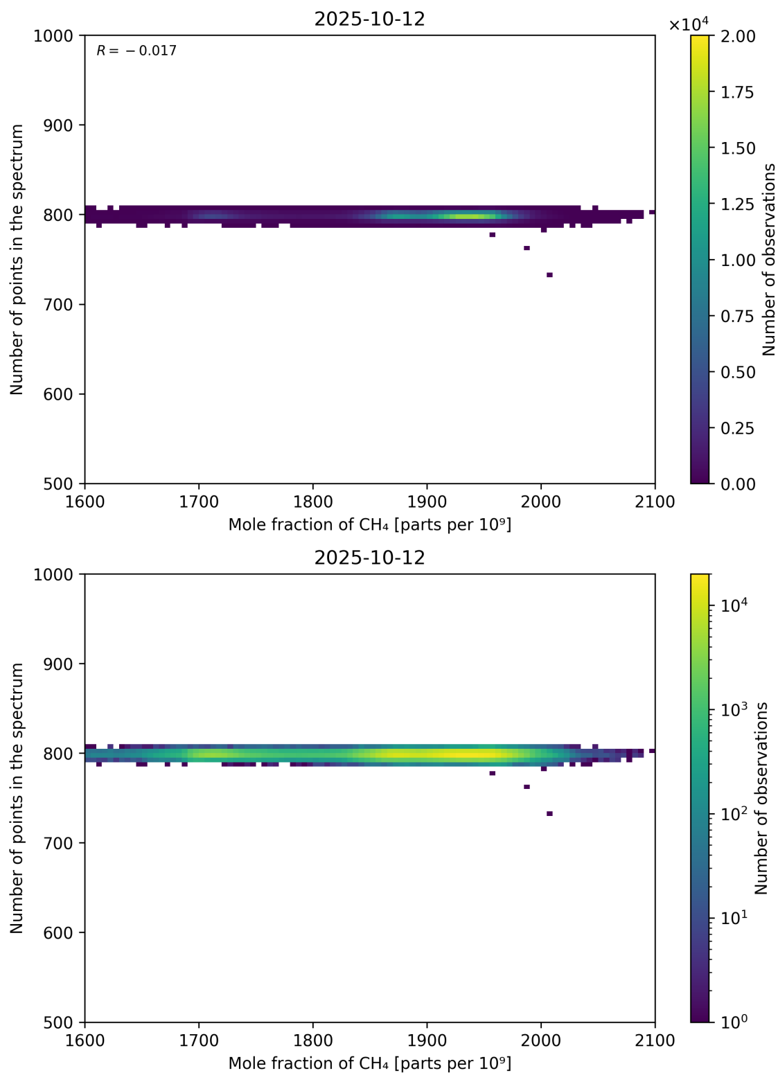
Figure 77: Scatter density plot of “Mole fraction of CH 4 ” against “Number of points in the spectrum” for 2025-10-11 to 2025-10-13.
