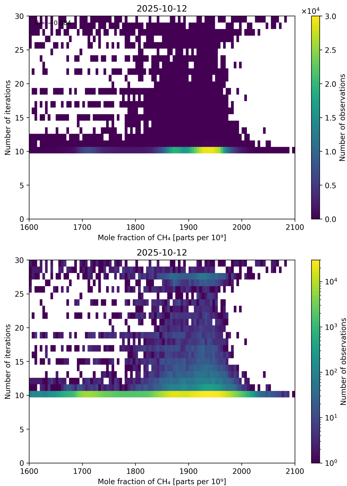
Figure 76: Scatter density plot of “Mole fraction of CH 4 ” against “Number of iterations” for 2025-10-11 to 2025-10-13.
