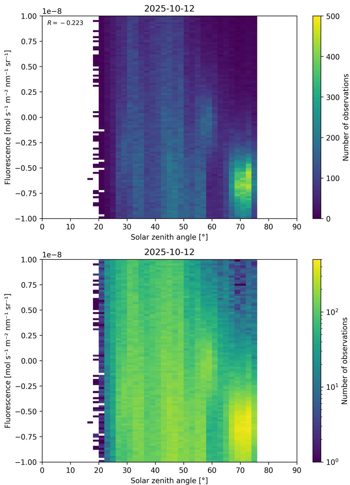
Figure 97: Scatter density plot of “Solar zenith angle” against “Fluorescence” for 2025-10-11 to 2025-10-13.
