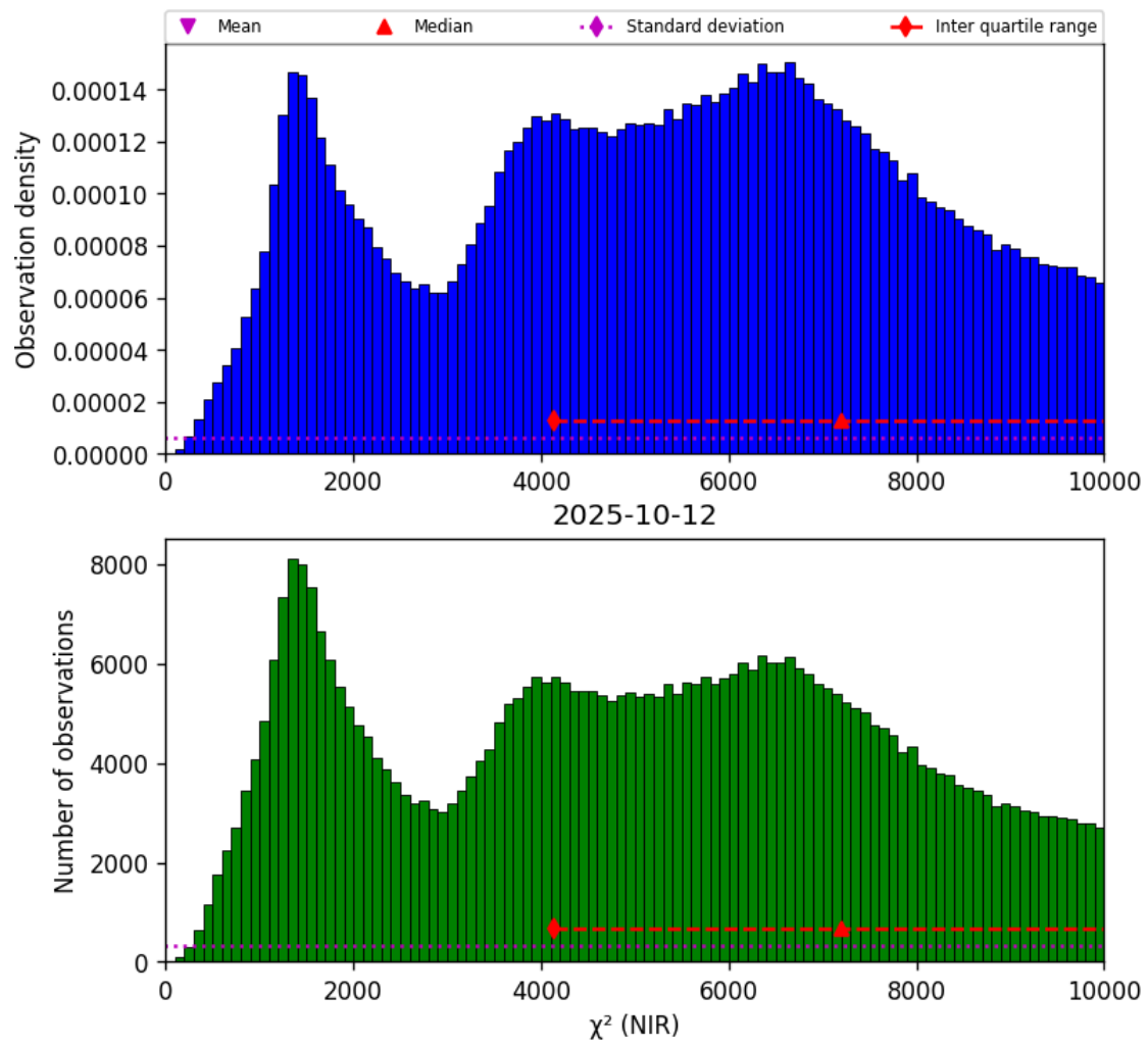
Figure 29: Histogram of “ \chi^2 (NIR)” for 2025-10-11 to 2025-10-13
