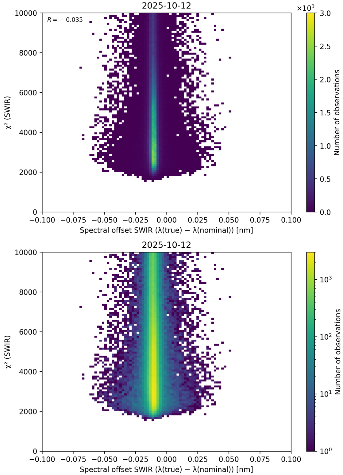
Figure 118: Scatter density plot of “Spectral offset SWIR ( \lambda_{\text{true}} - \lambda_{\text{nominal}} )” against “ \chi^2 (SWIR)” for 2025-10-11 to 2025-10-13.
