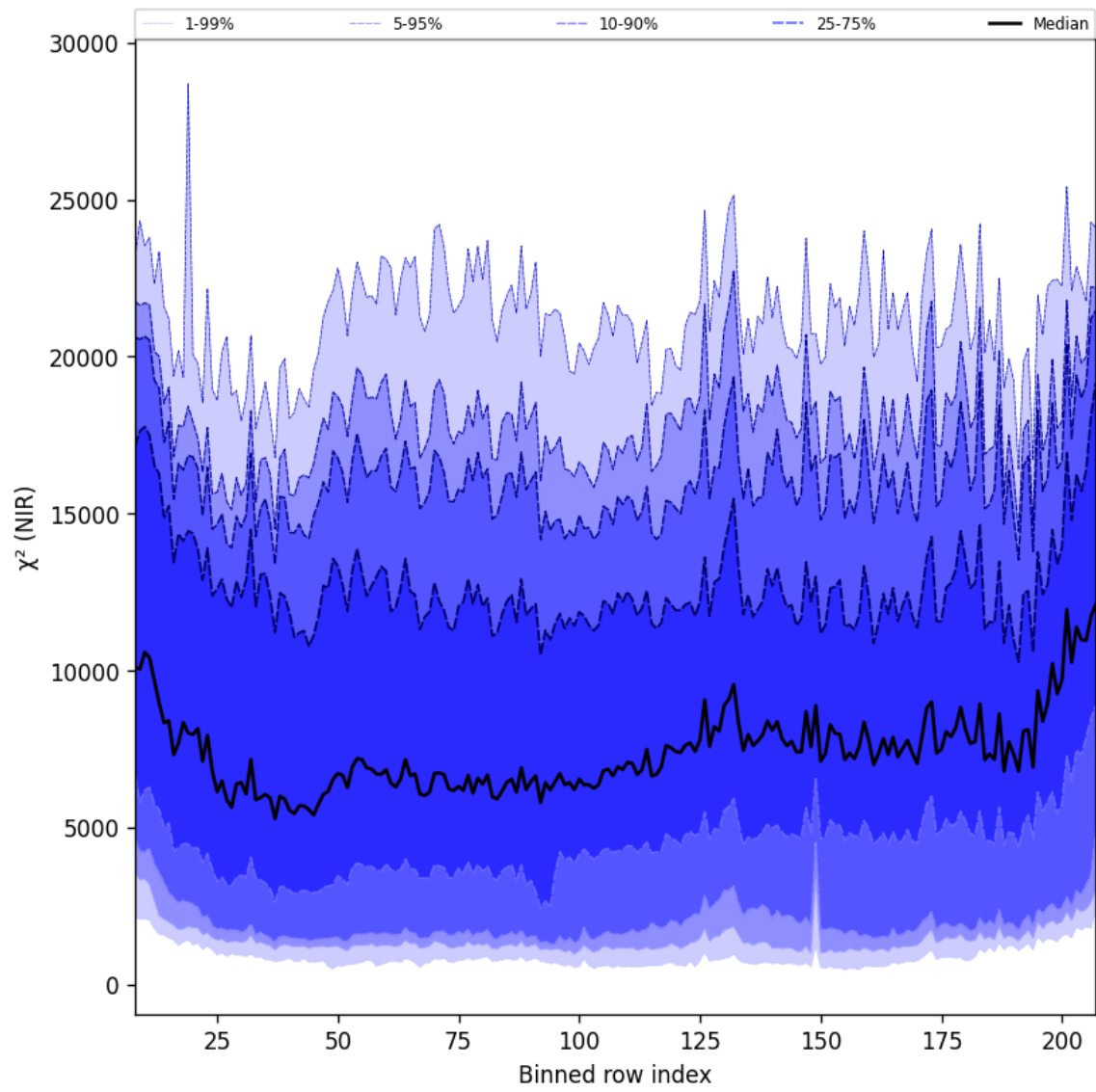
Figure 40: Along track statistics of “ \chi^2 (NIR)” for 2025-10-11 to 2025-10-13
