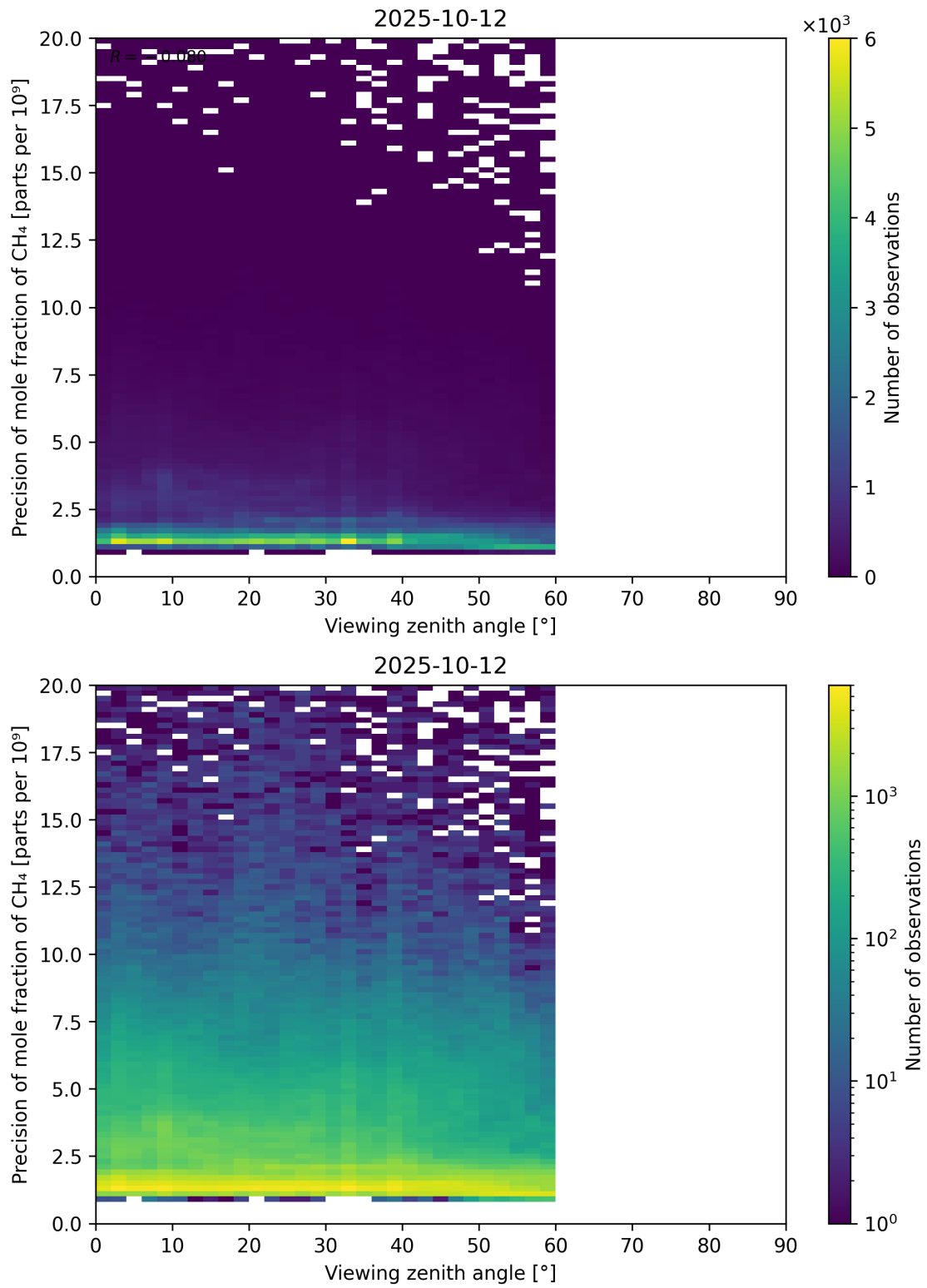
Figure 112: Scatter density plot of “Viewing zenith angle” against “Precision of mole fraction of CH 4 ” for 2025-10-11 to 2025-10-13.
