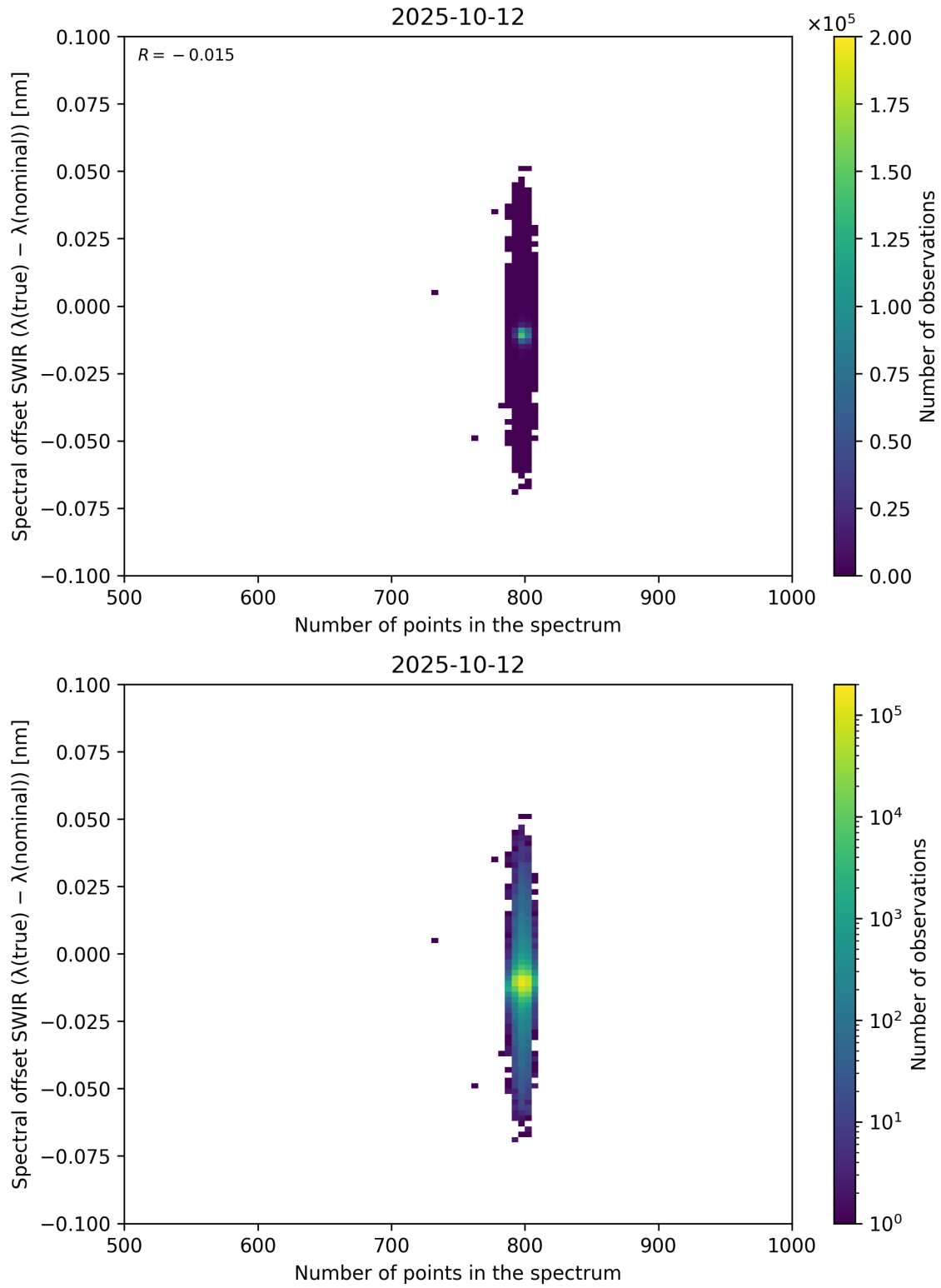
Figure 93: Scatter density plot of “Number of points in the spectrum” against “Spectral offset SWIR ( \lambda_{\text{true}} - \lambda_{\text{nominal}} )” for 2025-10-11 to 2025-10-13.
