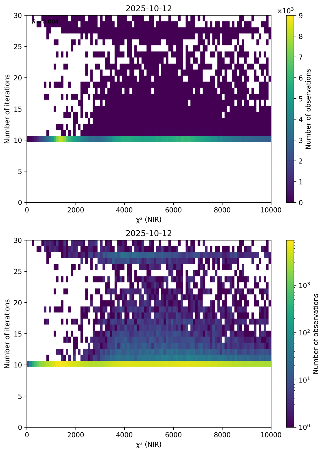
Figure 46: Scatter density plot of “ \chi^2 (NIR)” against “Number of iterations” for 2025-10-11 to 2025-10-13.
