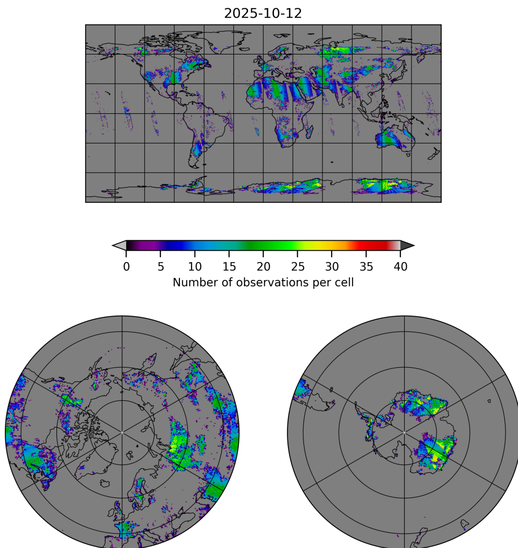
Figure 10: Map of the number of observations for 2025-10-11 to 2025-10-13
