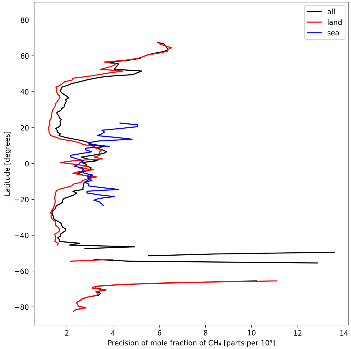
Figure 13: Zonal average of “Precision of mole fraction of CH 4 ” for 2025-10-11 to 2025-10-13.
