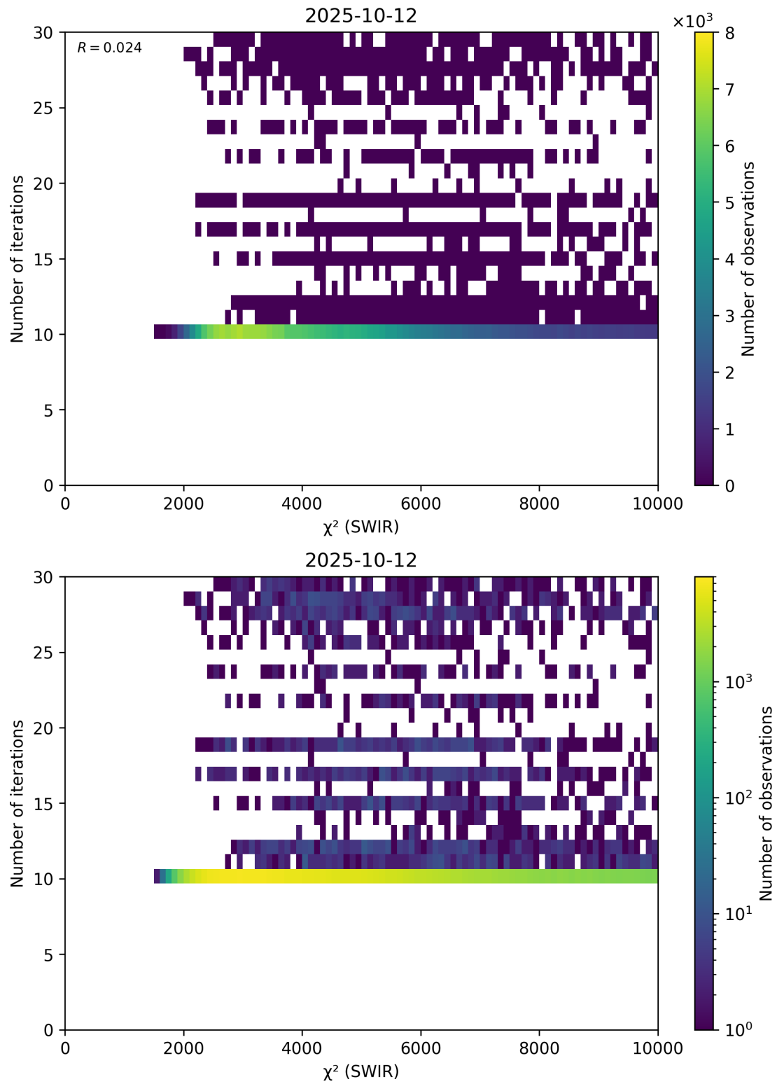
Figure 50: Scatter density plot of “ \chi^2 (SWIR)” against “Number of iterations” for 2025-10-11 to 2025-10-13.
