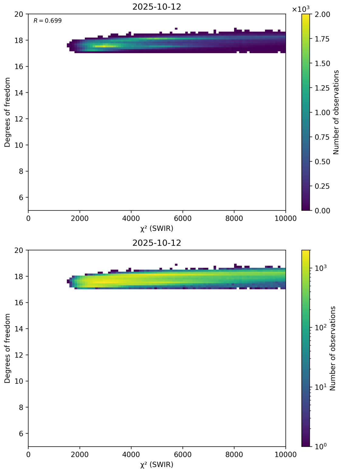
Figure 48: Scatter density plot of “ \chi^2 (SWIR)” against “Degrees of freedom” for 2025-10-11 to 2025-10-13.
