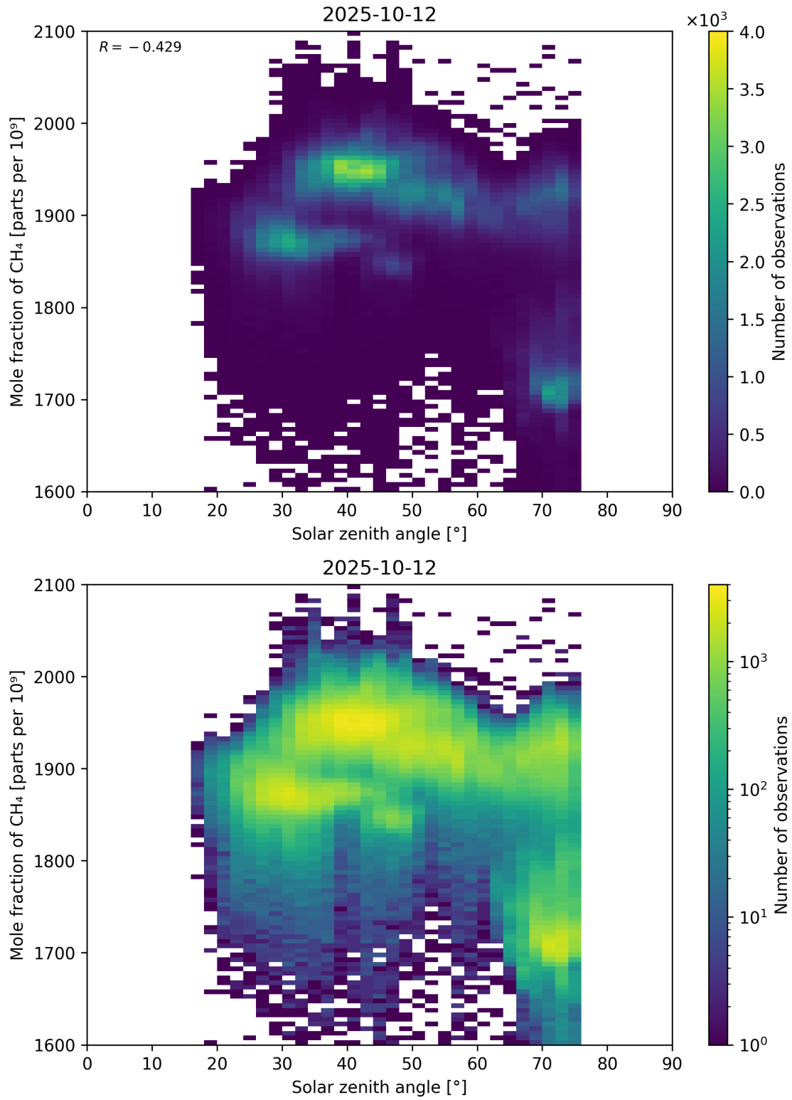
Figure 99: Scatter density plot of “Solar zenith angle” against “Mole fraction of CH 4 ” for 2025-10-11 to 2025-10-13.
