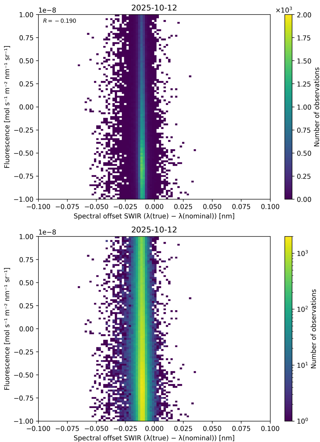
Figure 120: Scatter density plot of “Spectral offset SWIR ( \lambda_{\text{true}} - \lambda_{\text{nominal}} )” against “Fluorescence” for 2025-10-11 to 2025-10-13.
