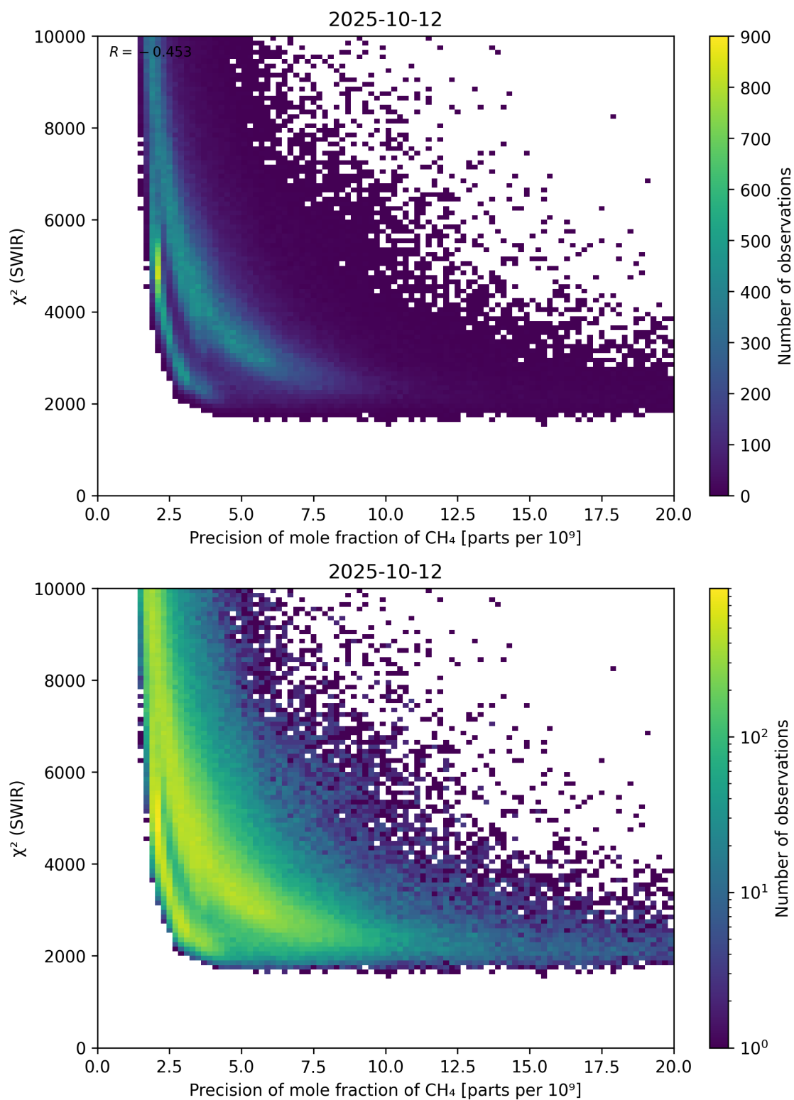
Figure 79: Scatter density plot of “Precision of mole fraction of CH 4 ” against “ \chi^2 (SWIR)” for 2025-10-11 to 2025-10-13.
