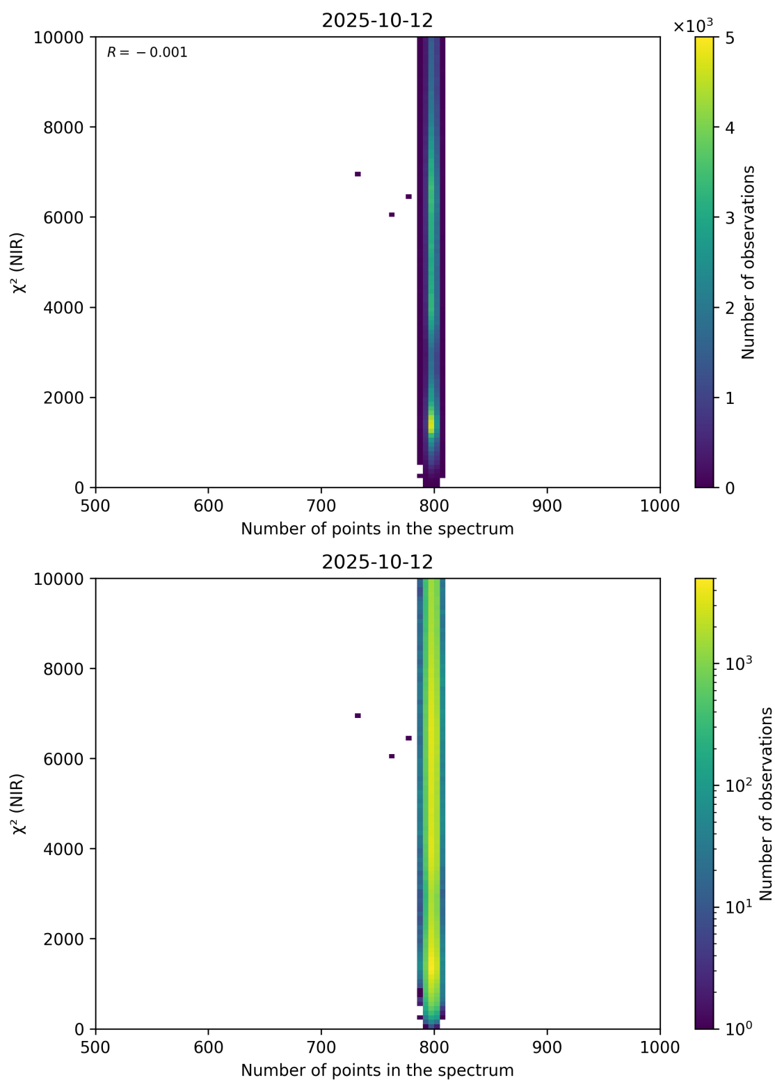
Figure 88: Scatter density plot of “Number of points in the spectrum” against “ \chi^2 (NIR)” for 2025-10-11 to 2025-10-13.
