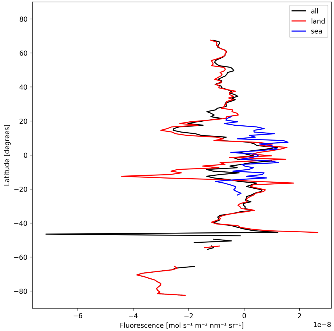
Figure 21: Zonal average of “Fluorescence” for 2025-10-11 to 2025-10-13.
