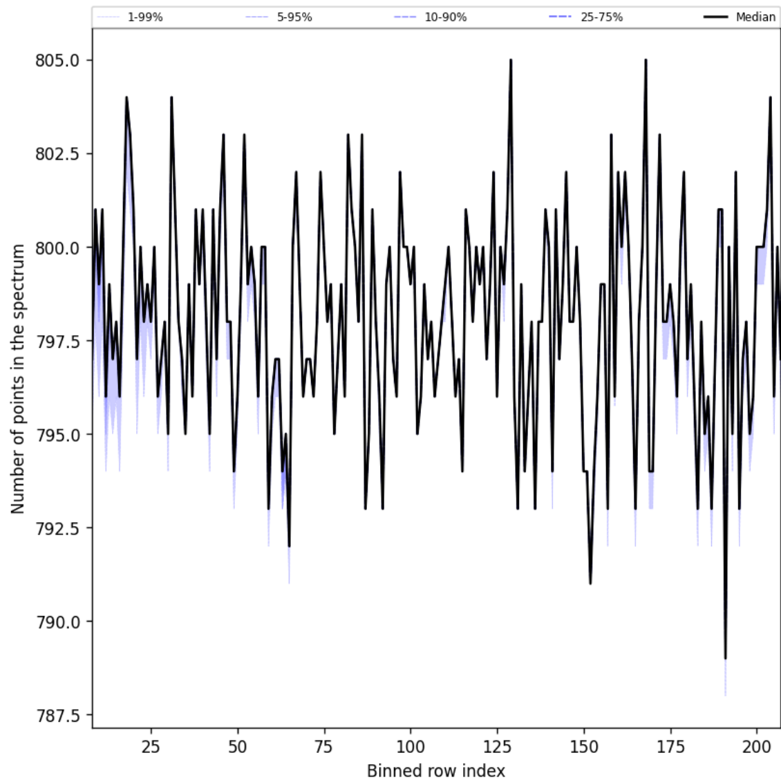
Figure 37: Along track statistics of “Number of points in the spectrum” for 2025-10-11 to 2025-10-13
