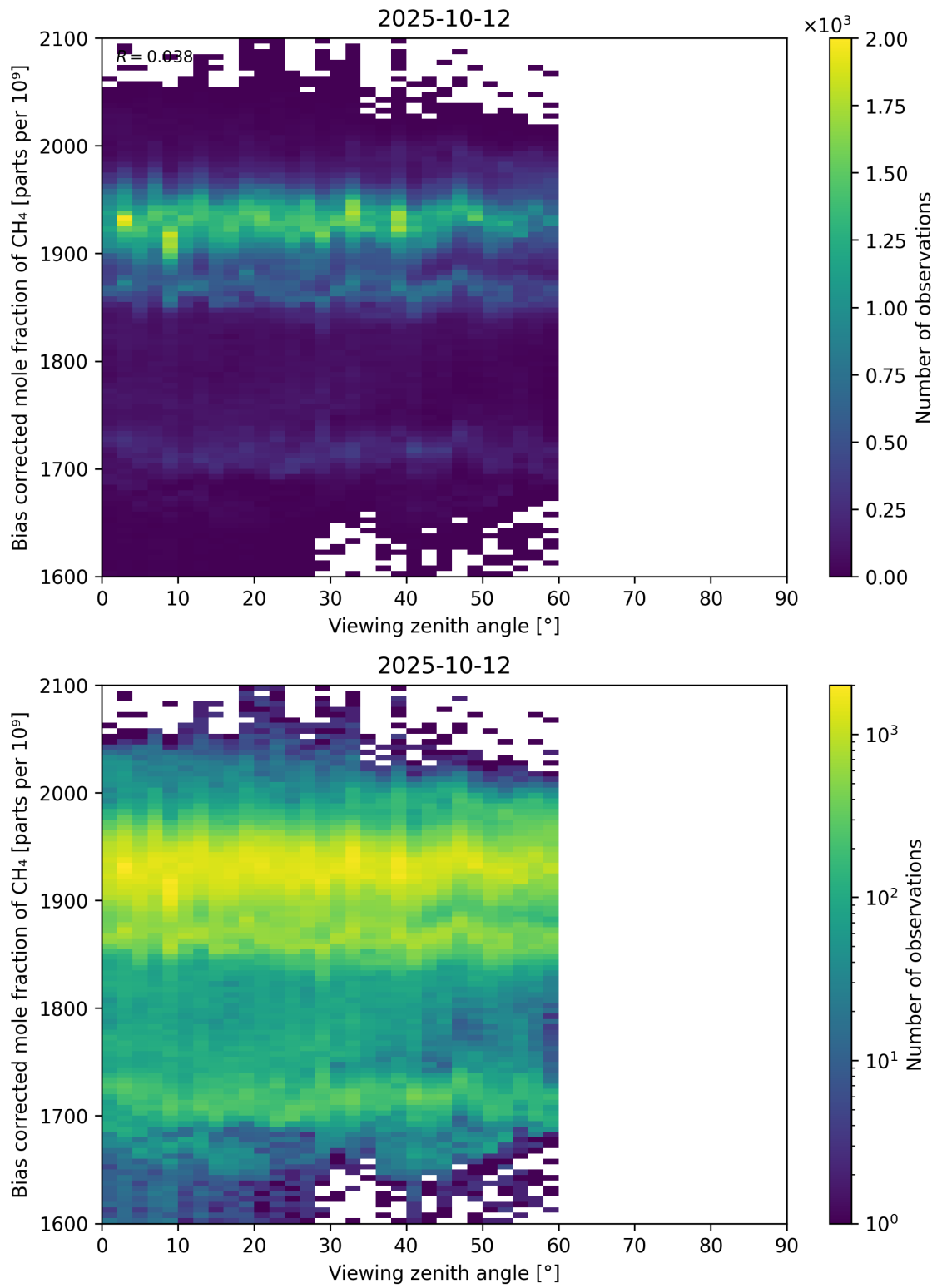
Figure 111: Scatter density plot of “Viewing zenith angle” against “Bias corrected mole fraction of CH 4 ” for 2025-10-11 to 2025-10-13.
