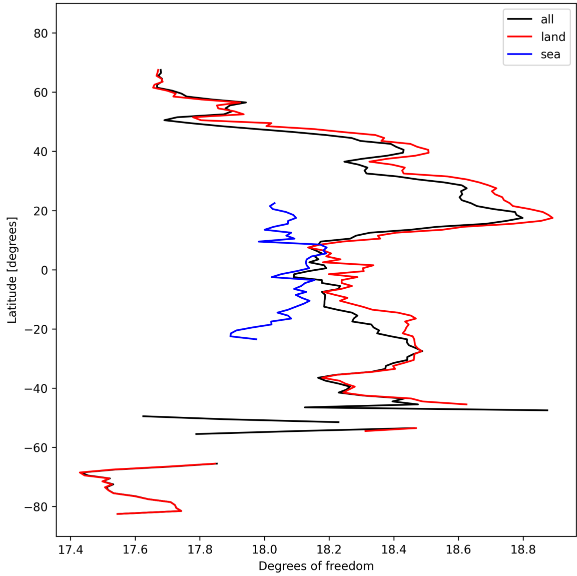
Figure 19: Zonal average of “Degrees of freedom” for 2025-10-11 to 2025-10-13.
