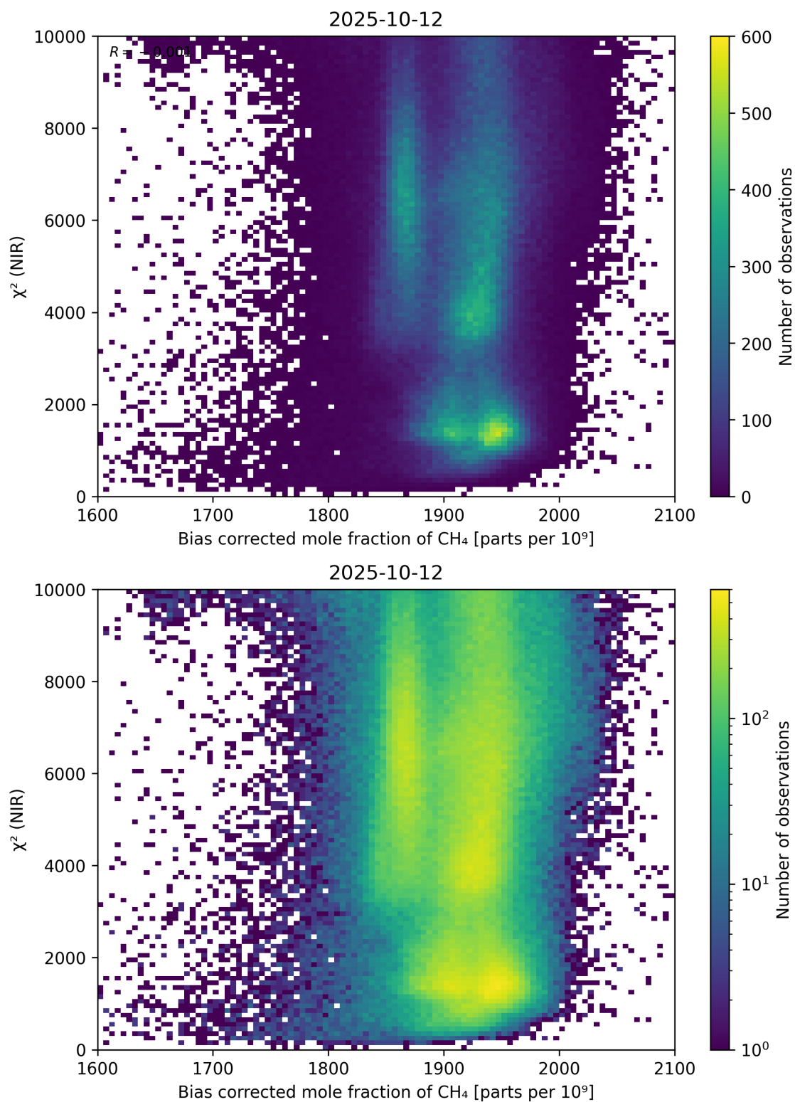
Figure 63: Scatter density plot of “Bias corrected mole fraction of \text{CH}_4 ” against “ \chi^2 (NIR)” for 2025-10-11 to 2025-10-13.
