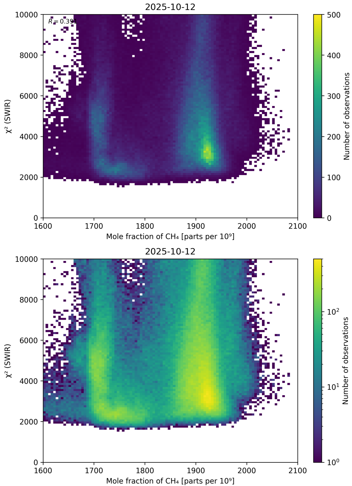
Figure 71: Scatter density plot of “Mole fraction of \text{CH}_4 ” against “ \chi^2 (SWIR)” for 2025-10-11 to 2025-10-13.
