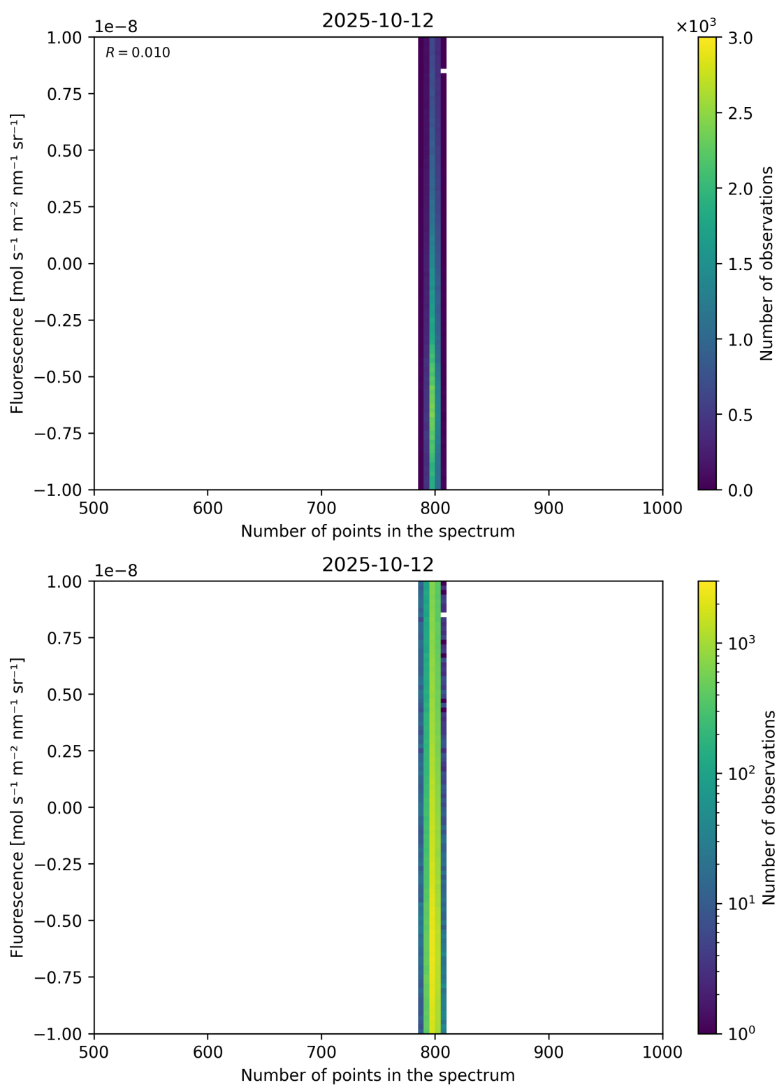
Figure 91: Scatter density plot of “Number of points in the spectrum” against “Fluorescence” for 2025-10-11 to 2025-10-13.
