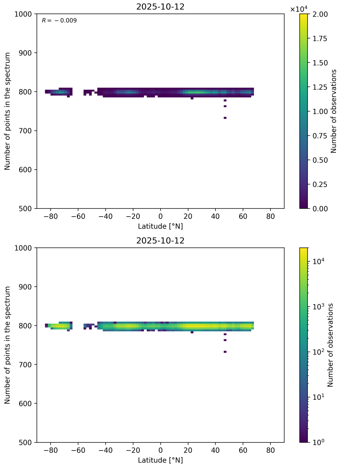
Figure 61: Scatter density plot of “Latitude” against “Number of points in the spectrum” for 2025-10-11 to 2025-10-13.
