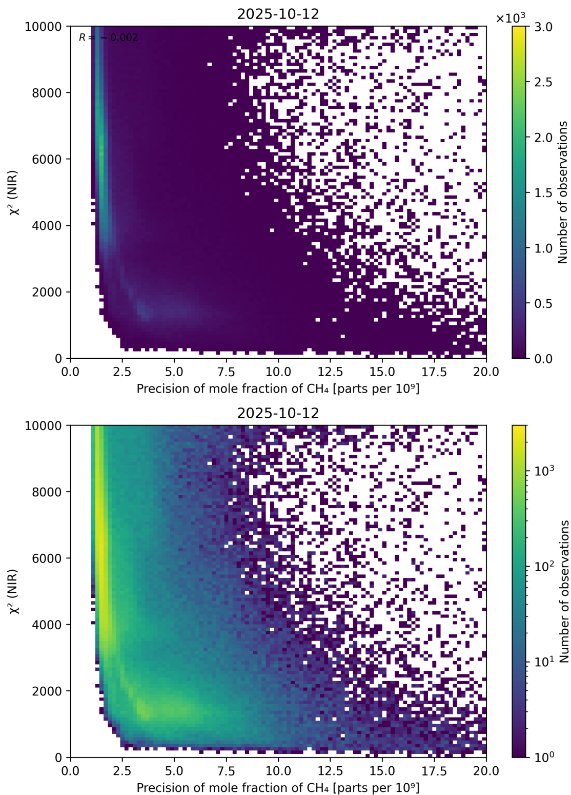
Figure 78: Scatter density plot of “Precision of mole fraction of CH 4 ” against “ \chi^2 (NIR)” for 2025-10-11 to 2025-10-13.
