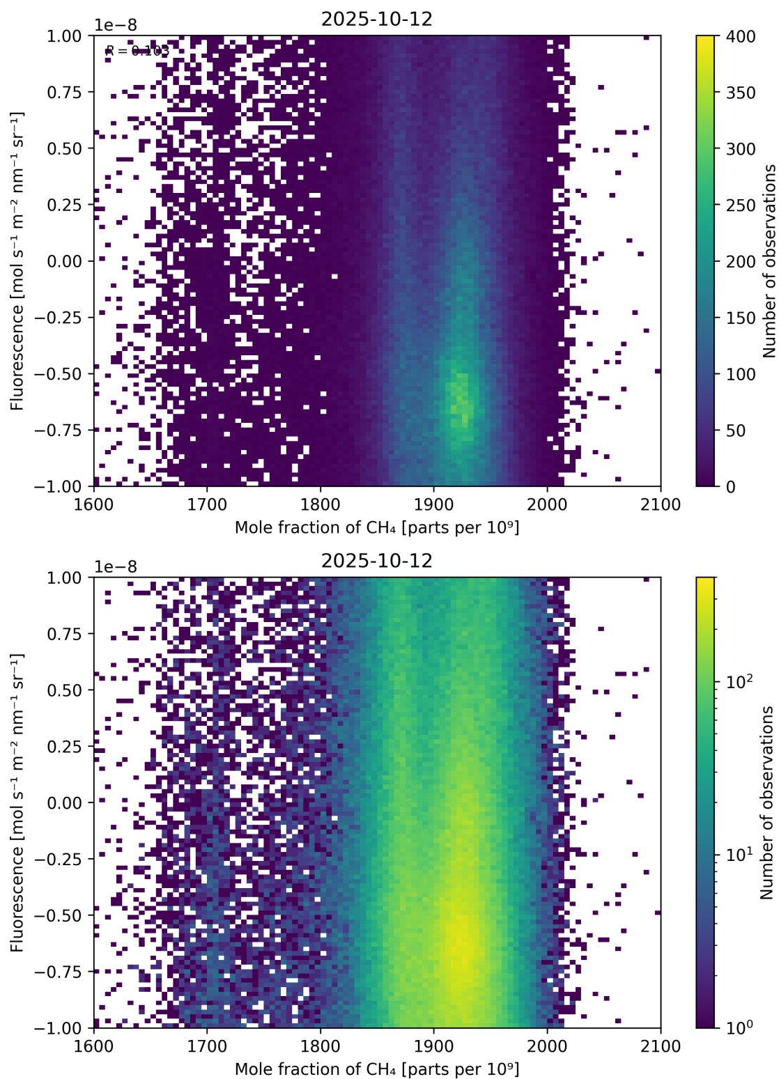
Figure 73: Scatter density plot of “Mole fraction of \text{CH}_4 ” against “Fluorescence” for 2025-10-11 to 2025-10-13.
