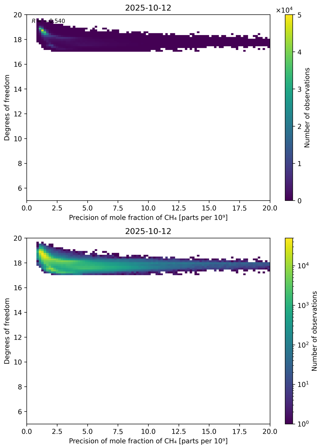
Figure 80: Scatter density plot of “Precision of mole fraction of CH 4 ” against “Degrees of freedom” for 2025-10-11 to 2025-10-13.
