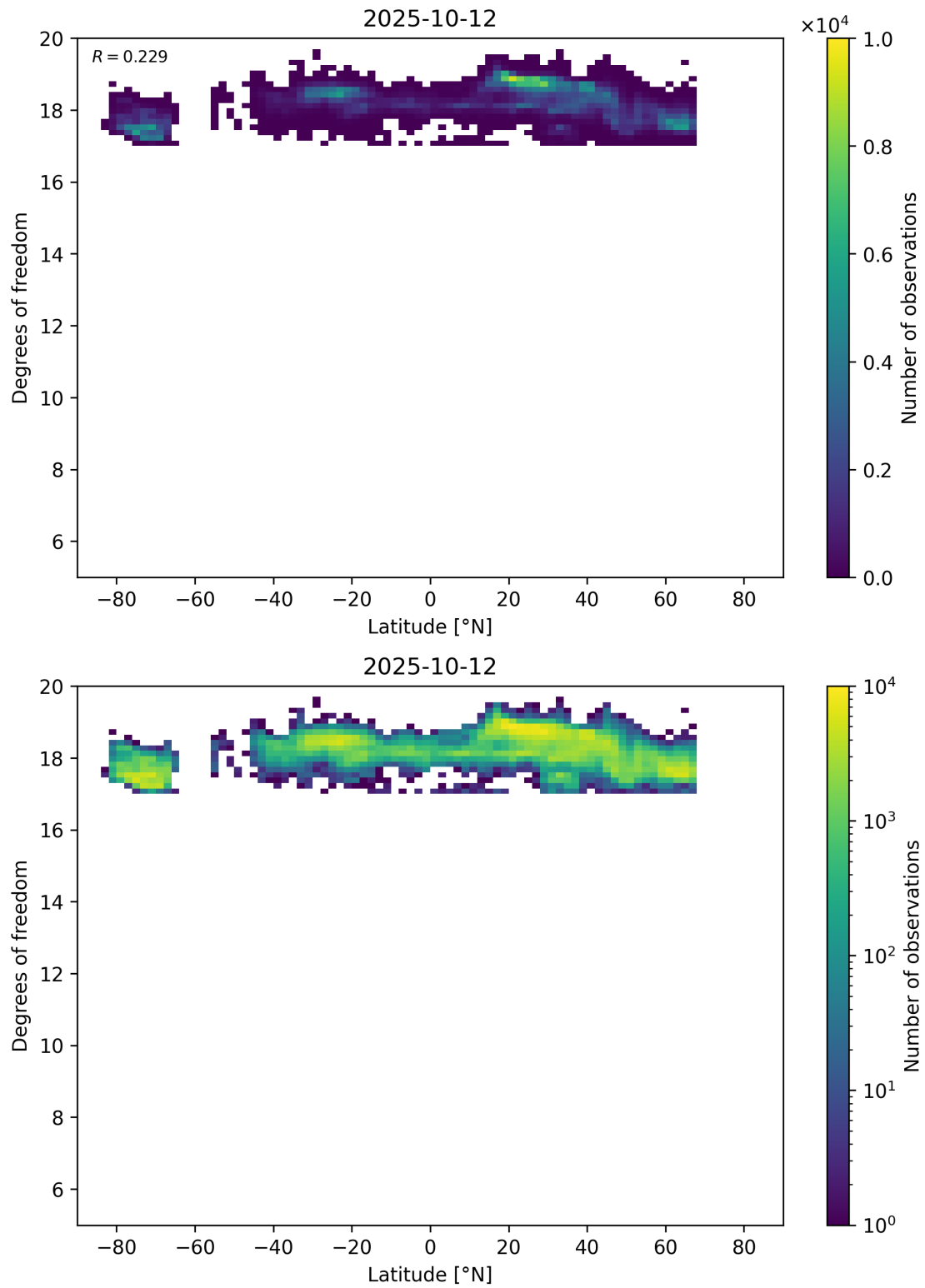
Figure 55: Scatter density plot of “Latitude” against “Degrees of freedom” for 2025-10-11 to 2025-10-13.
