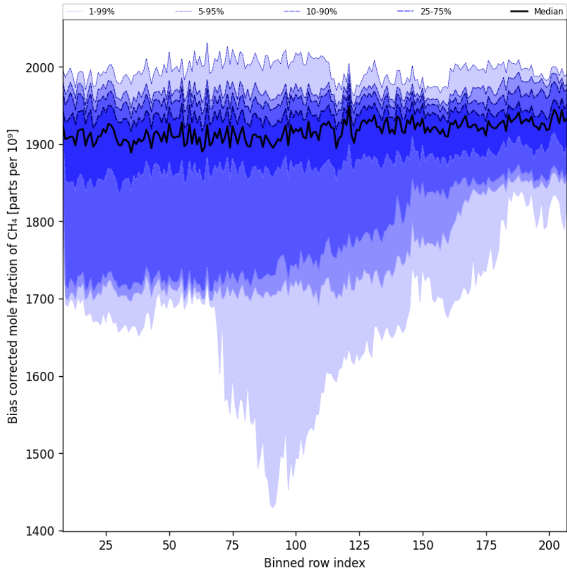
Figure 36: Along track statistics of “Bias corrected mole fraction of CH 4 ” for 2025-10-11 to 2025-10-13
