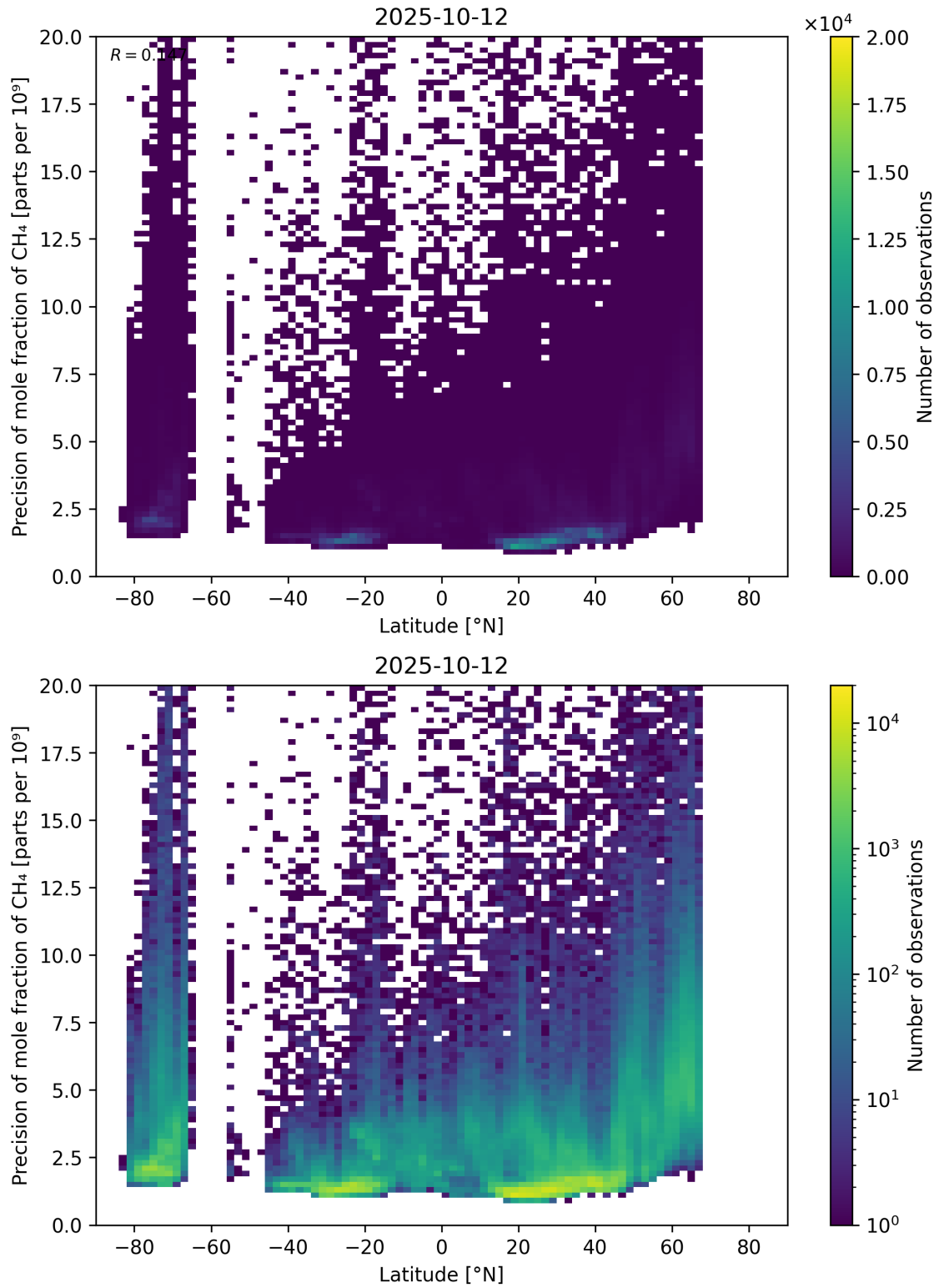
Figure 59: Scatter density plot of “Latitude” against “Precision of mole fraction of CH 4 ” for 2025-10-11 to 2025-10-13.
