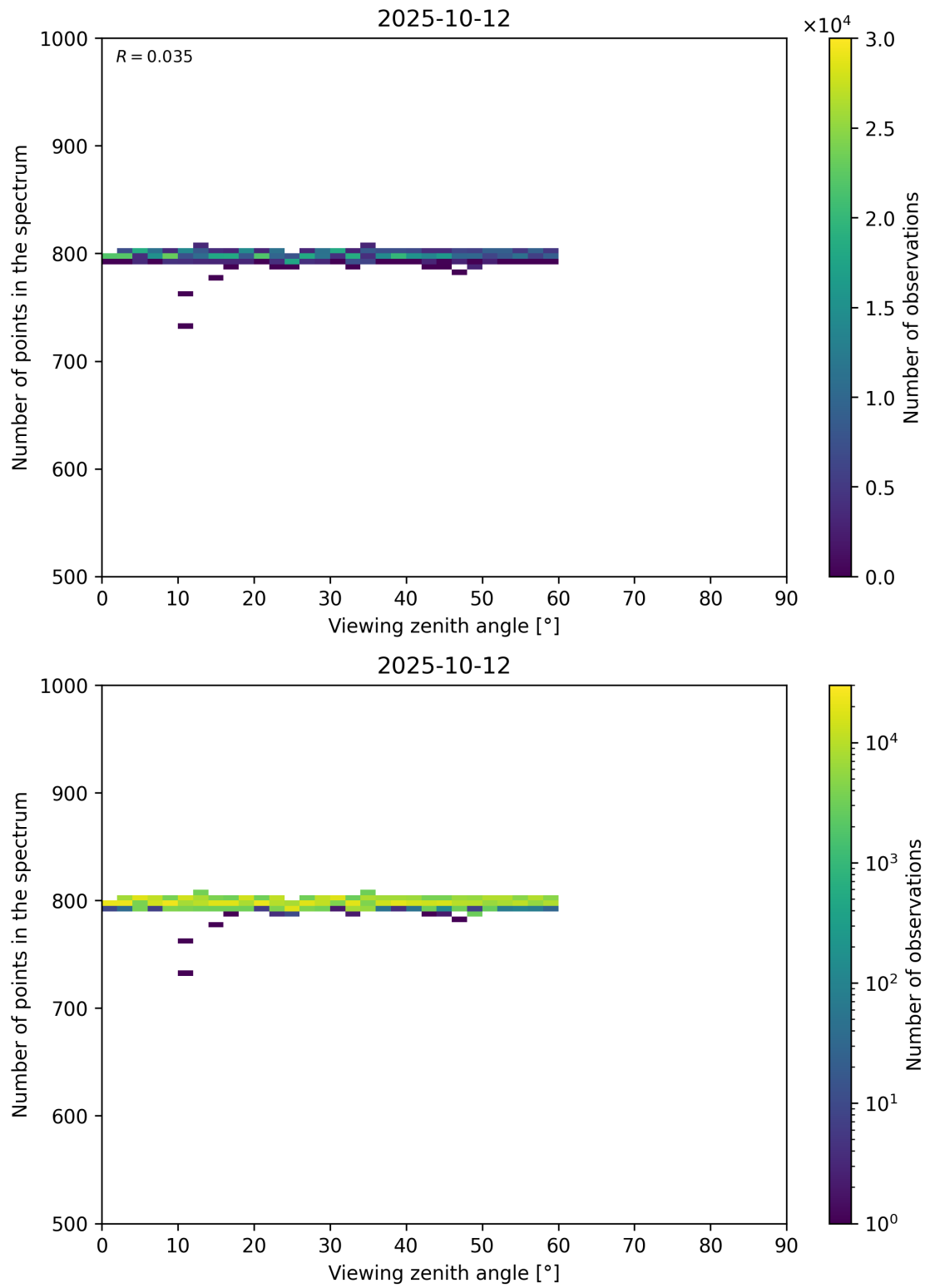
Figure 114: Scatter density plot of “Viewing zenith angle” against “Number of points in the spectrum” for 2025-10-11 to 2025-10-13.
