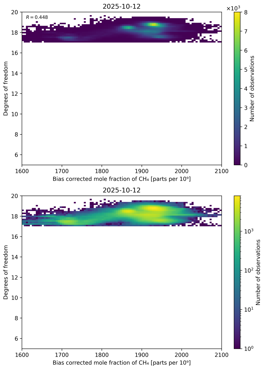
Figure 65: Scatter density plot of “Bias corrected mole fraction of CH 4 ” against “Degrees of freedom” for 2025-10-11 to 2025-10-13.
