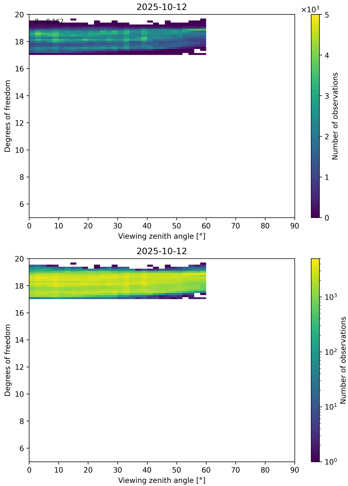
Figure 107: Scatter density plot of “Viewing zenith angle” against “Degrees of freedom” for 2025-10-11 to 2025-10-13.
