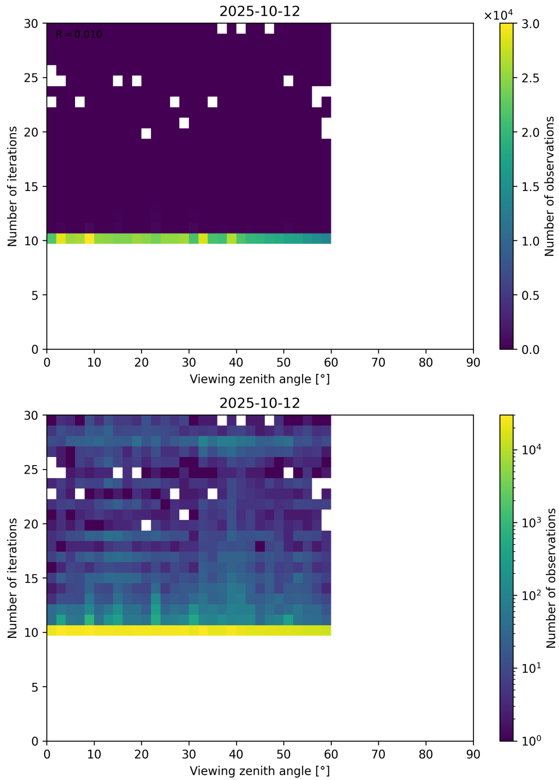
Figure 113: Scatter density plot of “Viewing zenith angle” against “Number of iterations” for 2025-10-11 to 2025-10-13.
