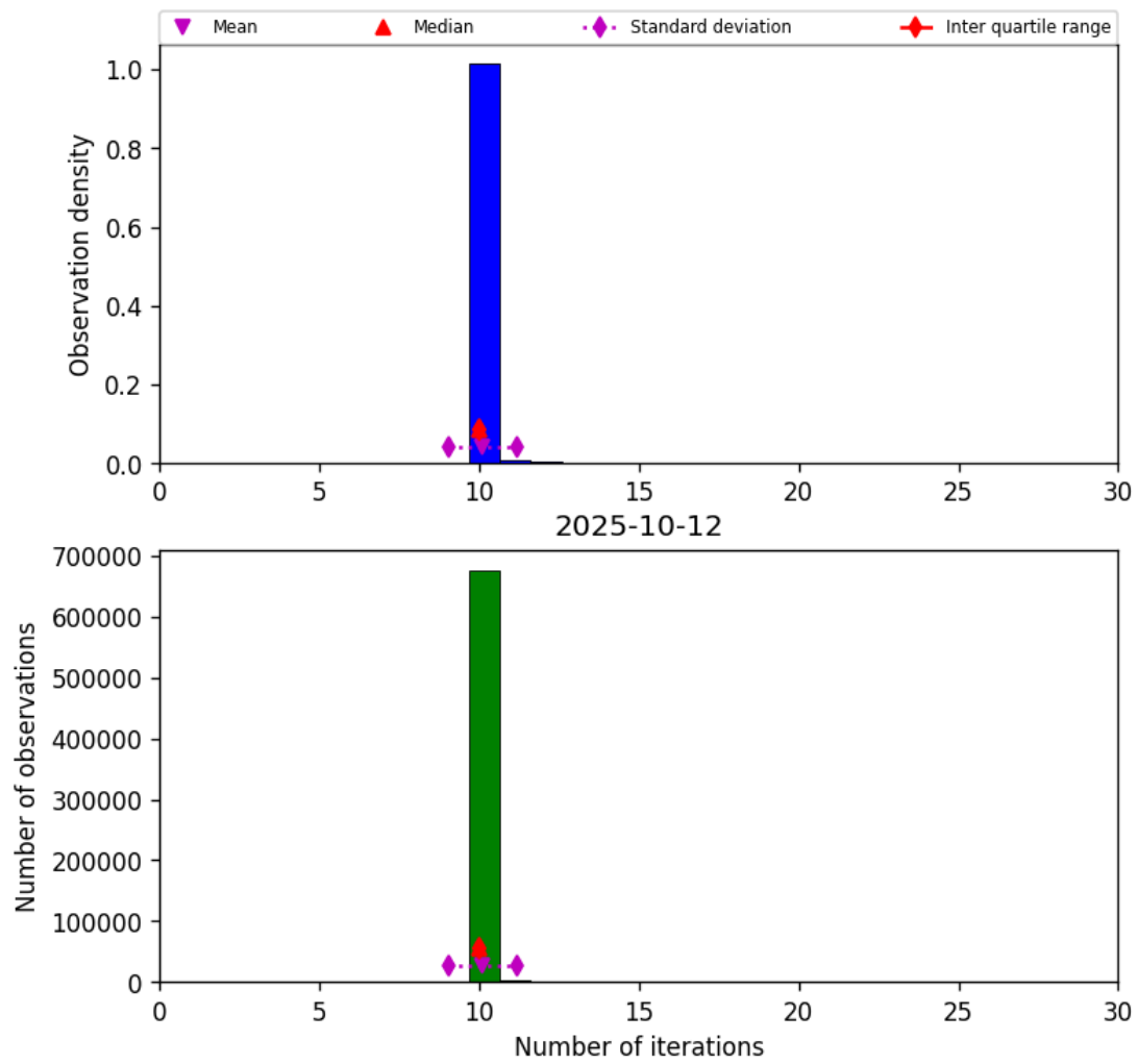
Figure 31: Histogram of “Number of iterations” for 2025-10-11 to 2025-10-13
