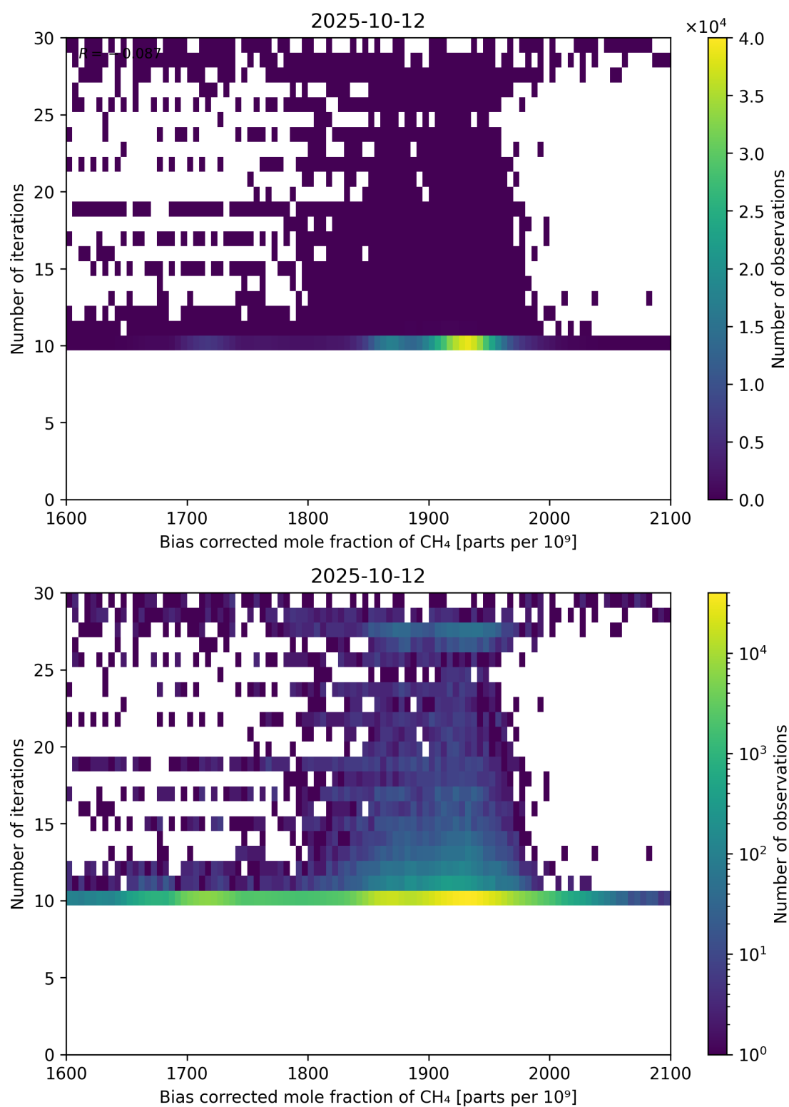
Figure 67: Scatter density plot of “Bias corrected mole fraction of \text{CH}_4 ” against “Number of iterations” for 2025-10-11 to 2025-10-13.
