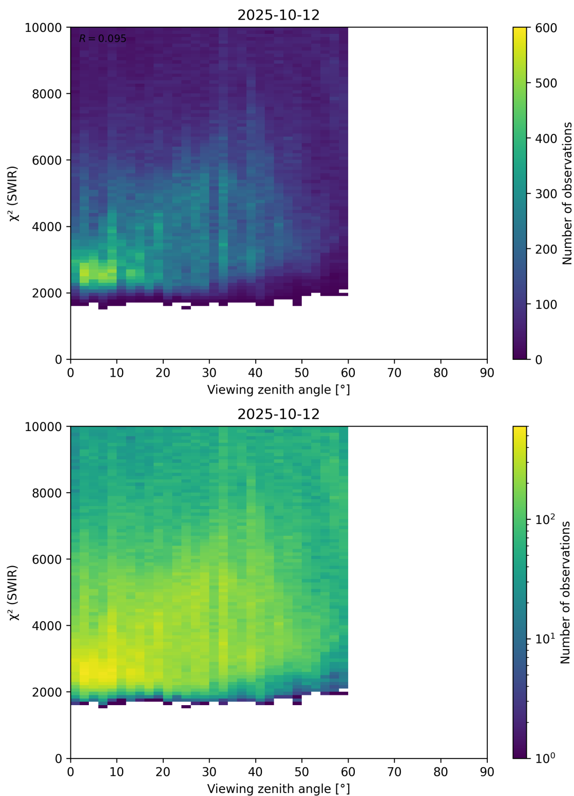
Figure 106: Scatter density plot of “Viewing zenith angle” against “ \chi^2 (SWIR)” for 2025-10-11 to 2025-10-13.
