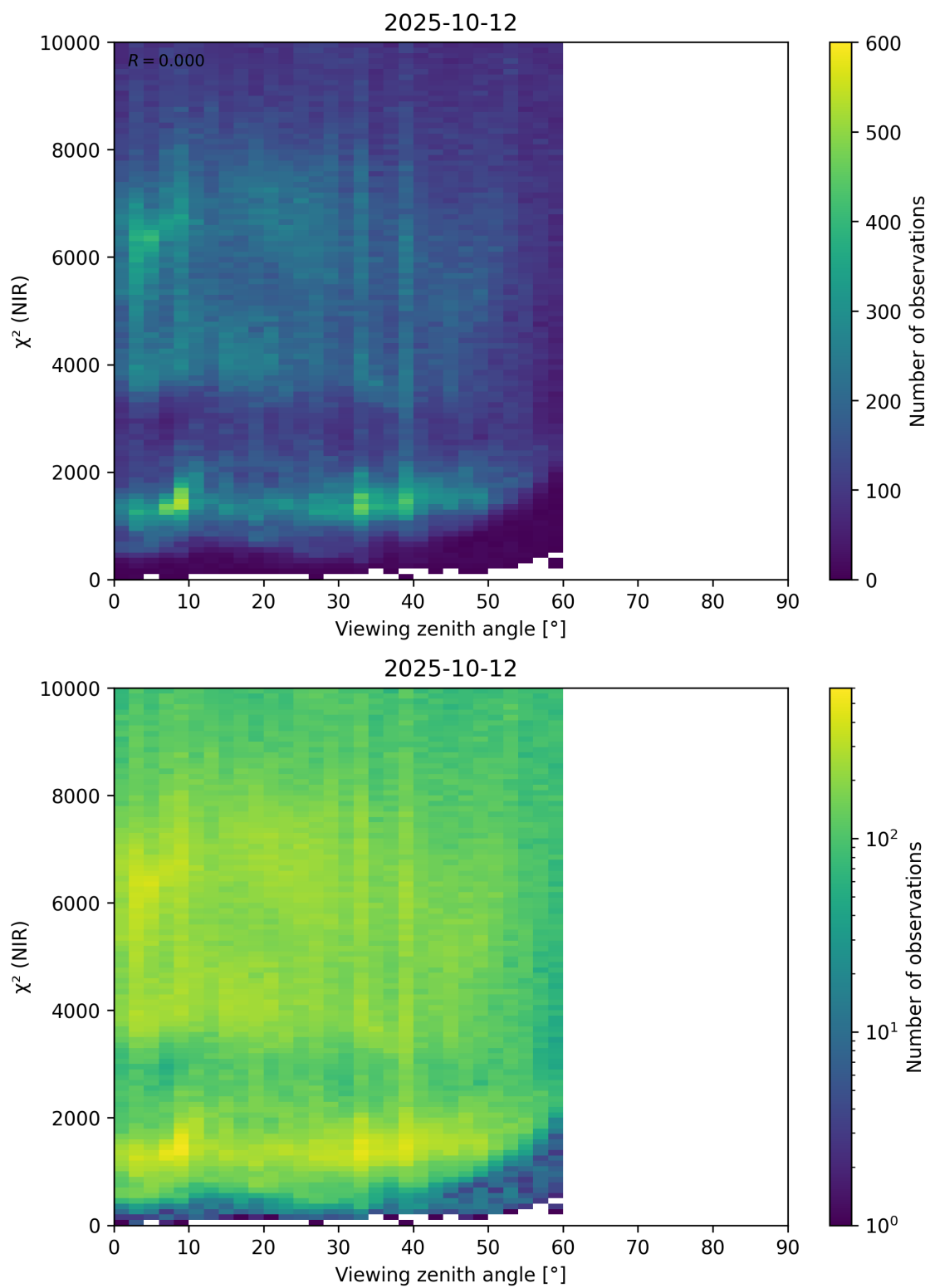
Figure 105: Scatter density plot of “Viewing zenith angle” against “ \chi^2 (NIR)” for 2025-10-11 to 2025-10-13.
