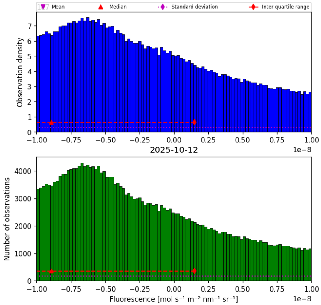
Figure 32: Histogram of “Fluorescence” for 2025-10-11 to 2025-10-13
