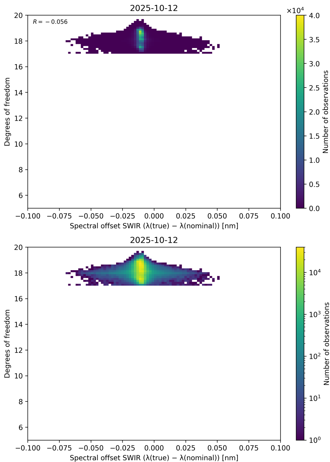
Figure 119: Scatter density plot of “Spectral offset SWIR ( \lambda_{\text{true}} - \lambda_{\text{nominal}} )” against “Degrees of freedom” for 2025-10-11 to 2025-10-13.
