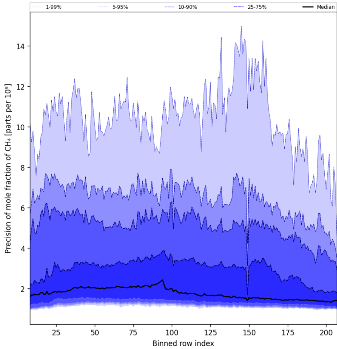
Figure 35: Along track statistics of “Precision of mole fraction of CH 4 ” for 2025-10-11 to 2025-10-13
