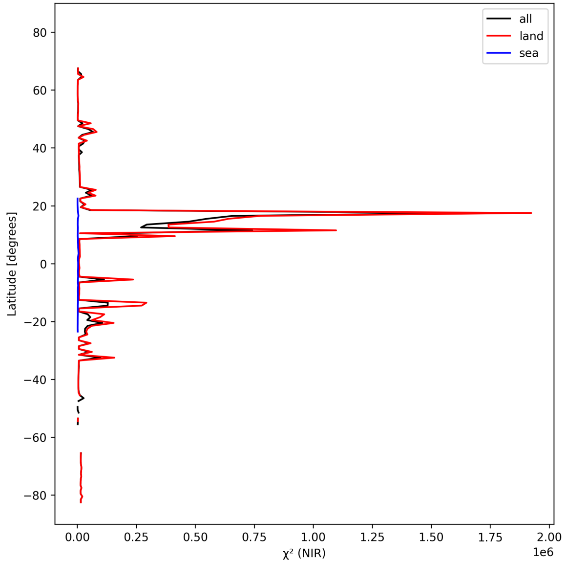
Figure 18: Zonal average of “ \chi^2 (NIR)” for 2025-10-11 to 2025-10-13.
