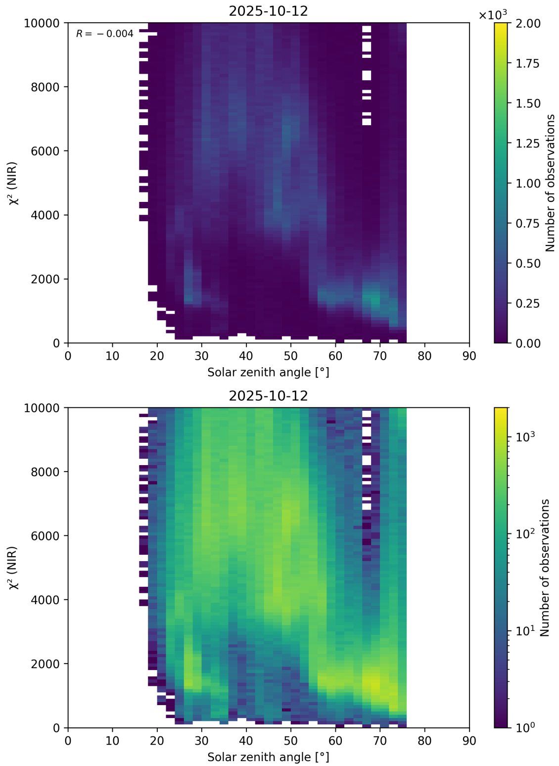
Figure 94: Scatter density plot of “Solar zenith angle” against “ \chi^2 (NIR)” for 2025-10-11 to 2025-10-13.
