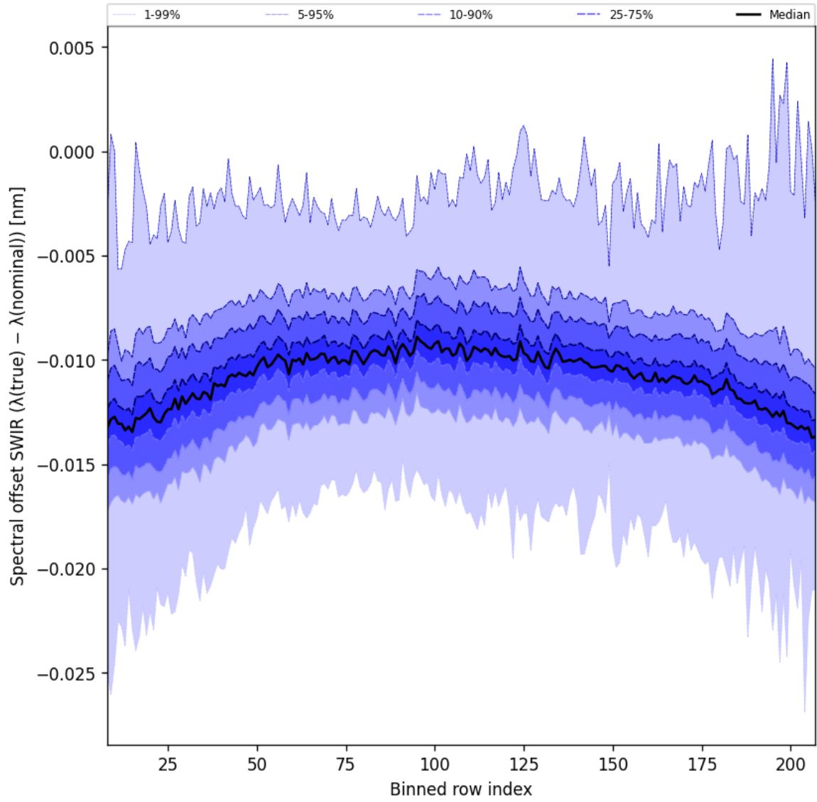
Figure 38: Along track statistics of “Spectral offset SWIR ( \lambda_{\text{true}} - \lambda_{\text{nominal}} )” for 2025-10-11 to 2025-10-13
