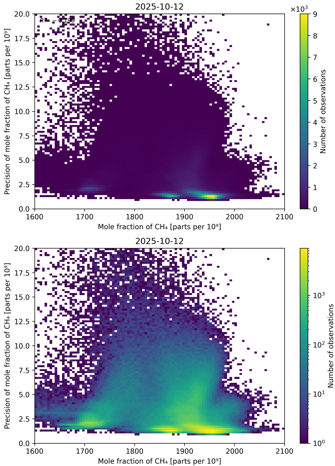
Figure 75: Scatter density plot of “Mole fraction of CH 4 ” against “Precision of mole fraction of CH 4 ” for 2025-10-11 to 2025-10-13.
