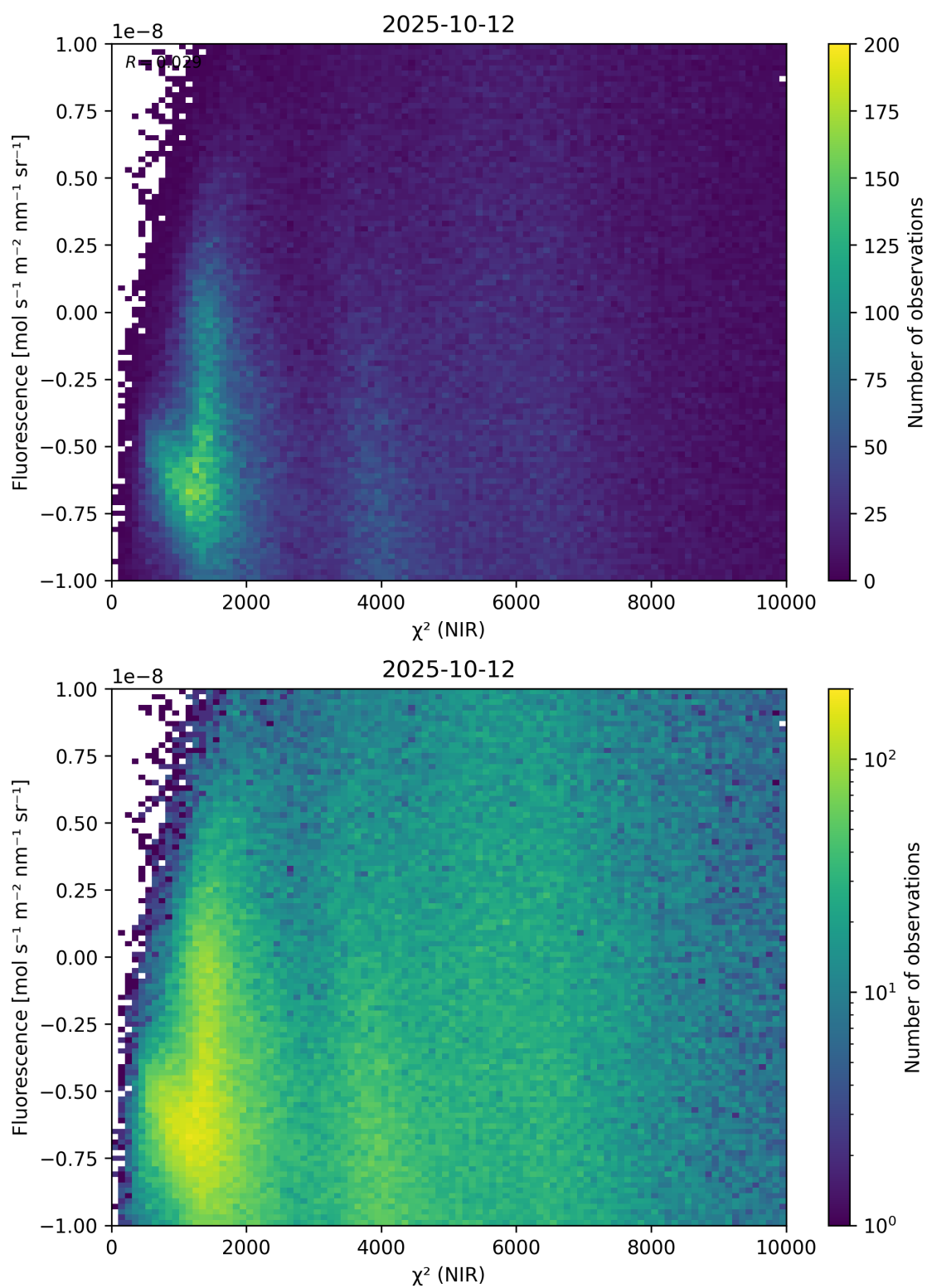
Figure 45: Scatter density plot of “ \chi^2 (NIR)” against “Fluorescence” for 2025-10-11 to 2025-10-13.
