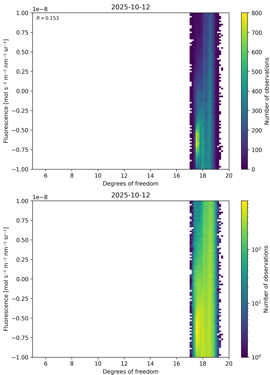
Figure 51: Scatter density plot of “Degrees of freedom” against “Fluorescence” for 2025-10-11 to 2025-10-13.
