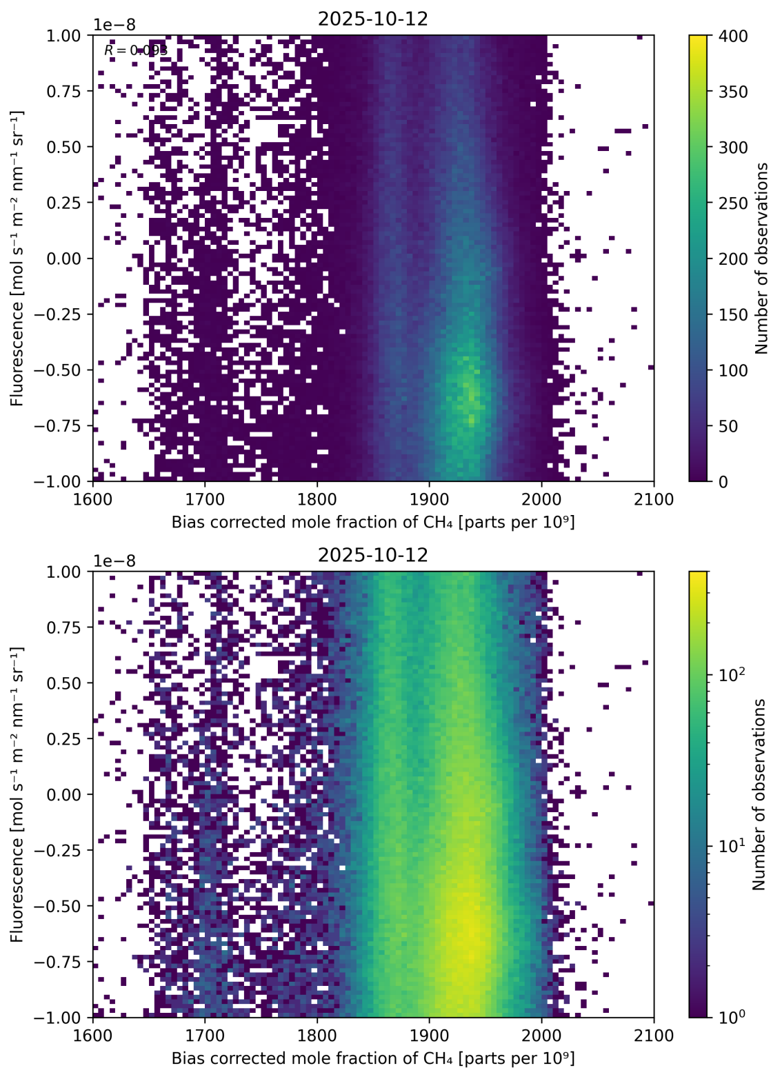
Figure 66: Scatter density plot of “Bias corrected mole fraction of CH 4 ” against “Fluorescence” for 2025-10-11 to 2025-10-13.
