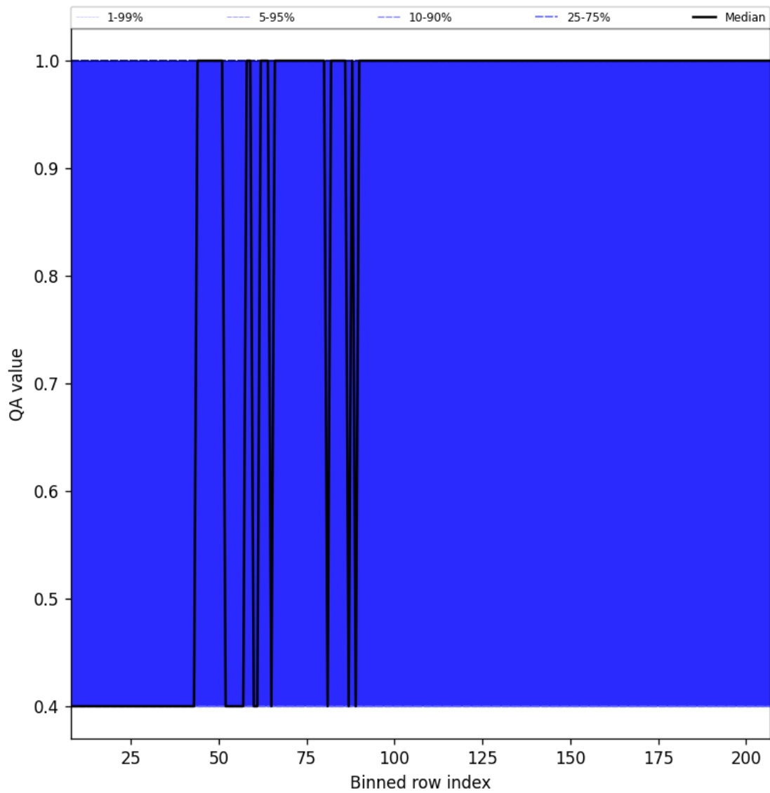
Figure 33: Along track statistics of “QA value” for 2025-10-11 to 2025-10-13
