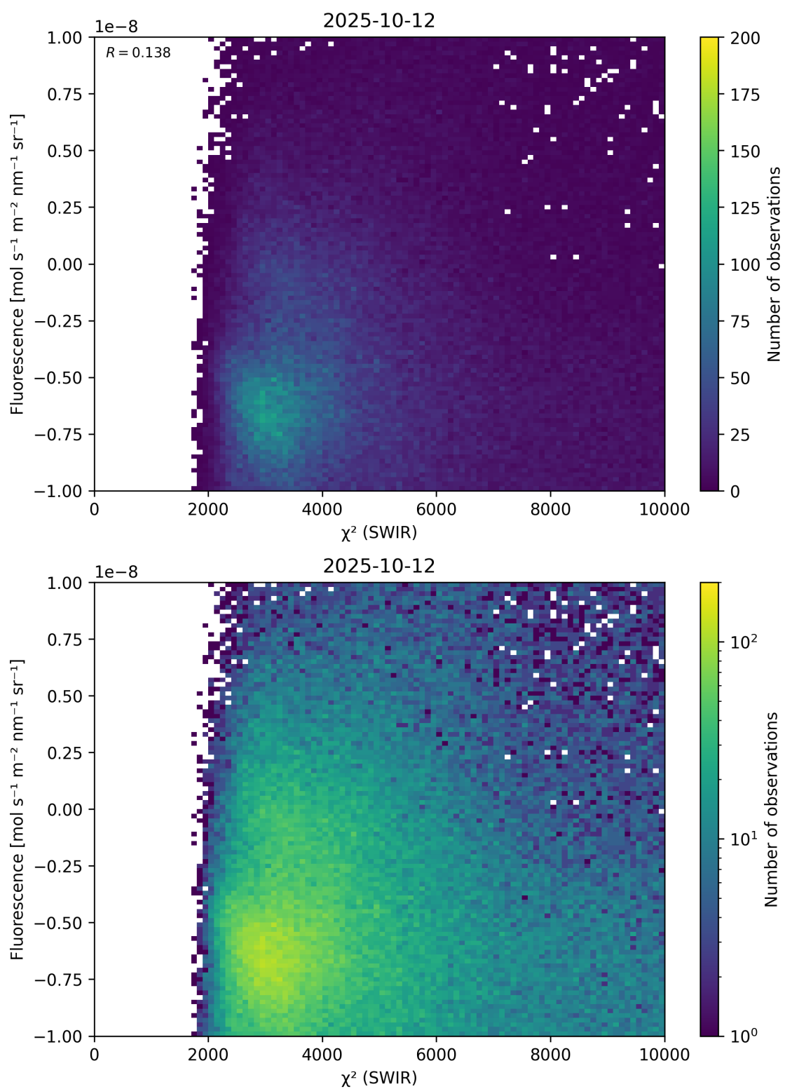
Figure 49: Scatter density plot of “ \chi^2 (SWIR)” against “Fluorescence” for 2025-10-11 to 2025-10-13.
