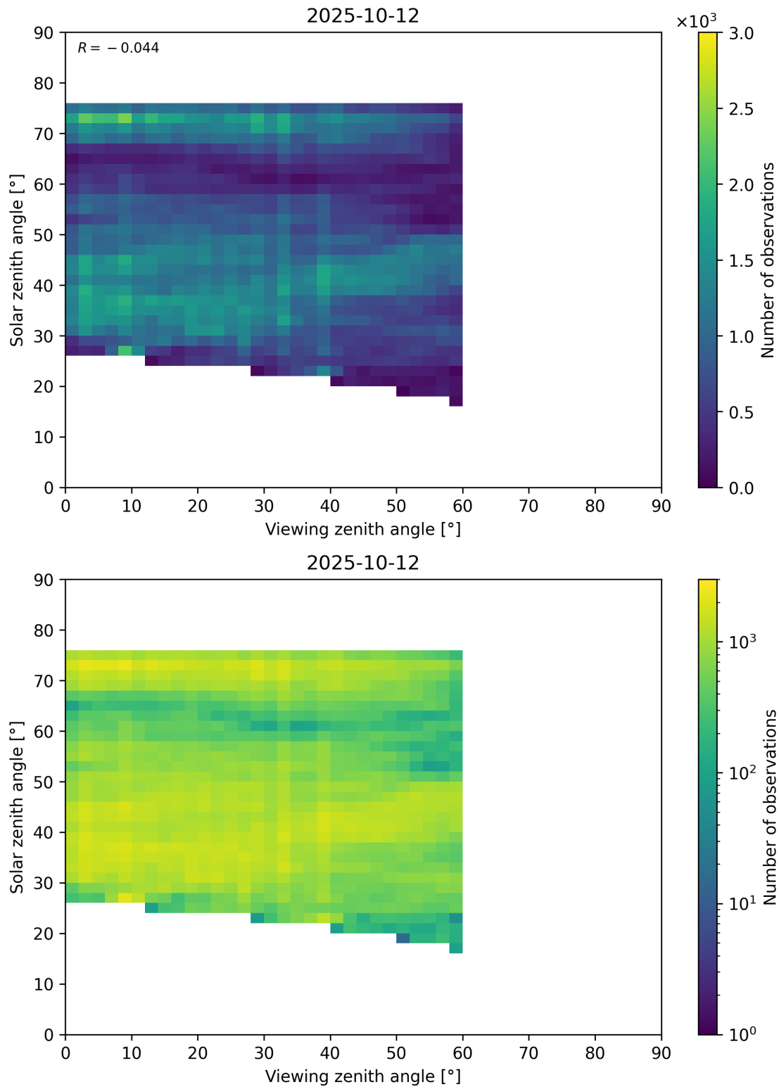
Figure 115: Scatter density plot of “Viewing zenith angle” against “Solar zenith angle” for 2025-10-11 to 2025-10-13.
