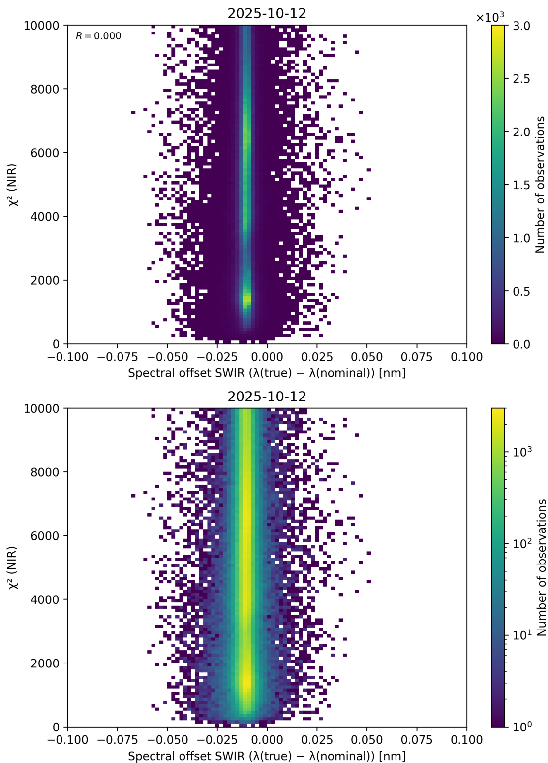
Figure 117: Scatter density plot of “Spectral offset SWIR ( \lambda_{\text{true}} - \lambda_{\text{nominal}} )” against “ \chi^2 (NIR)” for 2025-10-11 to 2025-10-13.
