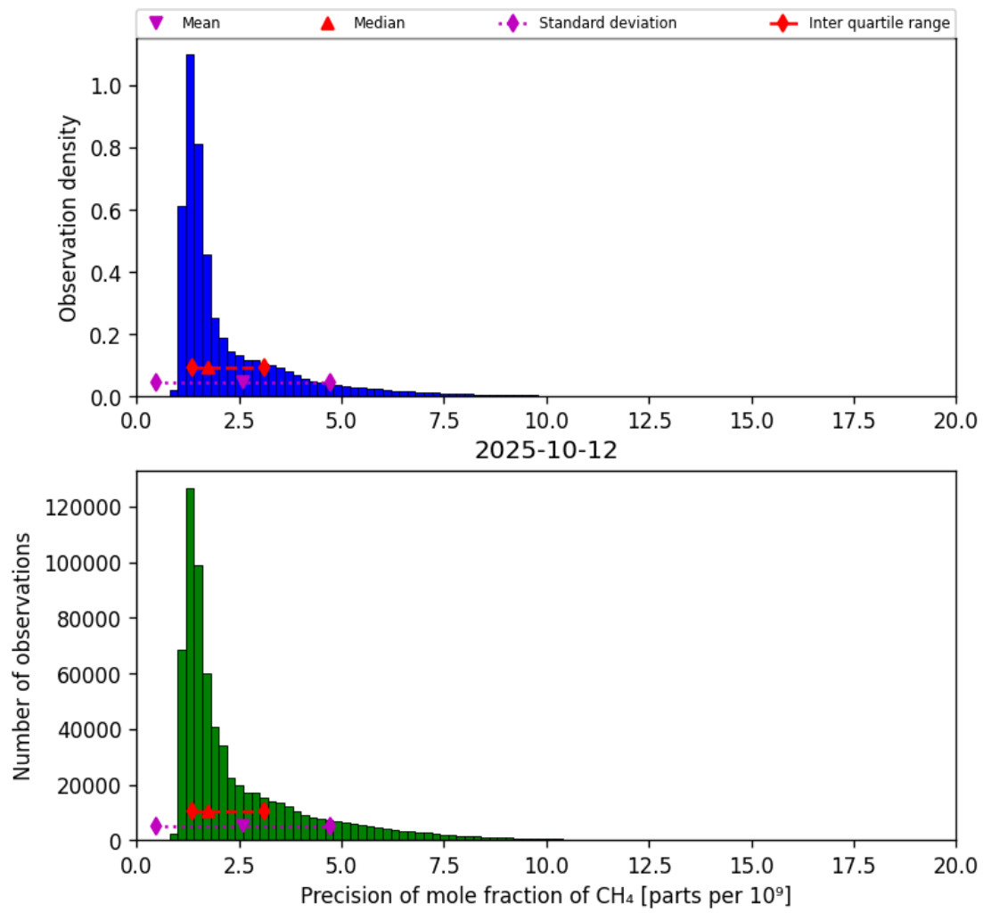
Figure 24: Histogram of “Precision of mole fraction of CH 4 ” for 2025-10-11 to 2025-10-13
