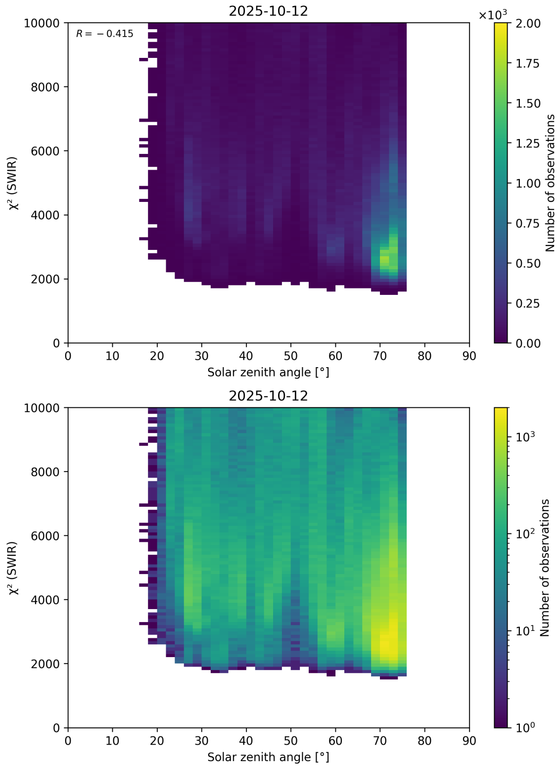
Figure 95: Scatter density plot of “Solar zenith angle” against “ \chi^2 (SWIR)” for 2025-10-11 to 2025-10-13.
