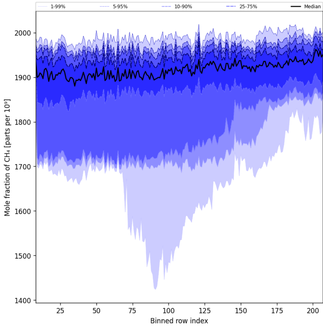
Figure 34: Along track statistics of “Mole fraction of CH 4 ” for 2025-10-11 to 2025-10-13
