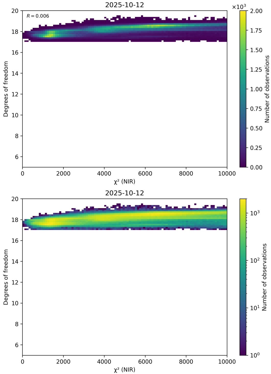
Figure 44: Scatter density plot of “ \chi^2 (NIR)” against “Degrees of freedom” for 2025-10-11 to 2025-10-13.
