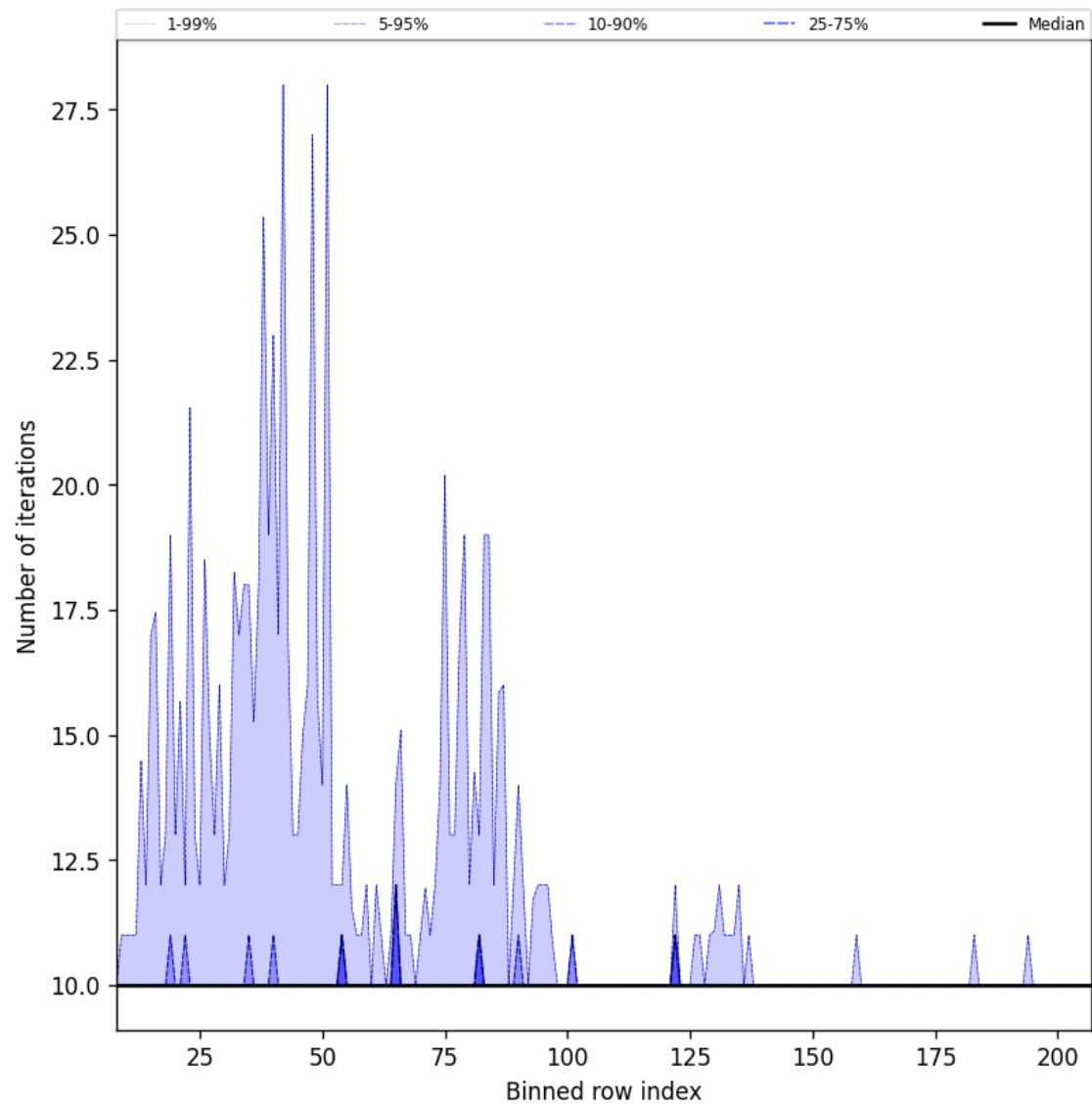
Figure 42: Along track statistics of “Number of iterations” for 2025-10-11 to 2025-10-13
