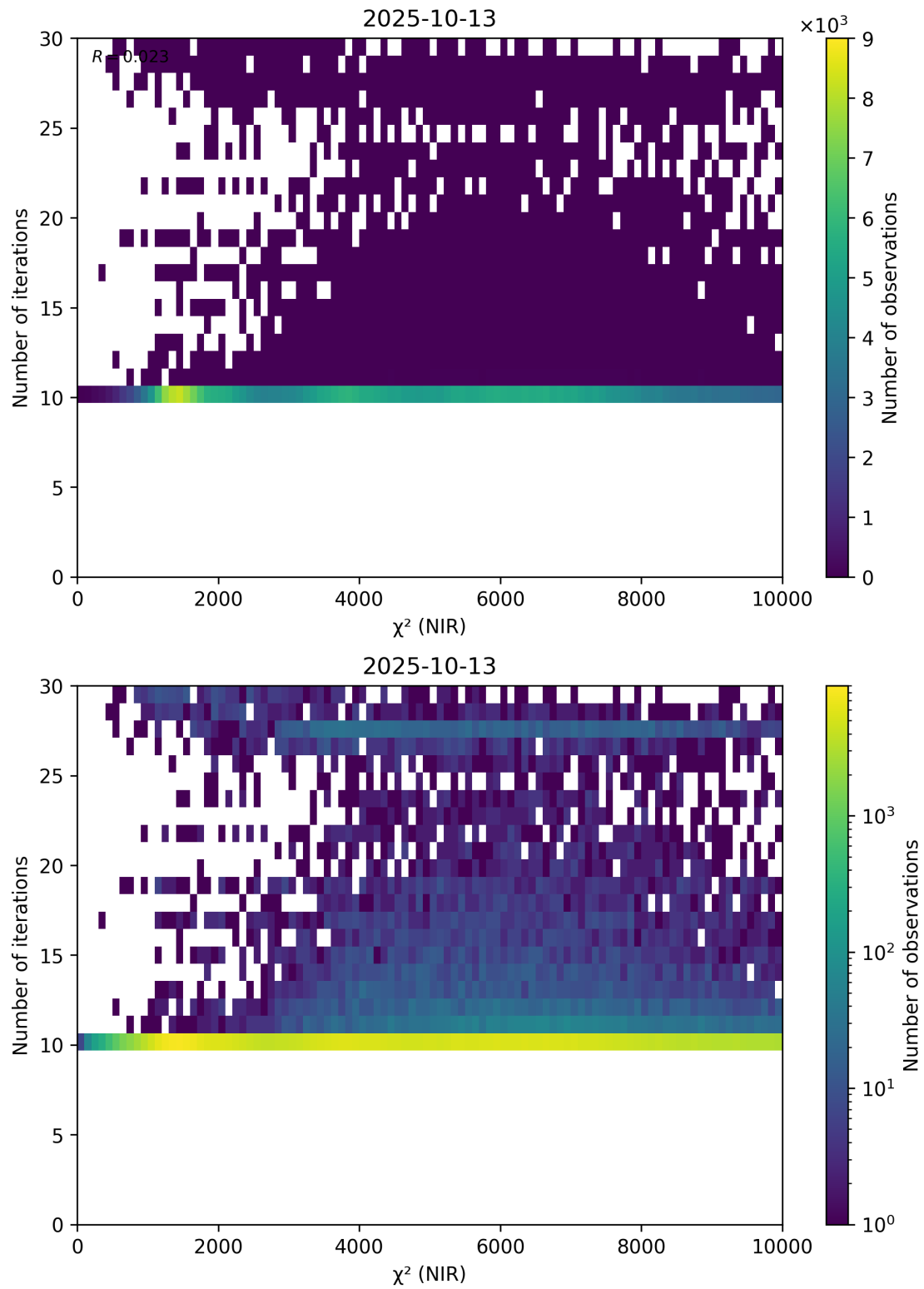
Figure 46: Scatter density plot of “ \chi^2 (NIR)” against “Number of iterations” for 2025-10-12 to 2025-10-14.
