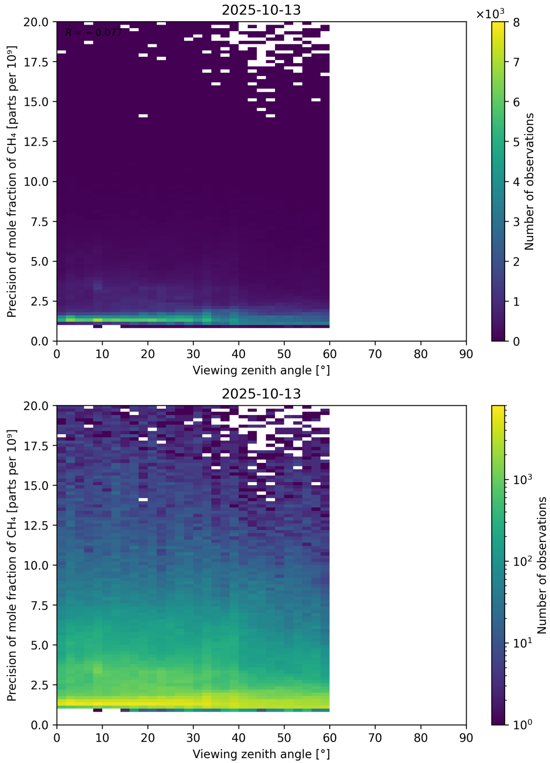
Figure 112: Scatter density plot of “Viewing zenith angle” against “Precision of mole fraction of CH 4 ” for 2025-10-12 to 2025-10-14.
