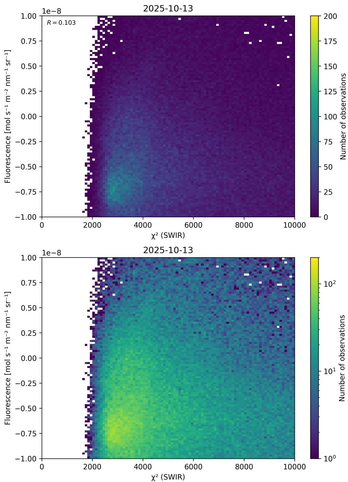
Figure 49: Scatter density plot of “ \chi^2 (SWIR)” against “Fluorescence” for 2025-10-12 to 2025-10-14.
