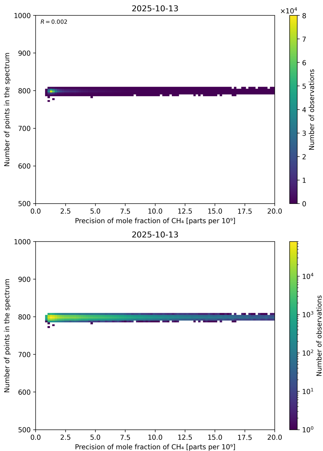
Figure 84: Scatter density plot of “Precision of mole fraction of CH 4 ” against “Number of points in the spectrum” for 2025-10-12 to 2025-10-14.
