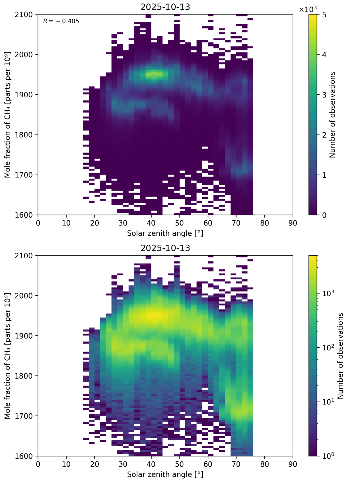
Figure 99: Scatter density plot of “Solar zenith angle” against “Mole fraction of \text{CH}_4 ” for 2025-10-12 to 2025-10-14.
