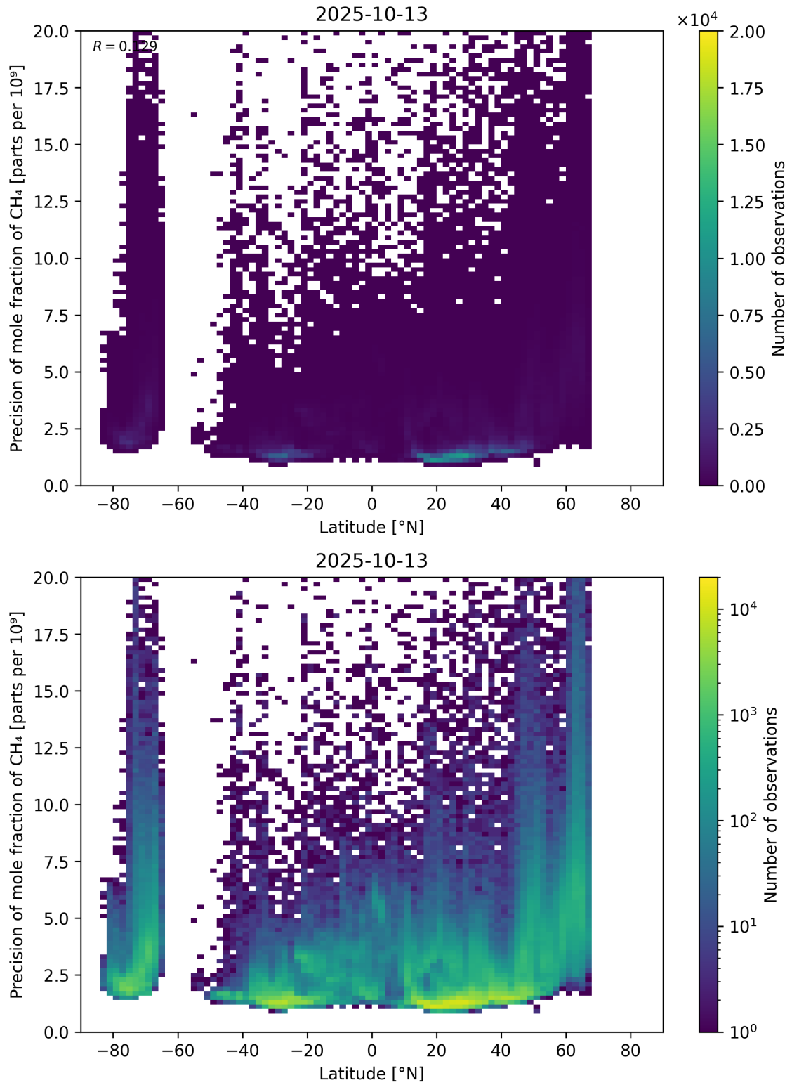
Figure 59: Scatter density plot of “Latitude” against “Precision of mole fraction of \text{CH}_4 ” for 2025-10-12 to 2025-10-14.
