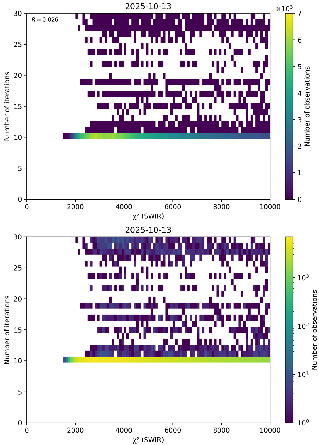
Figure 50: Scatter density plot of “ \chi^2 (SWIR)” against “Number of iterations” for 2025-10-12 to 2025-10-14.
