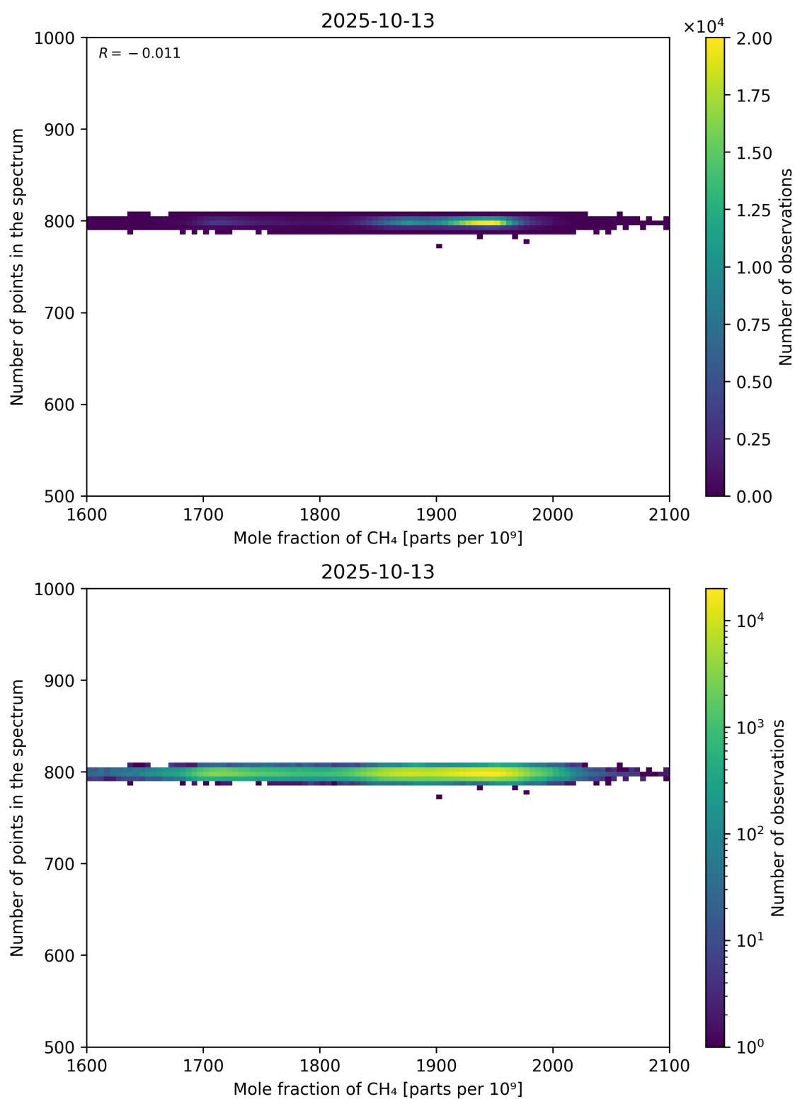
Figure 77: Scatter density plot of “Mole fraction of CH 4 ” against “Number of points in the spectrum” for 2025-10-12 to 2025-10-14.
