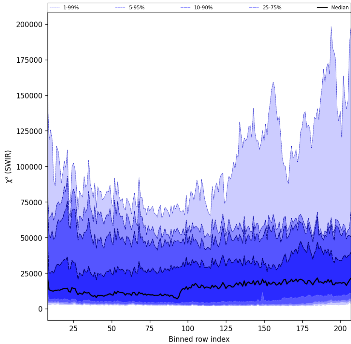
Figure 39: Along track statistics of “ \chi^2 (SWIR)” for 2025-10-12 to 2025-10-14
