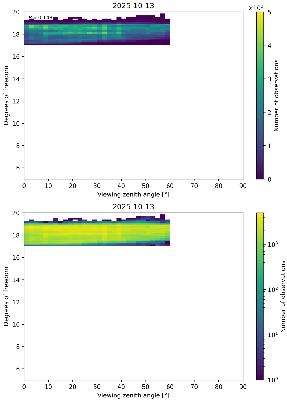
Figure 107: Scatter density plot of “Viewing zenith angle” against “Degrees of freedom” for 2025-10-12 to 2025-10-14.
