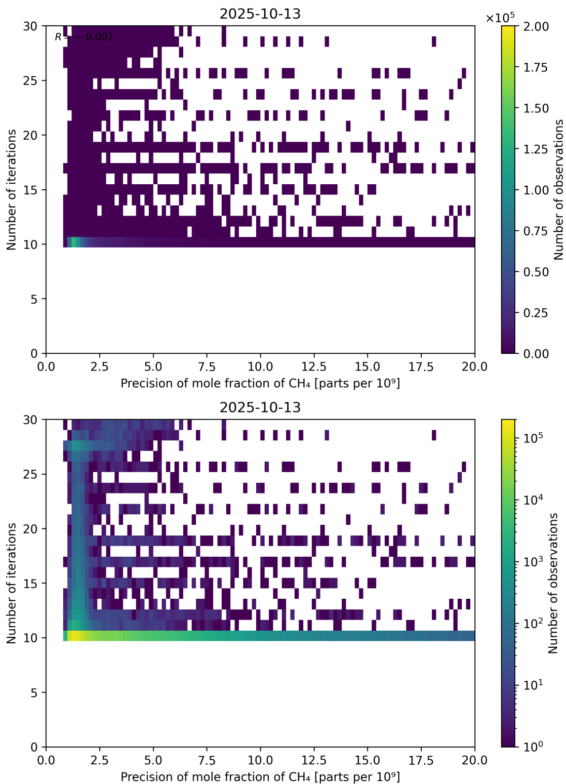
Figure 83: Scatter density plot of “Precision of mole fraction of CH 4 ” against “Number of iterations” for 2025-10-12 to 2025-10-14.
