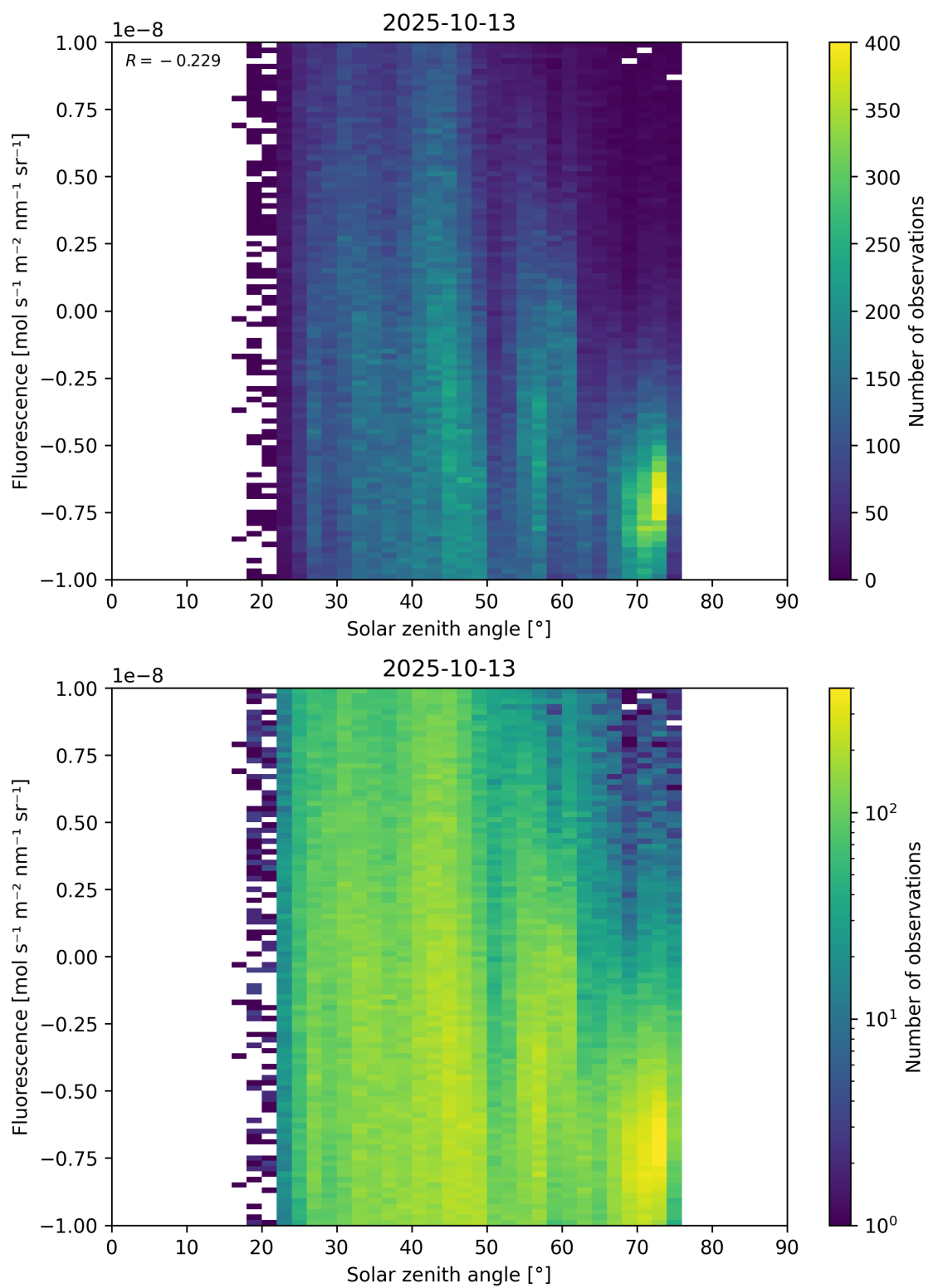
Figure 97: Scatter density plot of “Solar zenith angle” against “Fluorescence” for 2025-10-12 to 2025-10-14.
