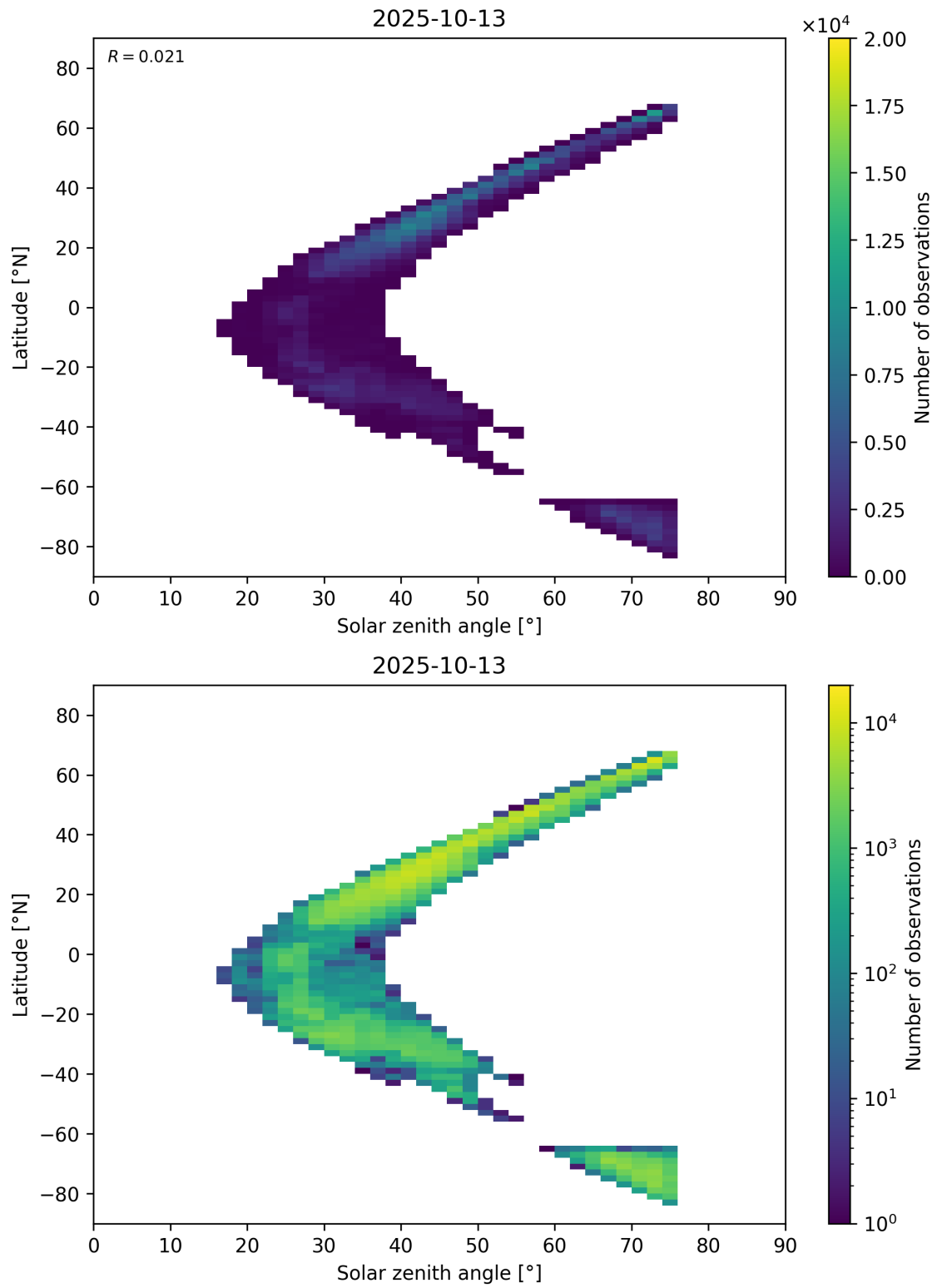
Figure 98: Scatter density plot of “Solar zenith angle” against “Latitude” for 2025-10-12 to 2025-10-14.
