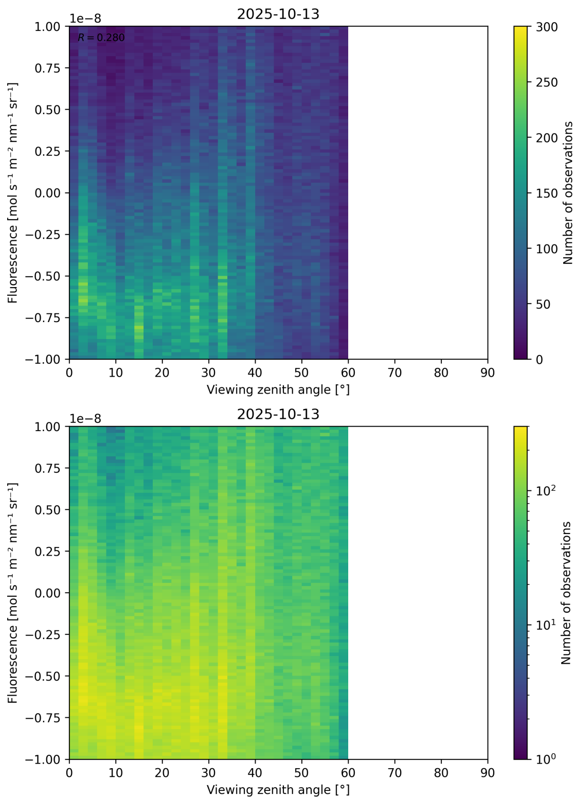
Figure 108: Scatter density plot of “Viewing zenith angle” against “Fluorescence” for 2025-10-12 to 2025-10-14.
