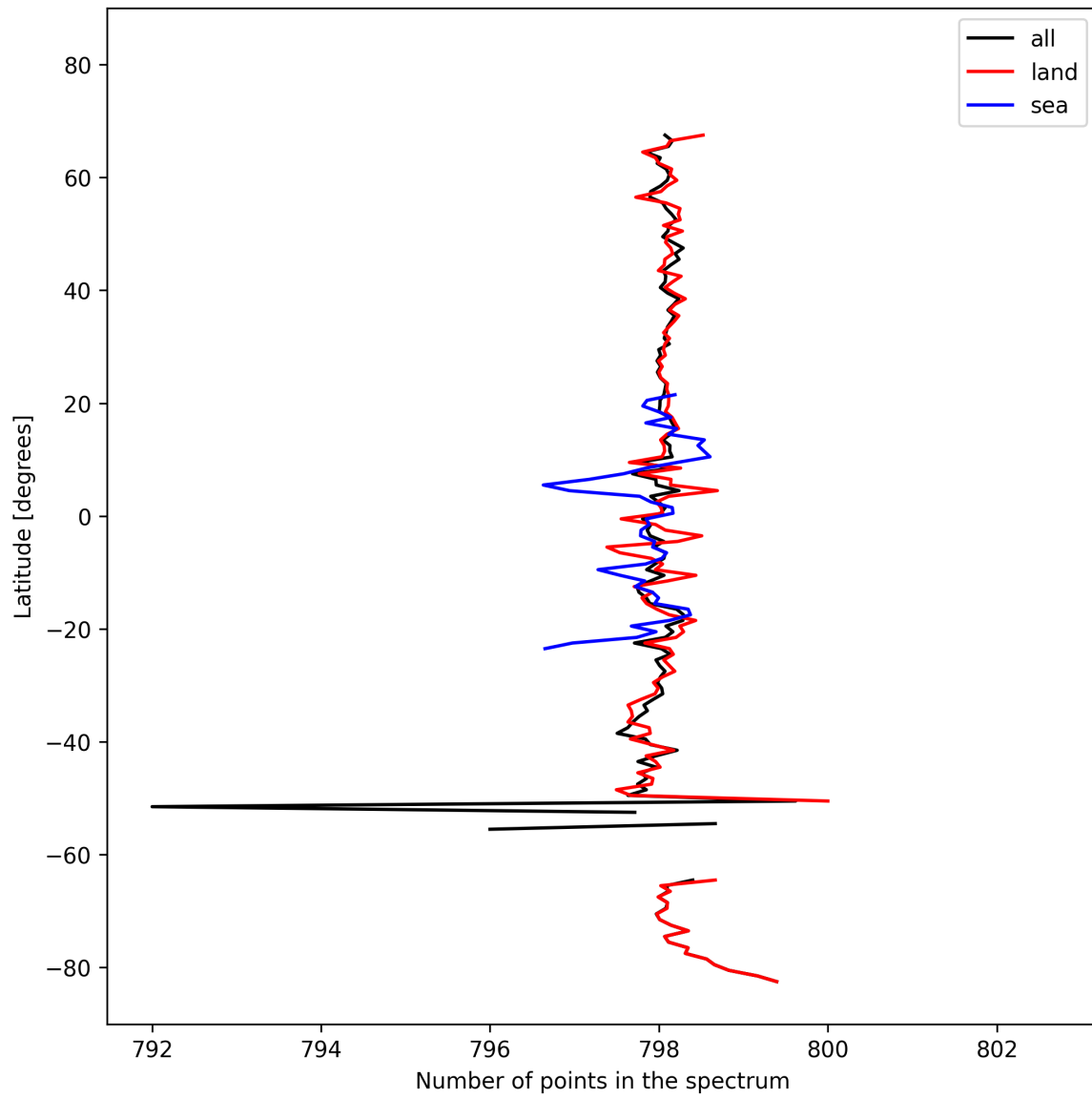
Figure 15: Zonal average of “Number of points in the spectrum” for 2025-10-12 to 2025-10-14.
