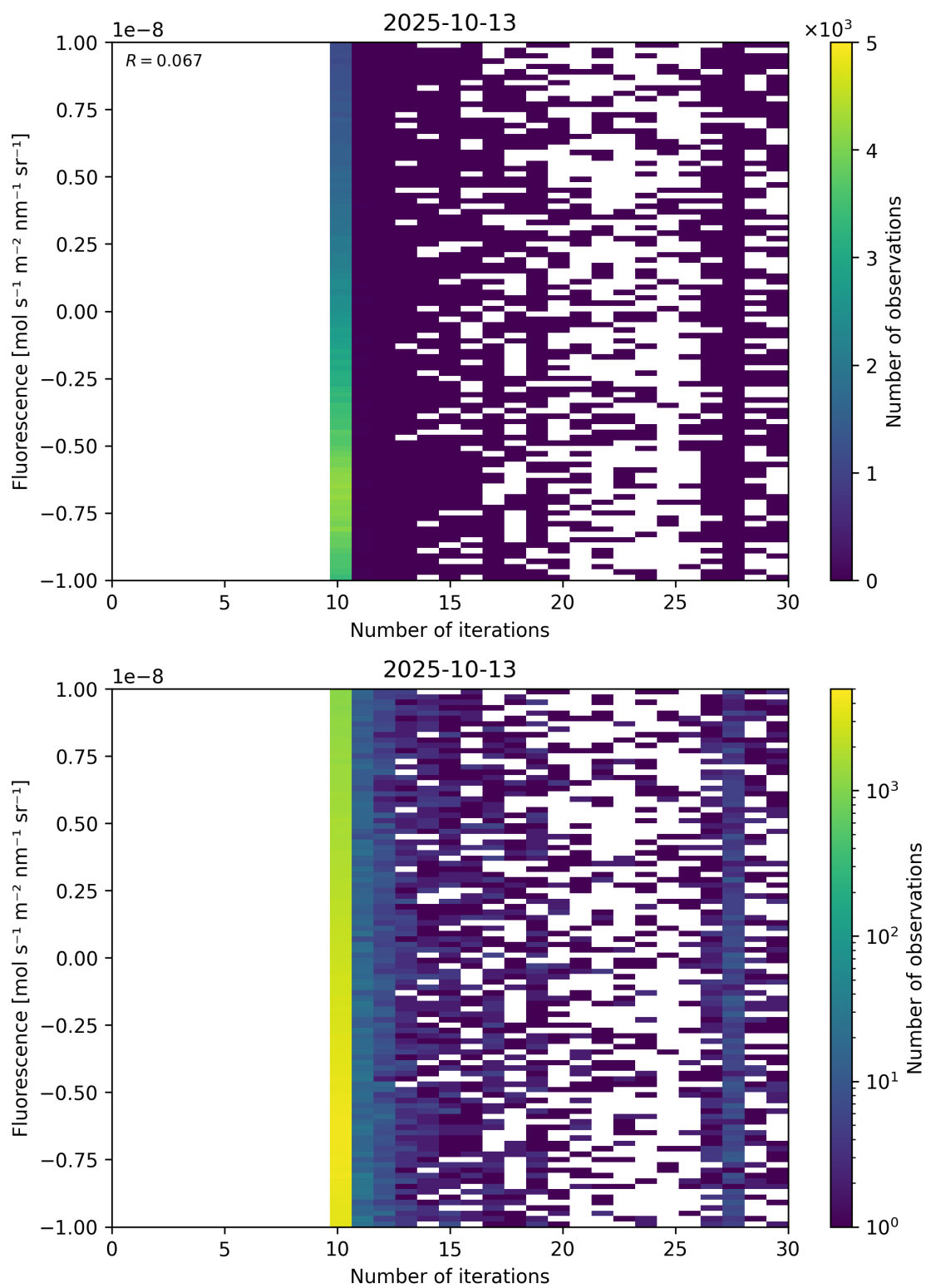
Figure 87: Scatter density plot of “Number of iterations” against “Fluorescence” for 2025-10-12 to 2025-10-14.
