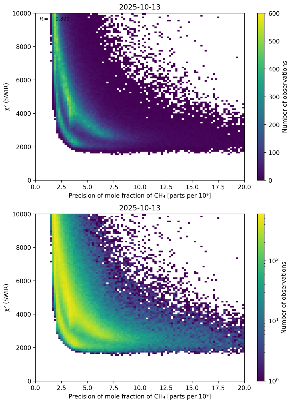
Figure 79: Scatter density plot of “Precision of mole fraction of \text{CH}_4 ” against “ \chi^2 (SWIR)” for 2025-10-12 to 2025-10-14.
