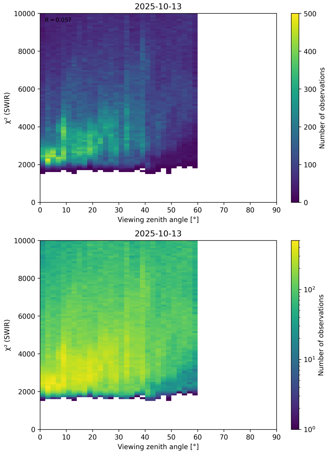
Figure 106: Scatter density plot of “Viewing zenith angle” against “ \chi^2 (SWIR)” for 2025-10-12 to 2025-10-14.
