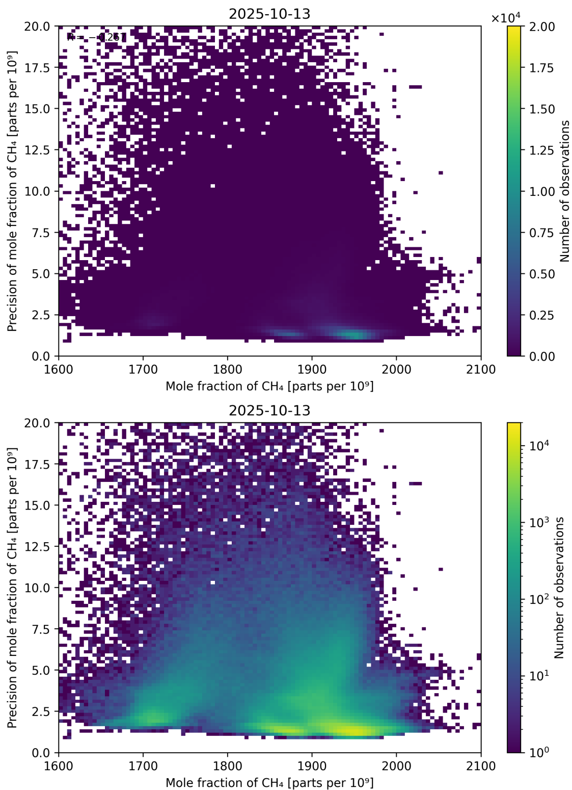
Figure 75: Scatter density plot of “Mole fraction of CH 4 ” against “Precision of mole fraction of CH 4 ” for 2025-10-12 to 2025-10-14.
