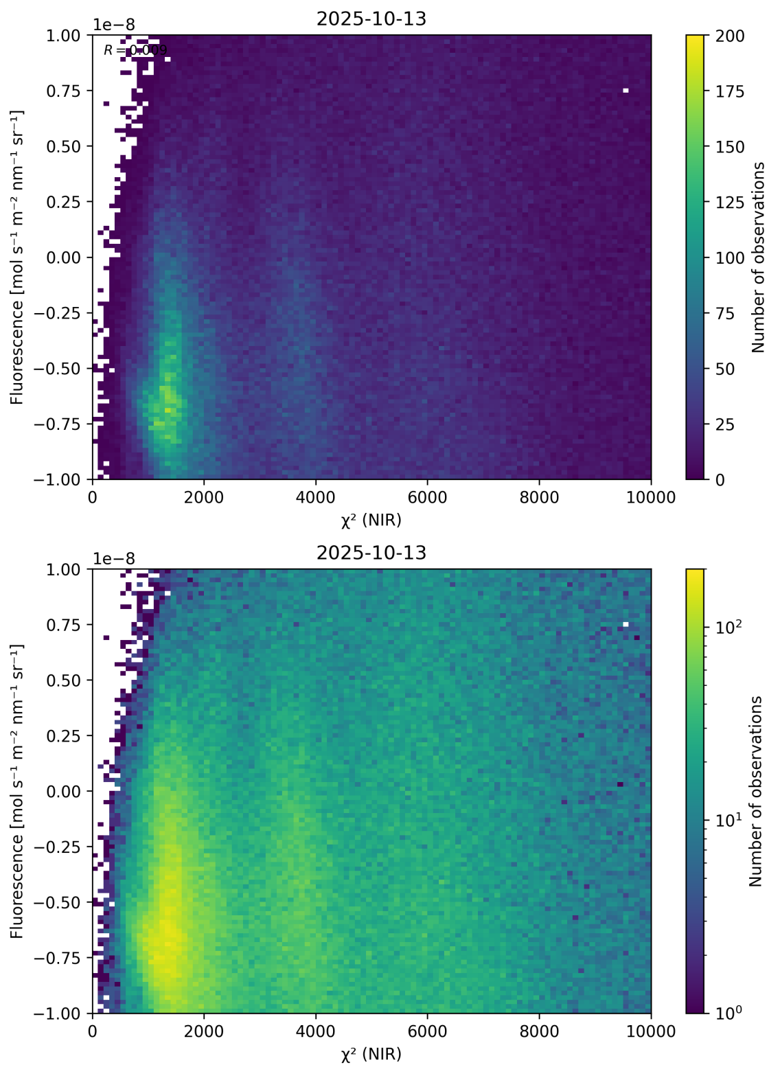
Figure 45: Scatter density plot of “ \chi^2 (NIR)” against “Fluorescence” for 2025-10-12 to 2025-10-14.
