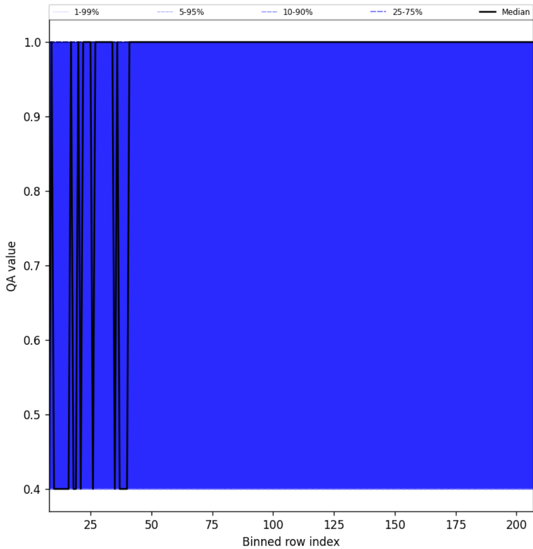
Figure 33: Along track statistics of “QA value” for 2025-10-12 to 2025-10-14
