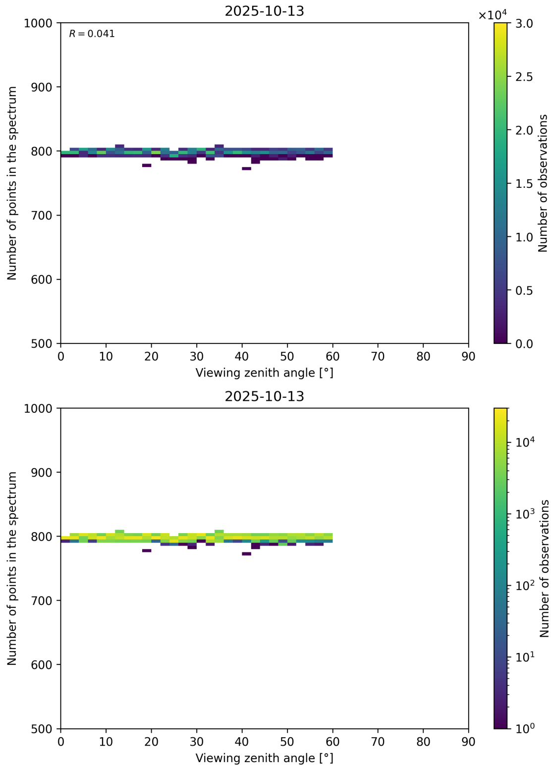
Figure 114: Scatter density plot of “Viewing zenith angle” against “Number of points in the spectrum” for 2025-10-12 to 2025-10-14.
