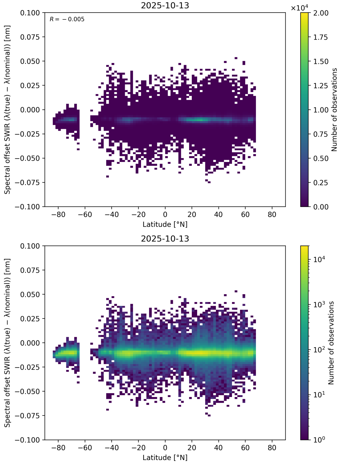
Figure 62: Scatter density plot of “Latitude” against “Spectral offset SWIR ( \lambda_{\text{true}} - \lambda_{\text{nominal}} )” for 2025-10-12 to 2025-10-14.
