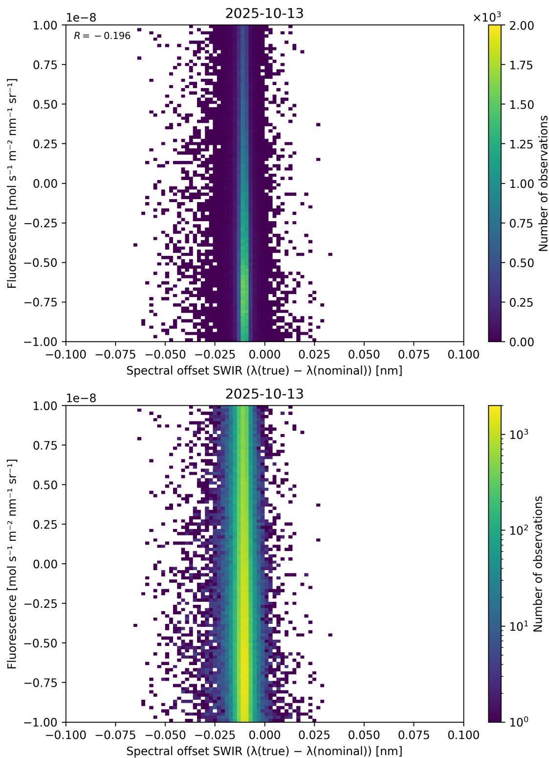
Figure 120: Scatter density plot of “Spectral offset SWIR ( \lambda_{\text{true}} - \lambda_{\text{nominal}} )” against “Fluorescence” for 2025-10-12 to 2025-10-14.
