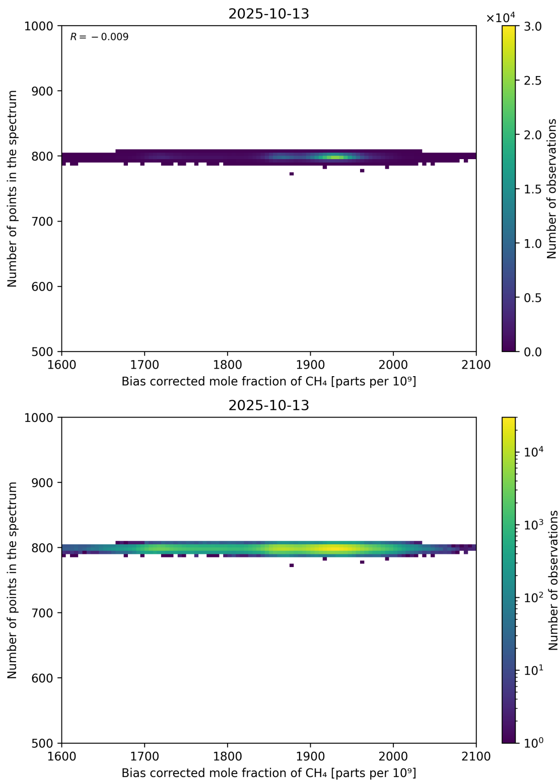
Figure 68: Scatter density plot of “Bias corrected mole fraction of CH 4 ” against “Number of points in the spectrum” for 2025-10-12 to 2025-10-14.
