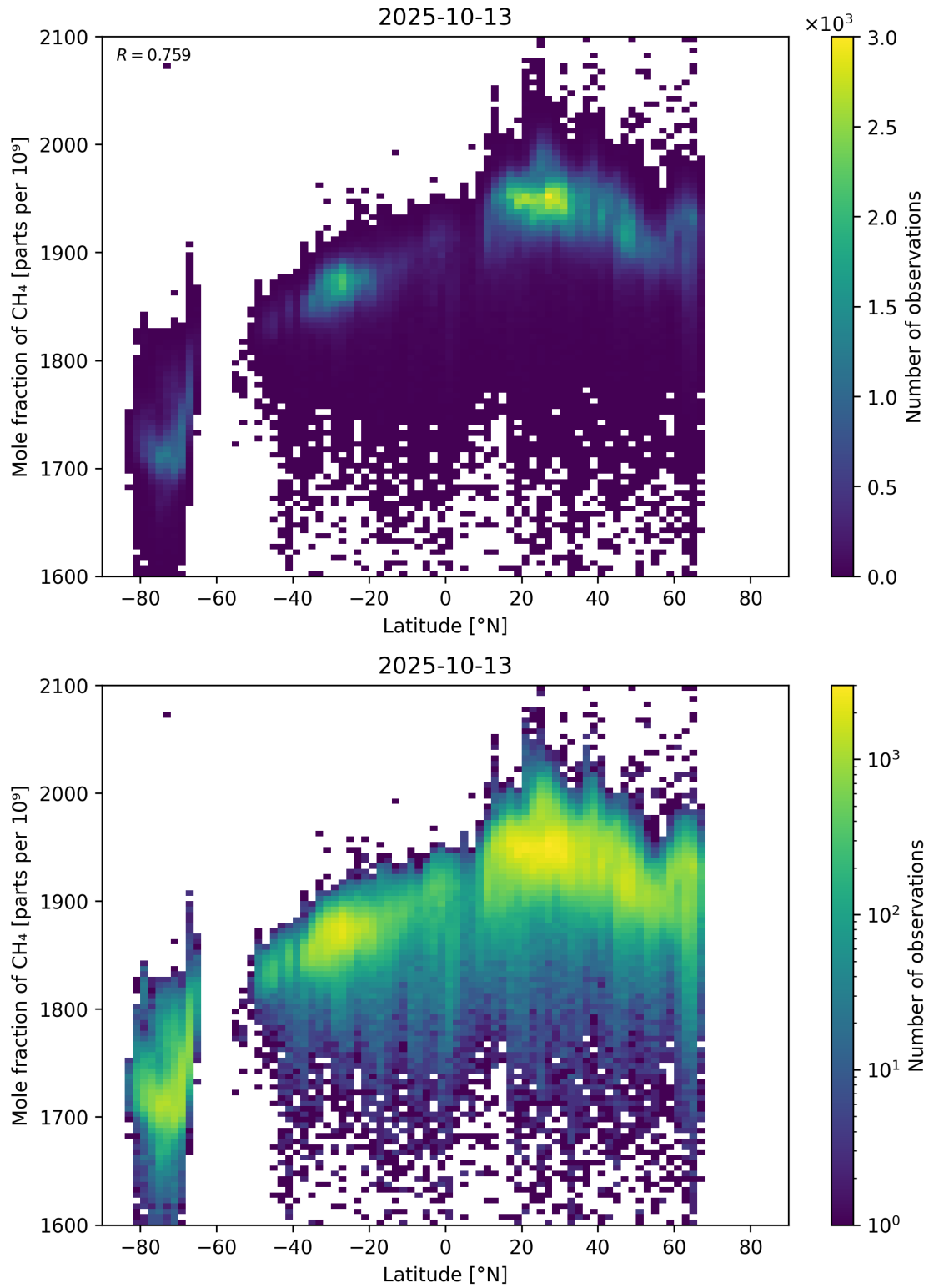
Figure 57: Scatter density plot of “Latitude” against “Mole fraction of CH 4 ” for 2025-10-12 to 2025-10-14.
