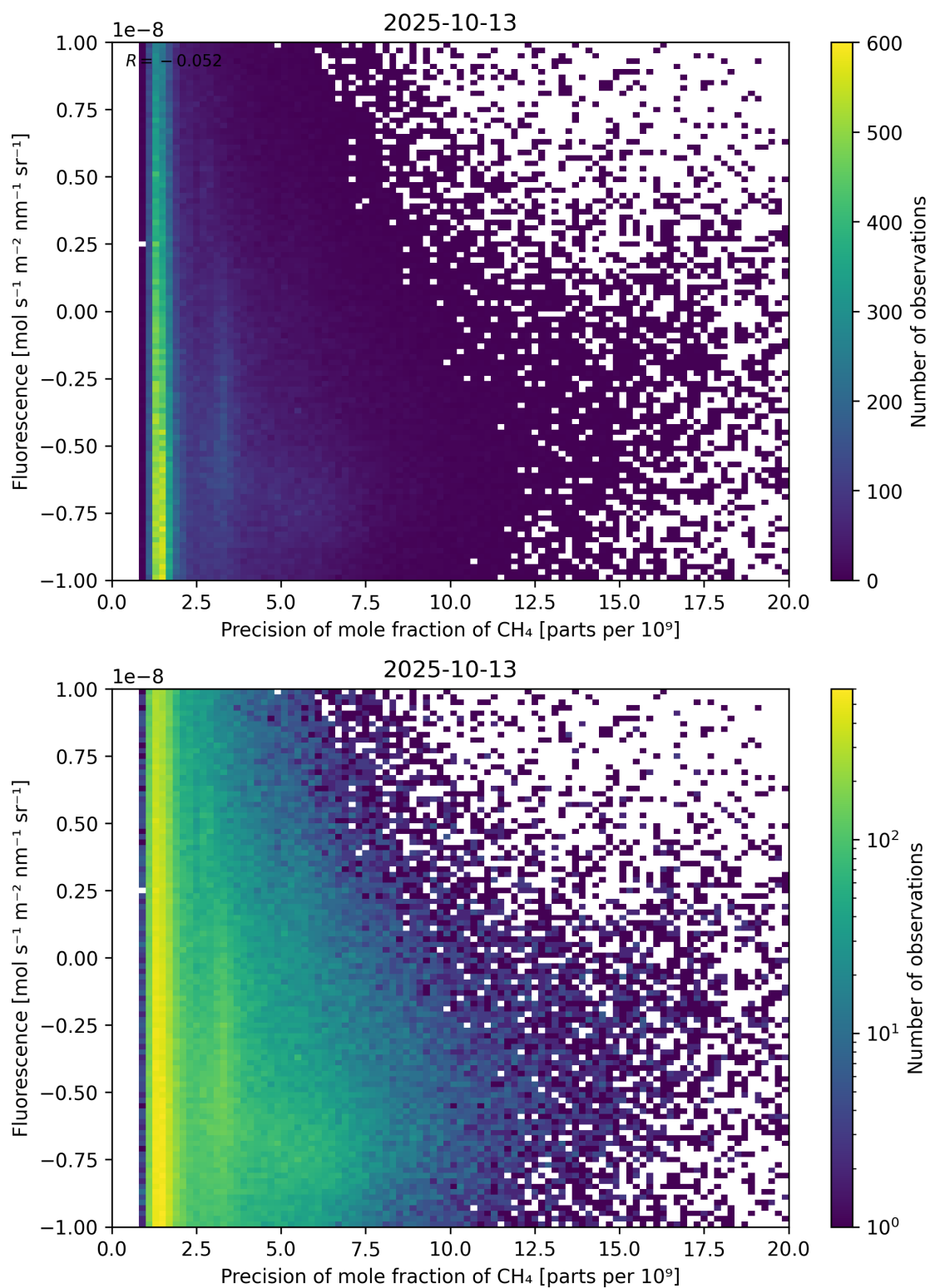
Figure 81: Scatter density plot of “Precision of mole fraction of CH 4 ” against “Fluorescence” for 2025-10-12 to 2025-10-14.
