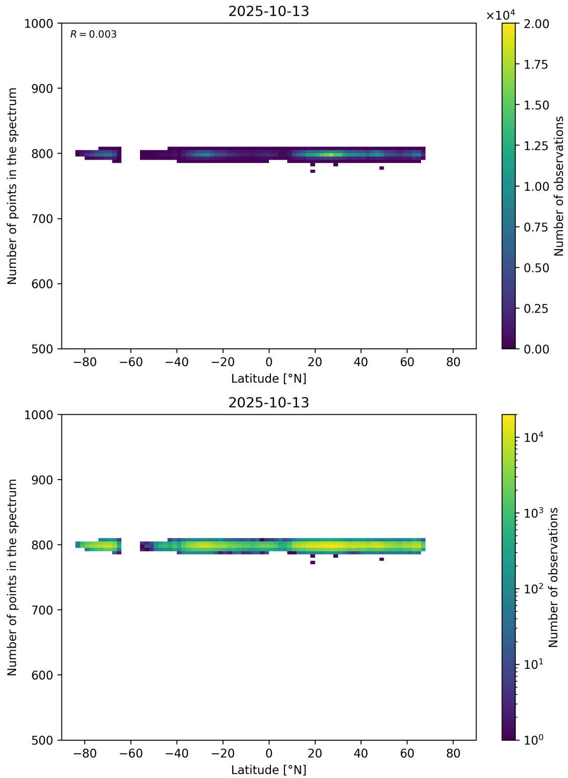
Figure 61: Scatter density plot of “Latitude” against “Number of points in the spectrum” for 2025-10-12 to 2025-10-14.
