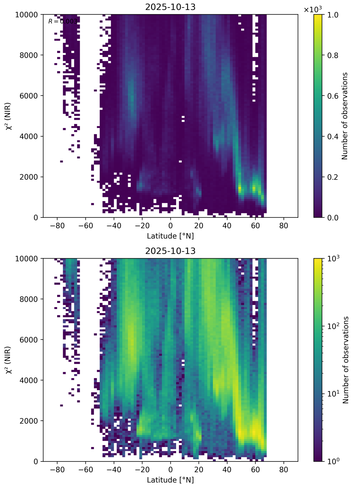
Figure 53: Scatter density plot of “Latitude” against “ \chi^2 (NIR)” for 2025-10-12 to 2025-10-14.
