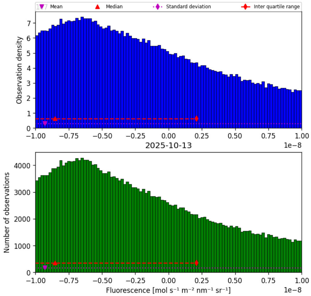
Figure 32: Histogram of “Fluorescence” for 2025-10-12 to 2025-10-14
