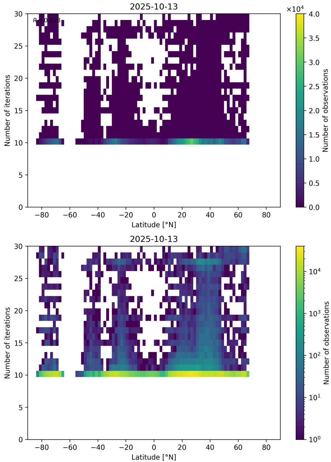
Figure 60: Scatter density plot of “Latitude” against “Number of iterations” for 2025-10-12 to 2025-10-14.
