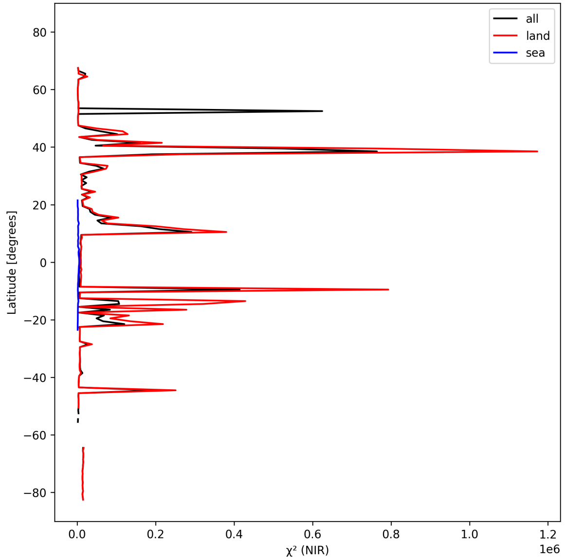
Figure 18: Zonal average of “ \chi^2 (NIR)” for 2025-10-12 to 2025-10-14.
