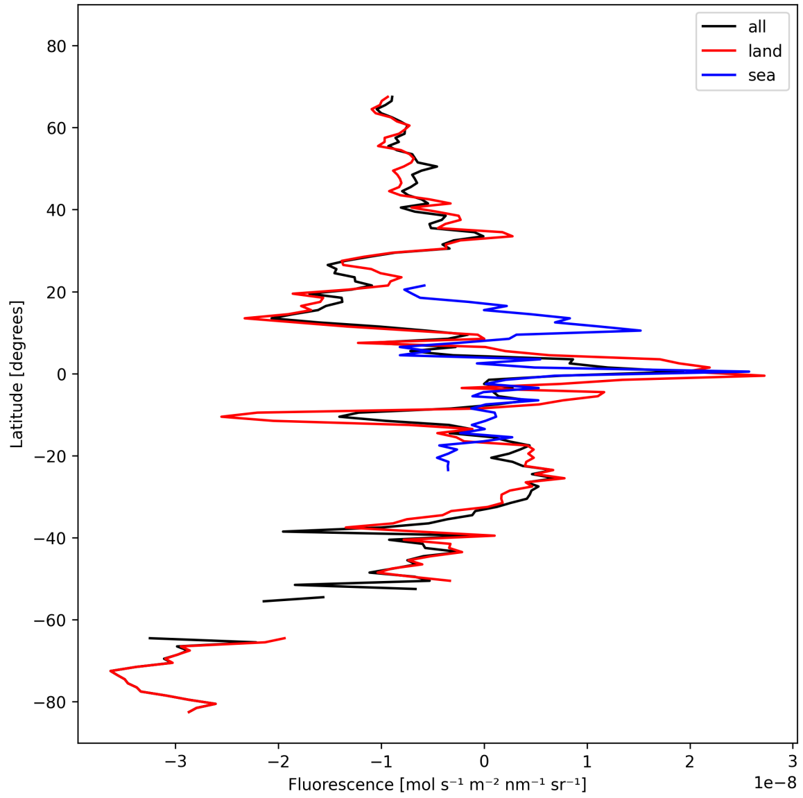
Figure 21: Zonal average of “Fluorescence” for 2025-10-12 to 2025-10-14.
