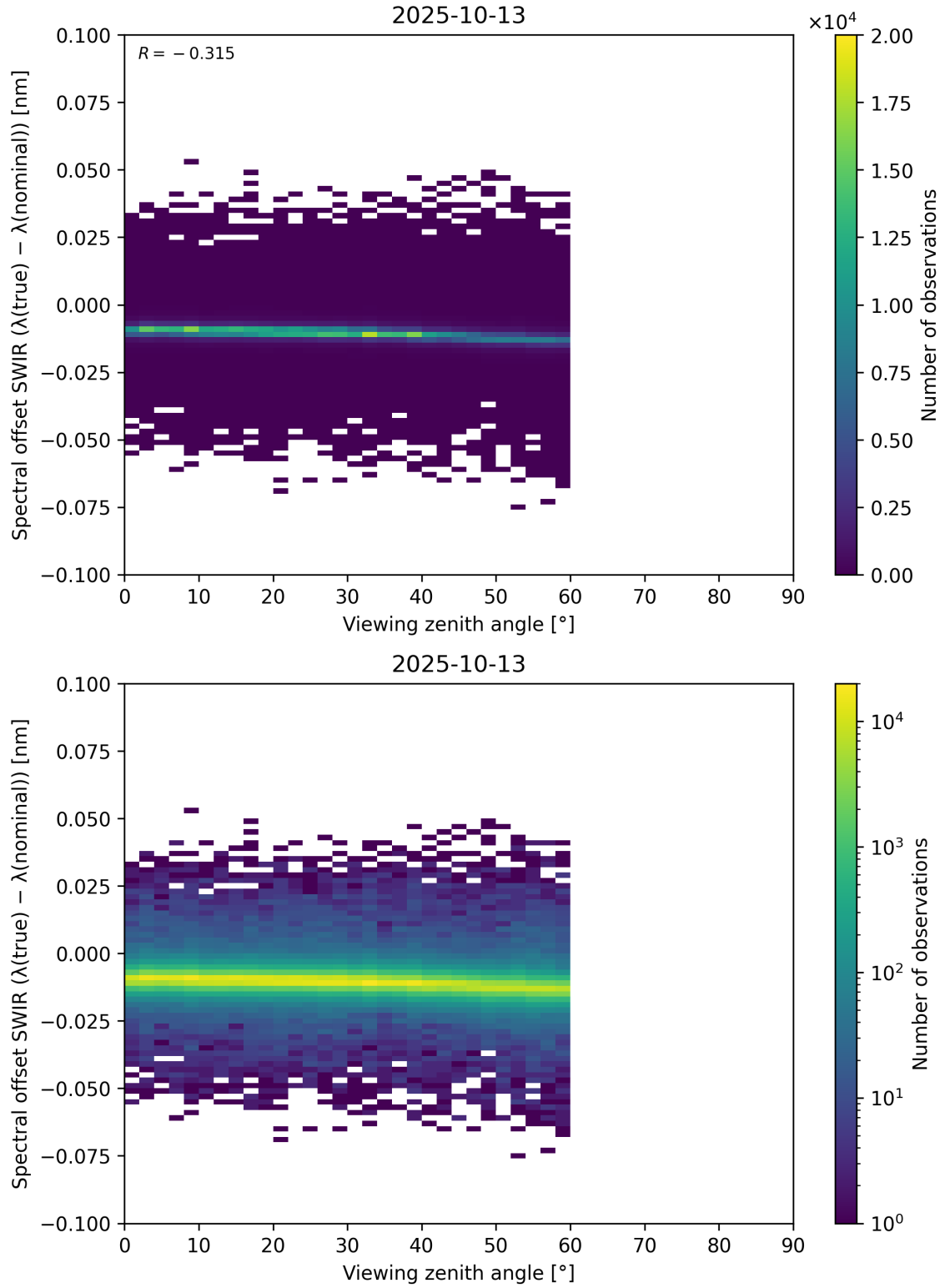
Figure 116: Scatter density plot of “Viewing zenith angle” against “Spectral offset SWIR ( \lambda_{\text{true}} - \lambda_{\text{nominal}} )” for 2025-10-12 to 2025-10-14.
