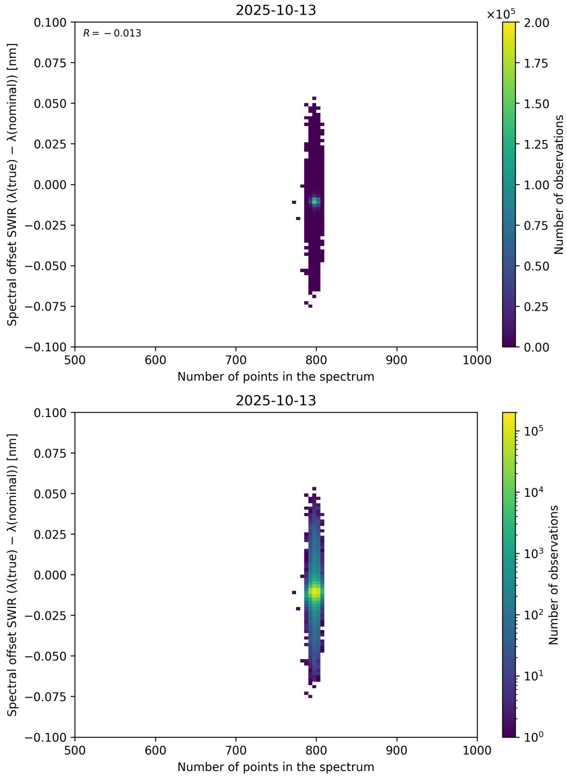
Figure 93: Scatter density plot of “Number of points in the spectrum” against “Spectral offset SWIR ( \lambda_{\text{true}} - \lambda_{\text{nominal}} )” for 2025-10-12 to 2025-10-14.
