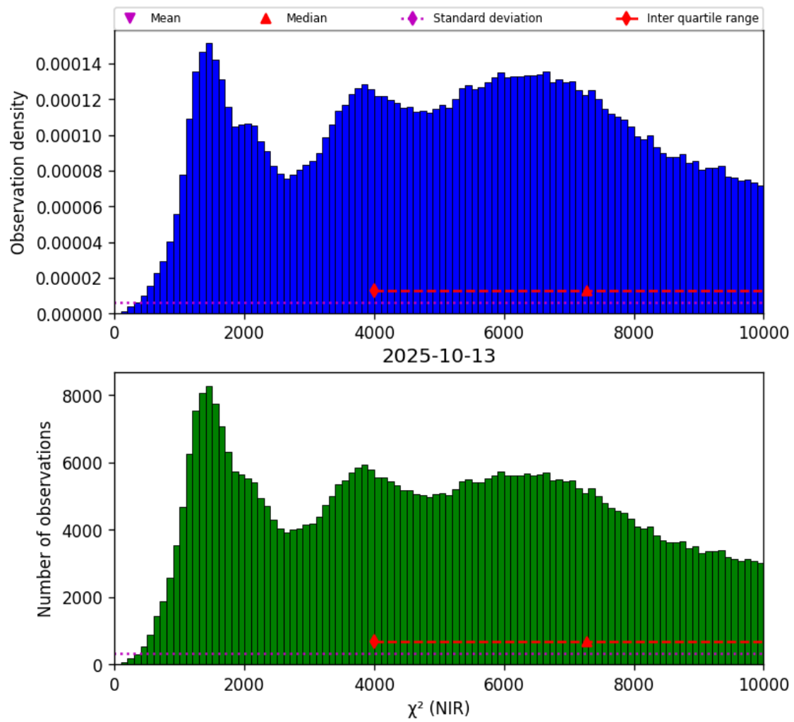
Figure 29: Histogram of “ \chi^2 (NIR)” for 2025-10-12 to 2025-10-14
