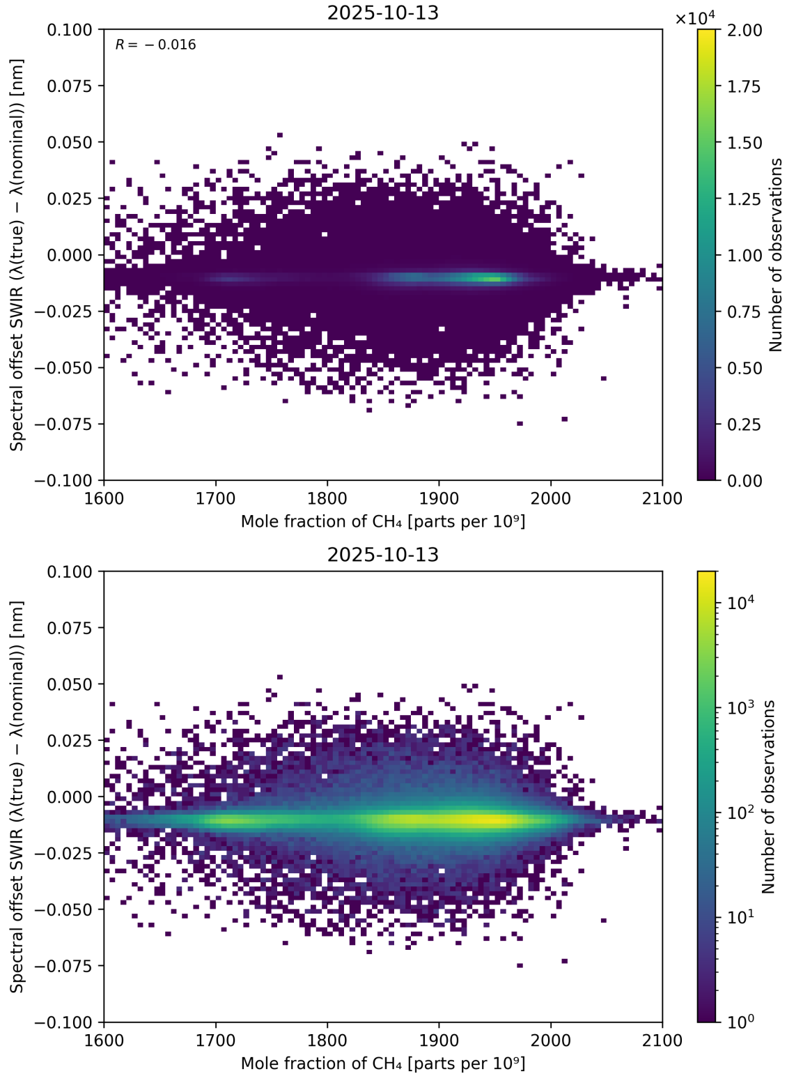
Figure 86: Scatter density plot of “Mole fraction of CH 4 ” against “Spectral offset SWIR ( \lambda_{\text{true}} - \lambda_{\text{nominal}} )” for 2025-10-12 to 2025-10-14.
