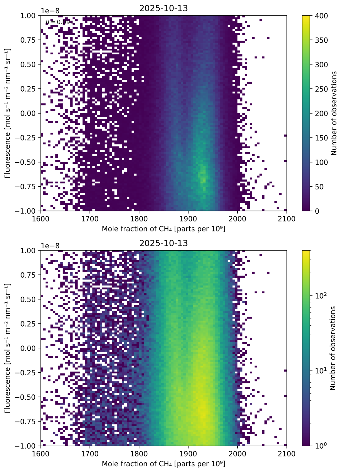
Figure 73: Scatter density plot of “Mole fraction of \text{CH}_4 ” against “Fluorescence” for 2025-10-12 to 2025-10-14.
