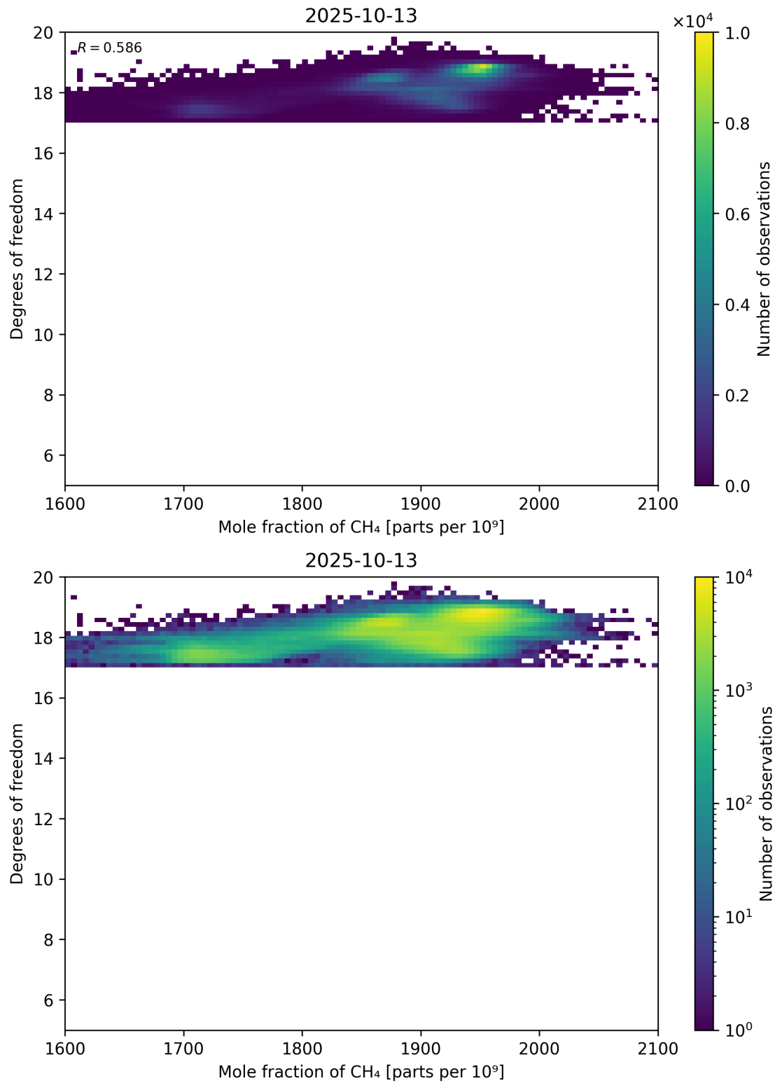
Figure 72: Scatter density plot of “Mole fraction of CH 4 ” against “Degrees of freedom” for 2025-10-12 to 2025-10-14.
