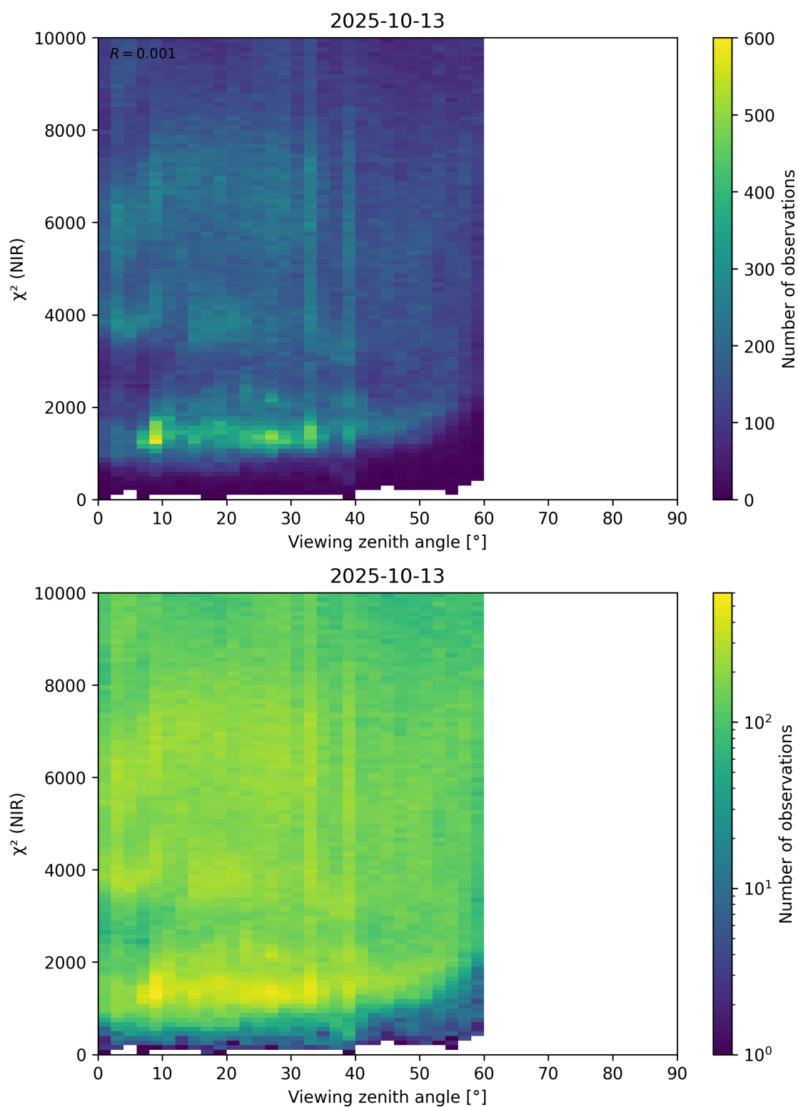
Figure 105: Scatter density plot of “Viewing zenith angle” against “ \chi^2 (NIR)” for 2025-10-12 to 2025-10-14.
