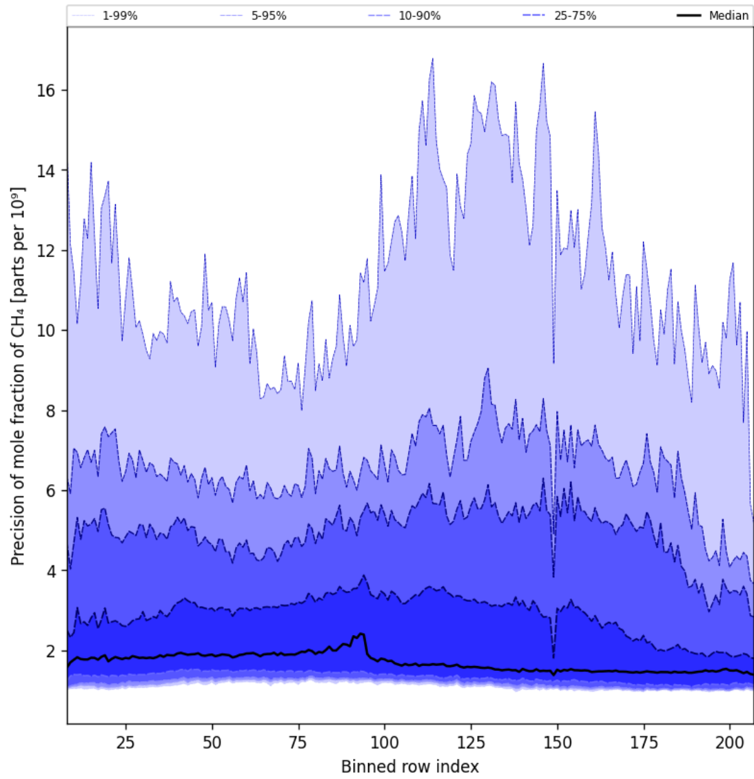
Figure 35: Along track statistics of “Precision of mole fraction of CH 4 ” for 2025-10-12 to 2025-10-14
