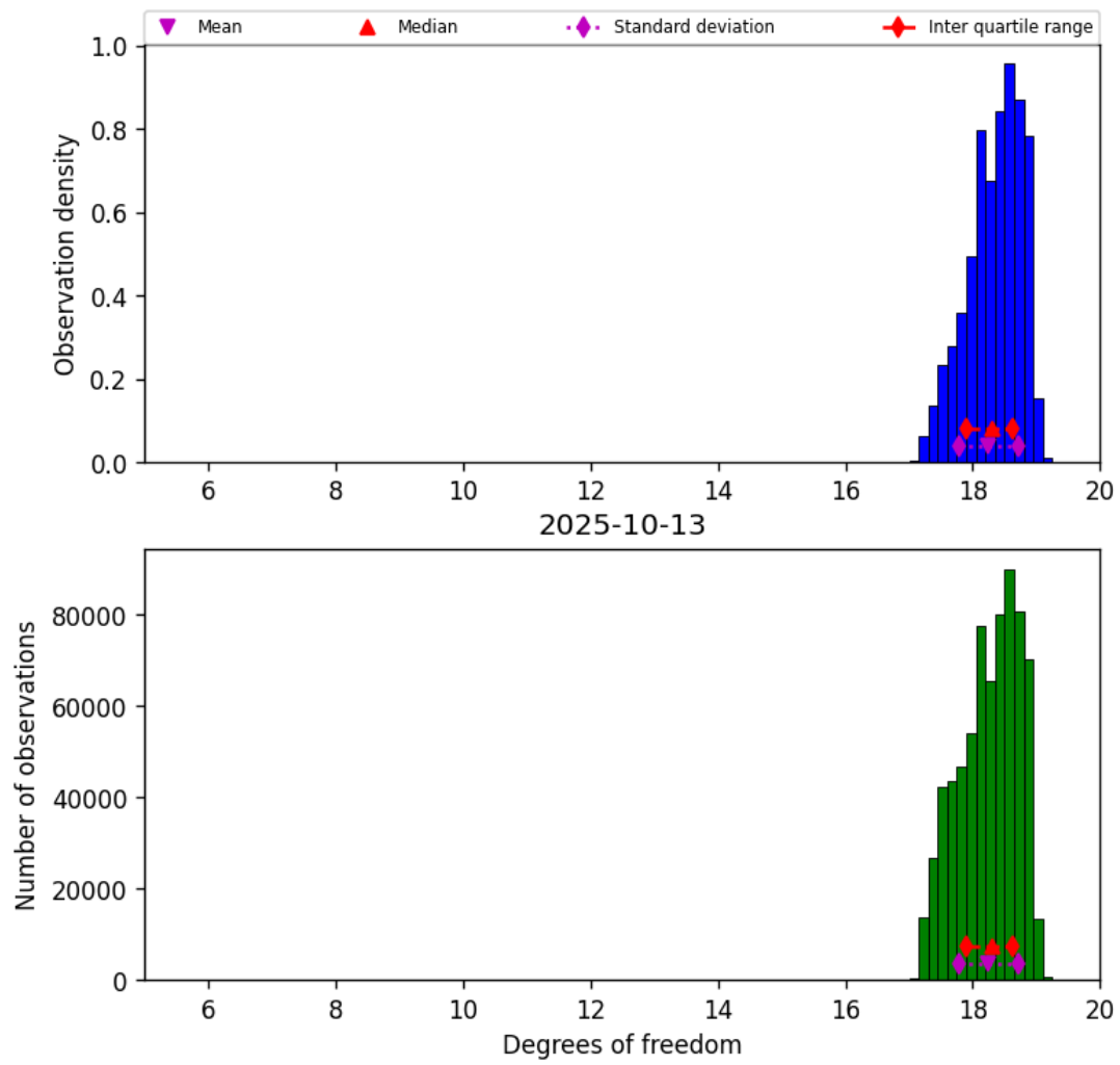
Figure 30: Histogram of “Degrees of freedom” for 2025-10-12 to 2025-10-14
