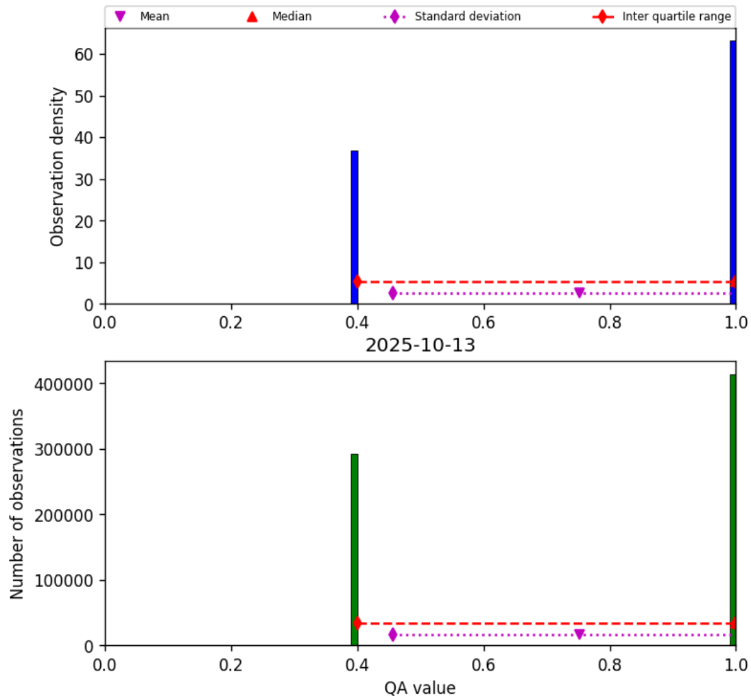
Figure 22: Histogram of “QA value” for 2025-10-12 to 2025-10-14
