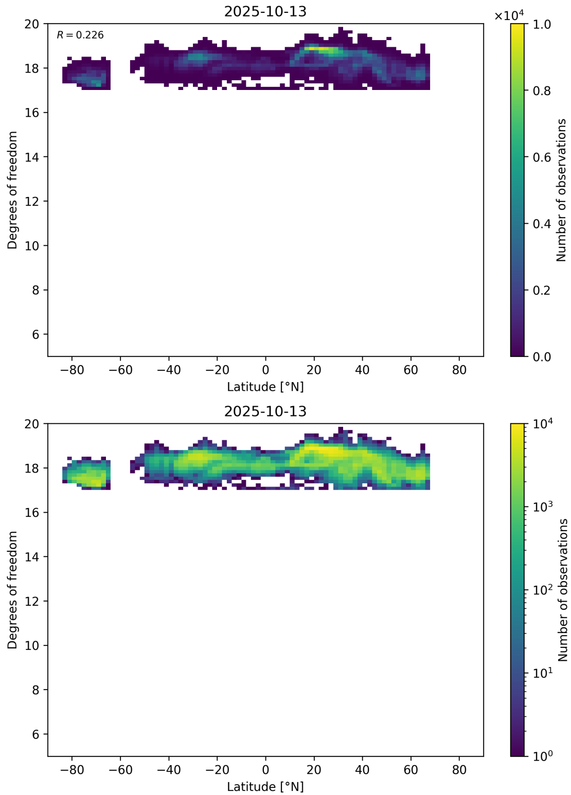
Figure 55: Scatter density plot of “Latitude” against “Degrees of freedom” for 2025-10-12 to 2025-10-14.
