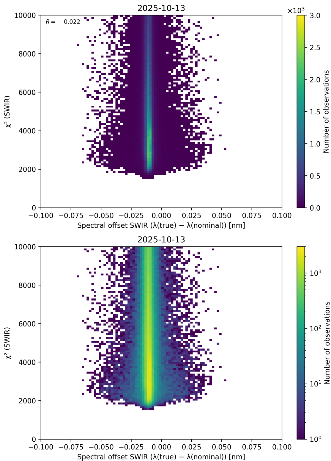
Figure 118: Scatter density plot of “Spectral offset SWIR ( \lambda_{\text{true}} - \lambda_{\text{nominal}} )” against “ \chi^2 (SWIR)” for 2025-10-12 to 2025-10-14.
