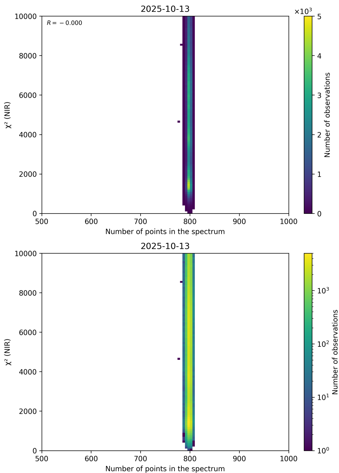
Figure 88: Scatter density plot of “Number of points in the spectrum” against “ \chi^2 (NIR)” for 2025-10-12 to 2025-10-14.
