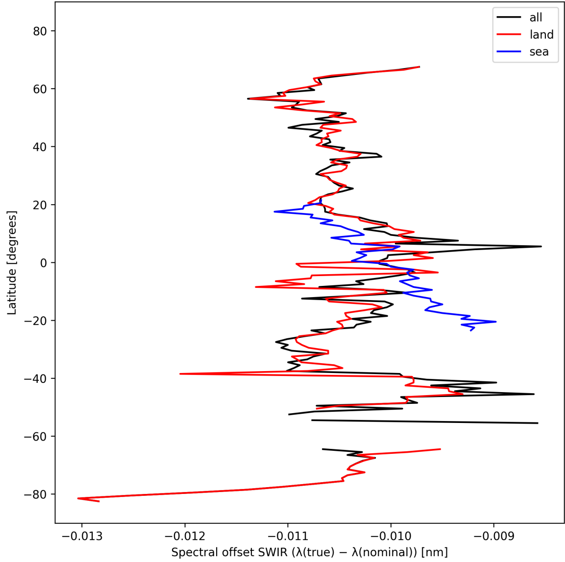
Figure 16: Zonal average of “Spectral offset SWIR ( \lambda_{\text{true}} - \lambda_{\text{nominal}} )” for 2025-10-12 to 2025-10-14.
