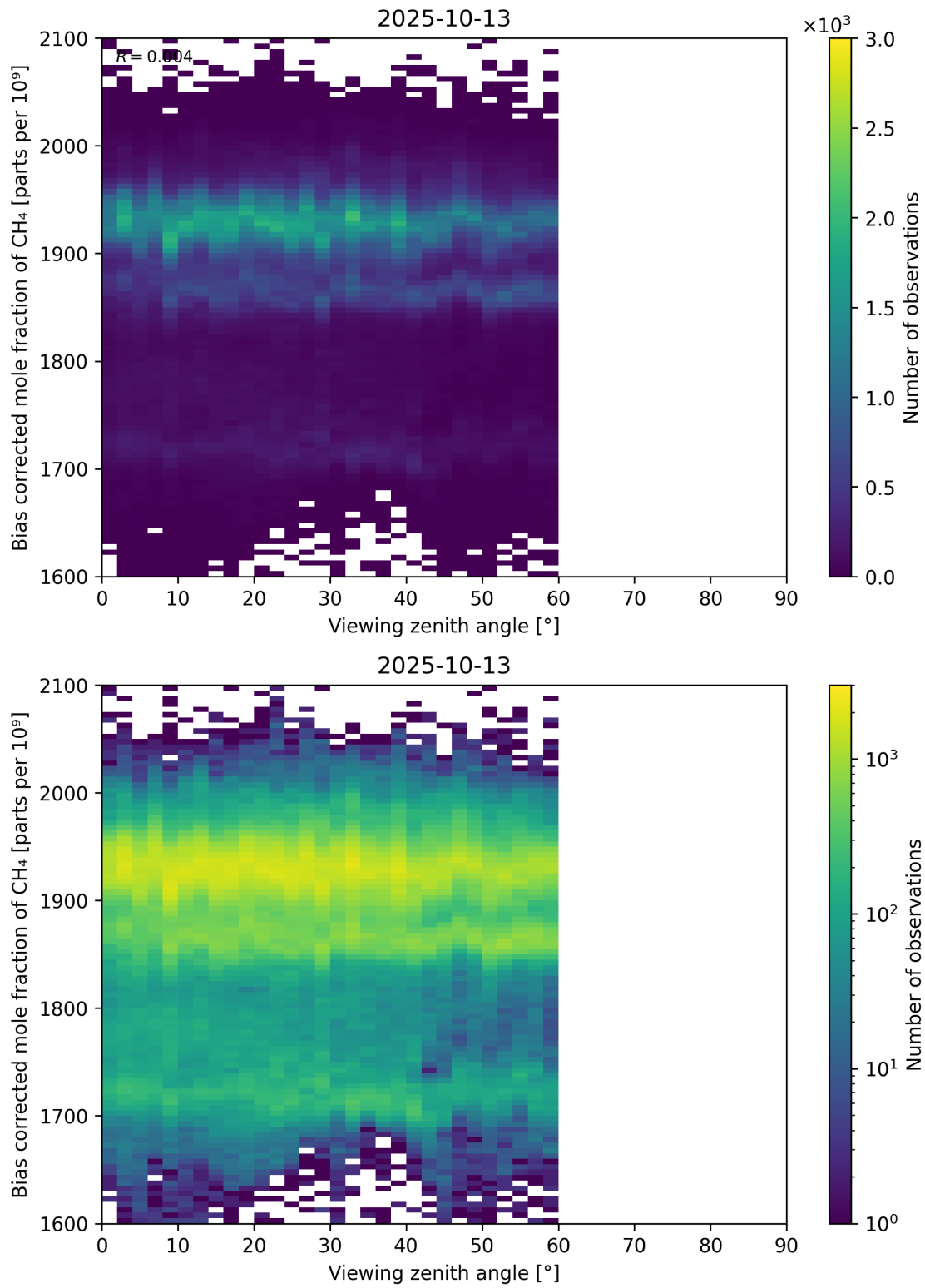
Figure 111: Scatter density plot of “Viewing zenith angle” against “Bias corrected mole fraction of CH 4 ” for 2025-10-12 to 2025-10-14.
