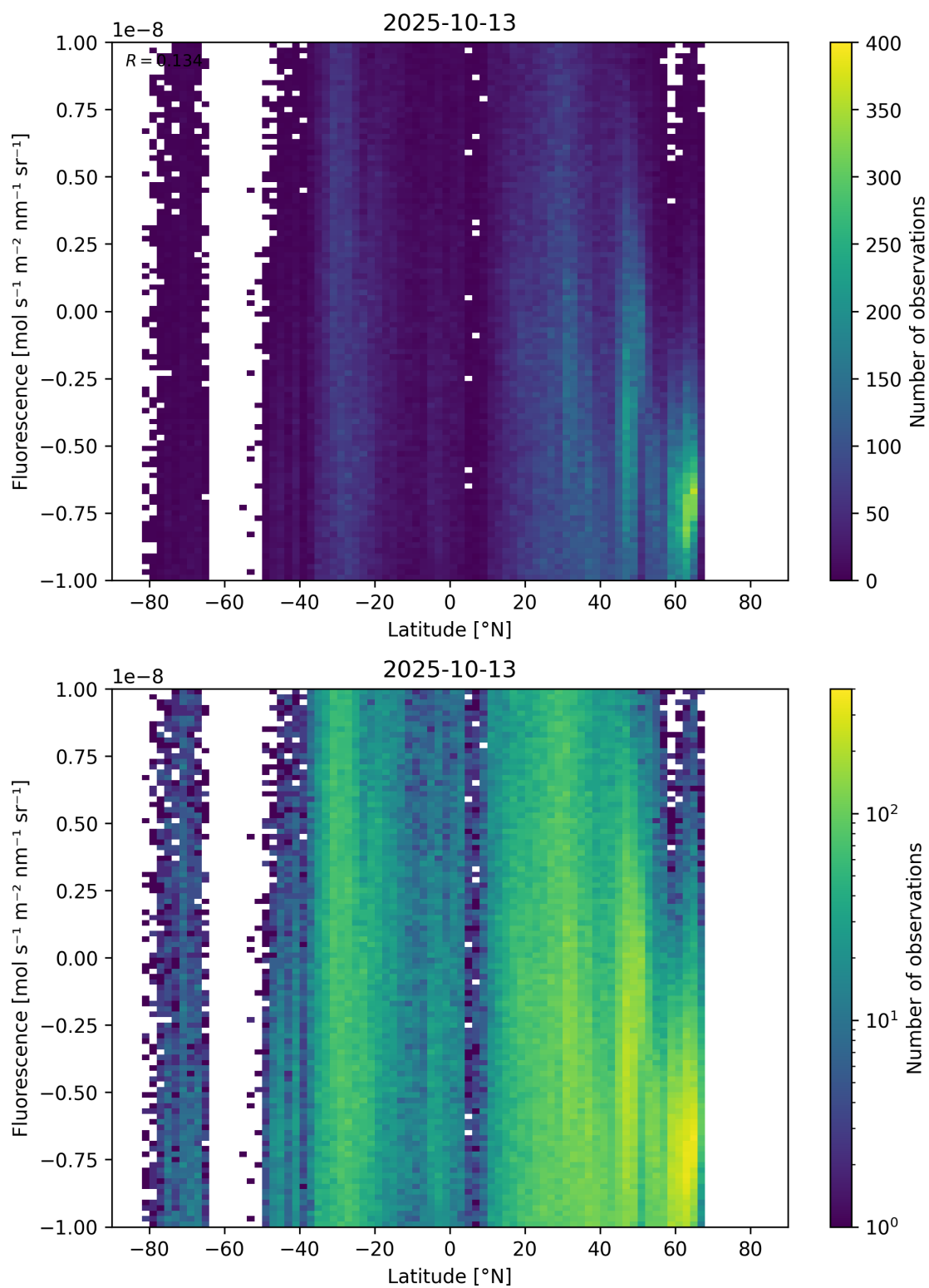
Figure 56: Scatter density plot of “Latitude” against “Fluorescence” for 2025-10-12 to 2025-10-14.
