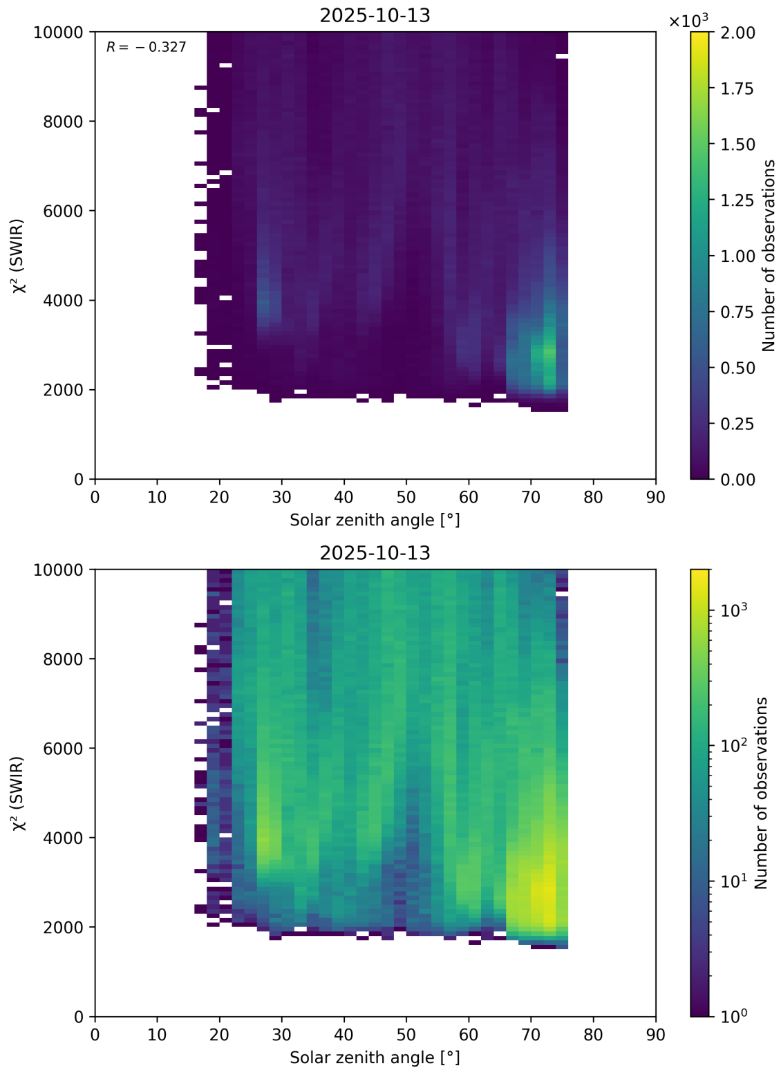
Figure 95: Scatter density plot of “Solar zenith angle” against “ \chi^2 (SWIR)” for 2025-10-12 to 2025-10-14.
