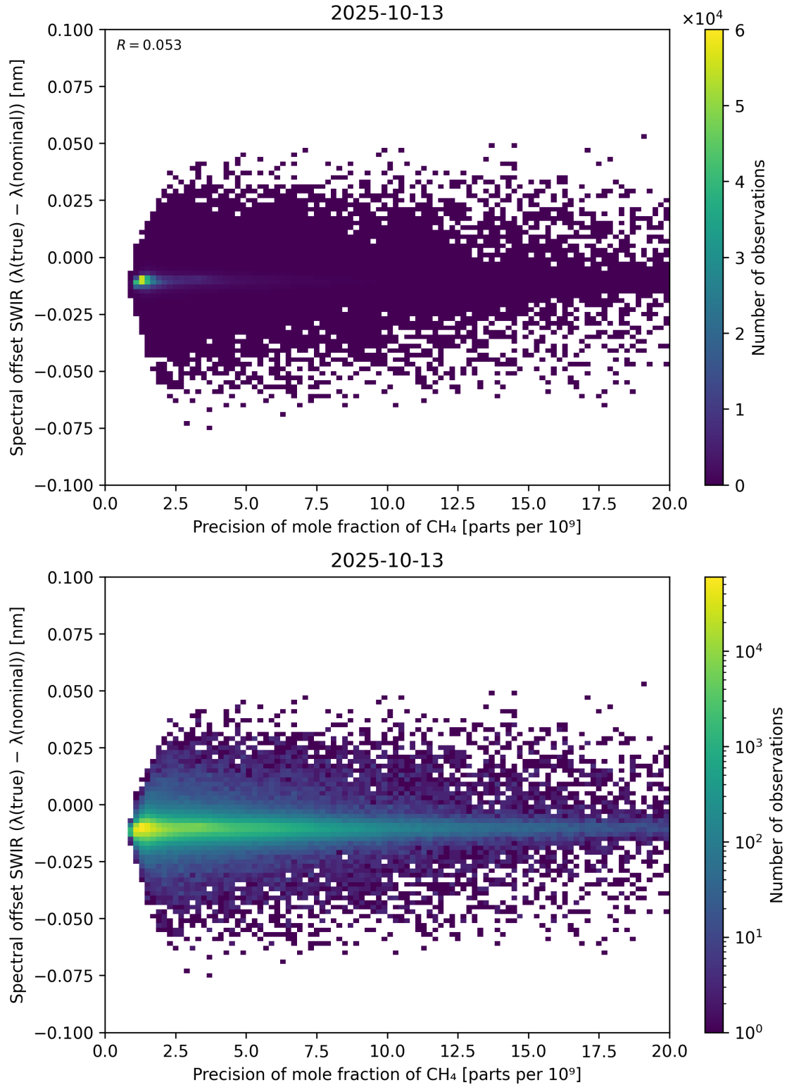
Figure 85: Scatter density plot of “Precision of mole fraction of \text{CH}_4 ” against “Spectral offset SWIR ( \lambda_{\text{true}} - \lambda_{\text{nominal}} )” for 2025-10-12 to 2025-10-14.
