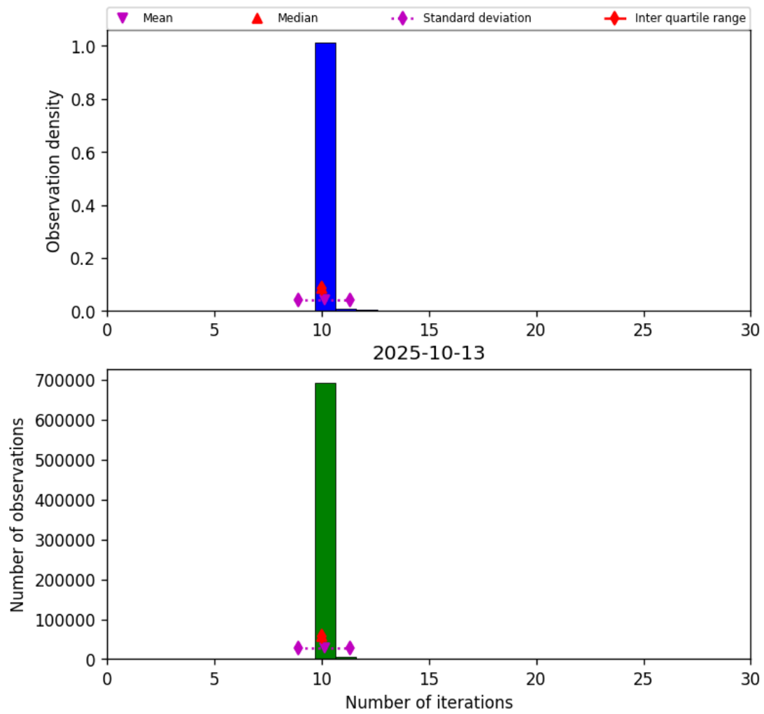
Figure 31: Histogram of “Number of iterations” for 2025-10-12 to 2025-10-14
