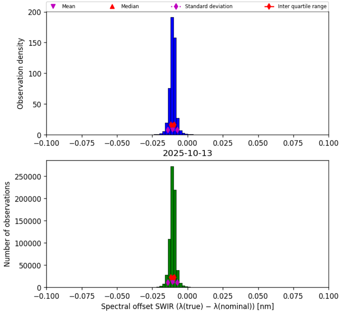
Figure 27: Histogram of “Spectral offset SWIR ( \lambda_{\text{true}} - \lambda_{\text{nominal}} )” for 2025-10-12 to 2025-10-14
