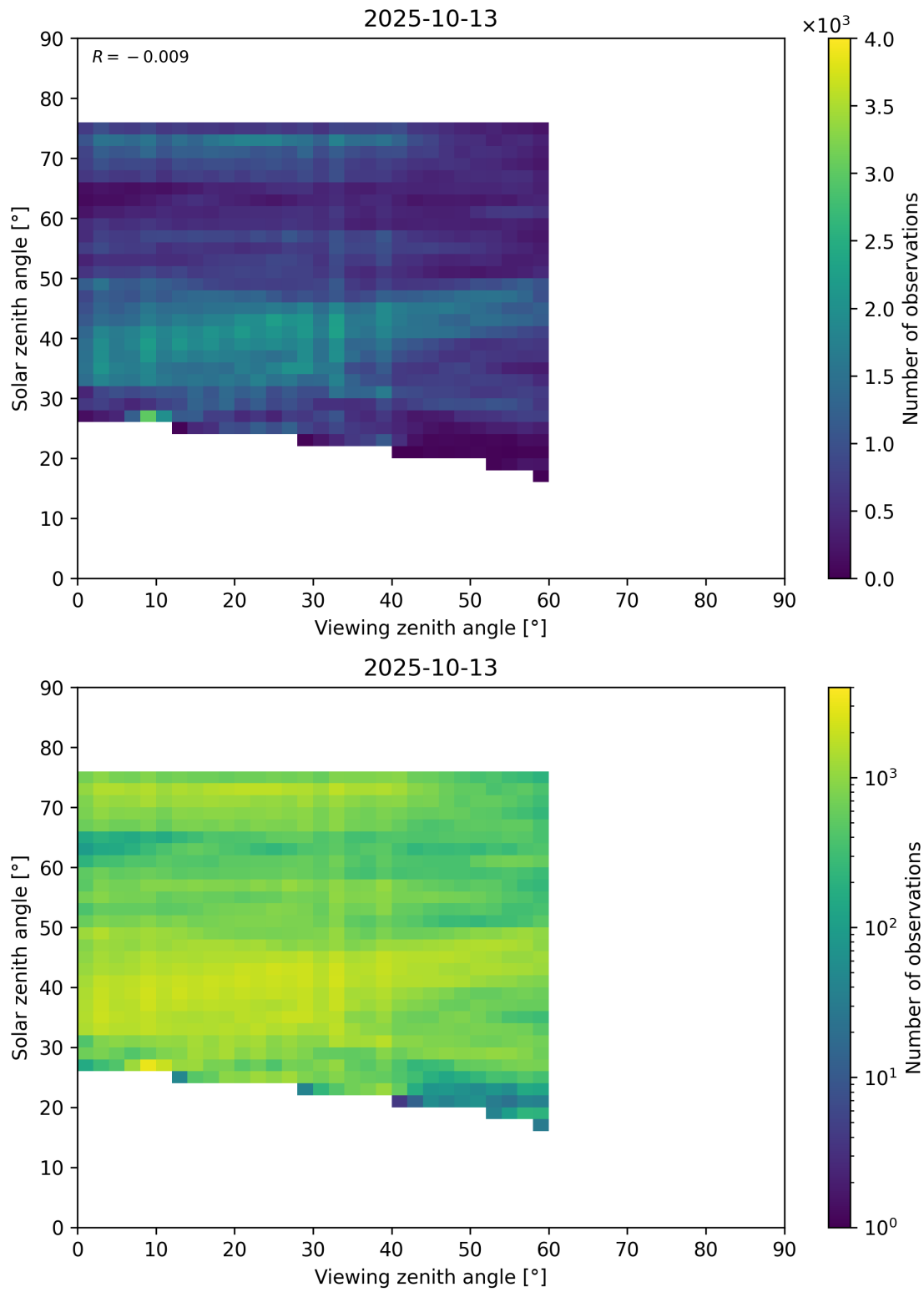
Figure 115: Scatter density plot of “Viewing zenith angle” against “Solar zenith angle” for 2025-10-12 to 2025-10-14.
