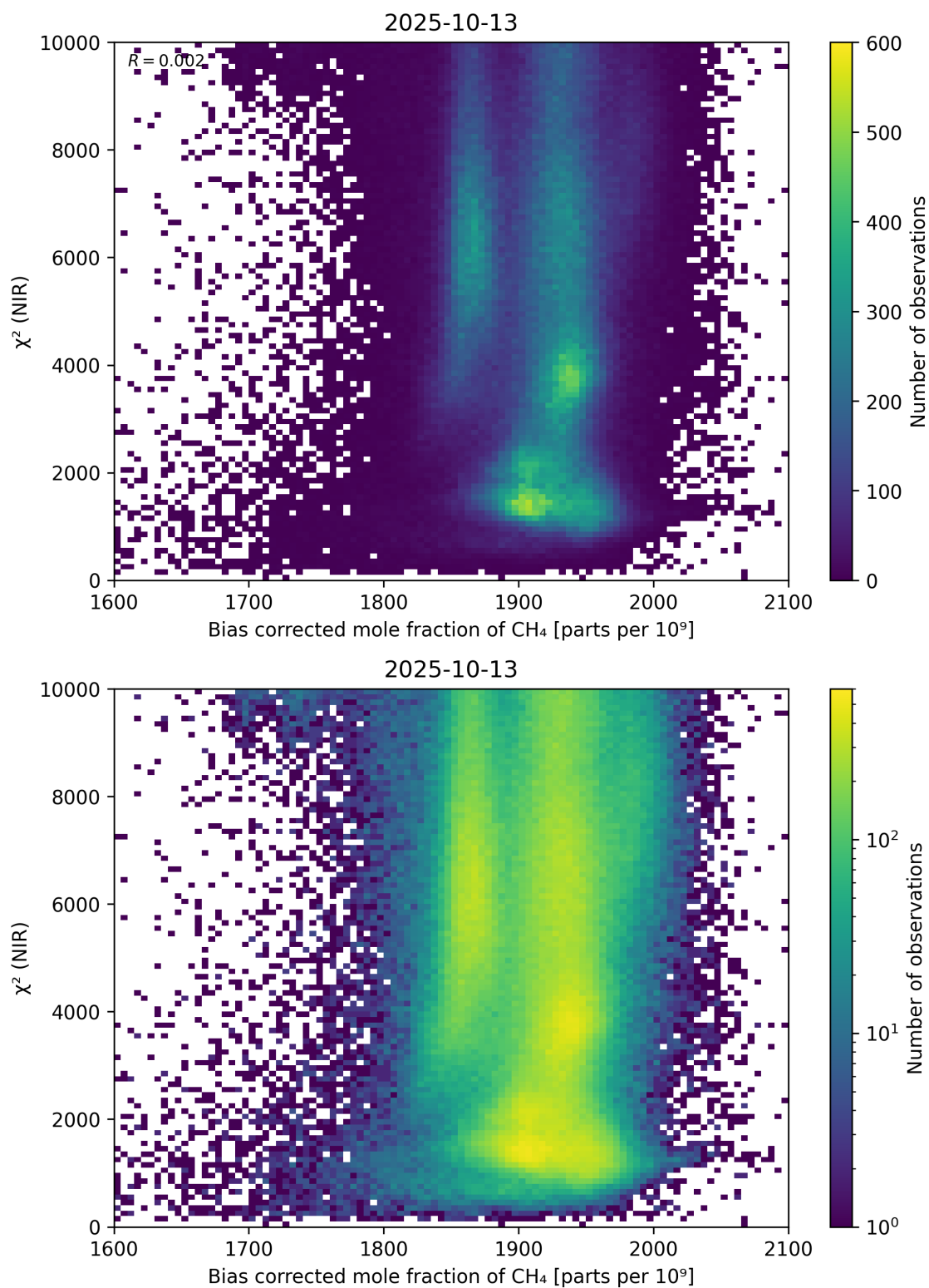
Figure 63: Scatter density plot of “Bias corrected mole fraction of \text{CH}_4 ” against “ \chi^2 (NIR)” for 2025-10-12 to 2025-10-14.
