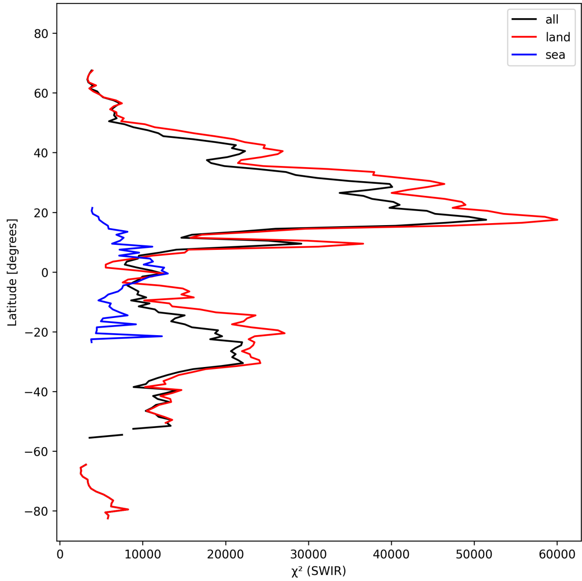
Figure 17: Zonal average of “ \chi^2 (SWIR)” for 2025-10-12 to 2025-10-14.
