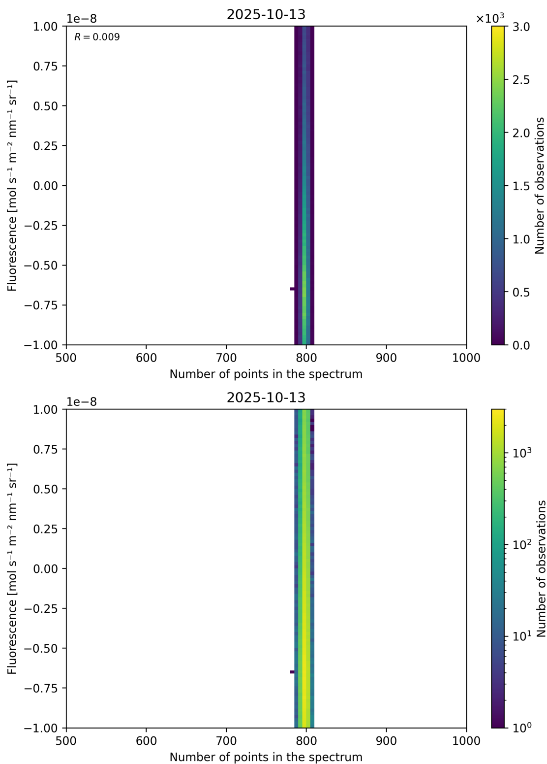
Figure 91: Scatter density plot of “Number of points in the spectrum” against “Fluorescence” for 2025-10-12 to 2025-10-14.
