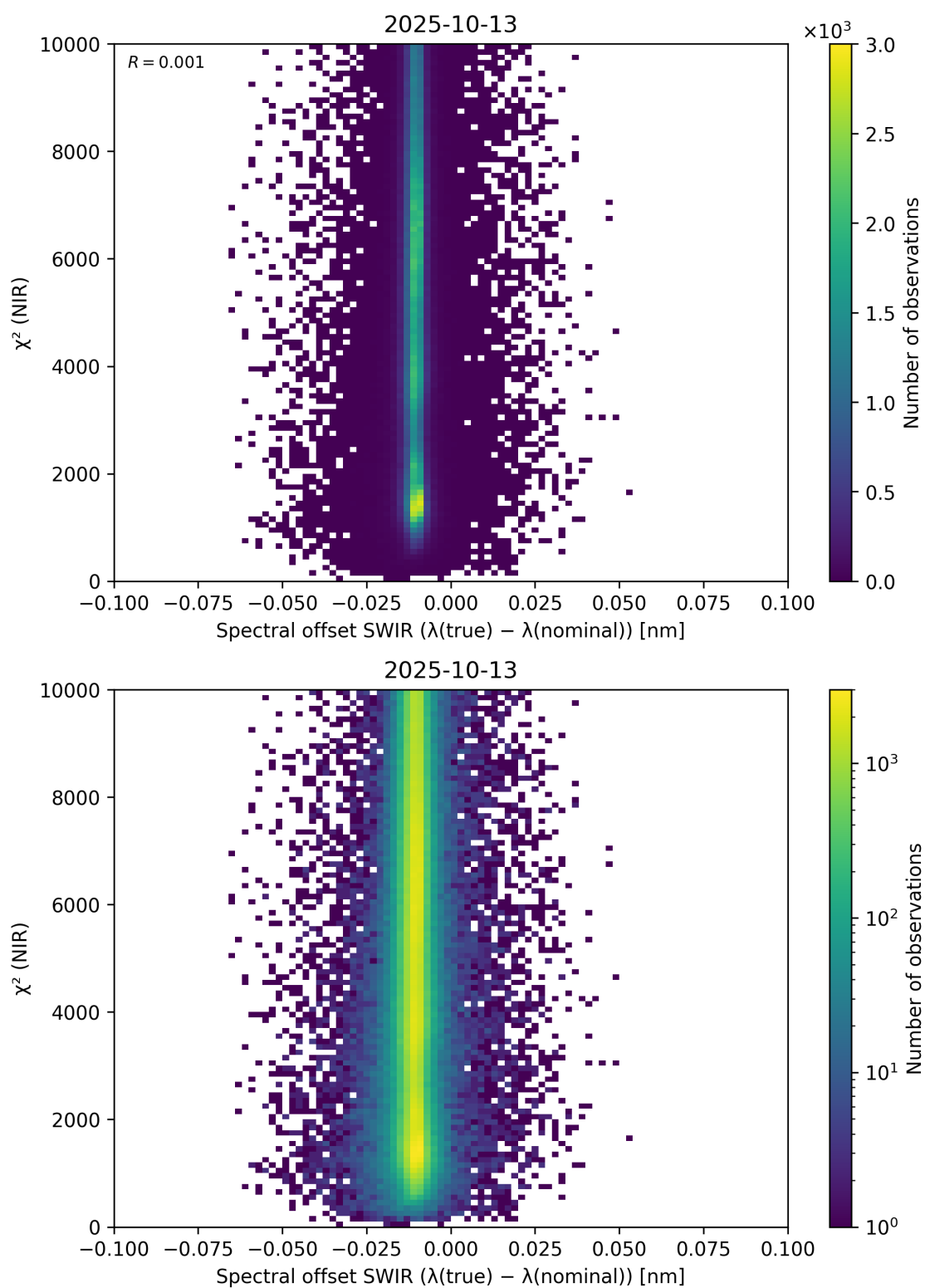
Figure 117: Scatter density plot of “Spectral offset SWIR ( \lambda_{\text{true}} - \lambda_{\text{nominal}} )” against “ \chi^2 (NIR)” for 2025-10-12 to 2025-10-14.
