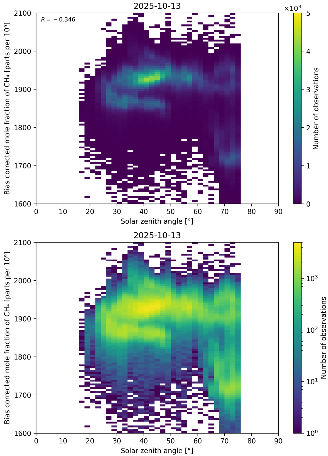
Figure 100: Scatter density plot of “Solar zenith angle” against “Bias corrected mole fraction of CH 4 ” for 2025-10-12 to 2025-10-14.
