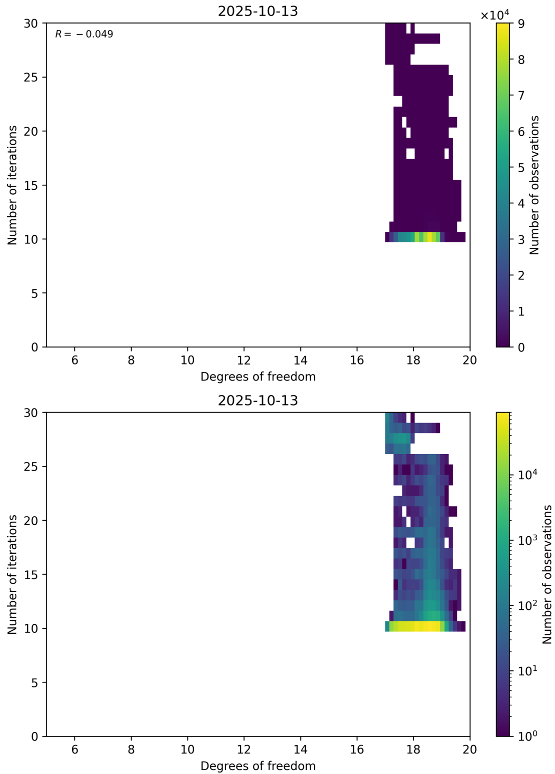
Figure 52: Scatter density plot of “Degrees of freedom” against “Number of iterations” for 2025-10-12 to 2025-10-14.
