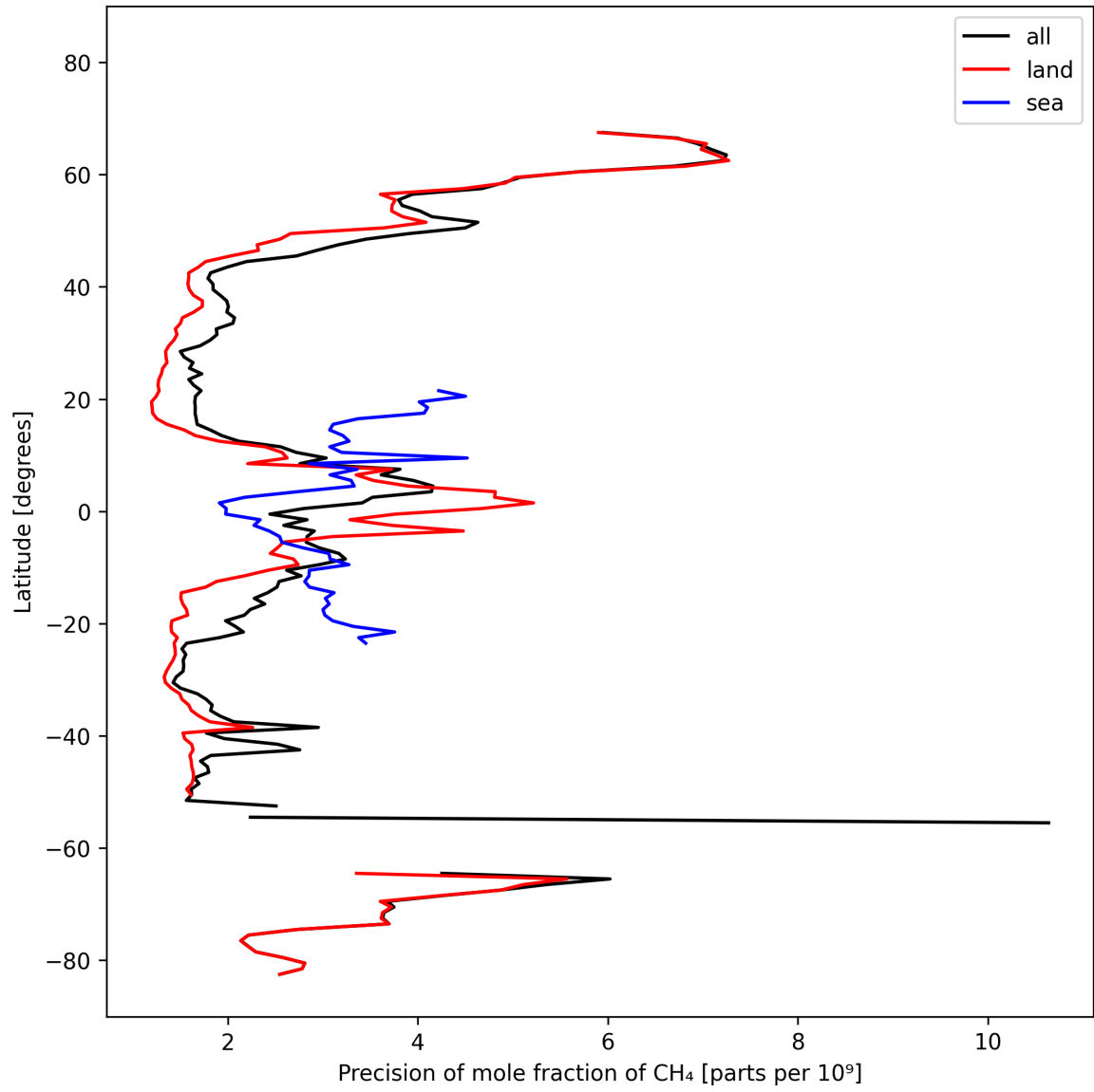
Figure 13: Zonal average of “Precision of mole fraction of CH 4 ” for 2025-10-12 to 2025-10-14.
