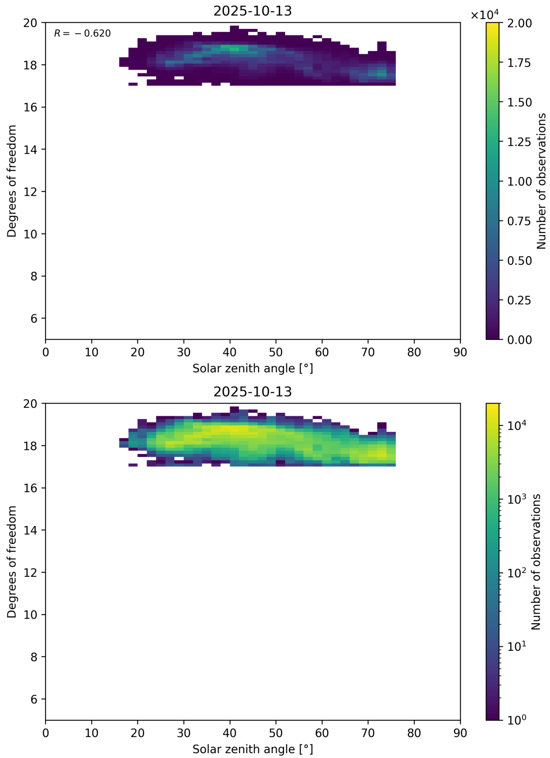
Figure 96: Scatter density plot of “Solar zenith angle” against “Degrees of freedom” for 2025-10-12 to 2025-10-14.
