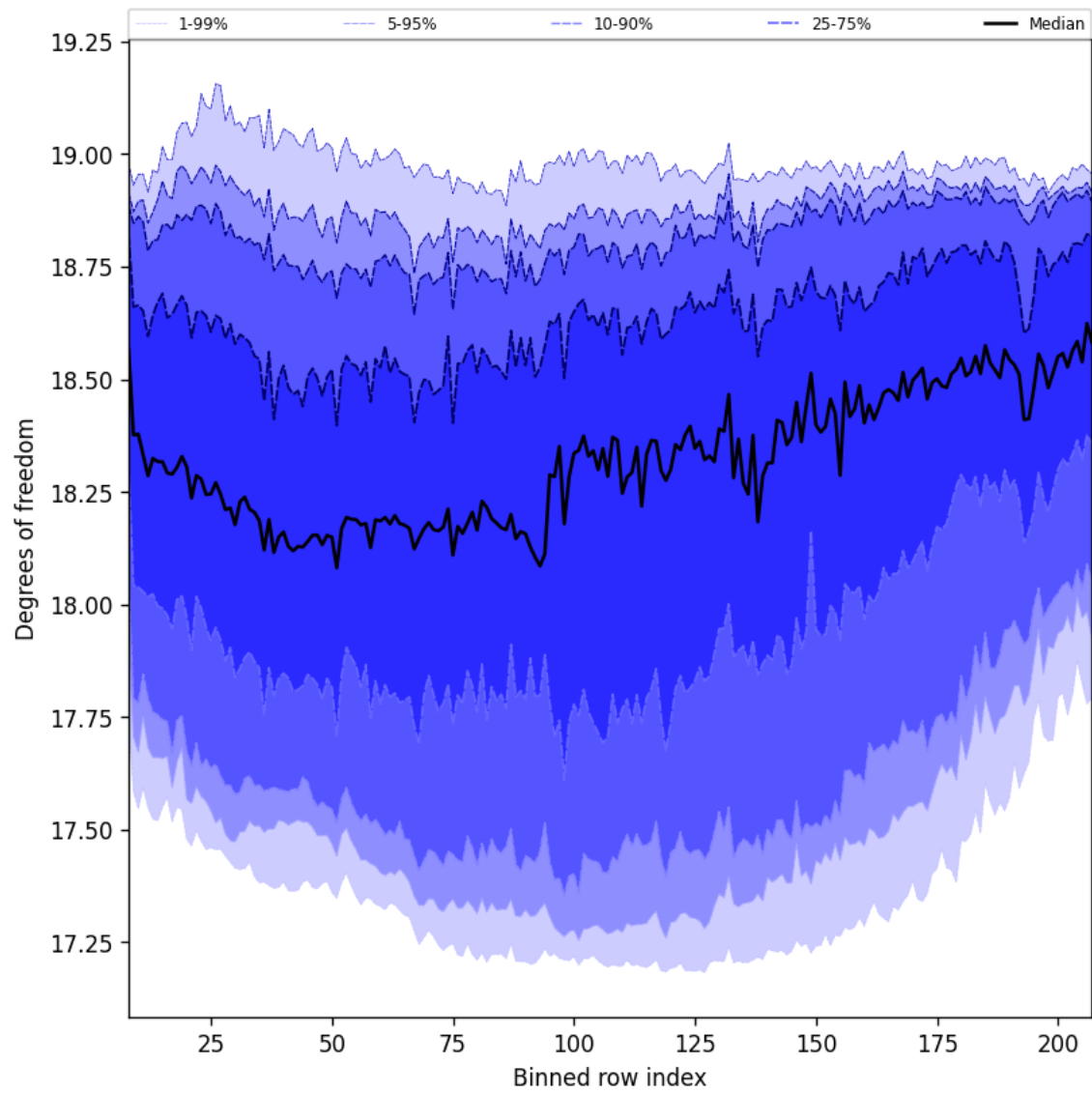
Figure 41: Along track statistics of “Degrees of freedom” for 2025-10-12 to 2025-10-14
