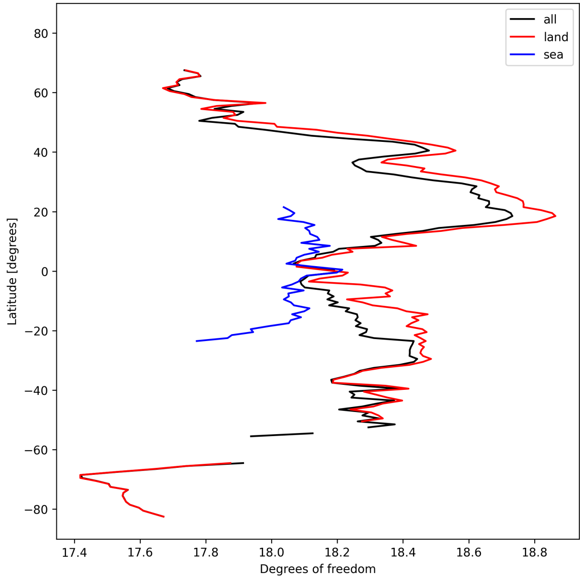
Figure 19: Zonal average of “Degrees of freedom” for 2025-10-12 to 2025-10-14.
