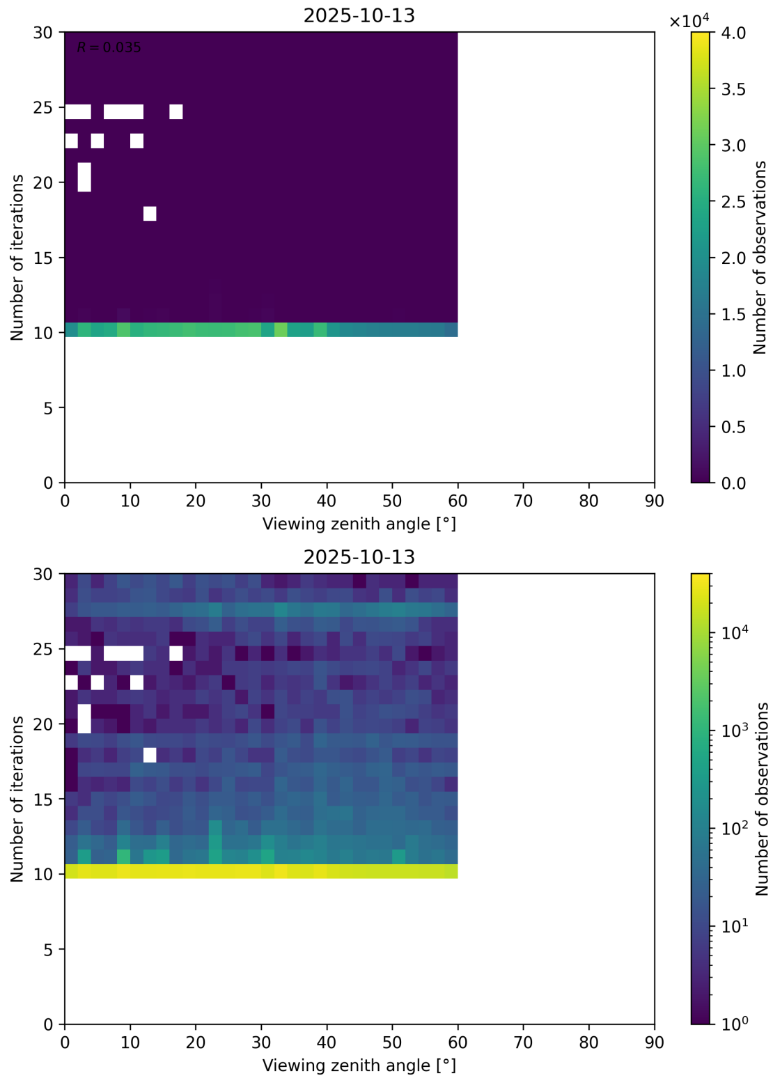
Figure 113: Scatter density plot of “Viewing zenith angle” against “Number of iterations” for 2025-10-12 to 2025-10-14.
