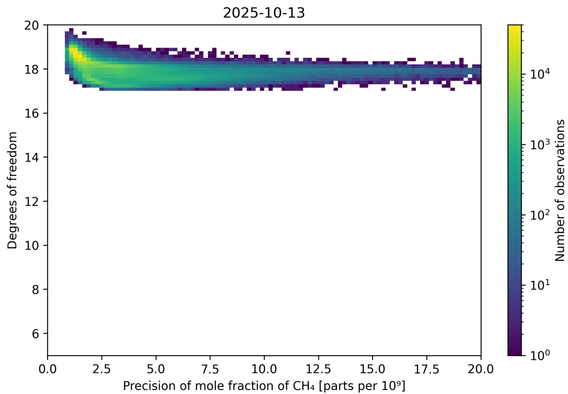
Figure 80: Scatter density plot of “Precision of mole fraction of CH 4 ” against “Degrees of freedom” for 2025-10-12 to 2025-10-14.
