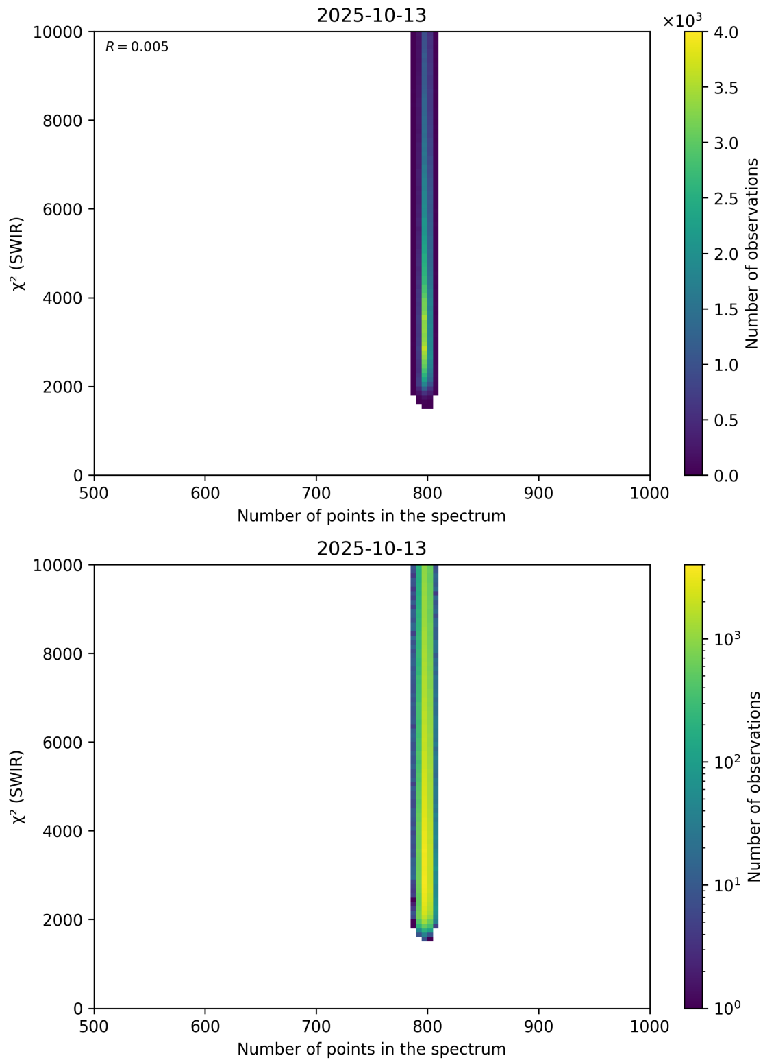
Figure 89: Scatter density plot of “Number of points in the spectrum” against “ \chi^2 (SWIR)” for 2025-10-12 to 2025-10-14.
