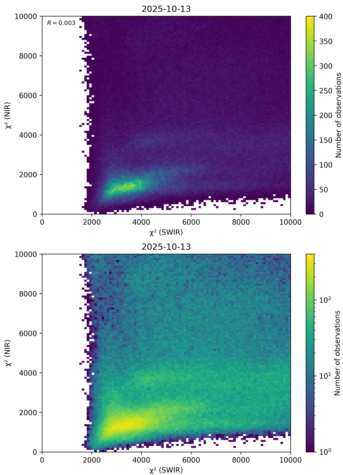
Figure 47: Scatter density plot of “ \chi^2 (SWIR)” against “ \chi^2 (NIR)” for 2025-10-12 to 2025-10-14.
