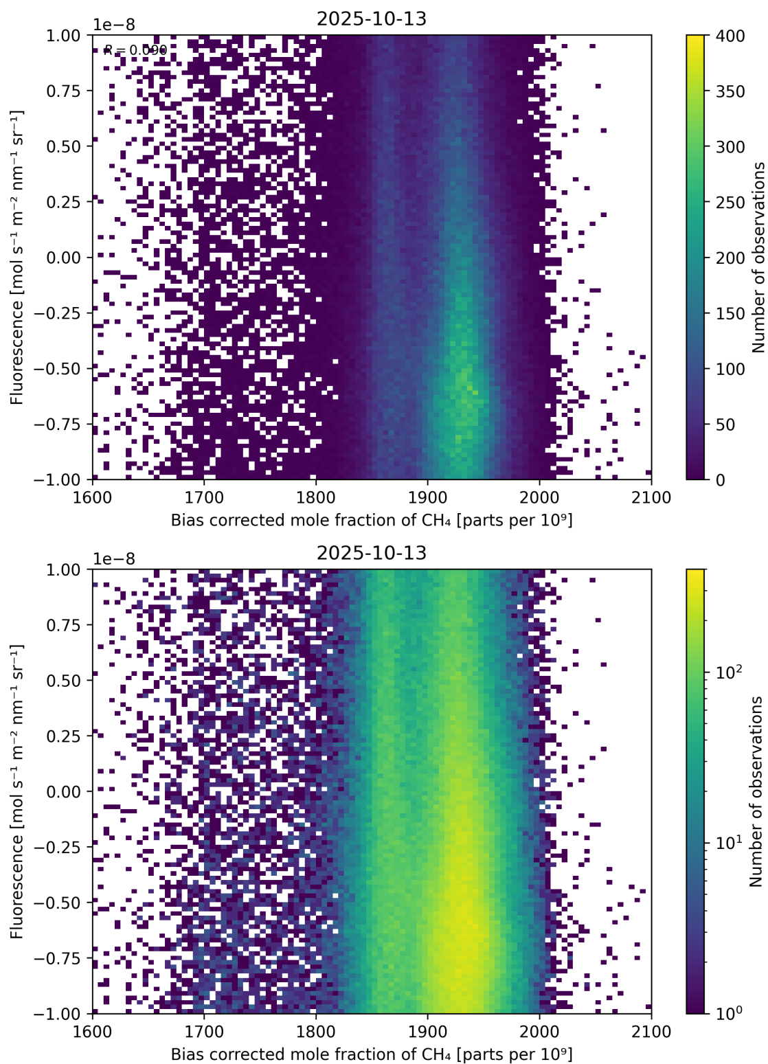
Figure 66: Scatter density plot of “Bias corrected mole fraction of \text{CH}_4 ” against “Fluorescence” for 2025-10-12 to 2025-10-14.
