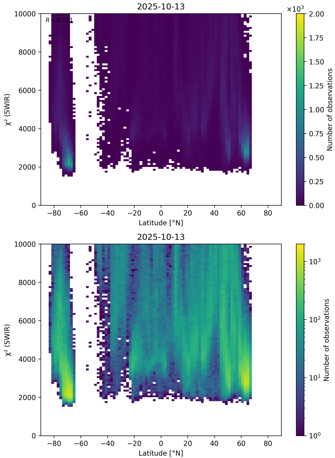
Figure 54: Scatter density plot of “Latitude” against “ \chi^2 (SWIR)” for 2025-10-12 to 2025-10-14.
