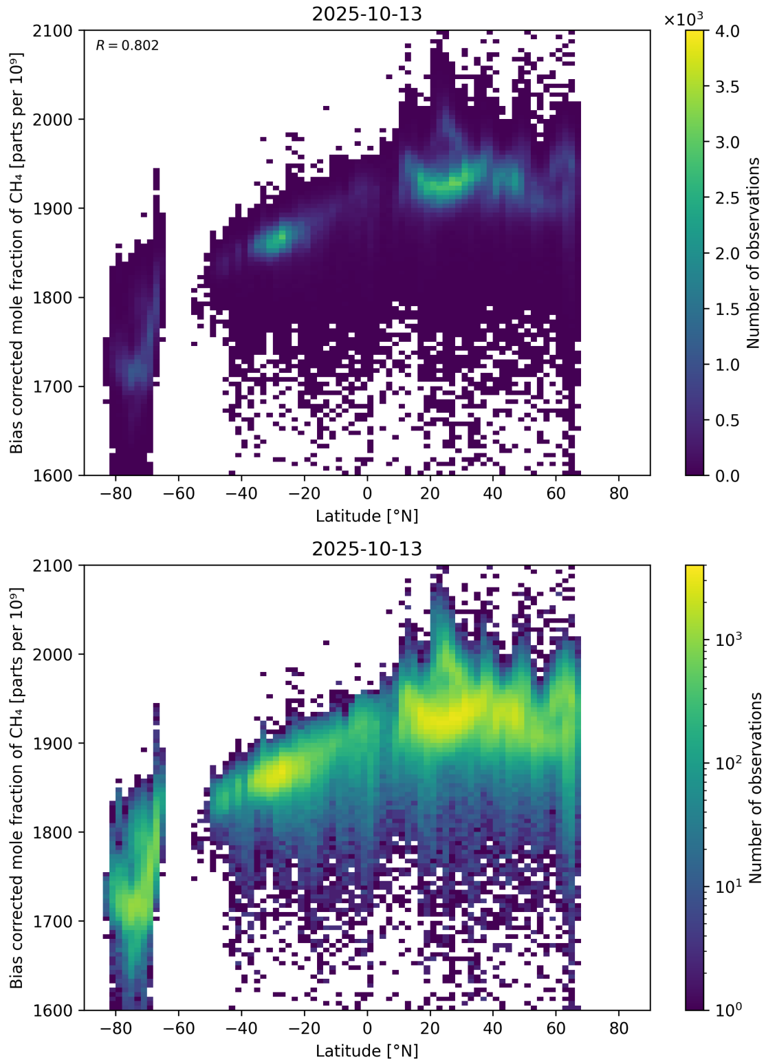
Figure 58: Scatter density plot of “Latitude” against “Bias corrected mole fraction of \text{CH}_4 ” for 2025-10-12 to 2025-10-14.
