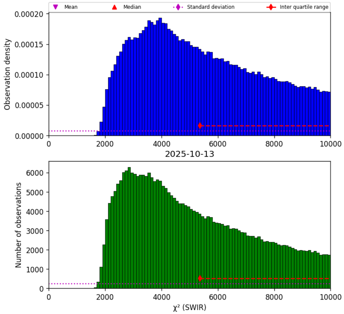
Figure 28: Histogram of “ \chi^2 (SWIR)” for 2025-10-12 to 2025-10-14
