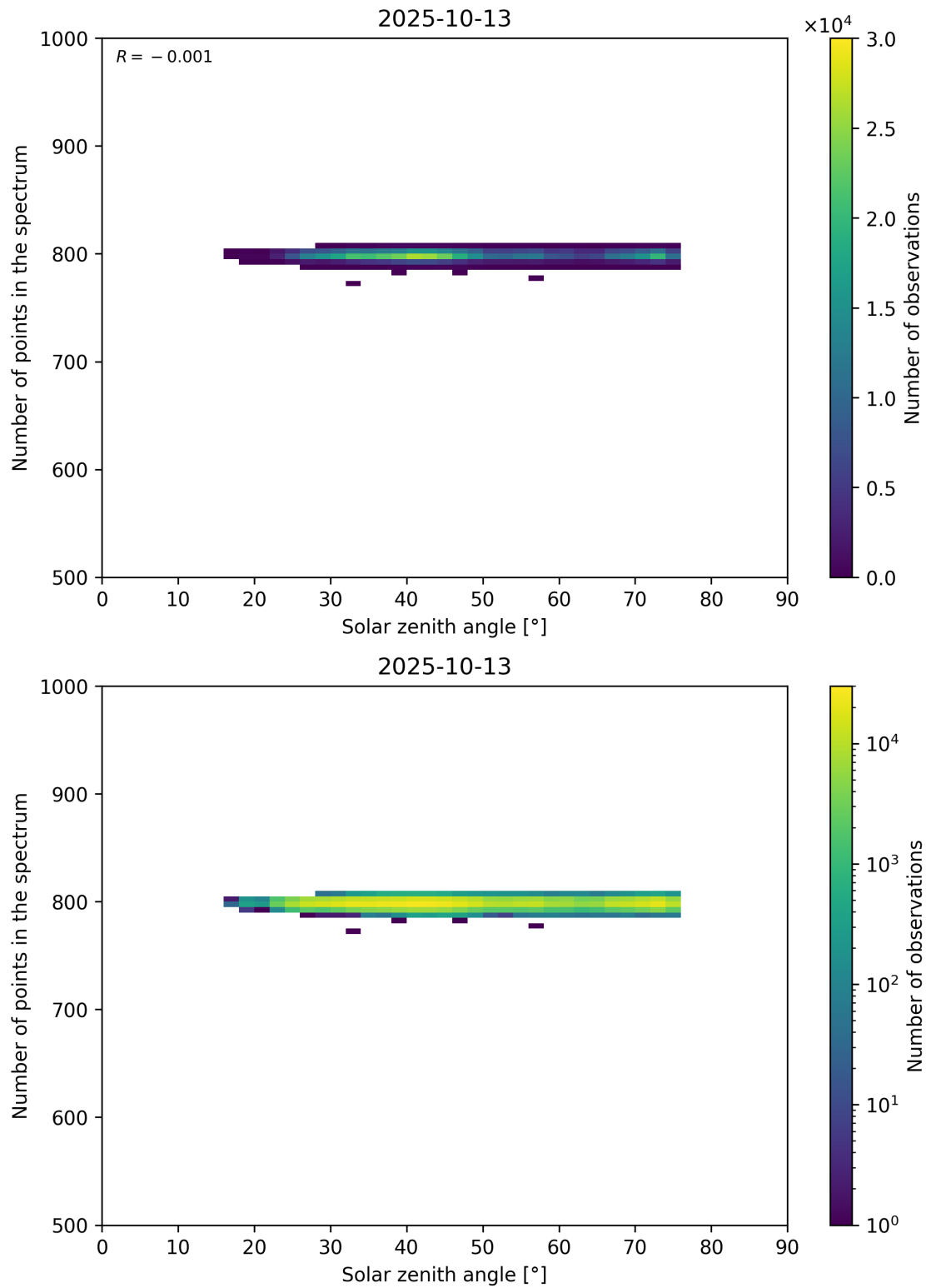
Figure 103: Scatter density plot of “Solar zenith angle” against “Number of points in the spectrum” for 2025-10-12 to 2025-10-14.
