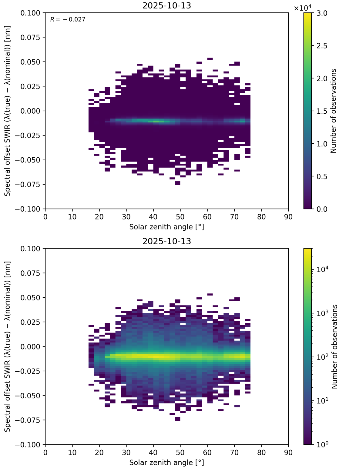
Figure 104: Scatter density plot of “Solar zenith angle” against “Spectral offset SWIR ( \lambda_{\text{true}} - \lambda_{\text{nominal}} )” for 2025-10-12 to 2025-10-14.
