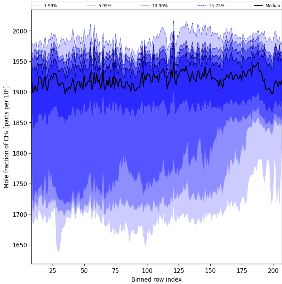
Figure 34: Along track statistics of “Mole fraction of CH 4 ” for 2025-10-12 to 2025-10-14
