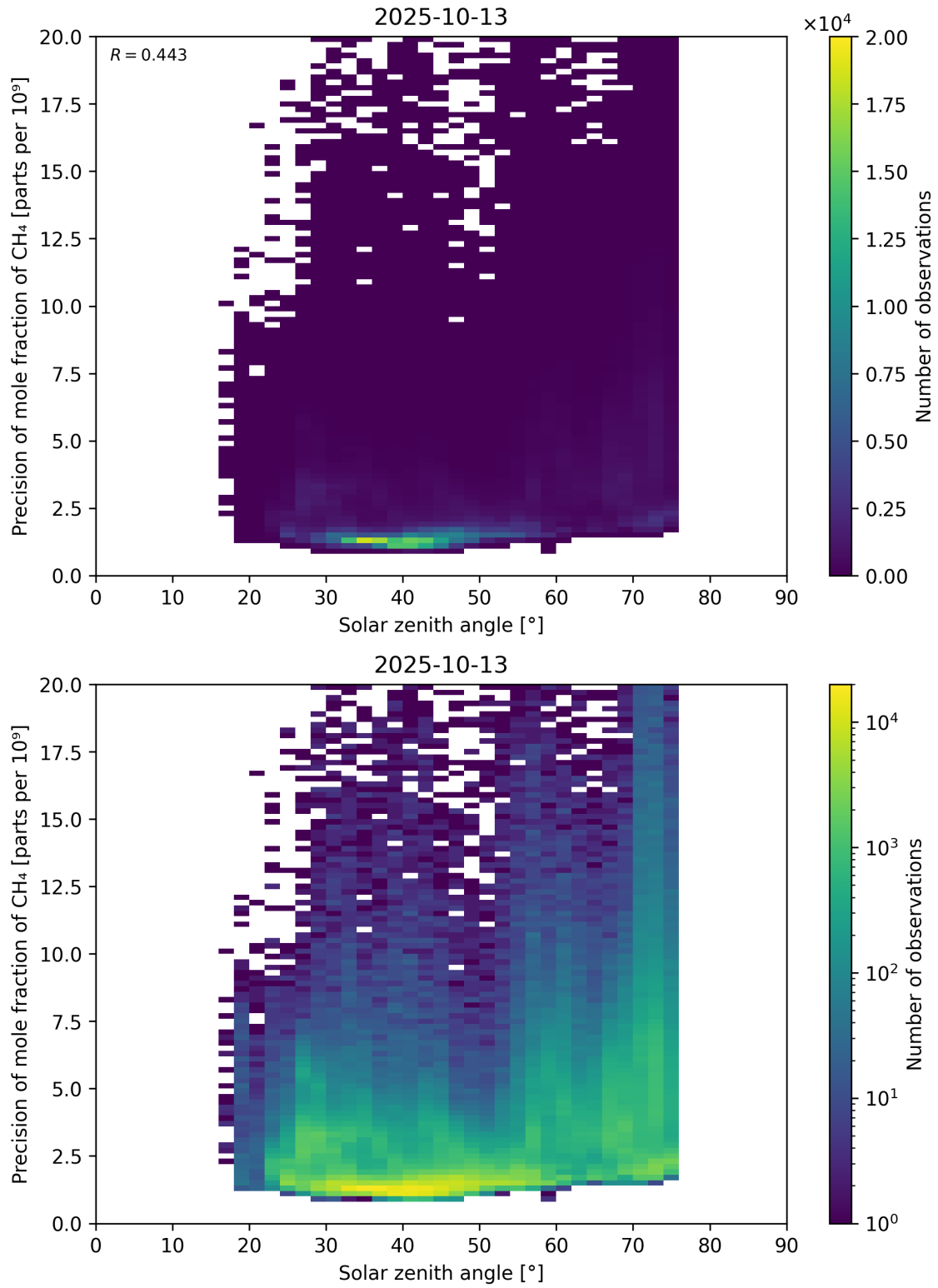
Figure 101: Scatter density plot of “Solar zenith angle” against “Precision of mole fraction of \text{CH}_4 ” for 2025-10-12 to 2025-10-14.
