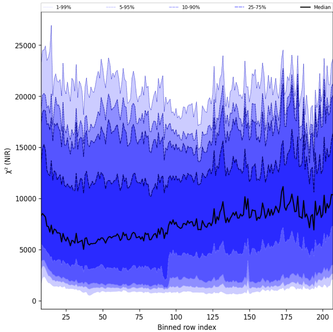
Figure 40: Along track statistics of “ \chi^2 (NIR)” for 2025-10-12 to 2025-10-14
