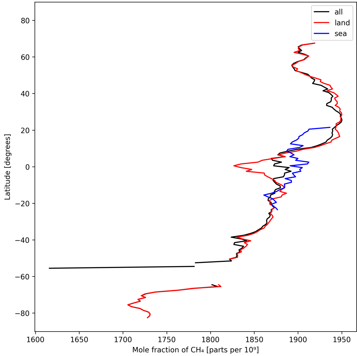
Figure 12: Zonal average of “Mole fraction of CH 4 ” for 2025-10-12 to 2025-10-14.
