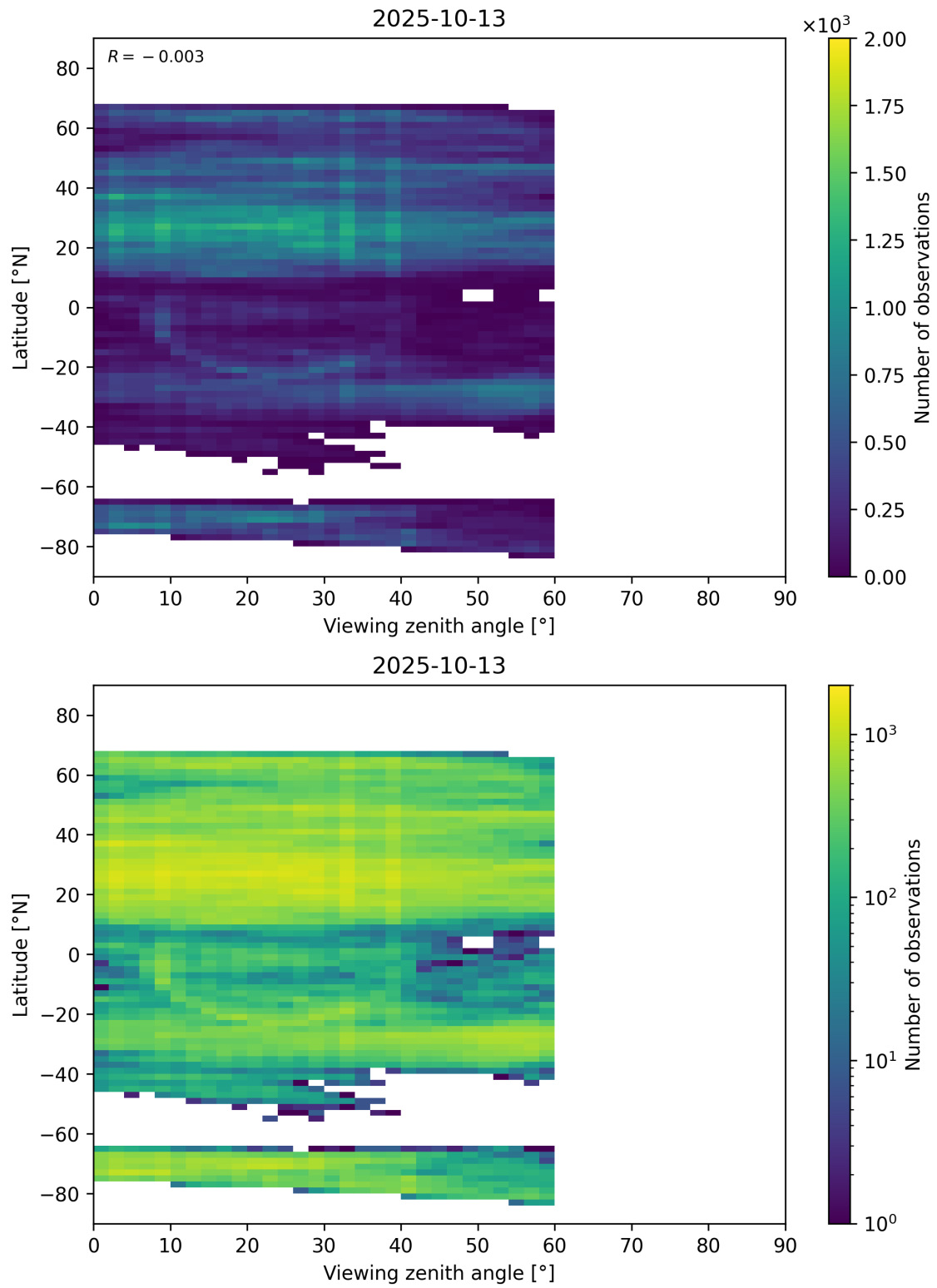
Figure 109: Scatter density plot of “Viewing zenith angle” against “Latitude” for 2025-10-12 to 2025-10-14.
