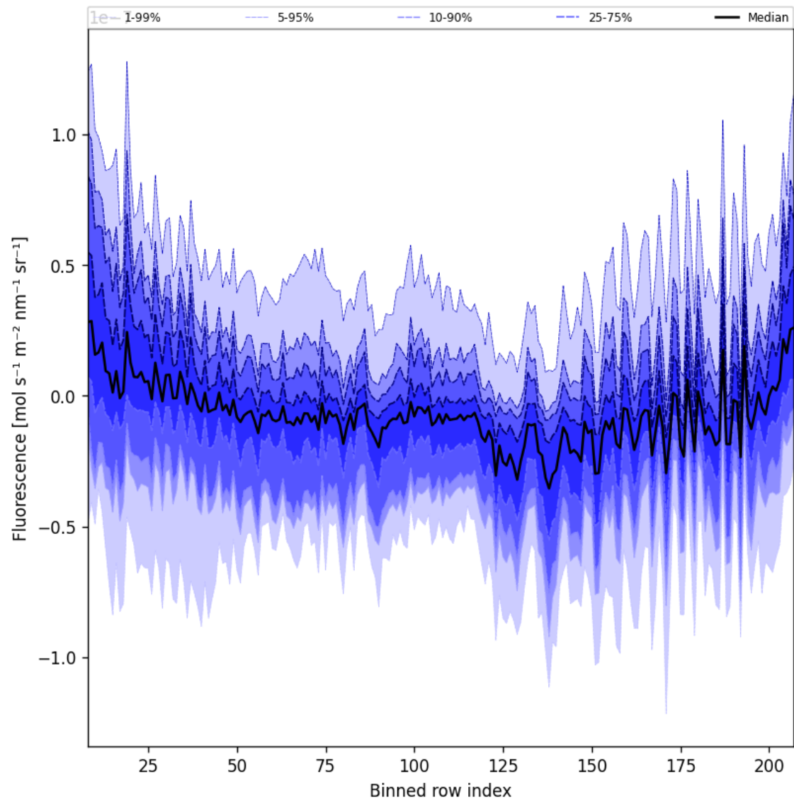
Figure 43: Along track statistics of “Fluorescence” for 2025-10-12 to 2025-10-14
