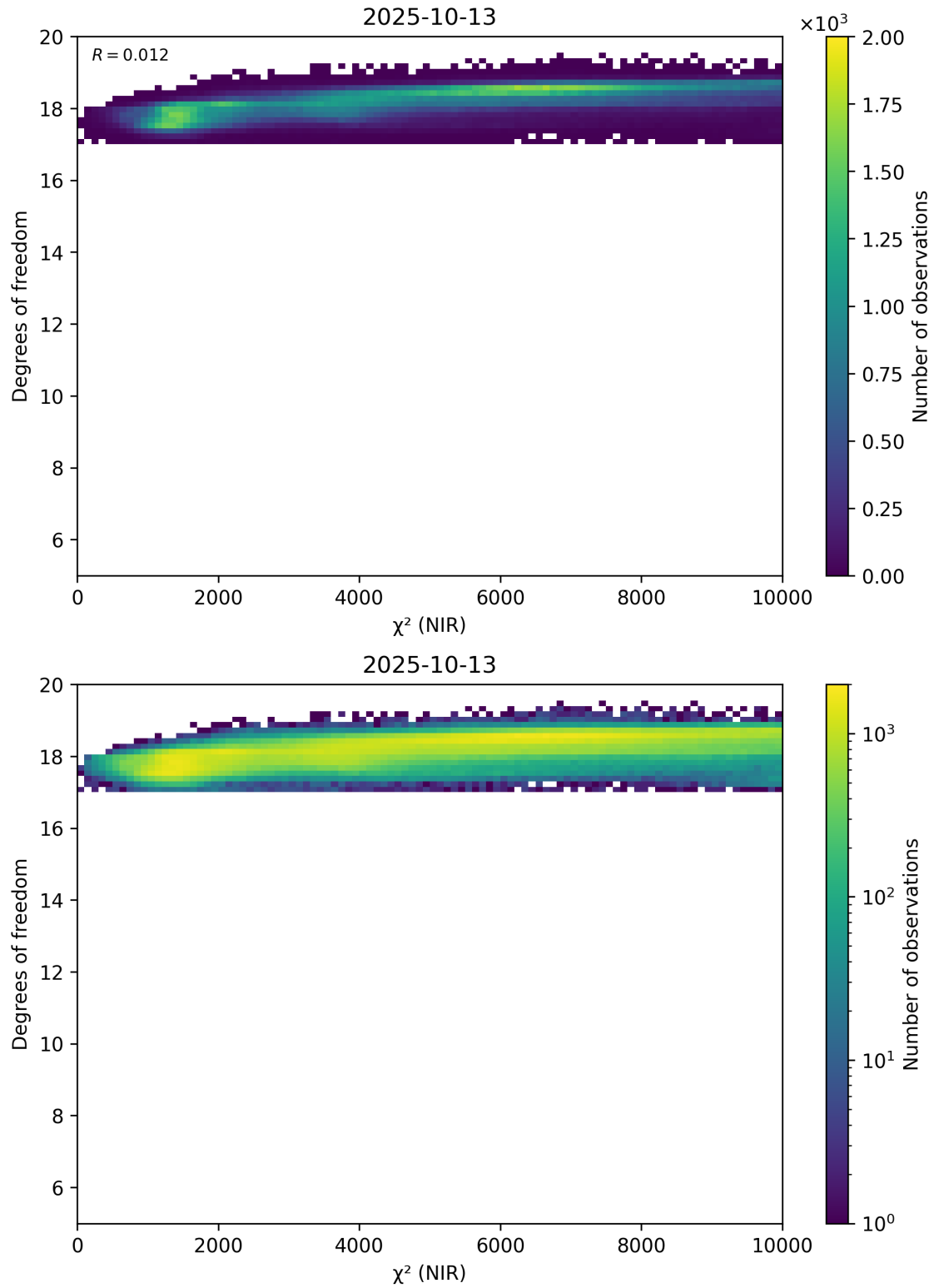
Figure 44: Scatter density plot of “ \chi^2 (NIR)” against “Degrees of freedom” for 2025-10-12 to 2025-10-14.
