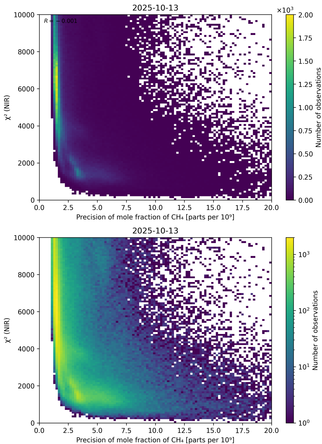
Figure 78: Scatter density plot of “Precision of mole fraction of \text{CH}_4 ” against “ \chi^2 (NIR)” for 2025-10-12 to 2025-10-14.
