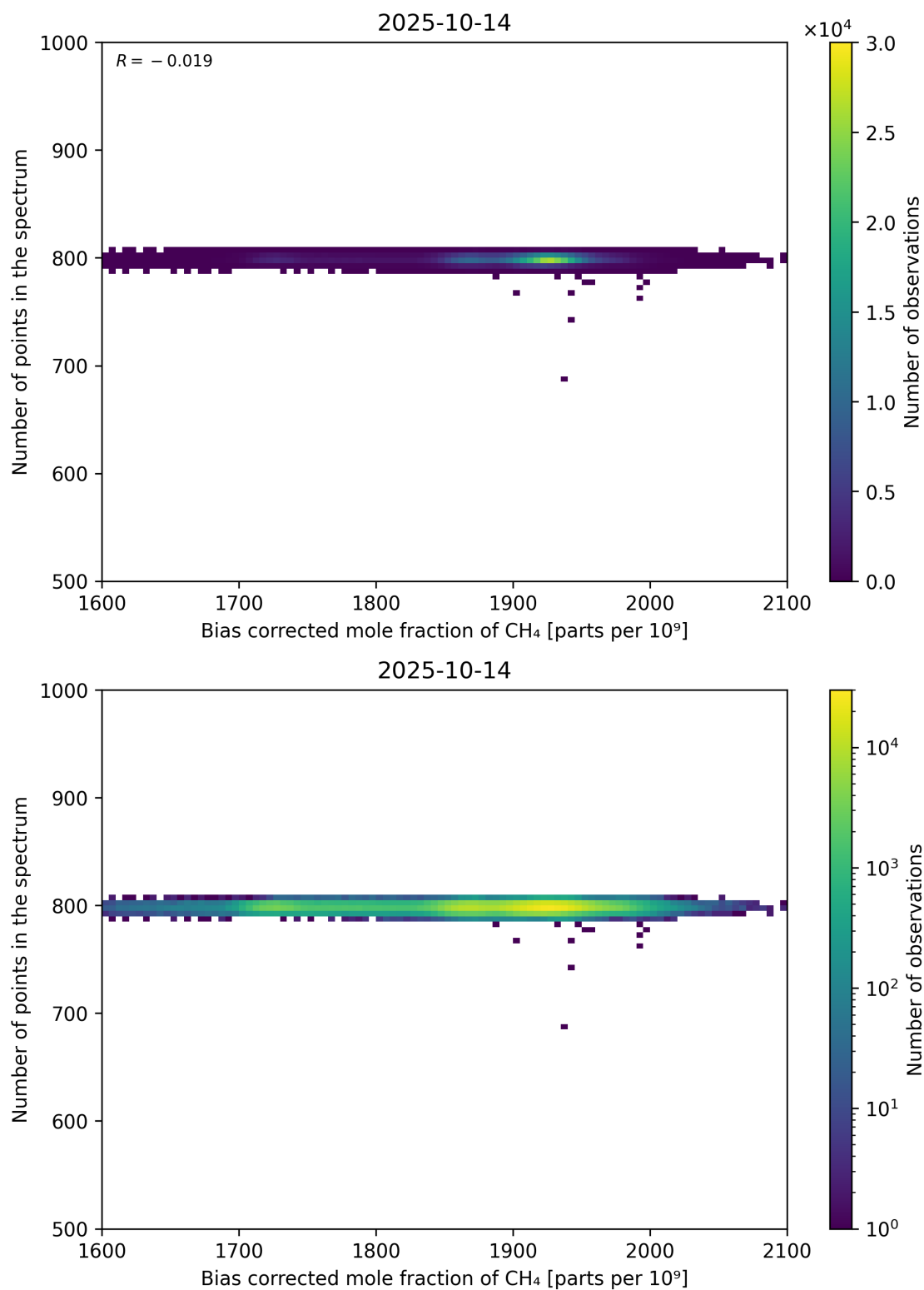
Figure 68: Scatter density plot of “Bias corrected mole fraction of CH 4 ” against “Number of points in the spectrum” for 2025-10-13 to 2025-10-15.
