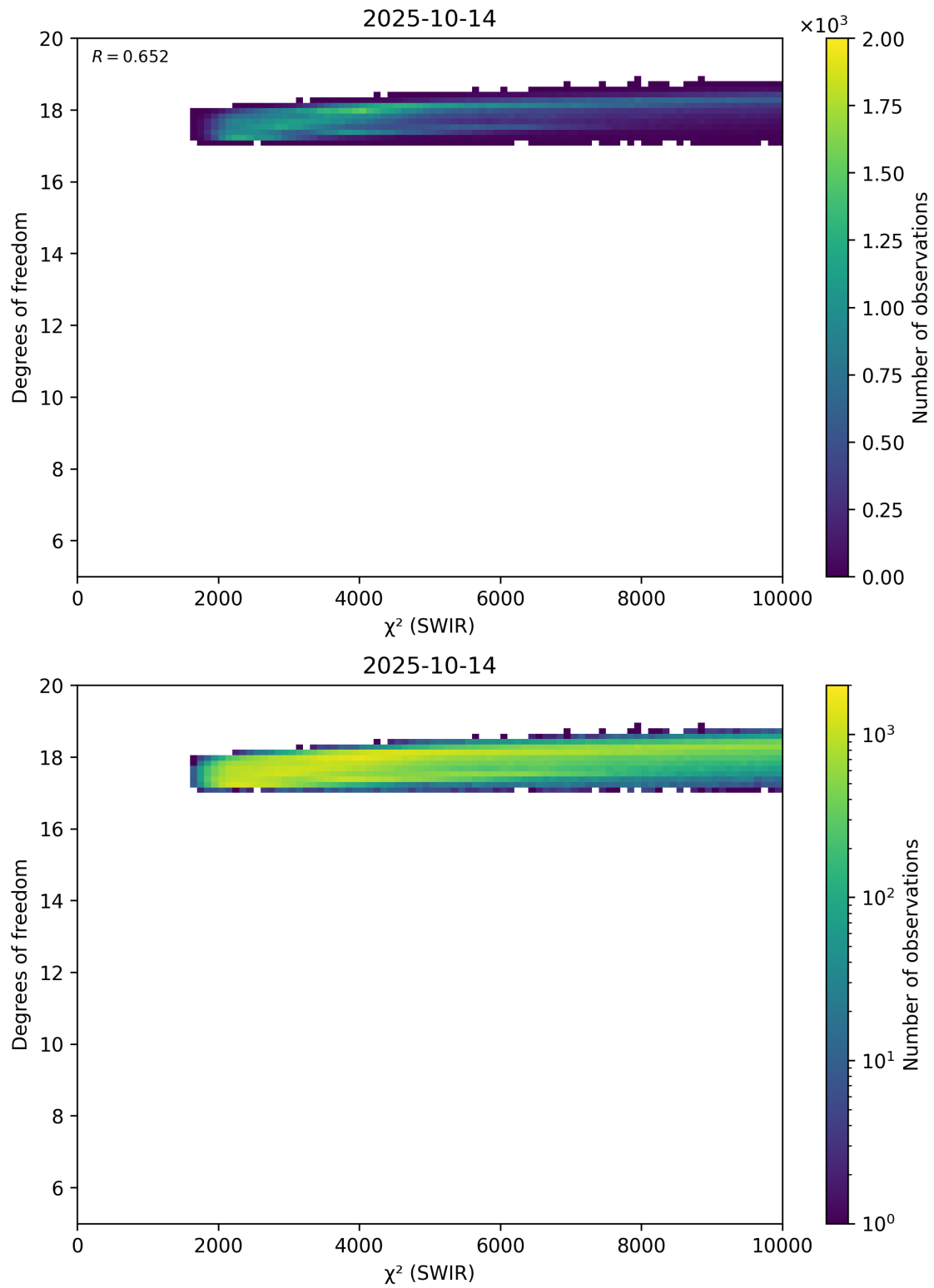
Figure 48: Scatter density plot of “ \chi^2 (SWIR)” against “Degrees of freedom” for 2025-10-13 to 2025-10-15.
