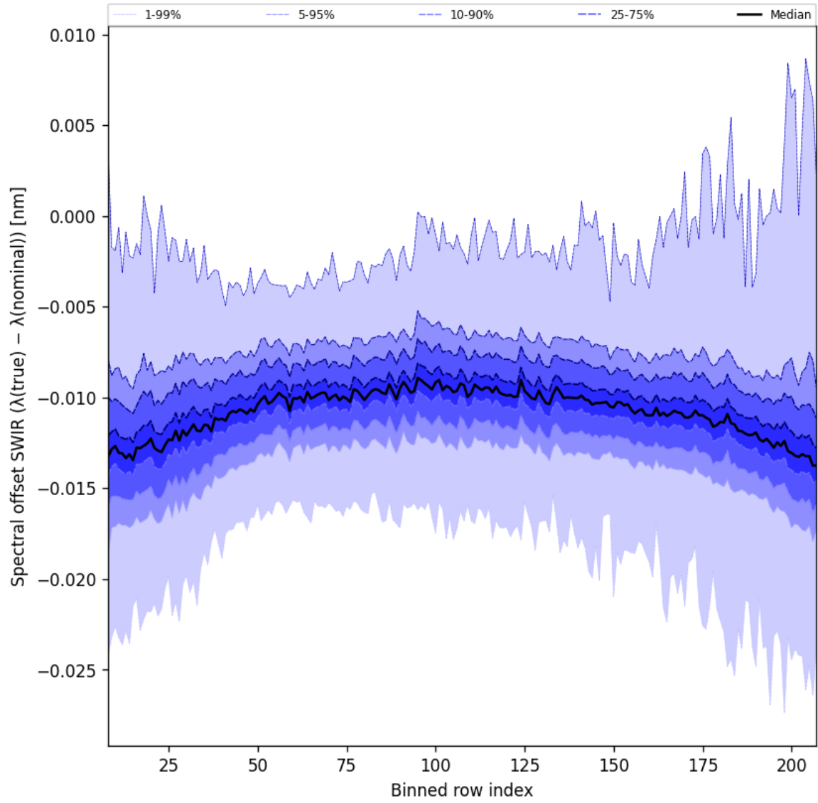
Figure 38: Along track statistics of “Spectral offset SWIR ( \lambda_{\text{true}} - \lambda_{\text{nominal}} )” for 2025-10-13 to 2025-10-15
