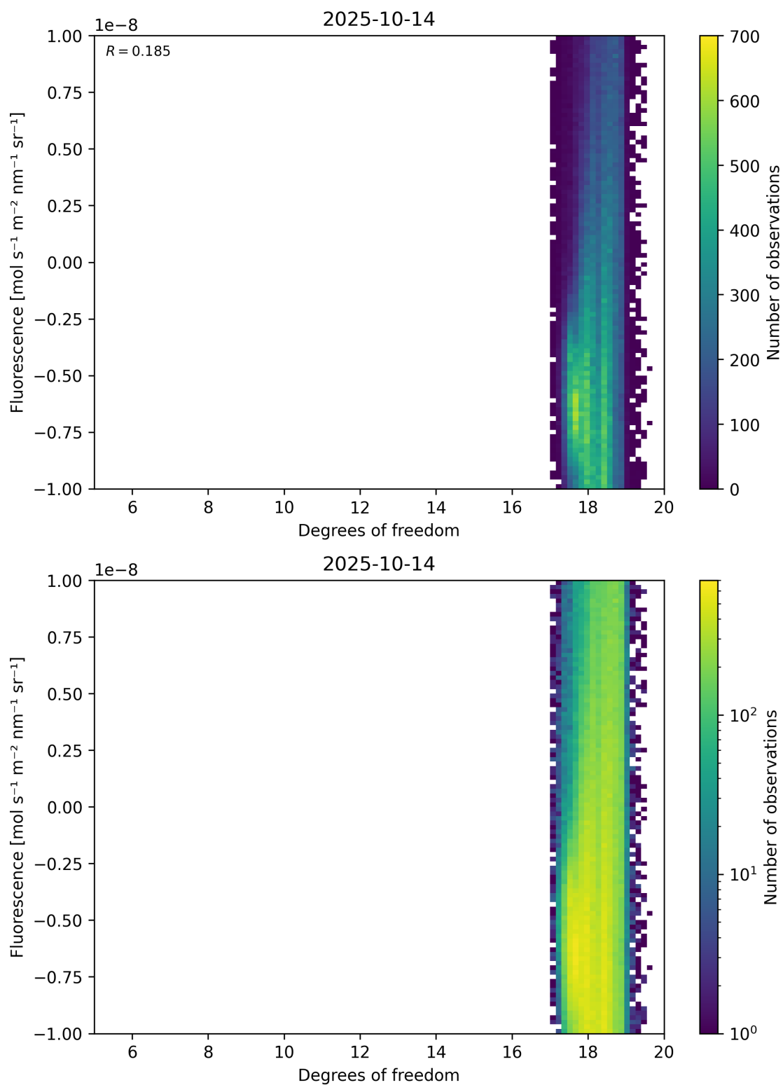
Figure 51: Scatter density plot of “Degrees of freedom” against “Fluorescence” for 2025-10-13 to 2025-10-15.
