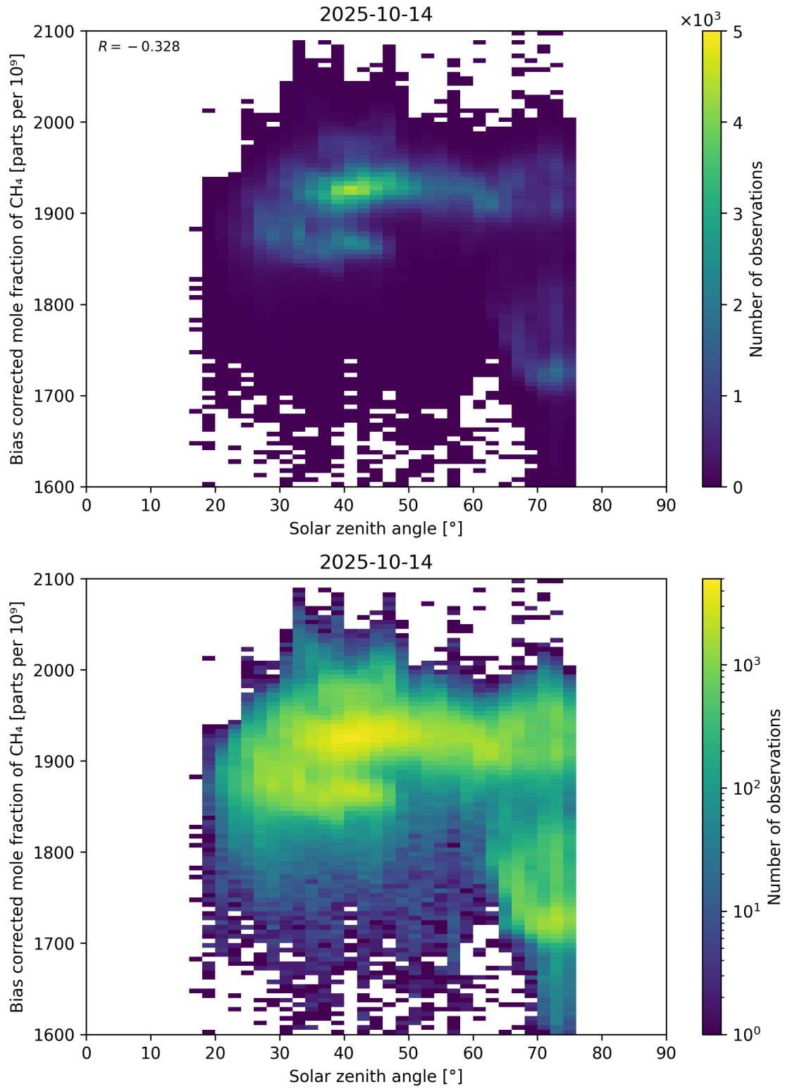
Figure 100: Scatter density plot of “Solar zenith angle” against “Bias corrected mole fraction of CH 4 ” for 2025-10-13 to 2025-10-15.
