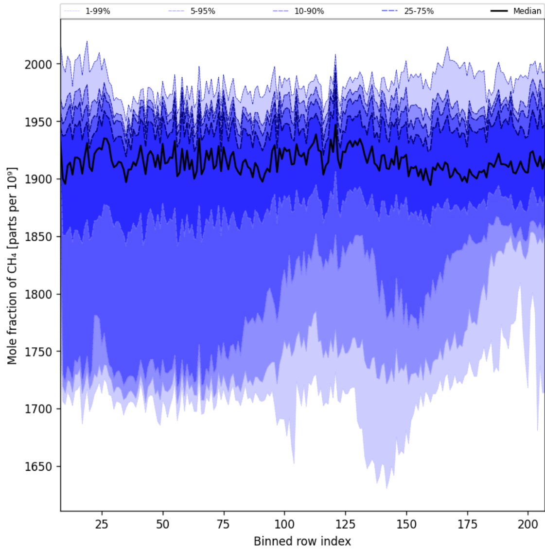
Figure 34: Along track statistics of “Mole fraction of CH 4 ” for 2025-10-13 to 2025-10-15
