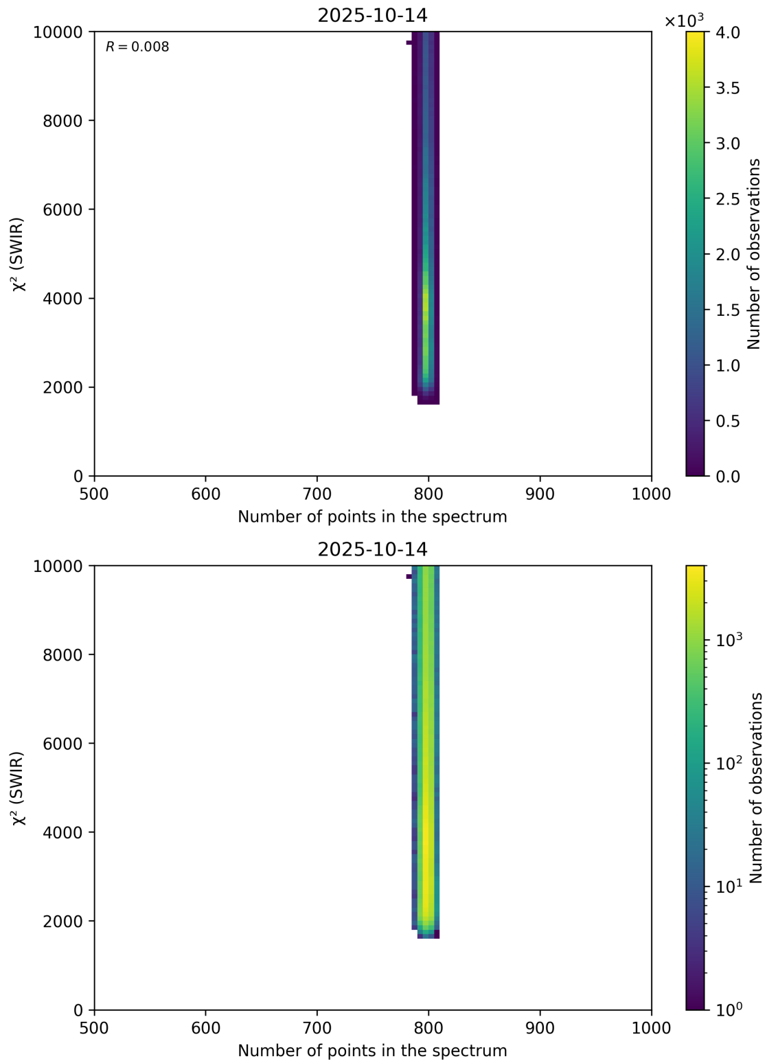
Figure 89: Scatter density plot of “Number of points in the spectrum” against “ \chi^2 (SWIR)” for 2025-10-13 to 2025-10-15.
