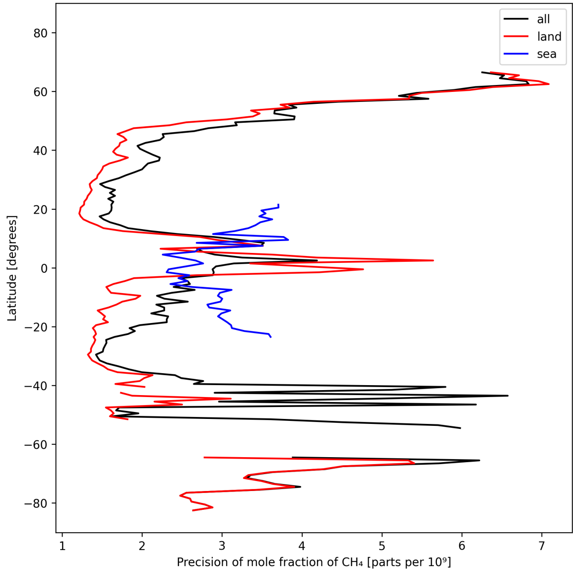
Figure 13: Zonal average of “Precision of mole fraction of CH 4 ” for 2025-10-13 to 2025-10-15.
