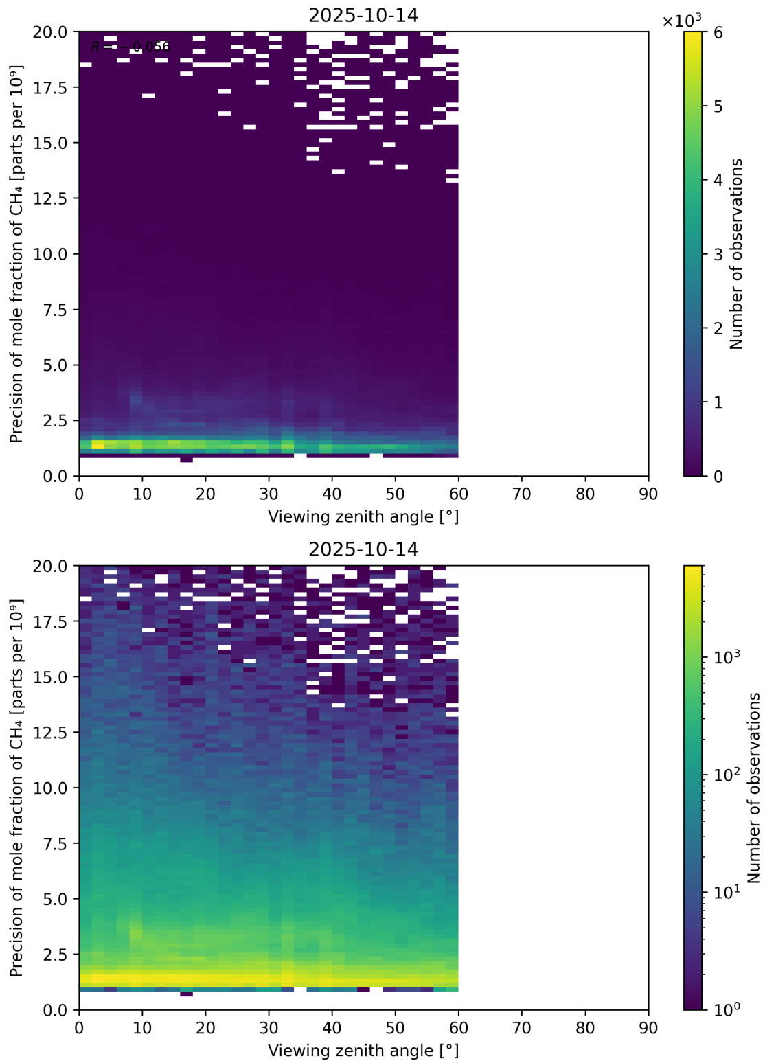
Figure 112: Scatter density plot of “Viewing zenith angle” against “Precision of mole fraction of CH 4 ” for 2025-10-13 to 2025-10-15.
