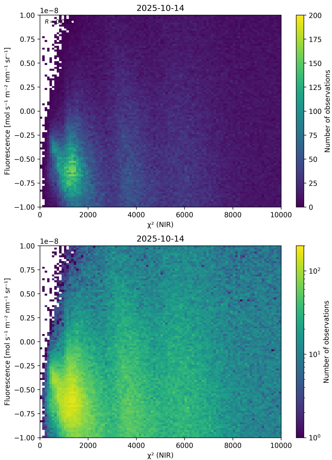
Figure 45: Scatter density plot of “ \chi^2 (NIR)” against “Fluorescence” for 2025-10-13 to 2025-10-15.
