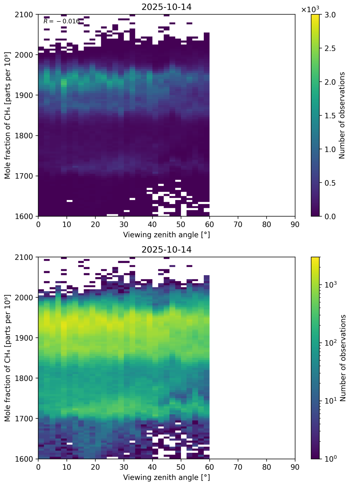
Figure 110: Scatter density plot of “Viewing zenith angle” against “Mole fraction of CH 4 ” for 2025-10-13 to 2025-10-15.
