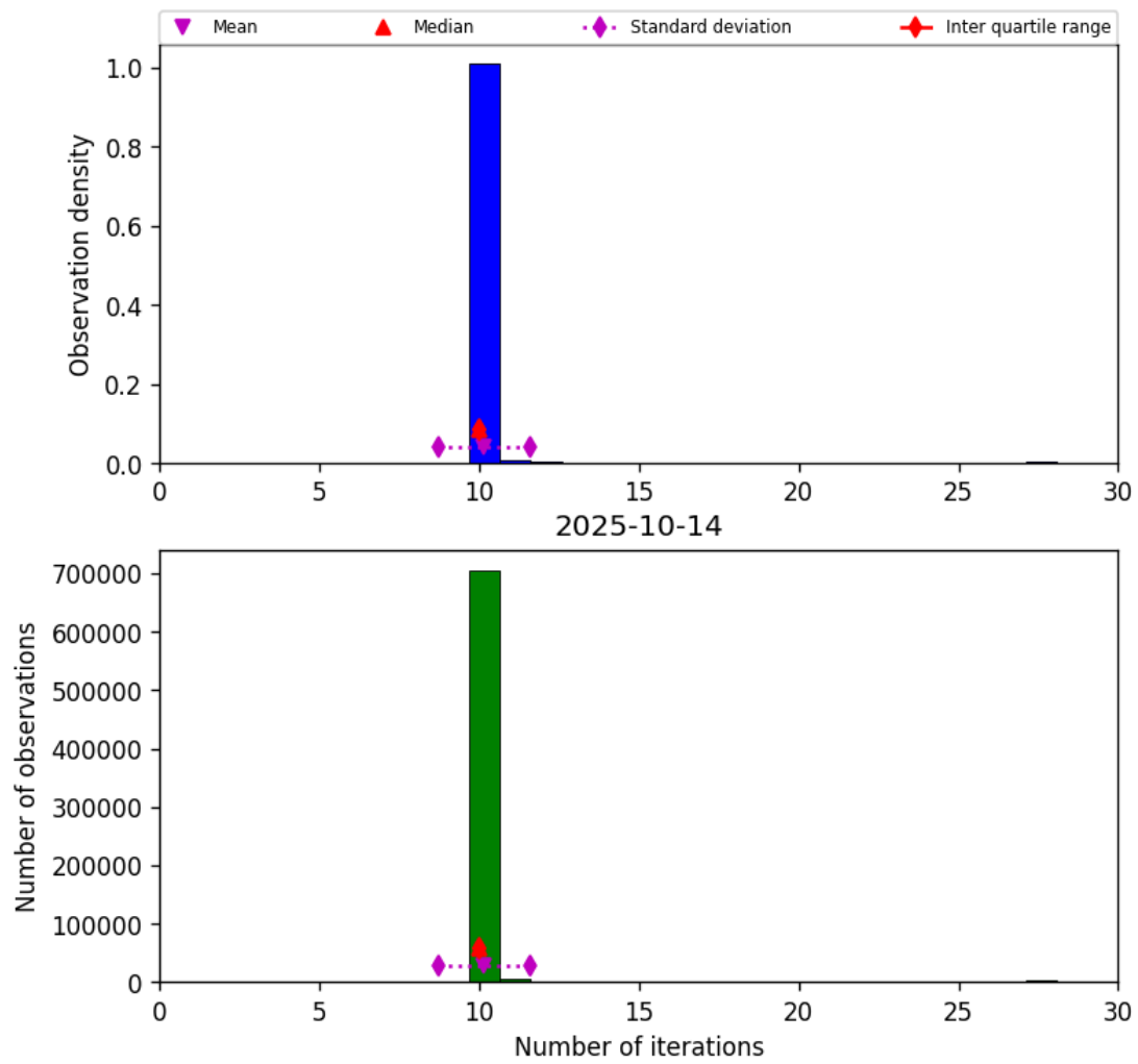
Figure 31: Histogram of “Number of iterations” for 2025-10-13 to 2025-10-15
