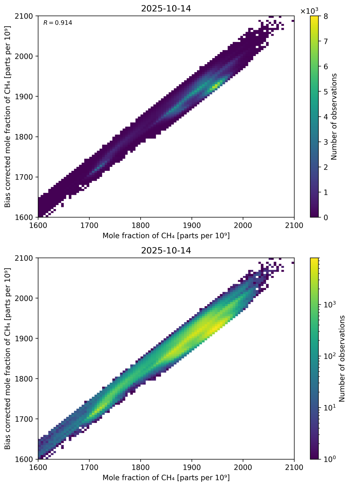
Figure 74: Scatter density plot of “Mole fraction of CH 4 ” against “Bias corrected mole fraction of CH 4 ” for 2025-10-13 to 2025-10-15.
