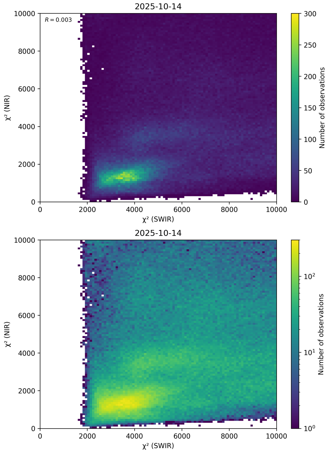
Figure 47: Scatter density plot of “ \chi^2 (SWIR)” against “ \chi^2 (NIR)” for 2025-10-13 to 2025-10-15.
