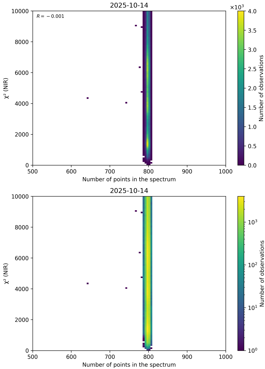
Figure 88: Scatter density plot of “Number of points in the spectrum” against “ \chi^2 (NIR)” for 2025-10-13 to 2025-10-15.
