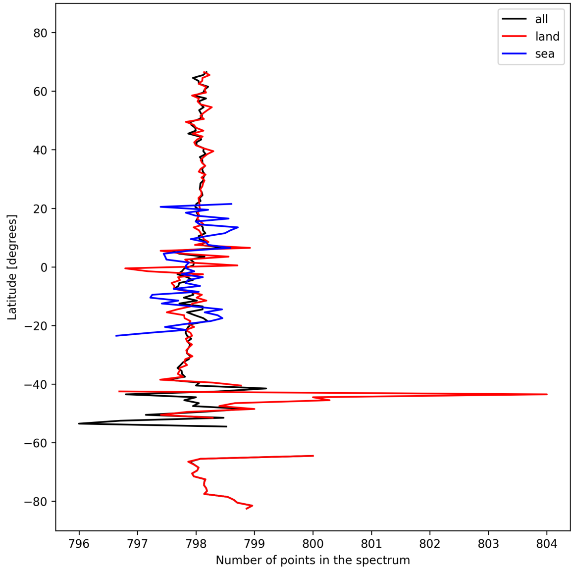
Figure 15: Zonal average of “Number of points in the spectrum” for 2025-10-13 to 2025-10-15.
