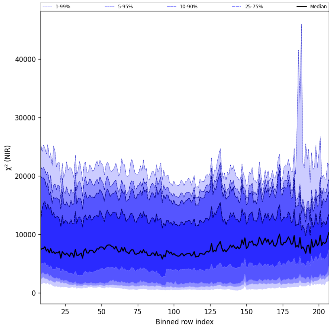
Figure 40: Along track statistics of " \chi^2 (NIR)" for 2025-10-13 to 2025-10-15
