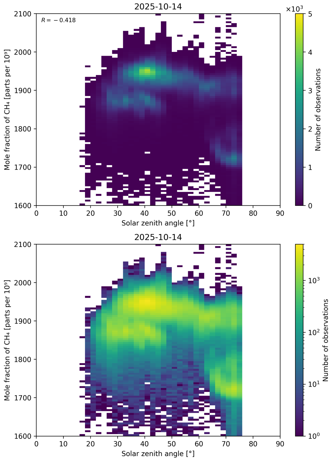
Figure 99: Scatter density plot of “Solar zenith angle” against “Mole fraction of CH 4 ” for 2025-10-13 to 2025-10-15.
