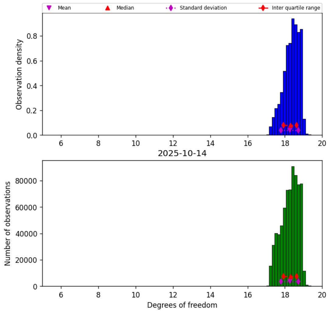
Figure 30: Histogram of “Degrees of freedom” for 2025-10-13 to 2025-10-15
