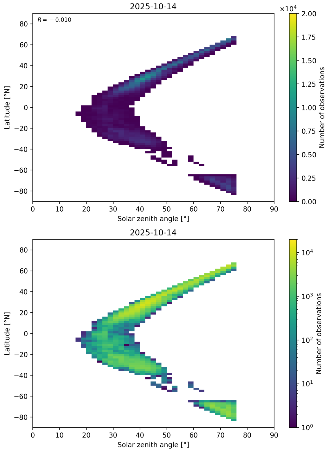
Figure 98: Scatter density plot of “Solar zenith angle” against “Latitude” for 2025-10-13 to 2025-10-15.
