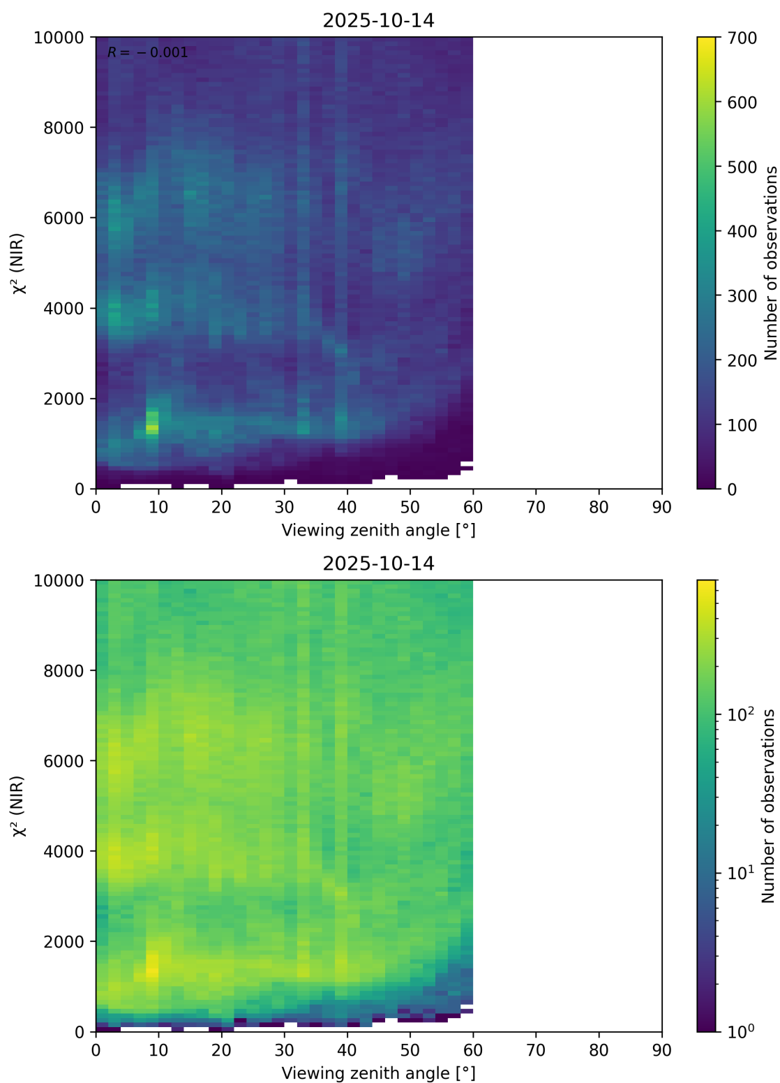
Figure 105: Scatter density plot of “Viewing zenith angle” against “ \chi^2 (NIR)” for 2025-10-13 to 2025-10-15.
