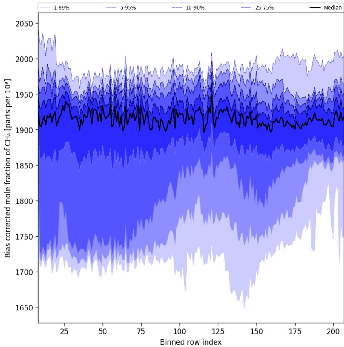
Figure 36: Along track statistics of “Bias corrected mole fraction of \text{CH}_4 ” for 2025-10-13 to 2025-10-15
