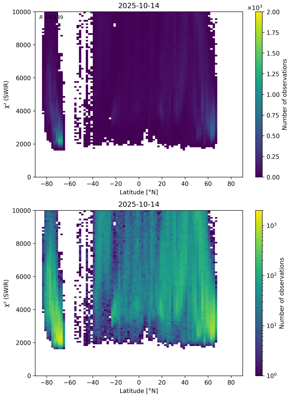
Figure 54: Scatter density plot of “Latitude” against “ \chi^2 (SWIR)” for 2025-10-13 to 2025-10-15.
