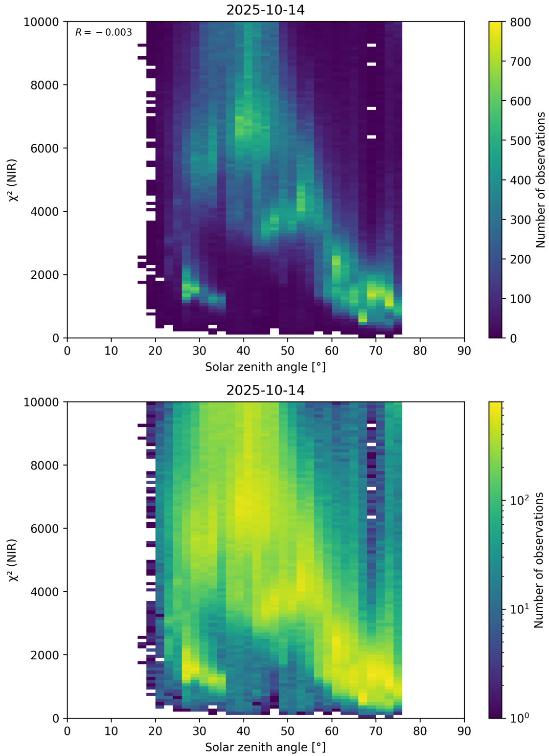
Figure 94: Scatter density plot of “Solar zenith angle” against “ \chi^2 (NIR)” for 2025-10-13 to 2025-10-15.
