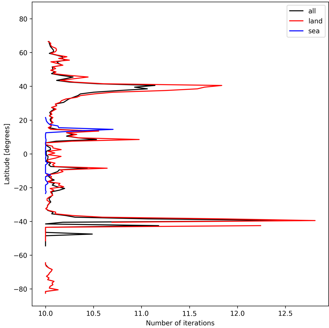
Figure 20: Zonal average of “Number of iterations” for 2025-10-13 to 2025-10-15.
