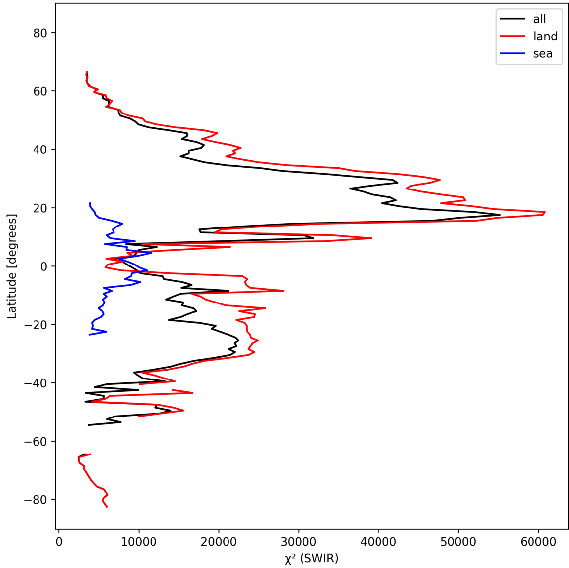
Figure 17: Zonal average of “ \chi^2 (SWIR)” for 2025-10-13 to 2025-10-15.
