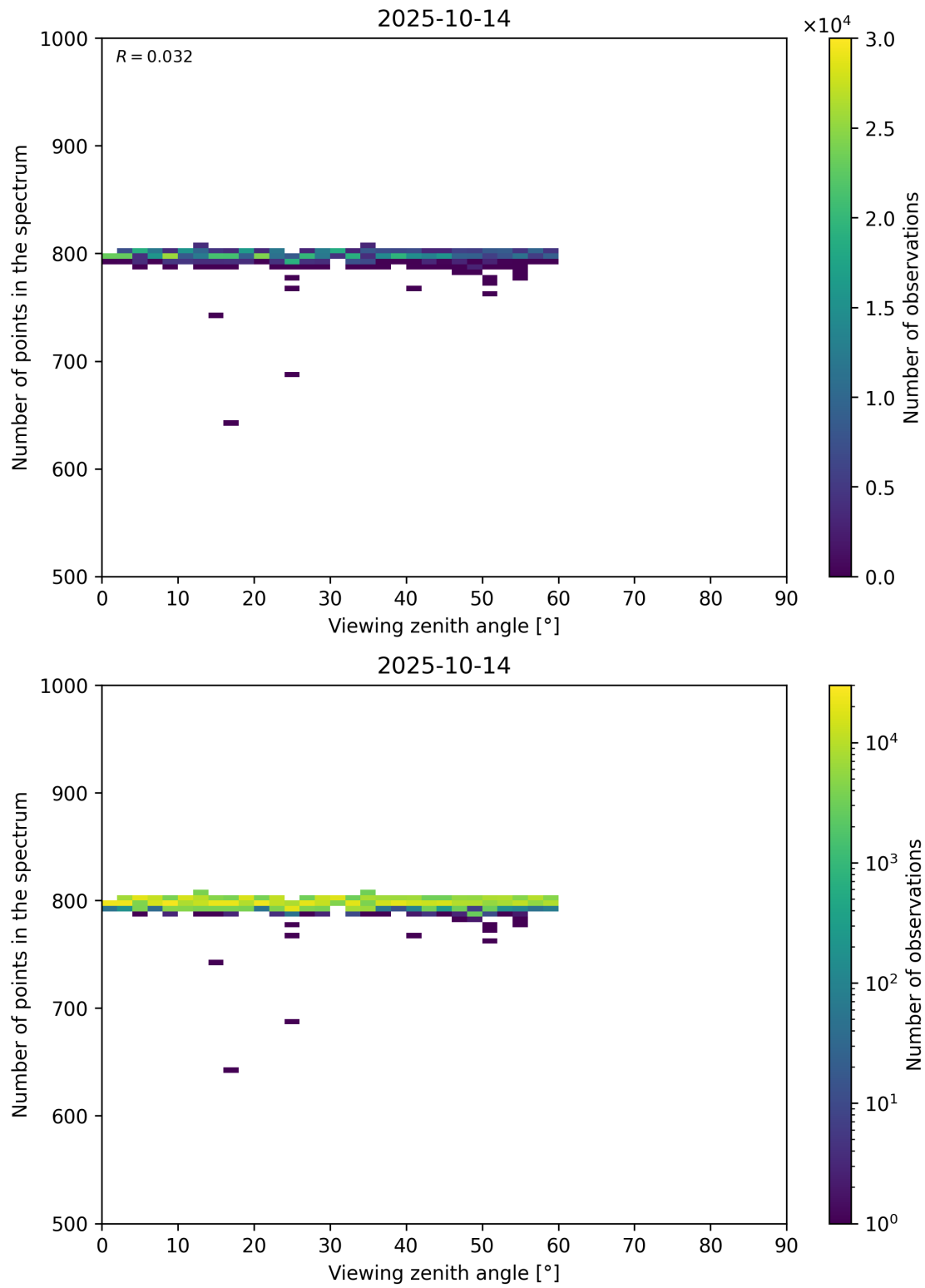
Figure 114: Scatter density plot of “Viewing zenith angle” against “Number of points in the spectrum” for 2025-10-13 to 2025-10-15.
