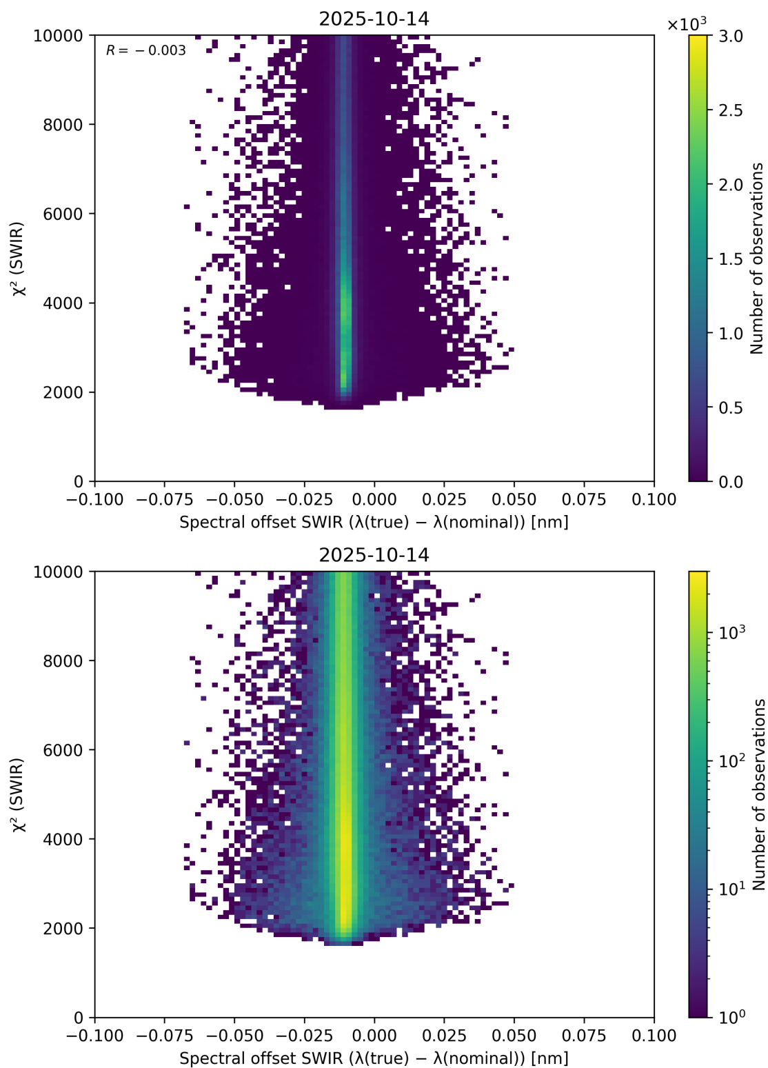
Figure 118: Scatter density plot of “Spectral offset SWIR ( \lambda_{\text{true}} - \lambda_{\text{nominal}} )” against “ \chi^2 (SWIR)” for 2025-10-13 to 2025-10-15.
