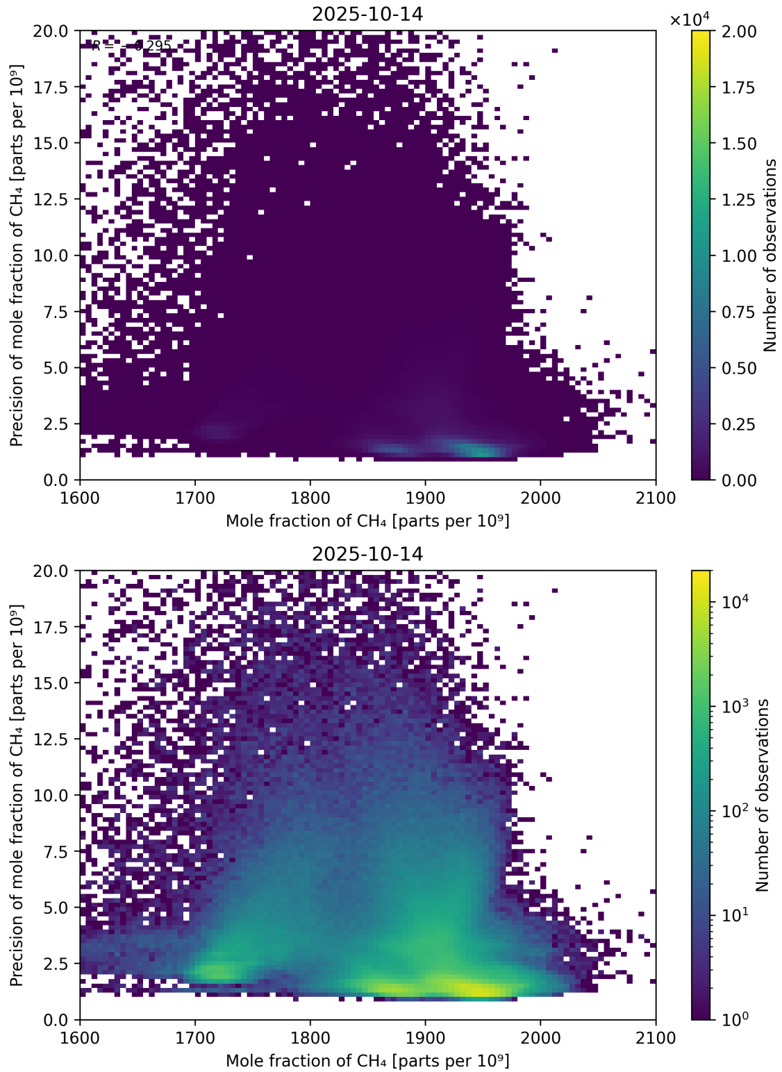
Figure 75: Scatter density plot of “Mole fraction of CH 4 ” against “Precision of mole fraction of CH 4 ” for 2025-10-13 to 2025-10-15.
