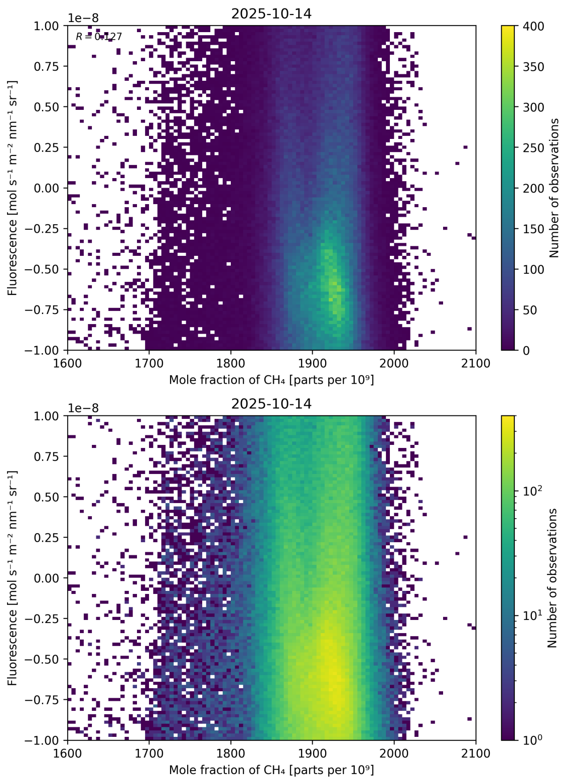
Figure 73: Scatter density plot of “Mole fraction of CH 4 ” against “Fluorescence” for 2025-10-13 to 2025-10-15.
