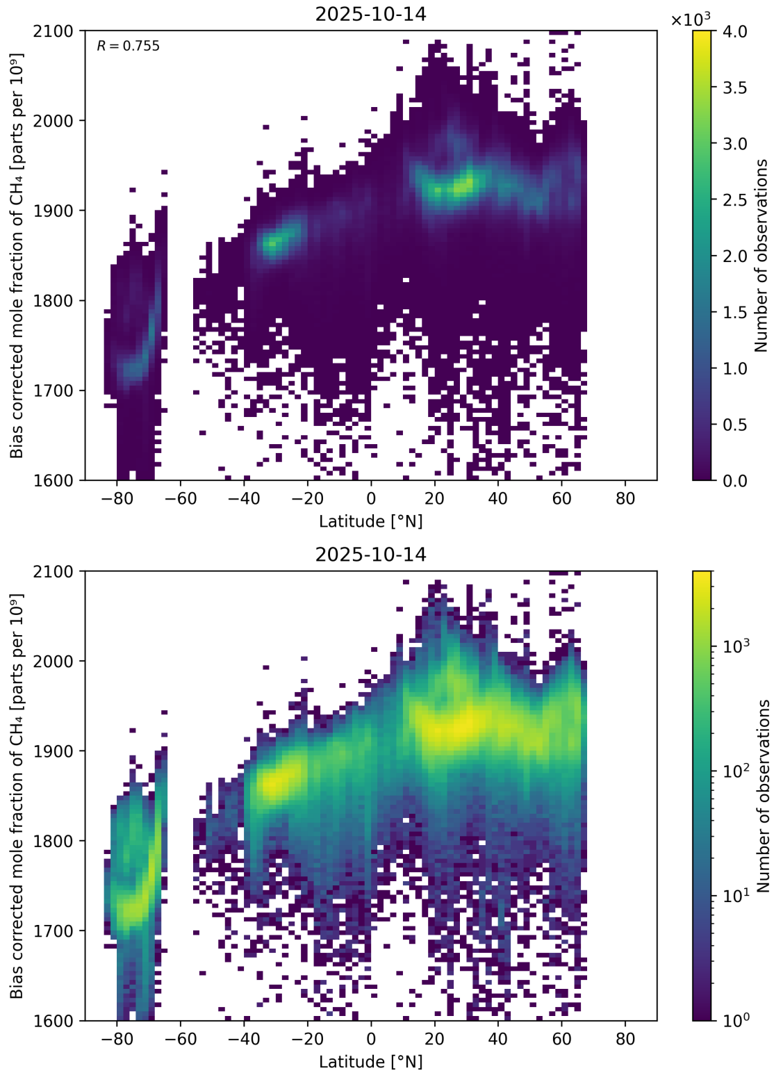
Figure 58: Scatter density plot of “Latitude” against “Bias corrected mole fraction of \text{CH}_4 ” for 2025-10-13 to 2025-10-15.
