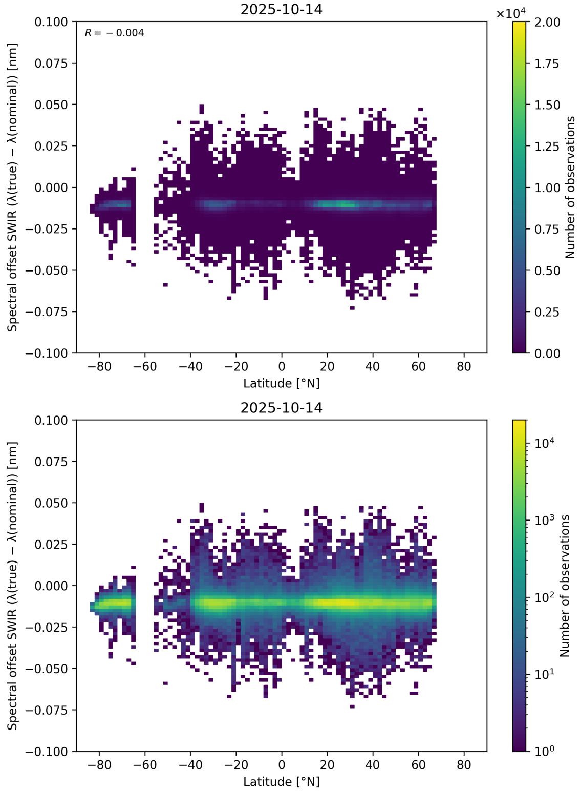
Figure 62: Scatter density plot of “Latitude” against “Spectral offset SWIR ( \lambda_{\text{true}} - \lambda_{\text{nominal}} )” for 2025-10-13 to 2025-10-15.
