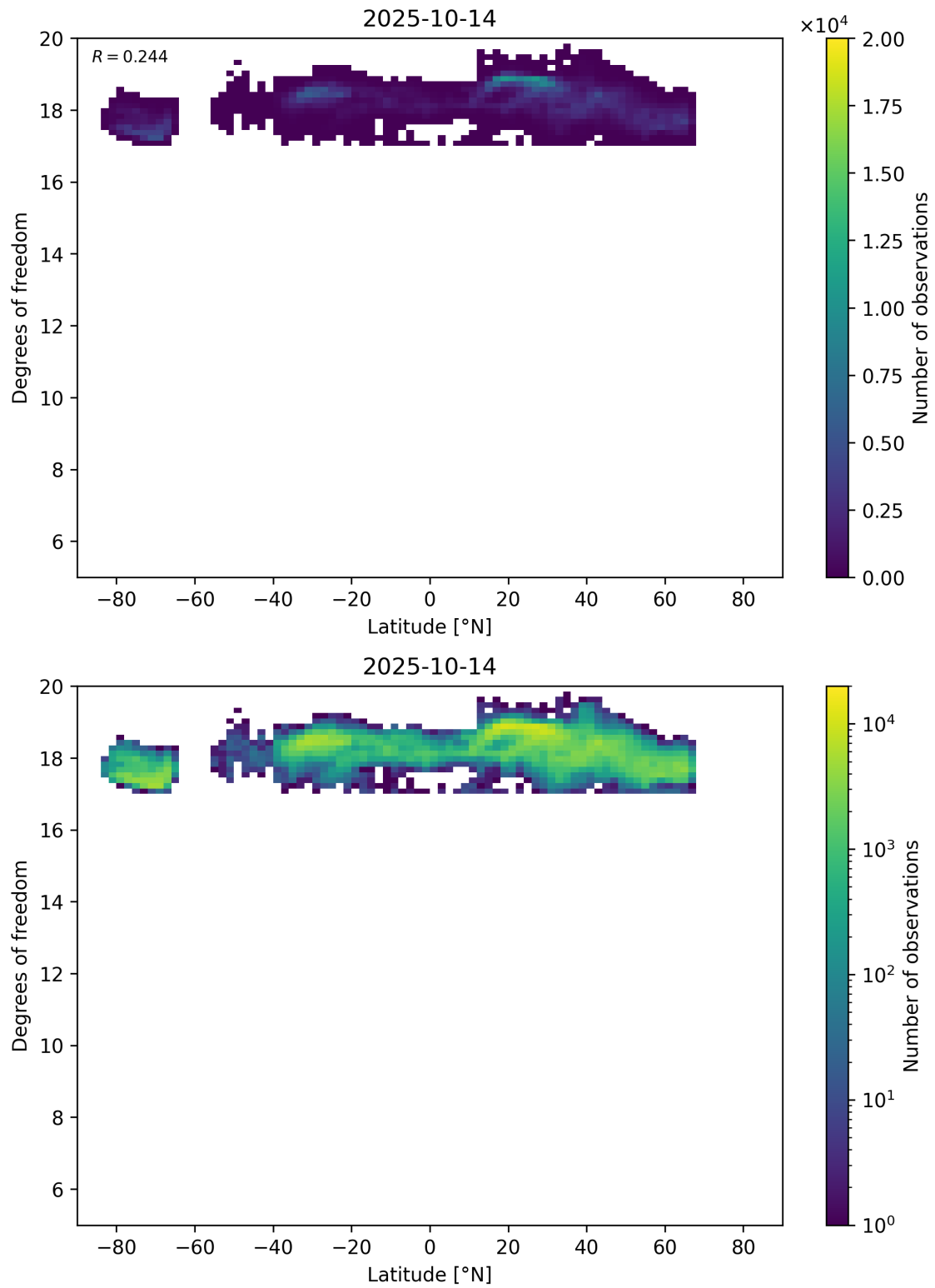
Figure 55: Scatter density plot of “Latitude” against “Degrees of freedom” for 2025-10-13 to 2025-10-15.
