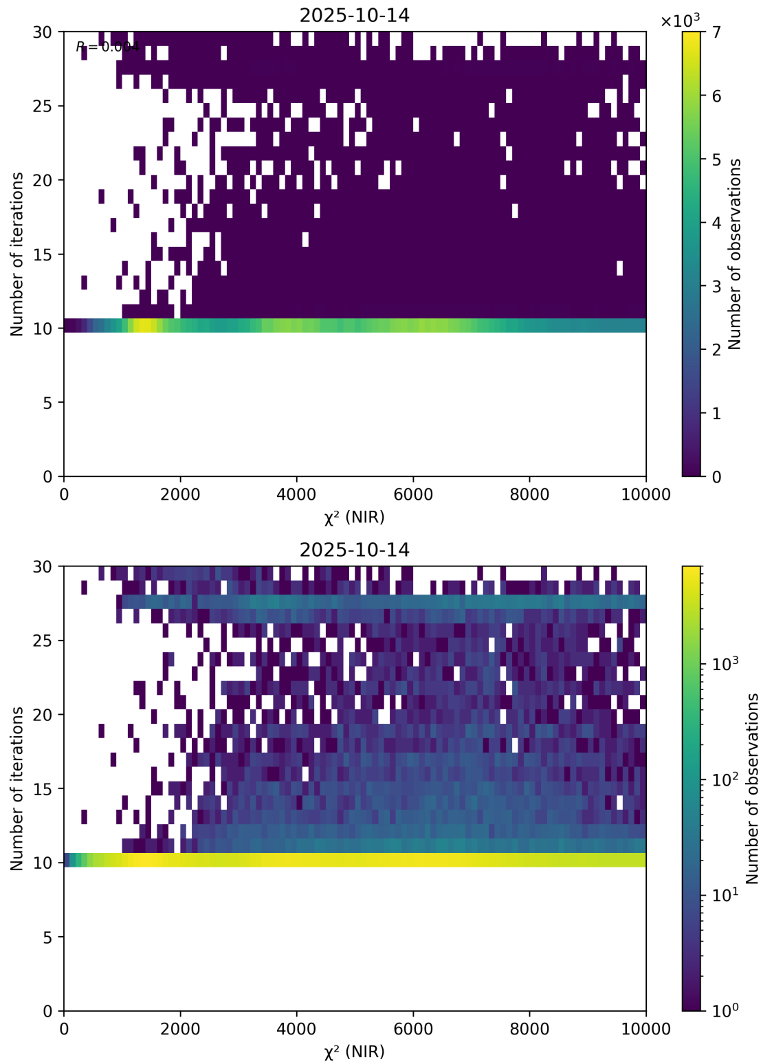
Figure 46: Scatter density plot of “ \chi^2 (NIR)” against “Number of iterations” for 2025-10-13 to 2025-10-15.
