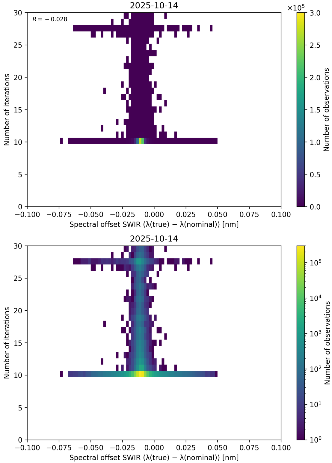
Figure 121: Scatter density plot of “Spectral offset SWIR ( \lambda_{\text{true}} - \lambda_{\text{nominal}} )” against “Number of iterations” for 2025-10-13 to 2025-10-15.
