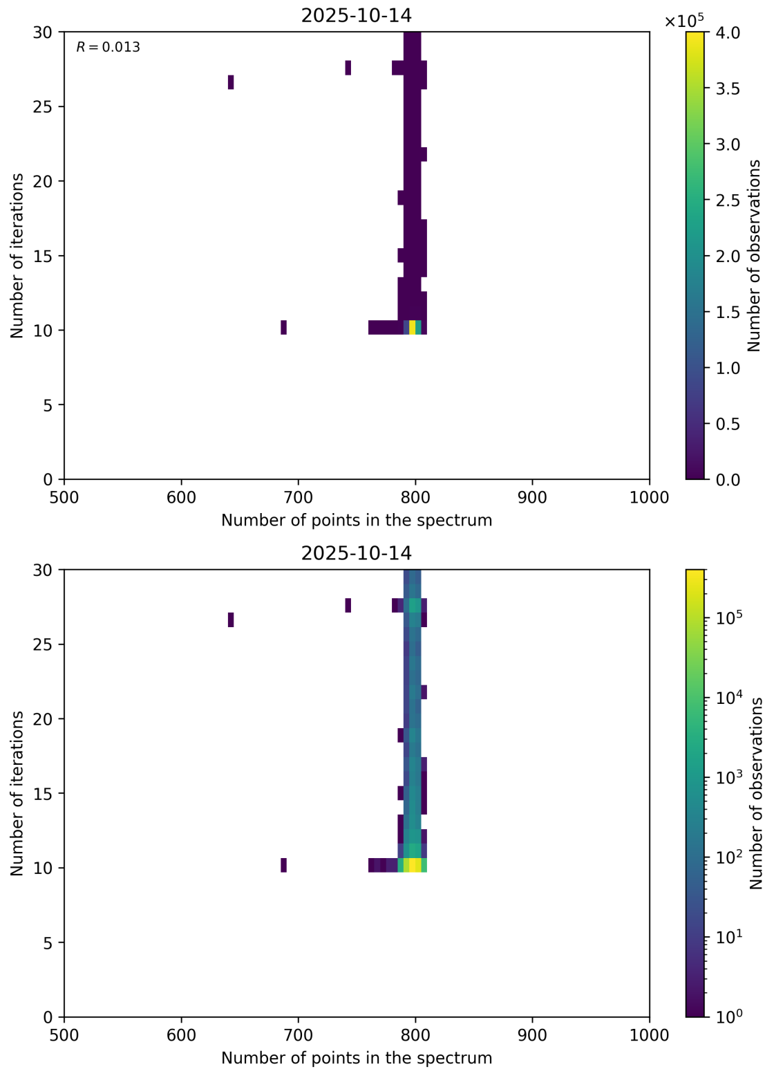
Figure 92: Scatter density plot of “Number of points in the spectrum” against “Number of iterations” for 2025-10-13 to 2025-10-15.
