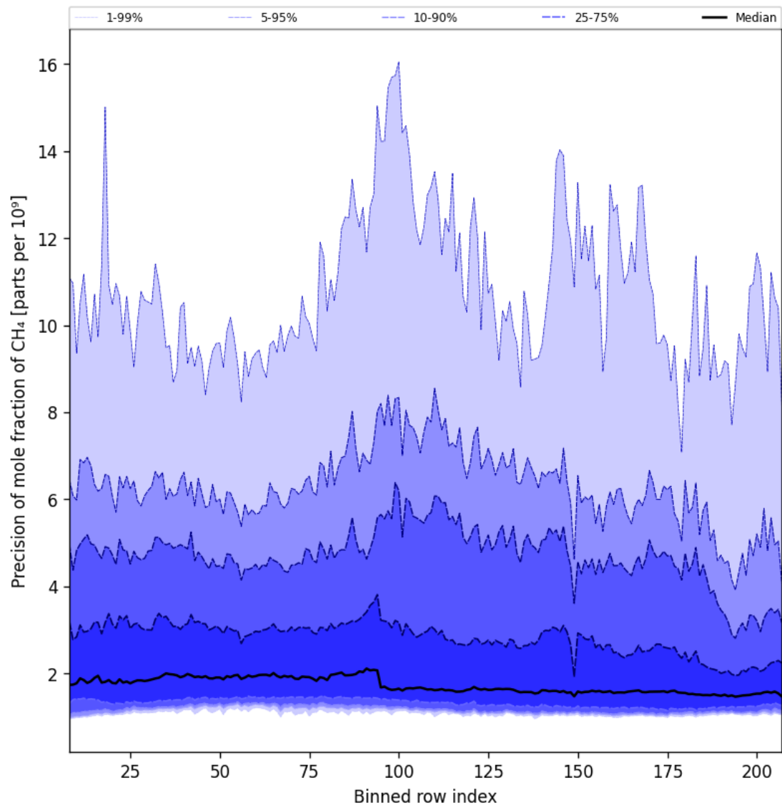
Figure 35: Along track statistics of “Precision of mole fraction of CH 4 ” for 2025-10-13 to 2025-10-15
