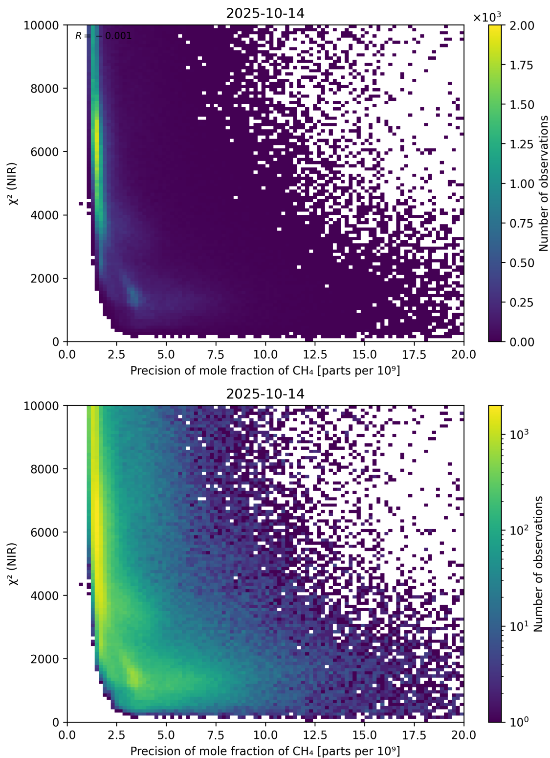
Figure 78: Scatter density plot of “Precision of mole fraction of \text{CH}_4 ” against “ \chi^2 (NIR)” for 2025-10-13 to 2025-10-15.
