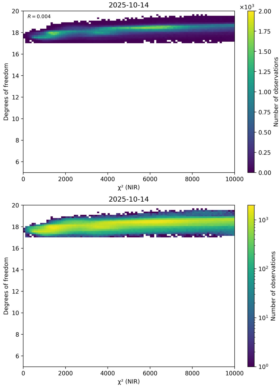
Figure 44: Scatter density plot of “ \chi^2 (NIR)” against “Degrees of freedom” for 2025-10-13 to 2025-10-15.
