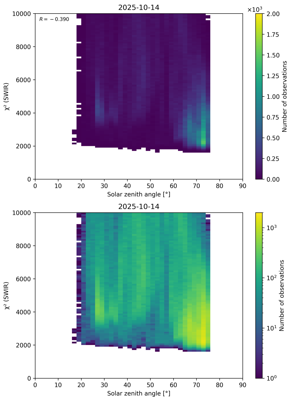
Figure 95: Scatter density plot of “Solar zenith angle” against “ \chi^2 (SWIR)” for 2025-10-13 to 2025-10-15.
