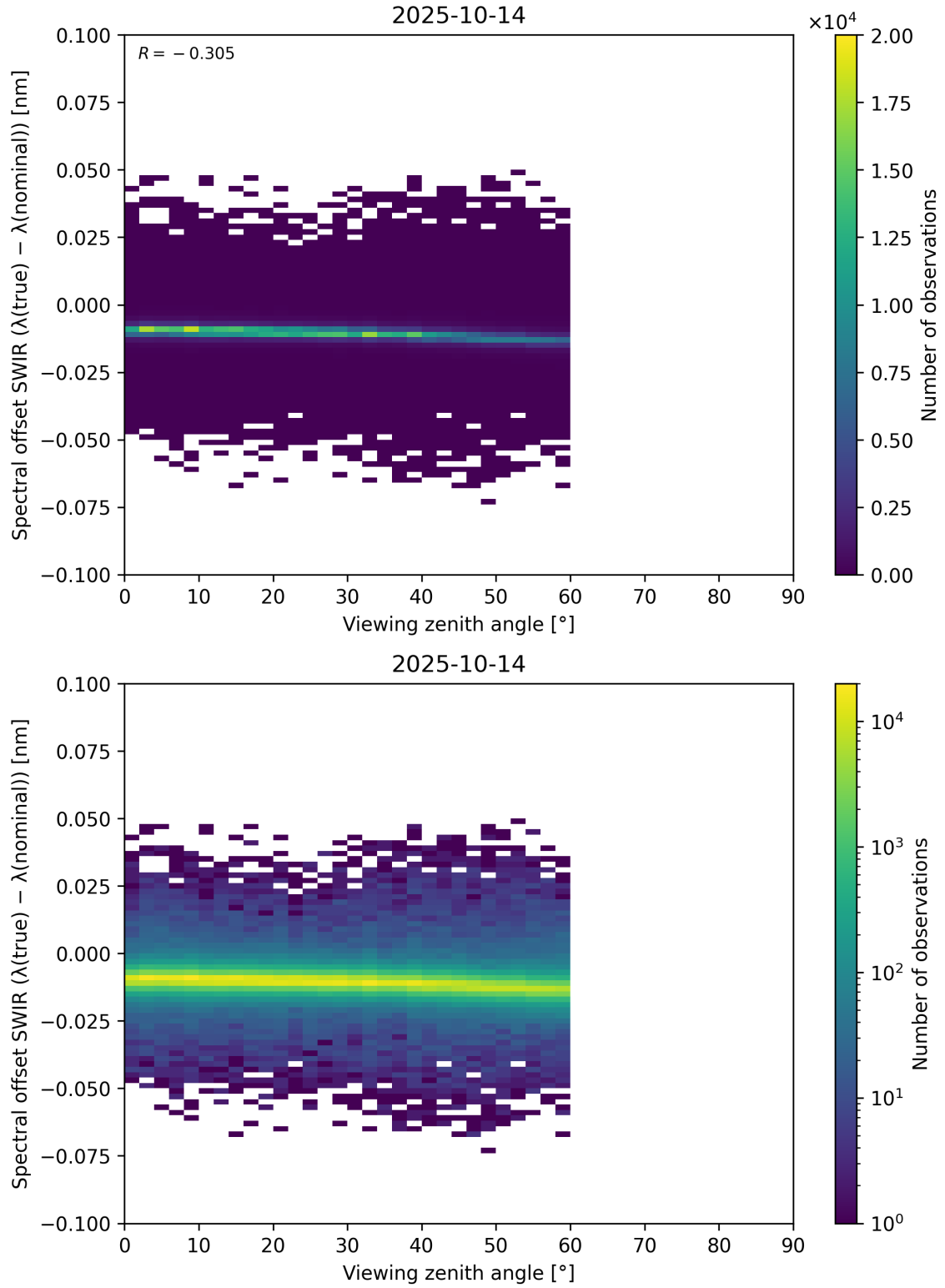
Figure 116: Scatter density plot of “Viewing zenith angle” against “Spectral offset SWIR ( \lambda_{\text{true}} - \lambda_{\text{nominal}} )” for 2025-10-13 to 2025-10-15.
