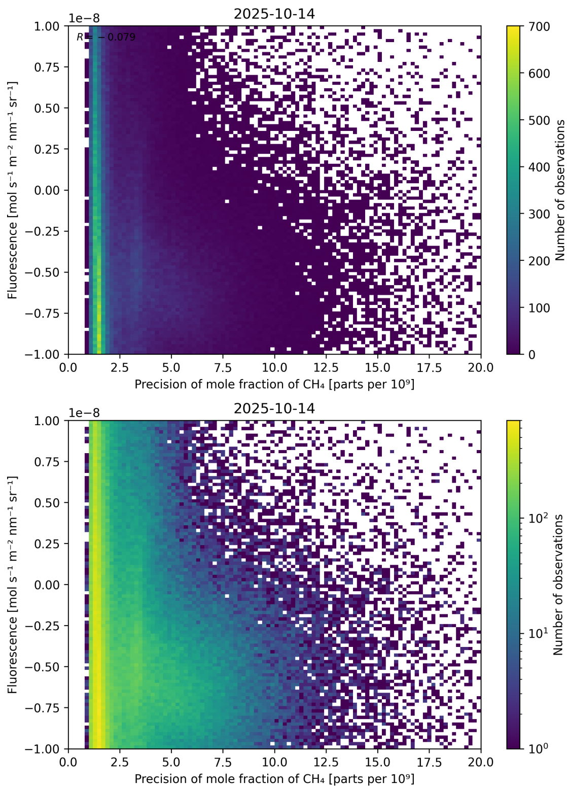
Figure 81: Scatter density plot of “Precision of mole fraction of CH 4 ” against “Fluorescence” for 2025-10-13 to 2025-10-15.
