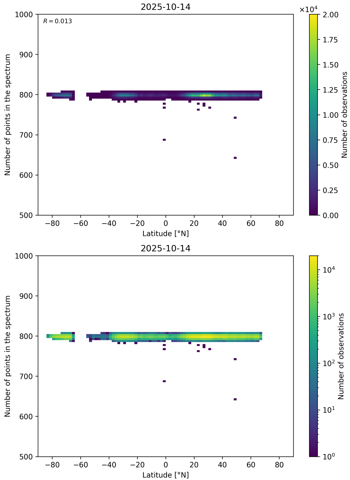
Figure 61: Scatter density plot of “Latitude” against “Number of points in the spectrum” for 2025-10-13 to 2025-10-15.
