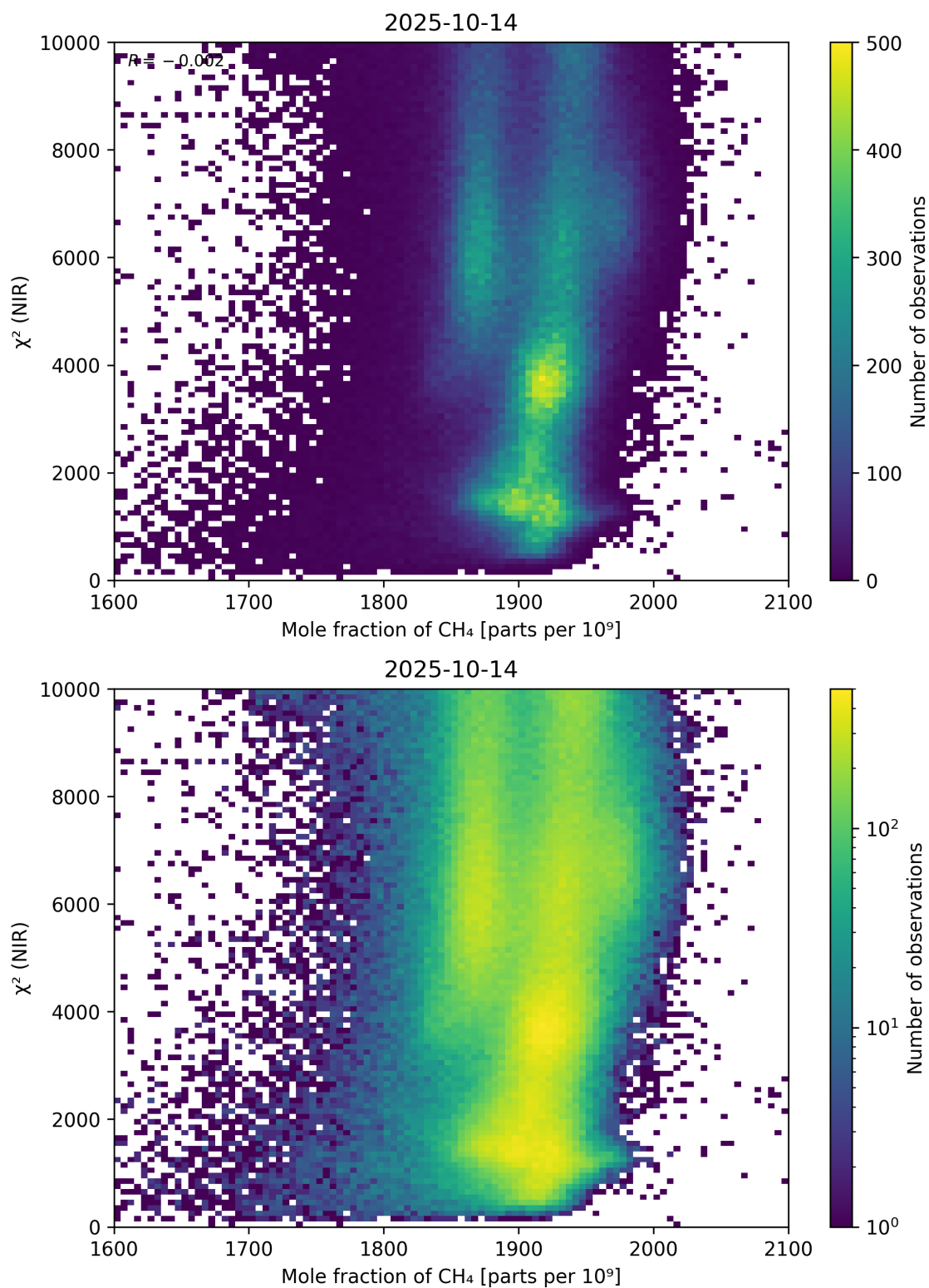
Figure 70: Scatter density plot of “Mole fraction of \text{CH}_4 ” against “ \chi^2 (NIR)” for 2025-10-13 to 2025-10-15.
