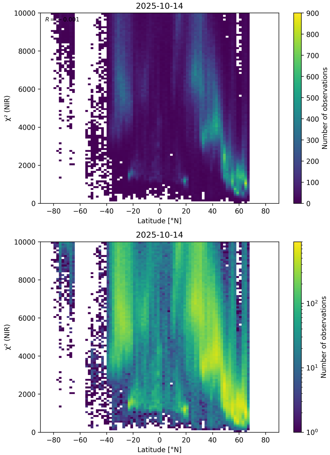
Figure 53: Scatter density plot of “Latitude” against “ \chi^2 (NIR)” for 2025-10-13 to 2025-10-15.
