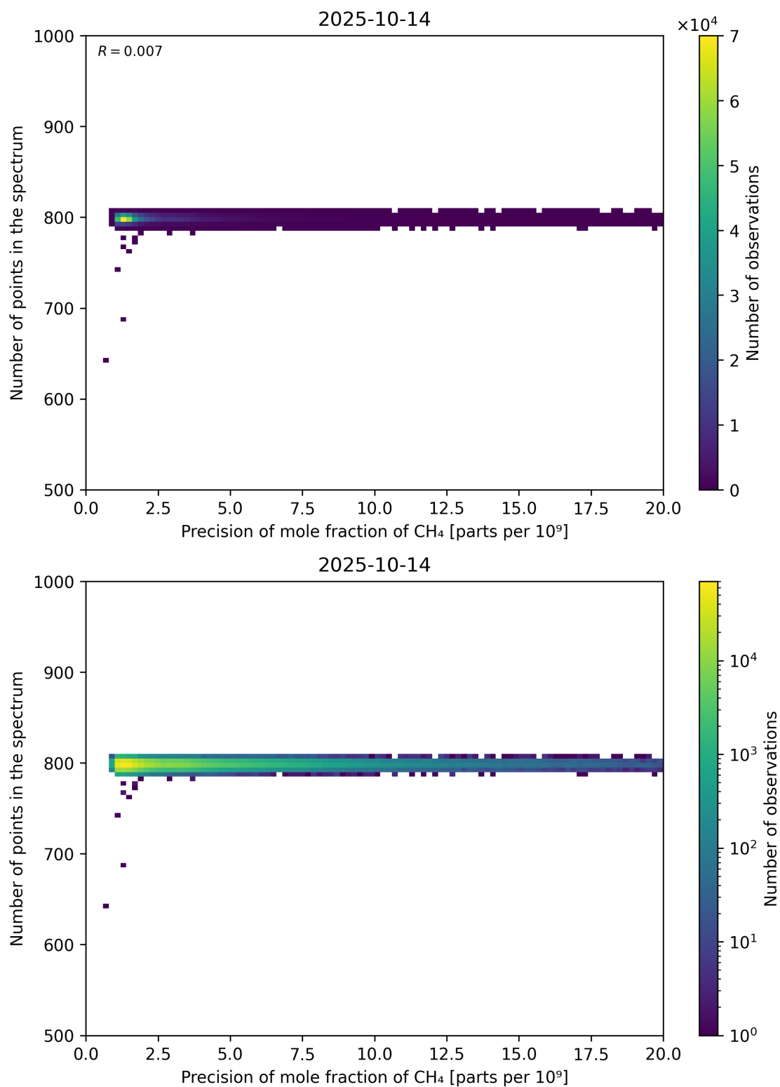
Figure 84: Scatter density plot of “Precision of mole fraction of CH 4 ” against “Number of points in the spectrum” for 2025-10-13 to 2025-10-15.
