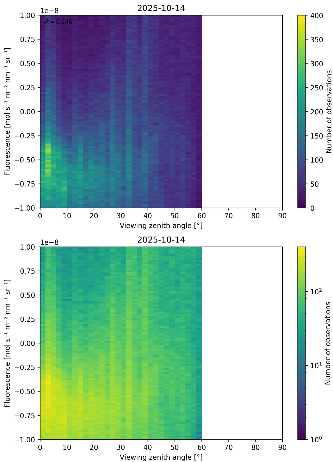
Figure 108: Scatter density plot of “Viewing zenith angle” against “Fluorescence” for 2025-10-13 to 2025-10-15.
