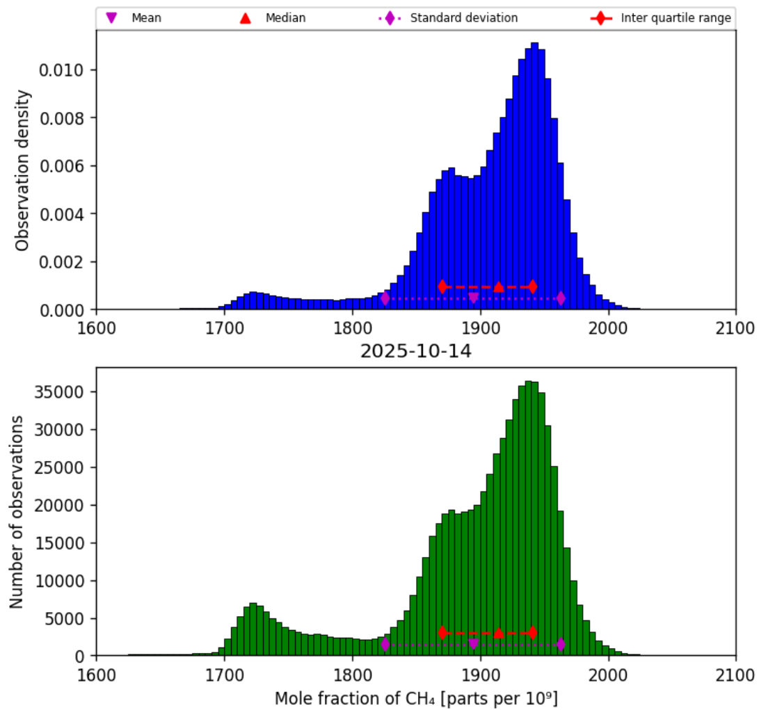
Figure 23: Histogram of “Mole fraction of CH 4 ” for 2025-10-13 to 2025-10-15
