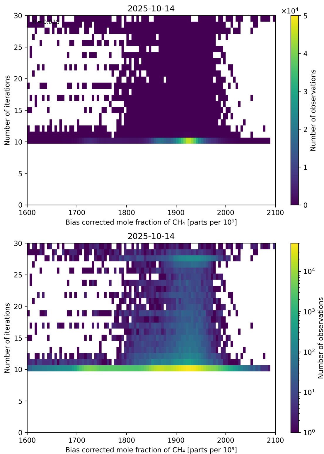
Figure 67: Scatter density plot of “Bias corrected mole fraction of \text{CH}_4 ” against “Number of iterations” for 2025-10-13 to 2025-10-15.
