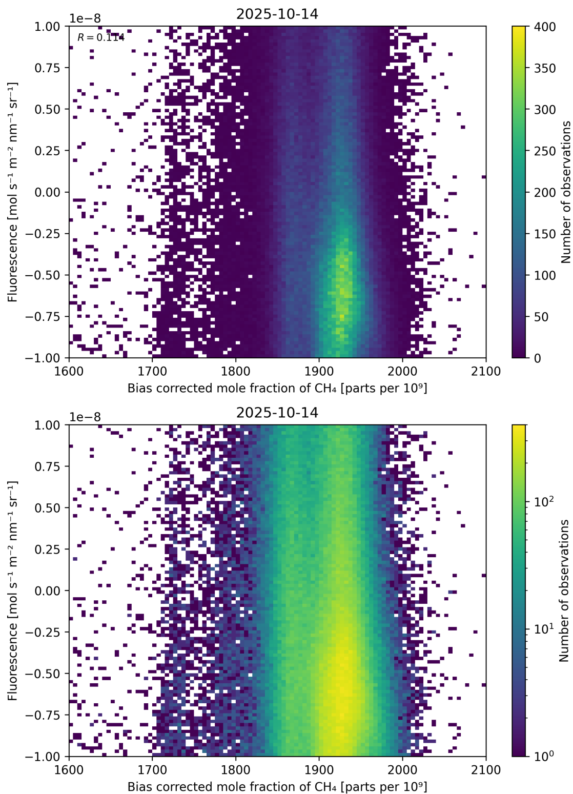
Figure 66: Scatter density plot of “Bias corrected mole fraction of \text{CH}_4 ” against “Fluorescence” for 2025-10-13 to 2025-10-15.
