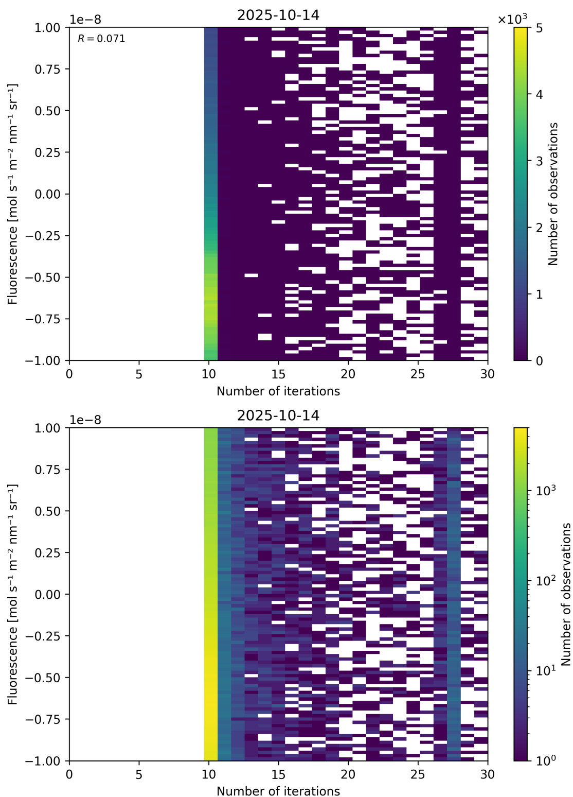
Figure 87: Scatter density plot of “Number of iterations” against “Fluorescence” for 2025-10-13 to 2025-10-15.
