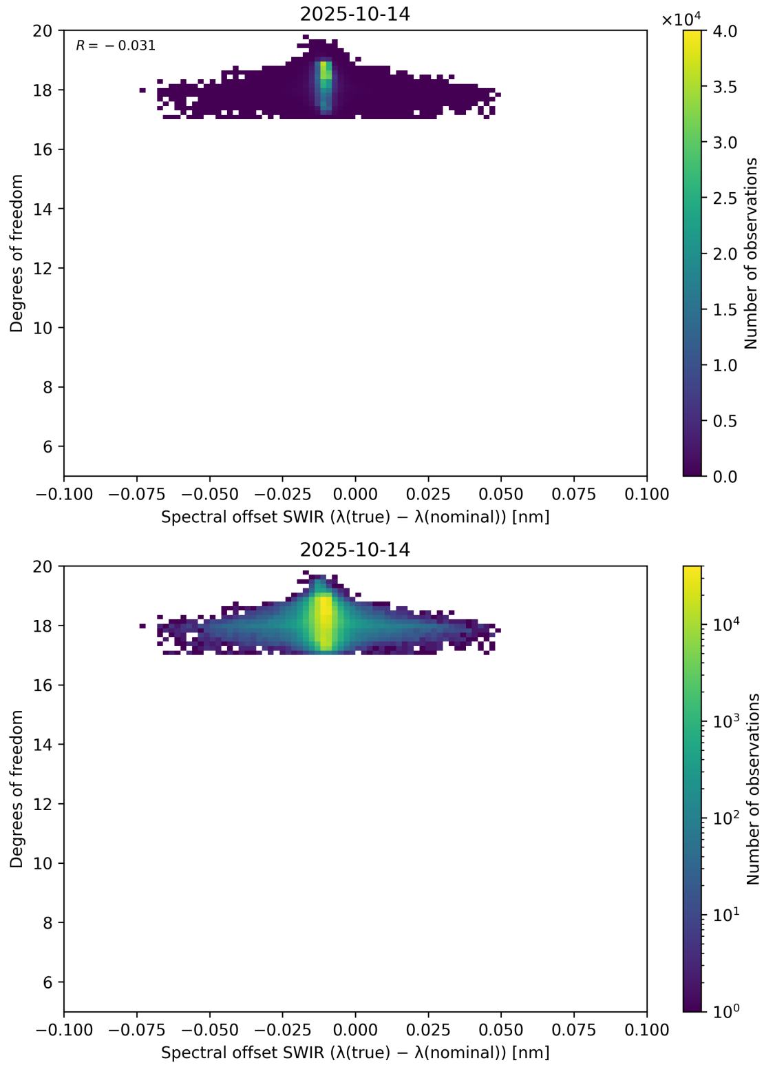
Figure 119: Scatter density plot of “Spectral offset SWIR ( \lambda_{\text{true}} - \lambda_{\text{nominal}} )” against “Degrees of freedom” for 2025-10-13 to 2025-10-15.
