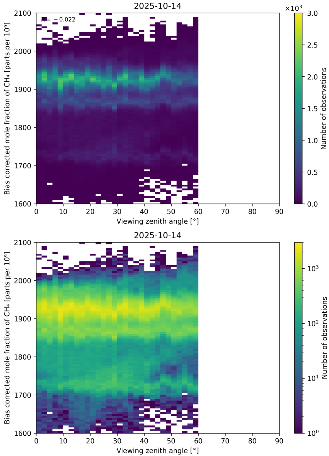
Figure 111: Scatter density plot of “Viewing zenith angle” against “Bias corrected mole fraction of CH 4 ” for 2025-10-13 to 2025-10-15.
