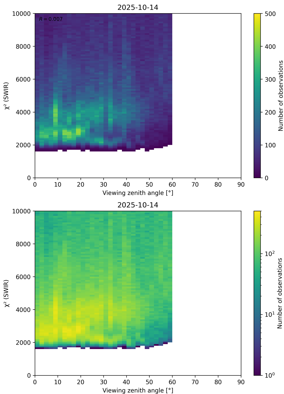
Figure 106: Scatter density plot of “Viewing zenith angle” against “ \chi^2 (SWIR)” for 2025-10-13 to 2025-10-15.
