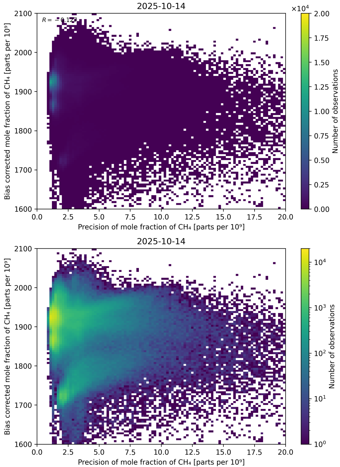
Figure 82: Scatter density plot of “Precision of mole fraction of CH 4 ” against “Bias corrected mole fraction of CH 4 ” for 2025-10-13 to 2025-10-15.
