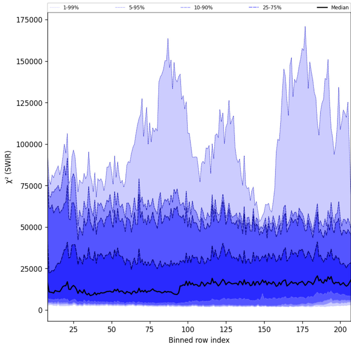
Figure 39: Along track statistics of “ \chi^2 (SWIR)” for 2025-10-13 to 2025-10-15
