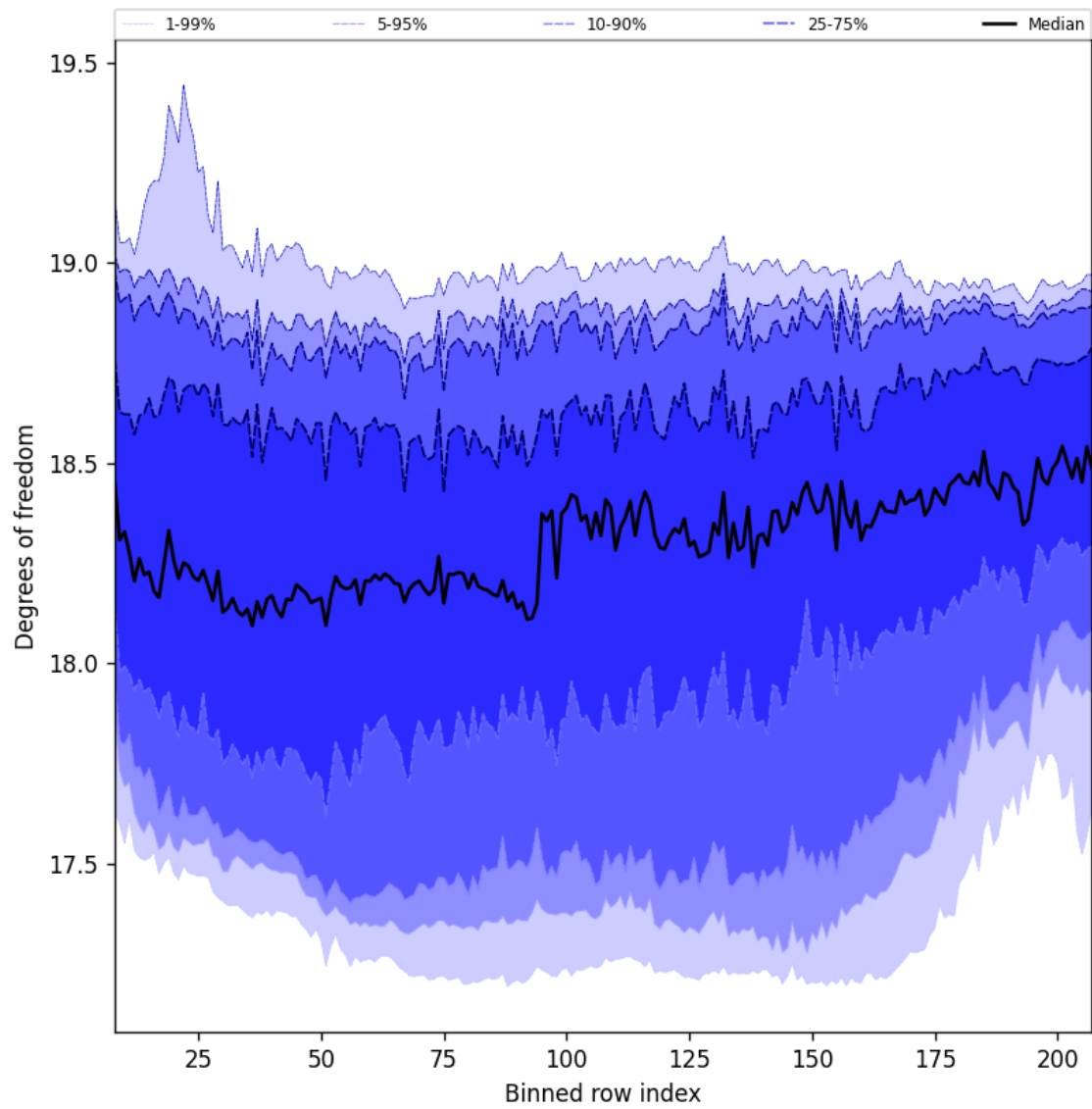
Figure 41: Along track statistics of “Degrees of freedom” for 2025-10-13 to 2025-10-15
