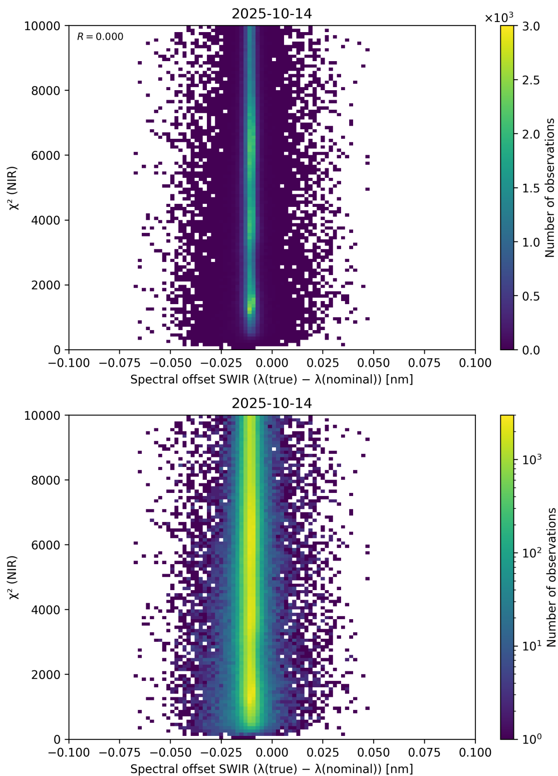
Figure 117: Scatter density plot of “Spectral offset SWIR ( \lambda_{\text{true}} - \lambda_{\text{nominal}} )” against “ \chi^2 (NIR)” for 2025-10-13 to 2025-10-15.
