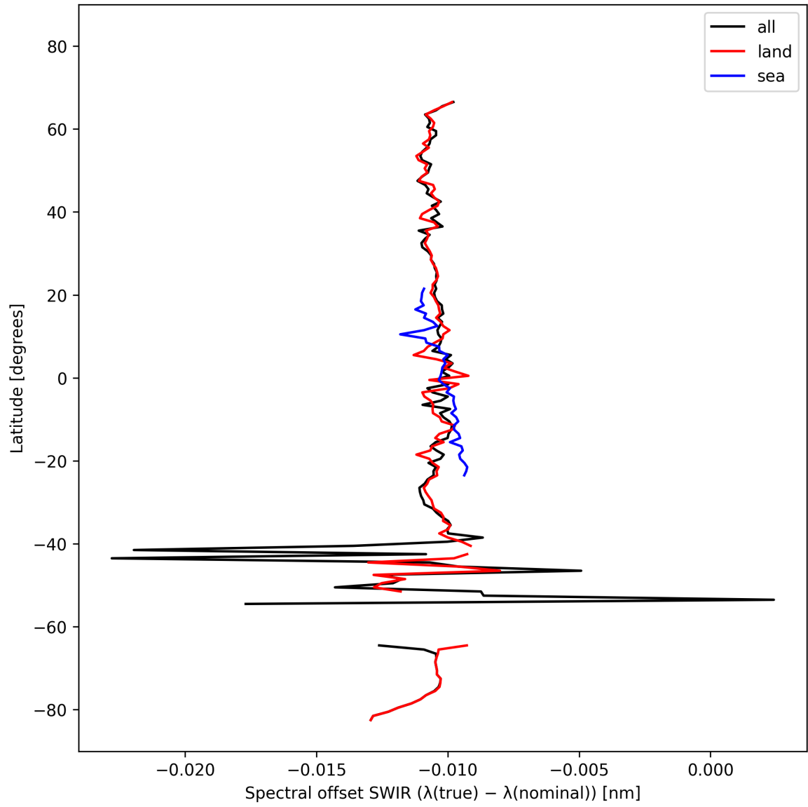
Figure 16: Zonal average of “Spectral offset SWIR ( \lambda_{\text{true}} - \lambda_{\text{nominal}} )” for 2025-10-13 to 2025-10-15.
