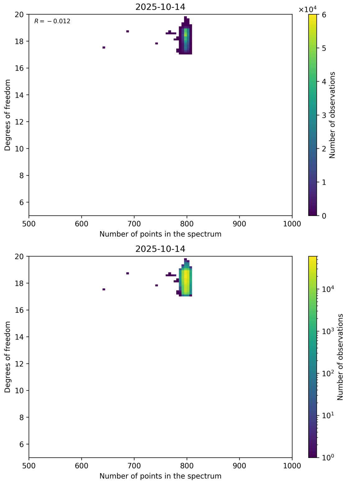
Figure 90: Scatter density plot of “Number of points in the spectrum” against “Degrees of freedom” for 2025-10-13 to 2025-10-15.
