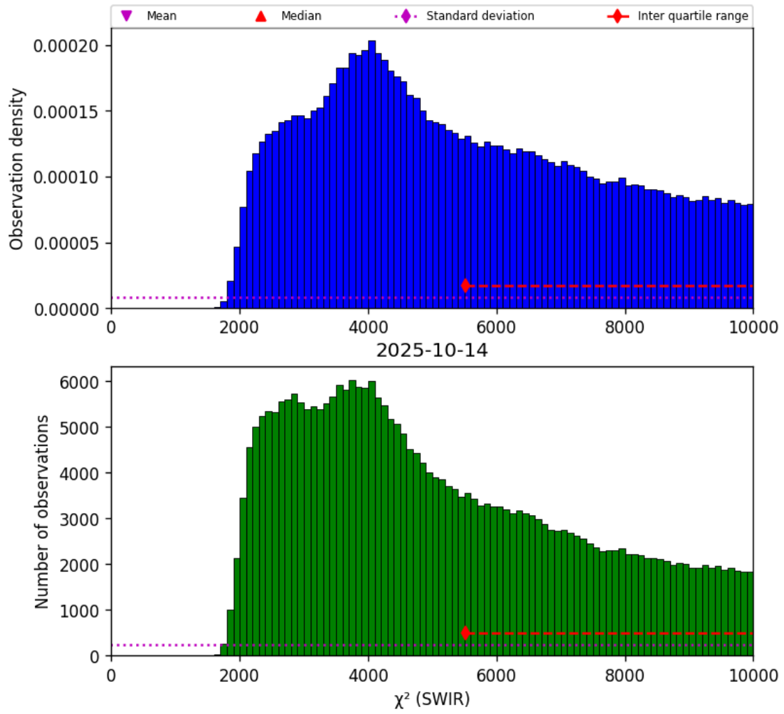
Figure 28: Histogram of “ \chi^2 (SWIR)” for 2025-10-13 to 2025-10-15
