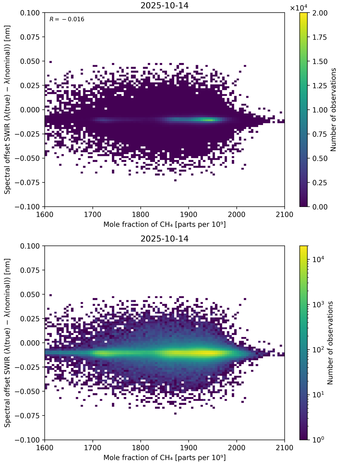
Figure 86: Scatter density plot of “Mole fraction of CH 4 ” against “Spectral offset SWIR ( \lambda_{\text{true}} - \lambda_{\text{nominal}} )” for 2025-10-13 to 2025-10-15.
