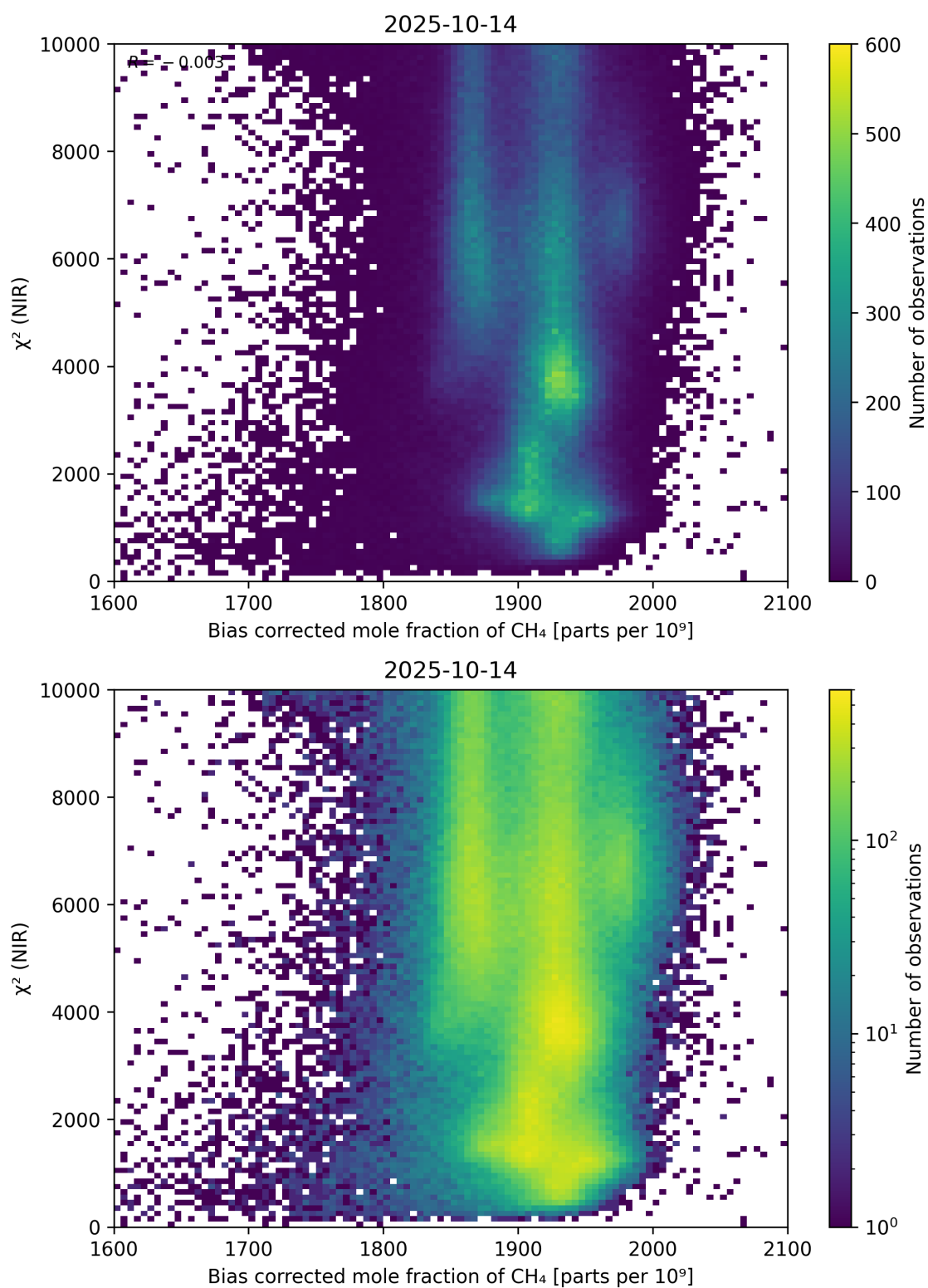
Figure 63: Scatter density plot of “Bias corrected mole fraction of \text{CH}_4 ” against “ \chi^2 (NIR)” for 2025-10-13 to 2025-10-15.
