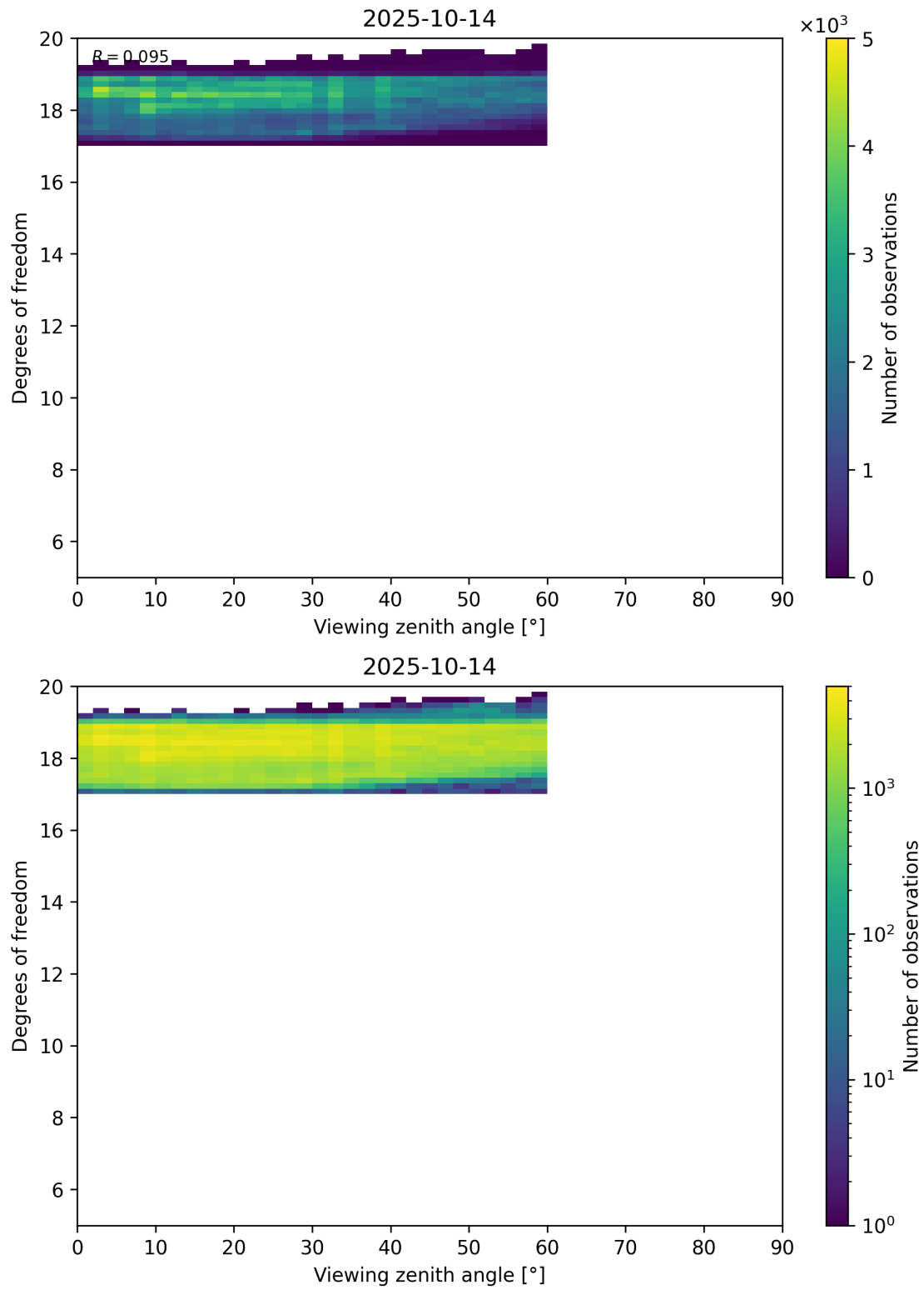
Figure 107: Scatter density plot of “Viewing zenith angle” against “Degrees of freedom” for 2025-10-13 to 2025-10-15.
