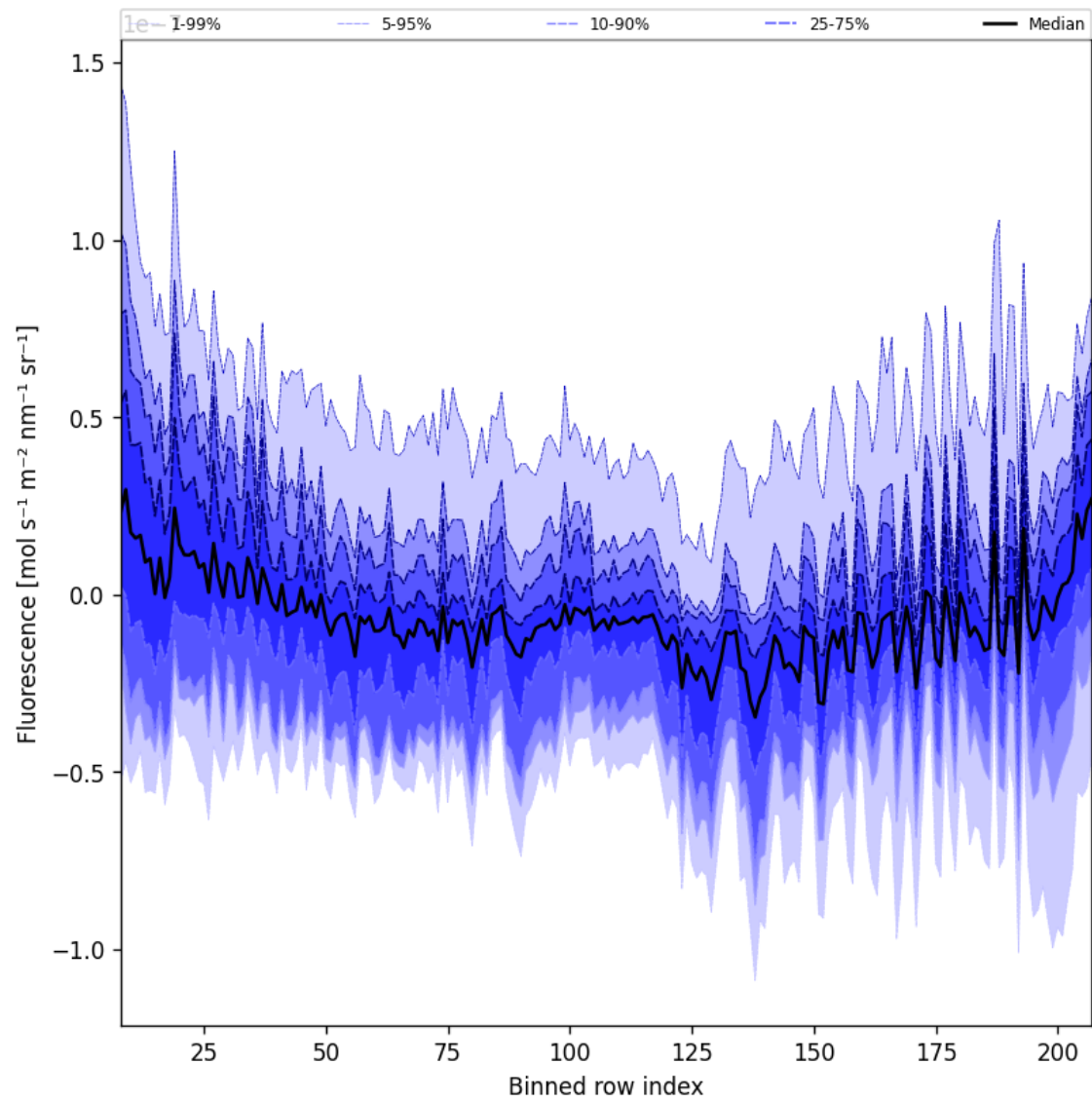
Figure 43: Along track statistics of "Fluorescence" for 2025-10-13 to 2025-10-15
