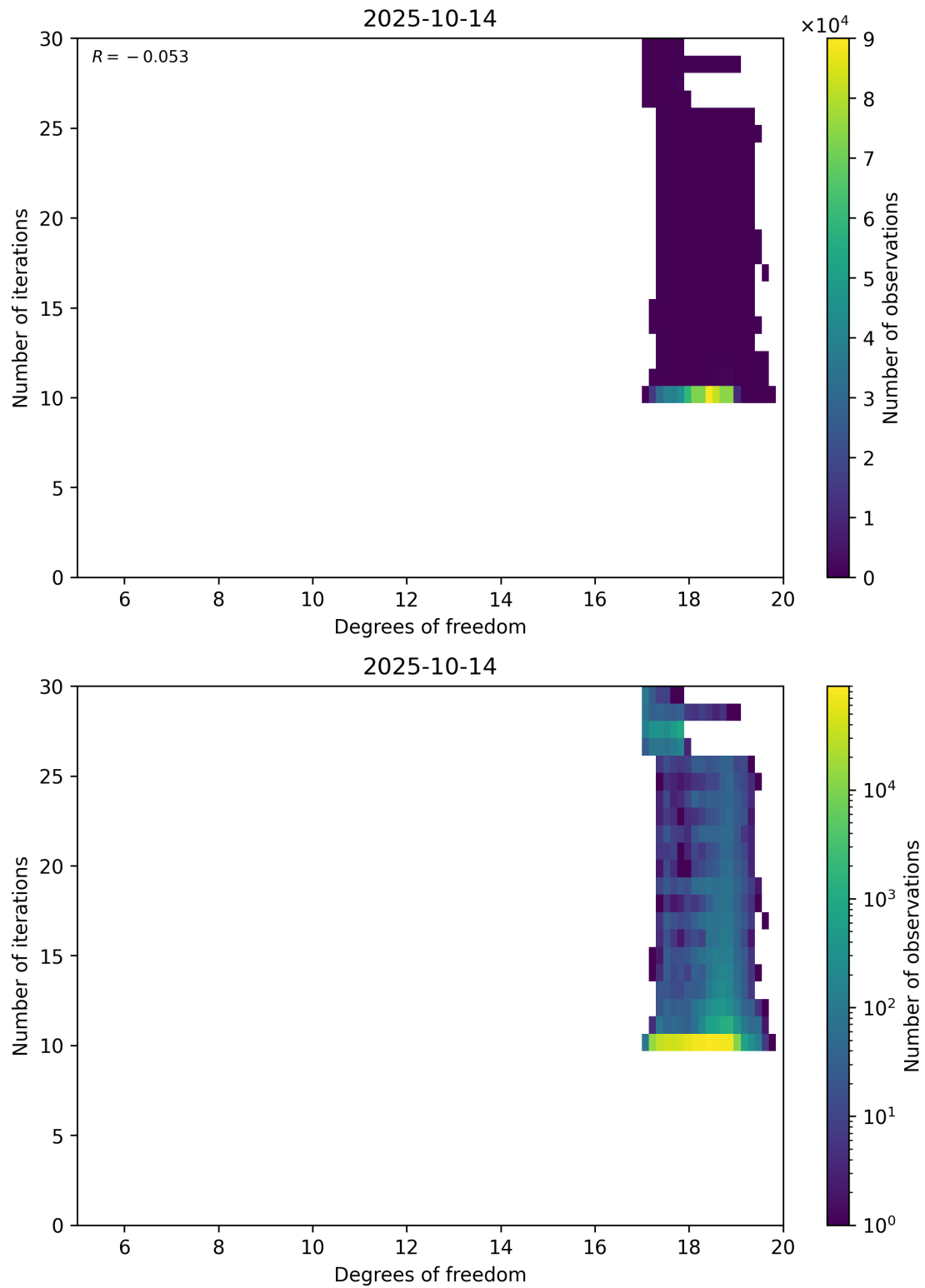
Figure 52: Scatter density plot of “Degrees of freedom” against “Number of iterations” for 2025-10-13 to 2025-10-15.
