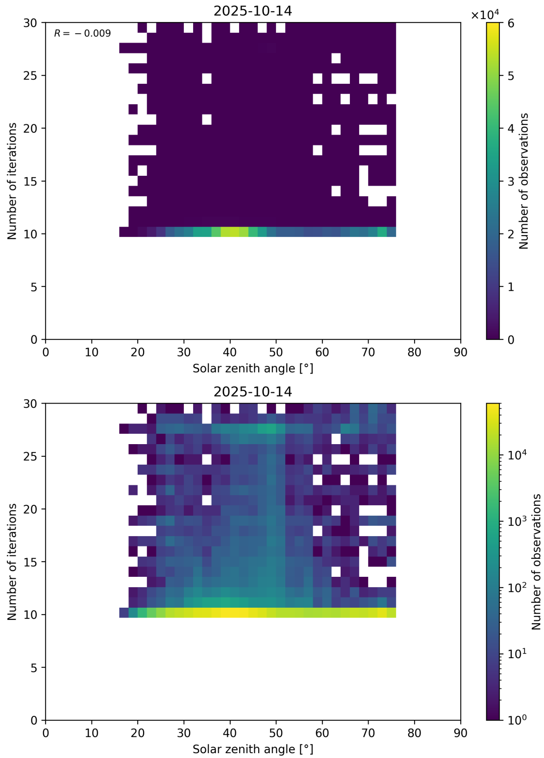
Figure 102: Scatter density plot of “Solar zenith angle” against “Number of iterations” for 2025-10-13 to 2025-10-15.
