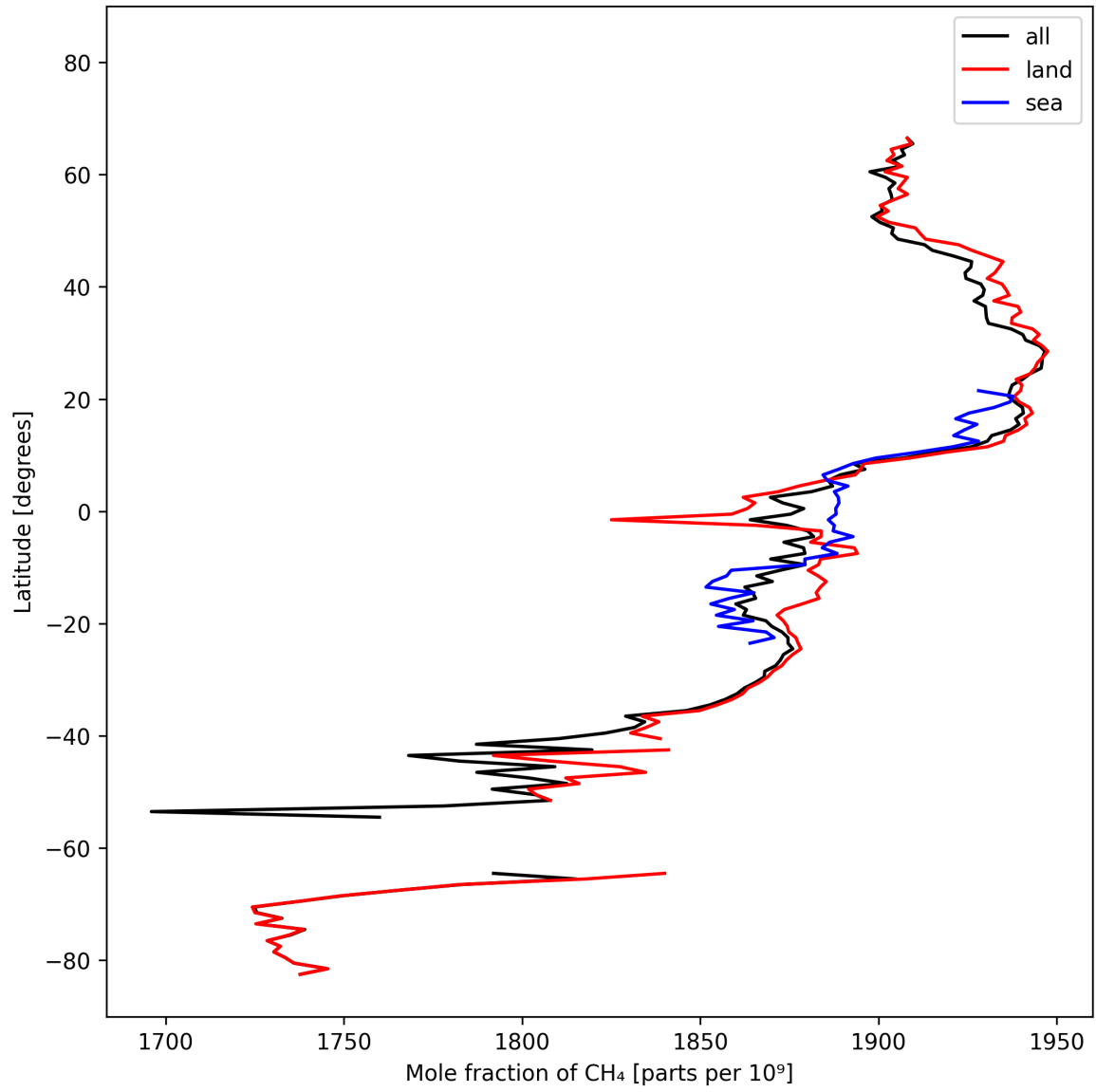
Figure 12: Zonal average of “Mole fraction of CH 4 ” for 2025-10-13 to 2025-10-15.
