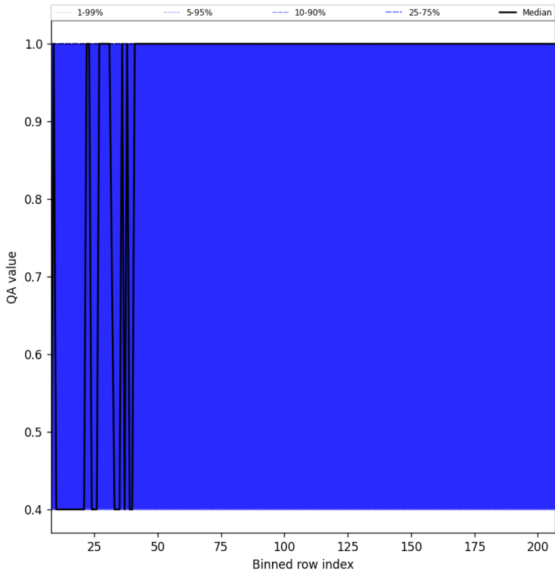
Figure 33: Along track statistics of “QA value” for 2025-10-13 to 2025-10-15
