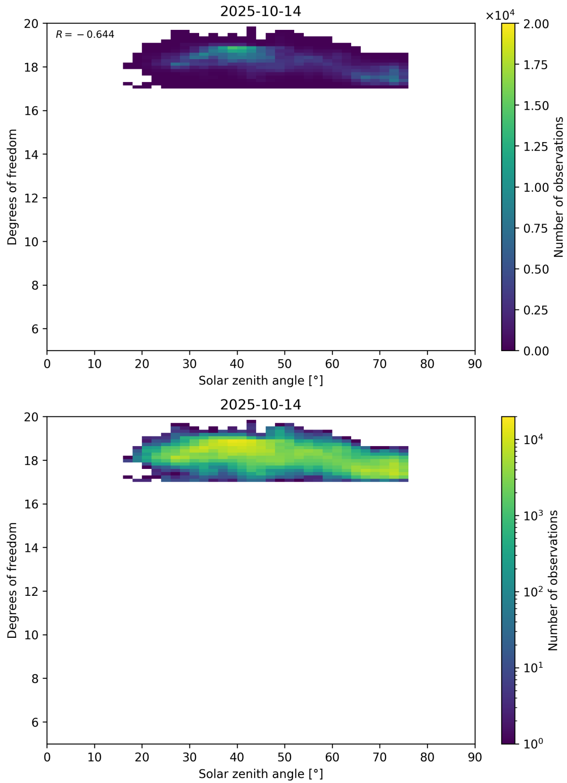
Figure 96: Scatter density plot of “Solar zenith angle” against “Degrees of freedom” for 2025-10-13 to 2025-10-15.
