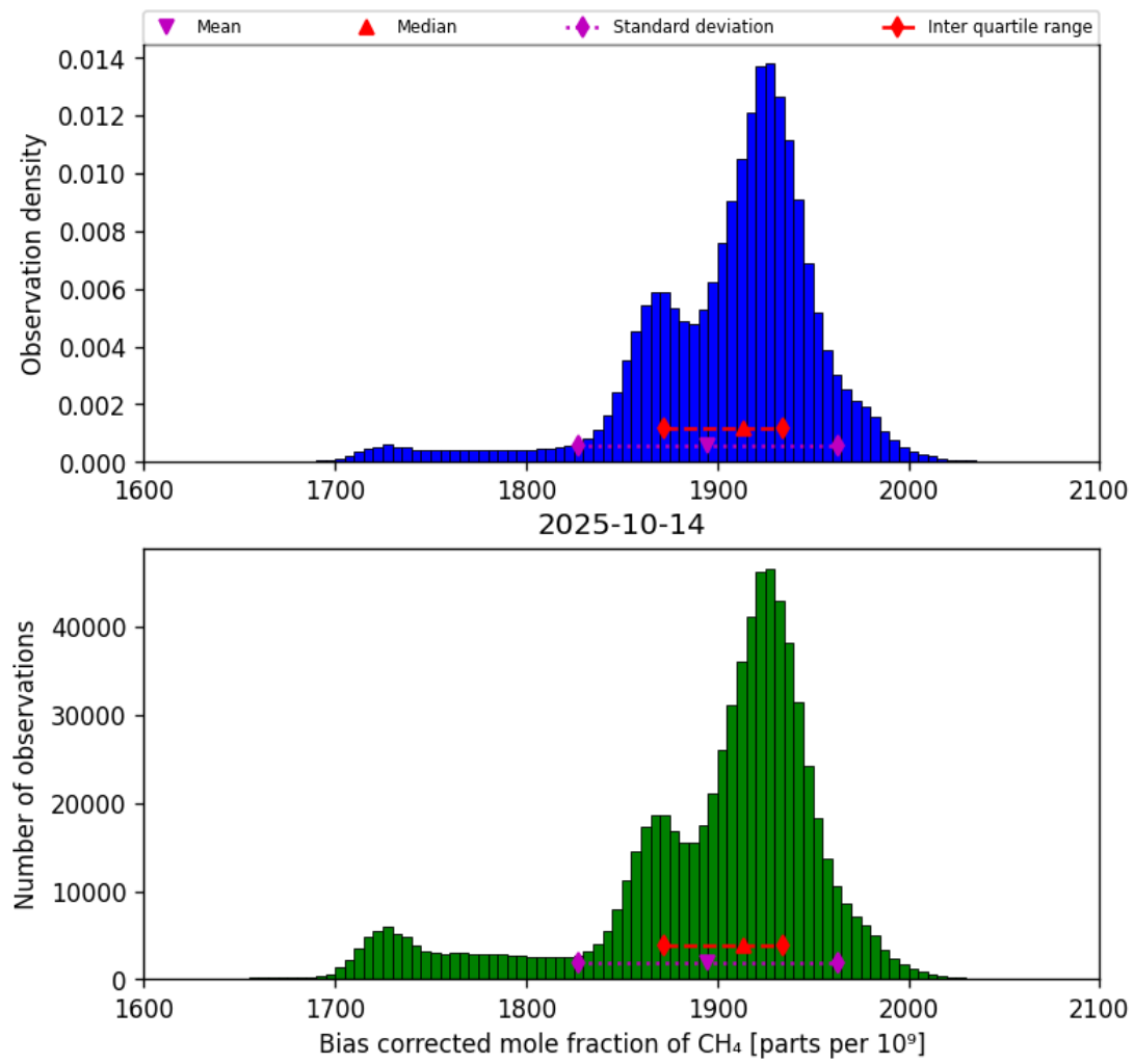
Figure 25: Histogram of “Bias corrected mole fraction of CH 4 ” for 2025-10-13 to 2025-10-15
