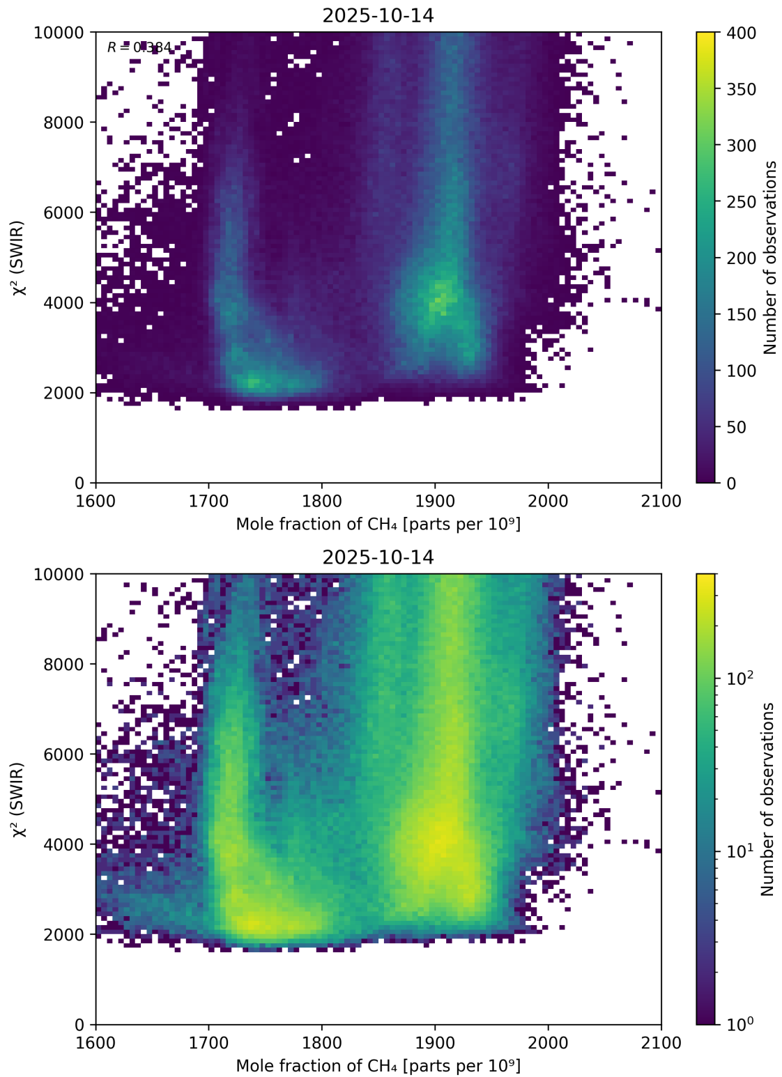
Figure 71: Scatter density plot of “Mole fraction of \text{CH}_4 ” against “ \chi^2 (SWIR)” for 2025-10-13 to 2025-10-15.
