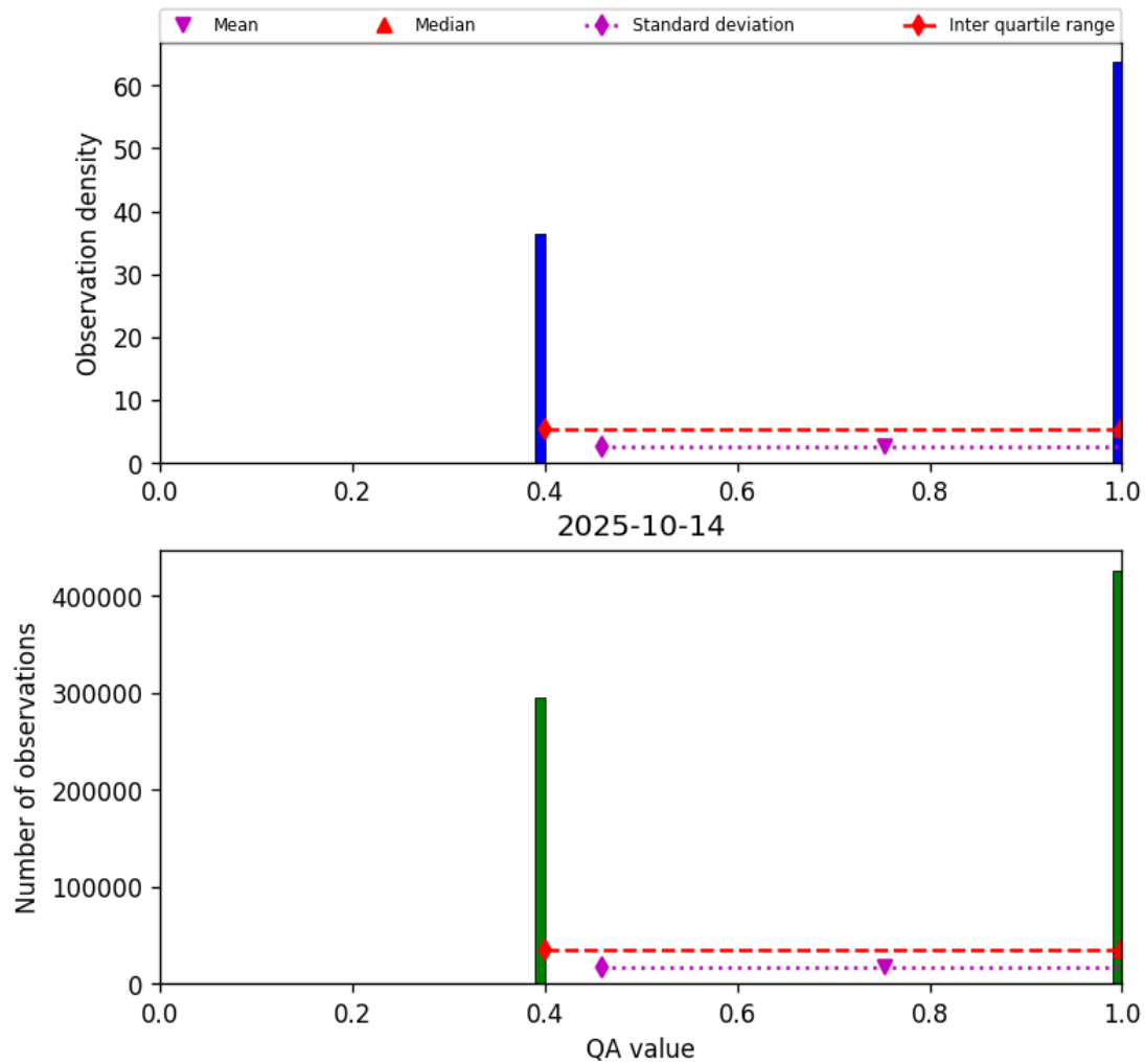
Figure 22: Histogram of “QA value” for 2025-10-13 to 2025-10-15
