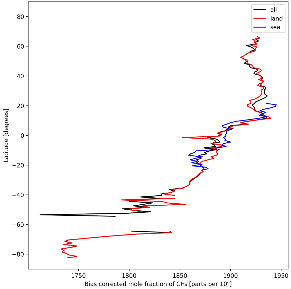
Figure 14: Zonal average of “Bias corrected mole fraction of CH 4 ” for 2025-10-13 to 2025-10-15.
