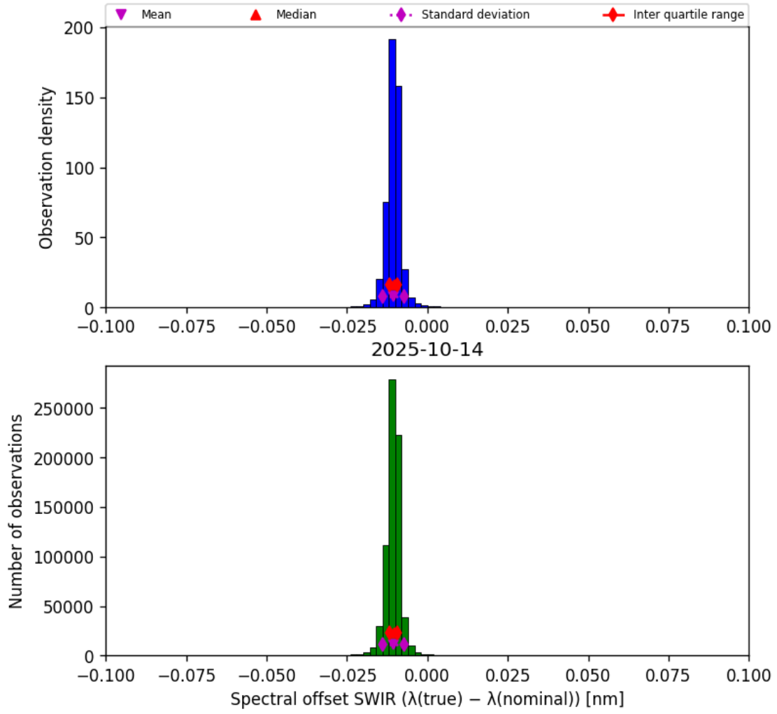
Figure 27: Histogram of “Spectral offset SWIR ( \lambda_{\text{true}} - \lambda_{\text{nominal}} )” for 2025-10-13 to 2025-10-15
