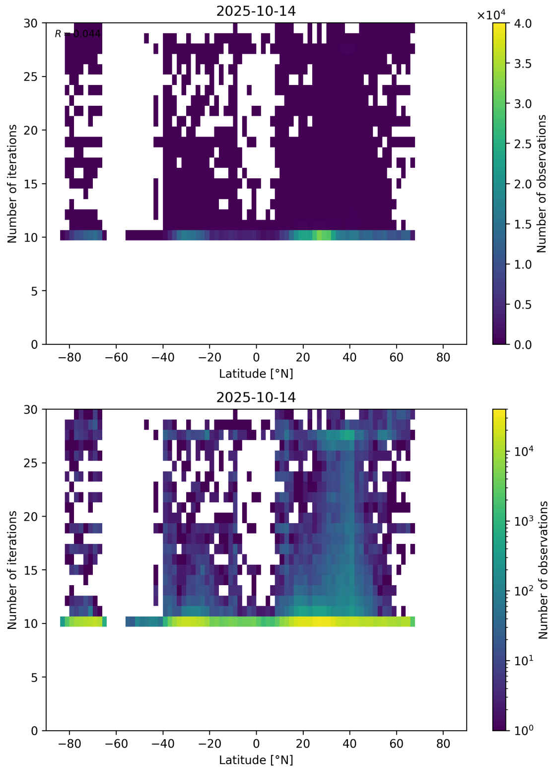
Figure 60: Scatter density plot of “Latitude” against “Number of iterations” for 2025-10-13 to 2025-10-15.
