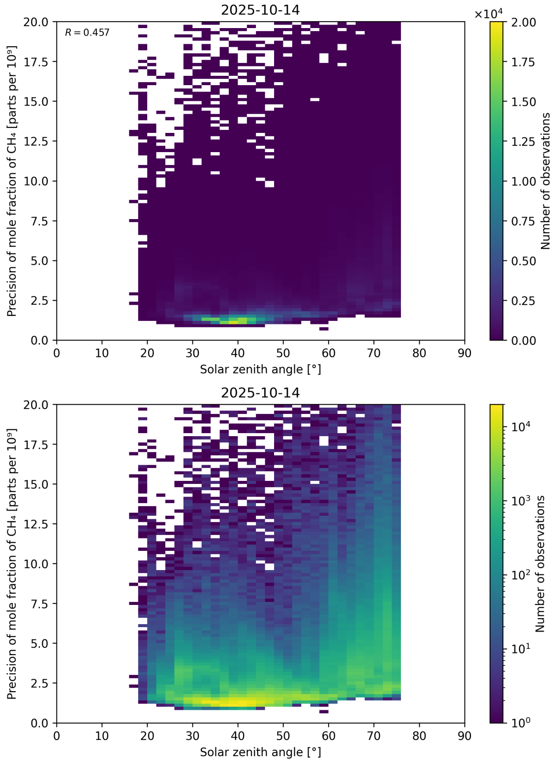
Figure 101: Scatter density plot of “Solar zenith angle” against “Precision of mole fraction of \text{CH}_4 ” for 2025-10-13 to 2025-10-15.
