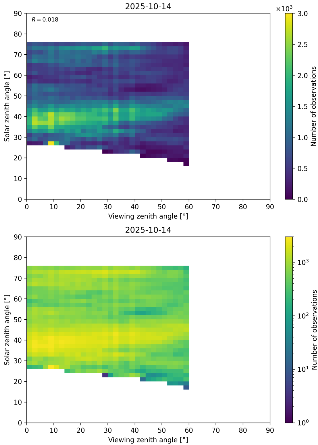
Figure 115: Scatter density plot of “Viewing zenith angle” against “Solar zenith angle” for 2025-10-13 to 2025-10-15.
