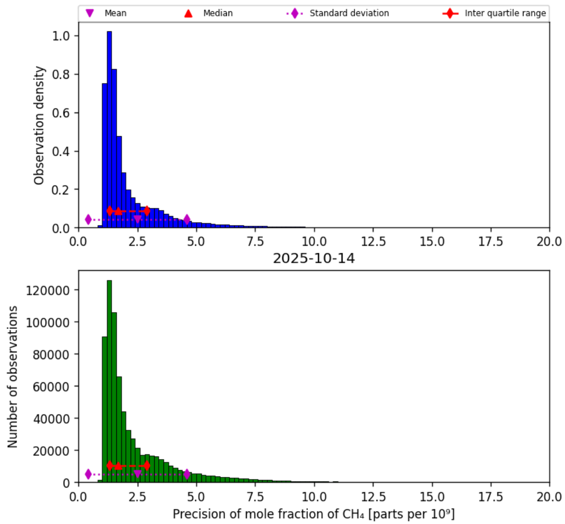
Figure 24: Histogram of “Precision of mole fraction of CH 4 ” for 2025-10-13 to 2025-10-15
