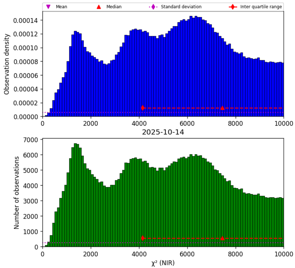
Figure 29: Histogram of “ \chi^2 (NIR)” for 2025-10-13 to 2025-10-15
