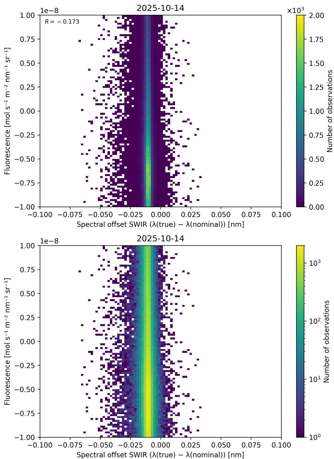
Figure 120: Scatter density plot of “Spectral offset SWIR ( \lambda_{\text{true}} - \lambda_{\text{nominal}} )” against “Fluorescence” for 2025-10-13 to 2025-10-15.
