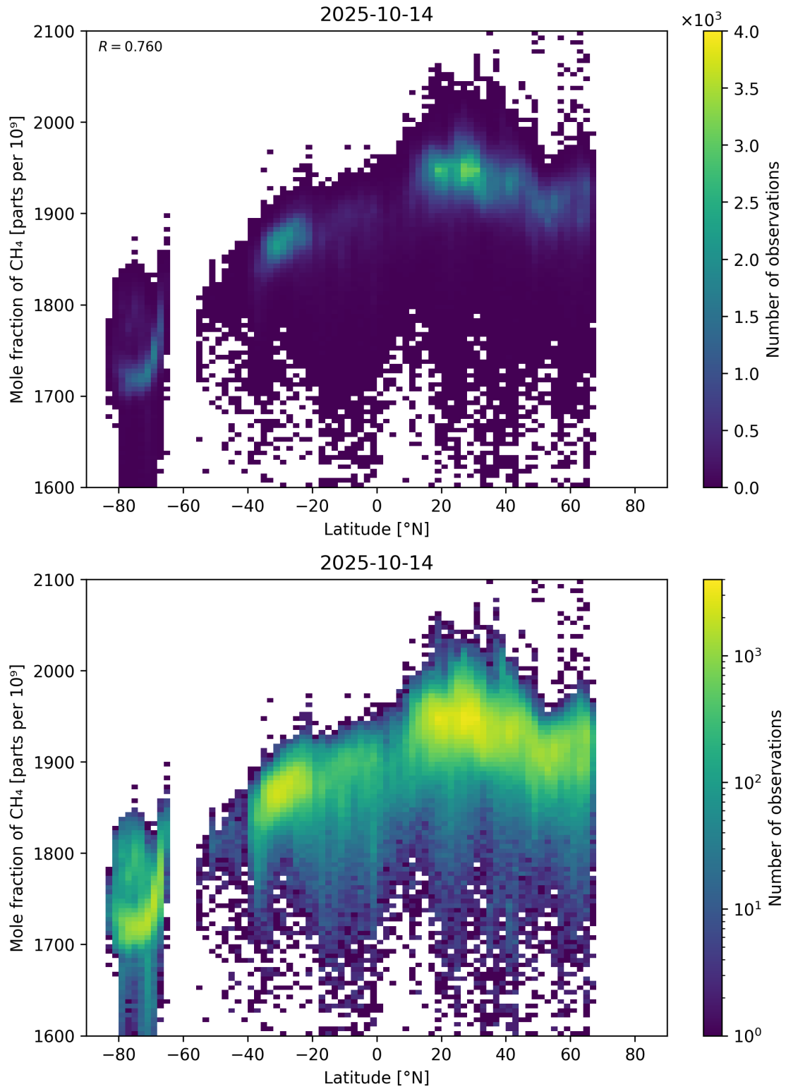
Figure 57: Scatter density plot of “Latitude” against “Mole fraction of \text{CH}_4 ” for 2025-10-13 to 2025-10-15.
