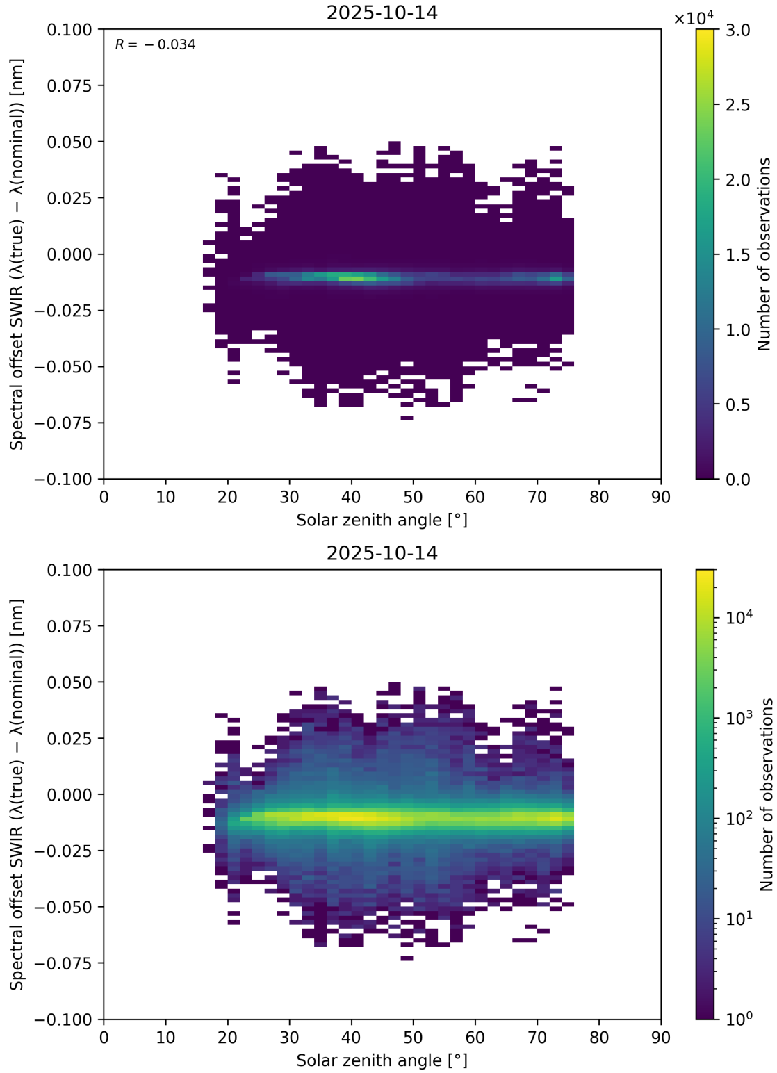
Figure 104: Scatter density plot of “Solar zenith angle” against “Spectral offset SWIR ( \lambda_{\text{true}} - \lambda_{\text{nominal}} )” for 2025-10-13 to 2025-10-15.
