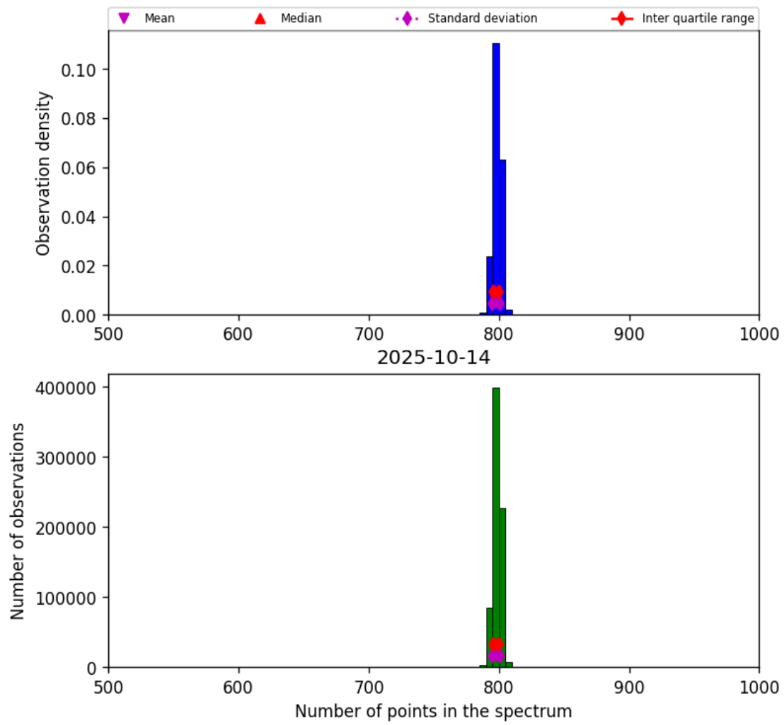
Figure 26: Histogram of “Number of points in the spectrum” for 2025-10-13 to 2025-10-15
