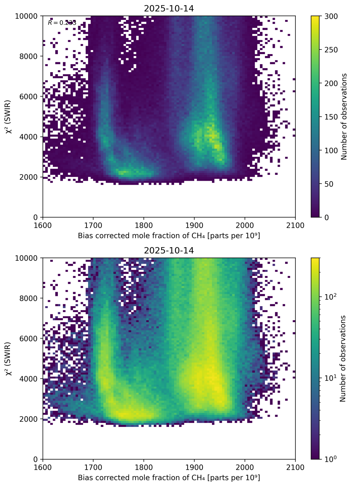
Figure 64: Scatter density plot of “Bias corrected mole fraction of \text{CH}_4 ” against “ \chi^2 (SWIR)” for 2025-10-13 to 2025-10-15.
