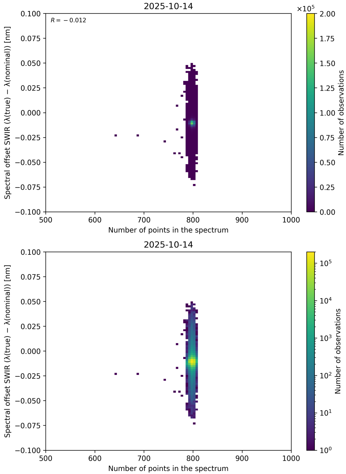
Figure 93: Scatter density plot of “Number of points in the spectrum” against “Spectral offset SWIR ( \lambda_{\text{true}} - \lambda_{\text{nominal}} )” for 2025-10-13 to 2025-10-15.
