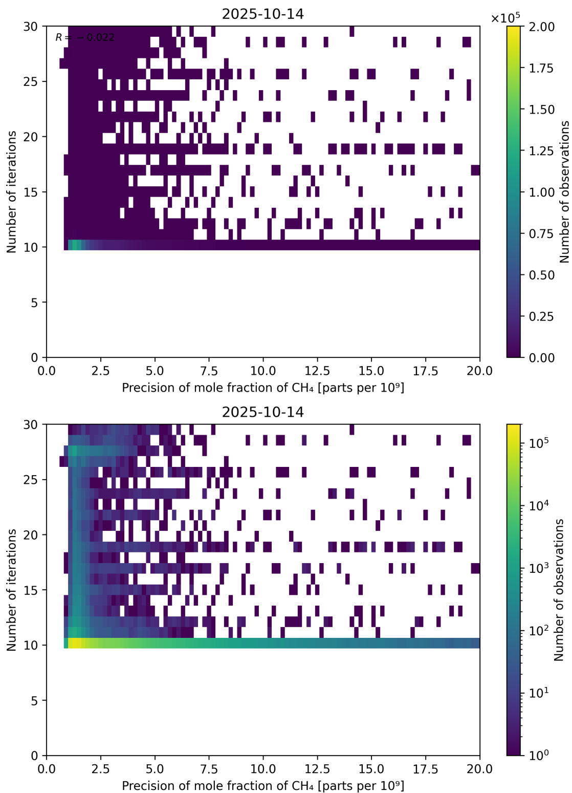
Figure 83: Scatter density plot of “Precision of mole fraction of CH 4 ” against “Number of iterations” for 2025-10-13 to 2025-10-15.
