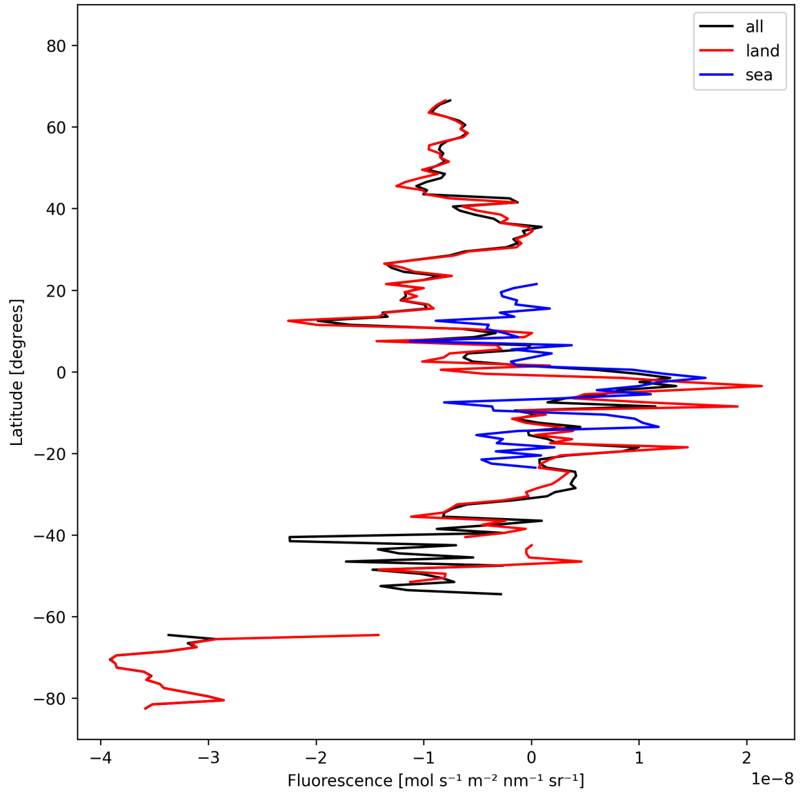
Figure 21: Zonal average of “Fluorescence” for 2025-10-13 to 2025-10-15.
