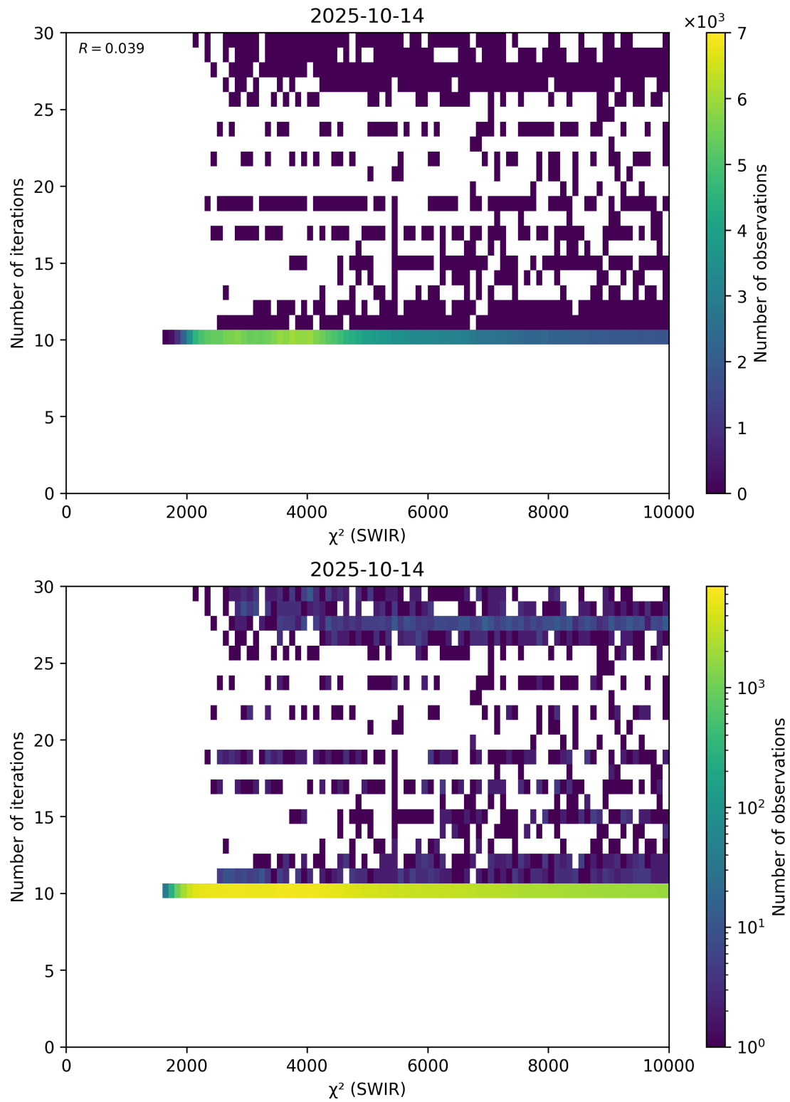
Figure 50: Scatter density plot of “ \chi^2 (SWIR)” against “Number of iterations” for 2025-10-13 to 2025-10-15.
