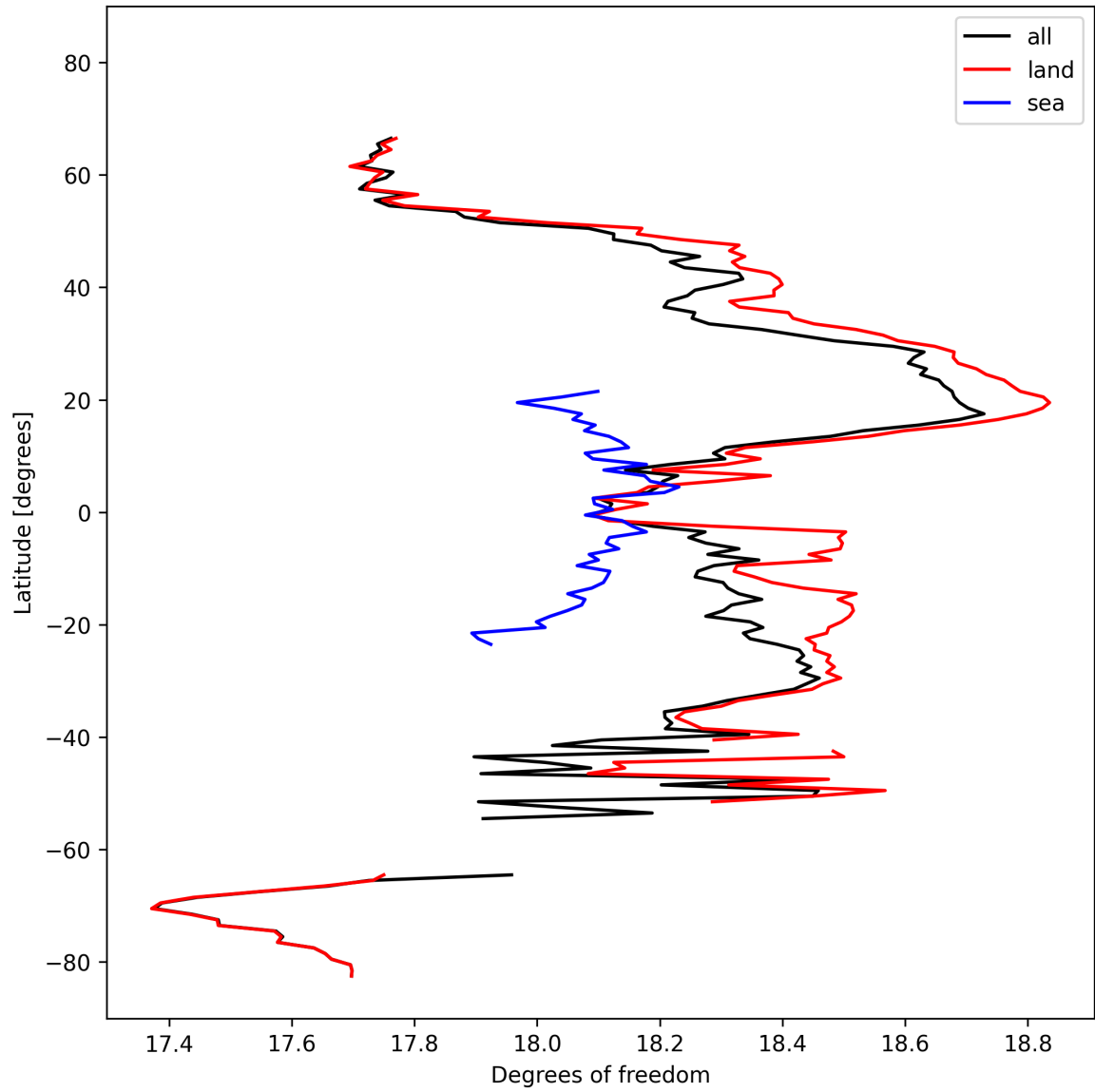
Figure 19: Zonal average of “Degrees of freedom” for 2025-10-13 to 2025-10-15.
