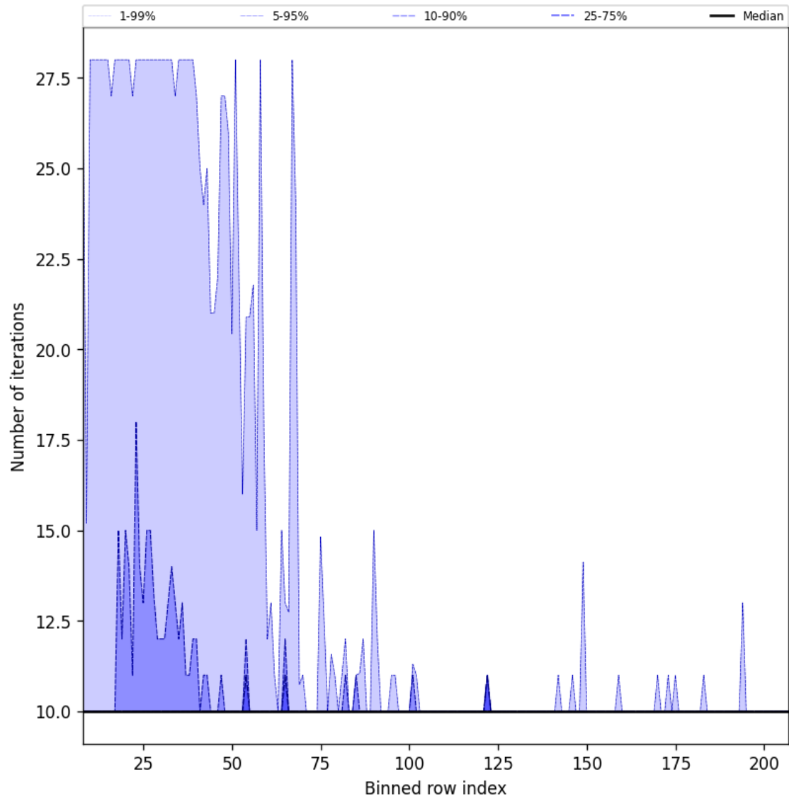
Figure 42: Along track statistics of “Number of iterations” for 2025-10-13 to 2025-10-15
