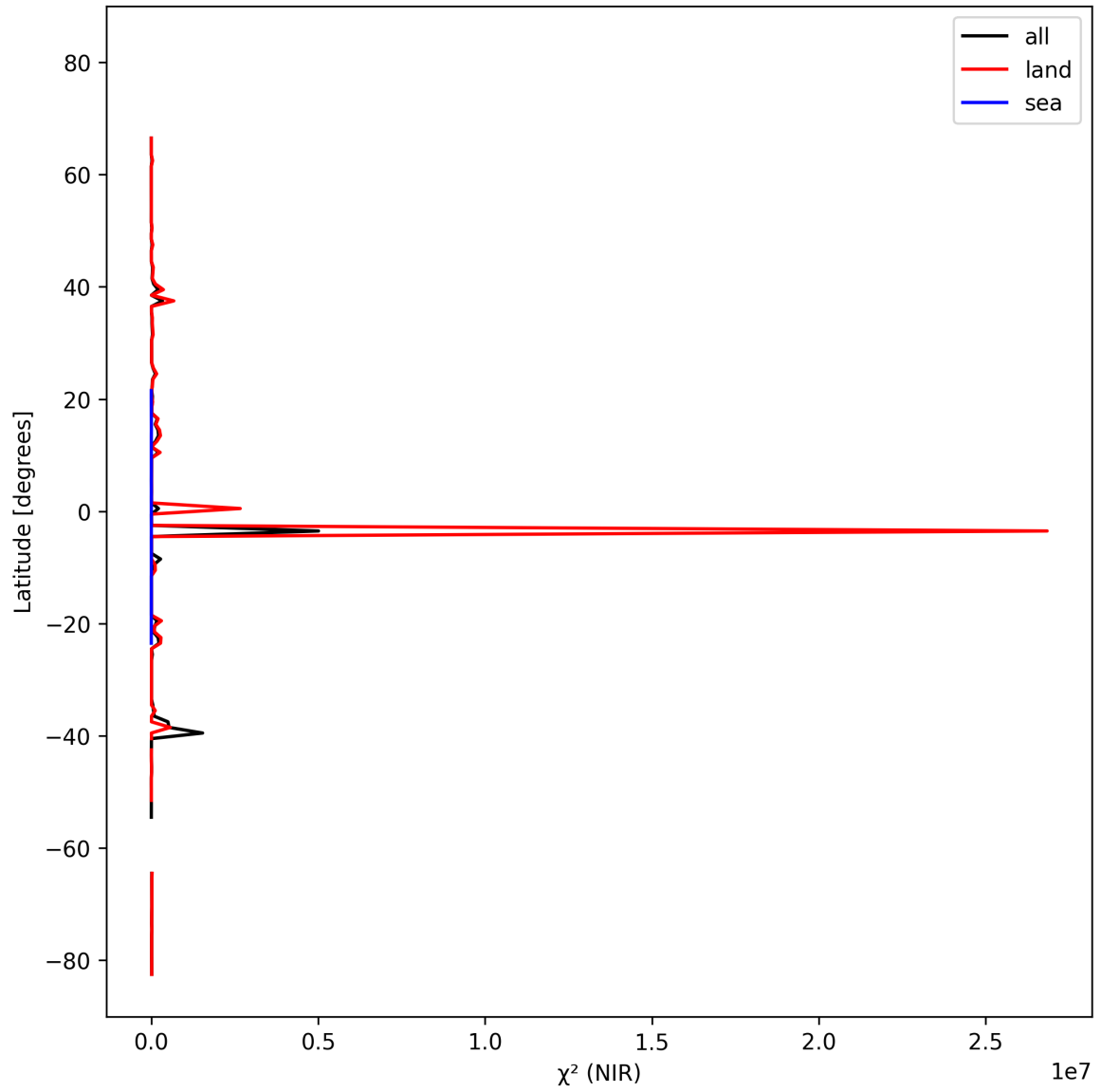
Figure 18: Zonal average of “ \chi^2 (NIR)” for 2025-10-13 to 2025-10-15.
