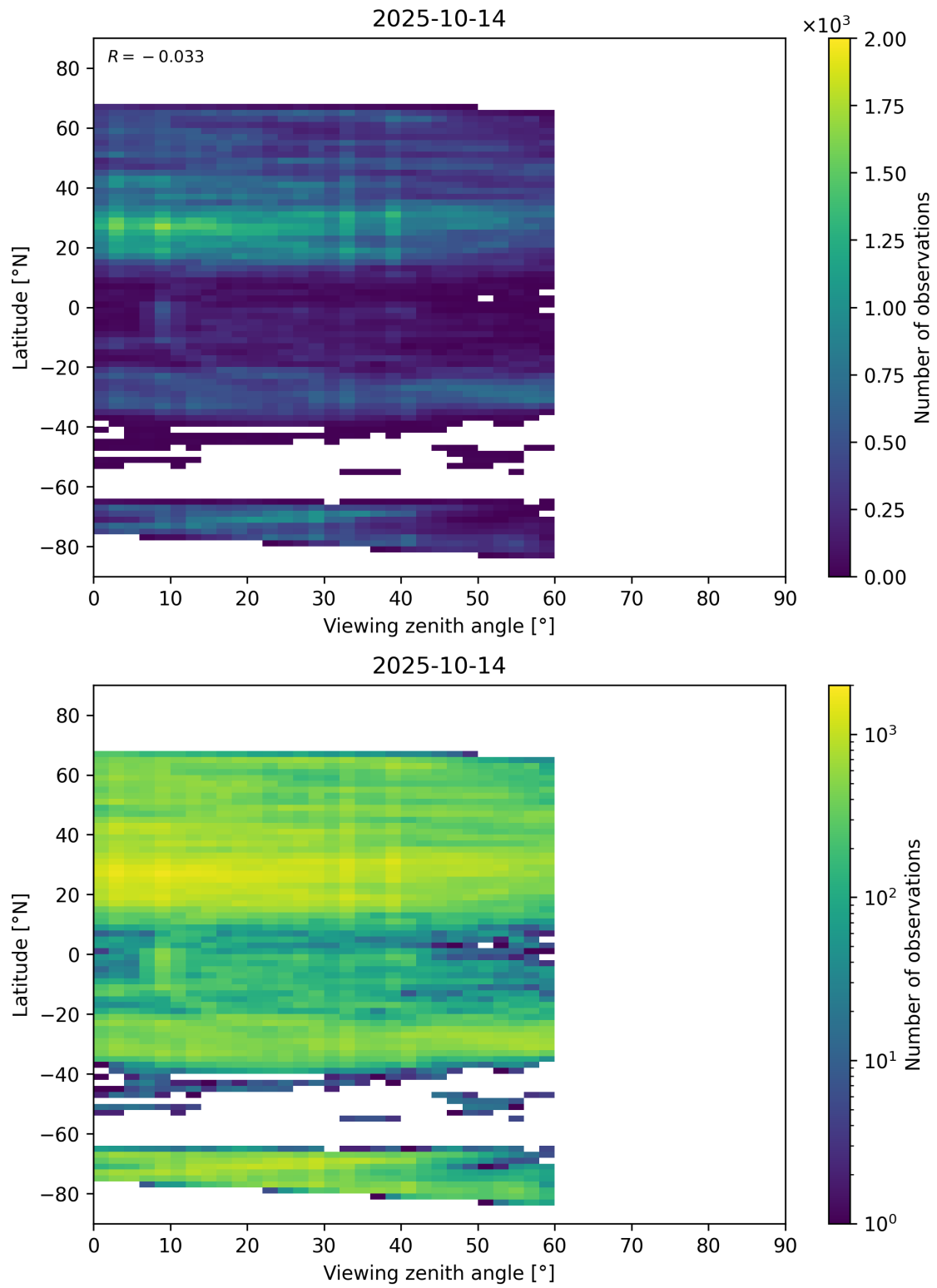
Figure 109: Scatter density plot of “Viewing zenith angle” against “Latitude” for 2025-10-13 to 2025-10-15.
