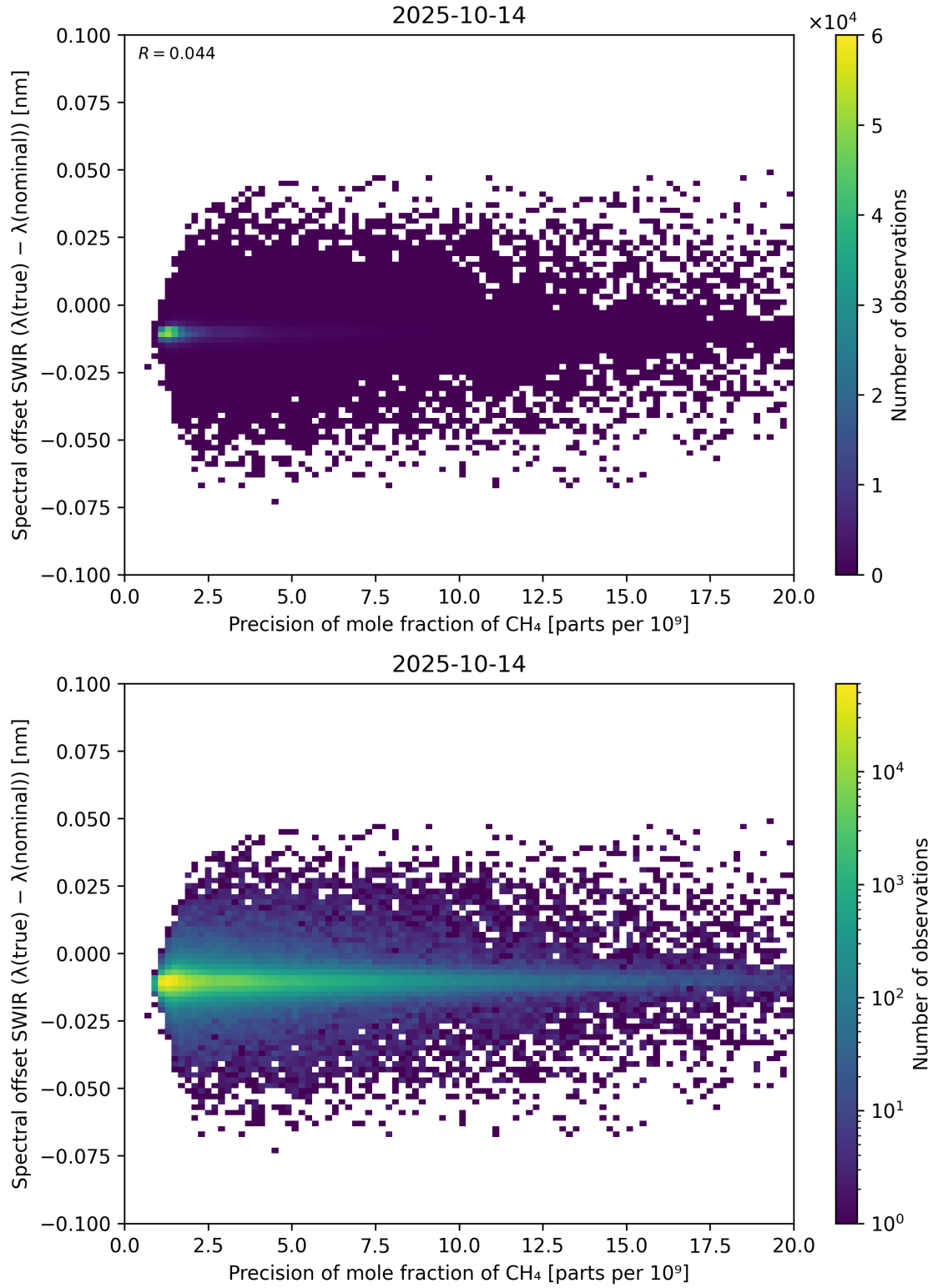
Figure 85: Scatter density plot of “Precision of mole fraction of CH 4 ” against “Spectral offset SWIR ( \lambda_{\text{true}} - \lambda_{\text{nominal}} )” for 2025-10-13 to 2025-10-15.
