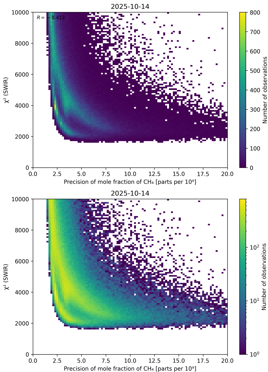
Figure 79: Scatter density plot of “Precision of mole fraction of CH 4 ” against “ \chi^2 (SWIR)” for 2025-10-13 to 2025-10-15.
