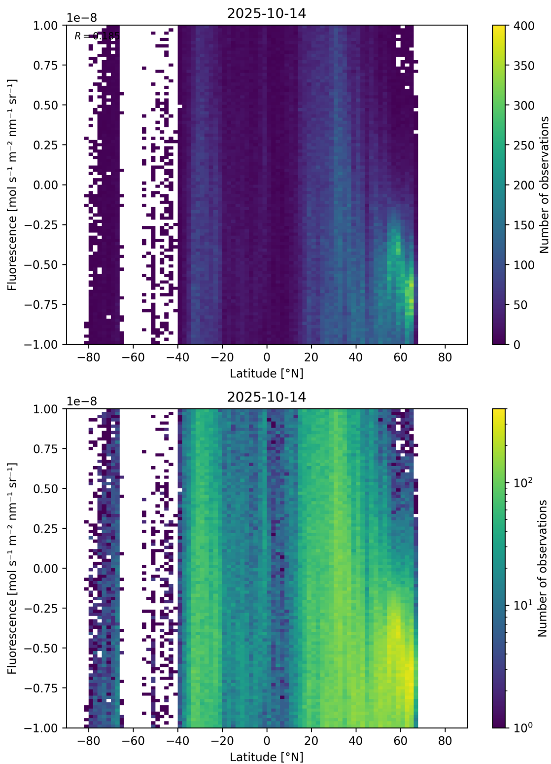
Figure 56: Scatter density plot of “Latitude” against “Fluorescence” for 2025-10-13 to 2025-10-15.
