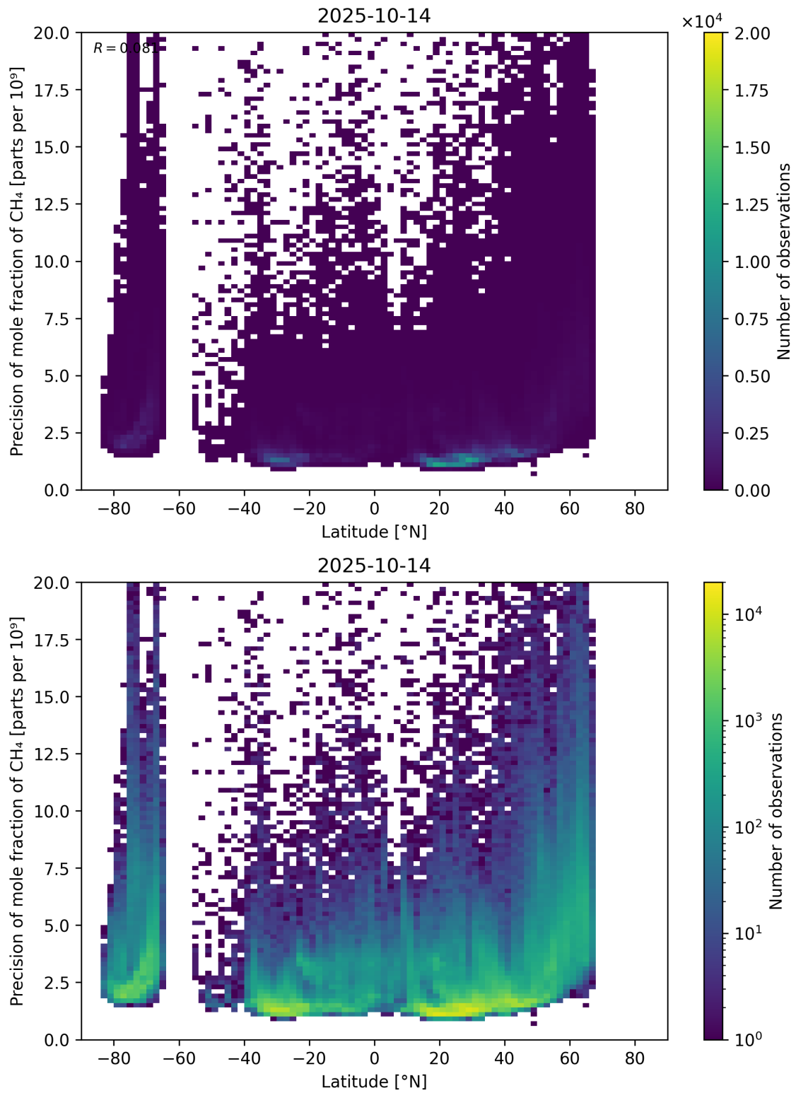
Figure 59: Scatter density plot of “Latitude” against “Precision of mole fraction of CH 4 ” for 2025-10-13 to 2025-10-15.
