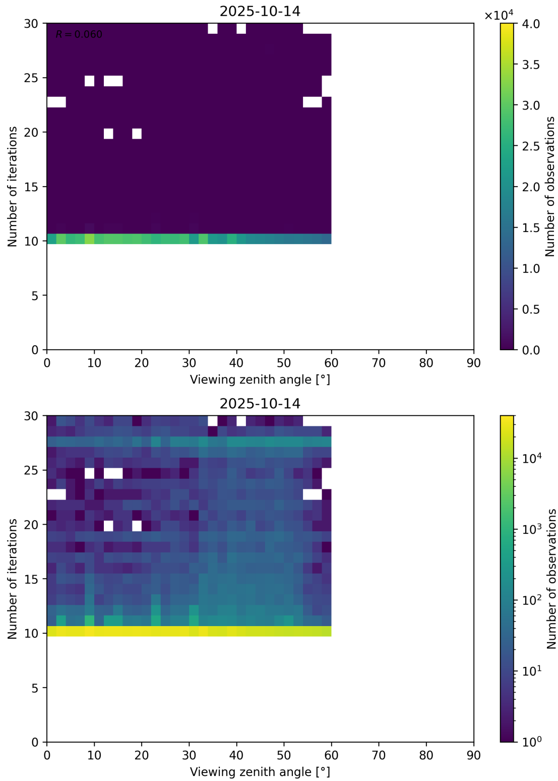
Figure 113: Scatter density plot of “Viewing zenith angle” against “Number of iterations” for 2025-10-13 to 2025-10-15.
