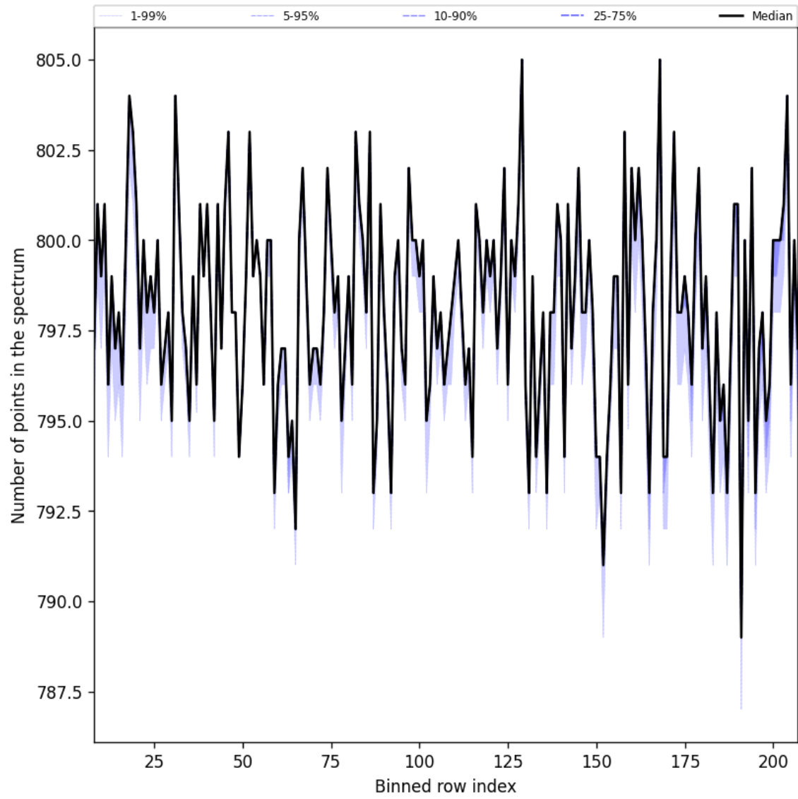
Figure 37: Along track statistics of “Number of points in the spectrum” for 2025-10-13 to 2025-10-15
