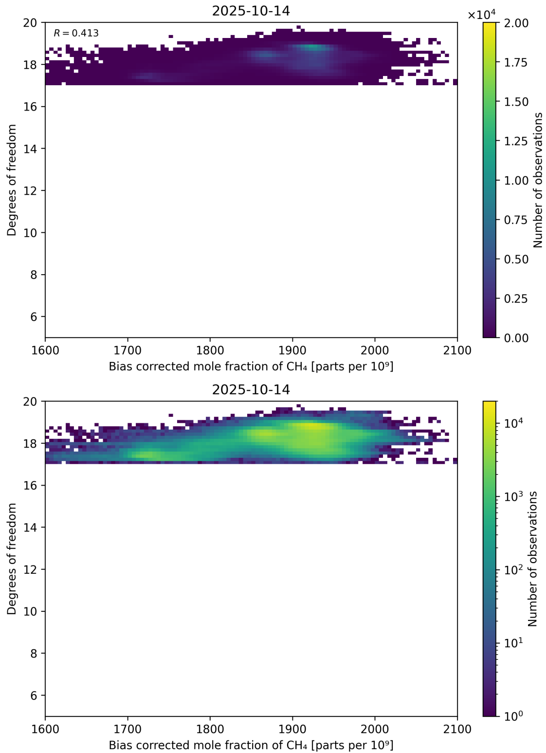
Figure 65: Scatter density plot of “Bias corrected mole fraction of \text{CH}_4 ” against “Degrees of freedom” for 2025-10-13 to 2025-10-15.
