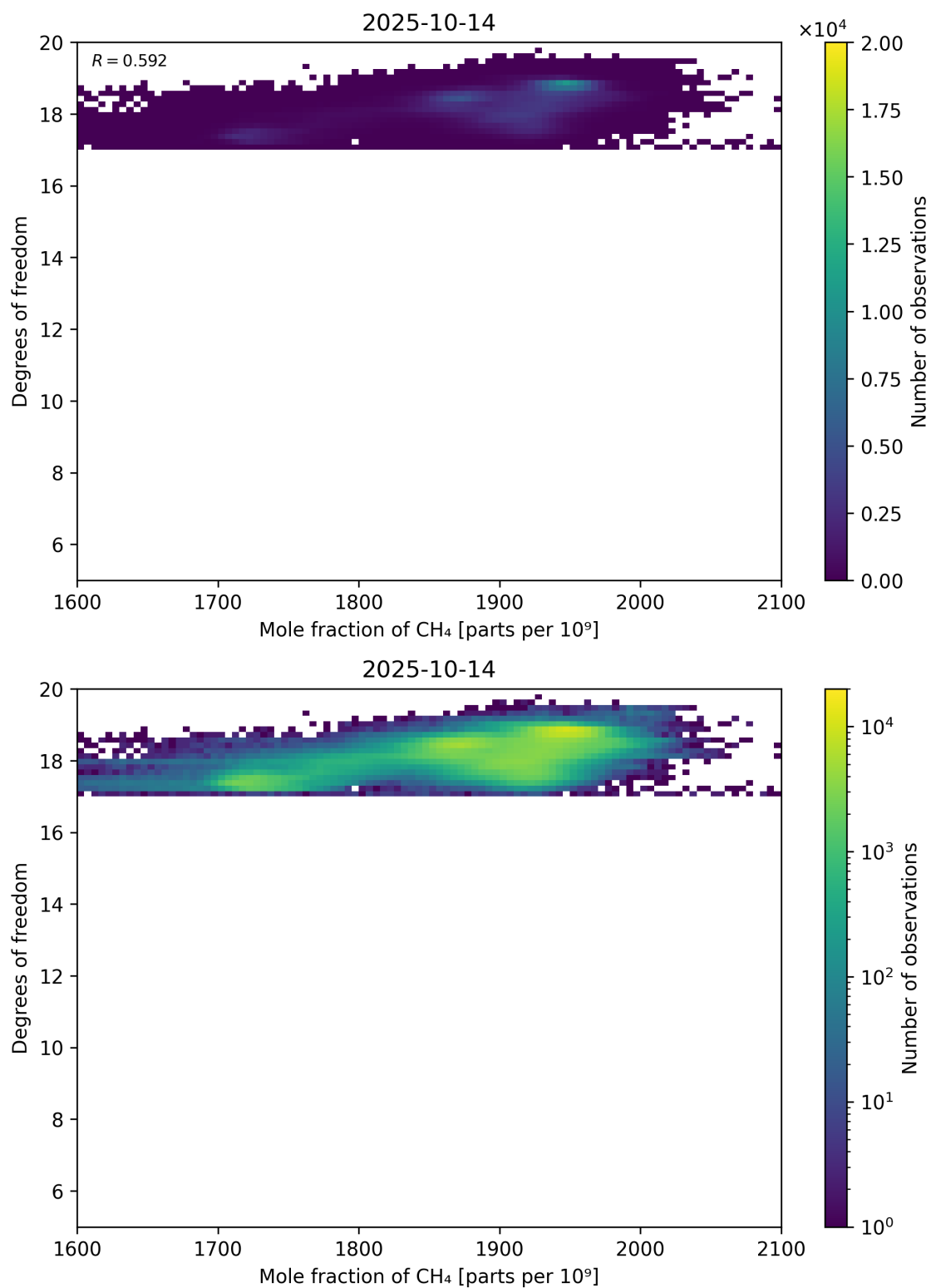
Figure 72: Scatter density plot of “Mole fraction of CH 4 ” against “Degrees of freedom” for 2025-10-13 to 2025-10-15.
