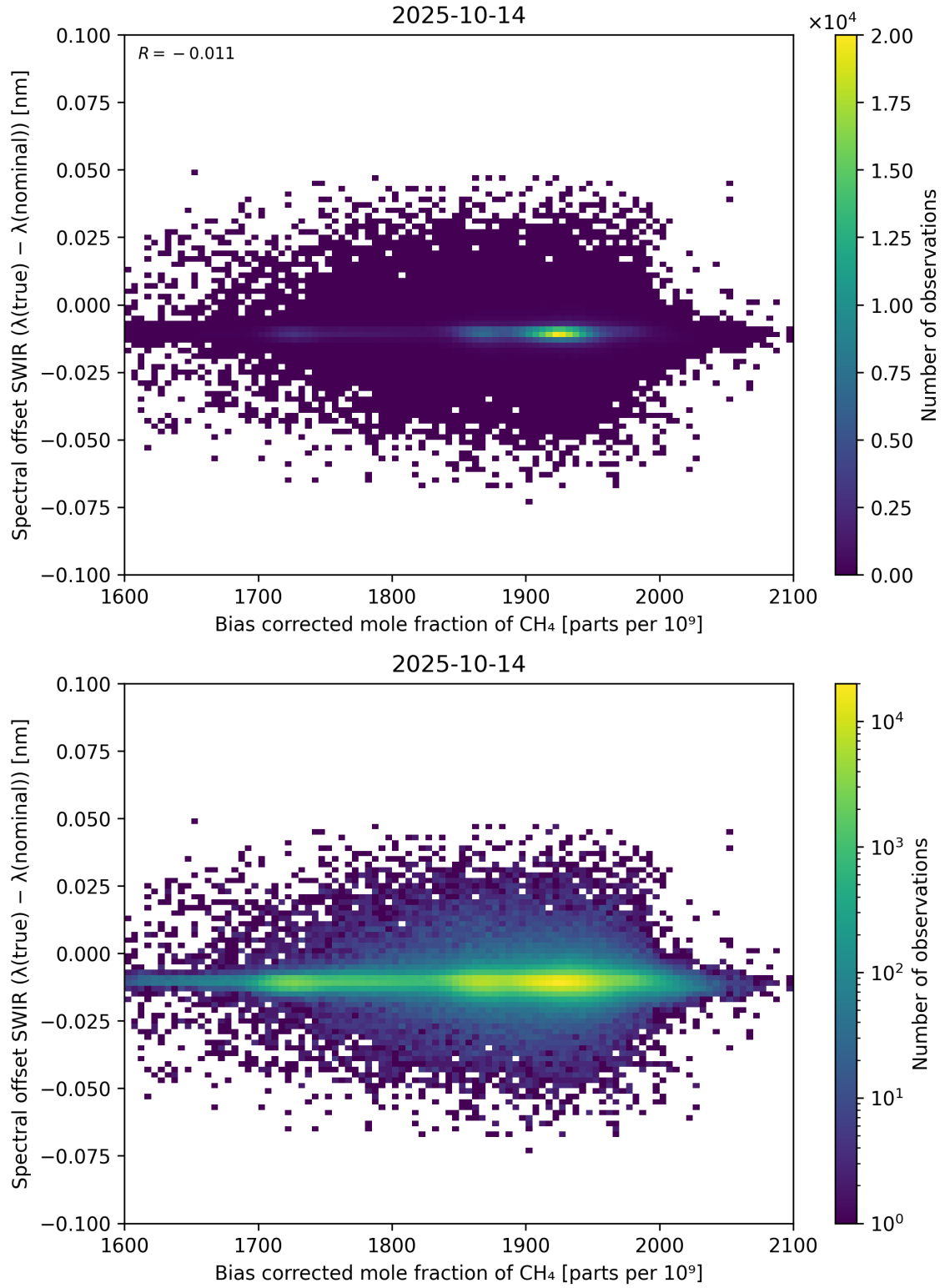
Figure 69: Scatter density plot of “Bias corrected mole fraction of \text{CH}_4 ” against “Spectral offset SWIR ( \lambda_{\text{true}} - \lambda_{\text{nominal}} )” for 2025-10-13 to 2025-10-15.
