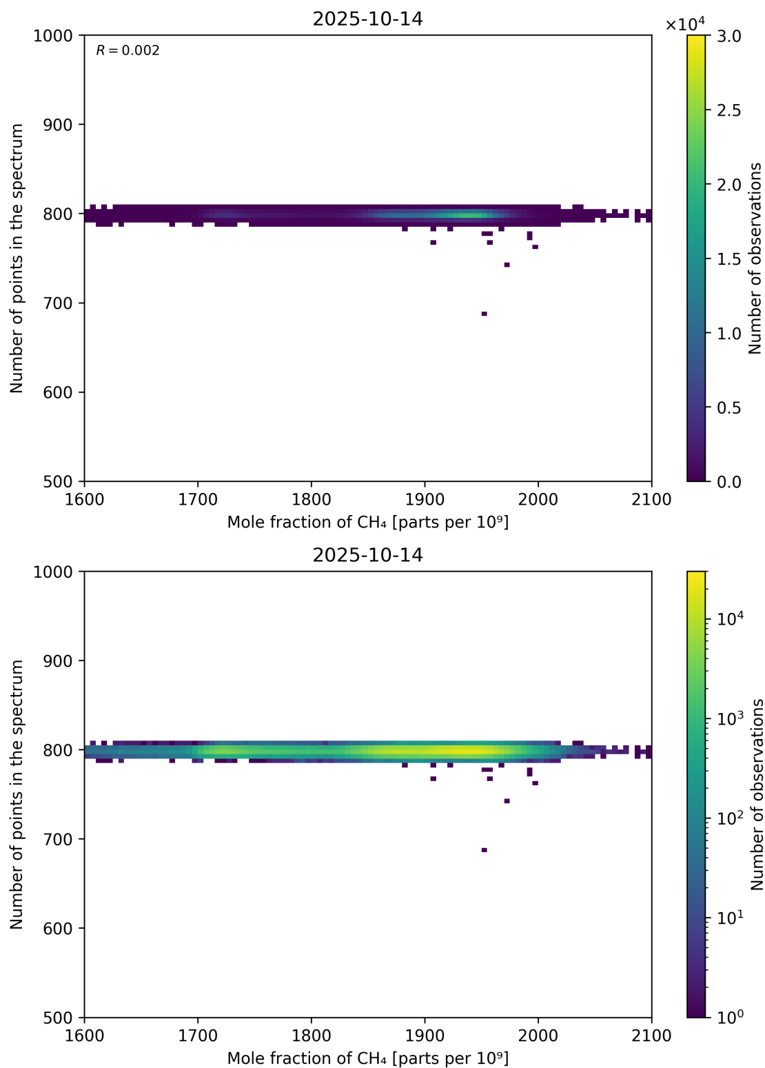
Figure 77: Scatter density plot of “Mole fraction of CH 4 ” against “Number of points in the spectrum” for 2025-10-13 to 2025-10-15.
