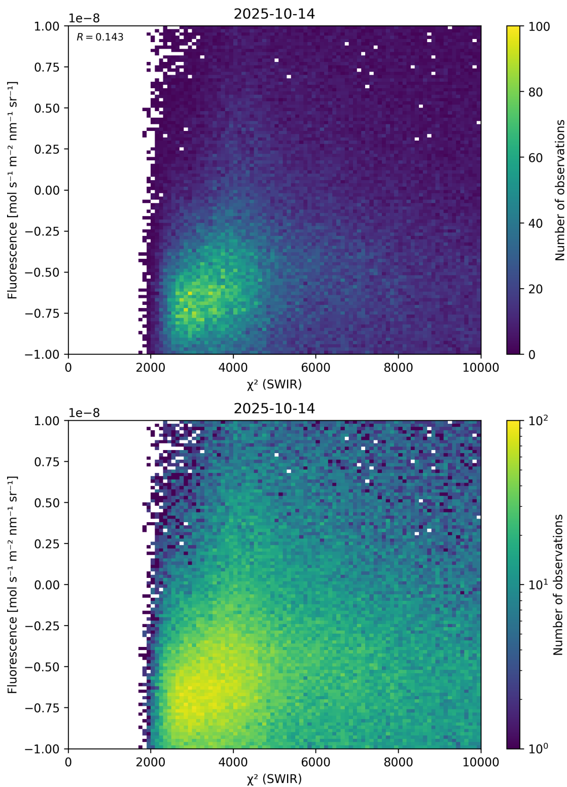
Figure 49: Scatter density plot of “ \chi^2 (SWIR)” against “Fluorescence” for 2025-10-13 to 2025-10-15.
