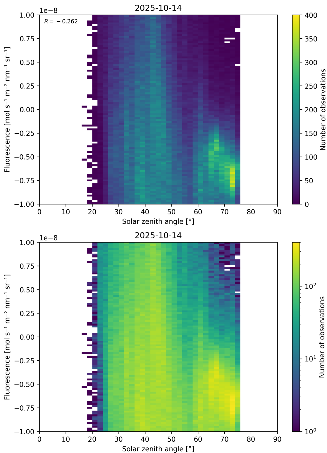
Figure 97: Scatter density plot of “Solar zenith angle” against “Fluorescence” for 2025-10-13 to 2025-10-15.
