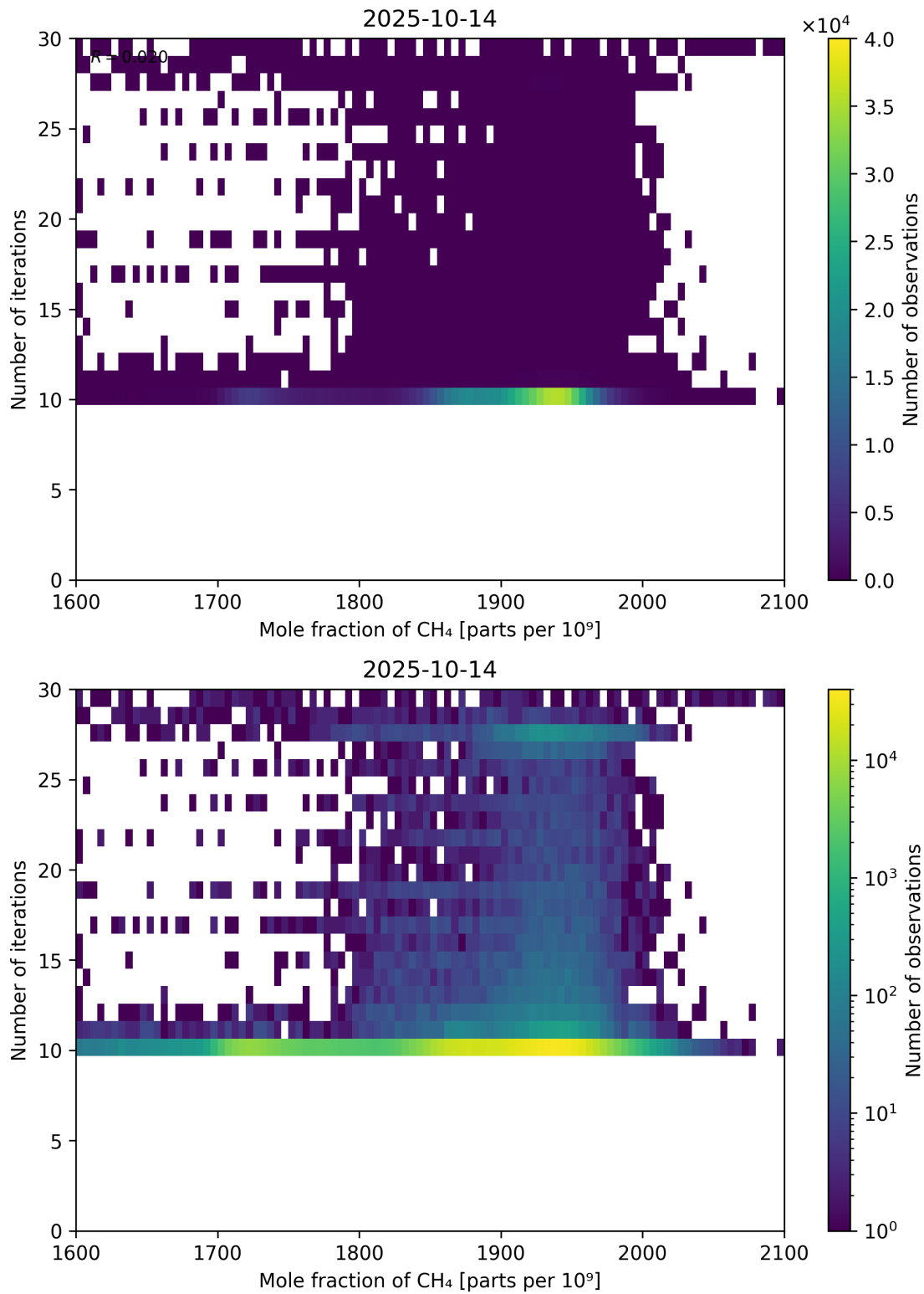
Figure 76: Scatter density plot of “Mole fraction of CH 4 ” against “Number of iterations” for 2025-10-13 to 2025-10-15.
