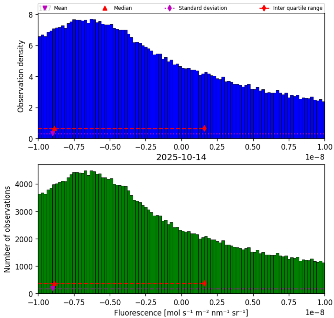
Figure 32: Histogram of “Fluorescence” for 2025-10-13 to 2025-10-15
