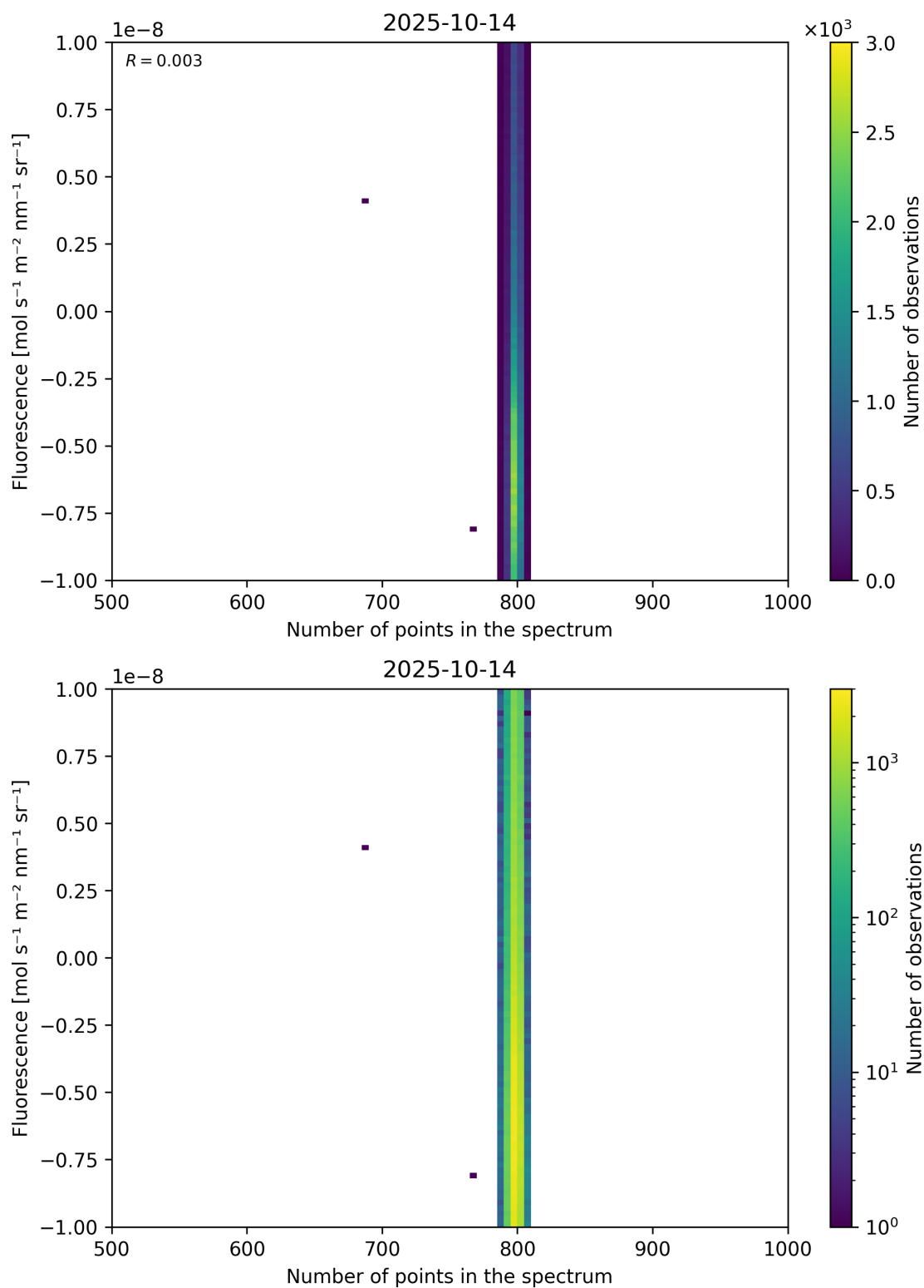
Figure 91: Scatter density plot of “Number of points in the spectrum” against “Fluorescence” for 2025-10-13 to 2025-10-15.
