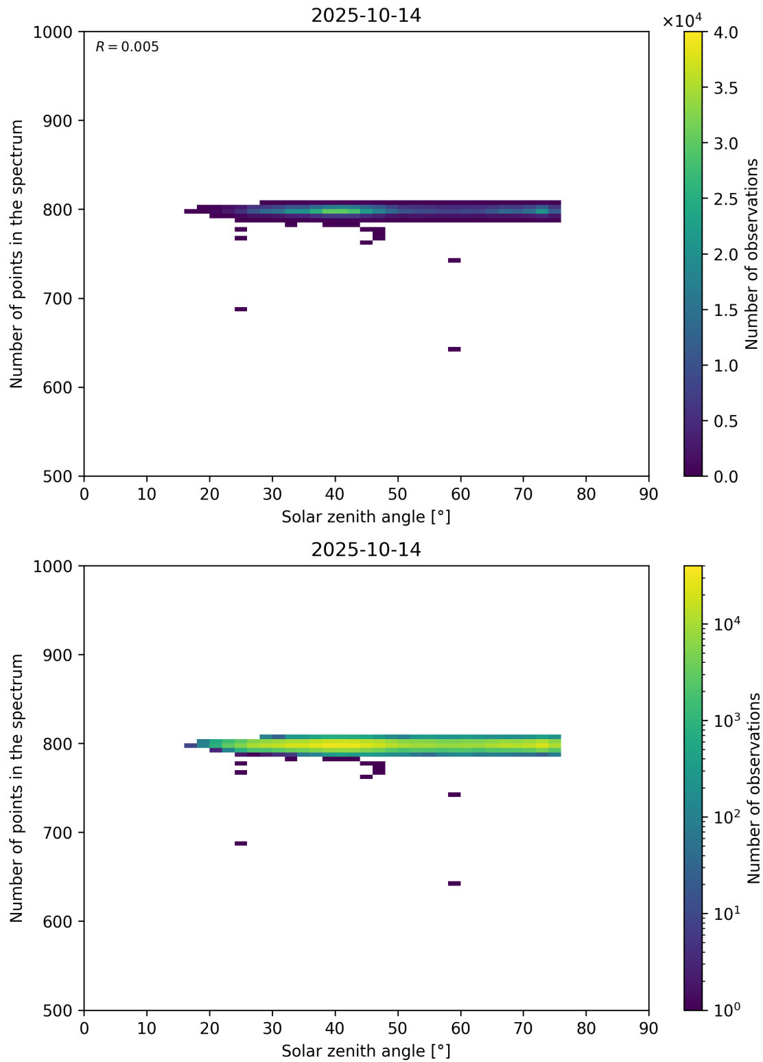
Figure 103: Scatter density plot of “Solar zenith angle” against “Number of points in the spectrum” for 2025-10-13 to 2025-10-15.
