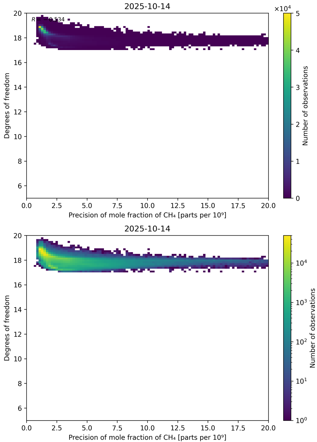
Figure 80: Scatter density plot of “Precision of mole fraction of CH 4 ” against “Degrees of freedom” for 2025-10-13 to 2025-10-15.
