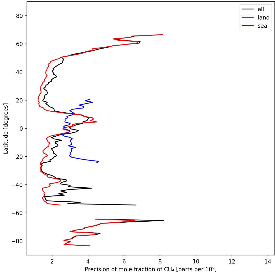
Figure 13: Zonal average of “Precision of mole fraction of CH 4 ” for 2025-10-15 to 2025-10-17.
