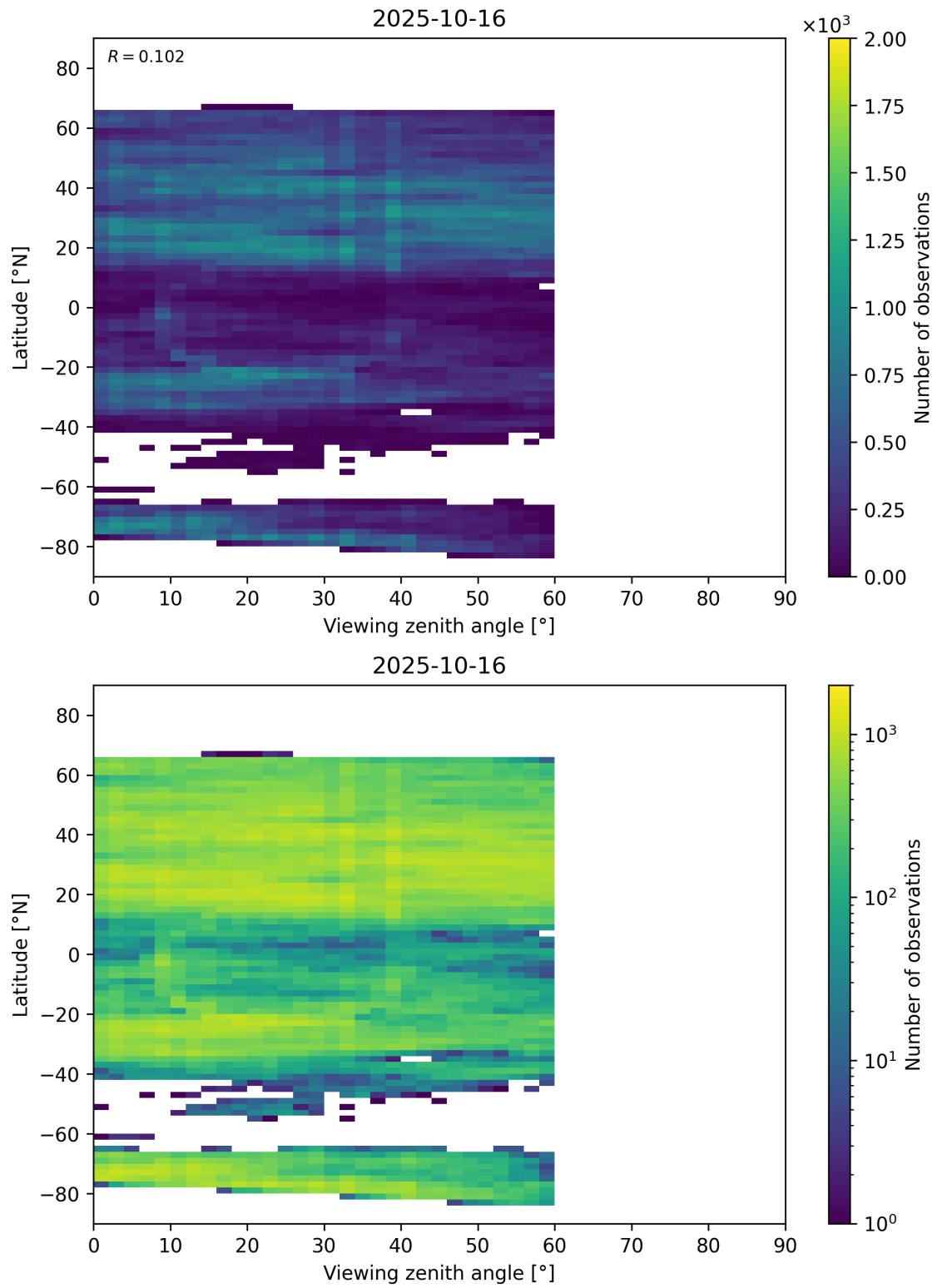
Figure 109: Scatter density plot of “Viewing zenith angle” against “Latitude” for 2025-10-15 to 2025-10-17.
