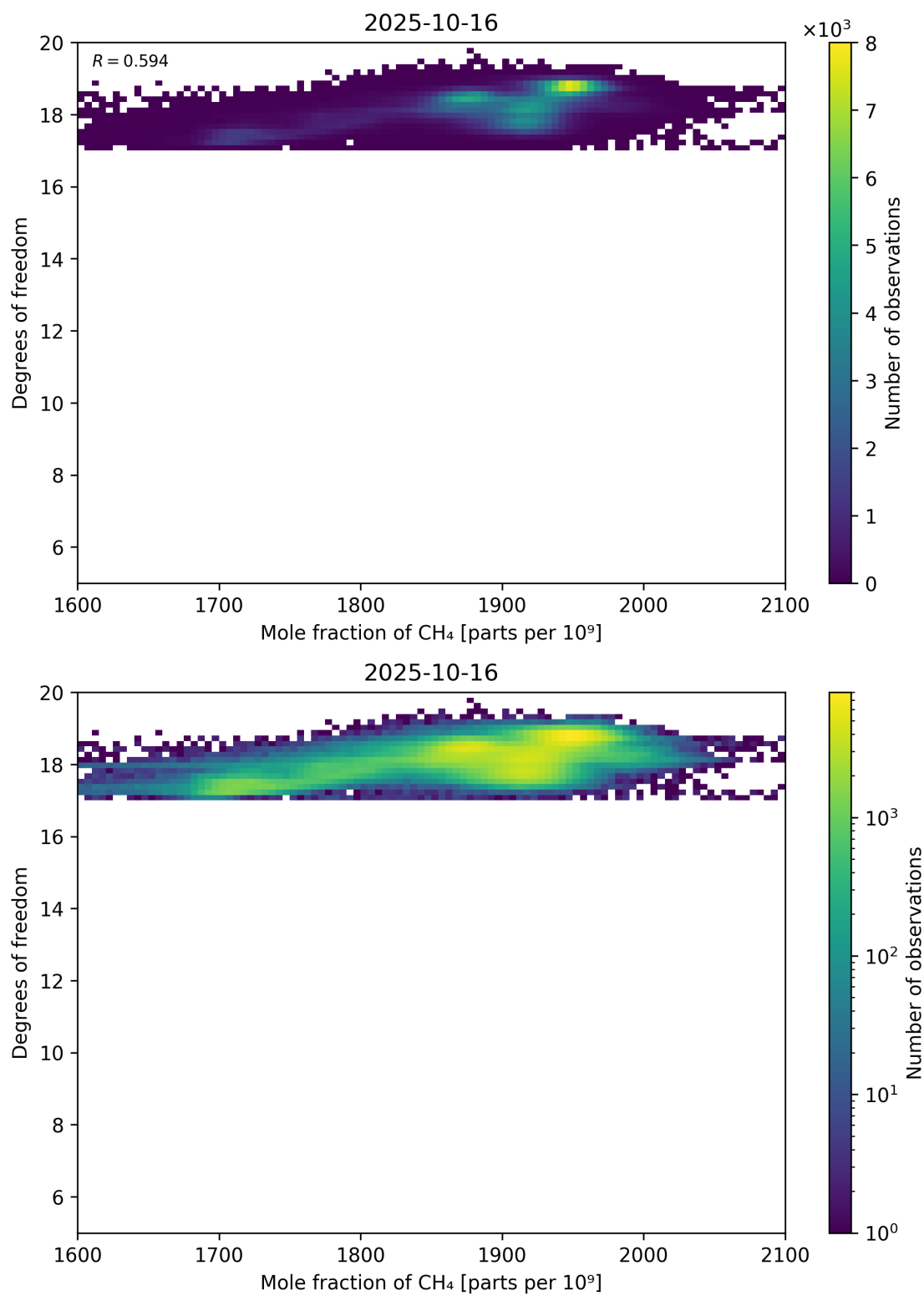
Figure 72: Scatter density plot of “Mole fraction of CH 4 ” against “Degrees of freedom” for 2025-10-15 to 2025-10-17.
