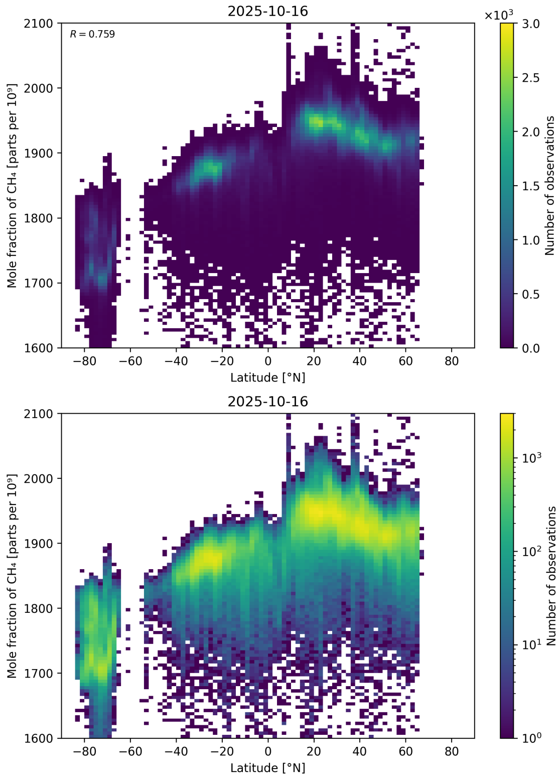
Figure 57: Scatter density plot of “Latitude” against “Mole fraction of CH 4 ” for 2025-10-15 to 2025-10-17.
