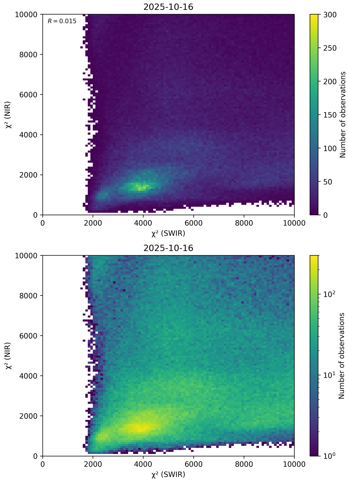
Figure 47: Scatter density plot of “ \chi^2 (SWIR)” against “ \chi^2 (NIR)” for 2025-10-15 to 2025-10-17.
