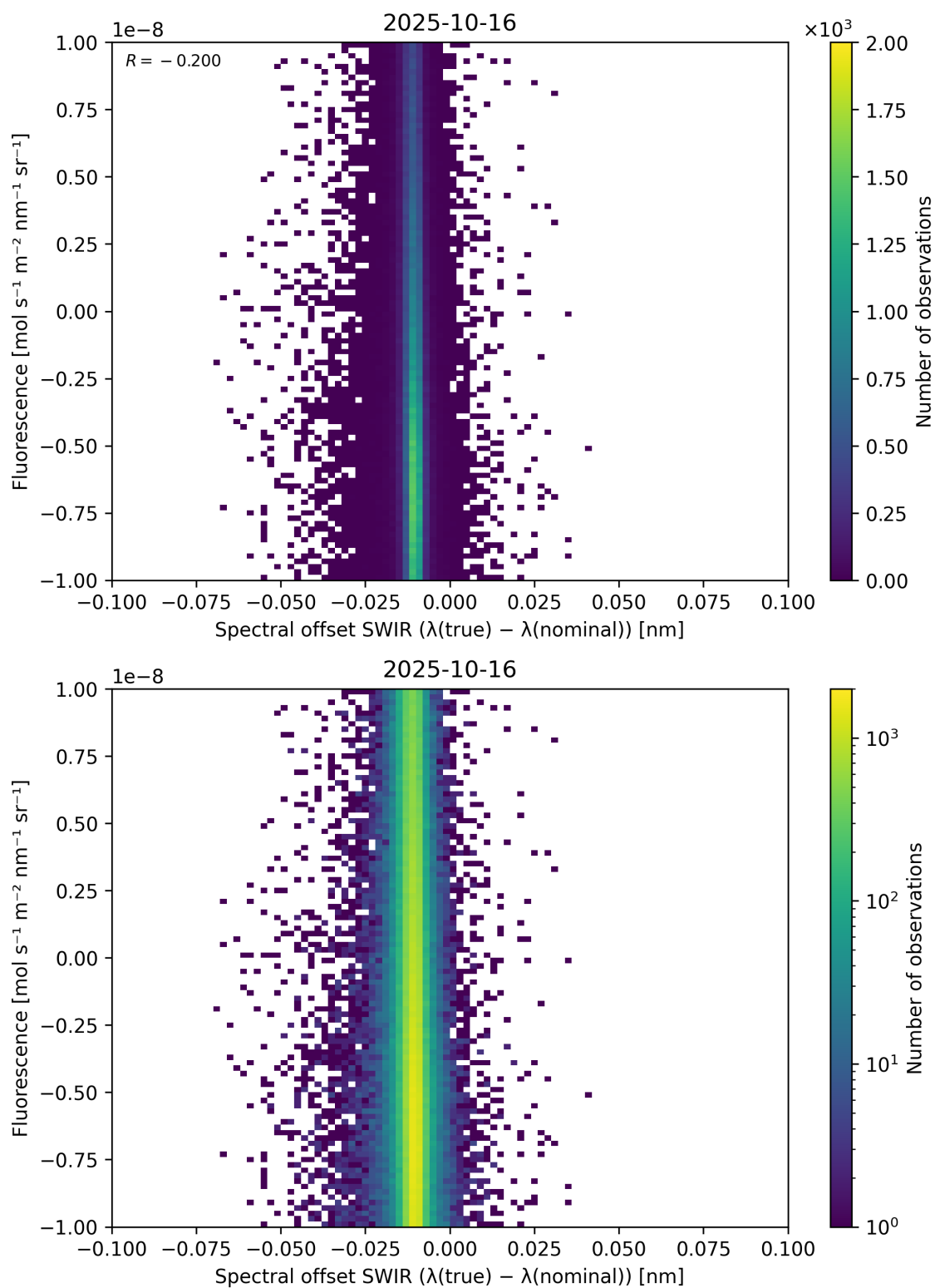
Figure 120: Scatter density plot of “Spectral offset SWIR ( \lambda_{\text{true}} - \lambda_{\text{nominal}} )” against “Fluorescence” for 2025-10-15 to 2025-10-17.
