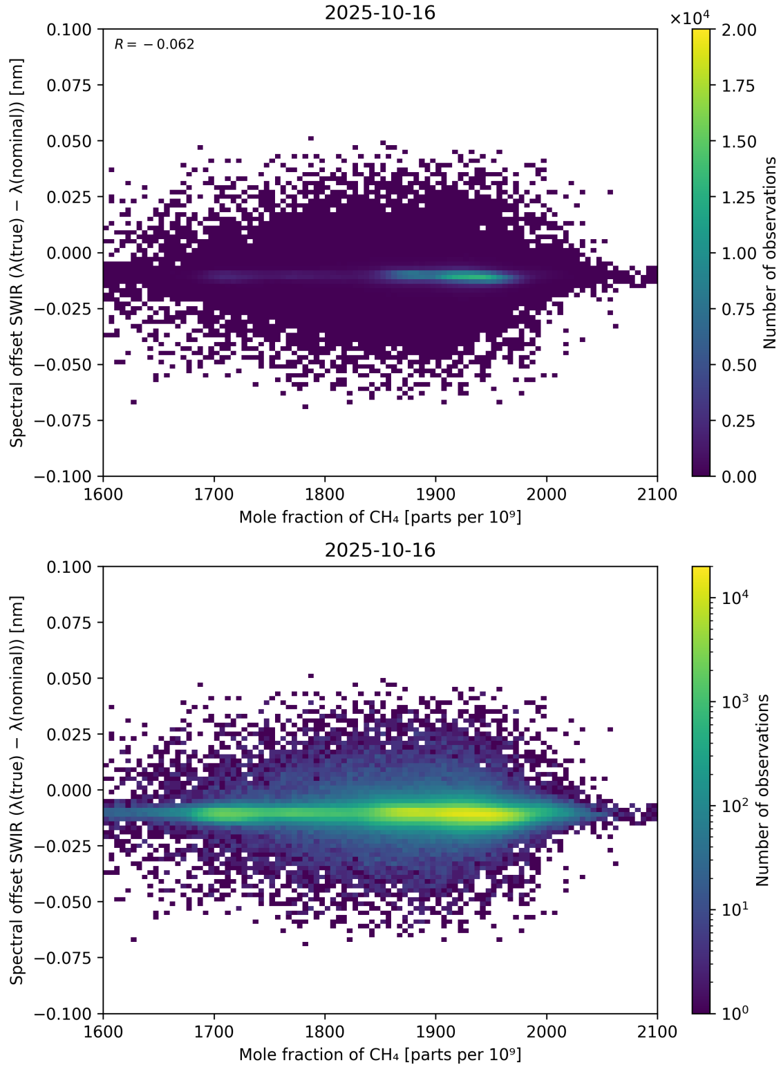
Figure 86: Scatter density plot of “Mole fraction of CH 4 ” against “Spectral offset SWIR ( \lambda_{\text{true}} - \lambda_{\text{nominal}} )” for 2025-10-15 to 2025-10-17.
