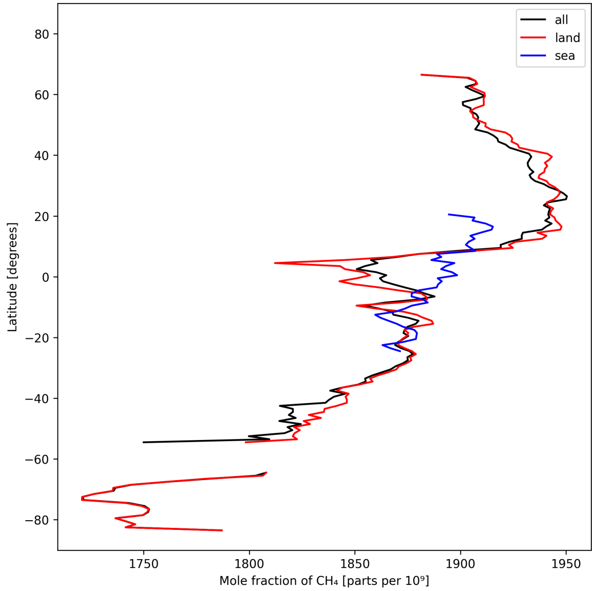
Figure 12: Zonal average of “Mole fraction of CH 4 ” for 2025-10-15 to 2025-10-17.
