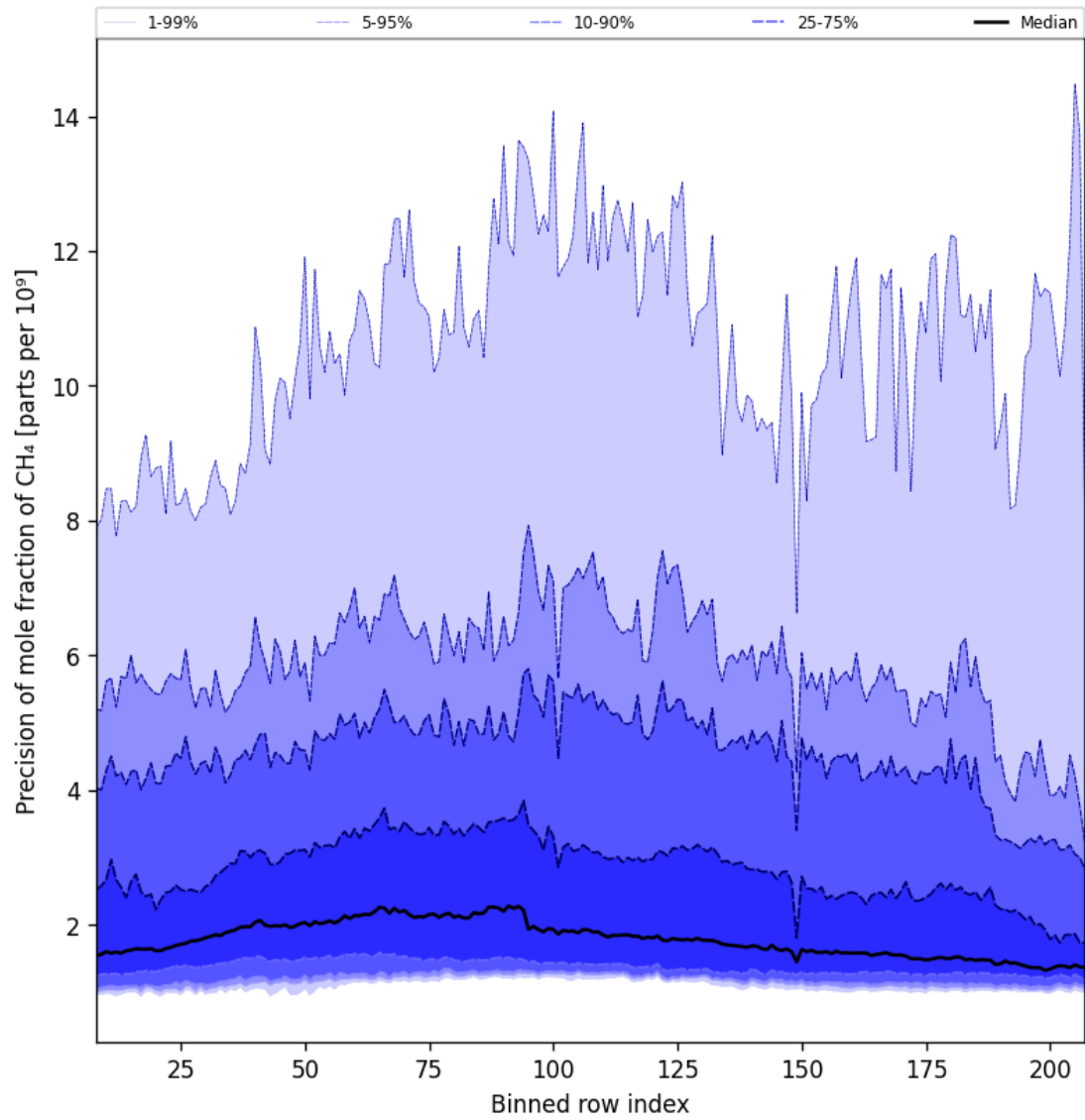
Figure 35: Along track statistics of “Precision of mole fraction of CH 4 ” for 2025-10-15 to 2025-10-17
