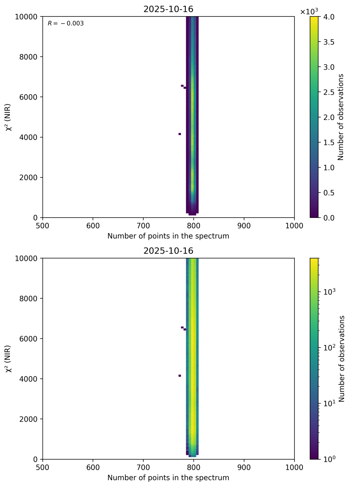
Figure 88: Scatter density plot of “Number of points in the spectrum” against “ \chi^2 (NIR)” for 2025-10-15 to 2025-10-17.
