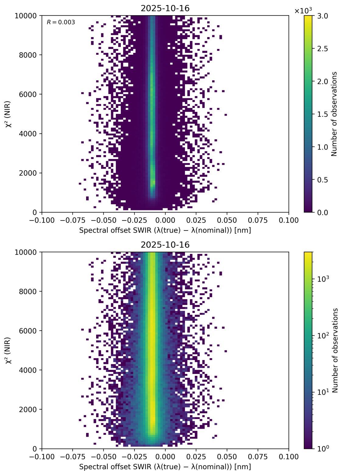
Figure 117: Scatter density plot of “Spectral offset SWIR ( \lambda_{\text{true}} - \lambda_{\text{nominal}} )” against “ \chi^2 (NIR)” for 2025-10-15 to 2025-10-17.
