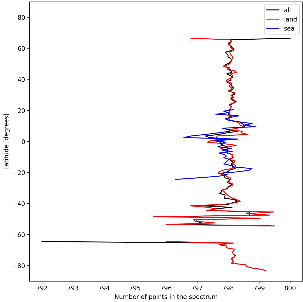
Figure 15: Zonal average of “Number of points in the spectrum” for 2025-10-15 to 2025-10-17.
