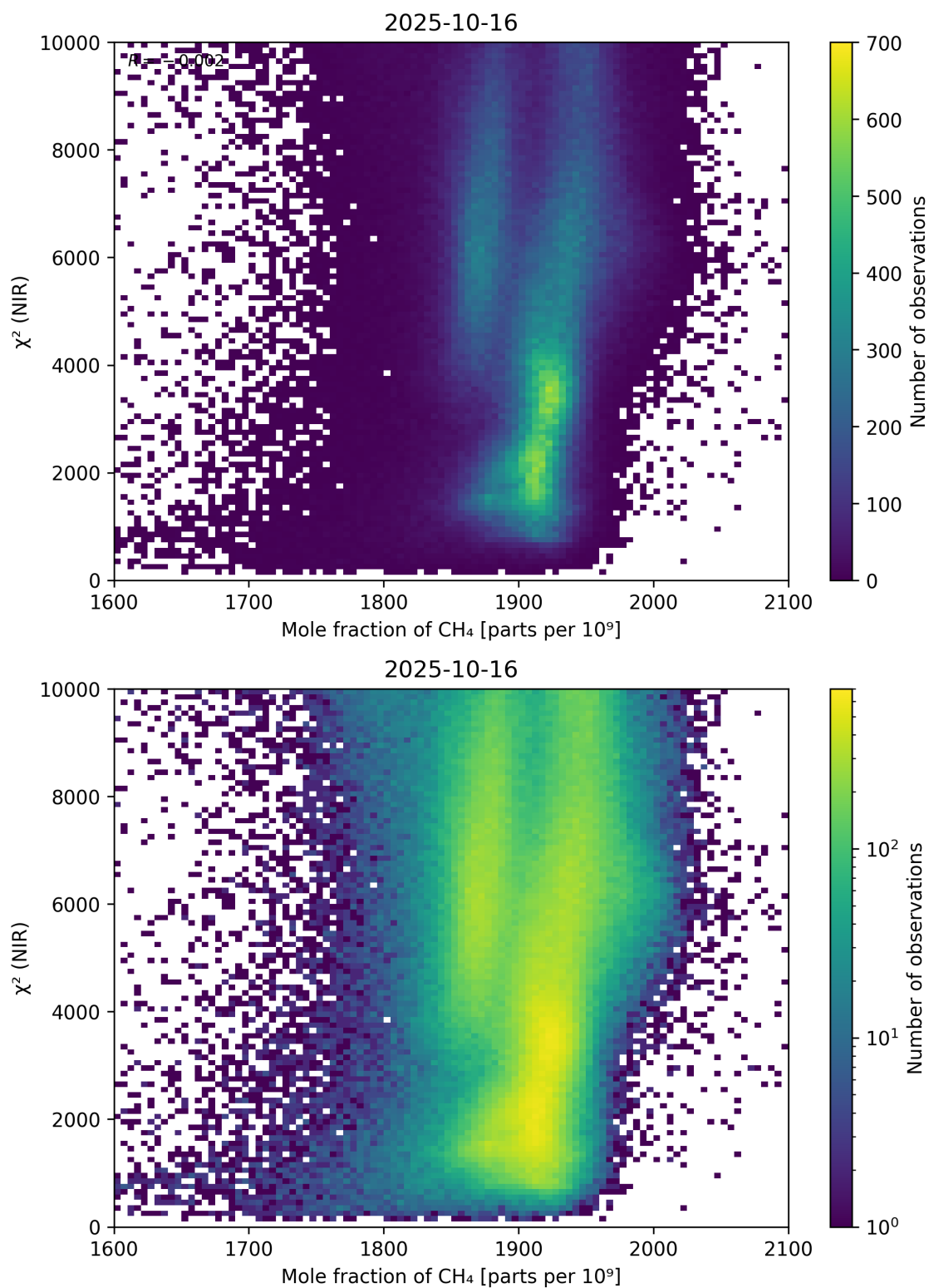
Figure 70: Scatter density plot of “Mole fraction of \text{CH}_4 ” against “ \chi^2 (NIR)” for 2025-10-15 to 2025-10-17.
