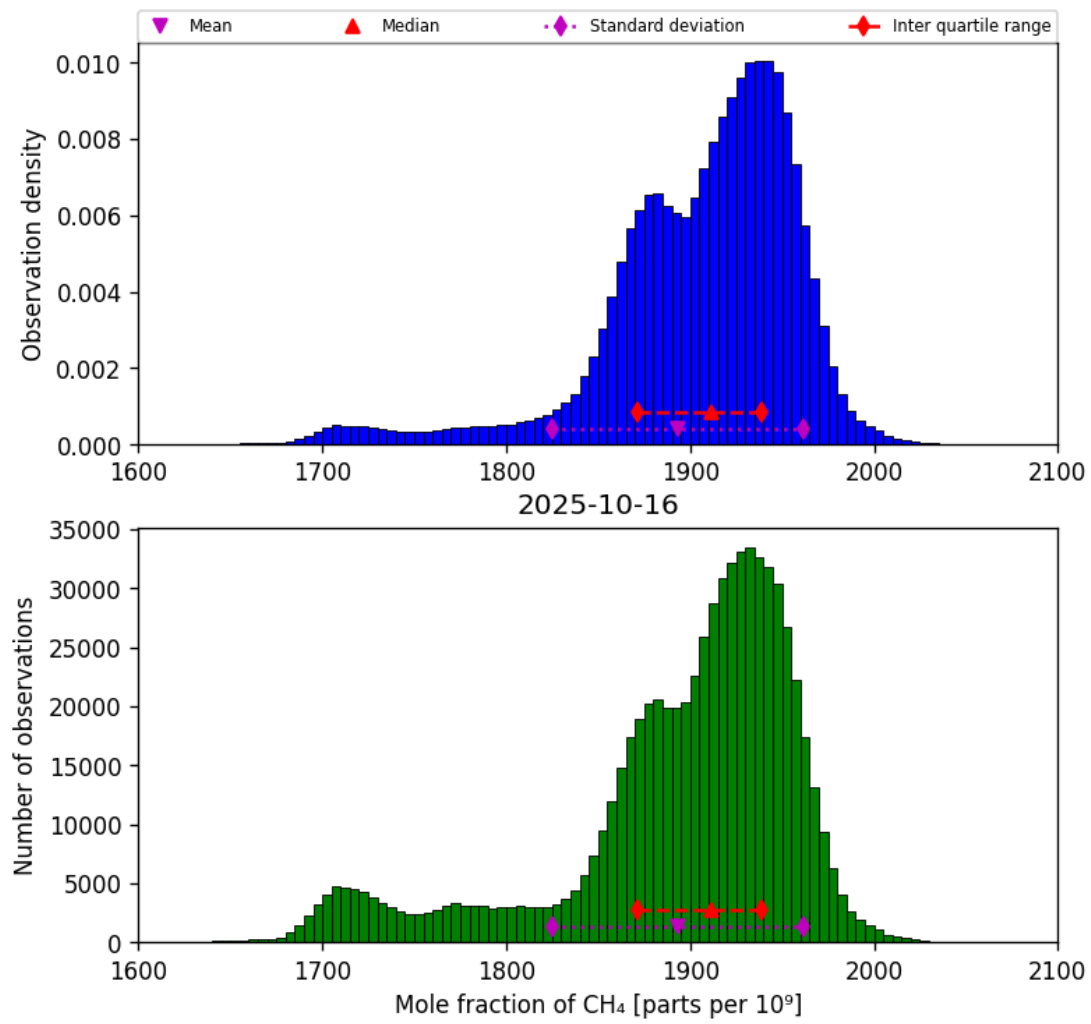
Figure 23: Histogram of “Mole fraction of CH 4 ” for 2025-10-15 to 2025-10-17
