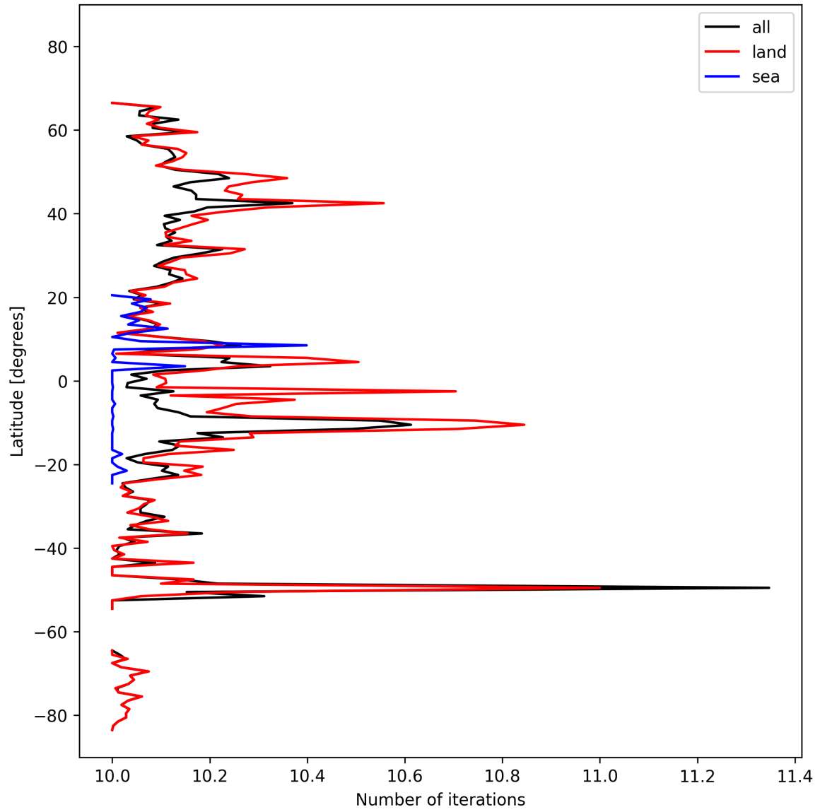
Figure 20: Zonal average of “Number of iterations” for 2025-10-15 to 2025-10-17.
