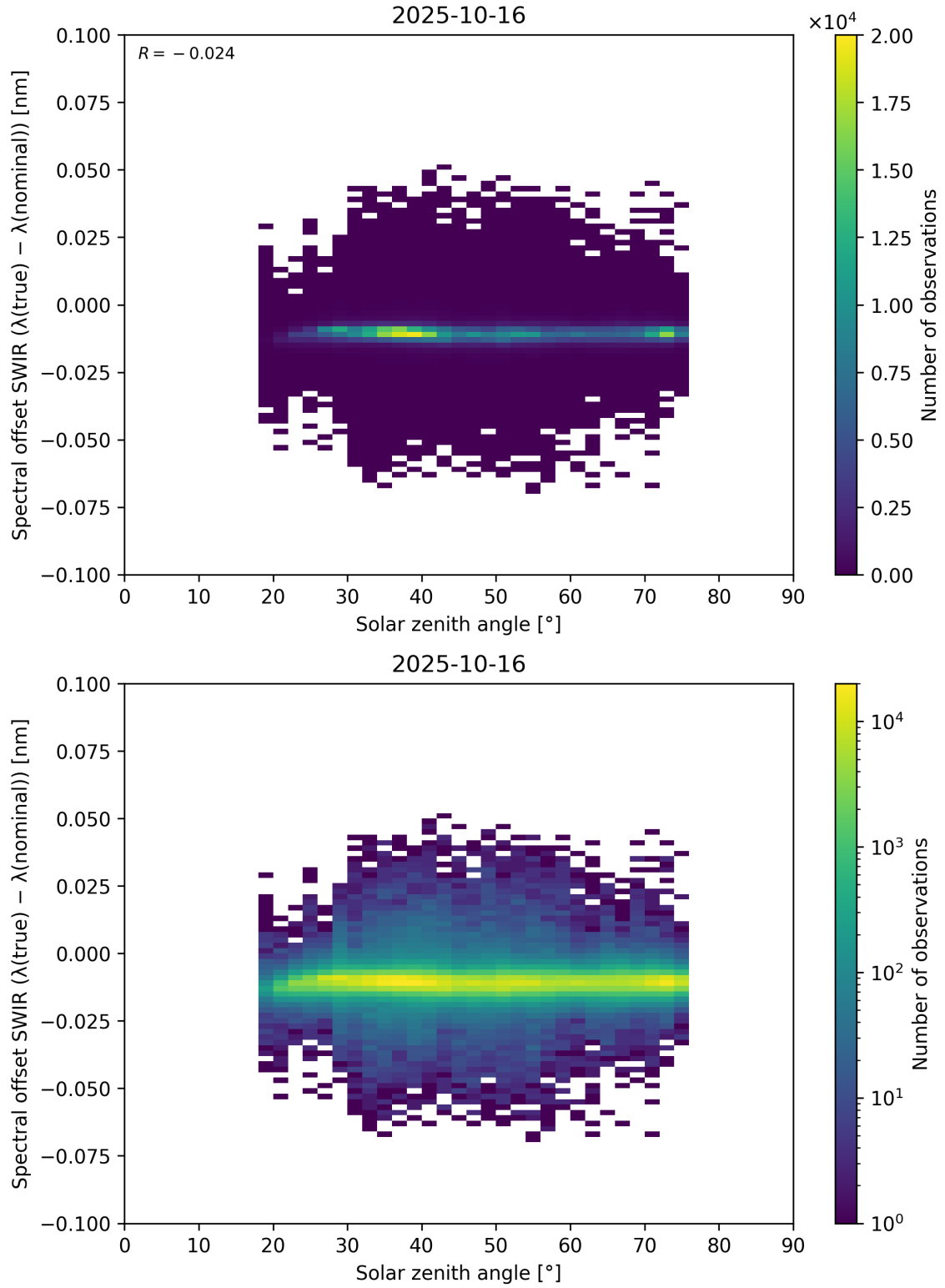
Figure 104: Scatter density plot of “Solar zenith angle” against “Spectral offset SWIR ( \lambda_{\text{true}} - \lambda_{\text{nominal}} )” for 2025-10-15 to 2025-10-17.
