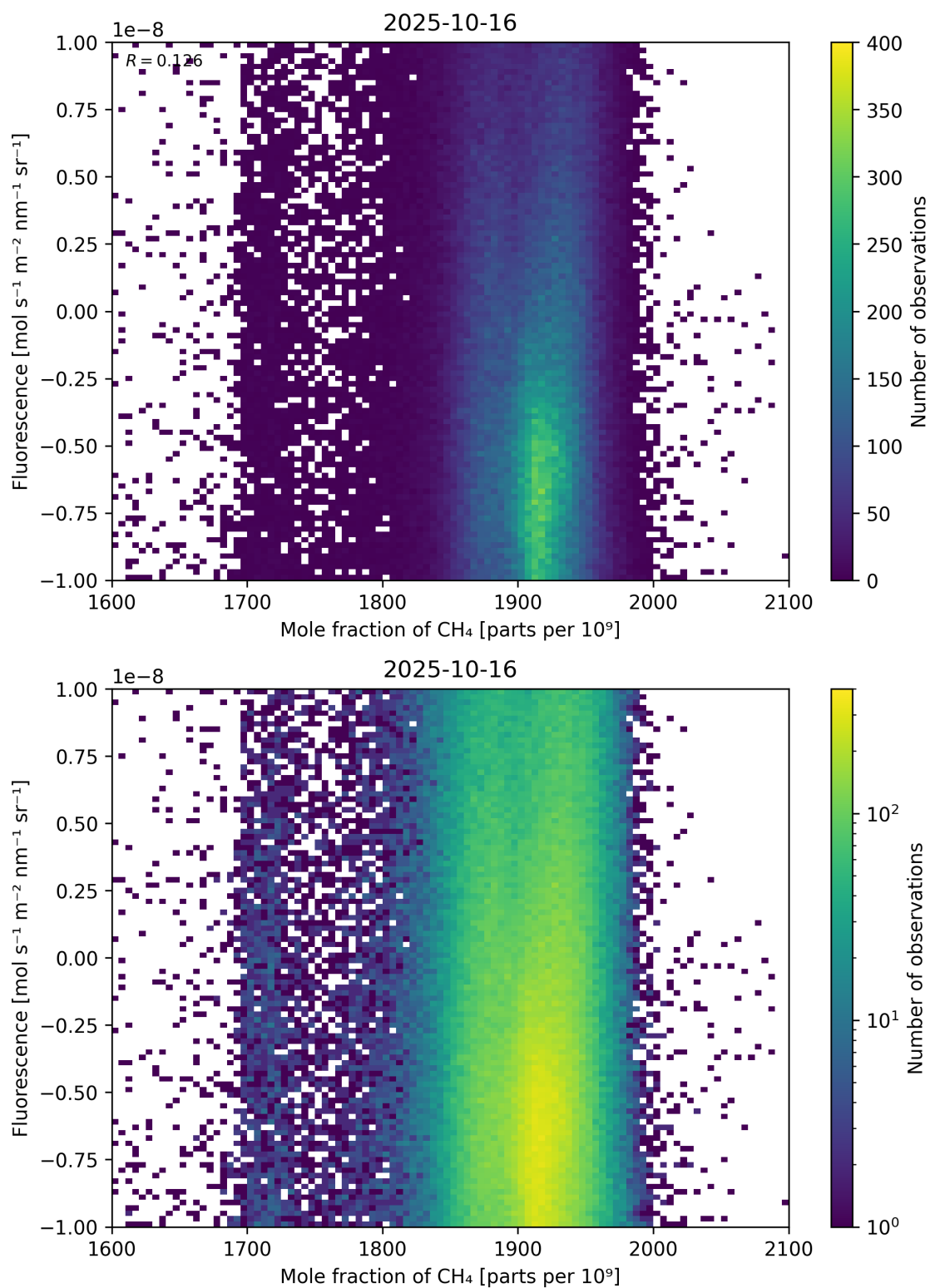
Figure 73: Scatter density plot of “Mole fraction of \text{CH}_4 ” against “Fluorescence” for 2025-10-15 to 2025-10-17.
