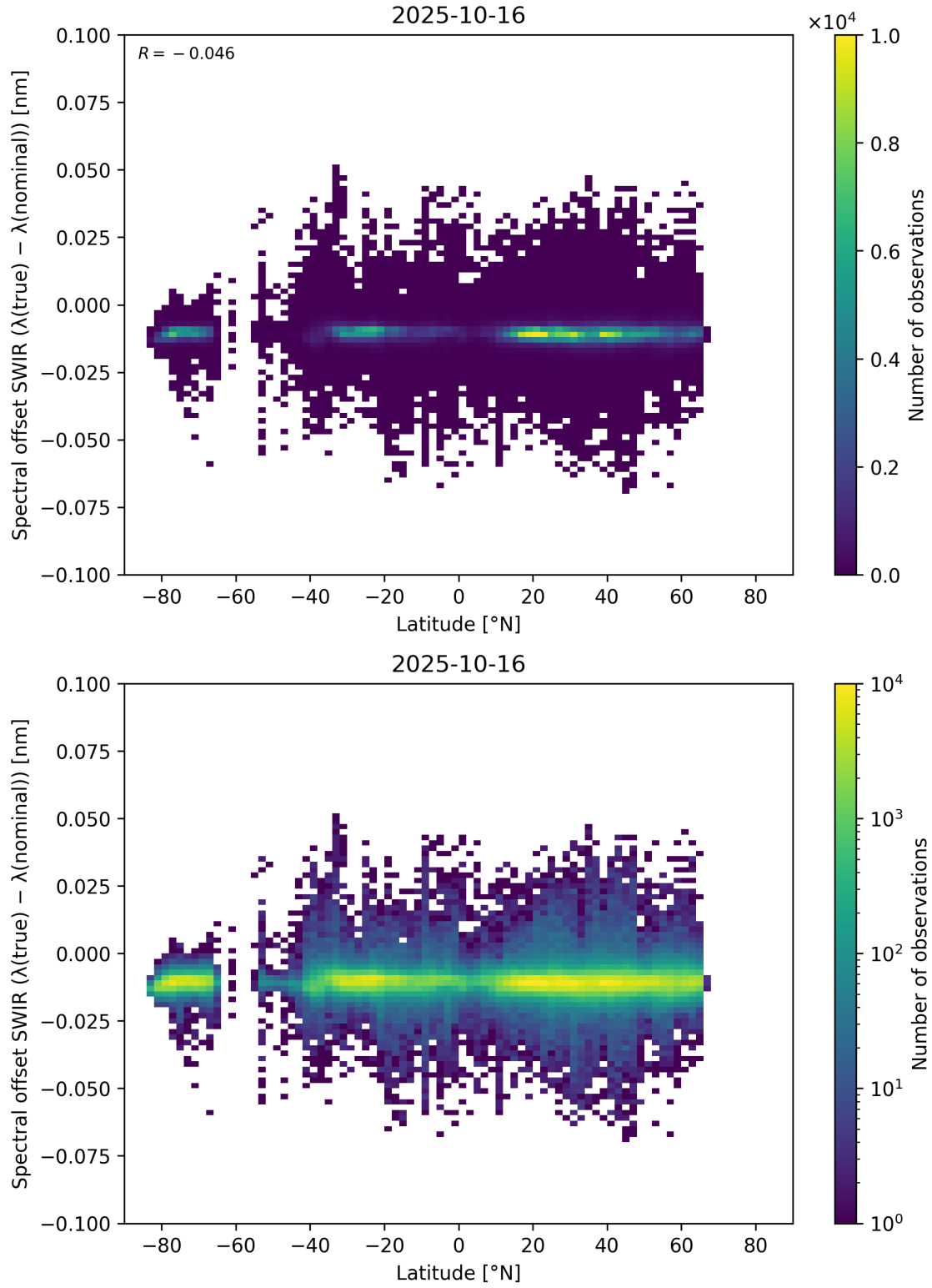
Figure 62: Scatter density plot of “Latitude” against “Spectral offset SWIR ( \lambda_{\text{true}} - \lambda_{\text{nominal}} )” for 2025-10-15 to 2025-10-17.
