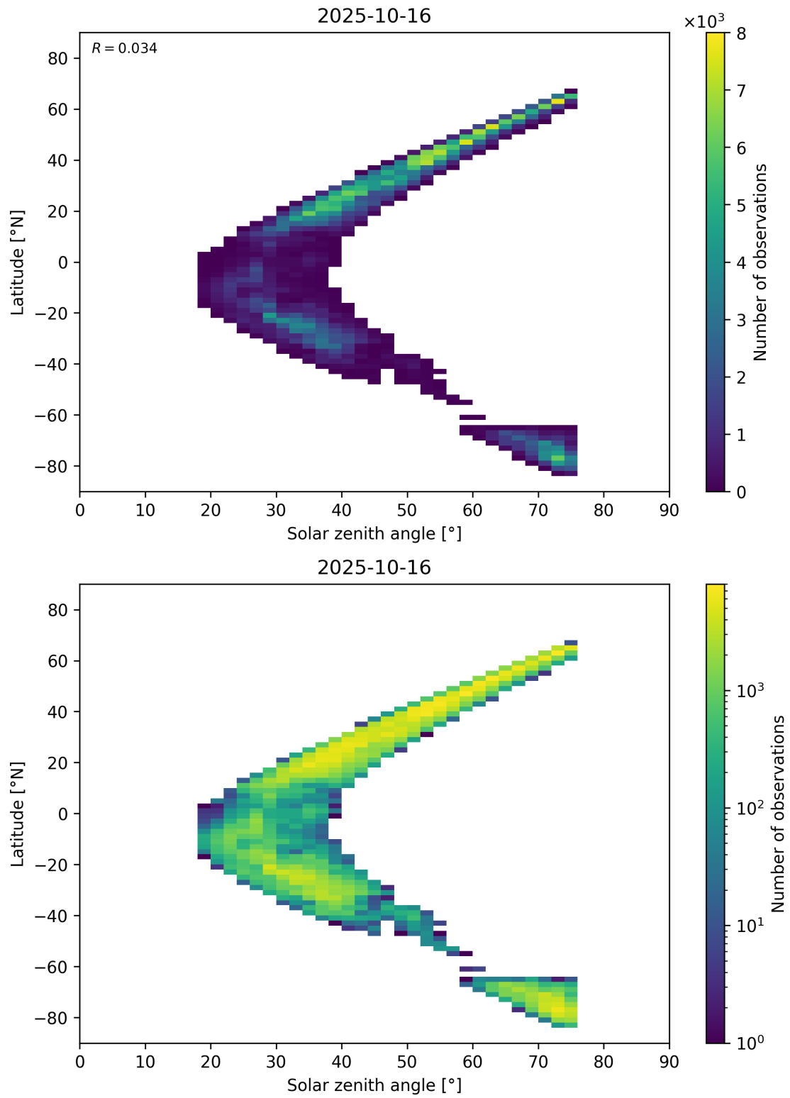
Figure 98: Scatter density plot of “Solar zenith angle” against “Latitude” for 2025-10-15 to 2025-10-17.
