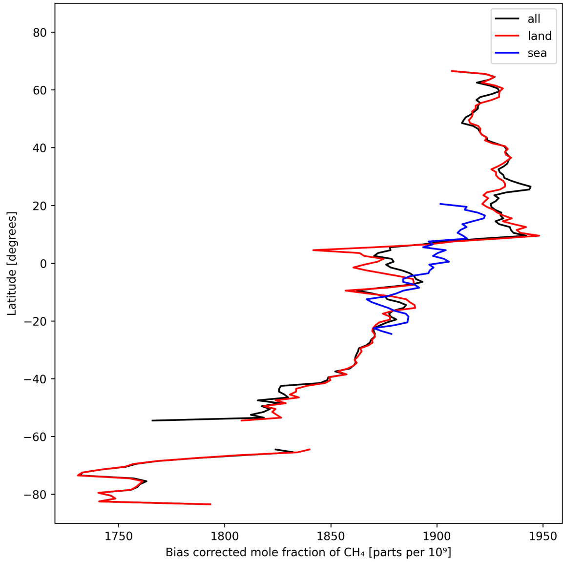
Figure 14: Zonal average of “Bias corrected mole fraction of CH 4 ” for 2025-10-15 to 2025-10-17.
