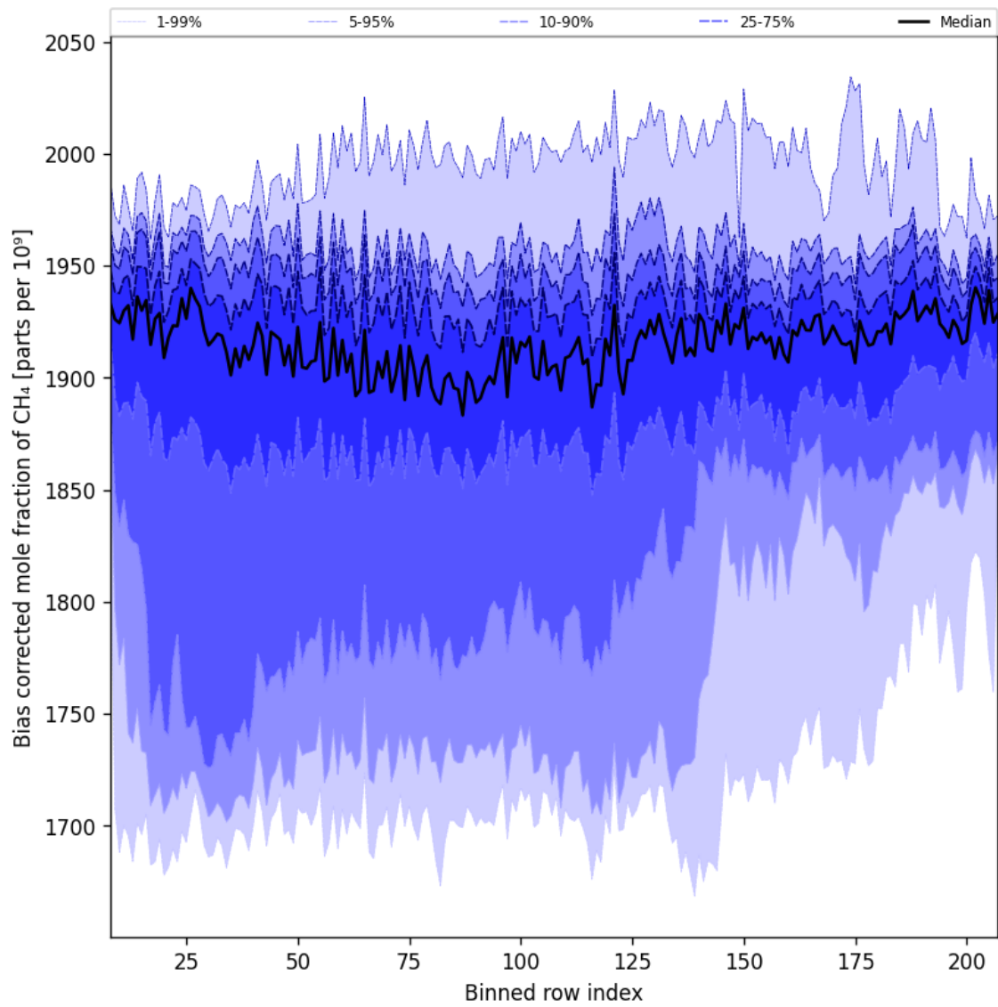
Figure 36: Along track statistics of “Bias corrected mole fraction of CH 4 ” for 2025-10-15 to 2025-10-17
