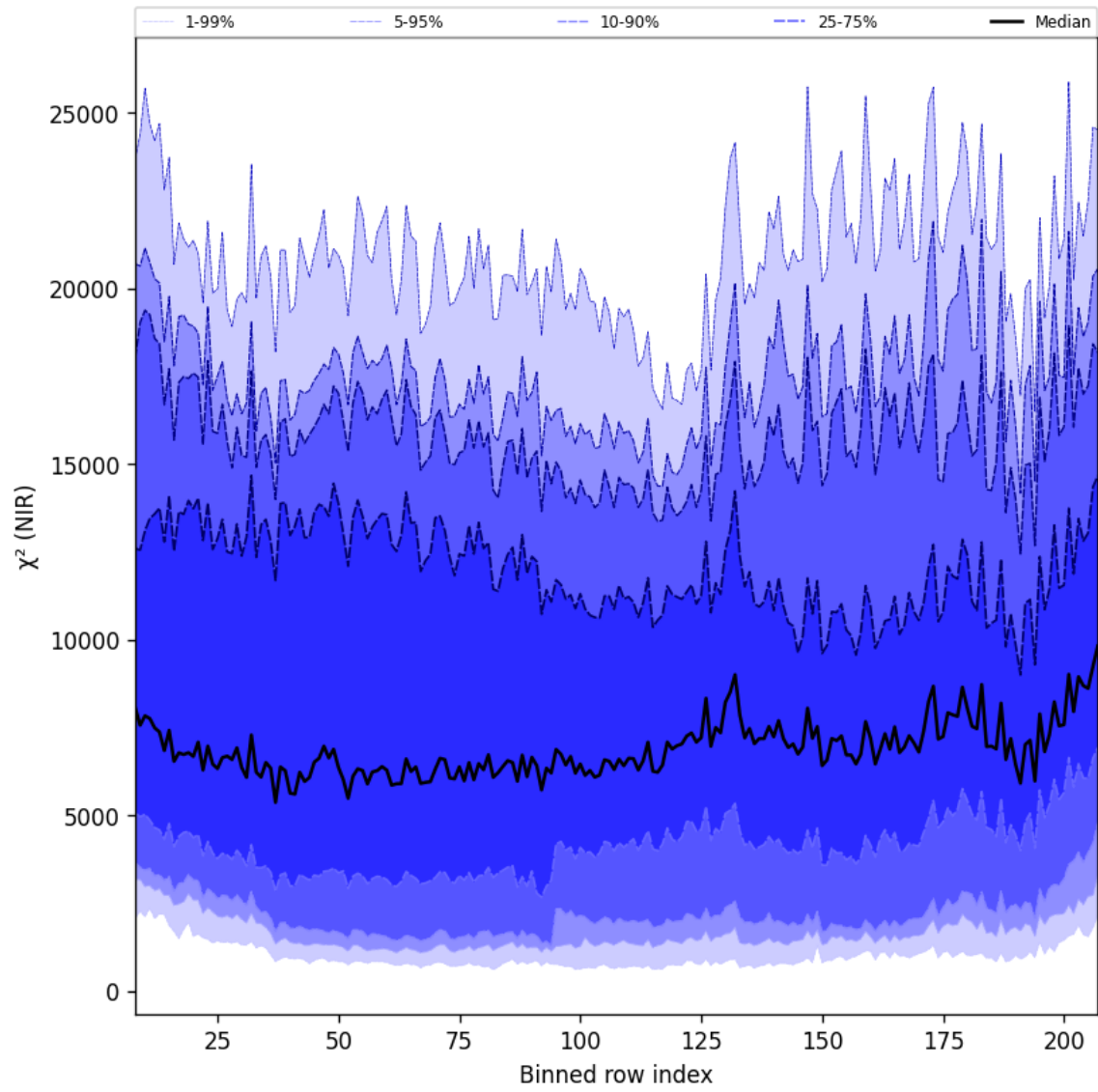
Figure 40: Along track statistics of " \chi^2 (NIR)" for 2025-10-15 to 2025-10-17
