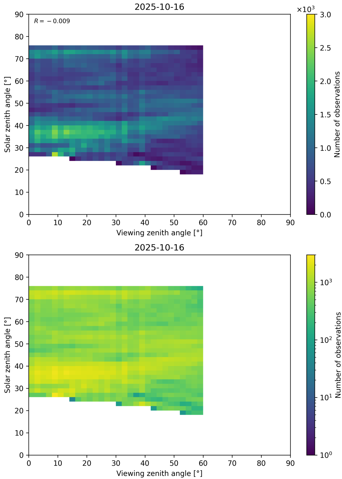
Figure 115: Scatter density plot of “Viewing zenith angle” against “Solar zenith angle” for 2025-10-15 to 2025-10-17.
