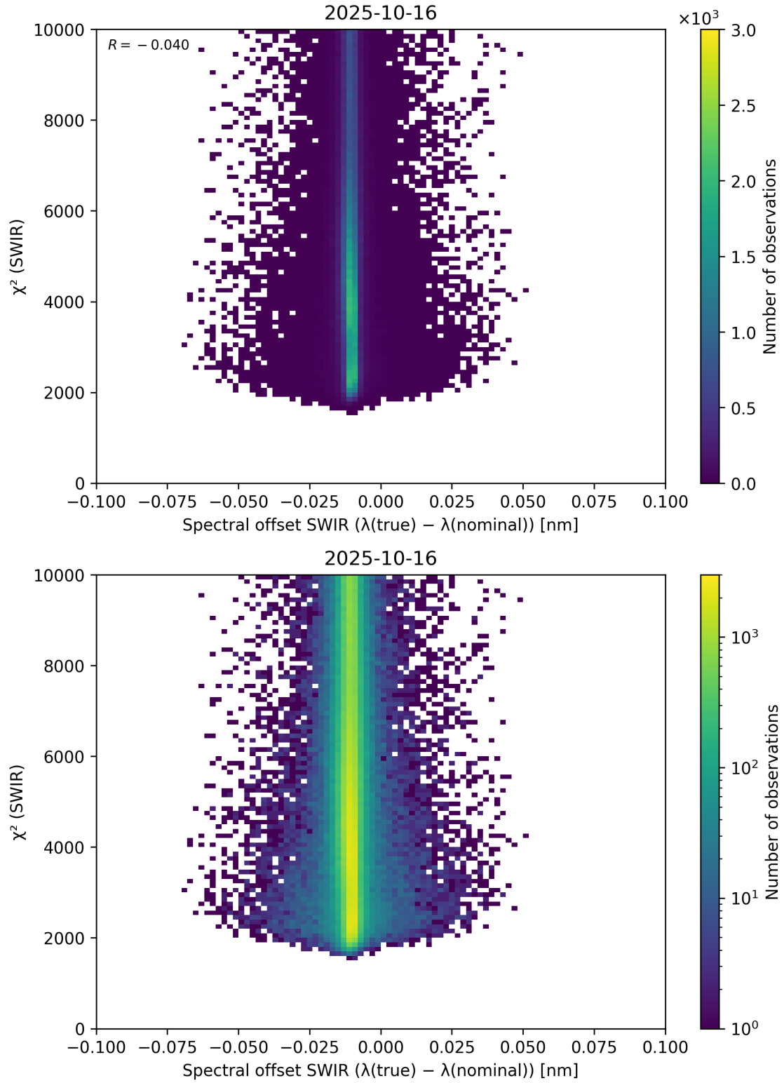
Figure 118: Scatter density plot of “Spectral offset SWIR ( \lambda_{\text{true}} - \lambda_{\text{nominal}} )” against “ \chi^2 (SWIR)” for 2025-10-15 to 2025-10-17.
