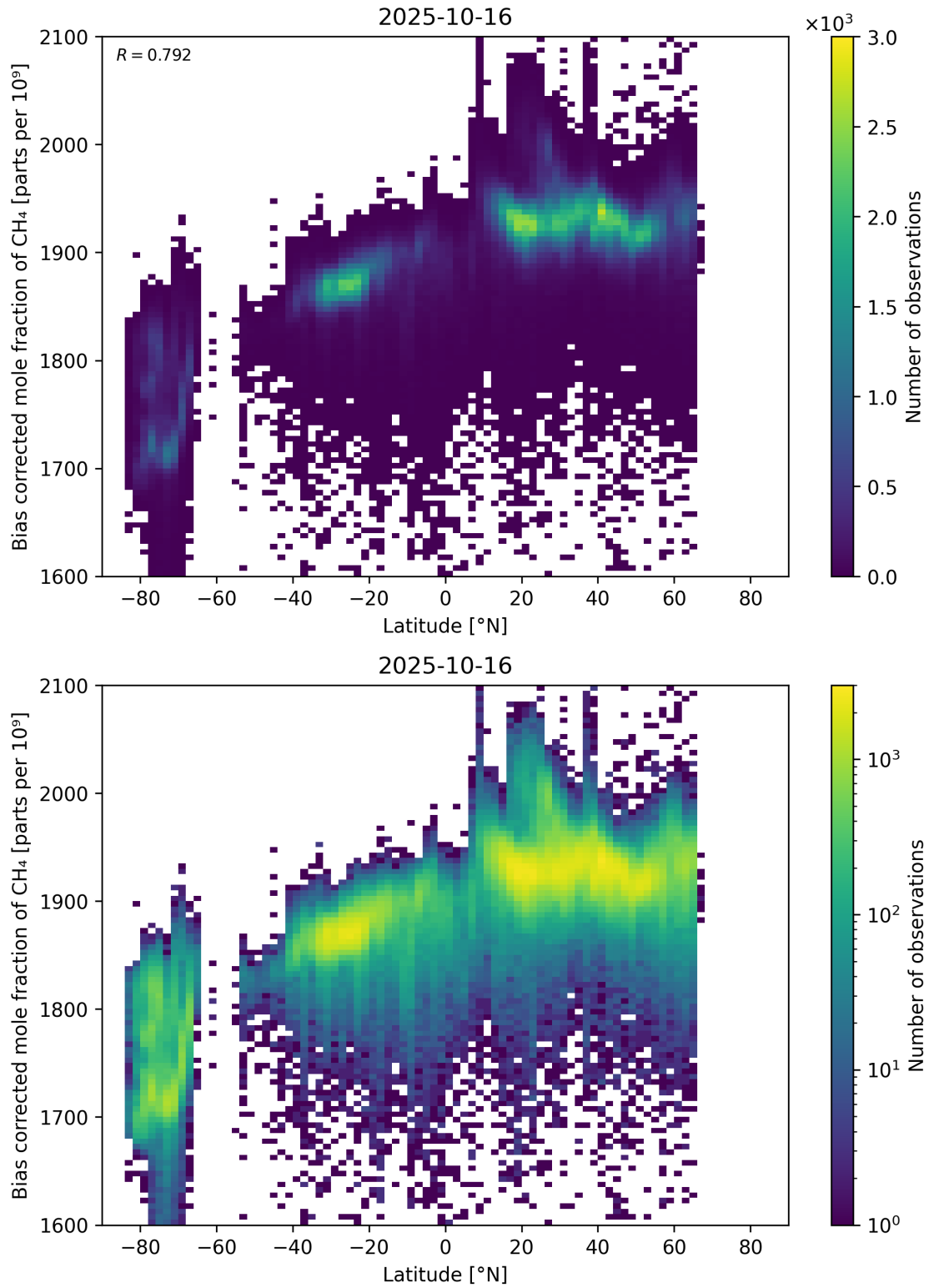
Figure 58: Scatter density plot of “Latitude” against “Bias corrected mole fraction of \text{CH}_4 ” for 2025-10-15 to 2025-10-17.
