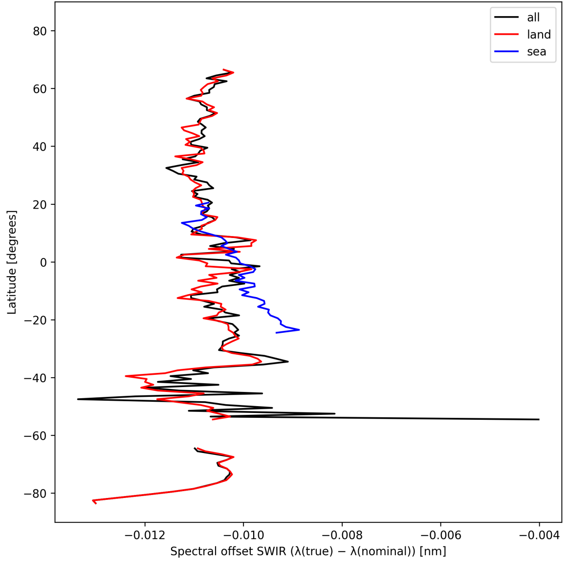
Figure 16: Zonal average of “Spectral offset SWIR ( \lambda_{\text{true}} - \lambda_{\text{nominal}} )” for 2025-10-15 to 2025-10-17.
