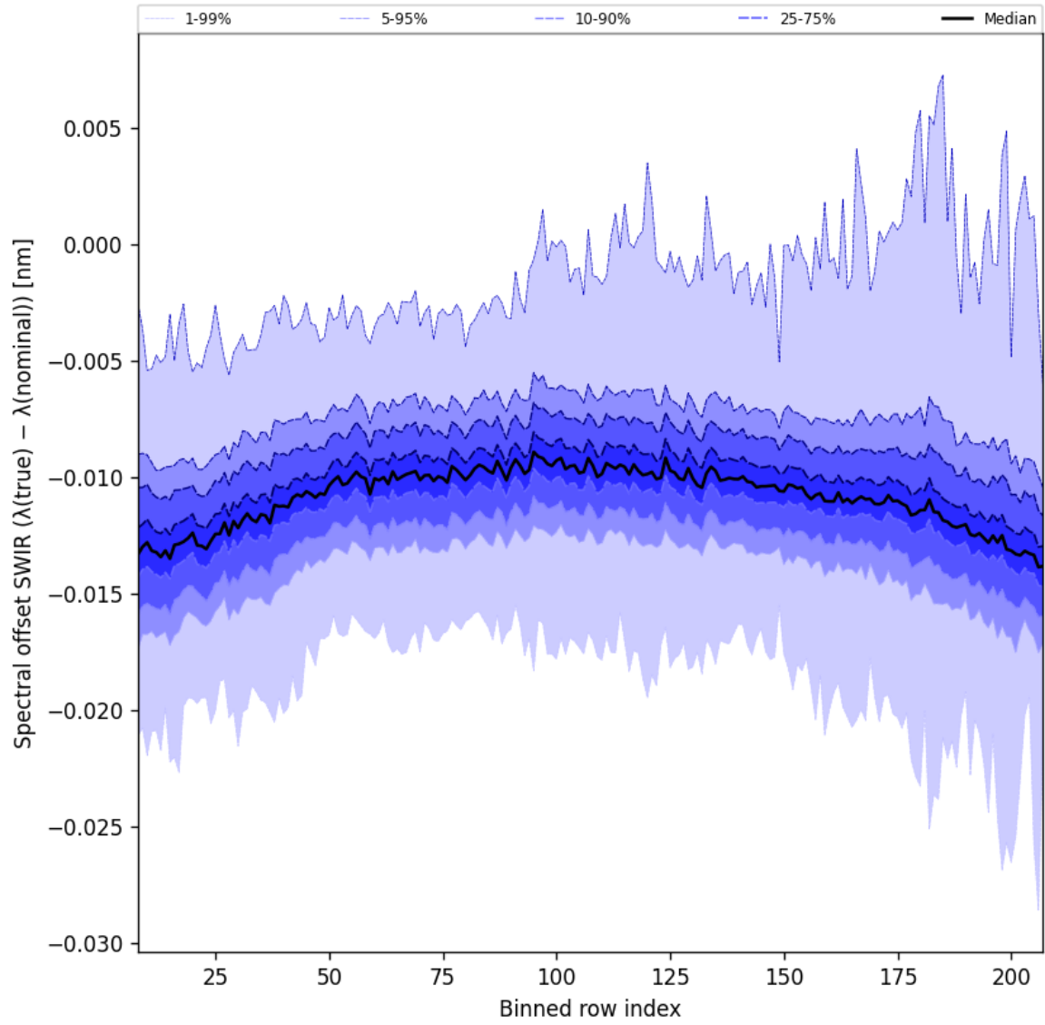
Figure 38: Along track statistics of “Spectral offset SWIR ( \lambda_{\text{true}} - \lambda_{\text{nominal}} )” for 2025-10-15 to 2025-10-17
