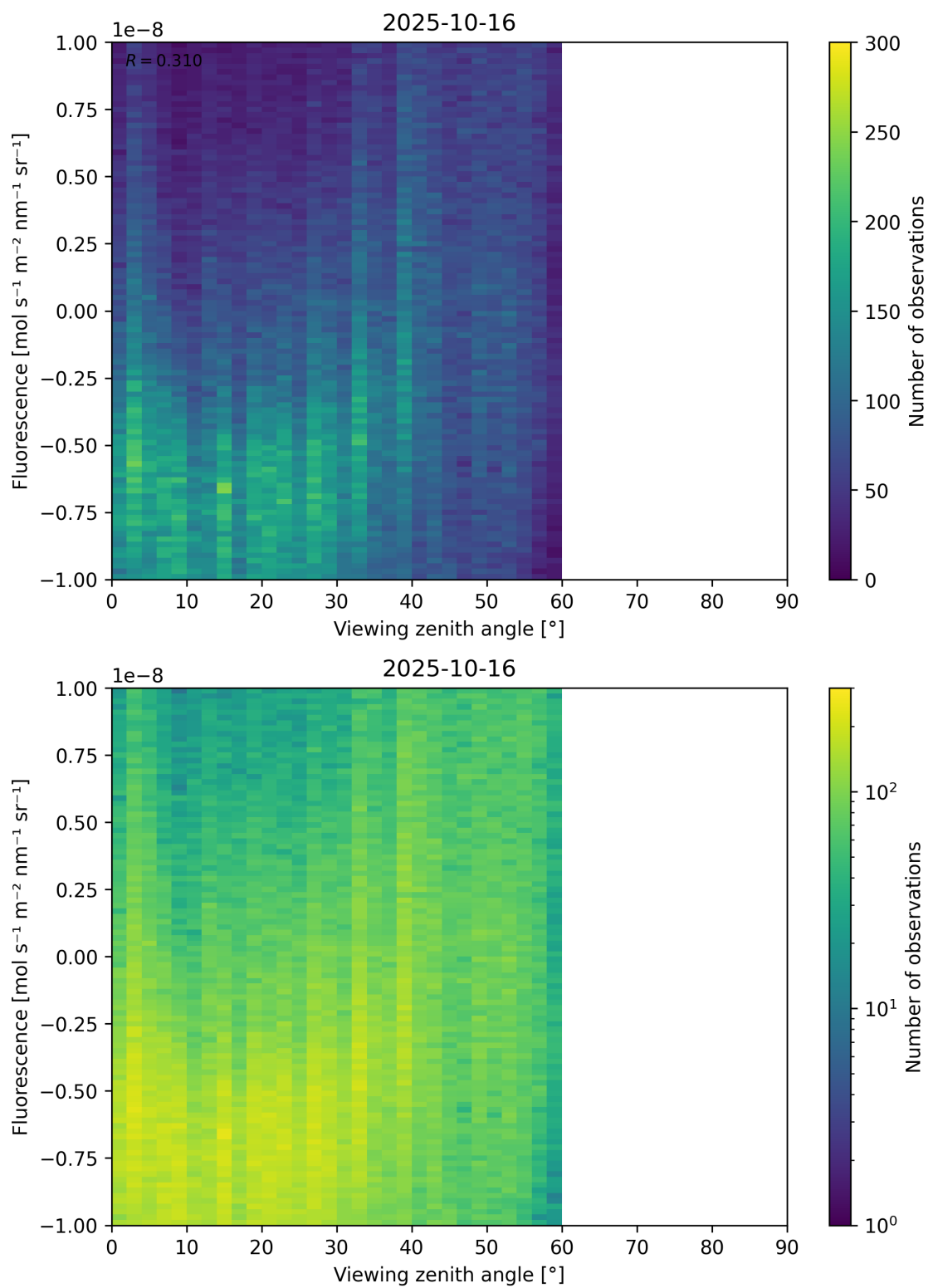
Figure 108: Scatter density plot of “Viewing zenith angle” against “Fluorescence” for 2025-10-15 to 2025-10-17.
