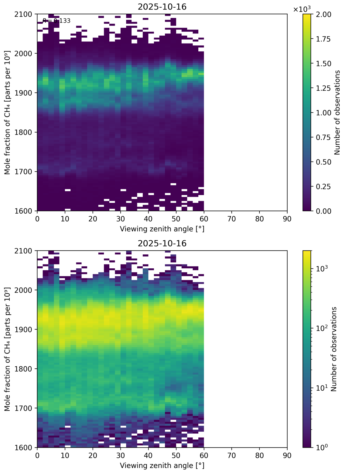
Figure 110: Scatter density plot of “Viewing zenith angle” against “Mole fraction of CH 4 ” for 2025-10-15 to 2025-10-17.
