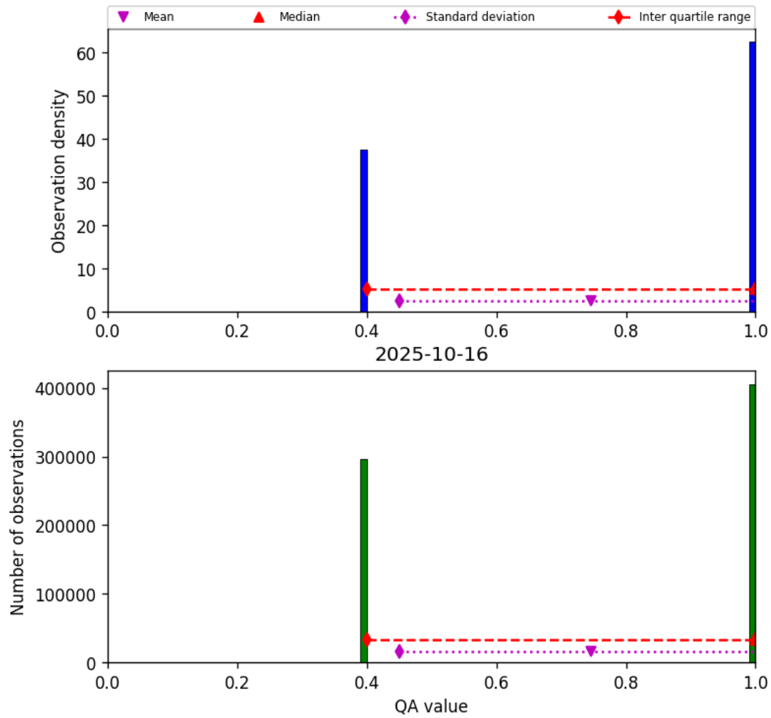
Figure 22: Histogram of “QA value” for 2025-10-15 to 2025-10-17
