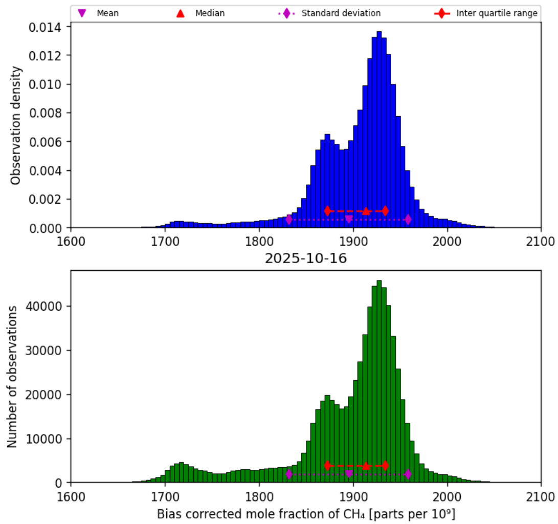
Figure 25: Histogram of “Bias corrected mole fraction of CH 4 ” for 2025-10-15 to 2025-10-17
