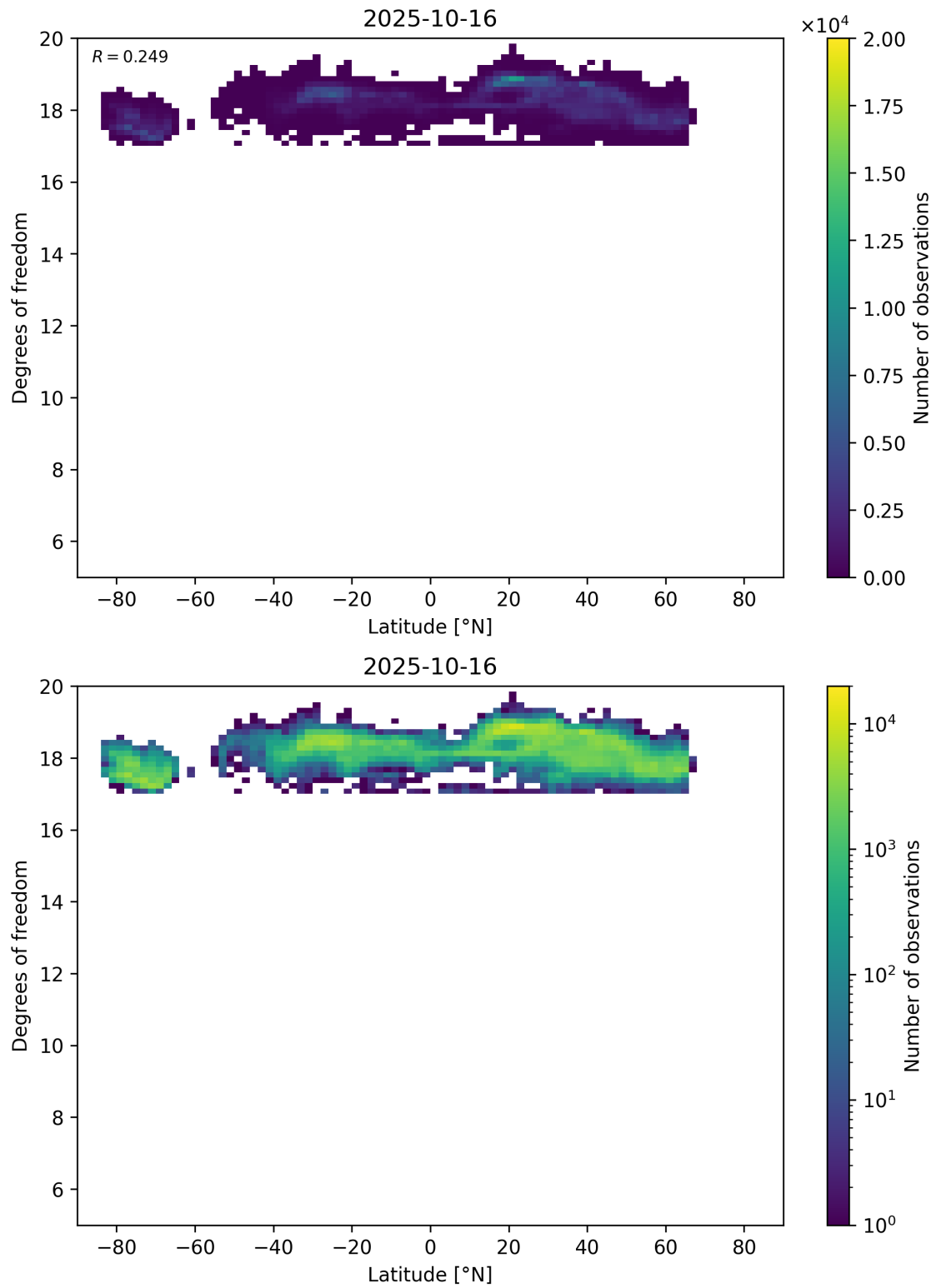
Figure 55: Scatter density plot of “Latitude” against “Degrees of freedom” for 2025-10-15 to 2025-10-17.
