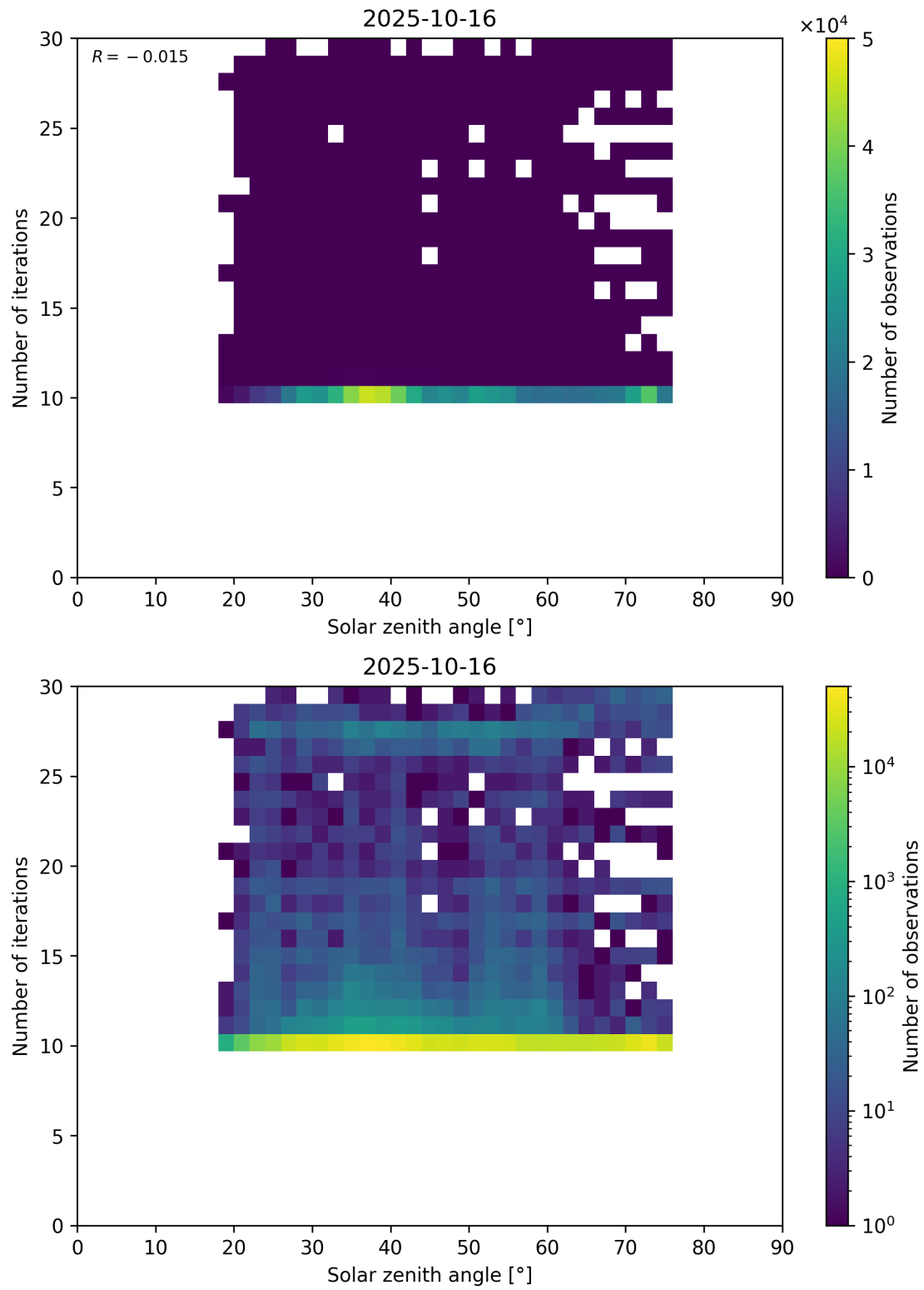
Figure 102: Scatter density plot of “Solar zenith angle” against “Number of iterations” for 2025-10-15 to 2025-10-17.
