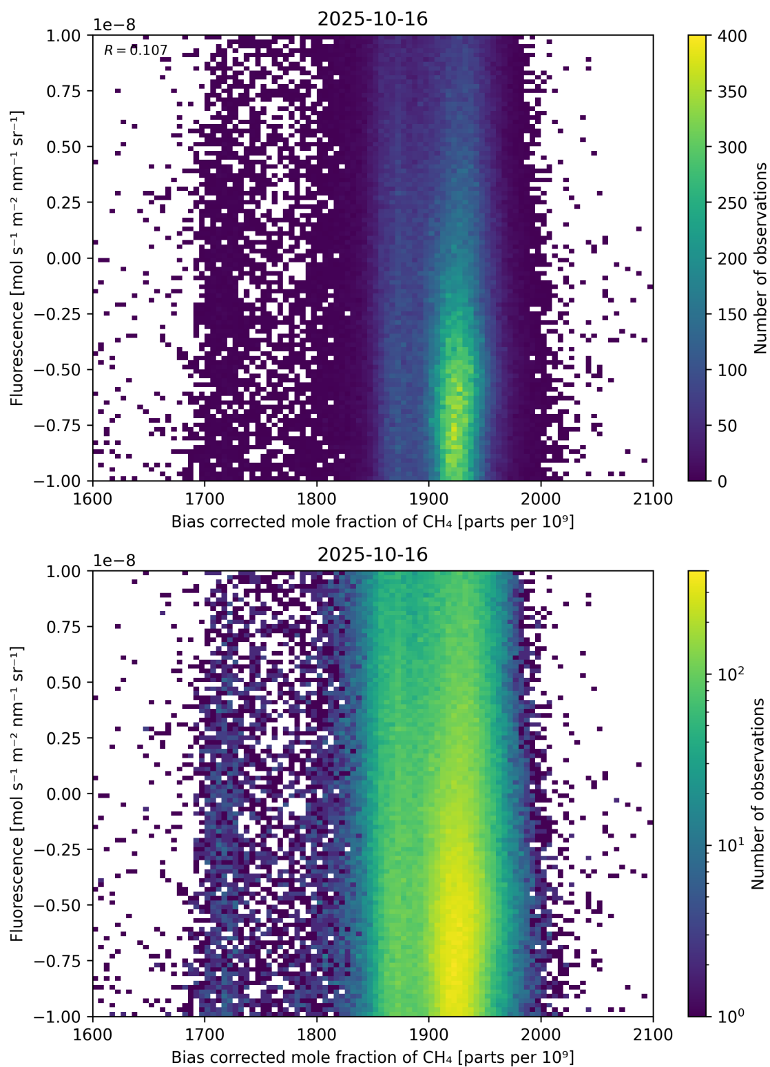
Figure 66: Scatter density plot of “Bias corrected mole fraction of \text{CH}_4 ” against “Fluorescence” for 2025-10-15 to 2025-10-17.
