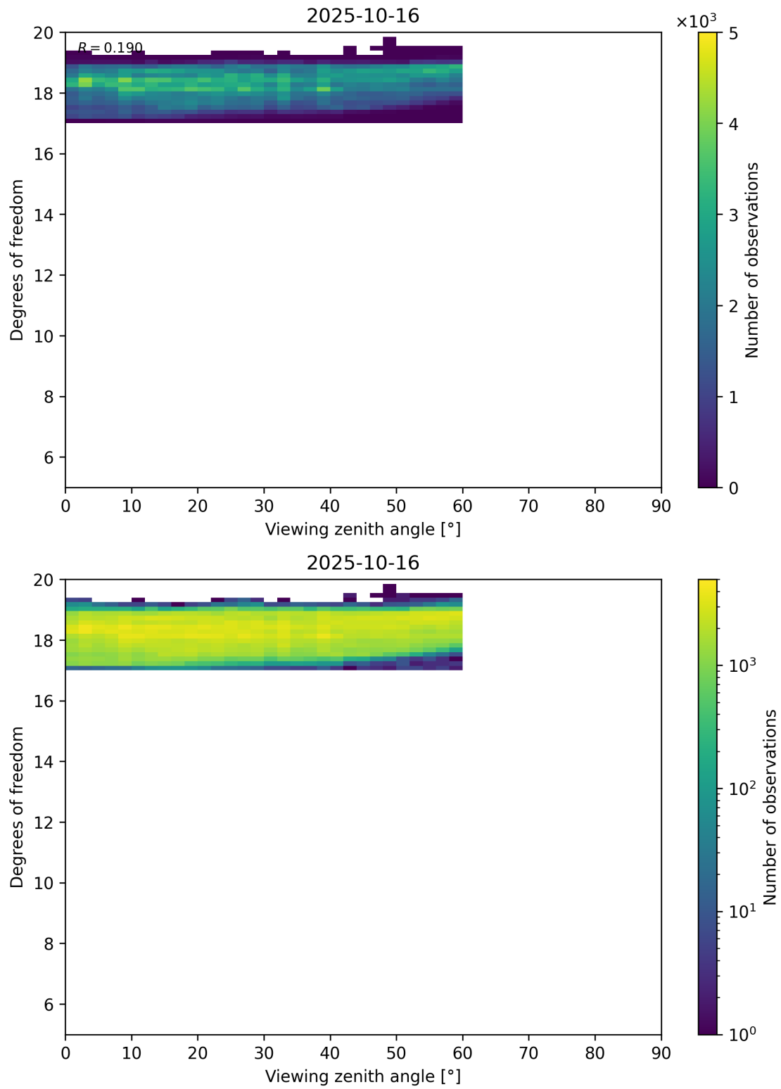
Figure 107: Scatter density plot of “Viewing zenith angle” against “Degrees of freedom” for 2025-10-15 to 2025-10-17.
