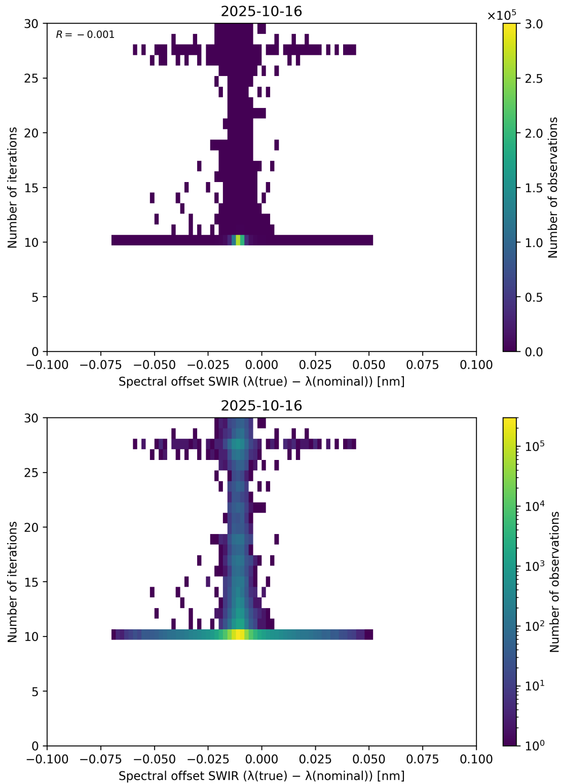
Figure 121: Scatter density plot of “Spectral offset SWIR ( \lambda_{\text{true}} - \lambda_{\text{nominal}} )” against “Number of iterations” for 2025-10-15 to 2025-10-17.
