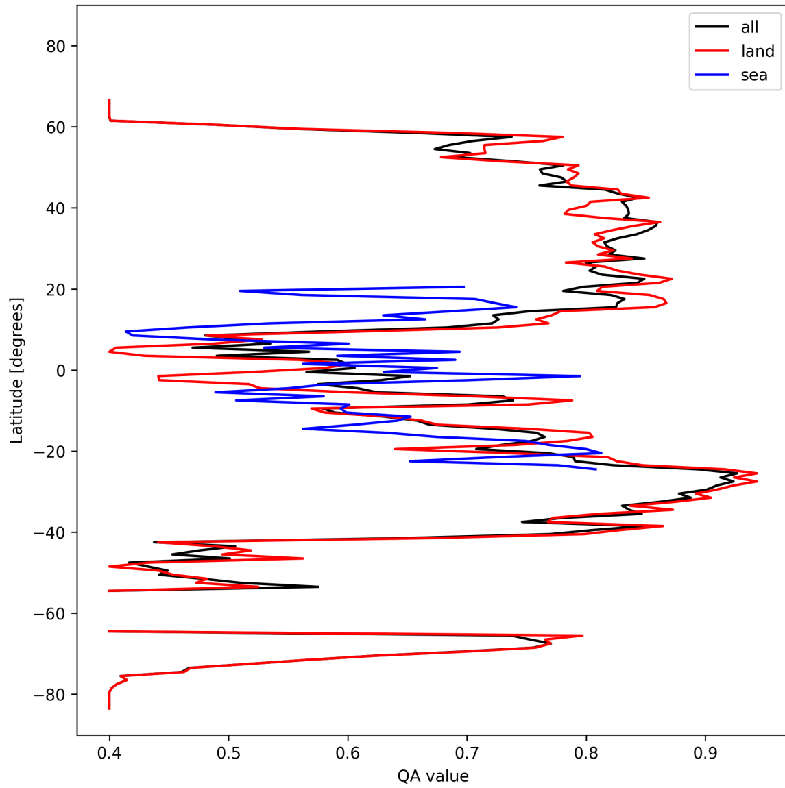
Figure 11: Zonal average of “QA value” for 2025-10-15 to 2025-10-17.
