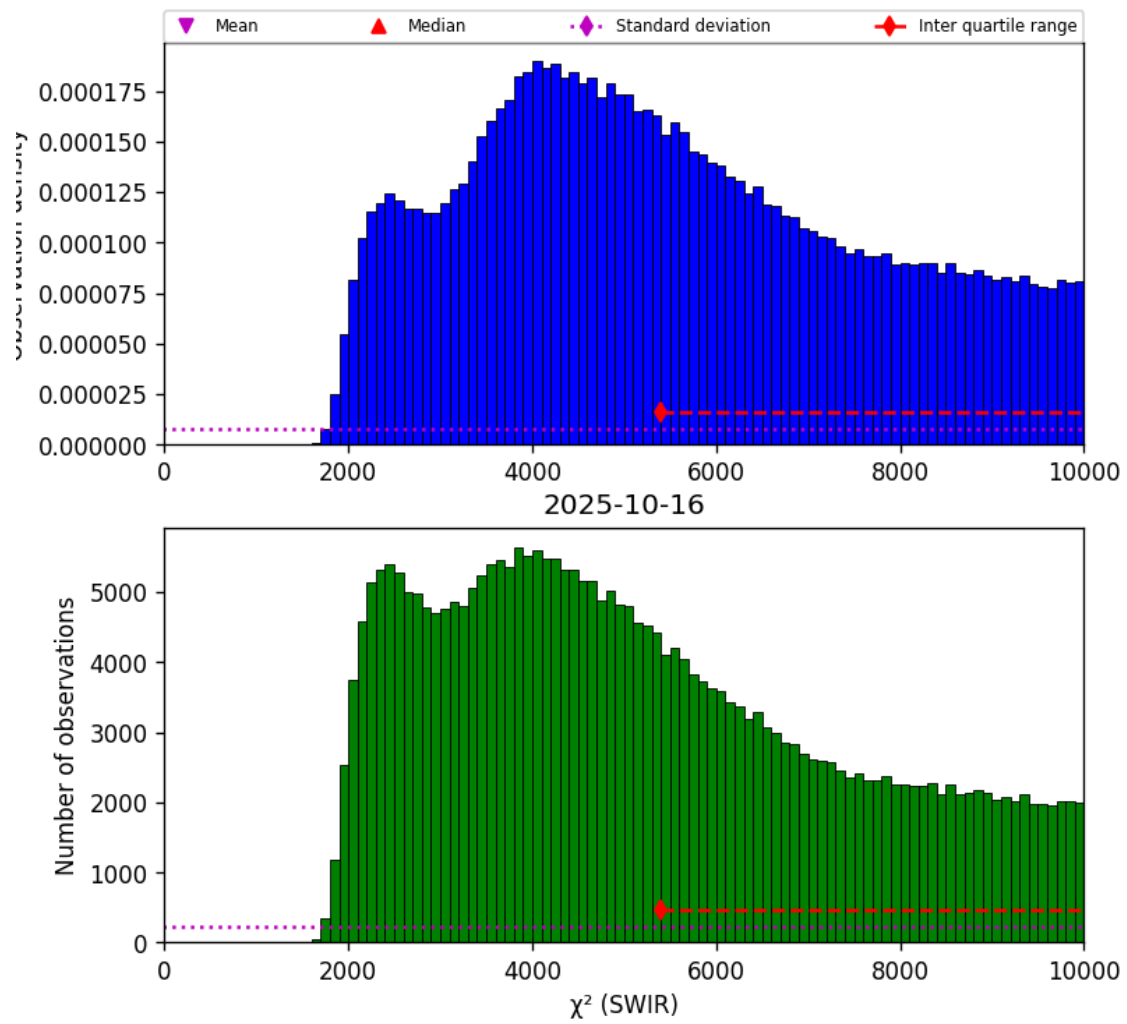
Figure 28: Histogram of “ \chi^2 (SWIR)” for 2025-10-15 to 2025-10-17
