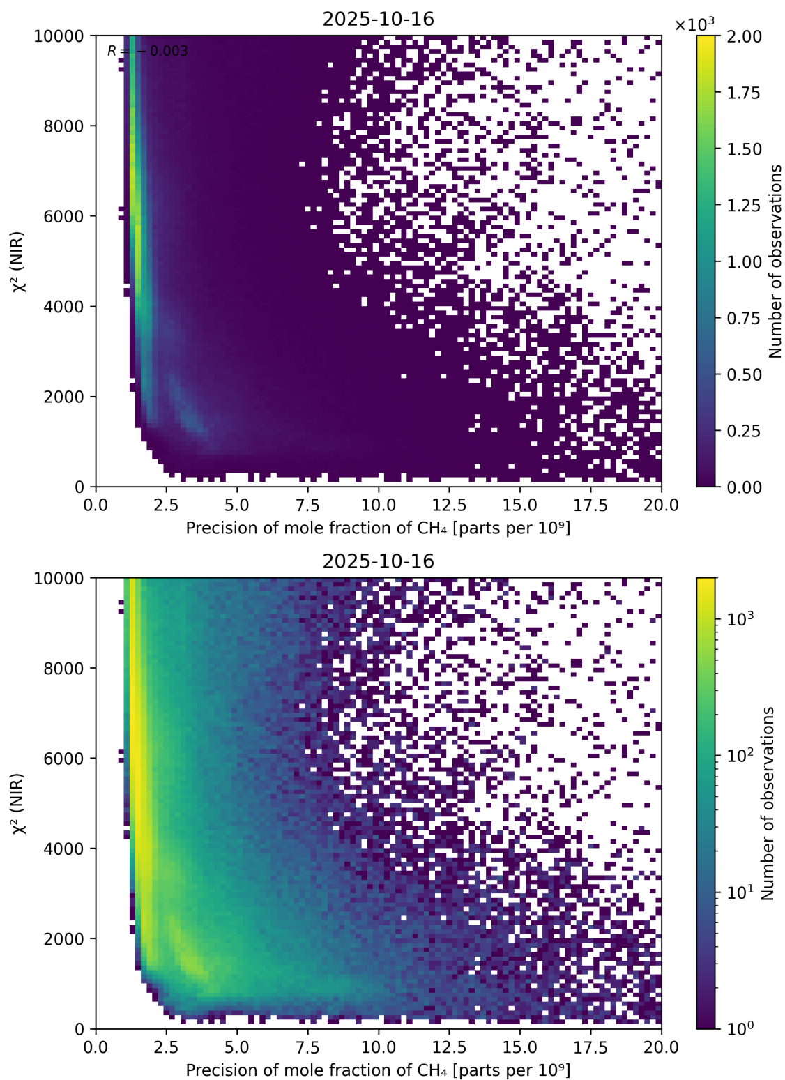
Figure 78: Scatter density plot of “Precision of mole fraction of \text{CH}_4 ” against “ \chi^2 (NIR)” for 2025-10-15 to 2025-10-17.
