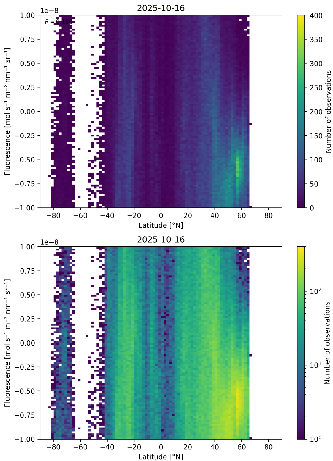
Figure 56: Scatter density plot of “Latitude” against “Fluorescence” for 2025-10-15 to 2025-10-17.
