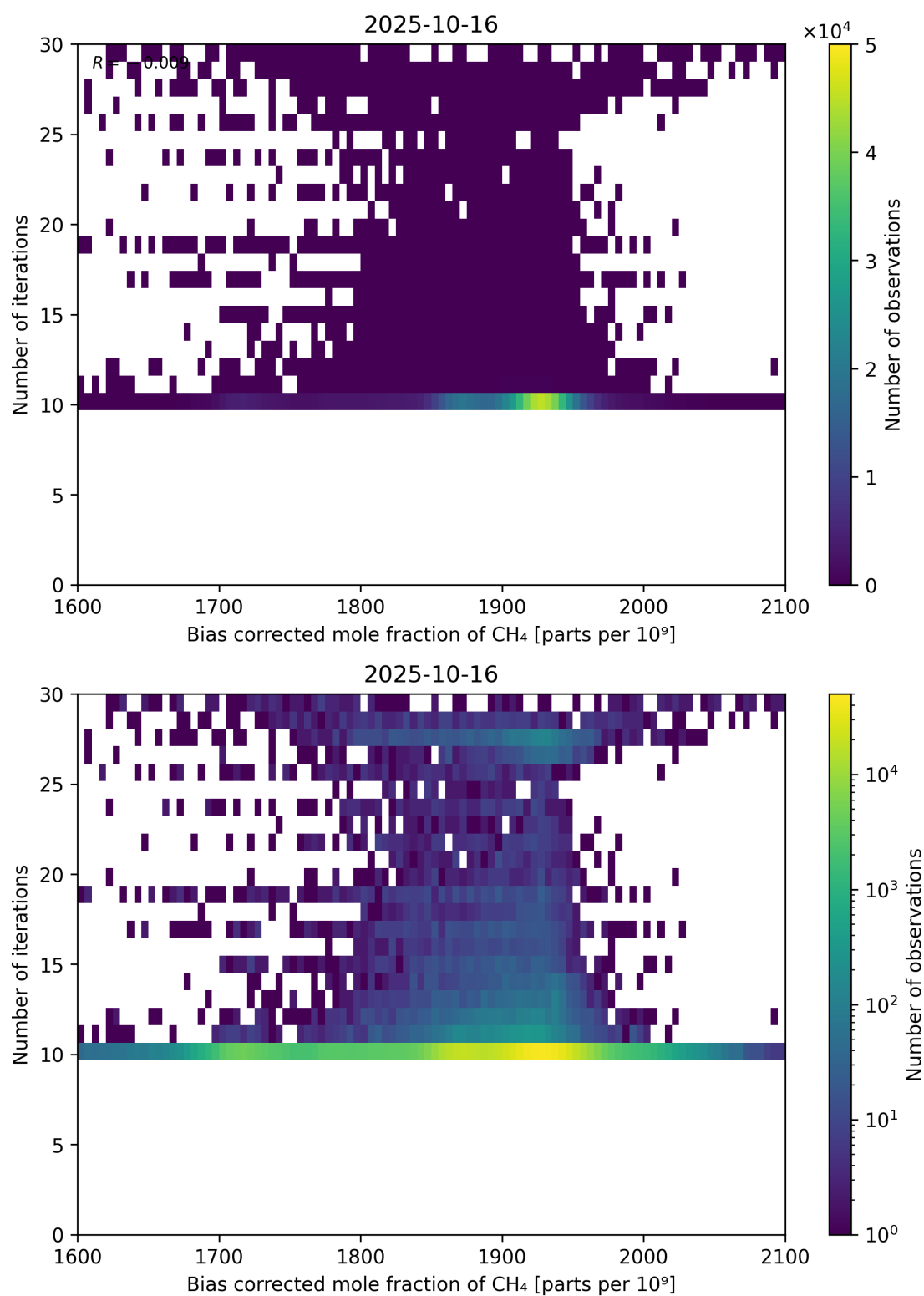
Figure 67: Scatter density plot of “Bias corrected mole fraction of CH 4 ” against “Number of iterations” for 2025-10-15 to 2025-10-17.
