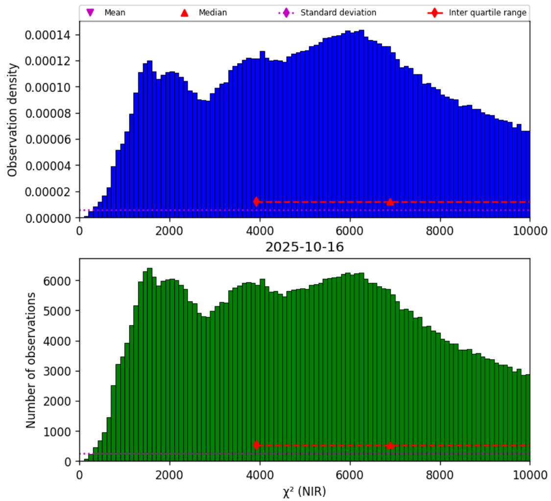
Figure 29: Histogram of “ \chi^2 (NIR)” for 2025-10-15 to 2025-10-17
