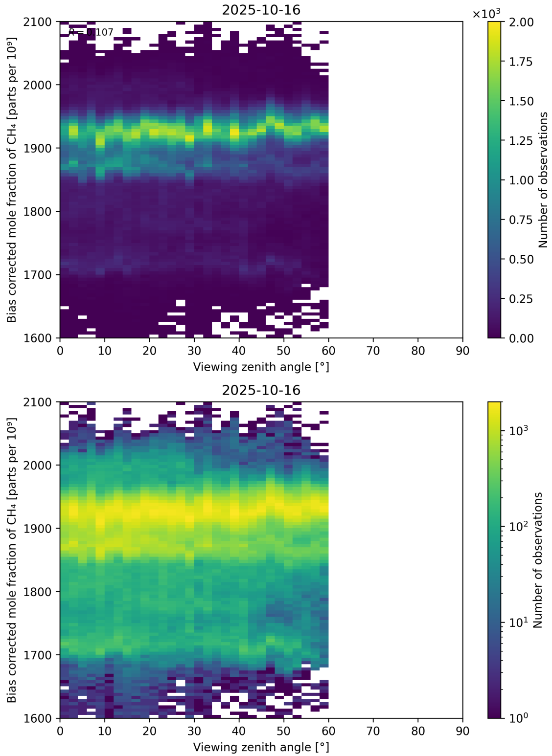
Figure 111: Scatter density plot of “Viewing zenith angle” against “Bias corrected mole fraction of CH 4 ” for 2025-10-15 to 2025-10-17.
