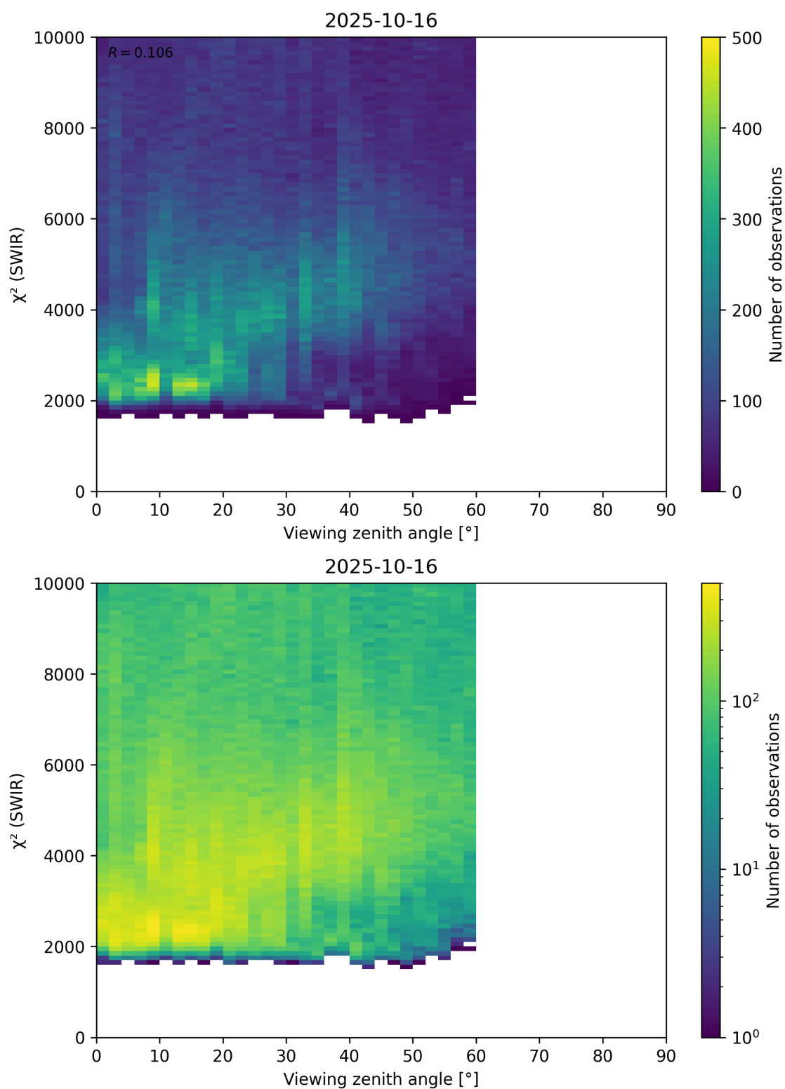
Figure 106: Scatter density plot of “Viewing zenith angle” against “ \chi^2 (SWIR)” for 2025-10-15 to 2025-10-17.
