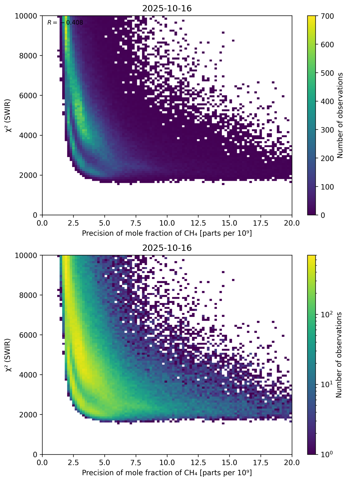
Figure 79: Scatter density plot of “Precision of mole fraction of CH 4 ” against “ \chi^2 (SWIR)” for 2025-10-15 to 2025-10-17.
