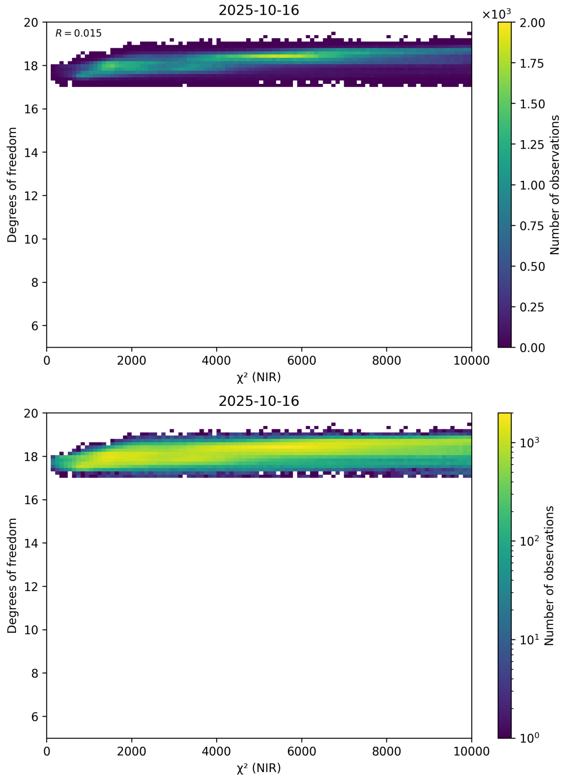
Figure 44: Scatter density plot of “ \chi^2 (NIR)” against “Degrees of freedom” for 2025-10-15 to 2025-10-17.
