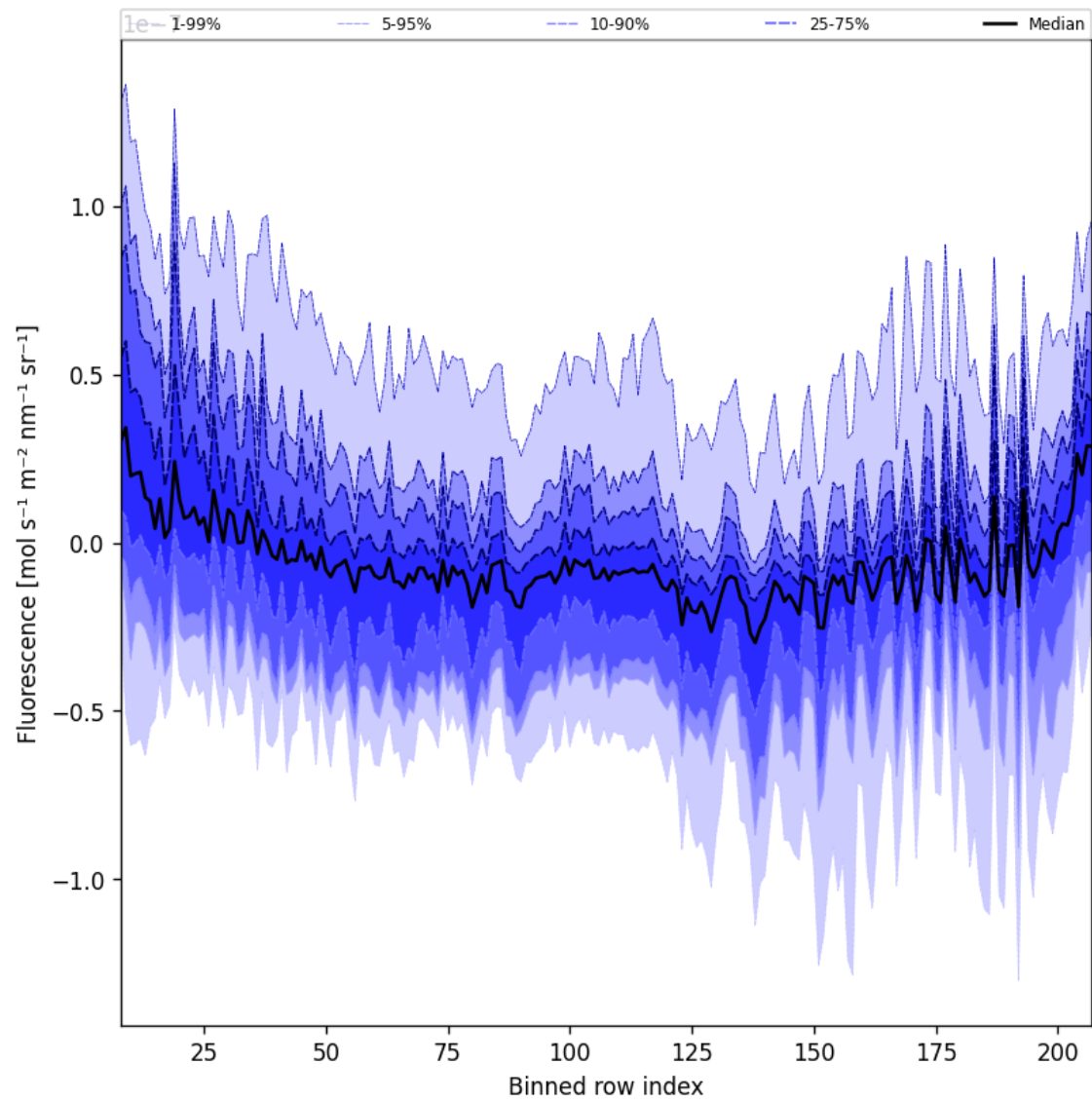
Figure 43: Along track statistics of “Fluorescence” for 2025-10-15 to 2025-10-17
