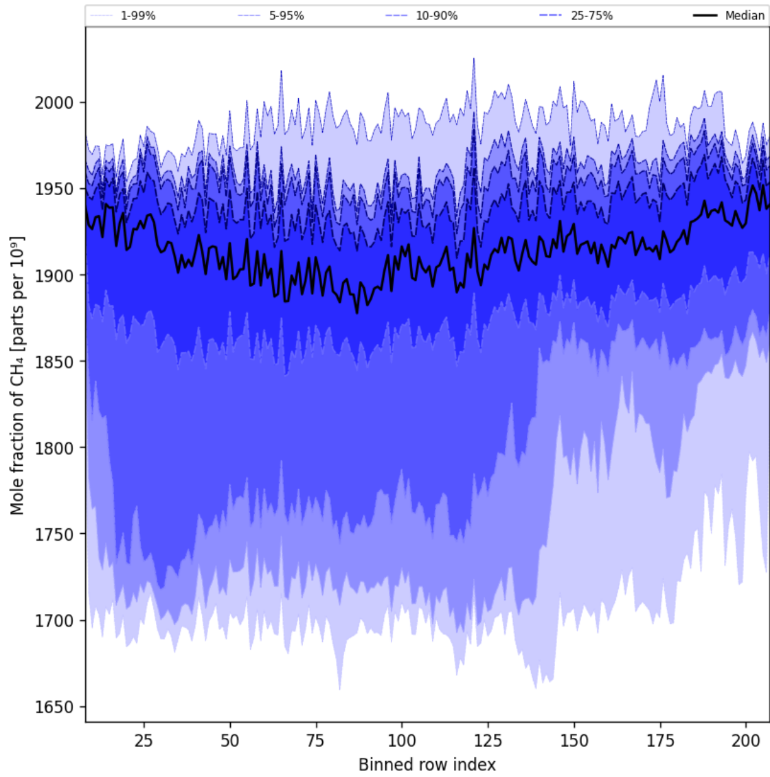
Figure 34: Along track statistics of “Mole fraction of CH 4 ” for 2025-10-15 to 2025-10-17
