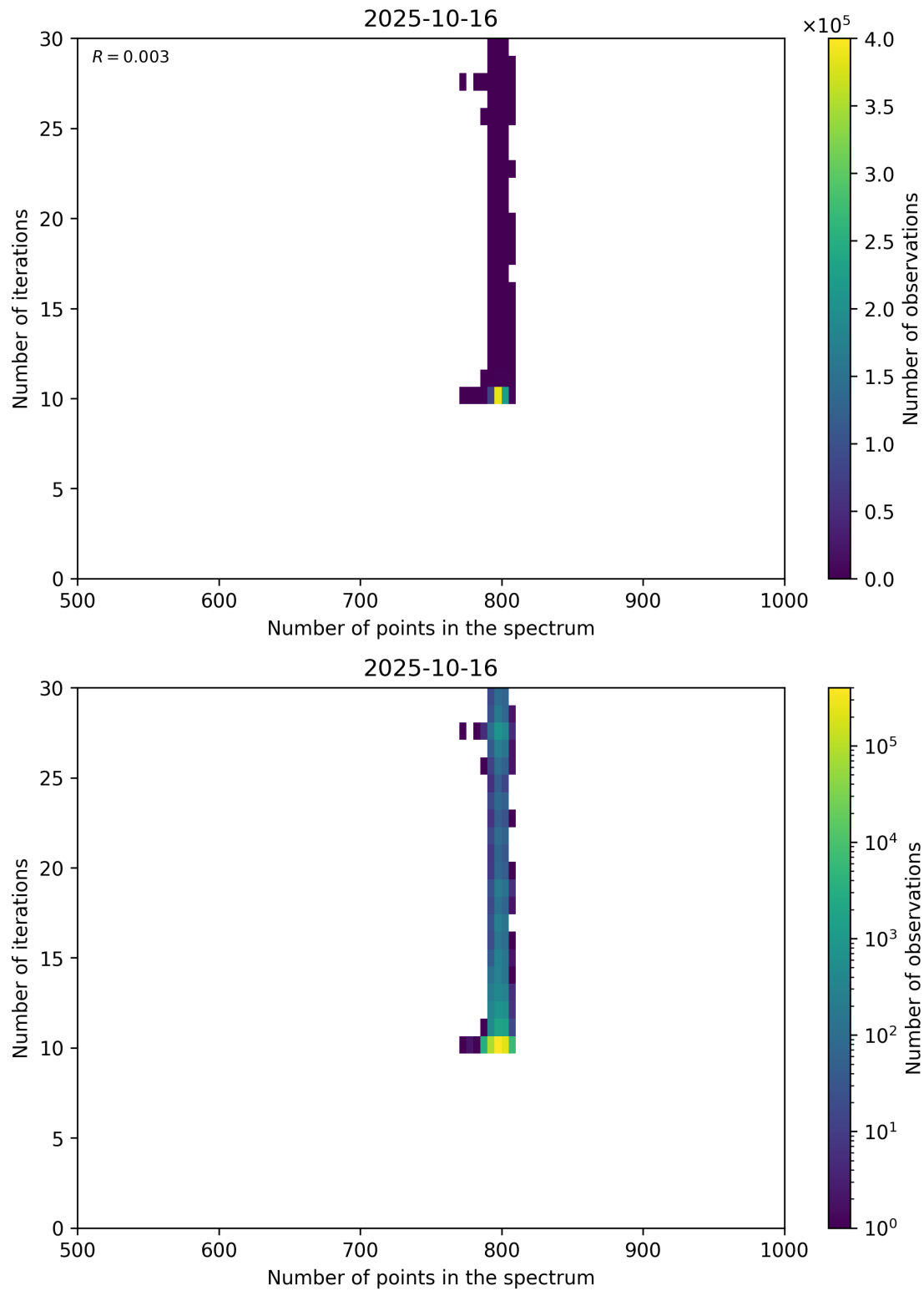
Figure 92: Scatter density plot of “Number of points in the spectrum” against “Number of iterations” for 2025-10-15 to 2025-10-17.
