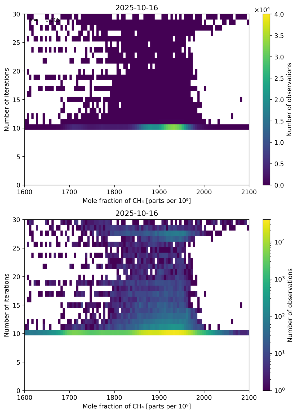
Figure 76: Scatter density plot of “Mole fraction of CH 4 ” against “Number of iterations” for 2025-10-15 to 2025-10-17.
