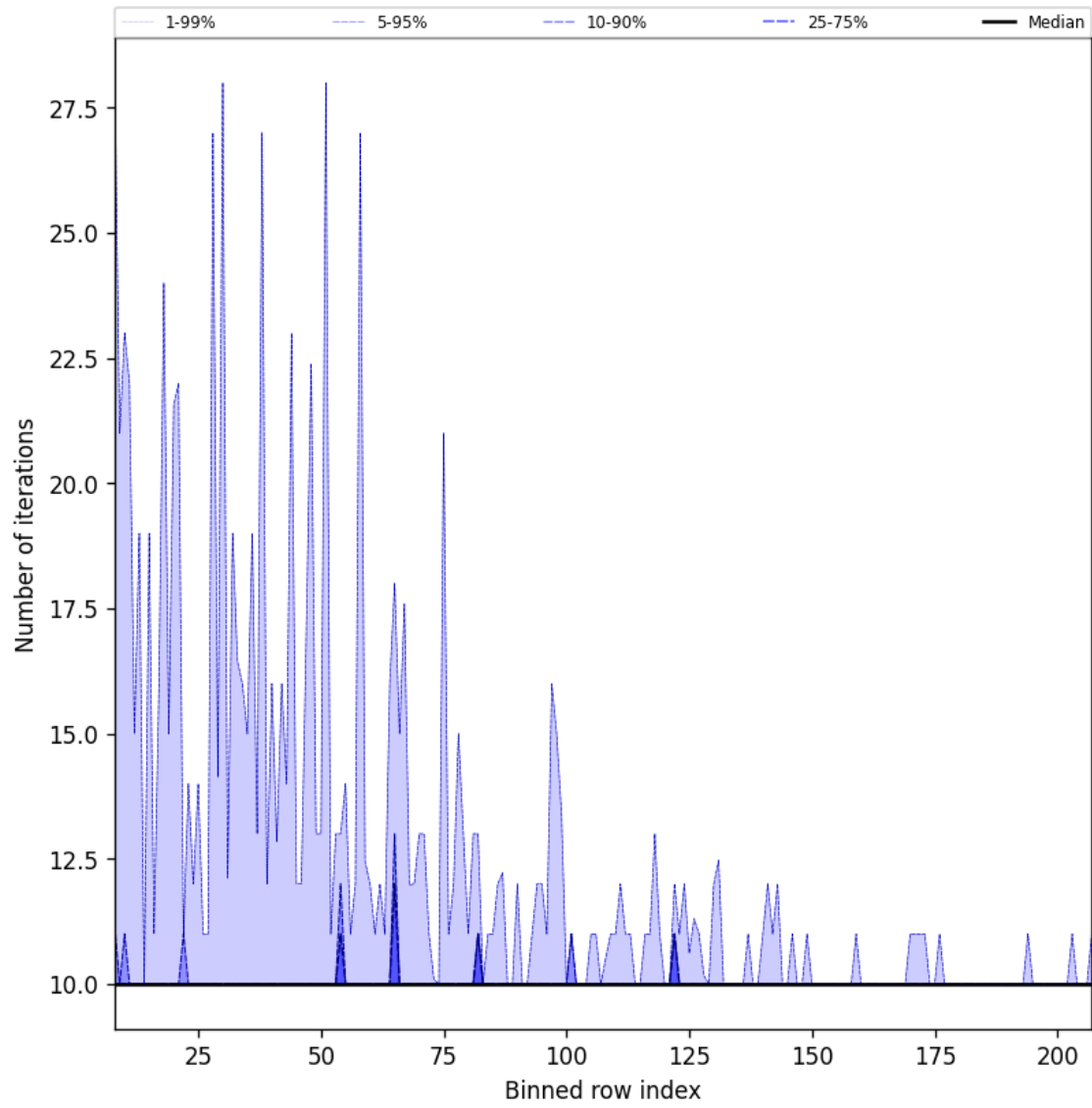
Figure 42: Along track statistics of “Number of iterations” for 2025-10-15 to 2025-10-17
