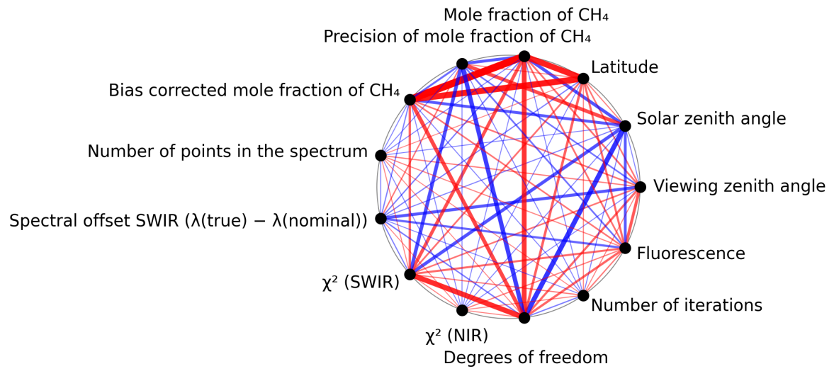
Figure 1: Map of correlation graph for 2025-10-15 to 2025-10-17.
