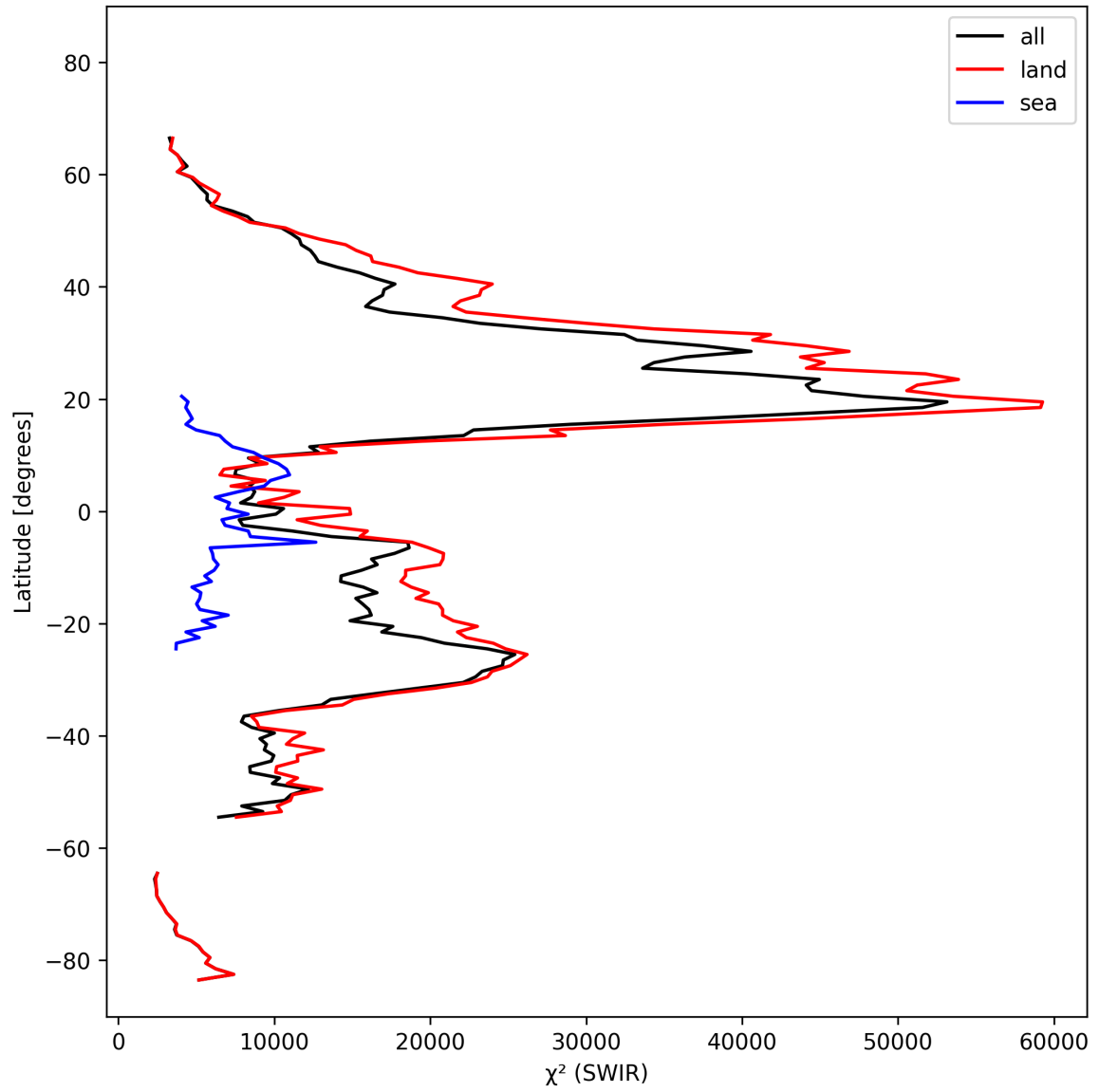
Figure 17: Zonal average of “ \chi^2 (SWIR)” for 2025-10-15 to 2025-10-17.
