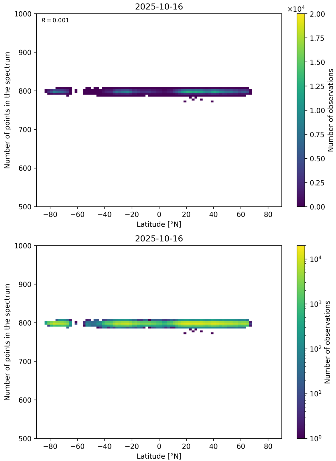
Figure 61: Scatter density plot of “Latitude” against “Number of points in the spectrum” for 2025-10-15 to 2025-10-17.
