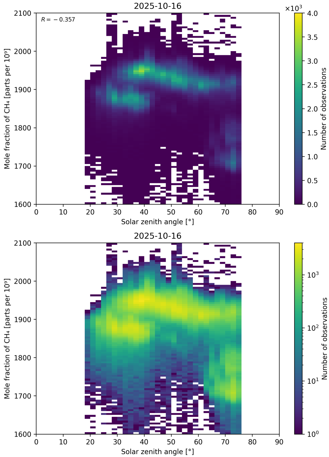
Figure 99: Scatter density plot of “Solar zenith angle” against “Mole fraction of CH 4 ” for 2025-10-15 to 2025-10-17.
