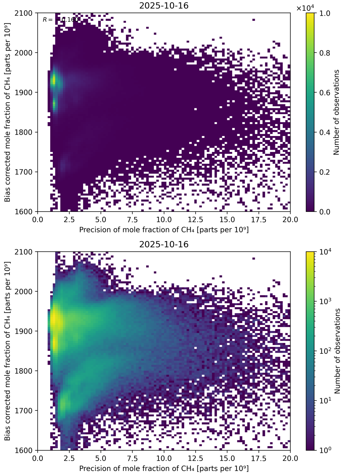
Figure 82: Scatter density plot of “Precision of mole fraction of CH 4 ” against “Bias corrected mole fraction of CH 4 ” for 2025-10-15 to 2025-10-17.
