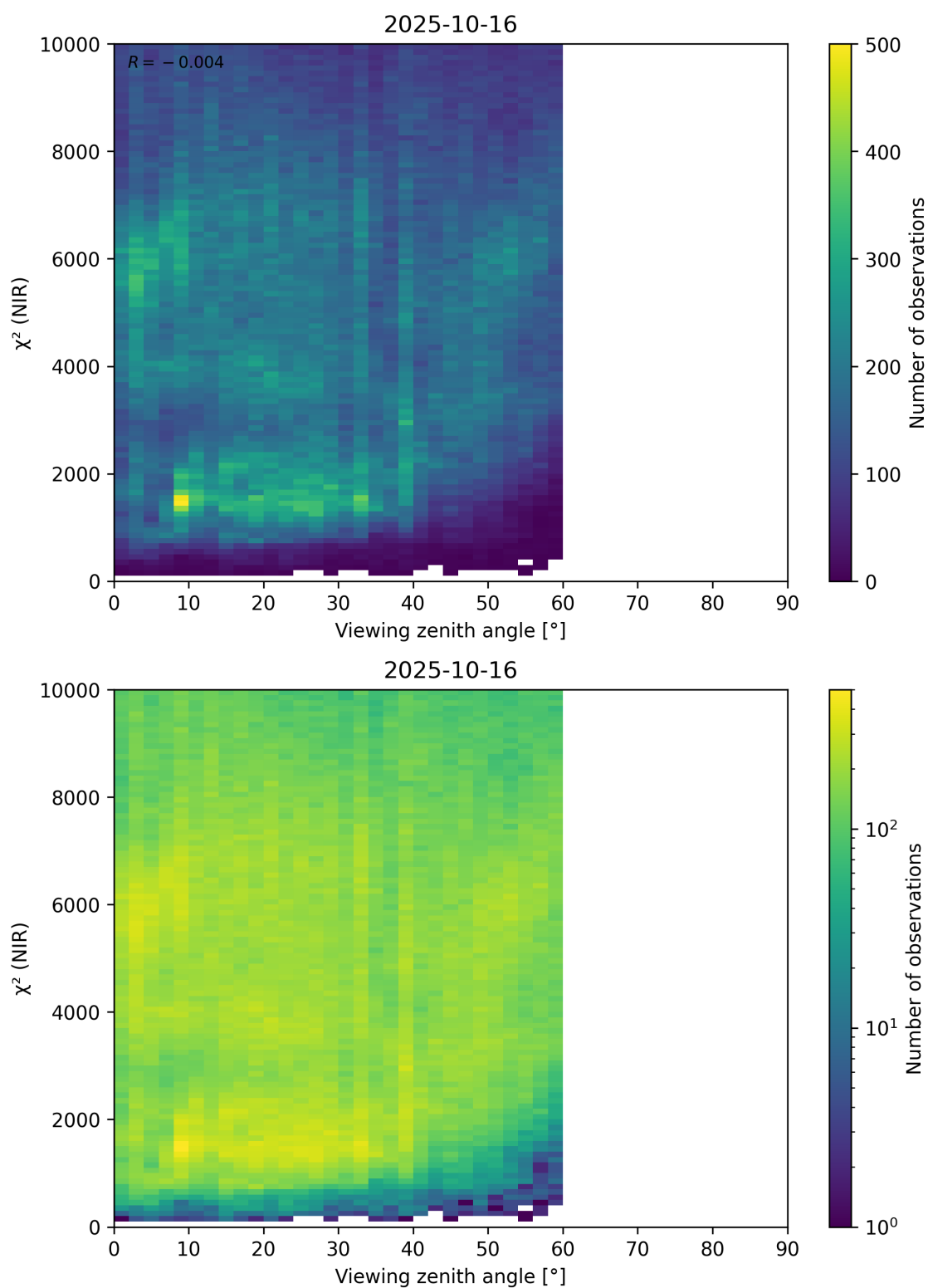
Figure 105: Scatter density plot of “Viewing zenith angle” against “ \chi^2 (NIR)” for 2025-10-15 to 2025-10-17.
