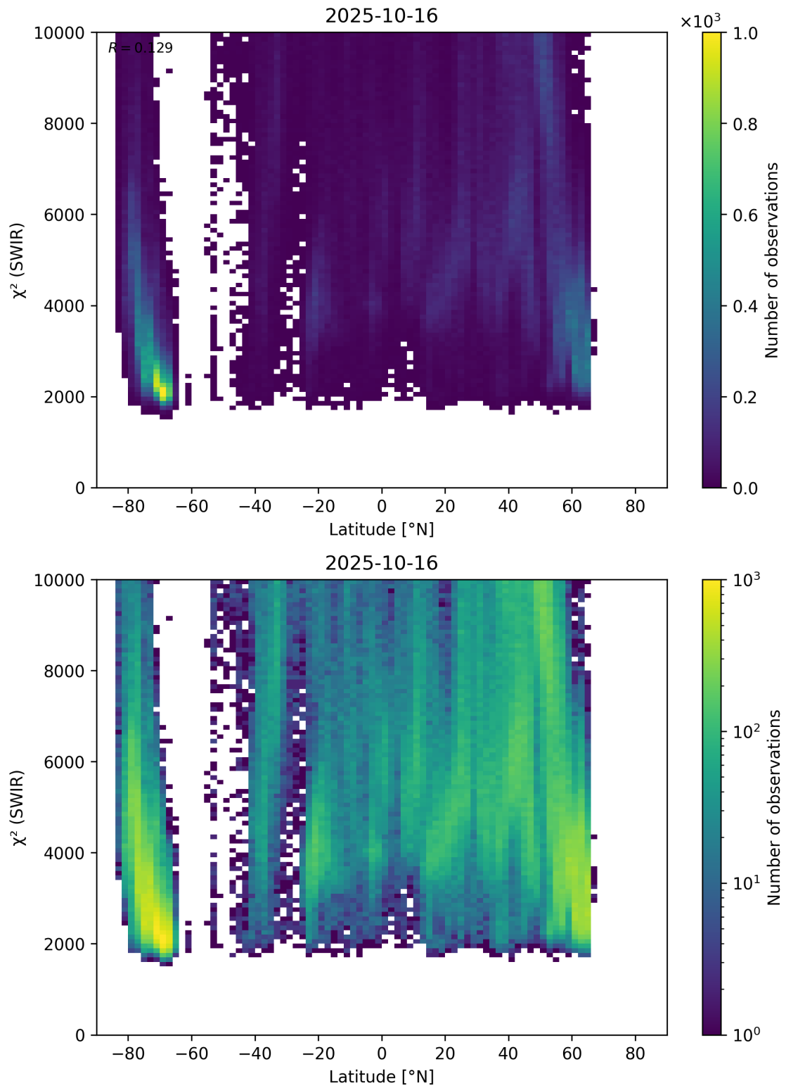
Figure 54: Scatter density plot of “Latitude” against “ \chi^2 (SWIR)” for 2025-10-15 to 2025-10-17.
