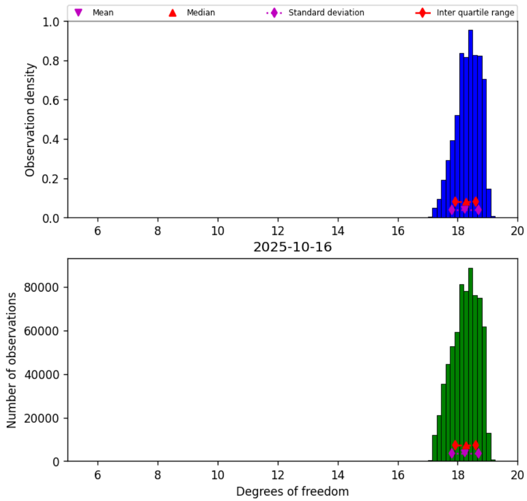
Figure 30: Histogram of “Degrees of freedom” for 2025-10-15 to 2025-10-17
