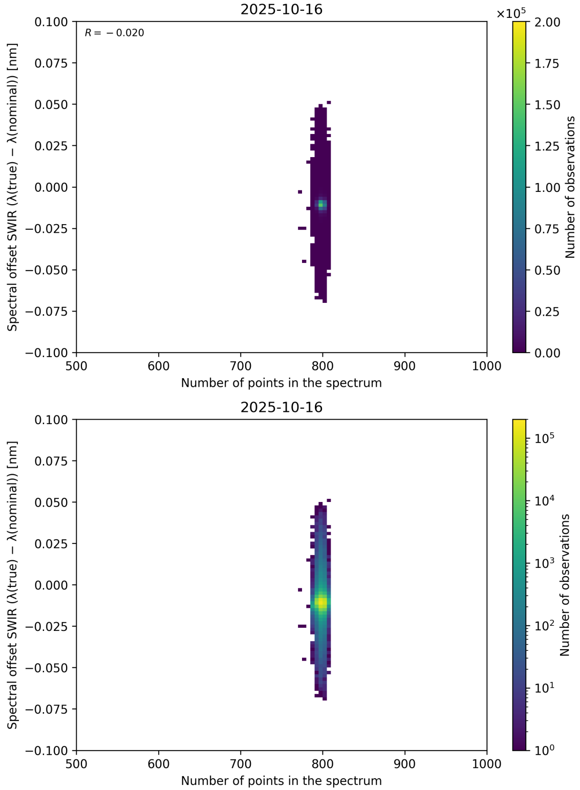
Figure 93: Scatter density plot of “Number of points in the spectrum” against “Spectral offset SWIR ( \lambda_{\text{true}} - \lambda_{\text{nominal}} )” for 2025-10-15 to 2025-10-17.
