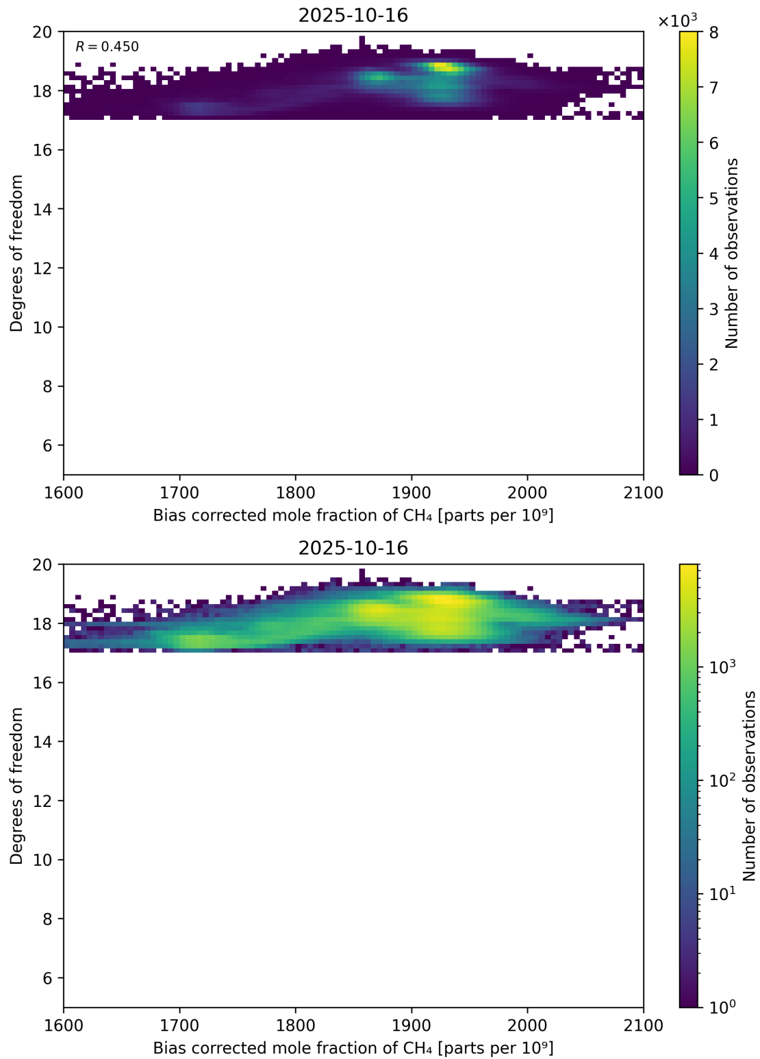
Figure 65: Scatter density plot of “Bias corrected mole fraction of CH 4 ” against “Degrees of freedom” for 2025-10-15 to 2025-10-17.
