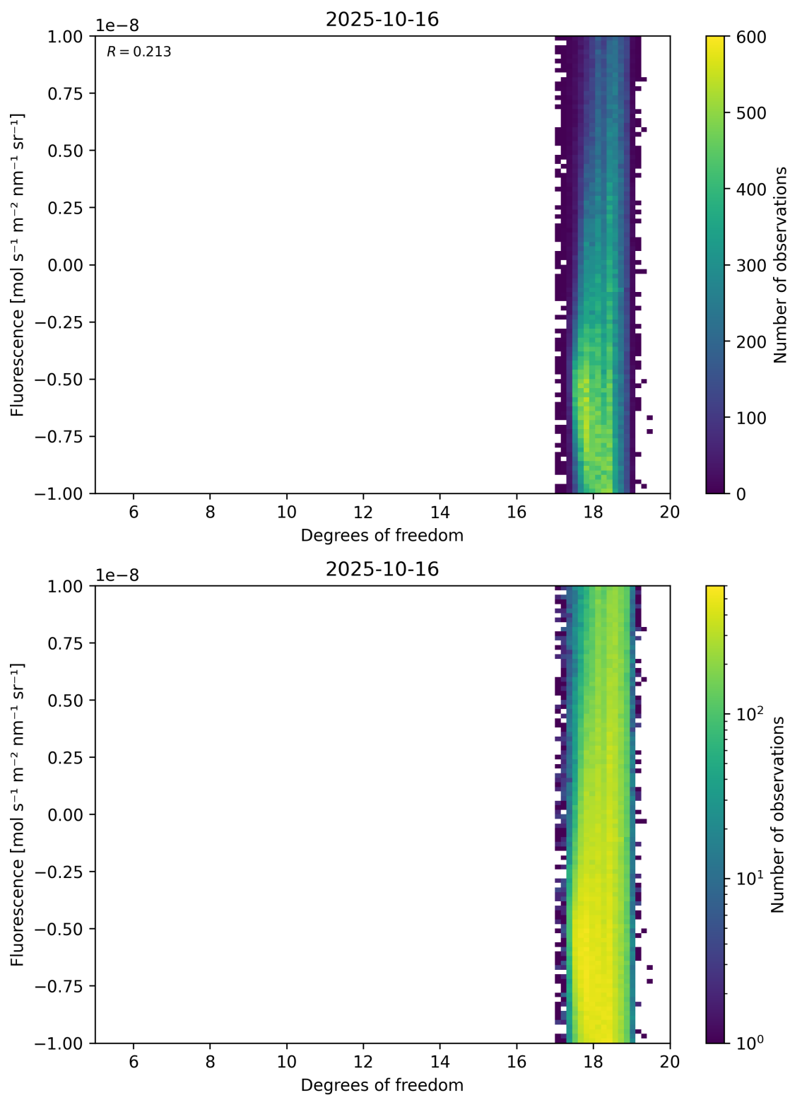
Figure 51: Scatter density plot of “Degrees of freedom” against “Fluorescence” for 2025-10-15 to 2025-10-17.
