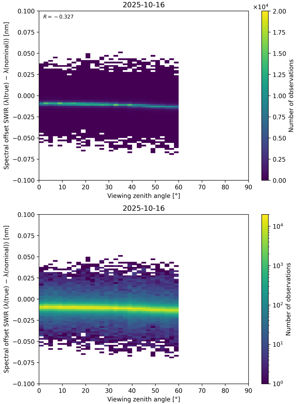
Figure 116: Scatter density plot of “Viewing zenith angle” against “Spectral offset SWIR ( \lambda_{\text{true}} - \lambda_{\text{nominal}} )” for 2025-10-15 to 2025-10-17.
