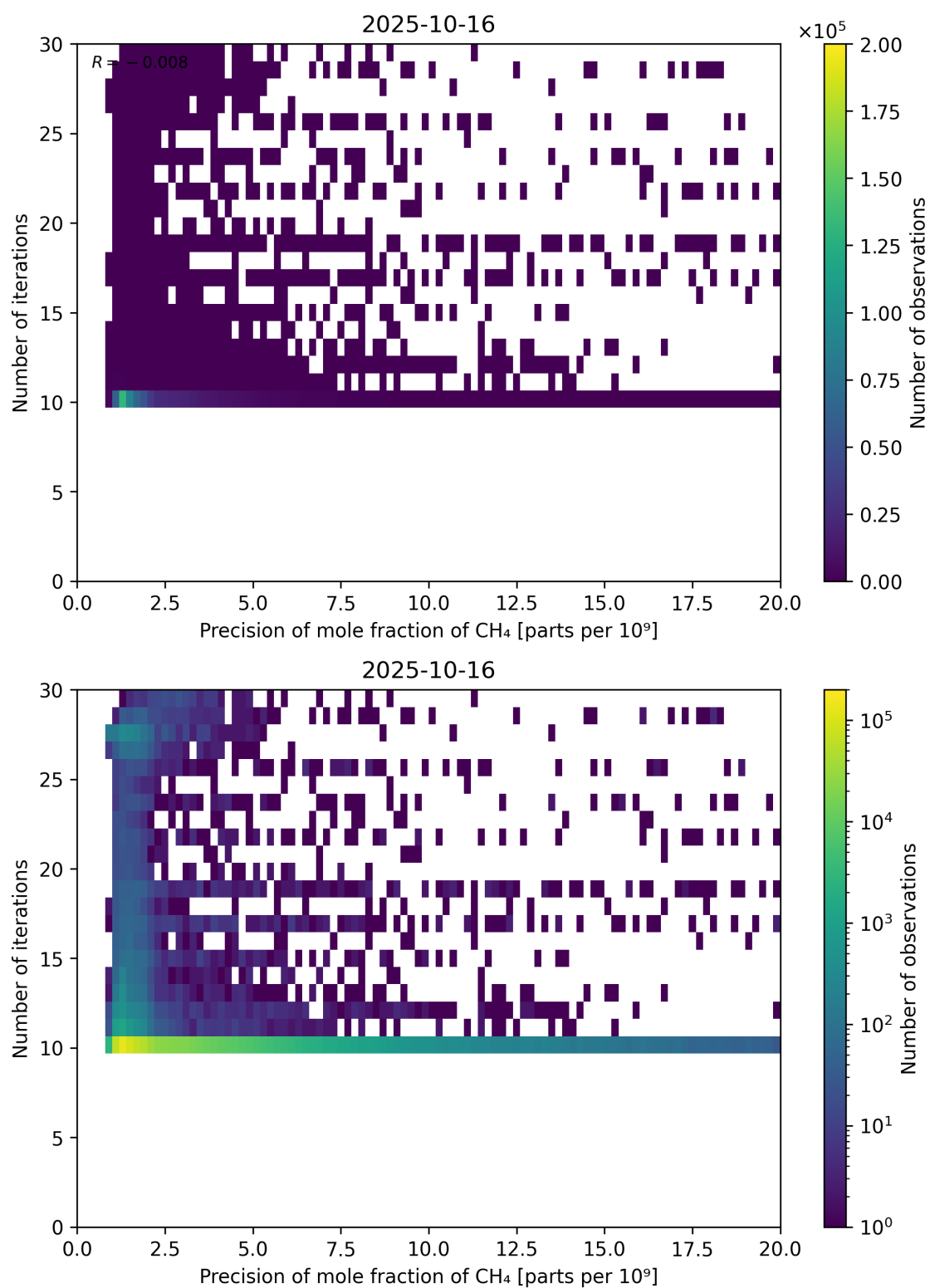
Figure 83: Scatter density plot of “Precision of mole fraction of CH 4 ” against “Number of iterations” for 2025-10-15 to 2025-10-17.
