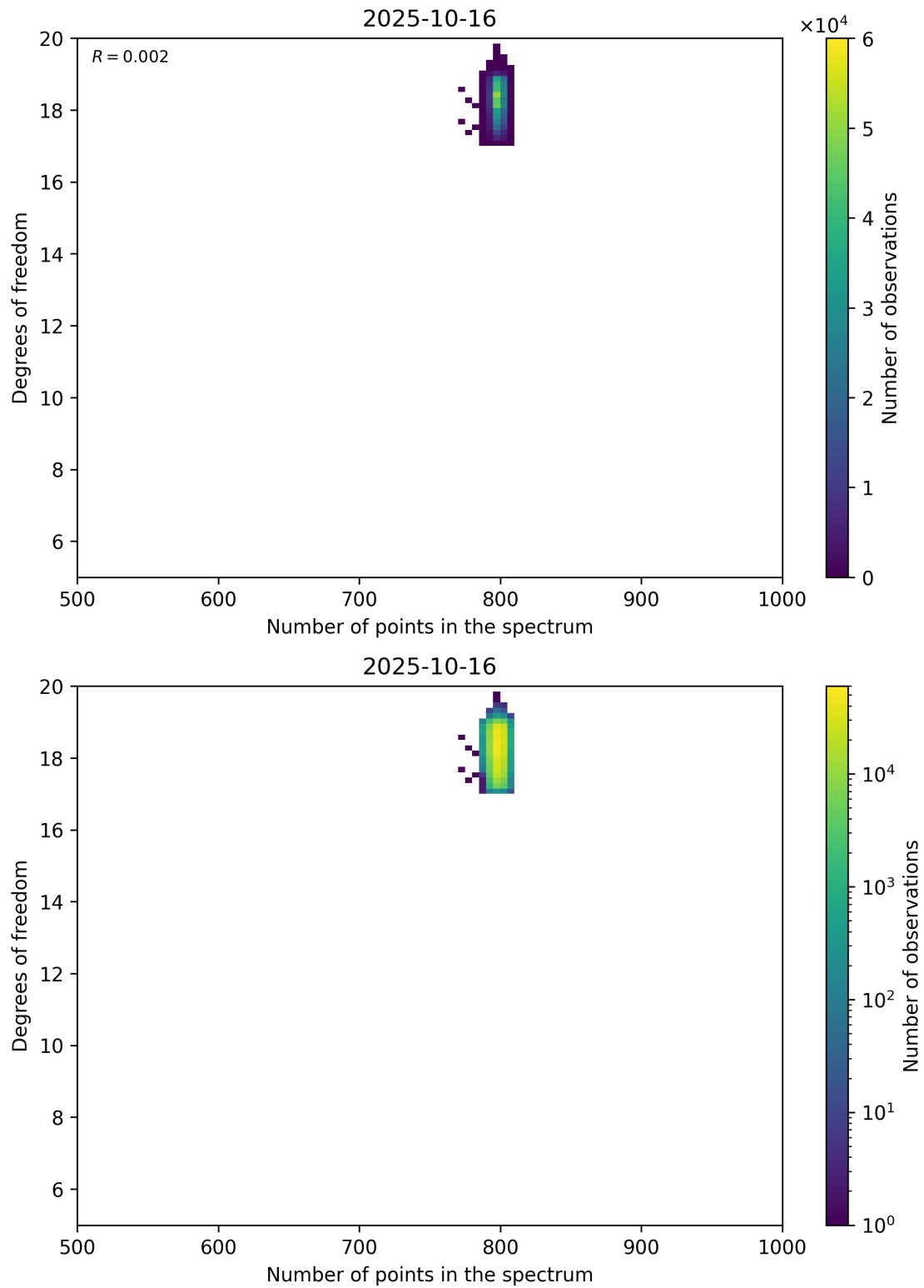
Figure 90: Scatter density plot of “Number of points in the spectrum” against “Degrees of freedom” for 2025-10-15 to 2025-10-17.
