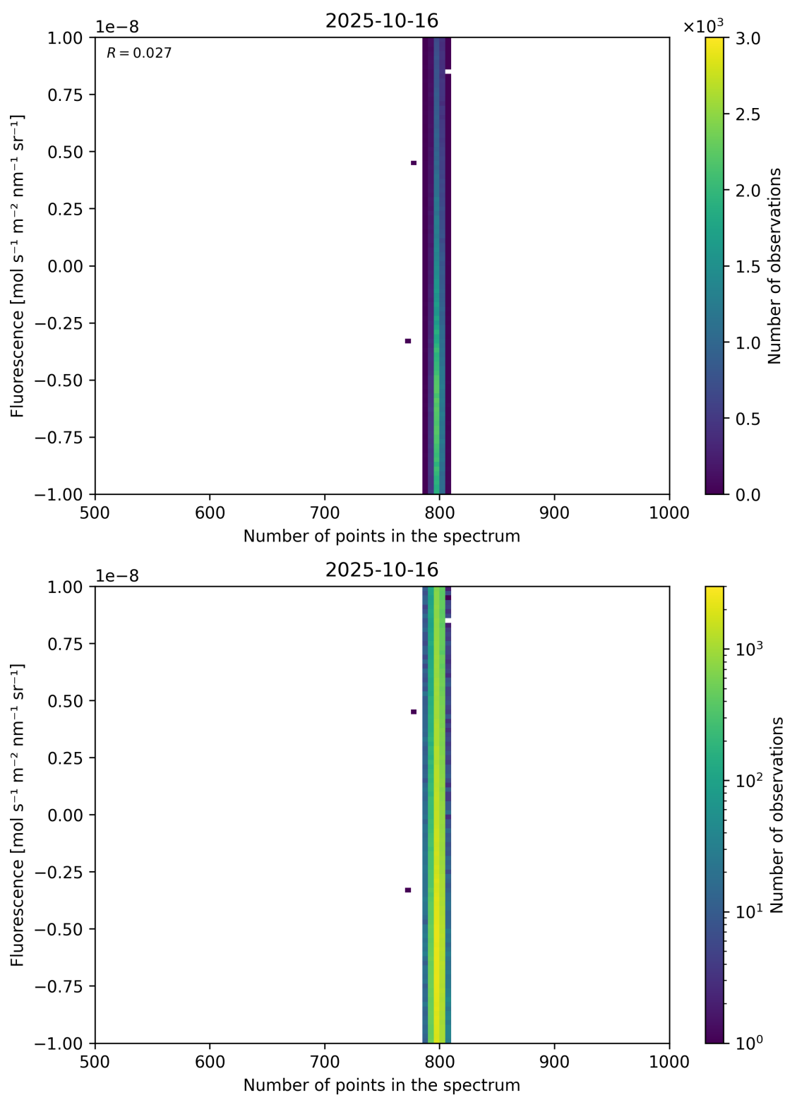
Figure 91: Scatter density plot of “Number of points in the spectrum” against “Fluorescence” for 2025-10-15 to 2025-10-17.
