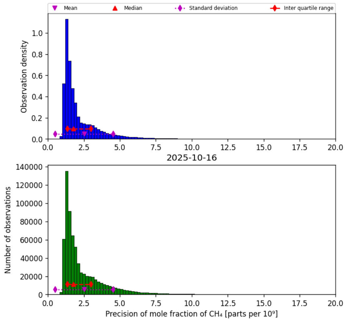
Figure 24: Histogram of “Precision of mole fraction of CH 4 ” for 2025-10-15 to 2025-10-17
