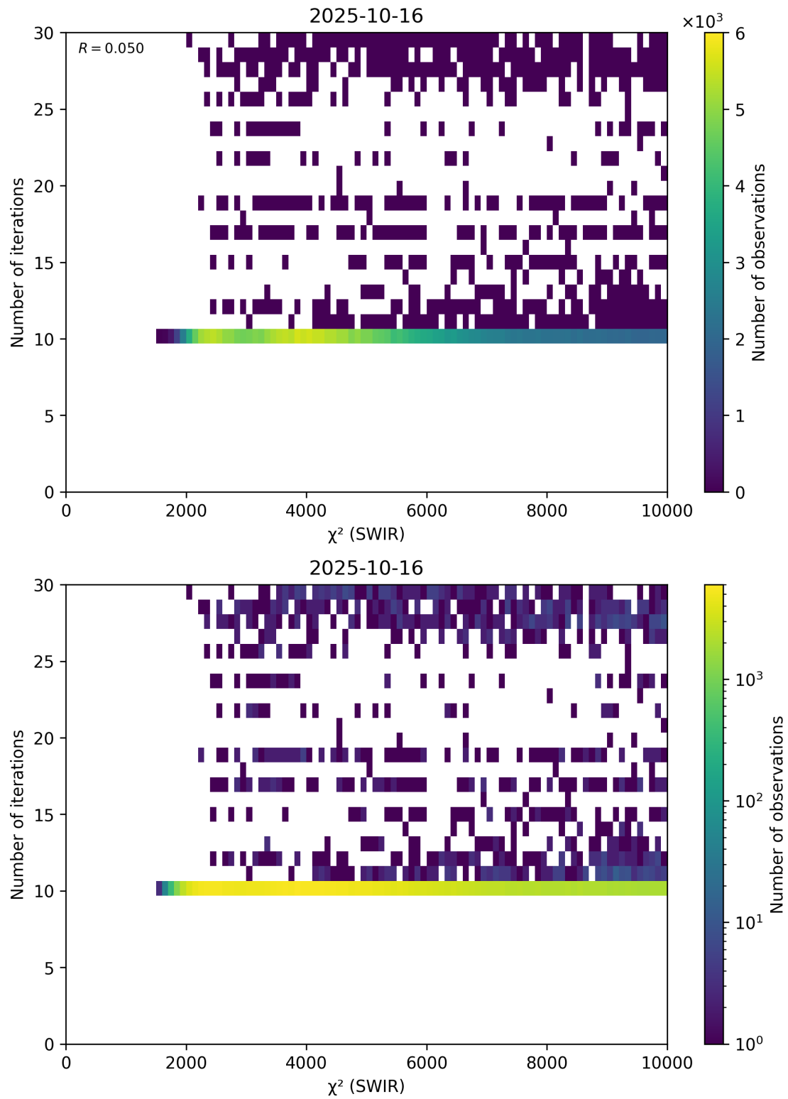
Figure 50: Scatter density plot of “ \chi^2 (SWIR)” against “Number of iterations” for 2025-10-15 to 2025-10-17.
