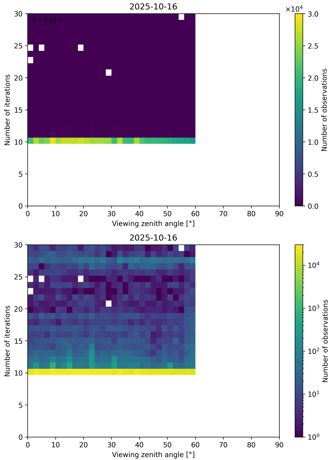
Figure 113: Scatter density plot of “Viewing zenith angle” against “Number of iterations” for 2025-10-15 to 2025-10-17.
