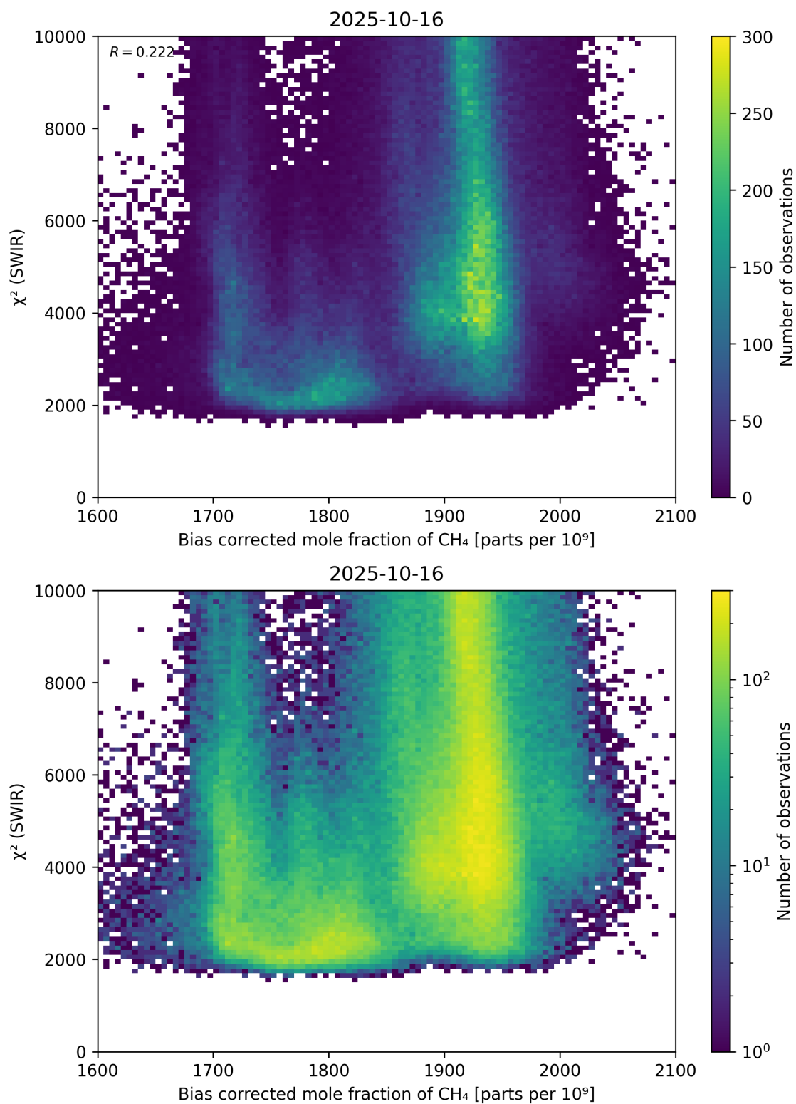
Figure 64: Scatter density plot of “Bias corrected mole fraction of \text{CH}_4 ” against “ \chi^2 (SWIR)” for 2025-10-15 to 2025-10-17.
