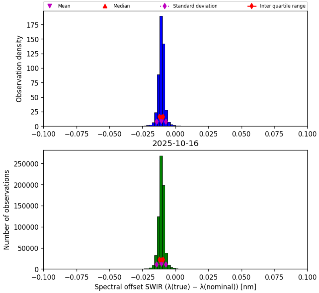
Figure 27: Histogram of “Spectral offset SWIR ( \lambda_{\text{true}} - \lambda_{\text{nominal}} )” for 2025-10-15 to 2025-10-17
