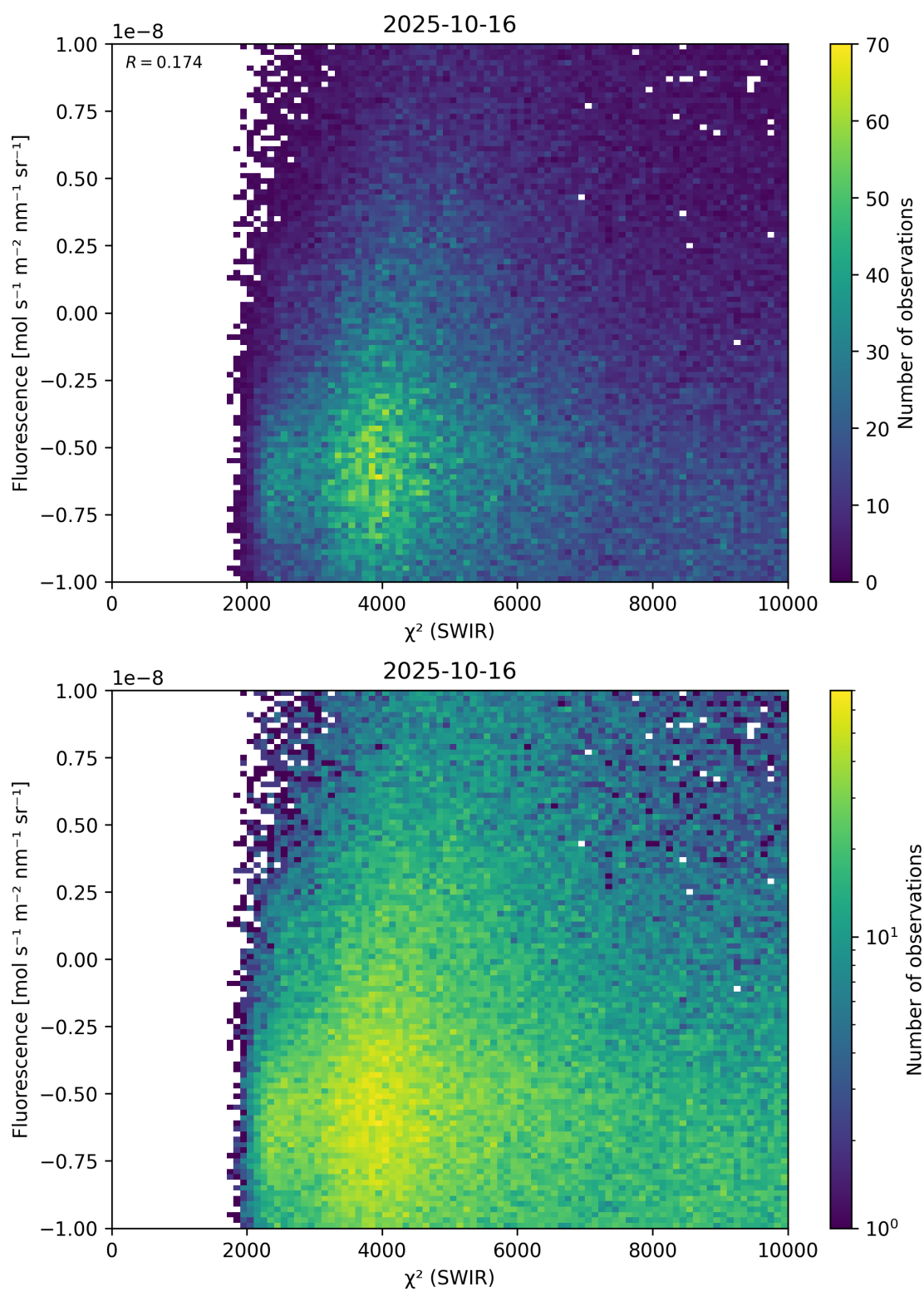
Figure 49: Scatter density plot of “ \chi^2 (SWIR)” against “Fluorescence” for 2025-10-15 to 2025-10-17.
