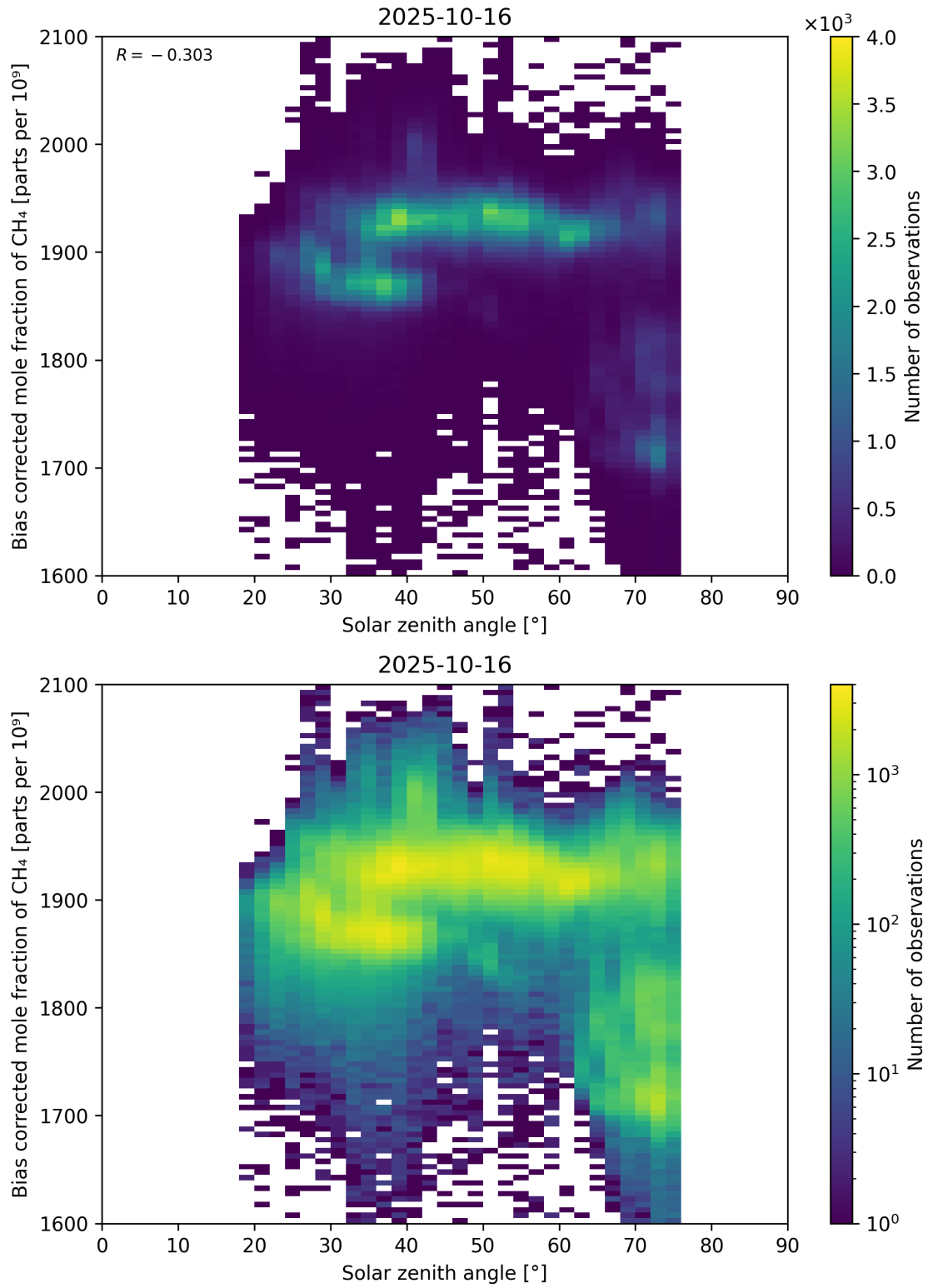
Figure 100: Scatter density plot of “Solar zenith angle” against “Bias corrected mole fraction of \text{CH}_4 ” for 2025-10-15 to 2025-10-17.
