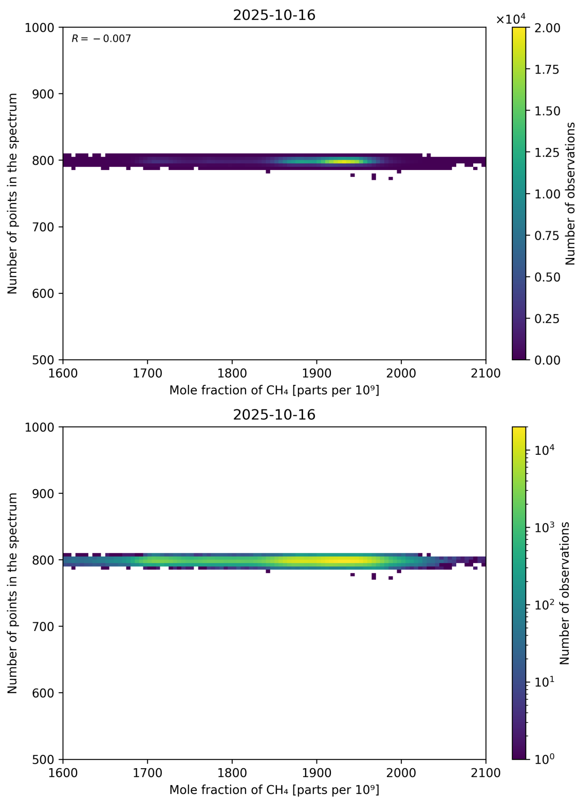
Figure 77: Scatter density plot of “Mole fraction of CH 4 ” against “Number of points in the spectrum” for 2025-10-15 to 2025-10-17.
