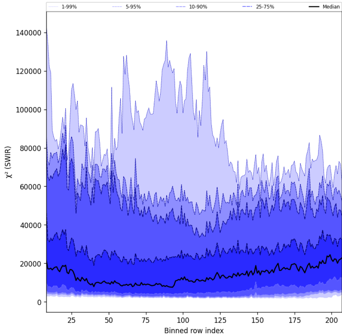
Figure 39: Along track statistics of “ \chi^2 (SWIR)” for 2025-10-15 to 2025-10-17
