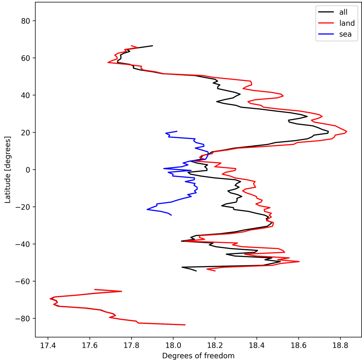
Figure 19: Zonal average of “Degrees of freedom” for 2025-10-15 to 2025-10-17.
