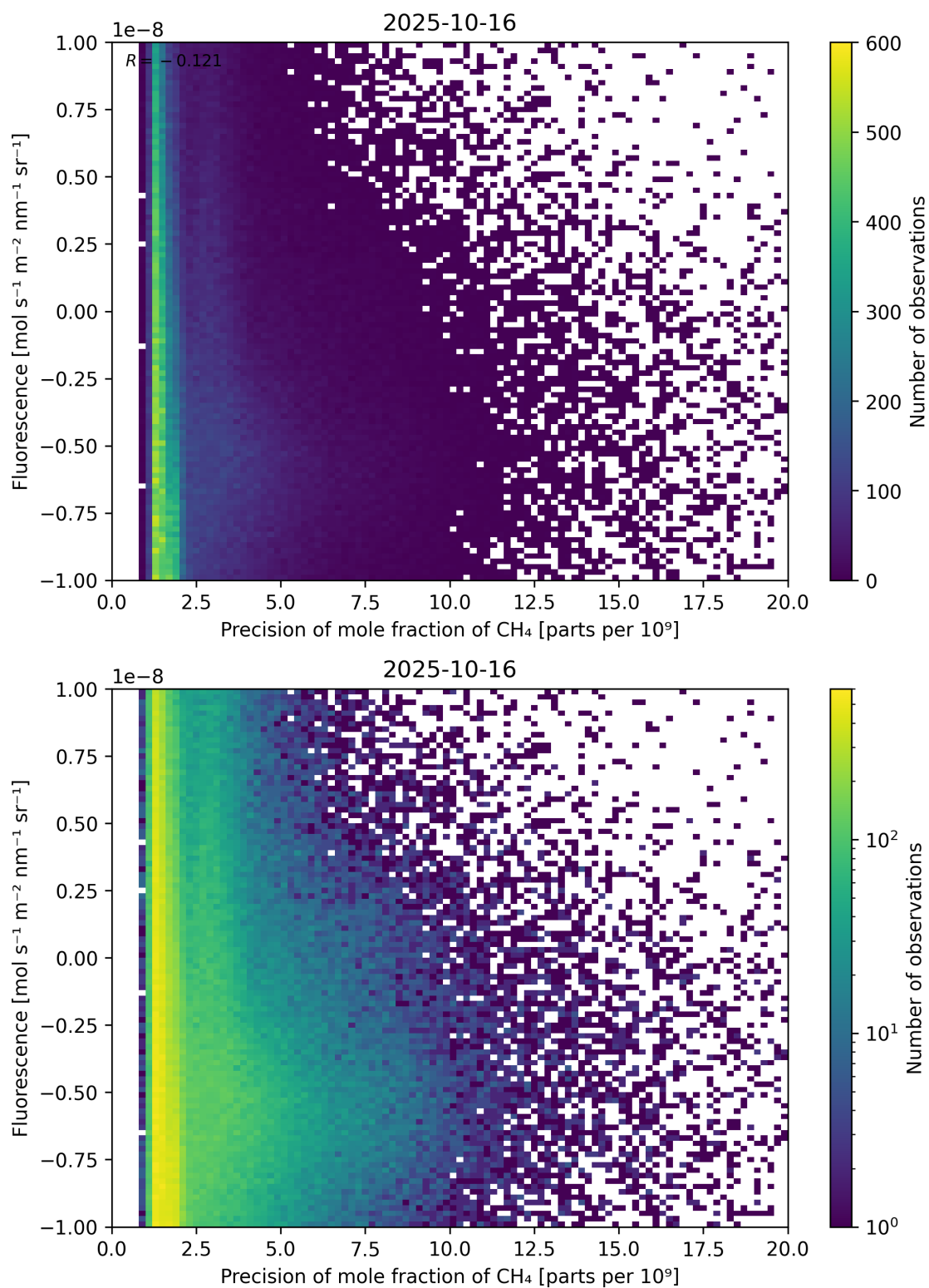
Figure 81: Scatter density plot of “Precision of mole fraction of CH 4 ” against “Fluorescence” for 2025-10-15 to 2025-10-17.
