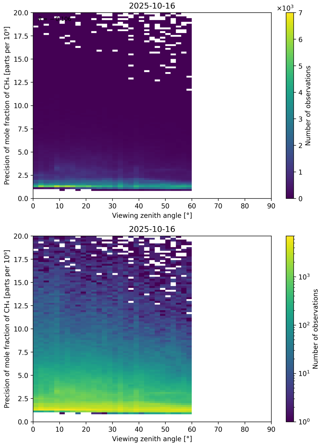
Figure 112: Scatter density plot of “Viewing zenith angle” against “Precision of mole fraction of CH 4 ” for 2025-10-15 to 2025-10-17.
