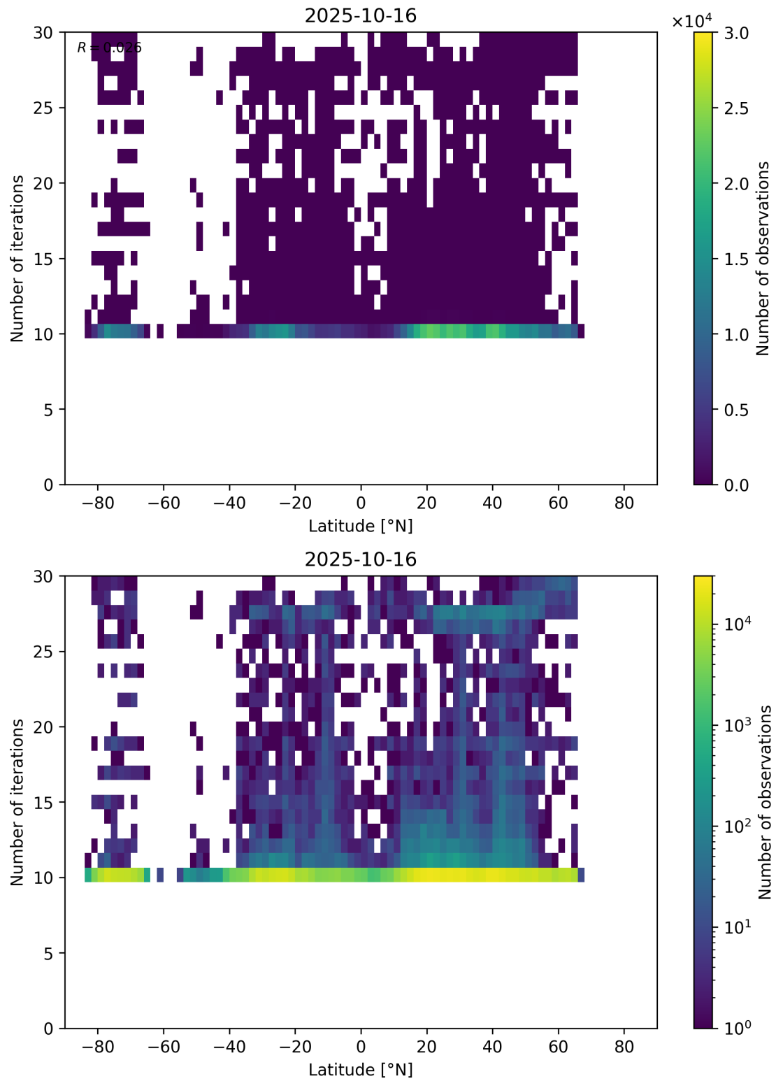
Figure 60: Scatter density plot of “Latitude” against “Number of iterations” for 2025-10-15 to 2025-10-17.
