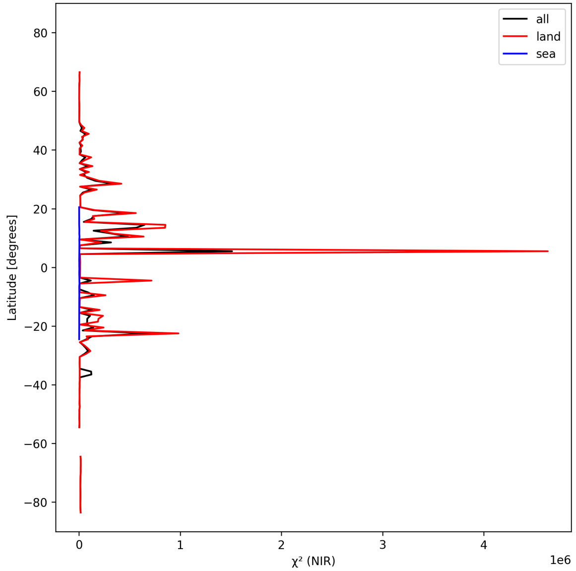
Figure 18: Zonal average of “ \chi^2 (NIR)” for 2025-10-15 to 2025-10-17.
