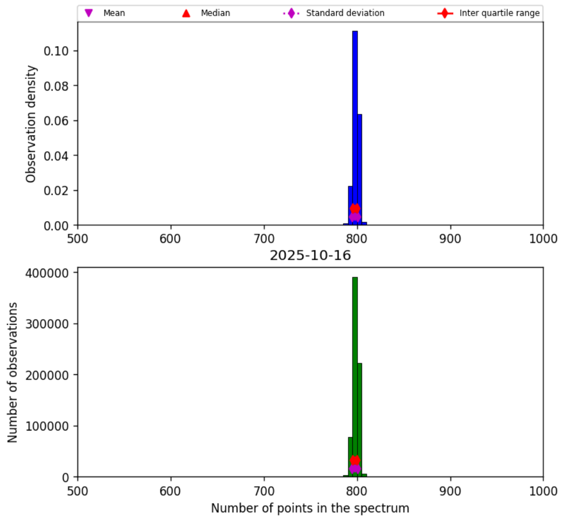
Figure 26: Histogram of “Number of points in the spectrum” for 2025-10-15 to 2025-10-17
