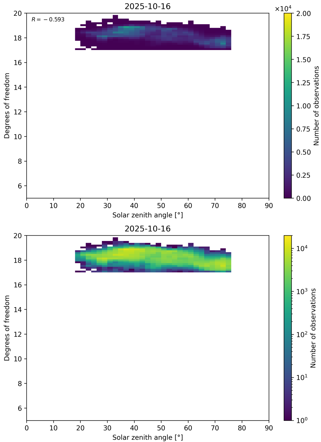
Figure 96: Scatter density plot of “Solar zenith angle” against “Degrees of freedom” for 2025-10-15 to 2025-10-17.
