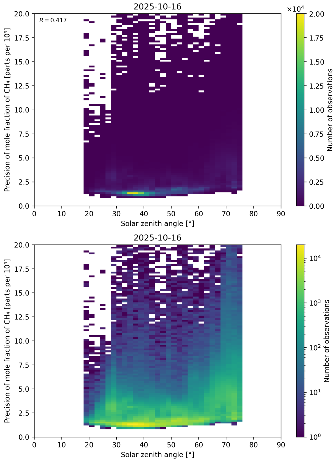
Figure 101: Scatter density plot of “Solar zenith angle” against “Precision of mole fraction of CH 4 ” for 2025-10-15 to 2025-10-17.
