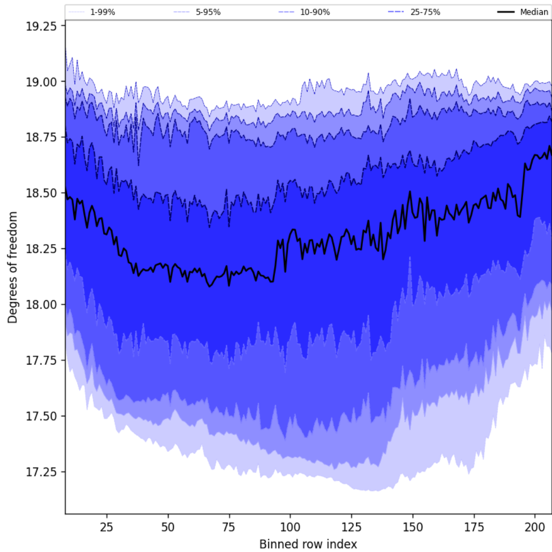
Figure 41: Along track statistics of “Degrees of freedom” for 2025-10-15 to 2025-10-17
