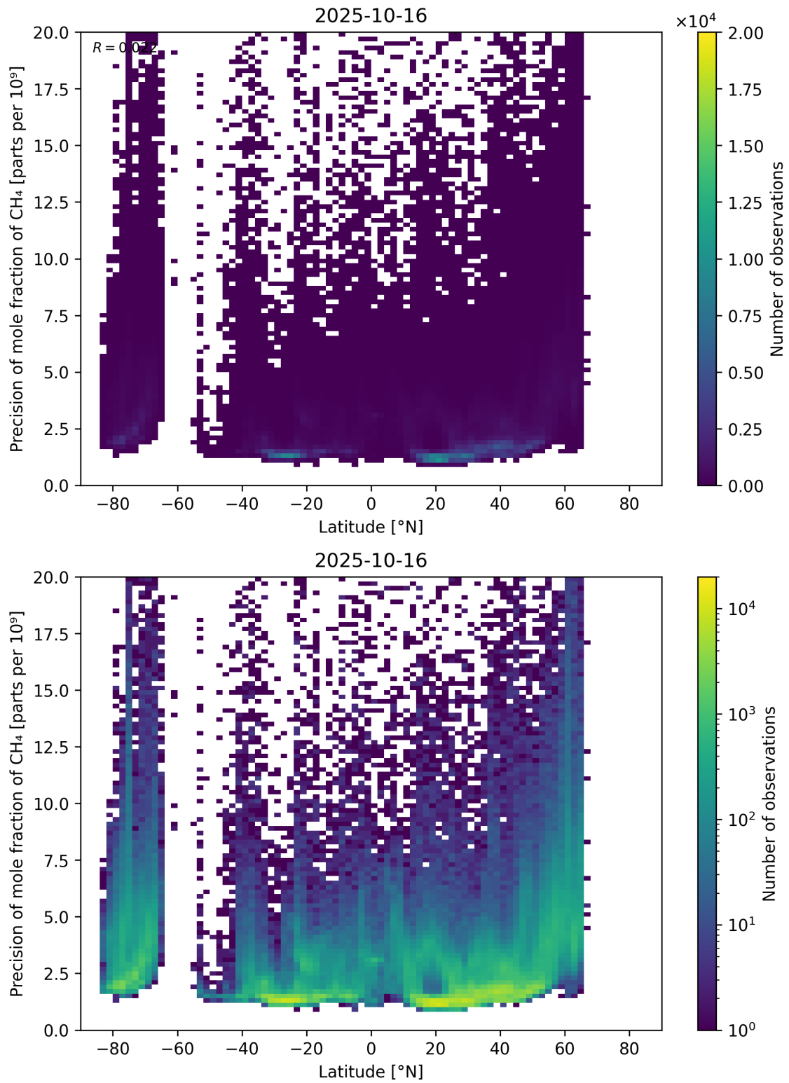
Figure 59: Scatter density plot of “Latitude” against “Precision of mole fraction of CH 4 ” for 2025-10-15 to 2025-10-17.
