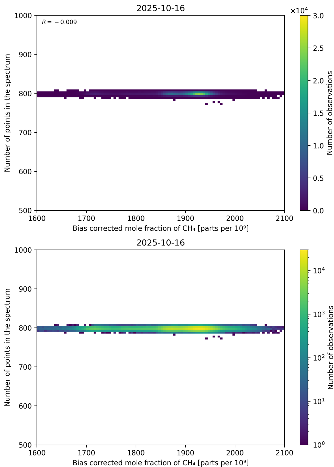
Figure 68: Scatter density plot of “Bias corrected mole fraction of CH 4 ” against “Number of points in the spectrum” for 2025-10-15 to 2025-10-17.
