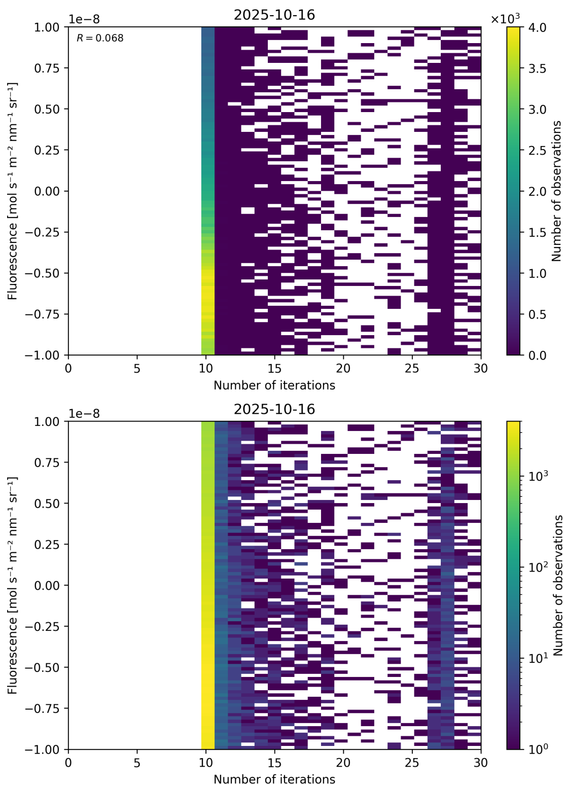
Figure 87: Scatter density plot of “Number of iterations” against “Fluorescence” for 2025-10-15 to 2025-10-17.
