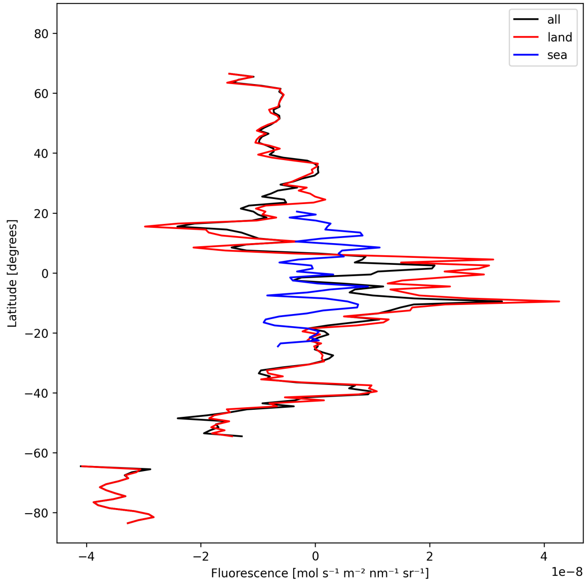
Figure 21: Zonal average of “Fluorescence” for 2025-10-15 to 2025-10-17.
