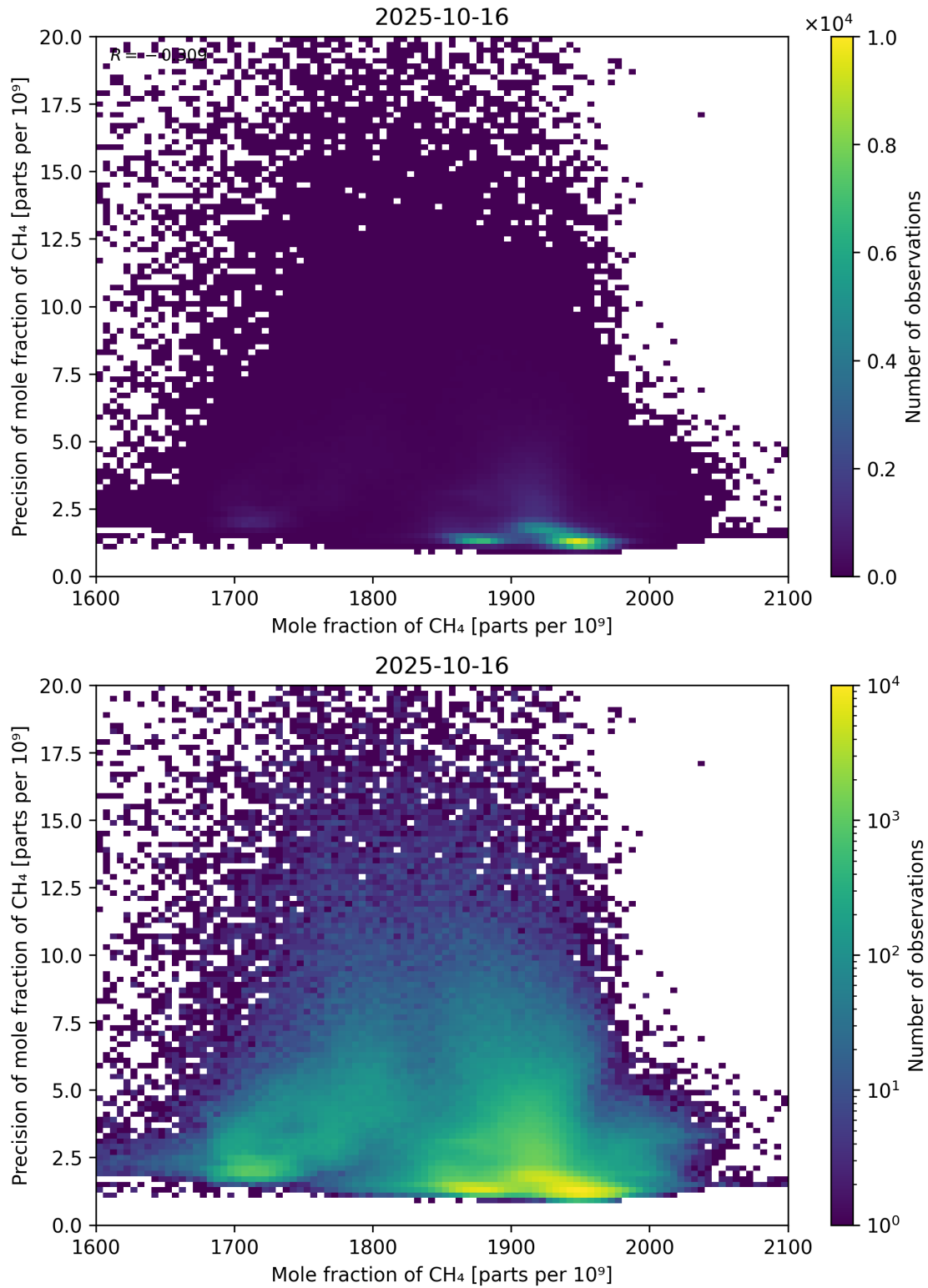
Figure 75: Scatter density plot of “Mole fraction of CH 4 ” against “Precision of mole fraction of CH 4 ” for 2025-10-15 to 2025-10-17.
