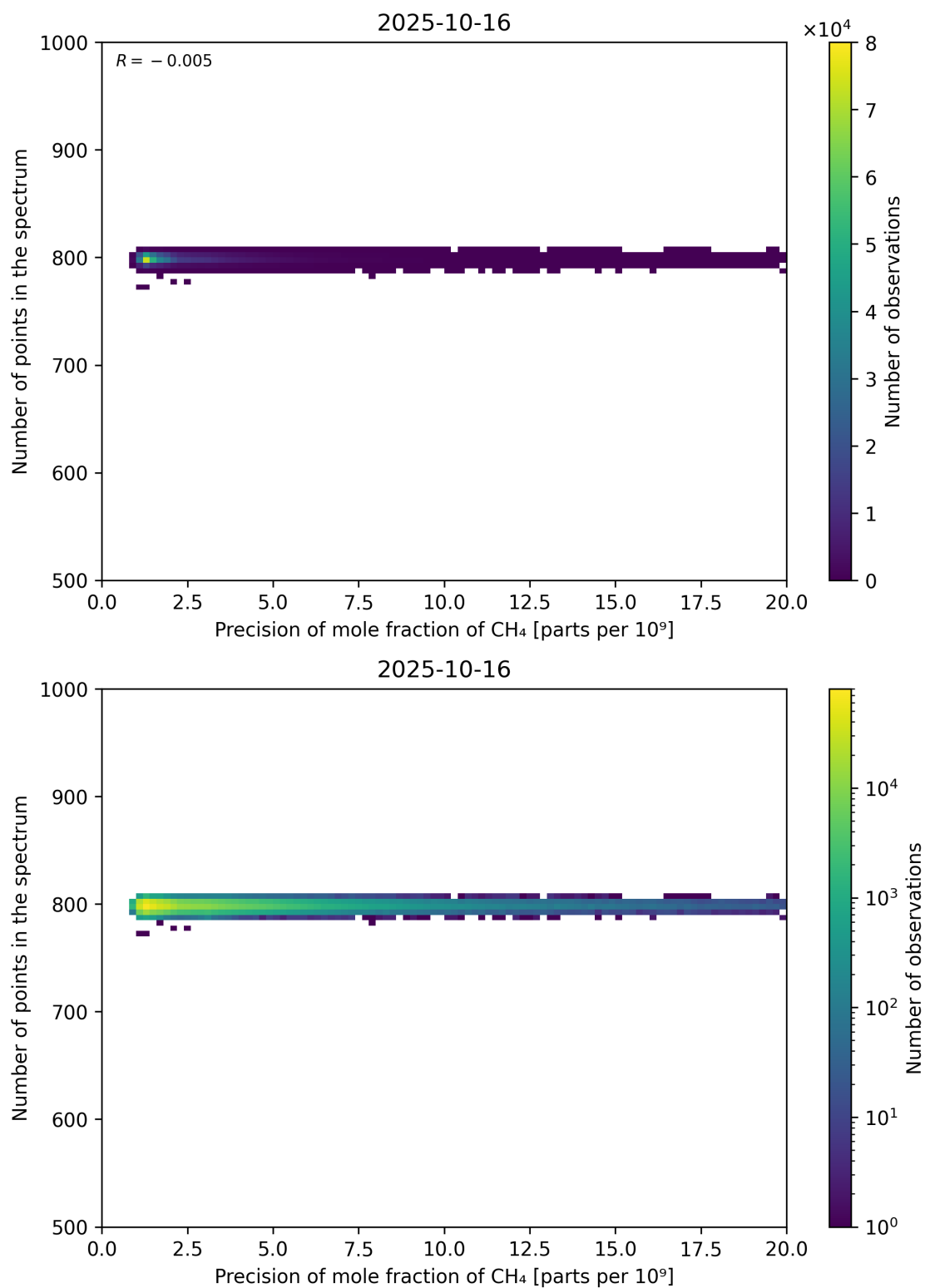
Figure 84: Scatter density plot of “Precision of mole fraction of CH 4 ” against “Number of points in the spectrum” for 2025-10-15 to 2025-10-17.
