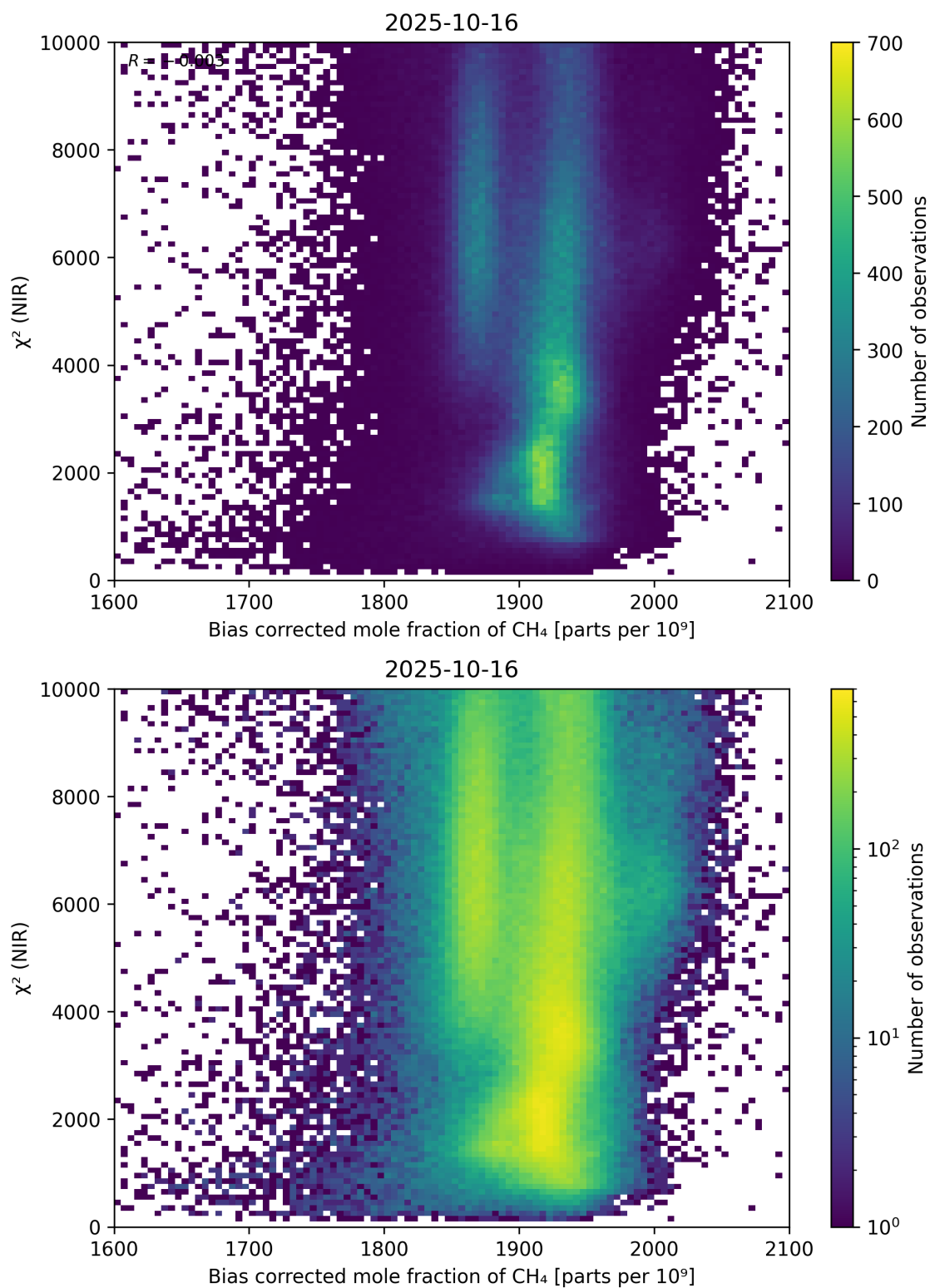
Figure 63: Scatter density plot of “Bias corrected mole fraction of \text{CH}_4 ” against “ \chi^2 (NIR)” for 2025-10-15 to 2025-10-17.
