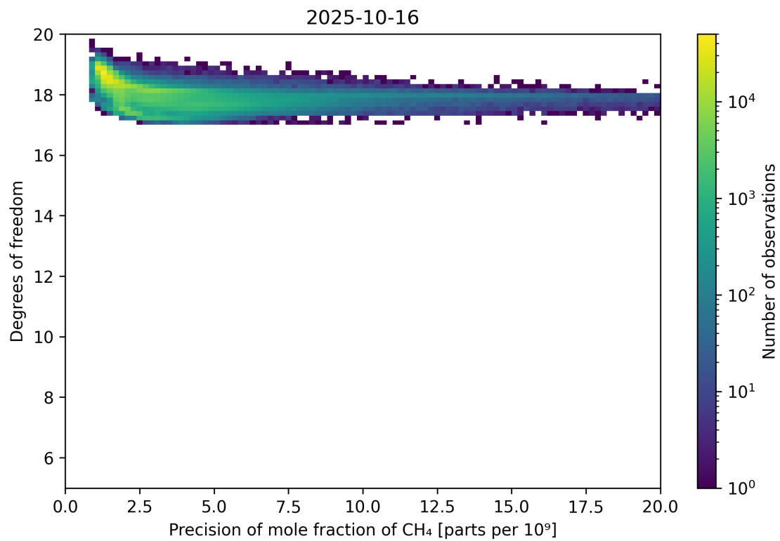
Figure 80: Scatter density plot of “Precision of mole fraction of CH 4 ” against “Degrees of freedom” for 2025-10-15 to 2025-10-17.
