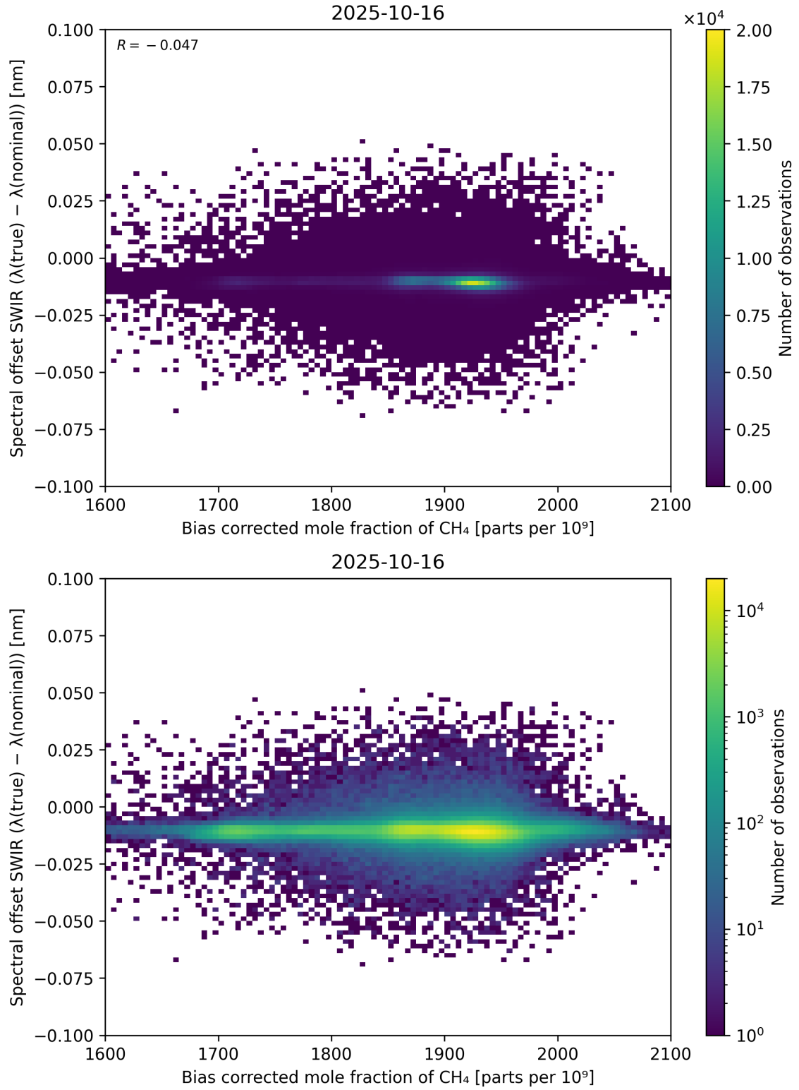
Figure 69: Scatter density plot of “Bias corrected mole fraction of \text{CH}_4 ” against “Spectral offset SWIR ( \lambda_{\text{true}} - \lambda_{\text{nominal}} )” for 2025-10-15 to 2025-10-17.
