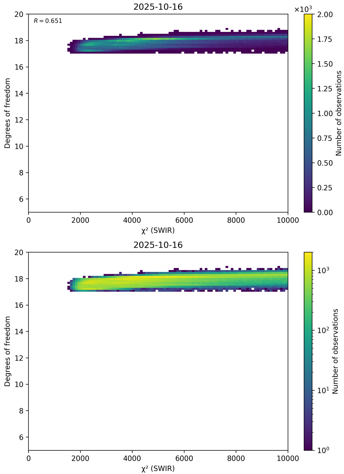
Figure 48: Scatter density plot of “ \chi^2 (SWIR)” against “Degrees of freedom” for 2025-10-15 to 2025-10-17.
