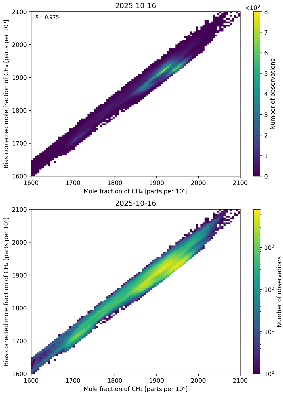
Figure 74: Scatter density plot of “Mole fraction of CH 4 ” against “Bias corrected mole fraction of CH 4 ” for 2025-10-15 to 2025-10-17.
