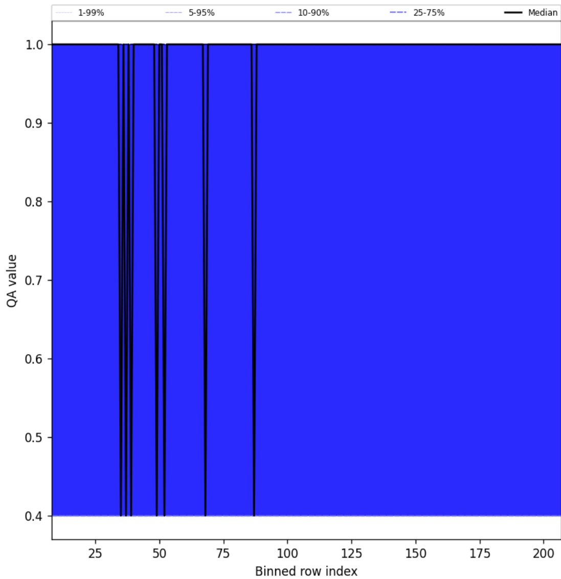
Figure 33: Along track statistics of “QA value” for 2025-10-15 to 2025-10-17
