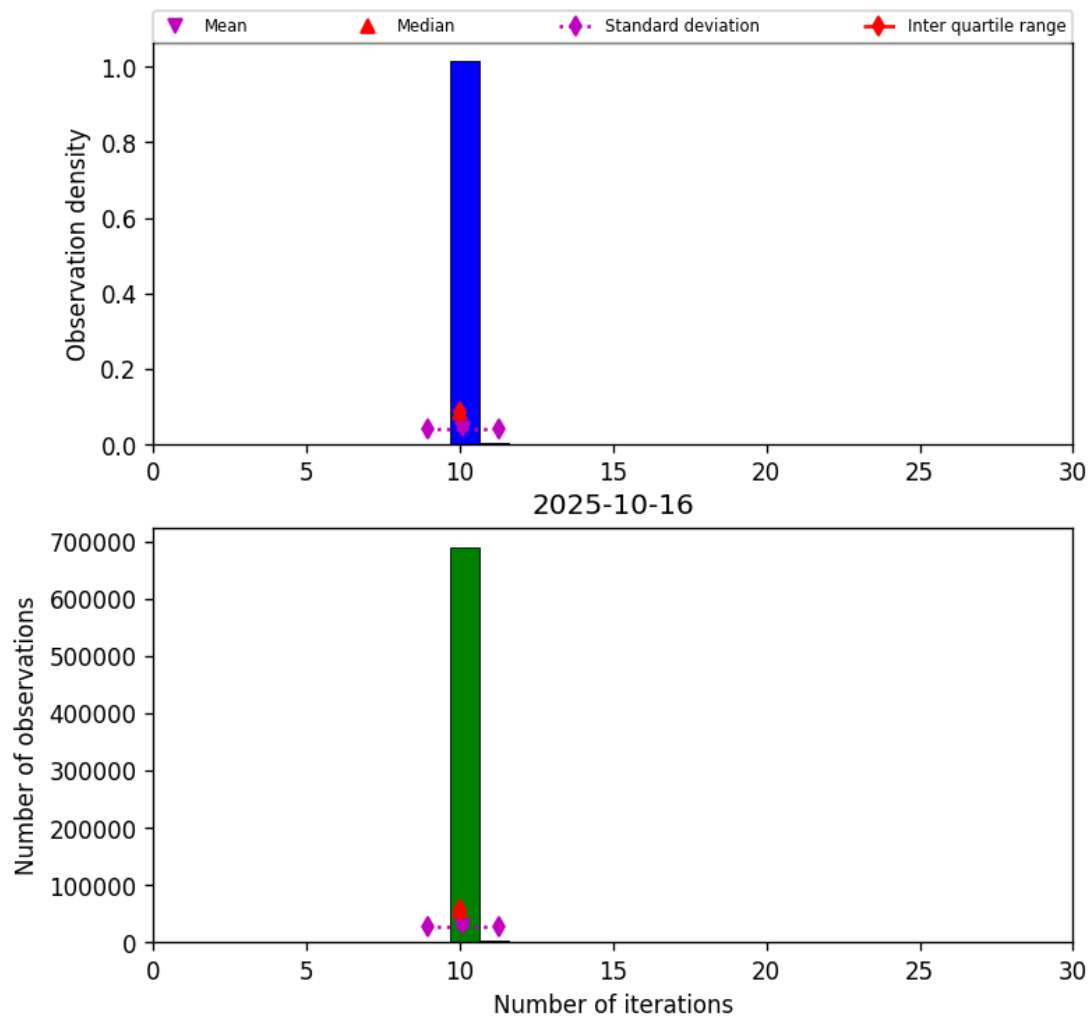
Figure 31: Histogram of “Number of iterations” for 2025-10-15 to 2025-10-17
