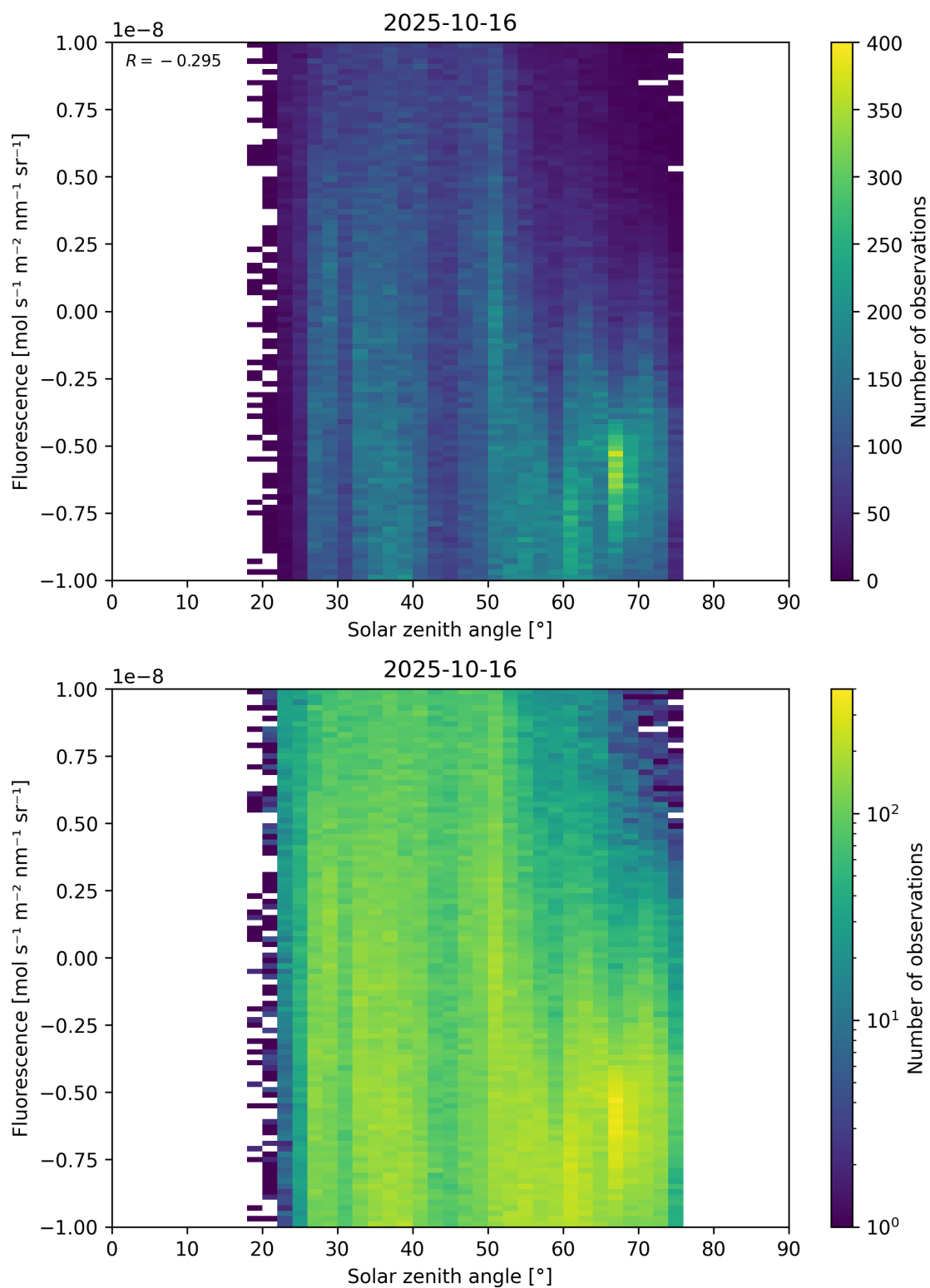
Figure 97: Scatter density plot of “Solar zenith angle” against “Fluorescence” for 2025-10-15 to 2025-10-17.
