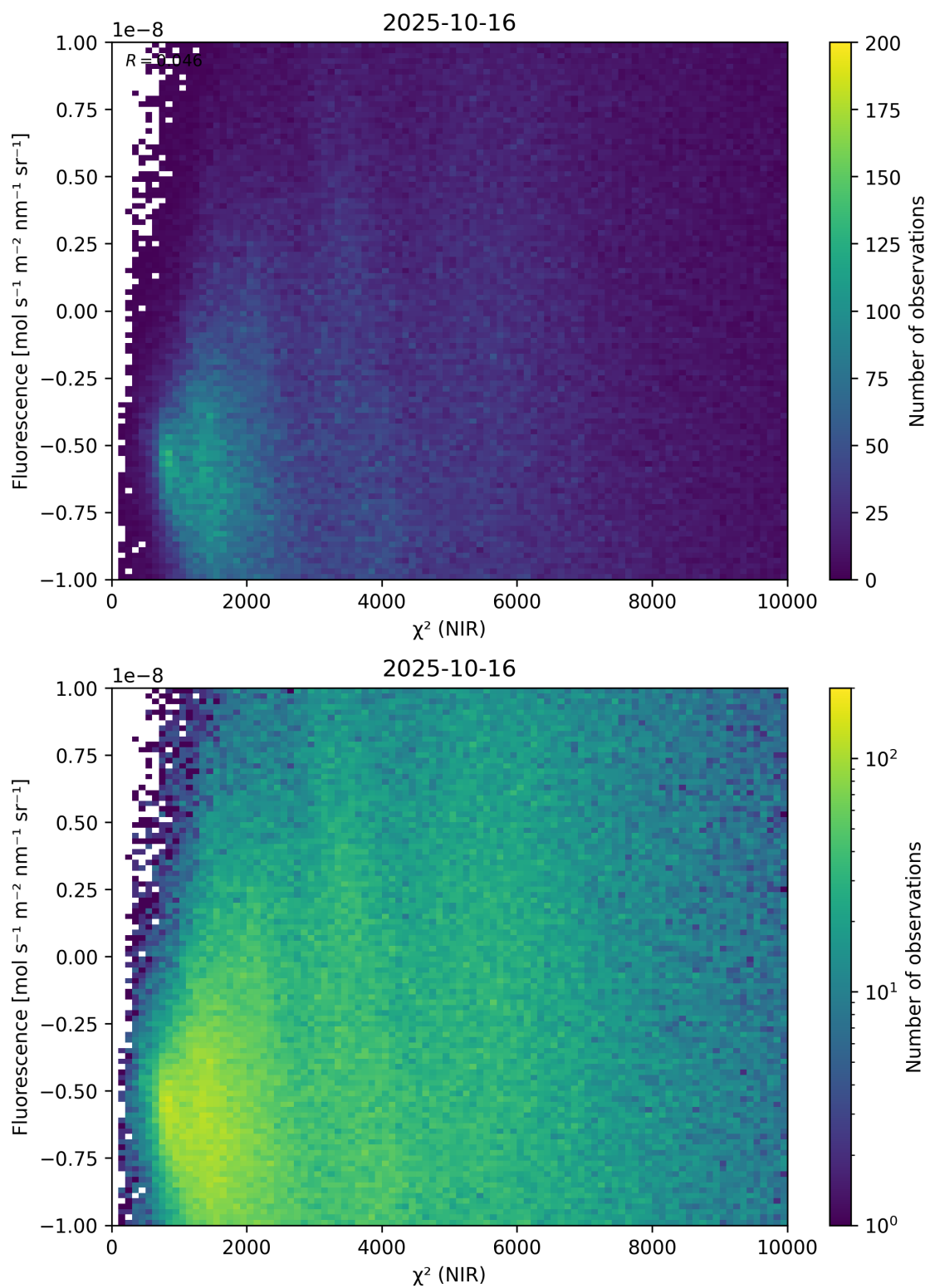
Figure 45: Scatter density plot of “ \chi^2 (NIR)” against “Fluorescence” for 2025-10-15 to 2025-10-17.
