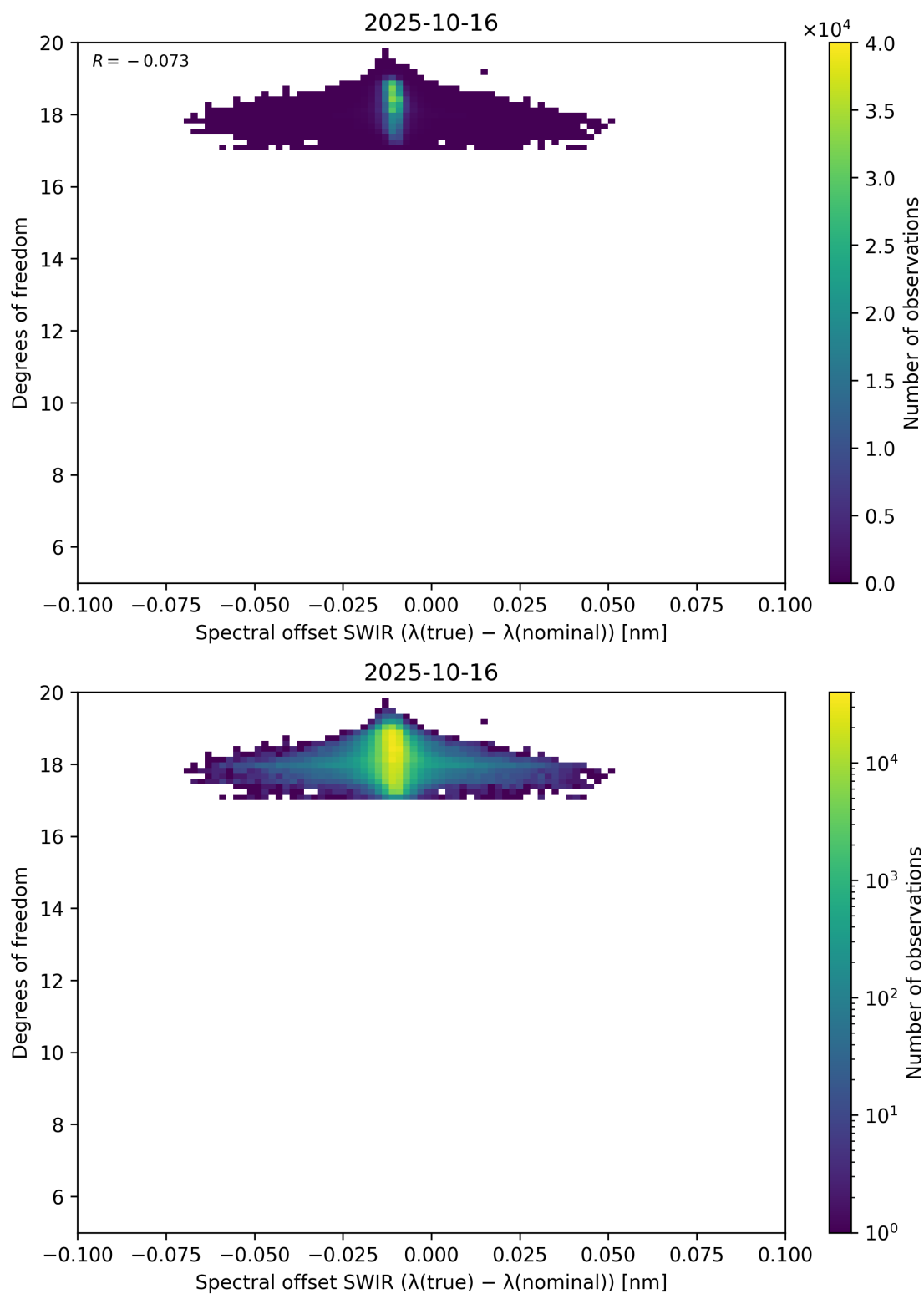
Figure 119: Scatter density plot of “Spectral offset SWIR ( \lambda_{\text{true}} - \lambda_{\text{nominal}} )” against “Degrees of freedom” for 2025-10-15 to 2025-10-17.
