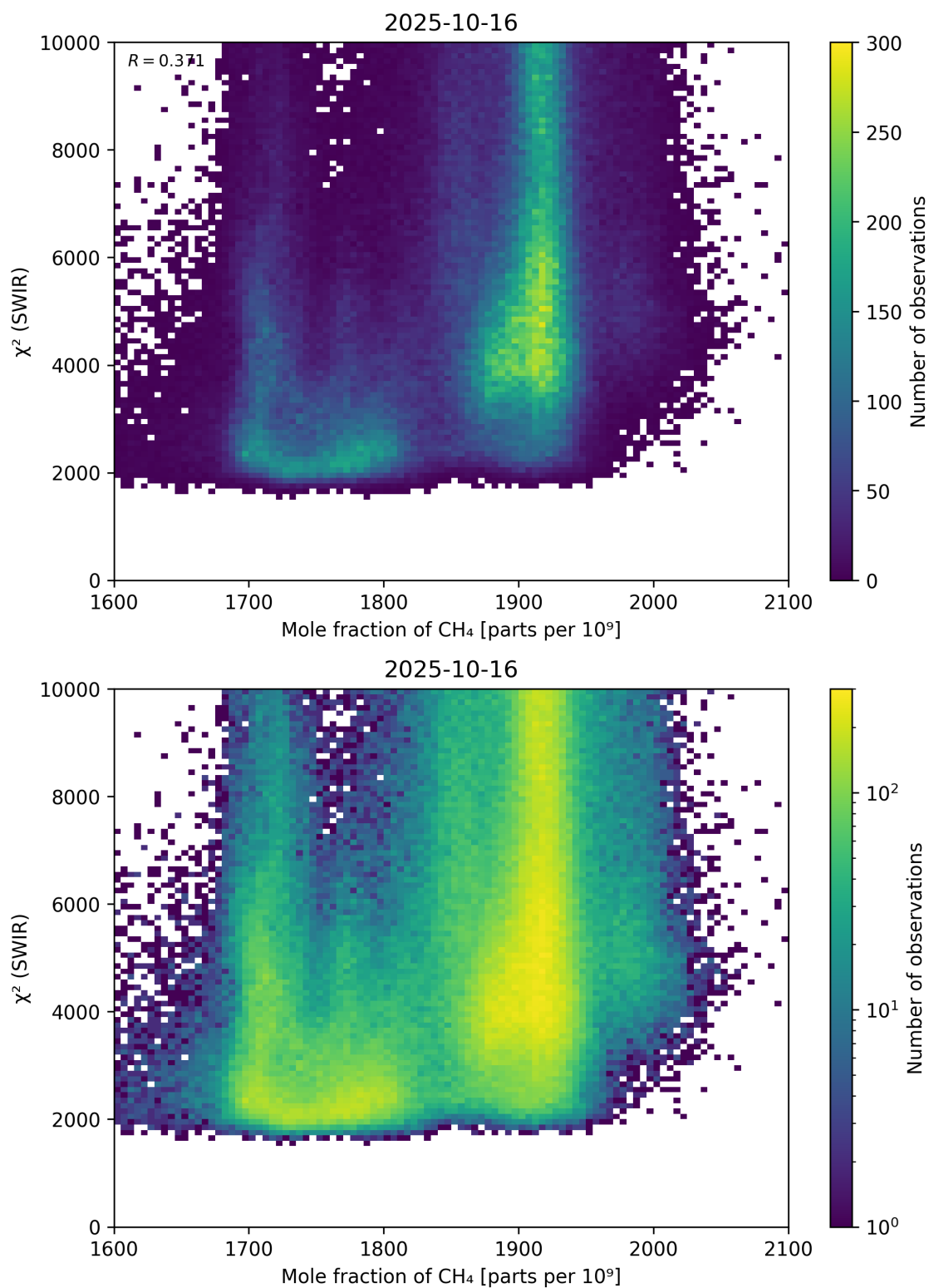
Figure 71: Scatter density plot of “Mole fraction of \text{CH}_4 ” against “ \chi^2 (SWIR)” for 2025-10-15 to 2025-10-17.
