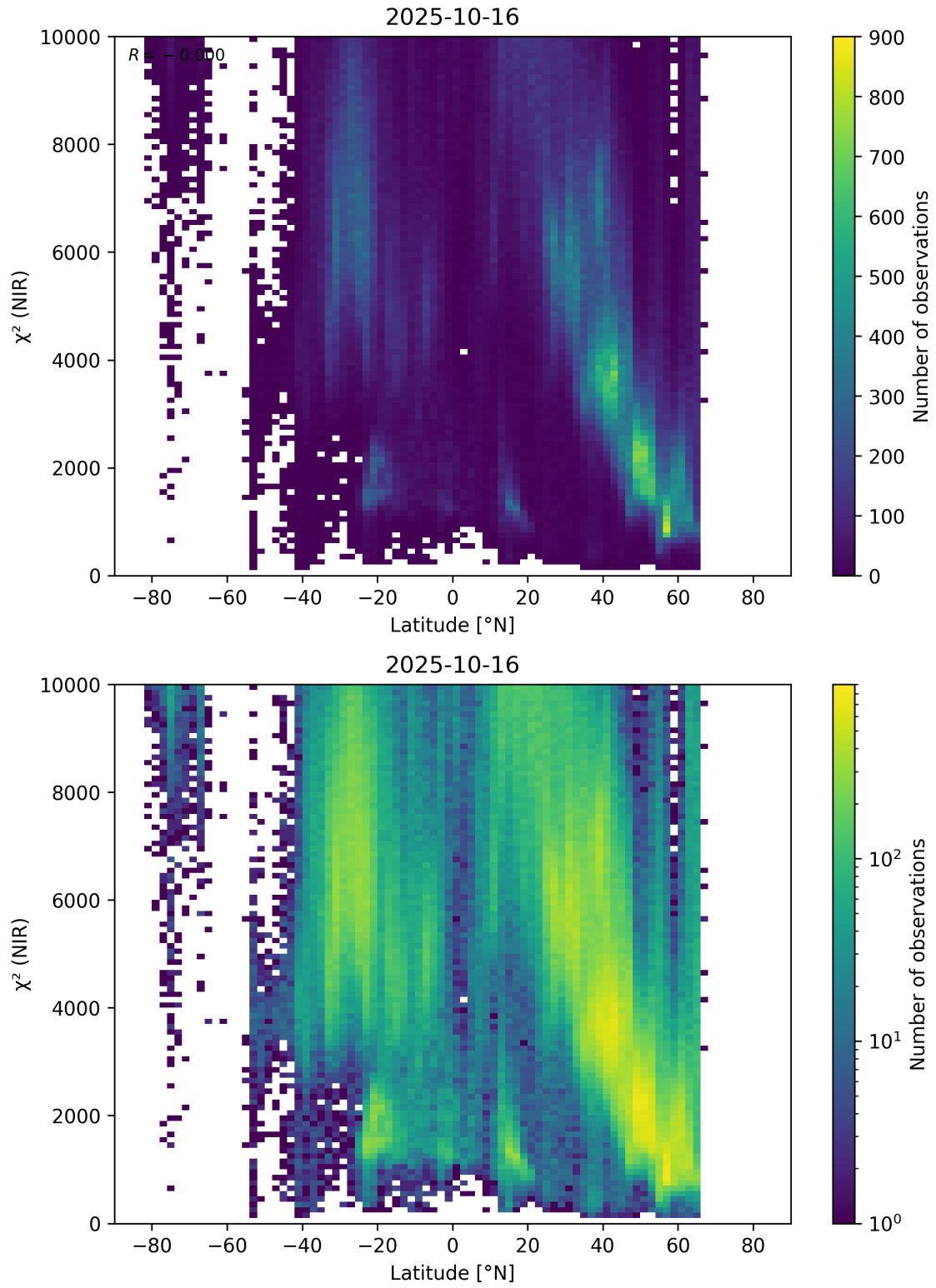
Figure 53: Scatter density plot of “Latitude” against “ \chi^2 (NIR)” for 2025-10-15 to 2025-10-17.
