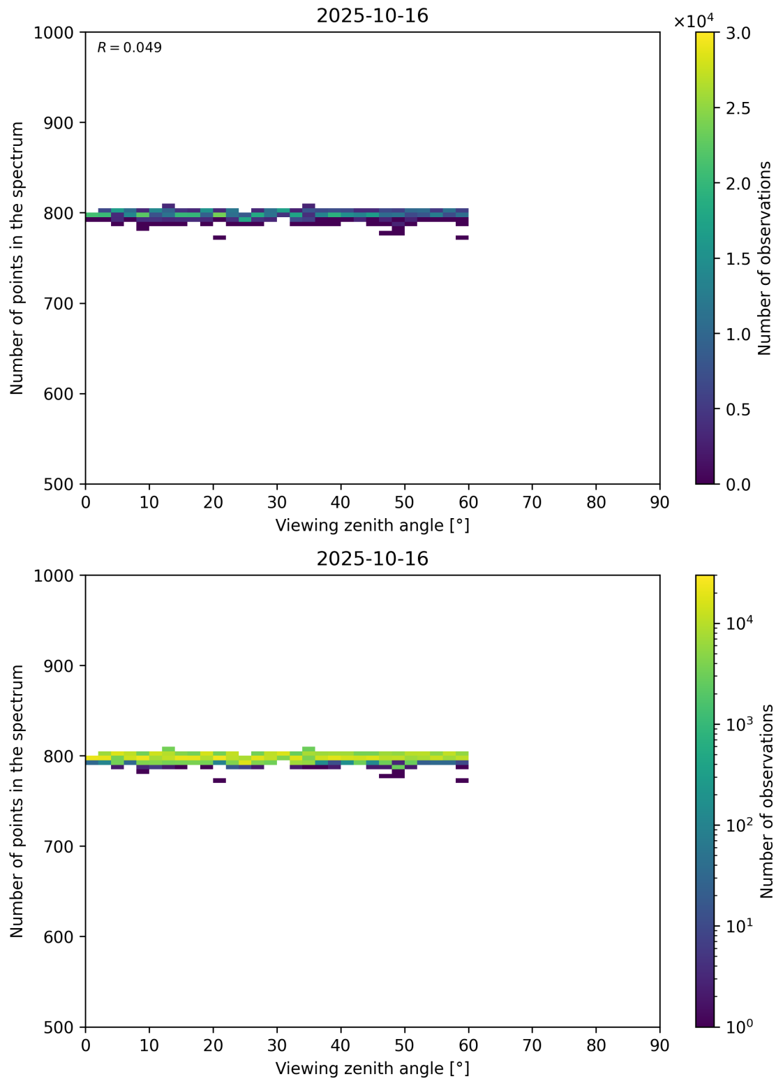
Figure 114: Scatter density plot of “Viewing zenith angle” against “Number of points in the spectrum” for 2025-10-15 to 2025-10-17.
