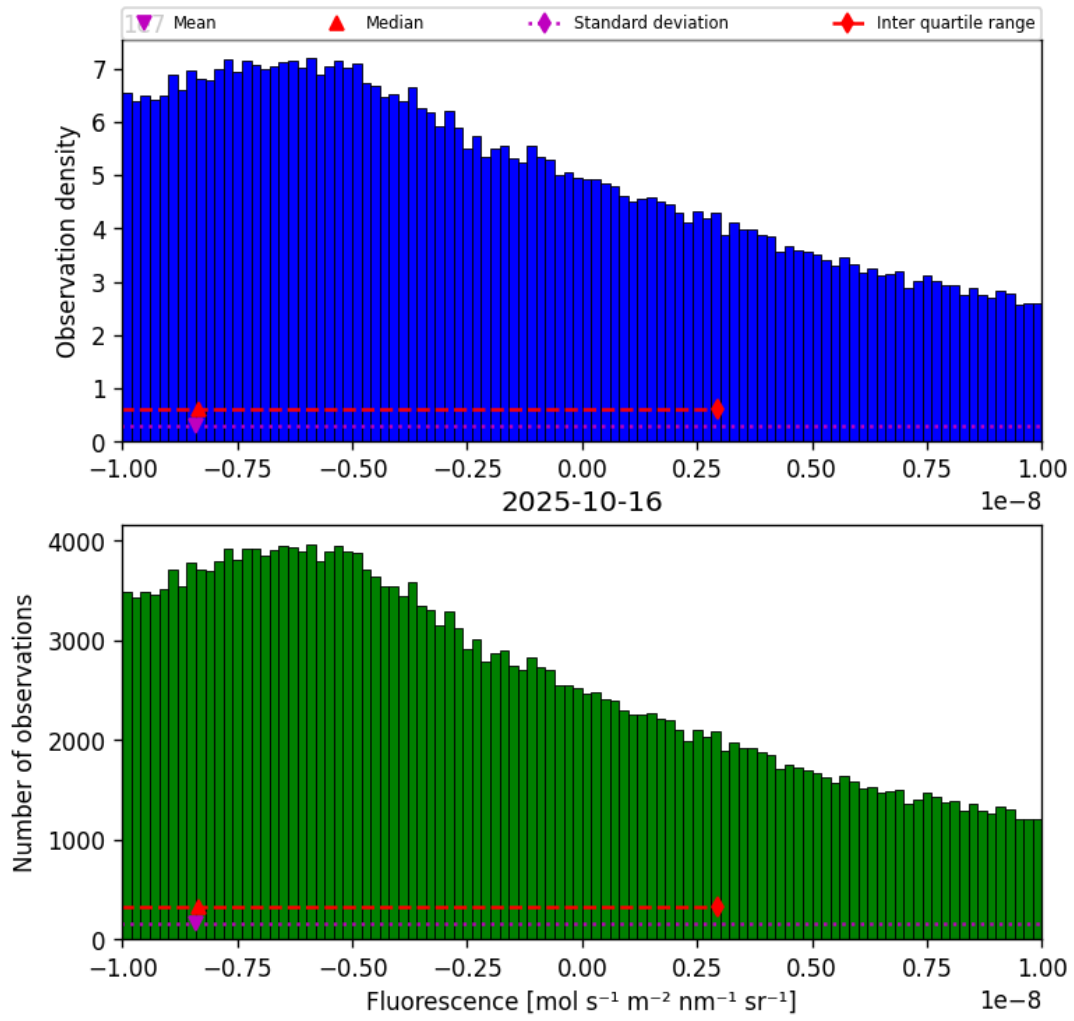
Figure 32: Histogram of “Fluorescence” for 2025-10-15 to 2025-10-17
