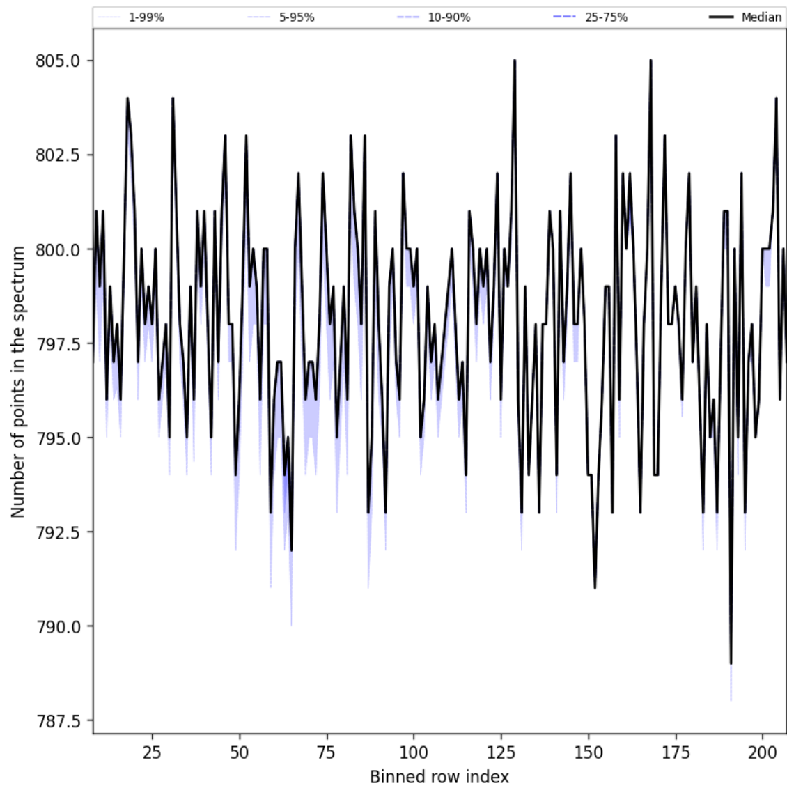
Figure 37: Along track statistics of “Number of points in the spectrum” for 2025-10-15 to 2025-10-17
