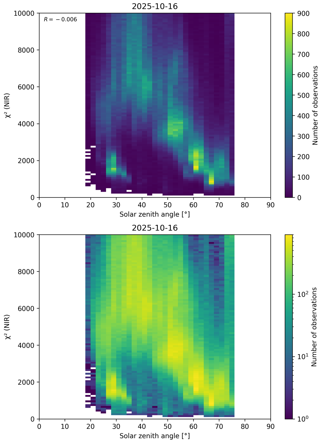
Figure 94: Scatter density plot of “Solar zenith angle” against “ \chi^2 (NIR)” for 2025-10-15 to 2025-10-17.
