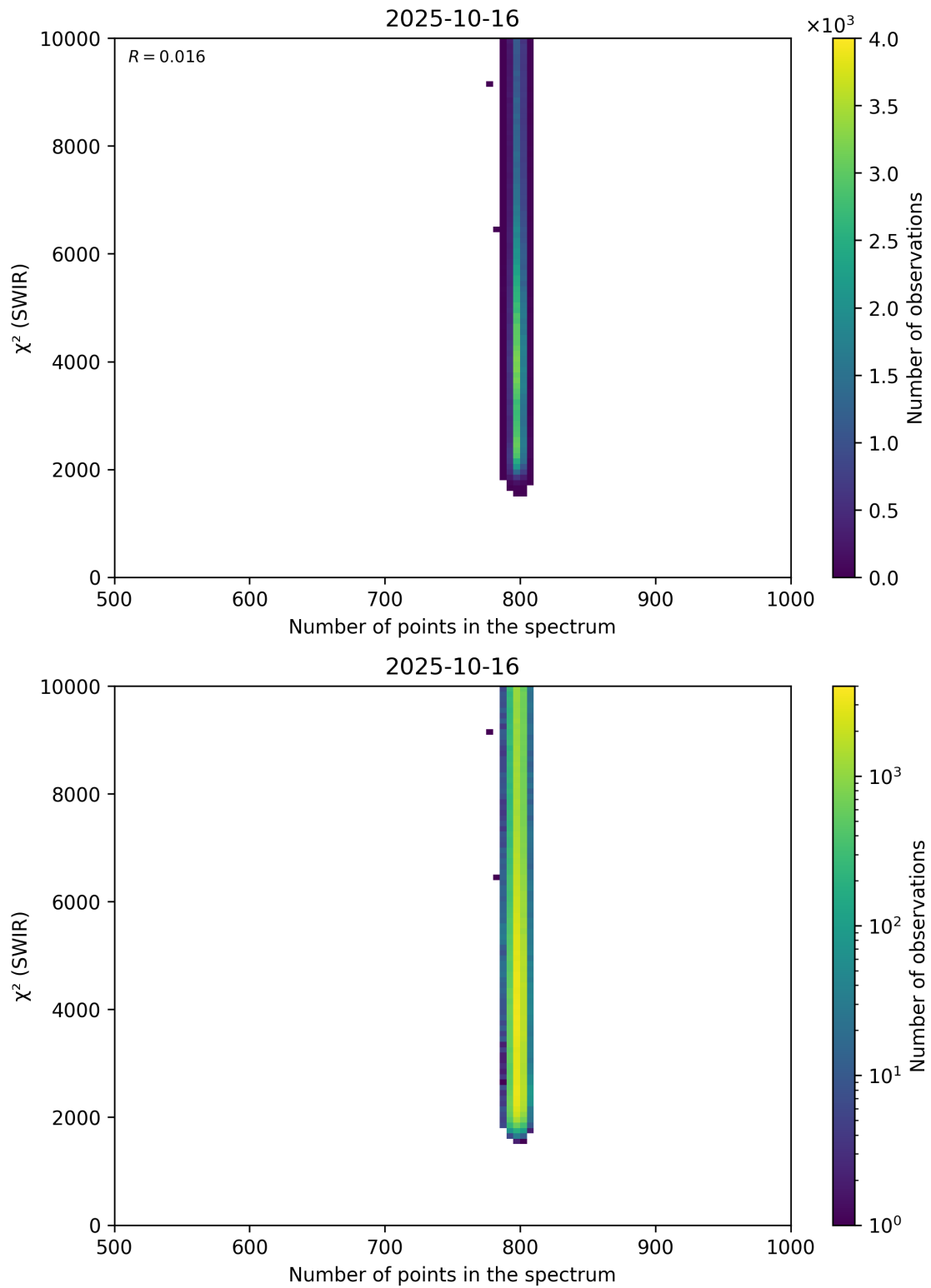
Figure 89: Scatter density plot of “Number of points in the spectrum” against “ \chi^2 (SWIR)” for 2025-10-15 to 2025-10-17.
