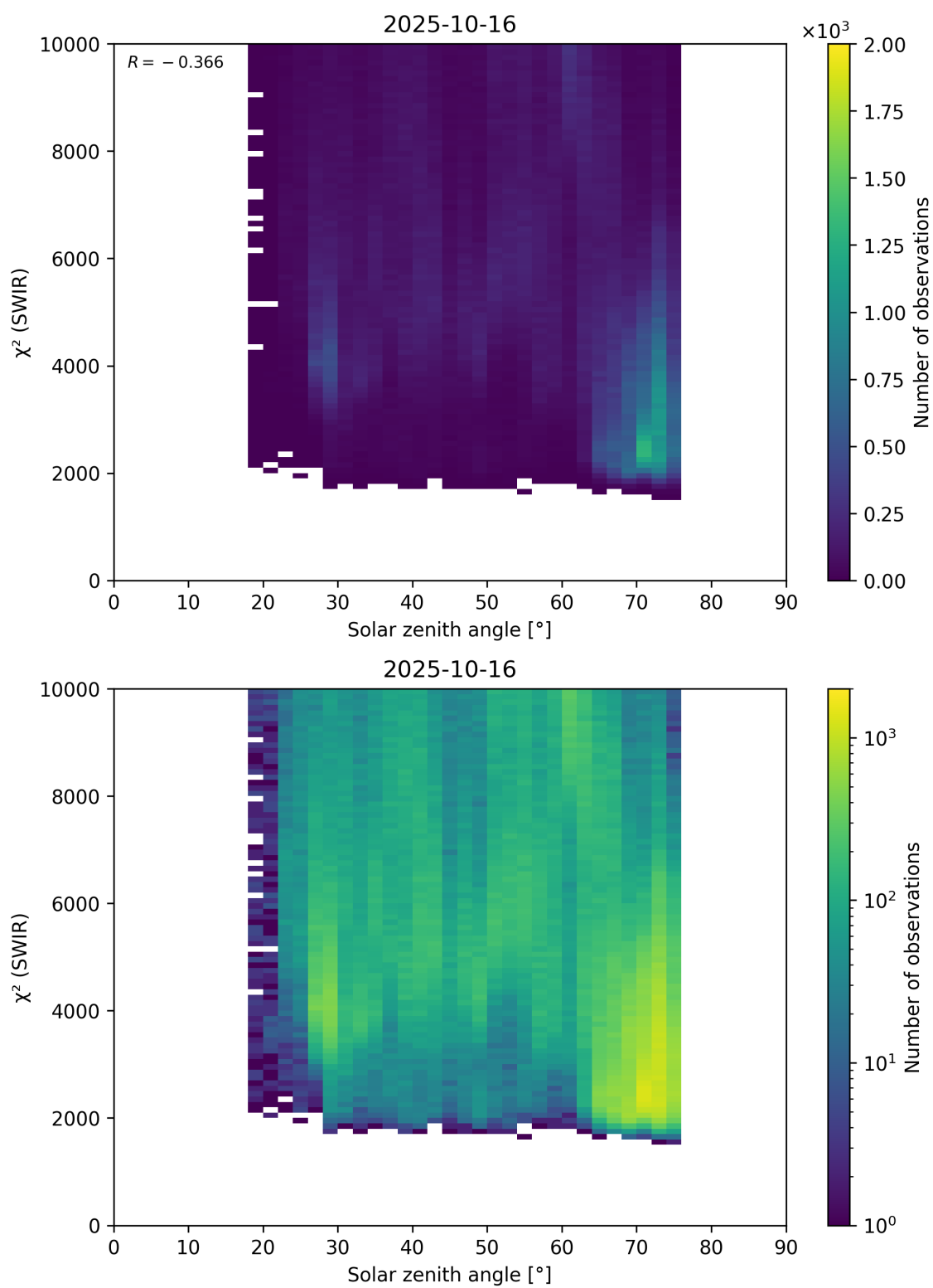
Figure 95: Scatter density plot of “Solar zenith angle” against “ \chi^2 (SWIR)” for 2025-10-15 to 2025-10-17.
