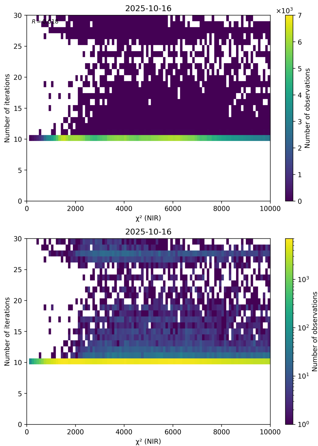
Figure 46: Scatter density plot of “ \chi^2 (NIR)” against “Number of iterations” for 2025-10-15 to 2025-10-17.
