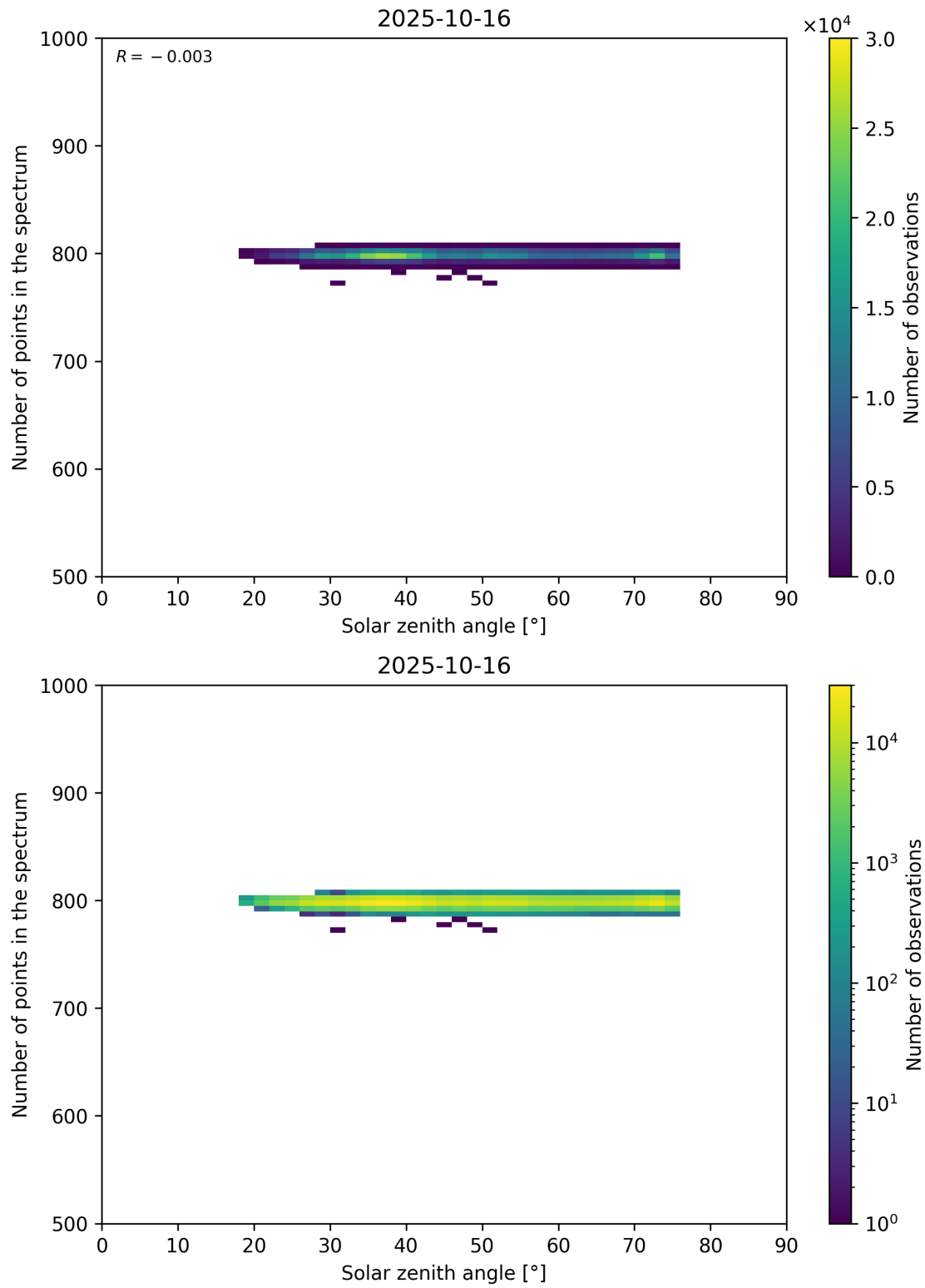
Figure 103: Scatter density plot of “Solar zenith angle” against “Number of points in the spectrum” for 2025-10-15 to 2025-10-17.
