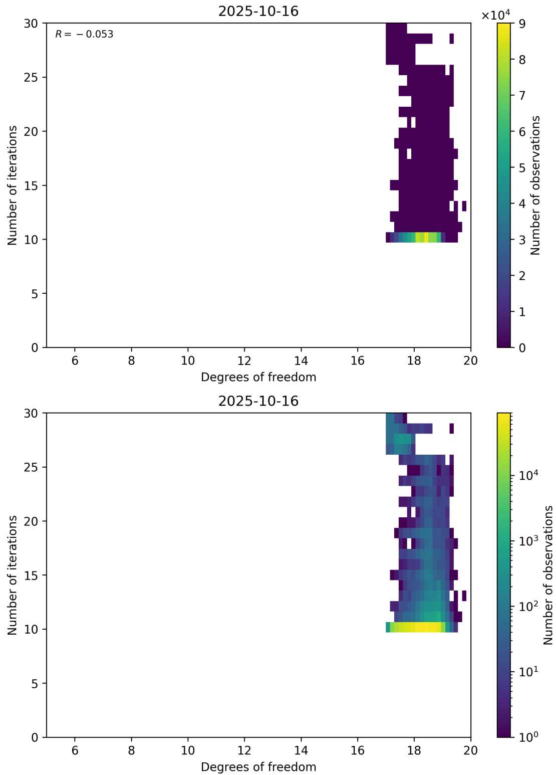
Figure 52: Scatter density plot of “Degrees of freedom” against “Number of iterations” for 2025-10-15 to 2025-10-17.
