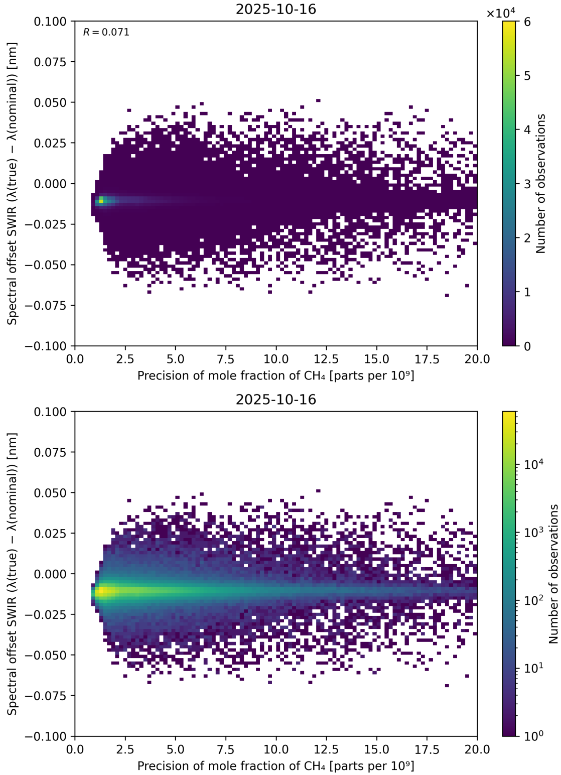
Figure 85: Scatter density plot of “Precision of mole fraction of \text{CH}_4 ” against “Spectral offset SWIR ( \lambda_{\text{true}} - \lambda_{\text{nominal}} )” for 2025-10-15 to 2025-10-17.
