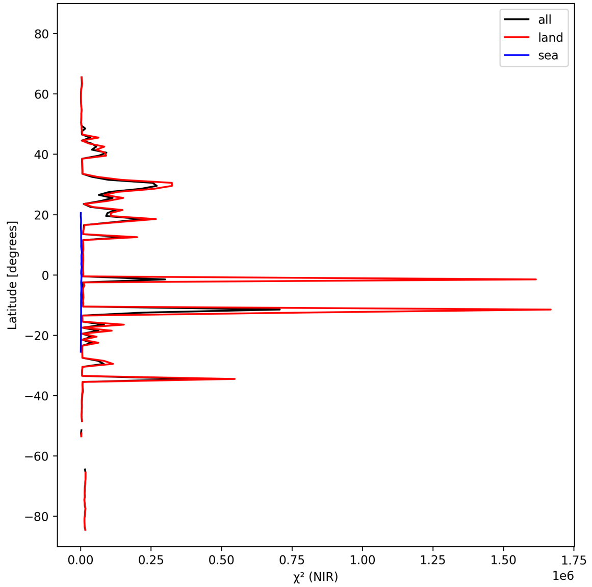
Figure 18: Zonal average of “ \chi^2 (NIR)” for 2025-10-17 to 2025-10-18.
