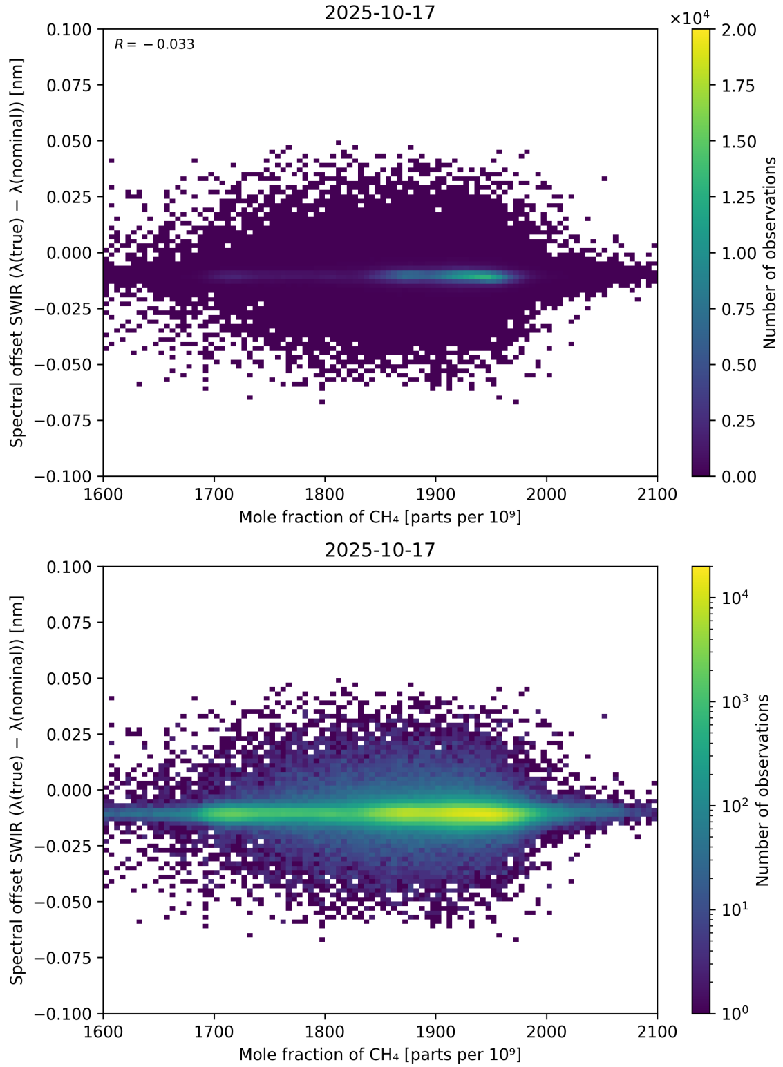
Figure 86: Scatter density plot of “Mole fraction of \text{CH}_4 ” against “Spectral offset SWIR ( \lambda_{\text{true}} - \lambda_{\text{nominal}} )” for 2025-10-17 to 2025-10-18.
