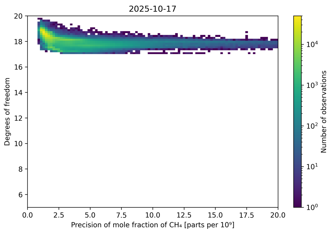
Figure 80: Scatter density plot of “Precision of mole fraction of CH 4 ” against “Degrees of freedom” for 2025-10-17 to 2025-10-18.
