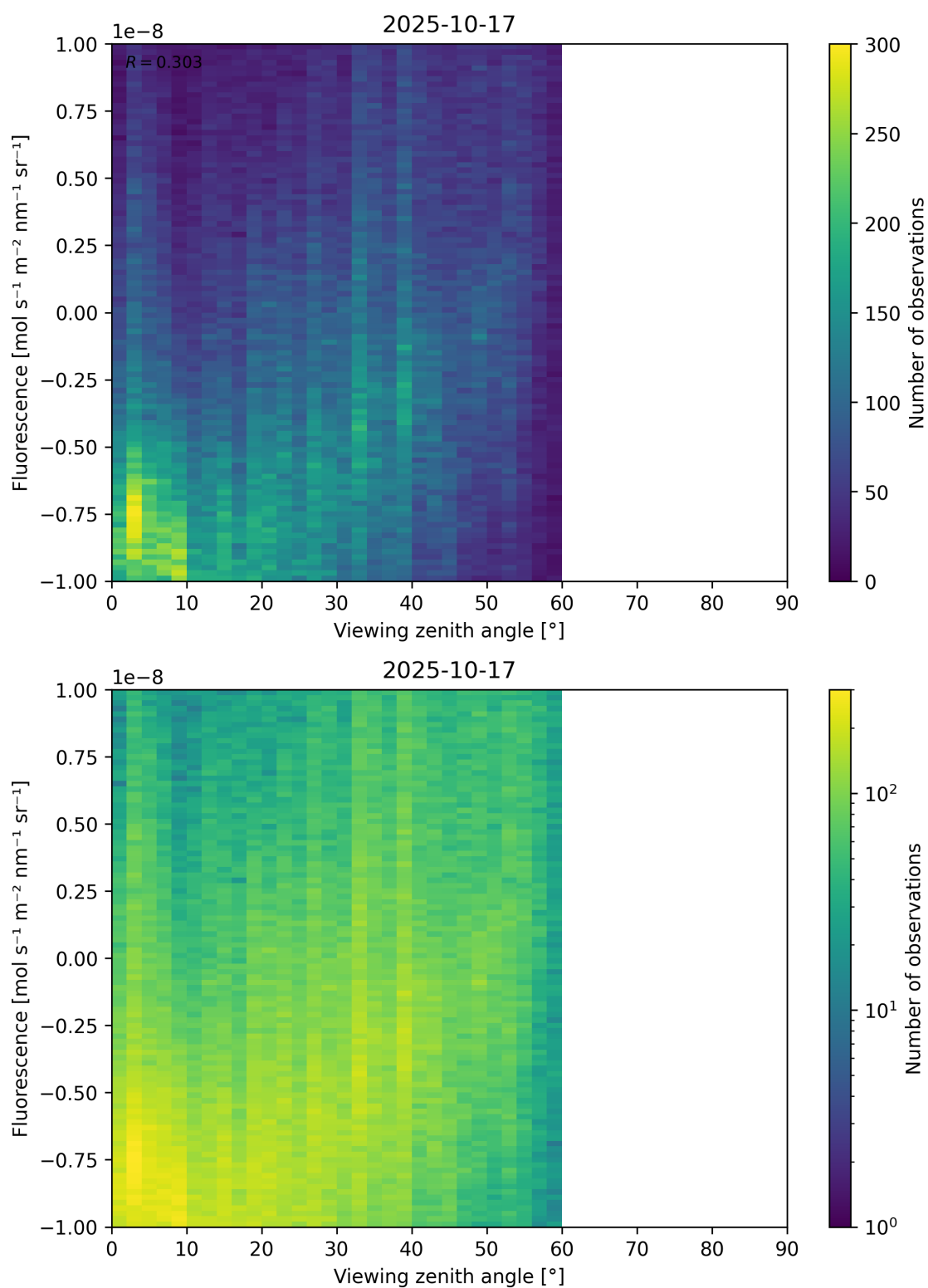
Figure 108: Scatter density plot of “Viewing zenith angle” against “Fluorescence” for 2025-10-17 to 2025-10-18.
