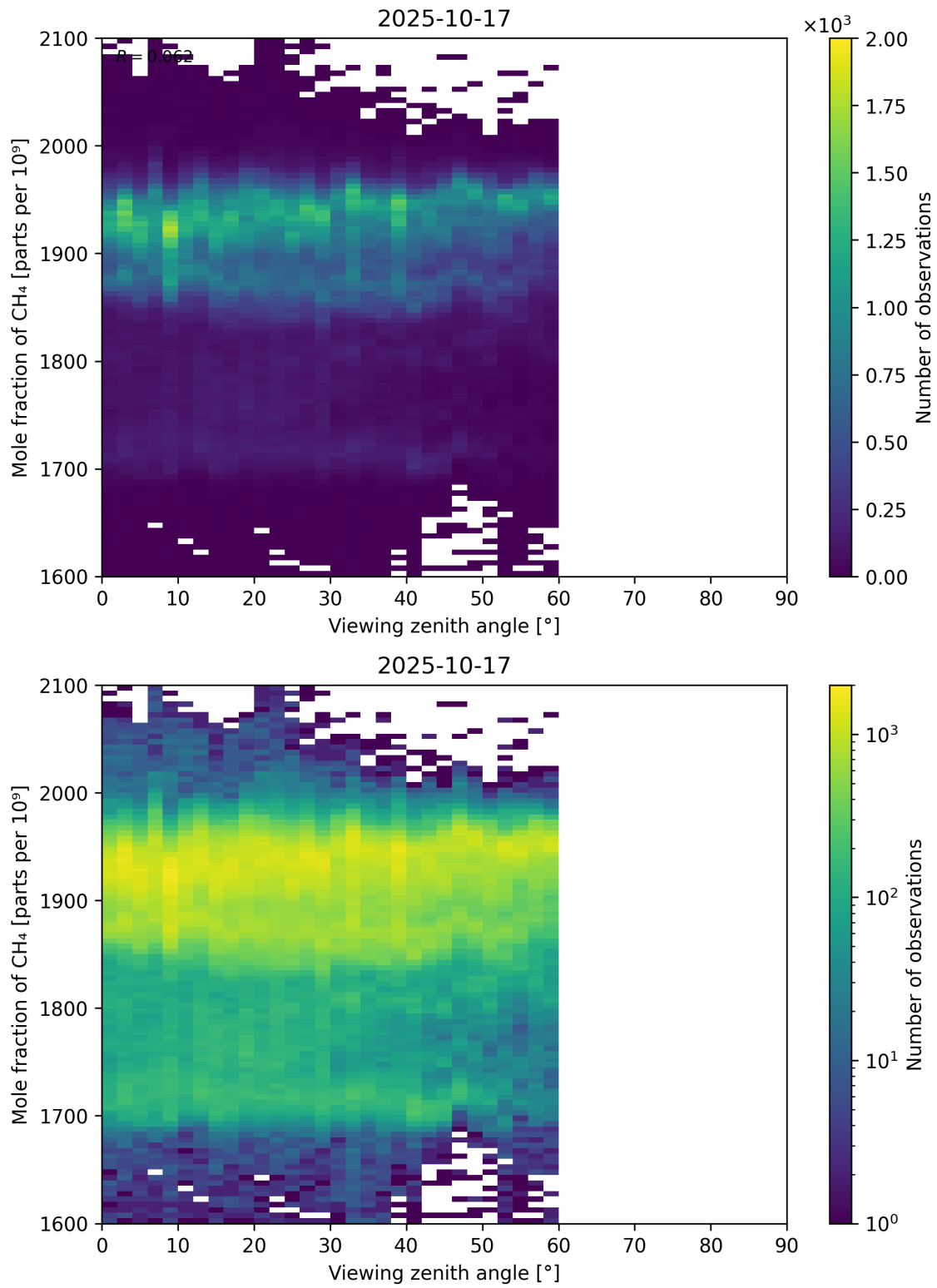
Figure 110: Scatter density plot of “Viewing zenith angle” against “Mole fraction of CH 4 ” for 2025-10-17 to 2025-10-18.
