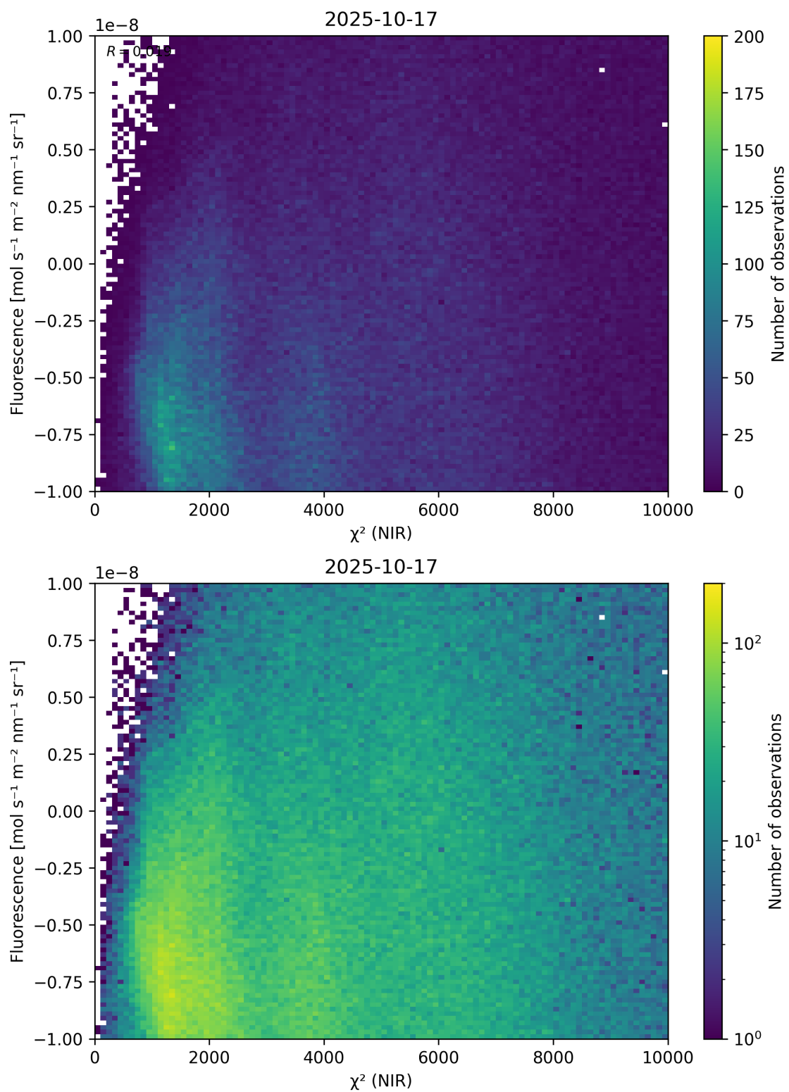
Figure 45: Scatter density plot of “ \chi^2 (NIR)” against “Fluorescence” for 2025-10-17 to 2025-10-18.
