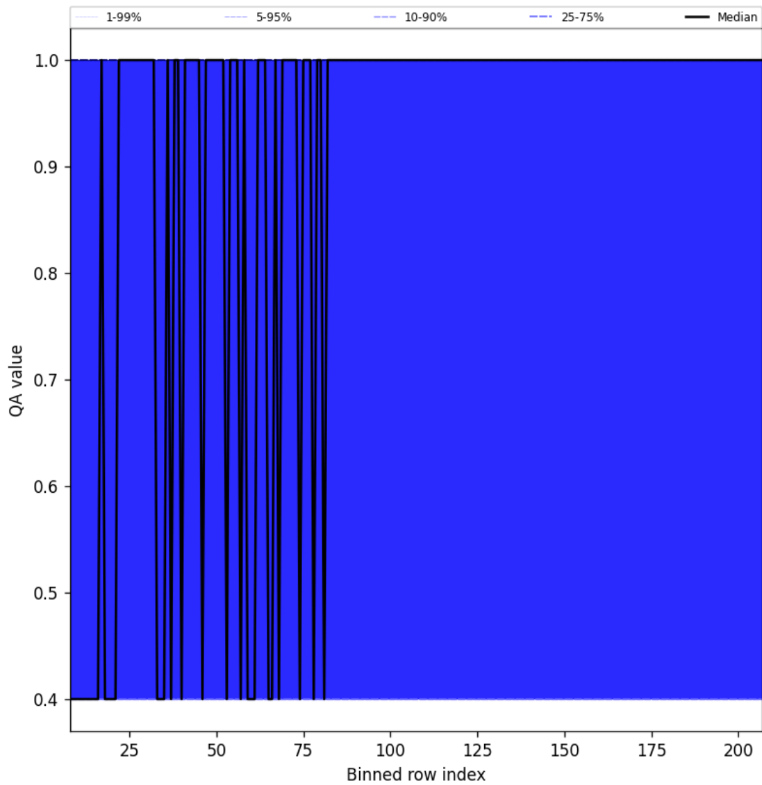
Figure 33: Along track statistics of “QA value” for 2025-10-17 to 2025-10-18
