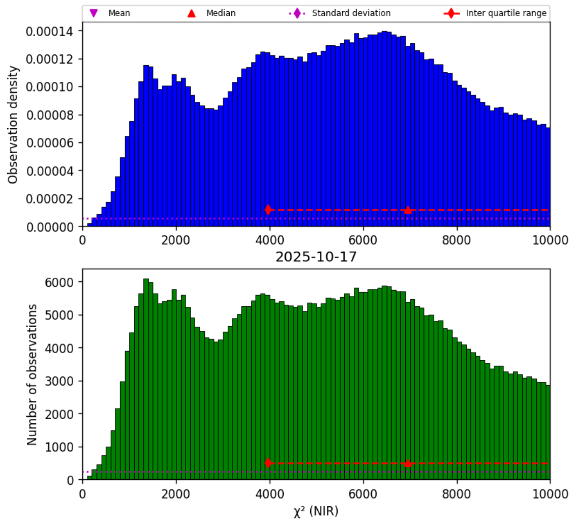
Figure 29: Histogram of “ \chi^2 (NIR)” for 2025-10-17 to 2025-10-18
