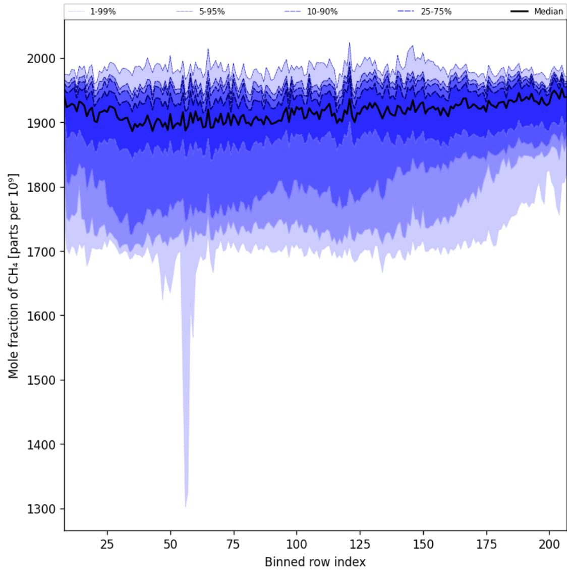
Figure 34: Along track statistics of “Mole fraction of CH 4 ” for 2025-10-17 to 2025-10-18
