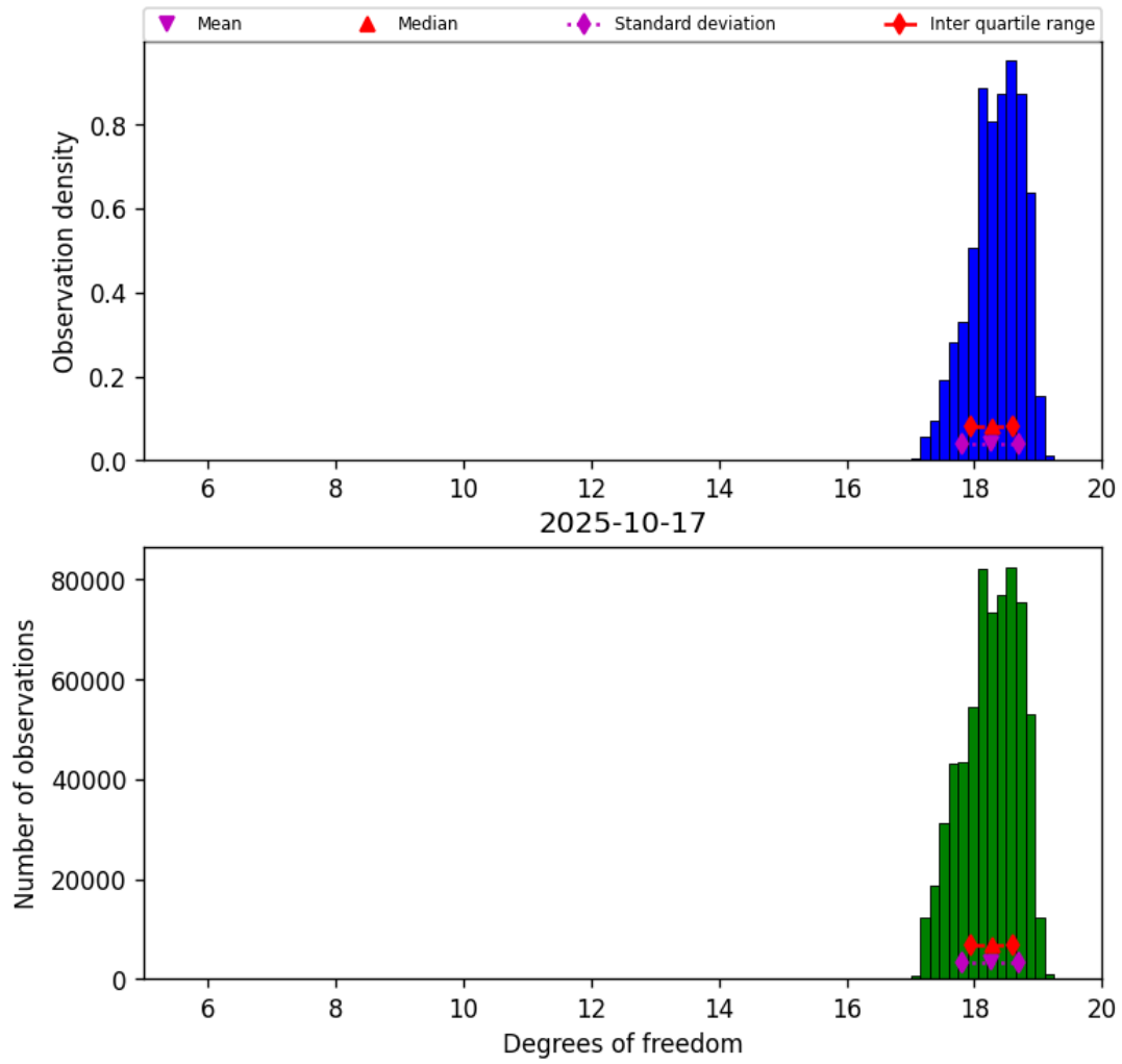
Figure 30: Histogram of “Degrees of freedom” for 2025-10-17 to 2025-10-18
