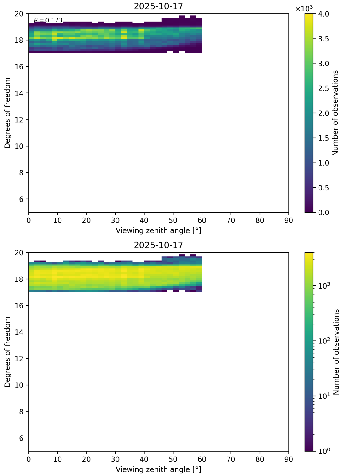
Figure 107: Scatter density plot of “Viewing zenith angle” against “Degrees of freedom” for 2025-10-17 to 2025-10-18.
