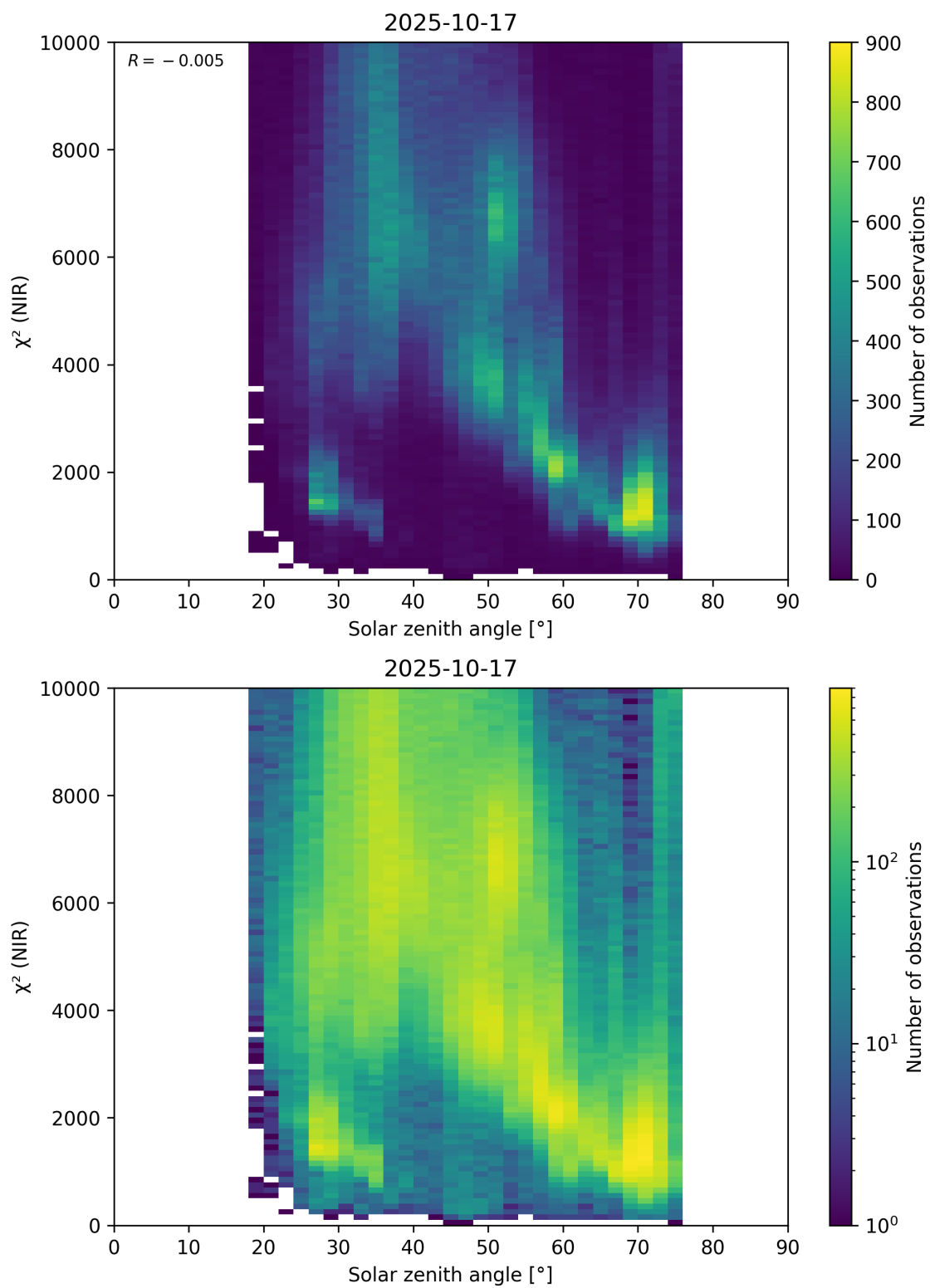
Figure 94: Scatter density plot of “Solar zenith angle” against “ \chi^2 (NIR)” for 2025-10-17 to 2025-10-18.
