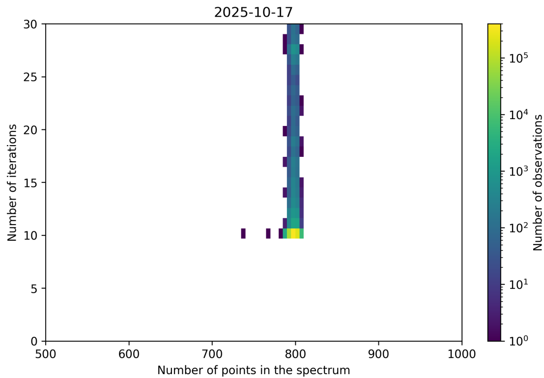
Figure 92: Scatter density plot of “Number of points in the spectrum” against “Number of iterations” for 2025-10-17 to 2025-10-18.
