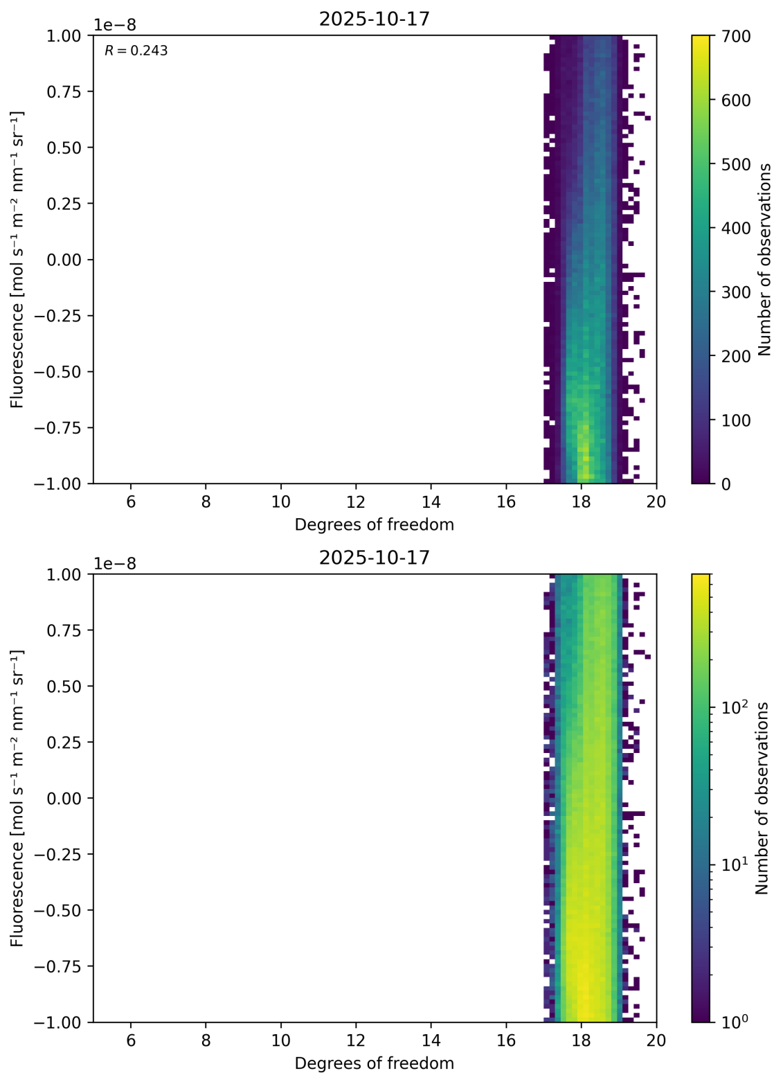
Figure 51: Scatter density plot of “Degrees of freedom” against “Fluorescence” for 2025-10-17 to 2025-10-18.
