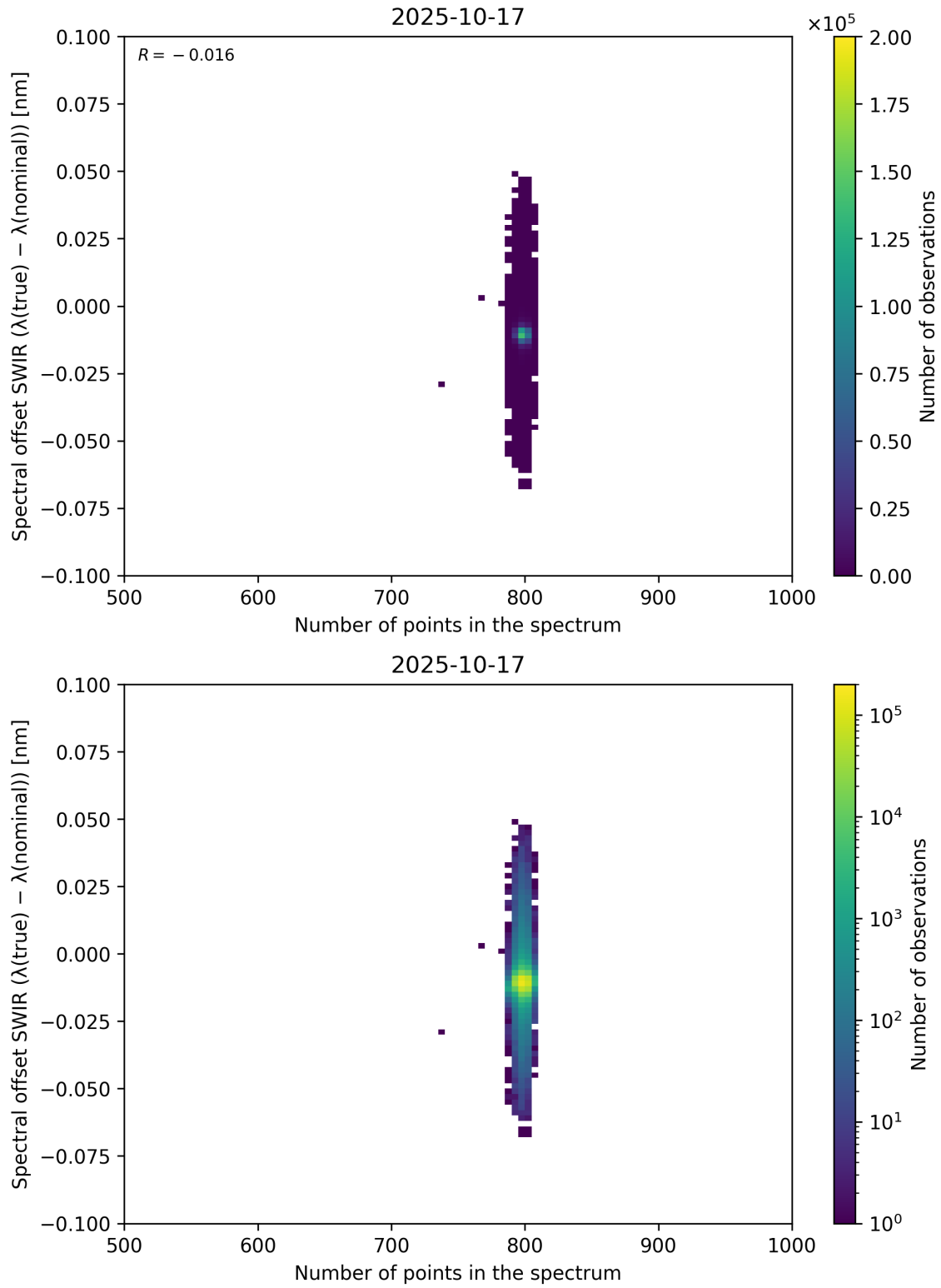
Figure 93: Scatter density plot of “Number of points in the spectrum” against “Spectral offset SWIR ( \lambda_{\text{true}} - \lambda_{\text{nominal}} )” for 2025-10-17 to 2025-10-18.
