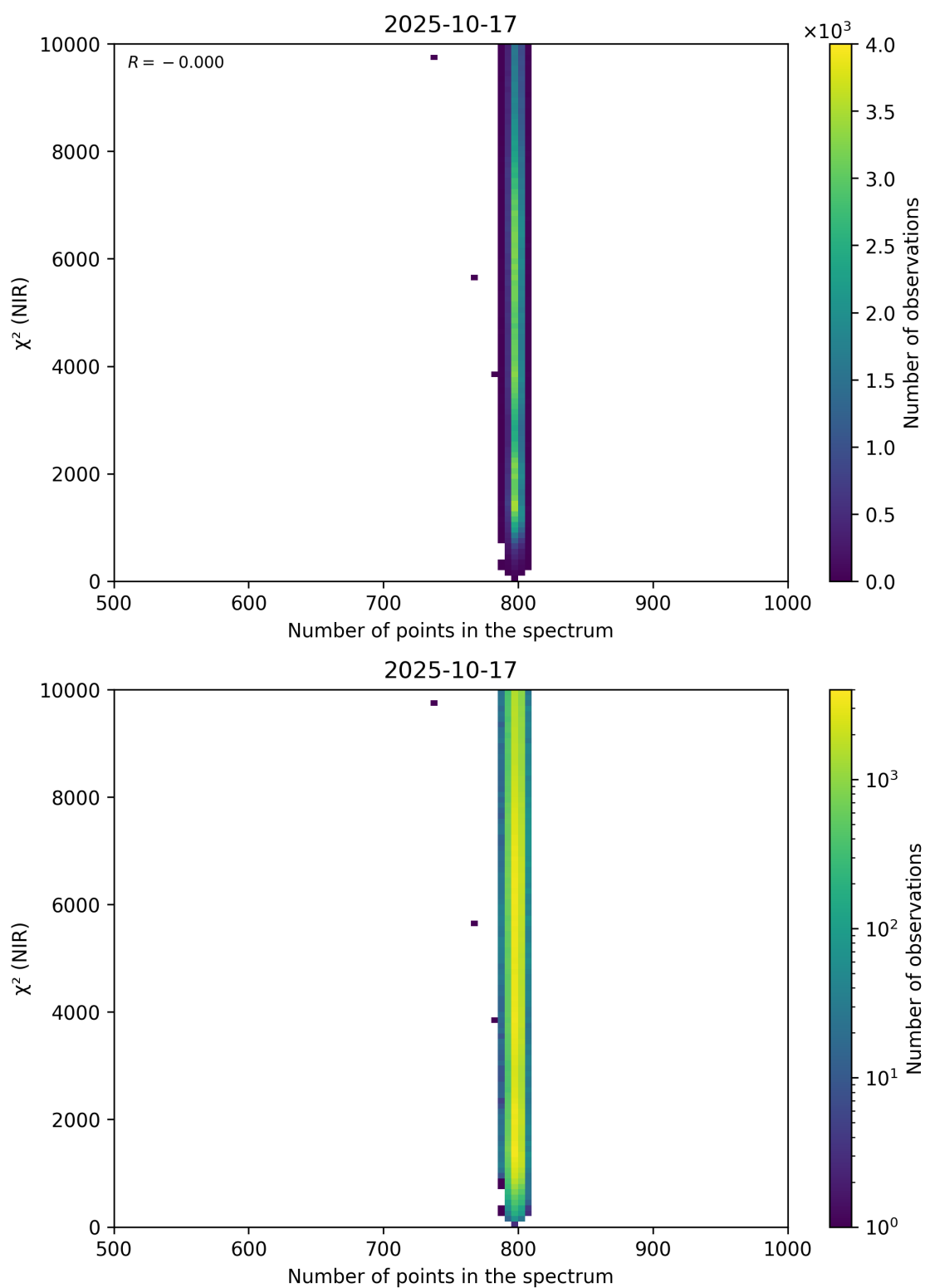
Figure 88: Scatter density plot of “Number of points in the spectrum” against “ \chi^2 (NIR)” for 2025-10-17 to 2025-10-18.
