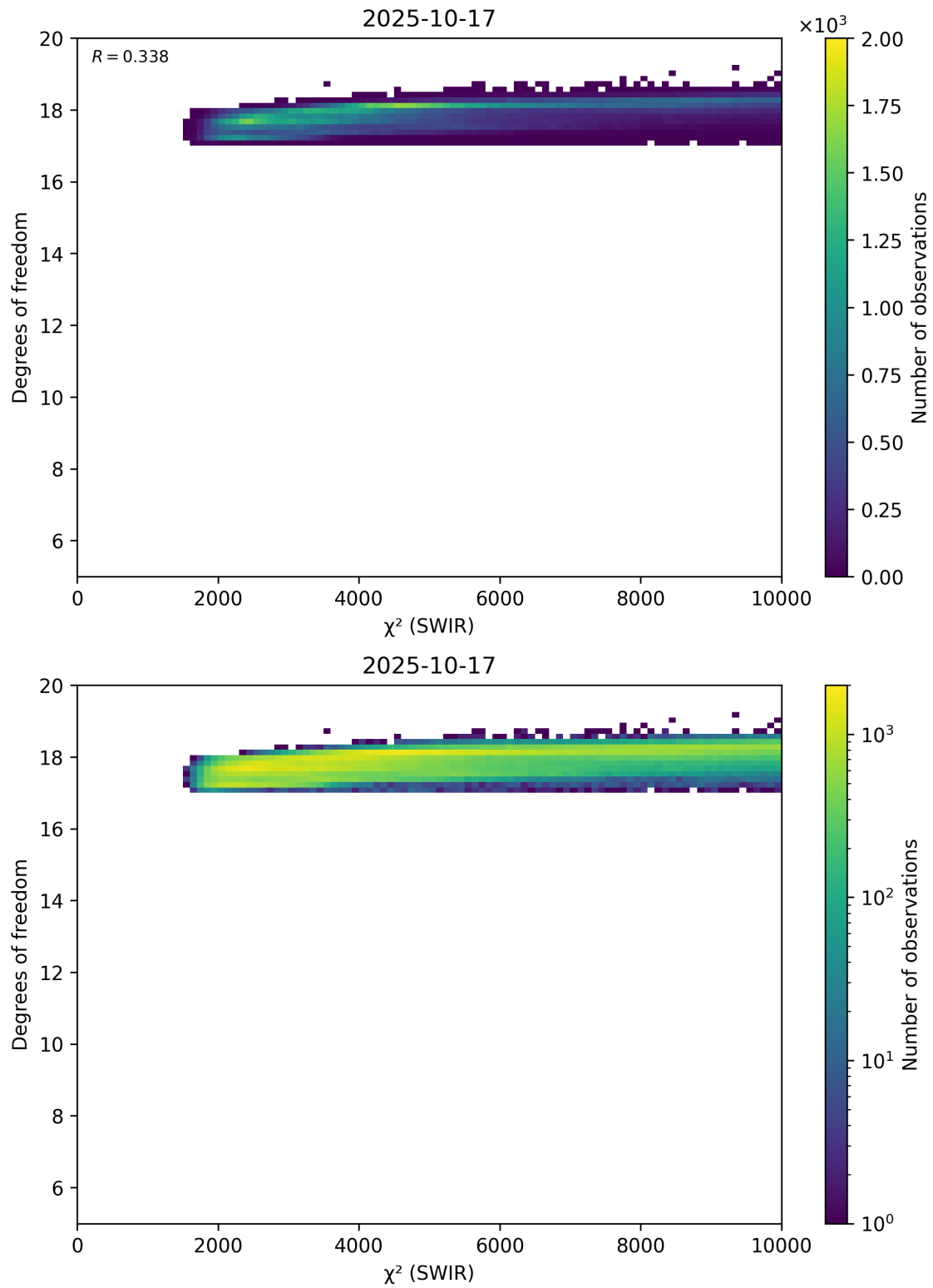
Figure 48: Scatter density plot of “ \chi^2 (SWIR)” against “Degrees of freedom” for 2025-10-17 to 2025-10-18.
