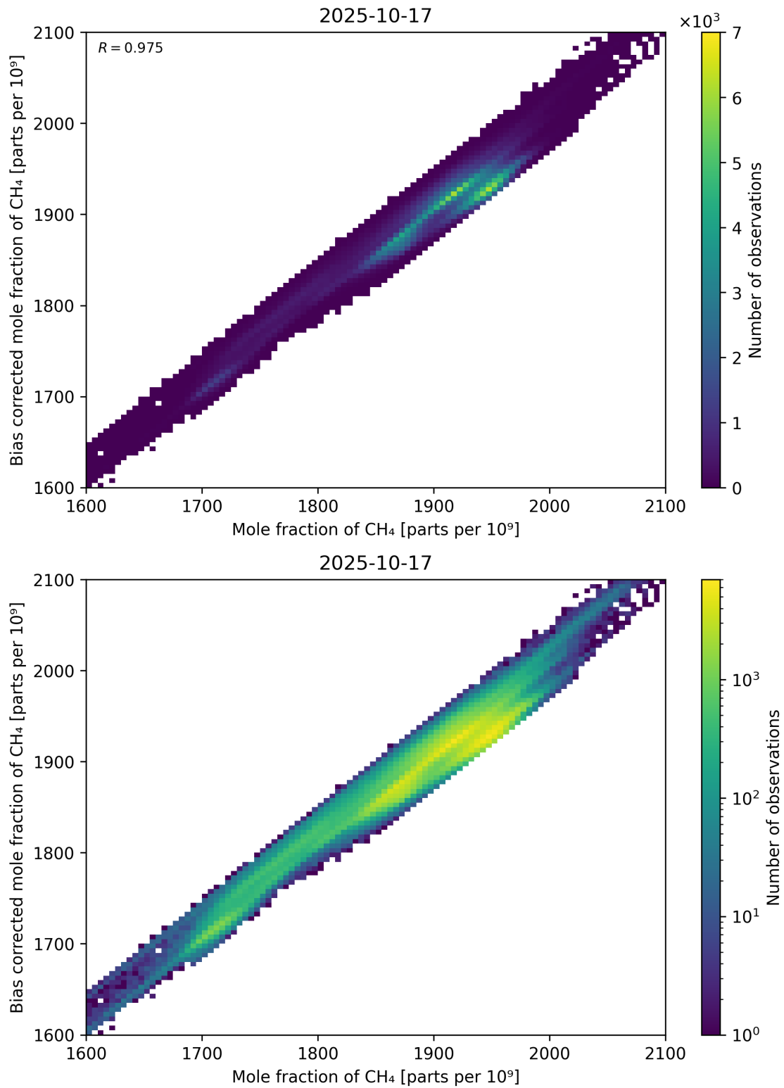
Figure 74: Scatter density plot of “Mole fraction of CH 4 ” against “Bias corrected mole fraction of CH 4 ” for 2025-10-17 to 2025-10-18.
