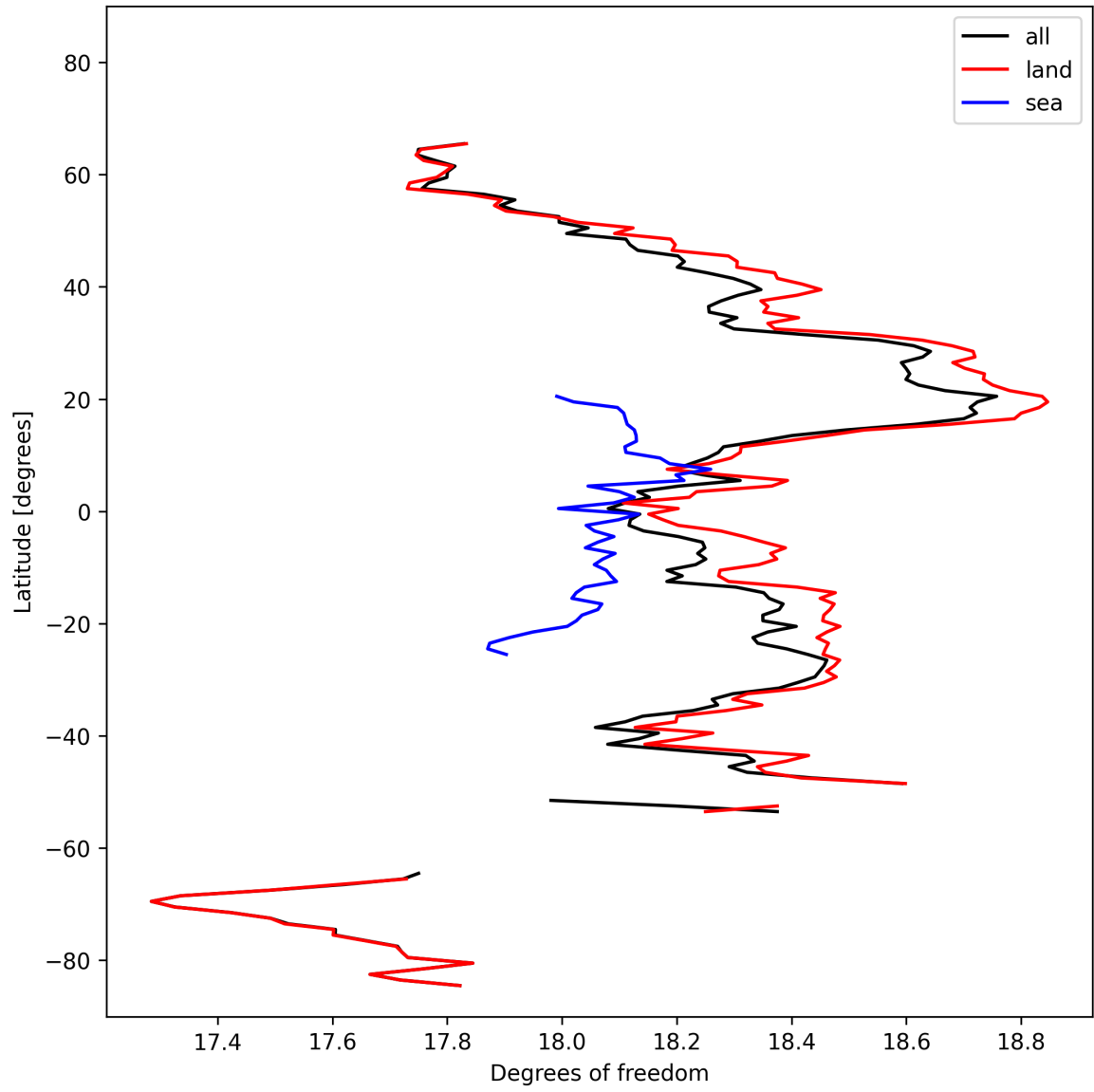
Figure 19: Zonal average of “Degrees of freedom” for 2025-10-17 to 2025-10-18.
