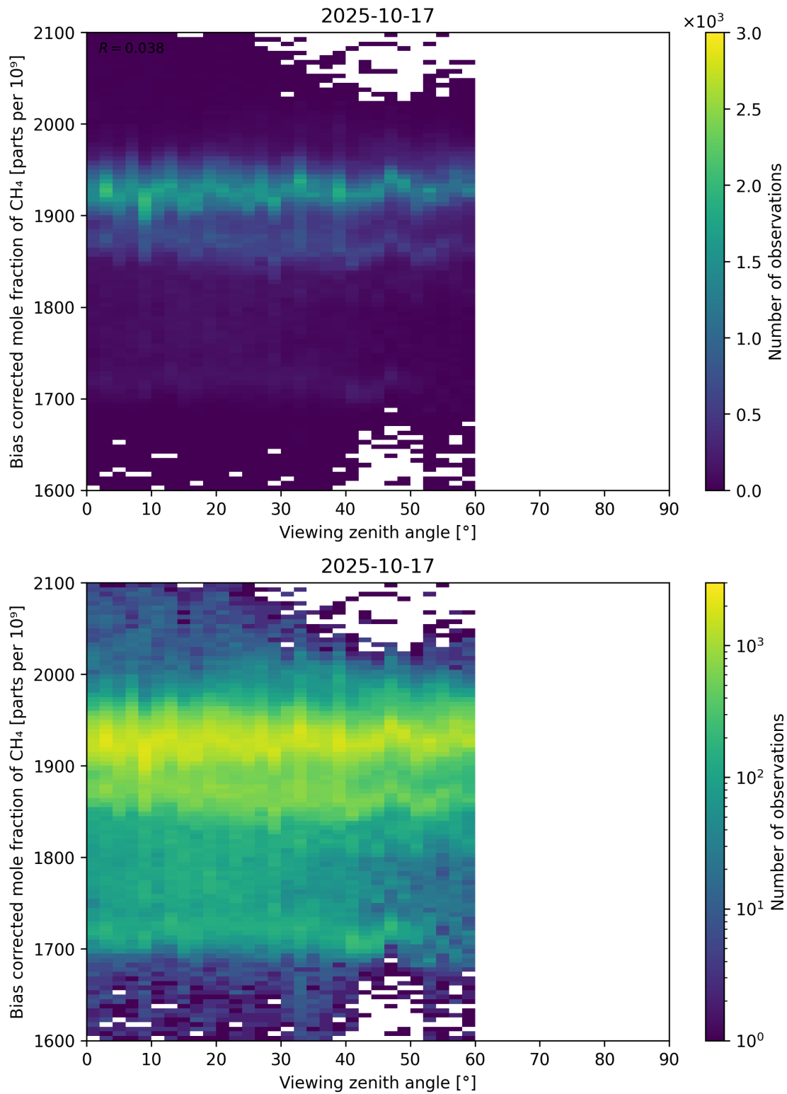
Figure 111: Scatter density plot of “Viewing zenith angle” against “Bias corrected mole fraction of CH 4 ” for 2025-10-17 to 2025-10-18.
