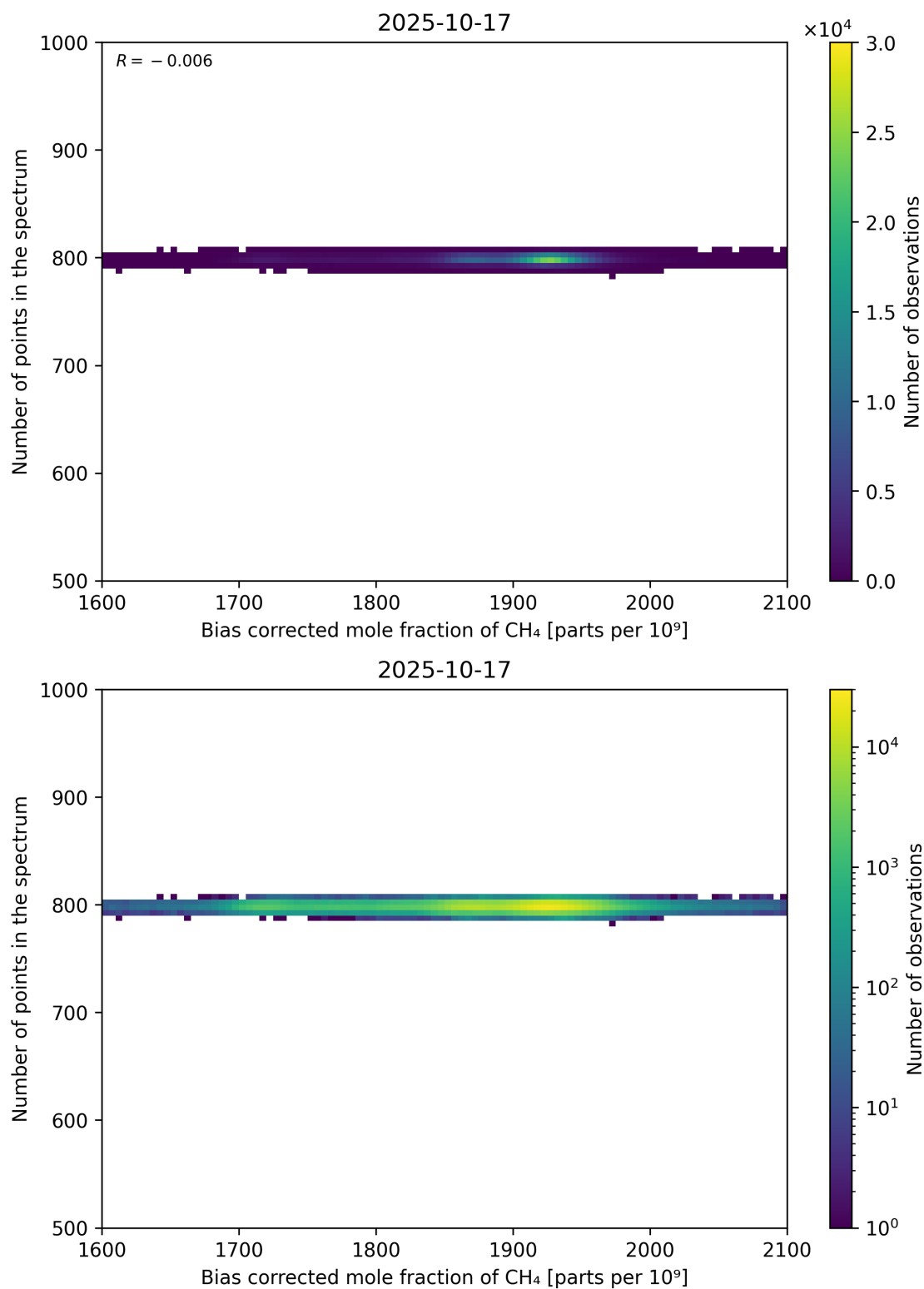
Figure 68: Scatter density plot of “Bias corrected mole fraction of CH 4 ” against “Number of points in the spectrum” for 2025-10-17 to 2025-10-18.
