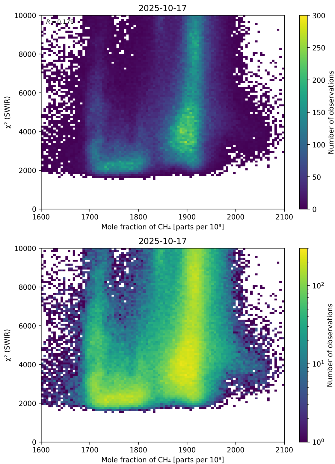
Figure 71: Scatter density plot of “Mole fraction of \text{CH}_4 ” against “ \chi^2 (SWIR)” for 2025-10-17 to 2025-10-18.
