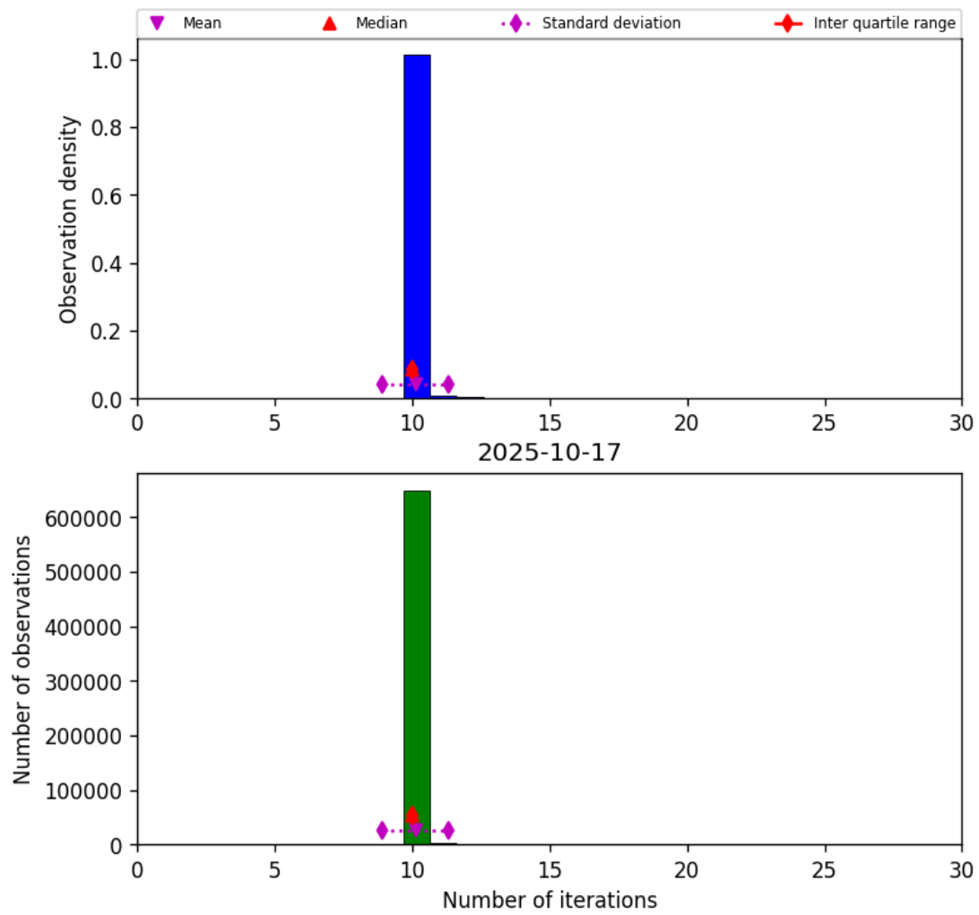
Figure 31: Histogram of “Number of iterations” for 2025-10-17 to 2025-10-18
