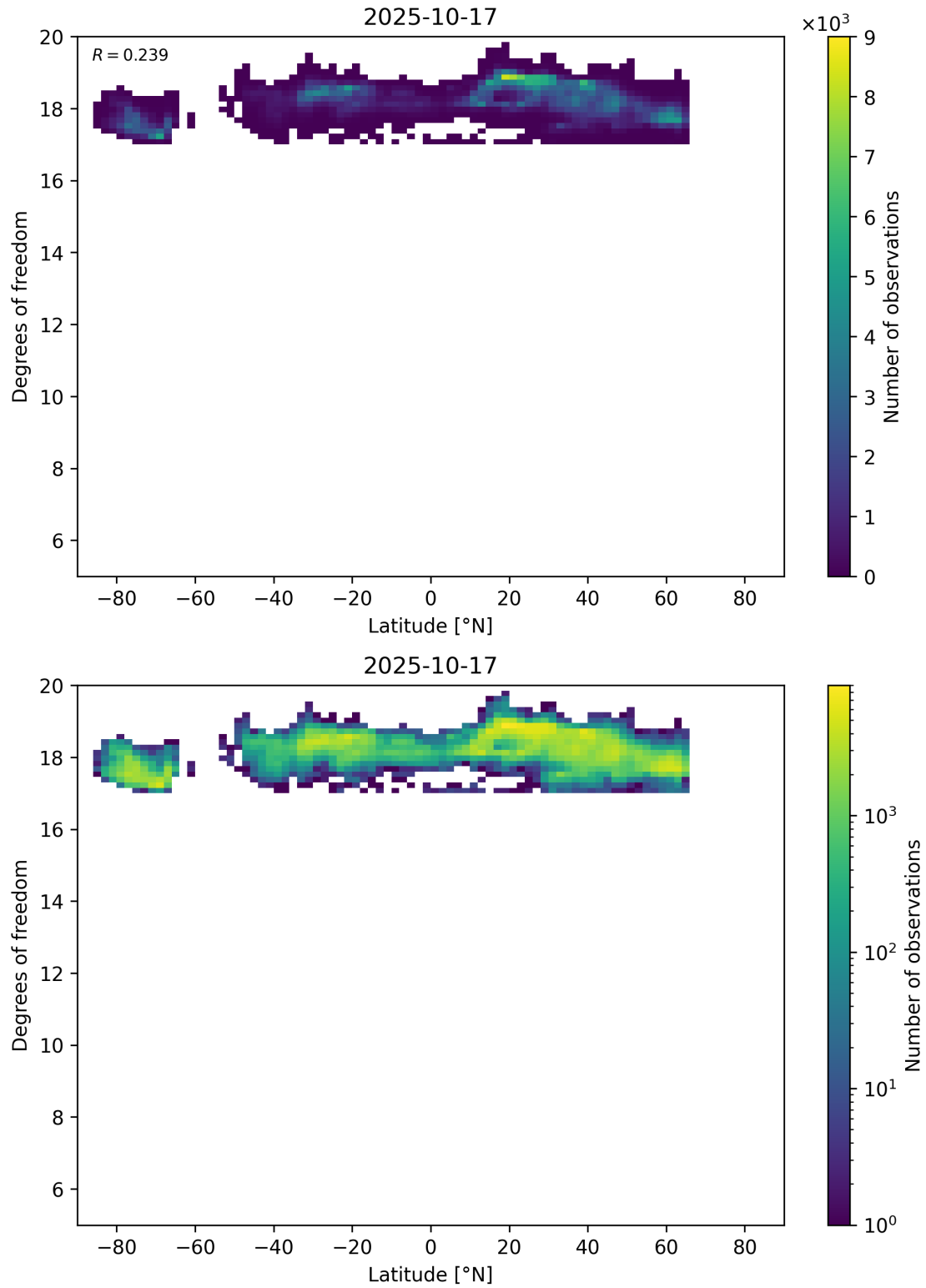
Figure 55: Scatter density plot of “Latitude” against “Degrees of freedom” for 2025-10-17 to 2025-10-18.
