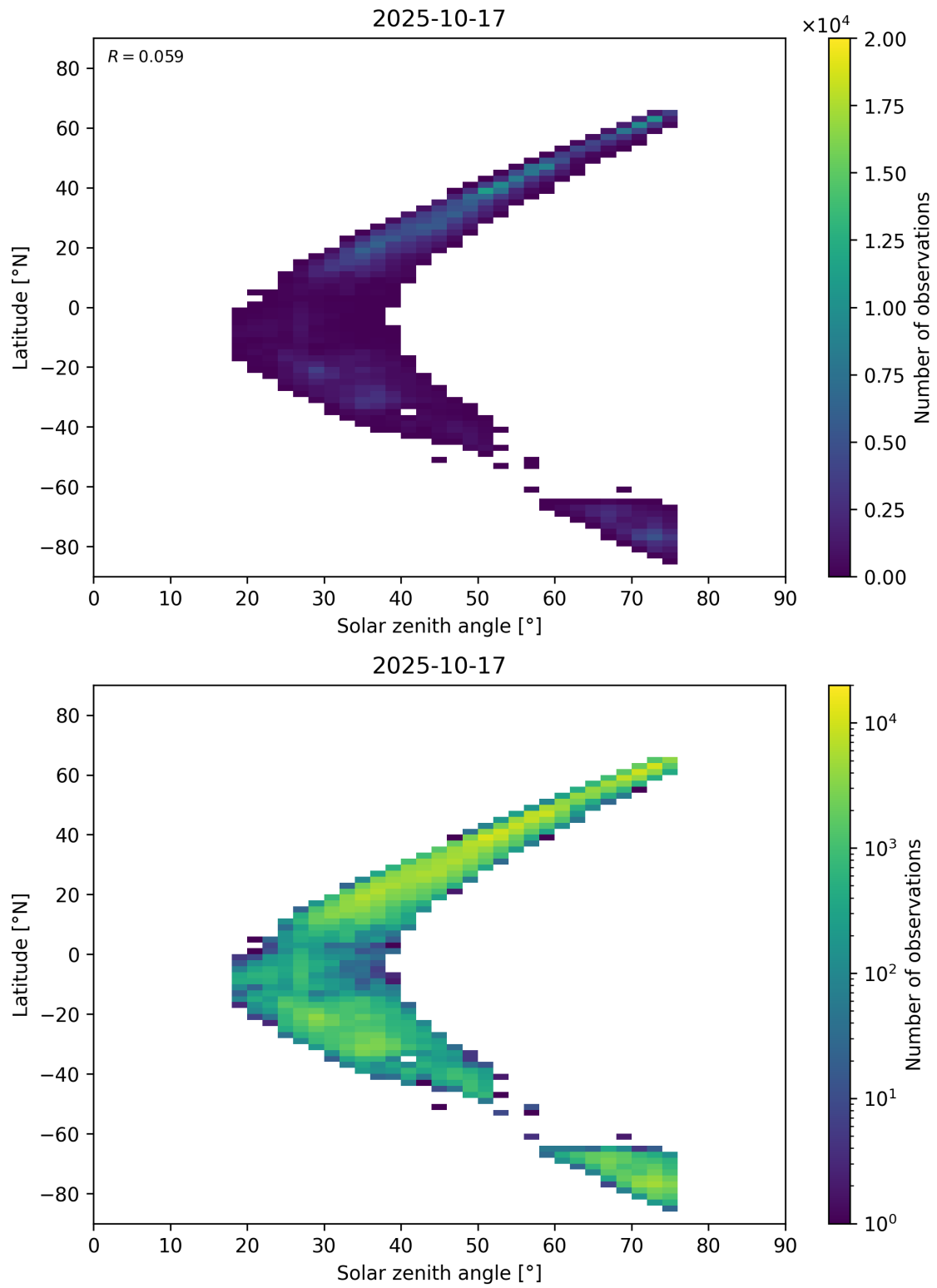
Figure 98: Scatter density plot of “Solar zenith angle” against “Latitude” for 2025-10-17 to 2025-10-18.
