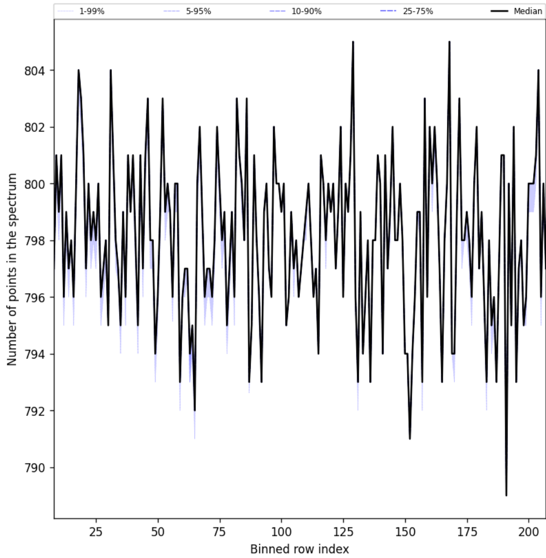
Figure 37: Along track statistics of “Number of points in the spectrum” for 2025-10-17 to 2025-10-18
