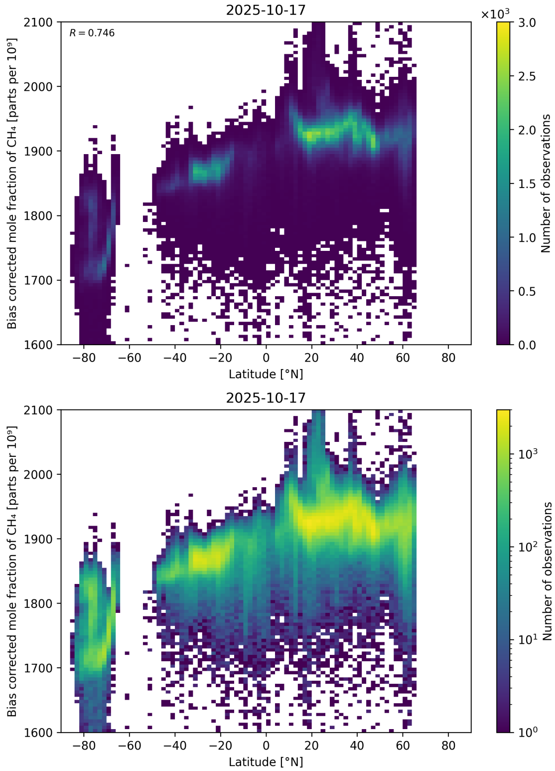
Figure 58: Scatter density plot of “Latitude” against “Bias corrected mole fraction of CH 4 ” for 2025-10-17 to 2025-10-18.
