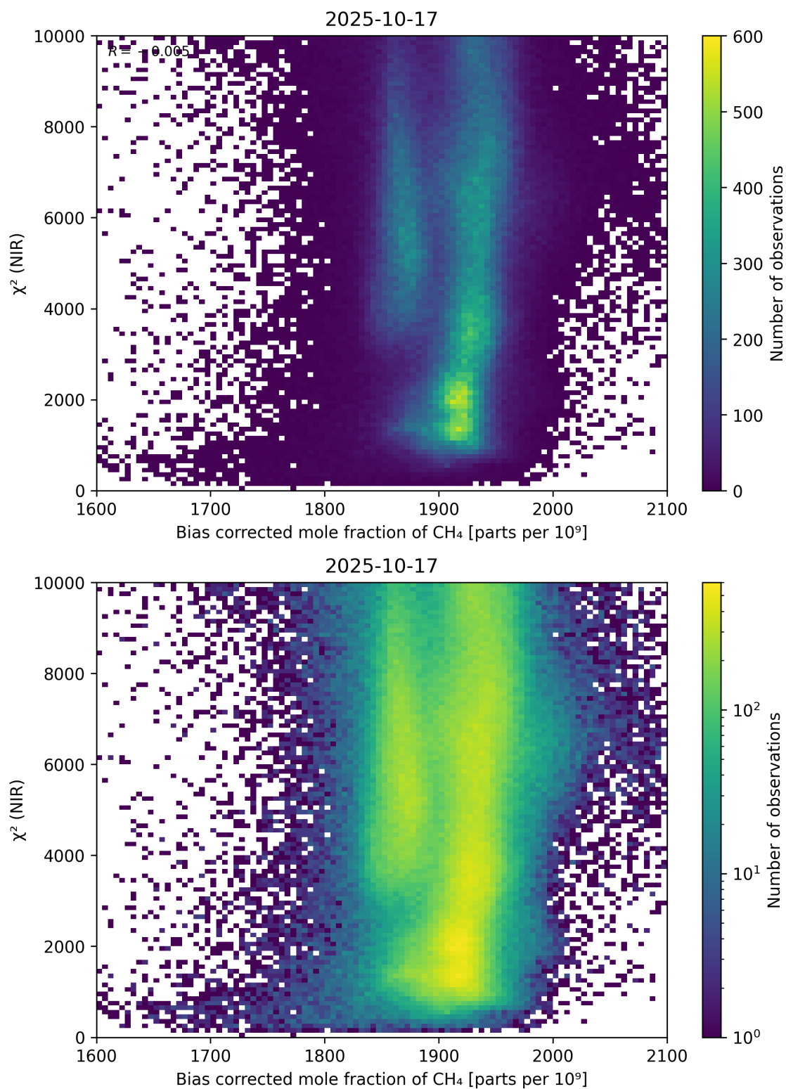
Figure 63: Scatter density plot of “Bias corrected mole fraction of \text{CH}_4 ” against “ \chi^2 (NIR)” for 2025-10-17 to 2025-10-18.
