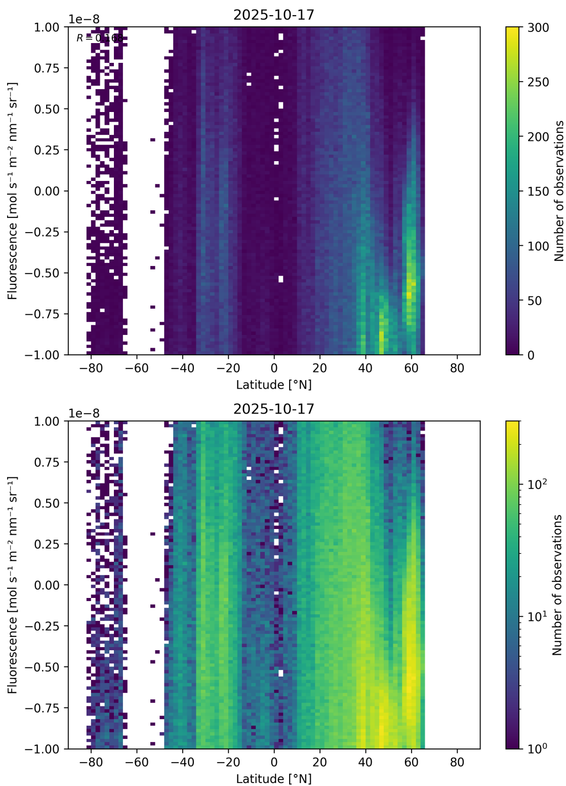
Figure 56: Scatter density plot of “Latitude” against “Fluorescence” for 2025-10-17 to 2025-10-18.
