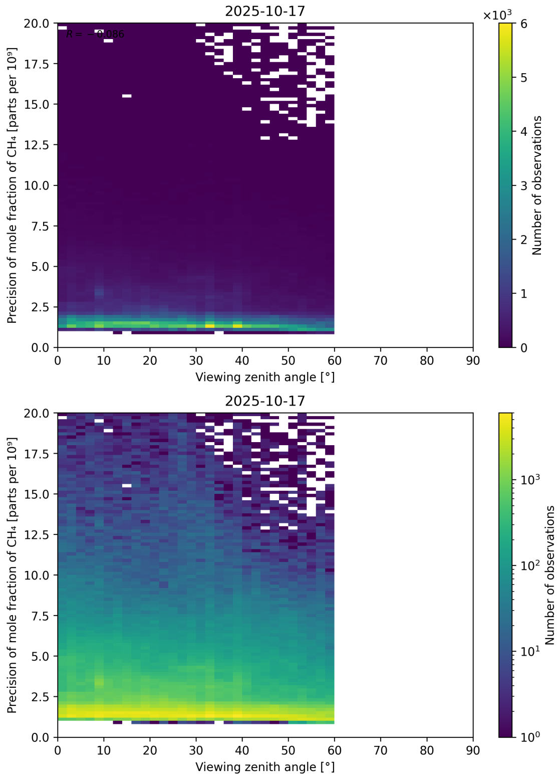
Figure 112: Scatter density plot of “Viewing zenith angle” against “Precision of mole fraction of CH 4 ” for 2025-10-17 to 2025-10-18.
