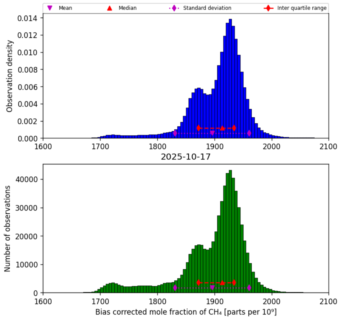
Figure 25: Histogram of “Bias corrected mole fraction of CH 4 ” for 2025-10-17 to 2025-10-18
