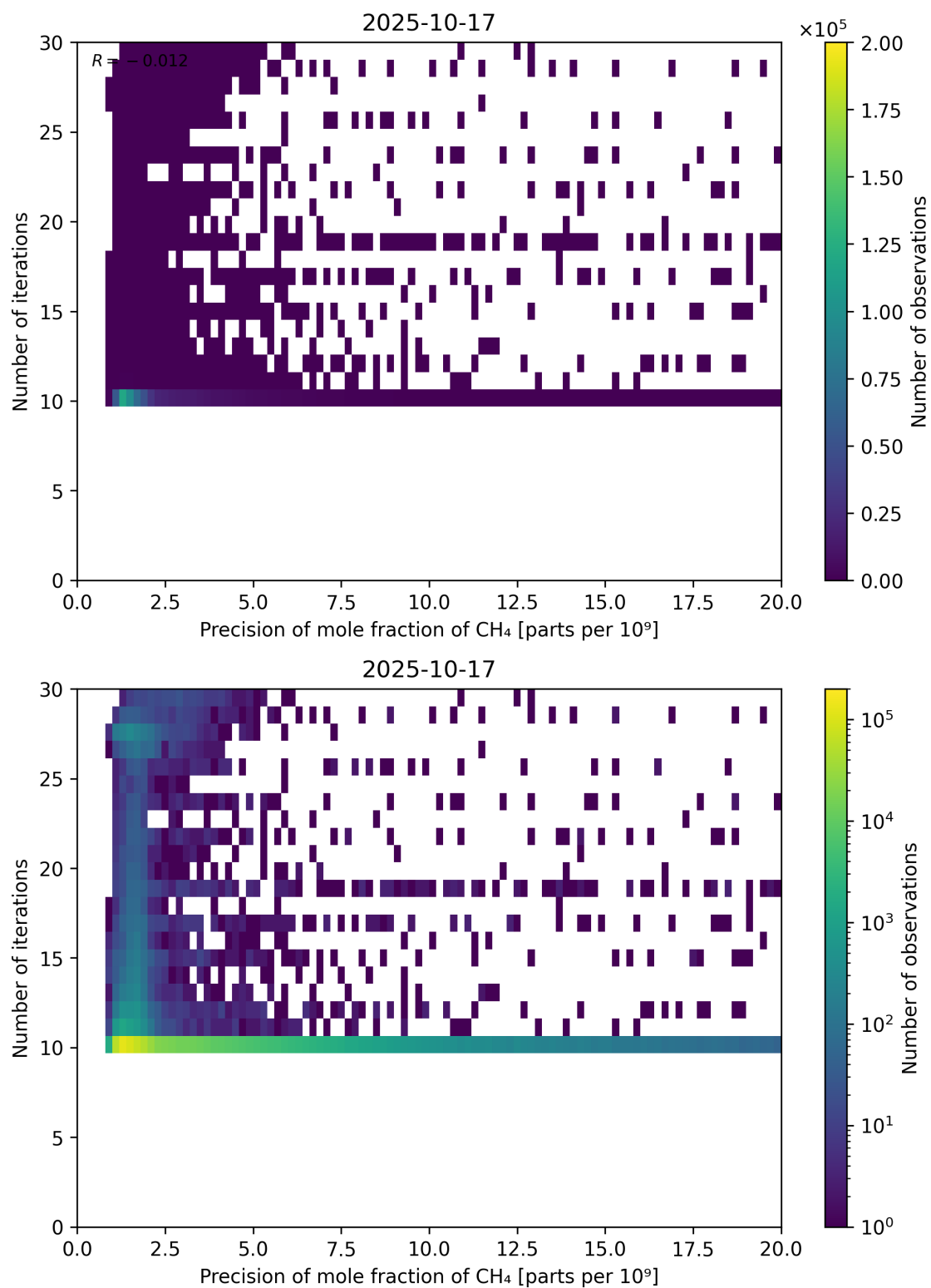
Figure 83: Scatter density plot of “Precision of mole fraction of CH 4 ” against “Number of iterations” for 2025-10-17 to 2025-10-18.
