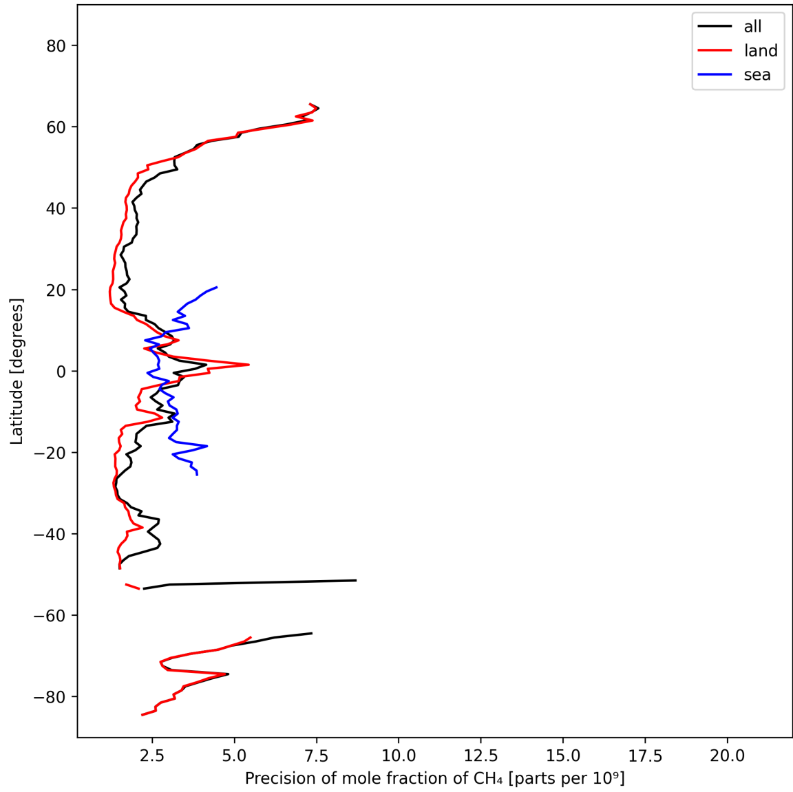
Figure 13: Zonal average of “Precision of mole fraction of CH 4 ” for 2025-10-17 to 2025-10-18.
