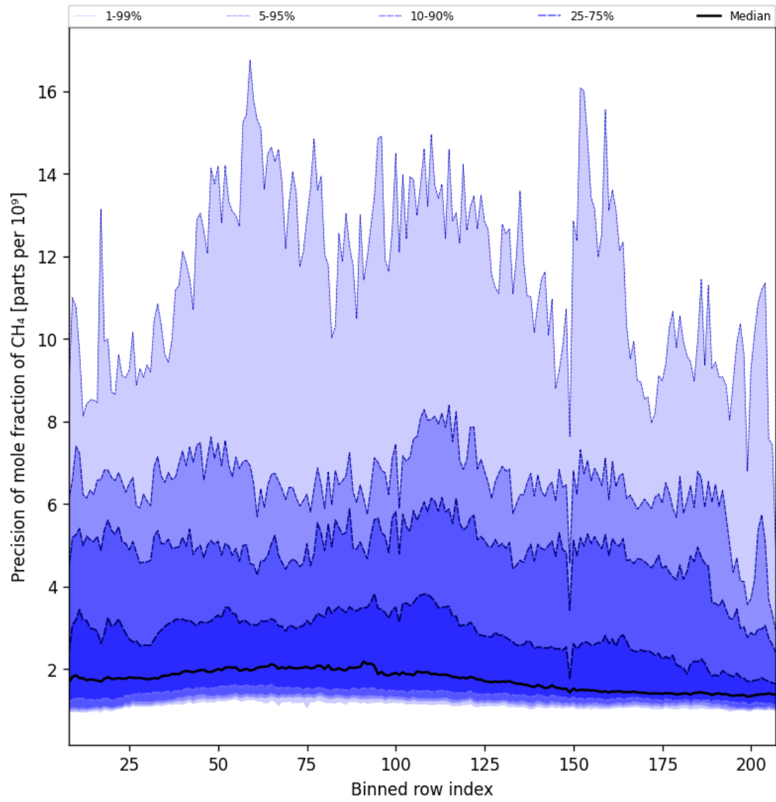
Figure 35: Along track statistics of “Precision of mole fraction of CH 4 ” for 2025-10-17 to 2025-10-18
