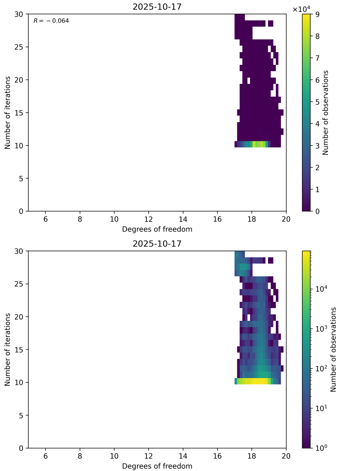
Figure 52: Scatter density plot of “Degrees of freedom” against “Number of iterations” for 2025-10-17 to 2025-10-18.
