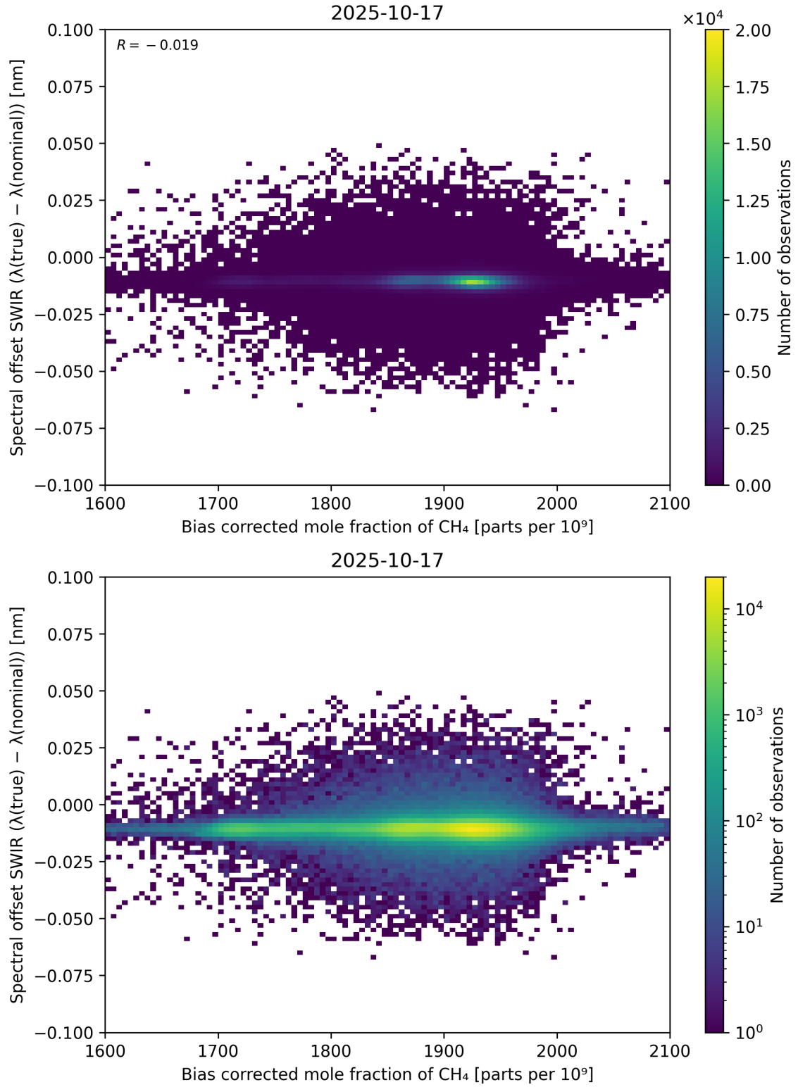
Figure 69: Scatter density plot of “Bias corrected mole fraction of CH 4 ” against “Spectral offset SWIR ( \lambda_{\text{true}} - \lambda_{\text{nominal}} )” for 2025-10-17 to 2025-10-18.
