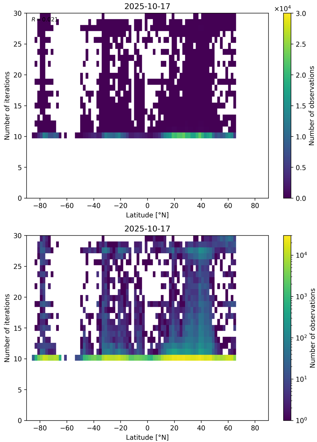
Figure 60: Scatter density plot of “Latitude” against “Number of iterations” for 2025-10-17 to 2025-10-18.
