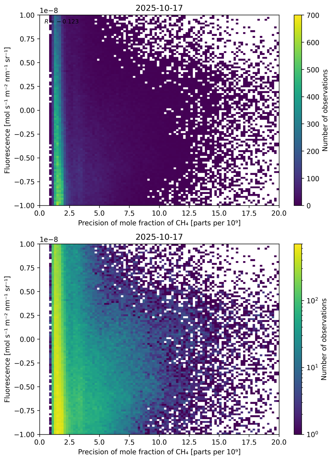
Figure 81: Scatter density plot of “Precision of mole fraction of CH 4 ” against “Fluorescence” for 2025-10-17 to 2025-10-18.
