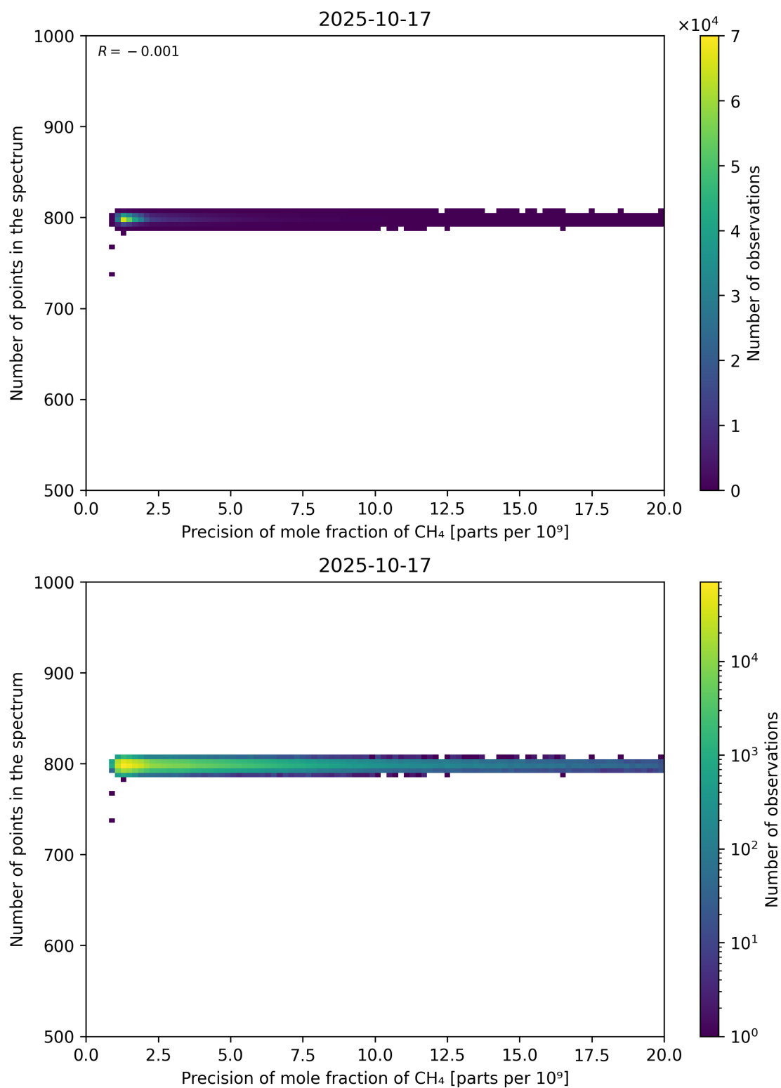
Figure 84: Scatter density plot of “Precision of mole fraction of CH 4 ” against “Number of points in the spectrum” for 2025-10-17 to 2025-10-18.
