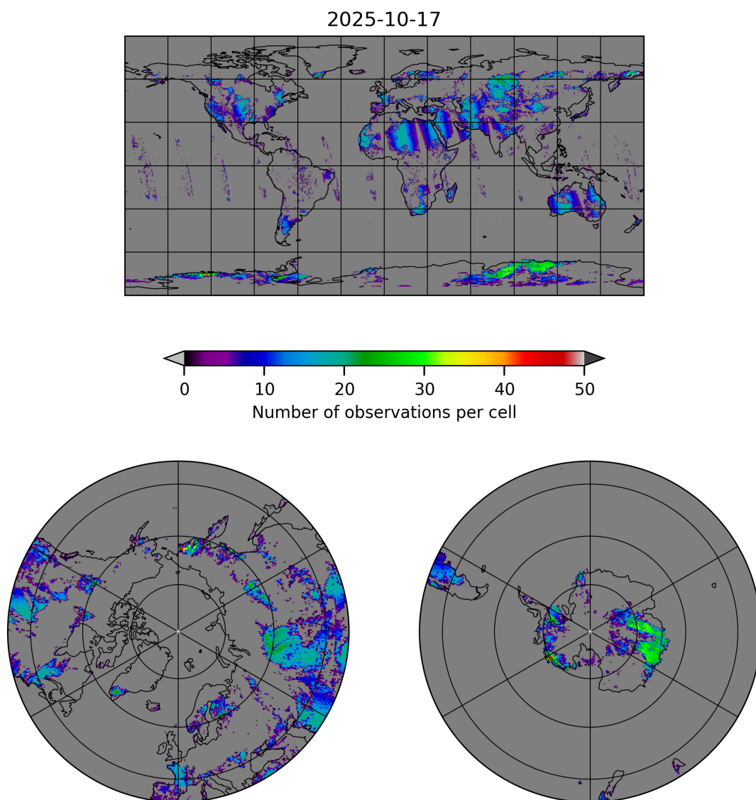
Figure 10: Map of the number of observations for 2025-10-17 to 2025-10-18
