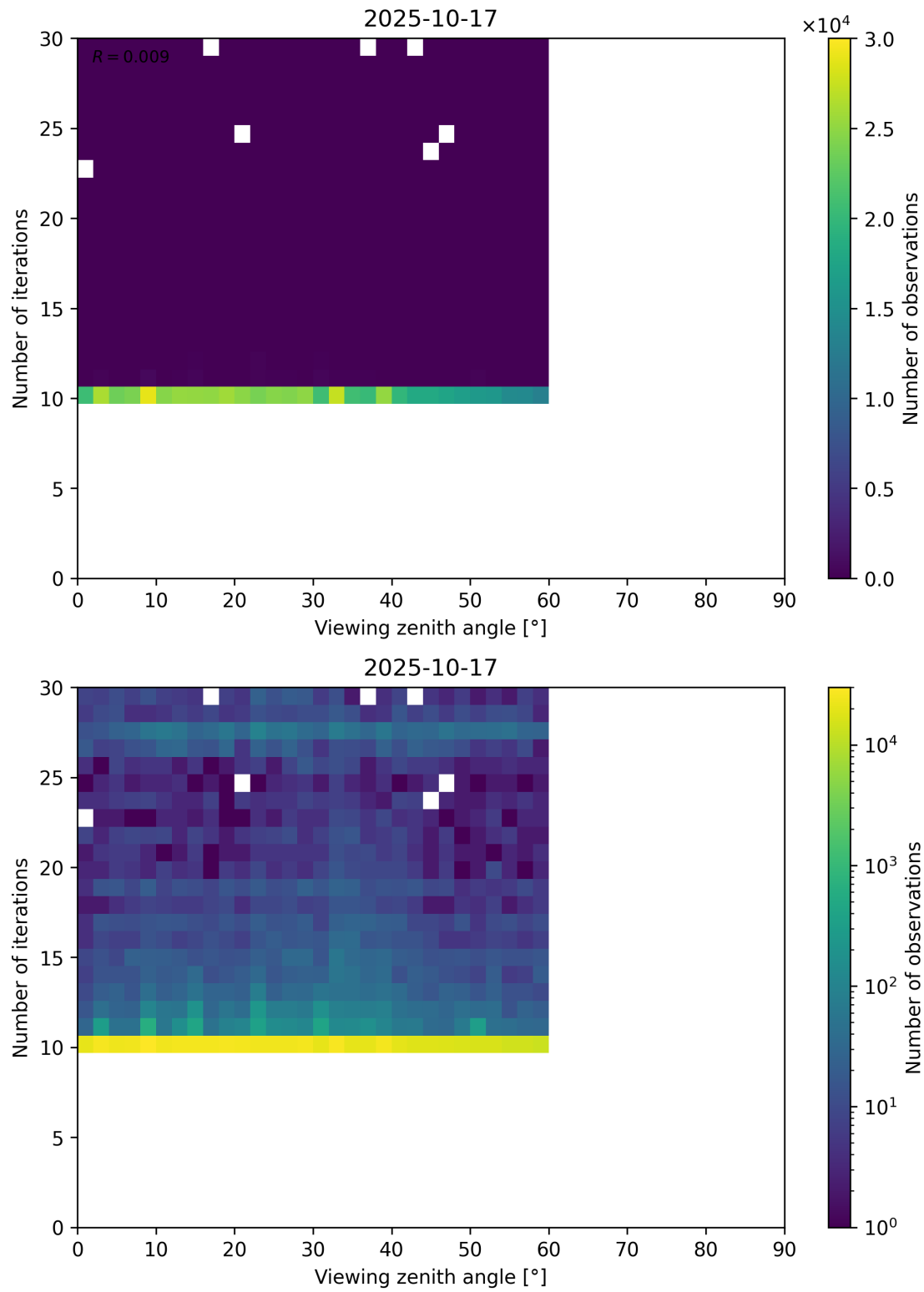
Figure 113: Scatter density plot of “Viewing zenith angle” against “Number of iterations” for 2025-10-17 to 2025-10-18.
