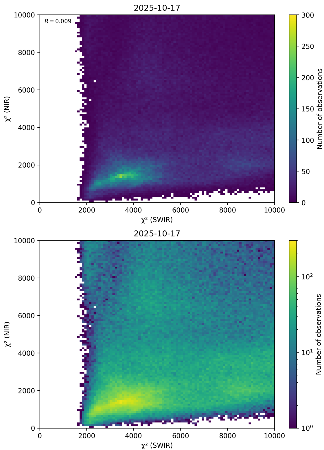
Figure 47: Scatter density plot of “ \chi^2 (SWIR)” against “ \chi^2 (NIR)” for 2025-10-17 to 2025-10-18.
