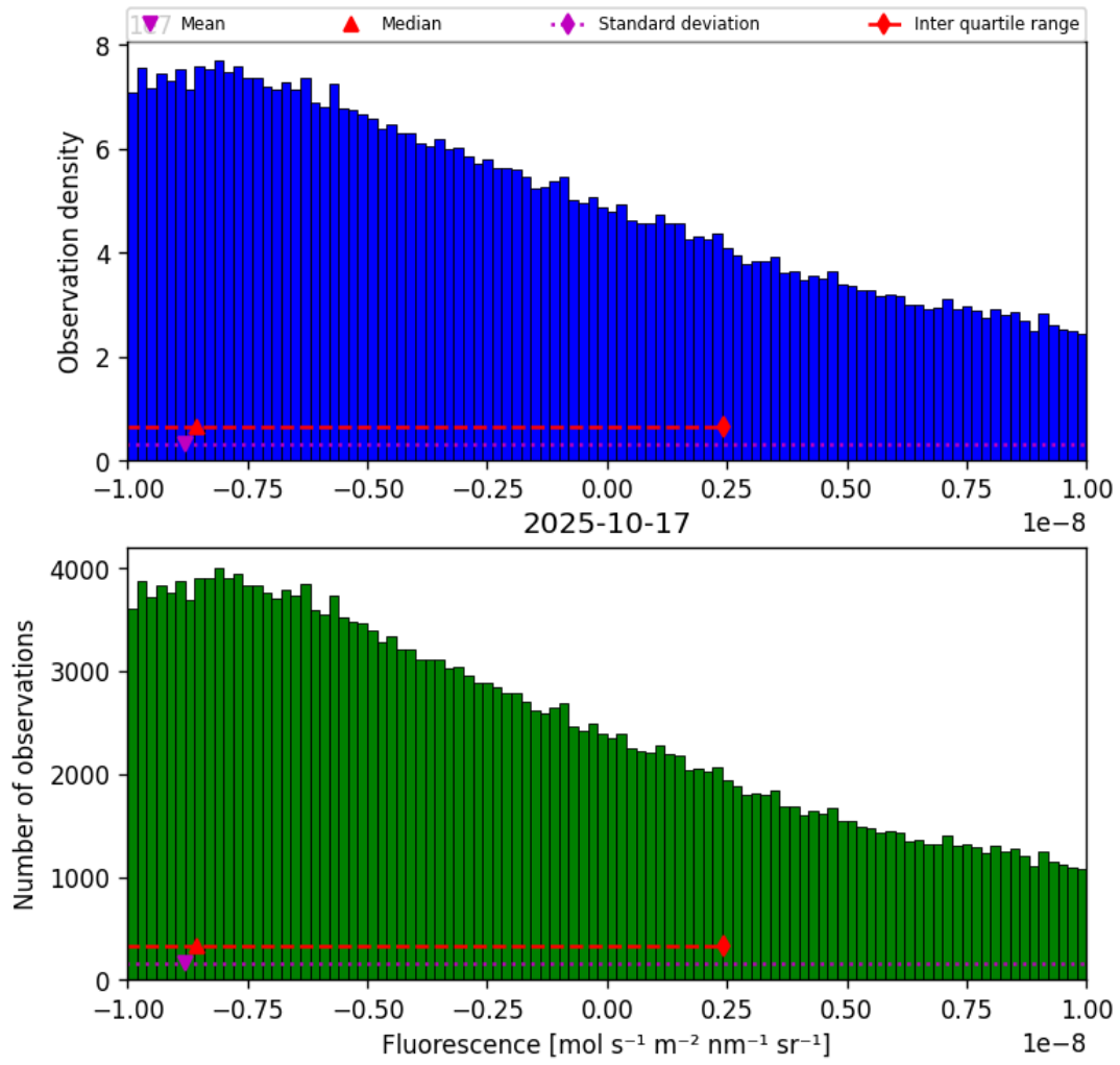
Figure 32: Histogram of “Fluorescence” for 2025-10-17 to 2025-10-18
