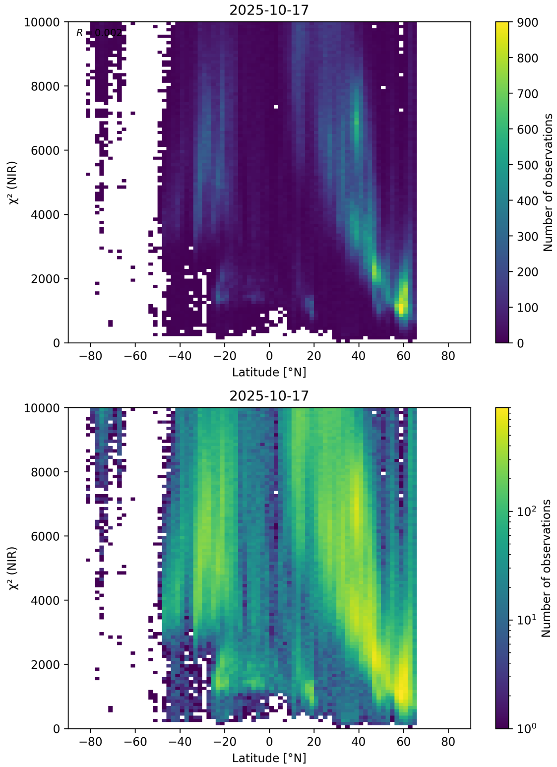
Figure 53: Scatter density plot of “Latitude” against “ \chi^2 (NIR)” for 2025-10-17 to 2025-10-18.
