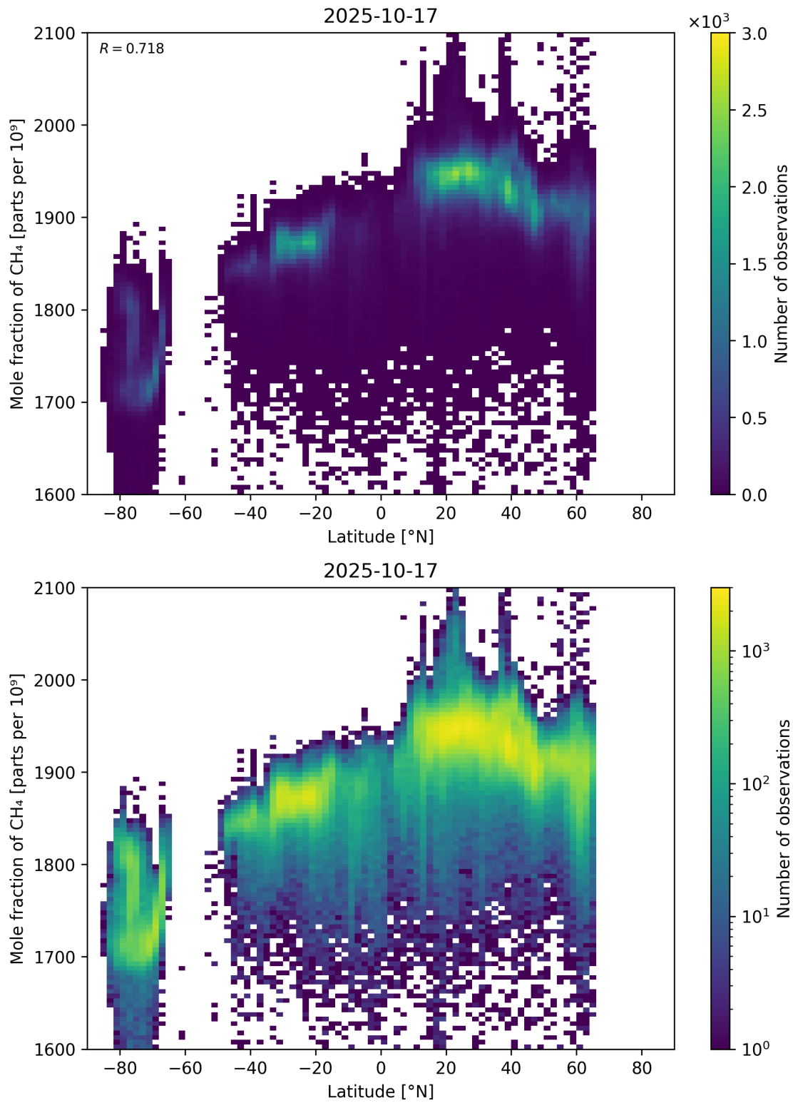
Figure 57: Scatter density plot of “Latitude” against “Mole fraction of \text{CH}_4 ” for 2025-10-17 to 2025-10-18.
