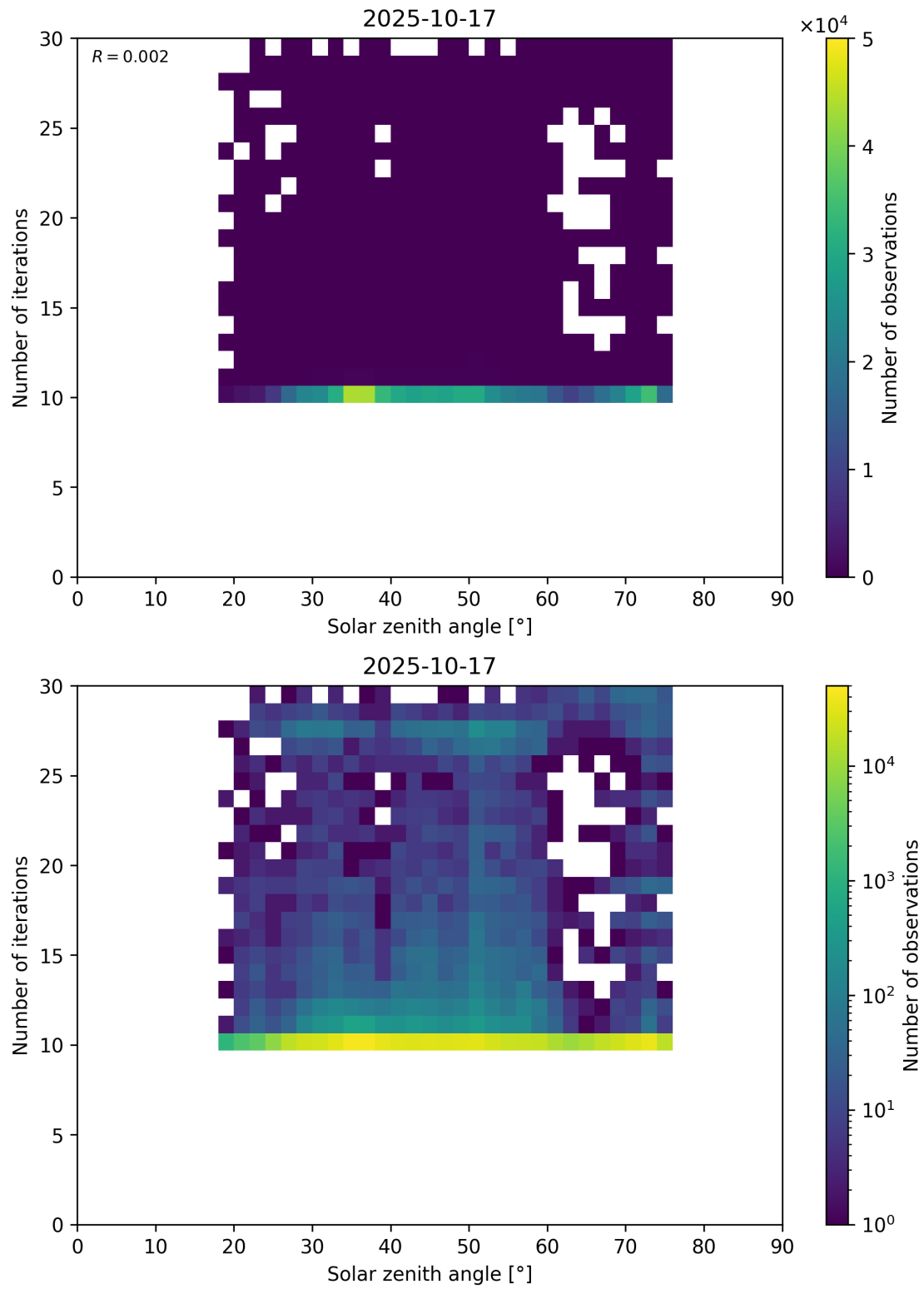
Figure 102: Scatter density plot of “Solar zenith angle” against “Number of iterations” for 2025-10-17 to 2025-10-18.
