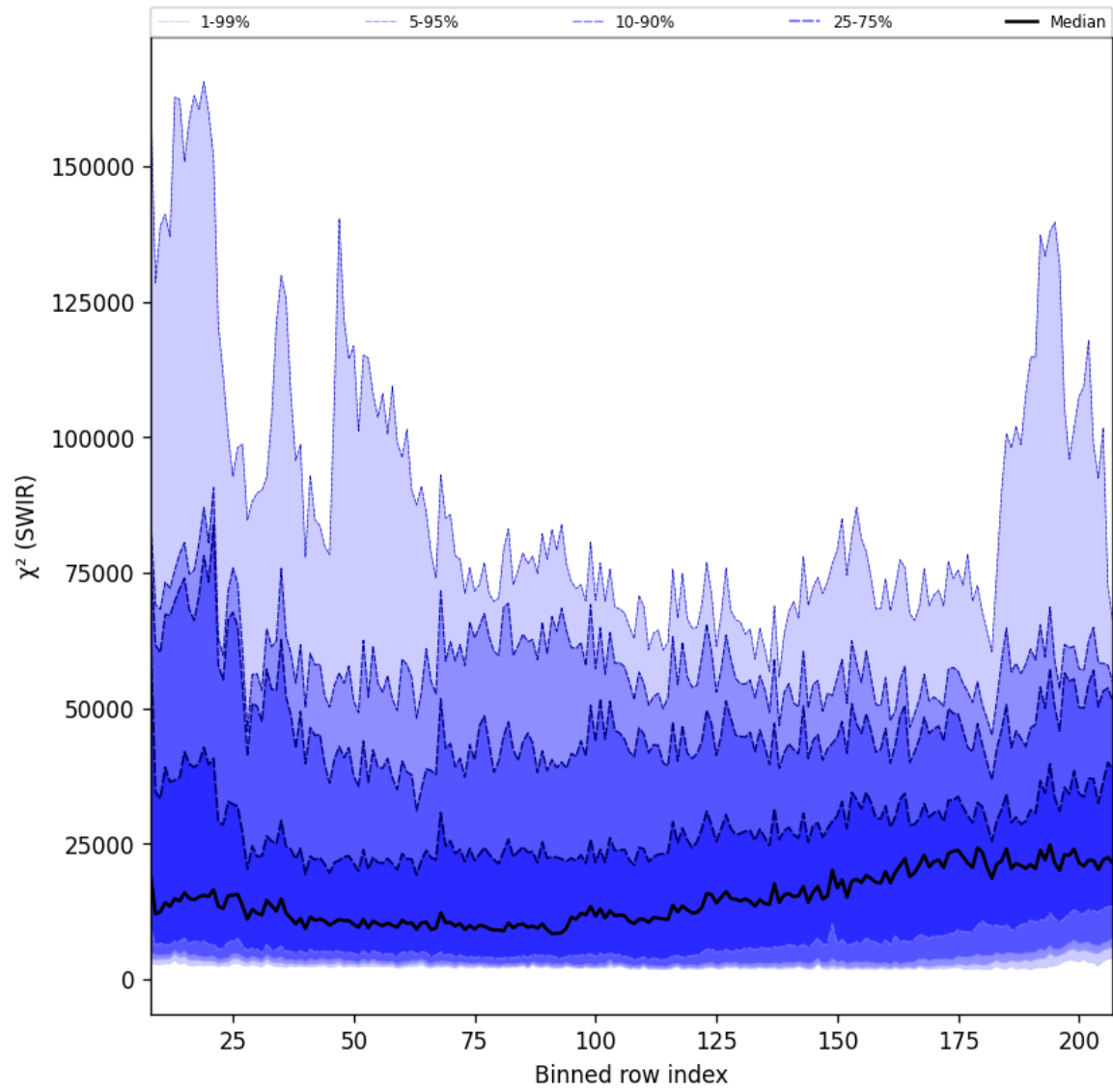
Figure 39: Along track statistics of “ \chi^2 (SWIR)” for 2025-10-17 to 2025-10-18
