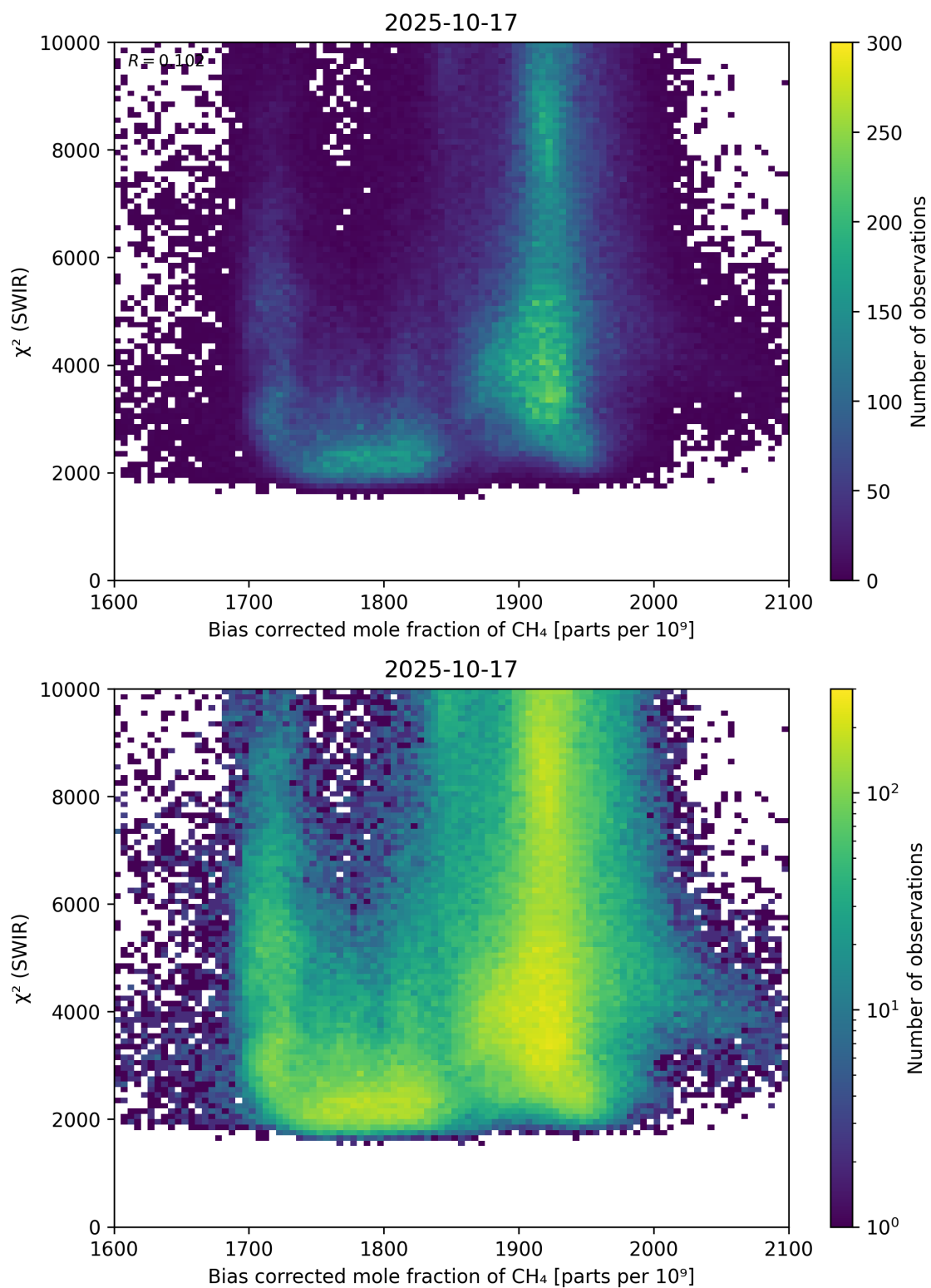
Figure 64: Scatter density plot of “Bias corrected mole fraction of CH 4 ” against “ \chi^2 (SWIR)” for 2025-10-17 to 2025-10-18.
