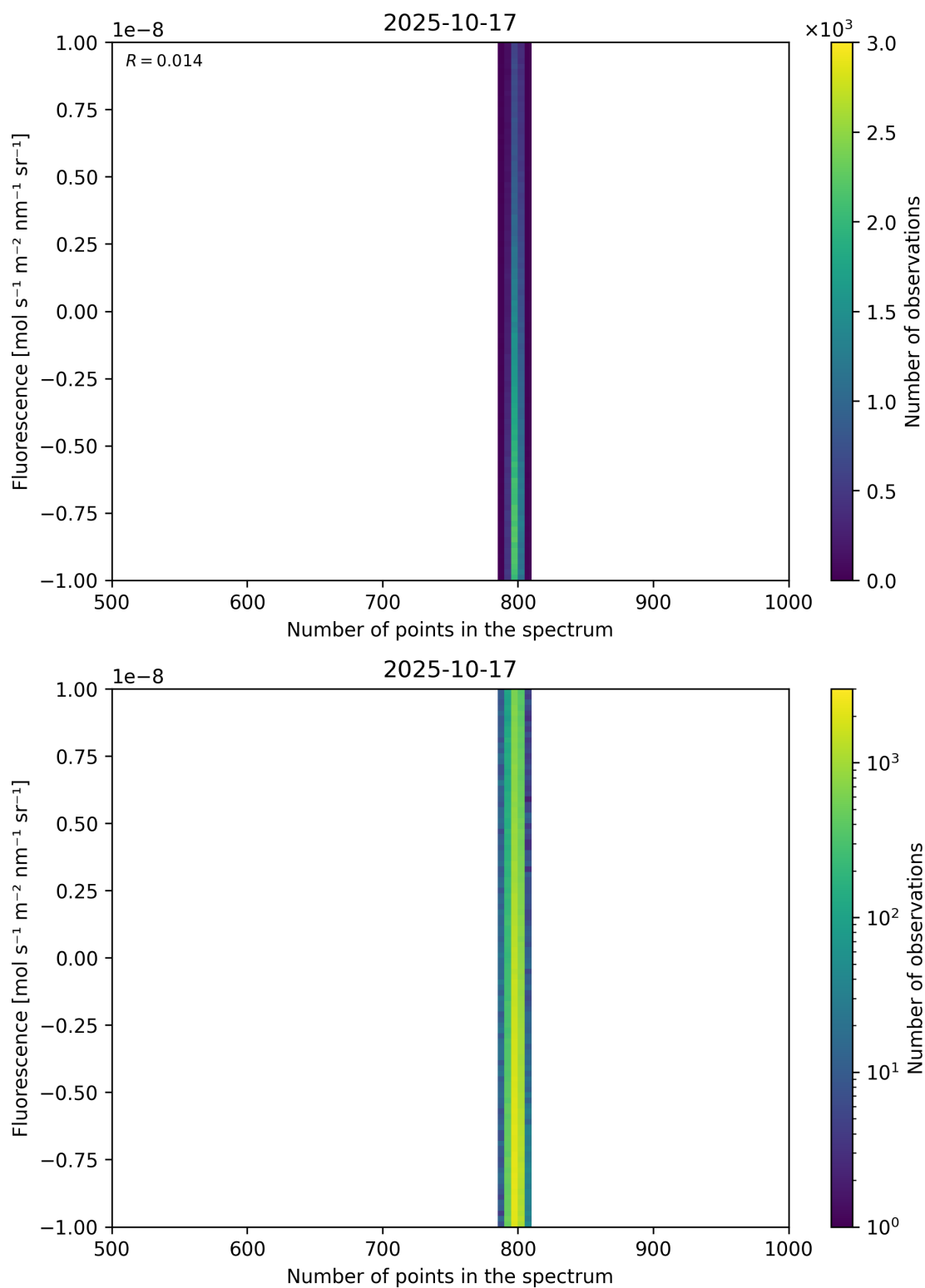
Figure 91: Scatter density plot of “Number of points in the spectrum” against “Fluorescence” for 2025-10-17 to 2025-10-18.
