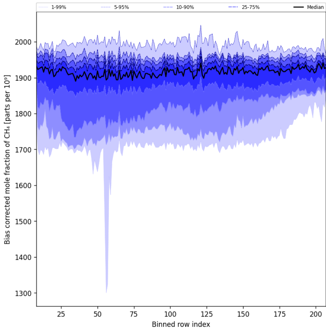
Figure 36: Along track statistics of “Bias corrected mole fraction of CH 4 ” for 2025-10-17 to 2025-10-18
