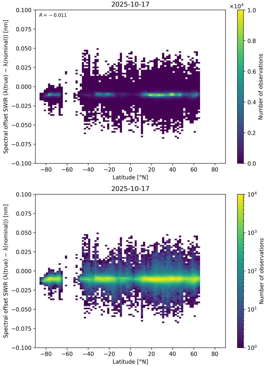
Figure 62: Scatter density plot of “Latitude” against “Spectral offset SWIR ( \lambda_{\text{true}} - \lambda_{\text{nominal}} )” for 2025-10-17 to 2025-10-18.
