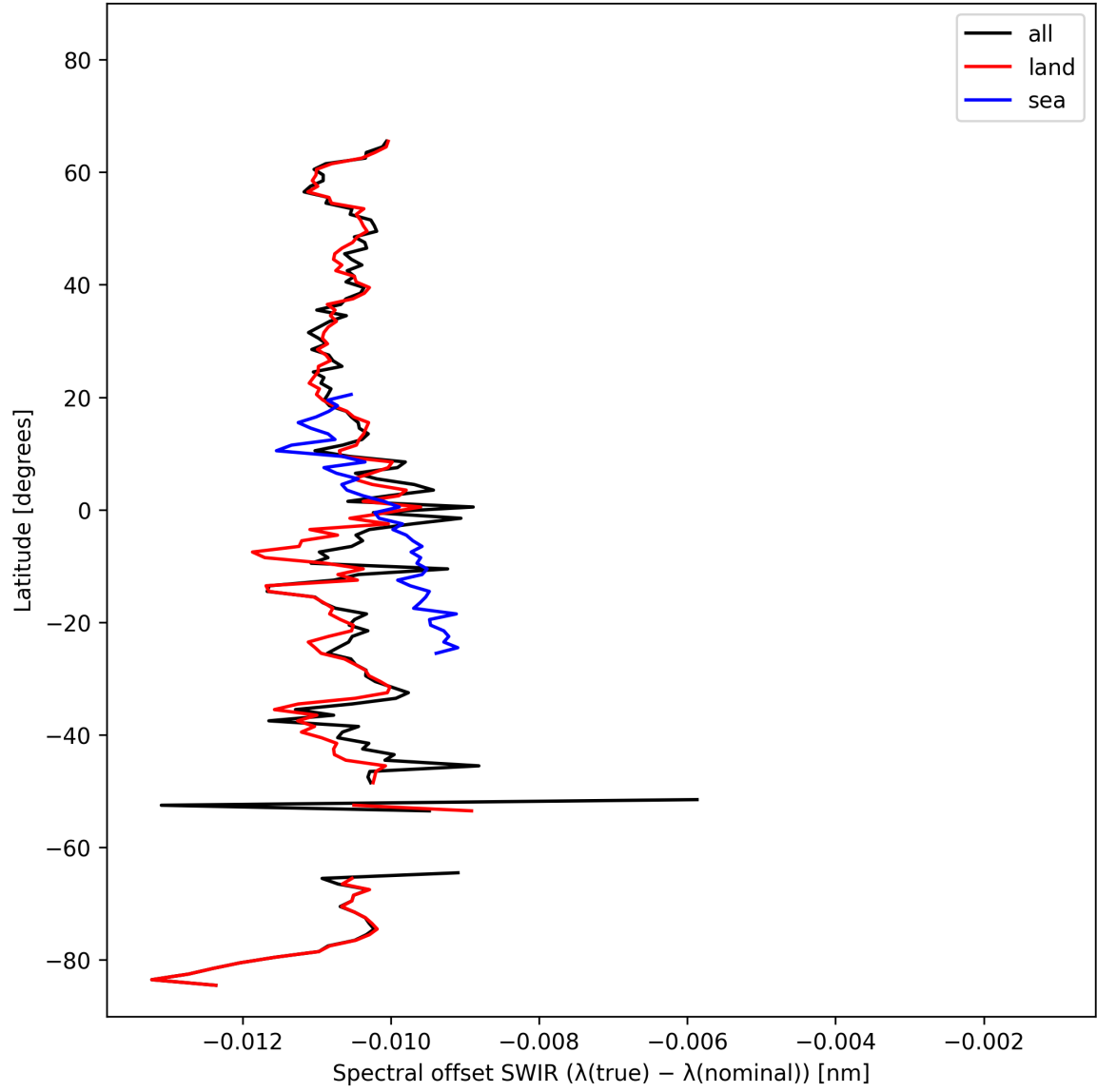
Figure 16: Zonal average of “Spectral offset SWIR ( \lambda_{\text{true}} - \lambda_{\text{nominal}} )” for 2025-10-17 to 2025-10-18.
