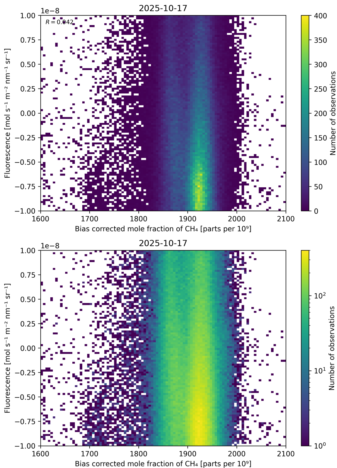
Figure 66: Scatter density plot of “Bias corrected mole fraction of \text{CH}_4 ” against “Fluorescence” for 2025-10-17 to 2025-10-18.
