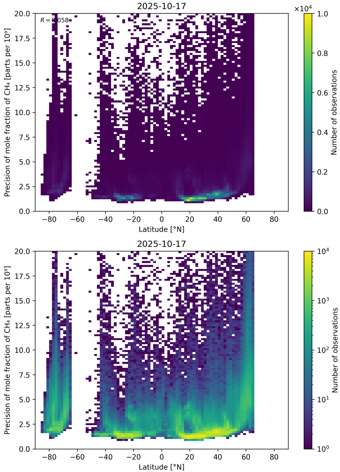
Figure 59: Scatter density plot of “Latitude” against “Precision of mole fraction of CH 4 ” for 2025-10-17 to 2025-10-18.
