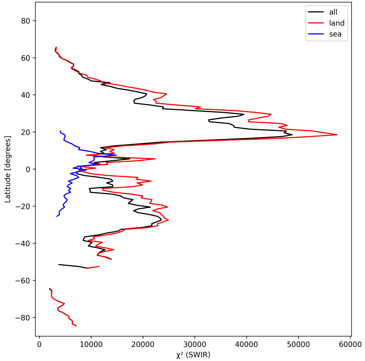
Figure 17: Zonal average of “ \chi^2 (SWIR)” for 2025-10-17 to 2025-10-18.
