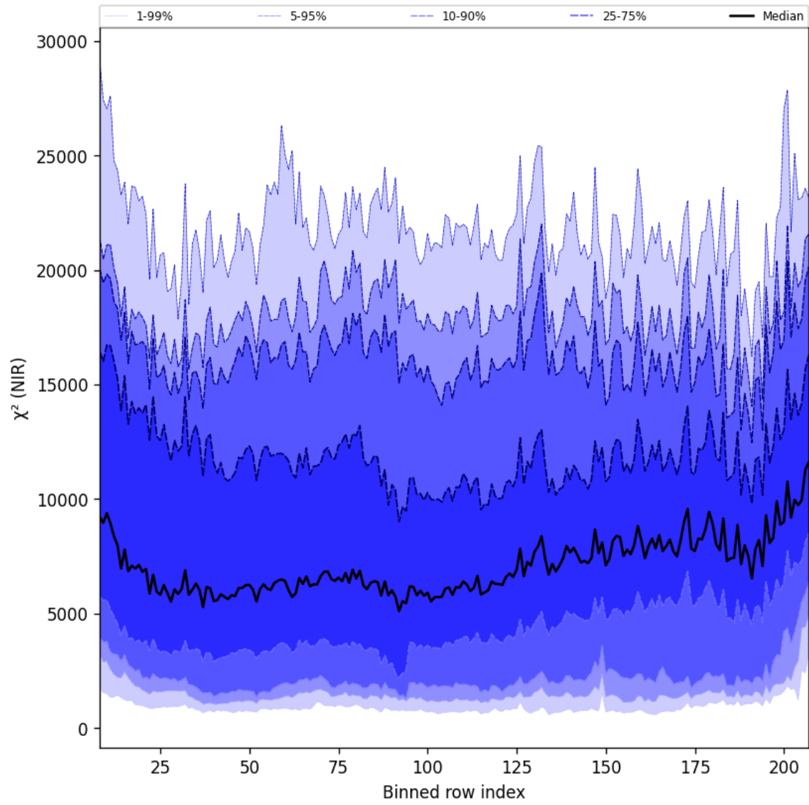
Figure 40: Along track statistics of “ \chi^2 (NIR)” for 2025-10-17 to 2025-10-18
