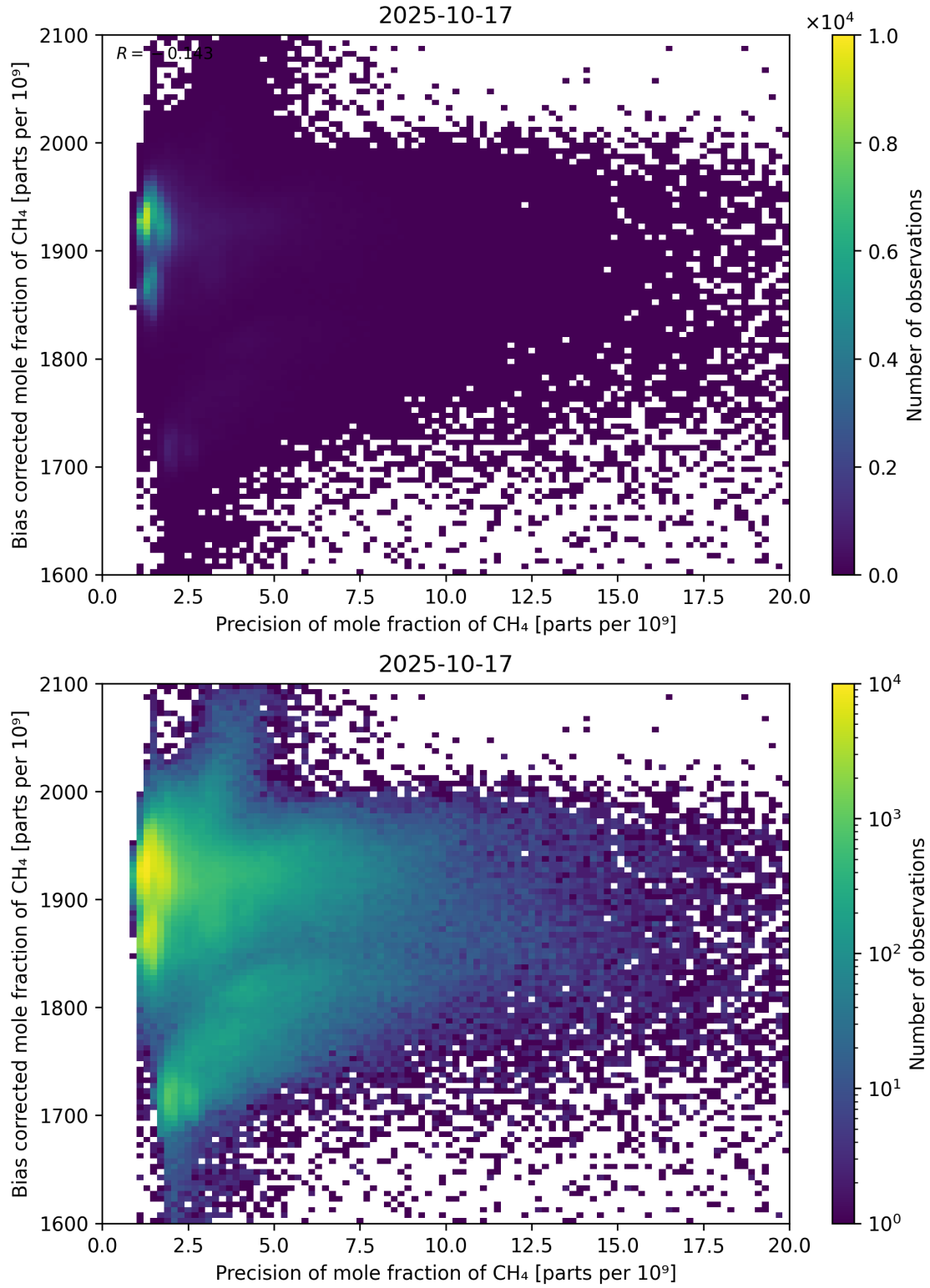
Figure 82: Scatter density plot of “Precision of mole fraction of \text{CH}_4 ” against “Bias corrected mole fraction of \text{CH}_4 ” for 2025-10-17 to 2025-10-18.
