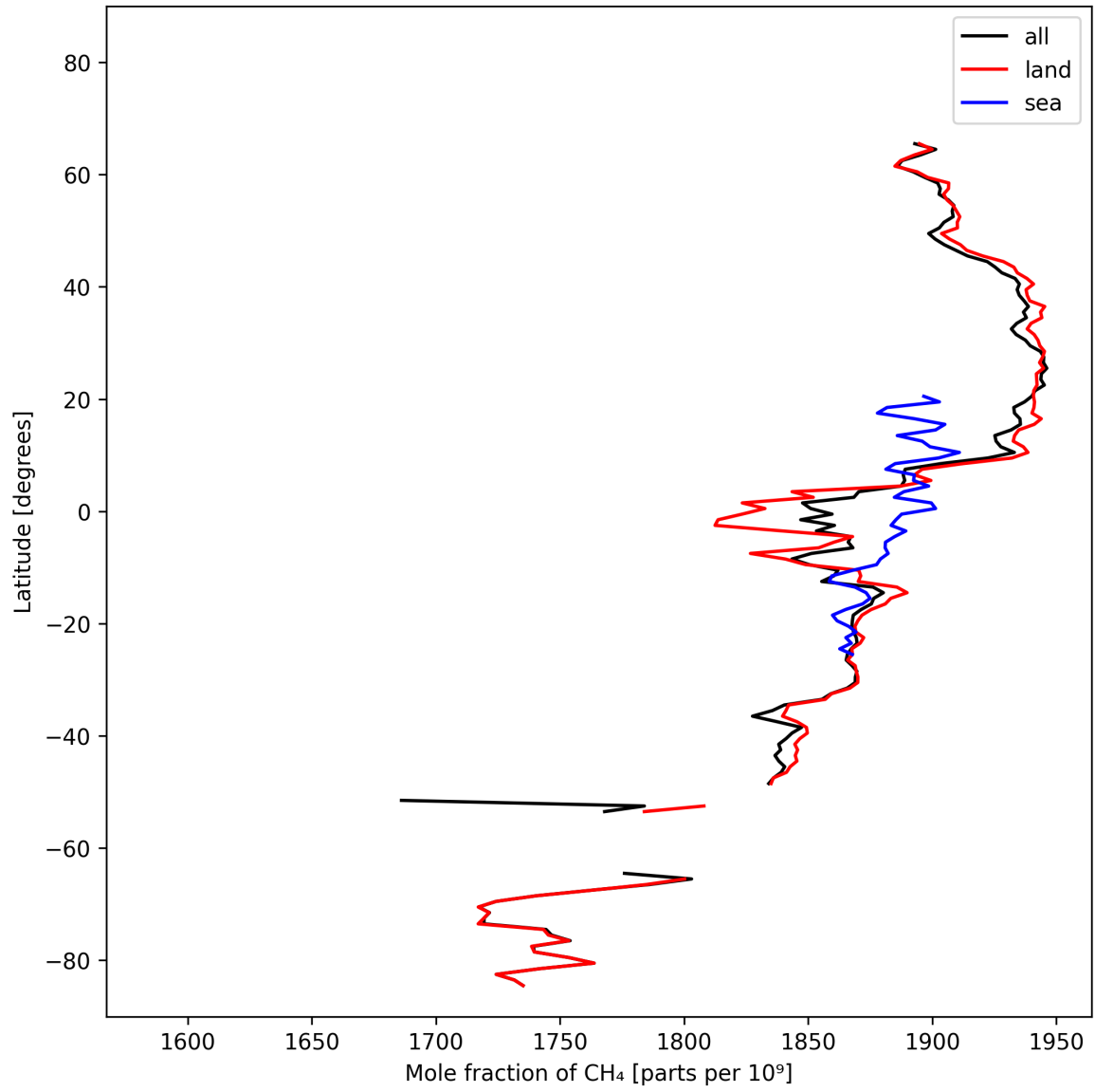
Figure 12: Zonal average of “Mole fraction of \text{CH}_4 ” for 2025-10-17 to 2025-10-18.
