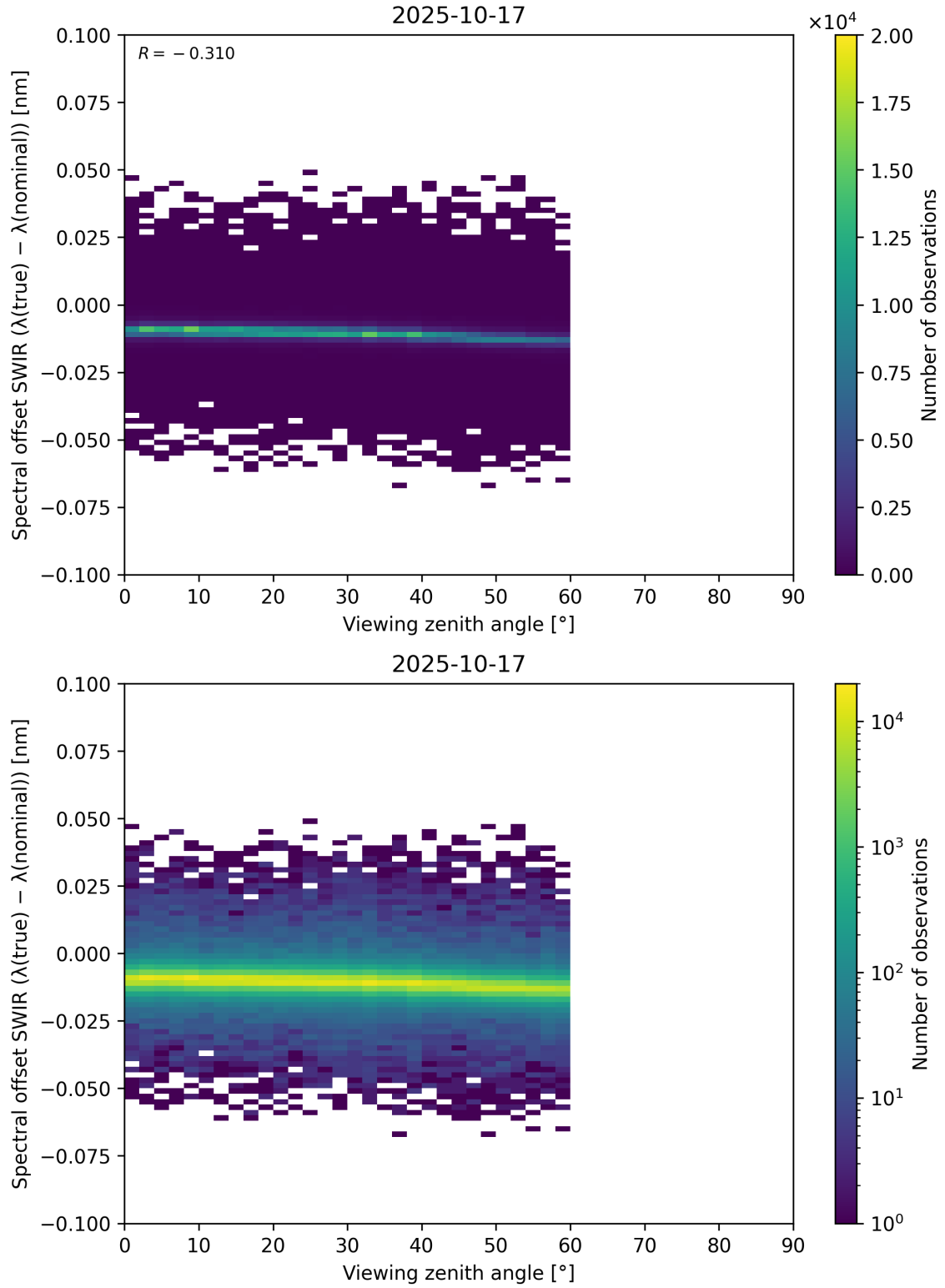
Figure 116: Scatter density plot of “Viewing zenith angle” against “Spectral offset SWIR ( \lambda_{\text{true}} - \lambda_{\text{nominal}} )” for 2025-10-17 to 2025-10-18.
