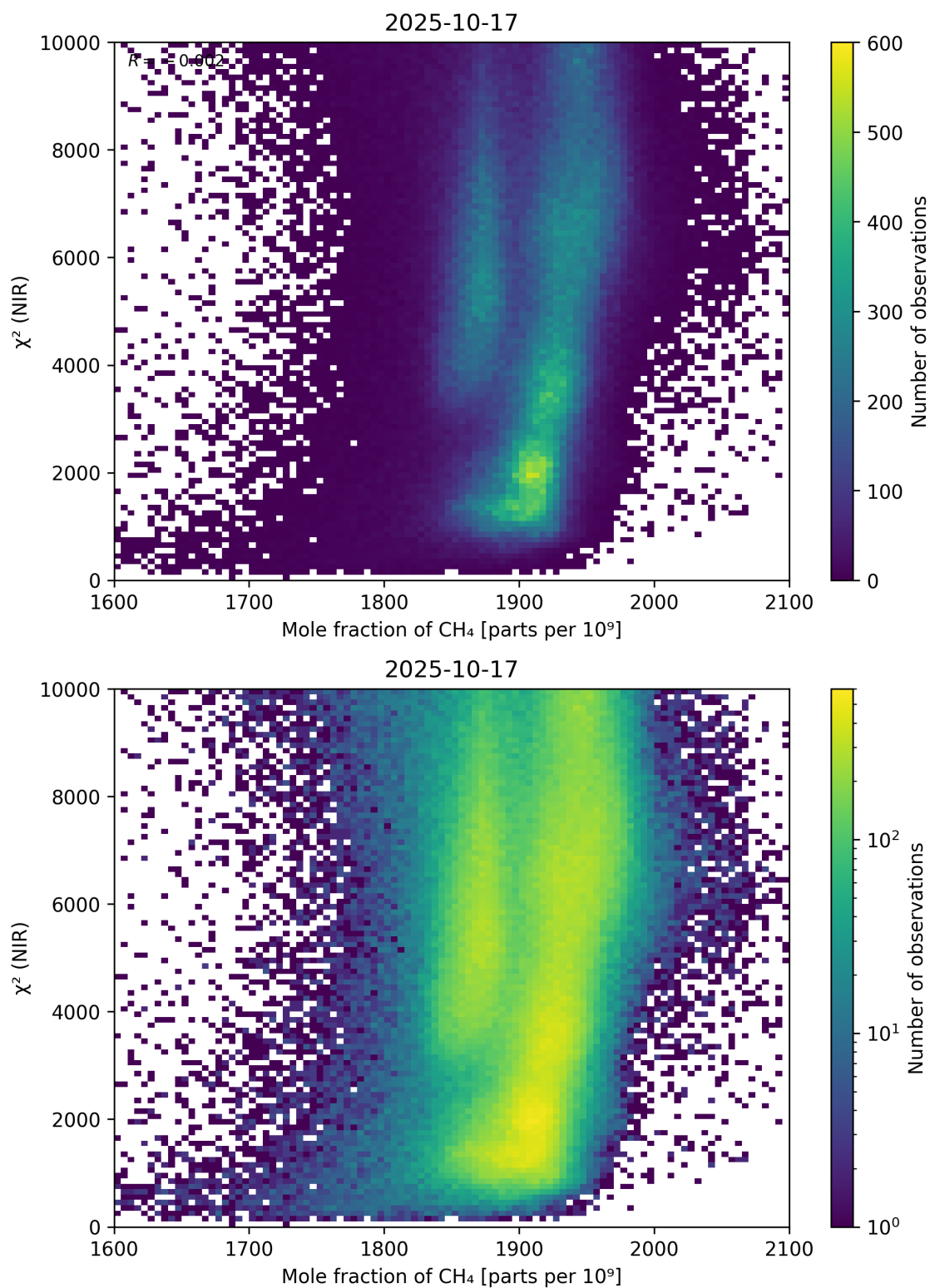
Figure 70: Scatter density plot of “Mole fraction of \text{CH}_4 ” against “ \chi^2 (NIR)” for 2025-10-17 to 2025-10-18.
