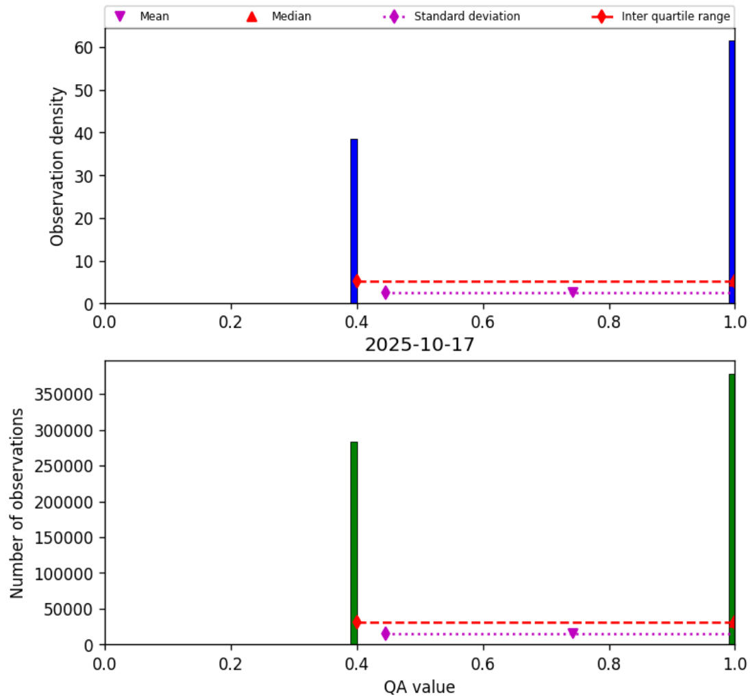
Figure 22: Histogram of “QA value” for 2025-10-17 to 2025-10-18
