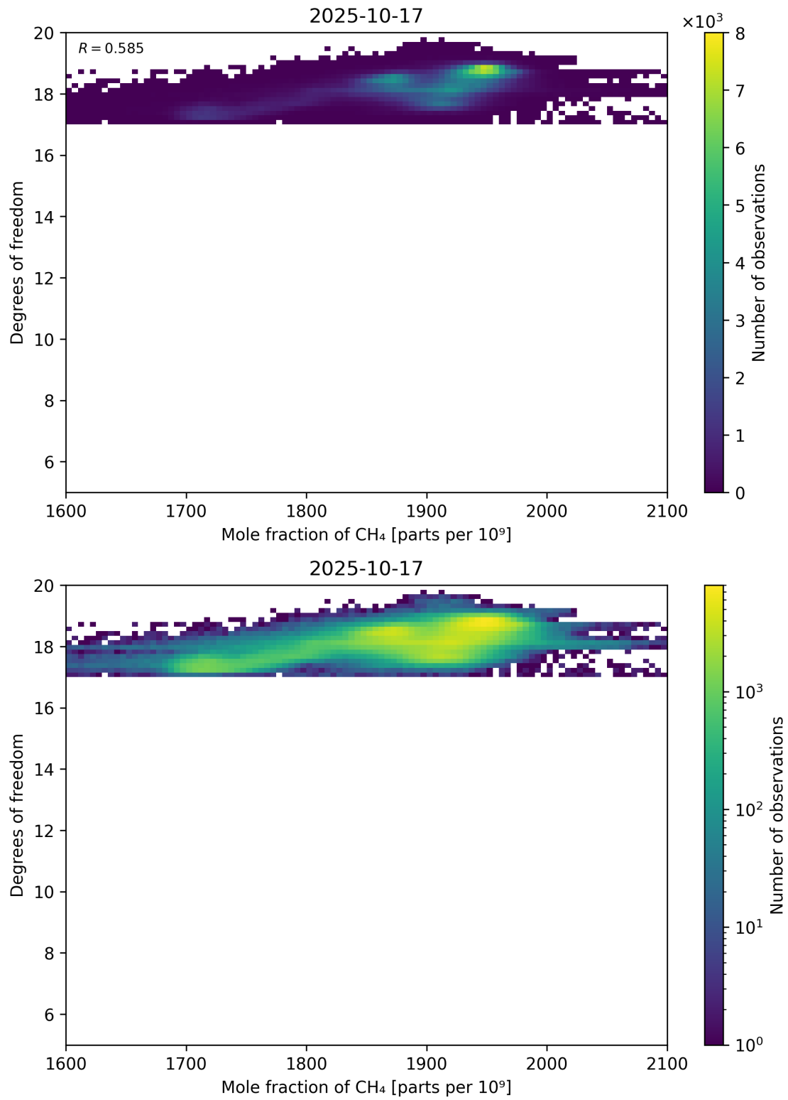
Figure 72: Scatter density plot of “Mole fraction of CH 4 ” against “Degrees of freedom” for 2025-10-17 to 2025-10-18.
