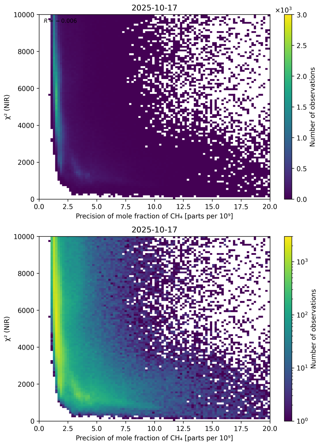
Figure 78: Scatter density plot of “Precision of mole fraction of CH 4 ” against “ \chi^2 (NIR)” for 2025-10-17 to 2025-10-18.
