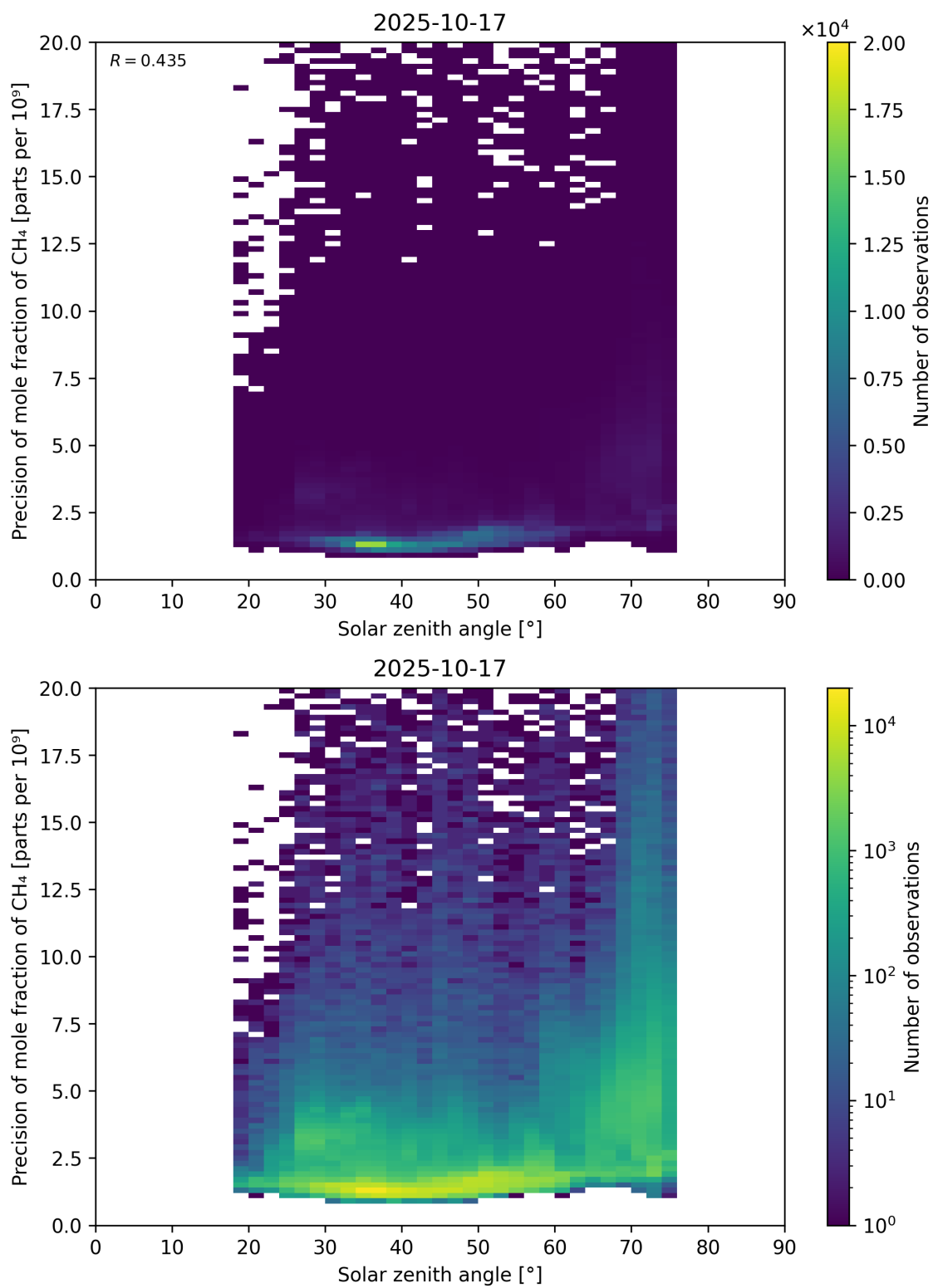
Figure 101: Scatter density plot of “Solar zenith angle” against “Precision of mole fraction of \text{CH}_4 ” for 2025-10-17 to 2025-10-18.
