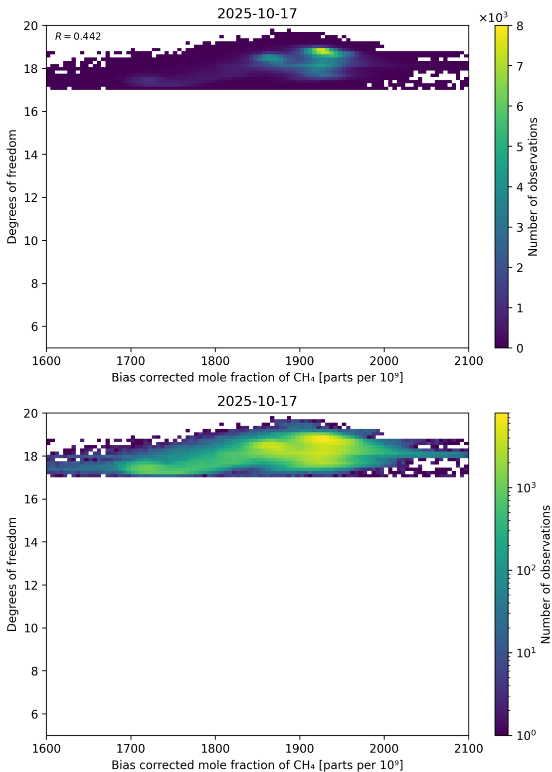
Figure 65: Scatter density plot of “Bias corrected mole fraction of CH 4 ” against “Degrees of freedom” for 2025-10-17 to 2025-10-18.
