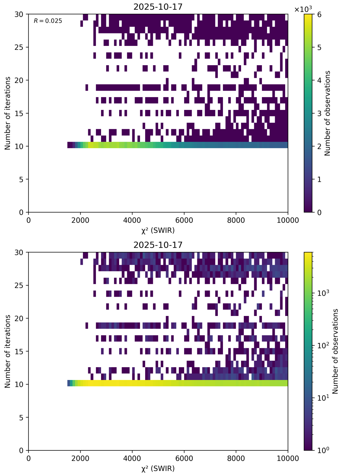
Figure 50: Scatter density plot of “ \chi^2 (SWIR)” against “Number of iterations” for 2025-10-17 to 2025-10-18.
