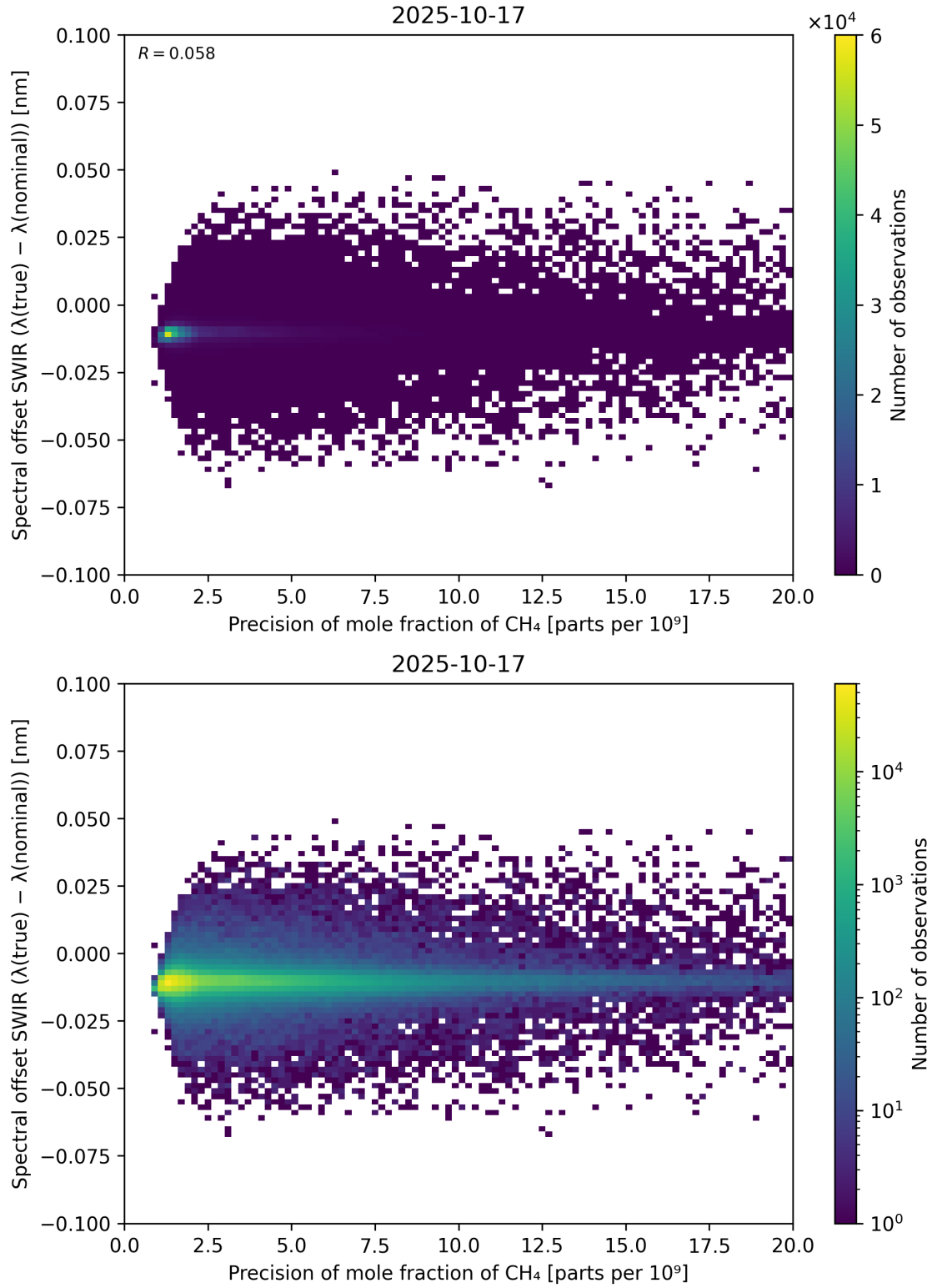
Figure 85: Scatter density plot of “Precision of mole fraction of \text{CH}_4 ” against “Spectral offset SWIR ( \lambda_{\text{true}} - \lambda_{\text{nominal}} )” for 2025-10-17 to 2025-10-18.
