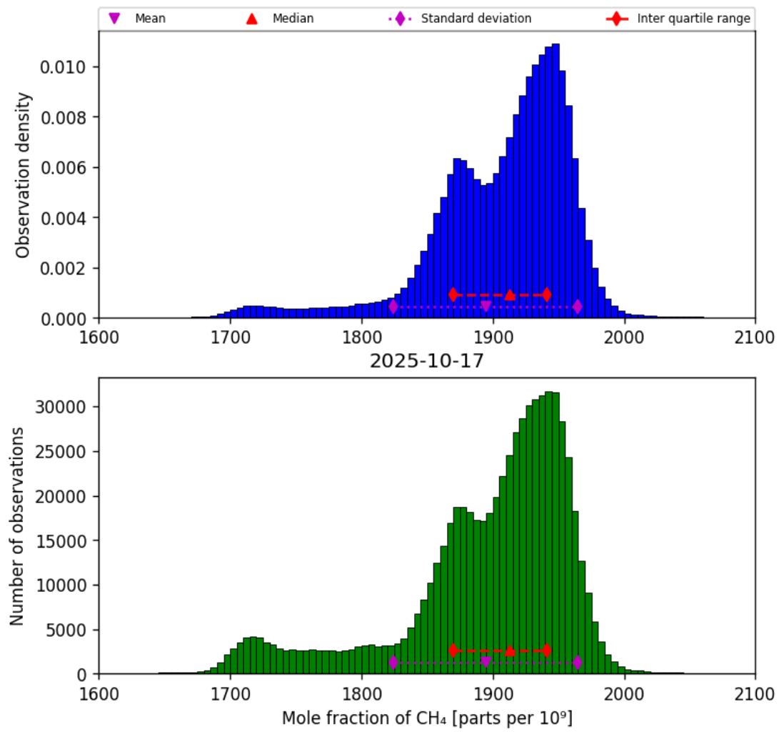
Figure 23: Histogram of “Mole fraction of CH 4 ” for 2025-10-17 to 2025-10-18
