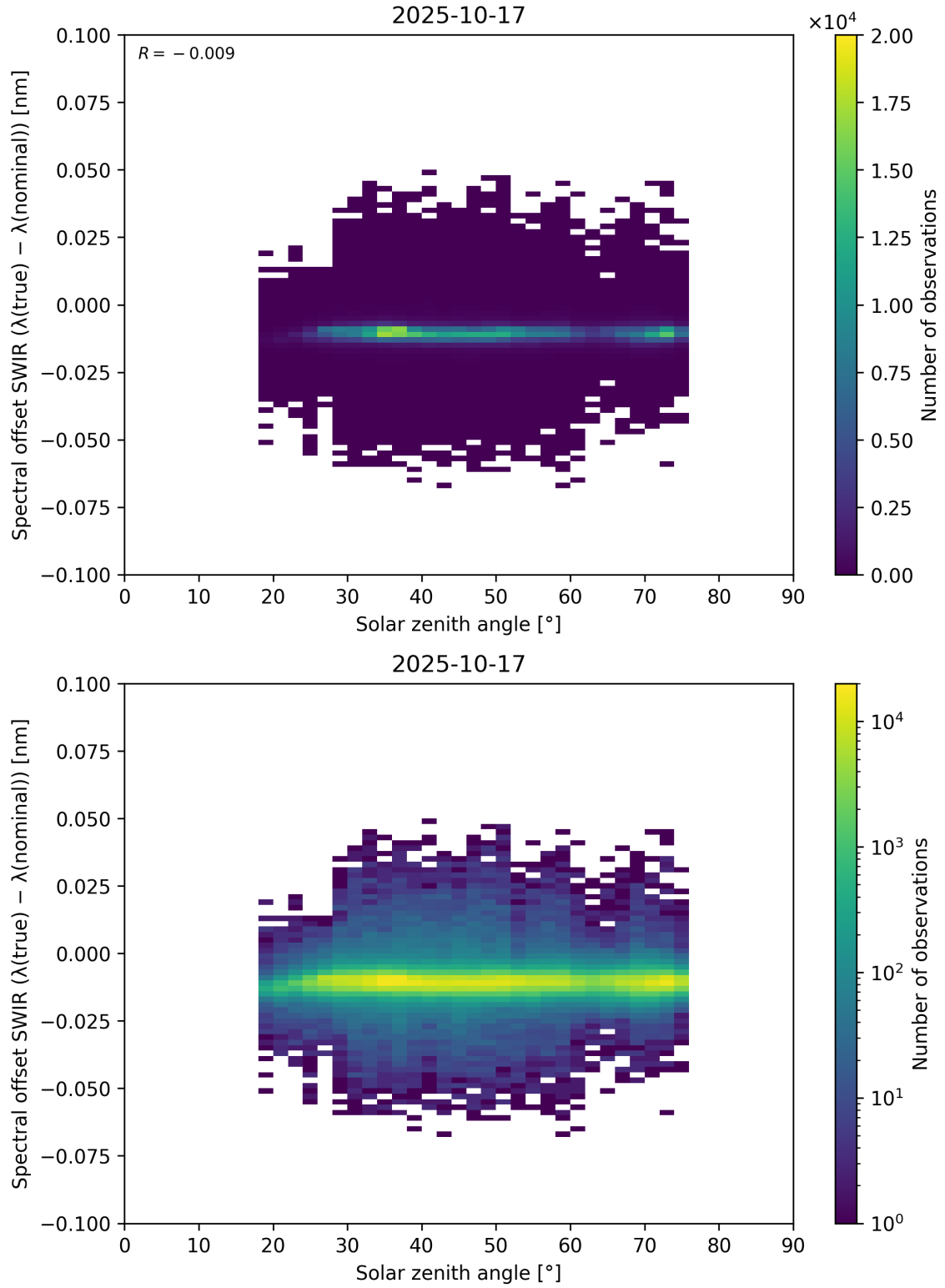
Figure 104: Scatter density plot of “Solar zenith angle” against “Spectral offset SWIR ( \lambda_{\text{true}} - \lambda_{\text{nominal}} )” for 2025-10-17 to 2025-10-18.
