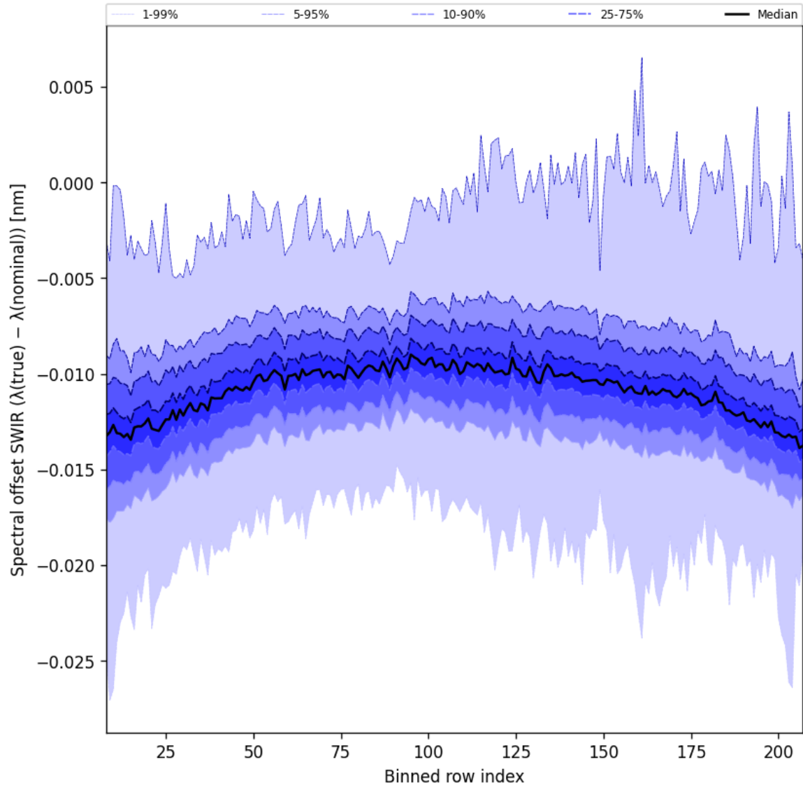
Figure 38: Along track statistics of “Spectral offset SWIR ( \lambda_{\text{true}} - \lambda_{\text{nominal}} )” for 2025-10-17 to 2025-10-18
