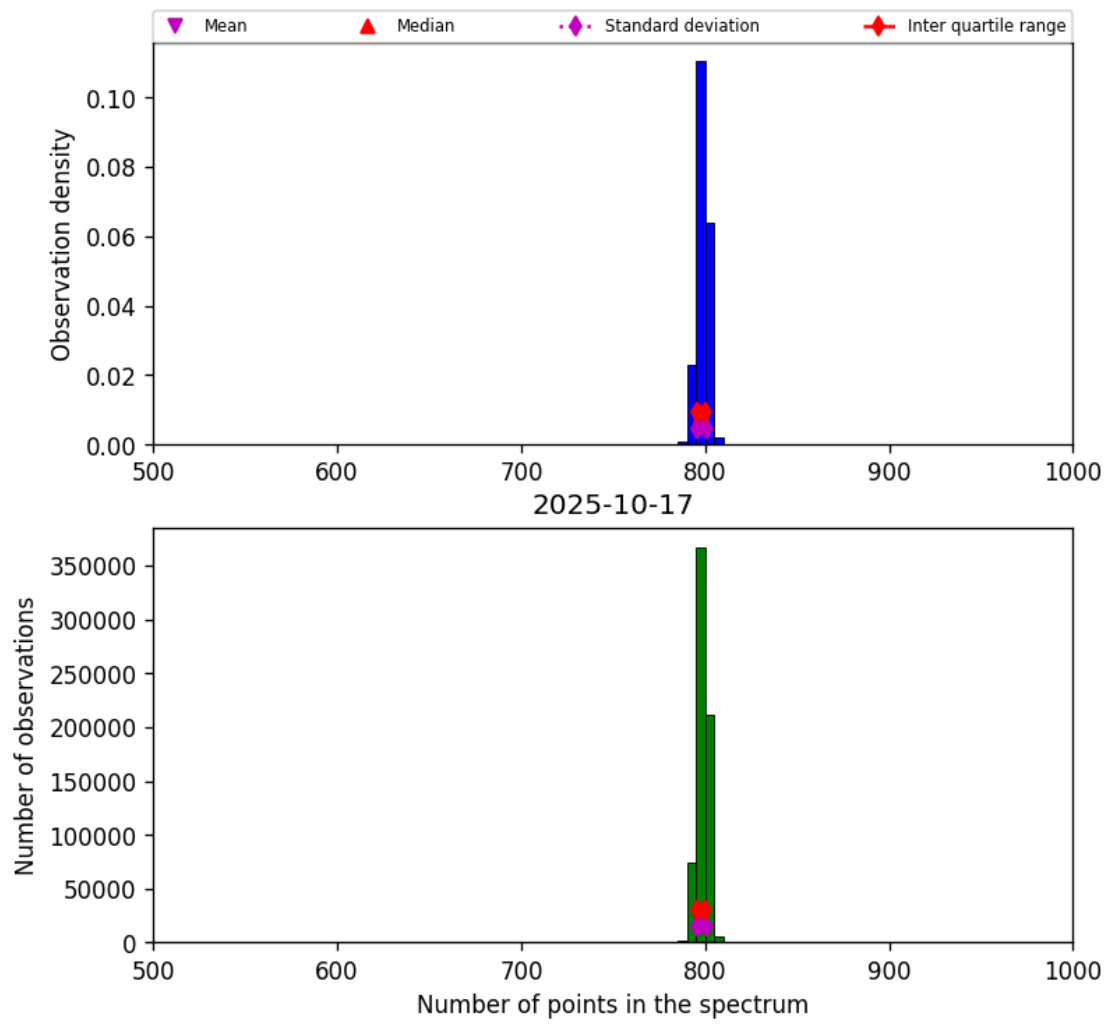
Figure 26: Histogram of “Number of points in the spectrum” for 2025-10-17 to 2025-10-18
