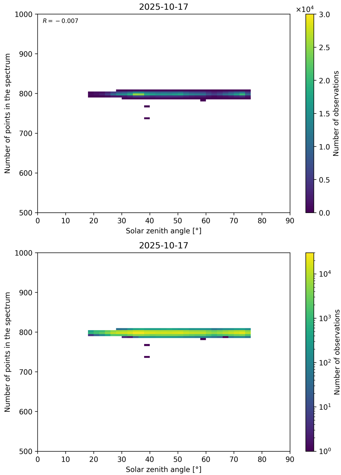
Figure 103: Scatter density plot of “Solar zenith angle” against “Number of points in the spectrum” for 2025-10-17 to 2025-10-18.
