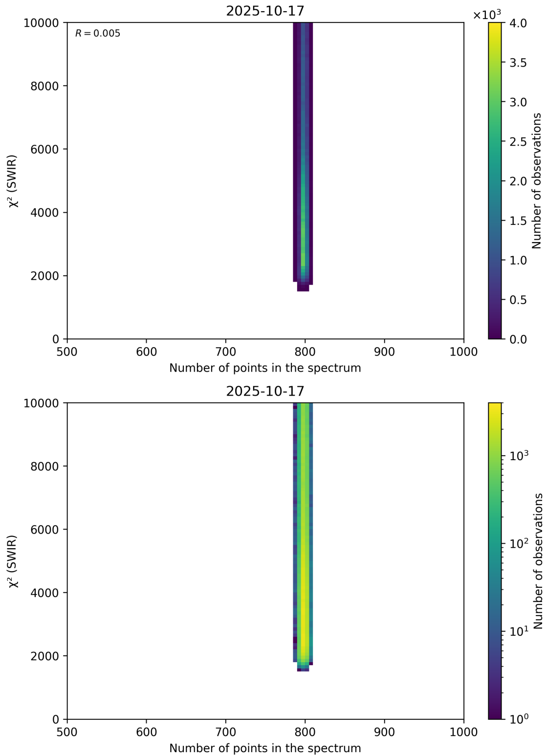
Figure 89: Scatter density plot of “Number of points in the spectrum” against “ \chi^2 (SWIR)” for 2025-10-17 to 2025-10-18.
