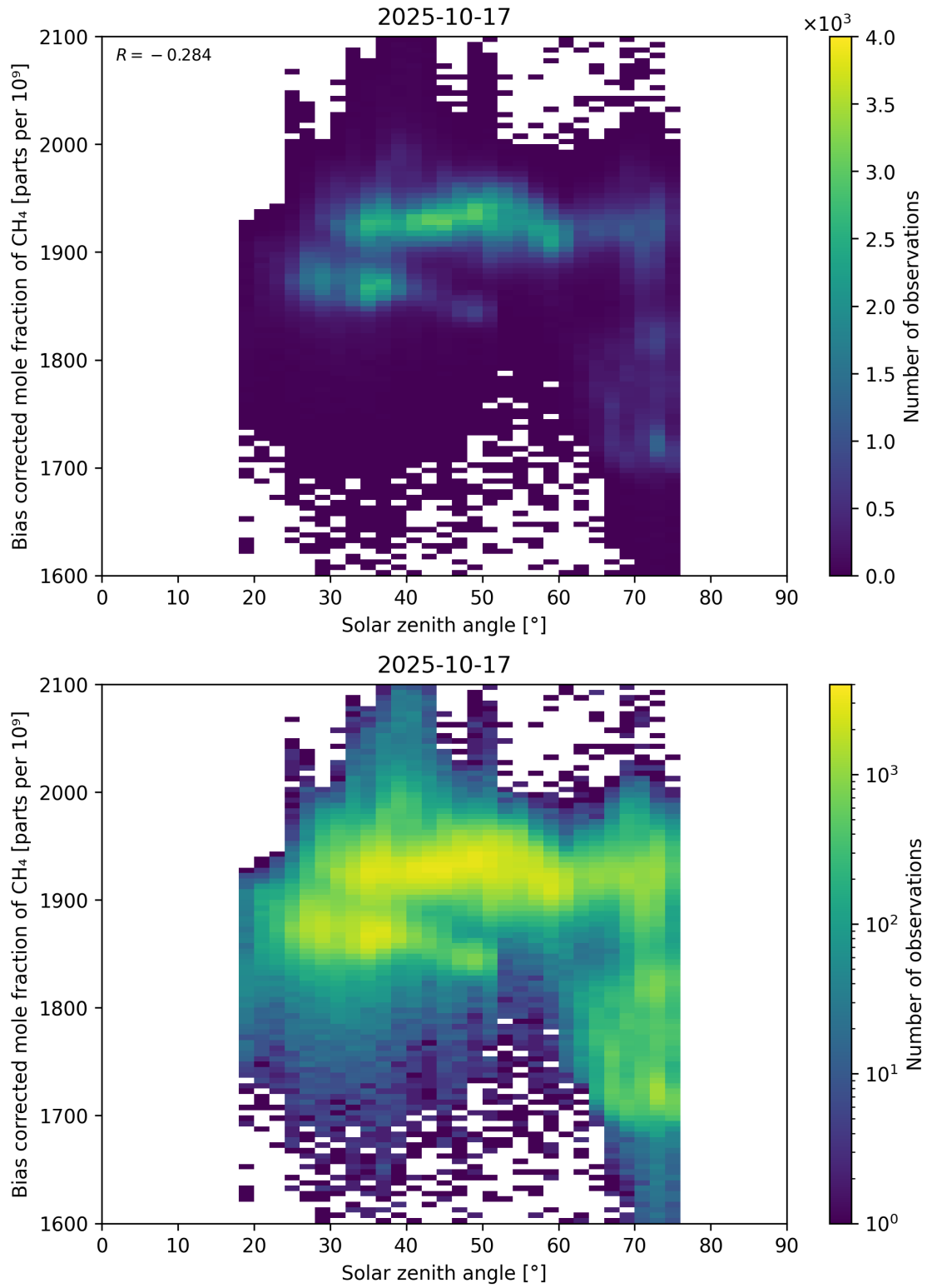
Figure 100: Scatter density plot of “Solar zenith angle” against “Bias corrected mole fraction of \text{CH}_4 ” for 2025-10-17 to 2025-10-18.
