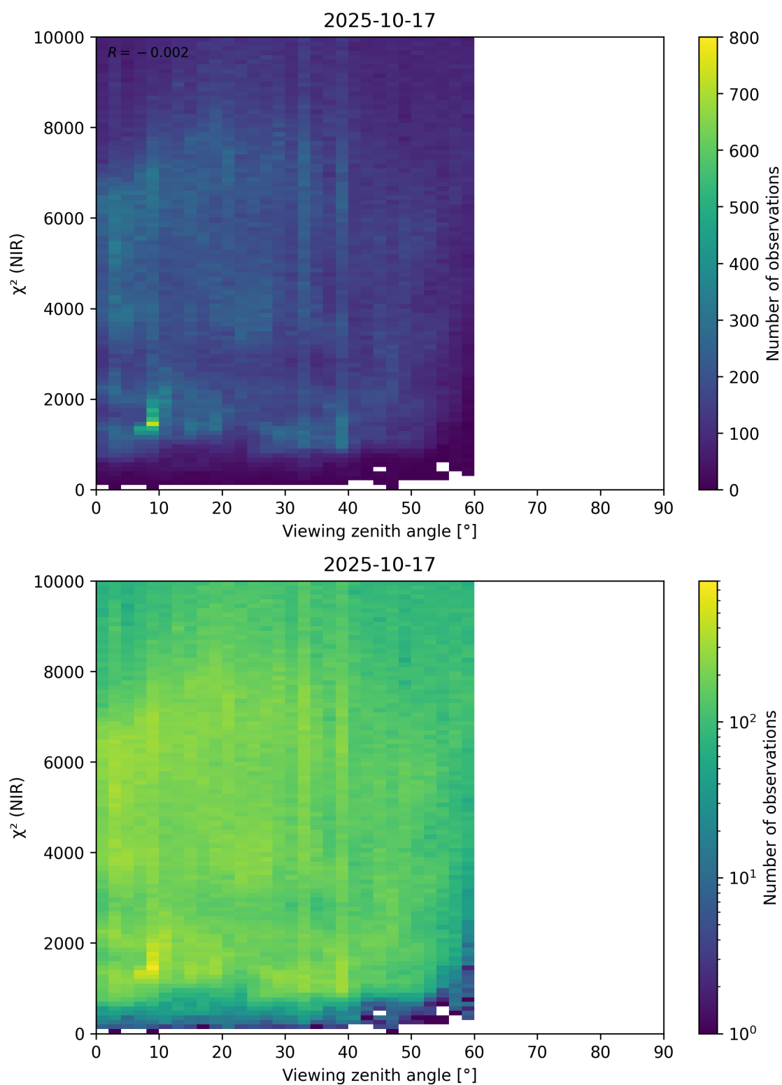
Figure 105: Scatter density plot of “Viewing zenith angle” against “ \chi^2 (NIR)” for 2025-10-17 to 2025-10-18.
