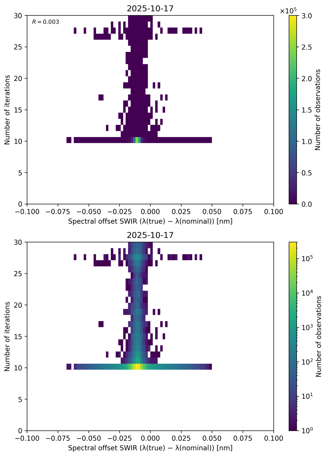
Figure 121: Scatter density plot of “Spectral offset SWIR ( \lambda_{\text{true}} - \lambda_{\text{nominal}} )” against “Number of iterations” for 2025-10-17 to 2025-10-18.
