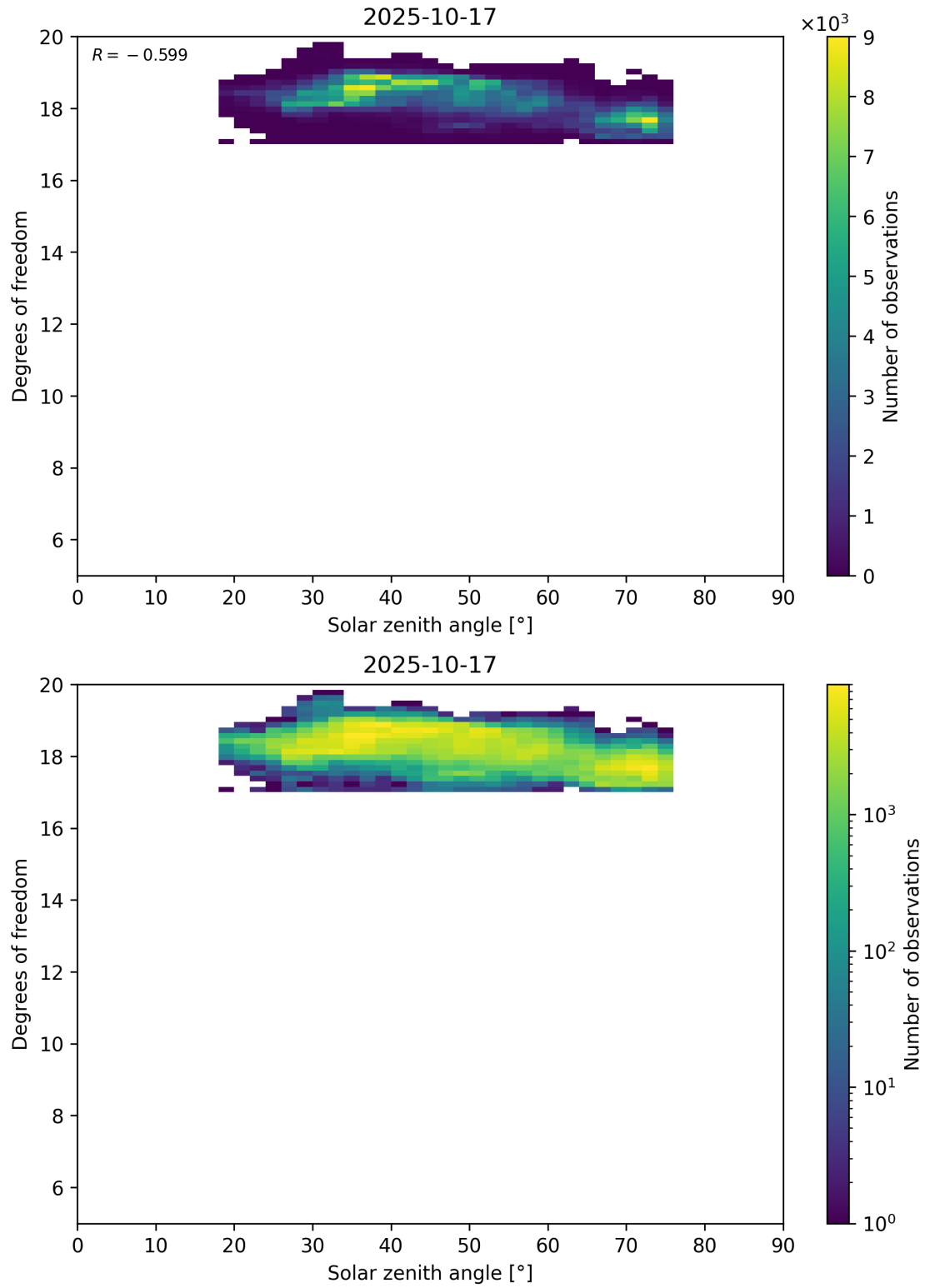
Figure 96: Scatter density plot of “Solar zenith angle” against “Degrees of freedom” for 2025-10-17 to 2025-10-18.
