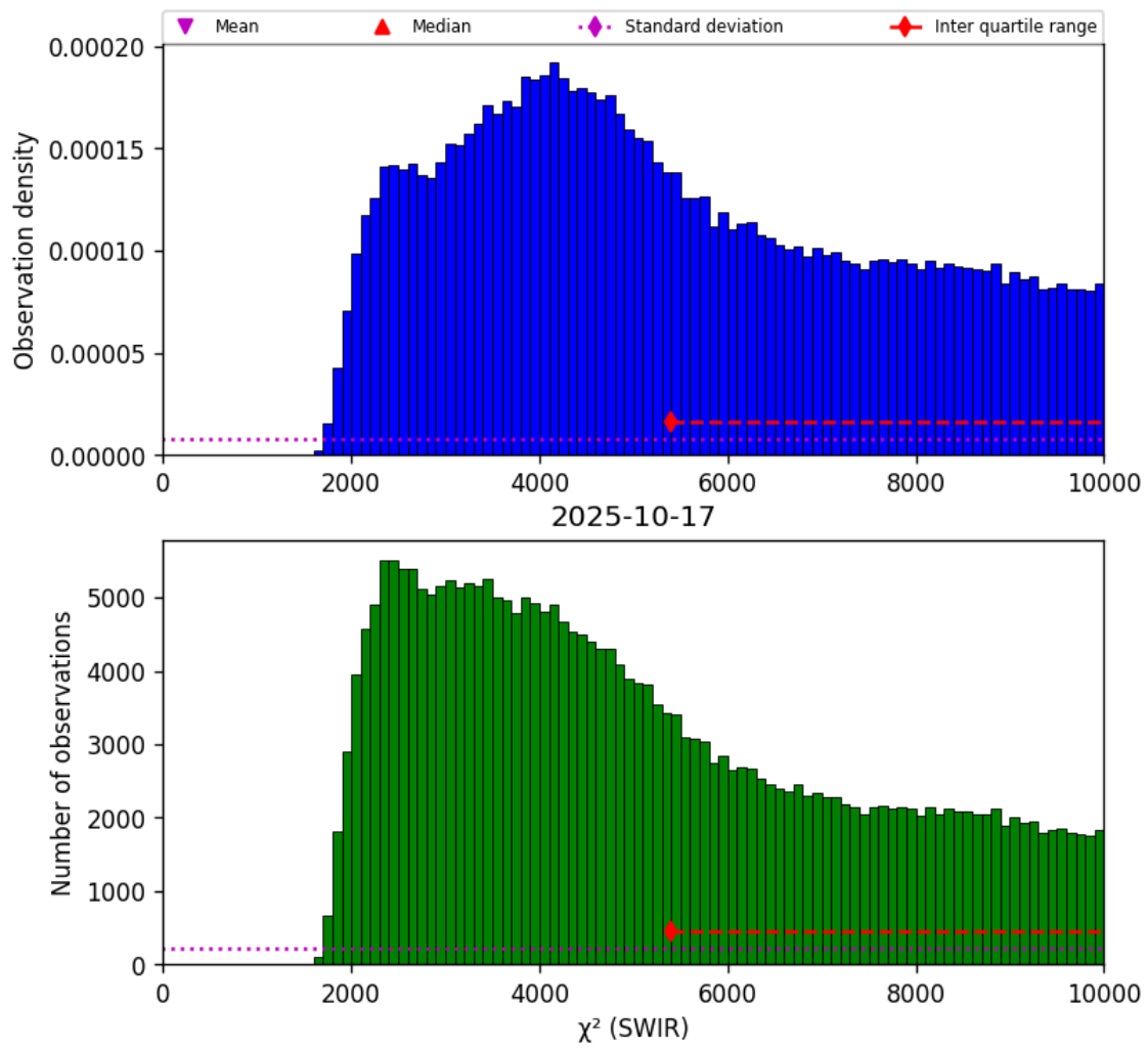
Figure 28: Histogram of " \chi^2 (SWIR)" for 2025-10-17 to 2025-10-18
