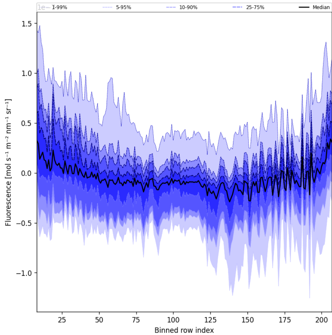
Figure 43: Along track statistics of “Fluorescence” for 2025-10-17 to 2025-10-18
