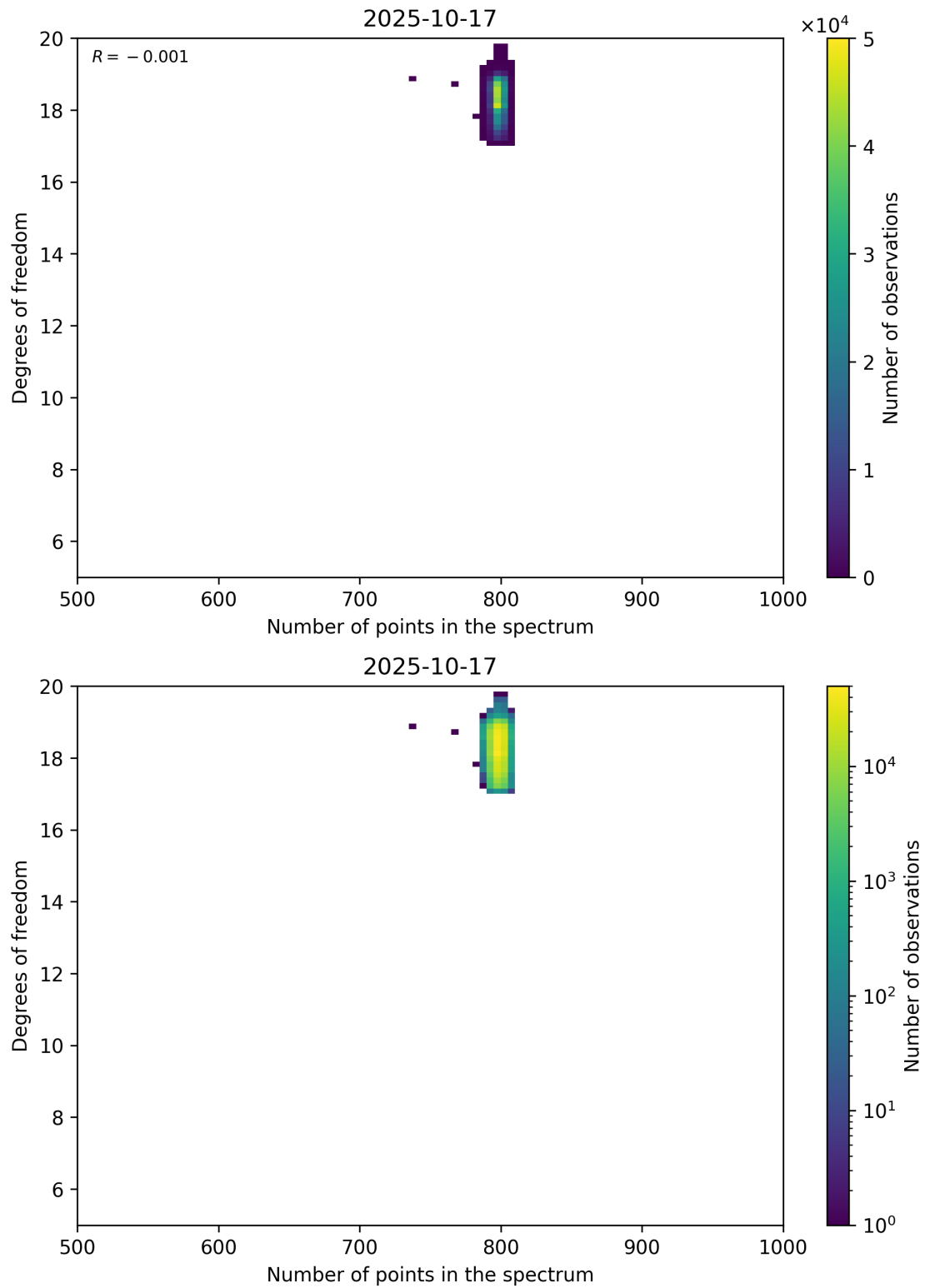
Figure 90: Scatter density plot of “Number of points in the spectrum” against “Degrees of freedom” for 2025-10-17 to 2025-10-18.
