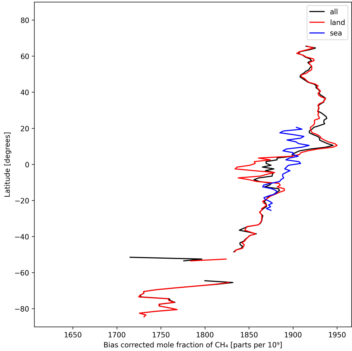
Figure 14: Zonal average of “Bias corrected mole fraction of CH 4 ” for 2025-10-17 to 2025-10-18.
