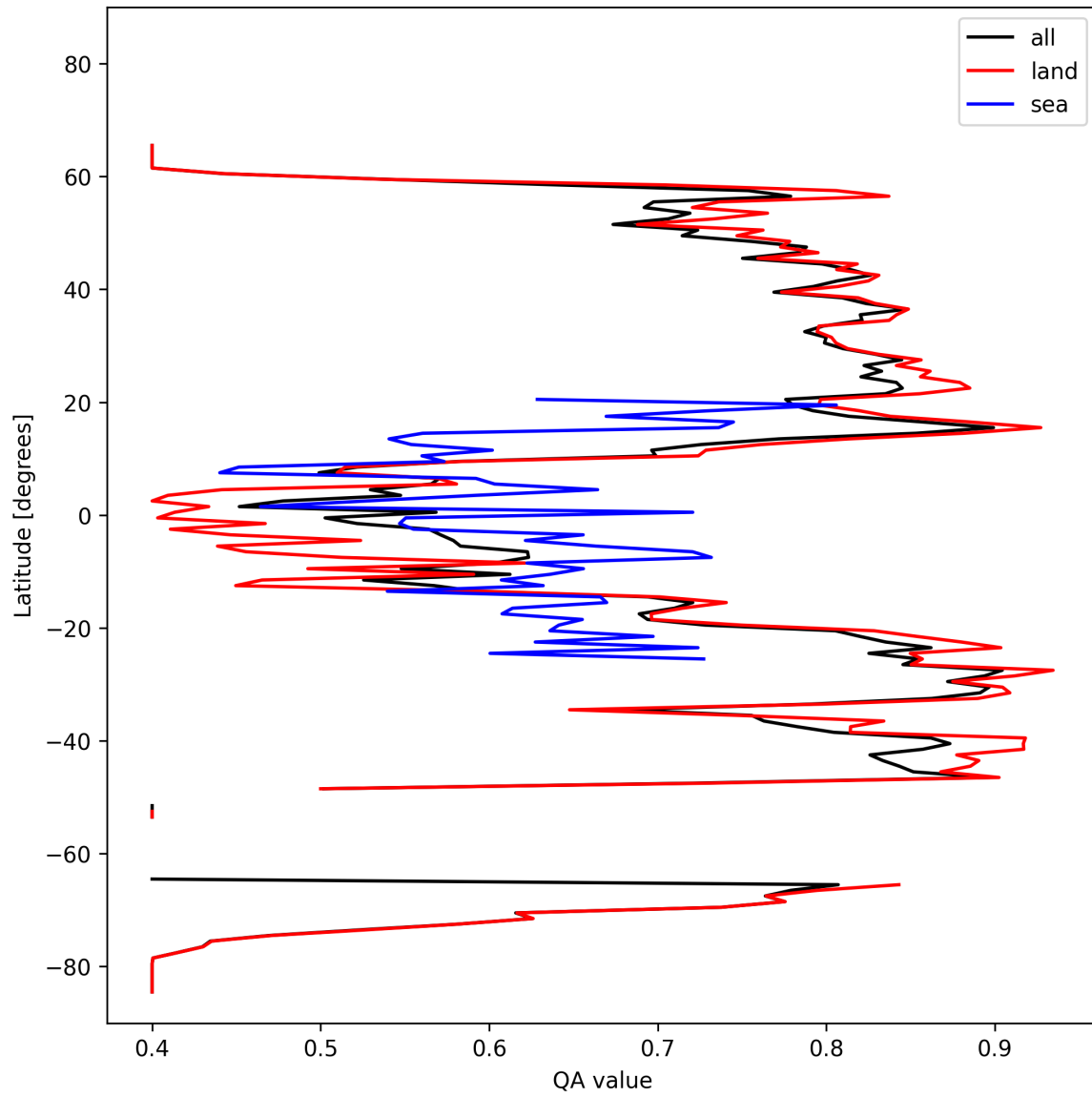
Figure 11: Zonal average of “QA value” for 2025-10-17 to 2025-10-18.
