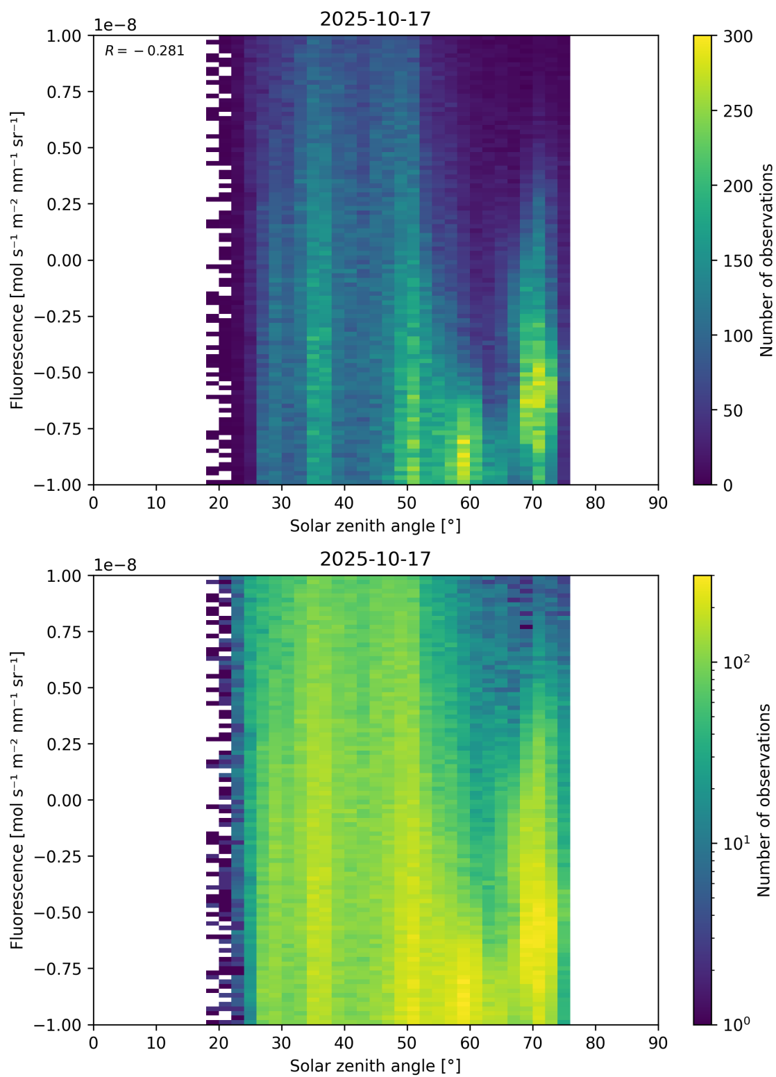
Figure 97: Scatter density plot of “Solar zenith angle” against “Fluorescence” for 2025-10-17 to 2025-10-18.
