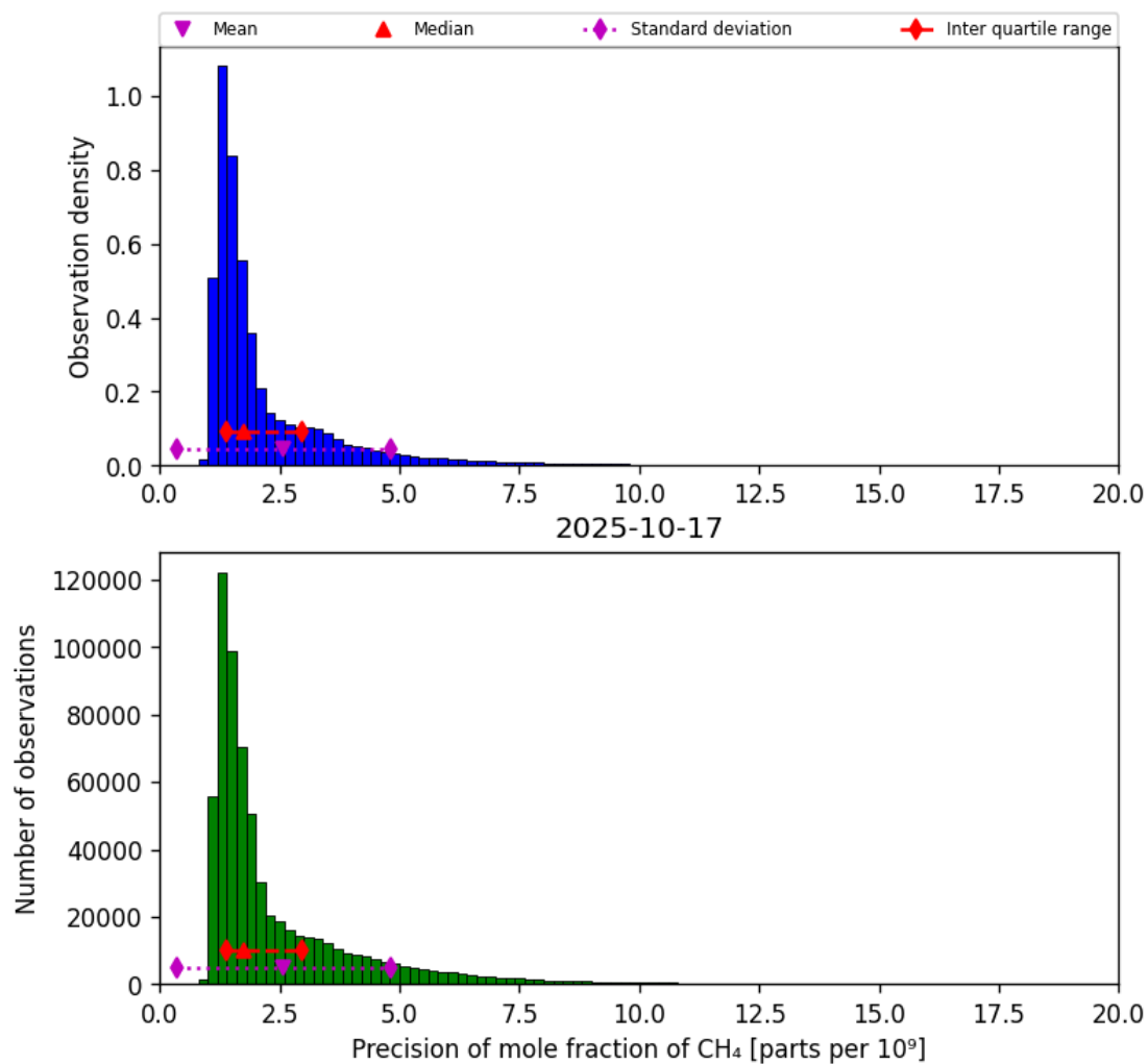
Figure 24: Histogram of “Precision of mole fraction of CH 4 ” for 2025-10-17 to 2025-10-18
