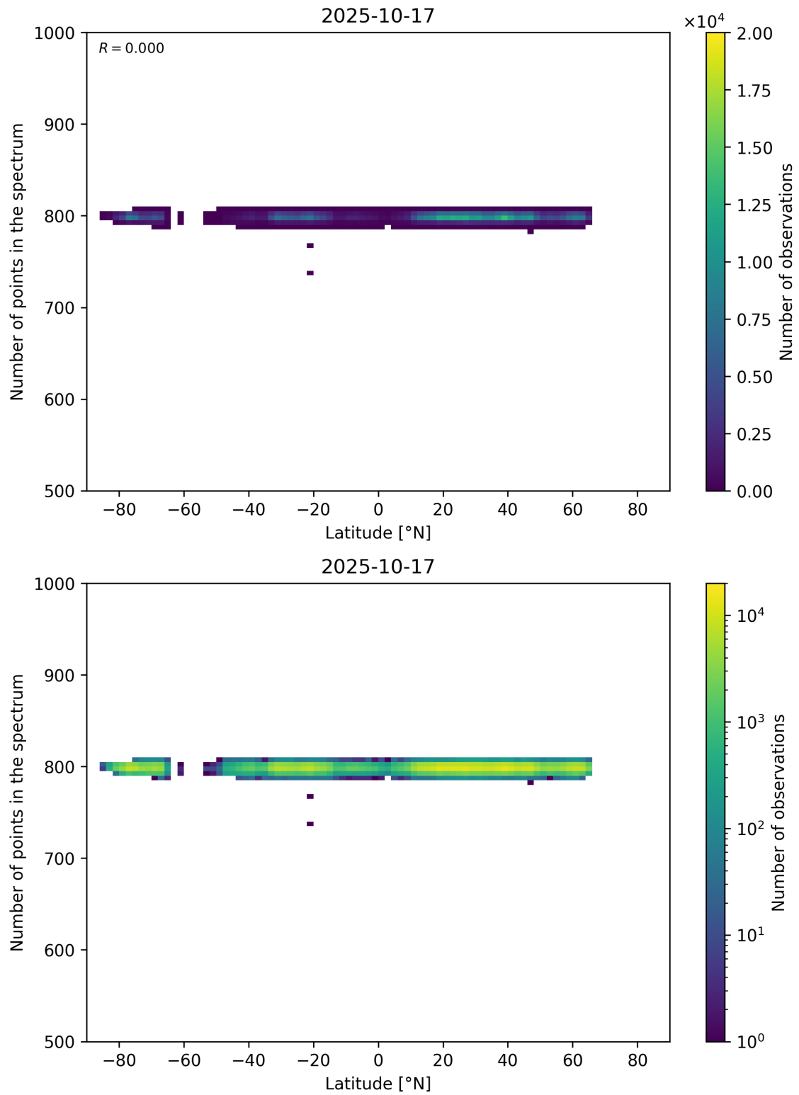
Figure 61: Scatter density plot of “Latitude” against “Number of points in the spectrum” for 2025-10-17 to 2025-10-18.
