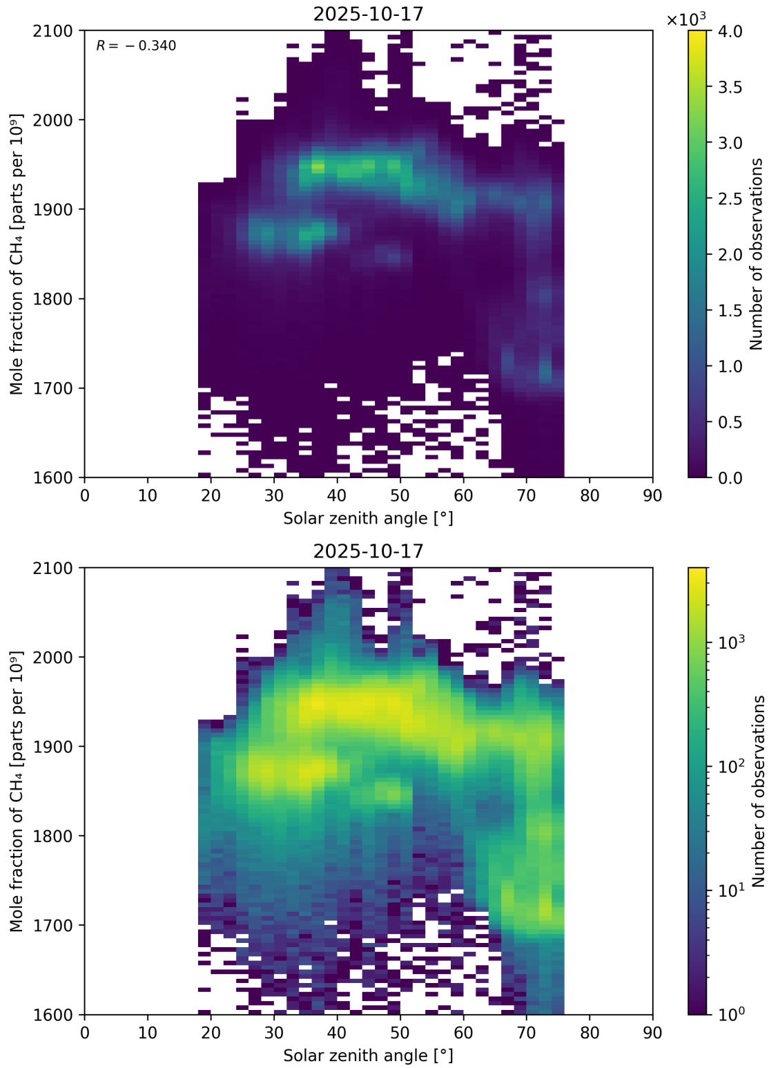
Figure 99: Scatter density plot of “Solar zenith angle” against “Mole fraction of \text{CH}_4 ” for 2025-10-17 to 2025-10-18.
