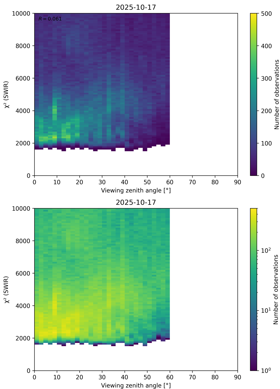
Figure 106: Scatter density plot of “Viewing zenith angle” against “ \chi^2 (SWIR)” for 2025-10-17 to 2025-10-18.
