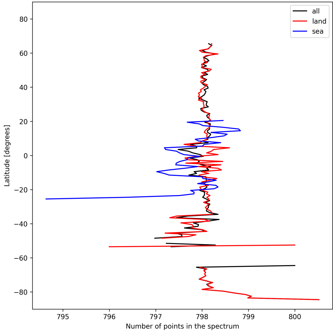
Figure 15: Zonal average of “Number of points in the spectrum” for 2025-10-17 to 2025-10-18.
