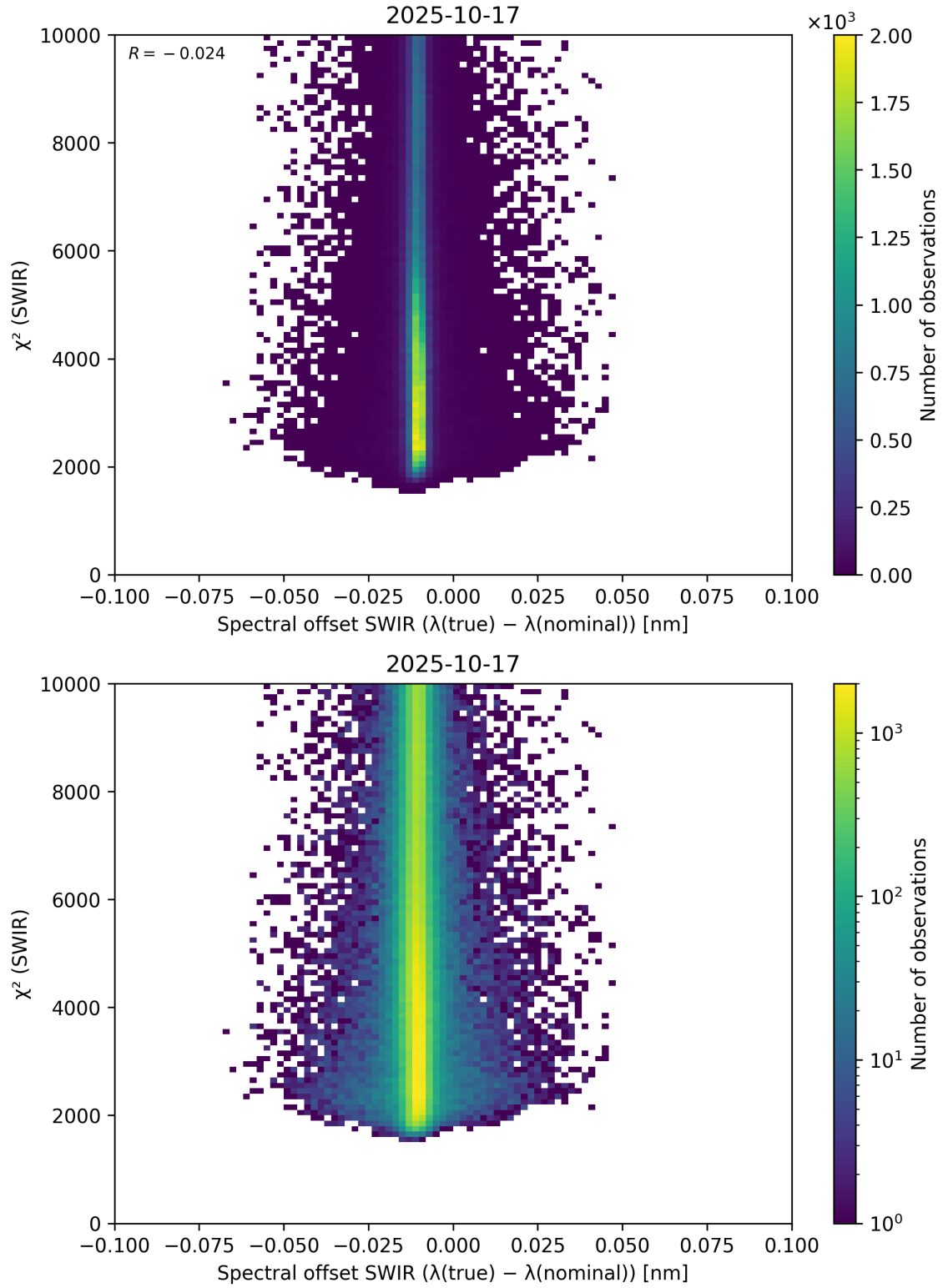
Figure 118: Scatter density plot of “Spectral offset SWIR ( \lambda_{\text{true}} - \lambda_{\text{nominal}} )” against “ \chi^2 (SWIR)” for 2025-10-17 to 2025-10-18.
