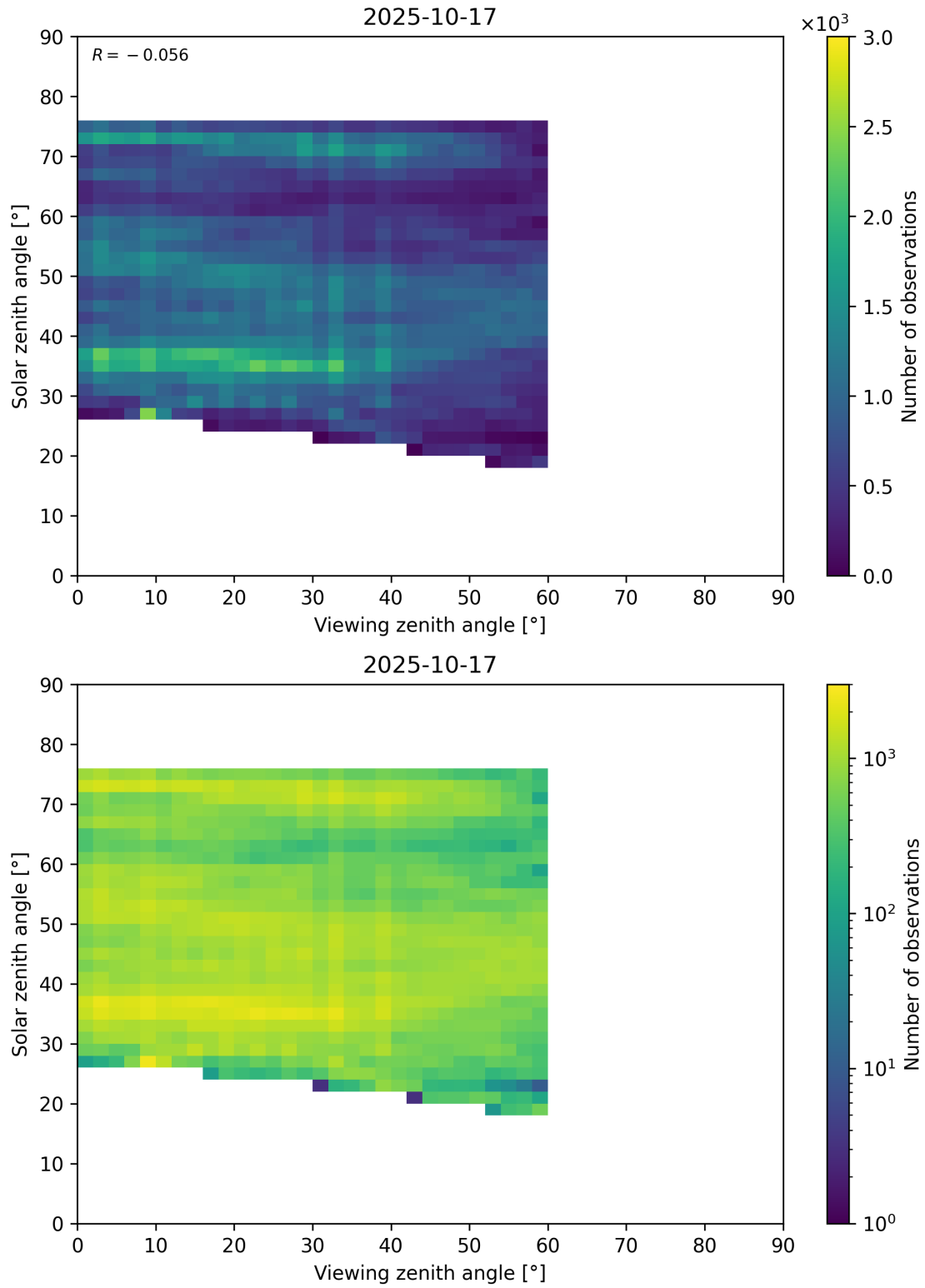
Figure 115: Scatter density plot of “Viewing zenith angle” against “Solar zenith angle” for 2025-10-17 to 2025-10-18.
