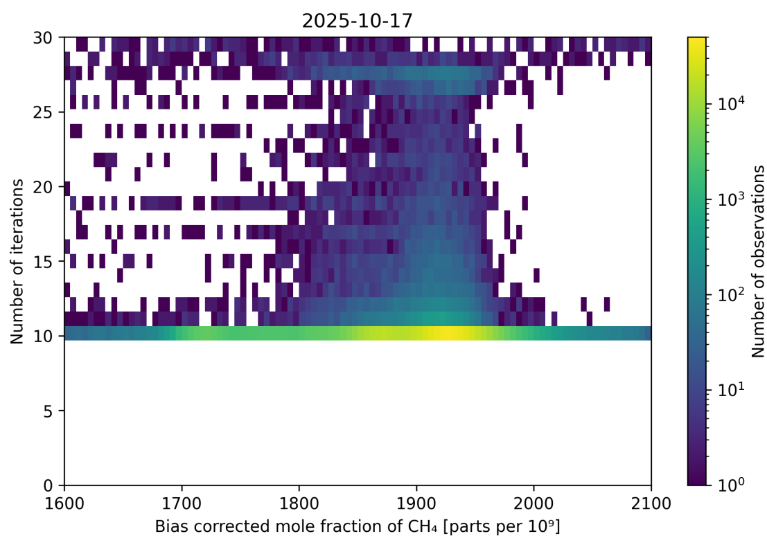
Figure 67: Scatter density plot of “Bias corrected mole fraction of CH 4 ” against “Number of iterations” for 2025-10-17 to 2025-10-18.
