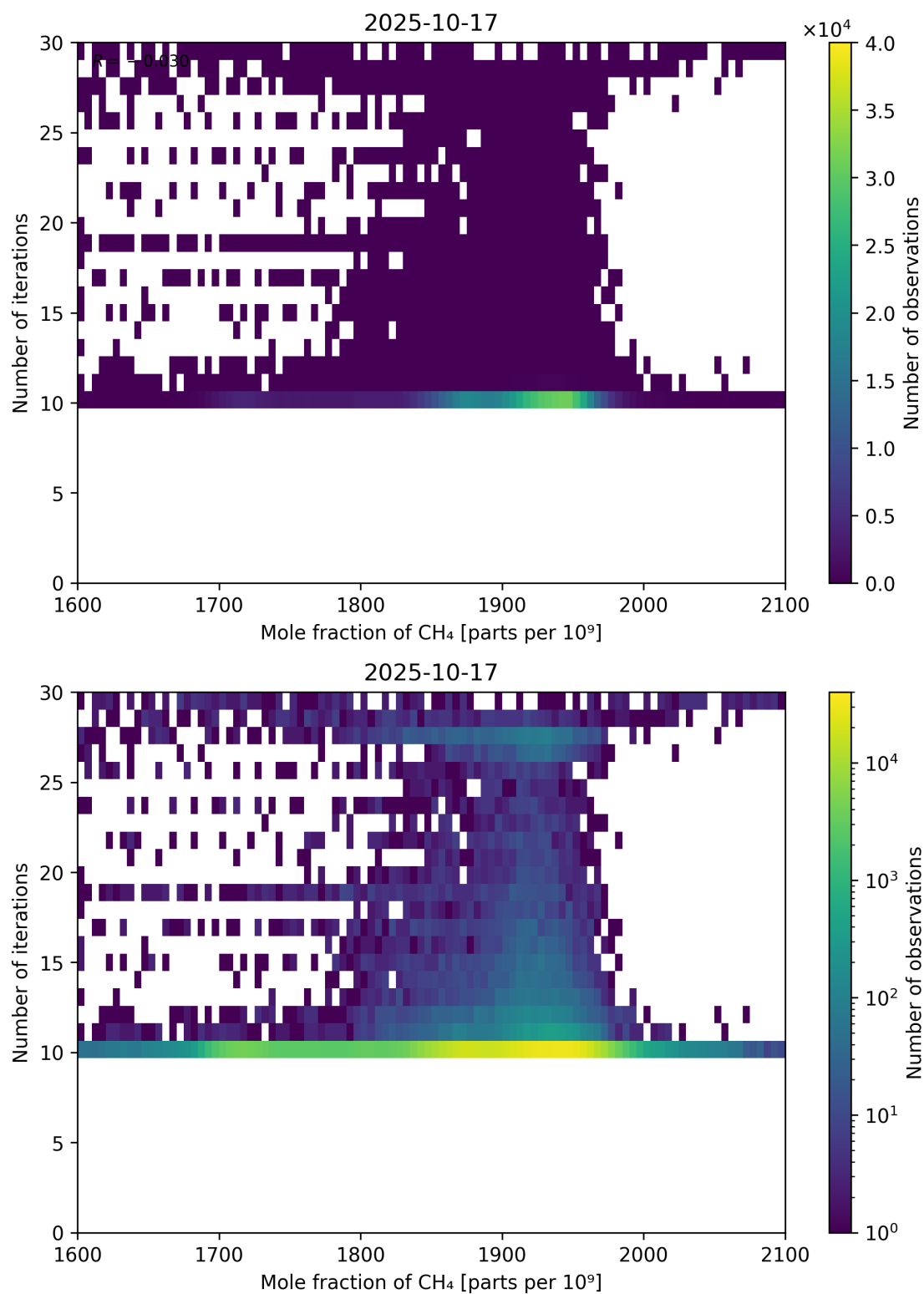
Figure 76: Scatter density plot of “Mole fraction of CH 4 ” against “Number of iterations” for 2025-10-17 to 2025-10-18.
