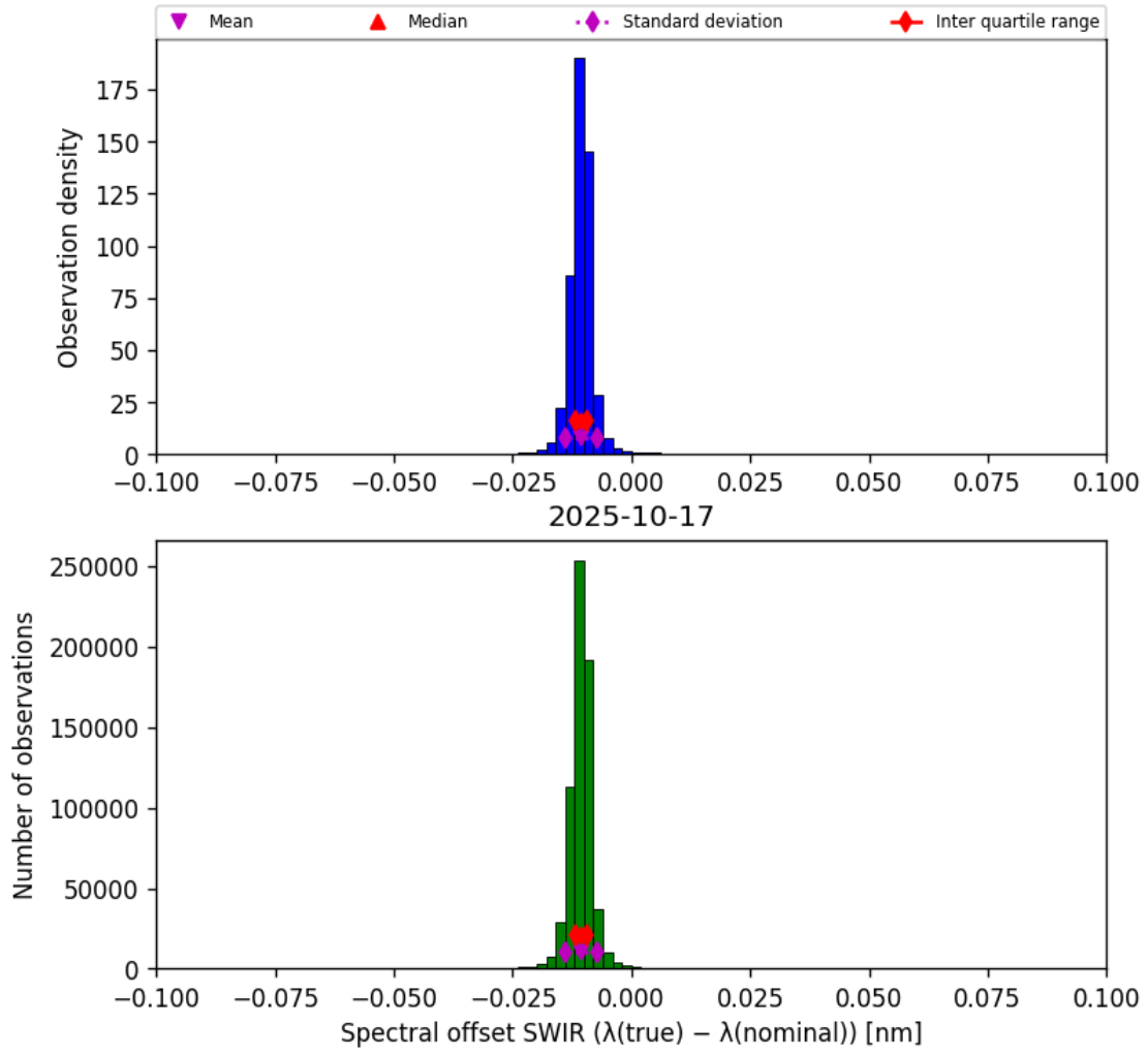
Figure 27: Histogram of “Spectral offset SWIR ( \lambda_{\text{true}} - \lambda_{\text{nominal}} )” for 2025-10-17 to 2025-10-18
