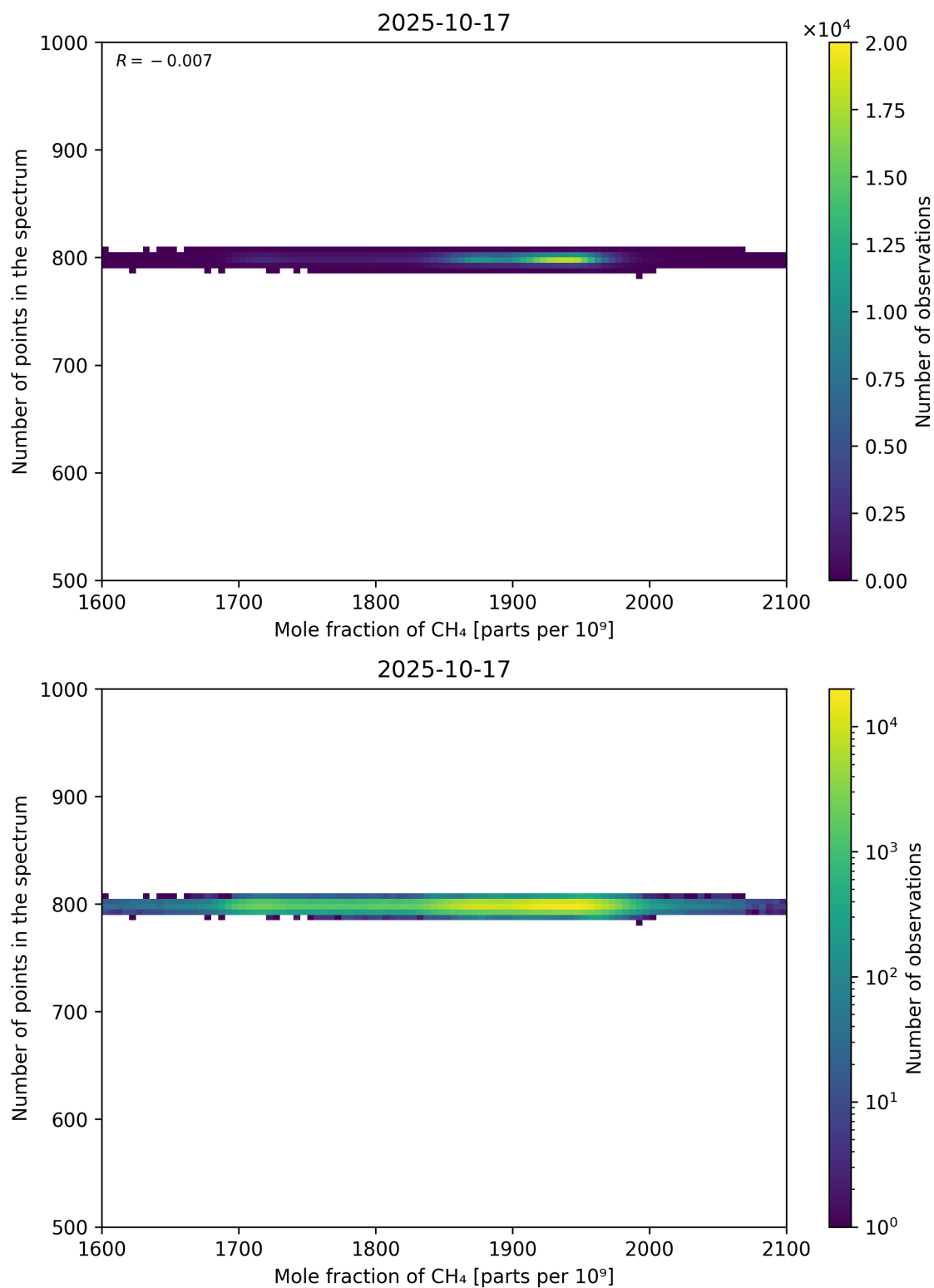
Figure 77: Scatter density plot of “Mole fraction of CH 4 ” against “Number of points in the spectrum” for 2025-10-17 to 2025-10-18.
