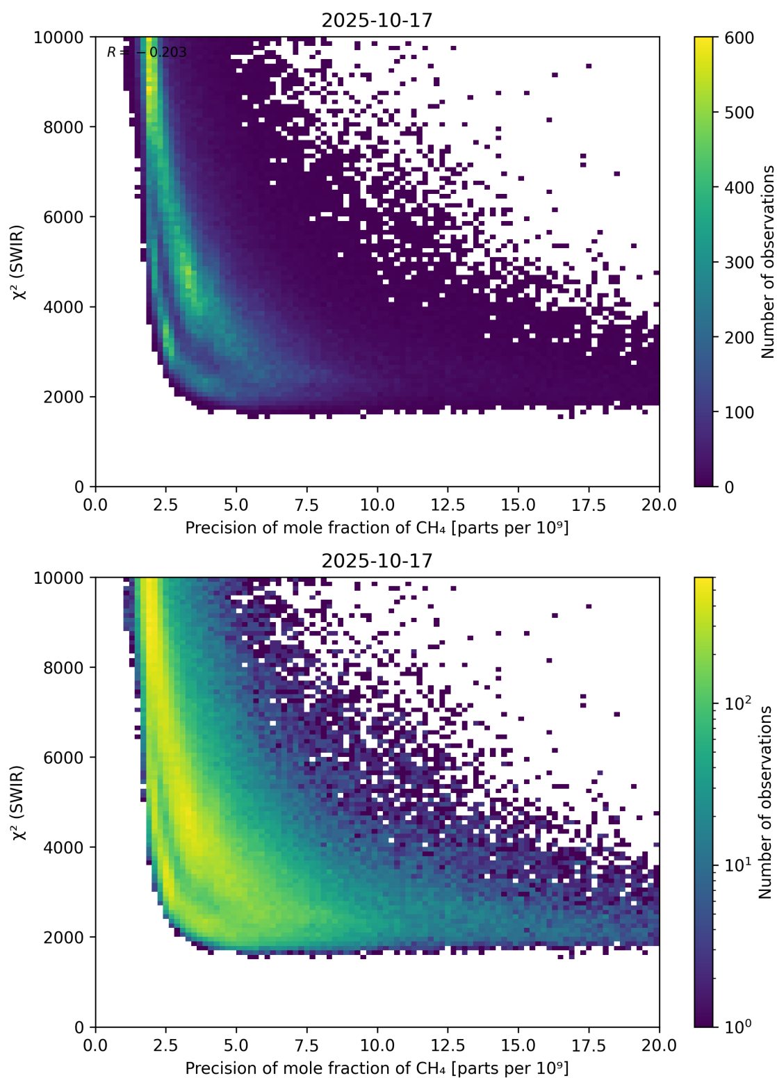
Figure 79: Scatter density plot of “Precision of mole fraction of \text{CH}_4 ” against “ \chi^2 (SWIR)” for 2025-10-17 to 2025-10-18.
