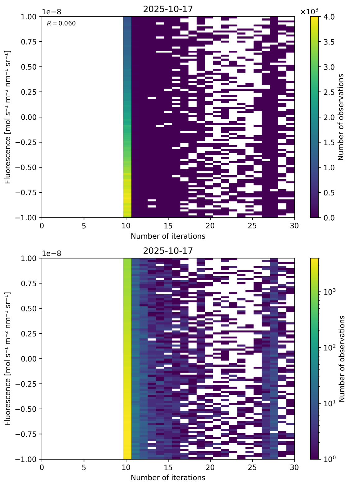
Figure 87: Scatter density plot of “Number of iterations” against “Fluorescence” for 2025-10-17 to 2025-10-18.
