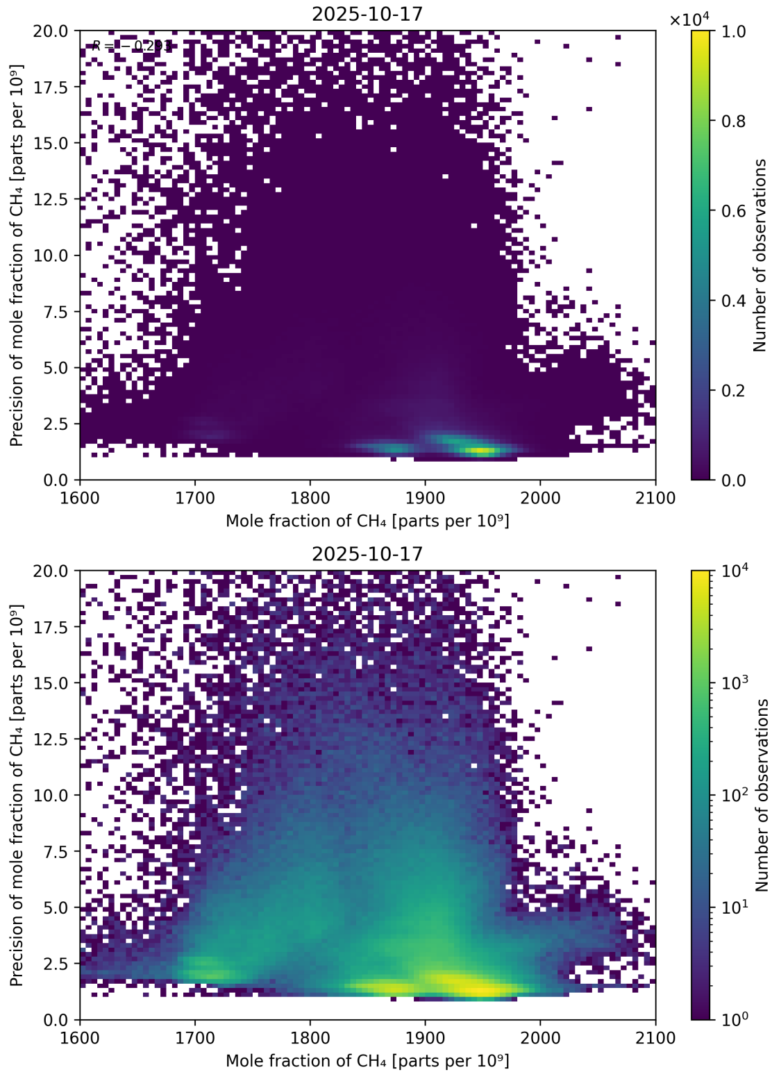
Figure 75: Scatter density plot of “Mole fraction of CH 4 ” against “Precision of mole fraction of CH 4 ” for 2025-10-17 to 2025-10-18.
