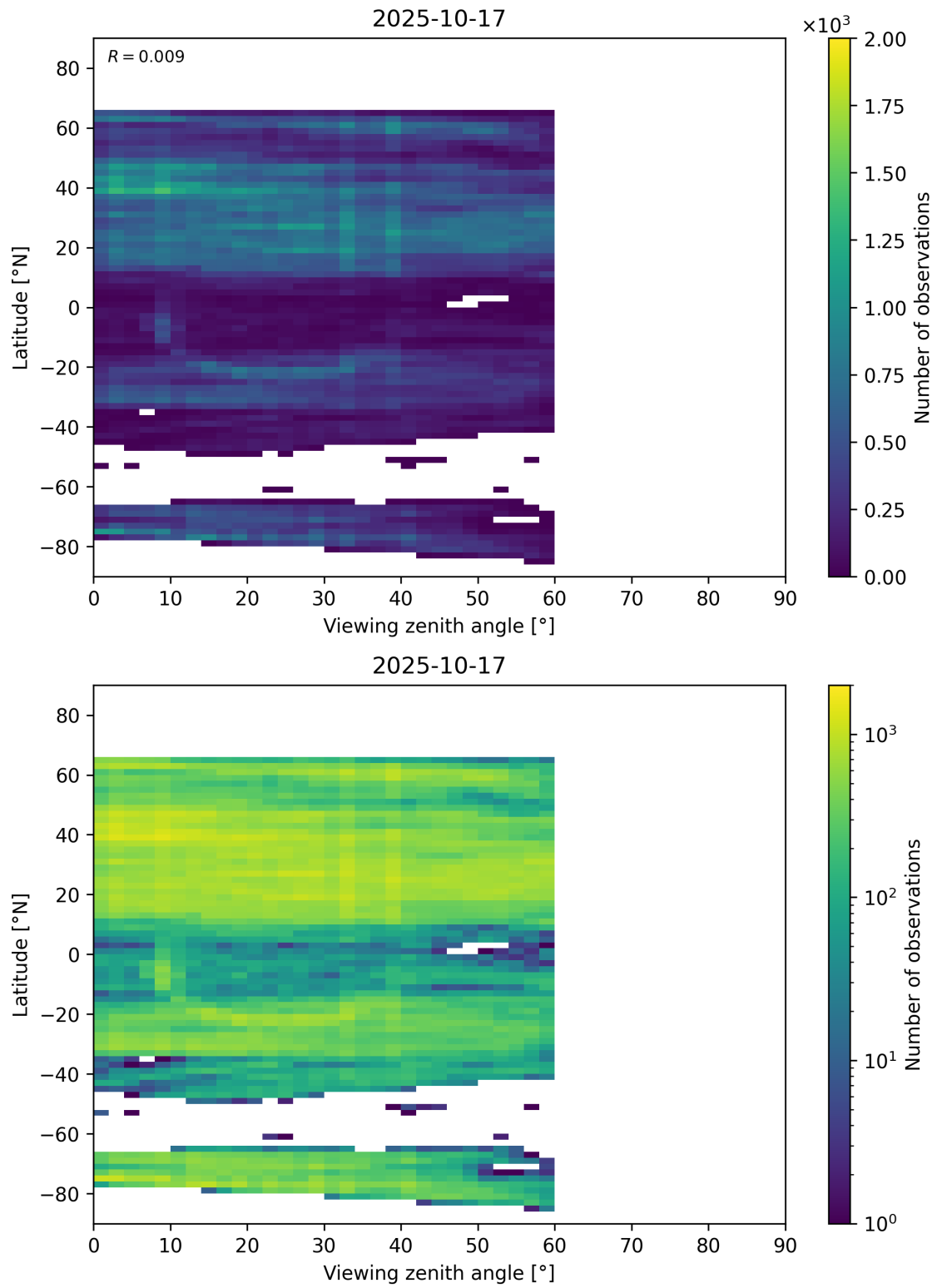
Figure 109: Scatter density plot of “Viewing zenith angle” against “Latitude” for 2025-10-17 to 2025-10-18.
