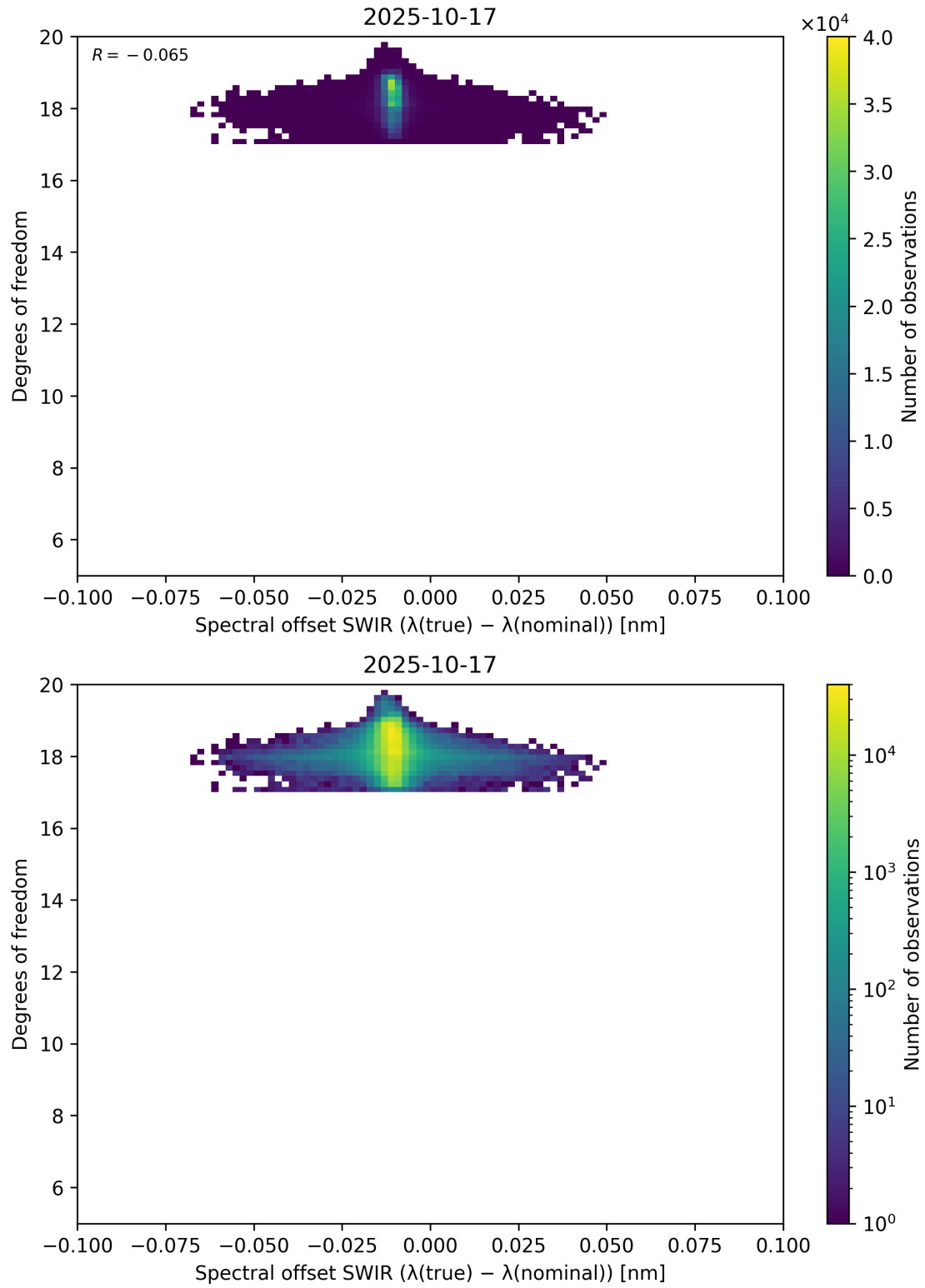
Figure 119: Scatter density plot of “Spectral offset SWIR ( \lambda_{\text{true}} - \lambda_{\text{nominal}} )” against “Degrees of freedom” for 2025-10-17 to 2025-10-18.
