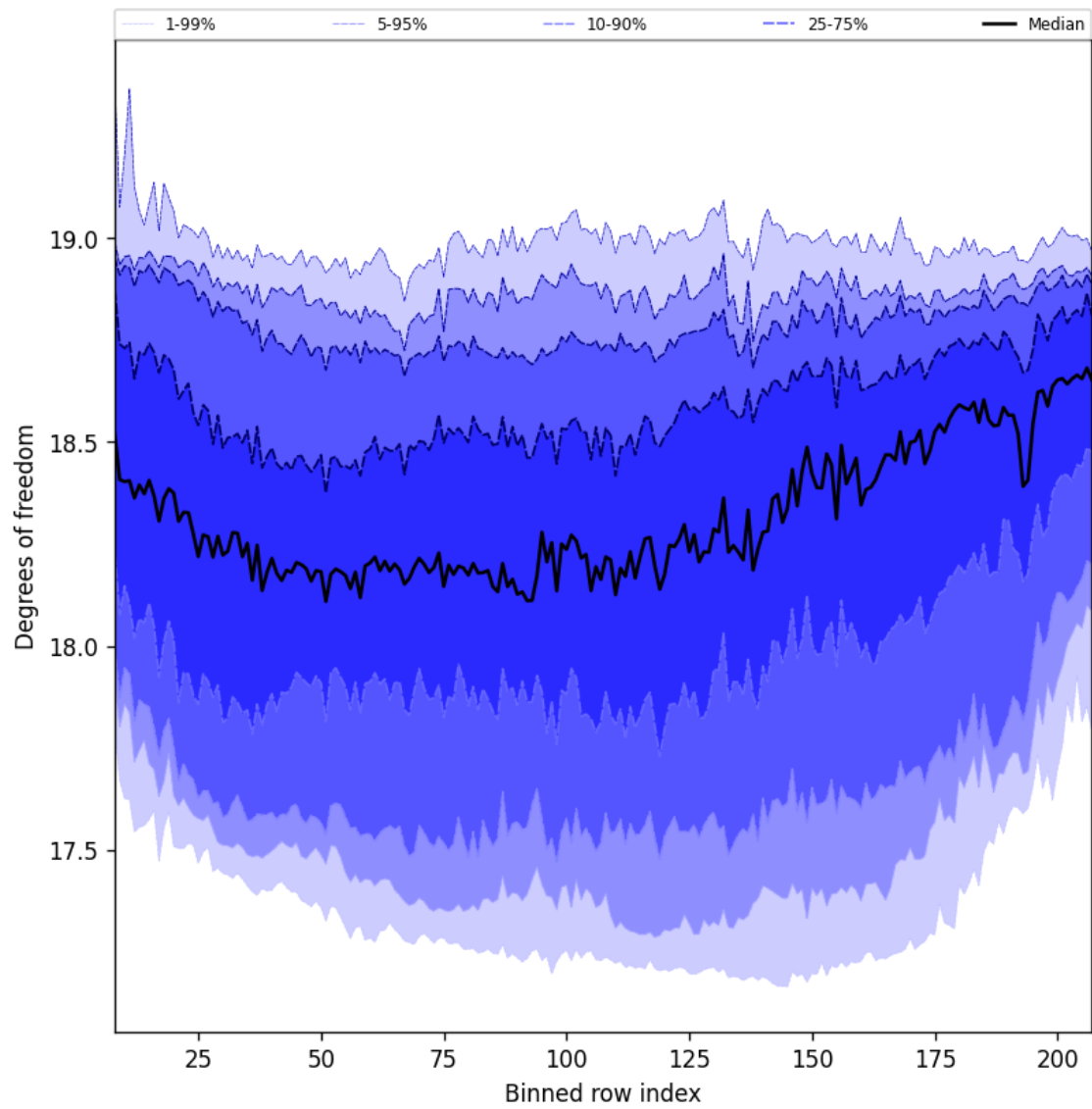
Figure 41: Along track statistics of “Degrees of freedom” for 2025-10-17 to 2025-10-18
