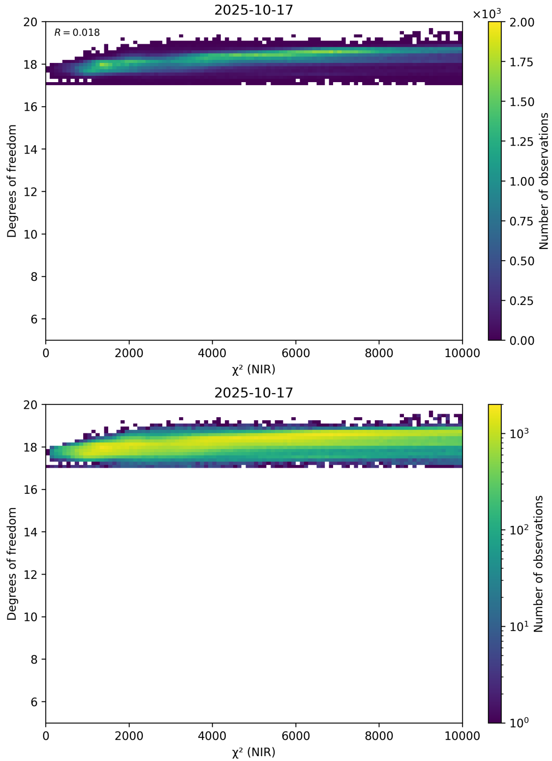
Figure 44: Scatter density plot of “ \chi^2 (NIR)” against “Degrees of freedom” for 2025-10-17 to 2025-10-18.
