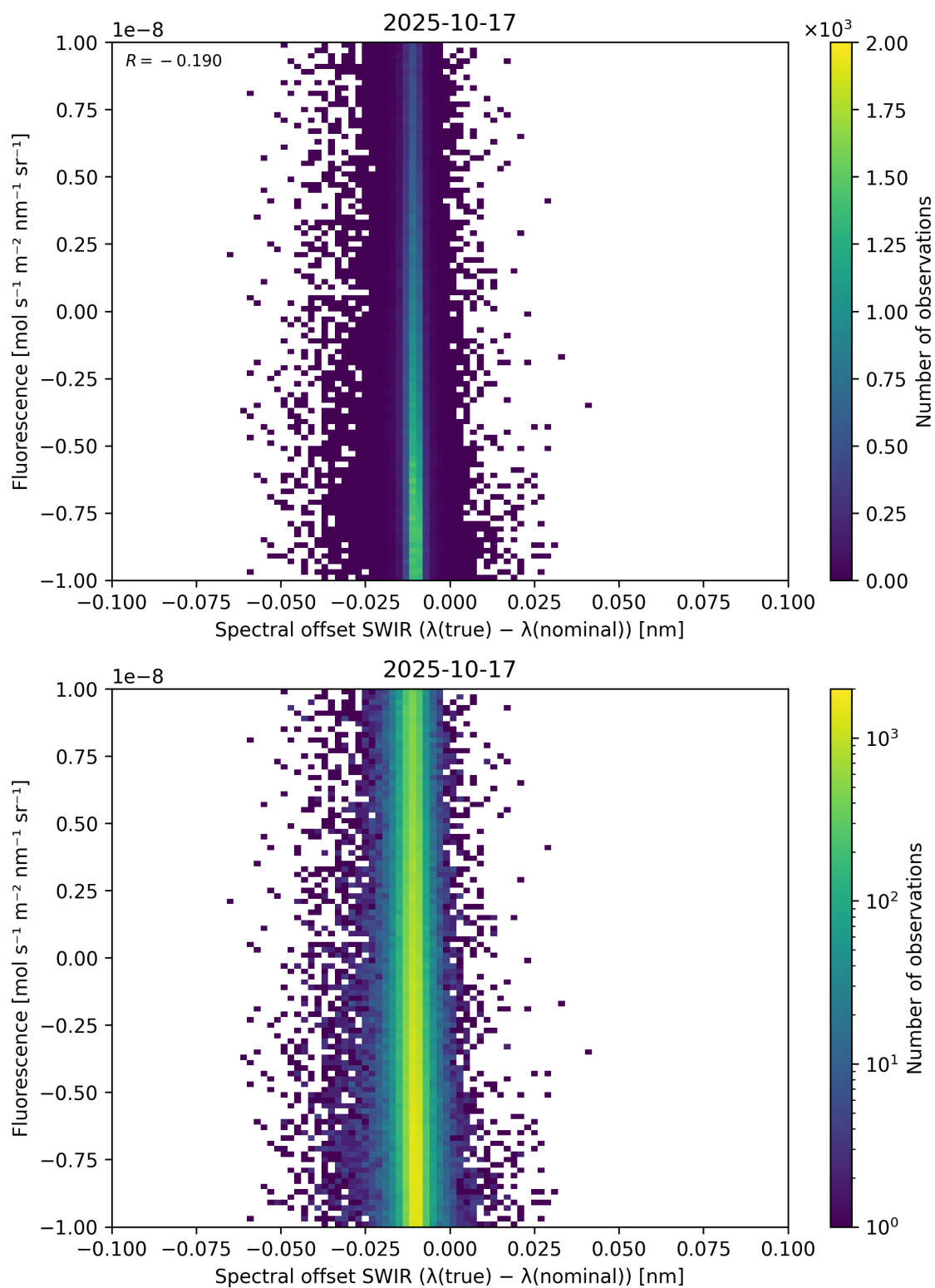
Figure 120: Scatter density plot of “Spectral offset SWIR ( \lambda_{\text{true}} - \lambda_{\text{nominal}} )” against “Fluorescence” for 2025-10-17 to 2025-10-18.
