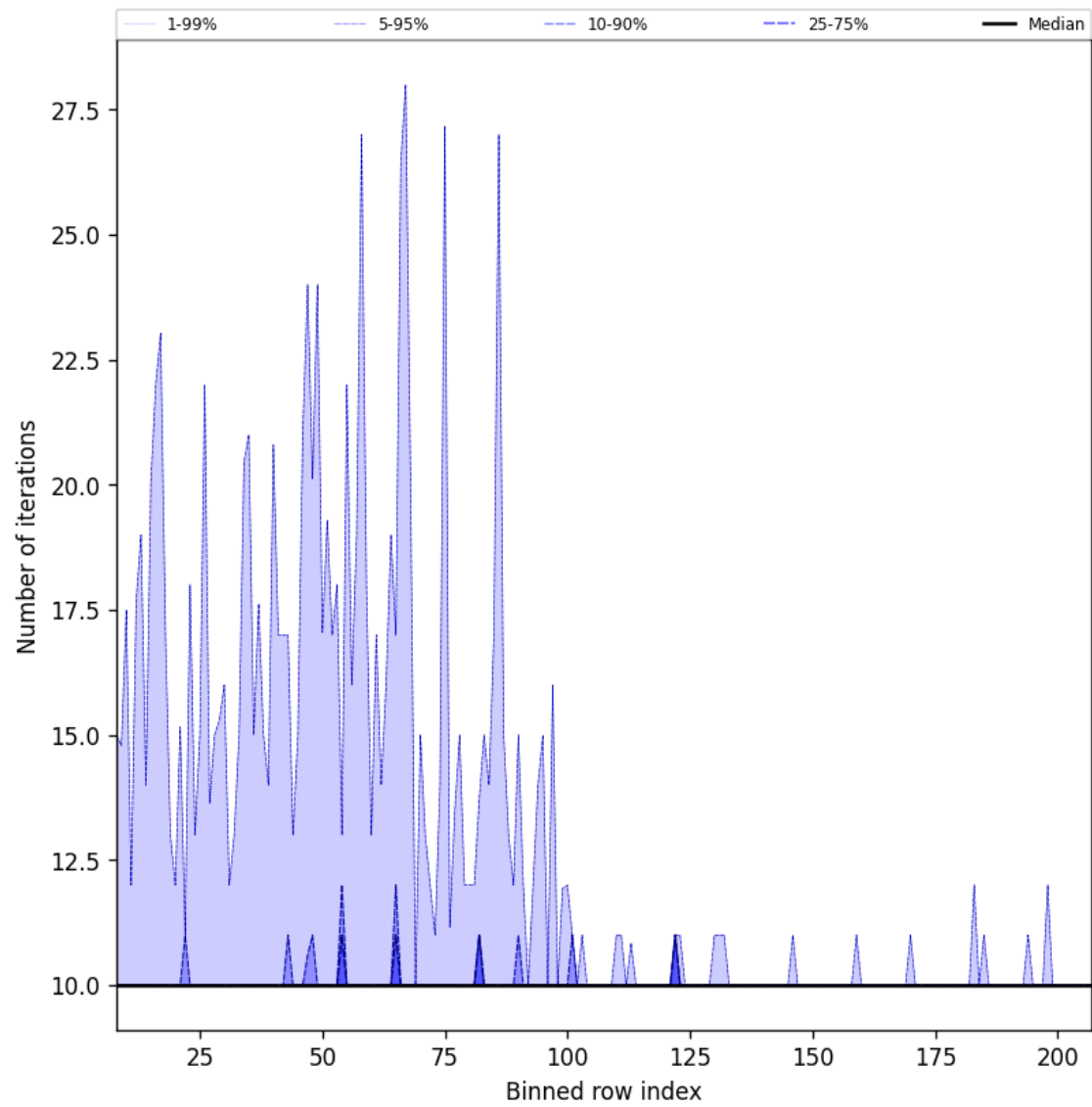
Figure 42: Along track statistics of “Number of iterations” for 2025-10-17 to 2025-10-18
