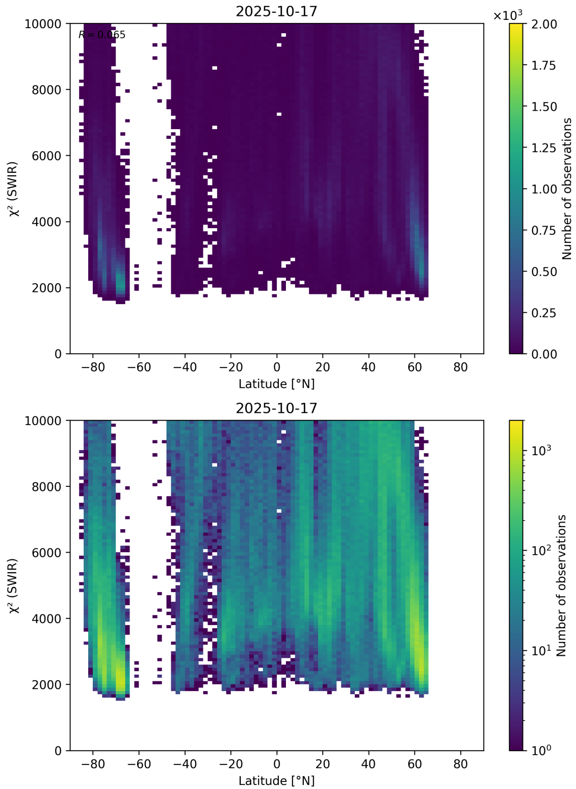
Figure 54: Scatter density plot of “Latitude” against “ \chi^2 (SWIR)” for 2025-10-17 to 2025-10-18.
