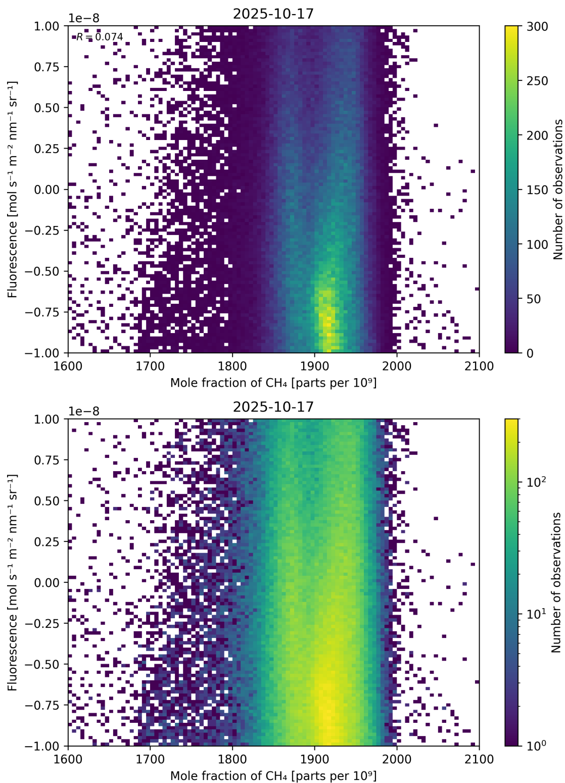
Figure 73: Scatter density plot of “Mole fraction of \text{CH}_4 ” against “Fluorescence” for 2025-10-17 to 2025-10-18.
