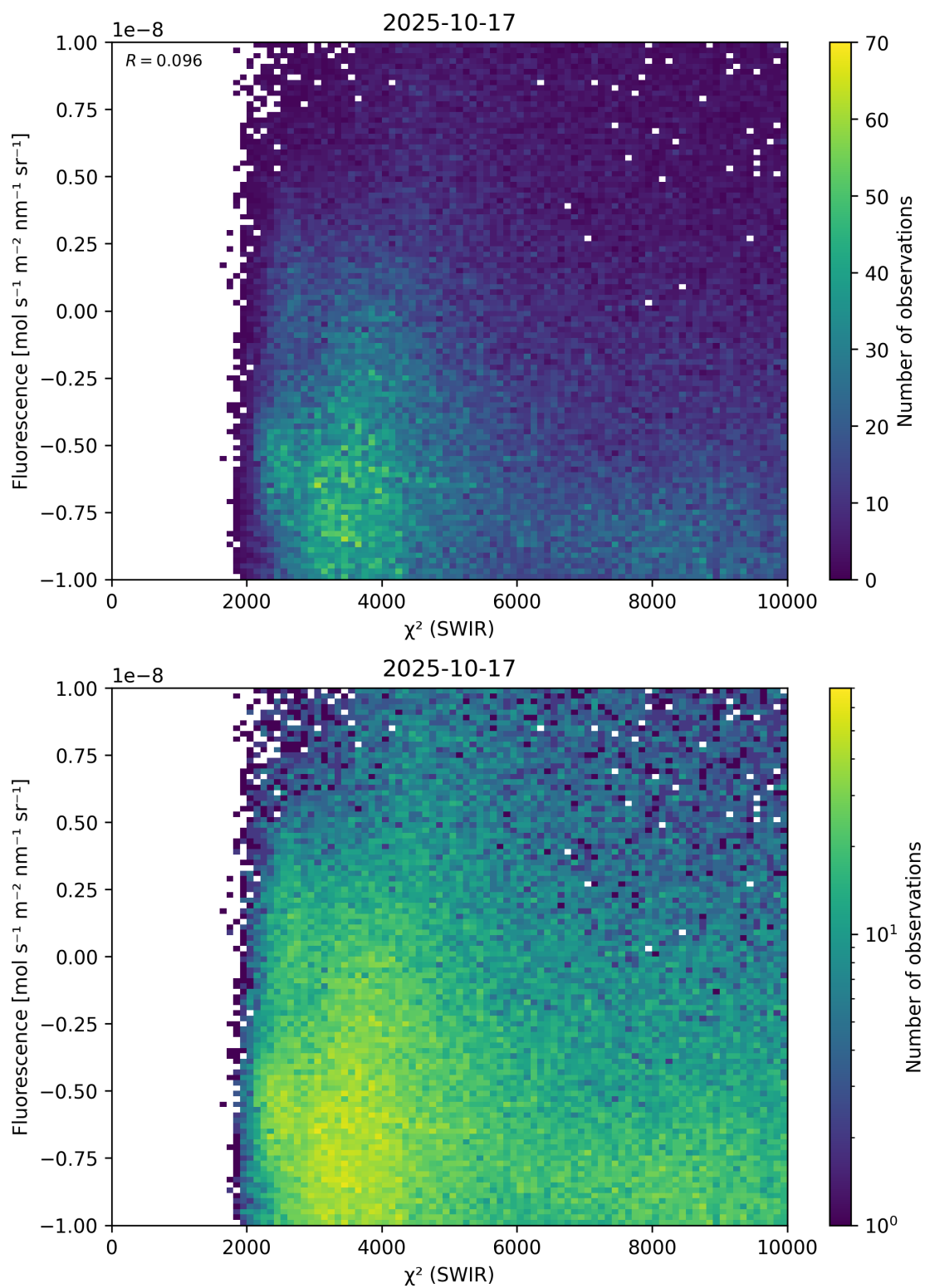
Figure 49: Scatter density plot of “ \chi^2 (SWIR)” against “Fluorescence” for 2025-10-17 to 2025-10-18.
