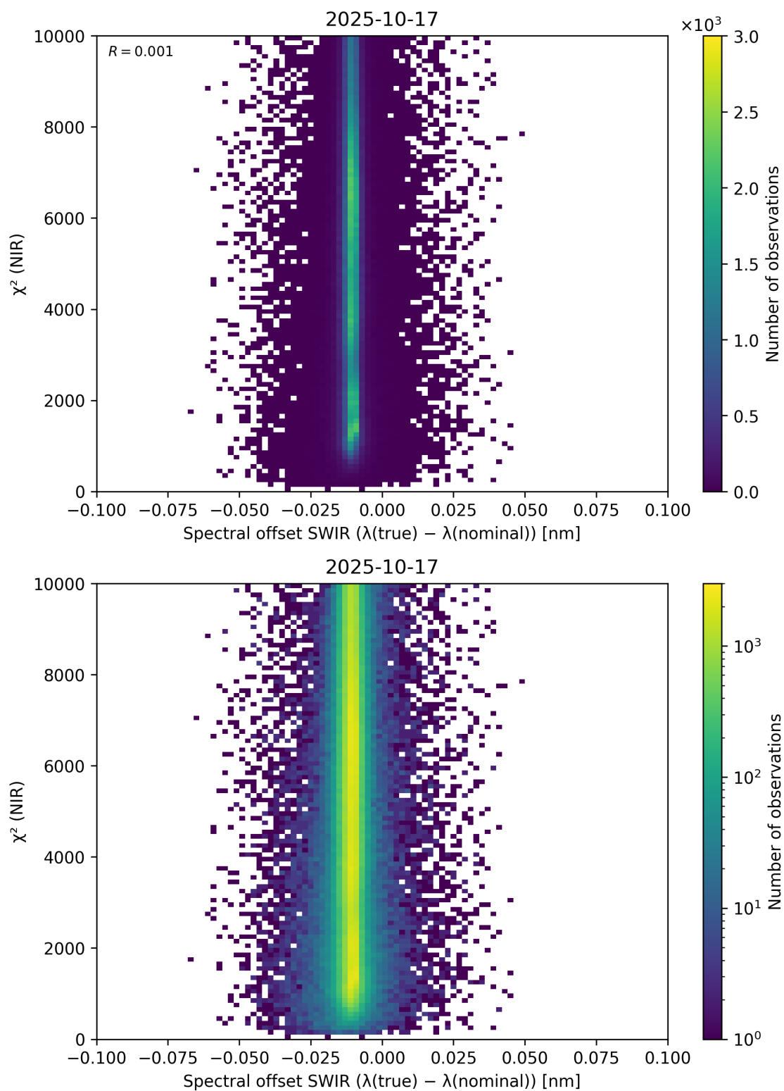
Figure 117: Scatter density plot of “Spectral offset SWIR ( \lambda_{\text{true}} - \lambda_{\text{nominal}} )” against “ \chi^2 (NIR)” for 2025-10-17 to 2025-10-18.
