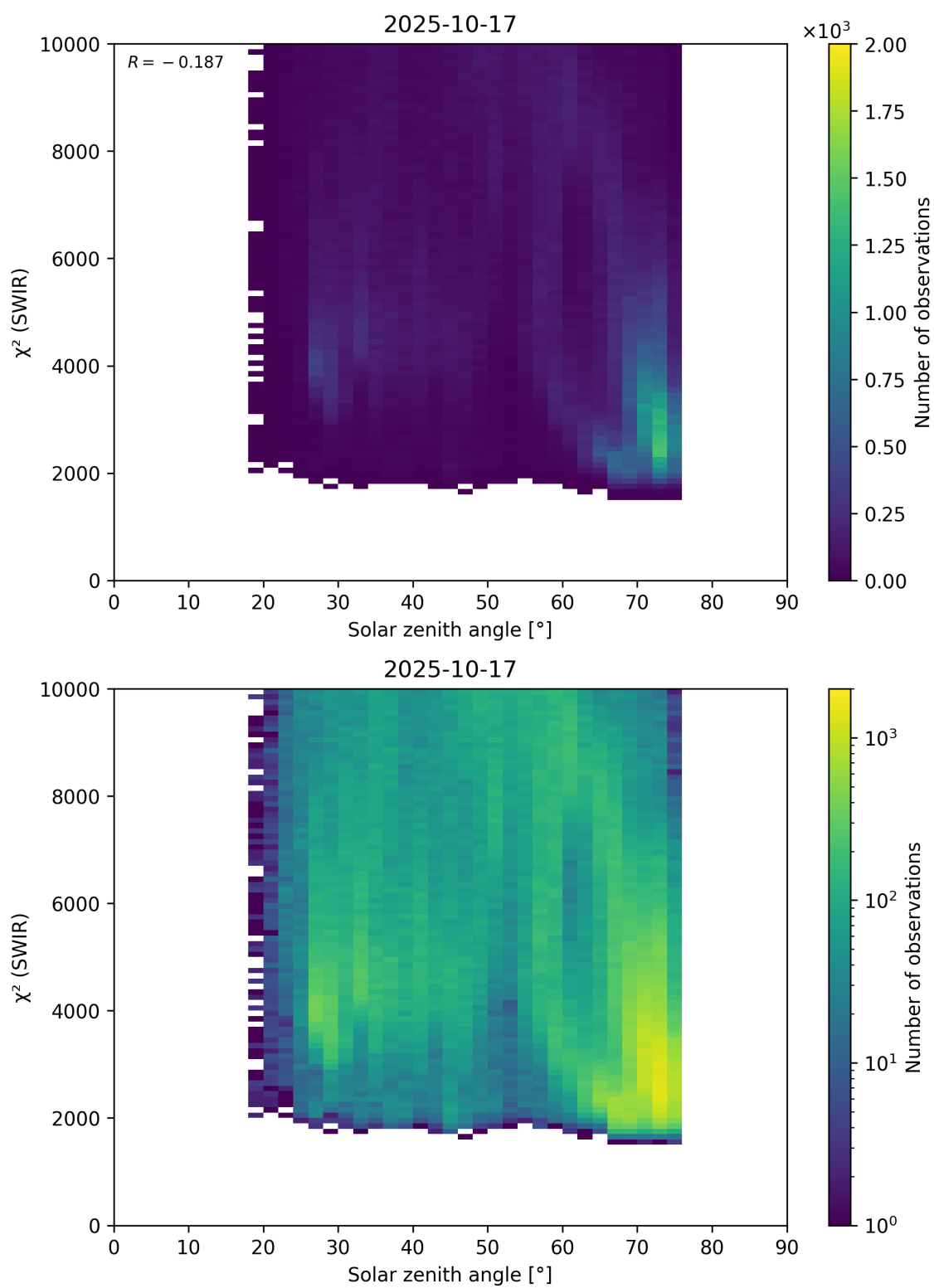
Figure 95: Scatter density plot of “Solar zenith angle” against “ \chi^2 (SWIR)” for 2025-10-17 to 2025-10-18.
