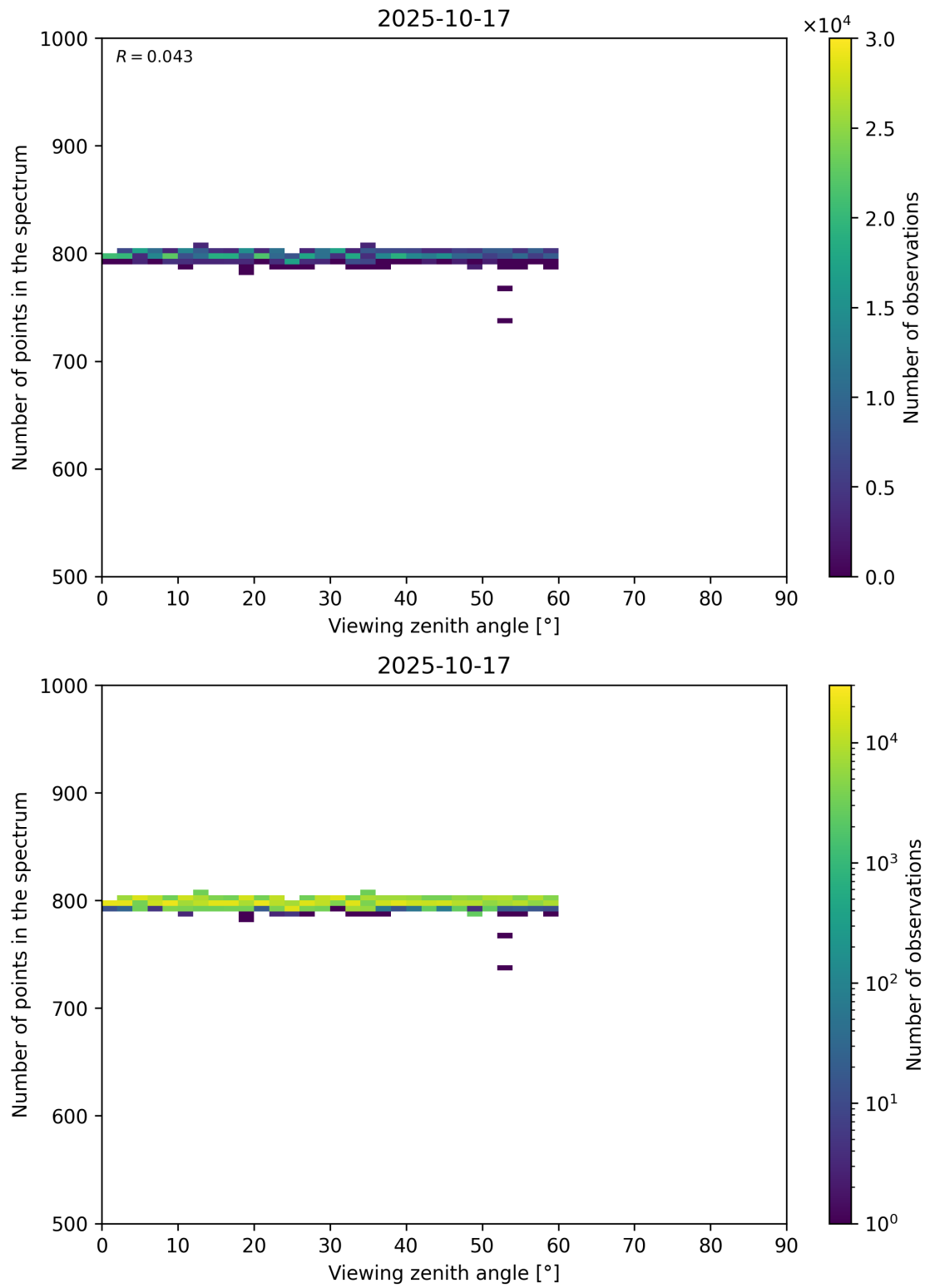
Figure 114: Scatter density plot of “Viewing zenith angle” against “Number of points in the spectrum” for 2025-10-17 to 2025-10-18.
