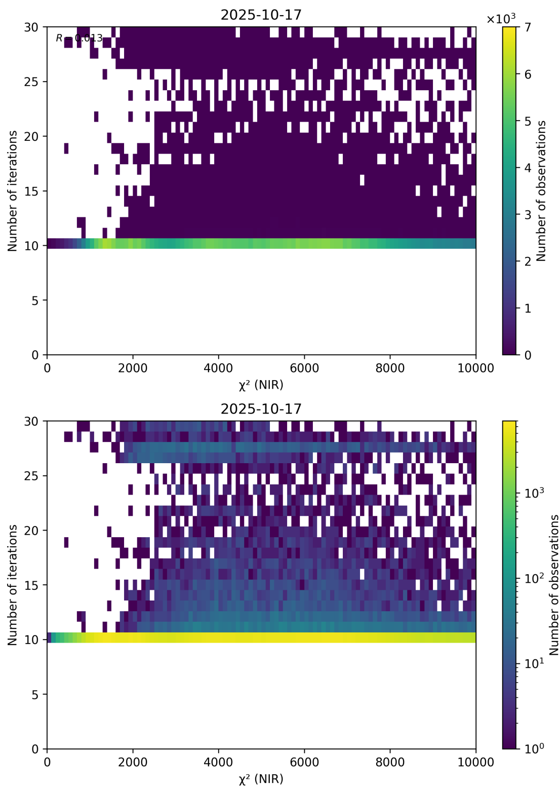
Figure 46: Scatter density plot of “ \chi^2 (NIR)” against “Number of iterations” for 2025-10-17 to 2025-10-18.
