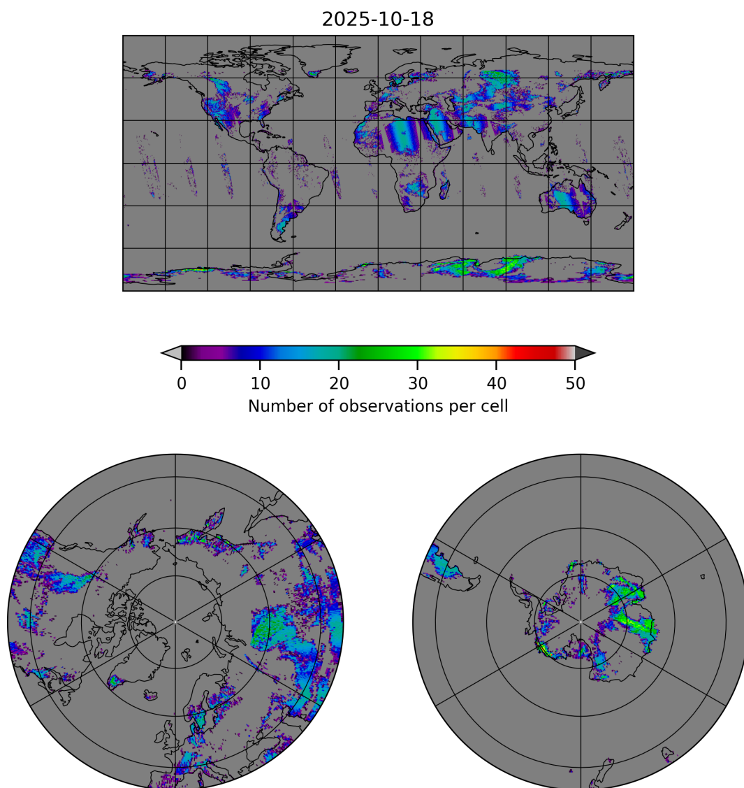
Figure 10: Map of the number of observations for 2025-10-17 to 2025-10-19
