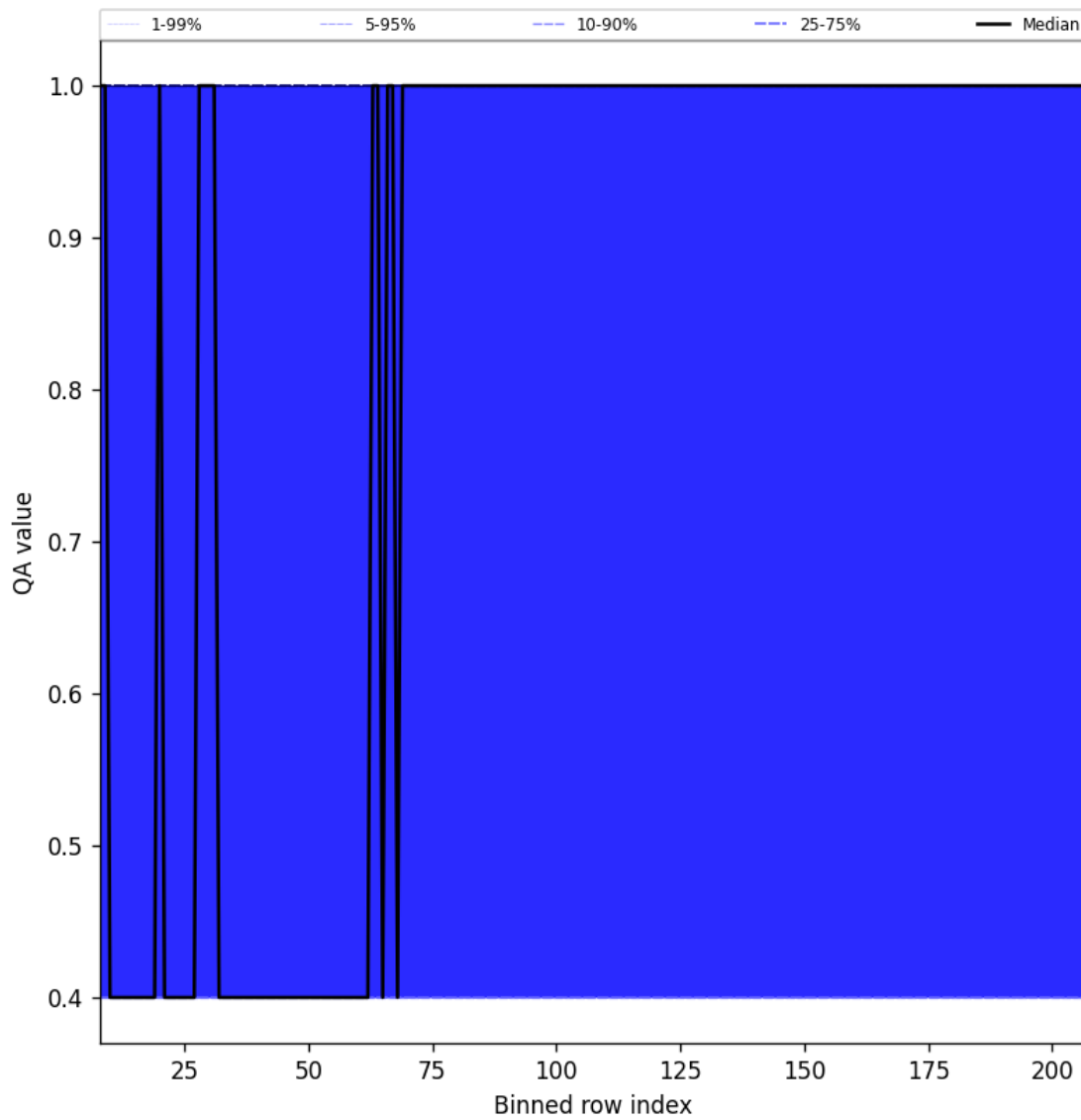
Figure 33: Along track statistics of “QA value” for 2025-10-17 to 2025-10-19
