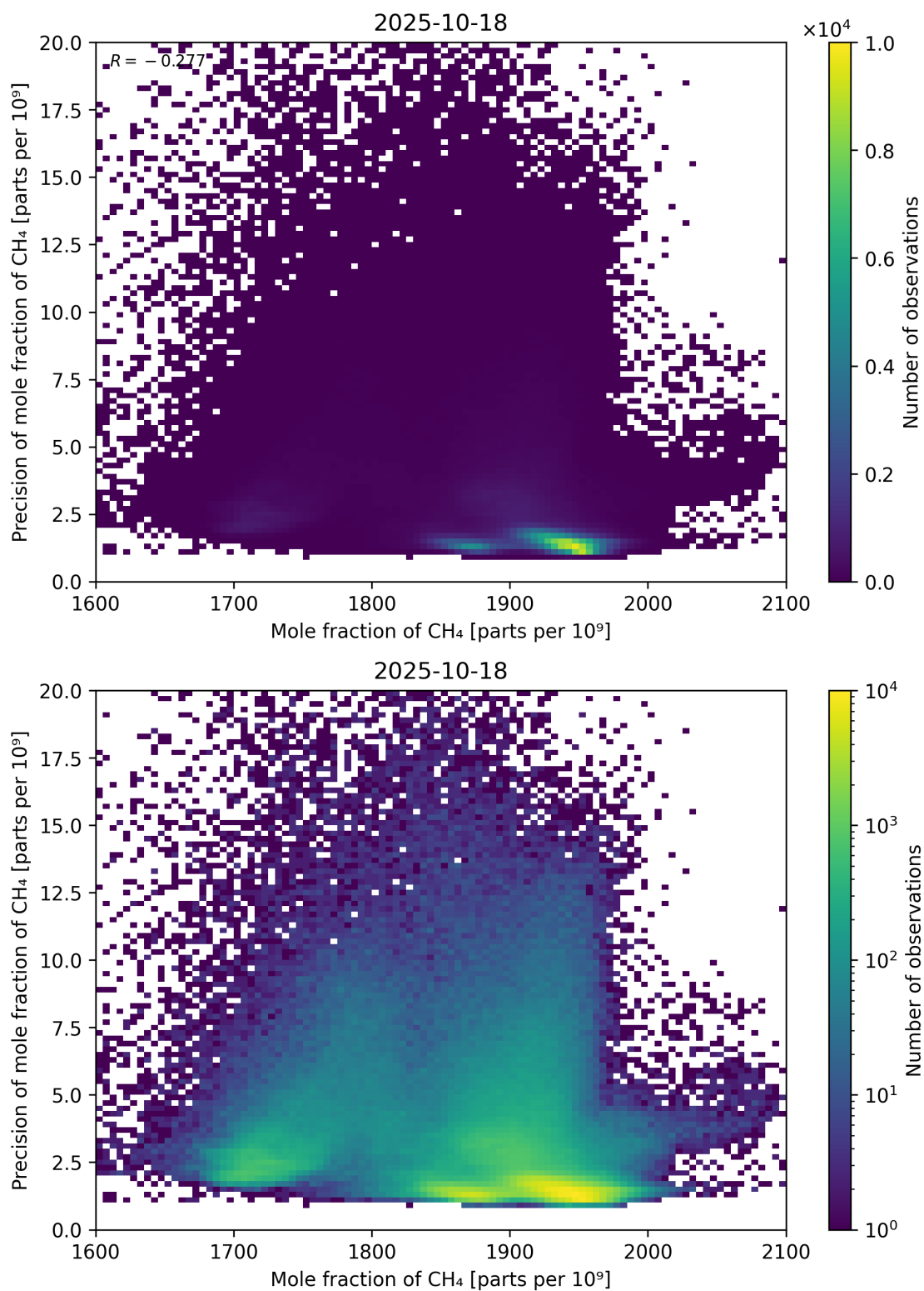
Figure 75: Scatter density plot of “Mole fraction of CH 4 ” against “Precision of mole fraction of CH 4 ” for 2025-10-17 to 2025-10-19.
