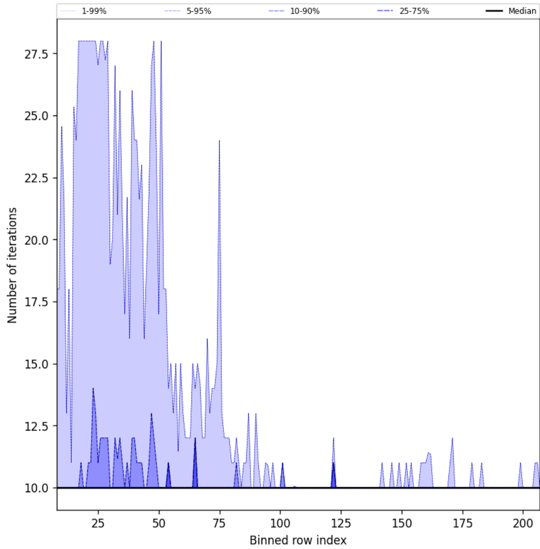
Figure 42: Along track statistics of “Number of iterations” for 2025-10-17 to 2025-10-19
