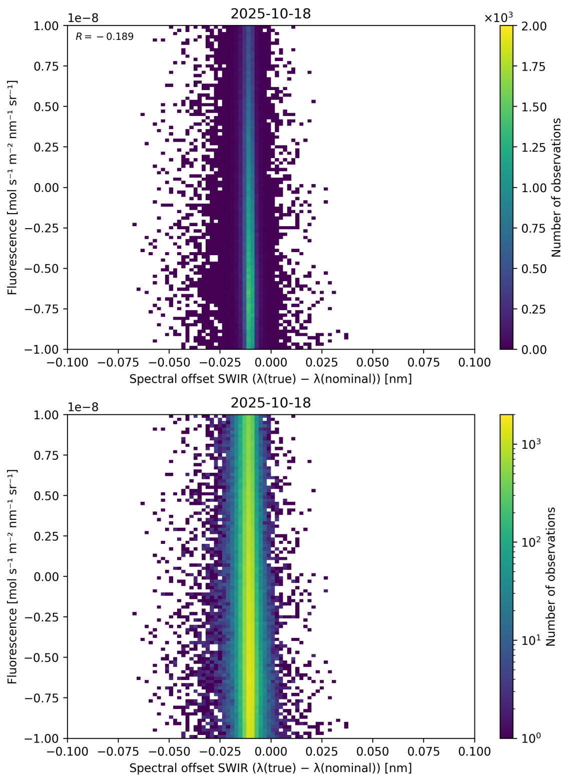
Figure 120: Scatter density plot of “Spectral offset SWIR ( \lambda_{\text{true}} - \lambda_{\text{nominal}} )” against “Fluorescence” for 2025-10-17 to 2025-10-19.
