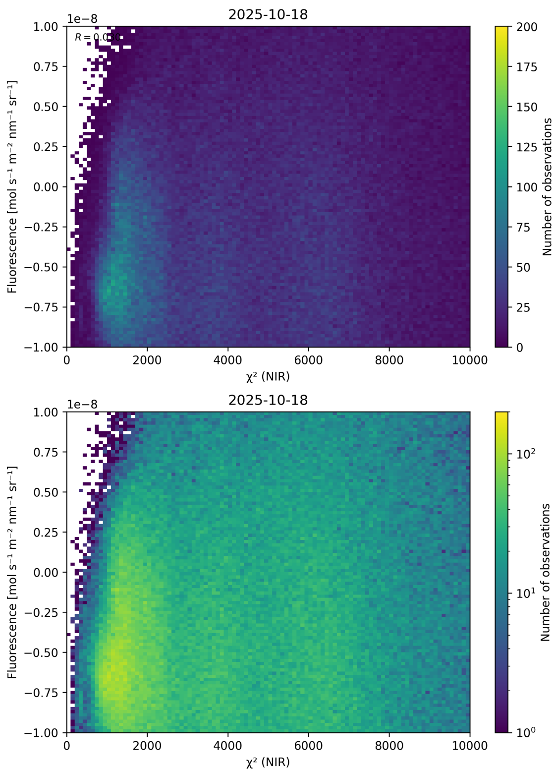
Figure 45: Scatter density plot of “ \chi^2 (NIR)” against “Fluorescence” for 2025-10-17 to 2025-10-19.
