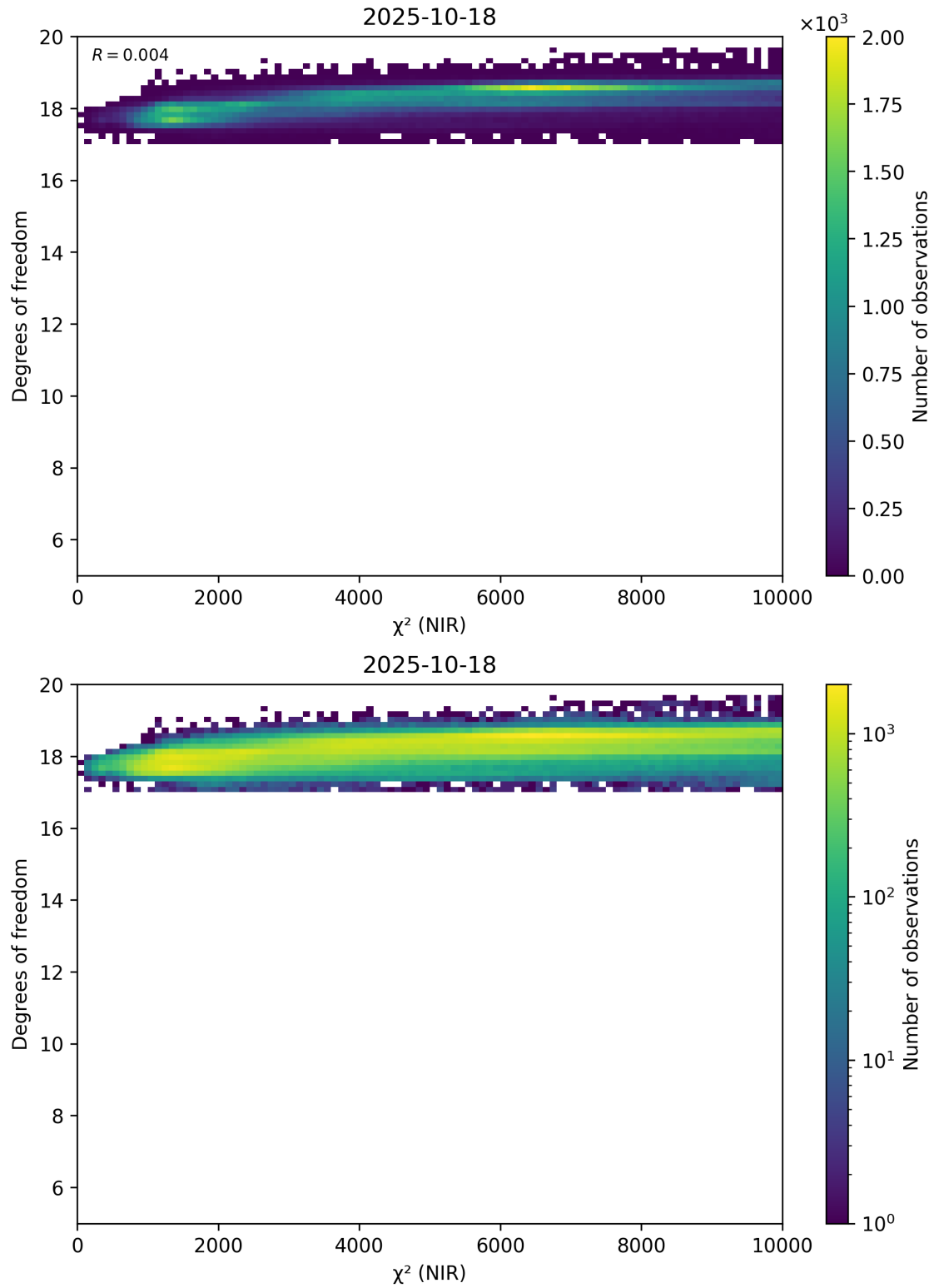
Figure 44: Scatter density plot of “ \chi^2 (NIR)” against “Degrees of freedom” for 2025-10-17 to 2025-10-19.
