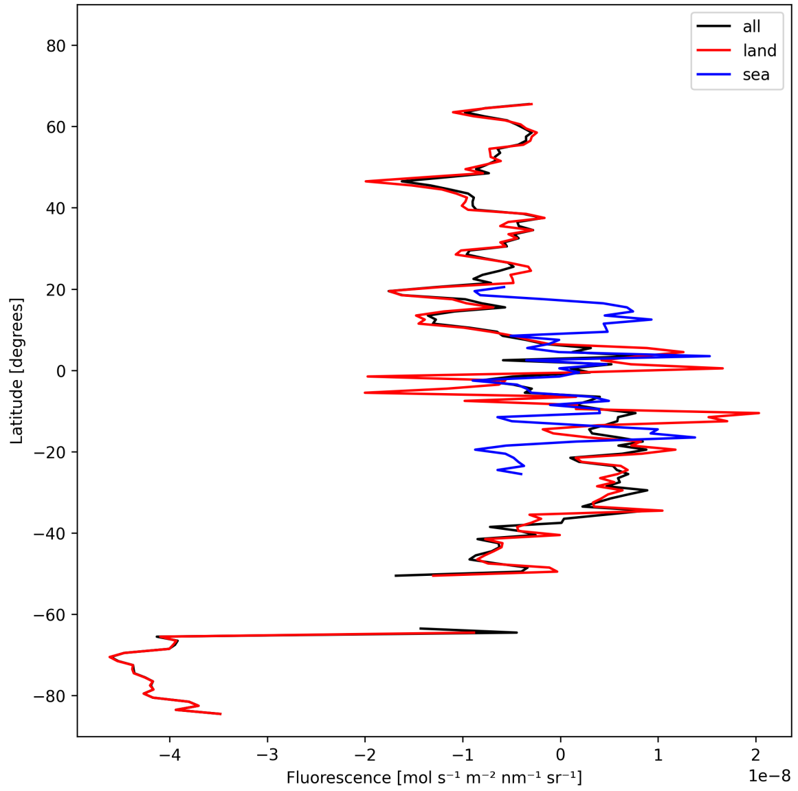
Figure 21: Zonal average of “Fluorescence” for 2025-10-17 to 2025-10-19.
