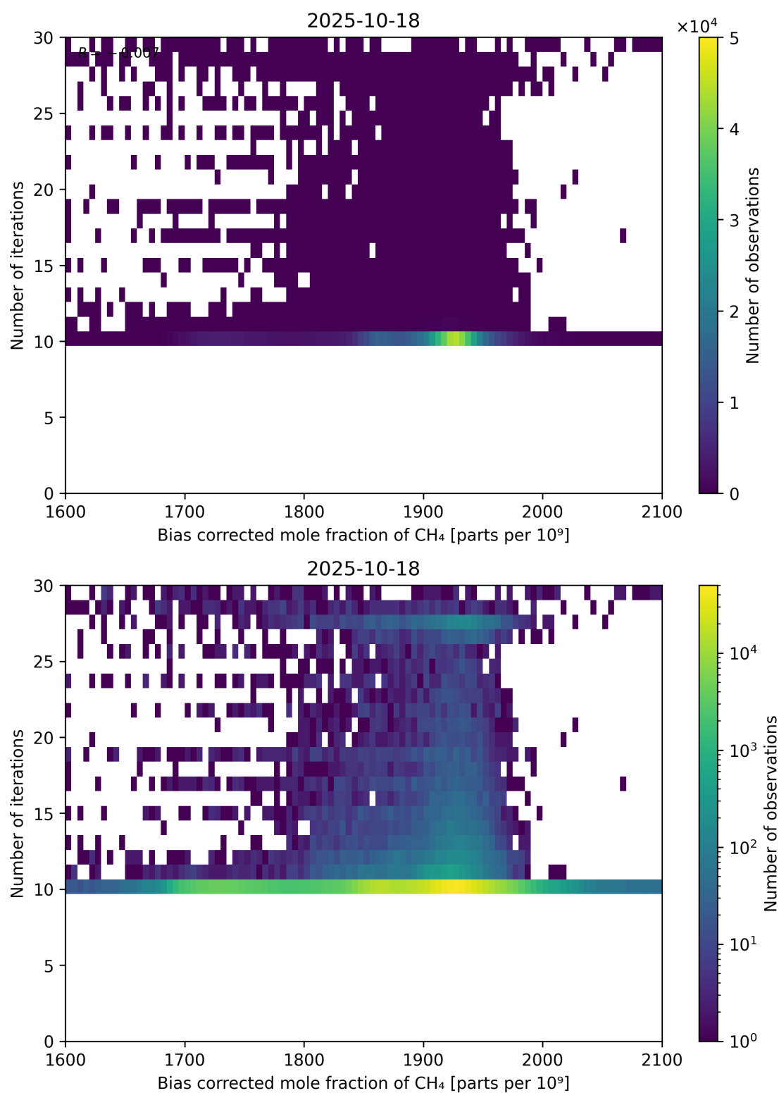
Figure 67: Scatter density plot of “Bias corrected mole fraction of \text{CH}_4 ” against “Number of iterations” for 2025-10-17 to 2025-10-19.
