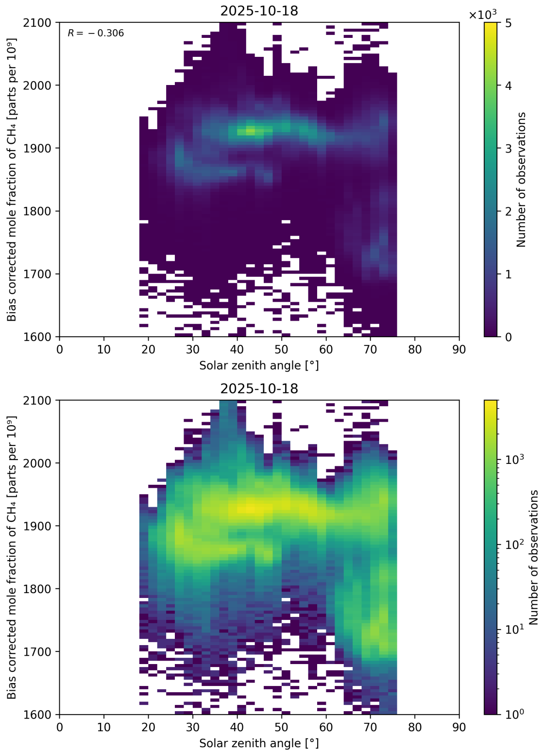
Figure 100: Scatter density plot of “Solar zenith angle” against “Bias corrected mole fraction of CH 4 ” for 2025-10-17 to 2025-10-19.
