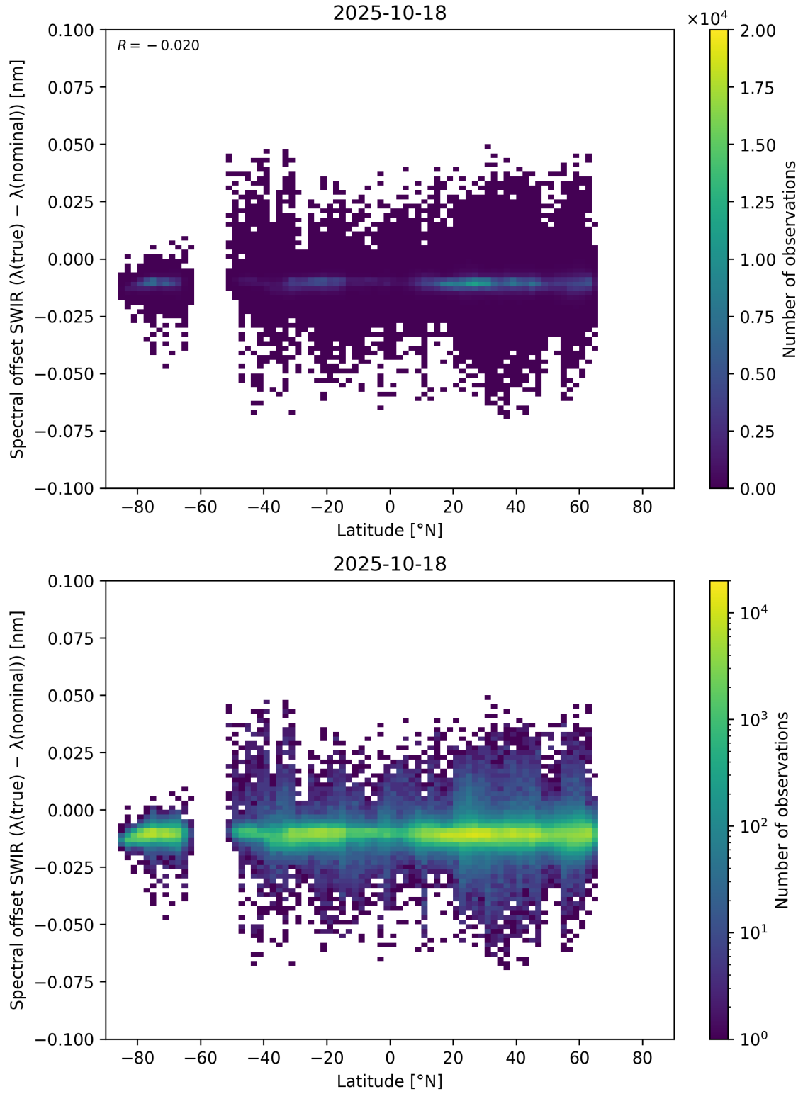
Figure 62: Scatter density plot of “Latitude” against “Spectral offset SWIR ( \lambda_{\text{true}} - \lambda_{\text{nominal}} )” for 2025-10-17 to 2025-10-19.
