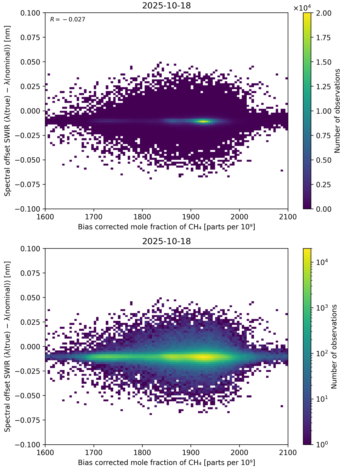
Figure 69: Scatter density plot of “Bias corrected mole fraction of \text{CH}_4 ” against “Spectral offset SWIR ( \lambda_{\text{true}} - \lambda_{\text{nominal}} )” for 2025-10-17 to 2025-10-19.
