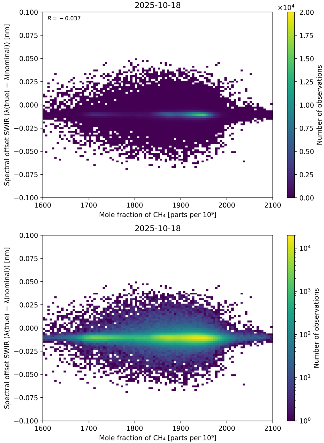
Figure 86: Scatter density plot of “Mole fraction of CH 4 ” against “Spectral offset SWIR ( \lambda_{\text{true}} - \lambda_{\text{nominal}} )” for 2025-10-17 to 2025-10-19.
