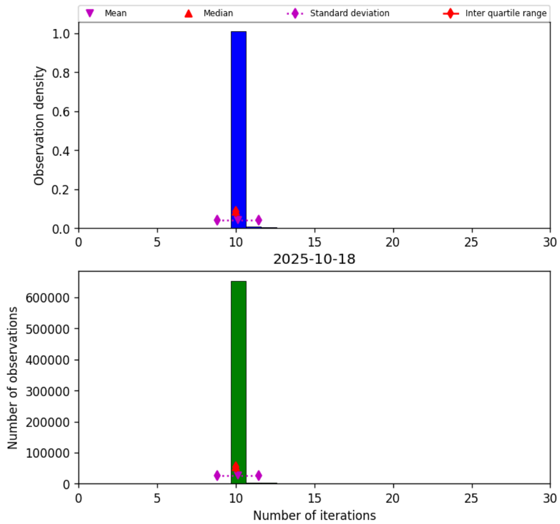
Figure 31: Histogram of “Number of iterations” for 2025-10-17 to 2025-10-19
