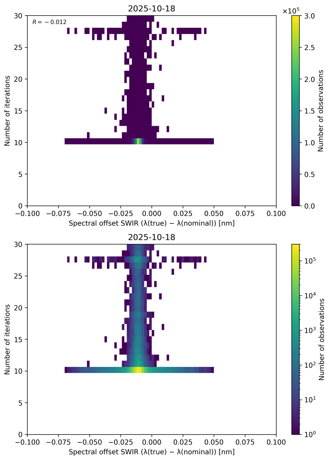
Figure 121: Scatter density plot of “Spectral offset SWIR ( \lambda_{\text{true}} - \lambda_{\text{nominal}} )” against “Number of iterations” for 2025-10-17 to 2025-10-19.
