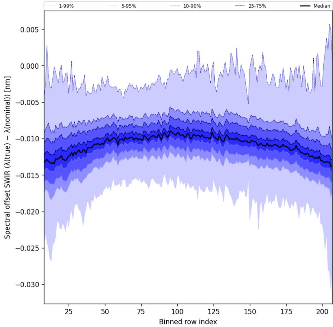
Figure 38: Along track statistics of “Spectral offset SWIR ( \lambda_{\text{true}} - \lambda_{\text{nominal}} )” for 2025-10-17 to 2025-10-19
