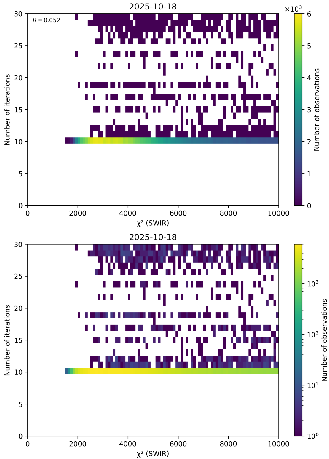
Figure 50: Scatter density plot of “ \chi^2 (SWIR)” against “Number of iterations” for 2025-10-17 to 2025-10-19.
