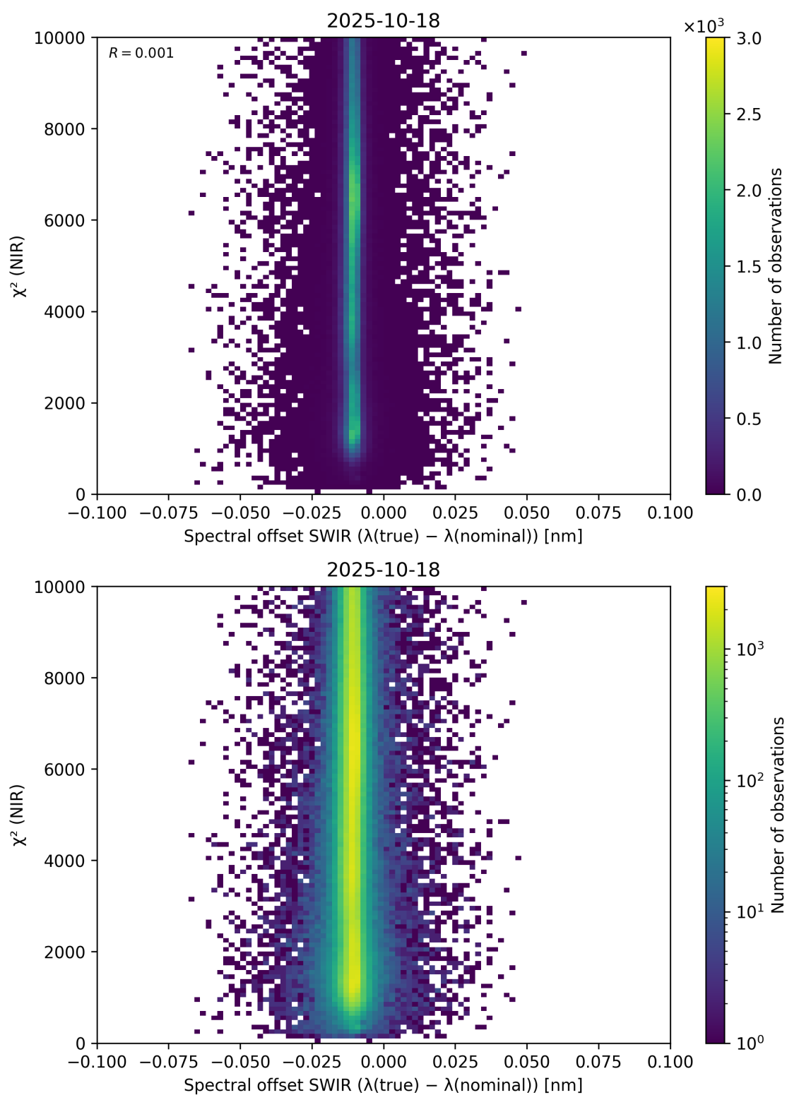
Figure 117: Scatter density plot of “Spectral offset SWIR ( \lambda_{\text{true}} - \lambda_{\text{nominal}} )” against “ \chi^2 (NIR)” for 2025-10-17 to 2025-10-19.
