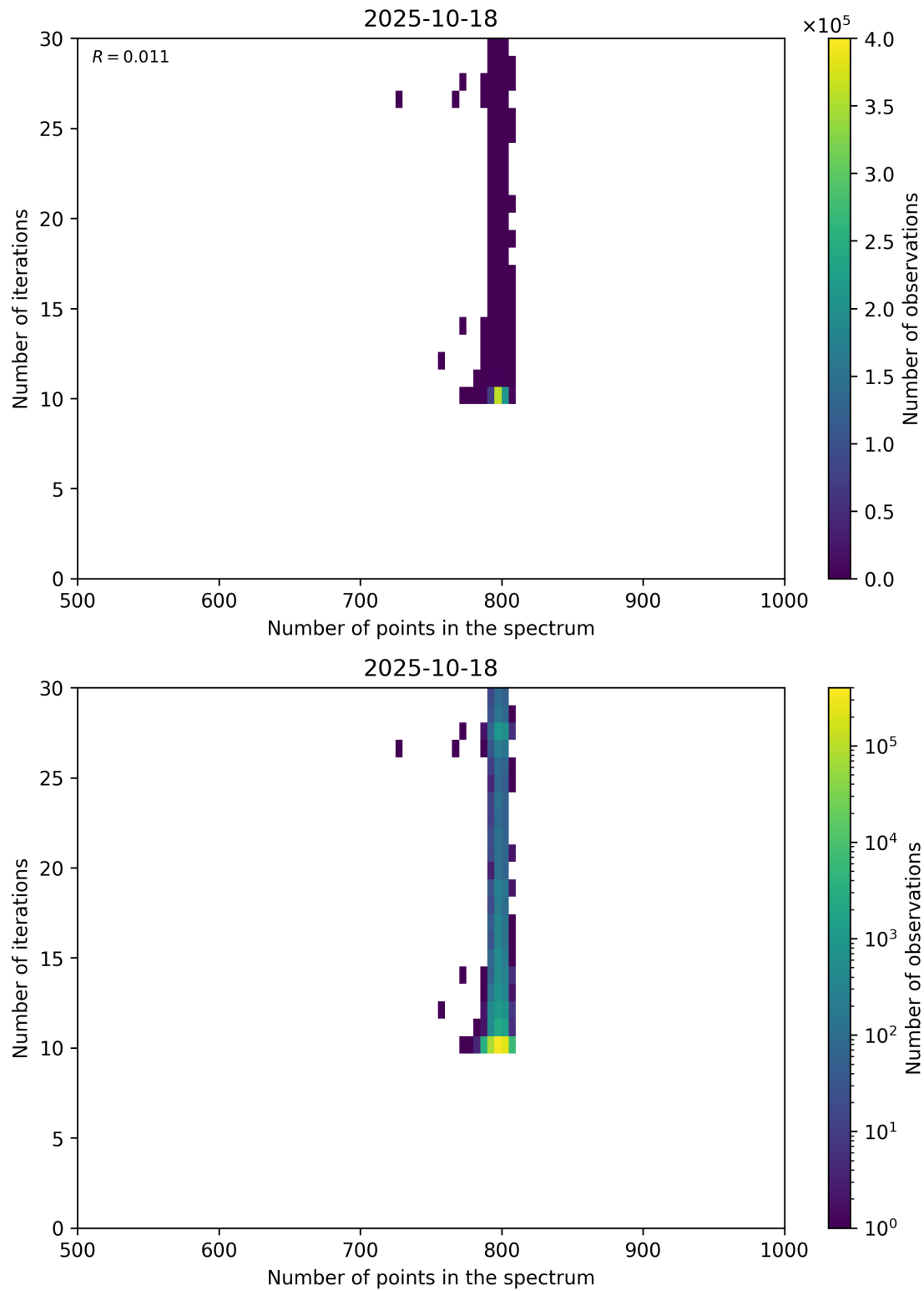
Figure 92: Scatter density plot of “Number of points in the spectrum” against “Number of iterations” for 2025-10-17 to 2025-10-19.
