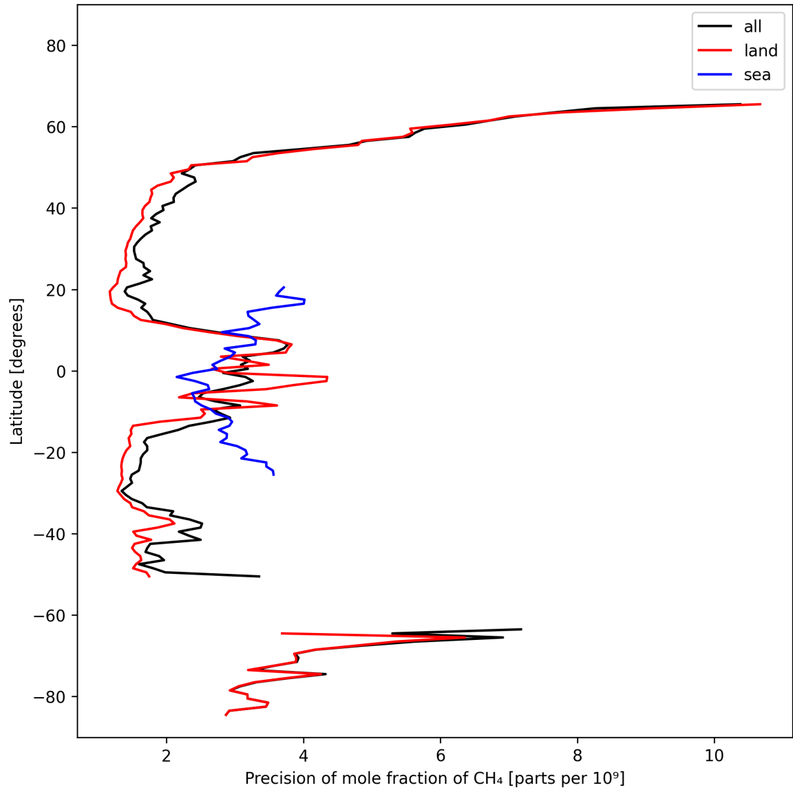
Figure 13: Zonal average of “Precision of mole fraction of CH 4 ” for 2025-10-17 to 2025-10-19.
