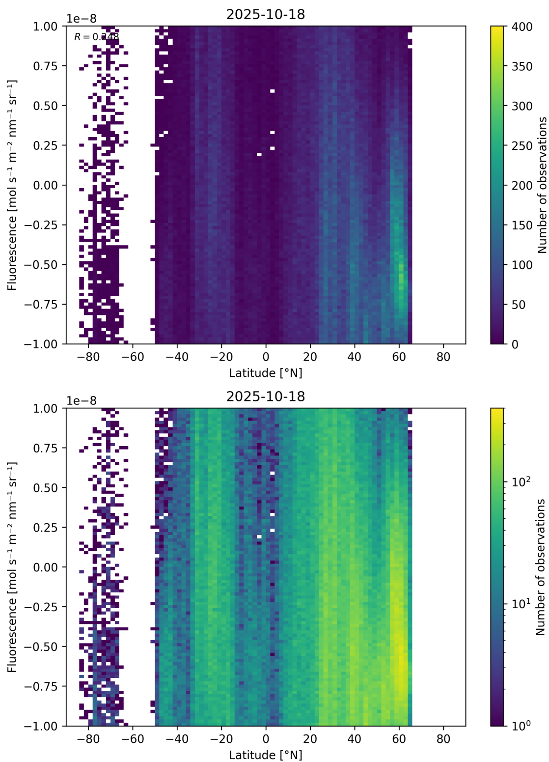
Figure 56: Scatter density plot of “Latitude” against “Fluorescence” for 2025-10-17 to 2025-10-19.
