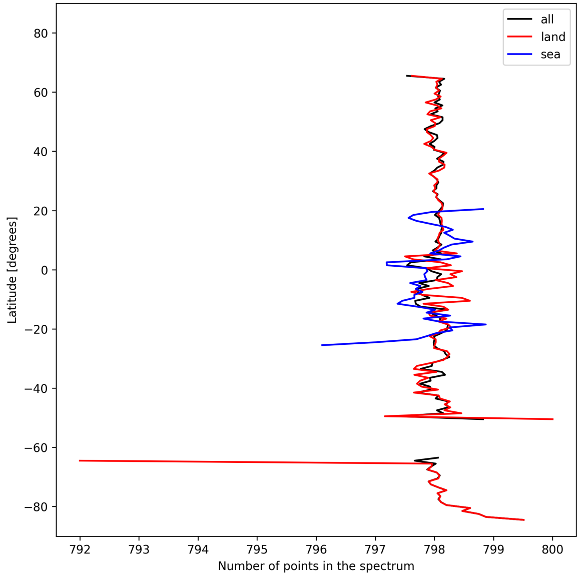
Figure 15: Zonal average of “Number of points in the spectrum” for 2025-10-17 to 2025-10-19.
