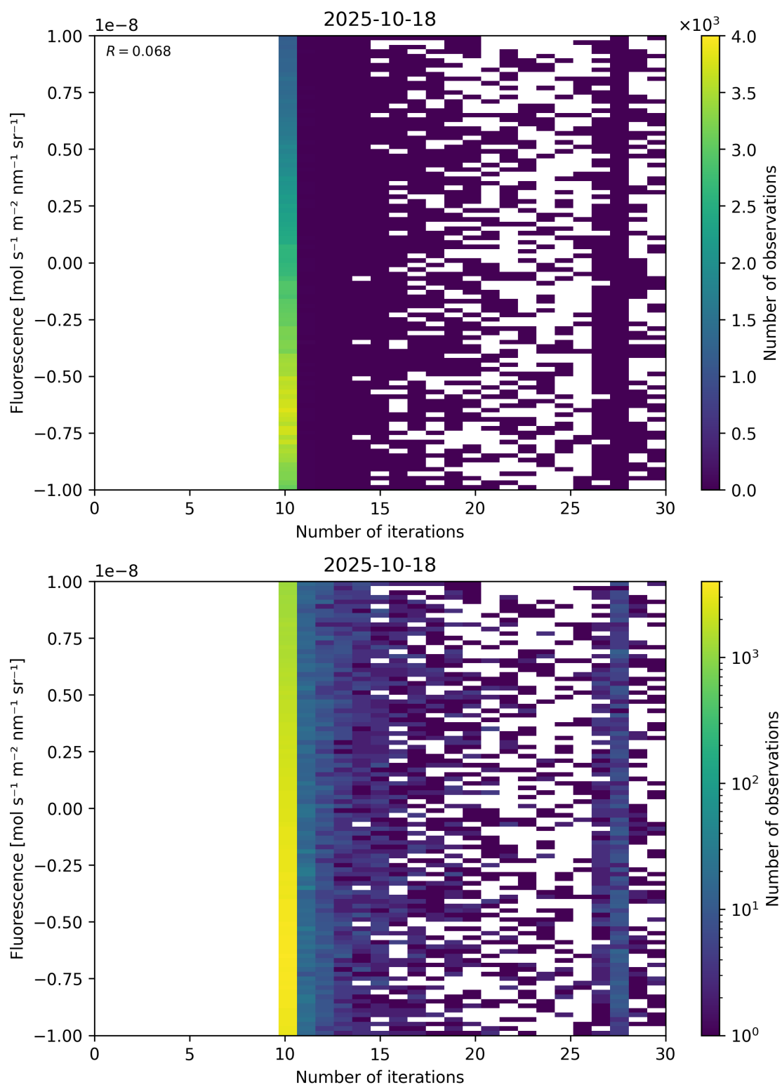
Figure 87: Scatter density plot of “Number of iterations” against “Fluorescence” for 2025-10-17 to 2025-10-19.
