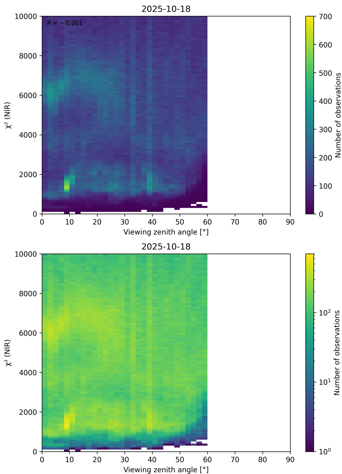
Figure 105: Scatter density plot of “Viewing zenith angle” against “ \chi^2 (NIR)” for 2025-10-17 to 2025-10-19.
