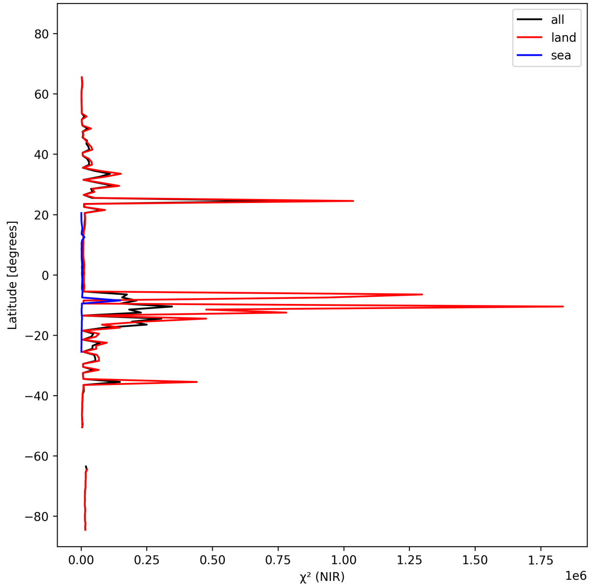
Figure 18: Zonal average of “ \chi^2 (NIR)” for 2025-10-17 to 2025-10-19.
