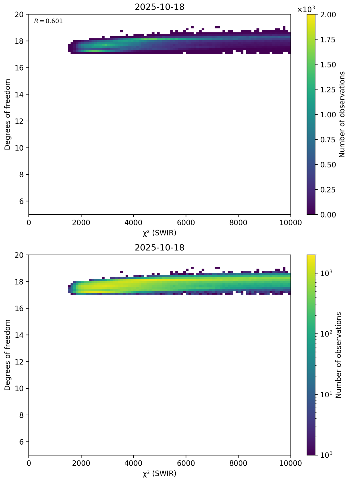
Figure 48: Scatter density plot of “ \chi^2 (SWIR)” against “Degrees of freedom” for 2025-10-17 to 2025-10-19.
