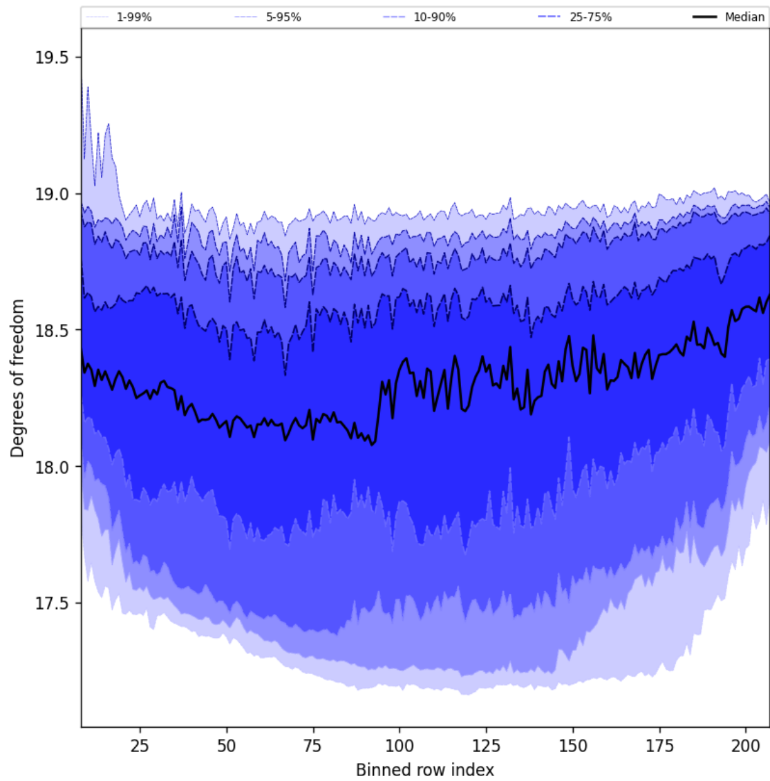
Figure 41: Along track statistics of “Degrees of freedom” for 2025-10-17 to 2025-10-19
