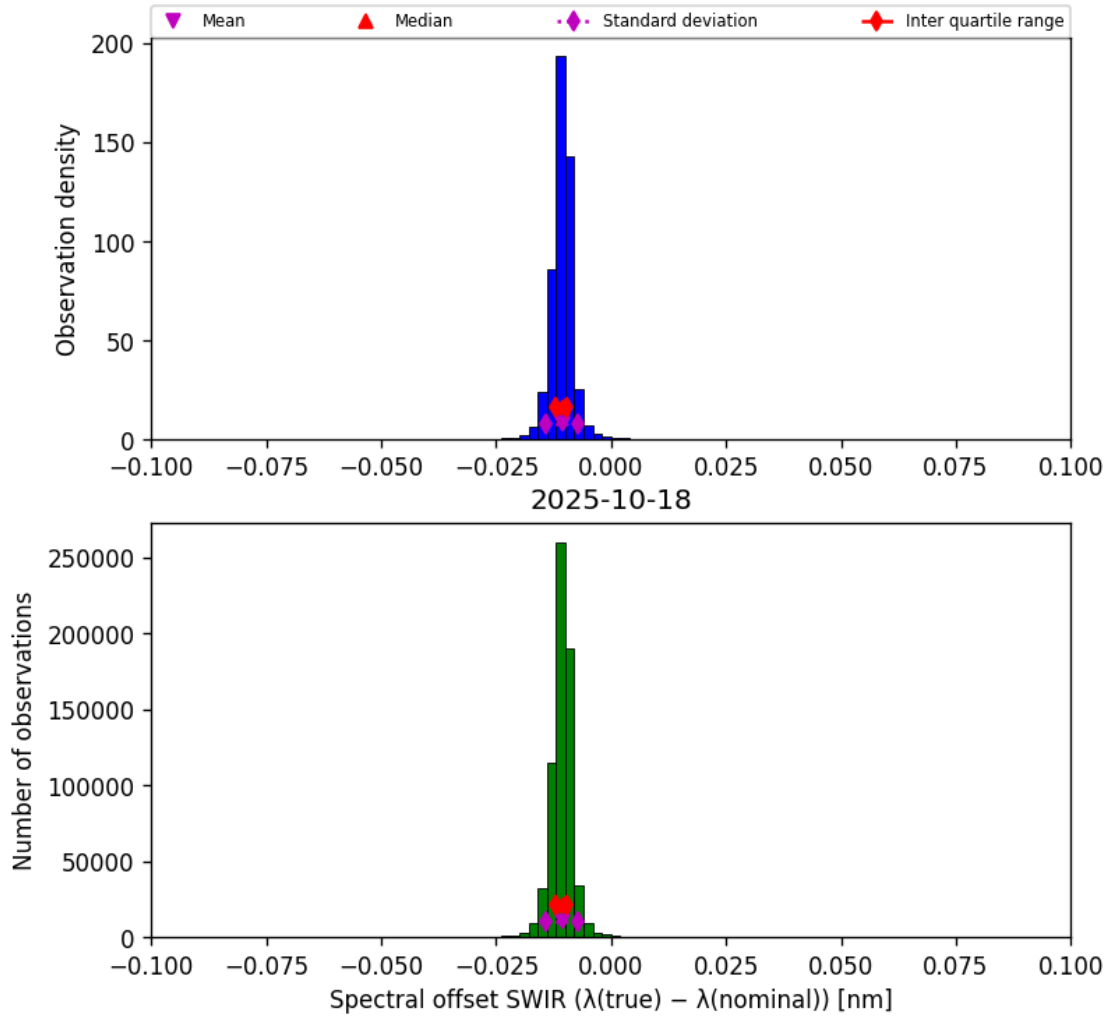
Figure 27: Histogram of “Spectral offset SWIR ( \lambda_{\text{true}} - \lambda_{\text{nominal}} )” for 2025-10-17 to 2025-10-19
