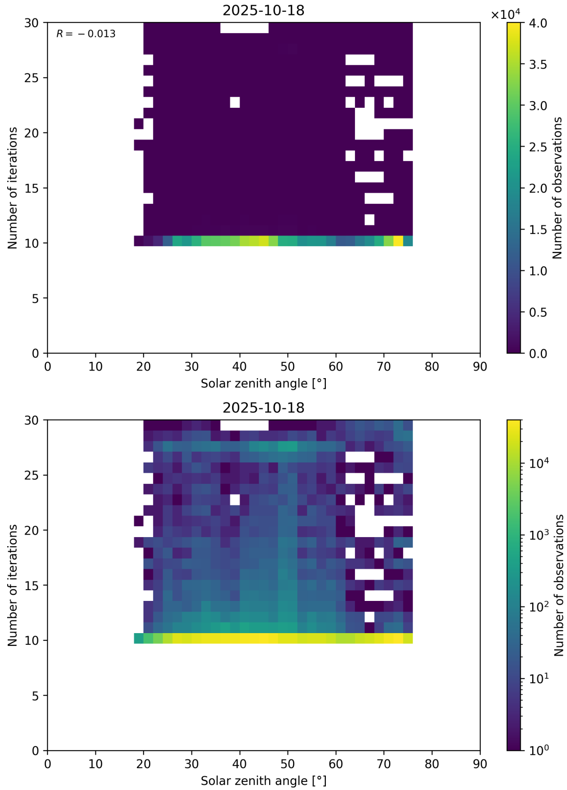
Figure 102: Scatter density plot of “Solar zenith angle” against “Number of iterations” for 2025-10-17 to 2025-10-19.
