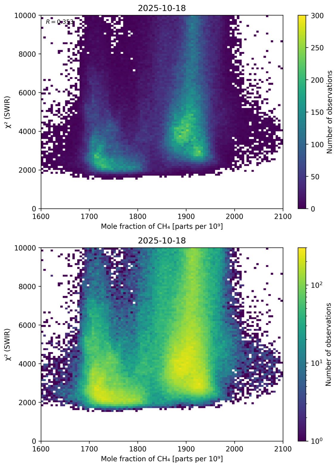
Figure 71: Scatter density plot of “Mole fraction of \text{CH}_4 ” against “ \chi^2 (SWIR)” for 2025-10-17 to 2025-10-19.
