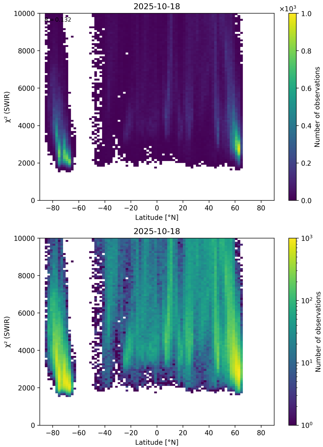
Figure 54: Scatter density plot of “Latitude” against “ \chi^2 (SWIR)” for 2025-10-17 to 2025-10-19.
