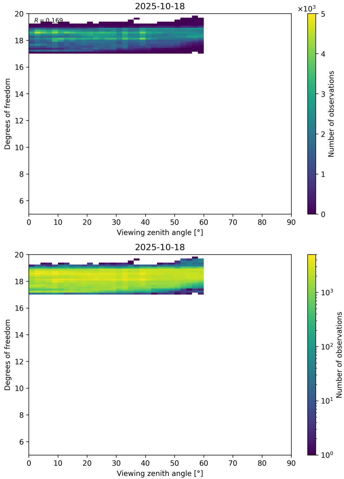
Figure 107: Scatter density plot of “Viewing zenith angle” against “Degrees of freedom” for 2025-10-17 to 2025-10-19.
