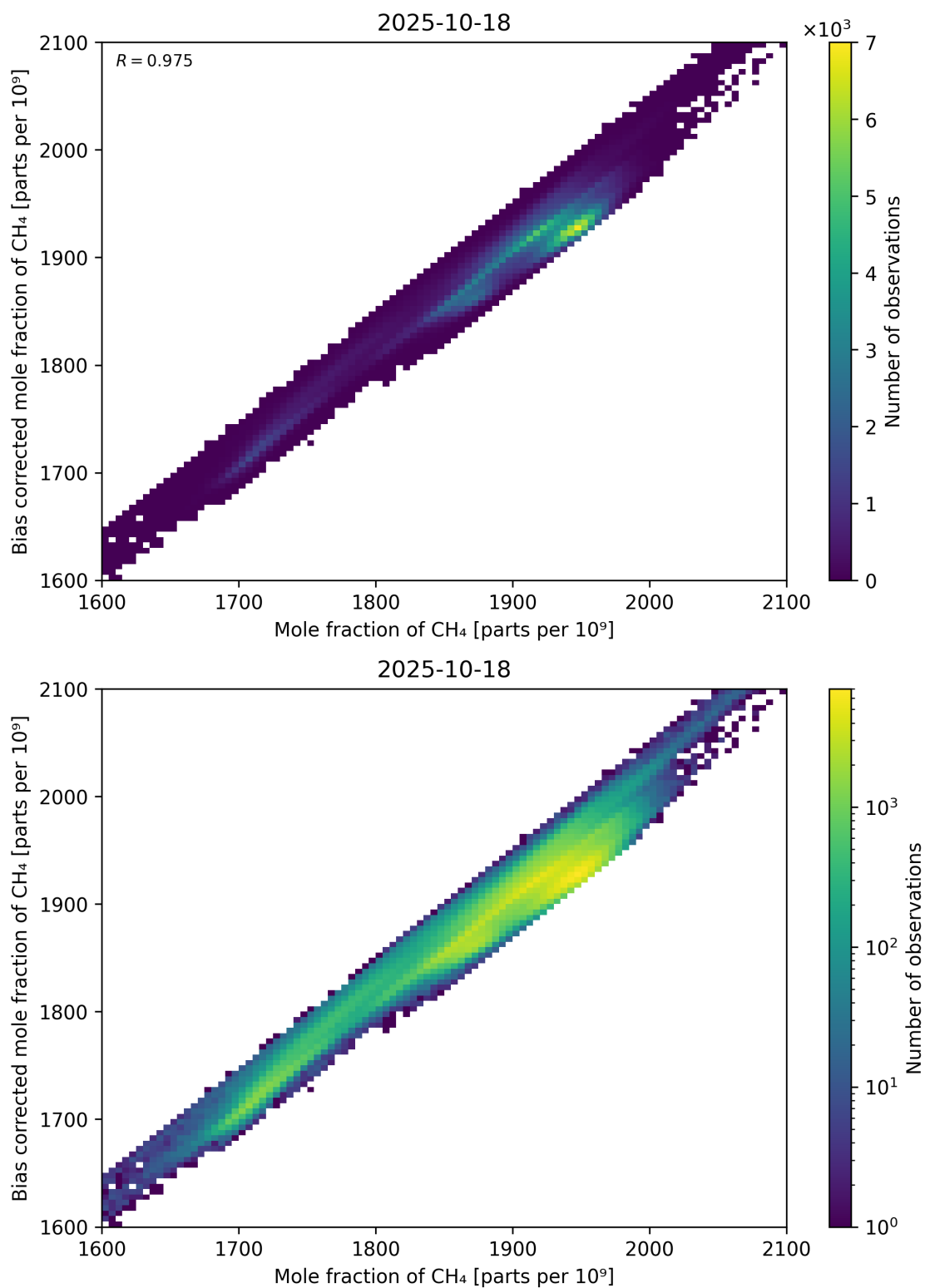
Figure 74: Scatter density plot of “Mole fraction of CH 4 ” against “Bias corrected mole fraction of CH 4 ” for 2025-10-17 to 2025-10-19.
