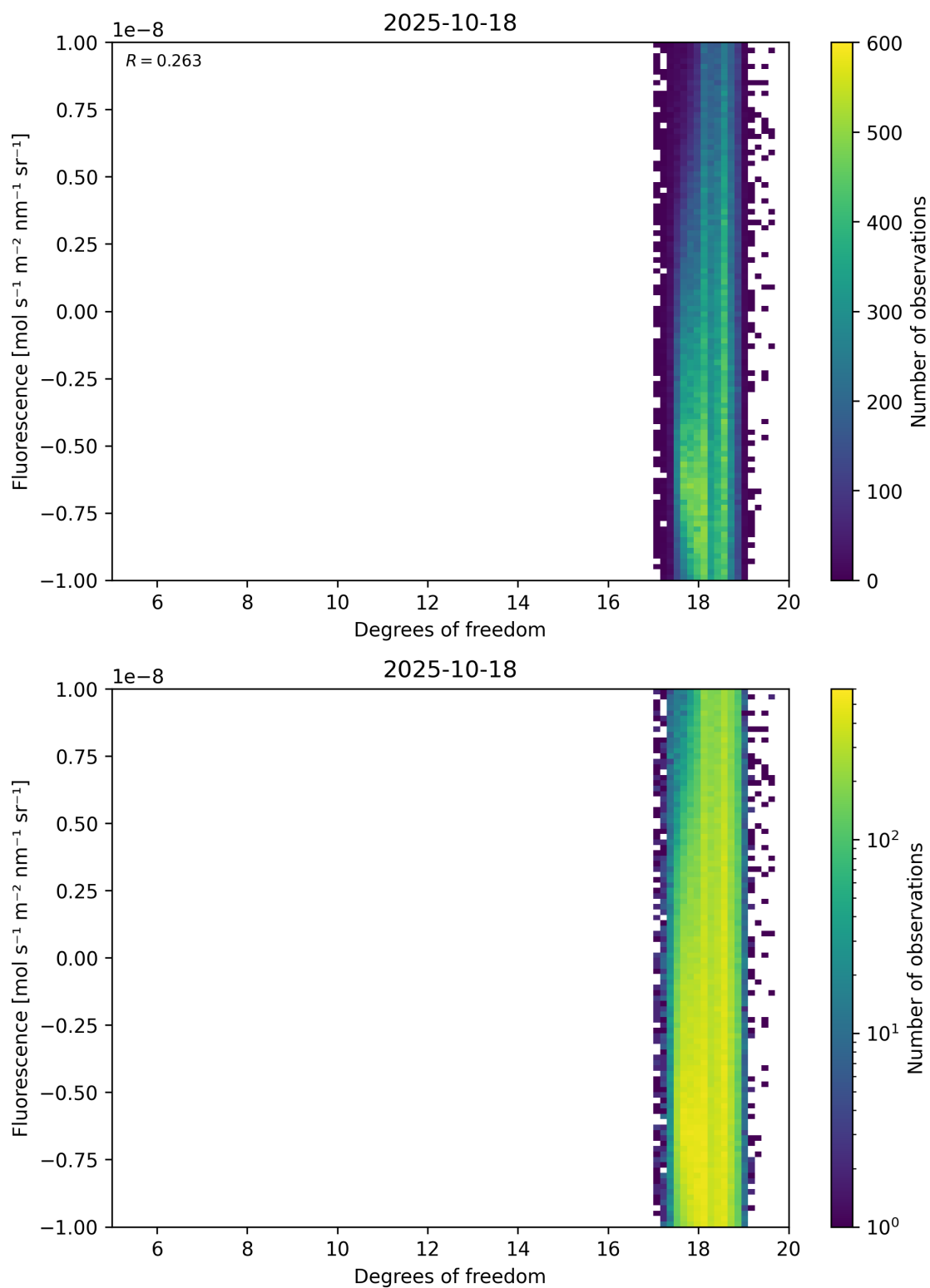
Figure 51: Scatter density plot of “Degrees of freedom” against “Fluorescence” for 2025-10-17 to 2025-10-19.
