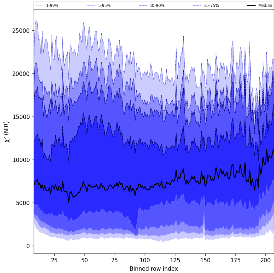
Figure 40: Along track statistics of “ \chi^2 (NIR)” for 2025-10-17 to 2025-10-19
