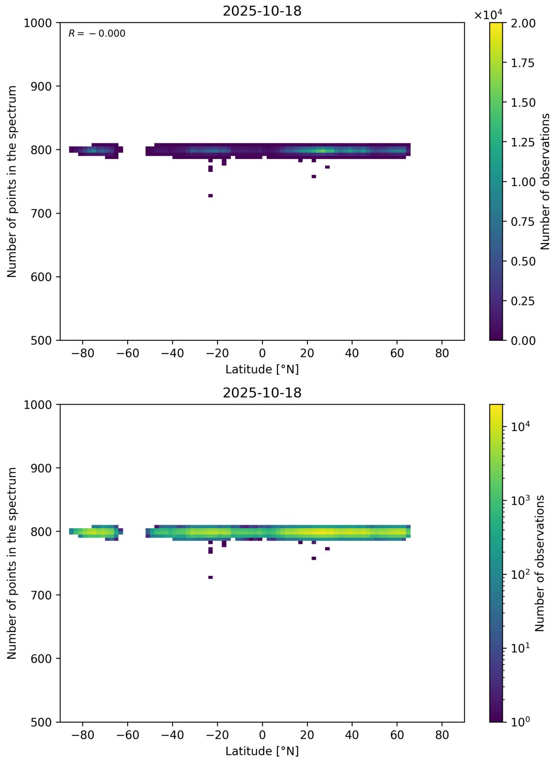
Figure 61: Scatter density plot of “Latitude” against “Number of points in the spectrum” for 2025-10-17 to 2025-10-19.
