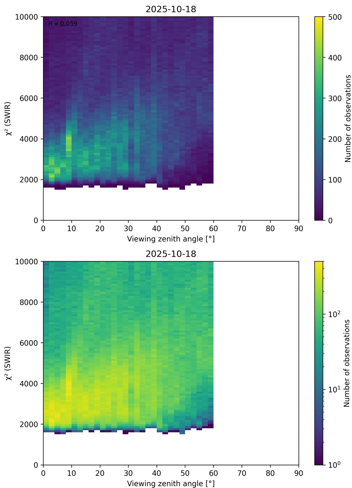
Figure 106: Scatter density plot of “Viewing zenith angle” against “ \chi^2 (SWIR)” for 2025-10-17 to 2025-10-19.
