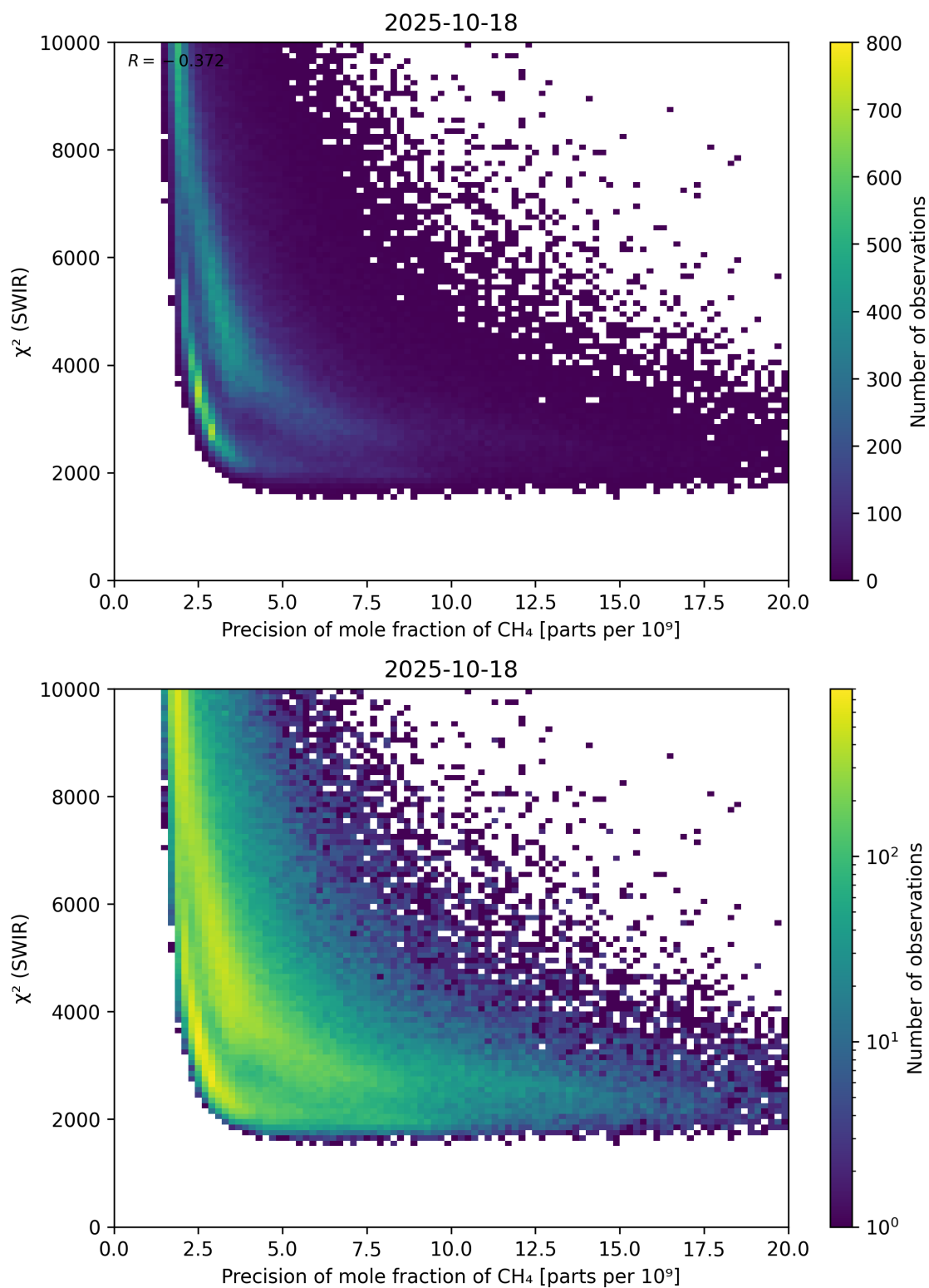
Figure 79: Scatter density plot of “Precision of mole fraction of CH 4 ” against “ \chi^2 (SWIR)” for 2025-10-17 to 2025-10-19.
