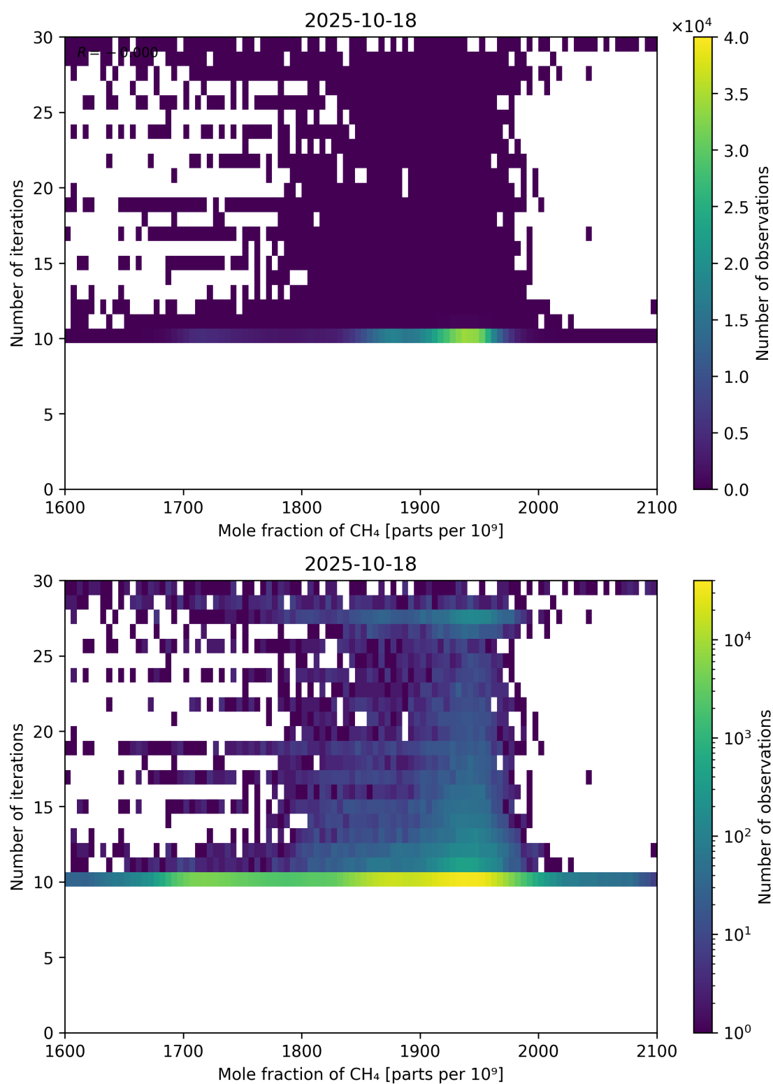
Figure 76: Scatter density plot of “Mole fraction of CH 4 ” against “Number of iterations” for 2025-10-17 to 2025-10-19.
