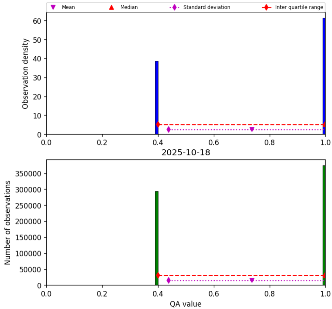
Figure 22: Histogram of “QA value” for 2025-10-17 to 2025-10-19
