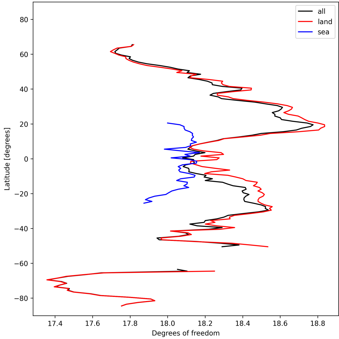
Figure 19: Zonal average of “Degrees of freedom” for 2025-10-17 to 2025-10-19.
