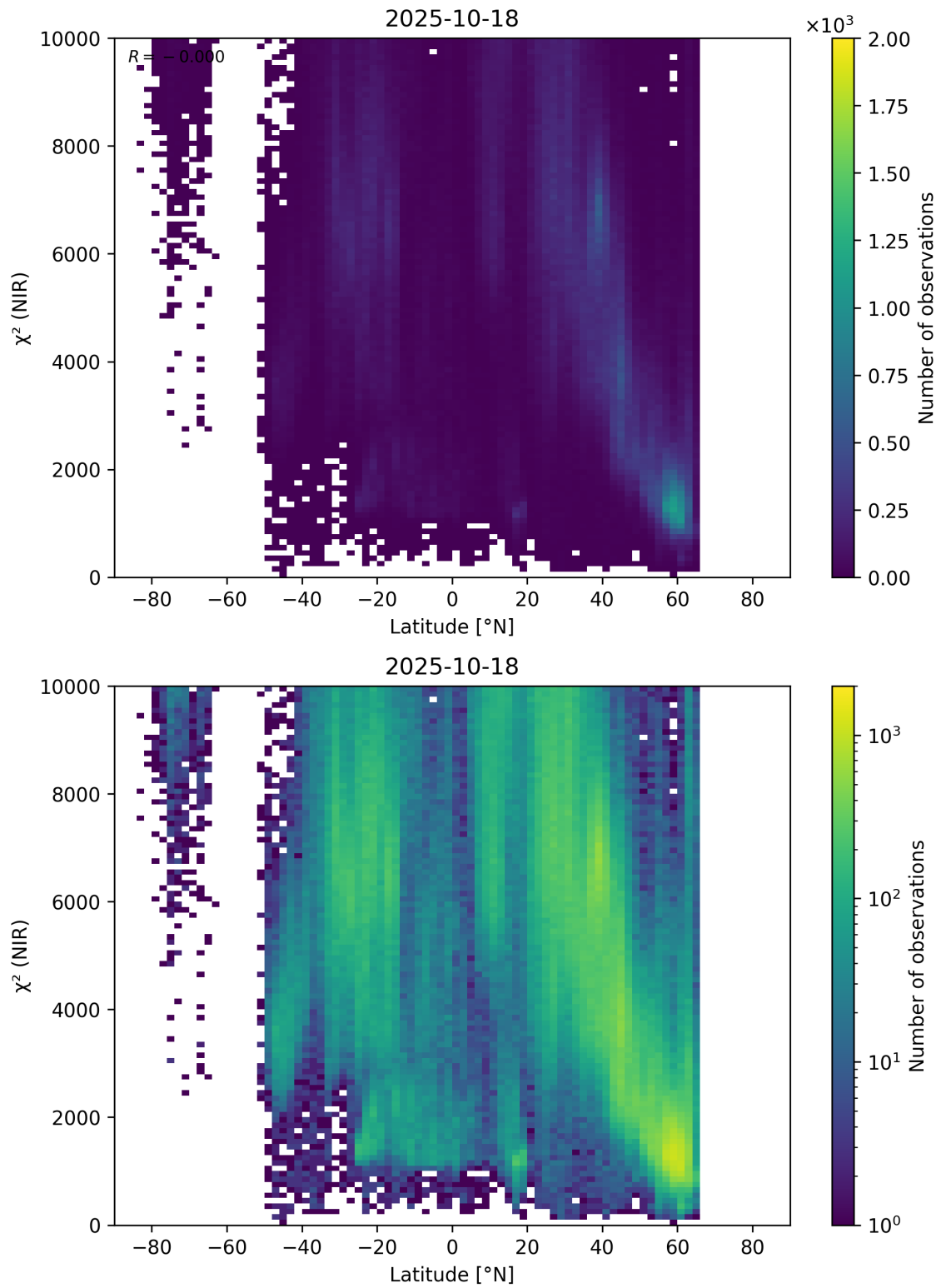
Figure 53: Scatter density plot of “Latitude” against “ \chi^2 (NIR)” for 2025-10-17 to 2025-10-19.
