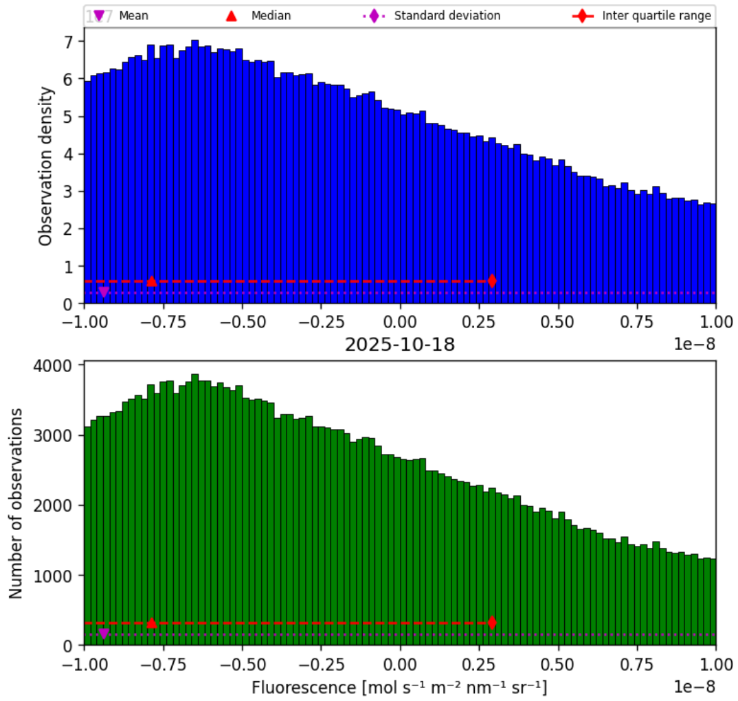
Figure 32: Histogram of “Fluorescence” for 2025-10-17 to 2025-10-19
