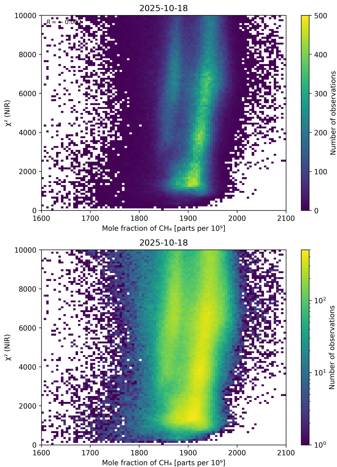
Figure 70: Scatter density plot of “Mole fraction of \text{CH}_4 ” against “ \chi^2 (NIR)” for 2025-10-17 to 2025-10-19.
