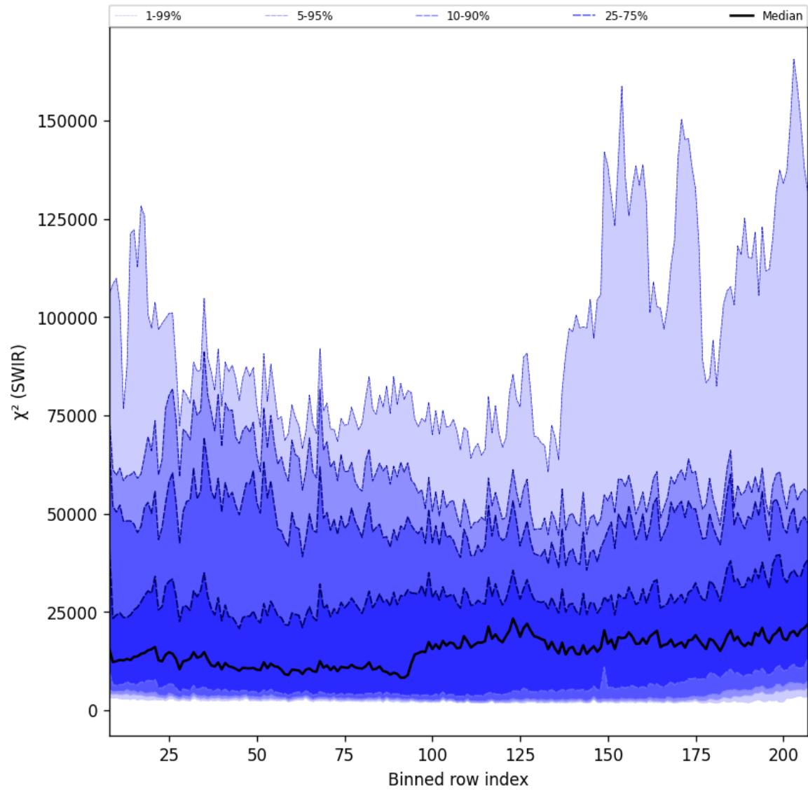
Figure 39: Along track statistics of “ \chi^2 (SWIR)” for 2025-10-17 to 2025-10-19
