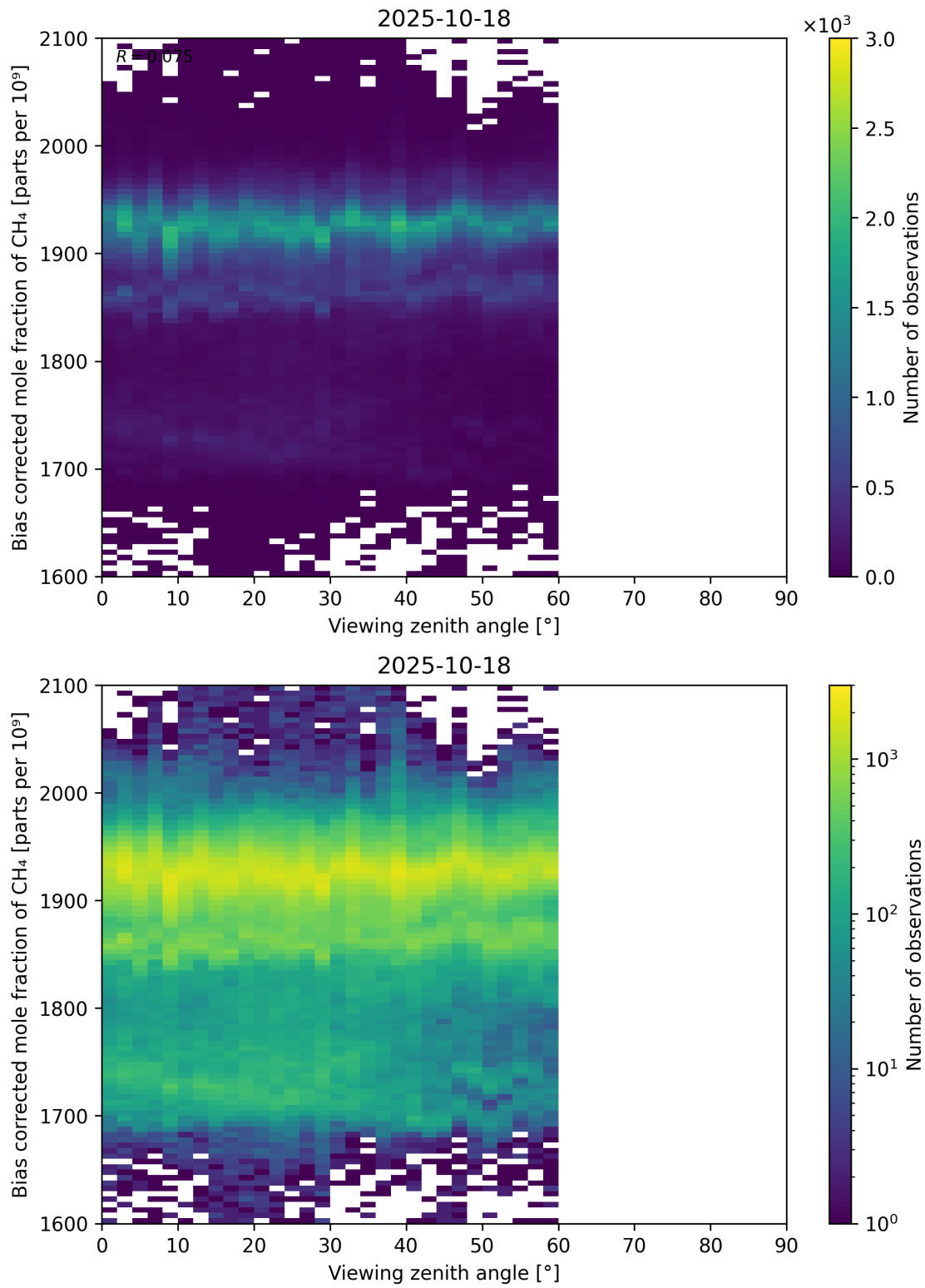
Figure 111: Scatter density plot of “Viewing zenith angle” against “Bias corrected mole fraction of CH 4 ” for 2025-10-17 to 2025-10-19.
