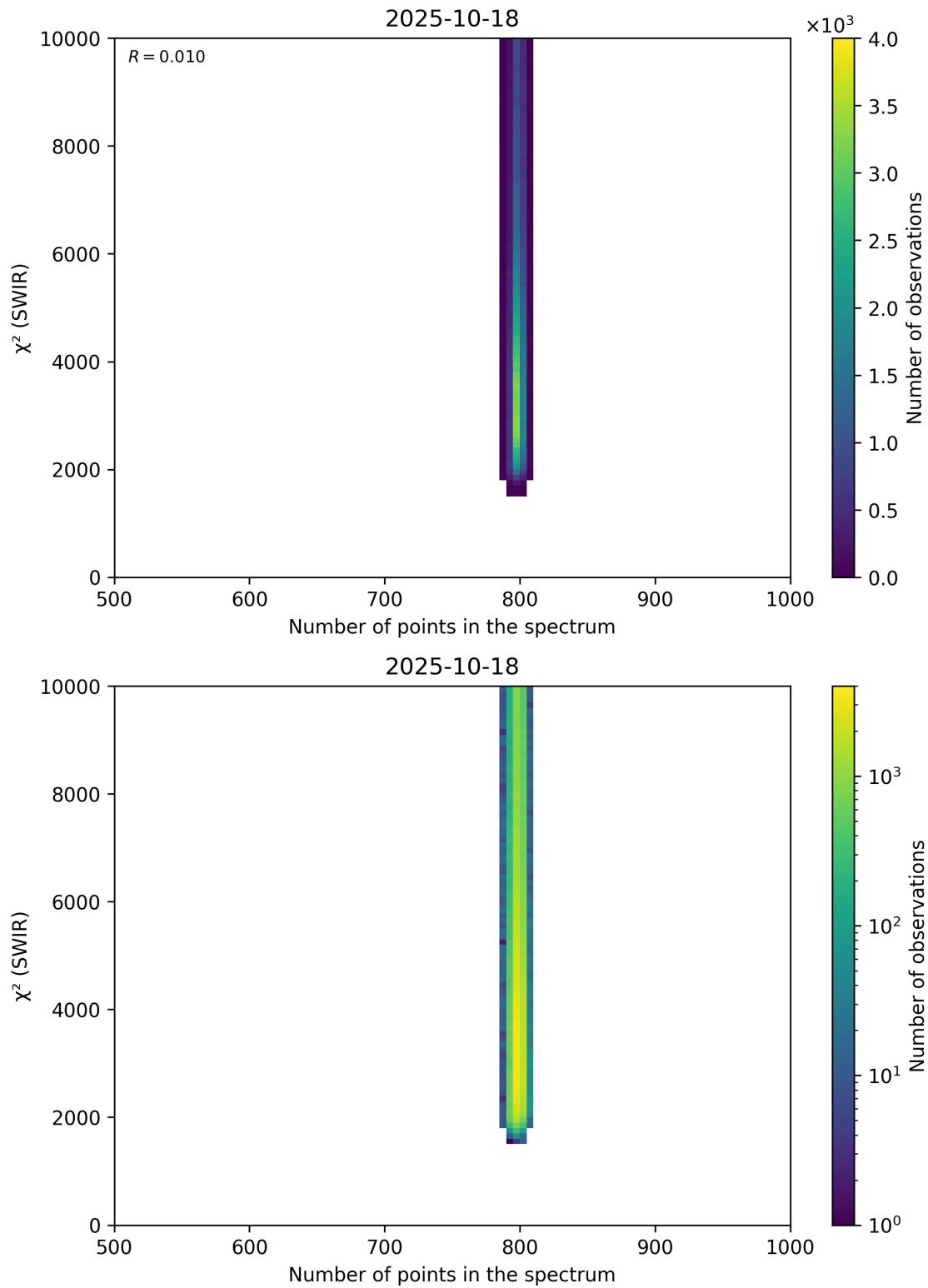
Figure 89: Scatter density plot of “Number of points in the spectrum” against “ \chi^2 (SWIR)” for 2025-10-17 to 2025-10-19.
