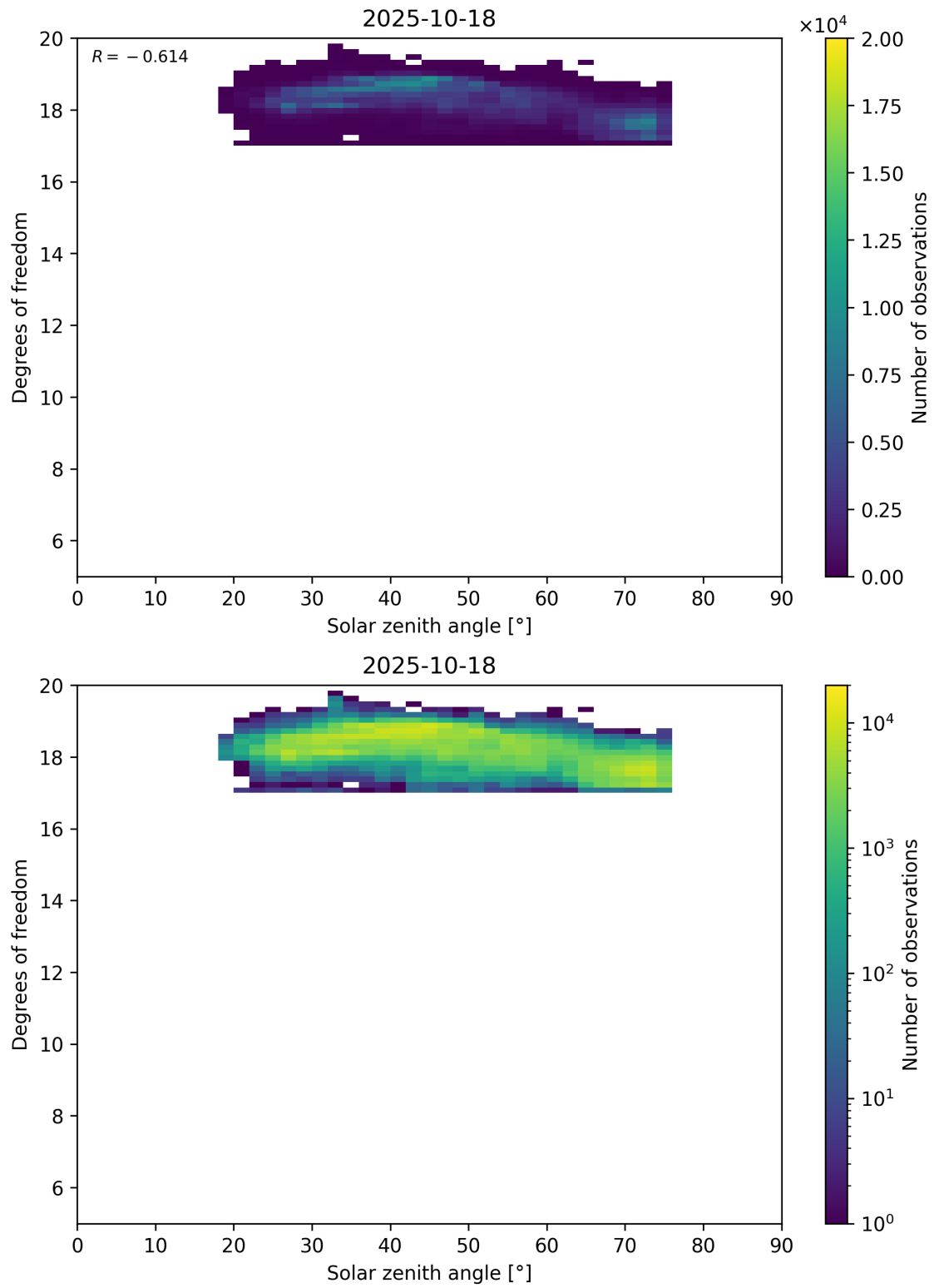
Figure 96: Scatter density plot of “Solar zenith angle” against “Degrees of freedom” for 2025-10-17 to 2025-10-19.
