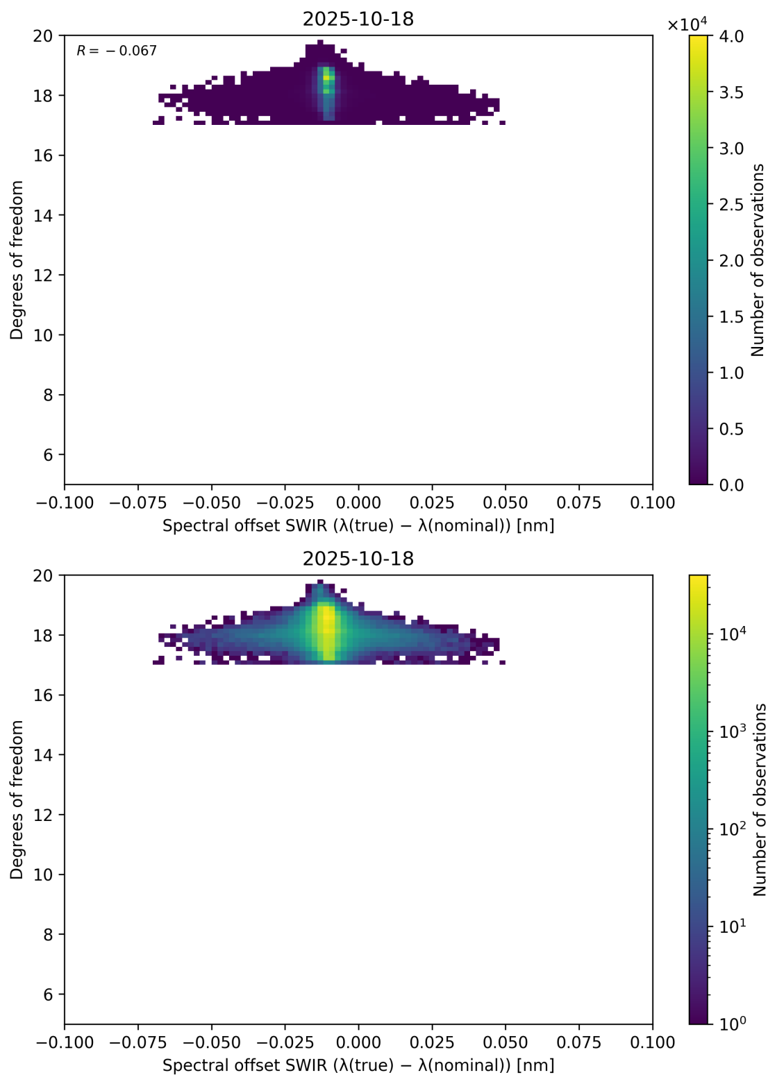
Figure 119: Scatter density plot of “Spectral offset SWIR ( \lambda_{\text{true}} - \lambda_{\text{nominal}} )” against “Degrees of freedom” for 2025-10-17 to 2025-10-19.
