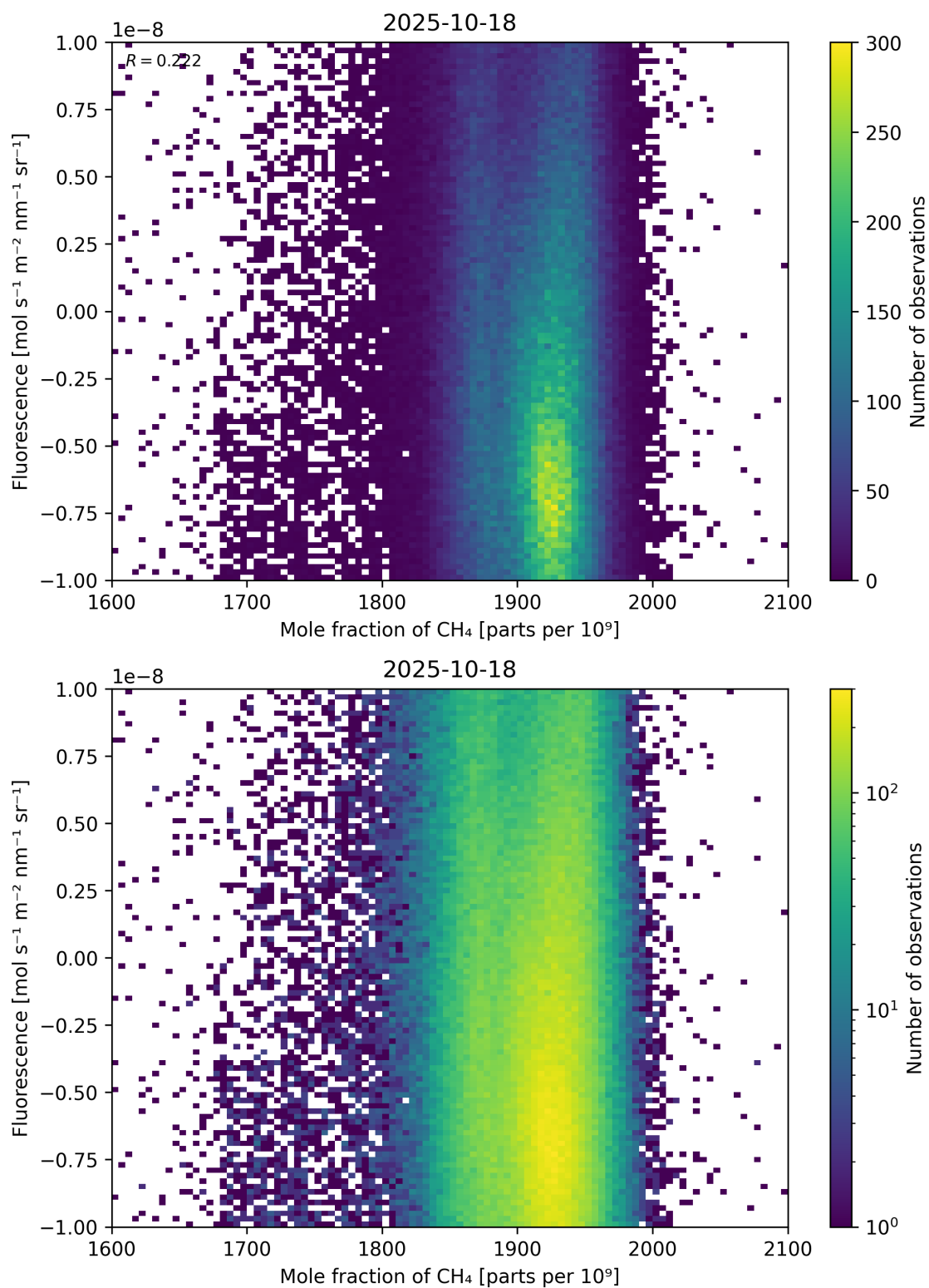
Figure 73: Scatter density plot of “Mole fraction of \text{CH}_4 ” against “Fluorescence” for 2025-10-17 to 2025-10-19.
