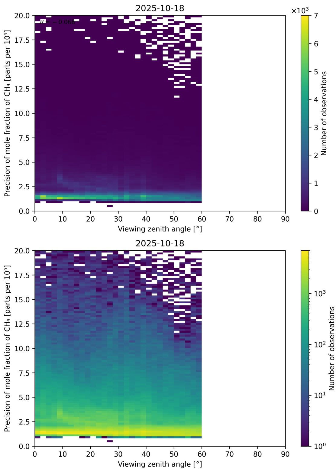
Figure 112: Scatter density plot of “Viewing zenith angle” against “Precision of mole fraction of CH 4 ” for 2025-10-17 to 2025-10-19.
