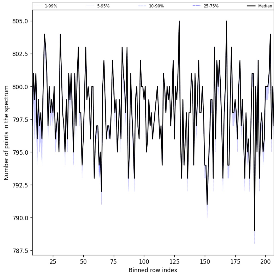
Figure 37: Along track statistics of “Number of points in the spectrum” for 2025-10-17 to 2025-10-19
