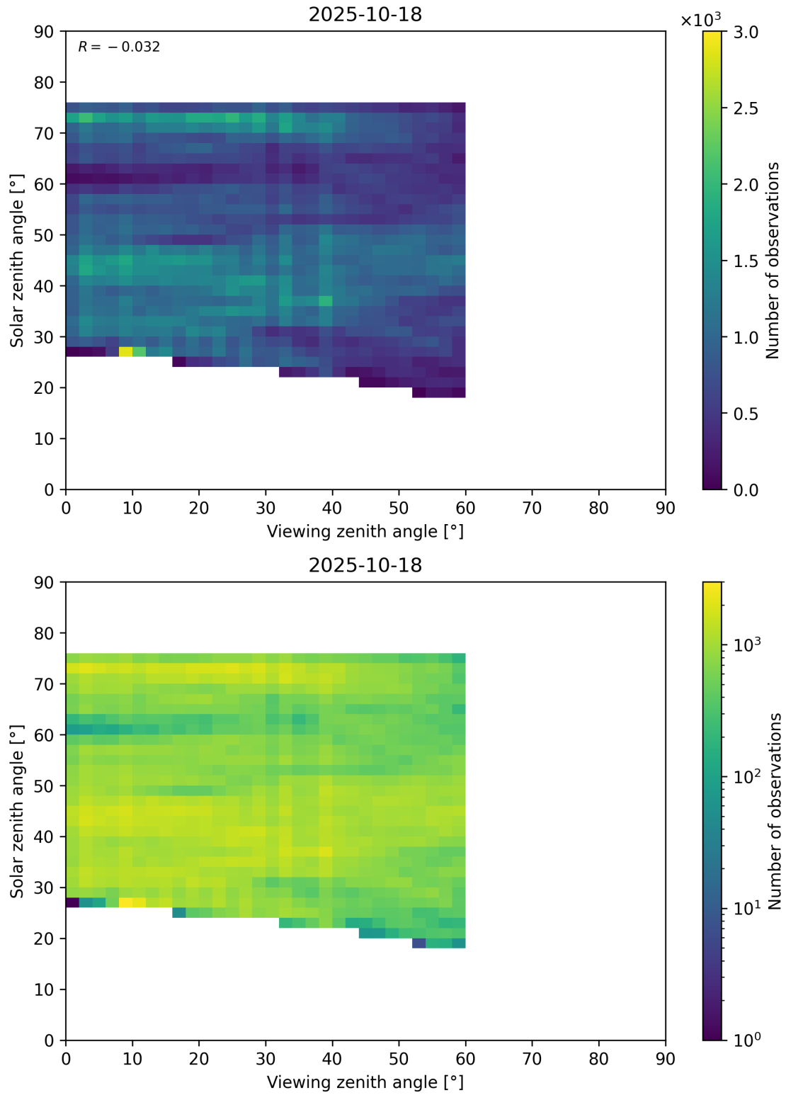
Figure 115: Scatter density plot of “Viewing zenith angle” against “Solar zenith angle” for 2025-10-17 to 2025-10-19.
