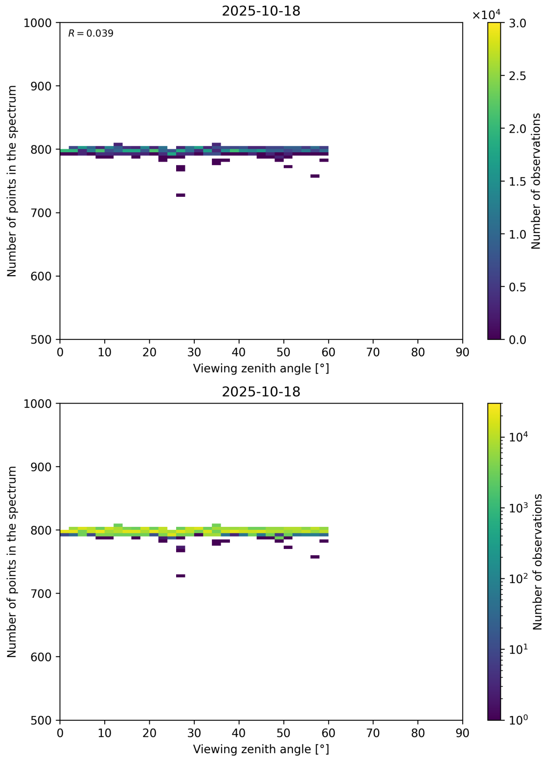
Figure 114: Scatter density plot of “Viewing zenith angle” against “Number of points in the spectrum” for 2025-10-17 to 2025-10-19.
