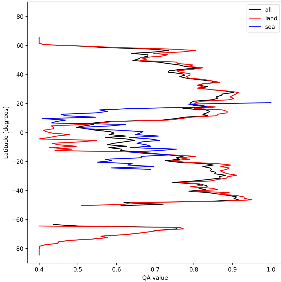
Figure 11: Zonal average of “QA value” for 2025-10-17 to 2025-10-19.
