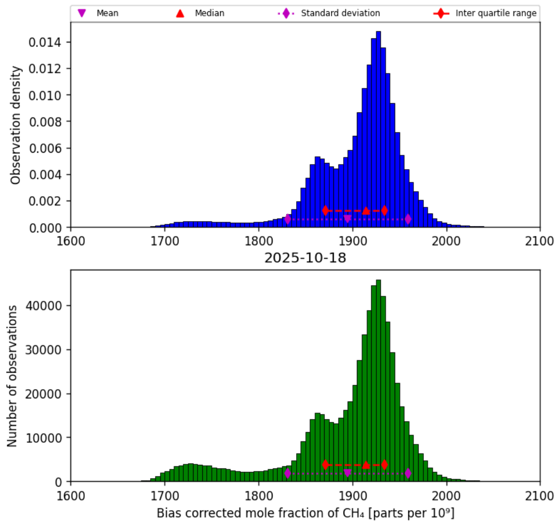
Figure 25: Histogram of “Bias corrected mole fraction of \text{CH}_4 ” for 2025-10-17 to 2025-10-19
