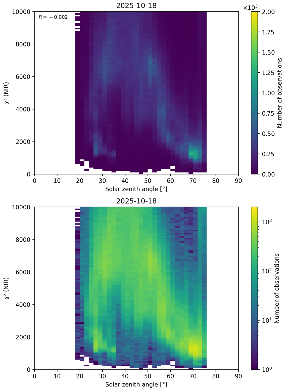
Figure 94: Scatter density plot of “Solar zenith angle” against “ \chi^2 (NIR)” for 2025-10-17 to 2025-10-19.
