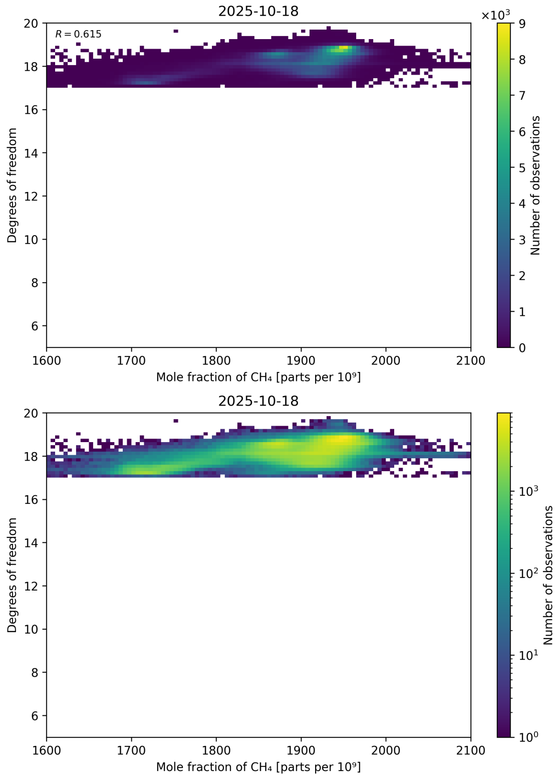
Figure 72: Scatter density plot of “Mole fraction of CH 4 ” against “Degrees of freedom” for 2025-10-17 to 2025-10-19.
