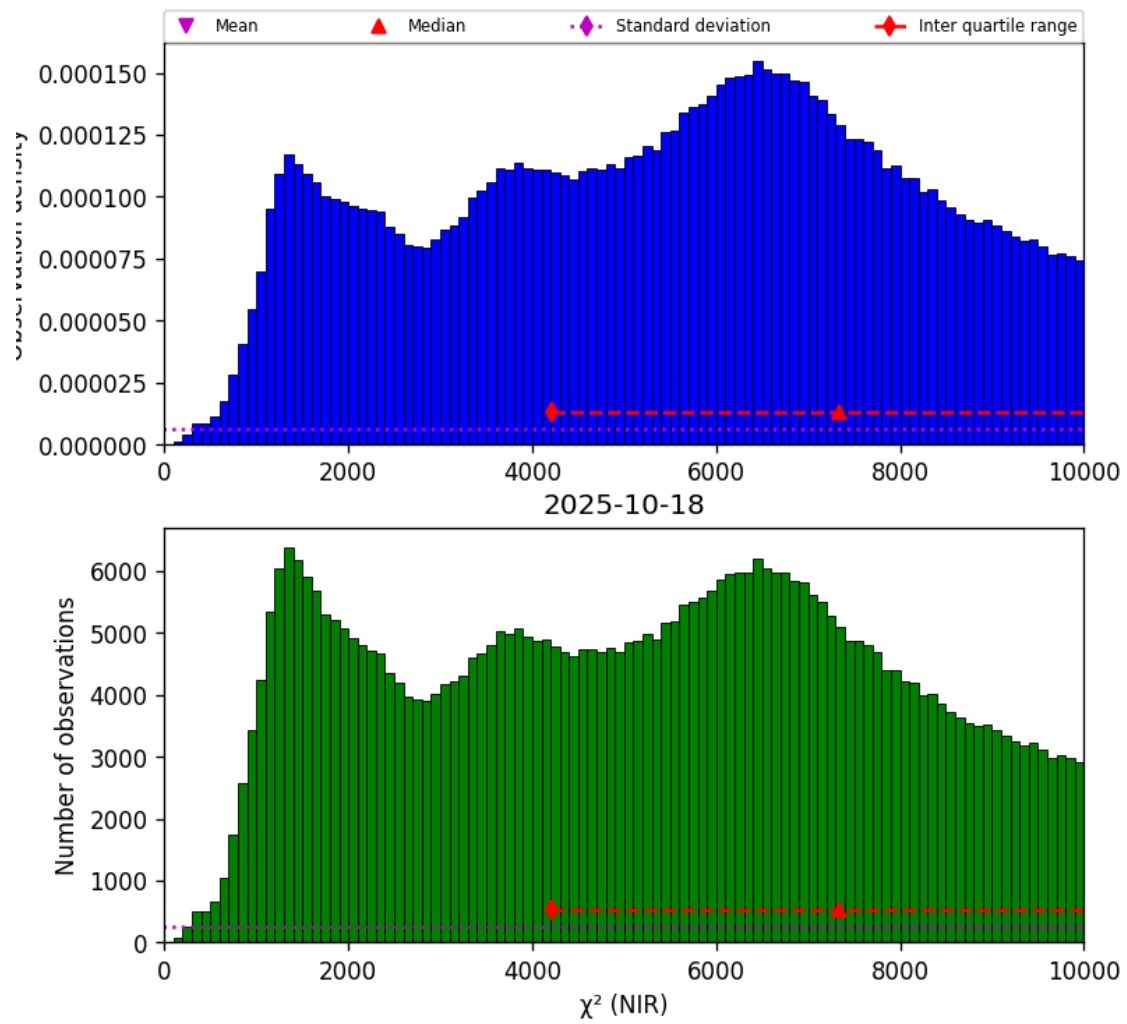
Figure 29: Histogram of “ \chi^2 (NIR)” for 2025-10-17 to 2025-10-19
