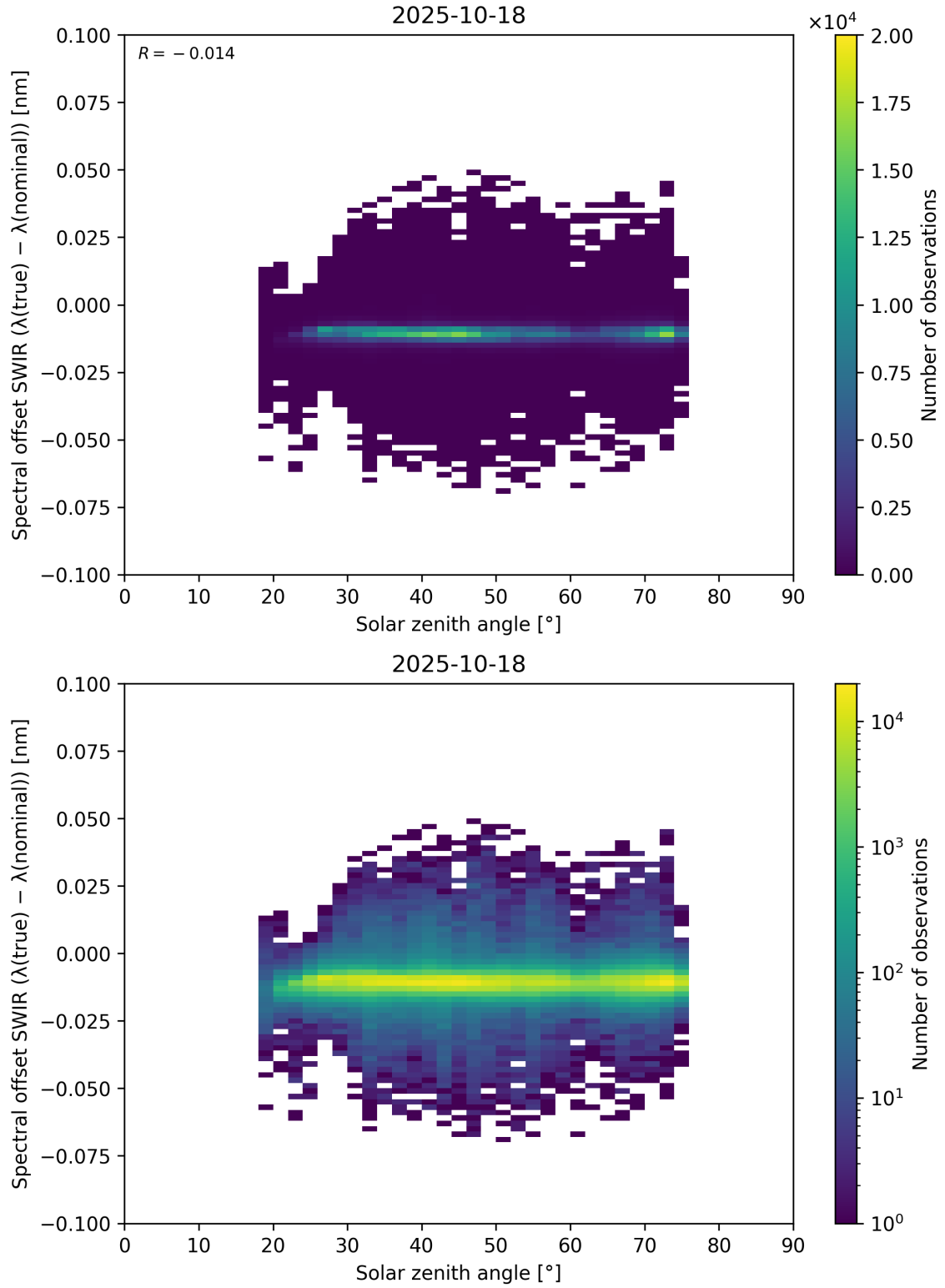
Figure 104: Scatter density plot of “Solar zenith angle” against “Spectral offset SWIR ( \lambda_{\text{true}} - \lambda_{\text{nominal}} )” for 2025-10-17 to 2025-10-19.
