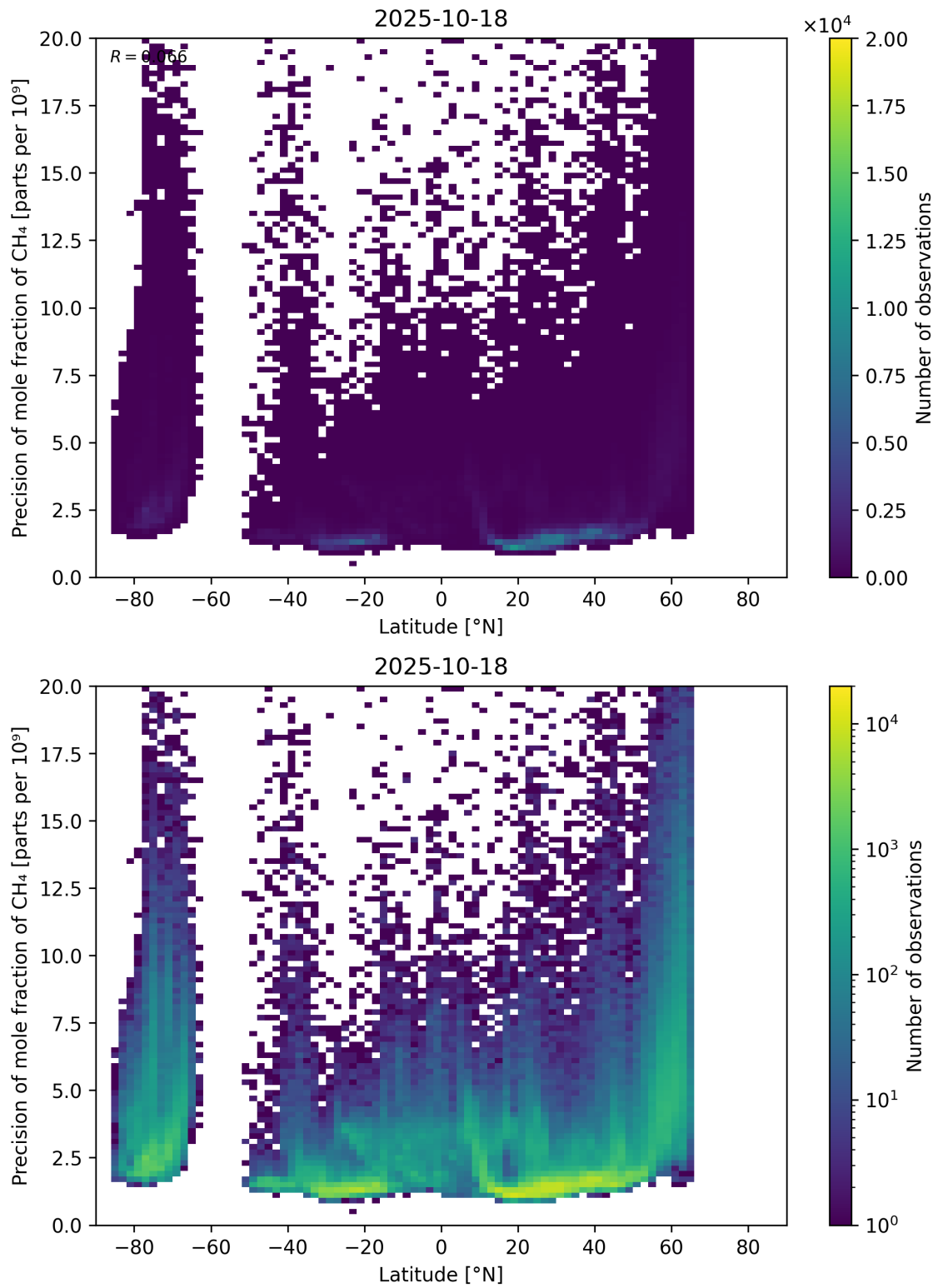
Figure 59: Scatter density plot of “Latitude” against “Precision of mole fraction of \text{CH}_4 ” for 2025-10-17 to 2025-10-19.
