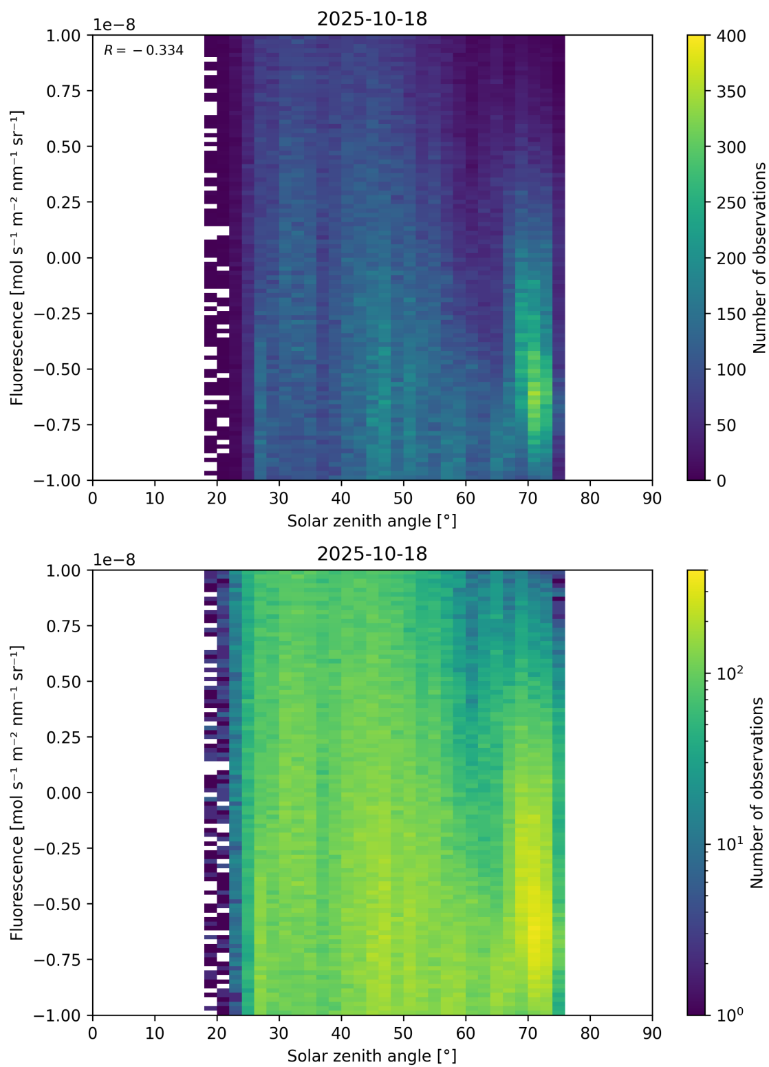
Figure 97: Scatter density plot of “Solar zenith angle” against “Fluorescence” for 2025-10-17 to 2025-10-19.
