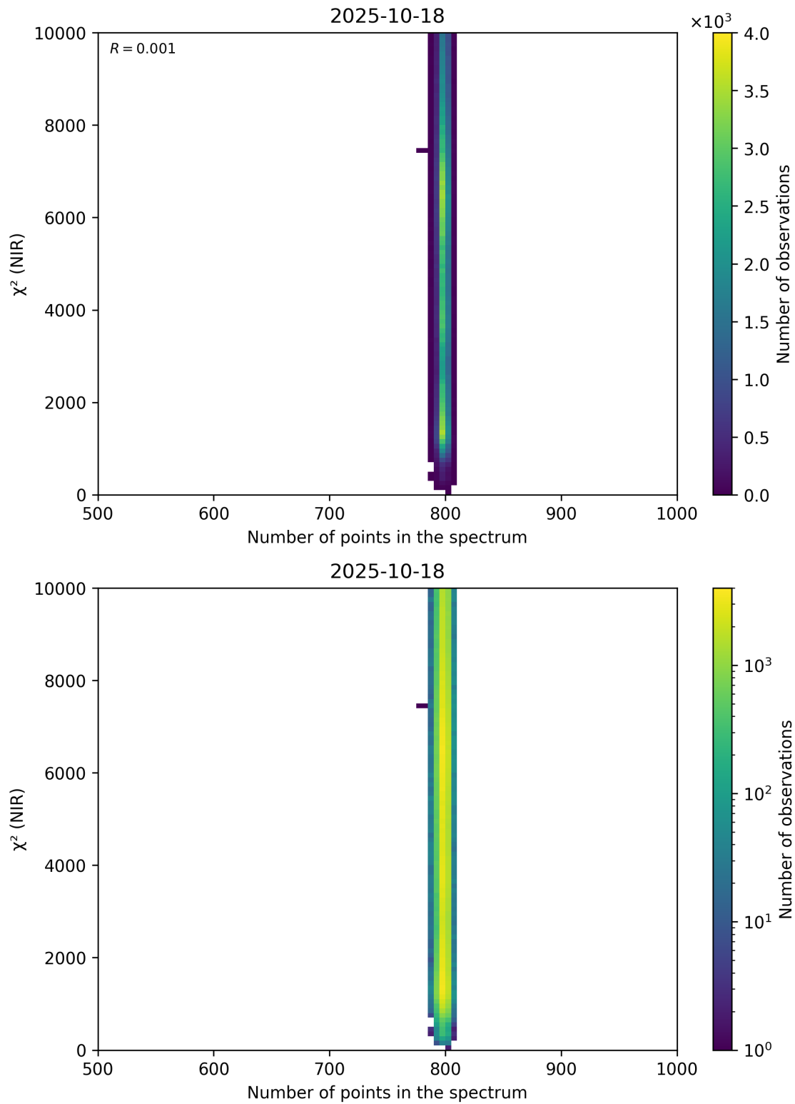
Figure 88: Scatter density plot of “Number of points in the spectrum” against “ \chi^2 (NIR)” for 2025-10-17 to 2025-10-19.
