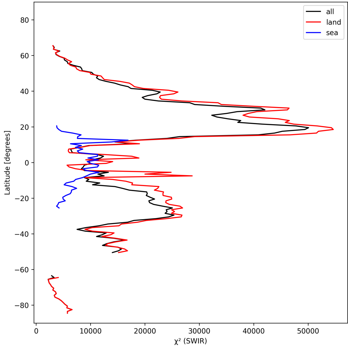
Figure 17: Zonal average of “ \chi^2 (SWIR)” for 2025-10-17 to 2025-10-19.
