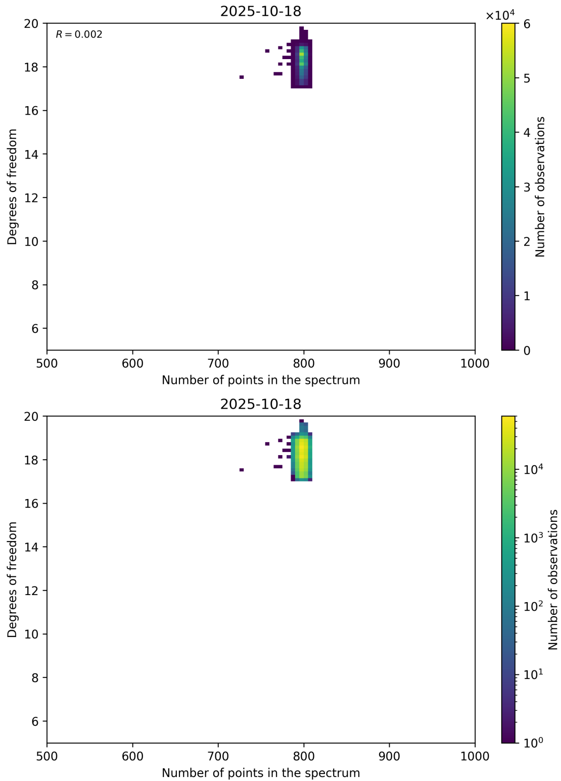
Figure 90: Scatter density plot of “Number of points in the spectrum” against “Degrees of freedom” for 2025-10-17 to 2025-10-19.
