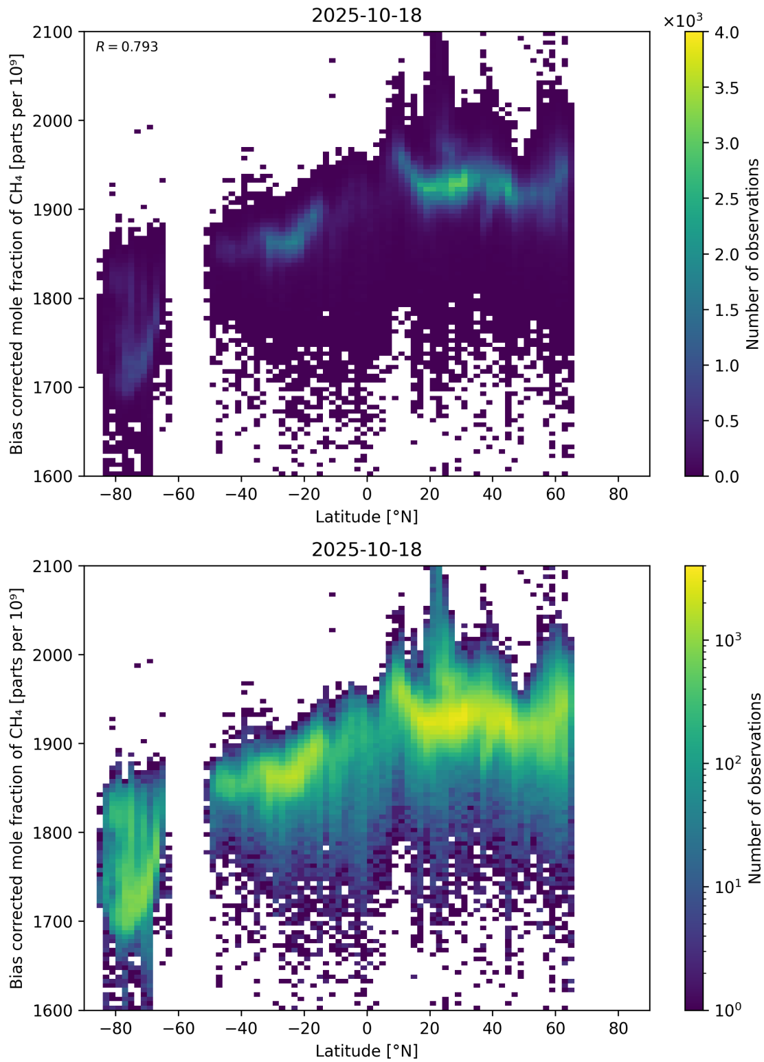
Figure 58: Scatter density plot of “Latitude” against “Bias corrected mole fraction of \text{CH}_4 ” for 2025-10-17 to 2025-10-19.
