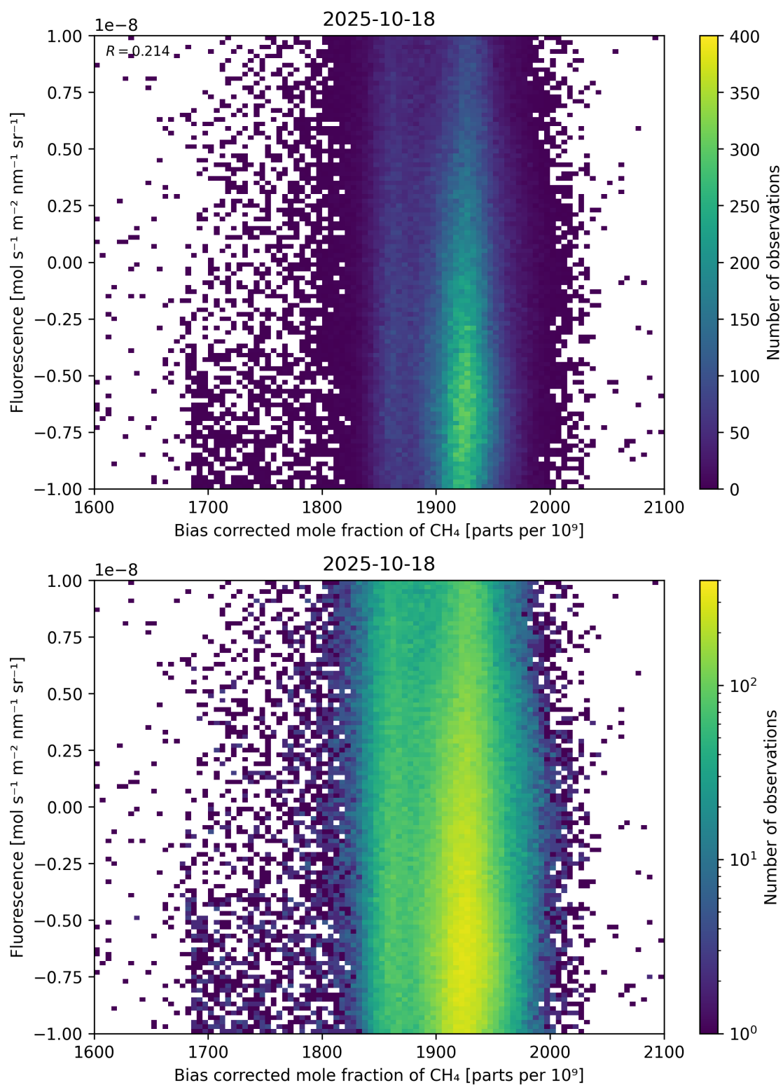
Figure 66: Scatter density plot of “Bias corrected mole fraction of \text{CH}_4 ” against “Fluorescence” for 2025-10-17 to 2025-10-19.
