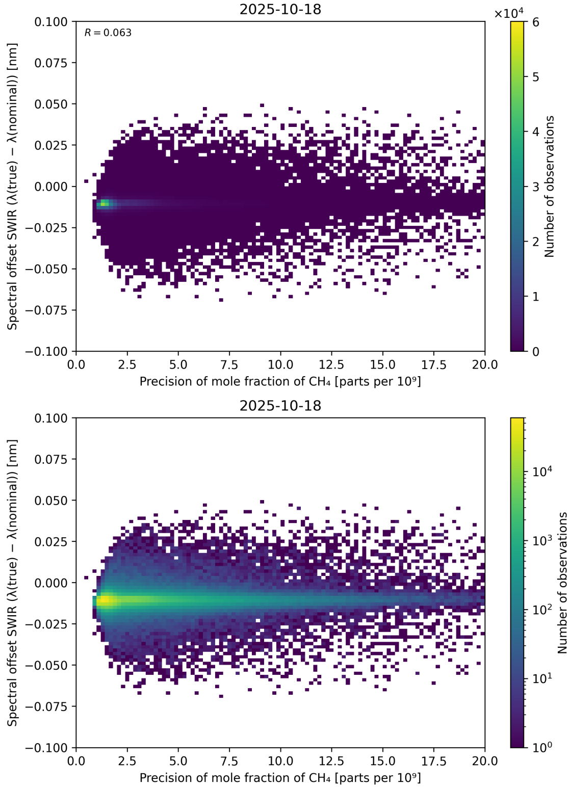
Figure 85: Scatter density plot of “Precision of mole fraction of \text{CH}_4 ” against “Spectral offset SWIR ( \lambda_{\text{true}} - \lambda_{\text{nominal}} )” for 2025-10-17 to 2025-10-19.
