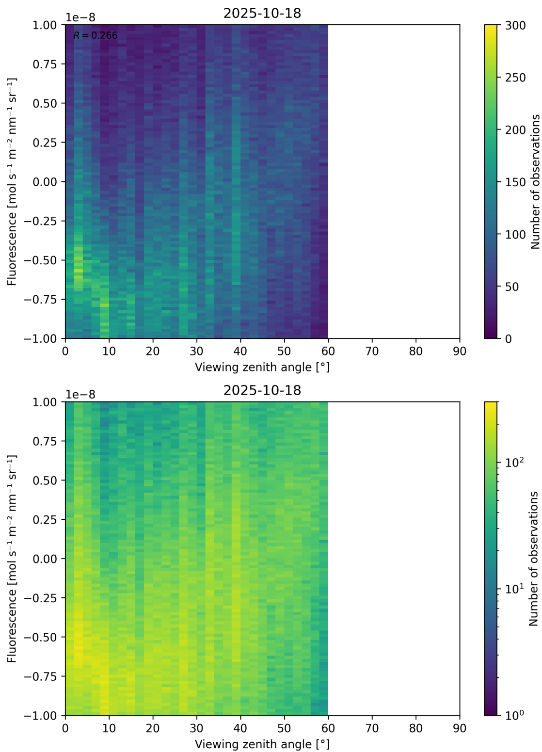
Figure 108: Scatter density plot of “Viewing zenith angle” against “Fluorescence” for 2025-10-17 to 2025-10-19.
