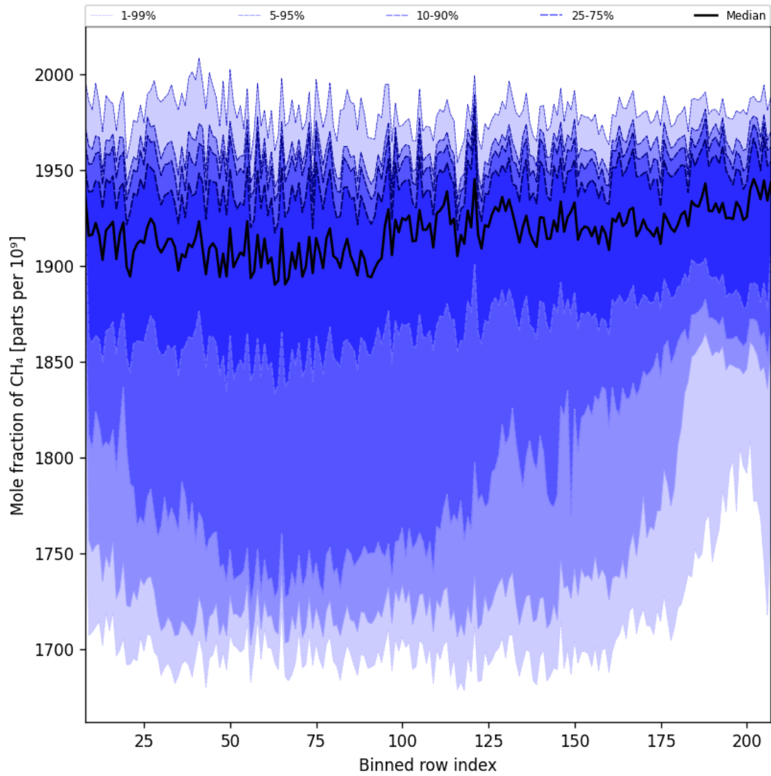
Figure 34: Along track statistics of “Mole fraction of CH 4 ” for 2025-10-17 to 2025-10-19
