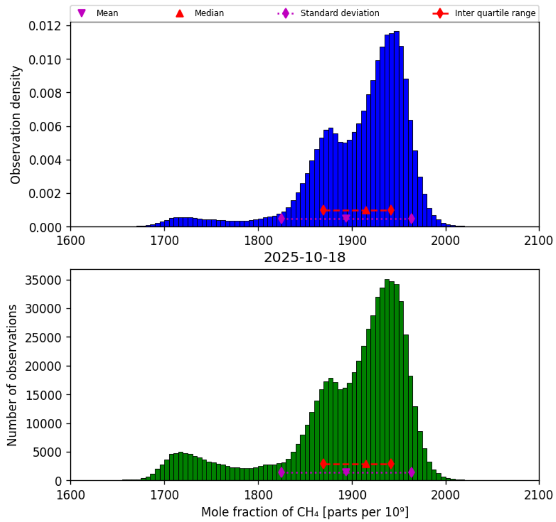
Figure 23: Histogram of “Mole fraction of CH 4 ” for 2025-10-17 to 2025-10-19
