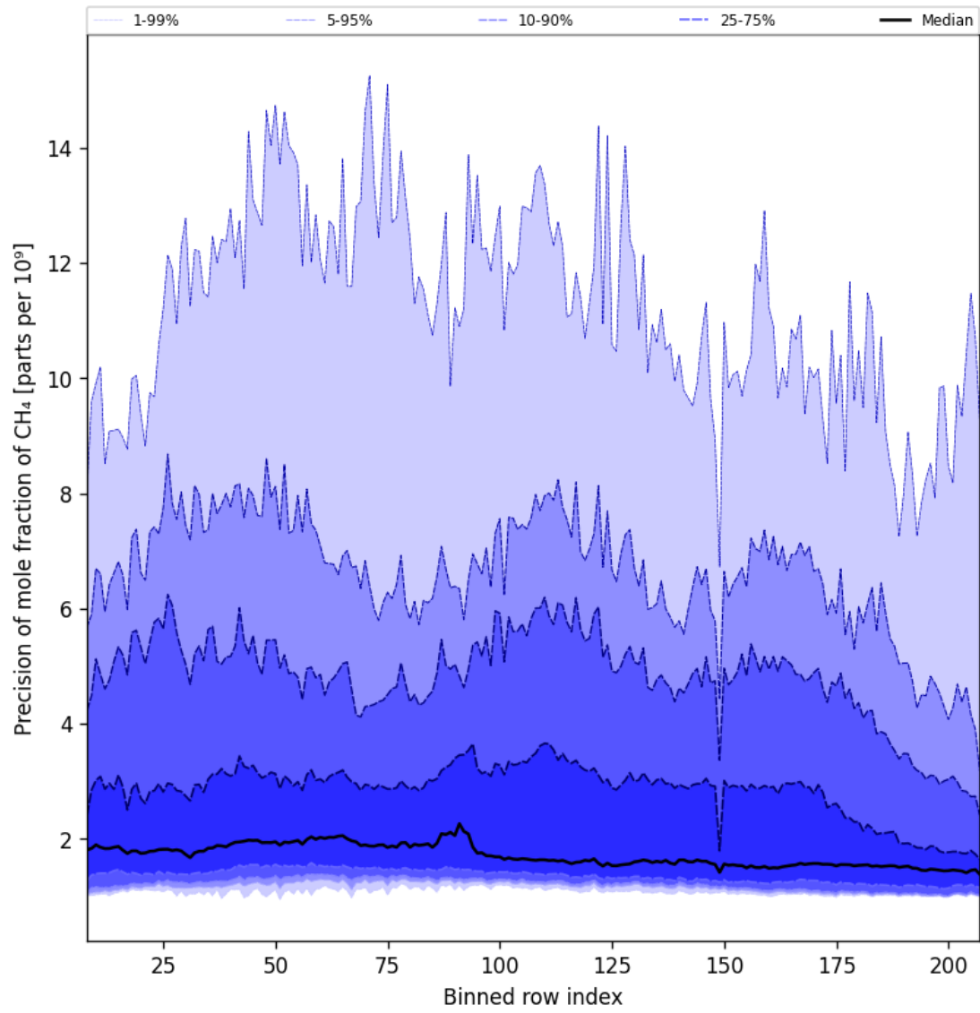
Figure 35: Along track statistics of “Precision of mole fraction of CH 4 ” for 2025-10-17 to 2025-10-19
