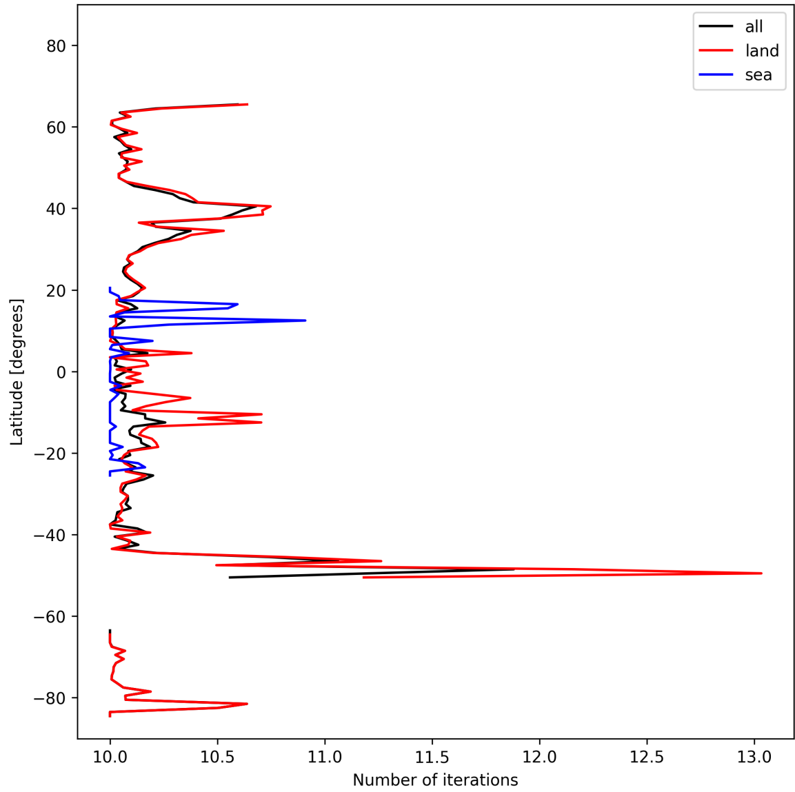
Figure 20: Zonal average of “Number of iterations” for 2025-10-17 to 2025-10-19.
