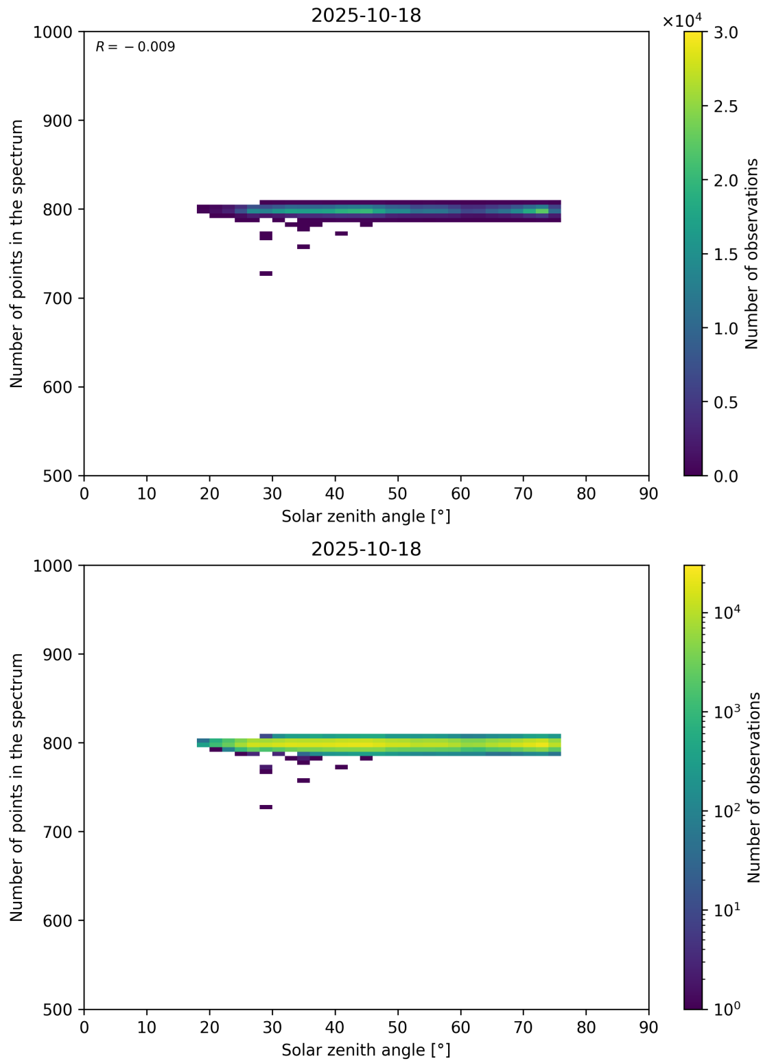
Figure 103: Scatter density plot of “Solar zenith angle” against “Number of points in the spectrum” for 2025-10-17 to 2025-10-19.
