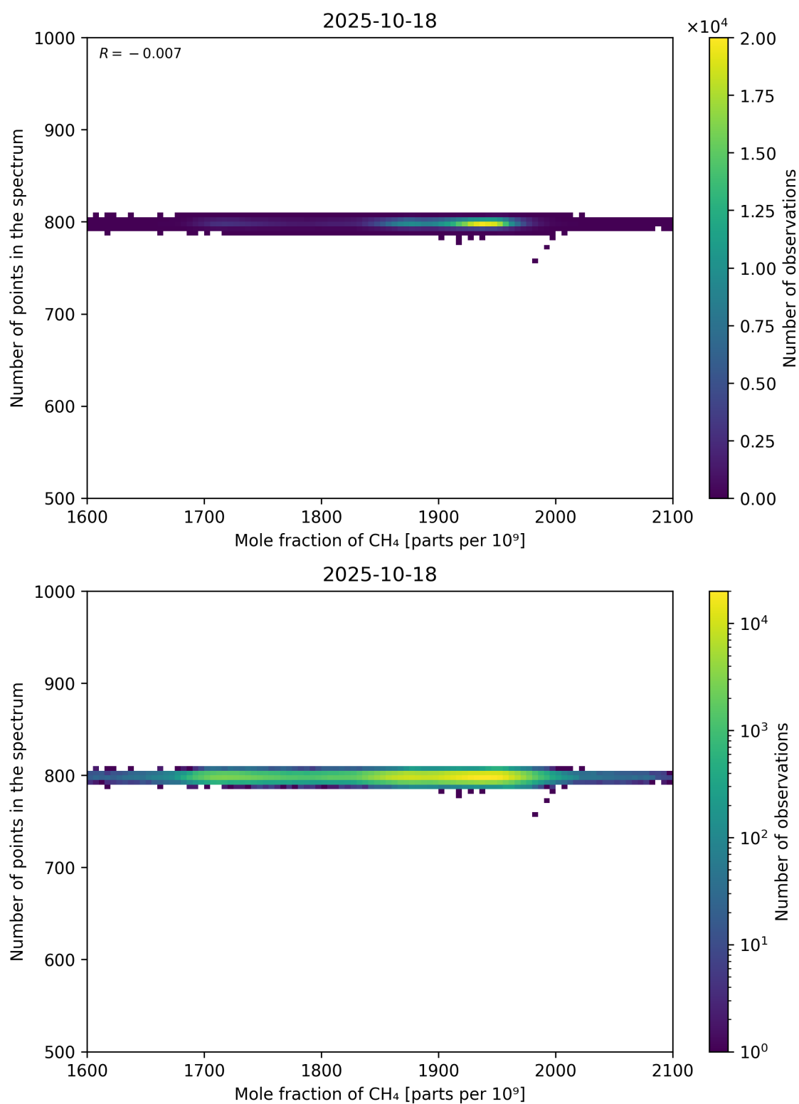
Figure 77: Scatter density plot of “Mole fraction of CH 4 ” against “Number of points in the spectrum” for 2025-10-17 to 2025-10-19.
