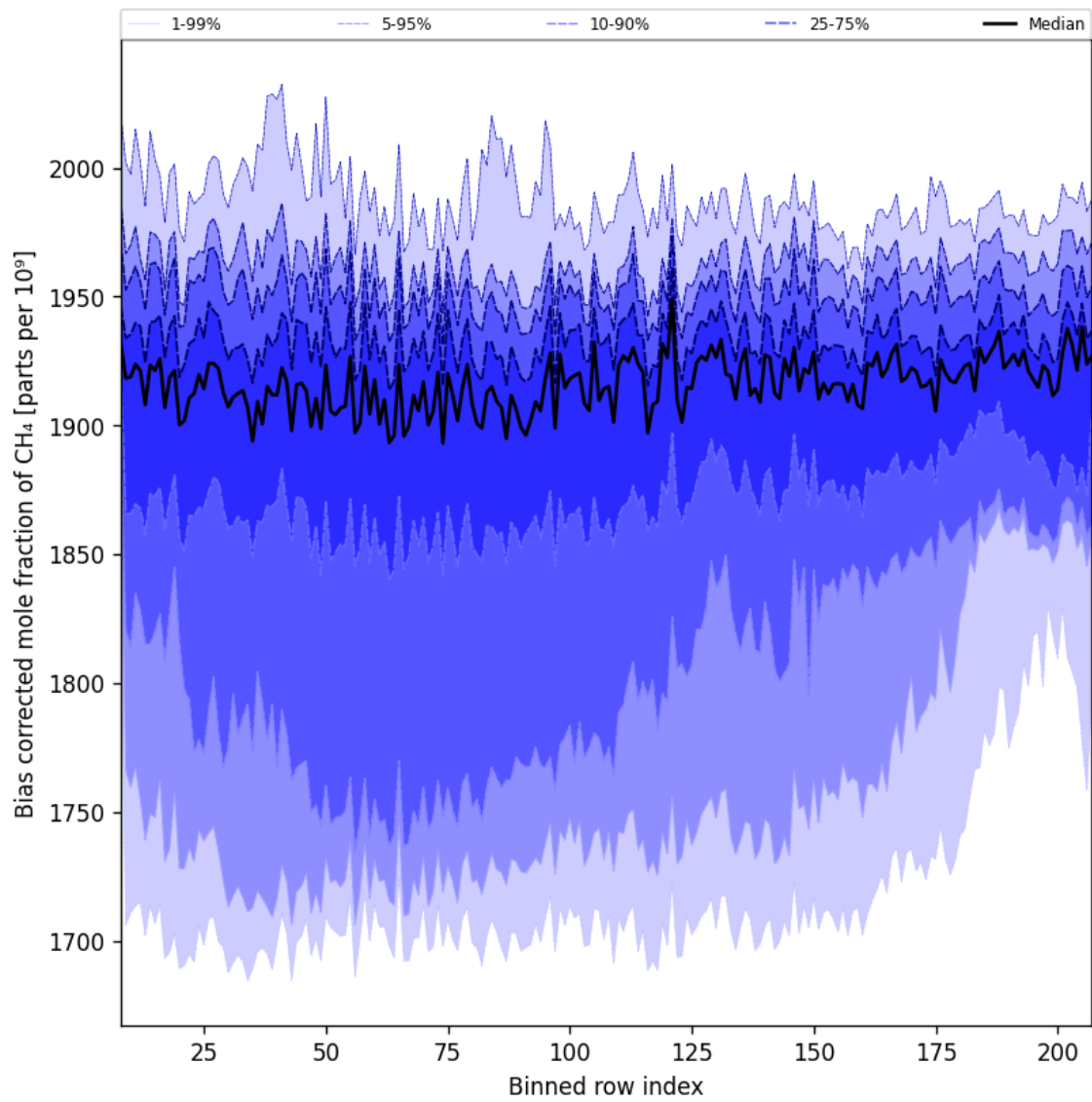
Figure 36: Along track statistics of “Bias corrected mole fraction of CH 4 ” for 2025-10-17 to 2025-10-19
