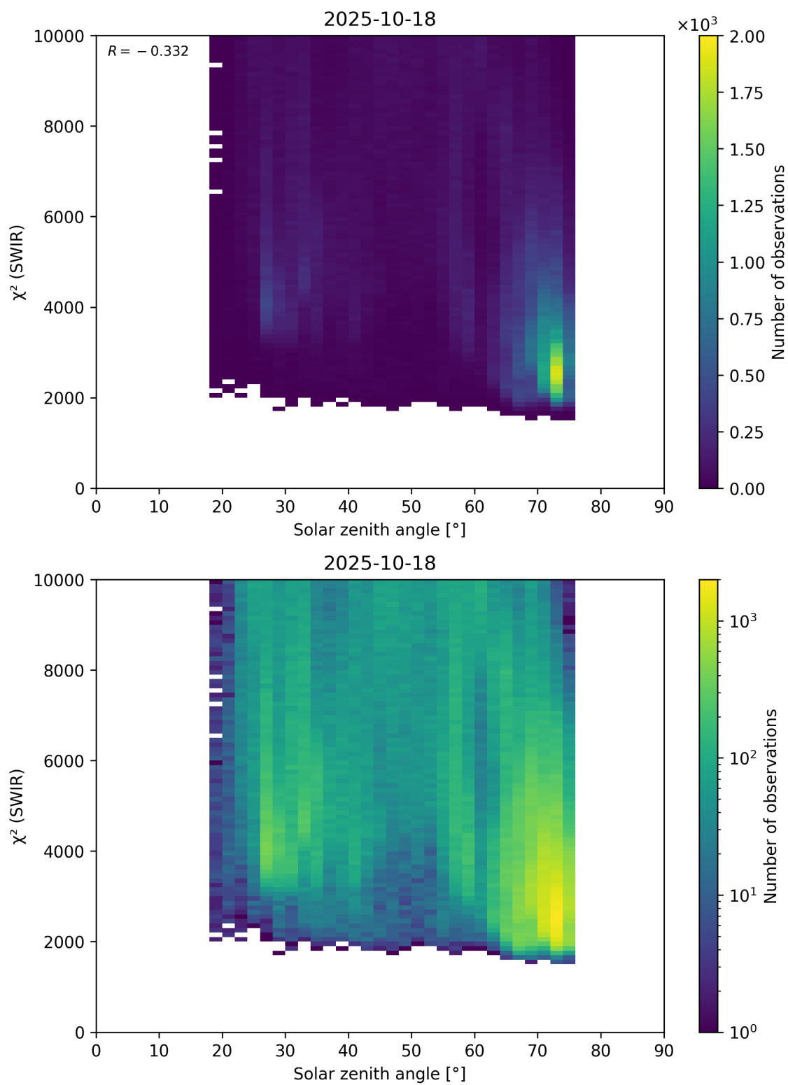
Figure 95: Scatter density plot of “Solar zenith angle” against “ \chi^2 (SWIR)” for 2025-10-17 to 2025-10-19.
