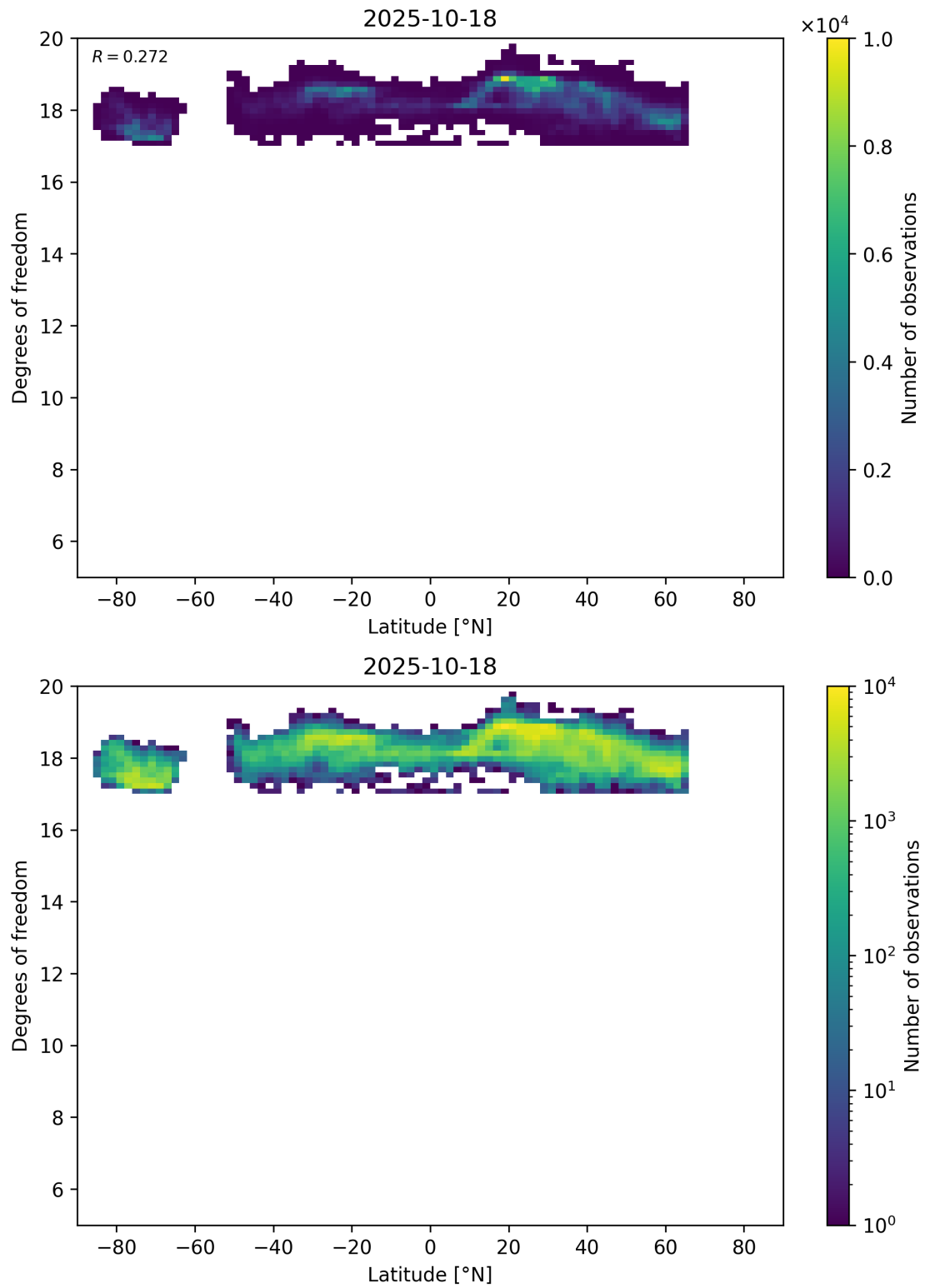
Figure 55: Scatter density plot of “Latitude” against “Degrees of freedom” for 2025-10-17 to 2025-10-19.
