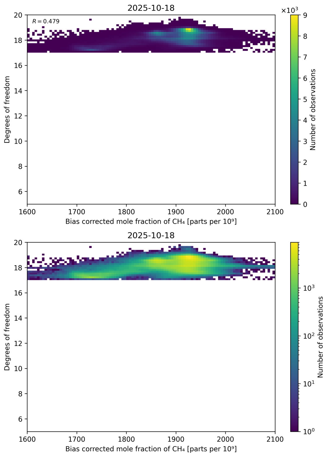
Figure 65: Scatter density plot of “Bias corrected mole fraction of CH 4 ” against “Degrees of freedom” for 2025-10-17 to 2025-10-19.
