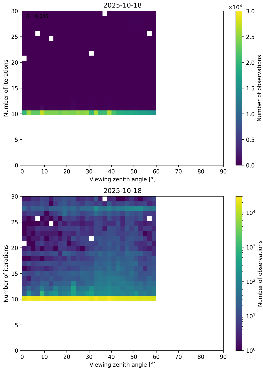
Figure 113: Scatter density plot of “Viewing zenith angle” against “Number of iterations” for 2025-10-17 to 2025-10-19.
