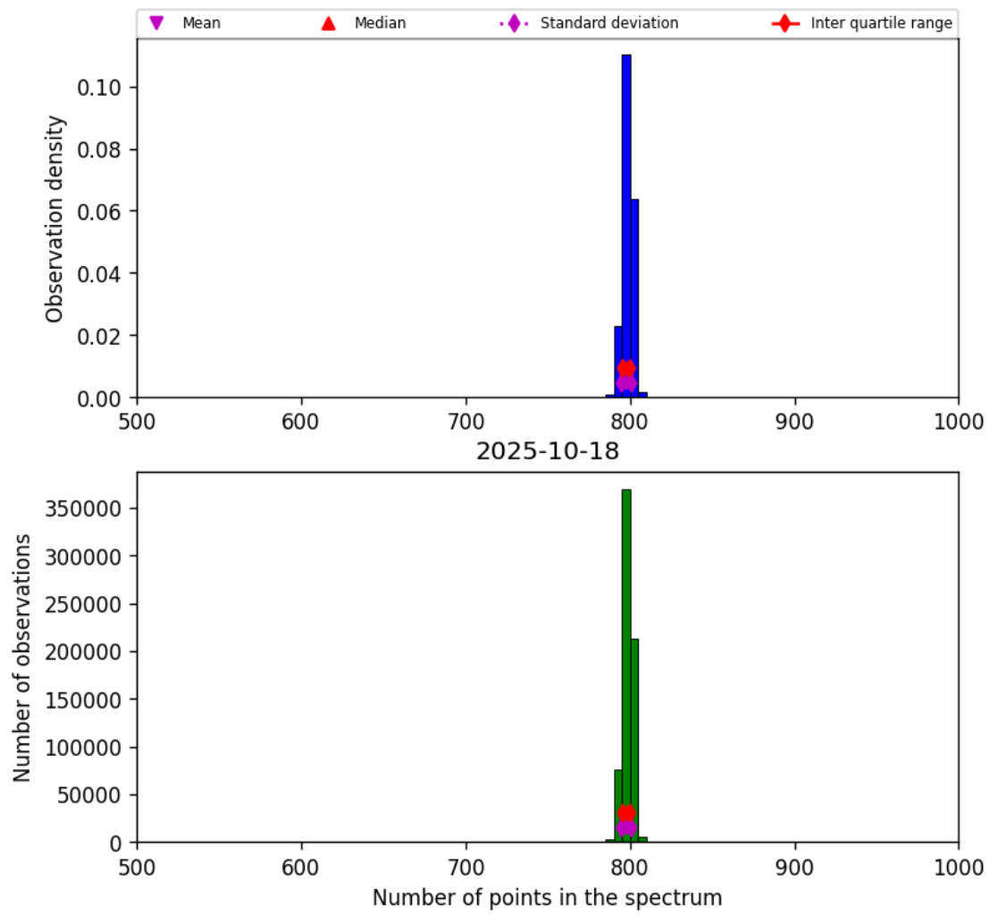
Figure 26: Histogram of “Number of points in the spectrum” for 2025-10-17 to 2025-10-19
