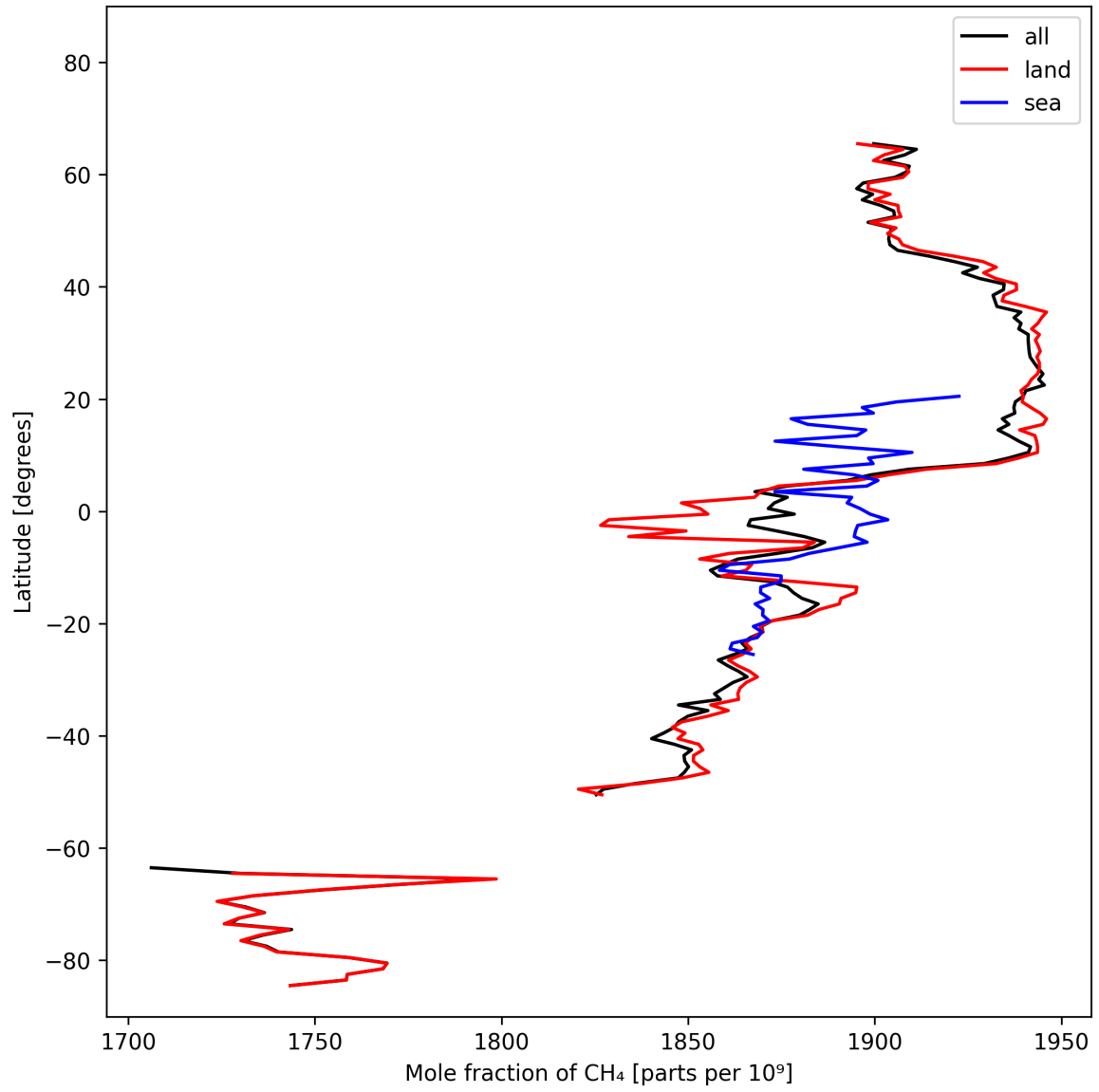
Figure 12: Zonal average of “Mole fraction of CH 4 ” for 2025-10-17 to 2025-10-19.
