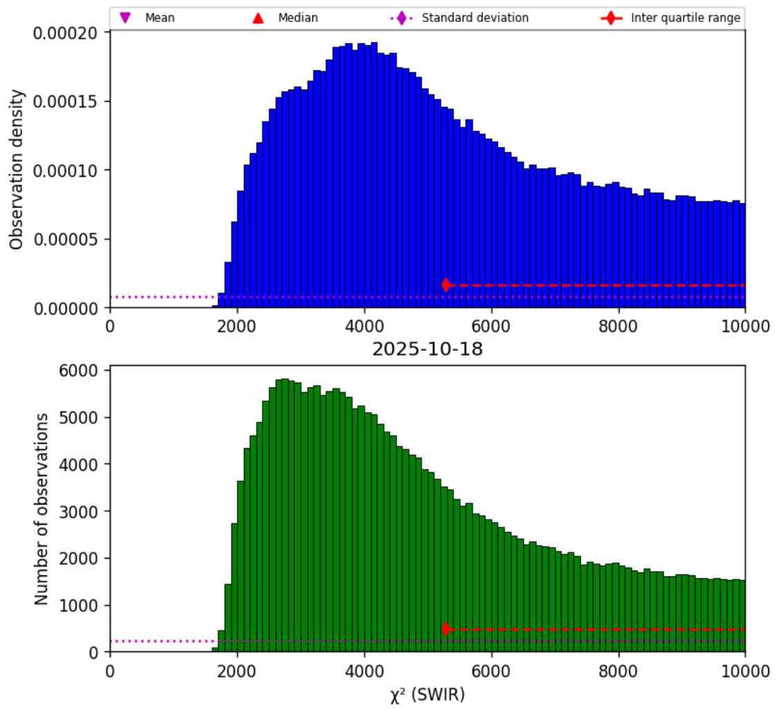
Figure 28: Histogram of “ \chi^2 (SWIR)” for 2025-10-17 to 2025-10-19
