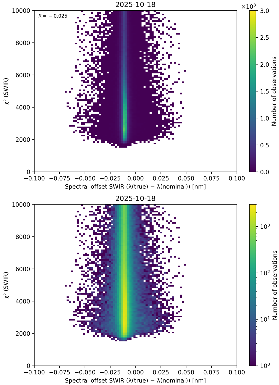
Figure 118: Scatter density plot of “Spectral offset SWIR ( \lambda_{\text{true}} - \lambda_{\text{nominal}} )” against “ \chi^2 (SWIR)” for 2025-10-17 to 2025-10-19.
