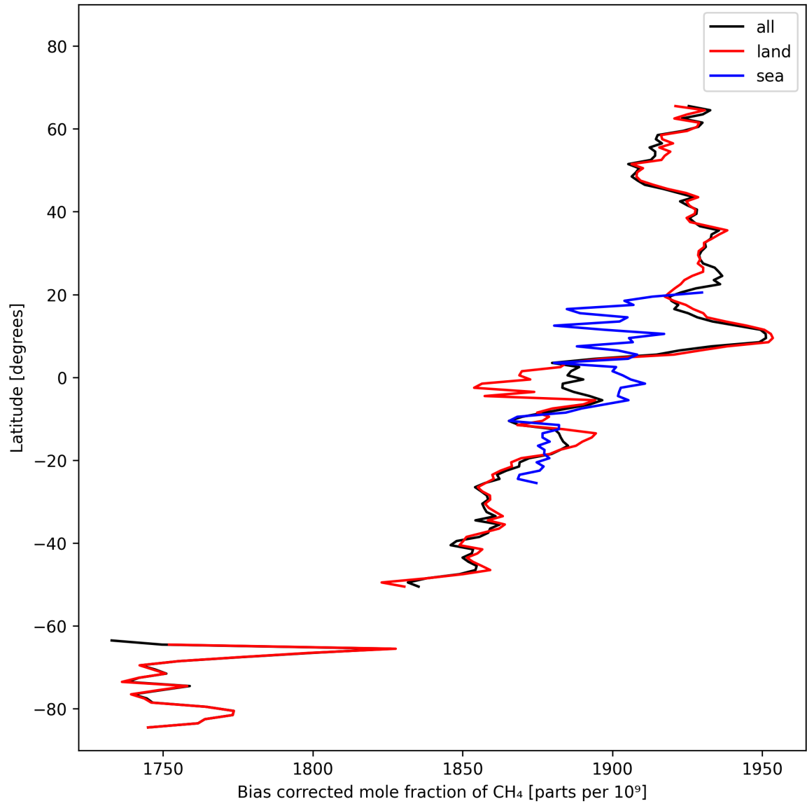
Figure 14: Zonal average of “Bias corrected mole fraction of CH 4 ” for 2025-10-17 to 2025-10-19.
