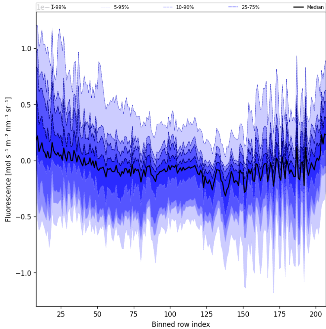
Figure 43: Along track statistics of “Fluorescence” for 2025-10-17 to 2025-10-19
