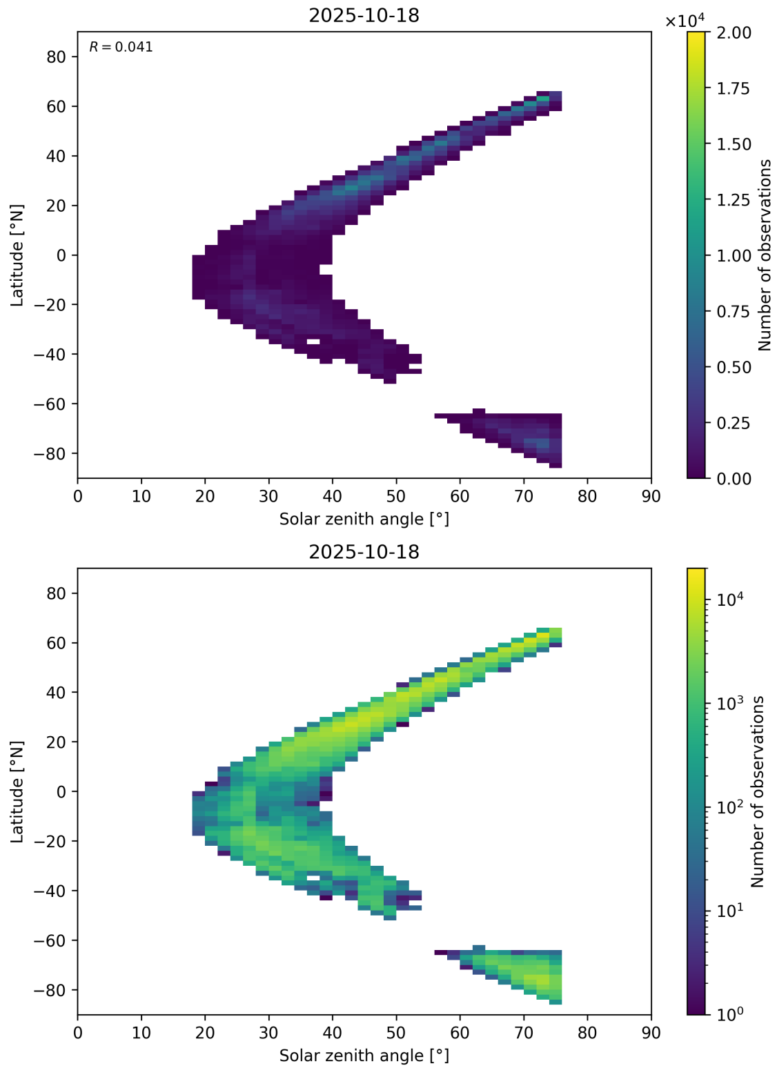
Figure 98: Scatter density plot of “Solar zenith angle” against “Latitude” for 2025-10-17 to 2025-10-19.
