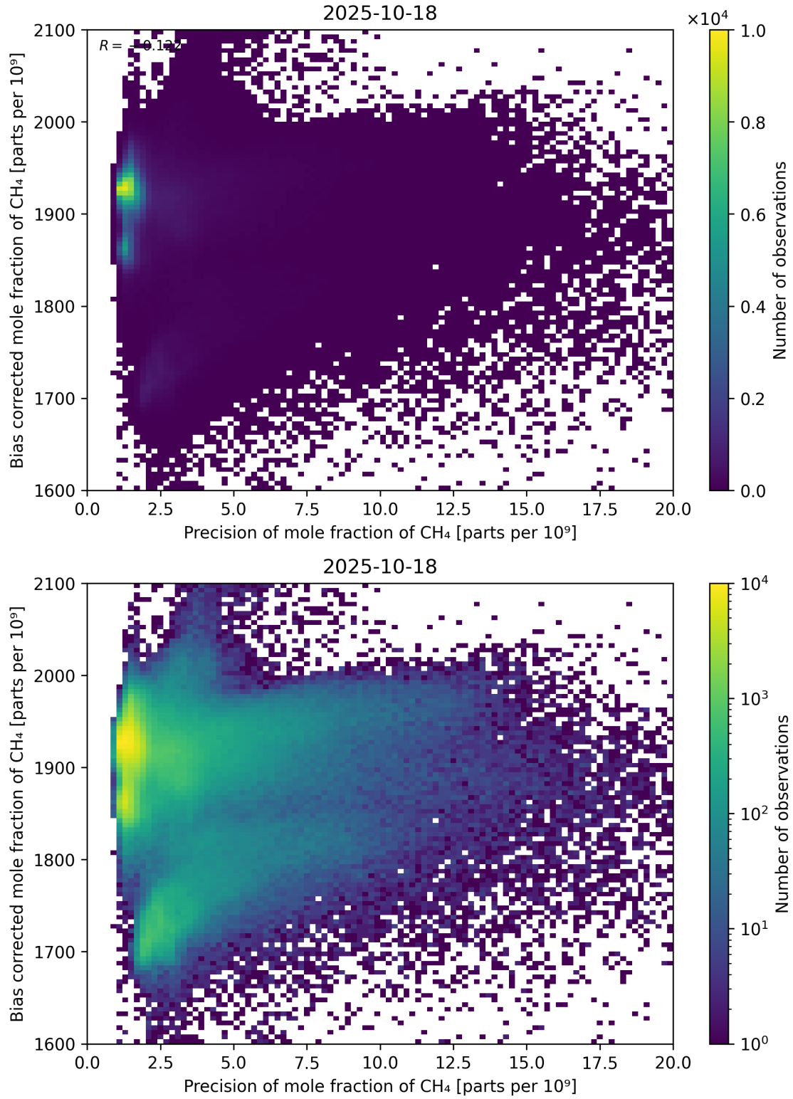
Figure 82: Scatter density plot of “Precision of mole fraction of CH 4 ” against “Bias corrected mole fraction of CH 4 ” for 2025-10-17 to 2025-10-19.
