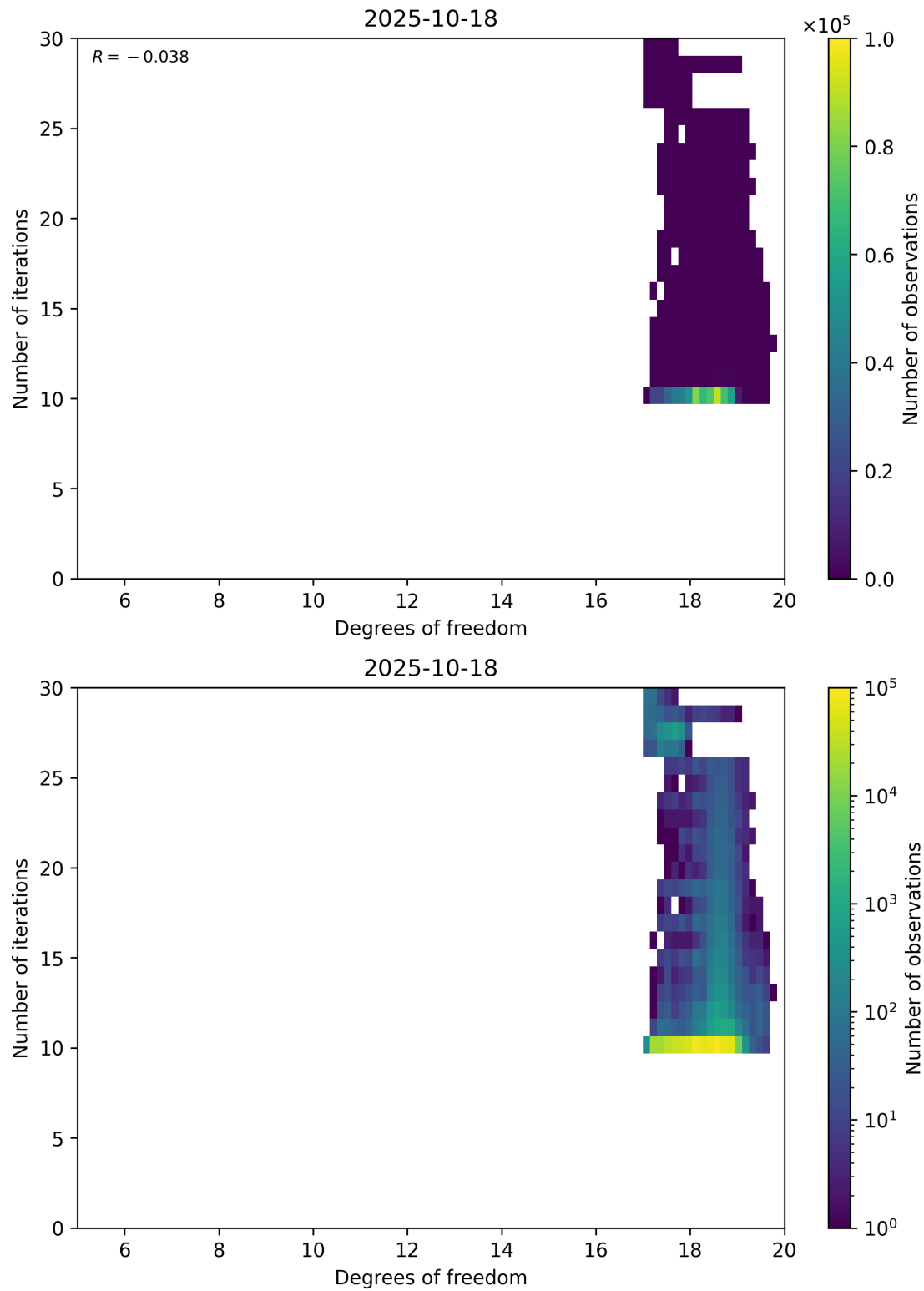
Figure 52: Scatter density plot of “Degrees of freedom” against “Number of iterations” for 2025-10-17 to 2025-10-19.
