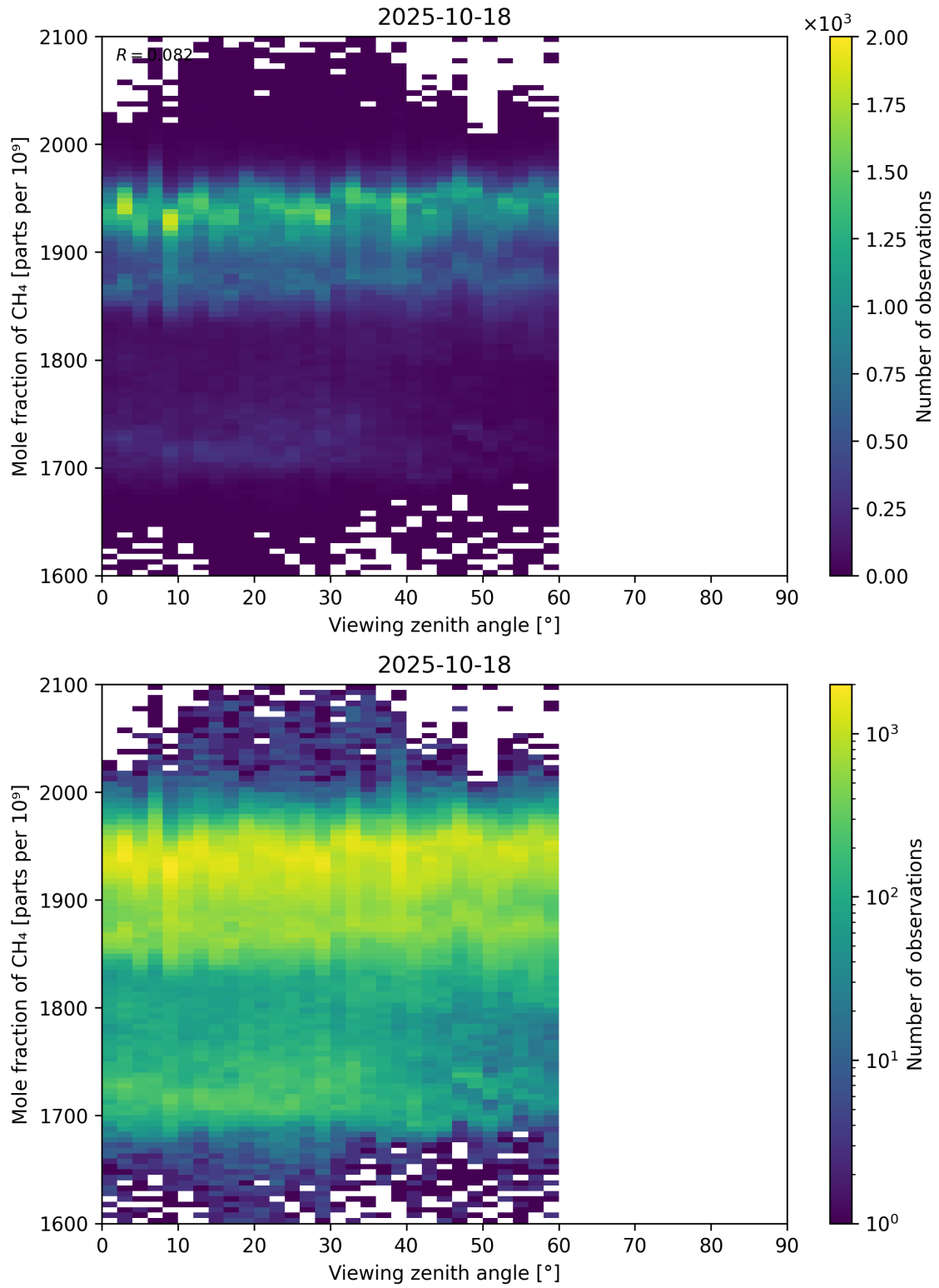
Figure 110: Scatter density plot of “Viewing zenith angle” against “Mole fraction of CH 4 ” for 2025-10-17 to 2025-10-19.
