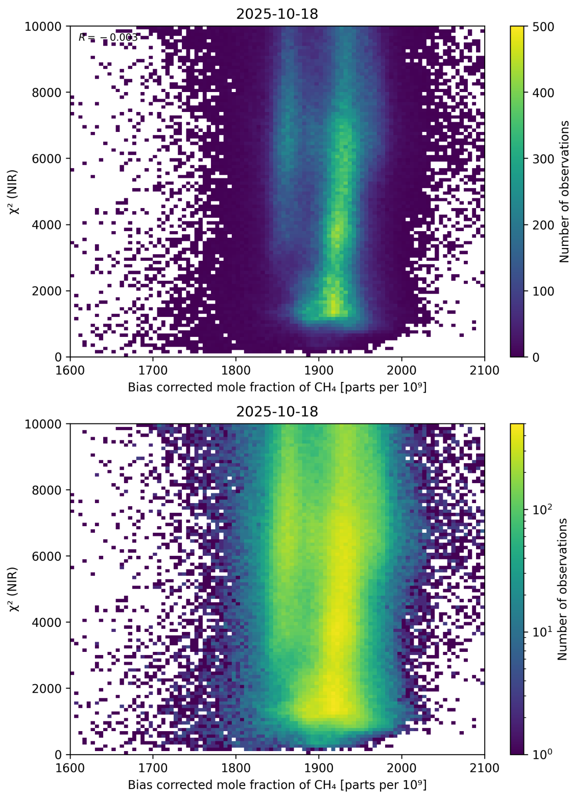
Figure 63: Scatter density plot of “Bias corrected mole fraction of \text{CH}_4 ” against “ \chi^2 (NIR)” for 2025-10-17 to 2025-10-19.
