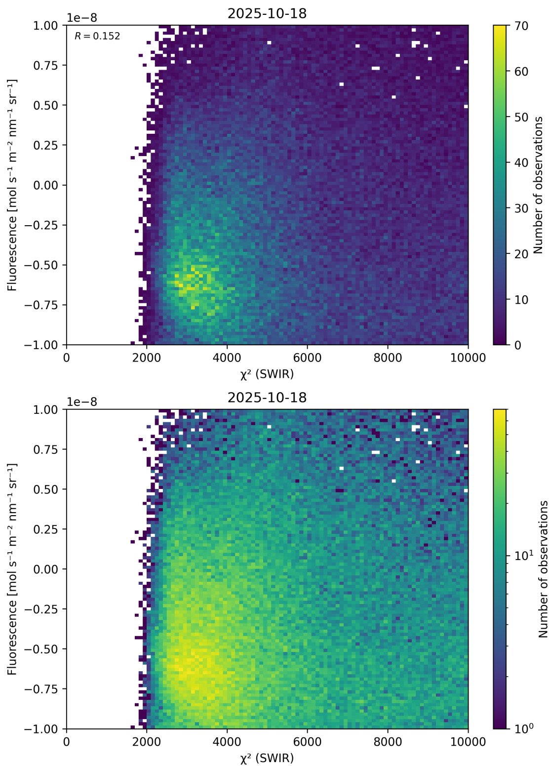
Figure 49: Scatter density plot of “ \chi^2 (SWIR)” against “Fluorescence” for 2025-10-17 to 2025-10-19.
