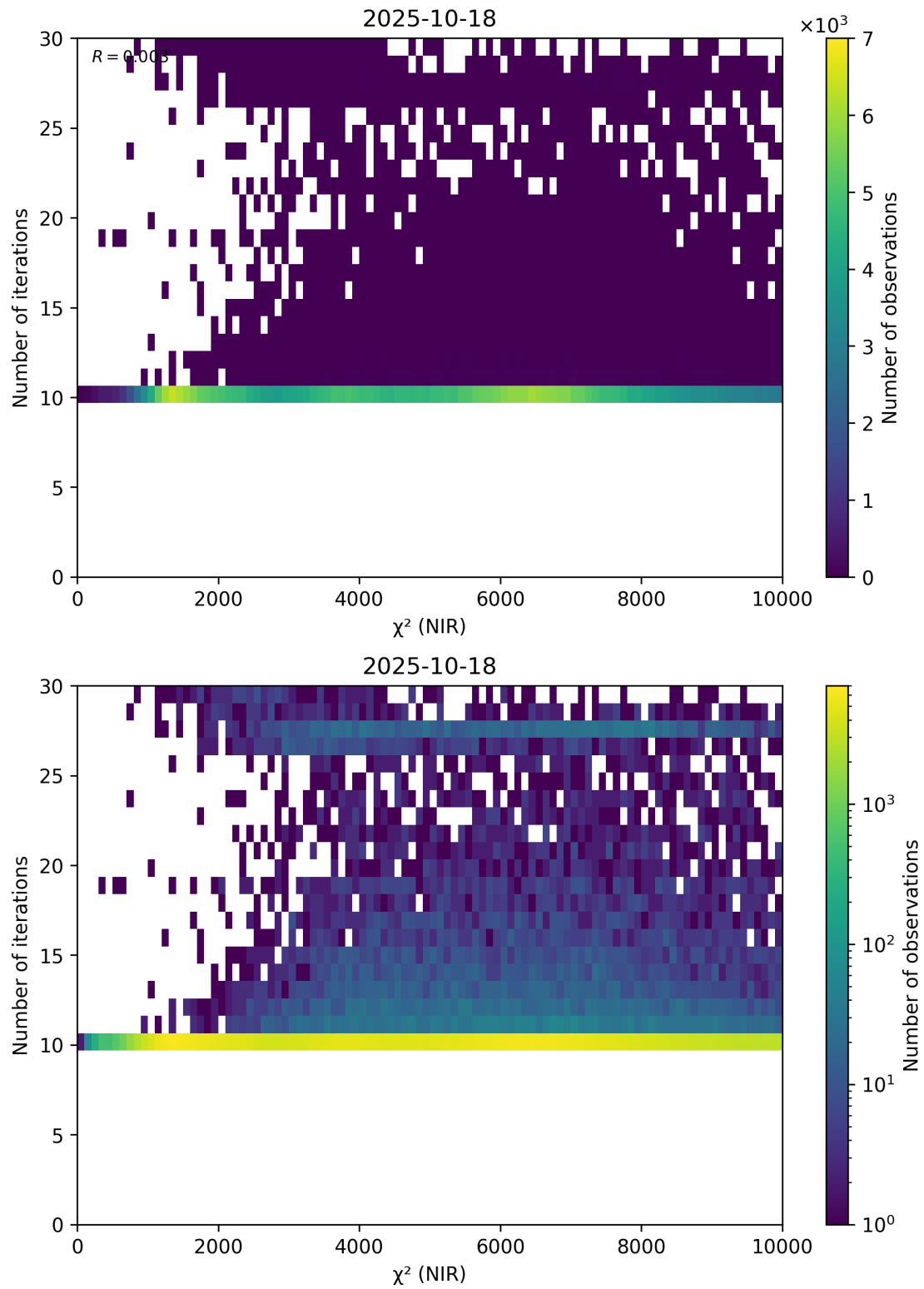
Figure 46: Scatter density plot of “ \chi^2 (NIR)” against “Number of iterations” for 2025-10-17 to 2025-10-19.
