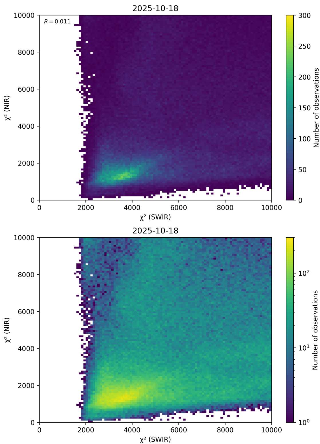
Figure 47: Scatter density plot of “ \chi^2 (SWIR)” against “ \chi^2 (NIR)” for 2025-10-17 to 2025-10-19.
