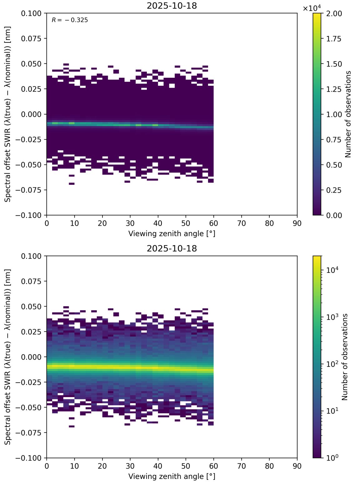
Figure 116: Scatter density plot of “Viewing zenith angle” against “Spectral offset SWIR ( \lambda_{\text{true}} - \lambda_{\text{nominal}} )” for 2025-10-17 to 2025-10-19.
