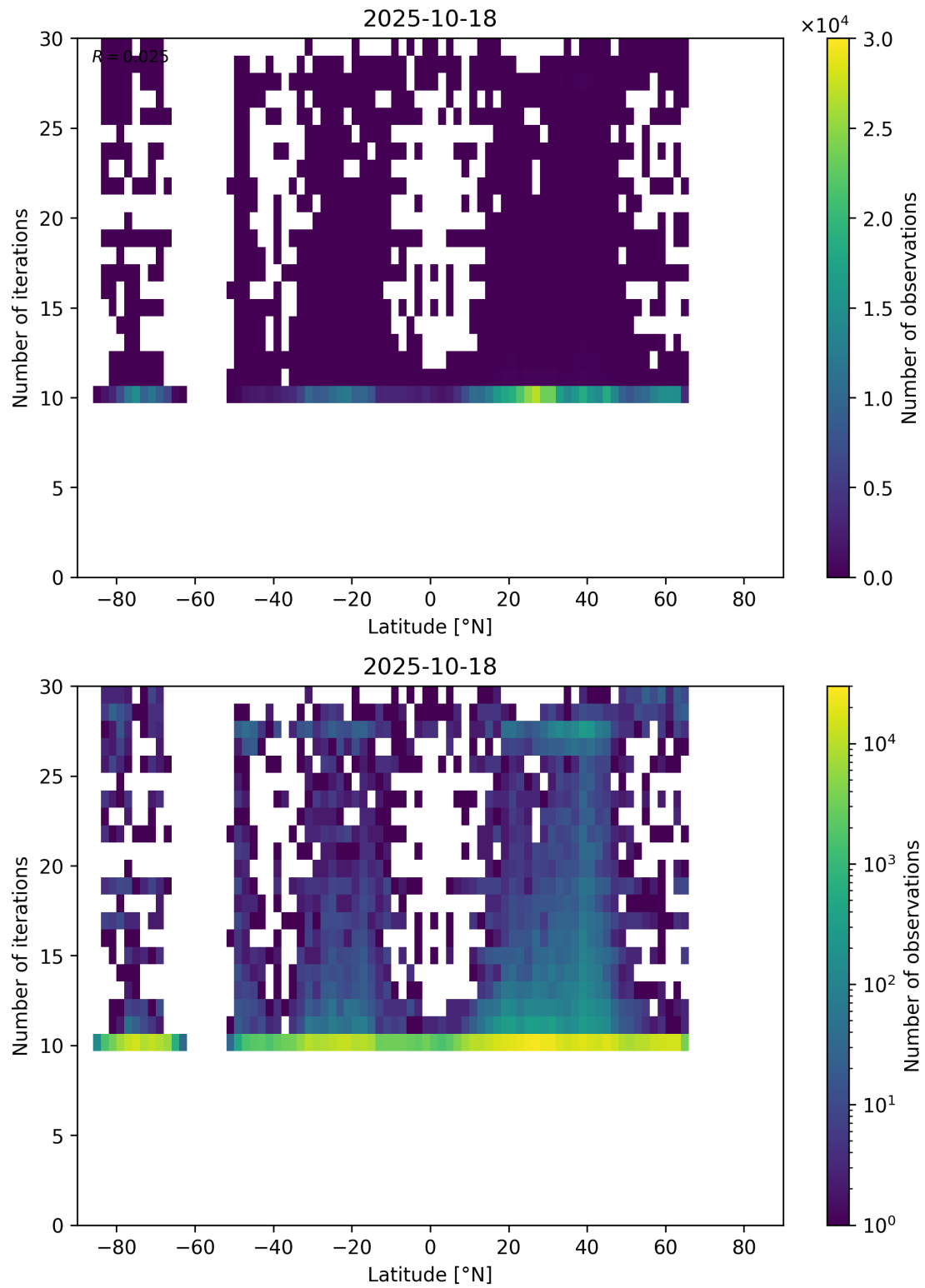
Figure 60: Scatter density plot of “Latitude” against “Number of iterations” for 2025-10-17 to 2025-10-19.
