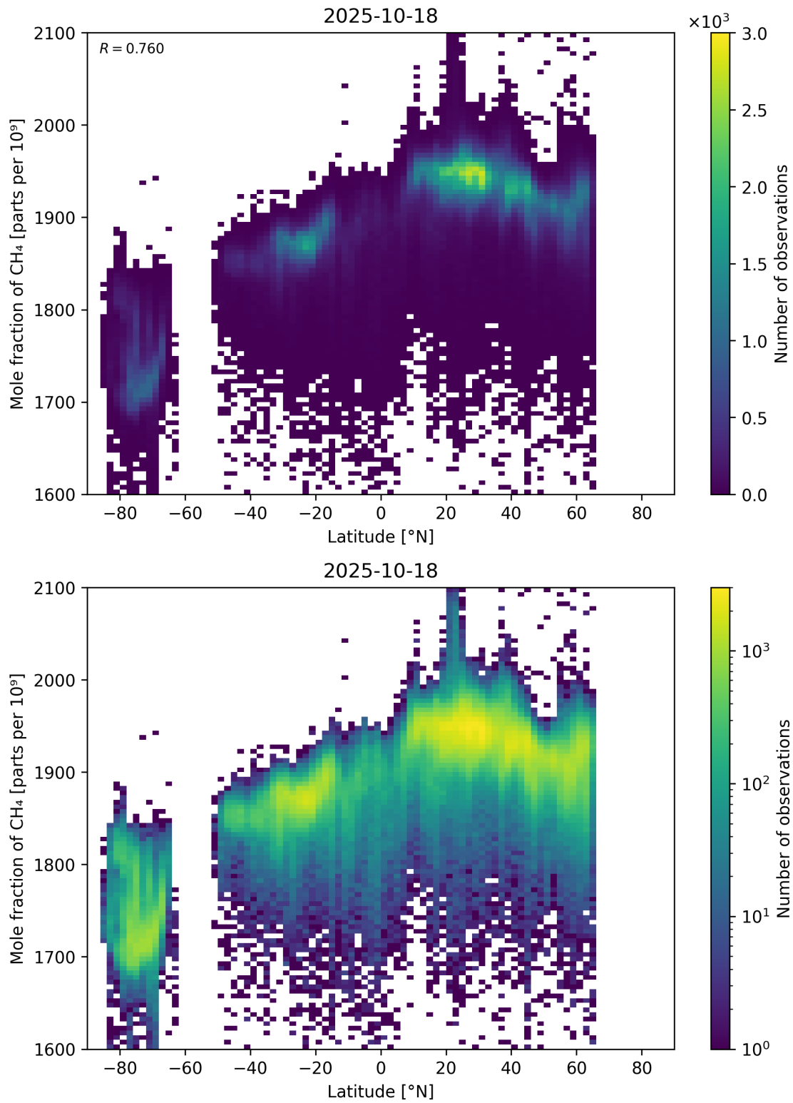
Figure 57: Scatter density plot of “Latitude” against “Mole fraction of CH 4 ” for 2025-10-17 to 2025-10-19.
