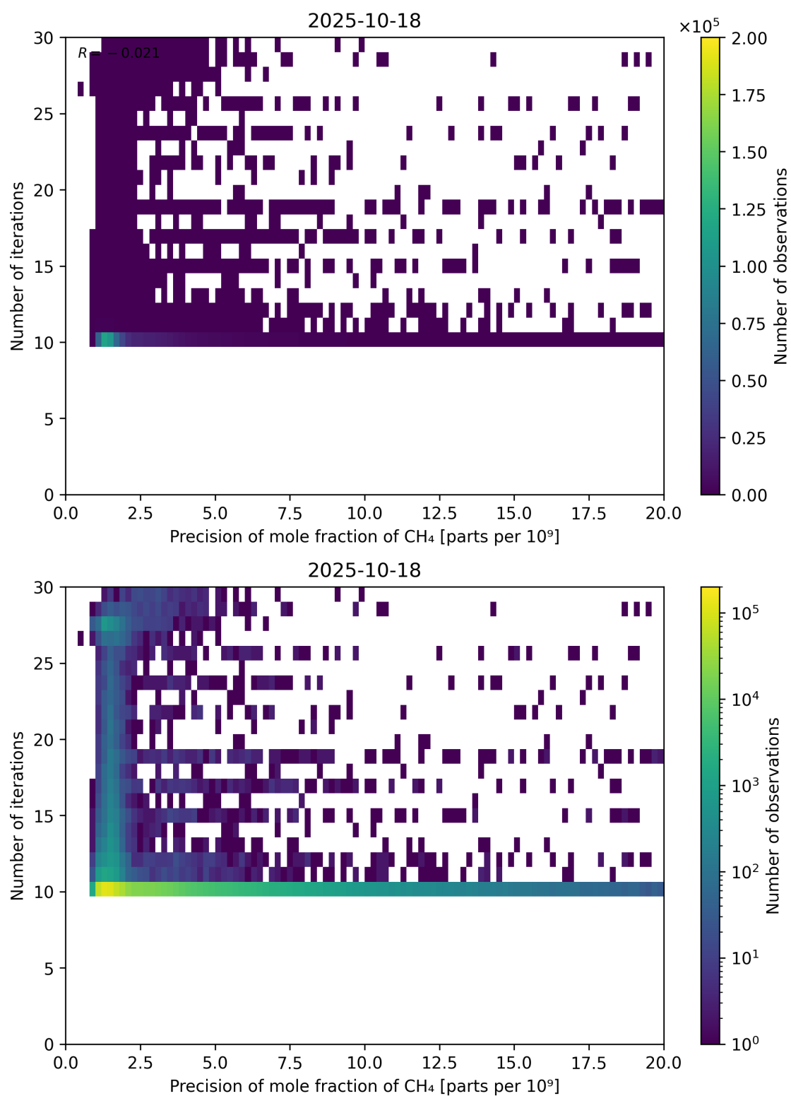
Figure 83: Scatter density plot of “Precision of mole fraction of CH 4 ” against “Number of iterations” for 2025-10-17 to 2025-10-19.
