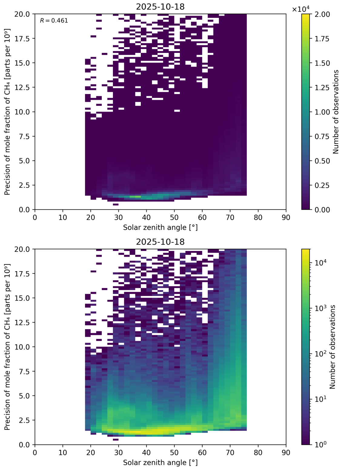
Figure 101: Scatter density plot of “Solar zenith angle” against “Precision of mole fraction of \text{CH}_4 ” for 2025-10-17 to 2025-10-19.
