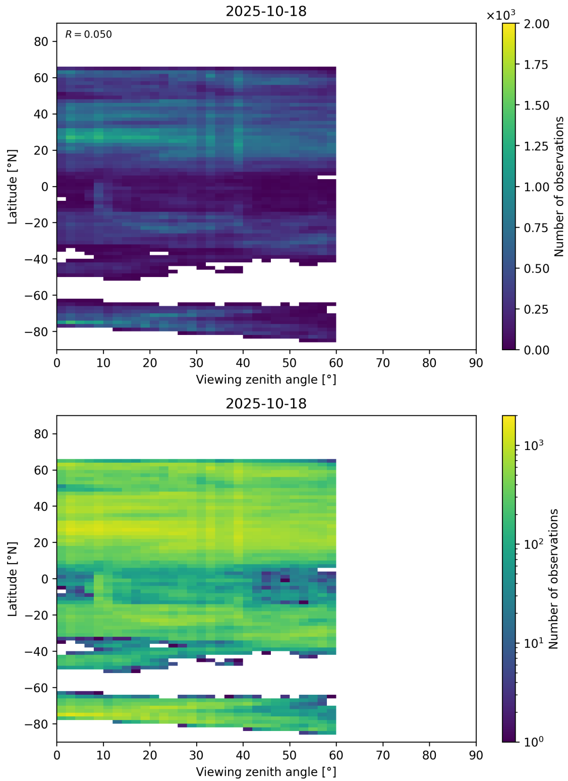
Figure 109: Scatter density plot of “Viewing zenith angle” against “Latitude” for 2025-10-17 to 2025-10-19.
