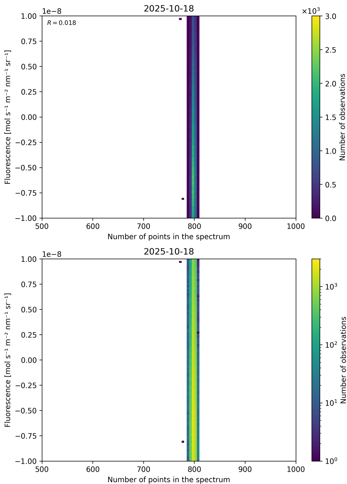
Figure 91: Scatter density plot of “Number of points in the spectrum” against “Fluorescence” for 2025-10-17 to 2025-10-19.
