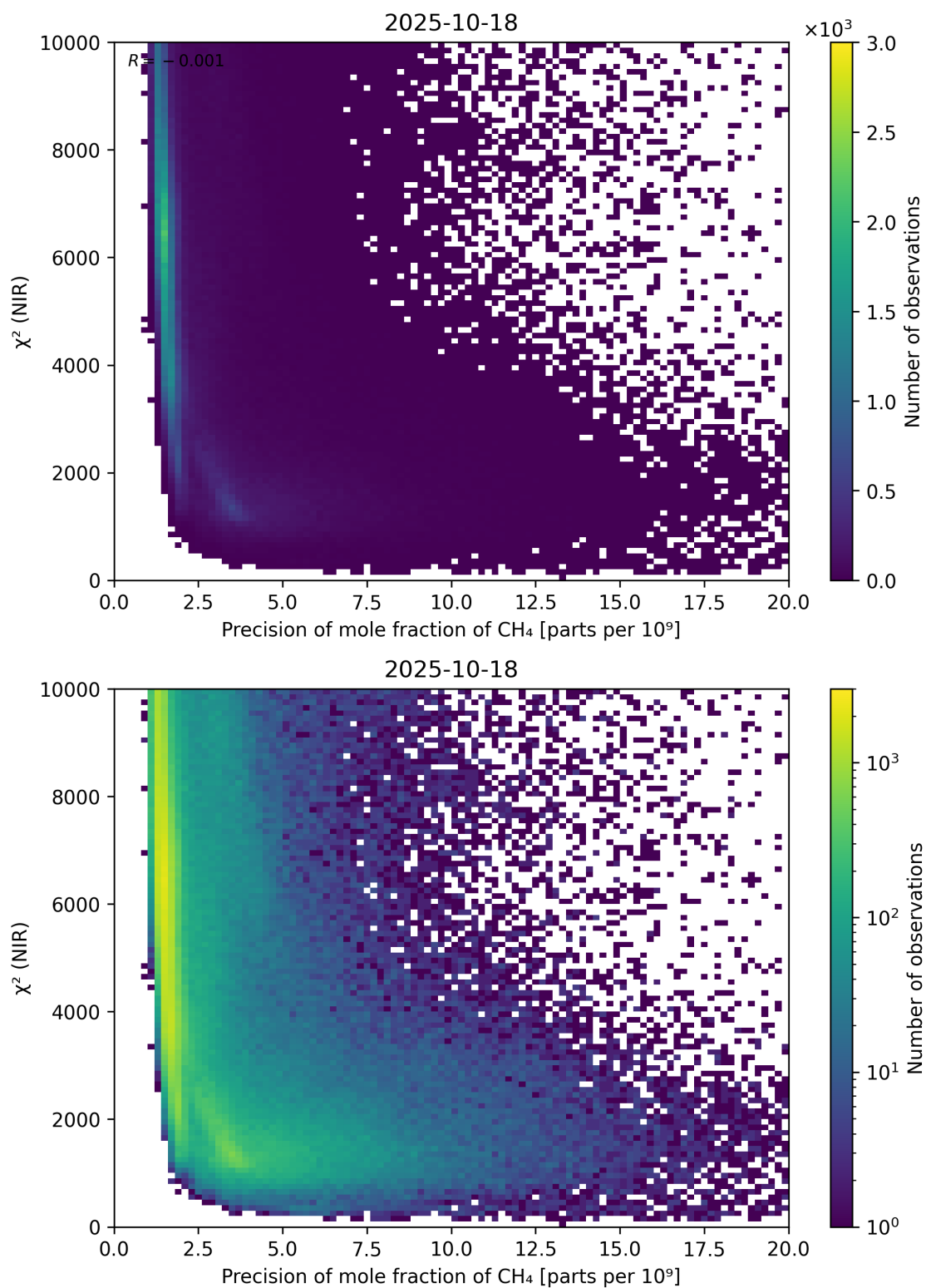
Figure 78: Scatter density plot of “Precision of mole fraction of CH 4 ” against “ \chi^2 (NIR)” for 2025-10-17 to 2025-10-19.
