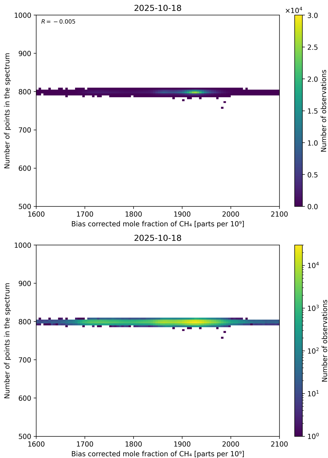
Figure 68: Scatter density plot of “Bias corrected mole fraction of CH 4 ” against “Number of points in the spectrum” for 2025-10-17 to 2025-10-19.
