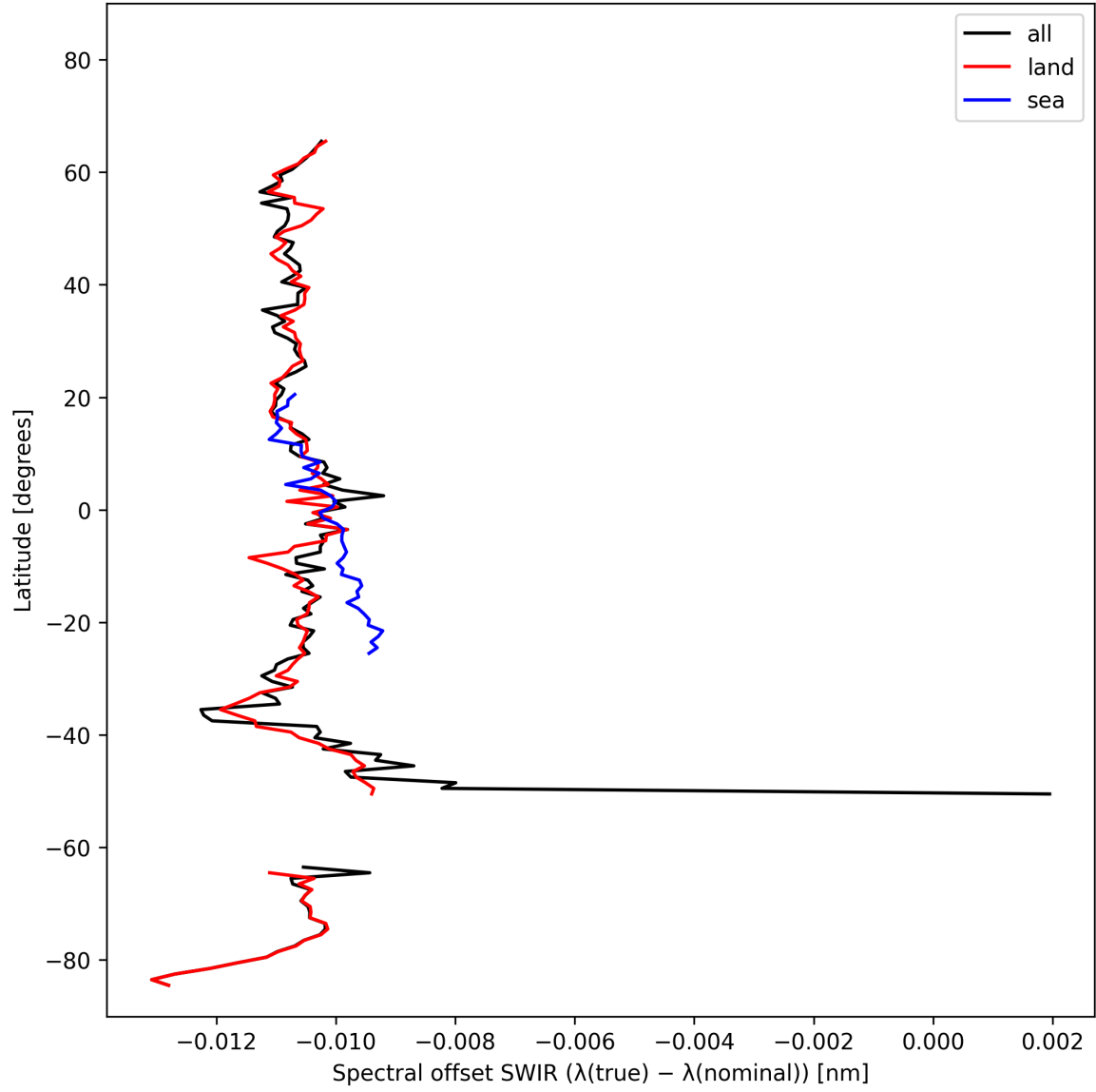
Figure 16: Zonal average of “Spectral offset SWIR ( \lambda_{\text{true}} - \lambda_{\text{nominal}} )” for 2025-10-17 to 2025-10-19.
