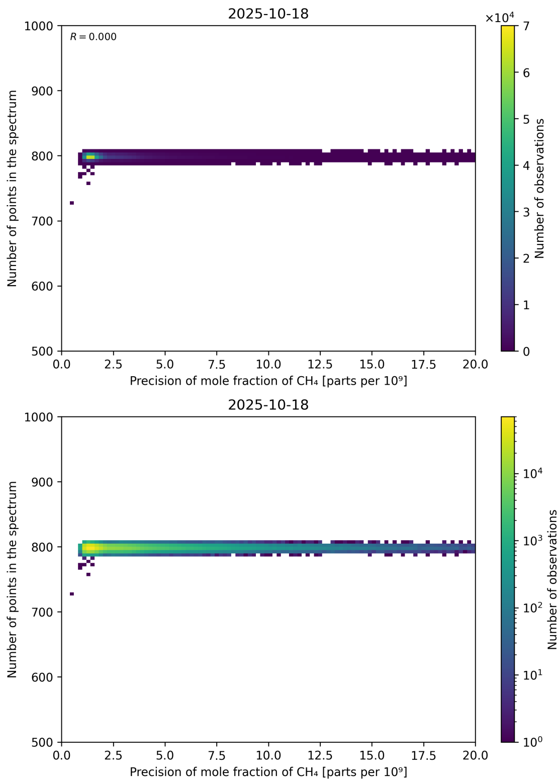
Figure 84: Scatter density plot of “Precision of mole fraction of CH 4 ” against “Number of points in the spectrum” for 2025-10-17 to 2025-10-19.
