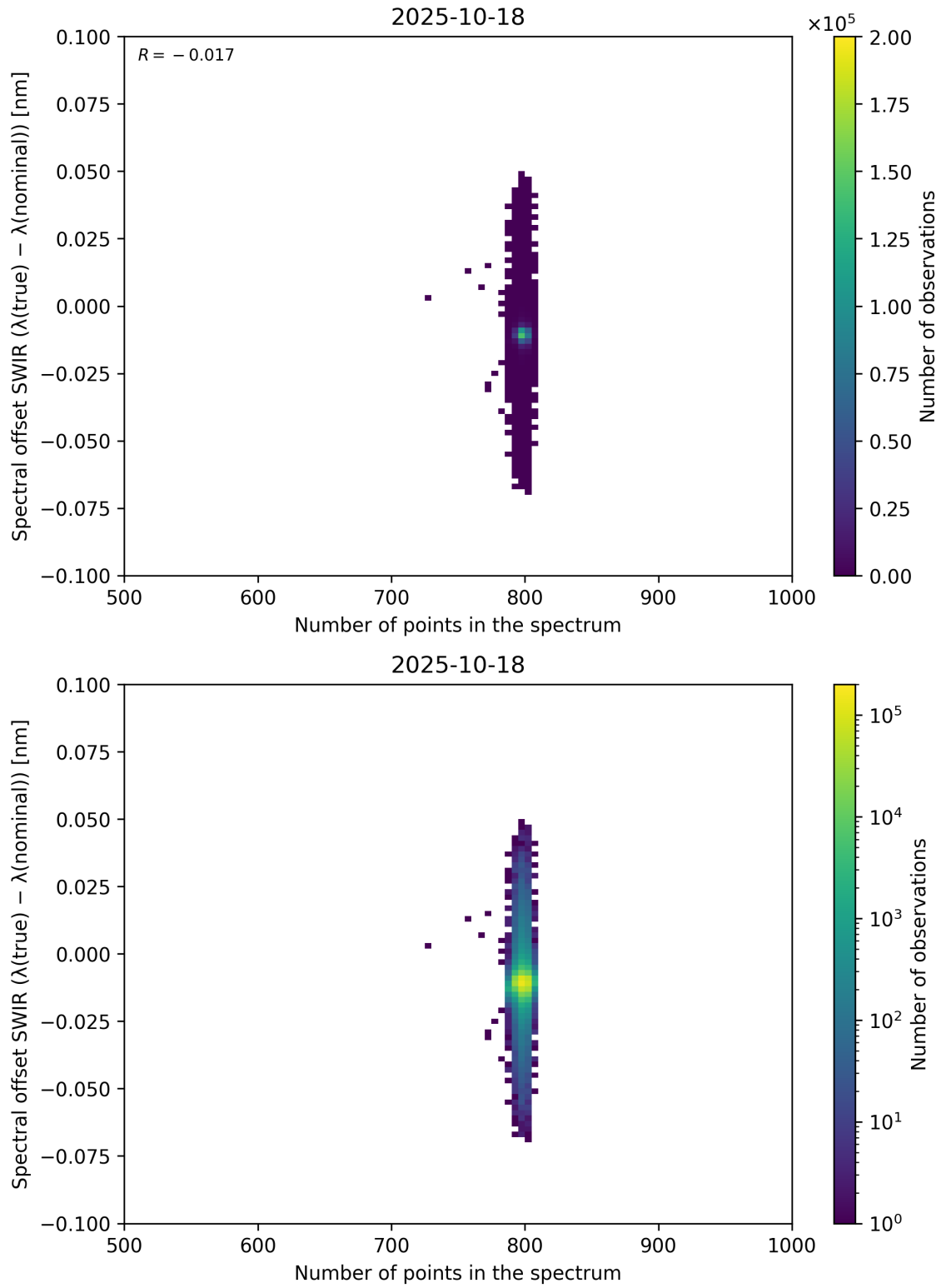
Figure 93: Scatter density plot of “Number of points in the spectrum” against “Spectral offset SWIR ( \lambda_{\text{true}} - \lambda_{\text{nominal}} )” for 2025-10-17 to 2025-10-19.
