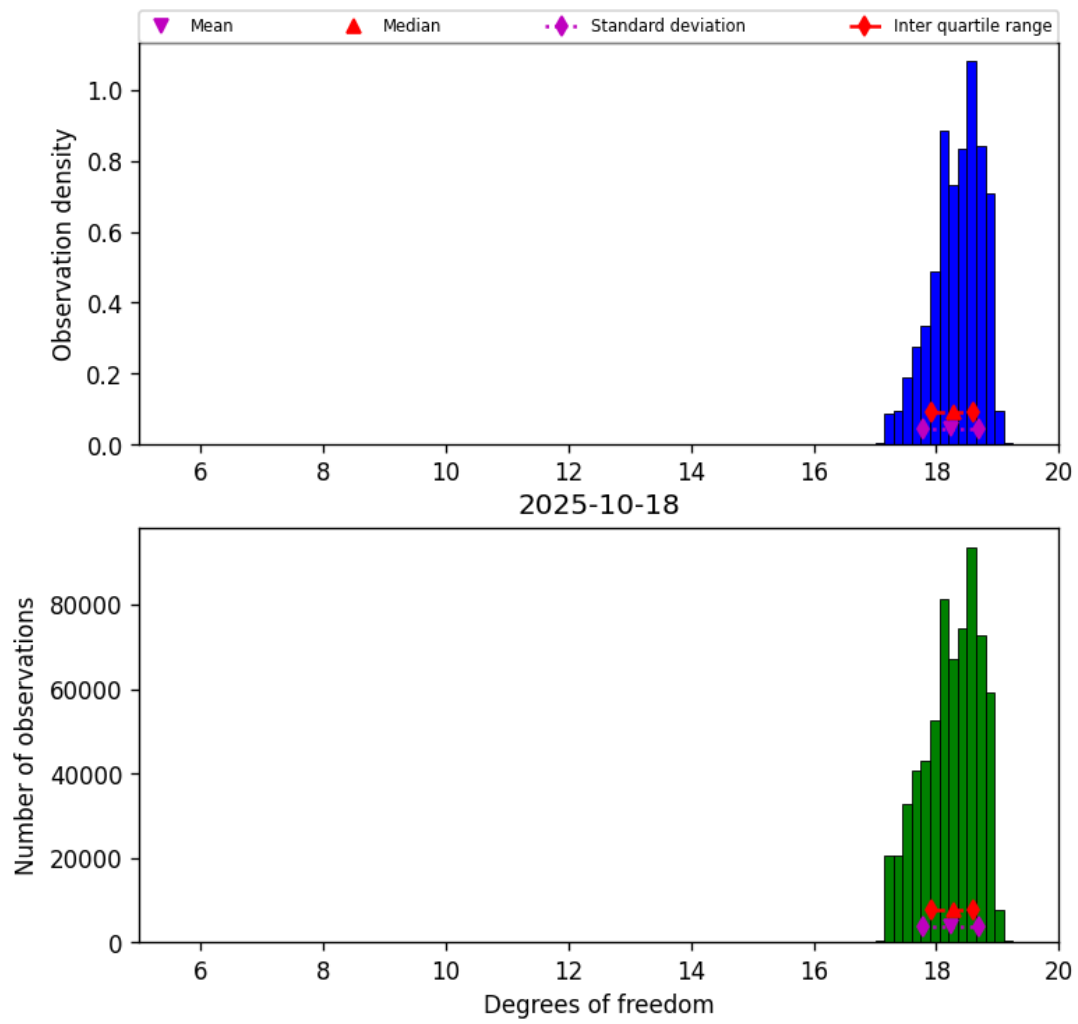
Figure 30: Histogram of “Degrees of freedom” for 2025-10-17 to 2025-10-19
