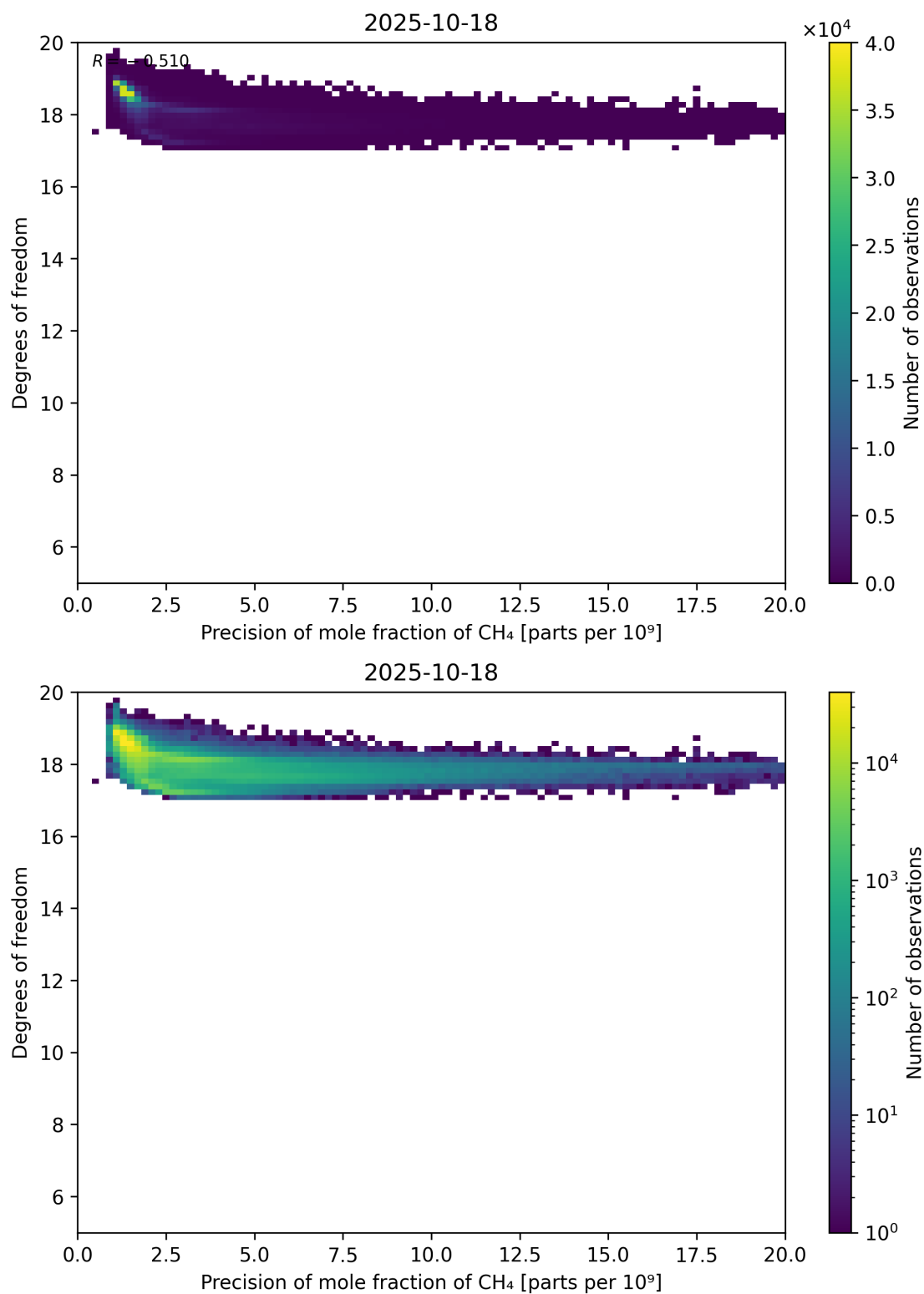
Figure 80: Scatter density plot of “Precision of mole fraction of CH 4 ” against “Degrees of freedom” for 2025-10-17 to 2025-10-19.
