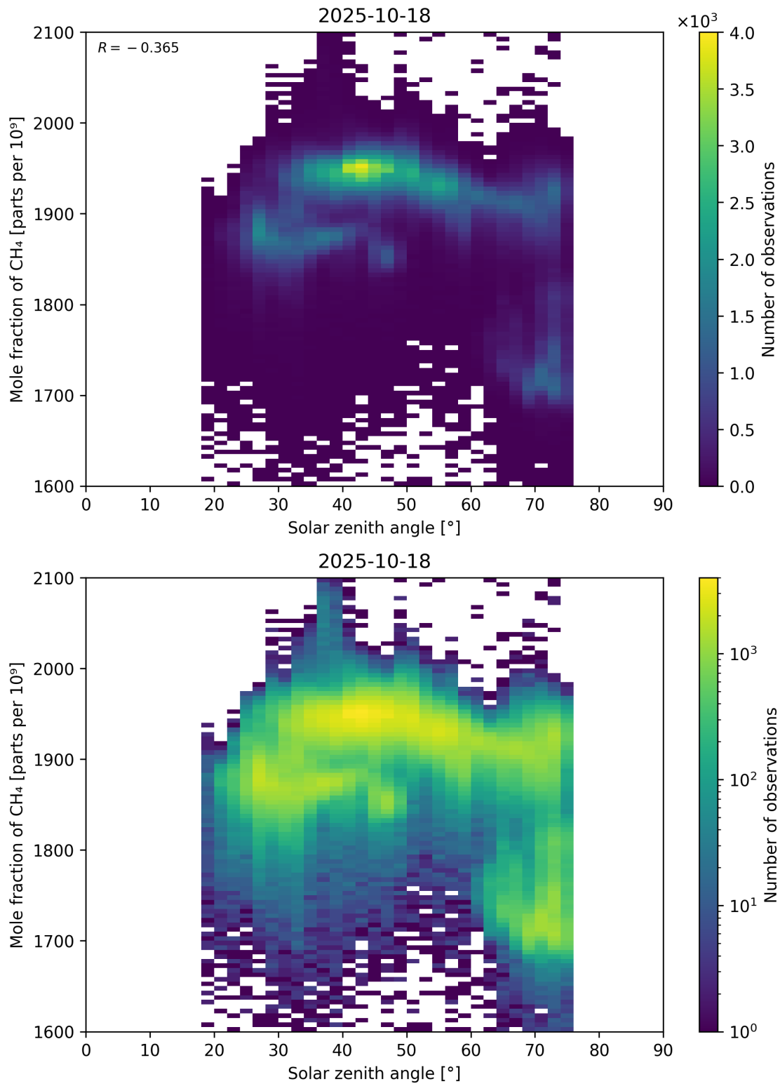
Figure 99: Scatter density plot of “Solar zenith angle” against “Mole fraction of \text{CH}_4 ” for 2025-10-17 to 2025-10-19.
