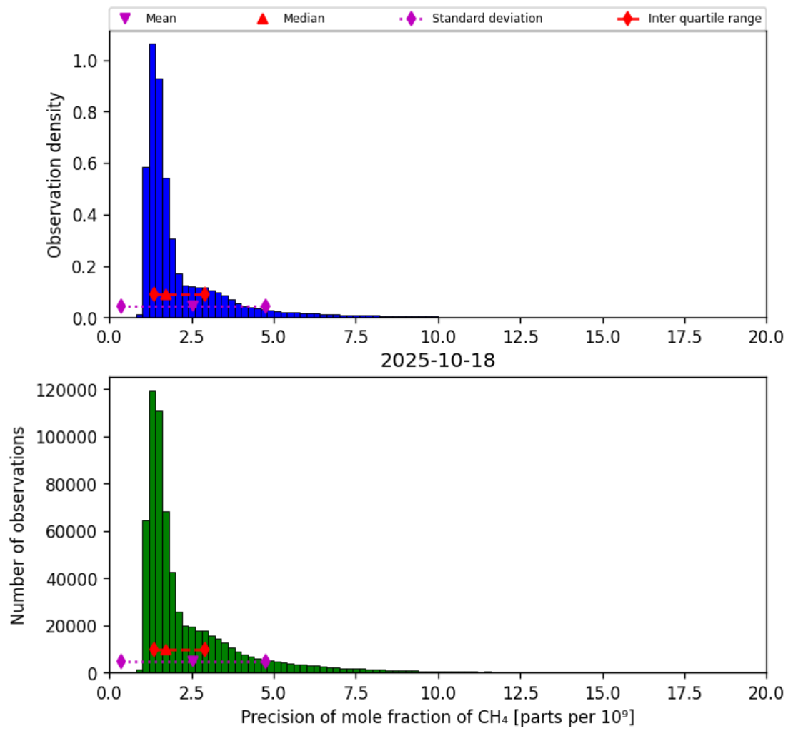
Figure 24: Histogram of “Precision of mole fraction of CH 4 ” for 2025-10-17 to 2025-10-19
