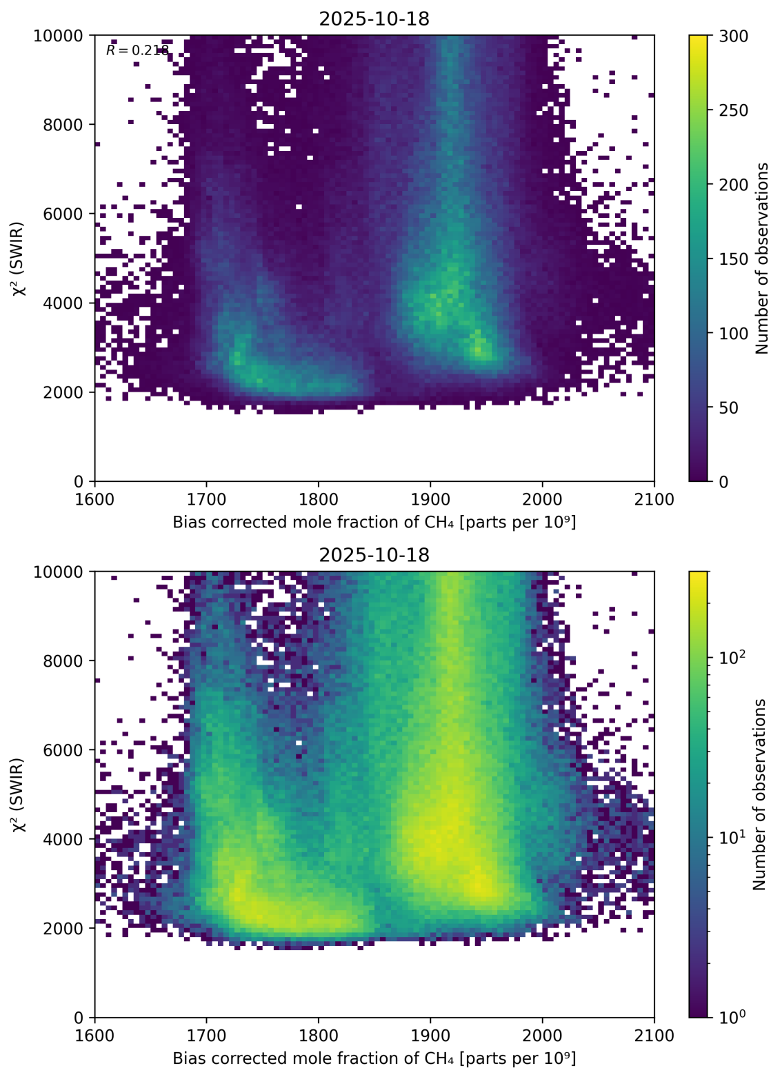
Figure 64: Scatter density plot of “Bias corrected mole fraction of CH 4 ” against “ \chi^2 (SWIR)” for 2025-10-17 to 2025-10-19.
