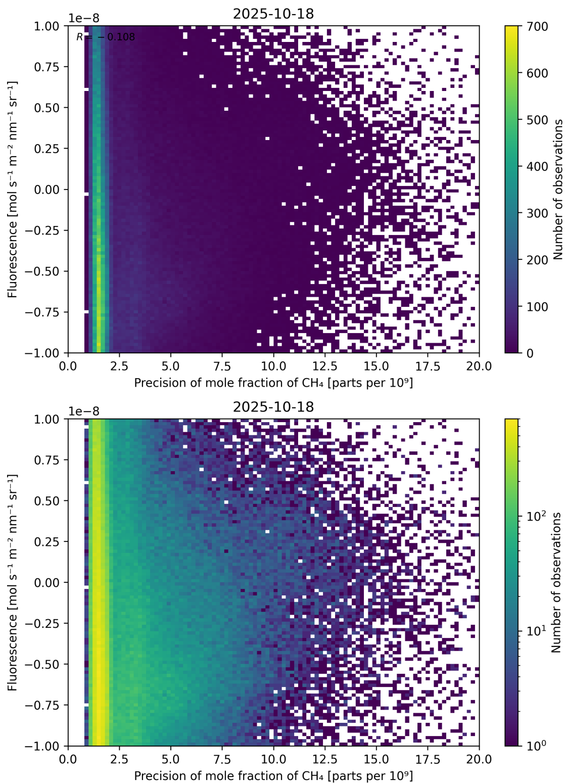
Figure 81: Scatter density plot of “Precision of mole fraction of CH 4 ” against “Fluorescence” for 2025-10-17 to 2025-10-19.
