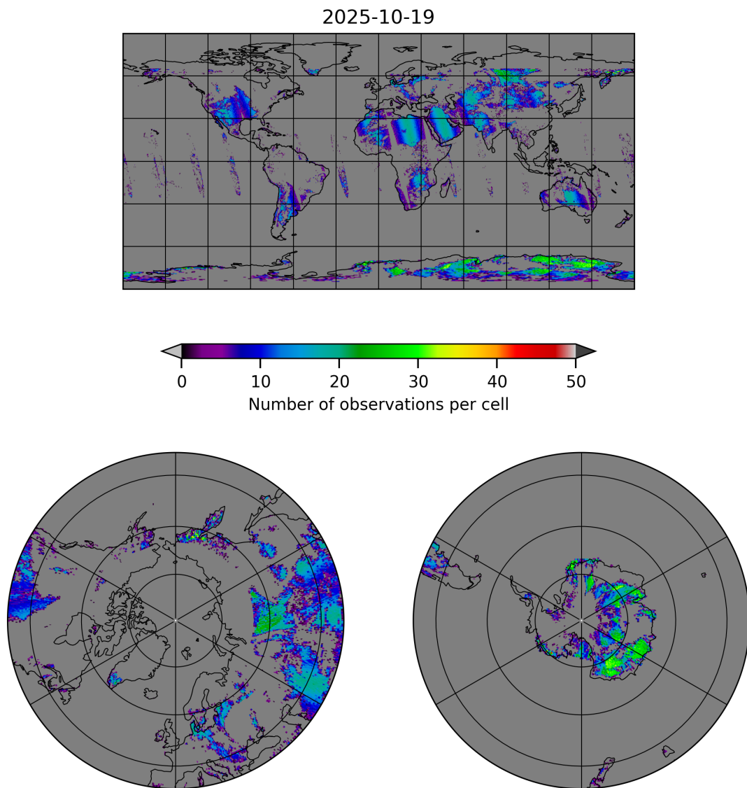
Figure 10: Map of the number of observations for 2025-10-18 to 2025-10-20
