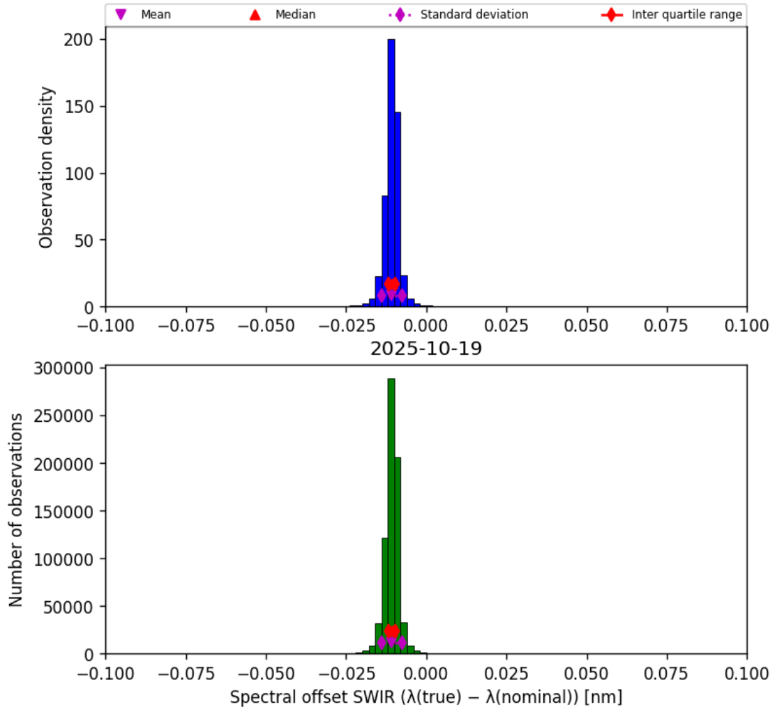
Figure 27: Histogram of “Spectral offset SWIR ( \lambda_{\text{true}} - \lambda_{\text{nominal}} )” for 2025-10-18 to 2025-10-20
