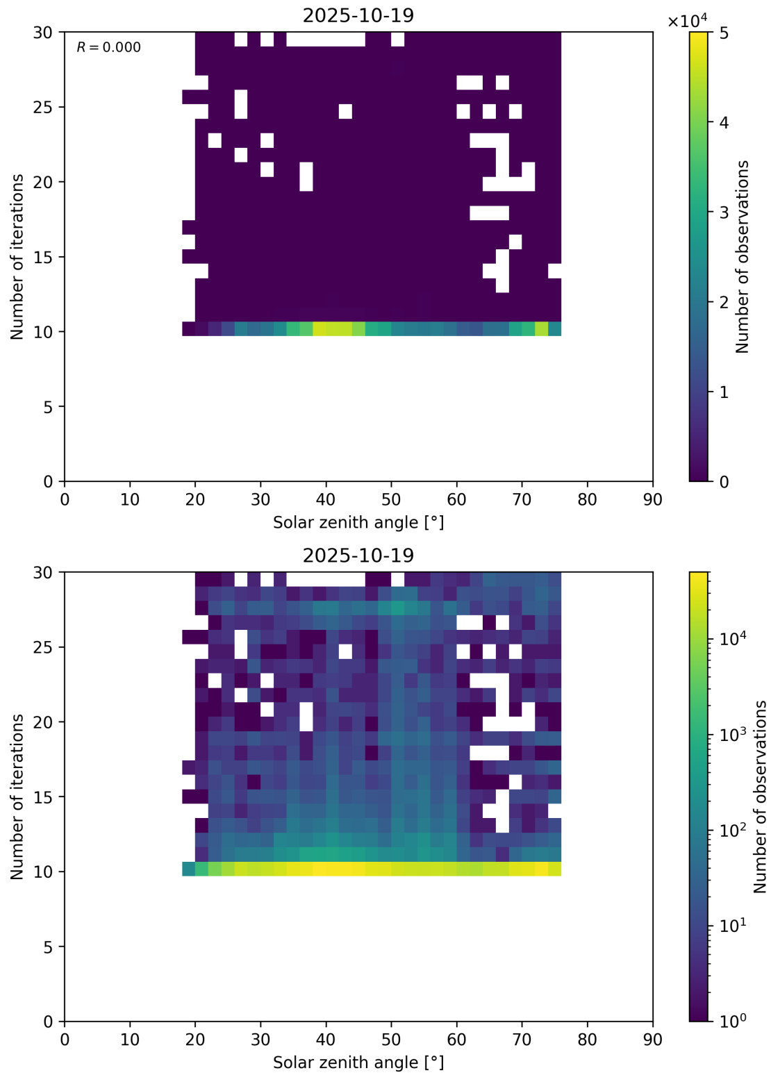
Figure 102: Scatter density plot of “Solar zenith angle” against “Number of iterations” for 2025-10-18 to 2025-10-20.
