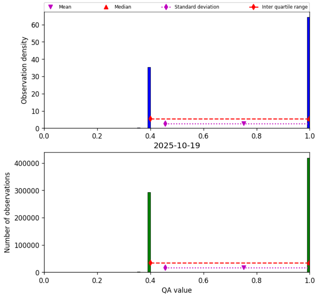
Figure 22: Histogram of “QA value” for 2025-10-18 to 2025-10-20
