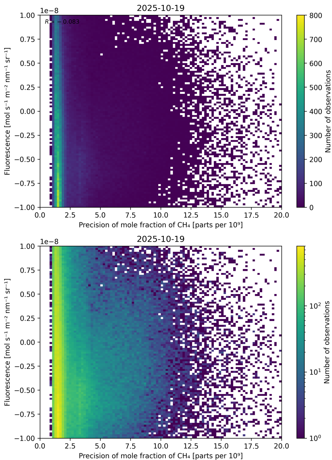
Figure 81: Scatter density plot of “Precision of mole fraction of CH 4 ” against “Fluorescence” for 2025-10-18 to 2025-10-20.
