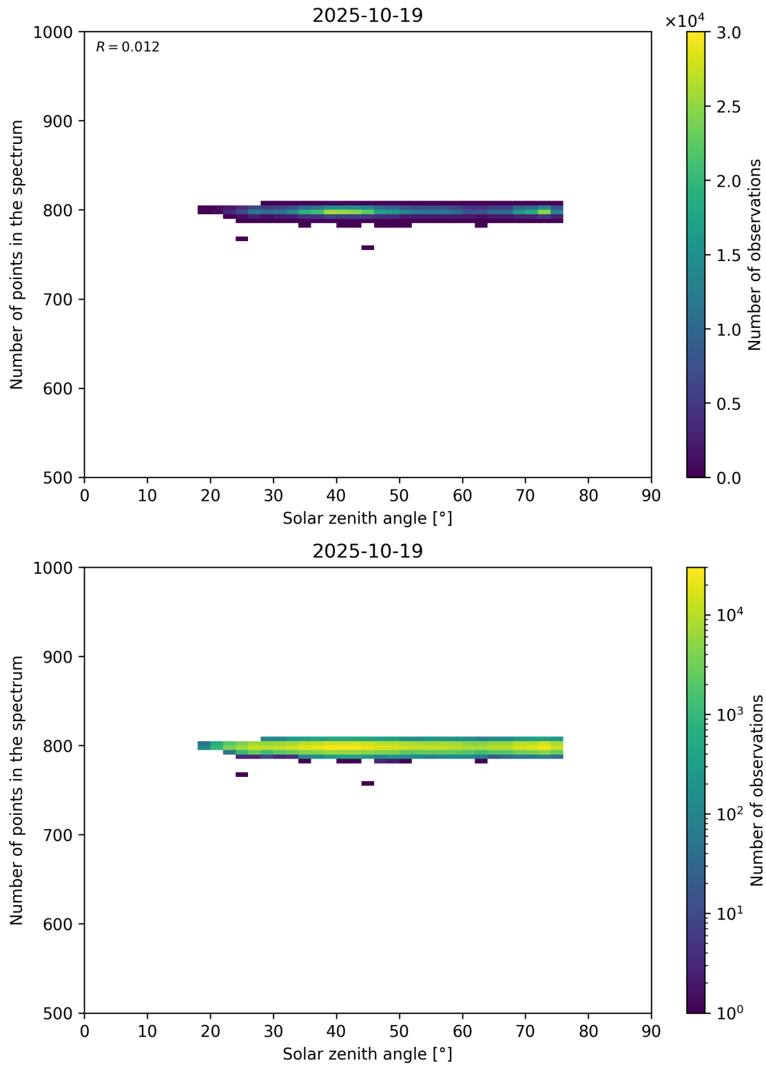
Figure 103: Scatter density plot of “Solar zenith angle” against “Number of points in the spectrum” for 2025-10-18 to 2025-10-20.
