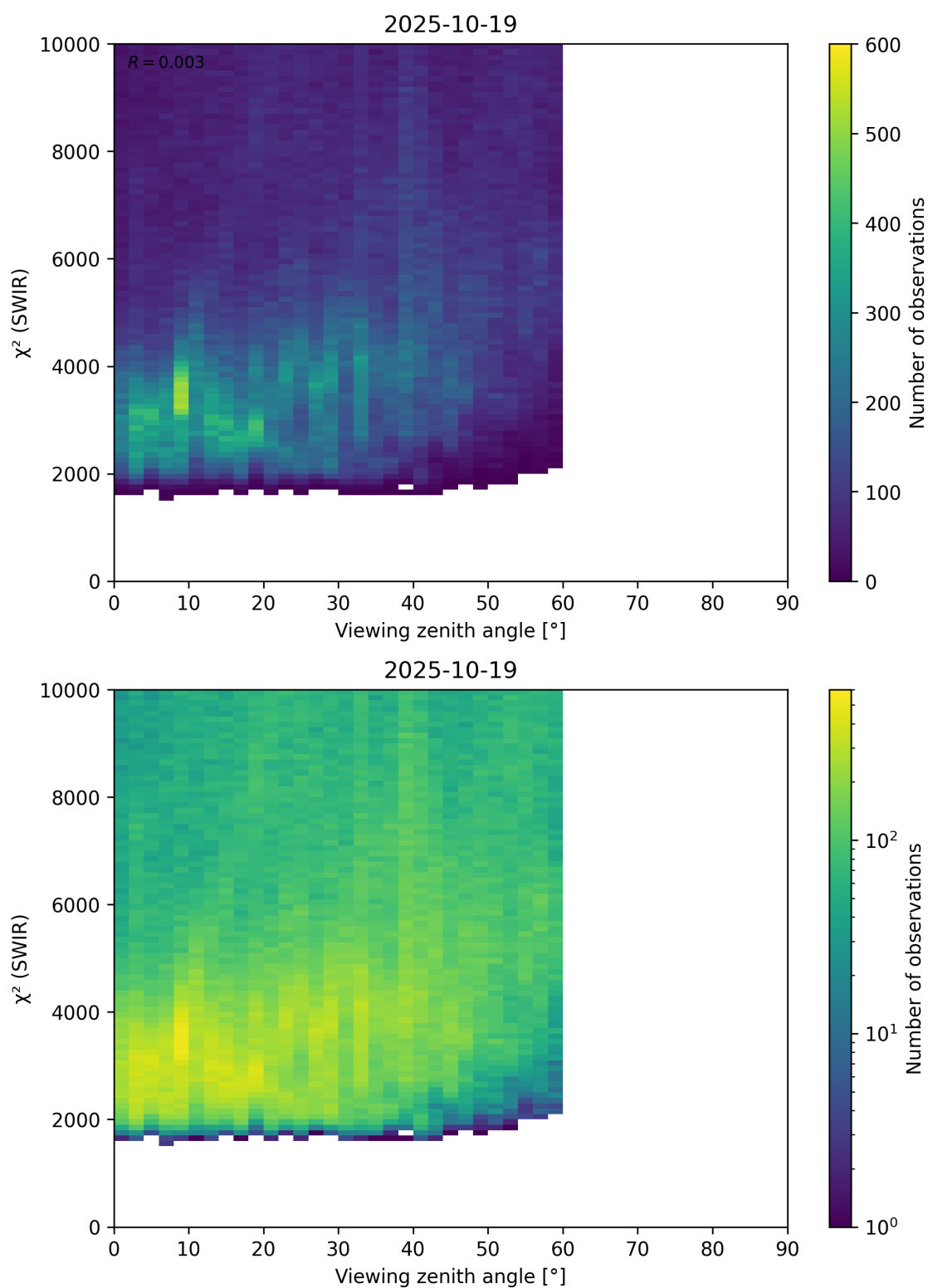
Figure 106: Scatter density plot of “Viewing zenith angle” against “ \chi^2 (SWIR)” for 2025-10-18 to 2025-10-20.
