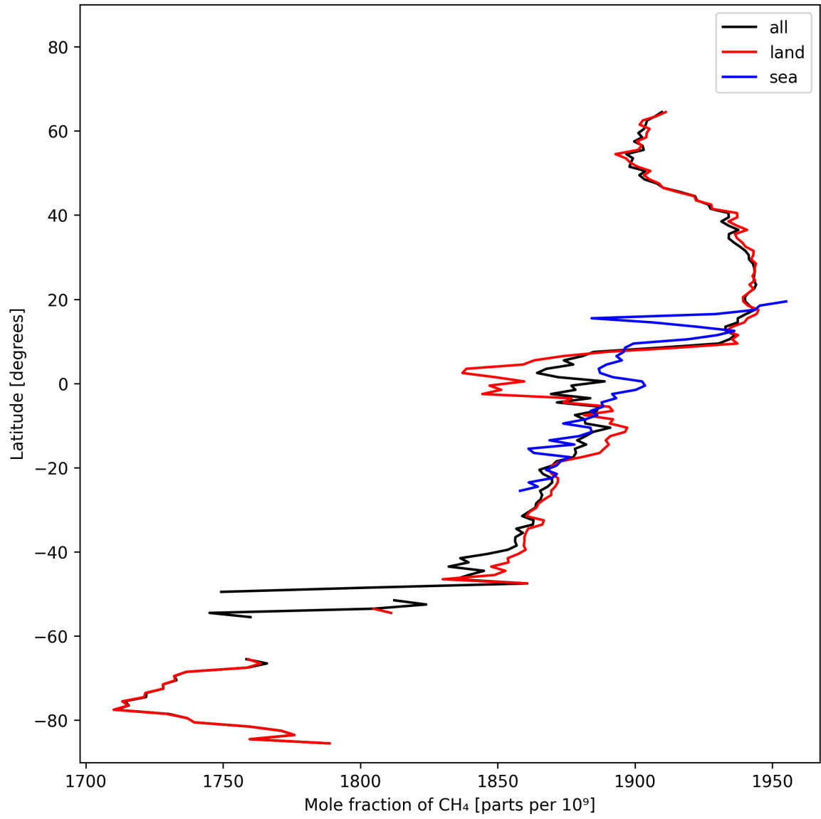
Figure 12: Zonal average of “Mole fraction of CH 4 ” for 2025-10-18 to 2025-10-20.
