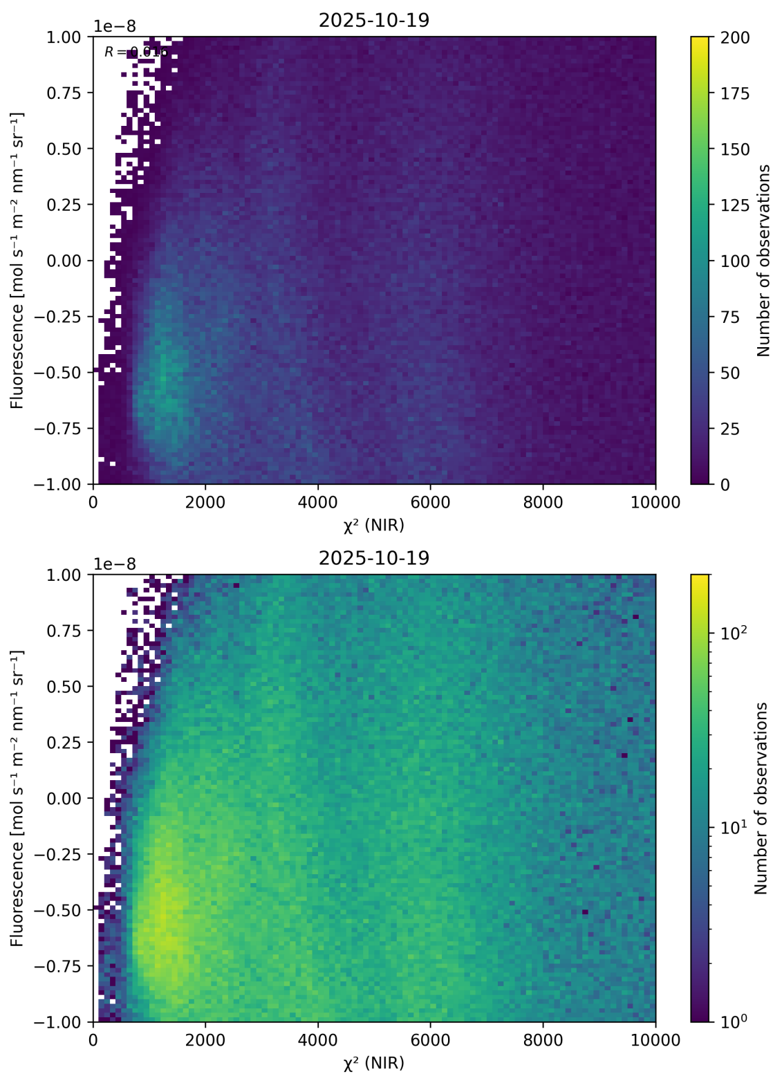
Figure 45: Scatter density plot of “ \chi^2 (NIR)” against “Fluorescence” for 2025-10-18 to 2025-10-20.
