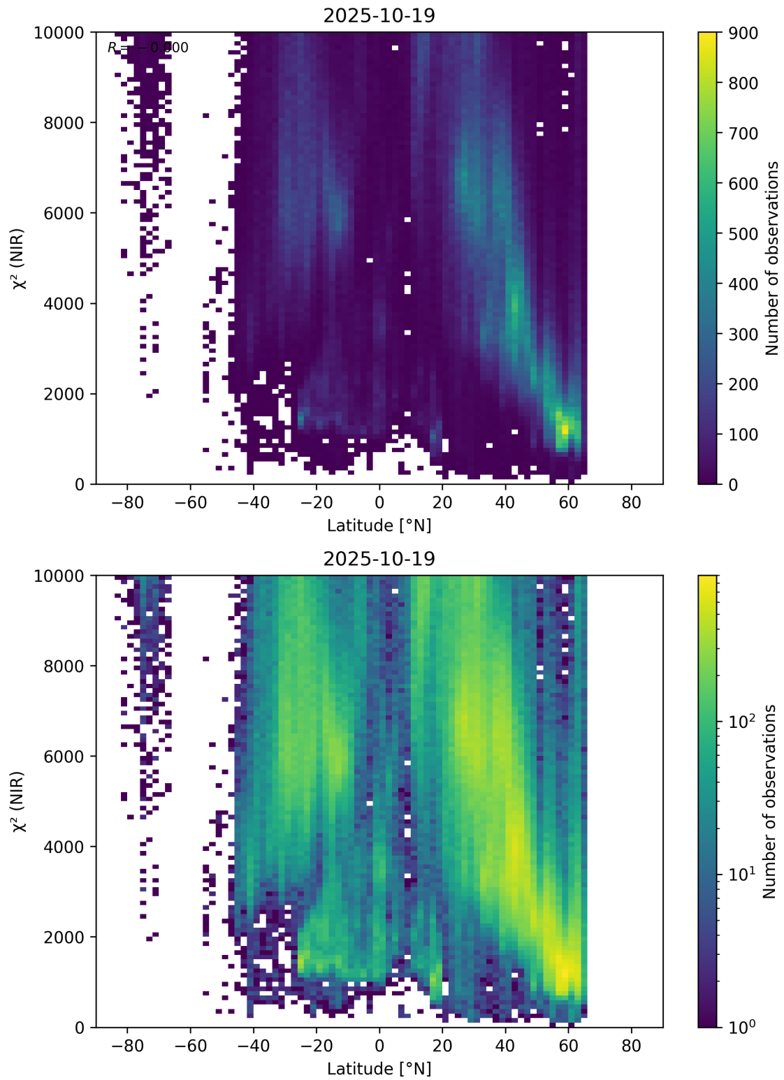
Figure 53: Scatter density plot of “Latitude” against “ \chi^2 (NIR)” for 2025-10-18 to 2025-10-20.
