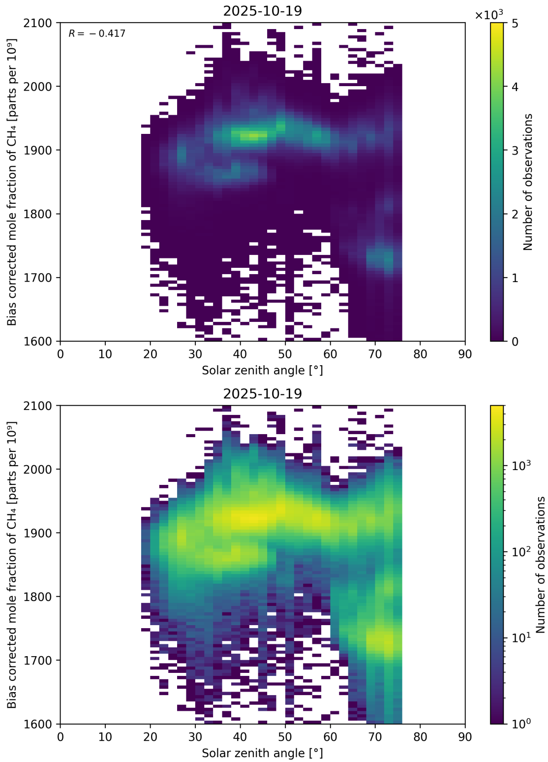
Figure 100: Scatter density plot of “Solar zenith angle” against “Bias corrected mole fraction of \text{CH}_4 ” for 2025-10-18 to 2025-10-20.
