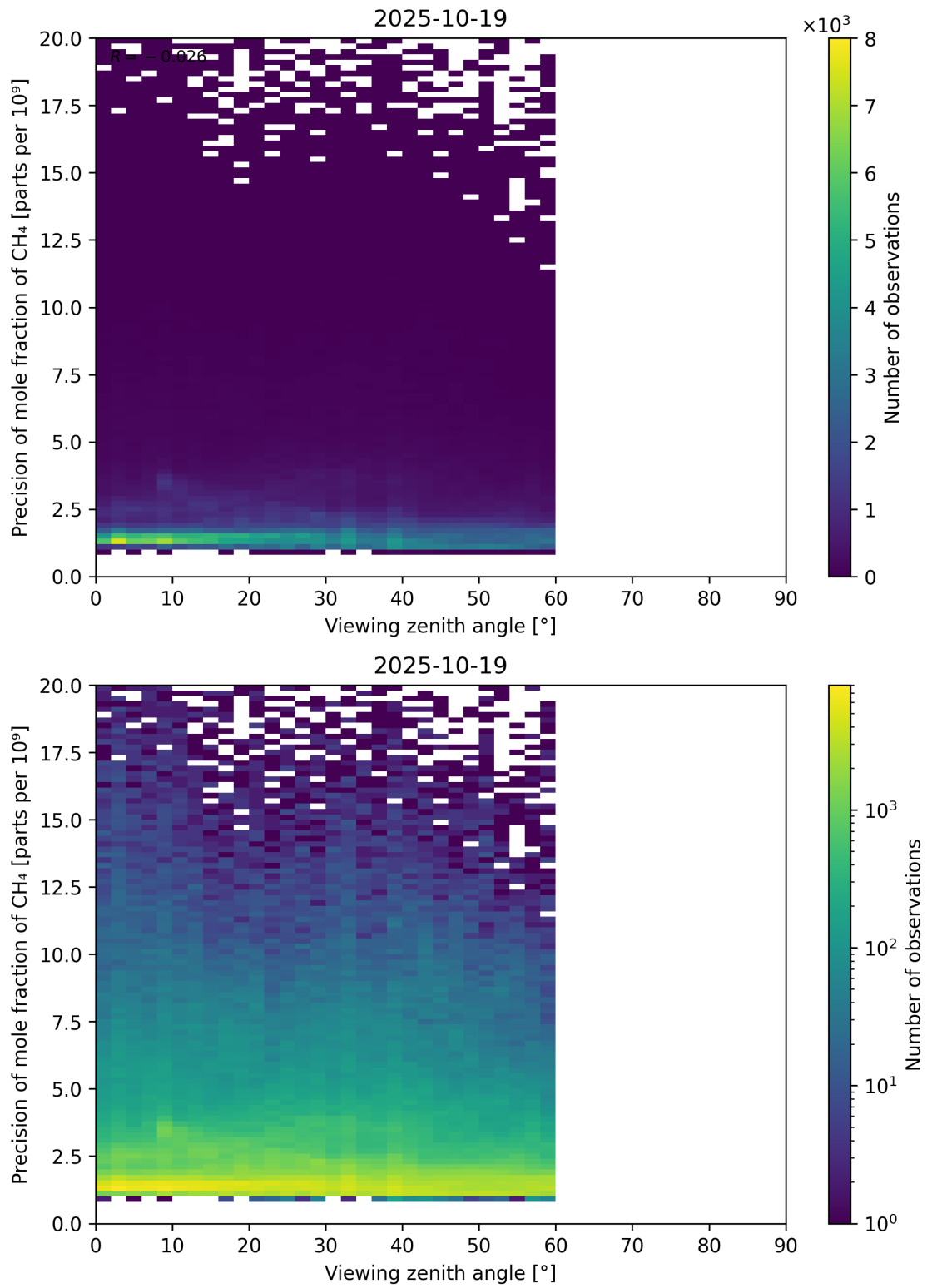
Figure 112: Scatter density plot of “Viewing zenith angle” against “Precision of mole fraction of CH 4 ” for 2025-10-18 to 2025-10-20.
