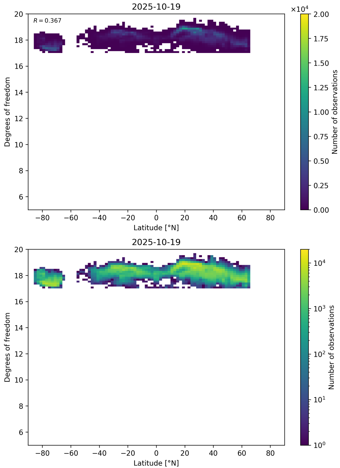
Figure 55: Scatter density plot of “Latitude” against “Degrees of freedom” for 2025-10-18 to 2025-10-20.
