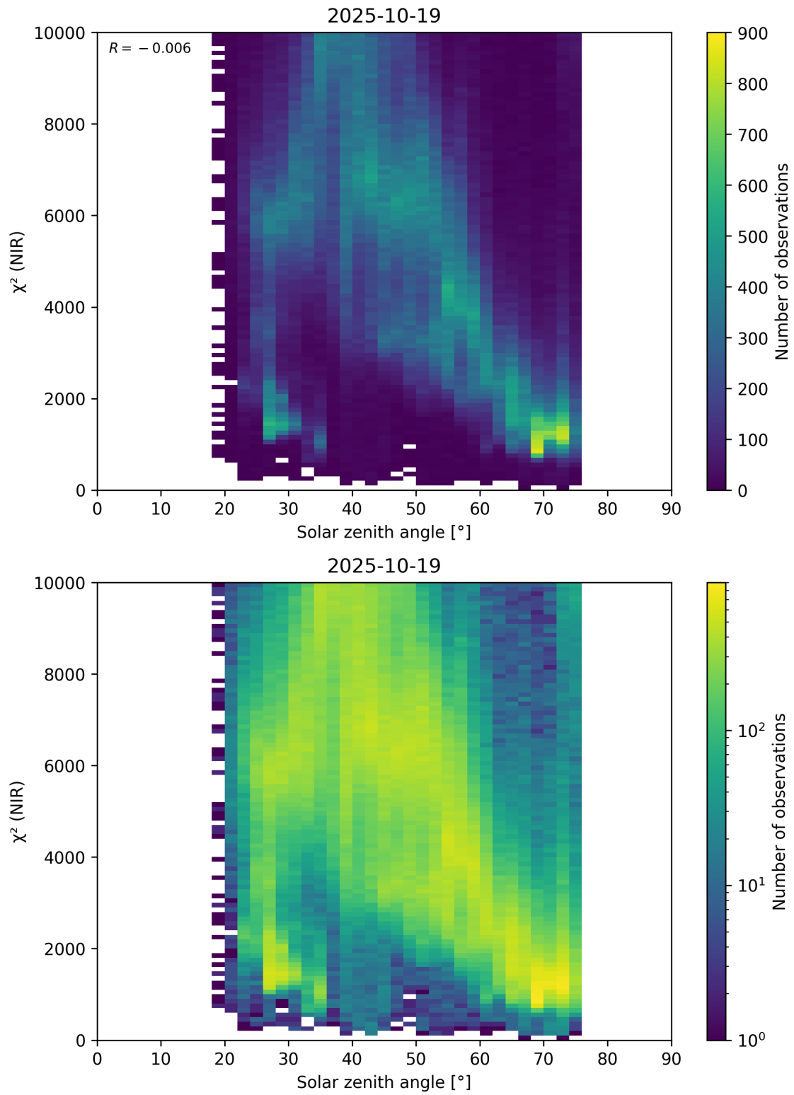
Figure 94: Scatter density plot of “Solar zenith angle” against “ \chi^2 (NIR)” for 2025-10-18 to 2025-10-20.
