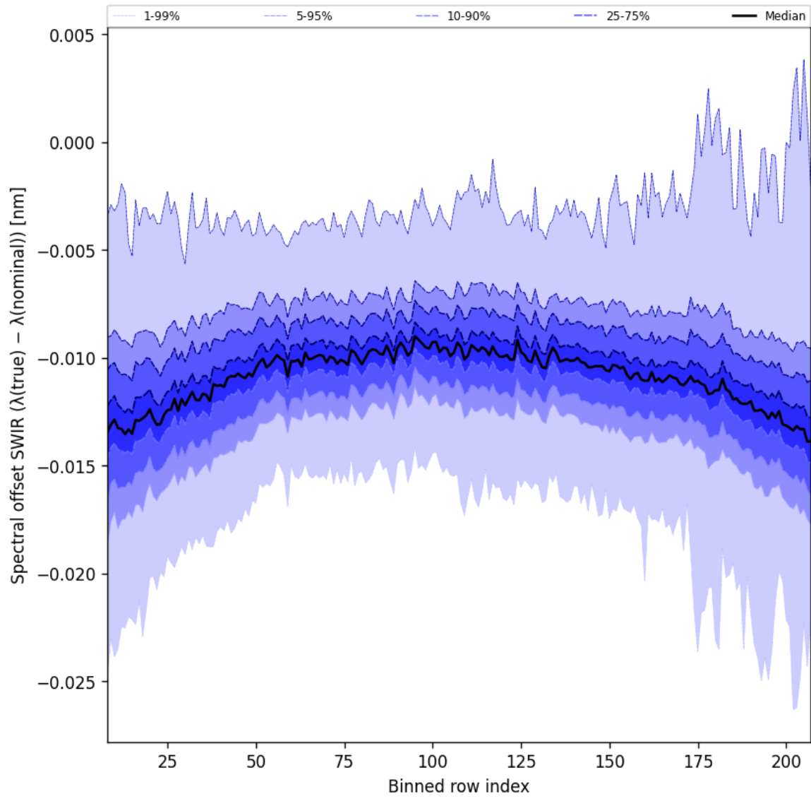
Figure 38: Along track statistics of “Spectral offset SWIR ( \lambda_{\text{true}} - \lambda_{\text{nominal}} )” for 2025-10-18 to 2025-10-20
