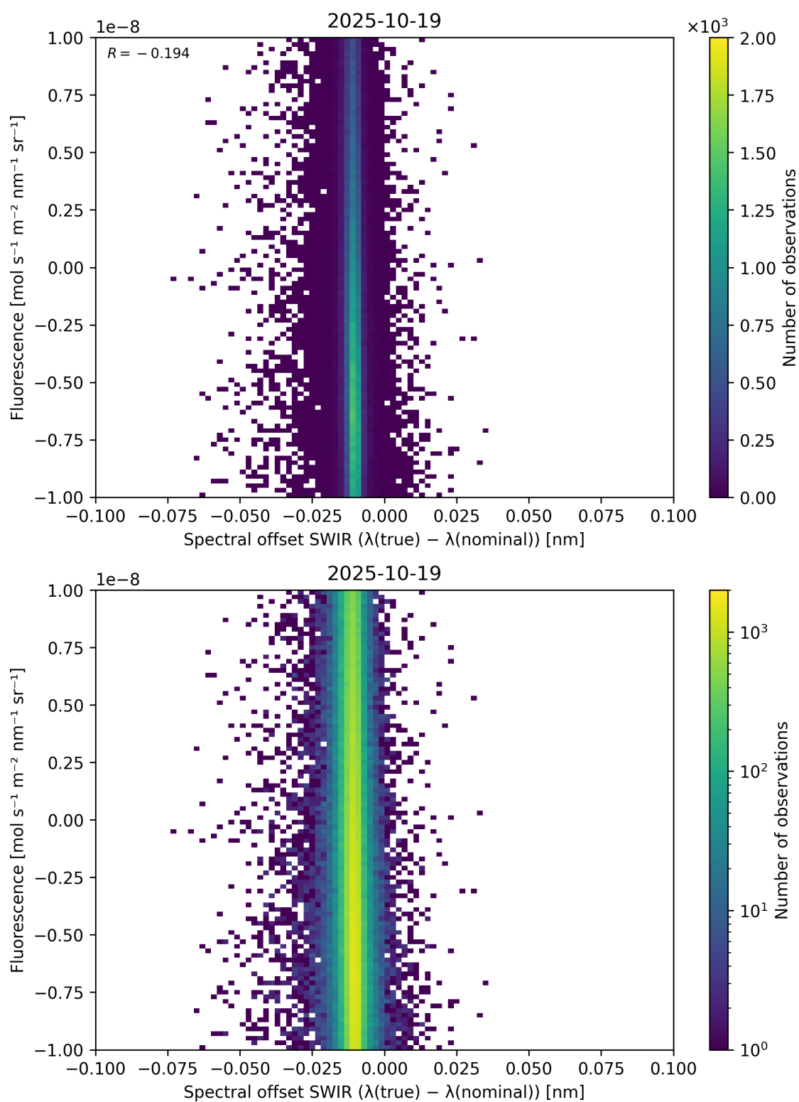
Figure 120: Scatter density plot of “Spectral offset SWIR ( \lambda_{\text{true}} - \lambda_{\text{nominal}} )” against “Fluorescence” for 2025-10-18 to 2025-10-20.
