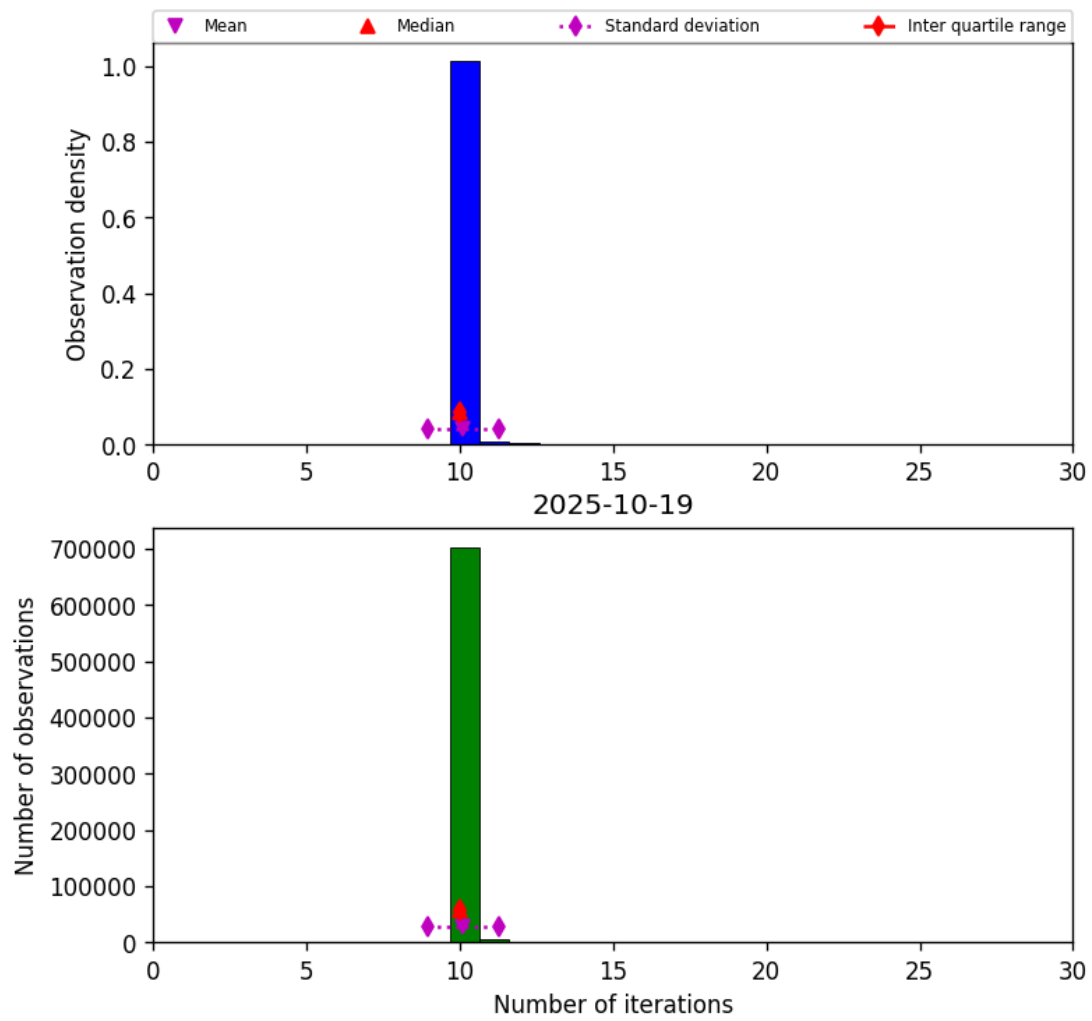
Figure 31: Histogram of “Number of iterations” for 2025-10-18 to 2025-10-20
