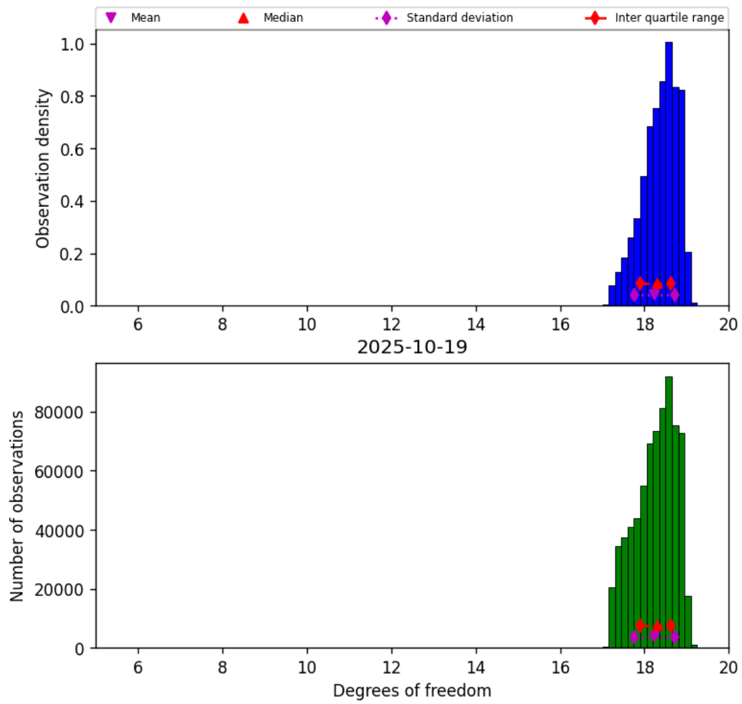
Figure 30: Histogram of “Degrees of freedom” for 2025-10-18 to 2025-10-20
