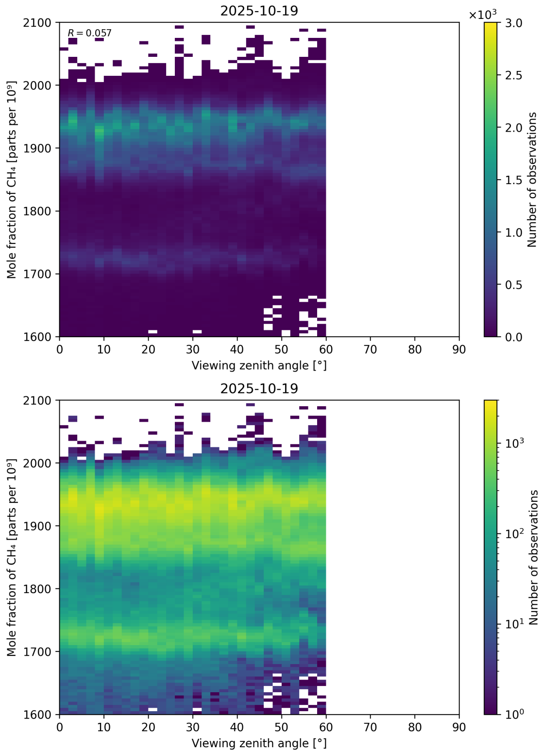
Figure 110: Scatter density plot of “Viewing zenith angle” against “Mole fraction of CH 4 ” for 2025-10-18 to 2025-10-20.
