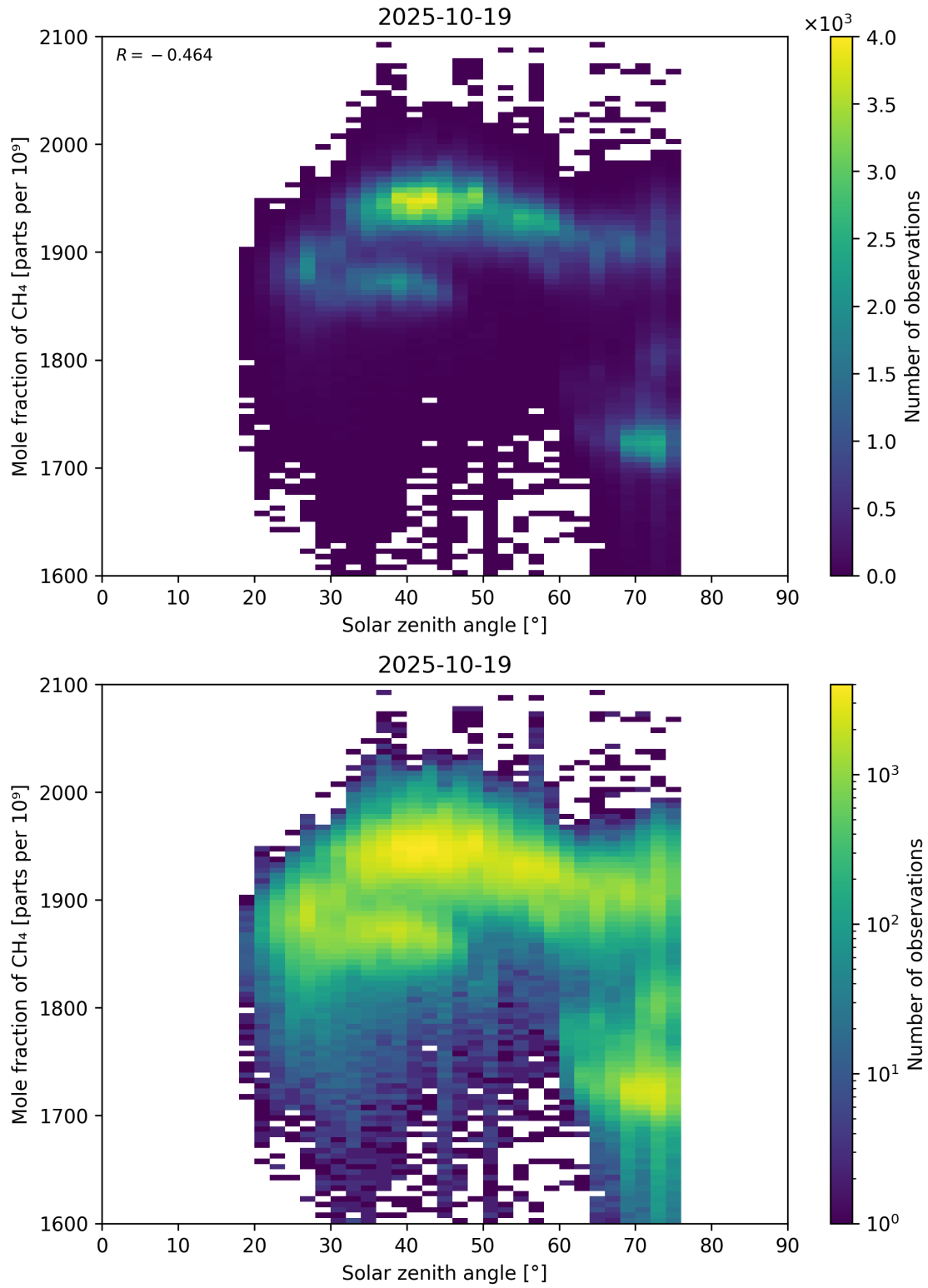
Figure 99: Scatter density plot of “Solar zenith angle” against “Mole fraction of CH 4 ” for 2025-10-18 to 2025-10-20.
