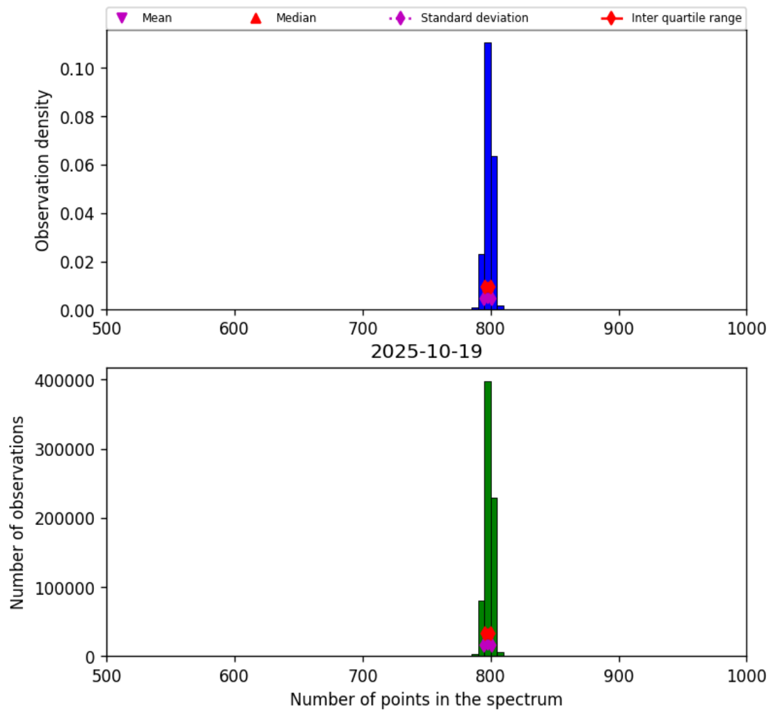
Figure 26: Histogram of “Number of points in the spectrum” for 2025-10-18 to 2025-10-20
