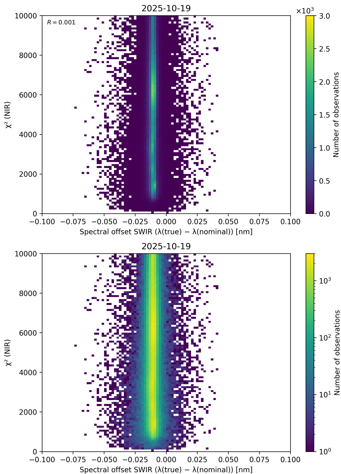
Figure 117: Scatter density plot of “Spectral offset SWIR ( \lambda_{\text{true}} - \lambda_{\text{nominal}} )” against “ \chi^2 (NIR)” for 2025-10-18 to 2025-10-20.
