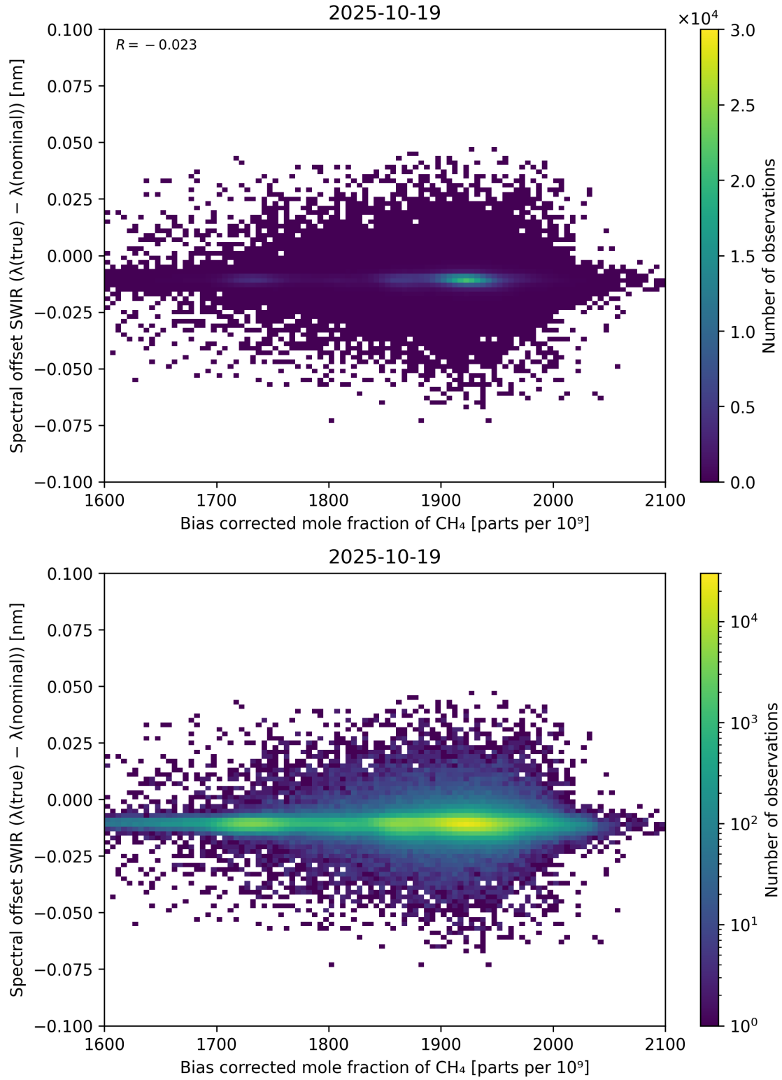
Figure 69: Scatter density plot of “Bias corrected mole fraction of CH 4 ” against “Spectral offset SWIR ( \lambda_{\text{true}} - \lambda_{\text{nominal}} )” for 2025-10-18 to 2025-10-20.
