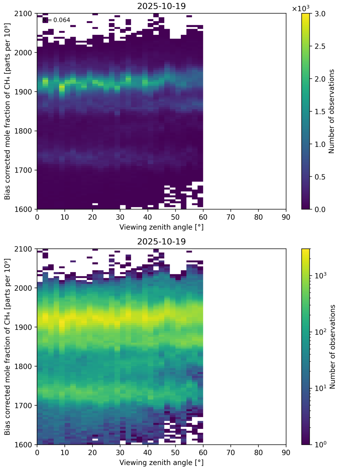
Figure 111: Scatter density plot of “Viewing zenith angle” against “Bias corrected mole fraction of CH 4 ” for 2025-10-18 to 2025-10-20.
