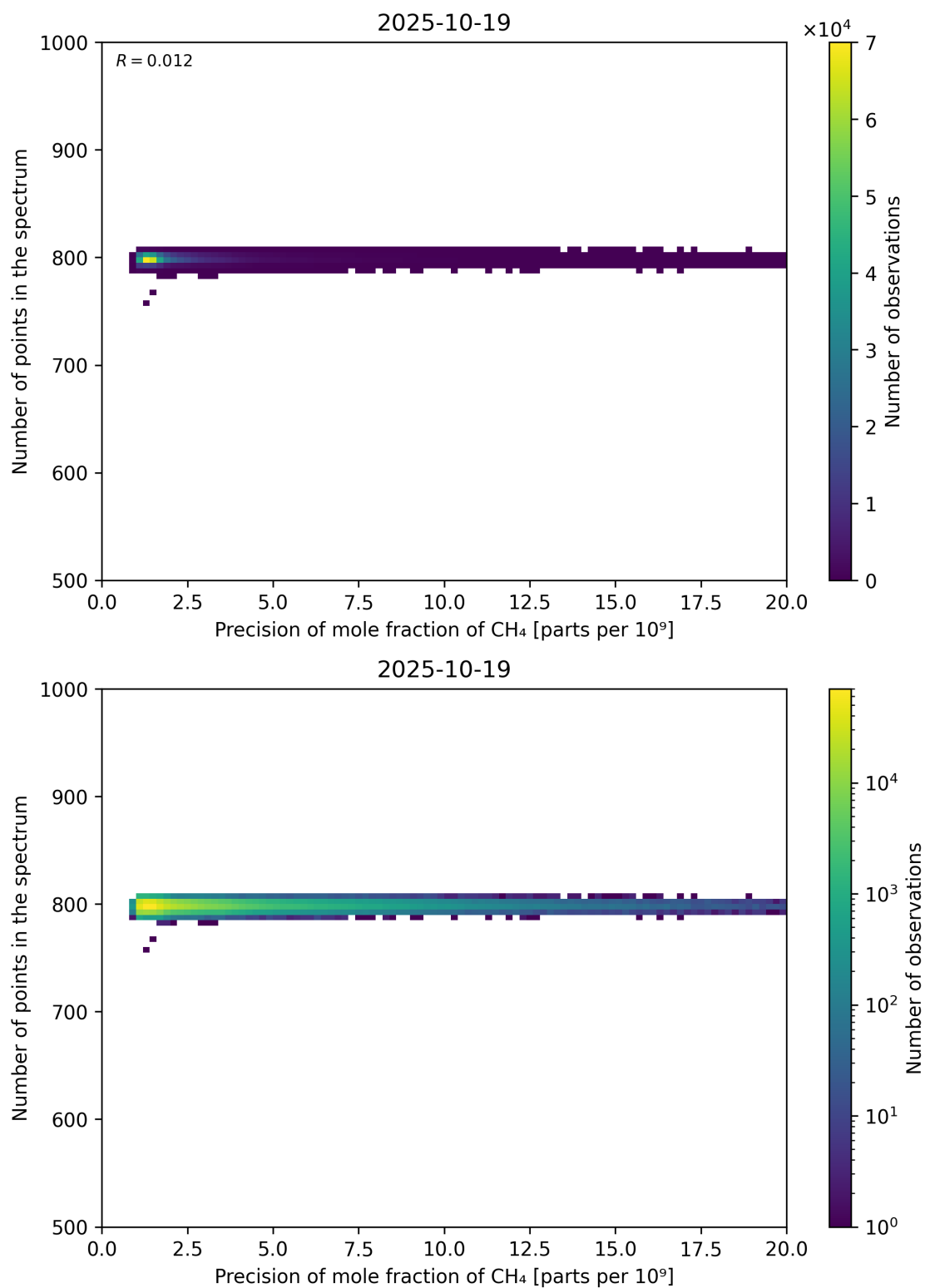
Figure 84: Scatter density plot of “Precision of mole fraction of CH 4 ” against “Number of points in the spectrum” for 2025-10-18 to 2025-10-20.
