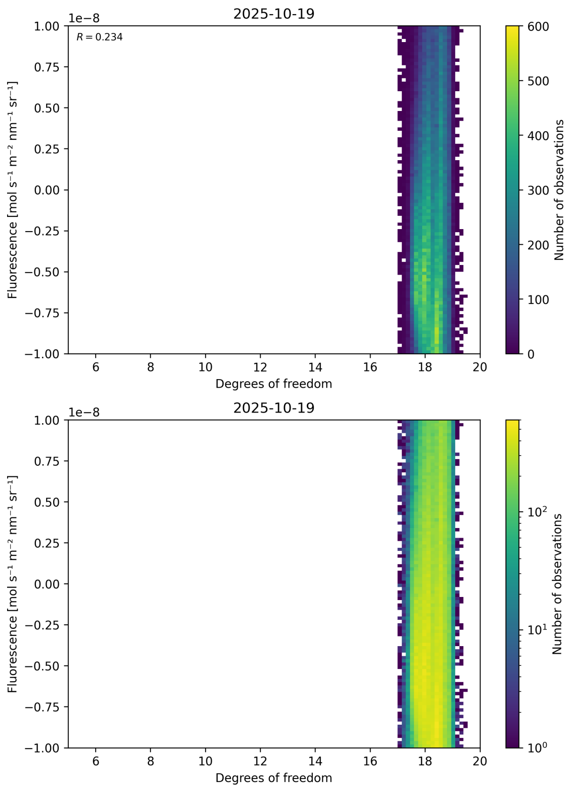
Figure 51: Scatter density plot of “Degrees of freedom” against “Fluorescence” for 2025-10-18 to 2025-10-20.
