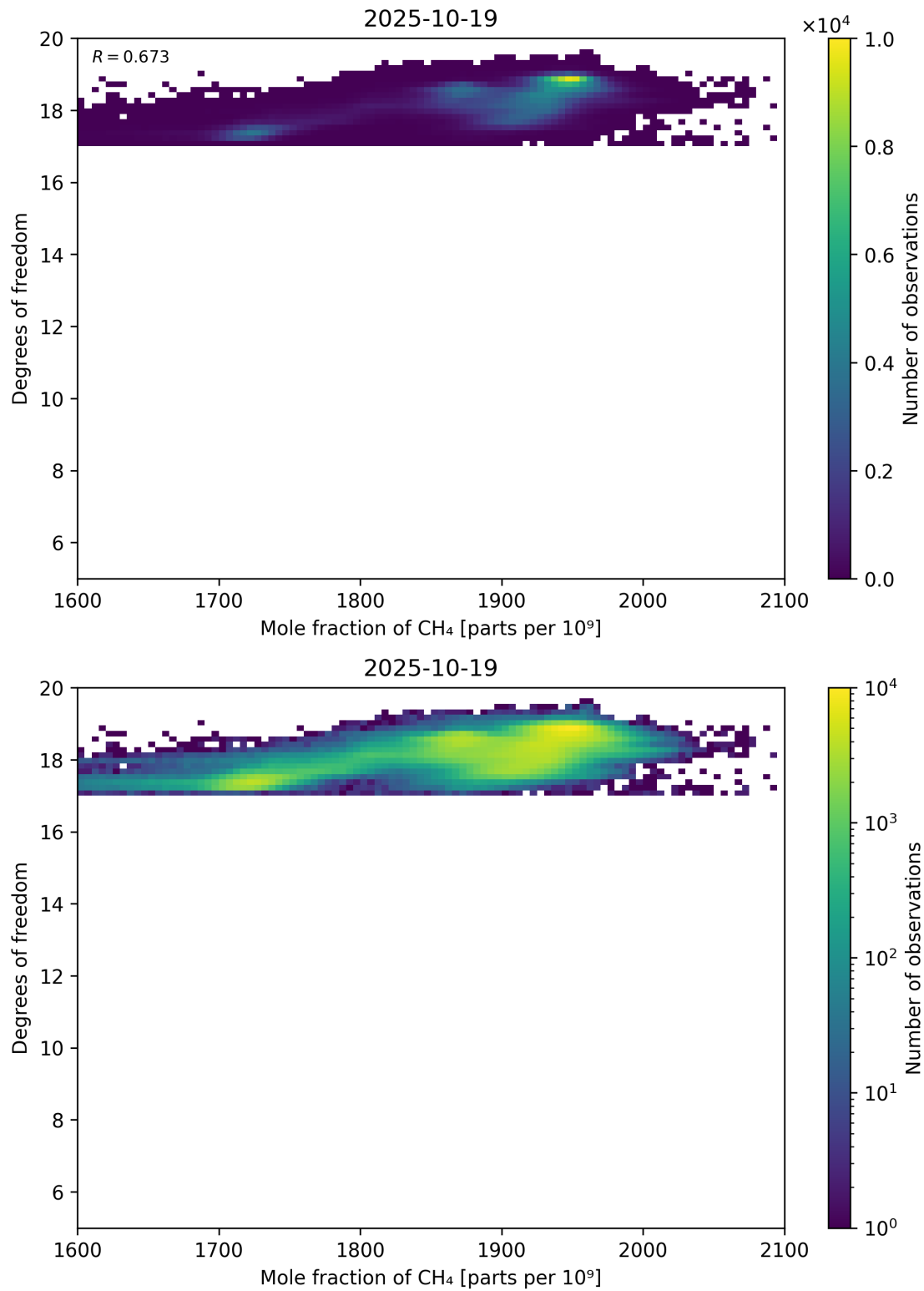
Figure 72: Scatter density plot of “Mole fraction of CH 4 ” against “Degrees of freedom” for 2025-10-18 to 2025-10-20.
