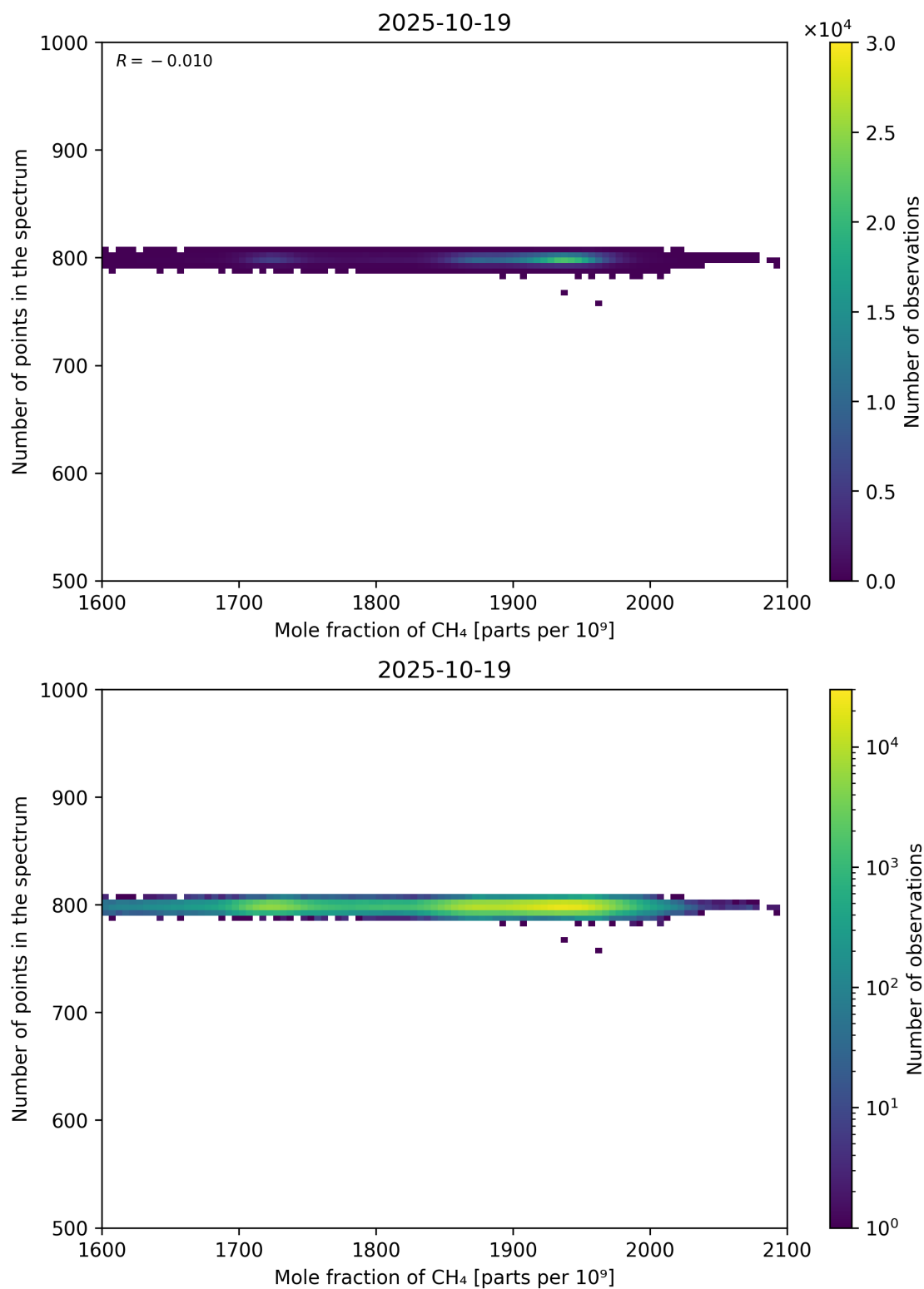
Figure 77: Scatter density plot of “Mole fraction of CH 4 ” against “Number of points in the spectrum” for 2025-10-18 to 2025-10-20.
