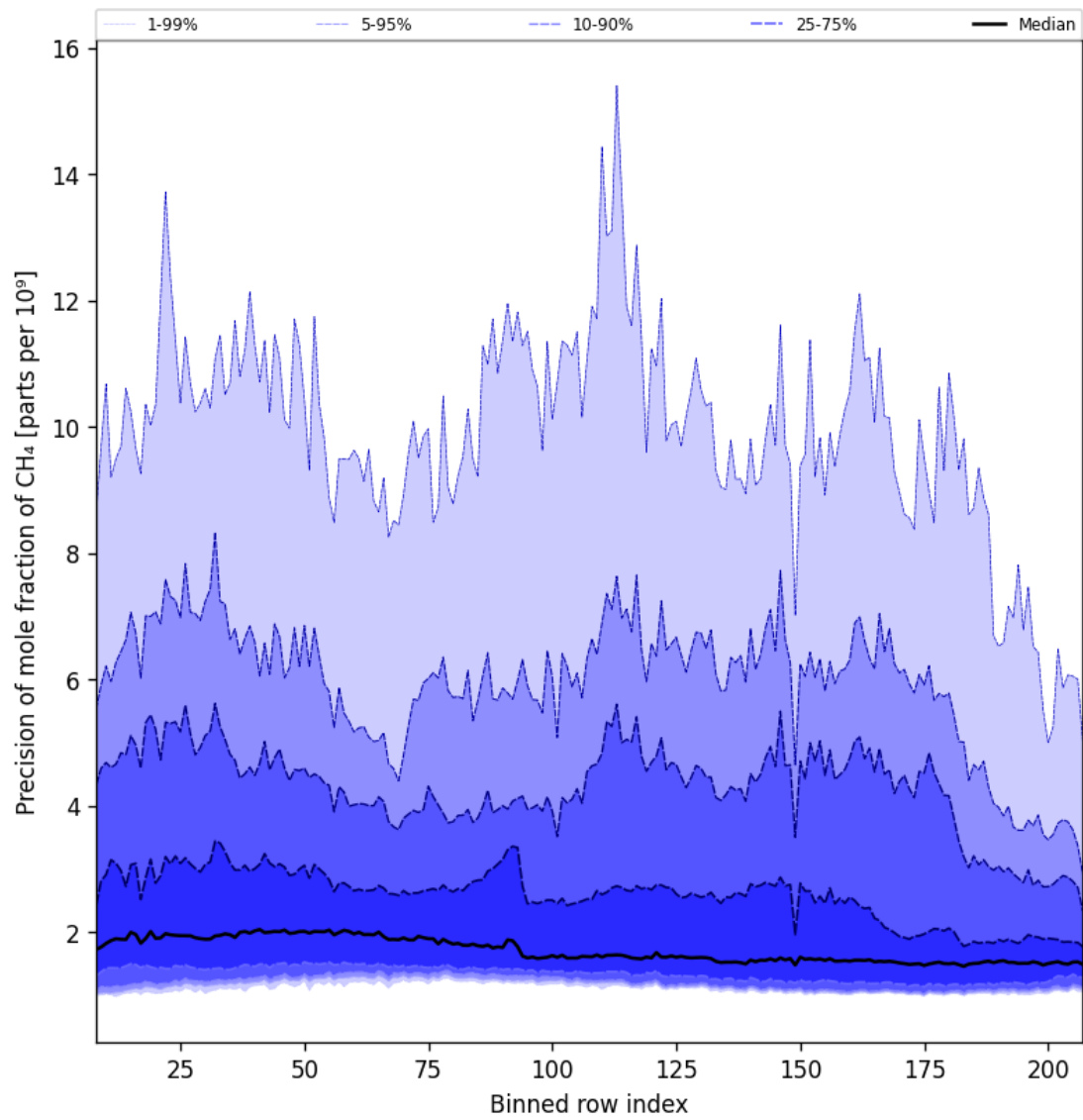
Figure 35: Along track statistics of “Precision of mole fraction of CH 4 ” for 2025-10-18 to 2025-10-20
