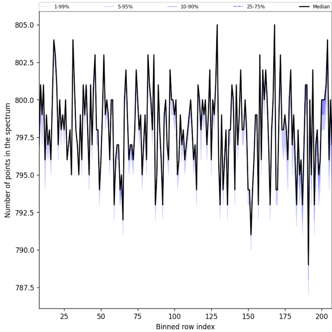
Figure 37: Along track statistics of “Number of points in the spectrum” for 2025-10-18 to 2025-10-20
