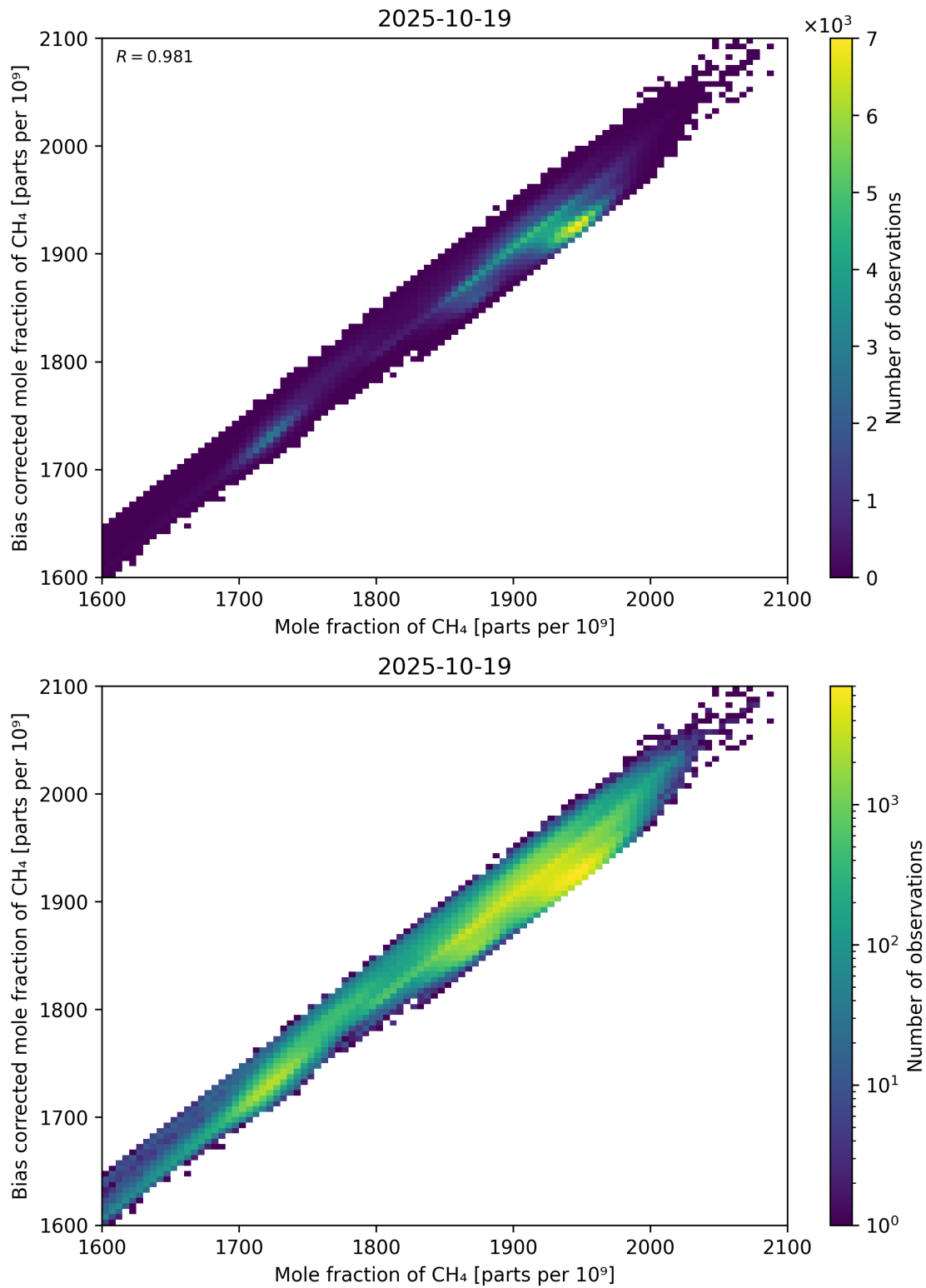
Figure 74: Scatter density plot of “Mole fraction of CH 4 ” against “Bias corrected mole fraction of CH 4 ” for 2025-10-18 to 2025-10-20.
