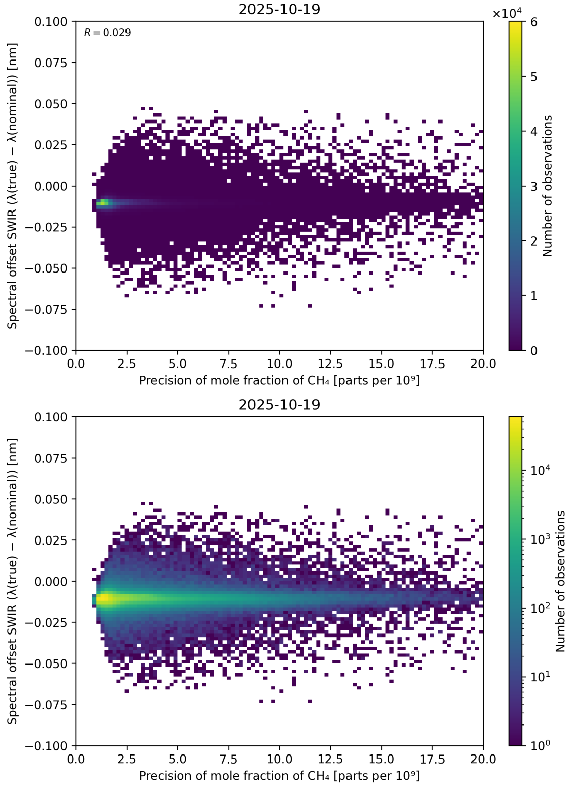
Figure 85: Scatter density plot of “Precision of mole fraction of CH 4 ” against “Spectral offset SWIR ( \lambda_{\text{true}} - \lambda_{\text{nominal}} )” for 2025-10-18 to 2025-10-20.
