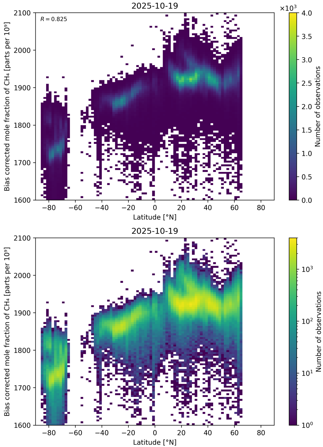
Figure 58: Scatter density plot of “Latitude” against “Bias corrected mole fraction of \text{CH}_4 ” for 2025-10-18 to 2025-10-20.
