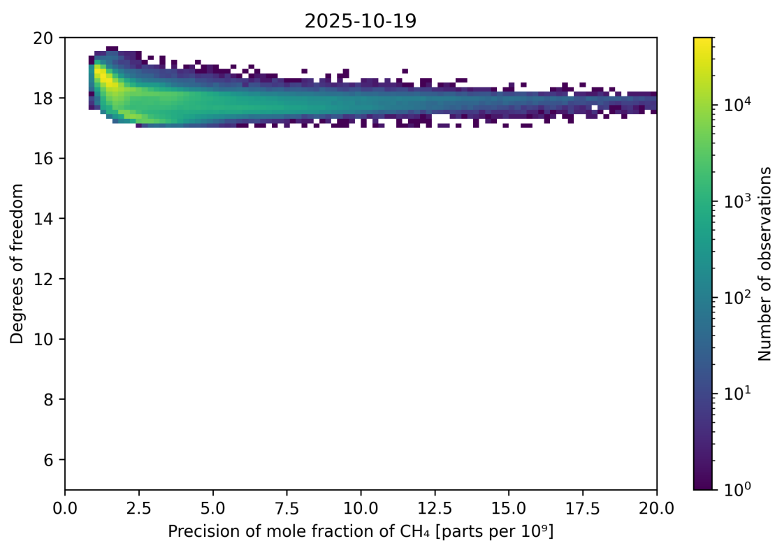
Figure 80: Scatter density plot of “Precision of mole fraction of CH 4 ” against “Degrees of freedom” for 2025-10-18 to 2025-10-20.
