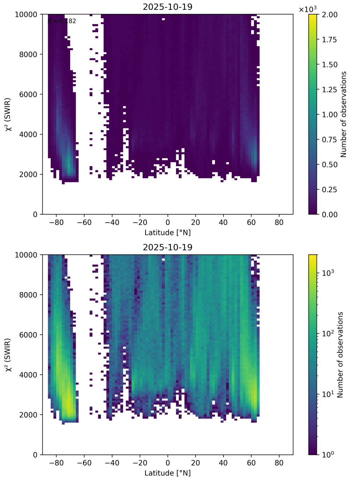
Figure 54: Scatter density plot of “Latitude” against “ \chi^2 (SWIR)” for 2025-10-18 to 2025-10-20.
