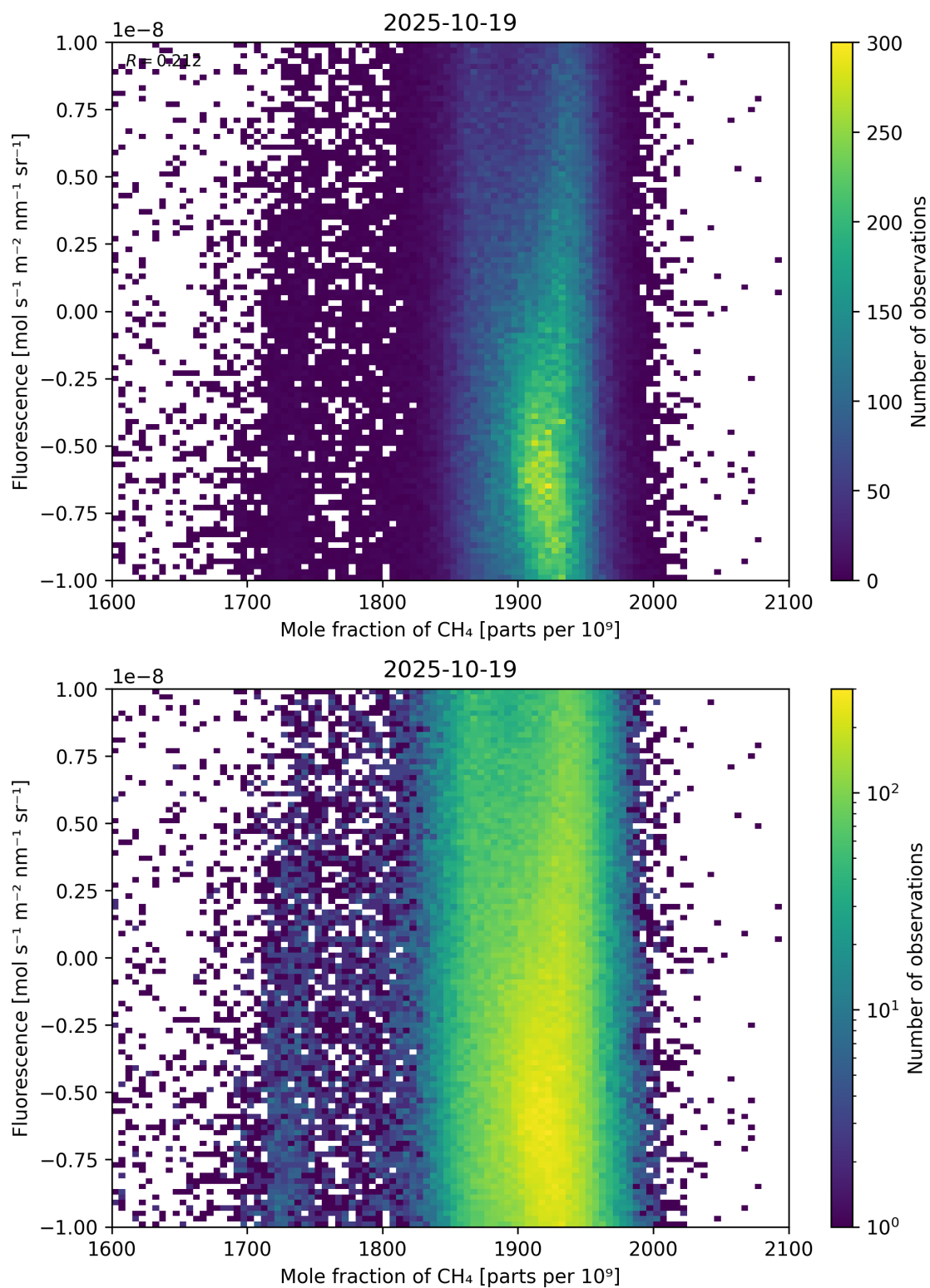
Figure 73: Scatter density plot of “Mole fraction of \text{CH}_4 ” against “Fluorescence” for 2025-10-18 to 2025-10-20.
