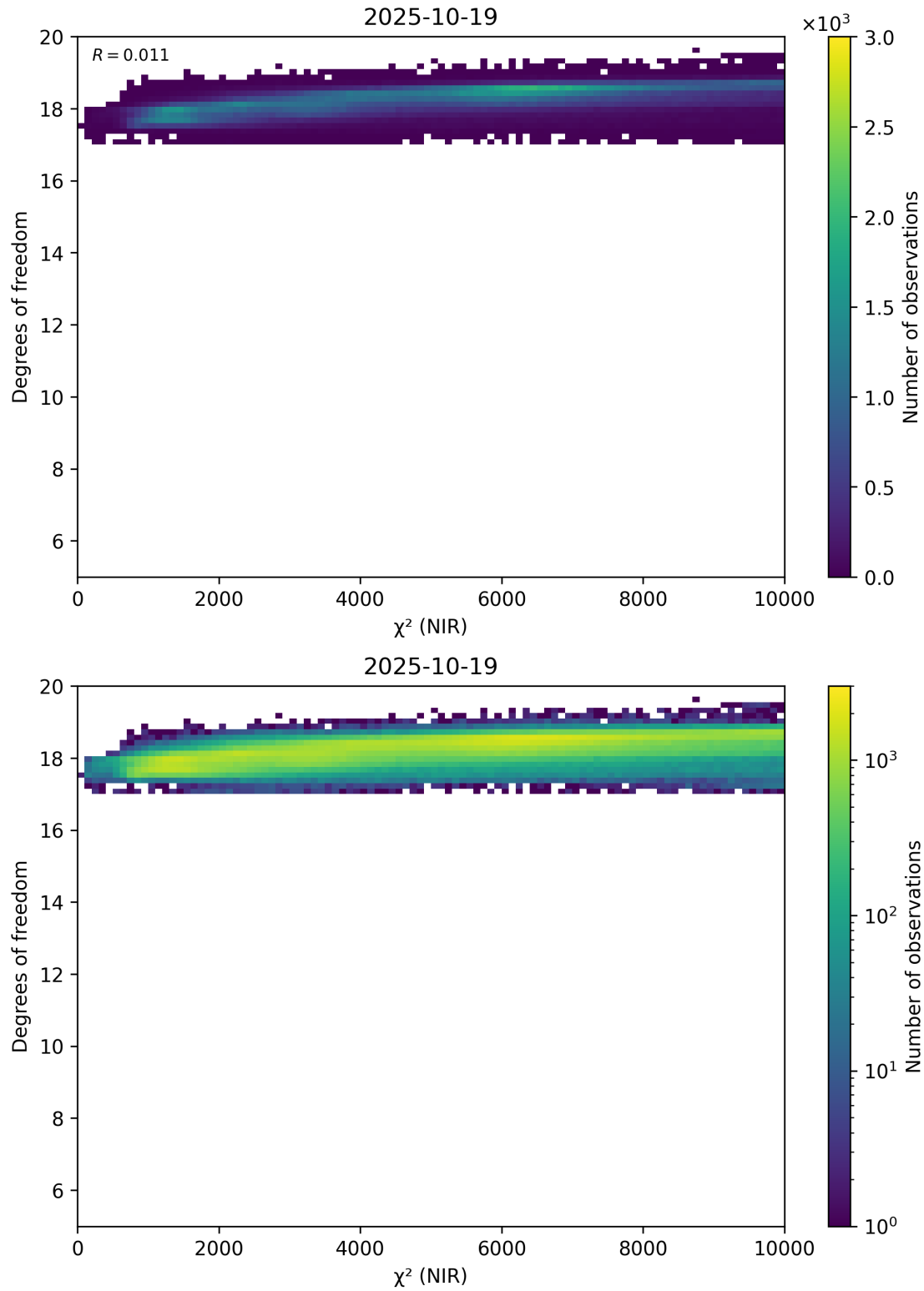
Figure 44: Scatter density plot of “ \chi^2 (NIR)” against “Degrees of freedom” for 2025-10-18 to 2025-10-20.
