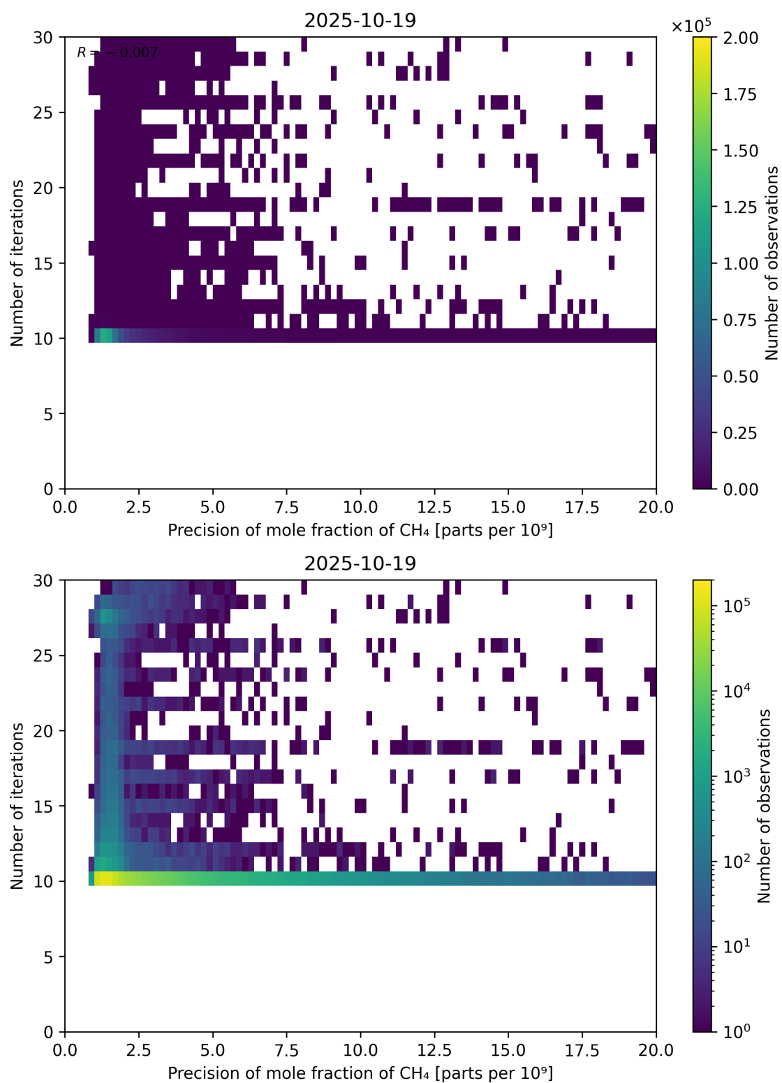
Figure 83: Scatter density plot of “Precision of mole fraction of CH 4 ” against “Number of iterations” for 2025-10-18 to 2025-10-20.
