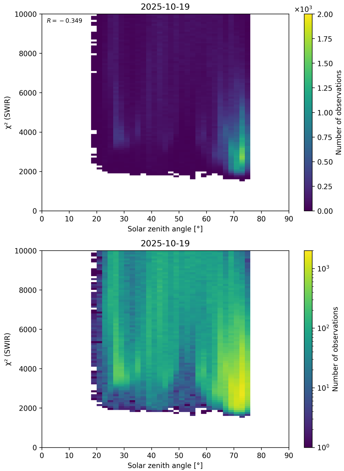
Figure 95: Scatter density plot of “Solar zenith angle” against “ \chi^2 (SWIR)” for 2025-10-18 to 2025-10-20.
