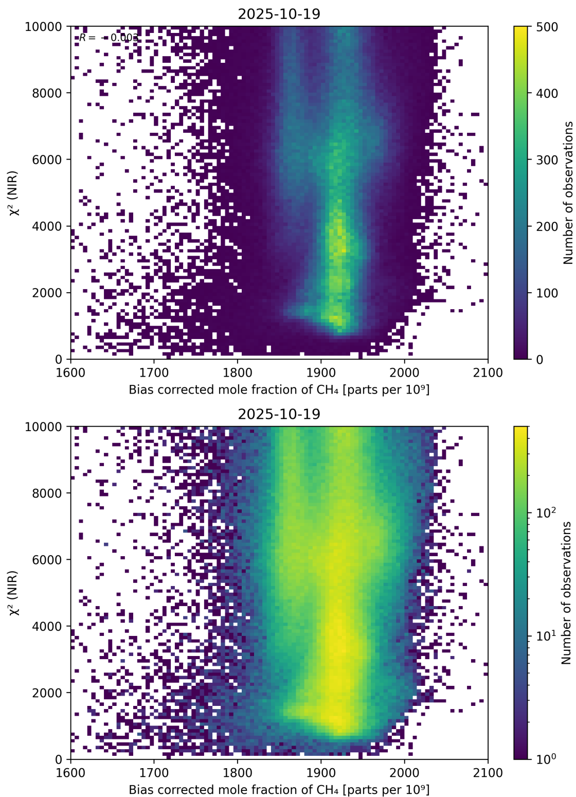
Figure 63: Scatter density plot of “Bias corrected mole fraction of CH 4 ” against “ \chi^2 (NIR)” for 2025-10-18 to 2025-10-20.
