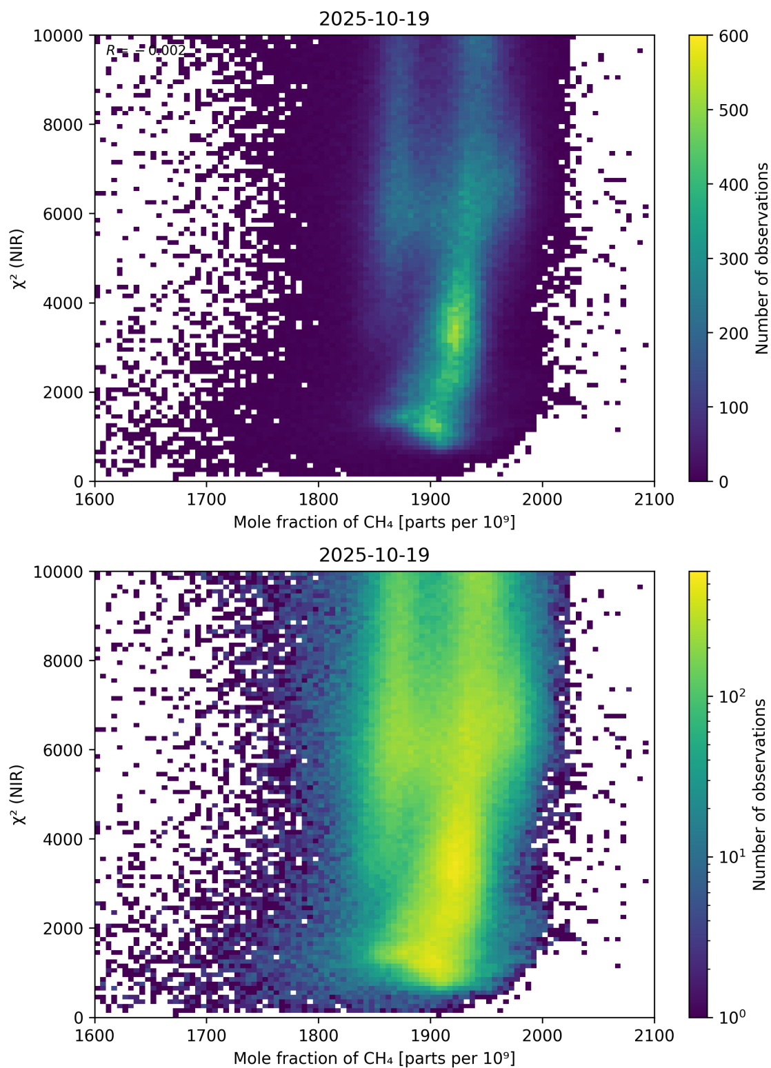
Figure 70: Scatter density plot of “Mole fraction of \text{CH}_4 ” against “ \chi^2 (NIR)” for 2025-10-18 to 2025-10-20.
