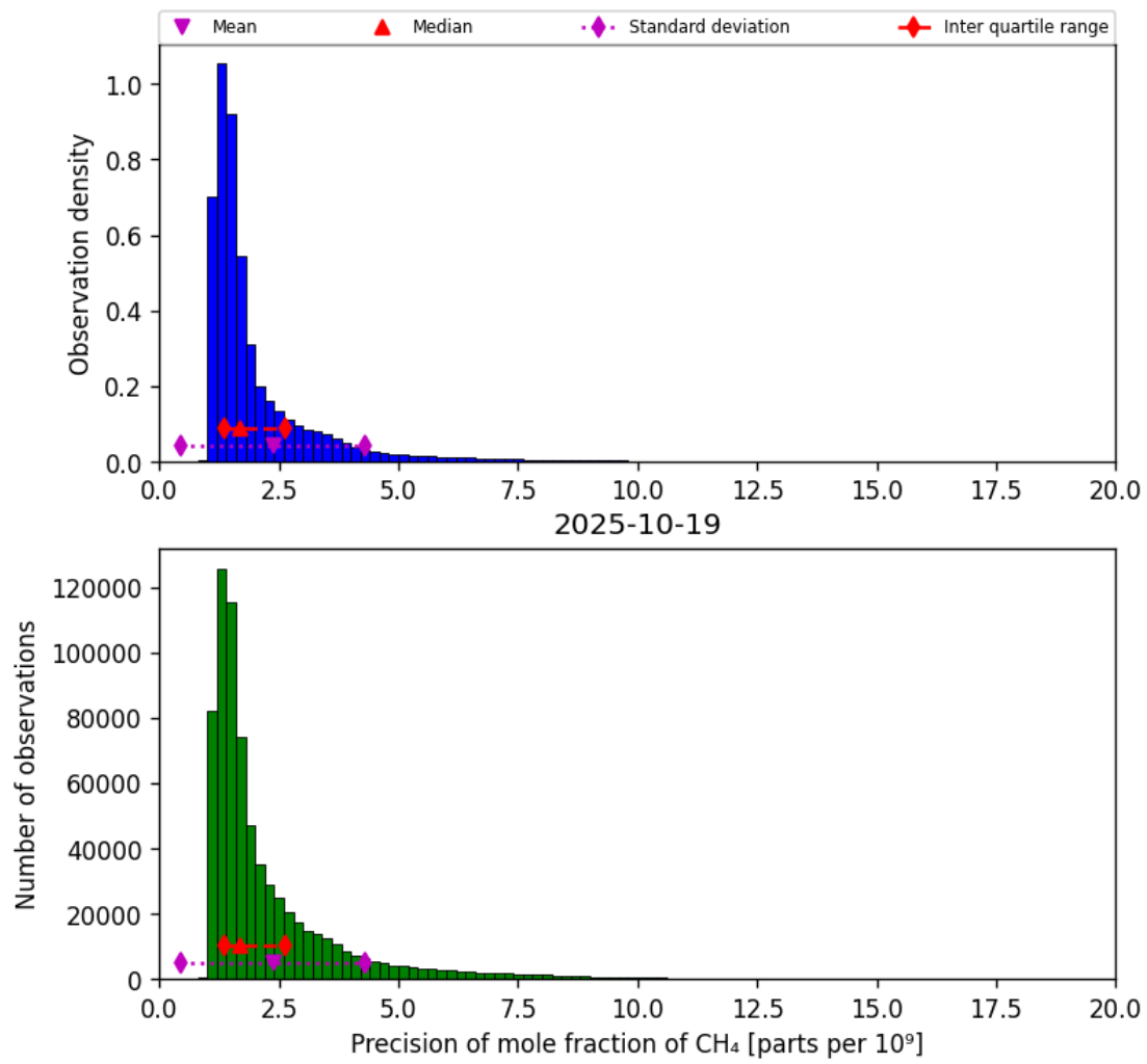
Figure 24: Histogram of “Precision of mole fraction of CH 4 ” for 2025-10-18 to 2025-10-20
