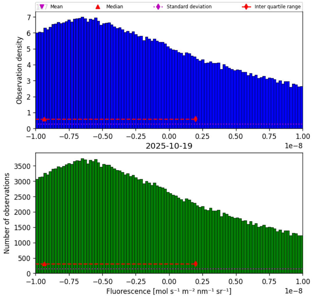
Figure 32: Histogram of “Fluorescence” for 2025-10-18 to 2025-10-20
