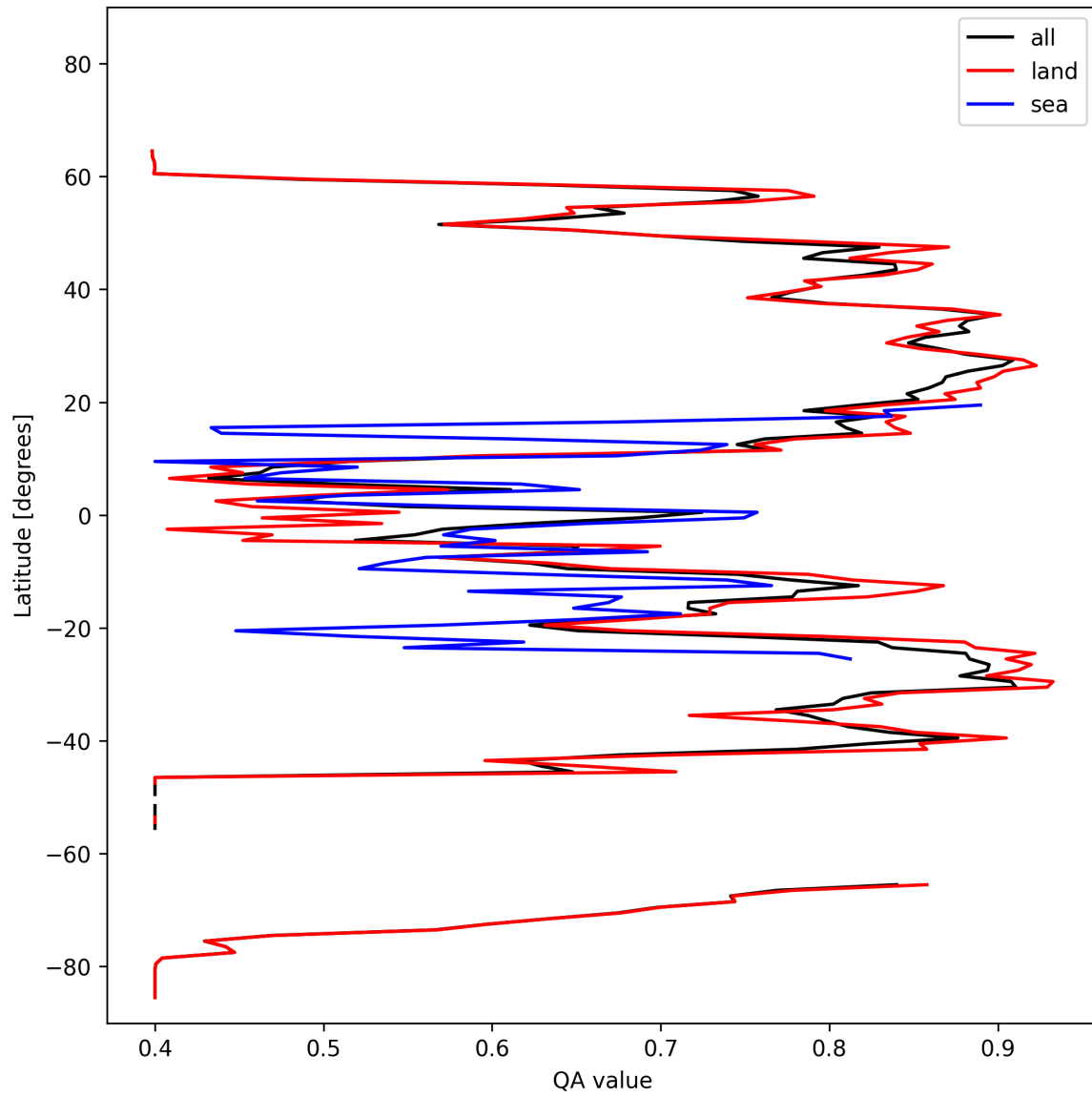
Figure 11: Zonal average of “QA value” for 2025-10-18 to 2025-10-20.
