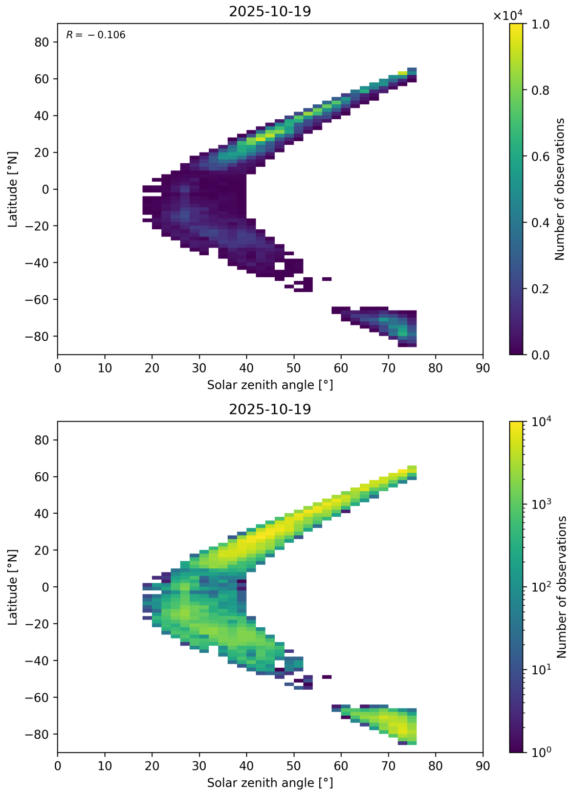
Figure 98: Scatter density plot of “Solar zenith angle” against “Latitude” for 2025-10-18 to 2025-10-20.
