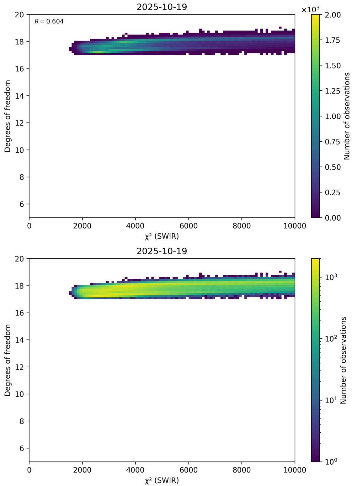
Figure 48: Scatter density plot of " \chi^2 (SWIR)" against "Degrees of freedom" for 2025-10-18 to 2025-10-20.
