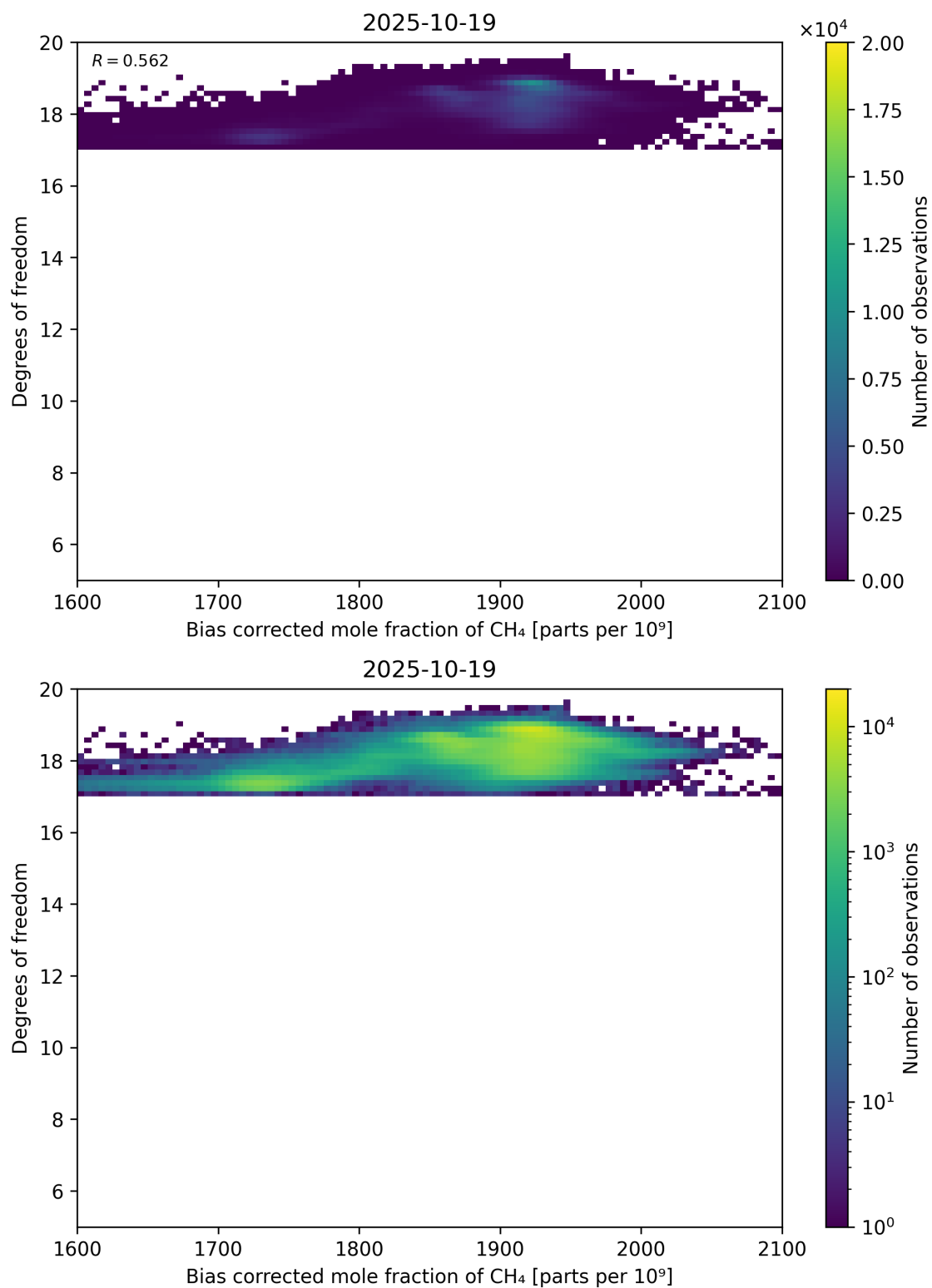
Figure 65: Scatter density plot of “Bias corrected mole fraction of \text{CH}_4 ” against “Degrees of freedom” for 2025-10-18 to 2025-10-20.
