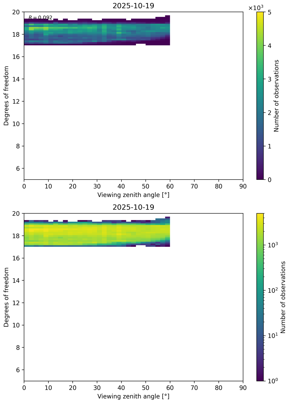
Figure 107: Scatter density plot of “Viewing zenith angle” against “Degrees of freedom” for 2025-10-18 to 2025-10-20.
