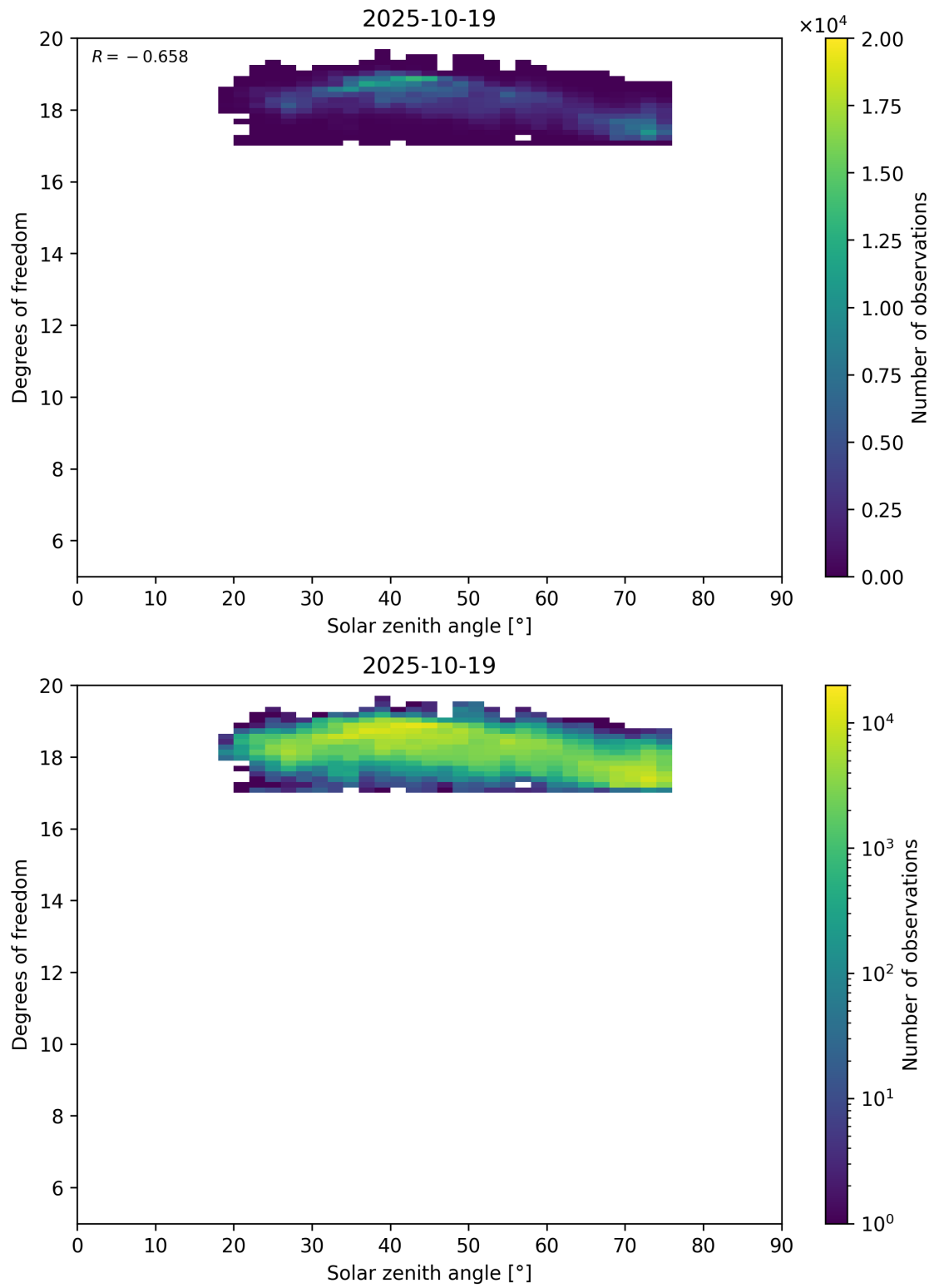
Figure 96: Scatter density plot of “Solar zenith angle” against “Degrees of freedom” for 2025-10-18 to 2025-10-20.
