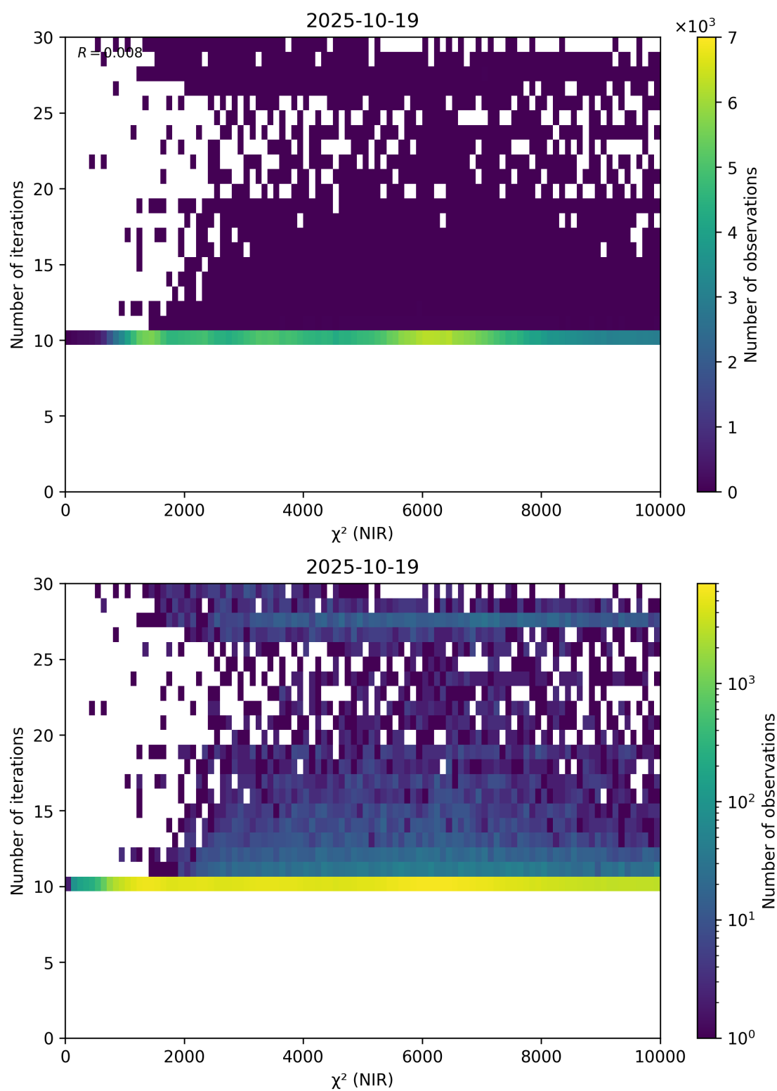
Figure 46: Scatter density plot of “ \chi^2 (NIR)” against “Number of iterations” for 2025-10-18 to 2025-10-20.
