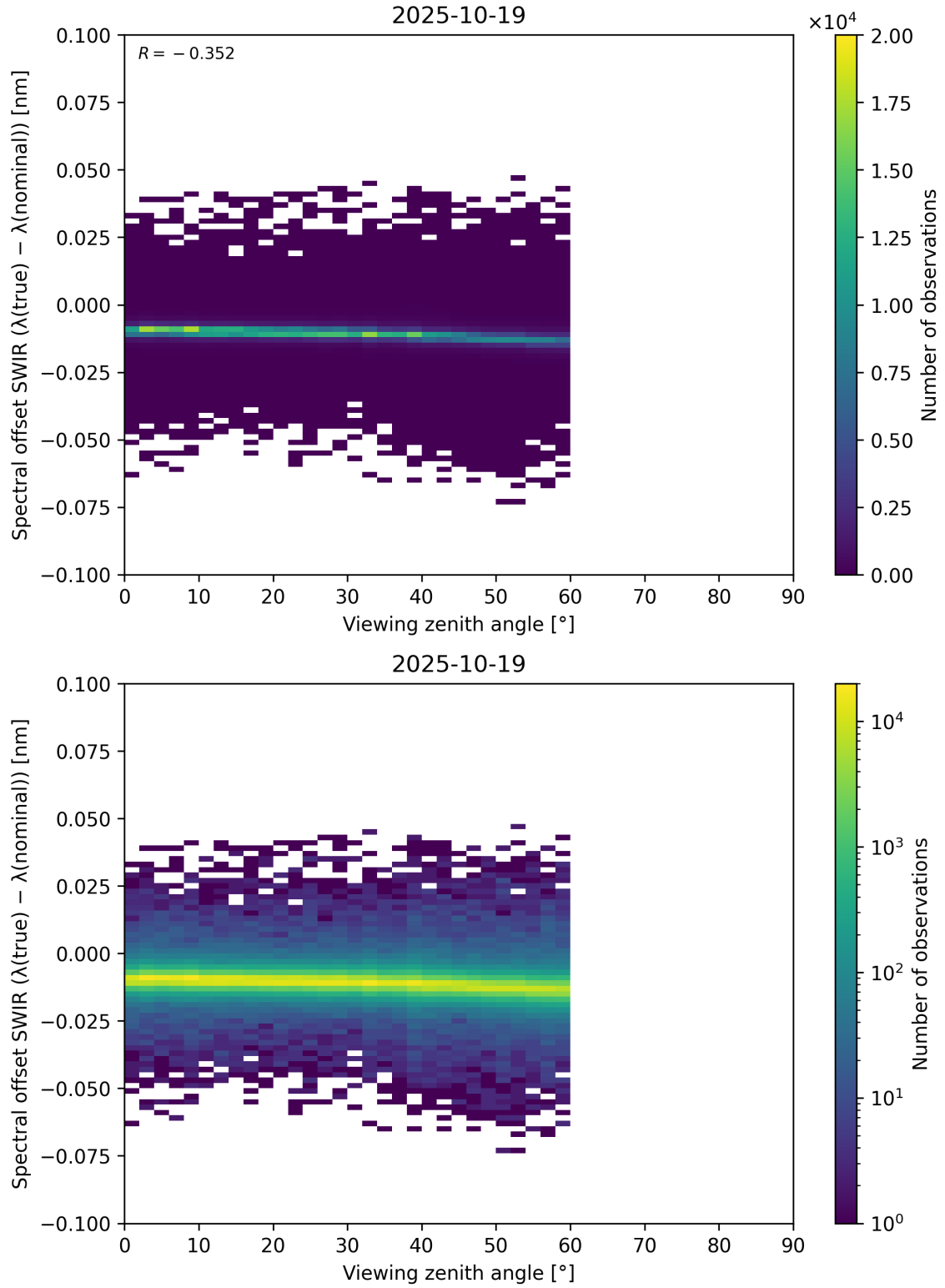
Figure 116: Scatter density plot of “Viewing zenith angle” against “Spectral offset SWIR ( \lambda_{\text{true}} - \lambda_{\text{nominal}} )” for 2025-10-18 to 2025-10-20.
