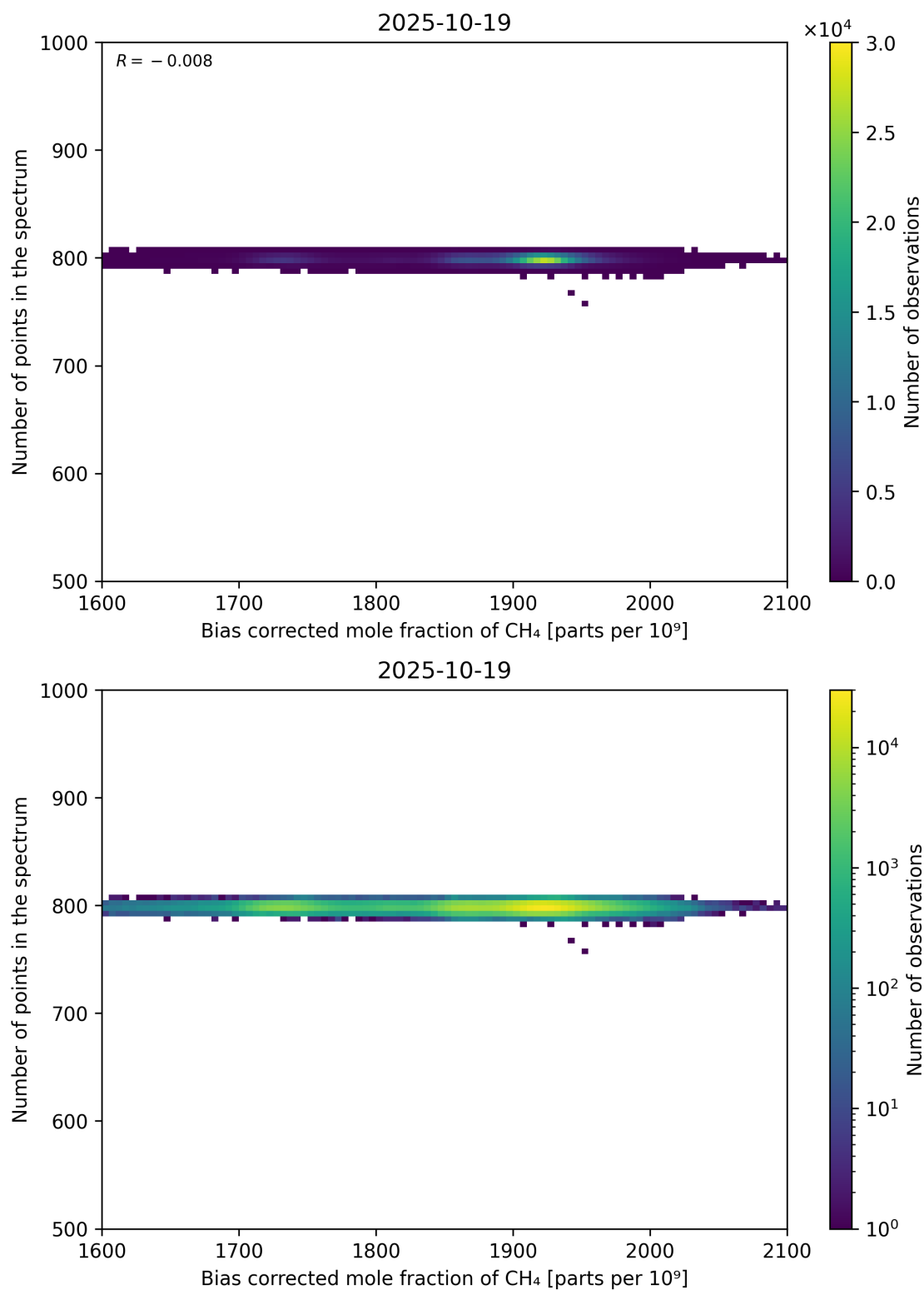
Figure 68: Scatter density plot of “Bias corrected mole fraction of CH 4 ” against “Number of points in the spectrum” for 2025-10-18 to 2025-10-20.
