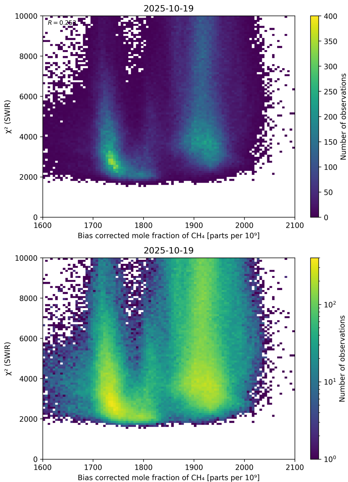
Figure 64: Scatter density plot of “Bias corrected mole fraction of \text{CH}_4 ” against “ \chi^2 (SWIR)” for 2025-10-18 to 2025-10-20.
