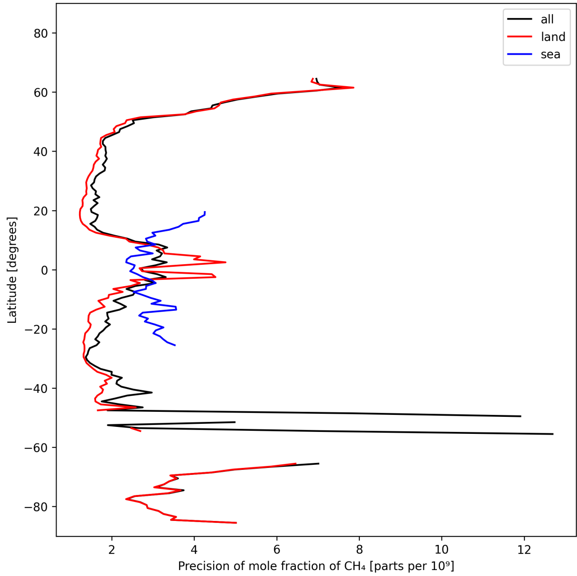
Figure 13: Zonal average of “Precision of mole fraction of CH 4 ” for 2025-10-18 to 2025-10-20.
