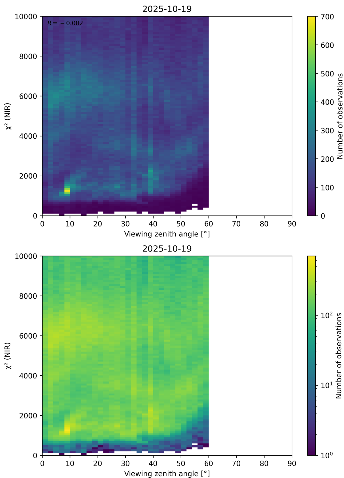
Figure 105: Scatter density plot of “Viewing zenith angle” against “ \chi^2 (NIR)” for 2025-10-18 to 2025-10-20.
