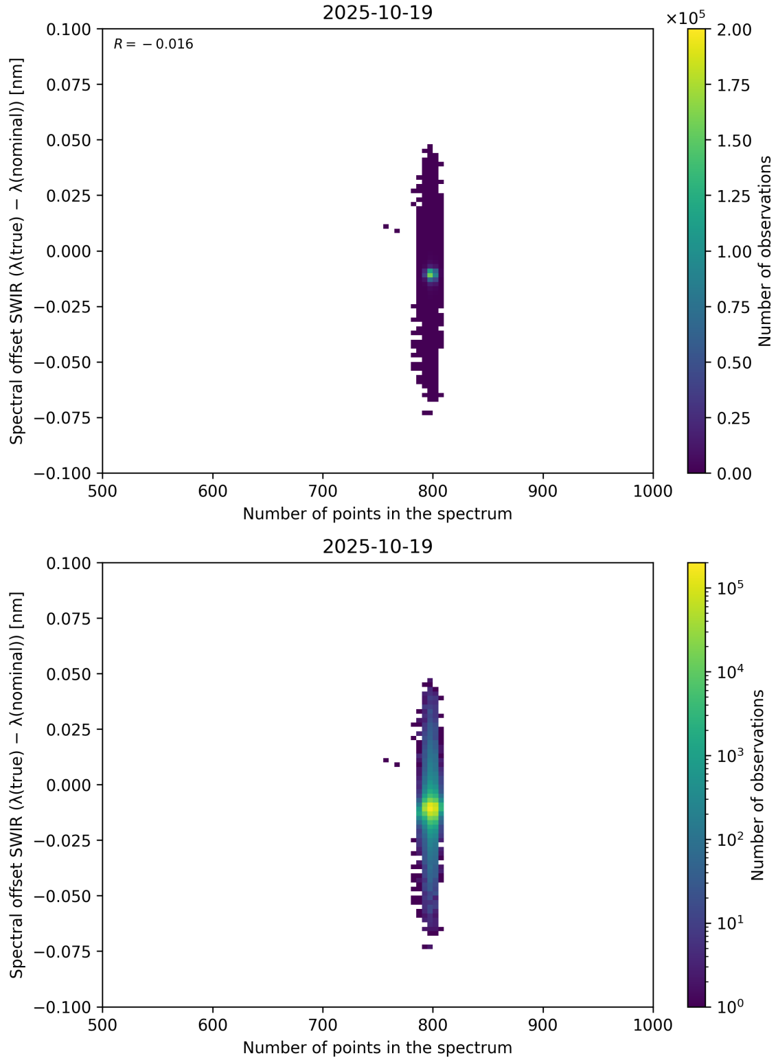
Figure 93: Scatter density plot of “Number of points in the spectrum” against “Spectral offset SWIR ( \lambda_{\text{true}} - \lambda_{\text{nominal}} )” for 2025-10-18 to 2025-10-20.
