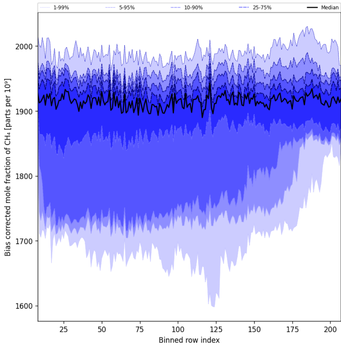
Figure 36: Along track statistics of “Bias corrected mole fraction of CH 4 ” for 2025-10-18 to 2025-10-20
