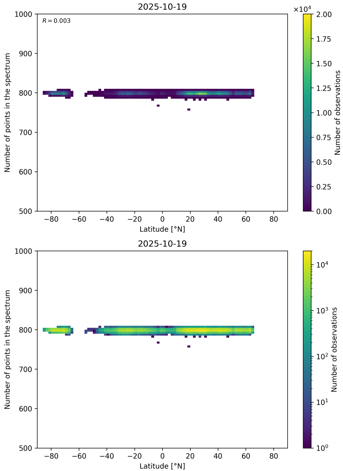
Figure 61: Scatter density plot of “Latitude” against “Number of points in the spectrum” for 2025-10-18 to 2025-10-20.
