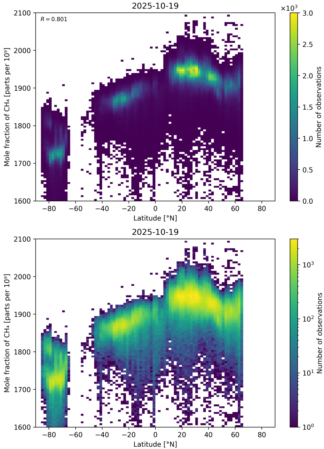
Figure 57: Scatter density plot of “Latitude” against “Mole fraction of CH 4 ” for 2025-10-18 to 2025-10-20.
