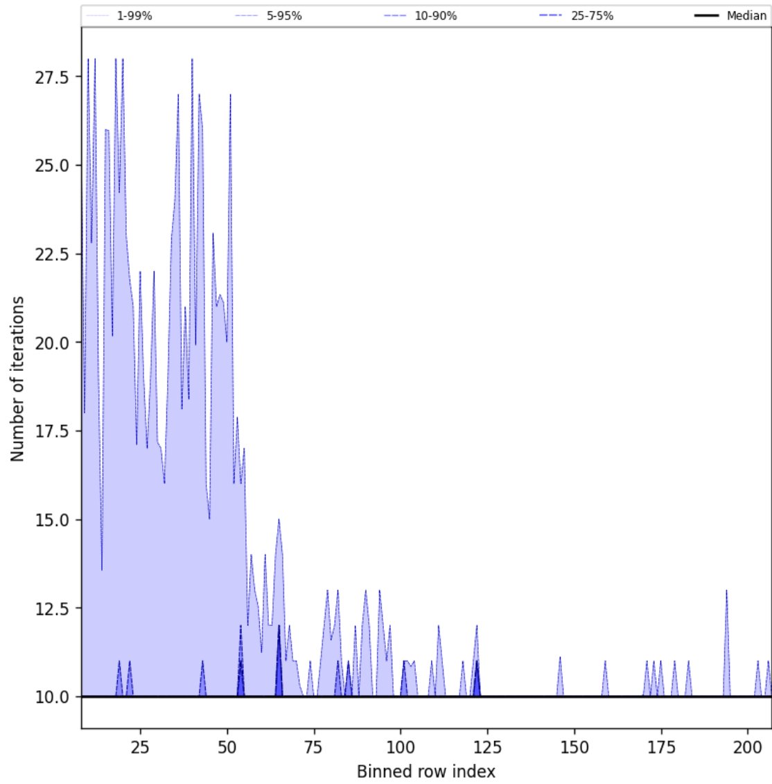
Figure 42: Along track statistics of “Number of iterations” for 2025-10-18 to 2025-10-20
