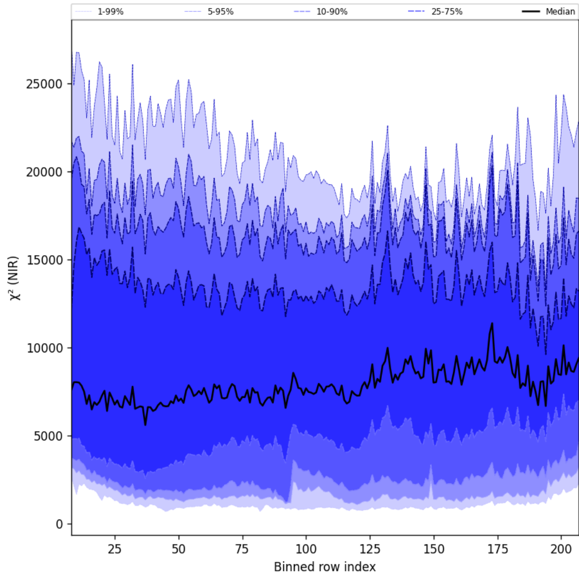
Figure 40: Along track statistics of “ \chi^2 (NIR)” for 2025-10-18 to 2025-10-20
