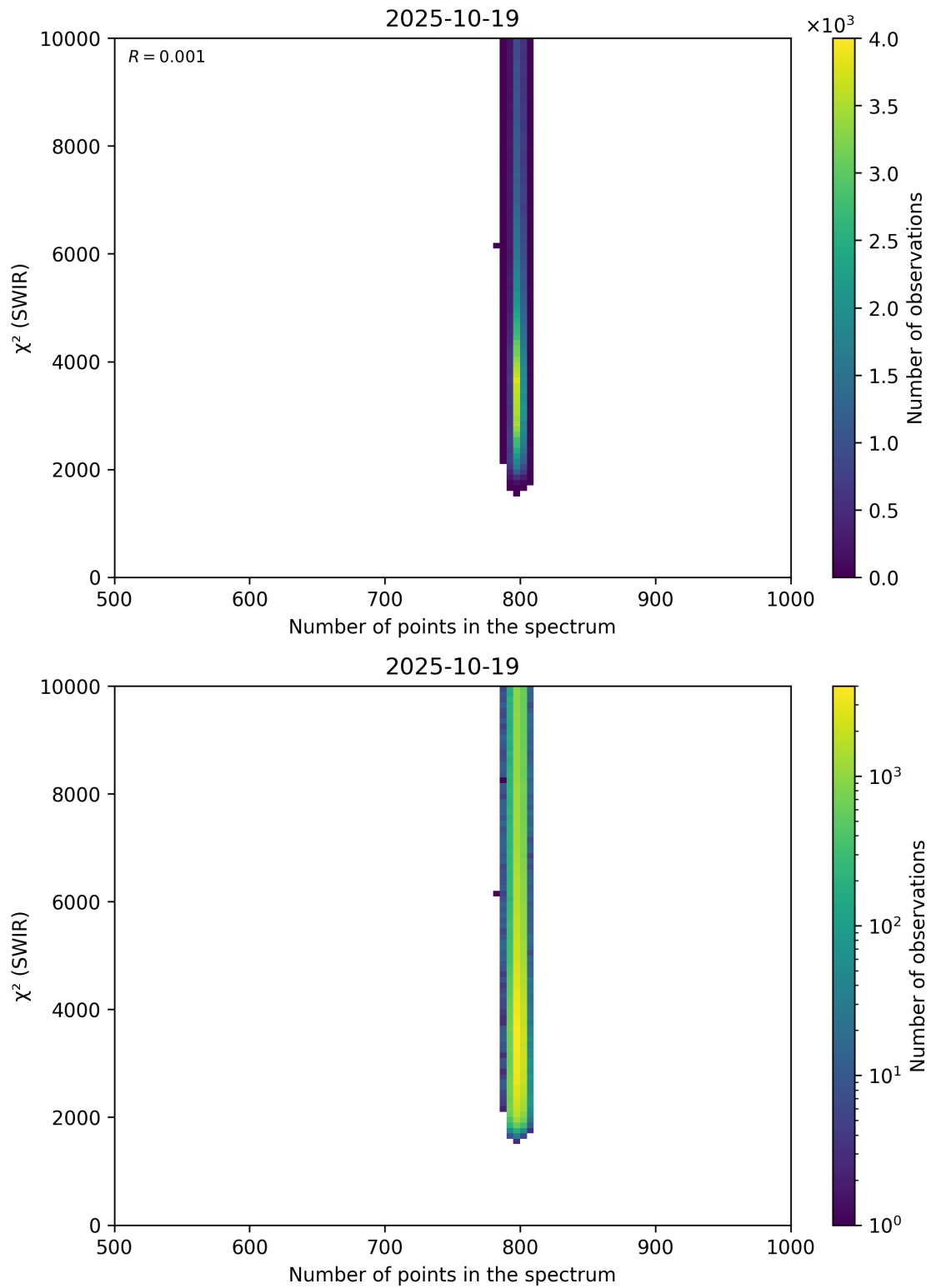
Figure 89: Scatter density plot of “Number of points in the spectrum” against “ \chi^2 (SWIR)” for 2025-10-18 to 2025-10-20.
