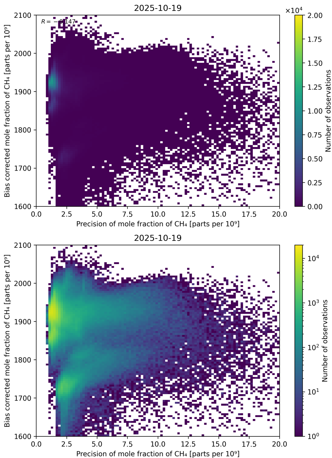
Figure 82: Scatter density plot of “Precision of mole fraction of CH 4 ” against “Bias corrected mole fraction of CH 4 ” for 2025-10-18 to 2025-10-20.
