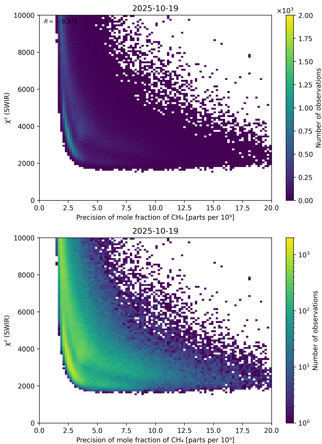
Figure 79: Scatter density plot of “Precision of mole fraction of \text{CH}_4 ” against “ \chi^2 (SWIR)” for 2025-10-18 to 2025-10-20.
