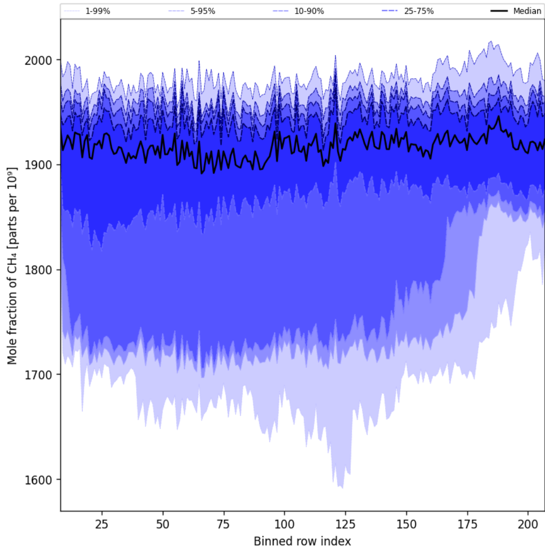
Figure 34: Along track statistics of “Mole fraction of CH 4 ” for 2025-10-18 to 2025-10-20
