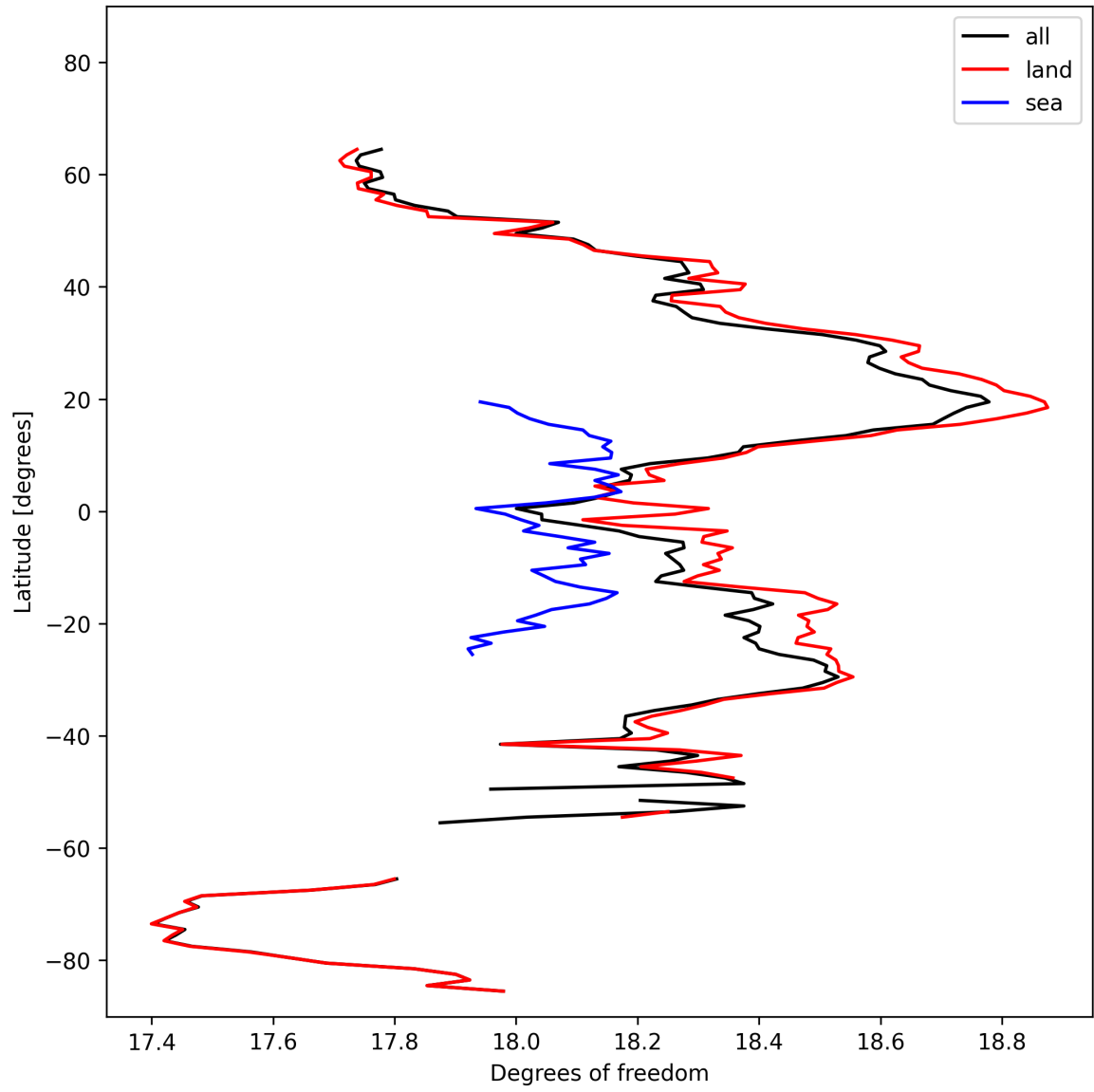
Figure 19: Zonal average of “Degrees of freedom” for 2025-10-18 to 2025-10-20.
