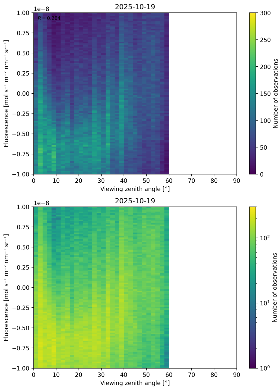
Figure 108: Scatter density plot of “Viewing zenith angle” against “Fluorescence” for 2025-10-18 to 2025-10-20.
