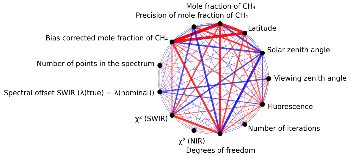
Figure 1: Map of correlation graph for 2025-10-18 to 2025-10-20.
