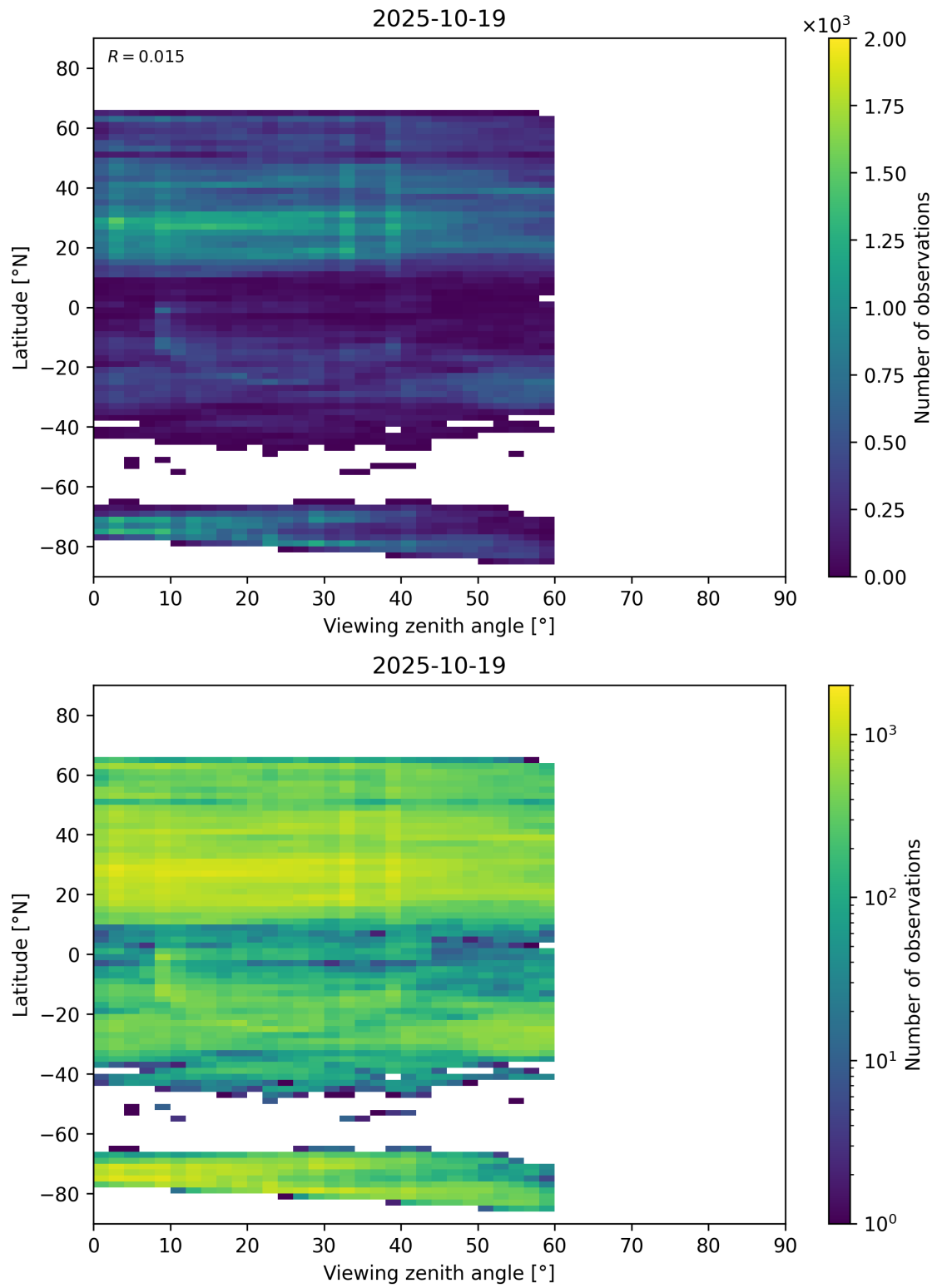
Figure 109: Scatter density plot of “Viewing zenith angle” against “Latitude” for 2025-10-18 to 2025-10-20.
