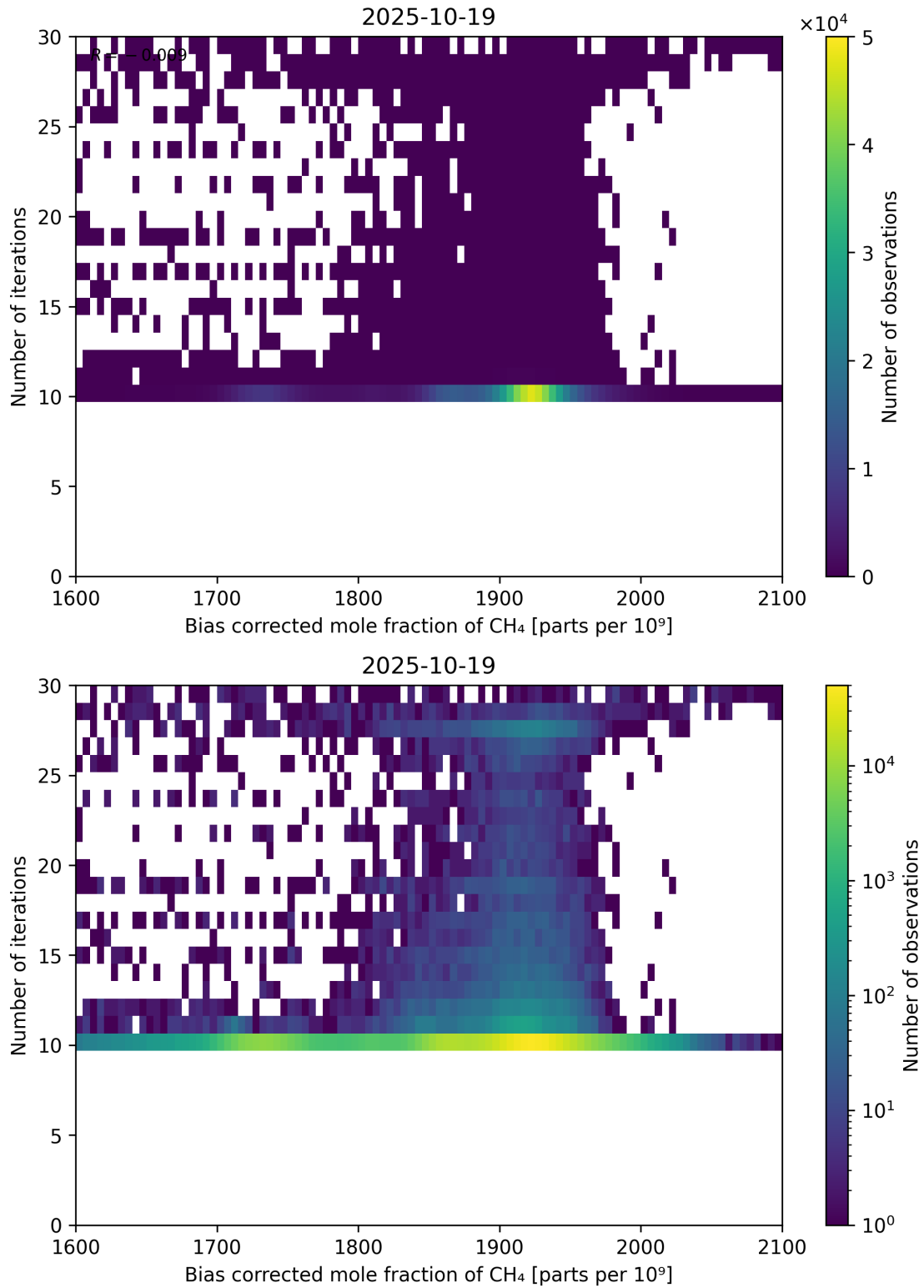
Figure 67: Scatter density plot of “Bias corrected mole fraction of CH 4 ” against “Number of iterations” for 2025-10-18 to 2025-10-20.
