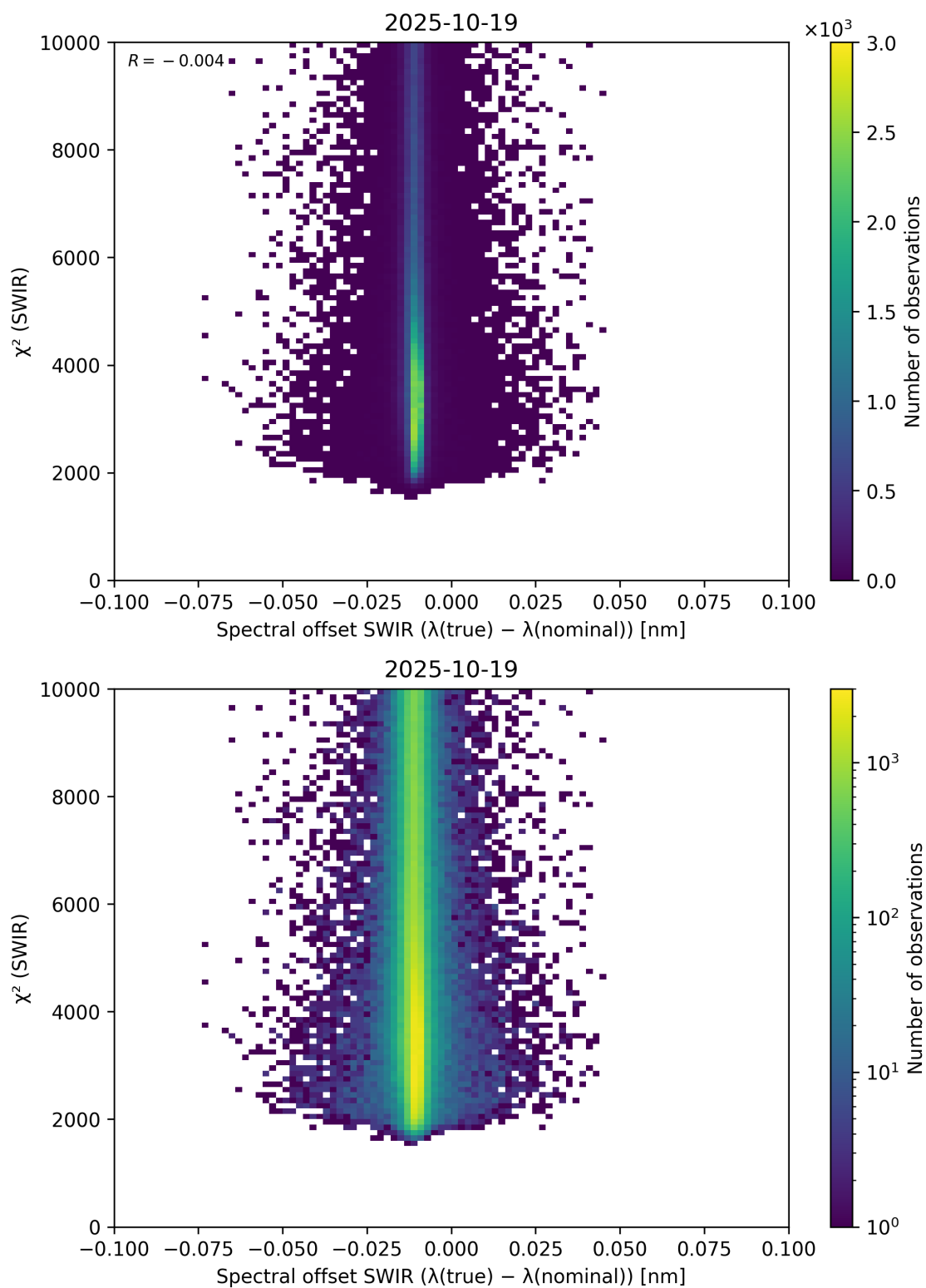
Figure 118: Scatter density plot of “Spectral offset SWIR ( \lambda_{\text{true}} - \lambda_{\text{nominal}} )” against “ \chi^2 (SWIR)” for 2025-10-18 to 2025-10-20.
