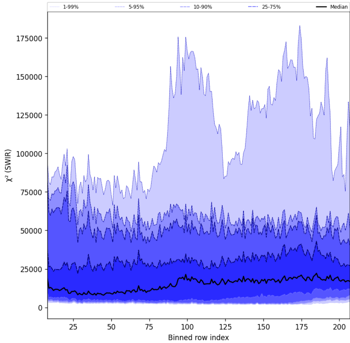
Figure 39: Along track statistics of “ \chi^2 (SWIR)” for 2025-10-18 to 2025-10-20
