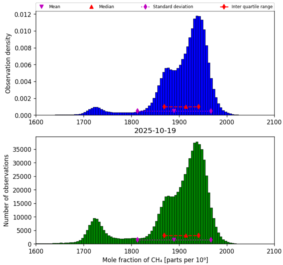
Figure 23: Histogram of “Mole fraction of CH 4 ” for 2025-10-18 to 2025-10-20
