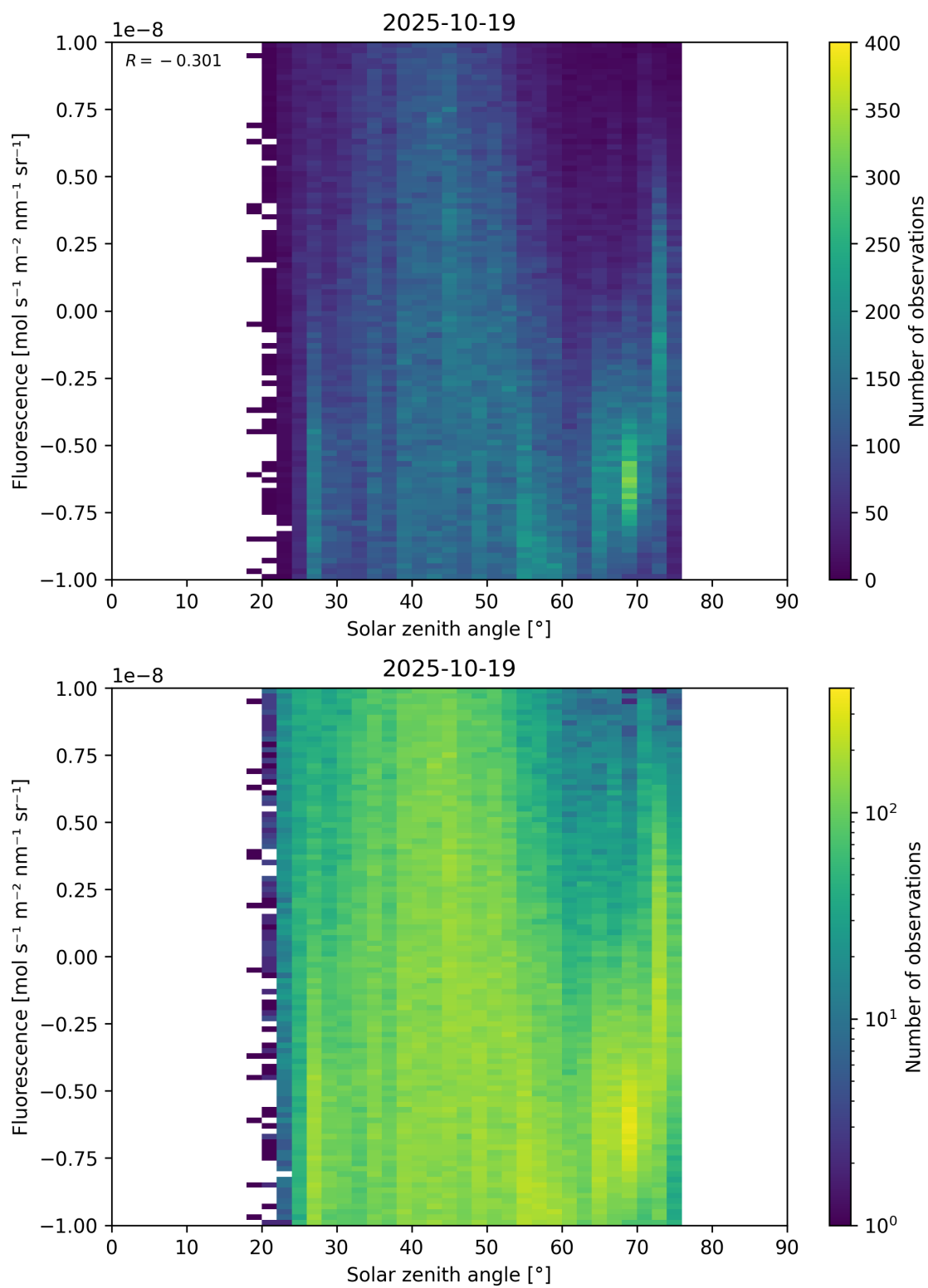
Figure 97: Scatter density plot of “Solar zenith angle” against “Fluorescence” for 2025-10-18 to 2025-10-20.
