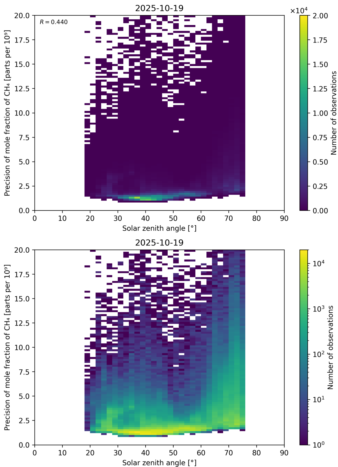
Figure 101: Scatter density plot of “Solar zenith angle” against “Precision of mole fraction of \text{CH}_4 ” for 2025-10-18 to 2025-10-20.
