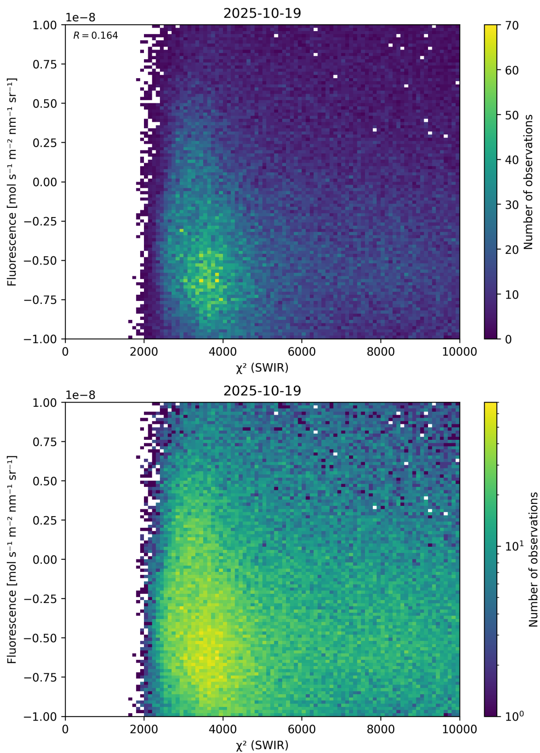
Figure 49: Scatter density plot of “ \chi^2 (SWIR)” against “Fluorescence” for 2025-10-18 to 2025-10-20.
