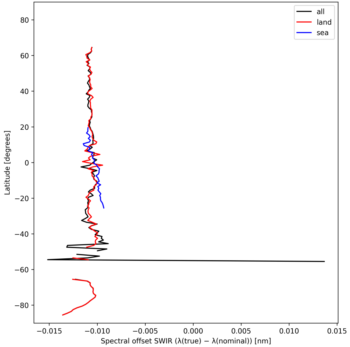
Figure 16: Zonal average of “Spectral offset SWIR ( \lambda_{\text{true}} - \lambda_{\text{nominal}} )” for 2025-10-18 to 2025-10-20.
