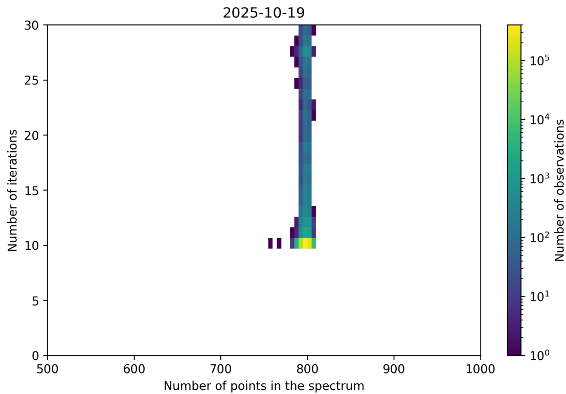
Figure 92: Scatter density plot of “Number of points in the spectrum” against “Number of iterations” for 2025-10-18 to 2025-10-20.
