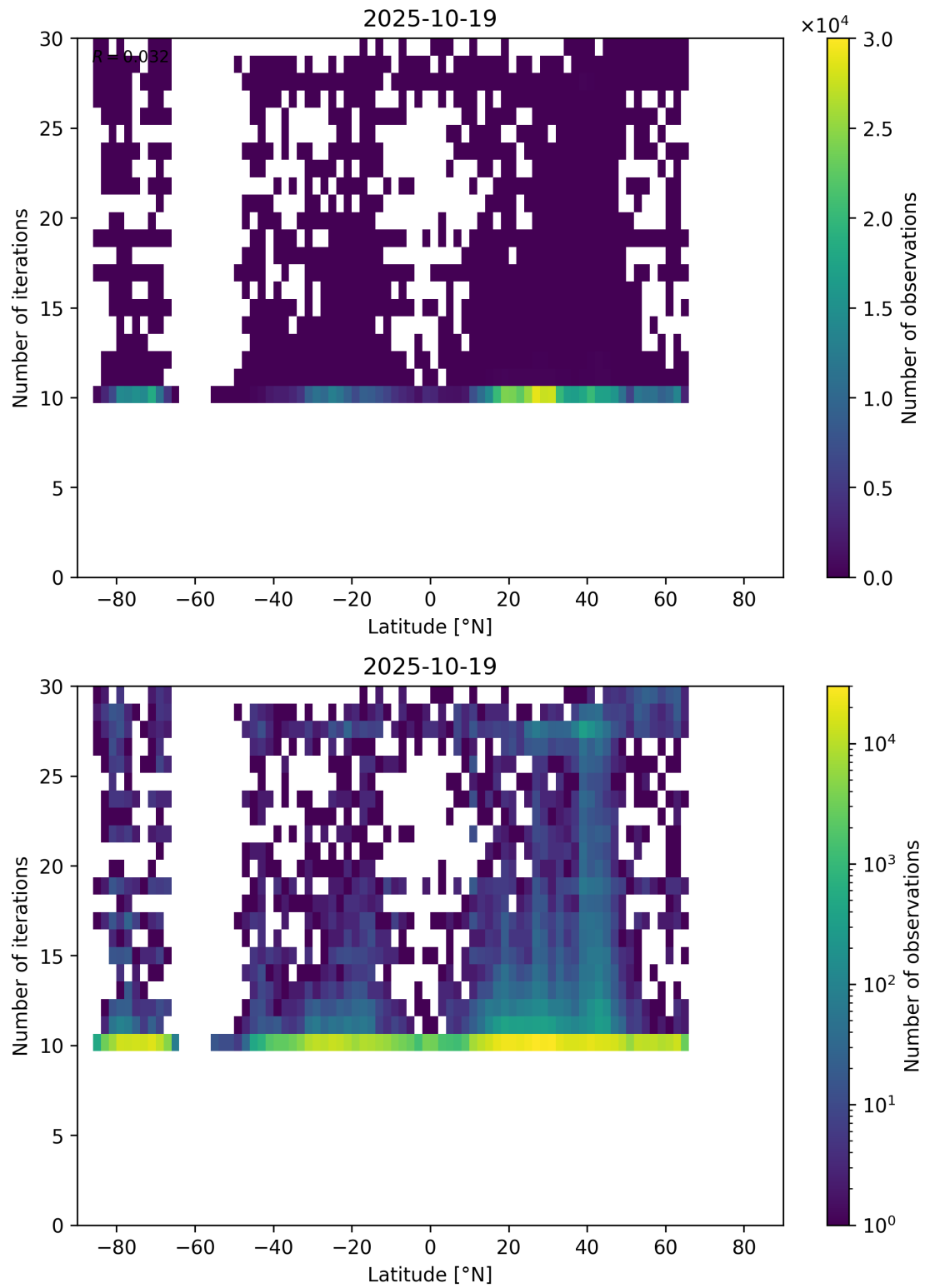
Figure 60: Scatter density plot of “Latitude” against “Number of iterations” for 2025-10-18 to 2025-10-20.
