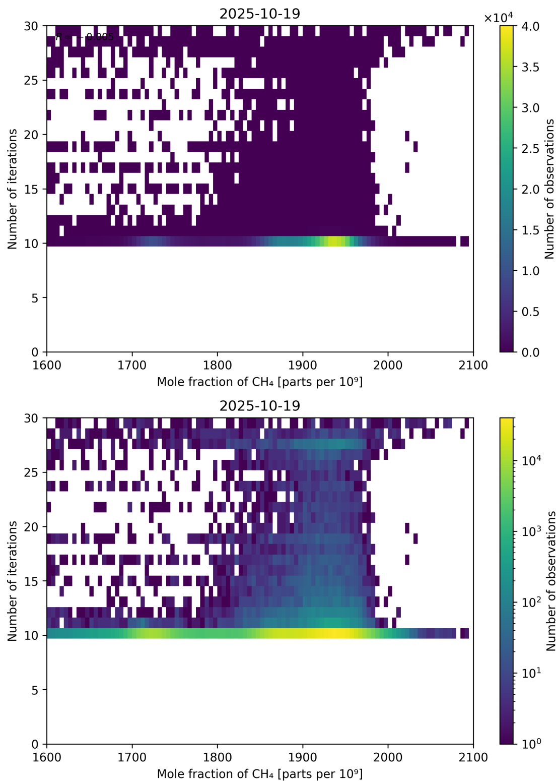
Figure 76: Scatter density plot of “Mole fraction of CH 4 ” against “Number of iterations” for 2025-10-18 to 2025-10-20.
