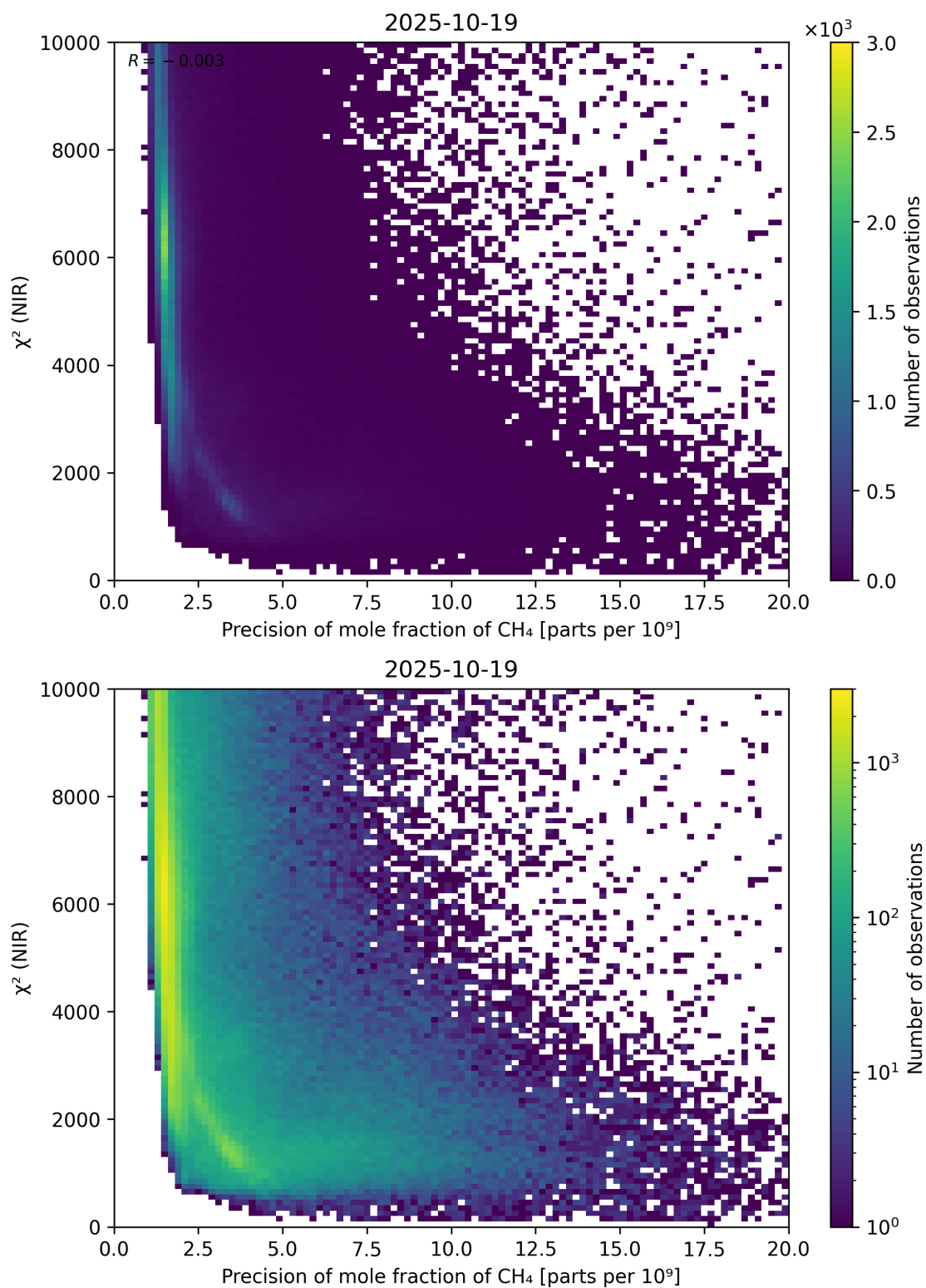
Figure 78: Scatter density plot of “Precision of mole fraction of CH 4 ” against “ \chi^2 (NIR)” for 2025-10-18 to 2025-10-20.
