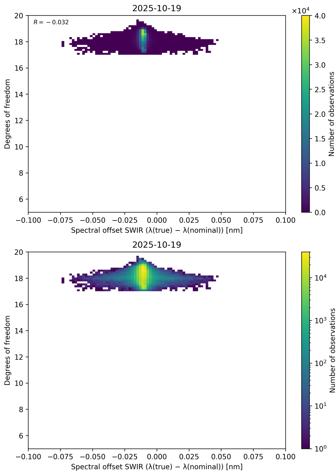
Figure 119: Scatter density plot of “Spectral offset SWIR ( \lambda_{\text{true}} - \lambda_{\text{nominal}} )” against “Degrees of freedom” for 2025-10-18 to 2025-10-20.
