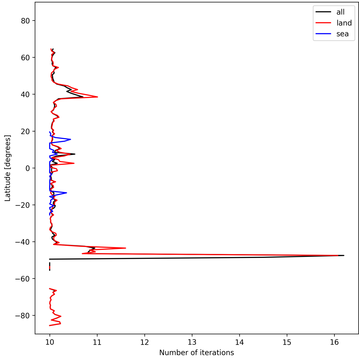
Figure 20: Zonal average of “Number of iterations” for 2025-10-18 to 2025-10-20.
