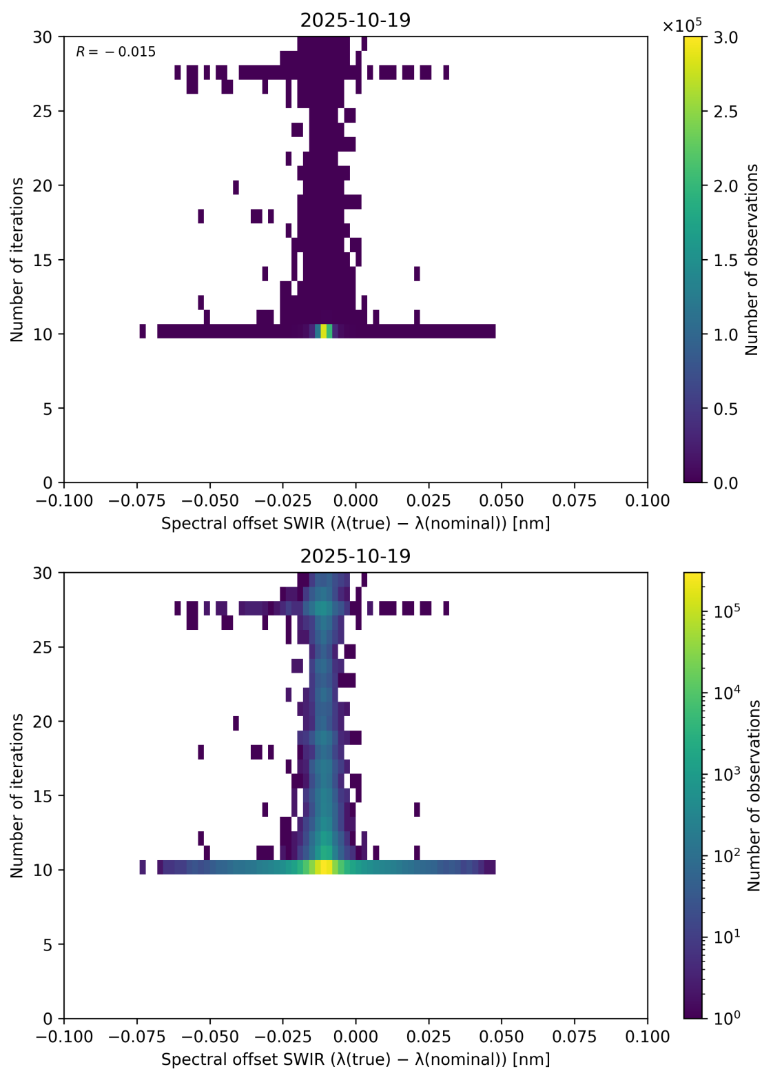
Figure 121: Scatter density plot of “Spectral offset SWIR ( \lambda_{\text{true}} - \lambda_{\text{nominal}} )” against “Number of iterations” for 2025-10-18 to 2025-10-20.
