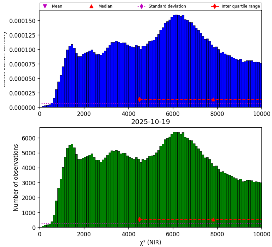
Figure 29: Histogram of “ \chi^2 (NIR)” for 2025-10-18 to 2025-10-20
