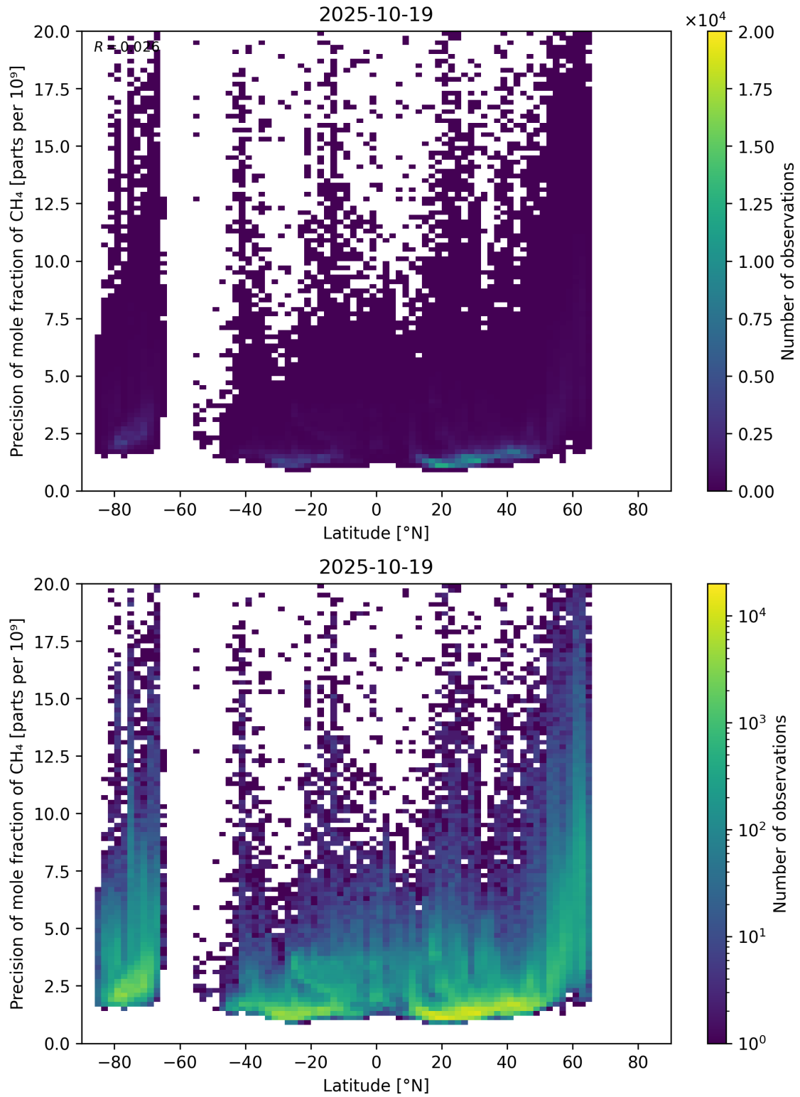
Figure 59: Scatter density plot of “Latitude” against “Precision of mole fraction of CH 4 ” for 2025-10-18 to 2025-10-20.
