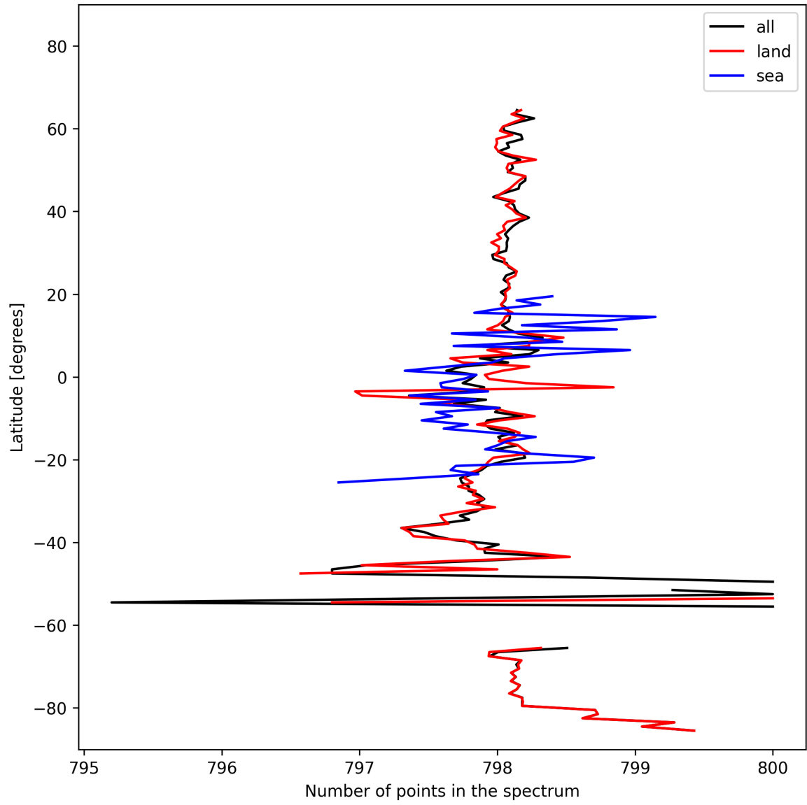
Figure 15: Zonal average of “Number of points in the spectrum” for 2025-10-18 to 2025-10-20.
