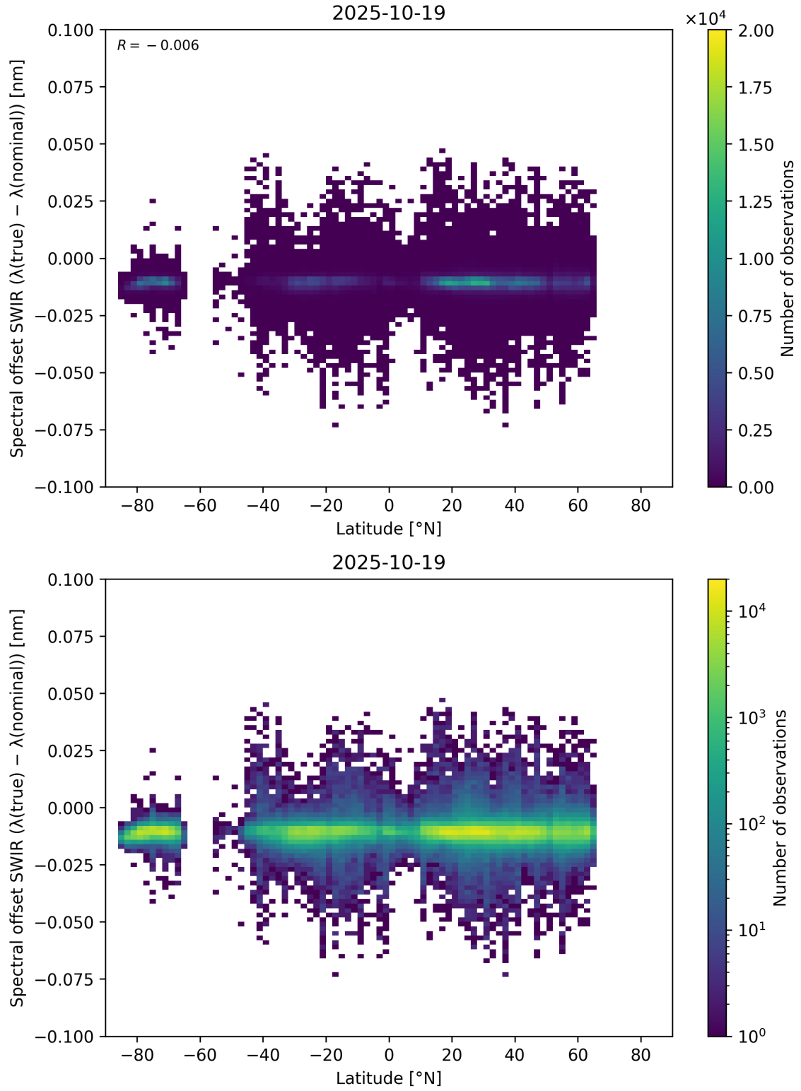
Figure 62: Scatter density plot of “Latitude” against “Spectral offset SWIR ( \lambda_{\text{true}} - \lambda_{\text{nominal}} )” for 2025-10-18 to 2025-10-20.
