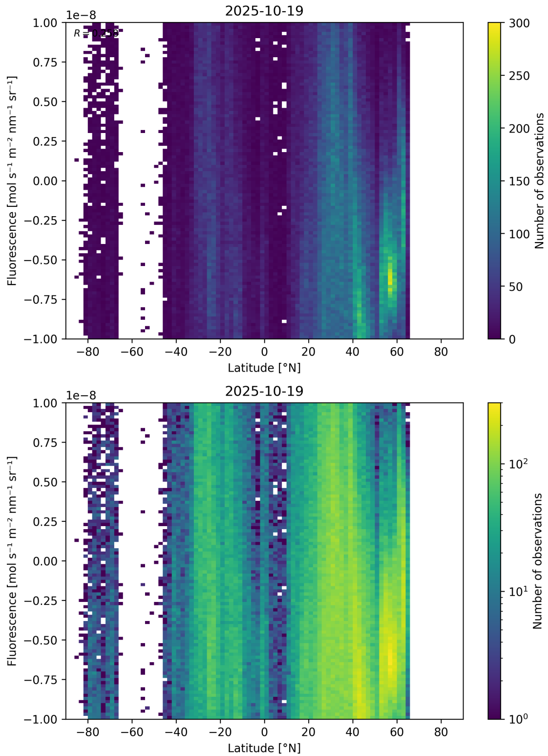
Figure 56: Scatter density plot of “Latitude” against “Fluorescence” for 2025-10-18 to 2025-10-20.
