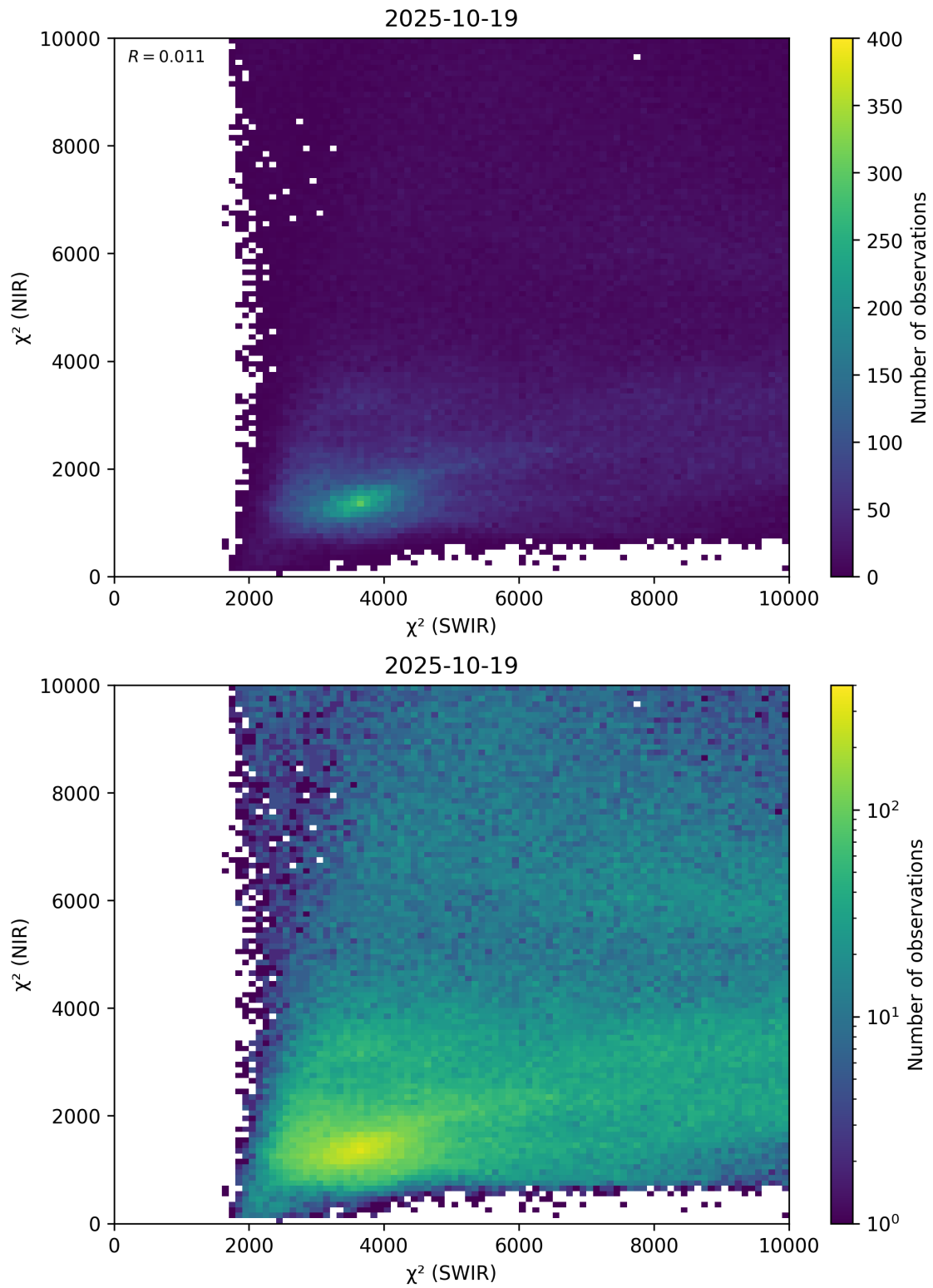
Figure 47: Scatter density plot of “ \chi^2 (SWIR)” against “ \chi^2 (NIR)” for 2025-10-18 to 2025-10-20.
