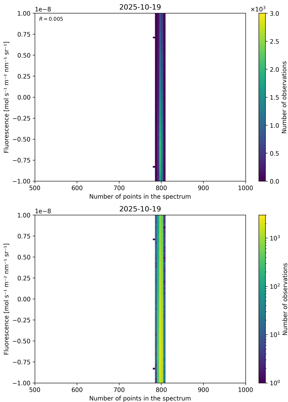
Figure 91: Scatter density plot of “Number of points in the spectrum” against “Fluorescence” for 2025-10-18 to 2025-10-20.
