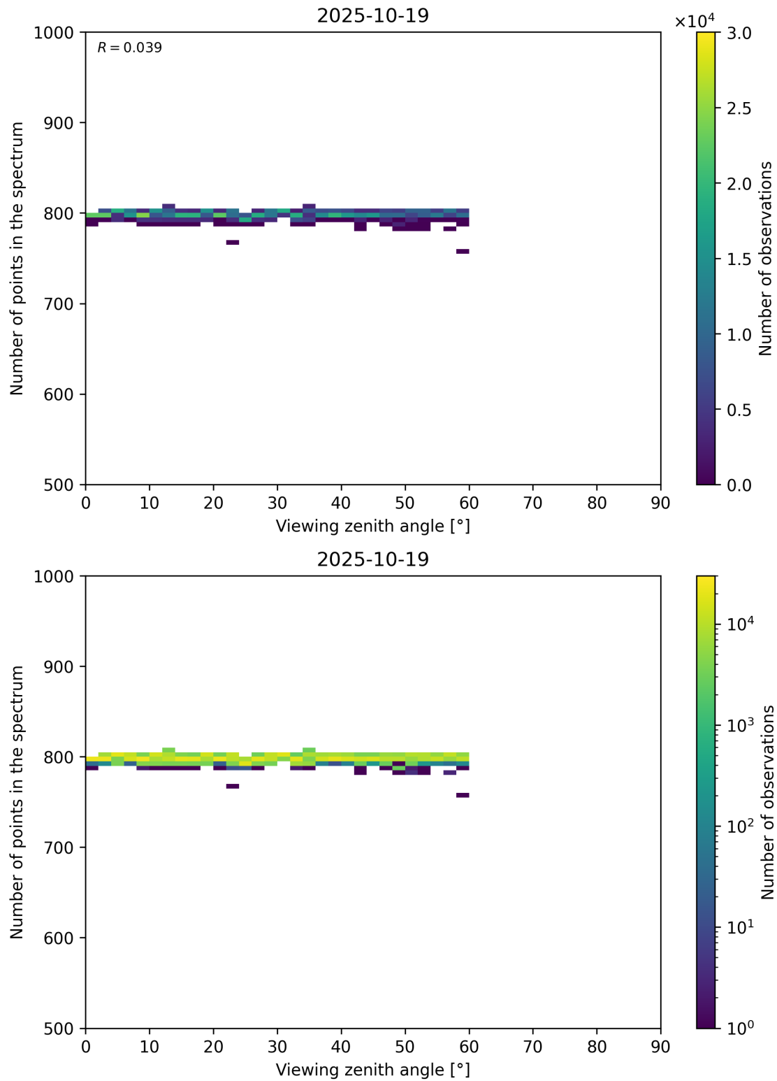
Figure 114: Scatter density plot of “Viewing zenith angle” against “Number of points in the spectrum” for 2025-10-18 to 2025-10-20.
