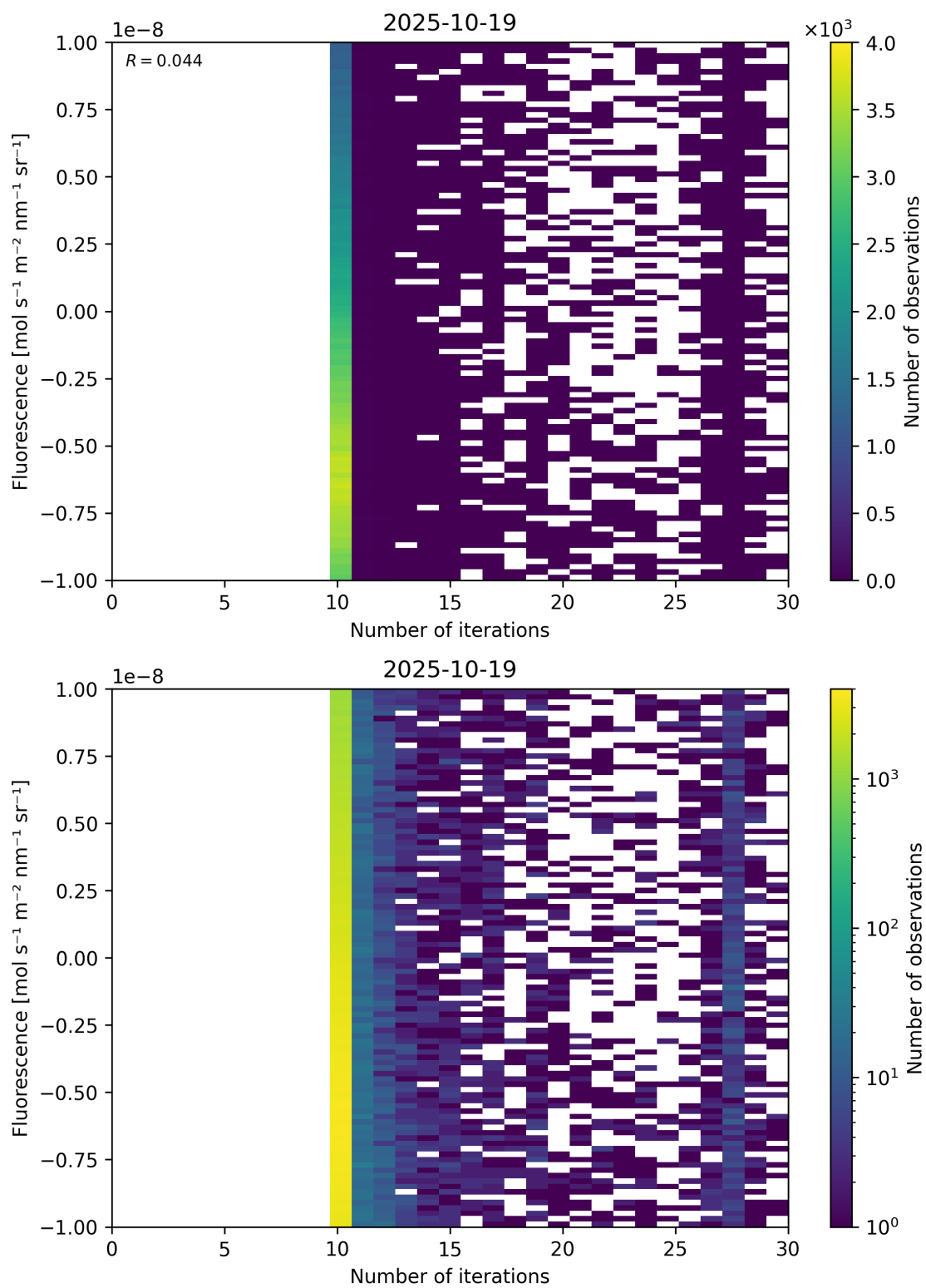
Figure 87: Scatter density plot of “Number of iterations” against “Fluorescence” for 2025-10-18 to 2025-10-20.
