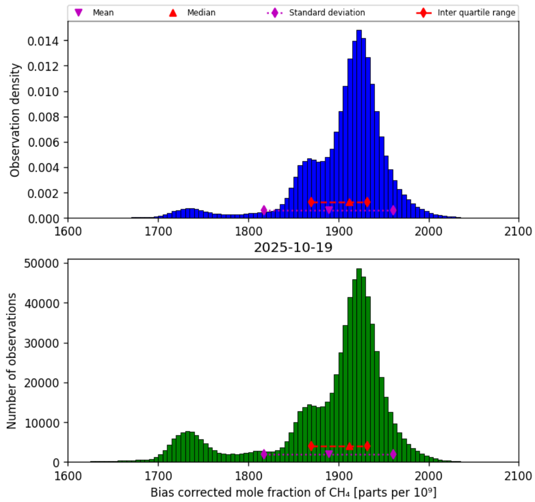
Figure 25: Histogram of "Bias corrected mole fraction of CH 4 " for 2025-10-18 to 2025-10-20
