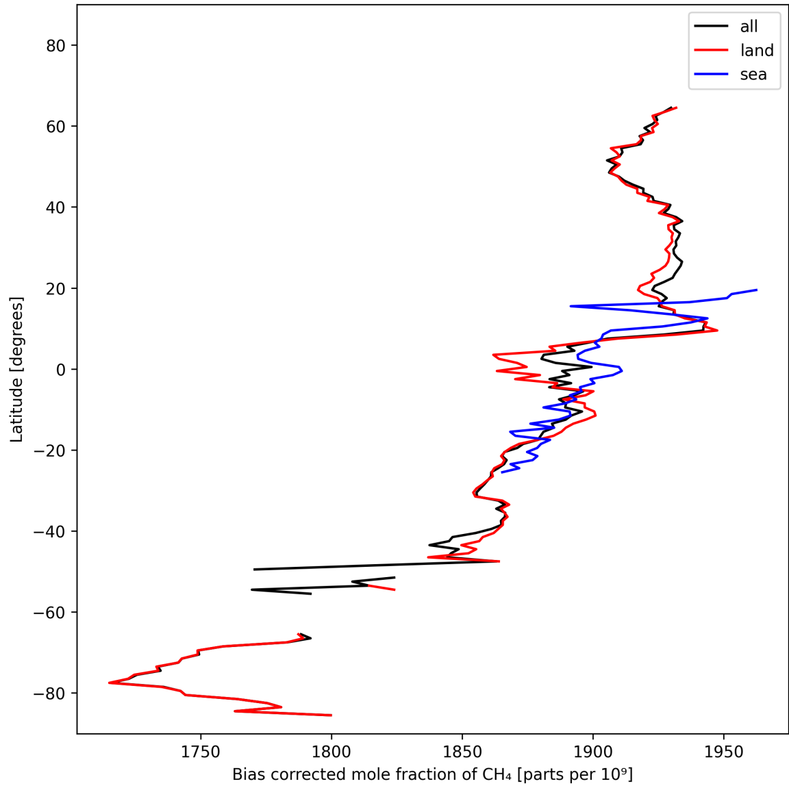
Figure 14: Zonal average of “Bias corrected mole fraction of CH 4 ” for 2025-10-18 to 2025-10-20.
