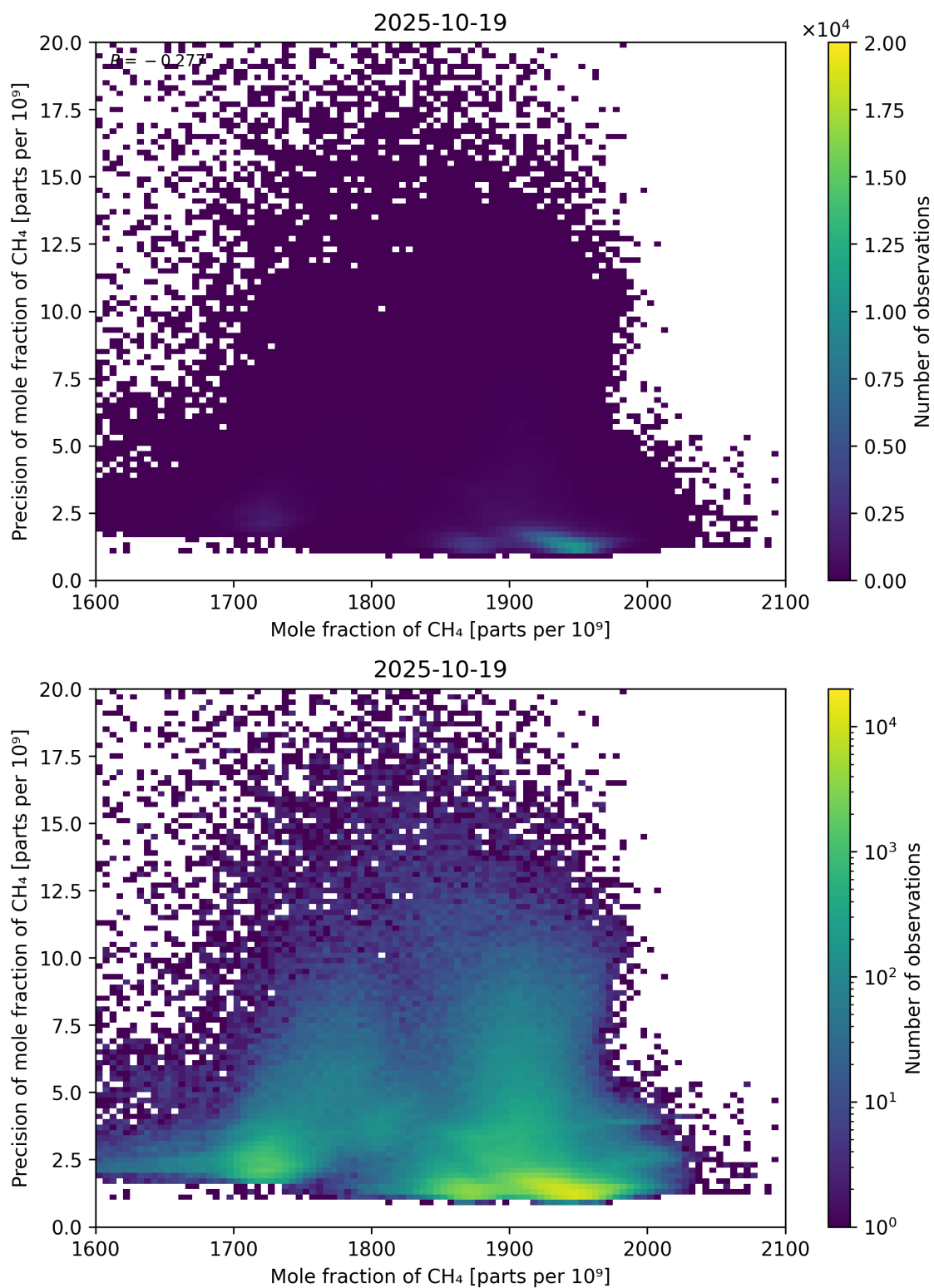
Figure 75: Scatter density plot of “Mole fraction of CH 4 ” against “Precision of mole fraction of CH 4 ” for 2025-10-18 to 2025-10-20.
