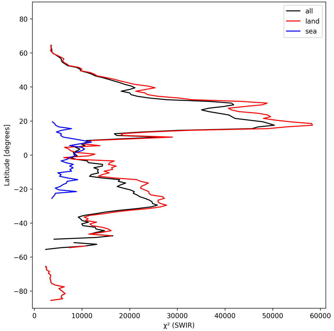
Figure 17: Zonal average of “ \chi^2 (SWIR)” for 2025-10-18 to 2025-10-20.
