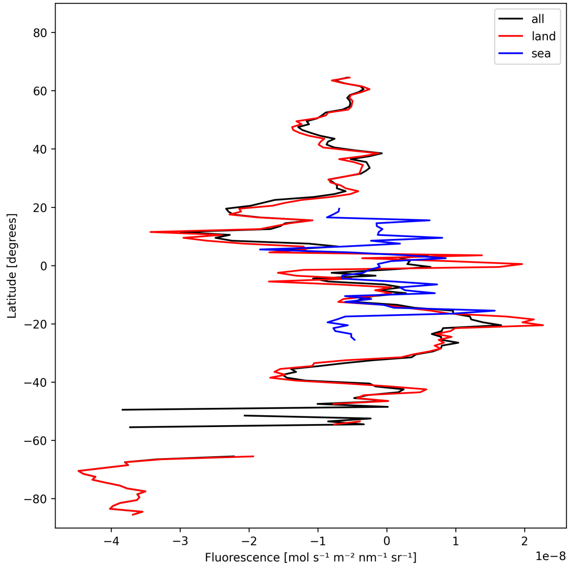
Figure 21: Zonal average of “Fluorescence” for 2025-10-18 to 2025-10-20.
