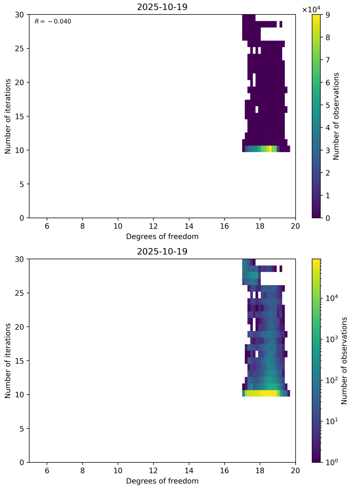
Figure 52: Scatter density plot of “Degrees of freedom” against “Number of iterations” for 2025-10-18 to 2025-10-20.
