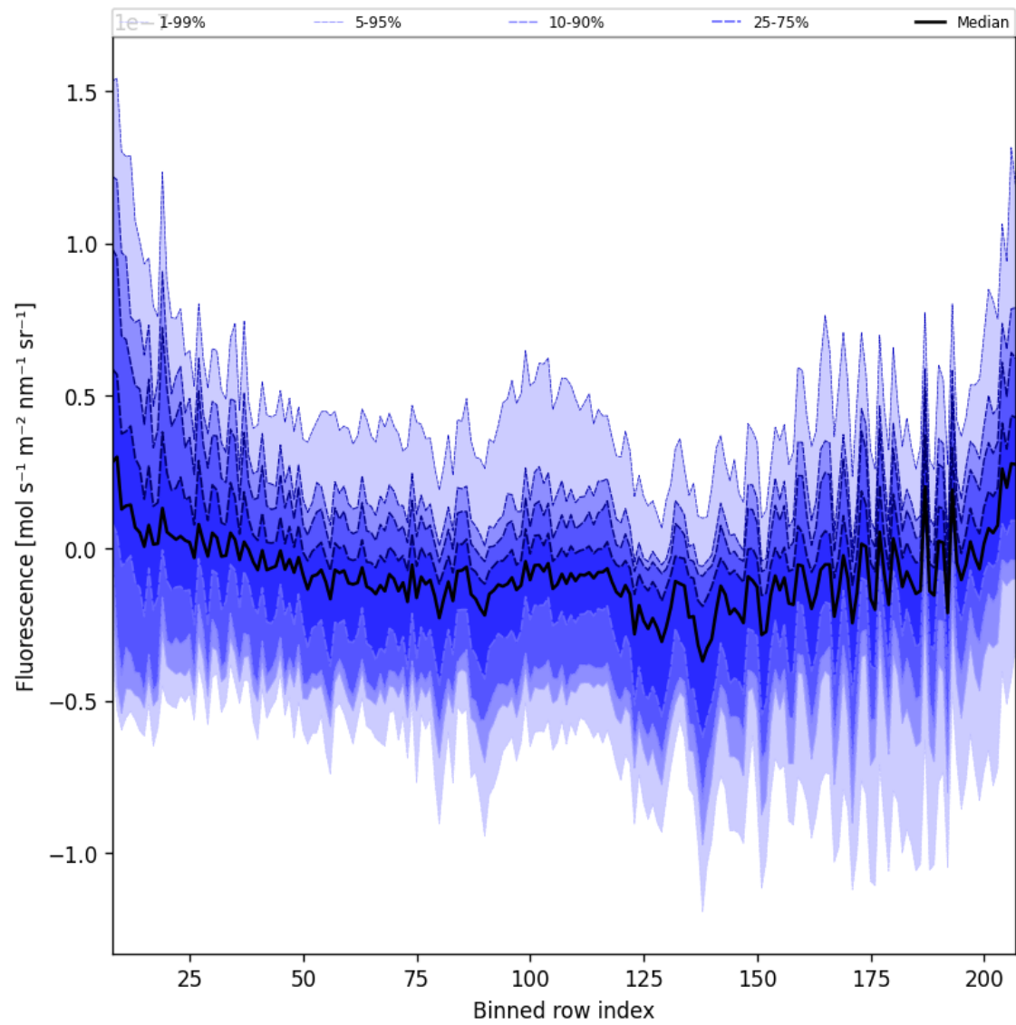
Figure 43: Along track statistics of “Fluorescence” for 2025-10-18 to 2025-10-20
