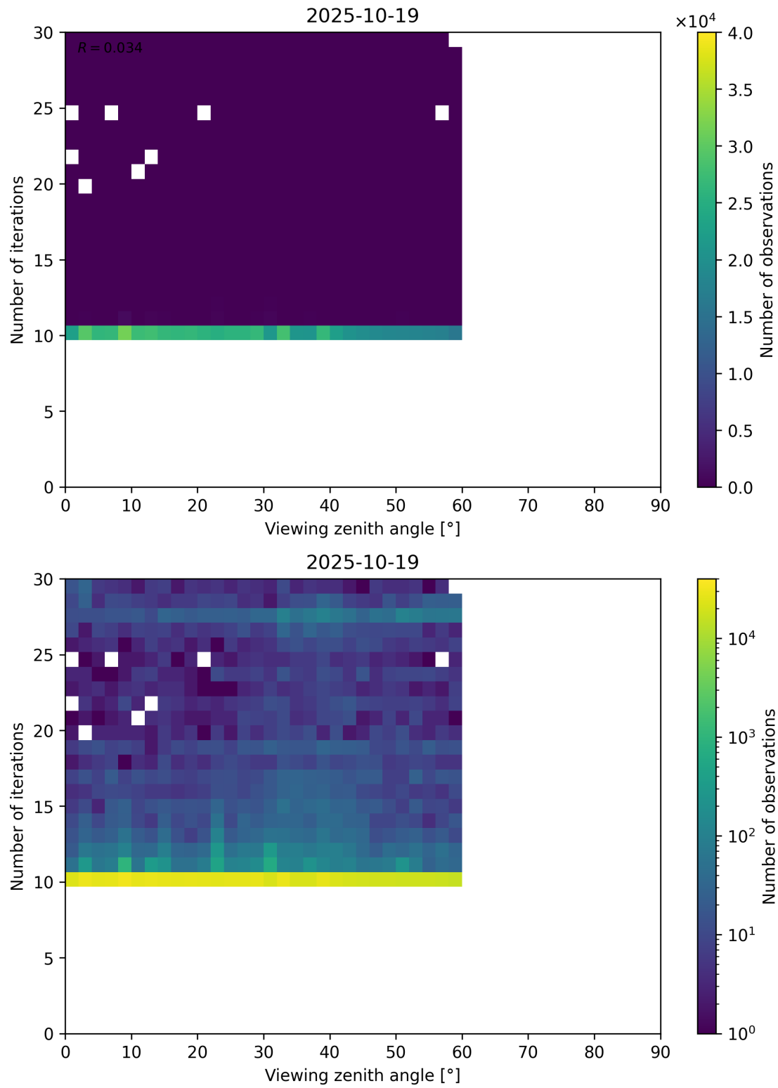
Figure 113: Scatter density plot of “Viewing zenith angle” against “Number of iterations” for 2025-10-18 to 2025-10-20.
