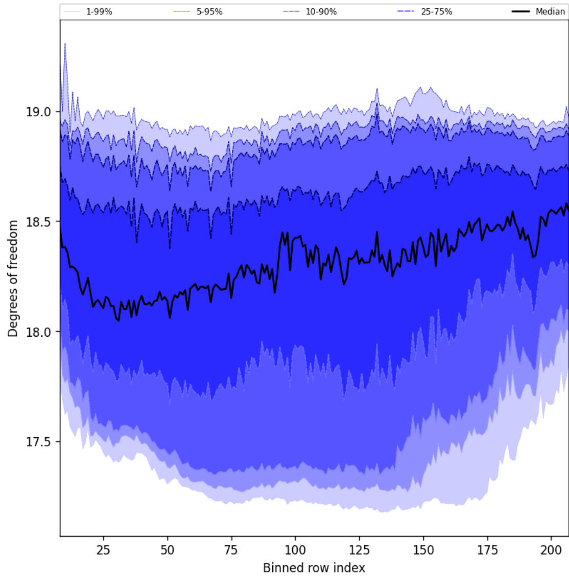
Figure 41: Along track statistics of “Degrees of freedom” for 2025-10-18 to 2025-10-20
