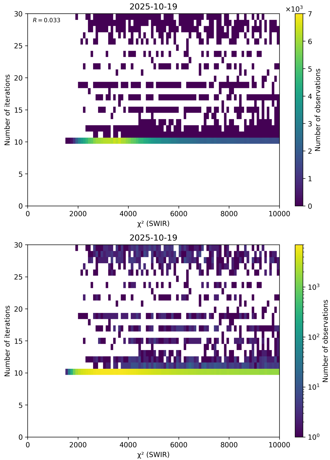
Figure 50: Scatter density plot of “ \chi^2 (SWIR)” against “Number of iterations” for 2025-10-18 to 2025-10-20.
