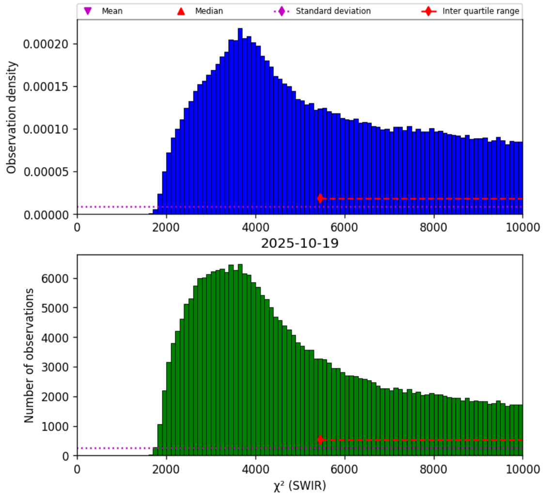
Figure 28: Histogram of “ \chi^2 (SWIR)” for 2025-10-18 to 2025-10-20
