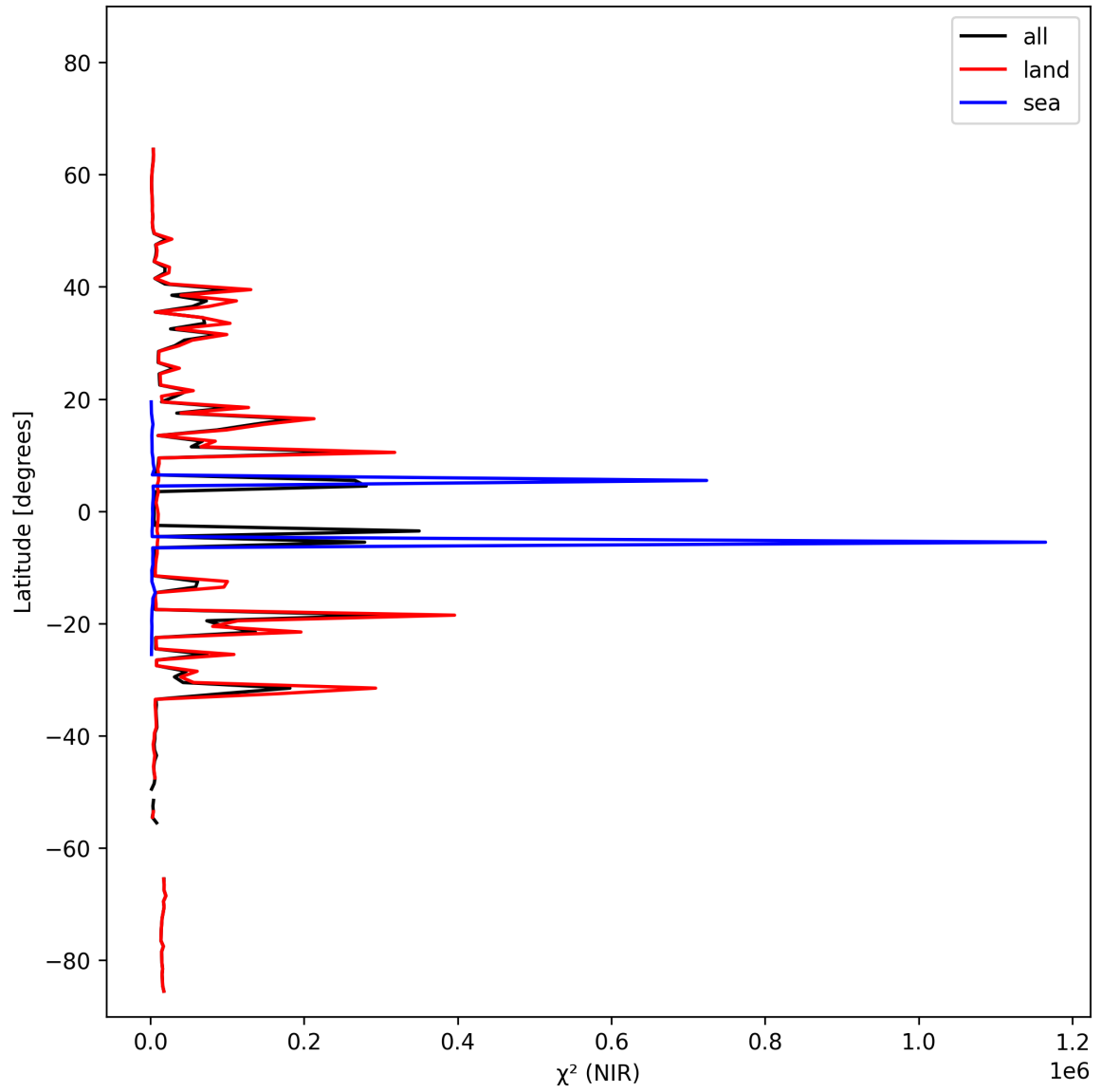
Figure 18: Zonal average of “ \chi^2 (NIR)” for 2025-10-18 to 2025-10-20.
