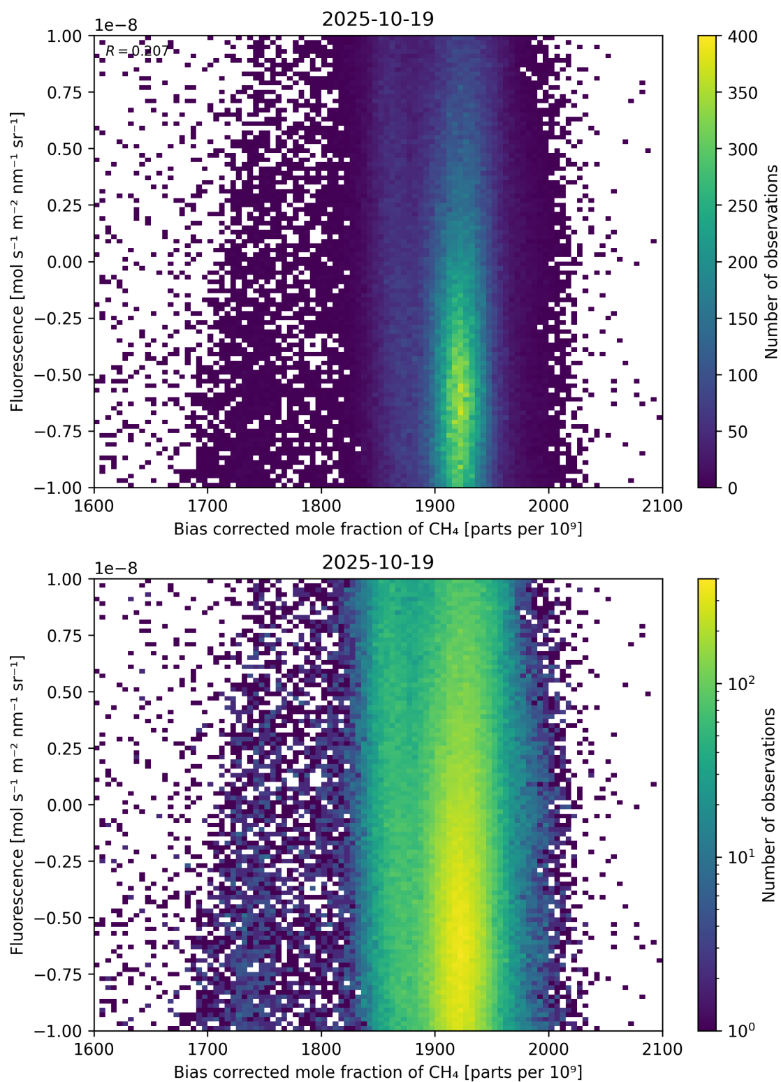
Figure 66: Scatter density plot of “Bias corrected mole fraction of \text{CH}_4 ” against “Fluorescence” for 2025-10-18 to 2025-10-20.
