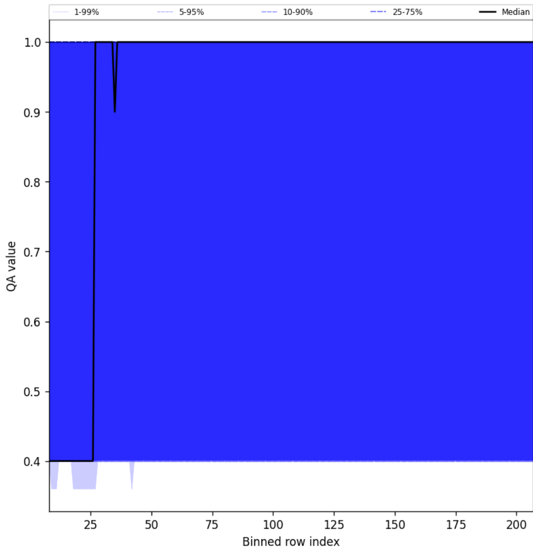
Figure 33: Along track statistics of “QA value” for 2025-10-18 to 2025-10-20
