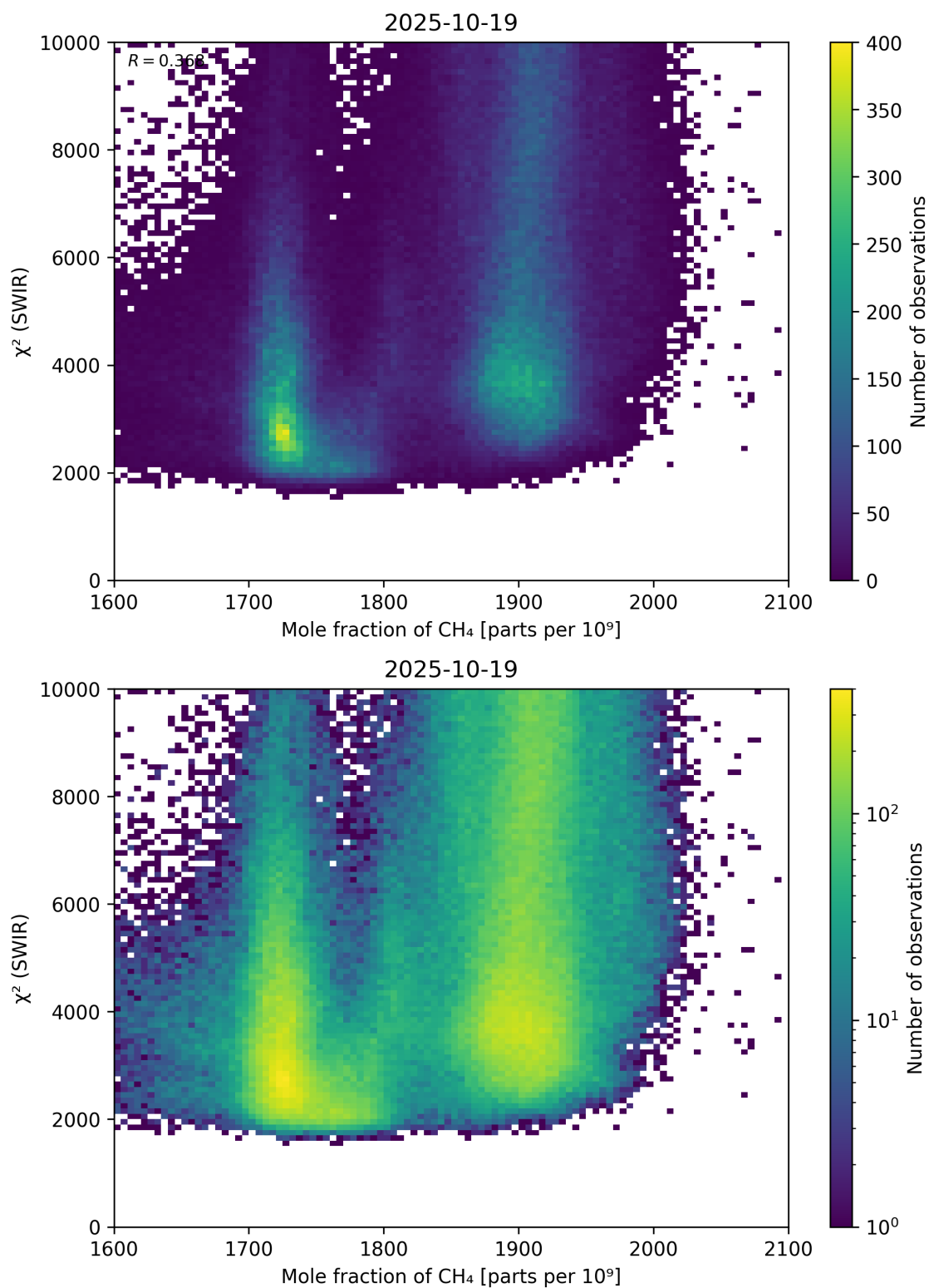
Figure 71: Scatter density plot of “Mole fraction of \text{CH}_4 ” against “ \chi^2 (SWIR)” for 2025-10-18 to 2025-10-20.
