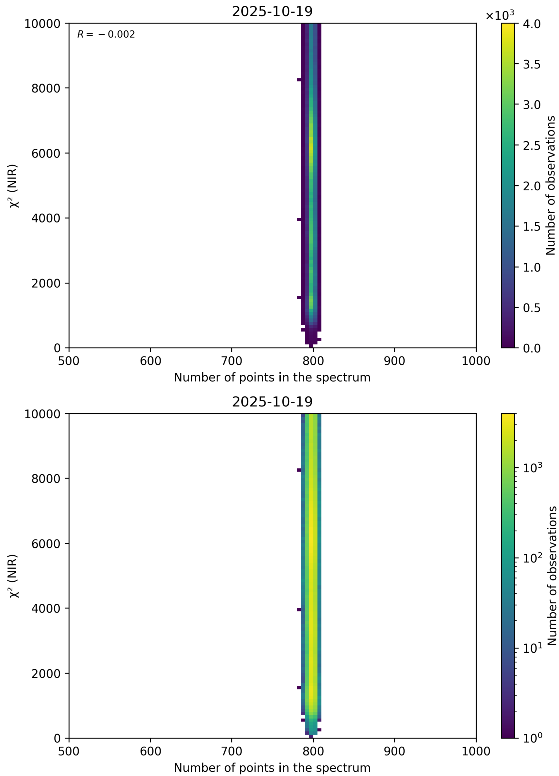
Figure 88: Scatter density plot of “Number of points in the spectrum” against “ \chi^2 (NIR)” for 2025-10-18 to 2025-10-20.
