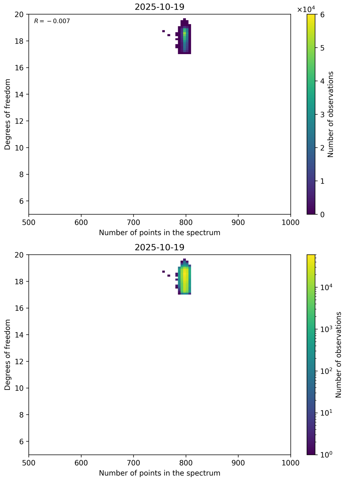
Figure 90: Scatter density plot of “Number of points in the spectrum” against “Degrees of freedom” for 2025-10-18 to 2025-10-20.
