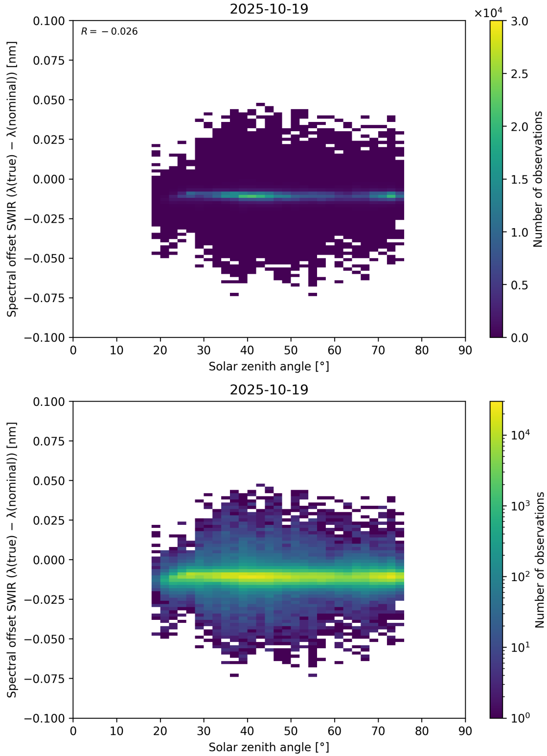
Figure 104: Scatter density plot of “Solar zenith angle” against “Spectral offset SWIR ( \lambda_{\text{true}} - \lambda_{\text{nominal}} )” for 2025-10-18 to 2025-10-20.
