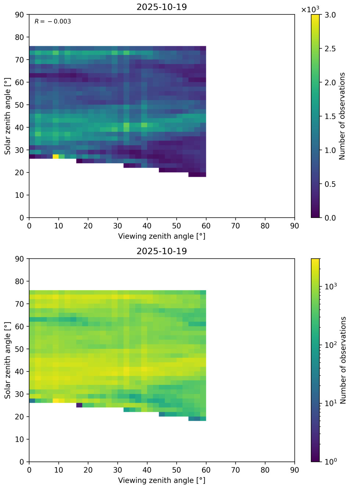
Figure 115: Scatter density plot of “Viewing zenith angle” against “Solar zenith angle” for 2025-10-18 to 2025-10-20.
