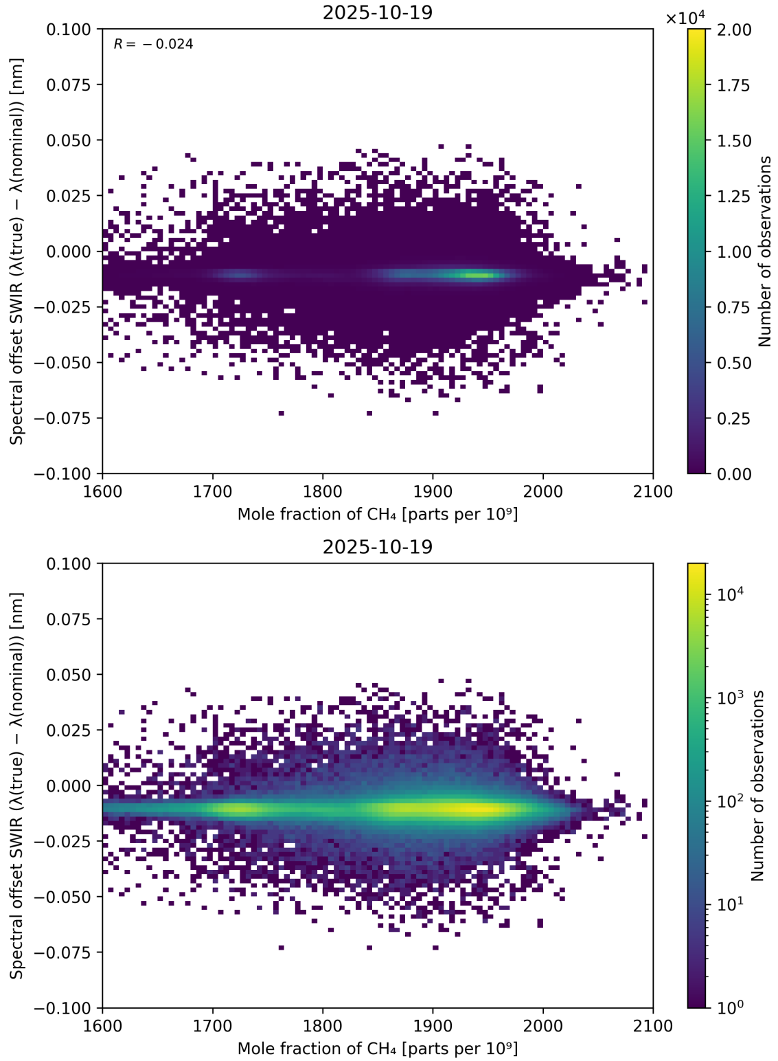
Figure 86: Scatter density plot of “Mole fraction of CH 4 ” against “Spectral offset SWIR ( \lambda_{\text{true}} - \lambda_{\text{nominal}} )” for 2025-10-18 to 2025-10-20.
