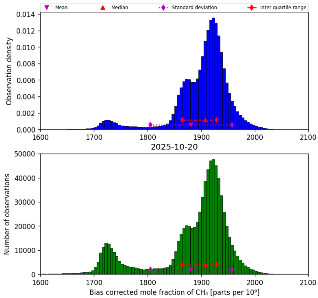
Figure 25: Histogram of “Bias corrected mole fraction of CH 4 ” for 2025-10-19 to 2025-10-21
