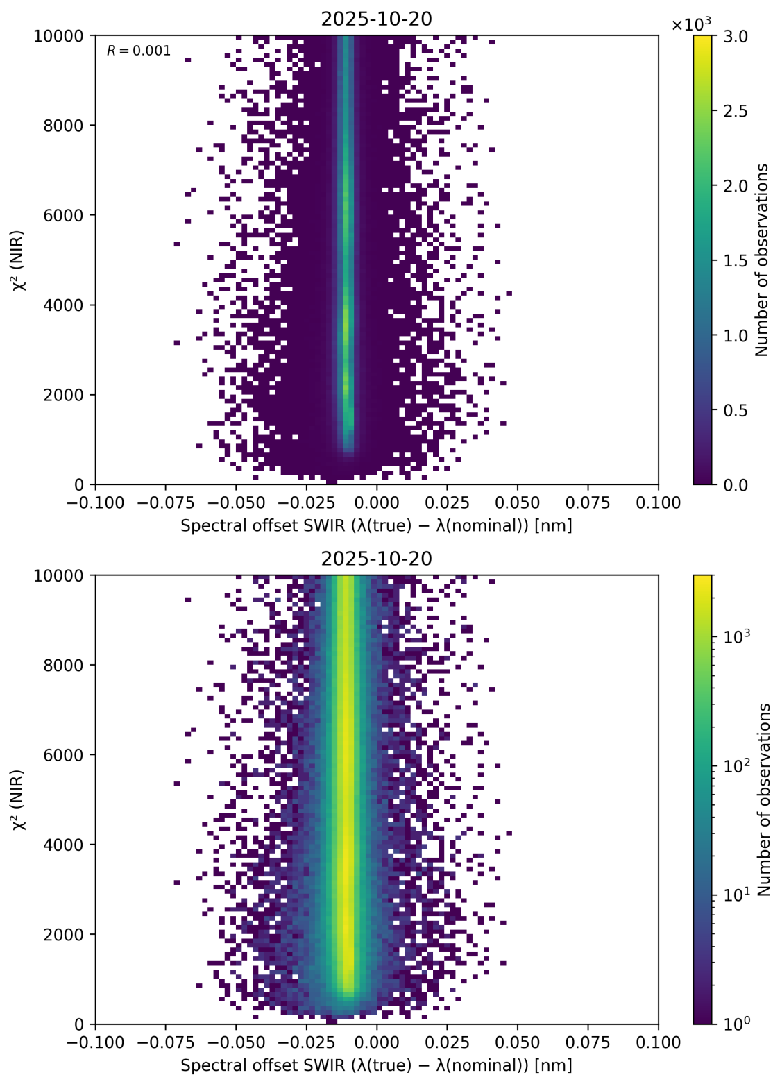
Figure 117: Scatter density plot of “Spectral offset SWIR ( \lambda_{\text{true}} - \lambda_{\text{nominal}} )” against “ \chi^2 (NIR)” for 2025-10-19 to 2025-10-21.
