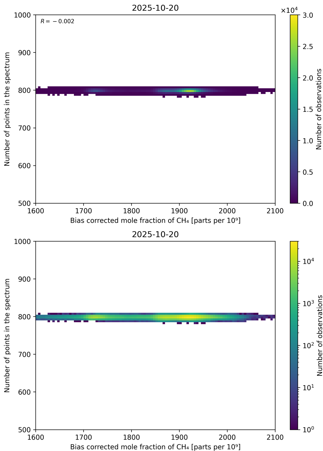
Figure 68: Scatter density plot of “Bias corrected mole fraction of CH 4 ” against “Number of points in the spectrum” for 2025-10-19 to 2025-10-21.
