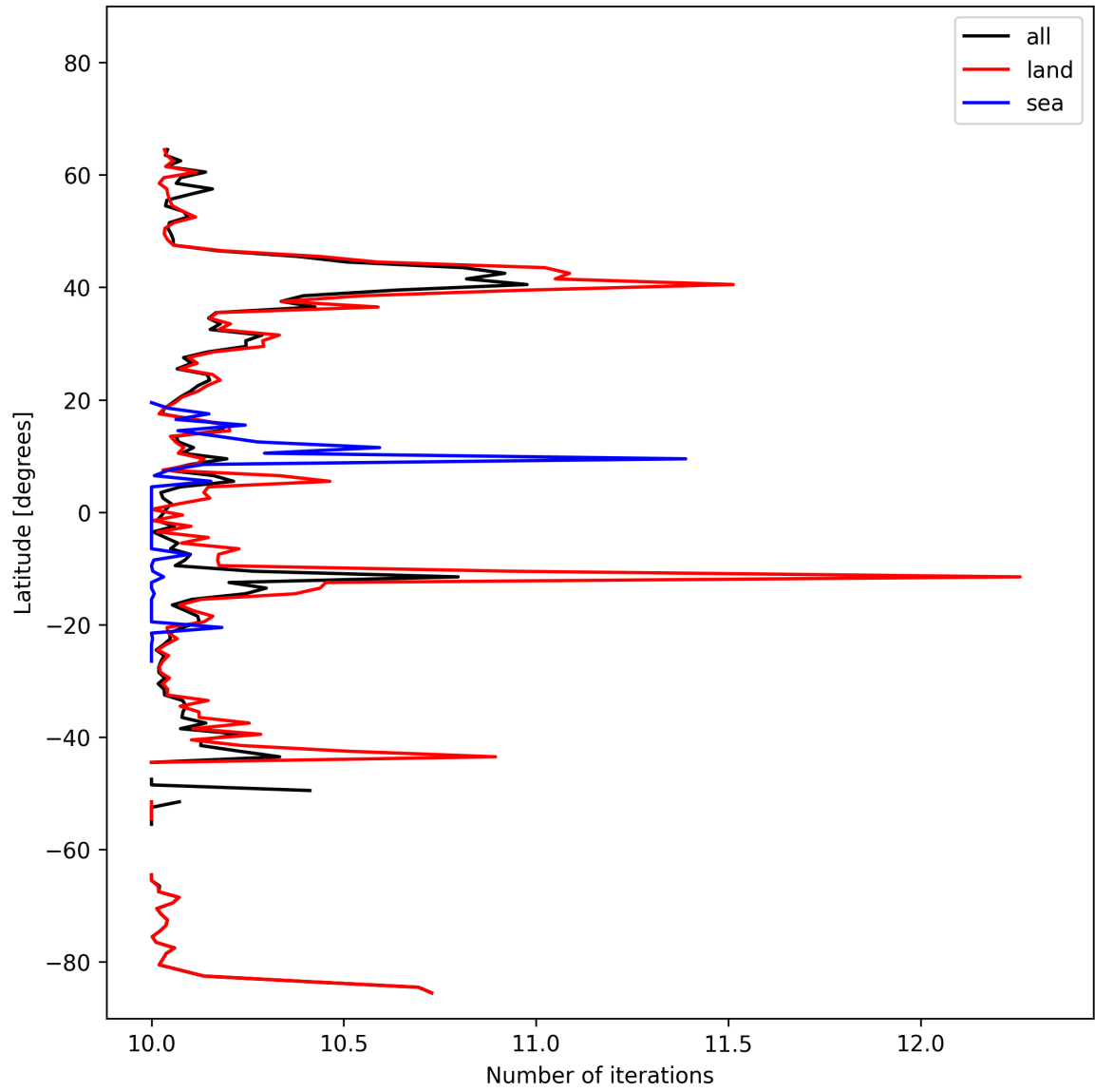
Figure 20: Zonal average of “Number of iterations” for 2025-10-19 to 2025-10-21.
