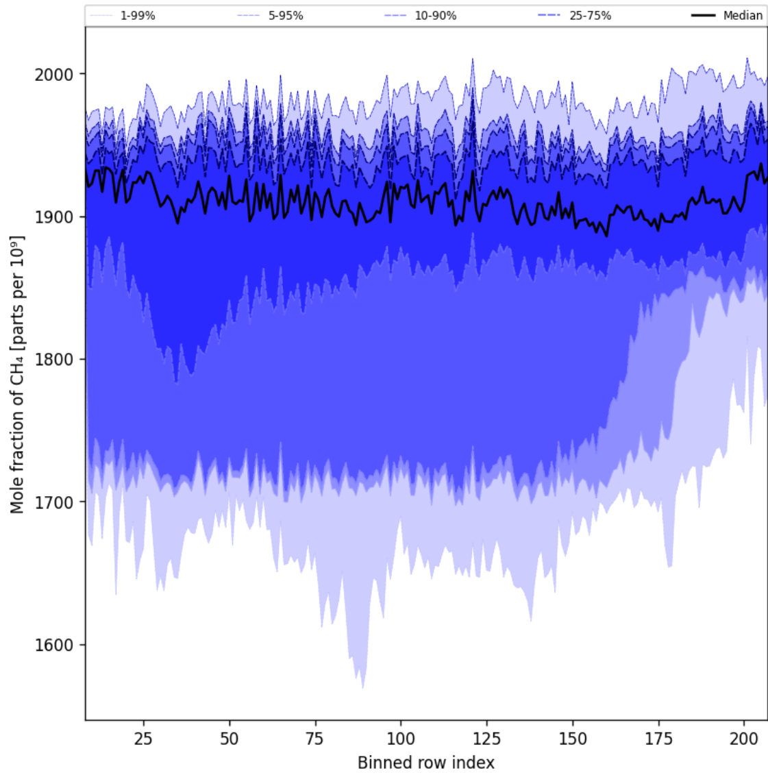
Figure 34: Along track statistics of “Mole fraction of CH 4 ” for 2025-10-19 to 2025-10-21
