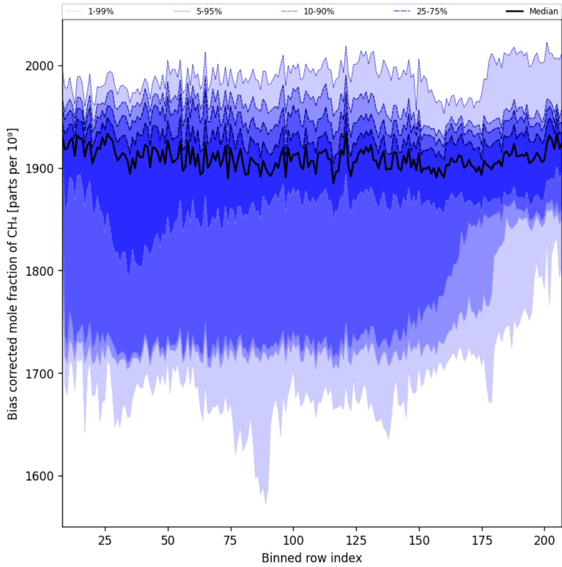
Figure 36: Along track statistics of “Bias corrected mole fraction of \text{CH}_4 ” for 2025-10-19 to 2025-10-21
