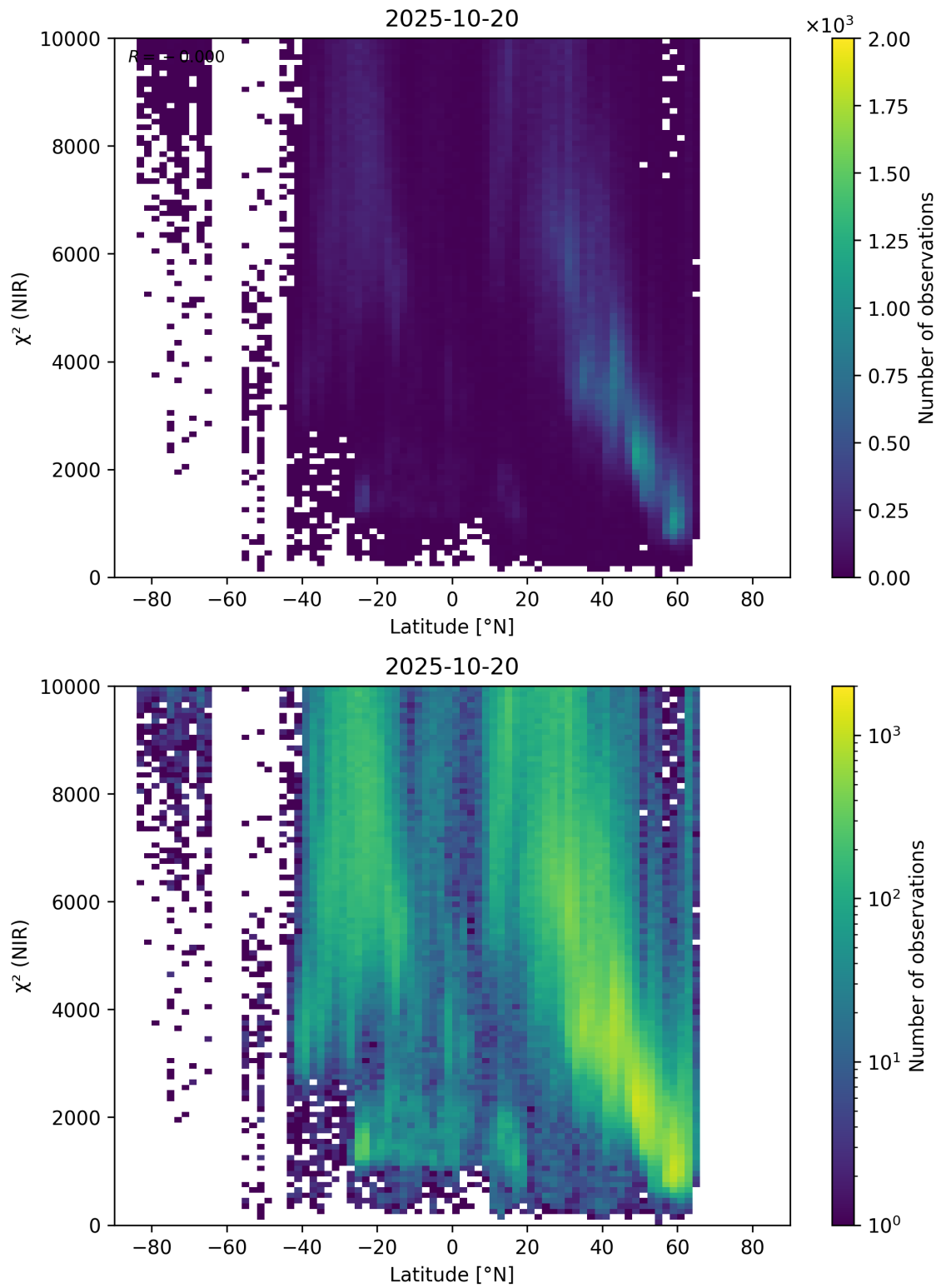
Figure 53: Scatter density plot of “Latitude” against “ \chi^2 (NIR)” for 2025-10-19 to 2025-10-21.
