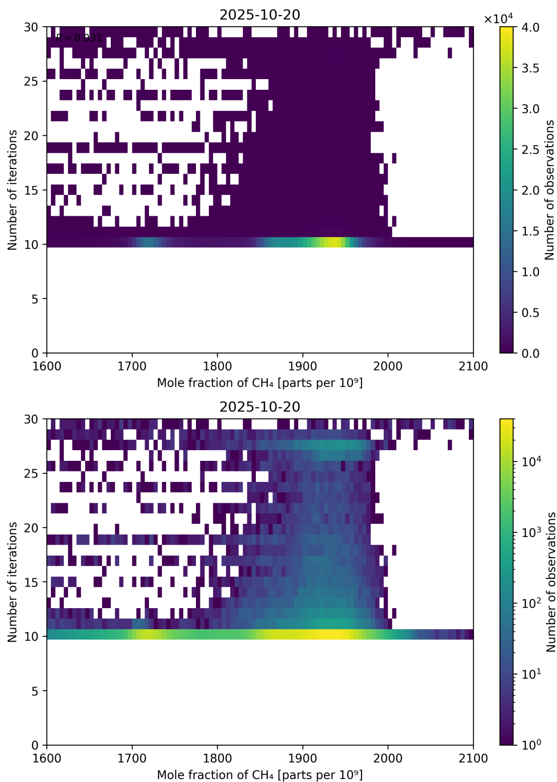
Figure 76: Scatter density plot of “Mole fraction of CH 4 ” against “Number of iterations” for 2025-10-19 to 2025-10-21.
