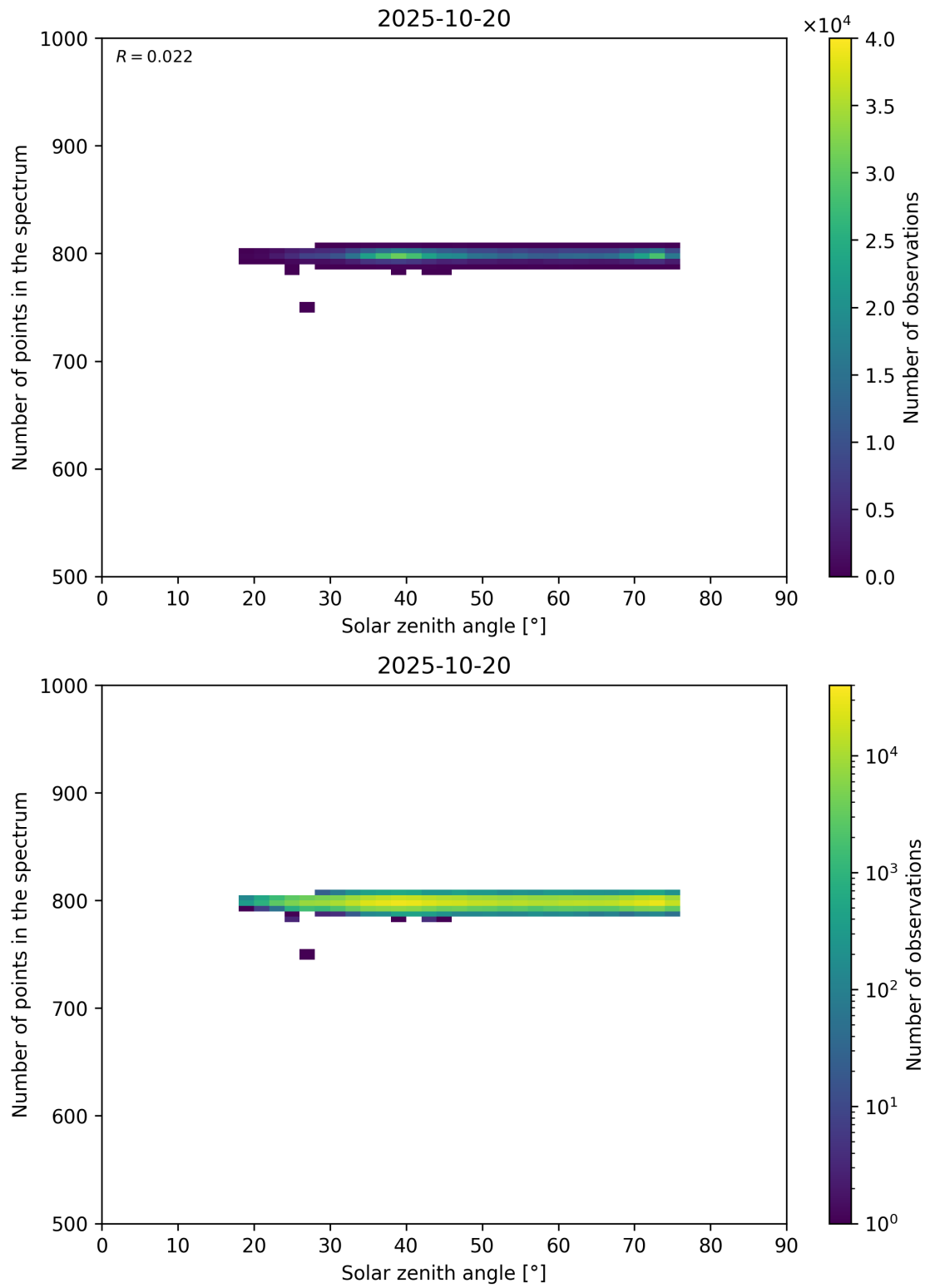
Figure 103: Scatter density plot of “Solar zenith angle” against “Number of points in the spectrum” for 2025-10-19 to 2025-10-21.
