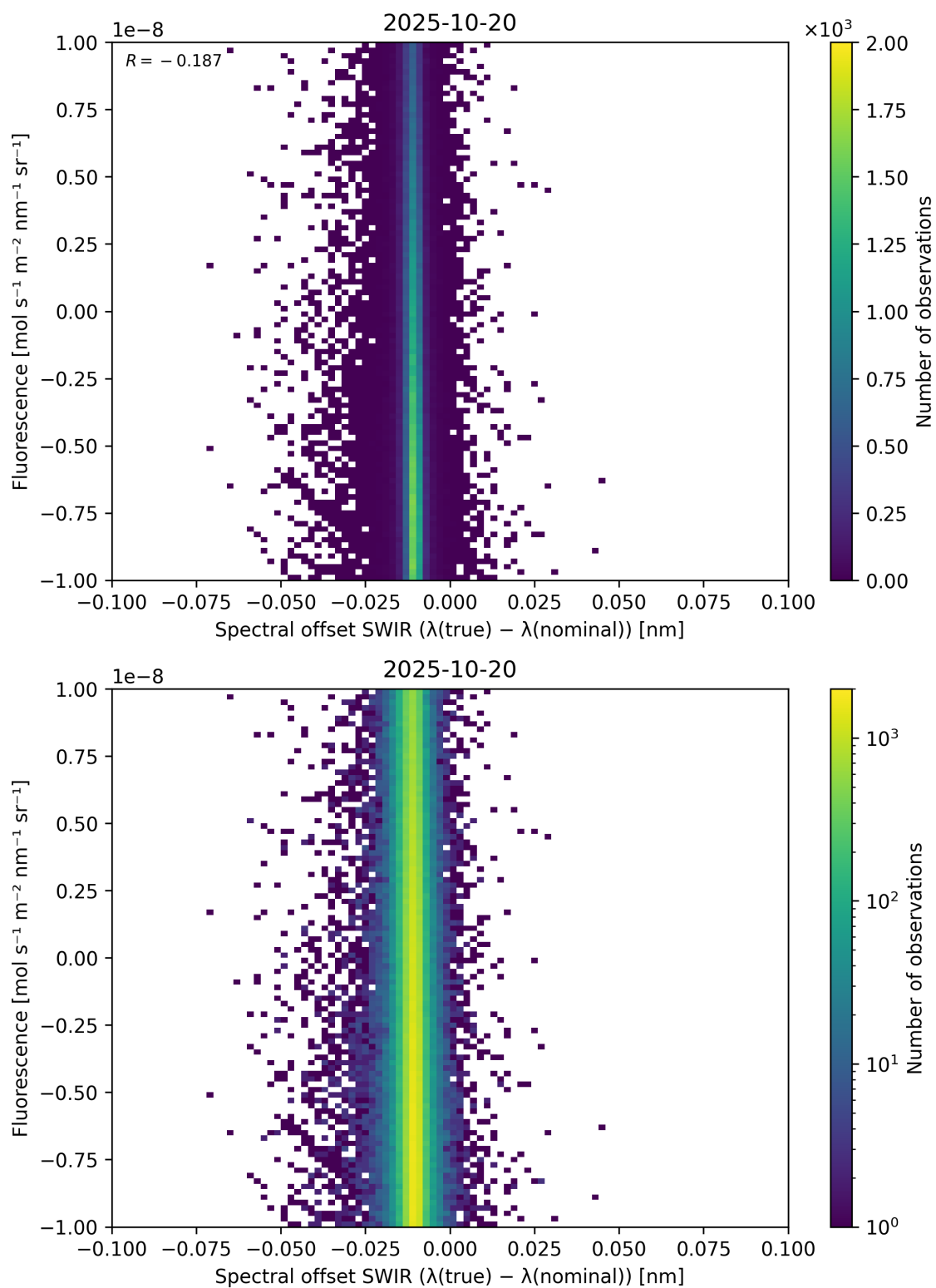
Figure 120: Scatter density plot of “Spectral offset SWIR ( \lambda_{\text{true}} - \lambda_{\text{nominal}} )” against “Fluorescence” for 2025-10-19 to 2025-10-21.
