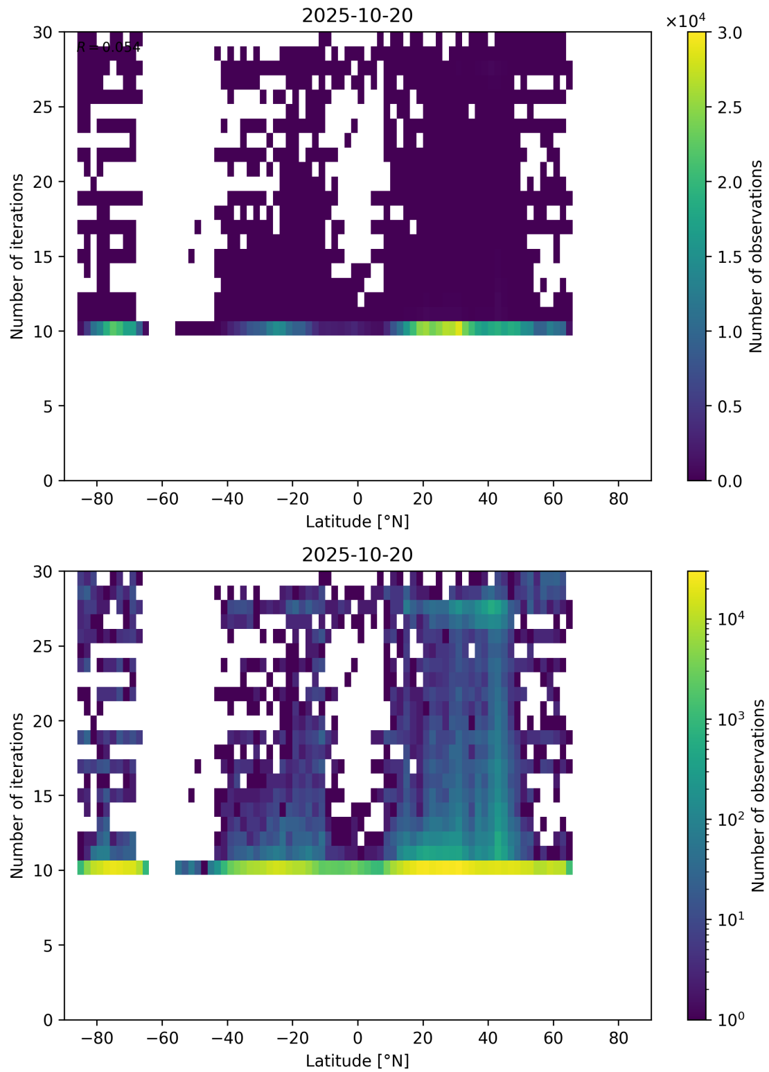
Figure 60: Scatter density plot of “Latitude” against “Number of iterations” for 2025-10-19 to 2025-10-21.
