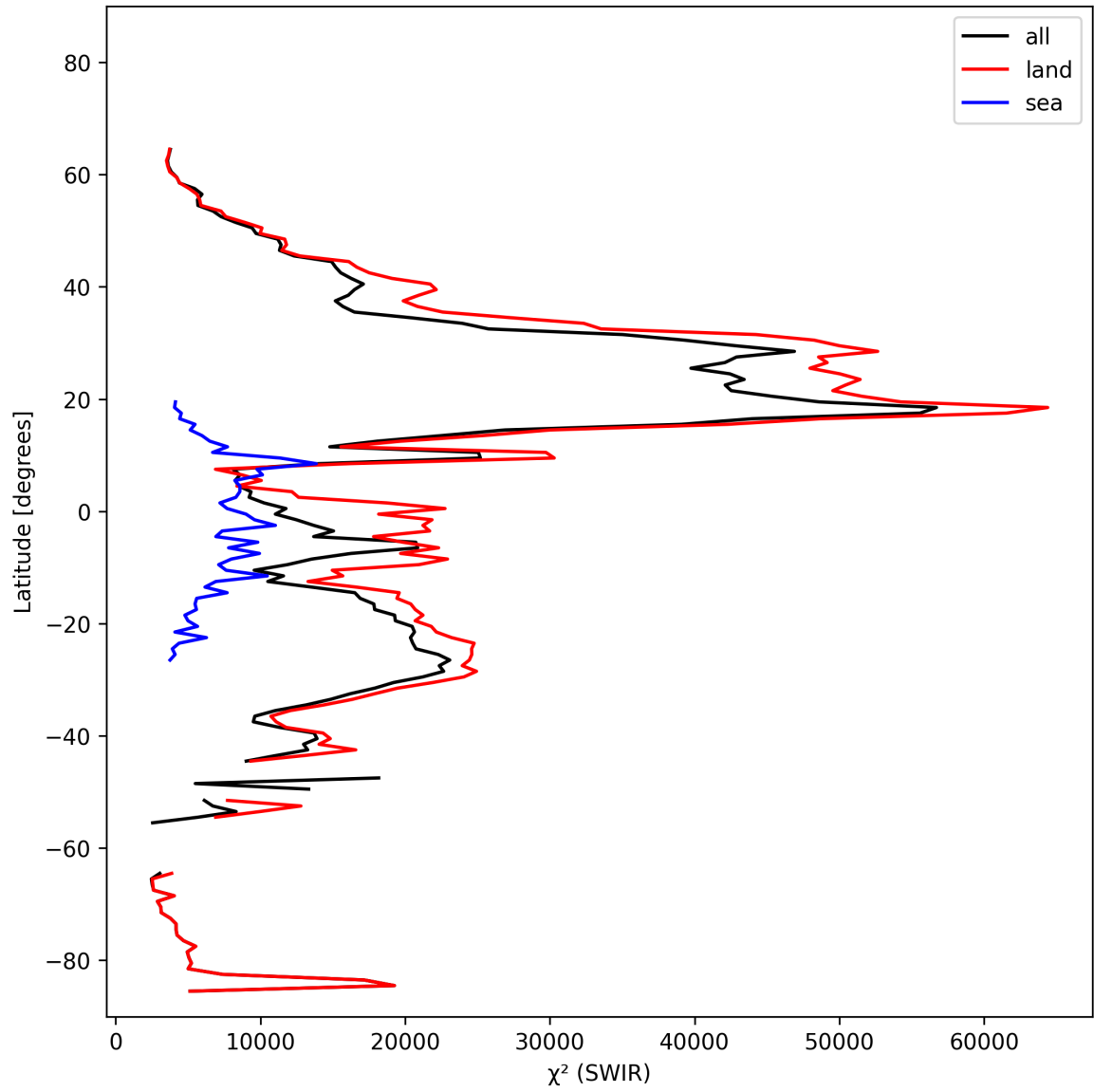
Figure 17: Zonal average of “ \chi^2 (SWIR)” for 2025-10-19 to 2025-10-21.
