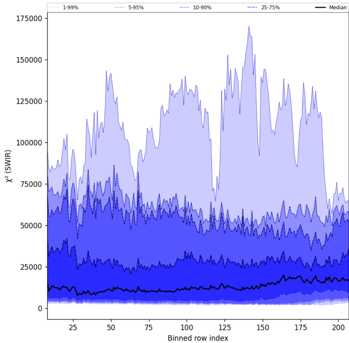
Figure 39: Along track statistics of “ \chi^2 (SWIR)” for 2025-10-19 to 2025-10-21
