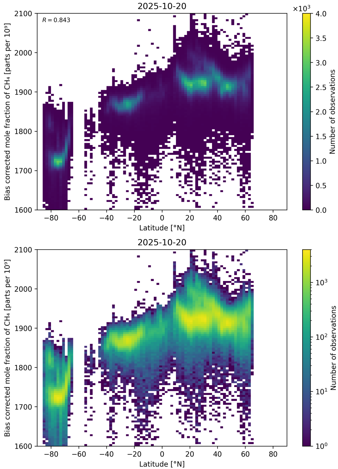
Figure 58: Scatter density plot of “Latitude” against “Bias corrected mole fraction of \text{CH}_4 ” for 2025-10-19 to 2025-10-21.
