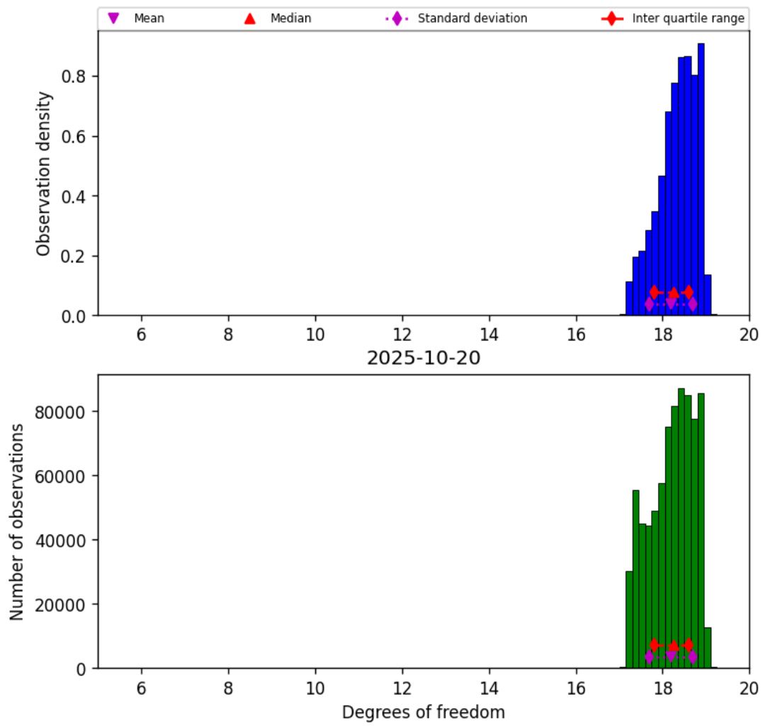
Figure 30: Histogram of “Degrees of freedom” for 2025-10-19 to 2025-10-21
