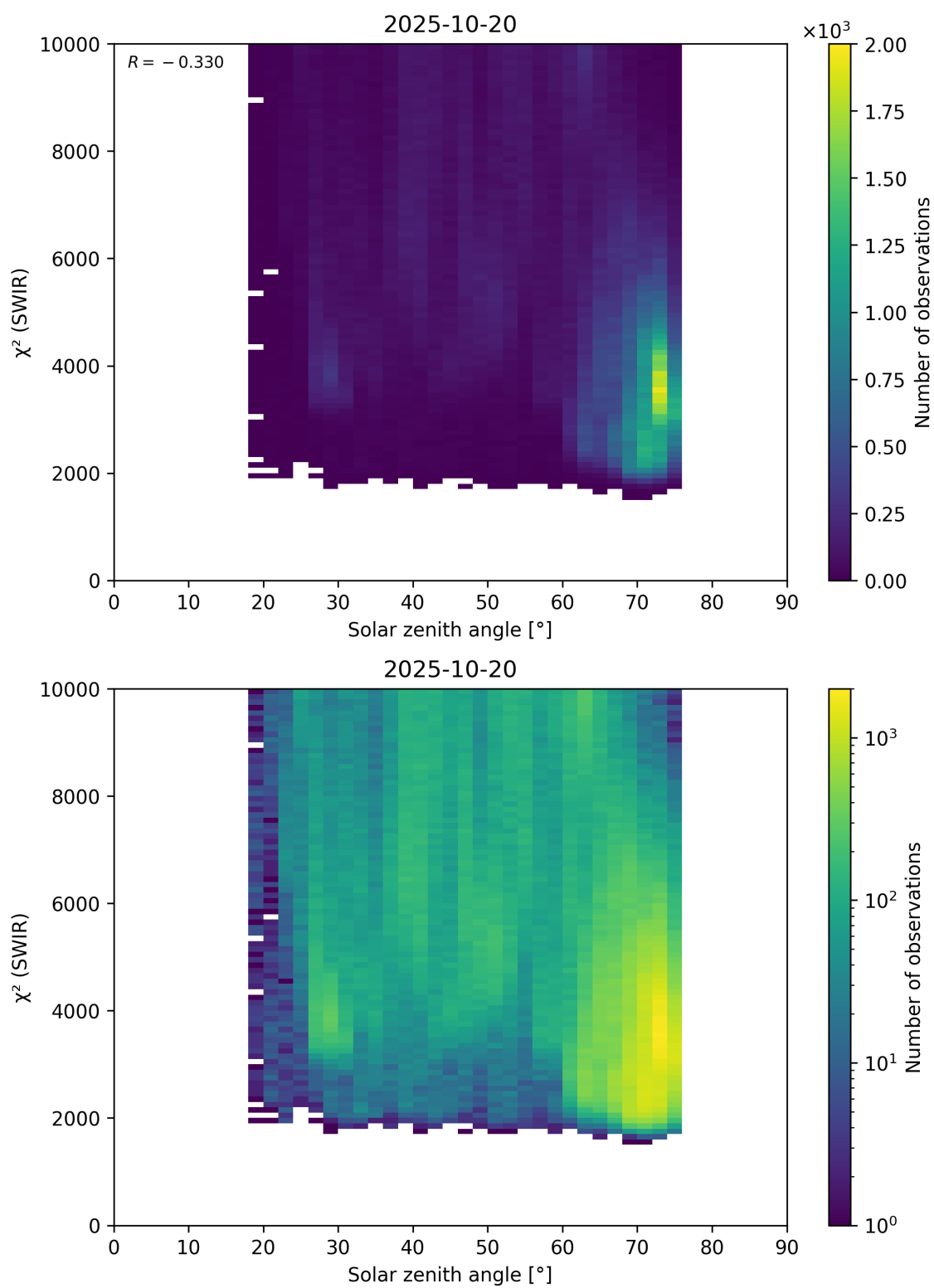
Figure 95: Scatter density plot of “Solar zenith angle” against “ \chi^2 (SWIR)” for 2025-10-19 to 2025-10-21.
