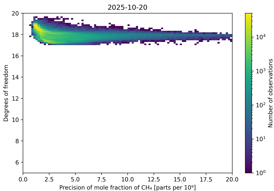
Figure 80: Scatter density plot of “Precision of mole fraction of CH 4 ” against “Degrees of freedom” for 2025-10-19 to 2025-10-21.
