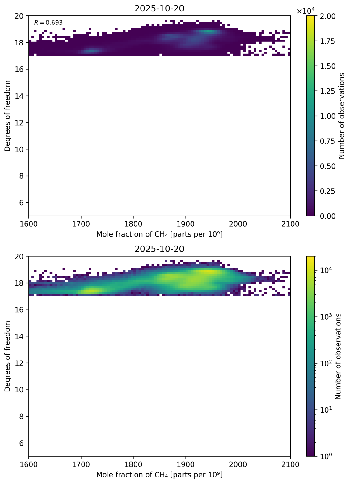
Figure 72: Scatter density plot of “Mole fraction of CH 4 ” against “Degrees of freedom” for 2025-10-19 to 2025-10-21.
