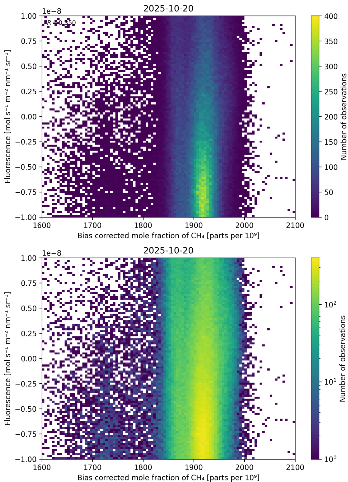
Figure 66: Scatter density plot of “Bias corrected mole fraction of \text{CH}_4 ” against “Fluorescence” for 2025-10-19 to 2025-10-21.
