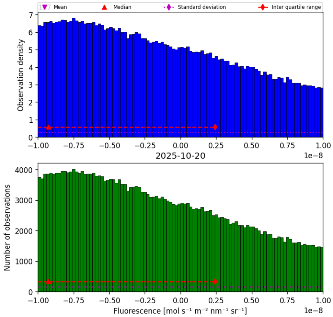
Figure 32: Histogram of “Fluorescence” for 2025-10-19 to 2025-10-21
