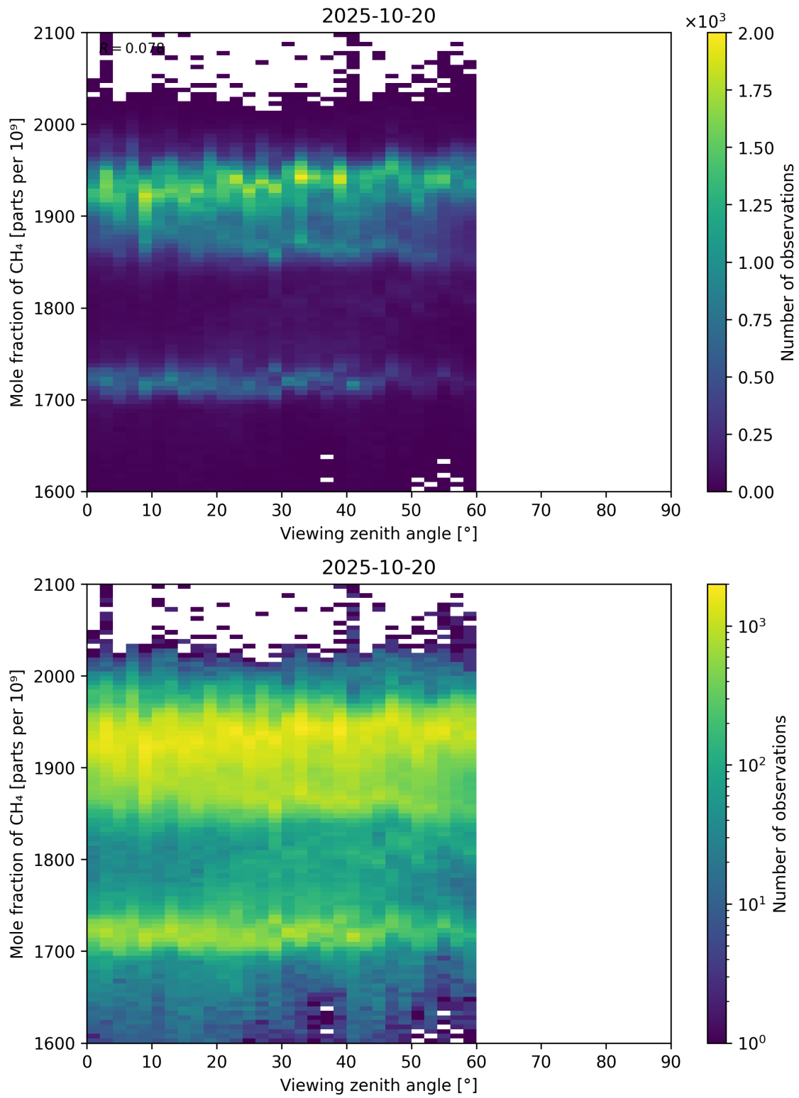
Figure 110: Scatter density plot of “Viewing zenith angle” against “Mole fraction of CH 4 ” for 2025-10-19 to 2025-10-21.
