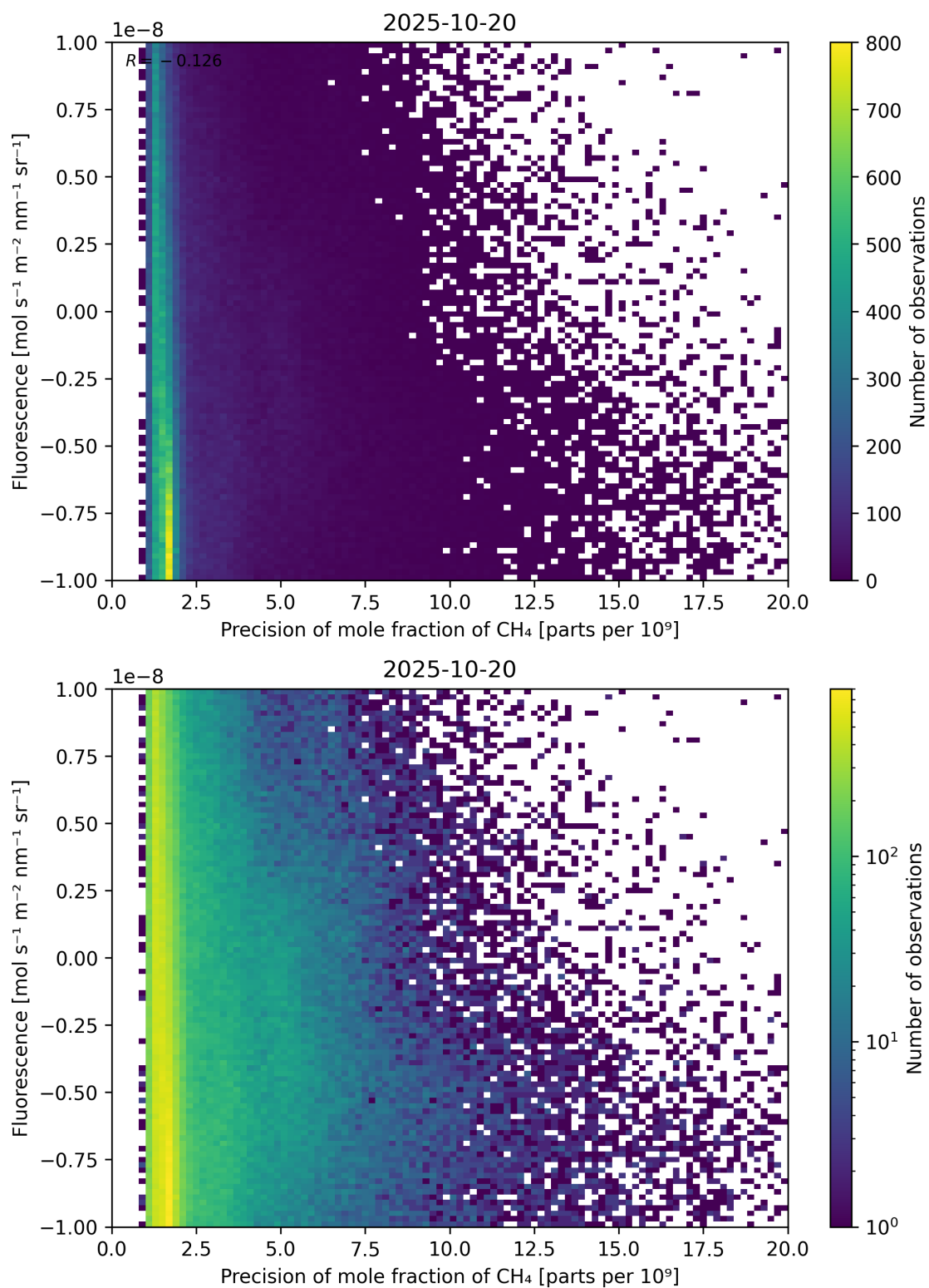
Figure 81: Scatter density plot of “Precision of mole fraction of \text{CH}_4 ” against “Fluorescence” for 2025-10-19 to 2025-10-21.
