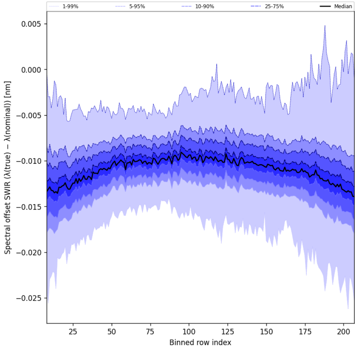
Figure 38: Along track statistics of “Spectral offset SWIR ( \lambda_{\text{true}} - \lambda_{\text{nominal}} )” for 2025-10-19 to 2025-10-21
