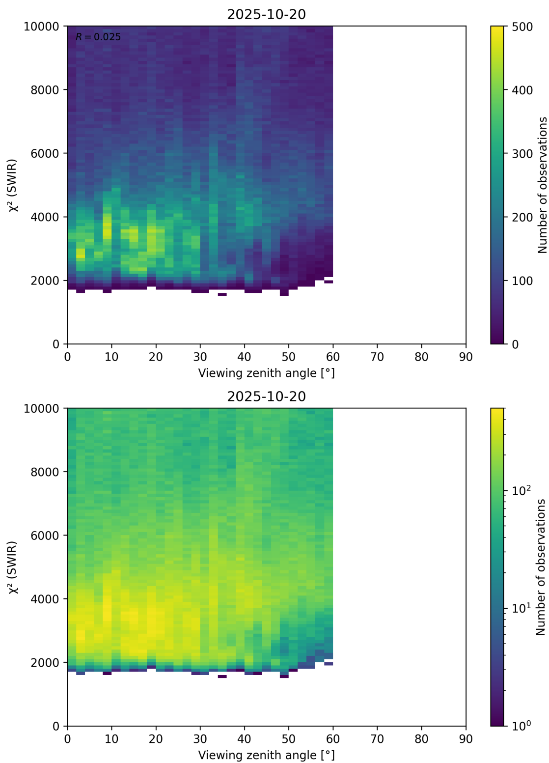
Figure 106: Scatter density plot of “Viewing zenith angle” against “ \chi^2 (SWIR)” for 2025-10-19 to 2025-10-21.
