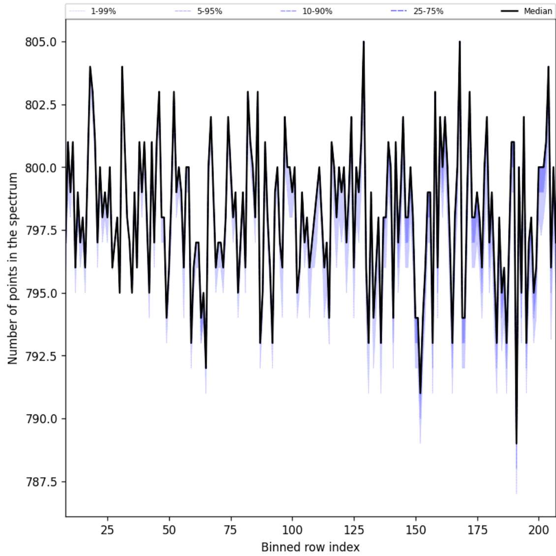
Figure 37: Along track statistics of “Number of points in the spectrum” for 2025-10-19 to 2025-10-21
