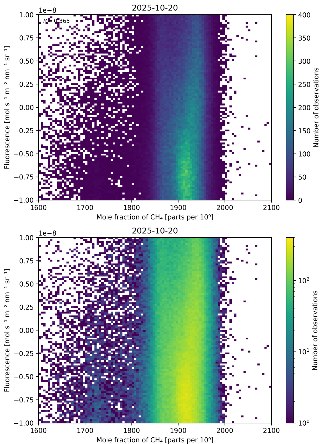
Figure 73: Scatter density plot of “Mole fraction of \text{CH}_4 ” against “Fluorescence” for 2025-10-19 to 2025-10-21.
