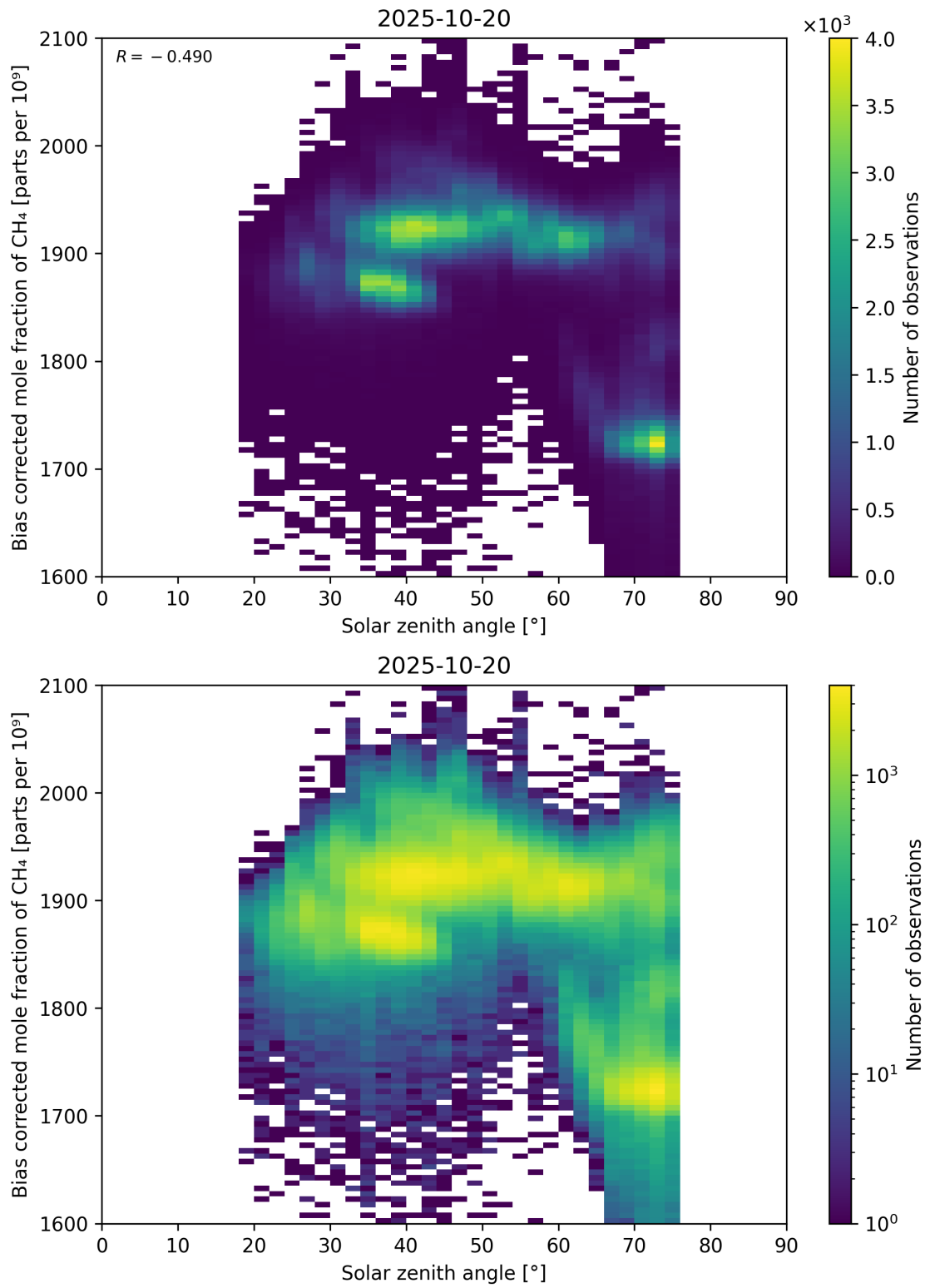
Figure 100: Scatter density plot of “Solar zenith angle” against “Bias corrected mole fraction of \text{CH}_4 ” for 2025-10-19 to 2025-10-21.
