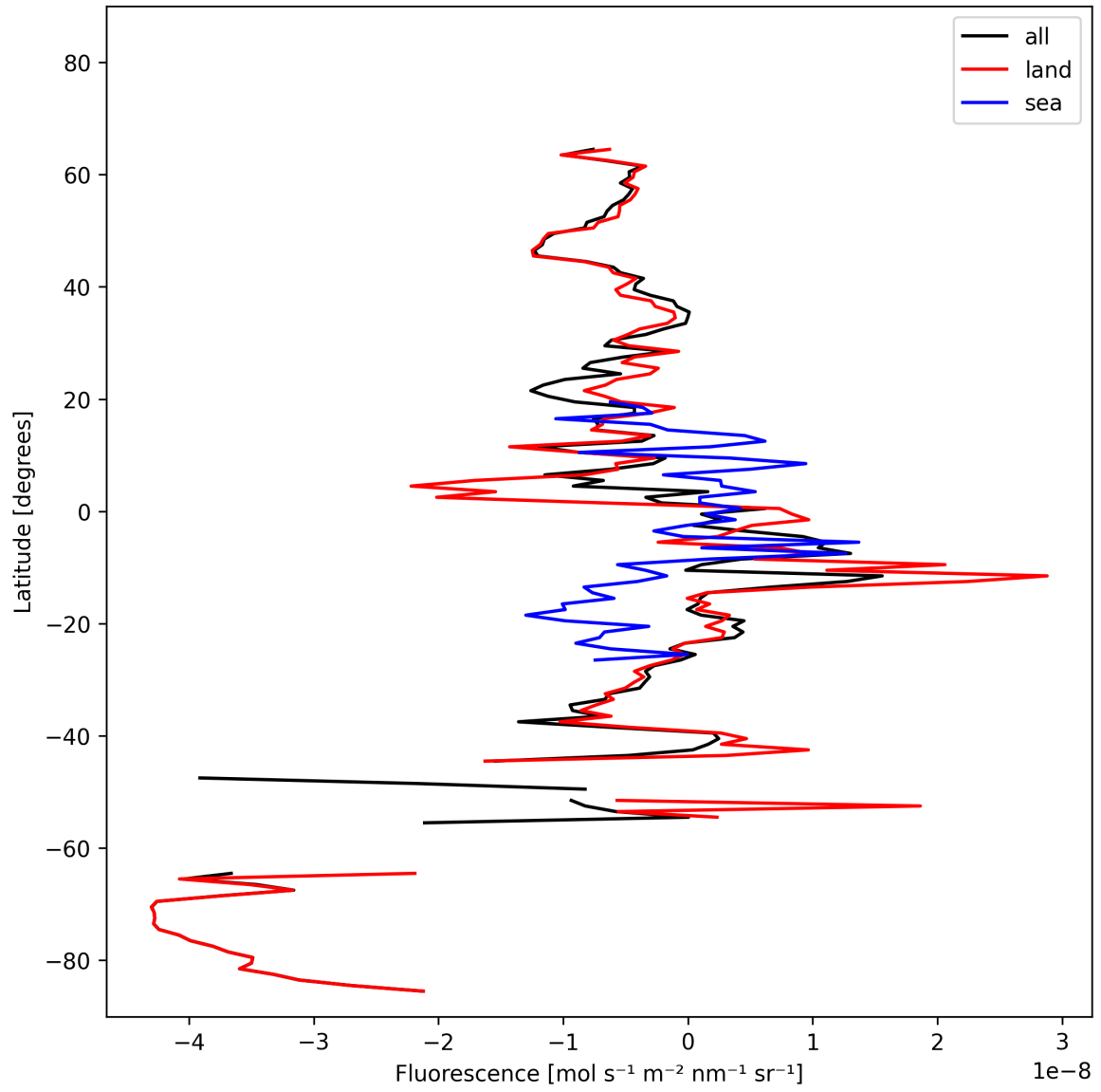
Figure 21: Zonal average of “Fluorescence” for 2025-10-19 to 2025-10-21.
