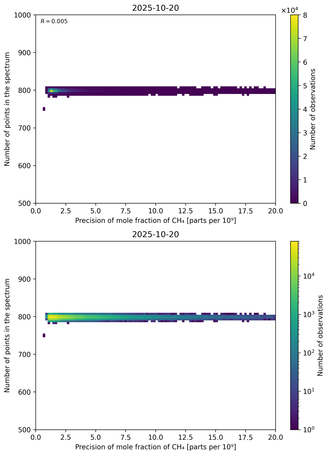
Figure 84: Scatter density plot of “Precision of mole fraction of CH 4 ” against “Number of points in the spectrum” for 2025-10-19 to 2025-10-21.
