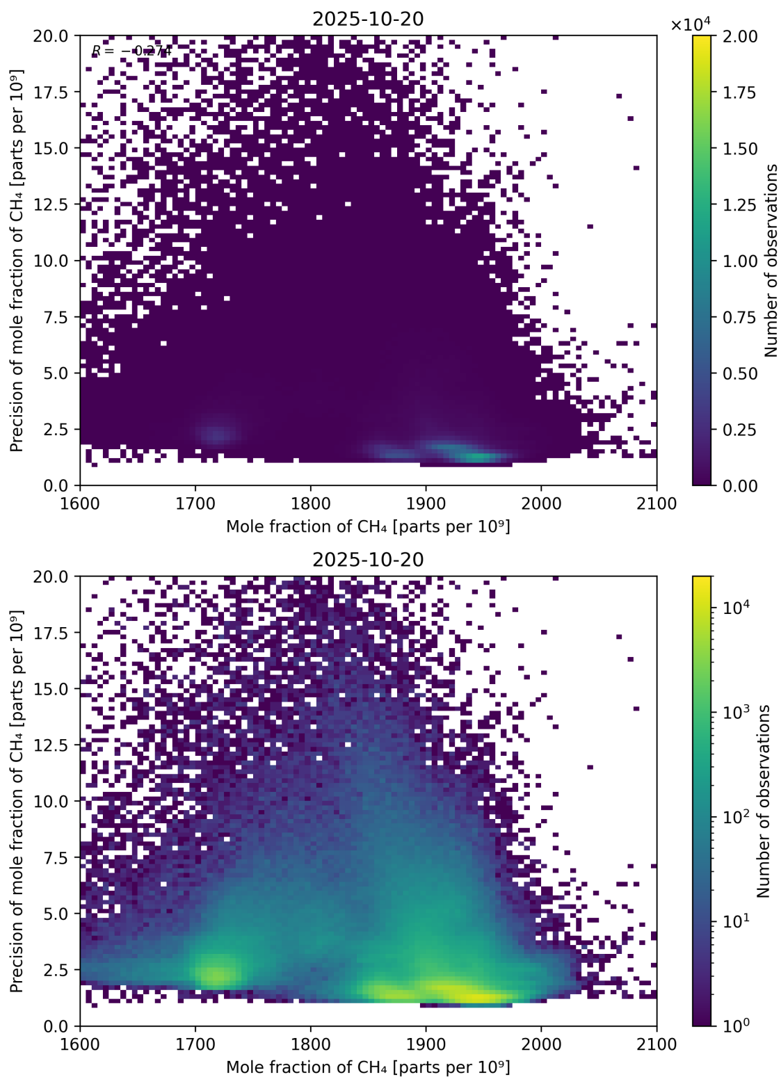
Figure 75: Scatter density plot of “Mole fraction of CH 4 ” against “Precision of mole fraction of CH 4 ” for 2025-10-19 to 2025-10-21.
