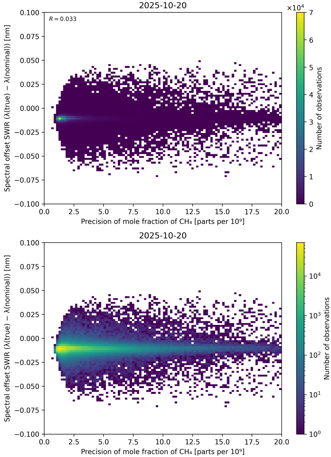
Figure 85: Scatter density plot of “Precision of mole fraction of \text{CH}_4 ” against “Spectral offset SWIR ( \lambda_{\text{true}} - \lambda_{\text{nominal}} )” for 2025-10-19 to 2025-10-21.
