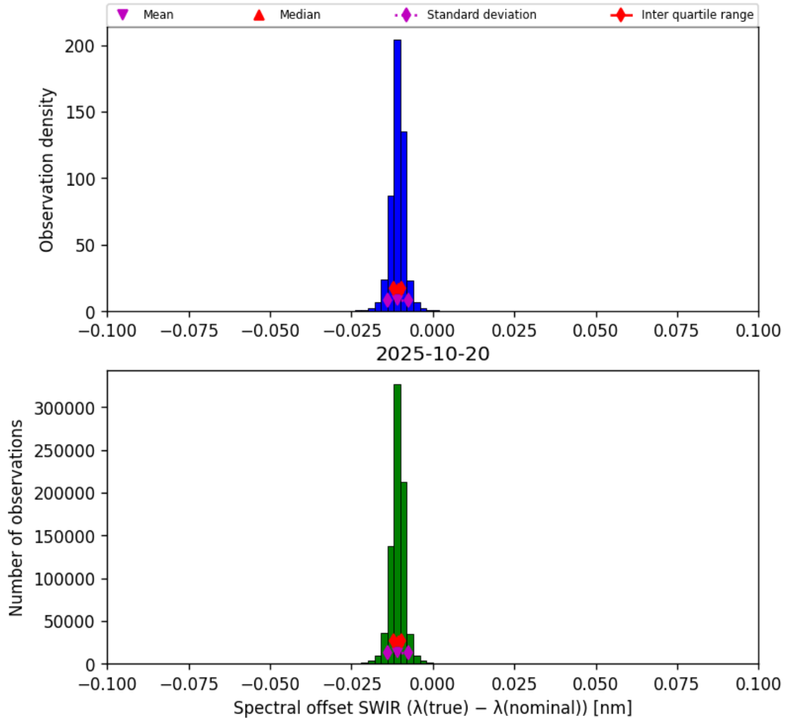
Figure 27: Histogram of “Spectral offset SWIR ( \lambda_{\text{true}} - \lambda_{\text{nominal}} )” for 2025-10-19 to 2025-10-21
