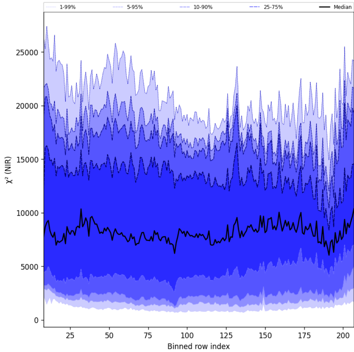
Figure 40: Along track statistics of “ \chi^2 (NIR)” for 2025-10-19 to 2025-10-21
