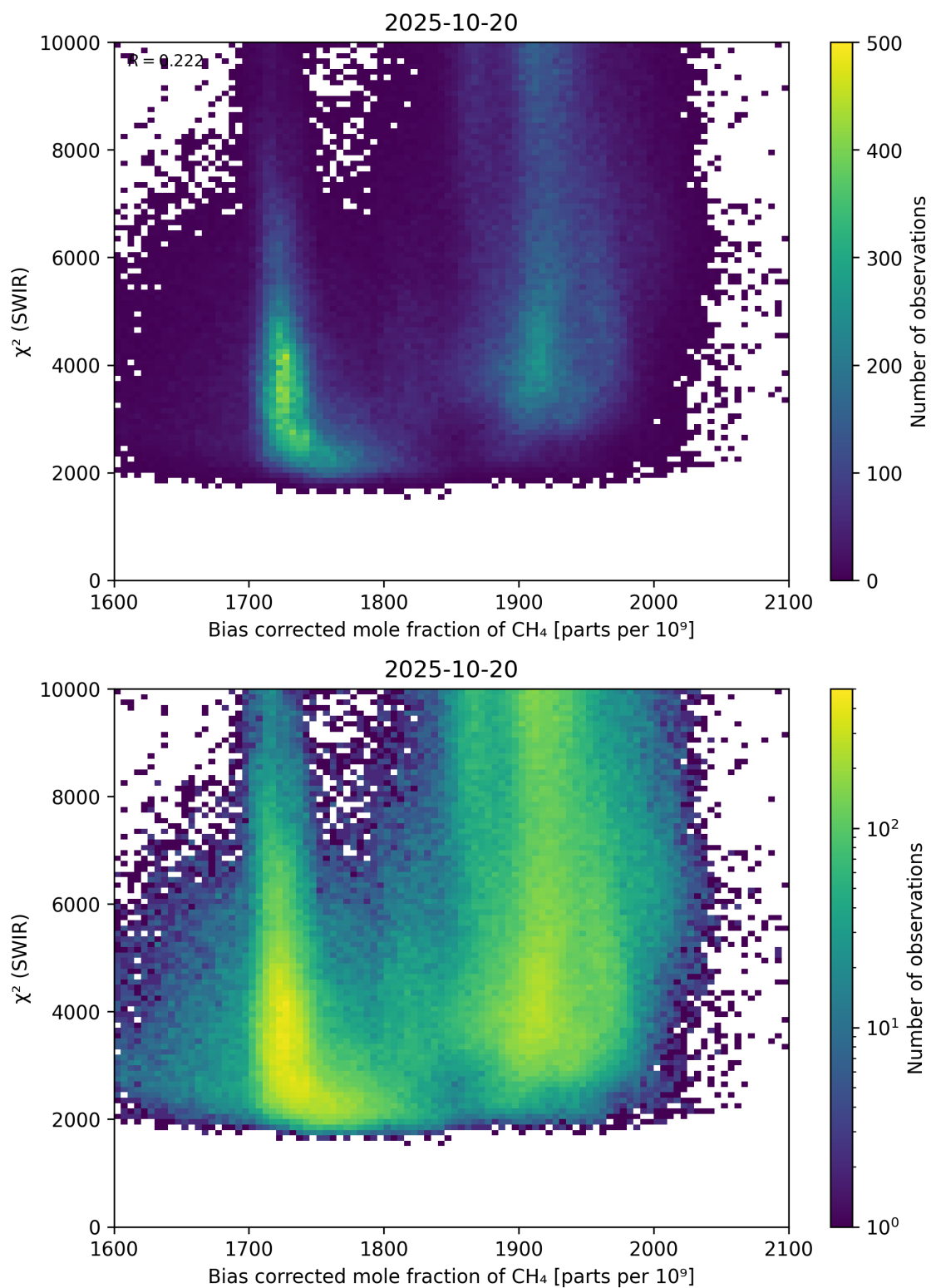
Figure 64: Scatter density plot of “Bias corrected mole fraction of \text{CH}_4 ” against “ \chi^2 (SWIR)” for 2025-10-19 to 2025-10-21.
