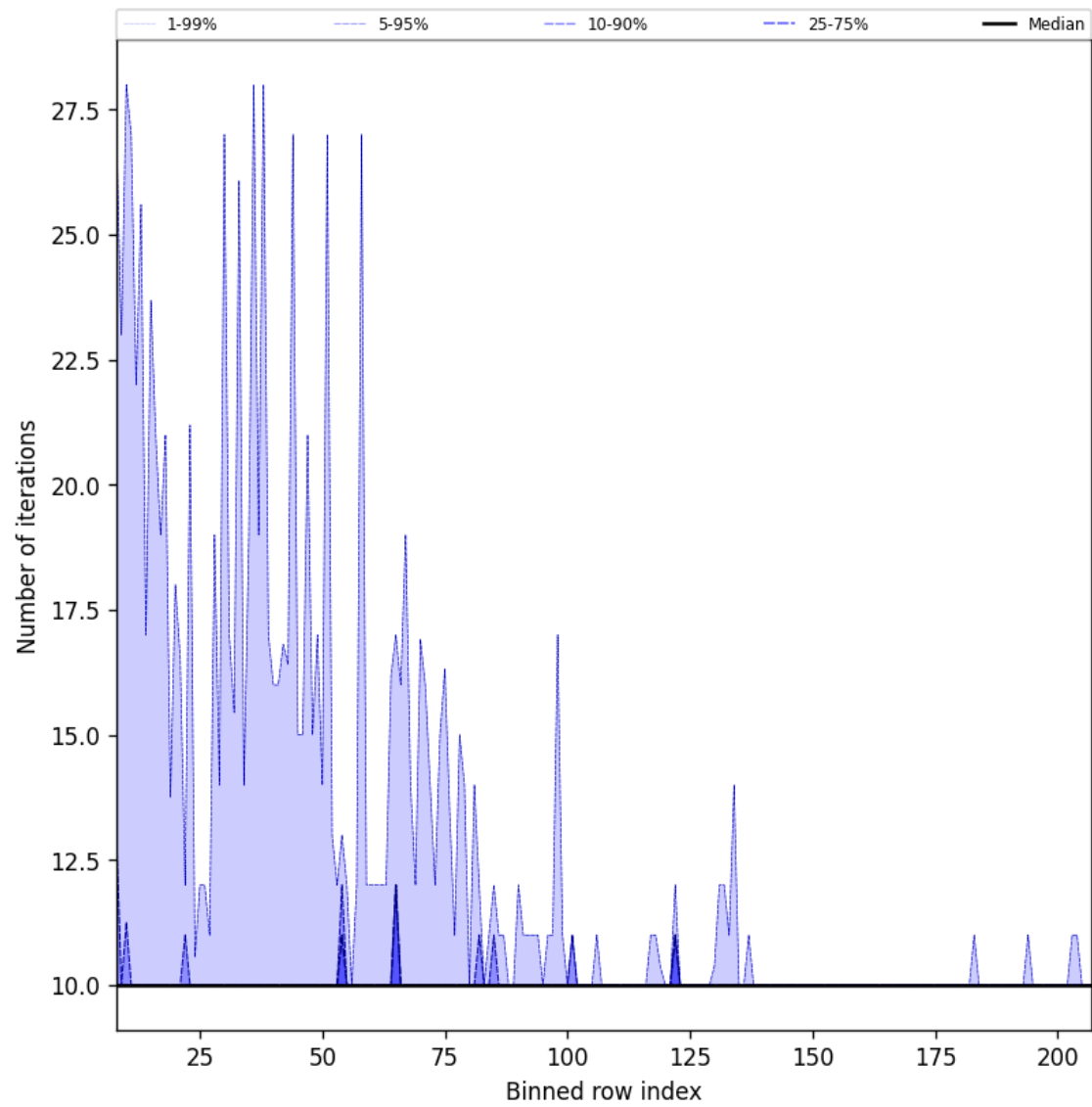
Figure 42: Along track statistics of “Number of iterations” for 2025-10-20 to 2025-10-22
