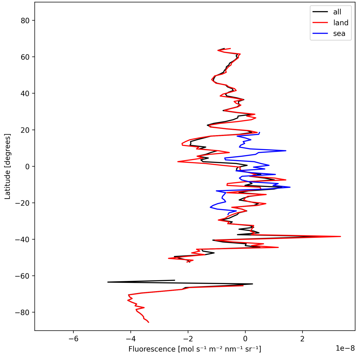
Figure 21: Zonal average of “Fluorescence” for 2025-10-20 to 2025-10-22.
