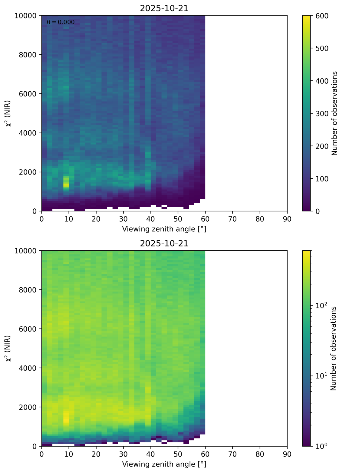
Figure 105: Scatter density plot of “Viewing zenith angle” against “ \chi^2 (NIR)” for 2025-10-20 to 2025-10-22.
