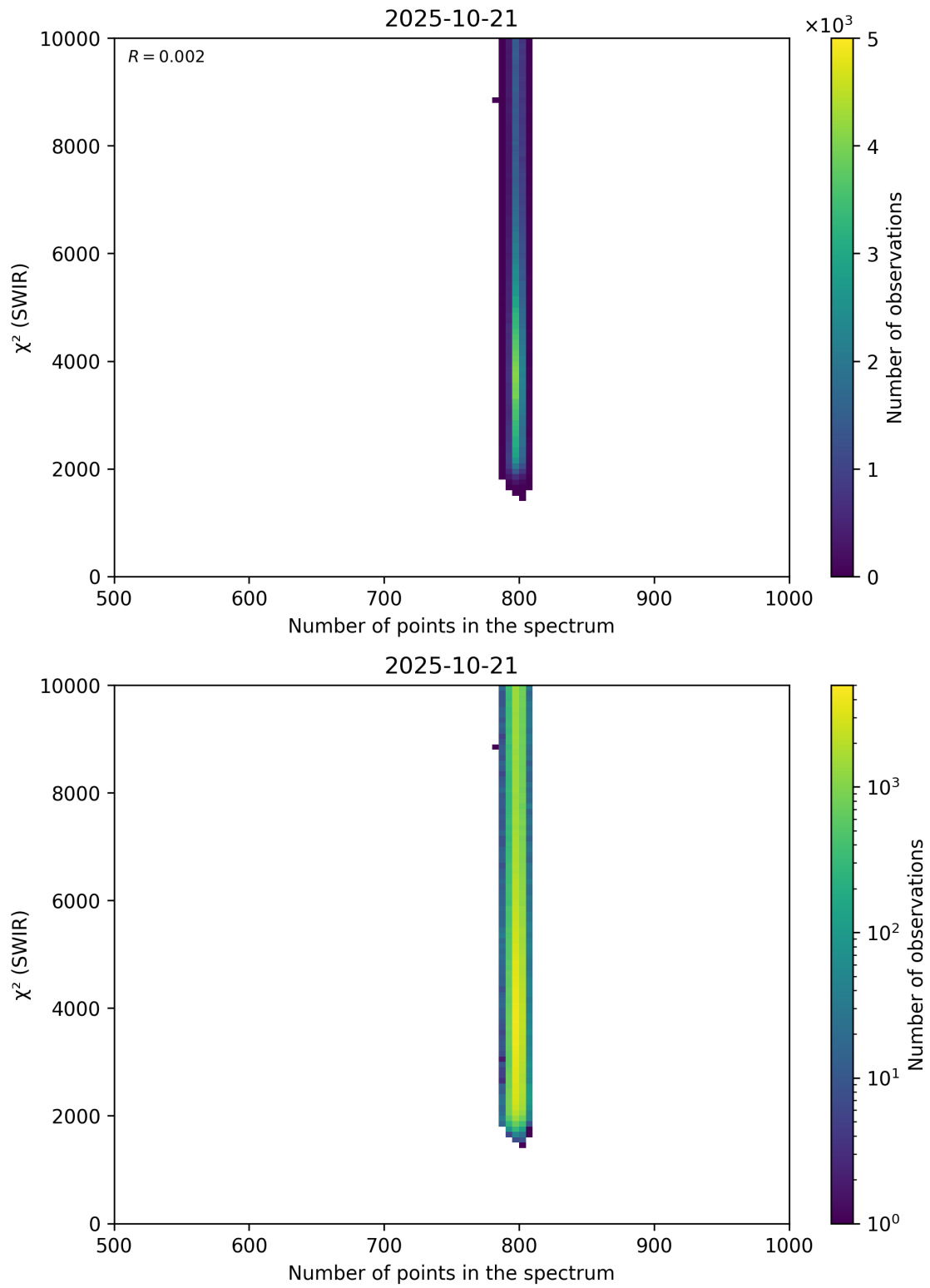
Figure 89: Scatter density plot of “Number of points in the spectrum” against “ \chi^2 (SWIR)” for 2025-10-20 to 2025-10-22.
