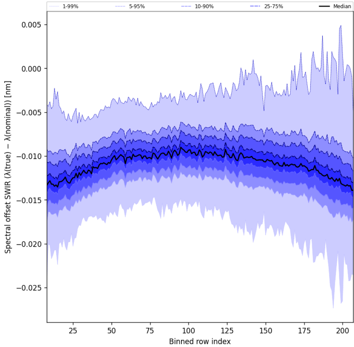
Figure 38: Along track statistics of “Spectral offset SWIR ( \lambda_{\text{true}} - \lambda_{\text{nominal}} )” for 2025-10-20 to 2025-10-22
