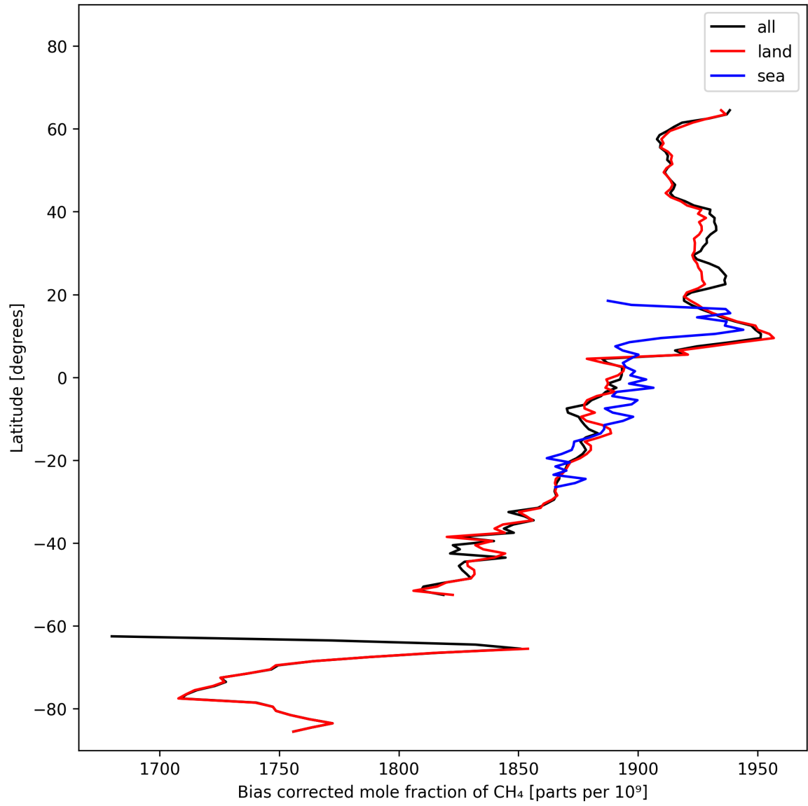
Figure 14: Zonal average of “Bias corrected mole fraction of CH 4 ” for 2025-10-20 to 2025-10-22.
