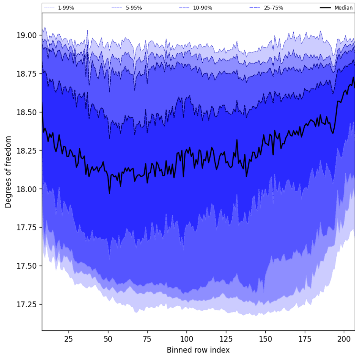
Figure 41: Along track statistics of “Degrees of freedom” for 2025-10-20 to 2025-10-22
