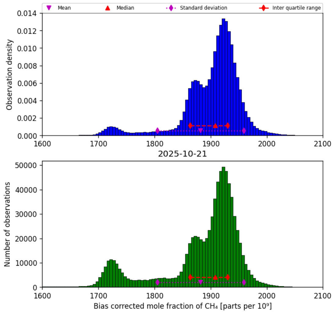
Figure 25: Histogram of “Bias corrected mole fraction of CH 4 ” for 2025-10-20 to 2025-10-22
