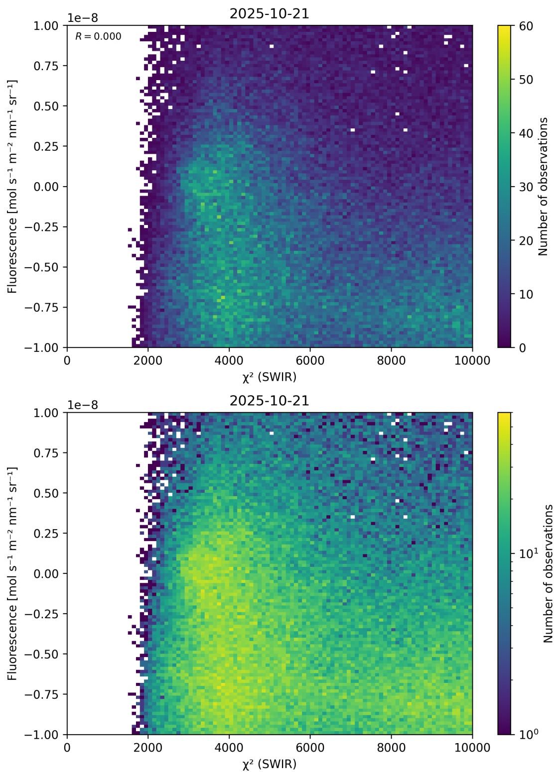
Figure 49: Scatter density plot of “ \chi^2 (SWIR)” against “Fluorescence” for 2025-10-20 to 2025-10-22.
