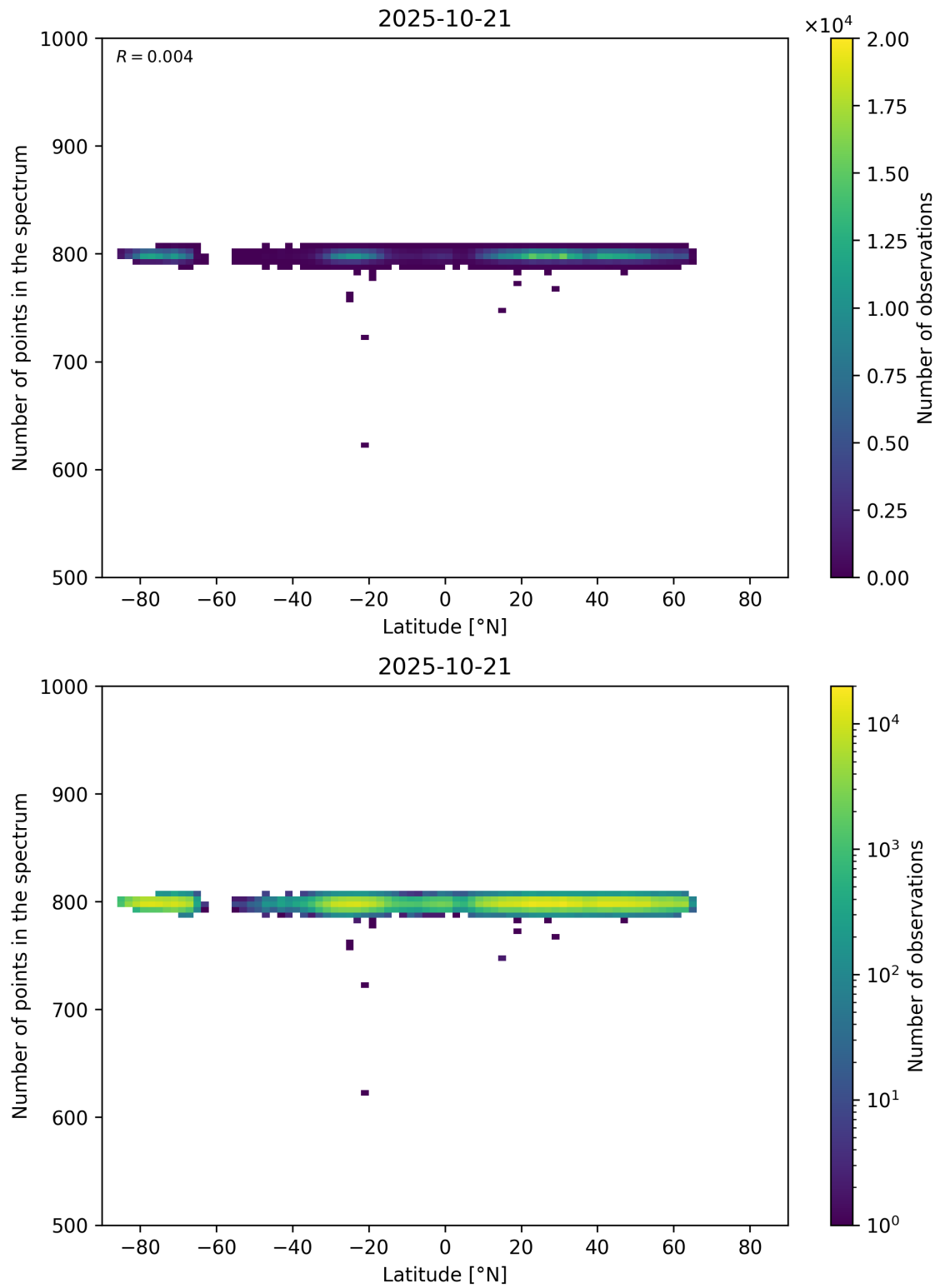
Figure 61: Scatter density plot of “Latitude” against “Number of points in the spectrum” for 2025-10-20 to 2025-10-22.
