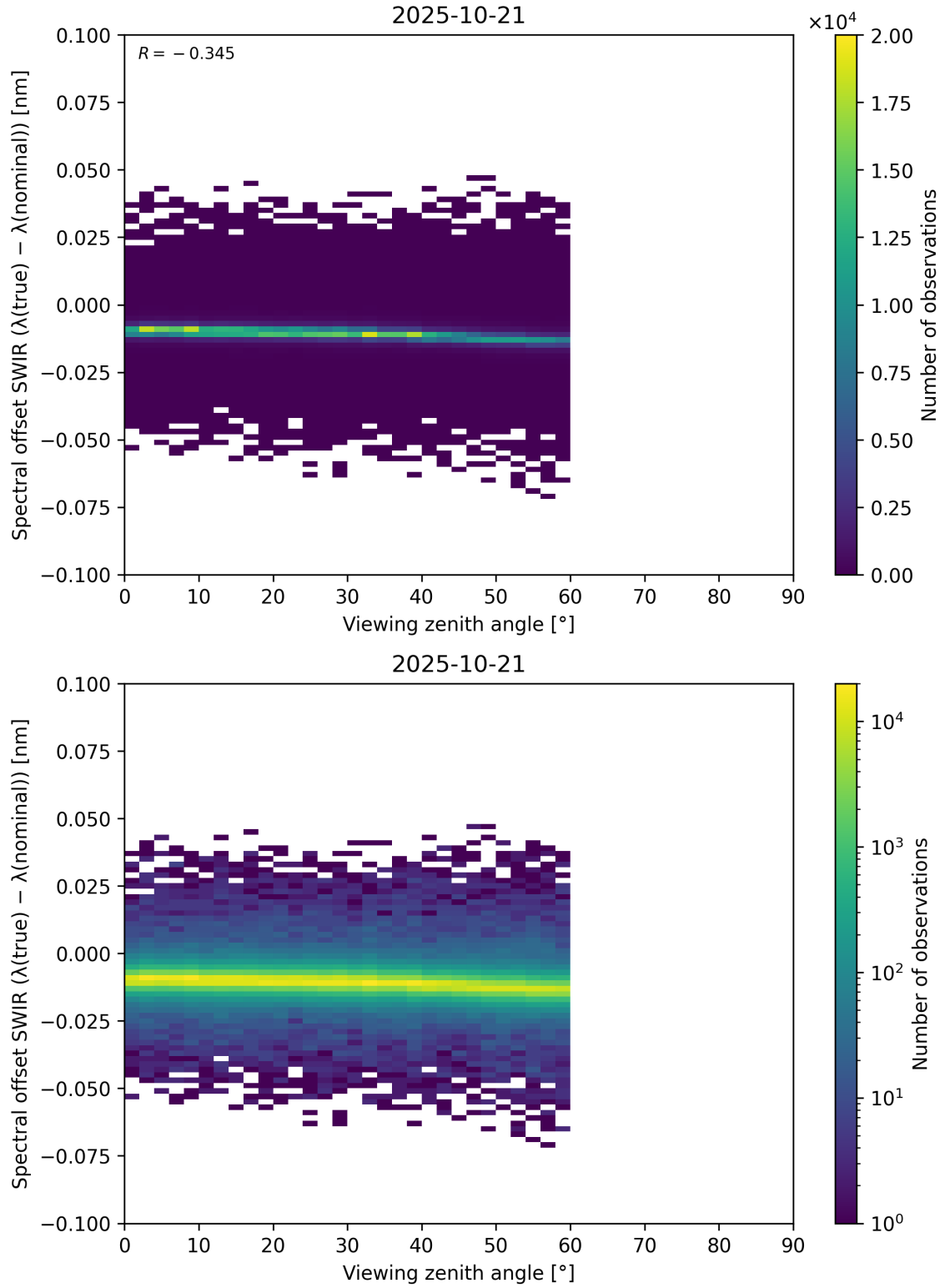
Figure 116: Scatter density plot of “Viewing zenith angle” against “Spectral offset SWIR ( \lambda_{\text{true}} - \lambda_{\text{nominal}} )” for 2025-10-20 to 2025-10-22.
