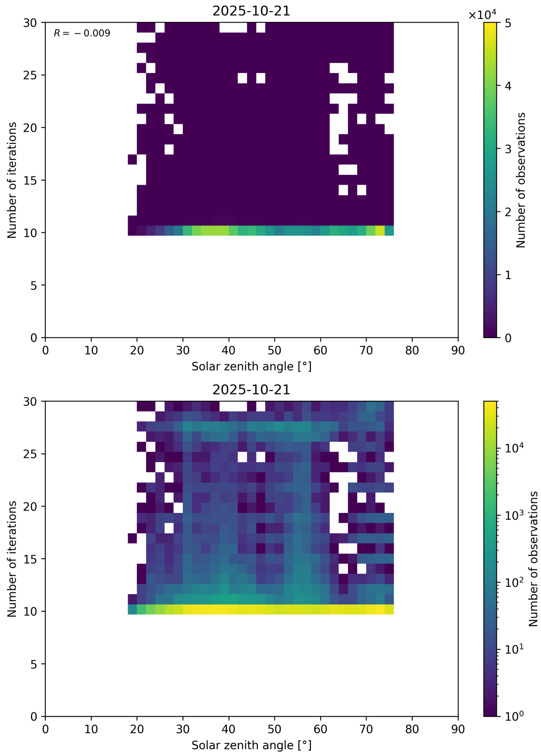
Figure 102: Scatter density plot of “Solar zenith angle” against “Number of iterations” for 2025-10-20 to 2025-10-22.
