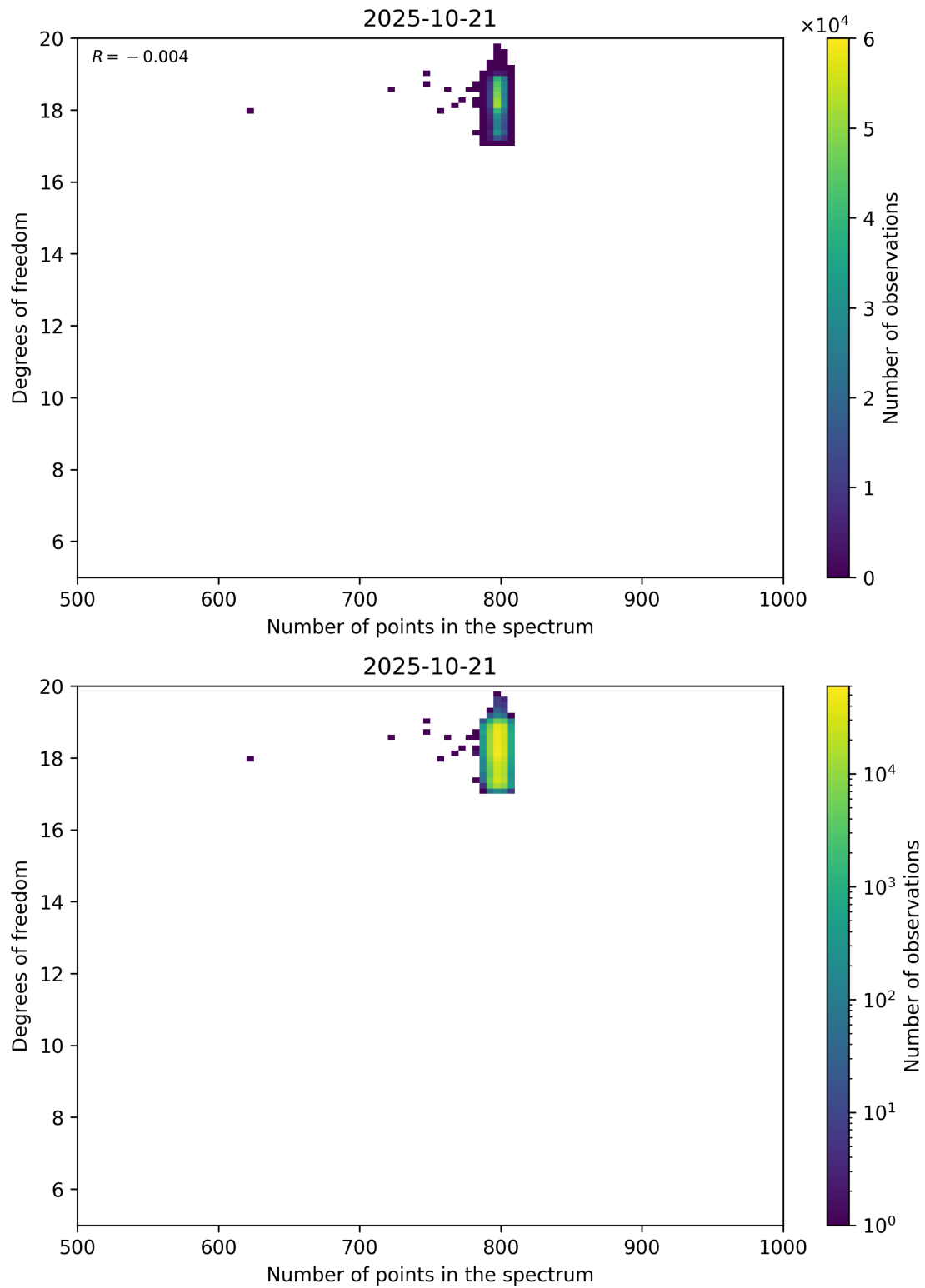
Figure 90: Scatter density plot of “Number of points in the spectrum” against “Degrees of freedom” for 2025-10-20 to 2025-10-22.
