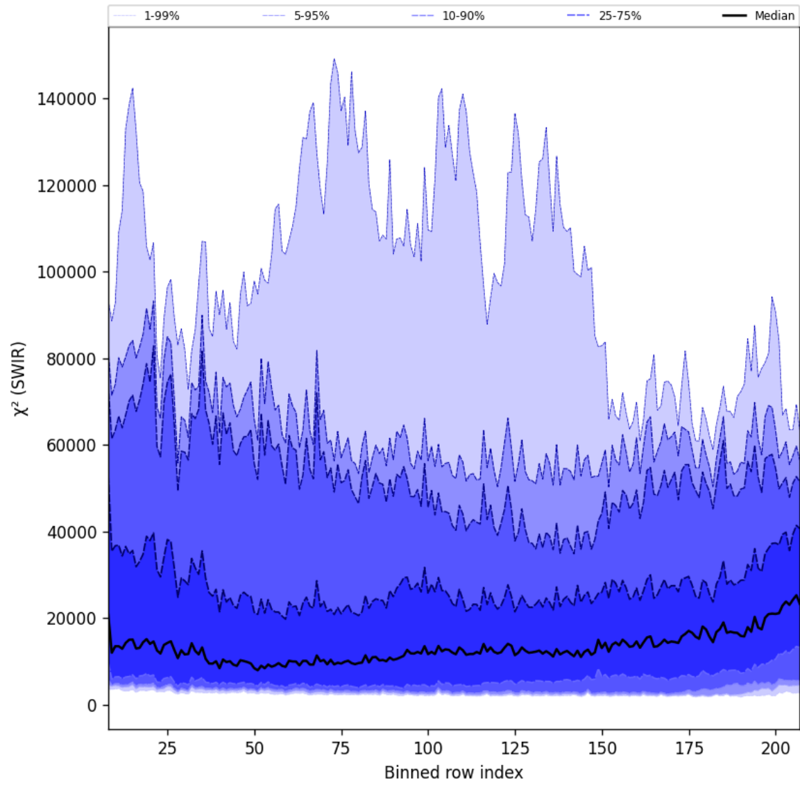
Figure 39: Along track statistics of “ \chi^2 (SWIR)” for 2025-10-20 to 2025-10-22
