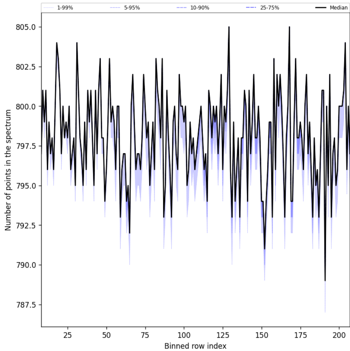
Figure 37: Along track statistics of “Number of points in the spectrum” for 2025-10-20 to 2025-10-22
