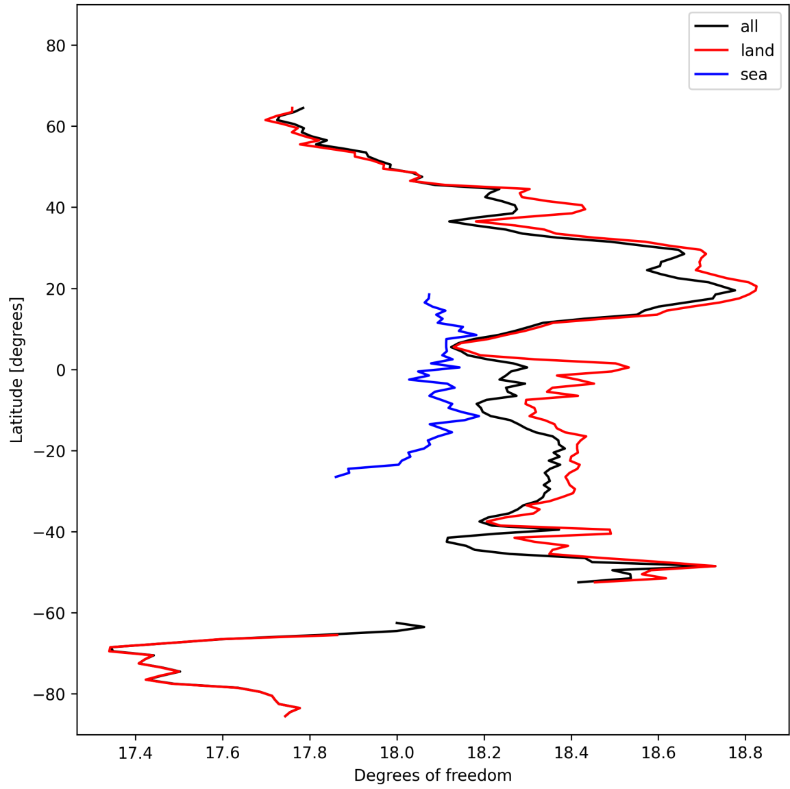
Figure 19: Zonal average of “Degrees of freedom” for 2025-10-20 to 2025-10-22.
