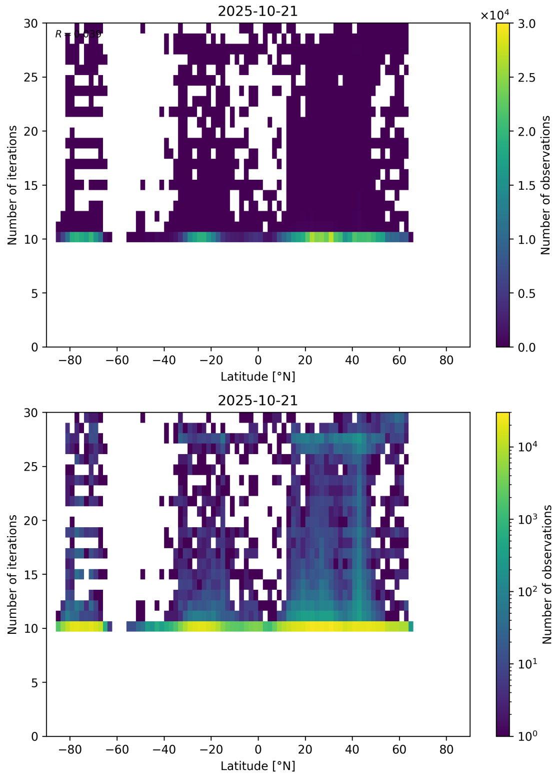
Figure 60: Scatter density plot of “Latitude” against “Number of iterations” for 2025-10-20 to 2025-10-22.
