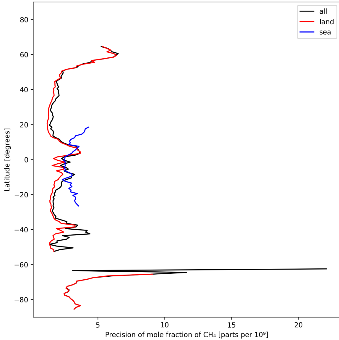
Figure 13: Zonal average of “Precision of mole fraction of CH 4 ” for 2025-10-20 to 2025-10-22.
