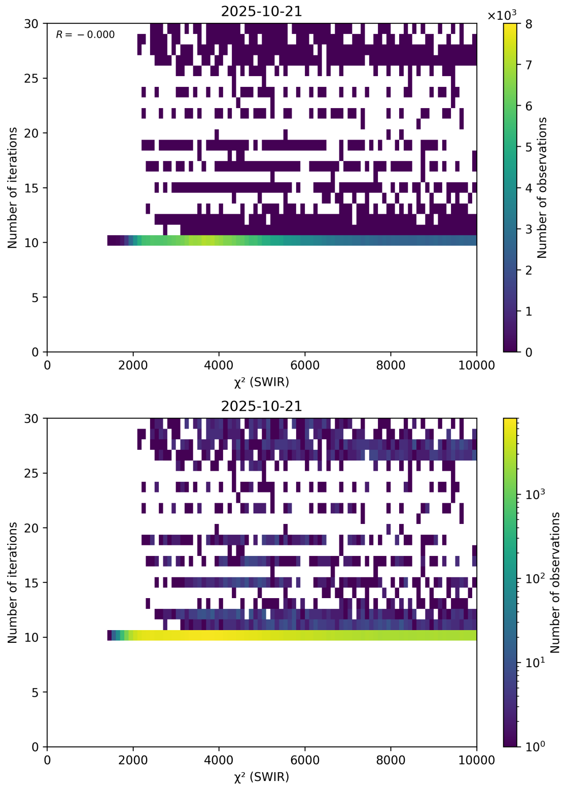
Figure 50: Scatter density plot of “ \chi^2 (SWIR)” against “Number of iterations” for 2025-10-20 to 2025-10-22.
