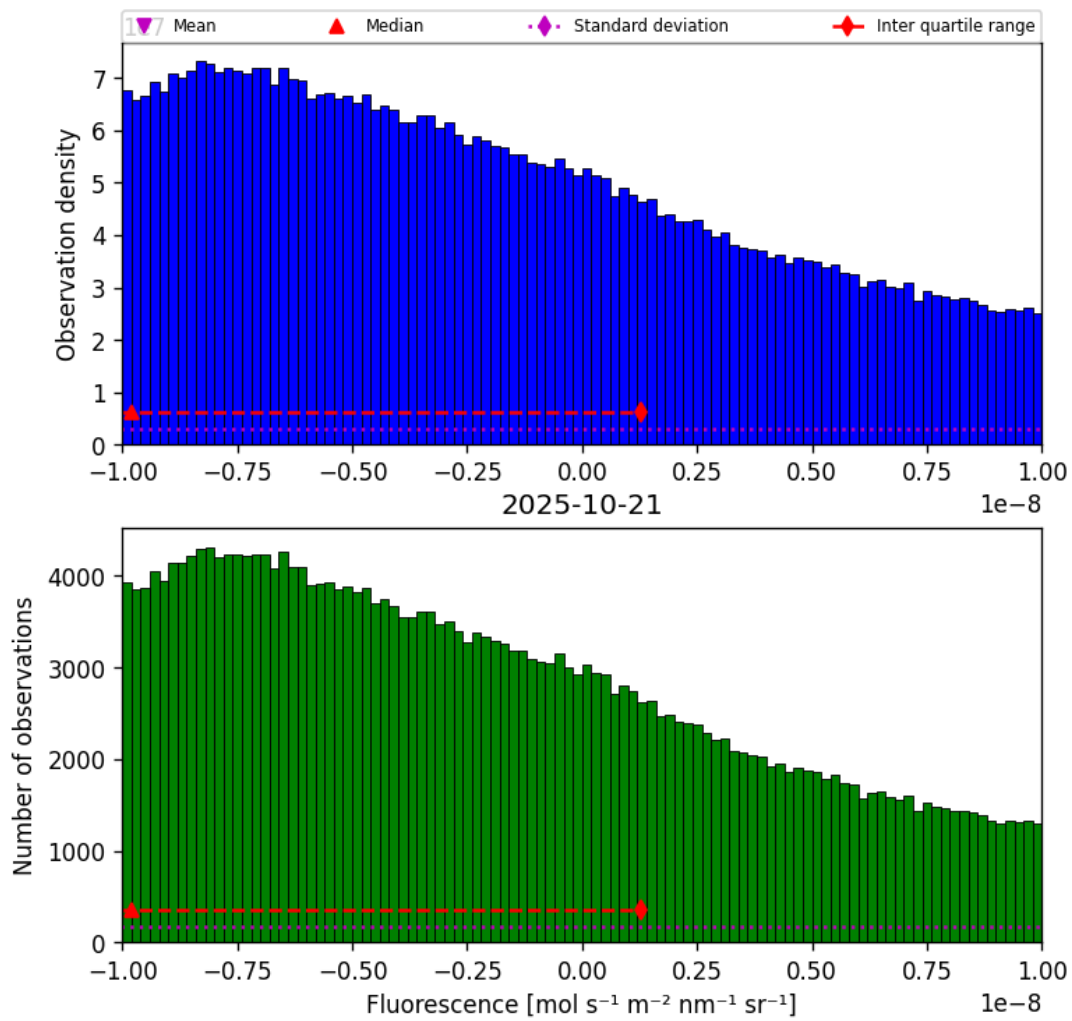
Figure 32: Histogram of “Fluorescence” for 2025-10-20 to 2025-10-22
