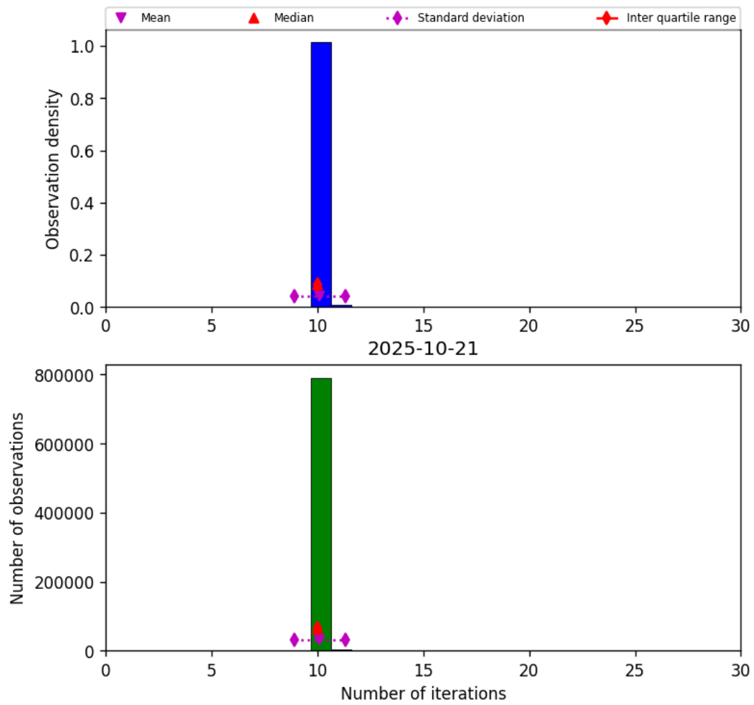
Figure 31: Histogram of “Number of iterations” for 2025-10-20 to 2025-10-22
