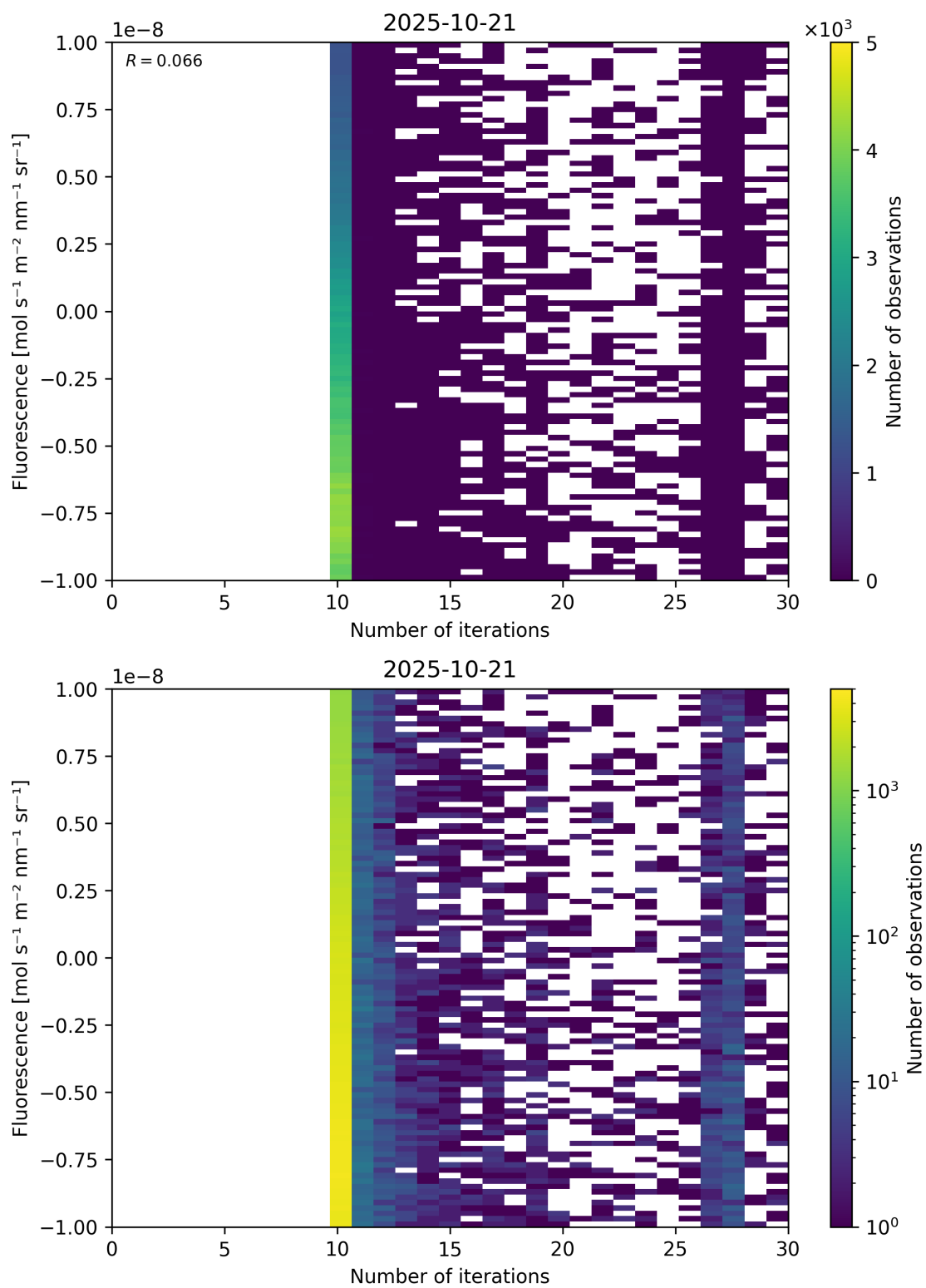
Figure 87: Scatter density plot of “Number of iterations” against “Fluorescence” for 2025-10-20 to 2025-10-22.
