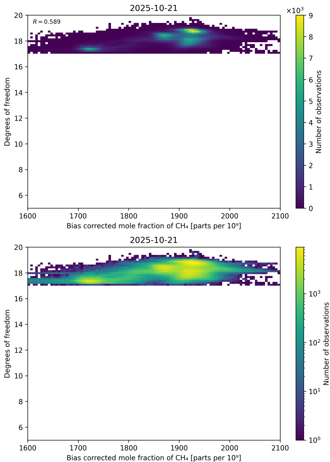
Figure 65: Scatter density plot of “Bias corrected mole fraction of CH 4 ” against “Degrees of freedom” for 2025-10-20 to 2025-10-22.
