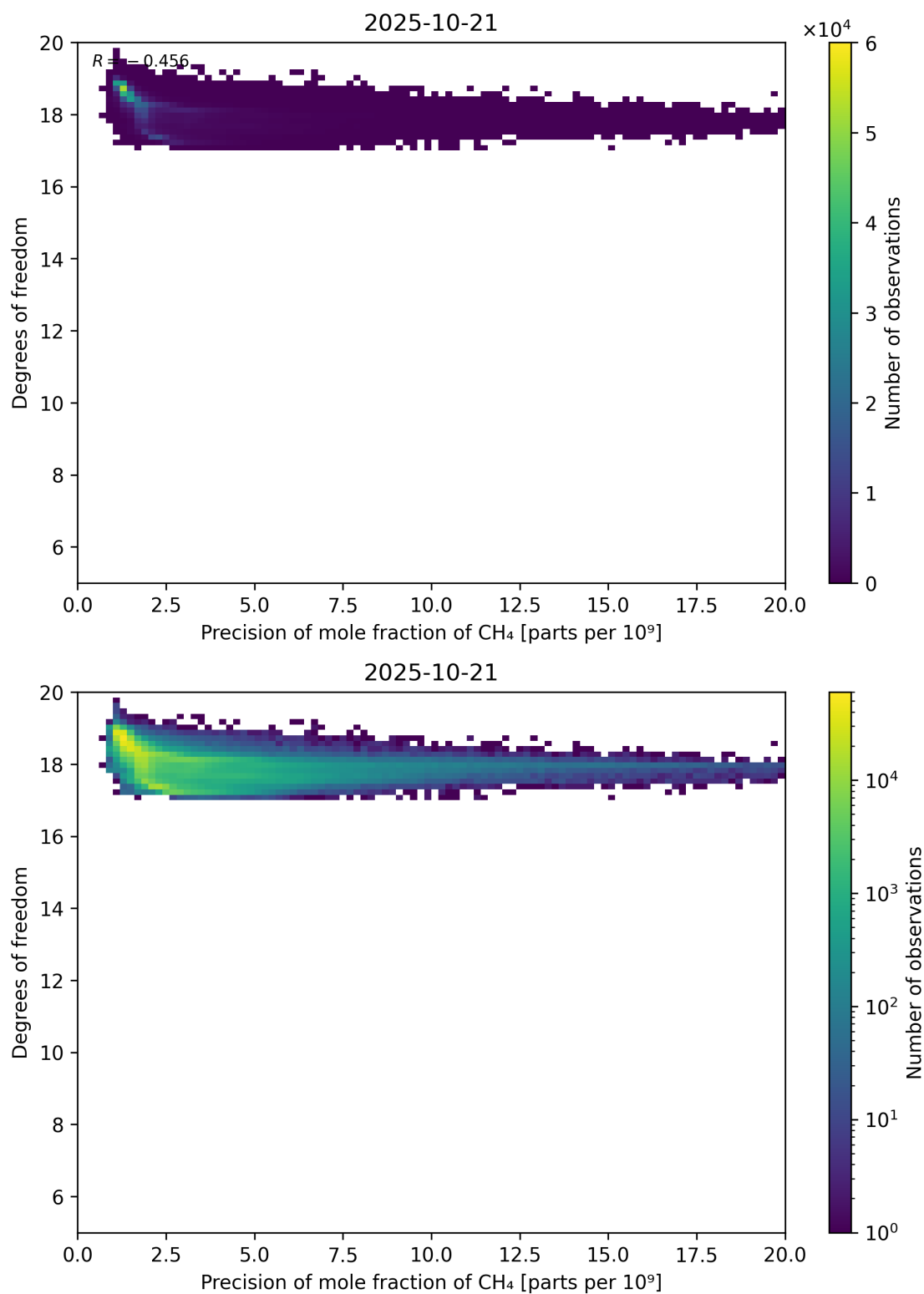
Figure 80: Scatter density plot of “Precision of mole fraction of CH 4 ” against “Degrees of freedom” for 2025-10-20 to 2025-10-22.
