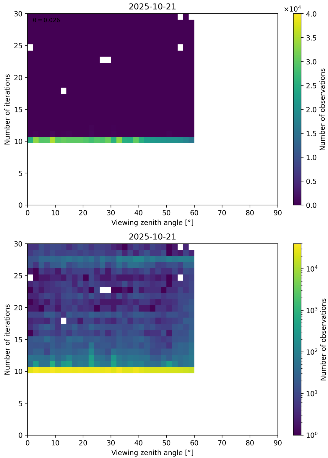
Figure 113: Scatter density plot of “Viewing zenith angle” against “Number of iterations” for 2025-10-20 to 2025-10-22.
