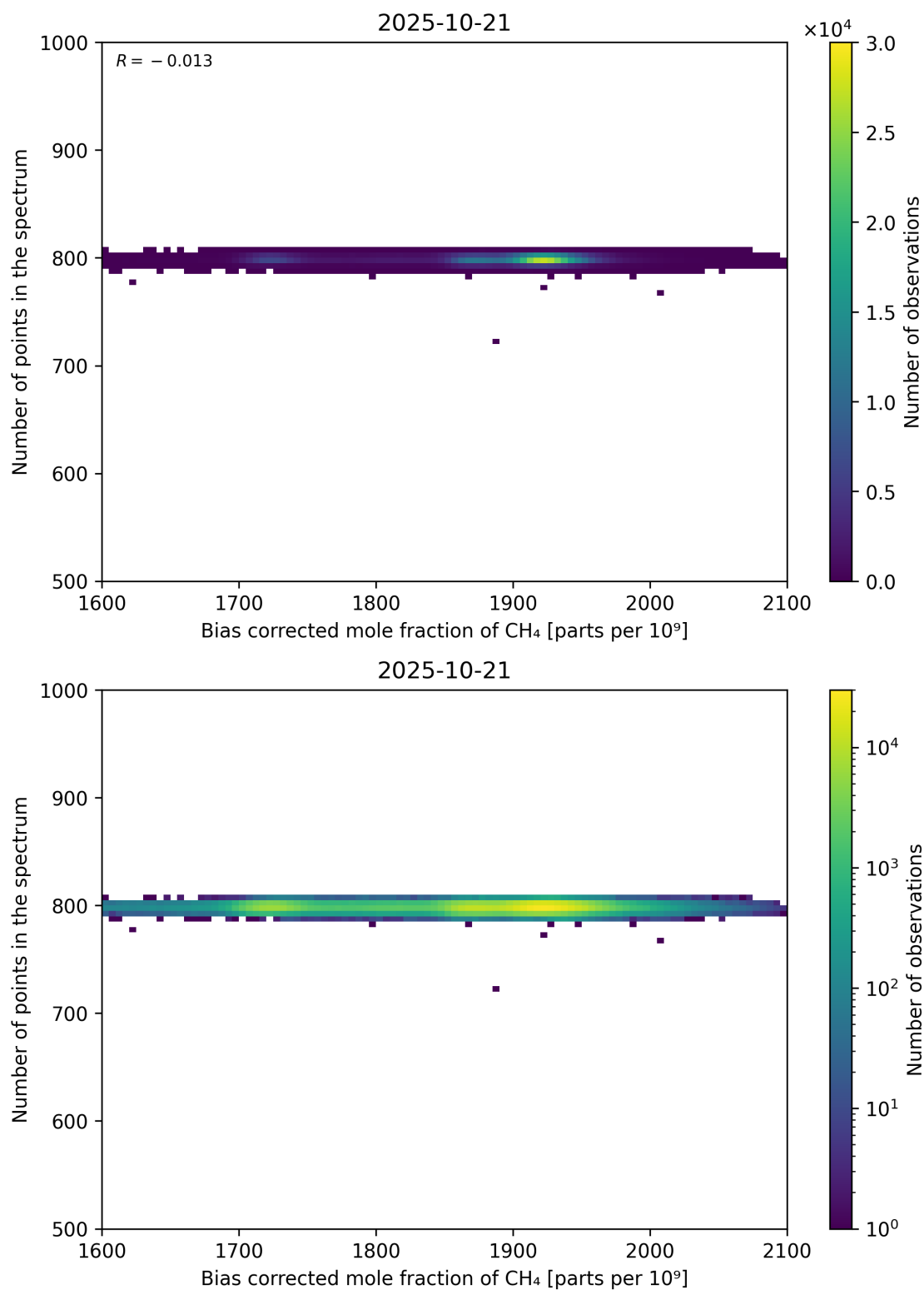
Figure 68: Scatter density plot of “Bias corrected mole fraction of CH 4 ” against “Number of points in the spectrum” for 2025-10-20 to 2025-10-22.
