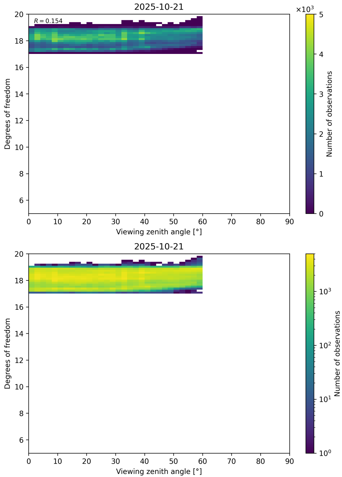
Figure 107: Scatter density plot of “Viewing zenith angle” against “Degrees of freedom” for 2025-10-20 to 2025-10-22.
