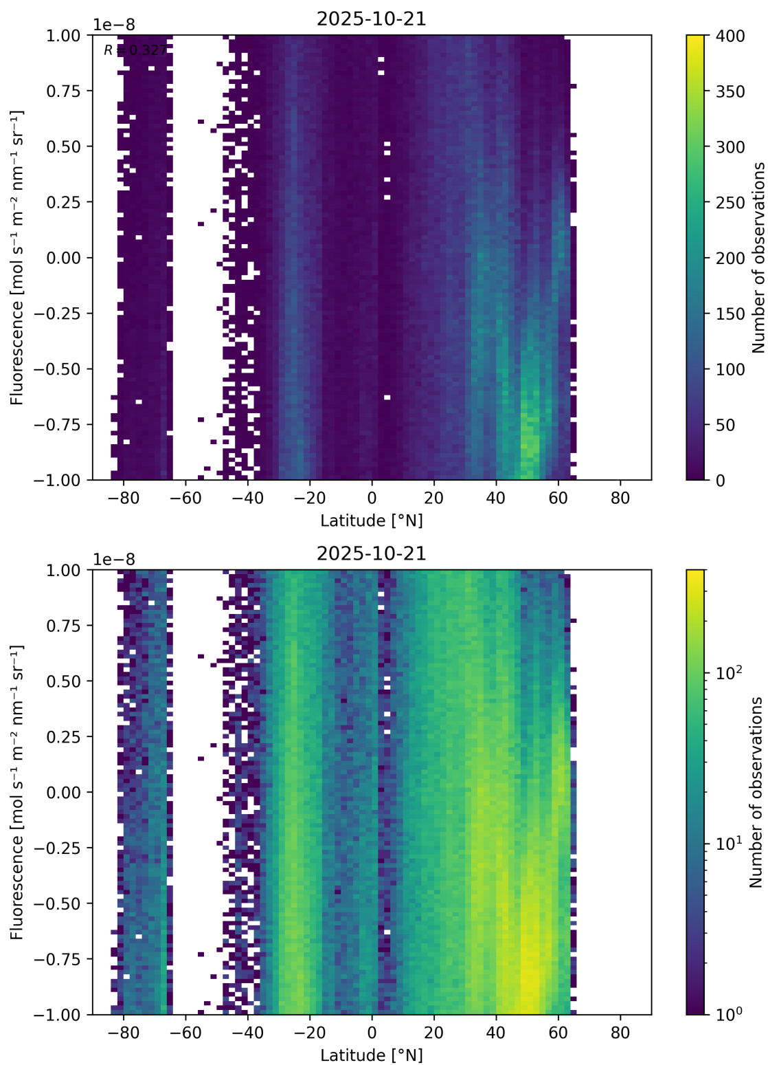
Figure 56: Scatter density plot of “Latitude” against “Fluorescence” for 2025-10-20 to 2025-10-22.
