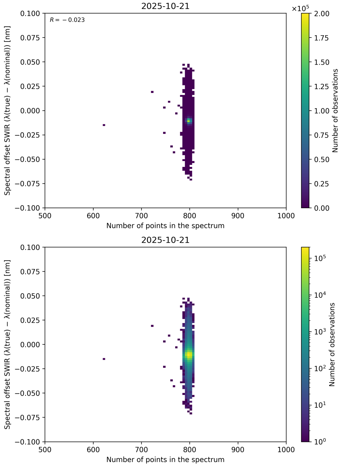
Figure 93: Scatter density plot of “Number of points in the spectrum” against “Spectral offset SWIR ( \lambda_{\text{true}} - \lambda_{\text{nominal}} )” for 2025-10-20 to 2025-10-22.
