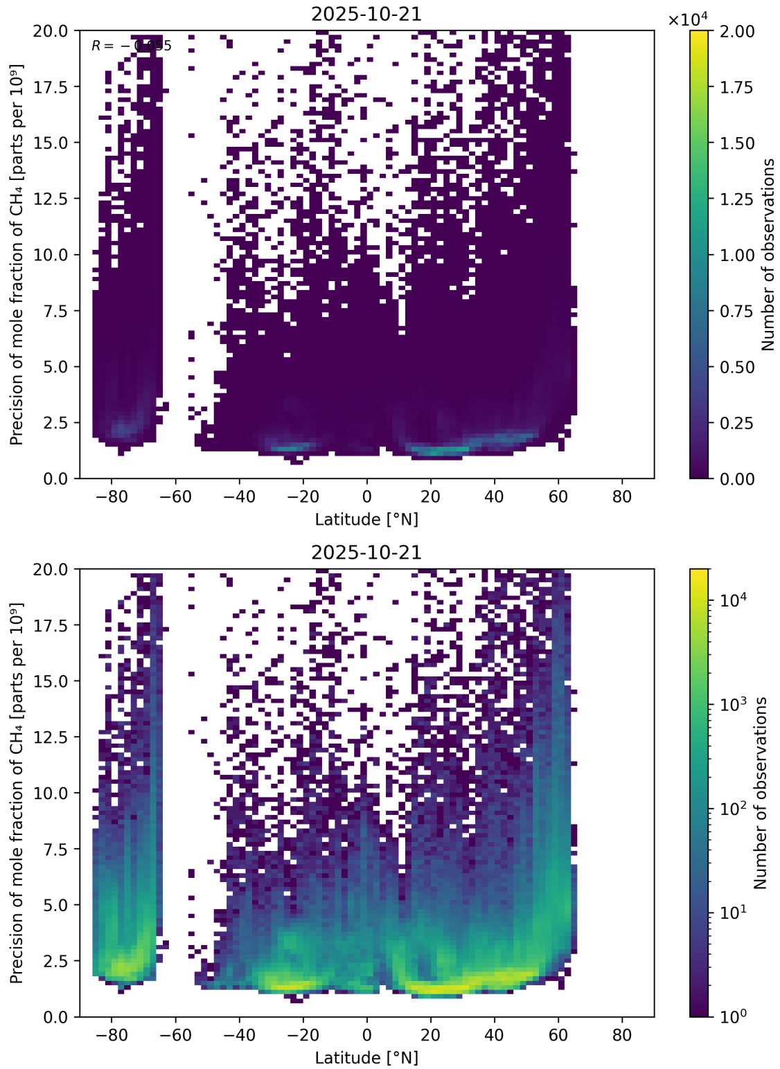
Figure 59: Scatter density plot of “Latitude” against “Precision of mole fraction of CH 4 ” for 2025-10-20 to 2025-10-22.
