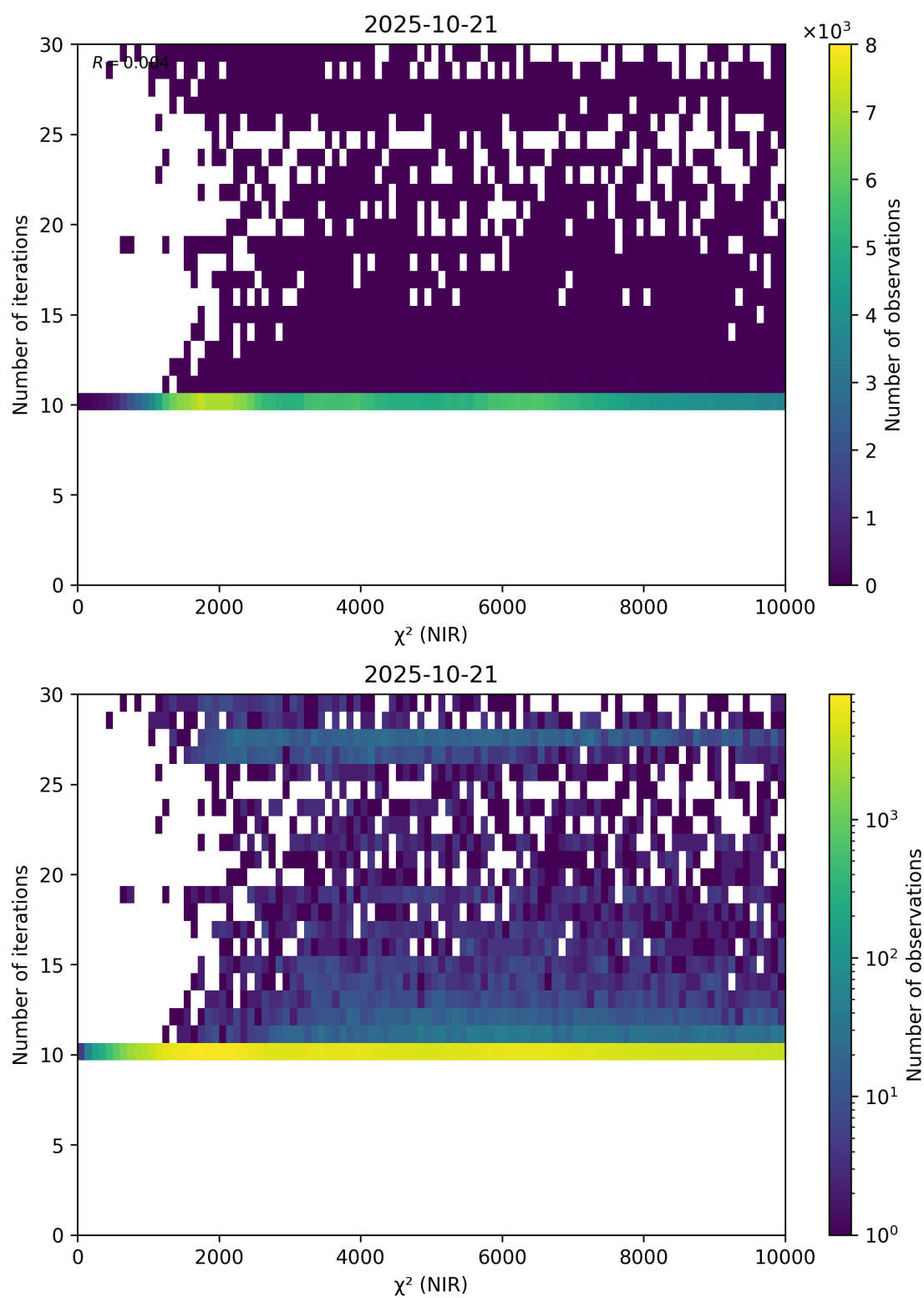
Figure 46: Scatter density plot of “ \chi^2 (NIR)” against “Number of iterations” for 2025-10-20 to 2025-10-22.
