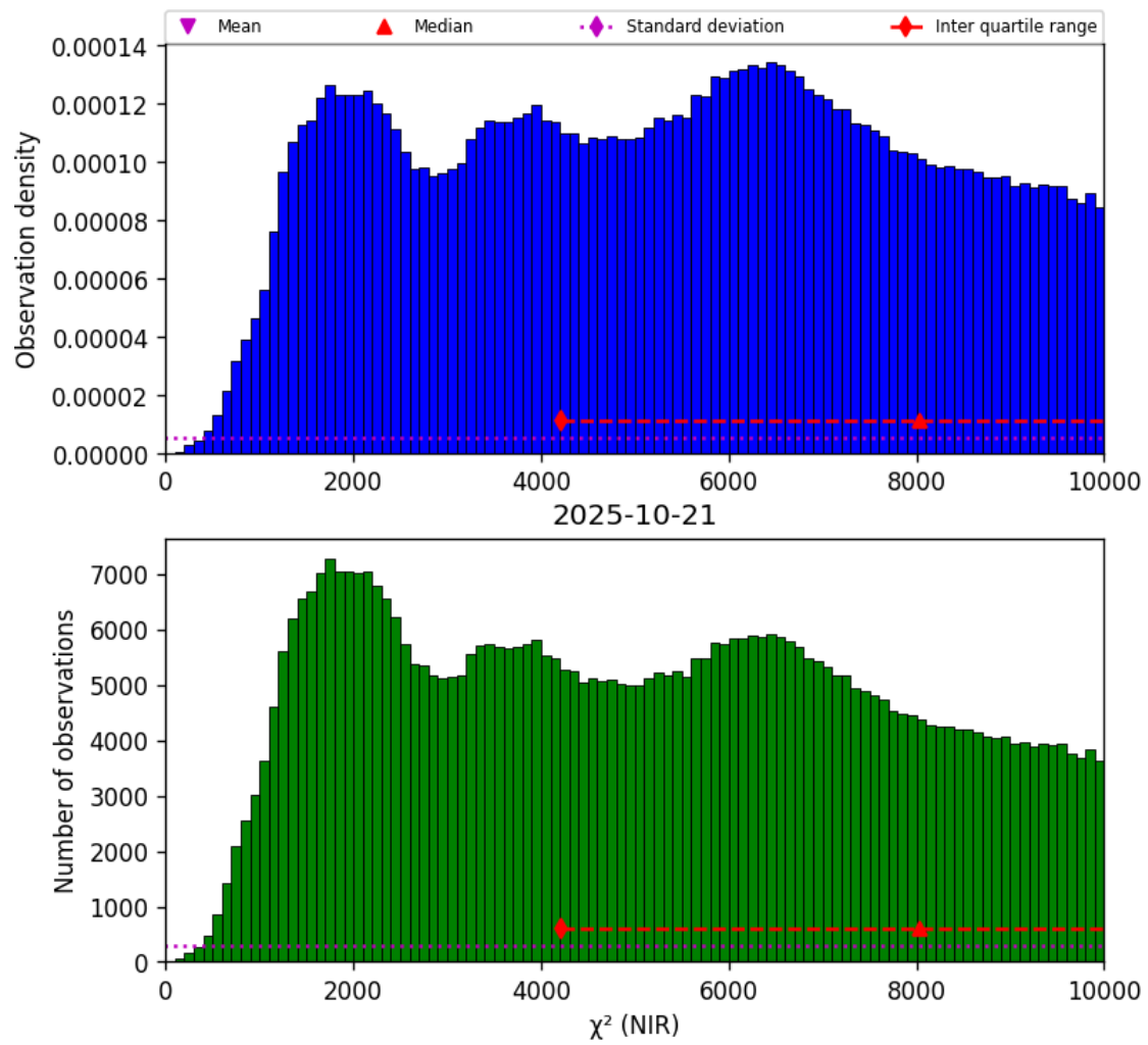
Figure 29: Histogram of “ \chi^2 (NIR)” for 2025-10-20 to 2025-10-22
