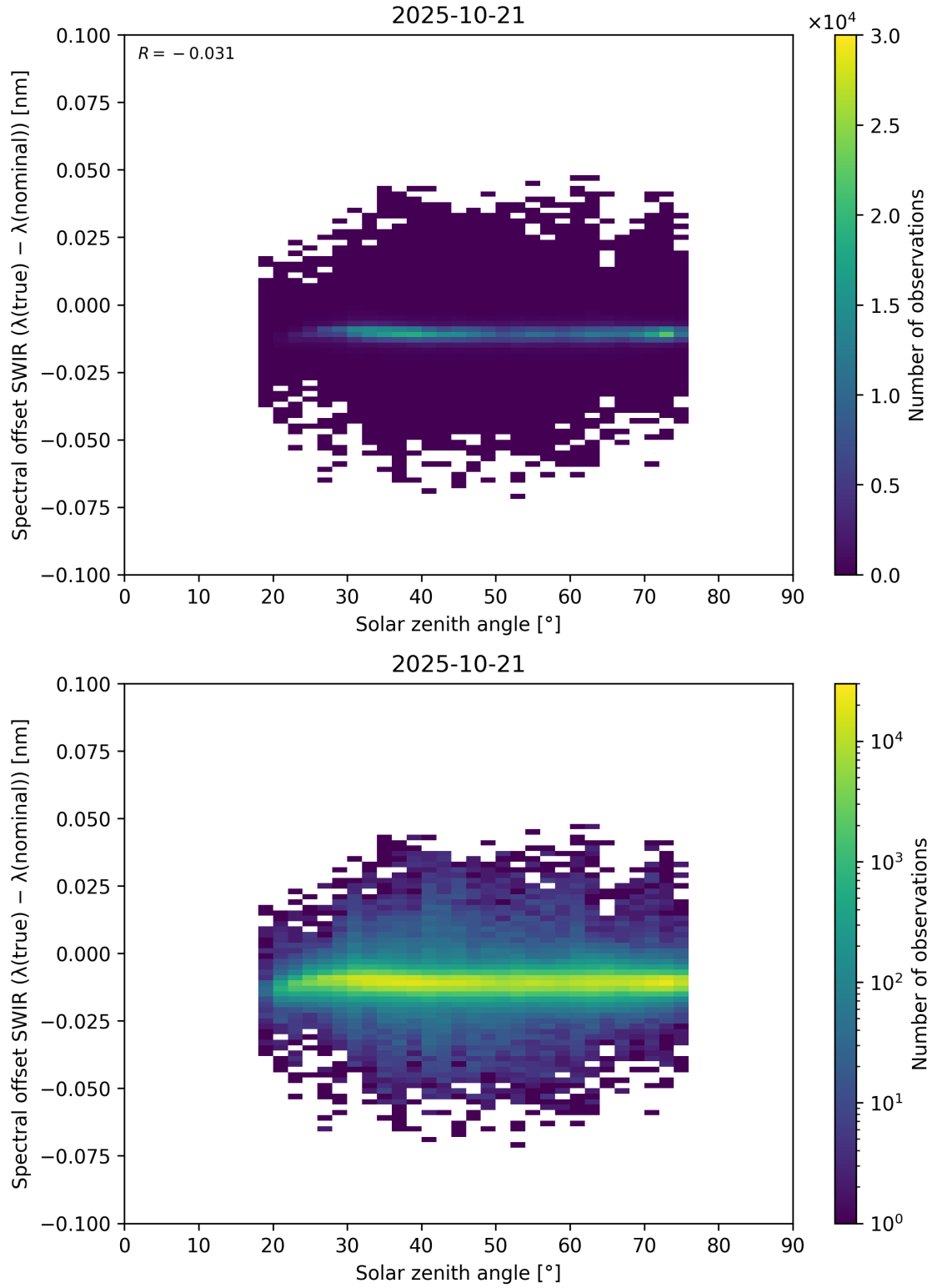
Figure 104: Scatter density plot of “Solar zenith angle” against “Spectral offset SWIR ( \lambda_{\text{true}} - \lambda_{\text{nominal}} )” for 2025-10-20 to 2025-10-22.
