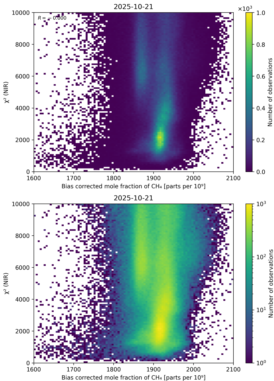
Figure 63: Scatter density plot of “Bias corrected mole fraction of \text{CH}_4 ” against “ \chi^2 (NIR)” for 2025-10-20 to 2025-10-22.
