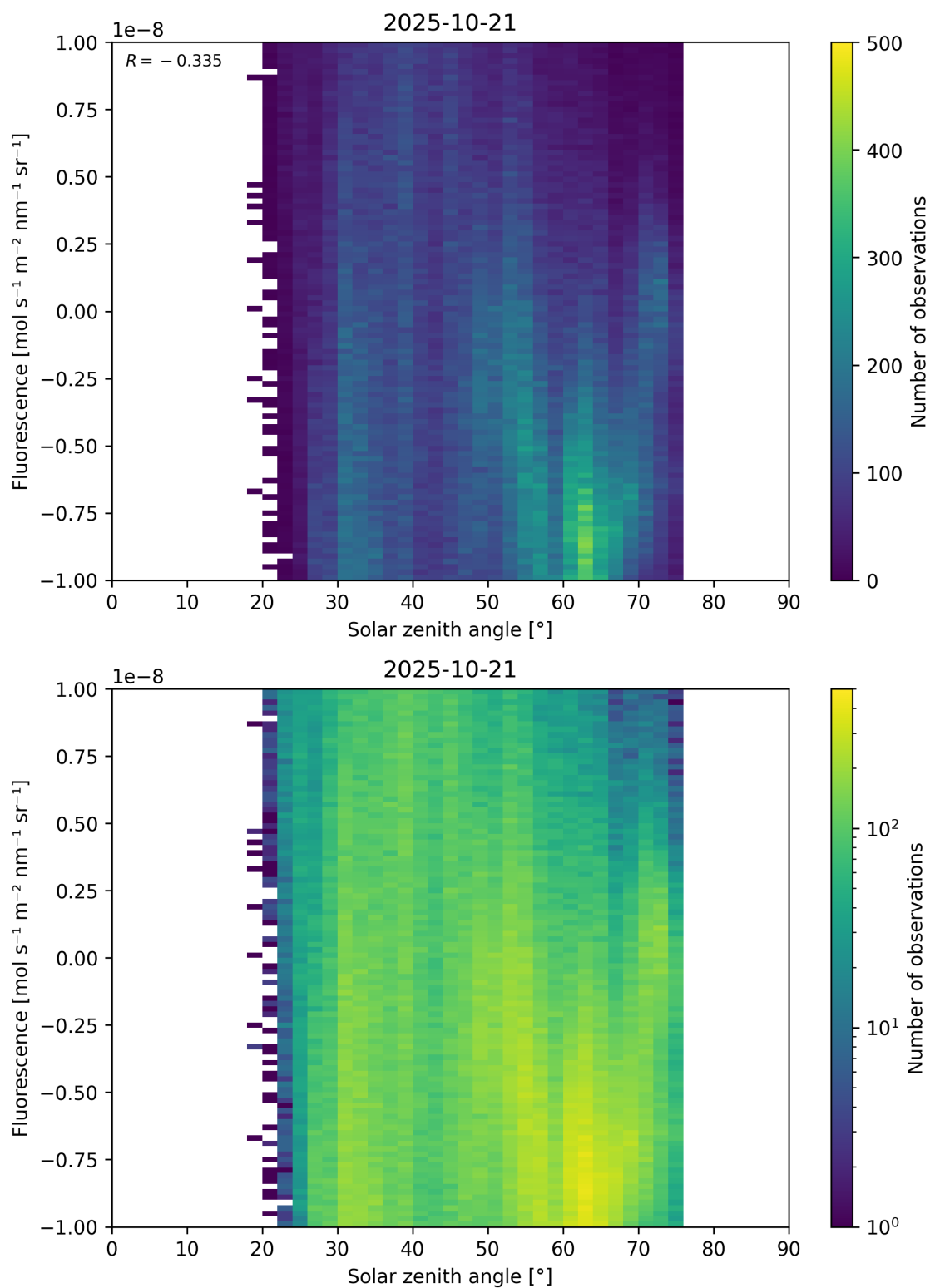
Figure 97: Scatter density plot of “Solar zenith angle” against “Fluorescence” for 2025-10-20 to 2025-10-22.
