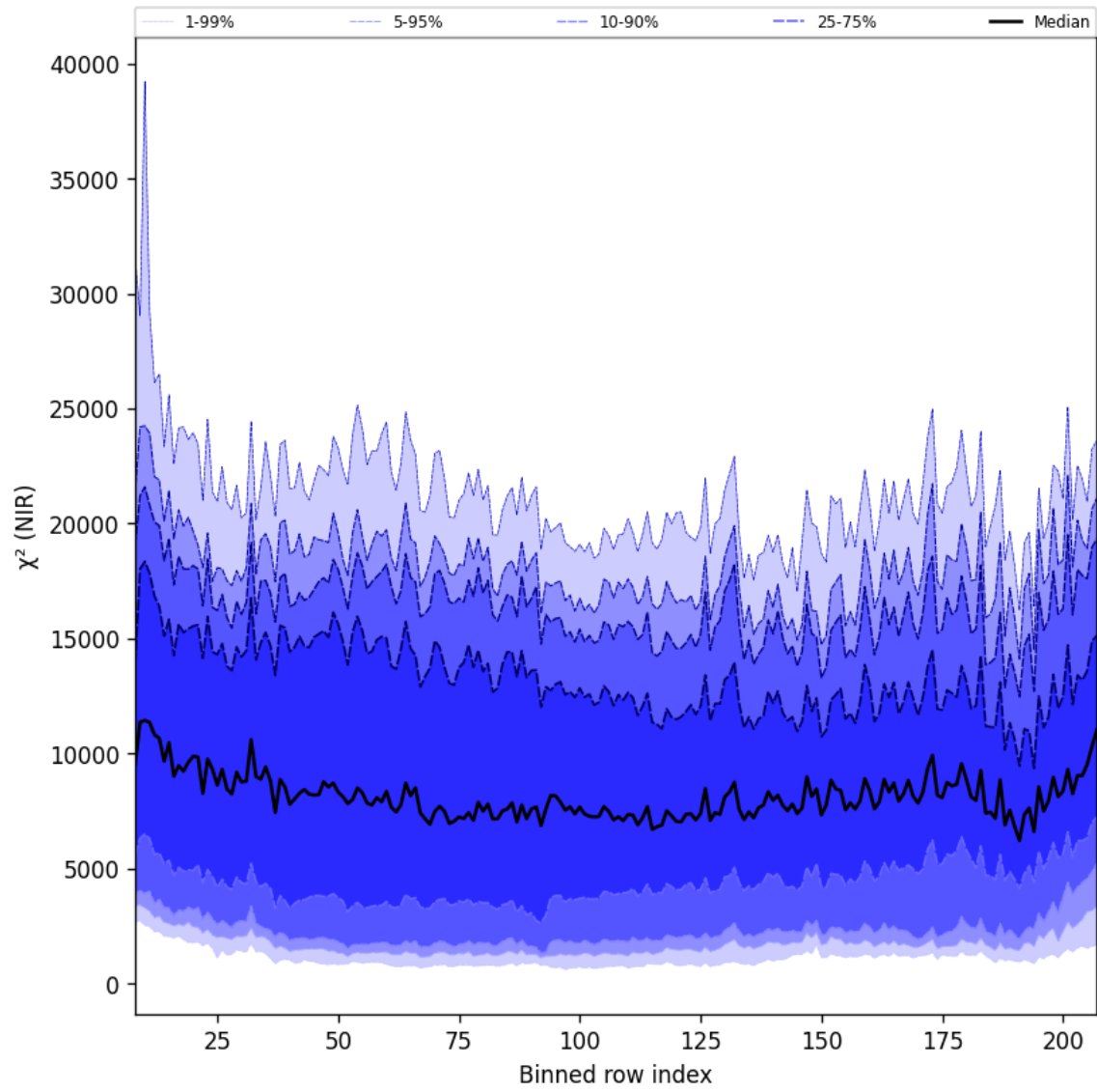
Figure 40: Along track statistics of “ \chi^2 (NIR)” for 2025-10-20 to 2025-10-22
