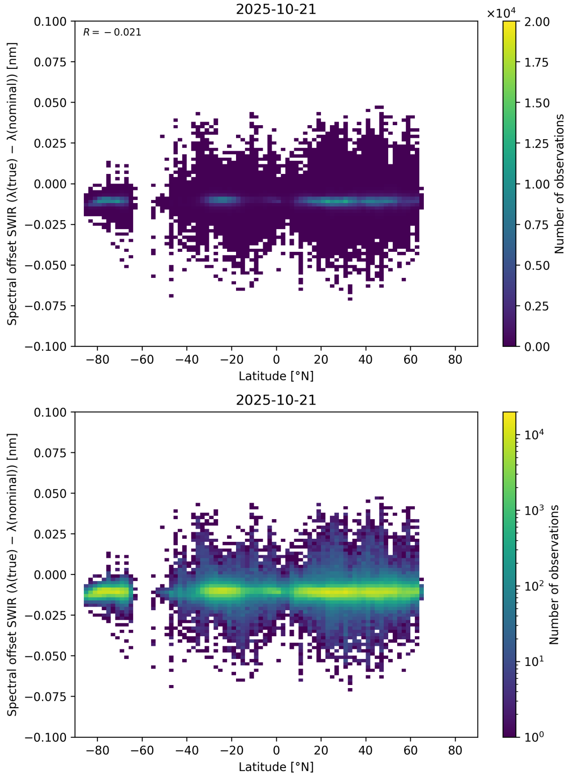
Figure 62: Scatter density plot of “Latitude” against “Spectral offset SWIR ( \lambda_{\text{true}} - \lambda_{\text{nominal}} )” for 2025-10-20 to 2025-10-22.
