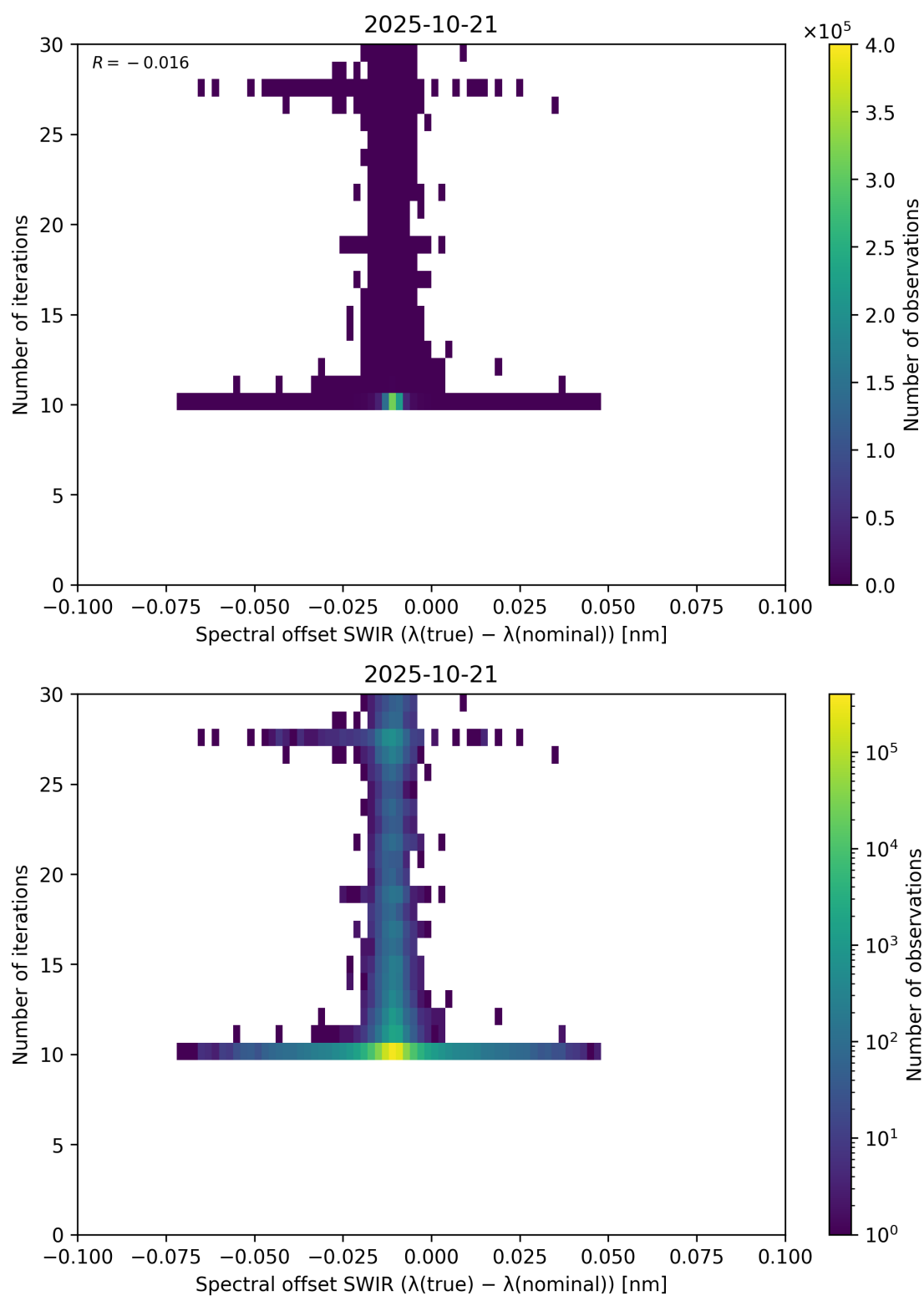
Figure 121: Scatter density plot of “Spectral offset SWIR ( \lambda_{\text{true}} - \lambda_{\text{nominal}} )” against “Number of iterations” for 2025-10-20 to 2025-10-22.
