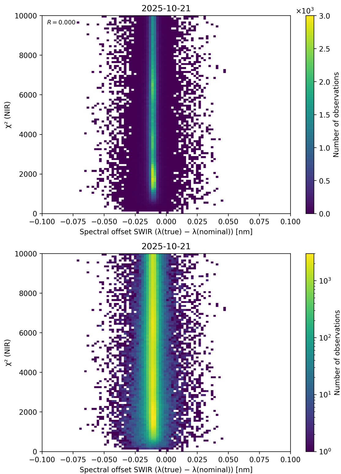
Figure 117: Scatter density plot of “Spectral offset SWIR ( \lambda_{\text{true}} - \lambda_{\text{nominal}} )” against “ \chi^2 (NIR)” for 2025-10-20 to 2025-10-22.
