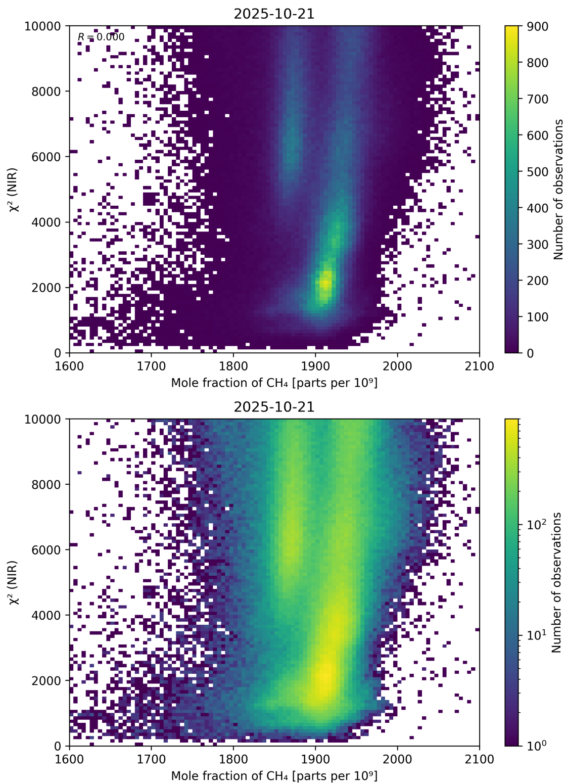
Figure 70: Scatter density plot of “Mole fraction of \text{CH}_4 ” against “ \chi^2 (NIR)” for 2025-10-20 to 2025-10-22.
