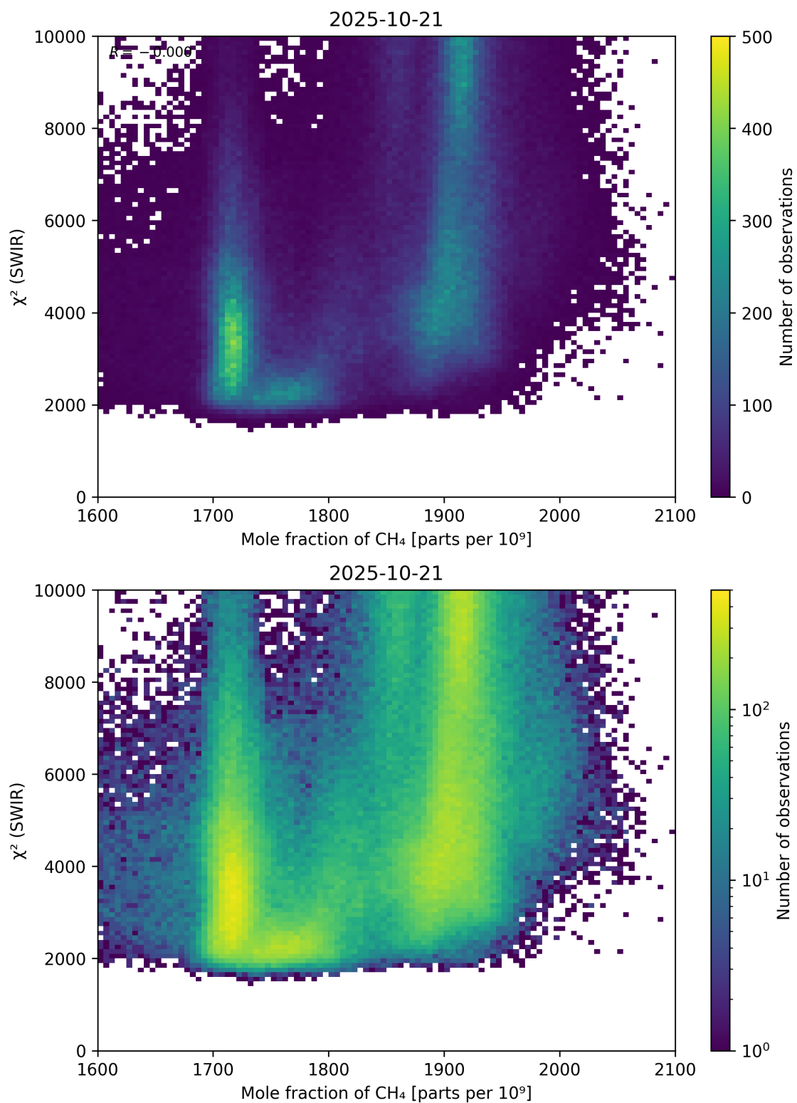
Figure 71: Scatter density plot of “Mole fraction of CH 4 ” against “ \chi^2 (SWIR)” for 2025-10-20 to 2025-10-22.
