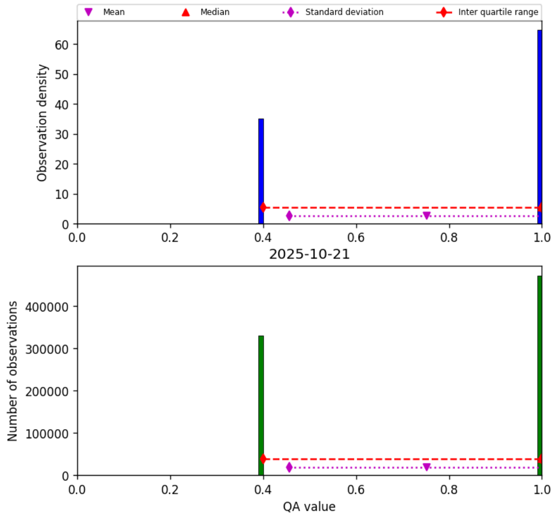
Figure 22: Histogram of “QA value” for 2025-10-20 to 2025-10-22
