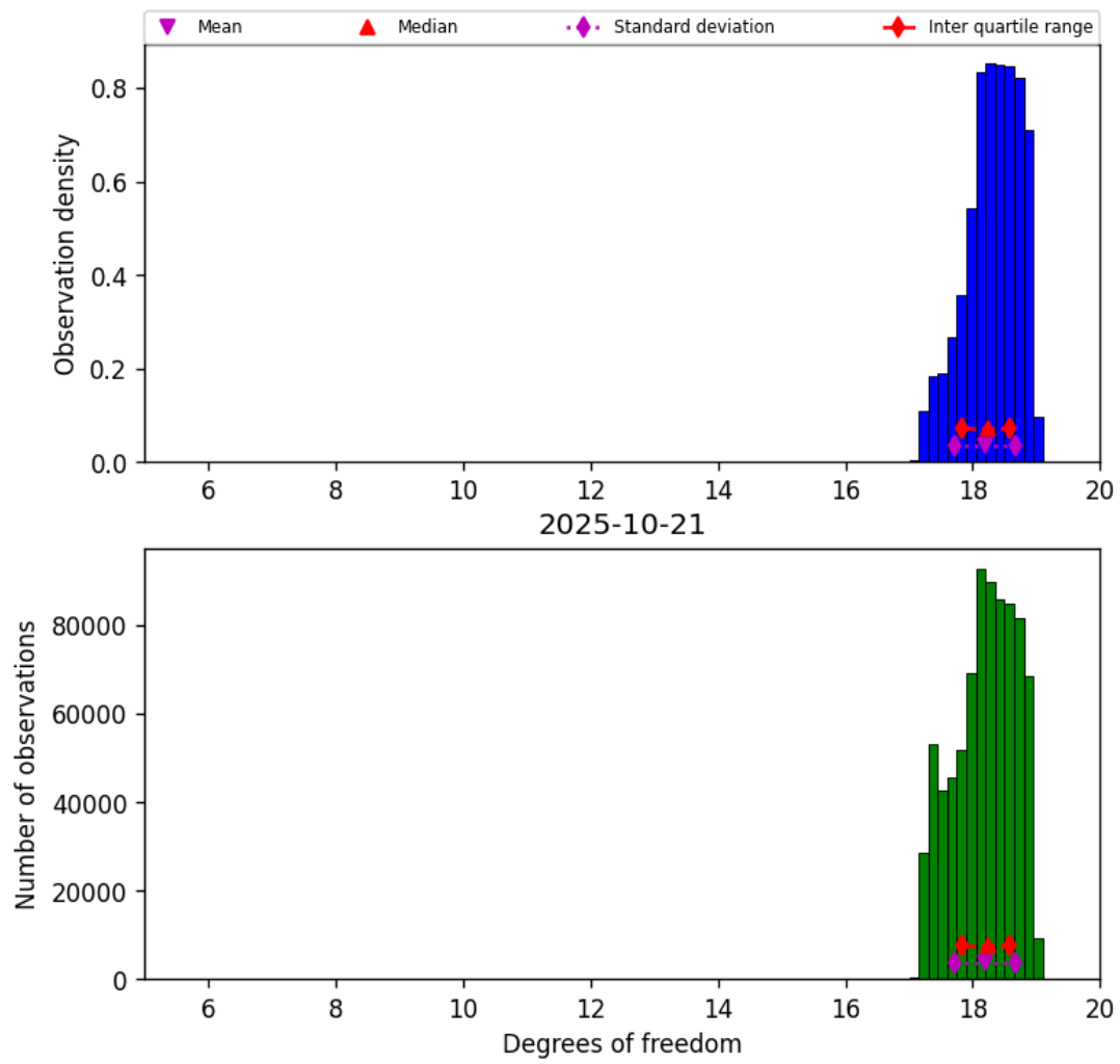
Figure 30: Histogram of “Degrees of freedom” for 2025-10-20 to 2025-10-22
