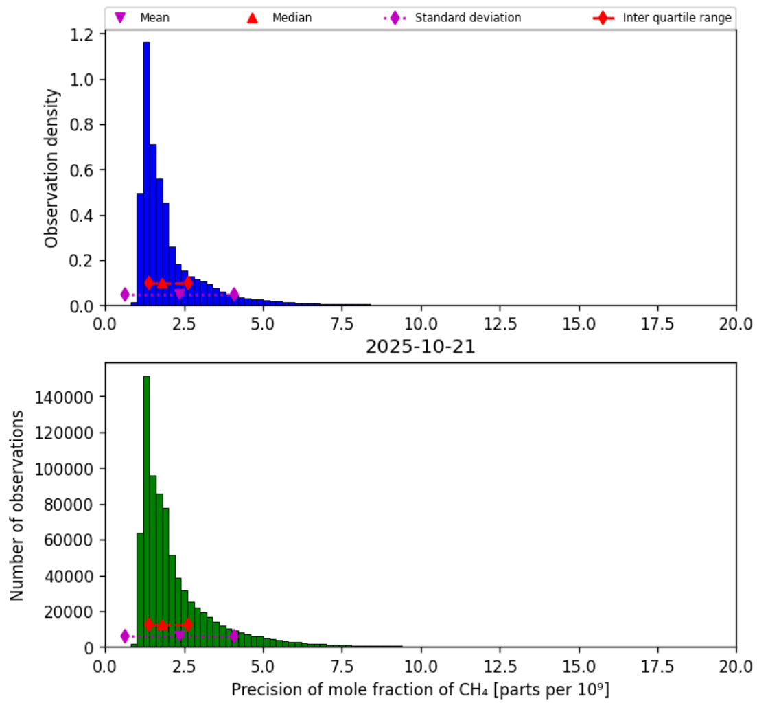
Figure 24: Histogram of “Precision of mole fraction of CH 4 ” for 2025-10-20 to 2025-10-22
