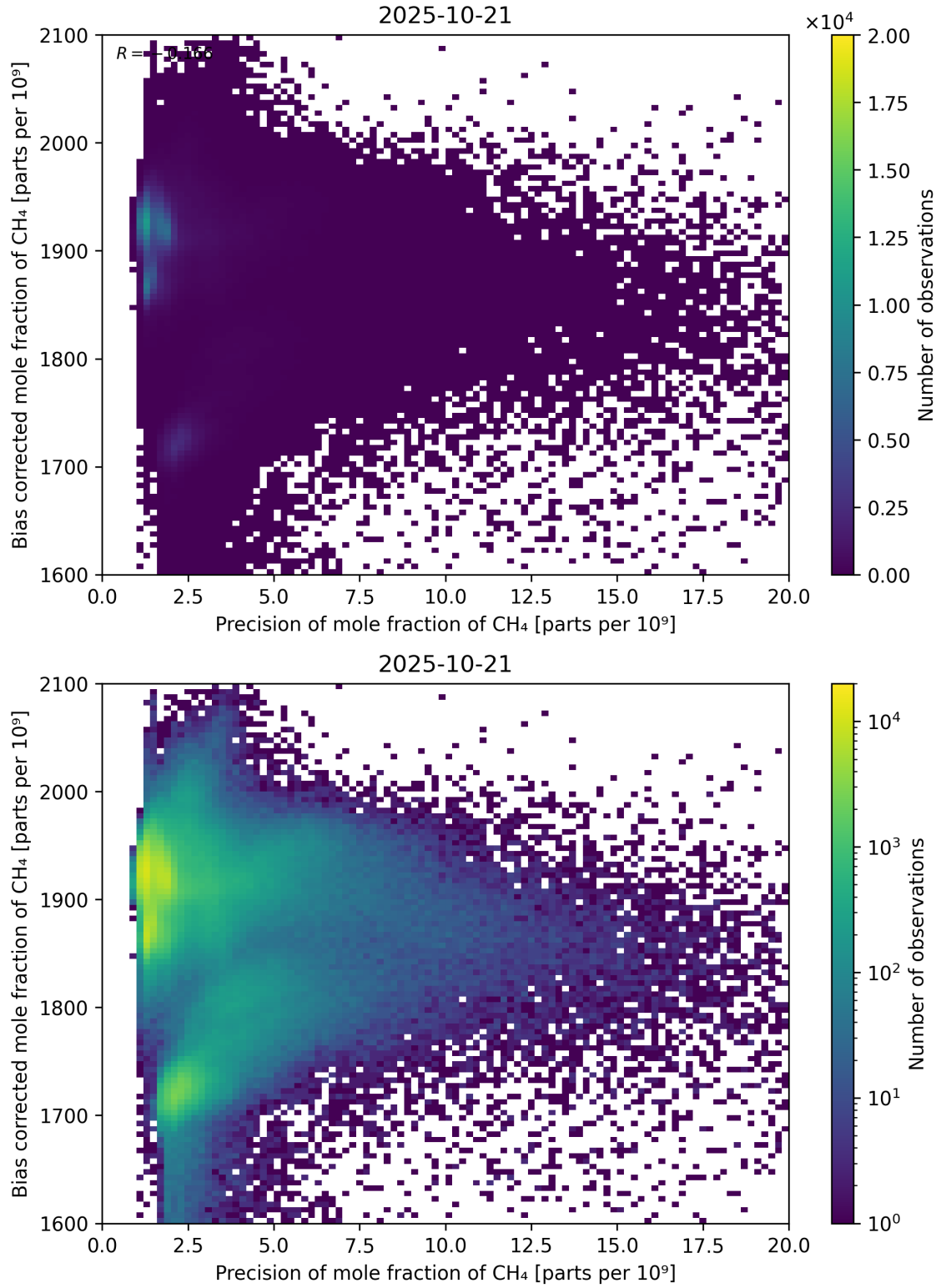
Figure 82: Scatter density plot of “Precision of mole fraction of CH 4 ” against “Bias corrected mole fraction of CH 4 ” for 2025-10-20 to 2025-10-22.
