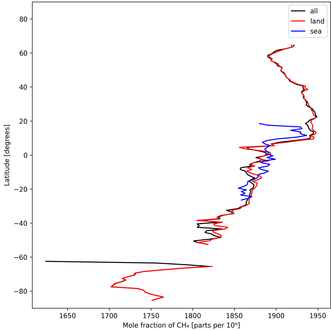
Figure 12: Zonal average of “Mole fraction of CH 4 ” for 2025-10-20 to 2025-10-22.
