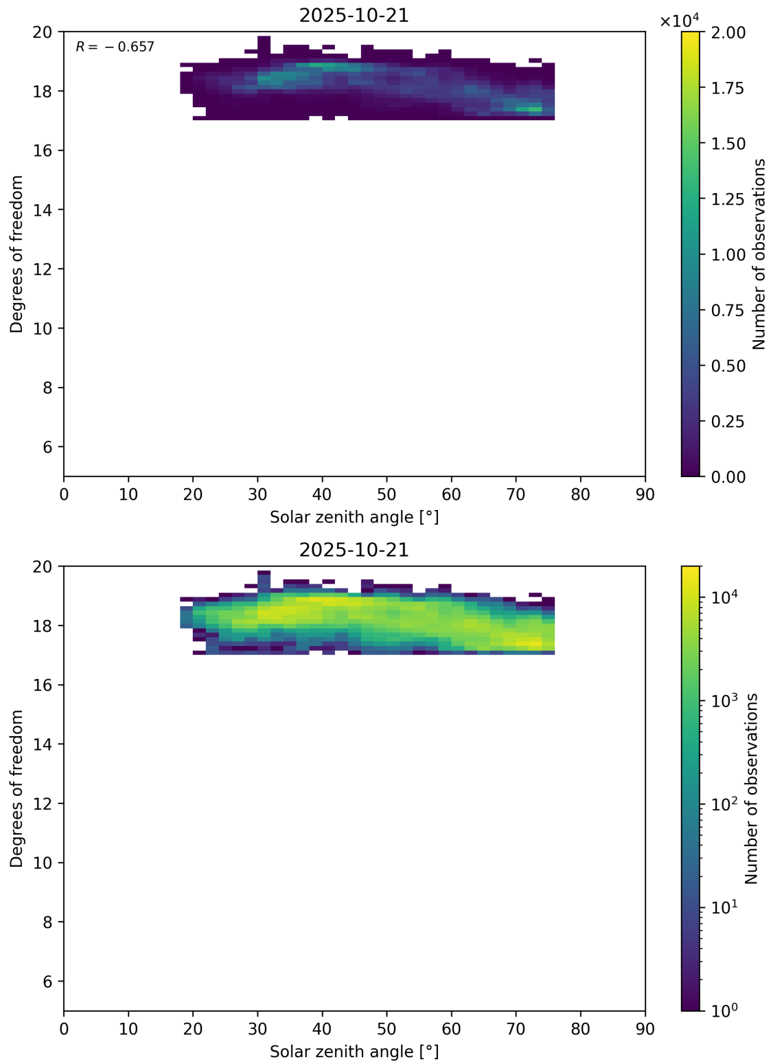
Figure 96: Scatter density plot of “Solar zenith angle” against “Degrees of freedom” for 2025-10-20 to 2025-10-22.
