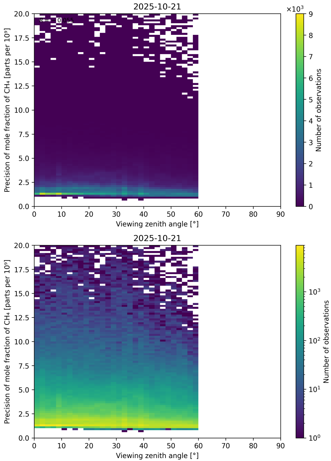
Figure 112: Scatter density plot of “Viewing zenith angle” against “Precision of mole fraction of CH 4 ” for 2025-10-20 to 2025-10-22.
