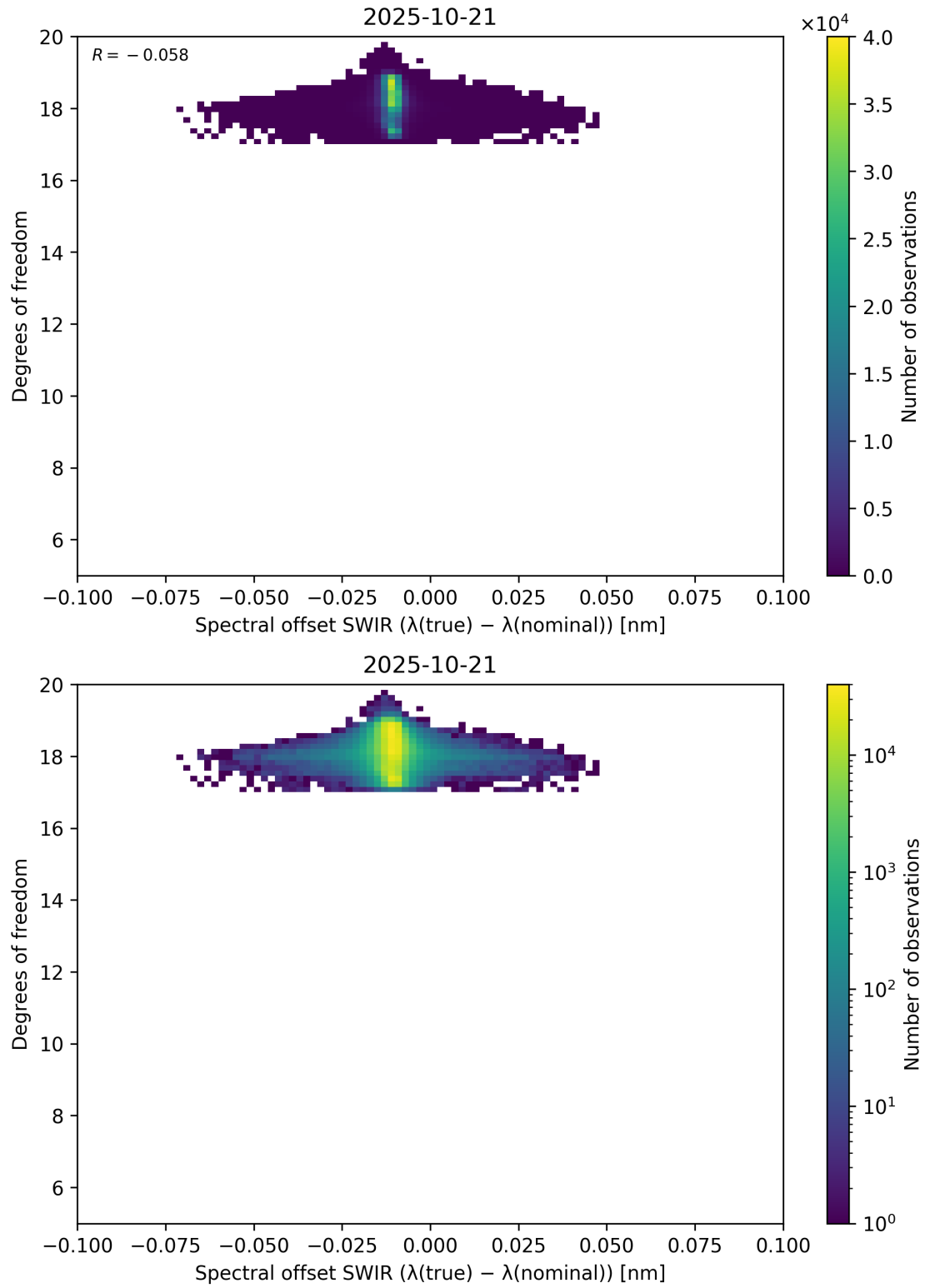
Figure 119: Scatter density plot of “Spectral offset SWIR ( \lambda_{\text{true}} - \lambda_{\text{nominal}} )” against “Degrees of freedom” for 2025-10-20 to 2025-10-22.
