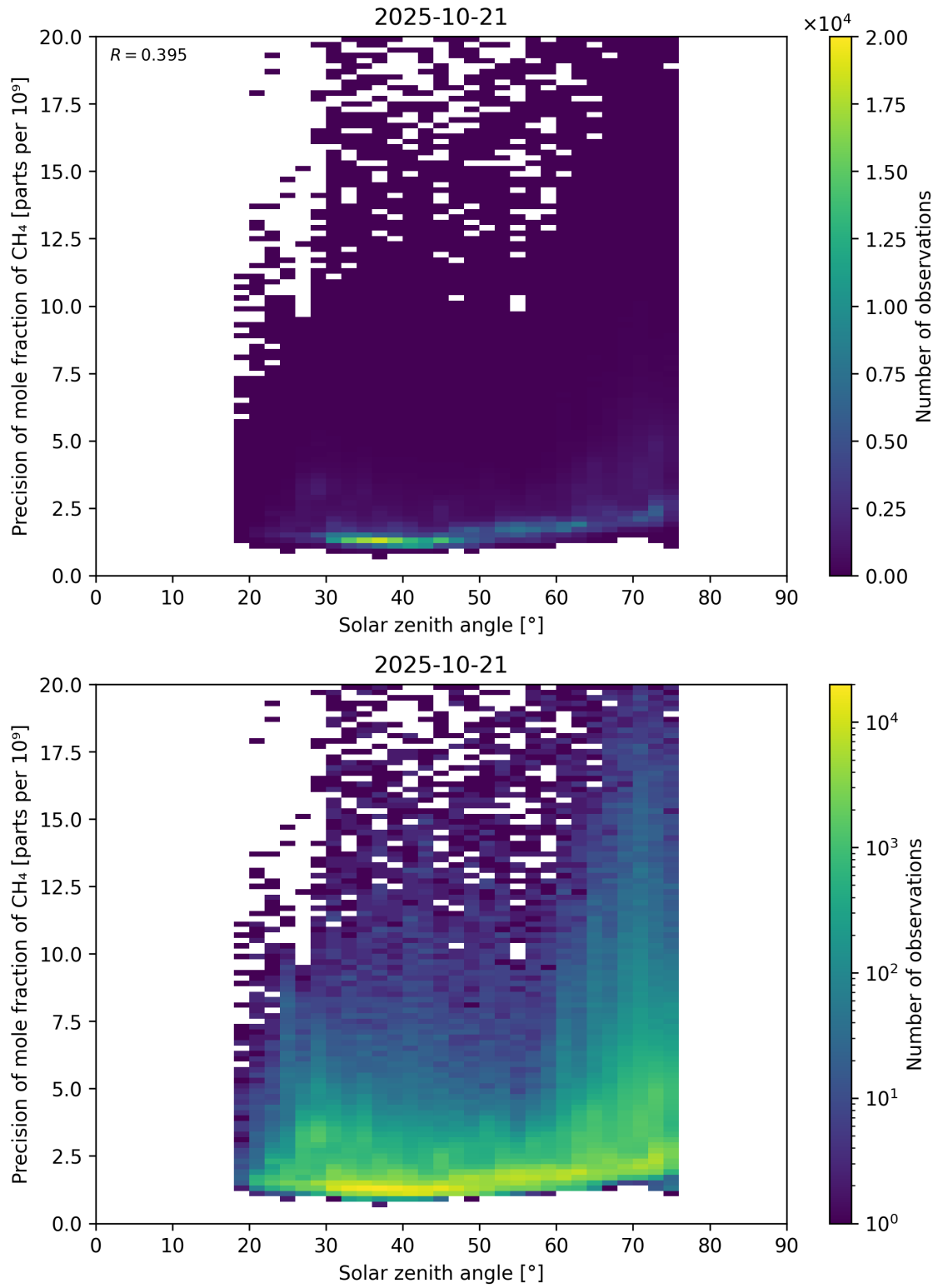
Figure 101: Scatter density plot of “Solar zenith angle” against “Precision of mole fraction of \text{CH}_4 ” for 2025-10-20 to 2025-10-22.
