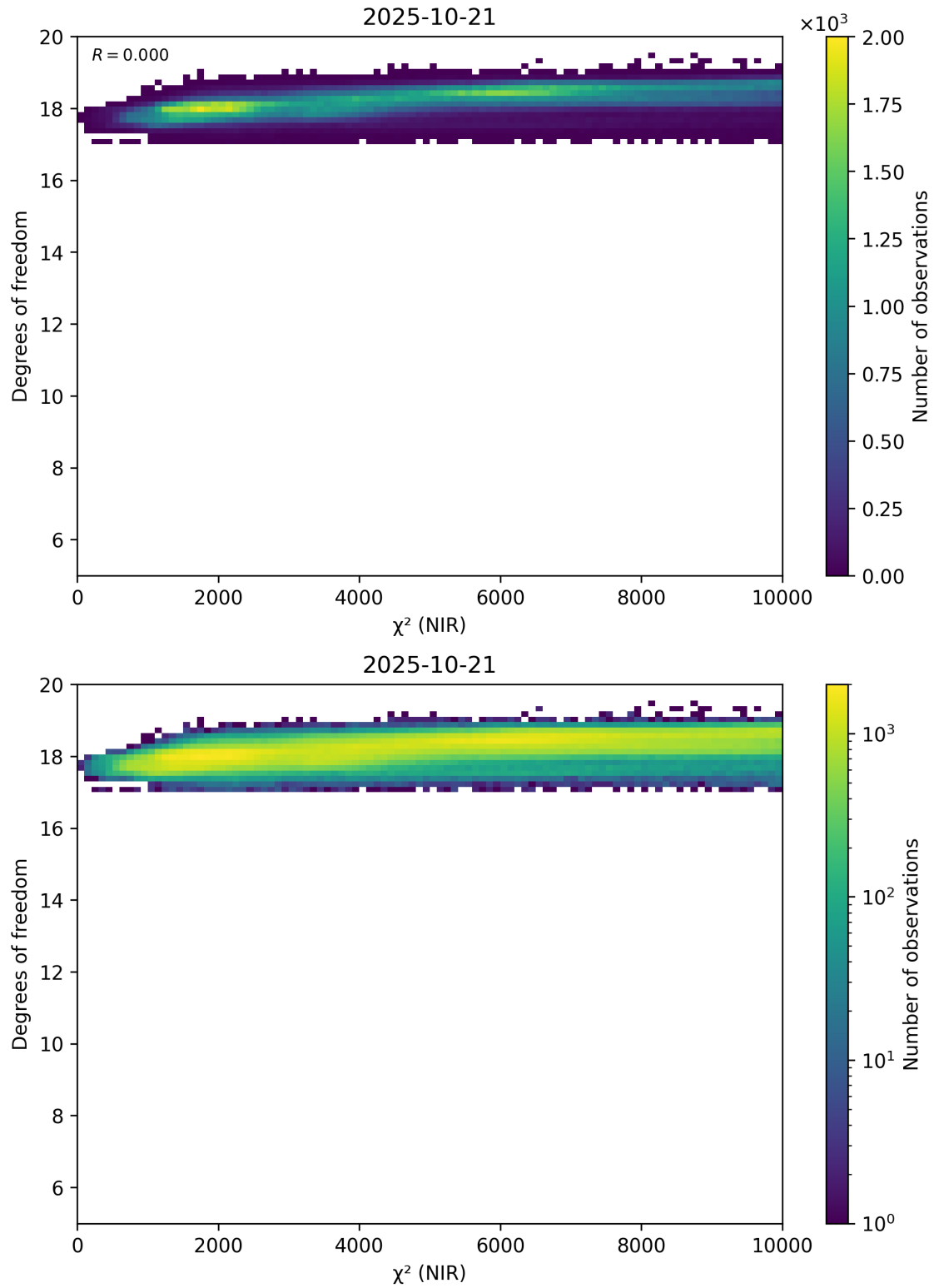
Figure 44: Scatter density plot of “ \chi^2 (NIR)” against “Degrees of freedom” for 2025-10-20 to 2025-10-22.
