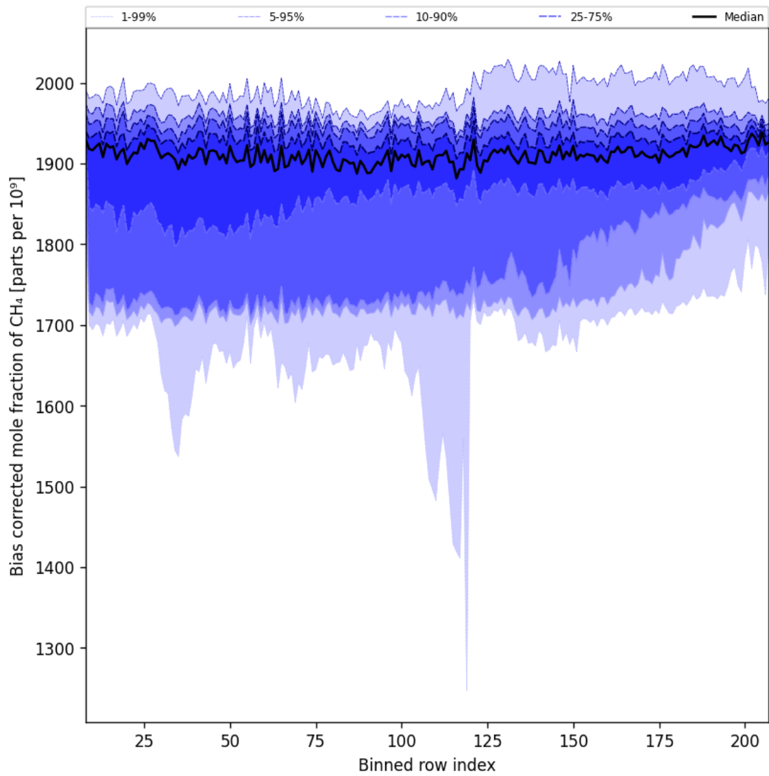
Figure 36: Along track statistics of “Bias corrected mole fraction of CH 4 ” for 2025-10-20 to 2025-10-22
