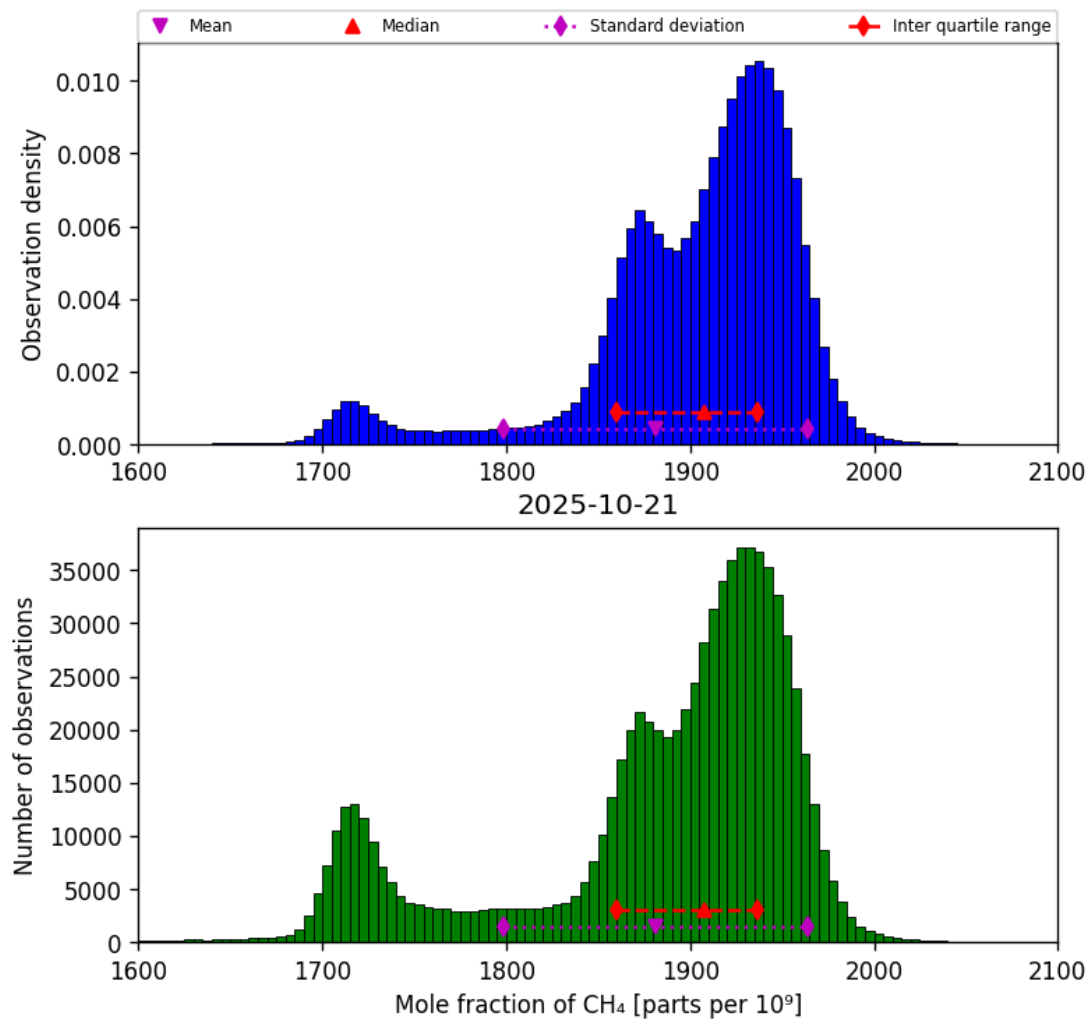
Figure 23: Histogram of “Mole fraction of CH 4 ” for 2025-10-20 to 2025-10-22
