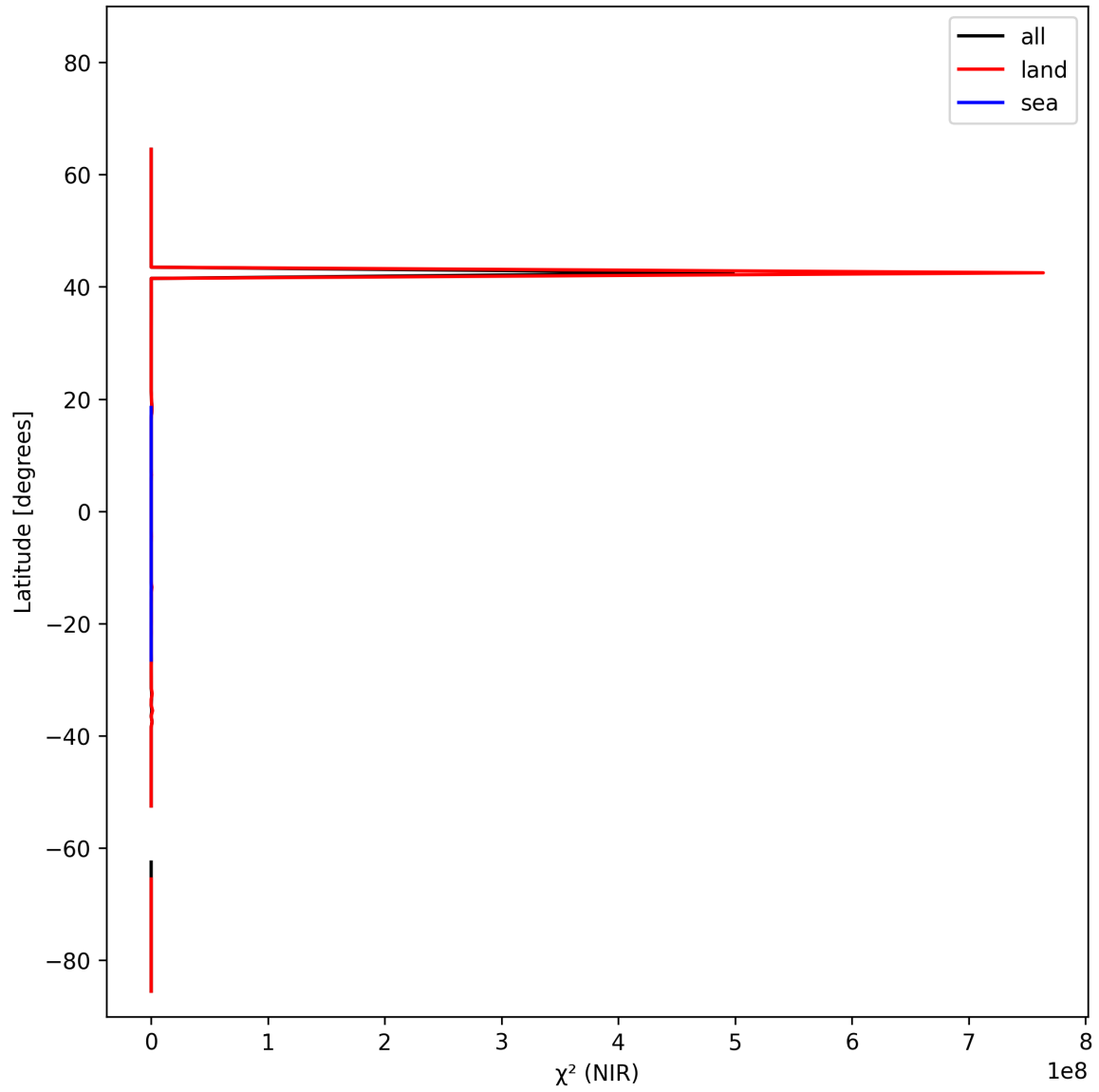
Figure 18: Zonal average of “ \chi^2 (NIR)” for 2025-10-20 to 2025-10-22.
