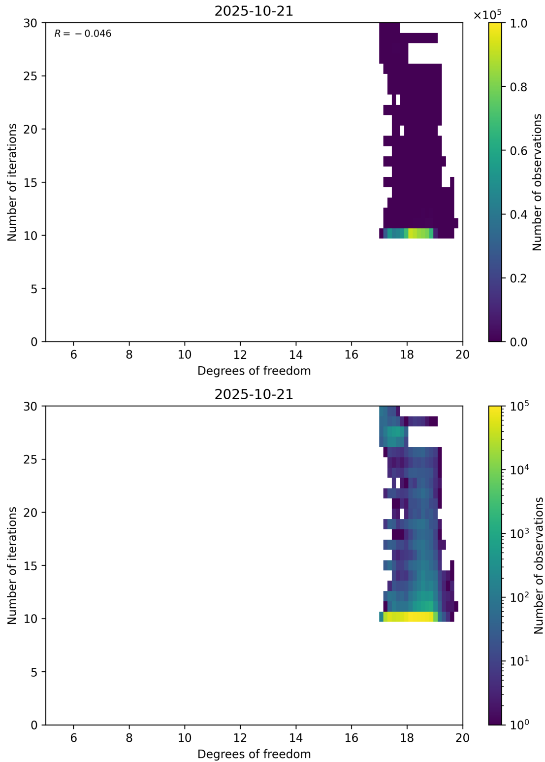
Figure 52: Scatter density plot of “Degrees of freedom” against “Number of iterations” for 2025-10-20 to 2025-10-22.
