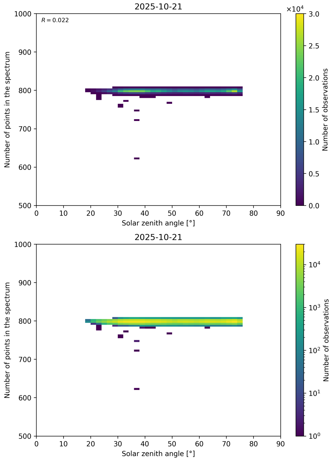
Figure 103: Scatter density plot of “Solar zenith angle” against “Number of points in the spectrum” for 2025-10-20 to 2025-10-22.
