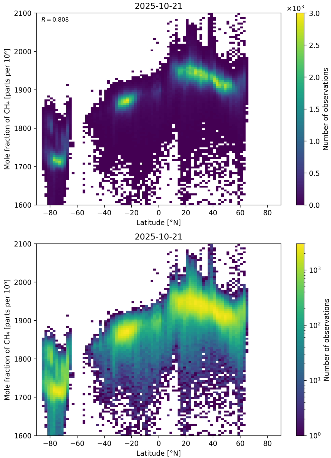
Figure 57: Scatter density plot of “Latitude” against “Mole fraction of \text{CH}_4 ” for 2025-10-20 to 2025-10-22.
