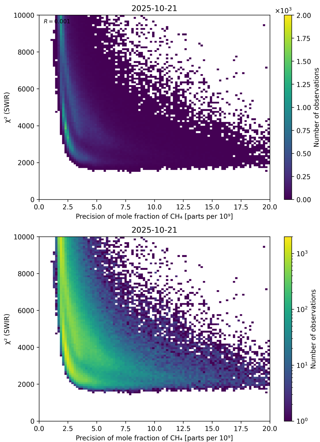
Figure 79: Scatter density plot of “Precision of mole fraction of CH 4 ” against “ \chi^2 (SWIR)” for 2025-10-20 to 2025-10-22.
