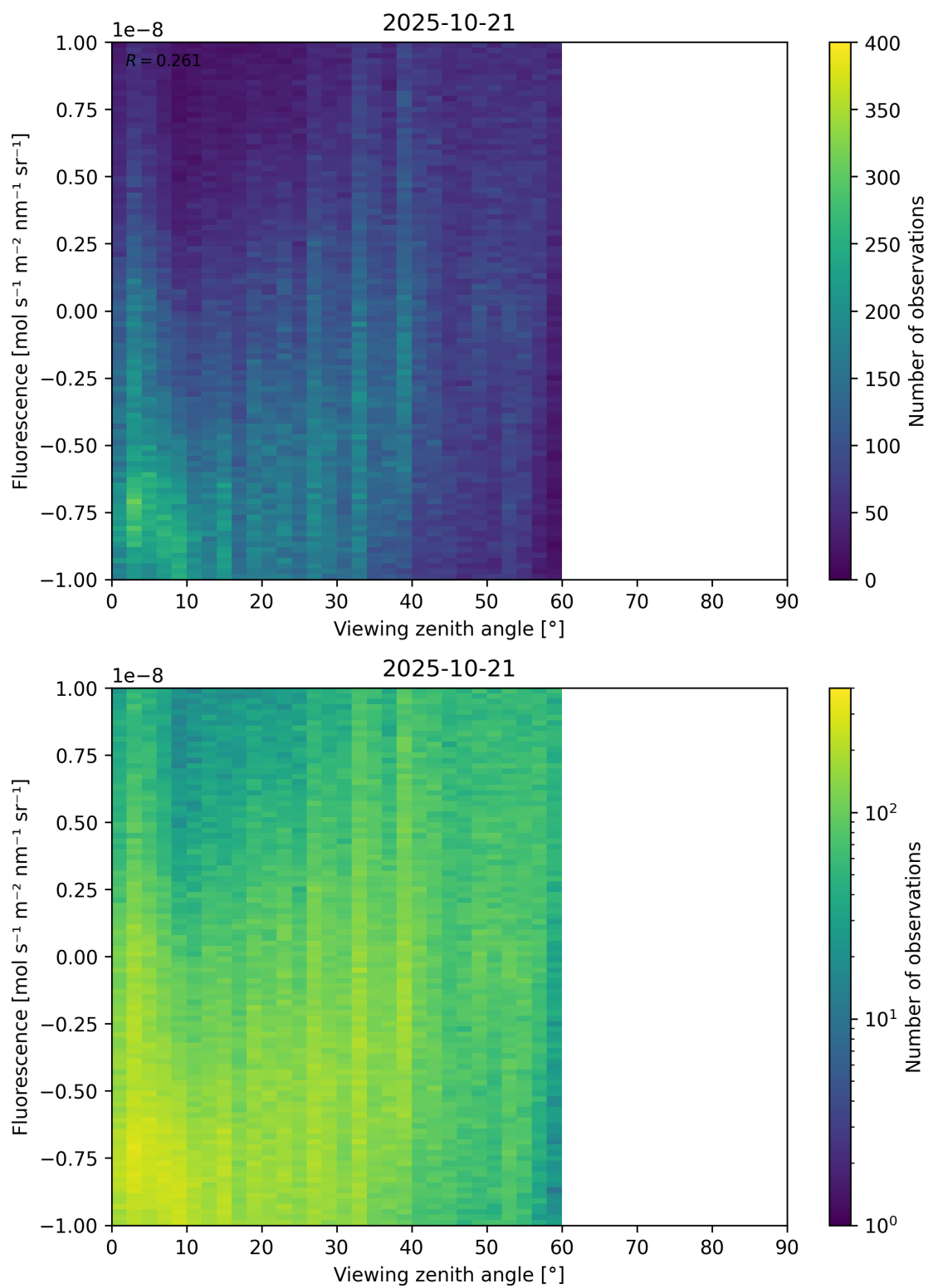
Figure 108: Scatter density plot of “Viewing zenith angle” against “Fluorescence” for 2025-10-20 to 2025-10-22.
