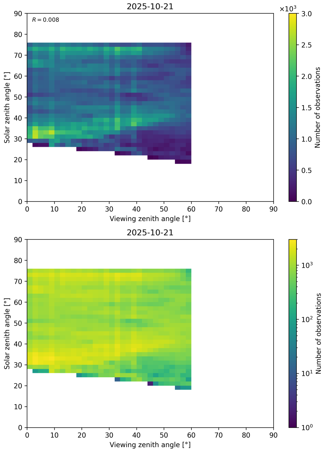
Figure 115: Scatter density plot of “Viewing zenith angle” against “Solar zenith angle” for 2025-10-20 to 2025-10-22.
