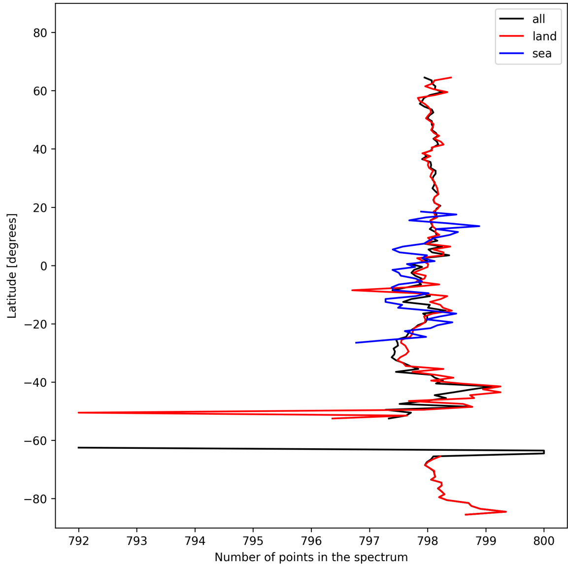
Figure 15: Zonal average of “Number of points in the spectrum” for 2025-10-20 to 2025-10-22.
