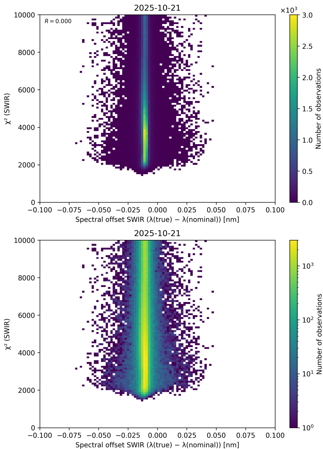
Figure 118: Scatter density plot of “Spectral offset SWIR ( \lambda_{\text{true}} - \lambda_{\text{nominal}} )” against “ \chi^2 (SWIR)” for 2025-10-20 to 2025-10-22.
