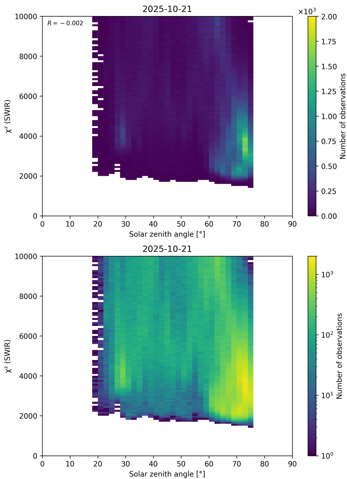
Figure 95: Scatter density plot of “Solar zenith angle” against “ \chi^2 (SWIR)” for 2025-10-20 to 2025-10-22.
