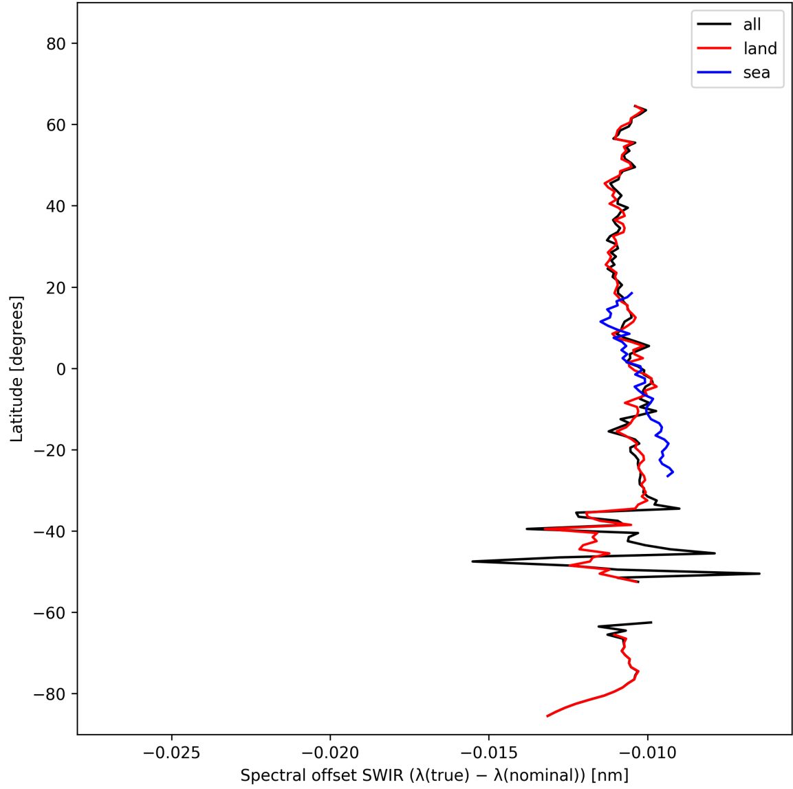
Figure 16: Zonal average of “Spectral offset SWIR ( \lambda_{\text{true}} - \lambda_{\text{nominal}} )” for 2025-10-20 to 2025-10-22.
