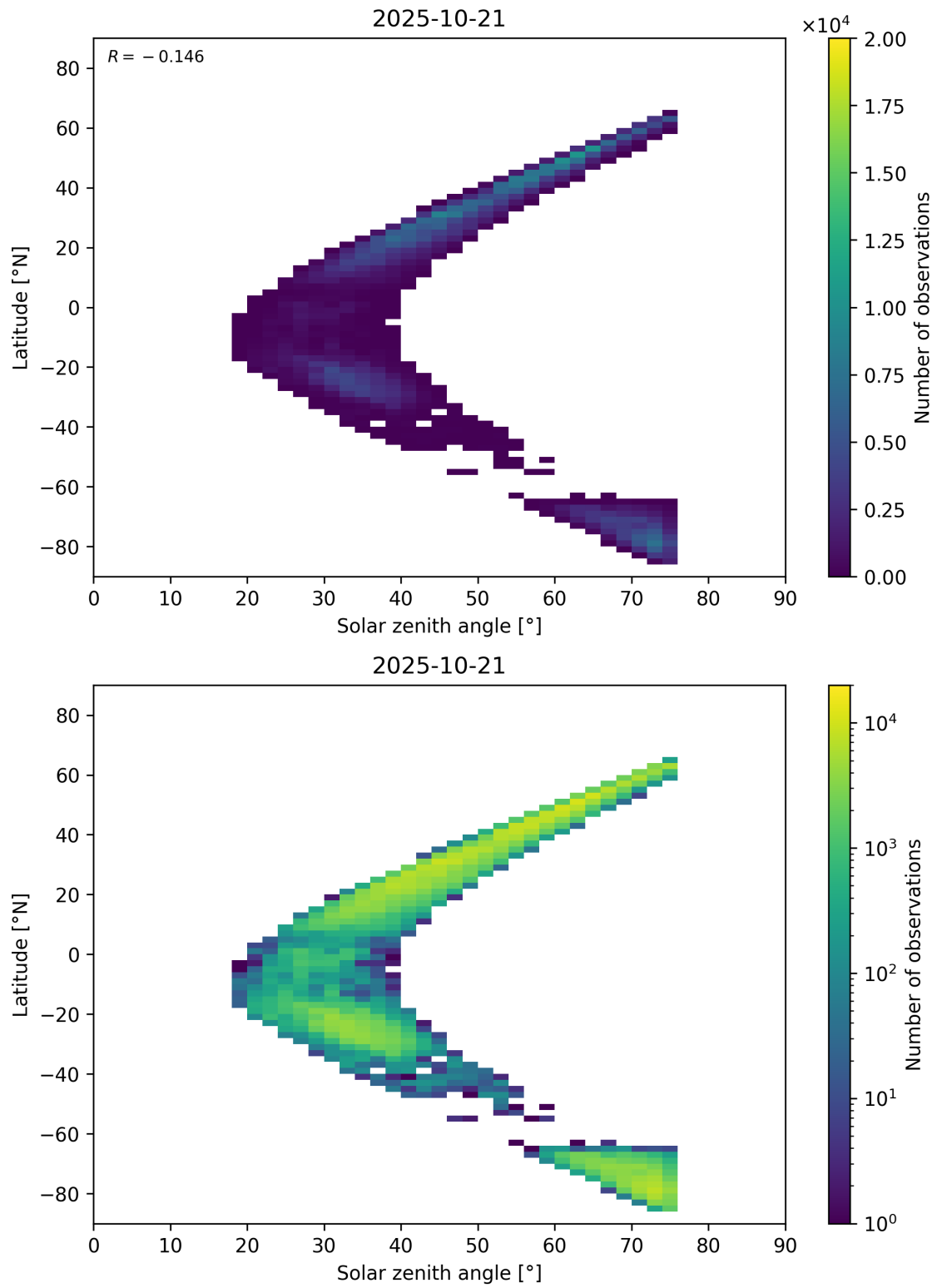
Figure 98: Scatter density plot of “Solar zenith angle” against “Latitude” for 2025-10-20 to 2025-10-22.
