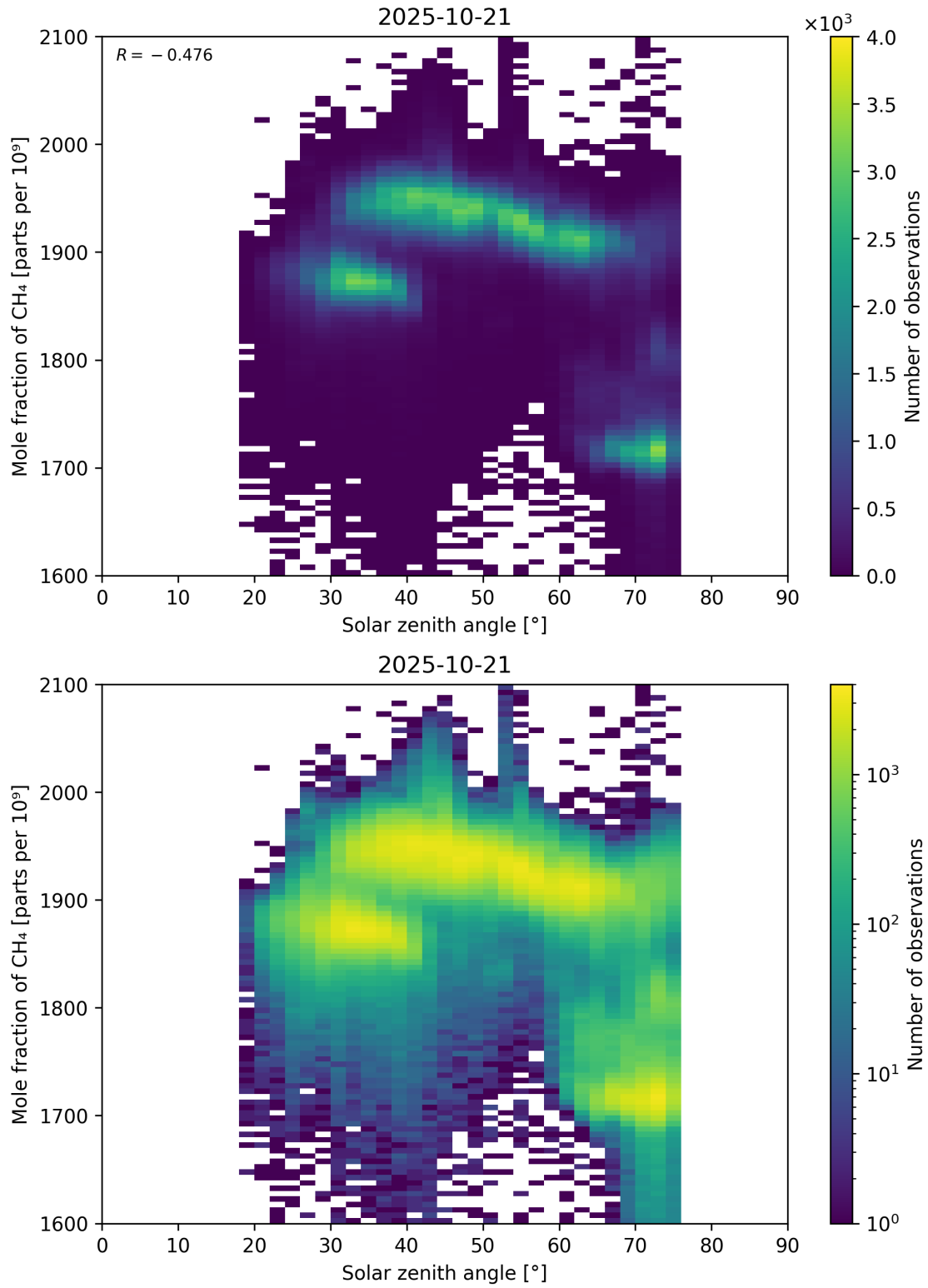
Figure 99: Scatter density plot of “Solar zenith angle” against “Mole fraction of CH 4 ” for 2025-10-20 to 2025-10-22.
