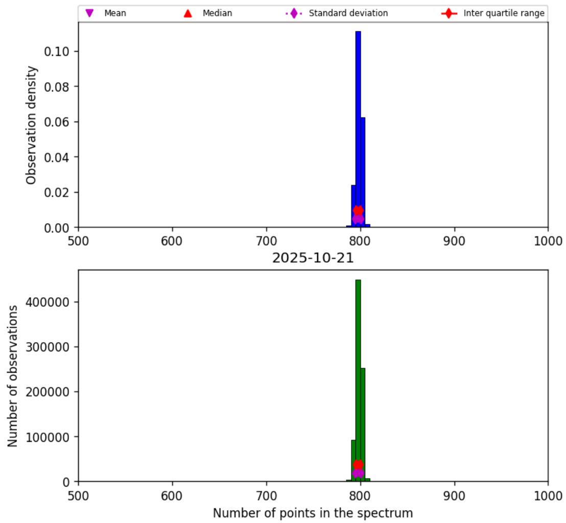
Figure 26: Histogram of “Number of points in the spectrum” for 2025-10-20 to 2025-10-22
