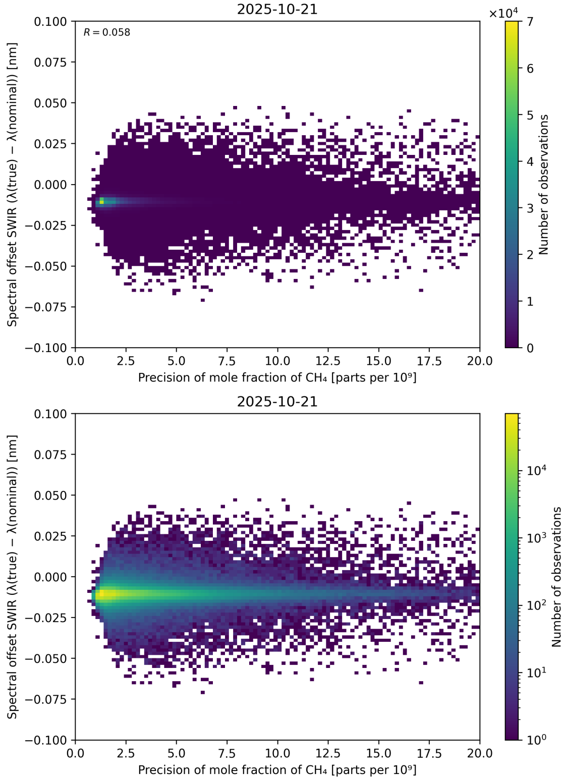
Figure 85: Scatter density plot of “Precision of mole fraction of \text{CH}_4 ” against “Spectral offset SWIR ( \lambda_{\text{true}} - \lambda_{\text{nominal}} )” for 2025-10-20 to 2025-10-22.
