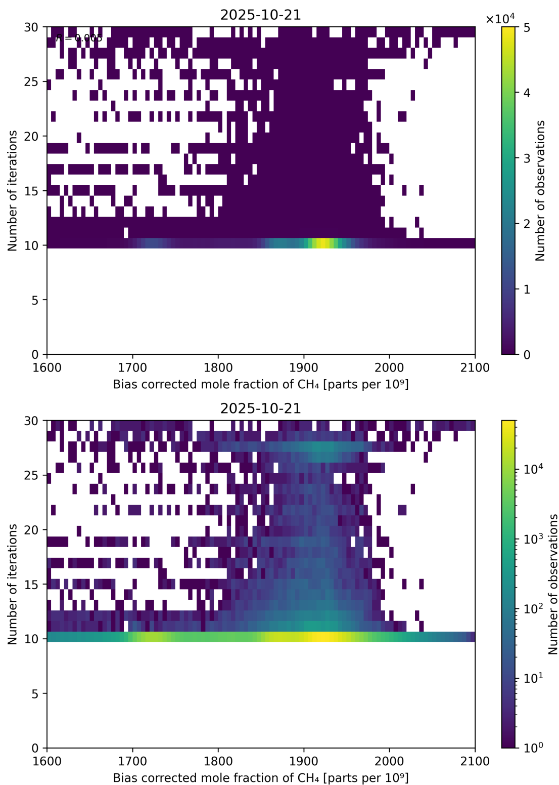
Figure 67: Scatter density plot of “Bias corrected mole fraction of CH 4 ” against “Number of iterations” for 2025-10-20 to 2025-10-22.
