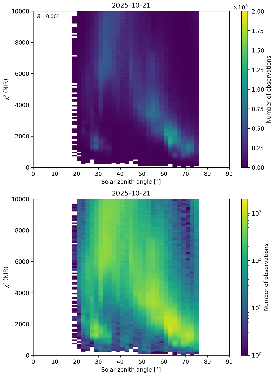
Figure 94: Scatter density plot of “Solar zenith angle” against “ \chi^2 (NIR)” for 2025-10-20 to 2025-10-22.
