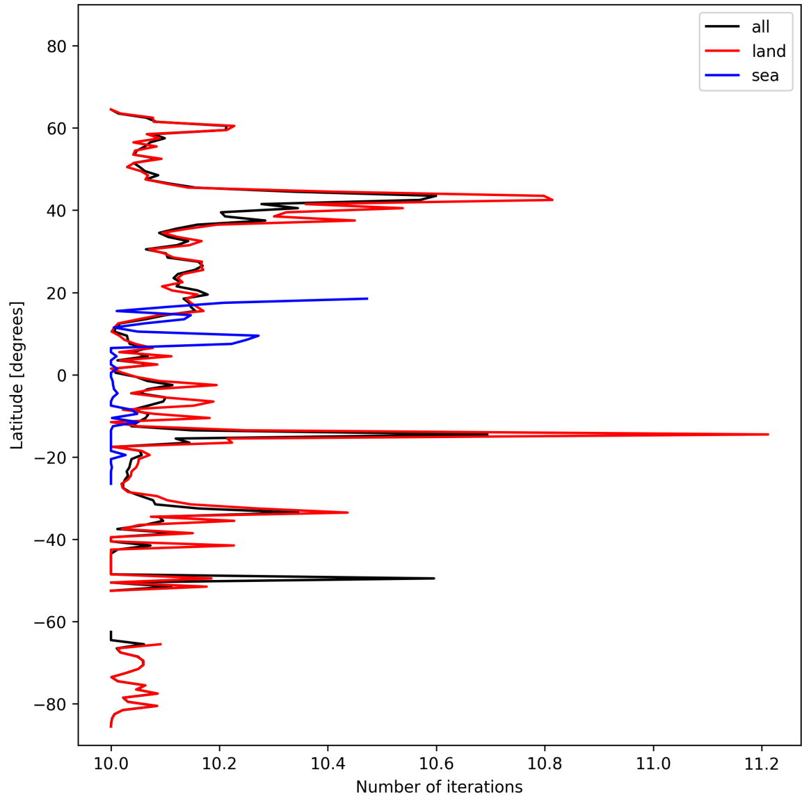
Figure 20: Zonal average of “Number of iterations” for 2025-10-20 to 2025-10-22.
