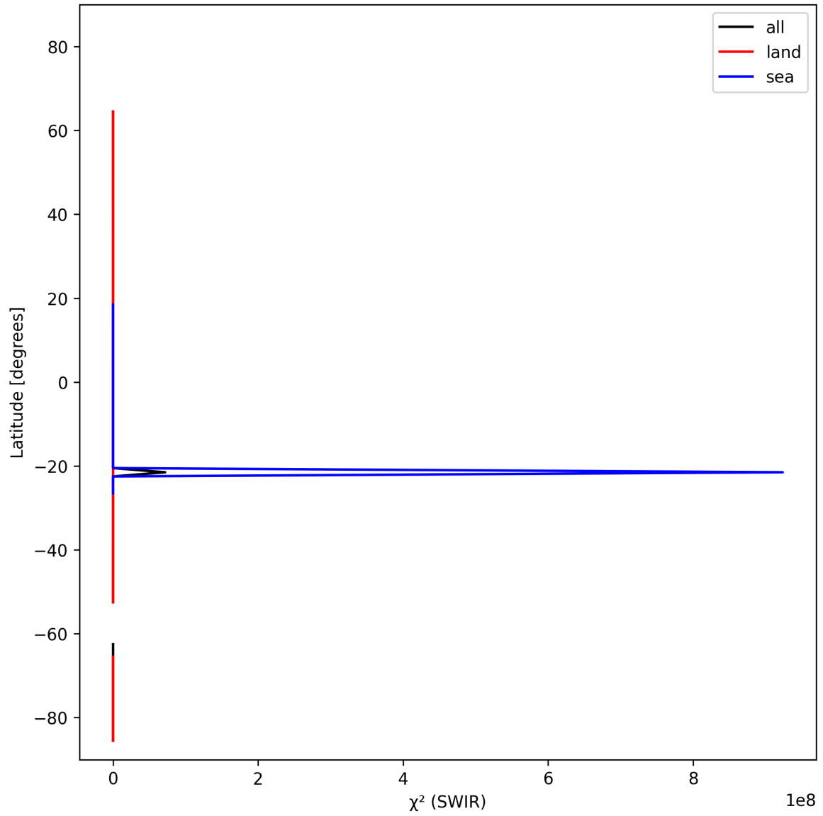
Figure 17: Zonal average of “ \chi^2 (SWIR)” for 2025-10-20 to 2025-10-22.
