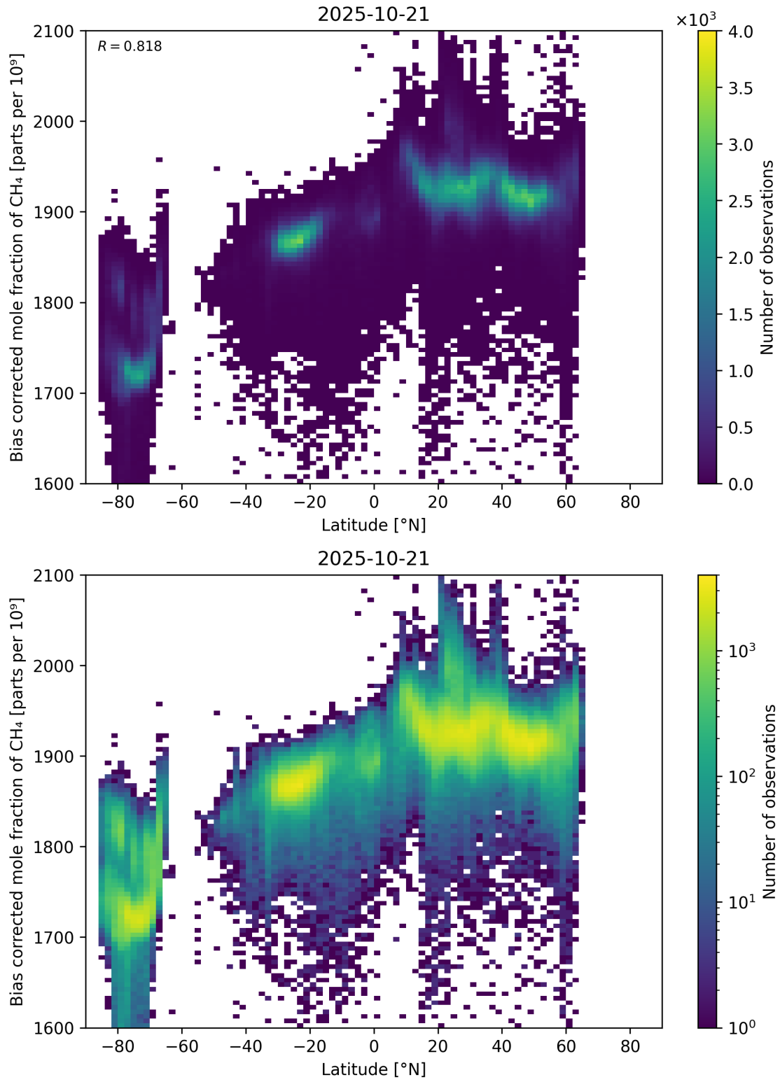
Figure 58: Scatter density plot of “Latitude” against “Bias corrected mole fraction of \text{CH}_4 ” for 2025-10-20 to 2025-10-22.
