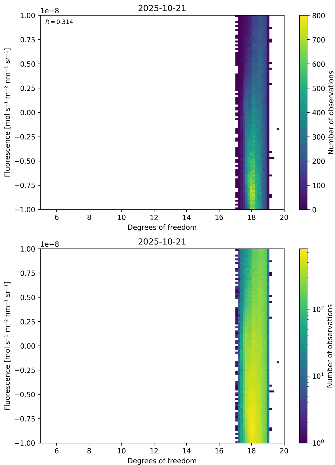
Figure 51: Scatter density plot of “Degrees of freedom” against “Fluorescence” for 2025-10-20 to 2025-10-22.
