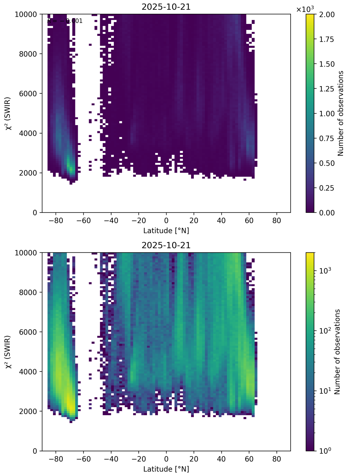
Figure 54: Scatter density plot of “Latitude” against “ \chi^2 (SWIR)” for 2025-10-20 to 2025-10-22.
