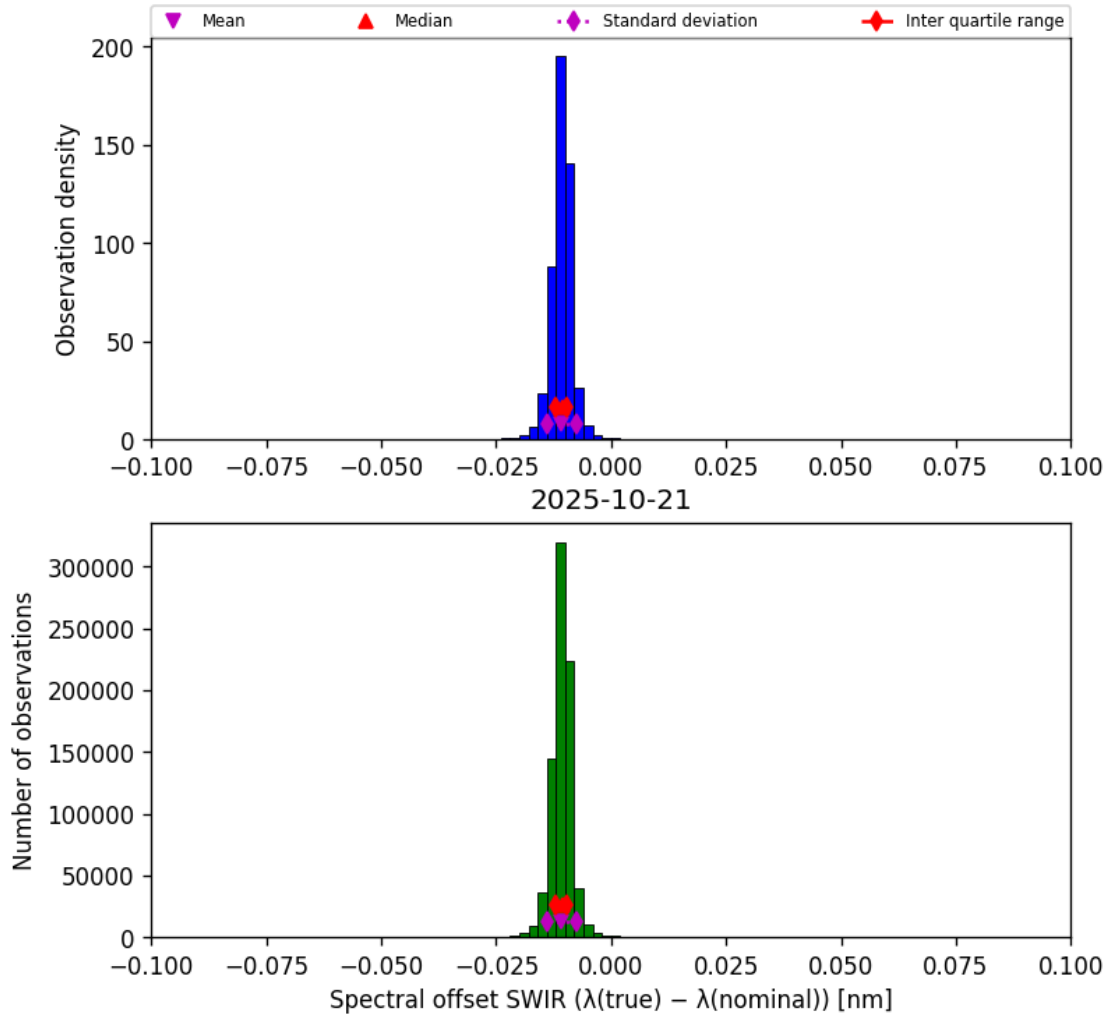
Figure 27: Histogram of “Spectral offset SWIR ( \lambda_{\text{true}} - \lambda_{\text{nominal}} )” for 2025-10-20 to 2025-10-22
