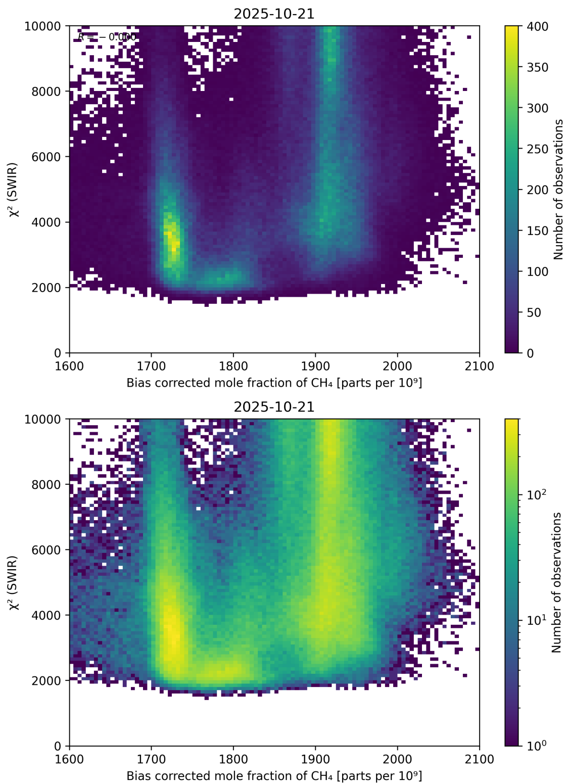
Figure 64: Scatter density plot of “Bias corrected mole fraction of CH 4 ” against “ \chi^2 (SWIR)” for 2025-10-20 to 2025-10-22.
