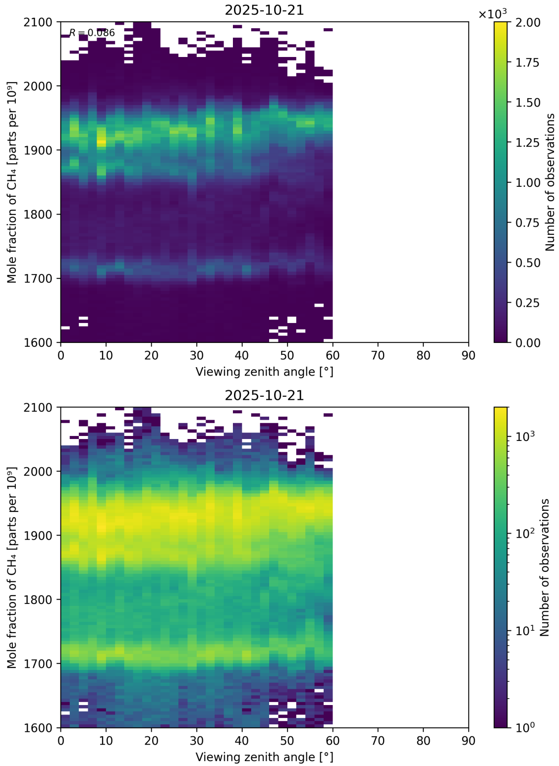
Figure 110: Scatter density plot of “Viewing zenith angle” against “Mole fraction of CH 4 ” for 2025-10-20 to 2025-10-22.
