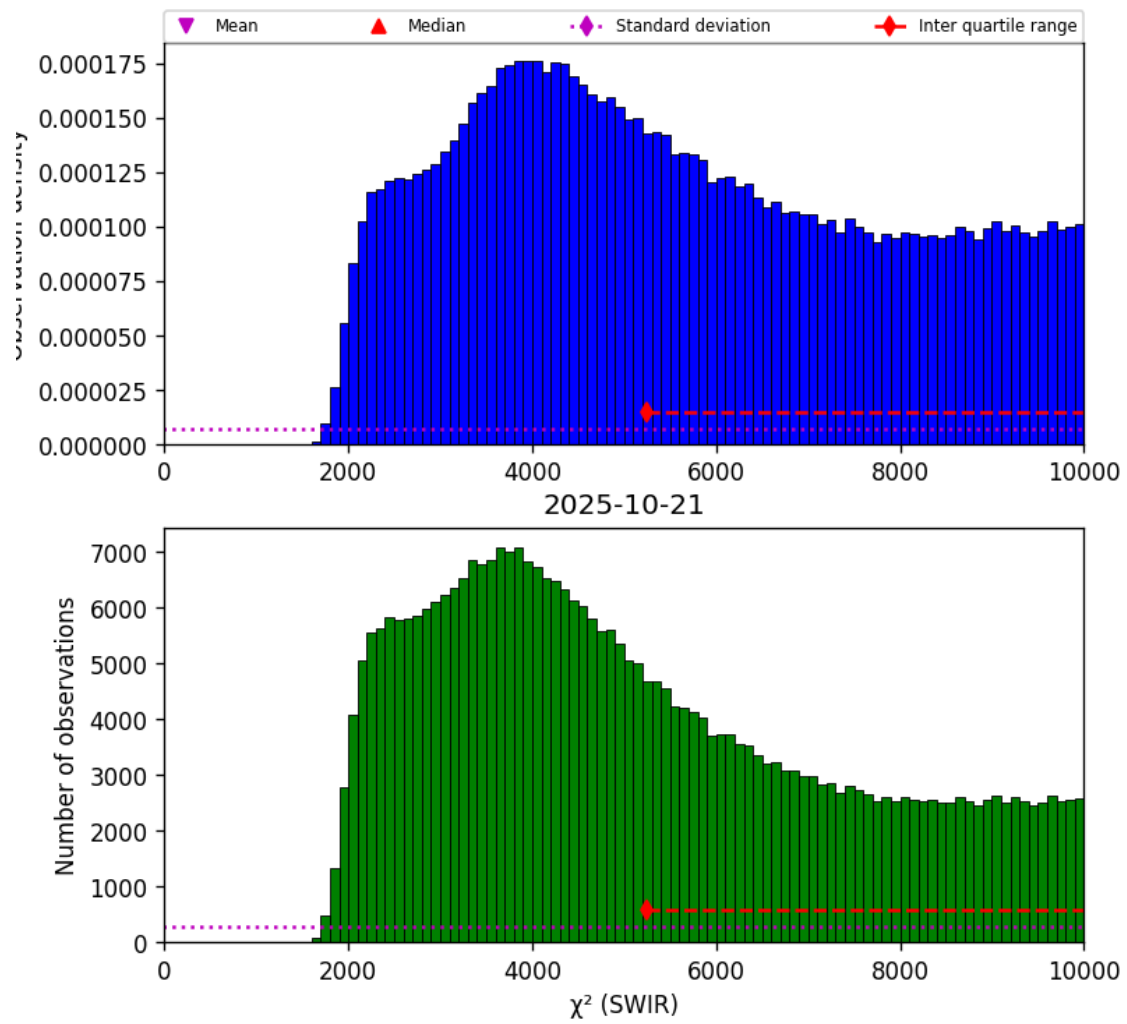
Figure 28: Histogram of “ \chi^2 (SWIR)” for 2025-10-20 to 2025-10-22
