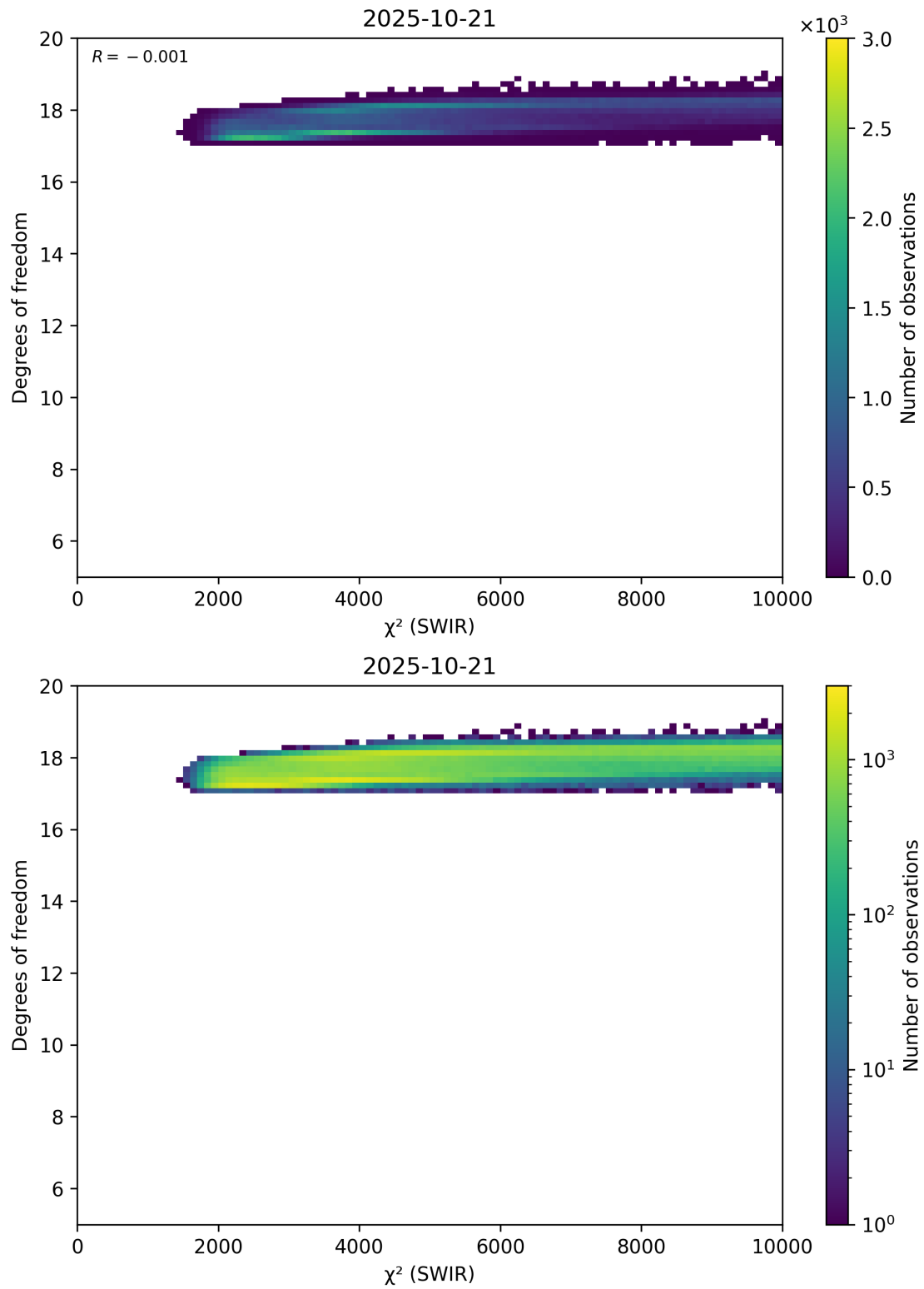
Figure 48: Scatter density plot of “ \chi^2 (SWIR)” against “Degrees of freedom” for 2025-10-20 to 2025-10-22.
