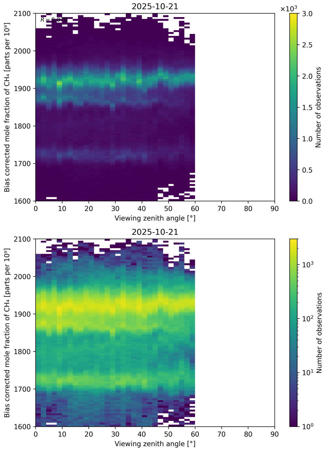
Figure 111: Scatter density plot of “Viewing zenith angle” against “Bias corrected mole fraction of CH 4 ” for 2025-10-20 to 2025-10-22.
