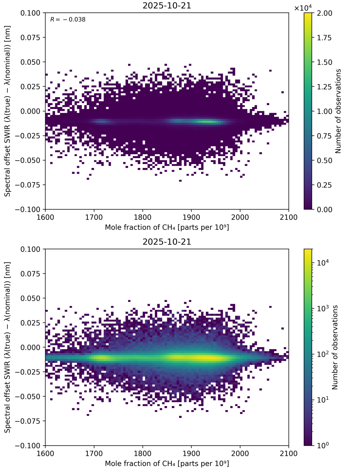
Figure 86: Scatter density plot of “Mole fraction of \text{CH}_4 ” against “Spectral offset SWIR ( \lambda_{\text{true}} - \lambda_{\text{nominal}} )” for 2025-10-20 to 2025-10-22.
