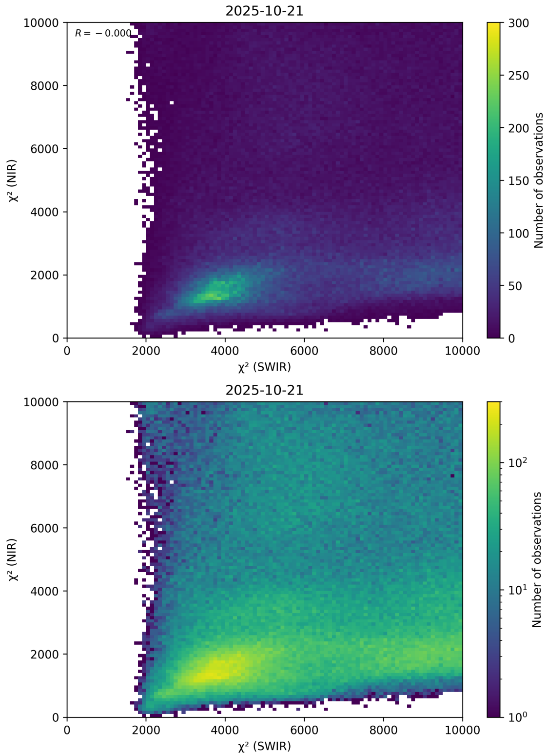
Figure 47: Scatter density plot of “ \chi^2 (SWIR)” against “ \chi^2 (NIR)” for 2025-10-20 to 2025-10-22.
