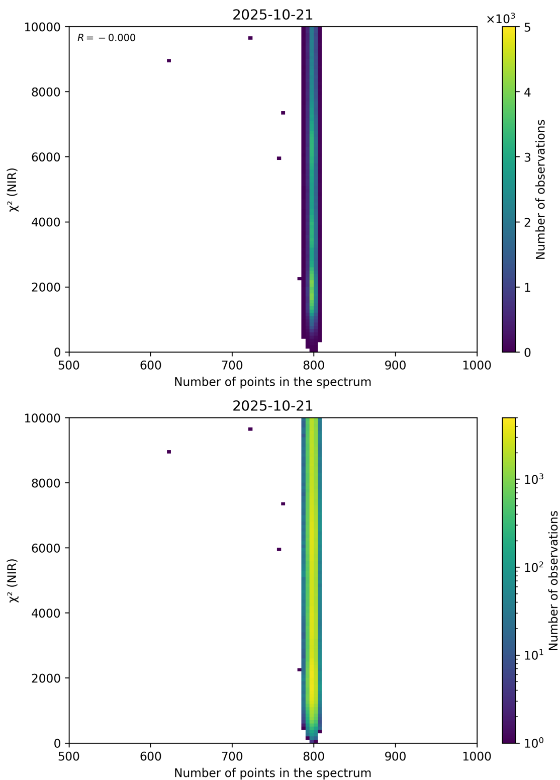
Figure 88: Scatter density plot of “Number of points in the spectrum” against “ \chi^2 (NIR)” for 2025-10-20 to 2025-10-22.
