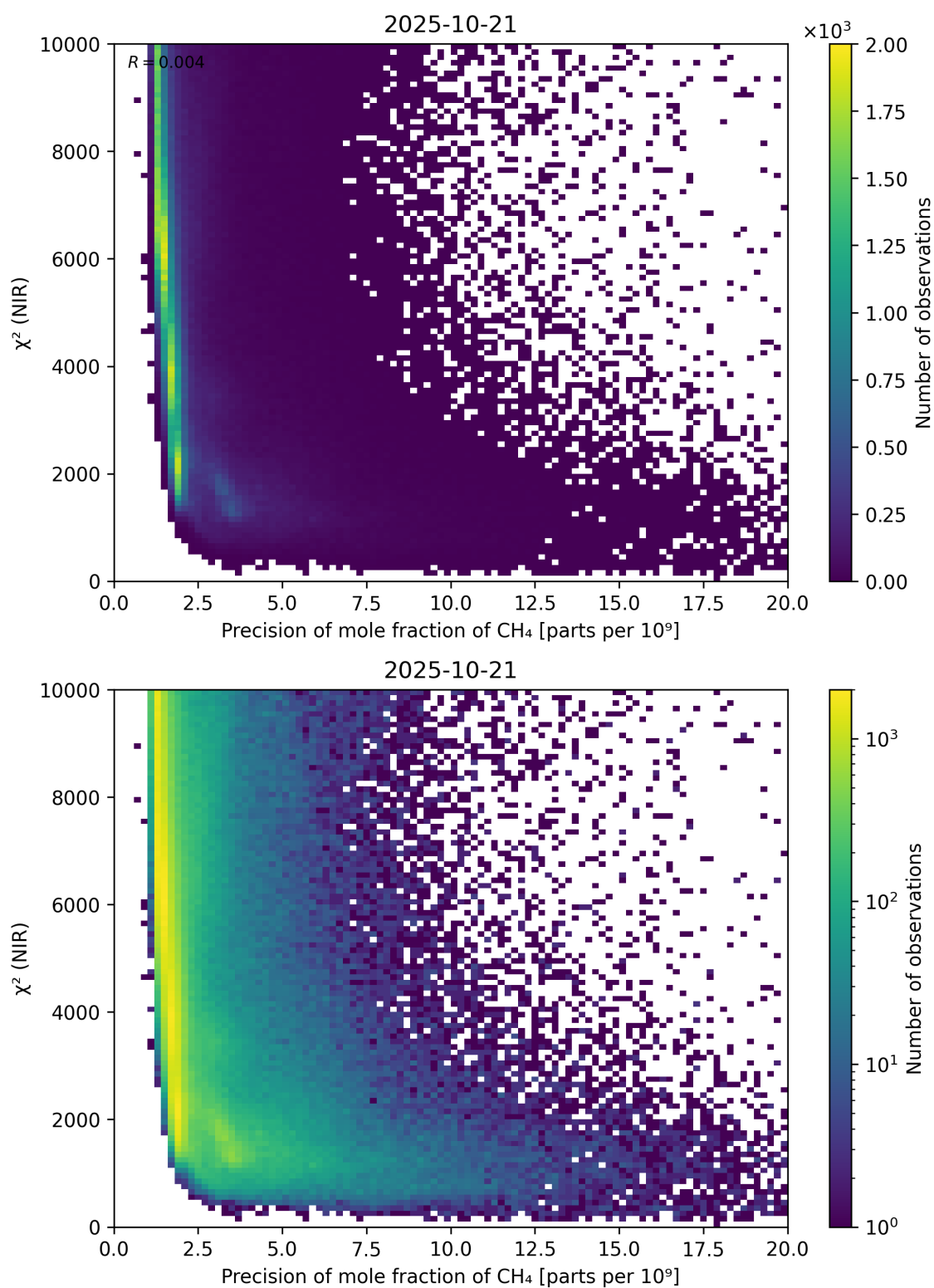
Figure 78: Scatter density plot of “Precision of mole fraction of \text{CH}_4 ” against “ \chi^2 (NIR)” for 2025-10-20 to 2025-10-22.
