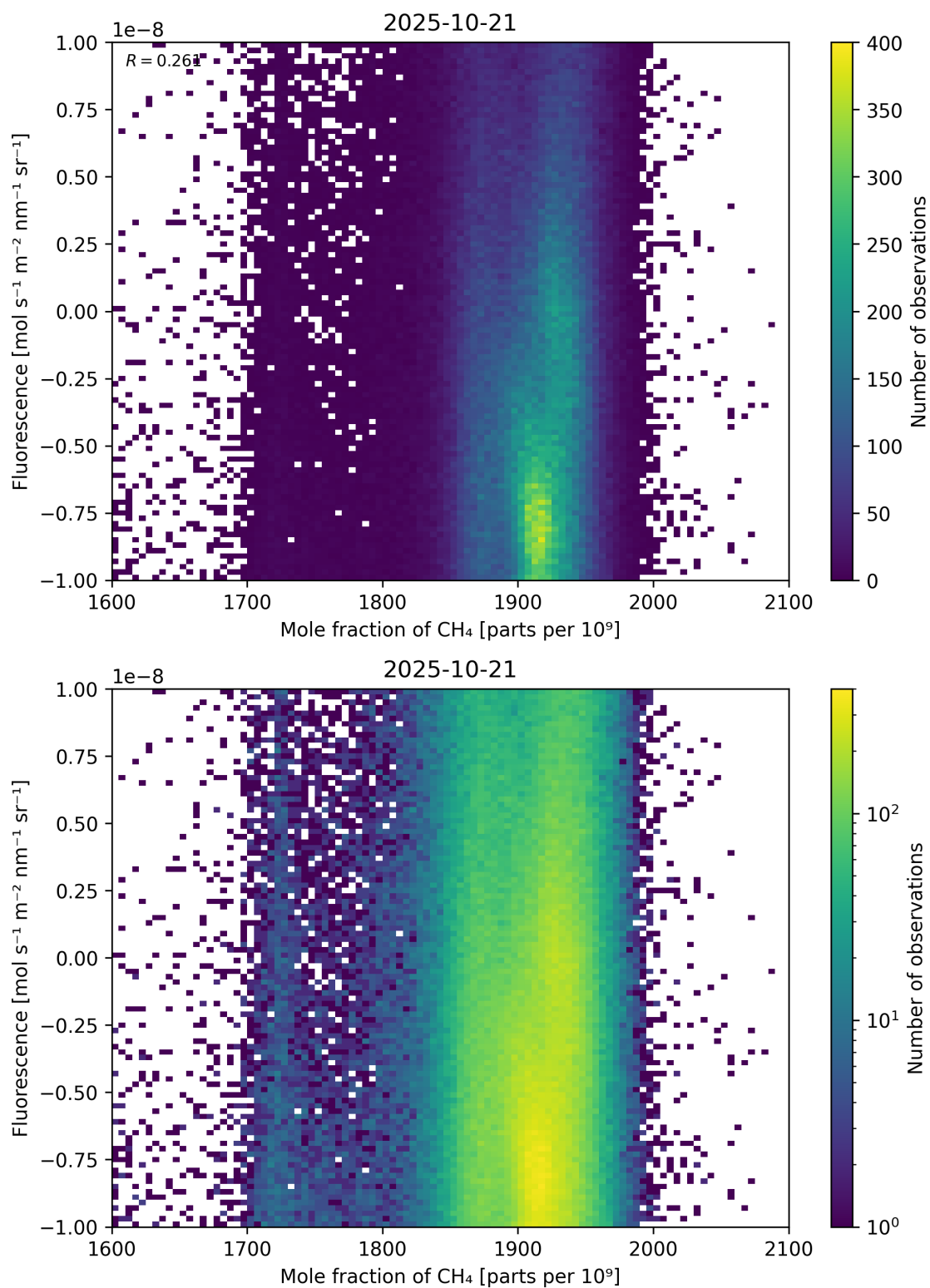
Figure 73: Scatter density plot of “Mole fraction of CH 4 ” against “Fluorescence” for 2025-10-20 to 2025-10-22.
