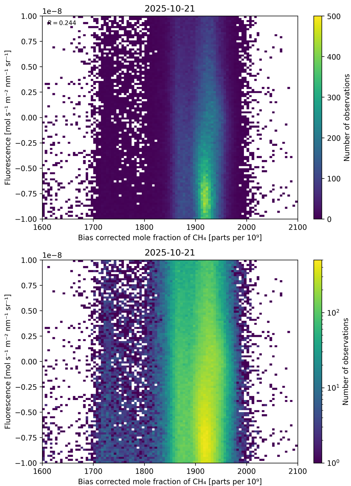
Figure 66: Scatter density plot of “Bias corrected mole fraction of \text{CH}_4 ” against “Fluorescence” for 2025-10-20 to 2025-10-22.
