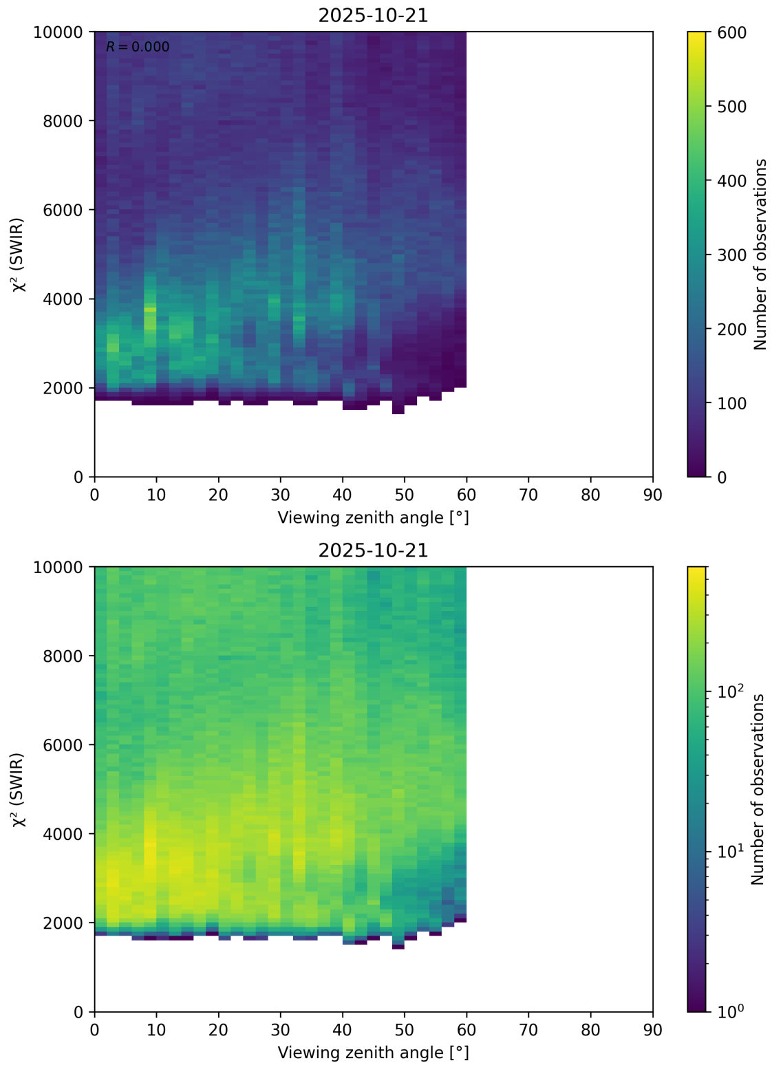
Figure 106: Scatter density plot of “Viewing zenith angle” against “ \chi^2 (SWIR)” for 2025-10-20 to 2025-10-22.
