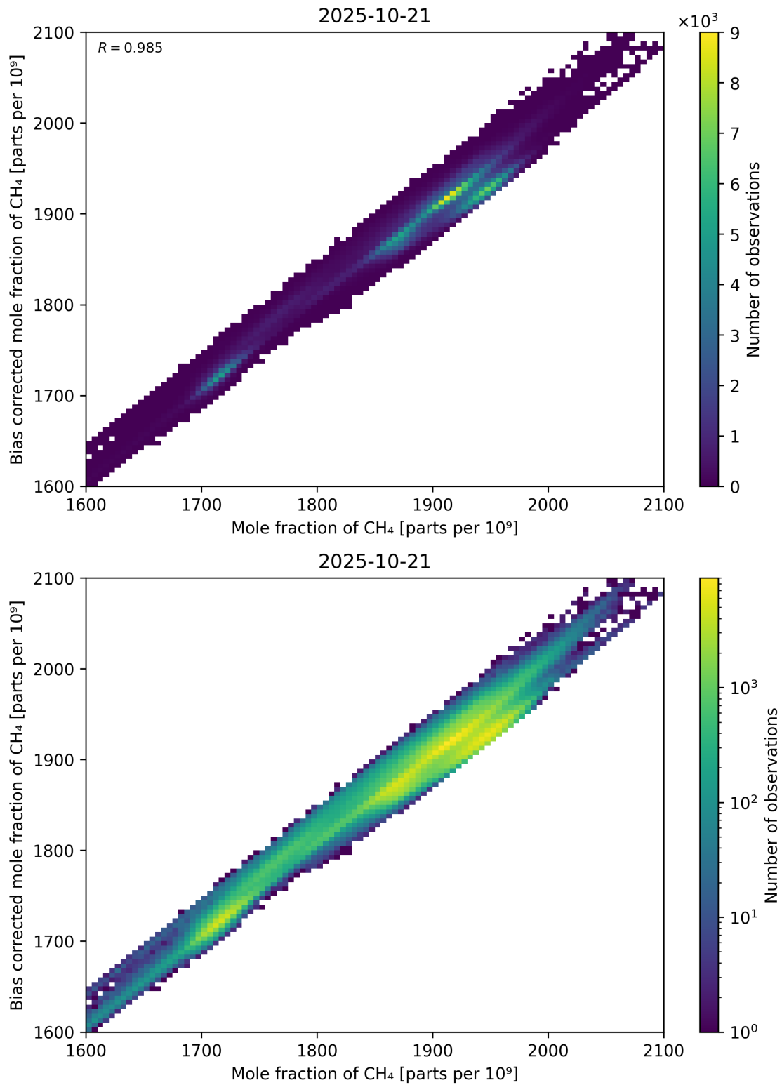
Figure 74: Scatter density plot of “Mole fraction of CH 4 ” against “Bias corrected mole fraction of CH 4 ” for 2025-10-20 to 2025-10-22.
