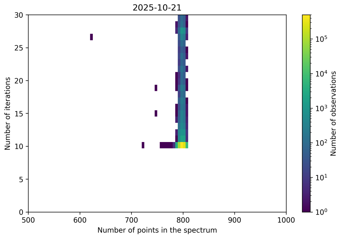
Figure 92: Scatter density plot of “Number of points in the spectrum” against “Number of iterations” for 2025-10-20 to 2025-10-22.
