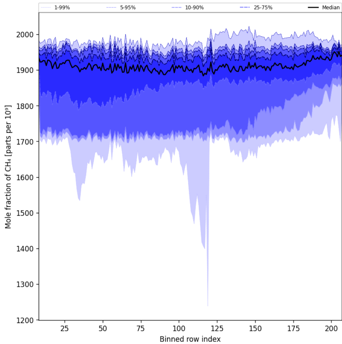
Figure 34: Along track statistics of “Mole fraction of CH 4 ” for 2025-10-20 to 2025-10-22
