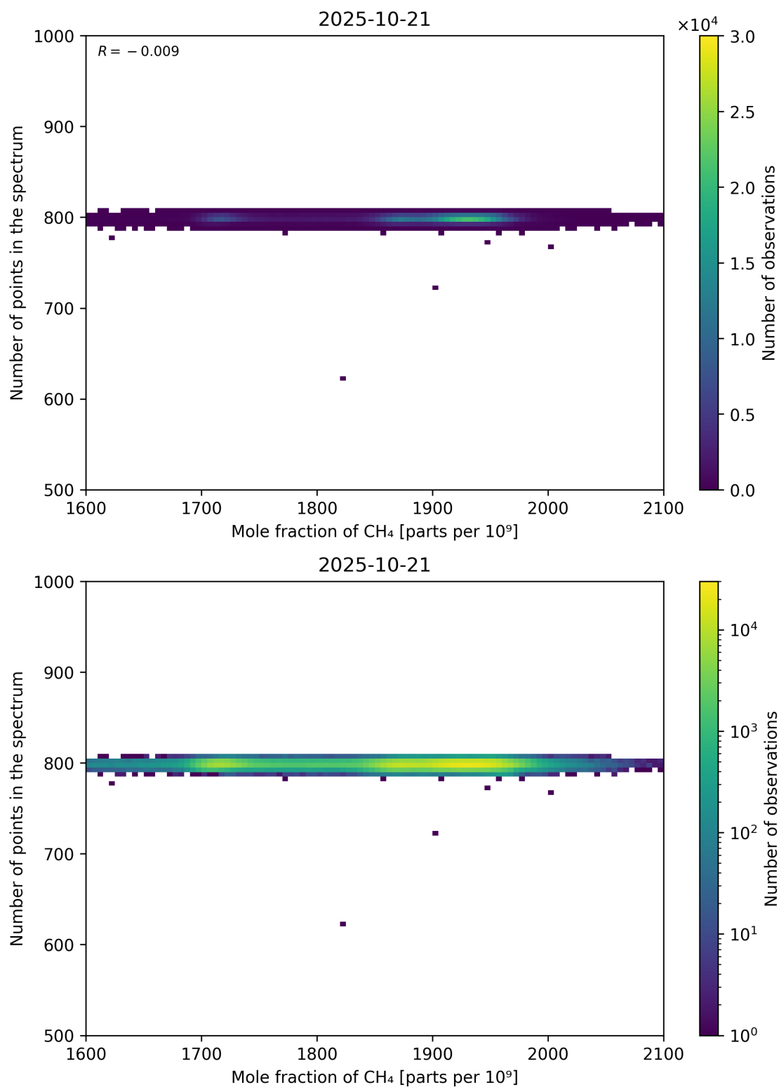
Figure 77: Scatter density plot of “Mole fraction of CH 4 ” against “Number of points in the spectrum” for 2025-10-20 to 2025-10-22.
