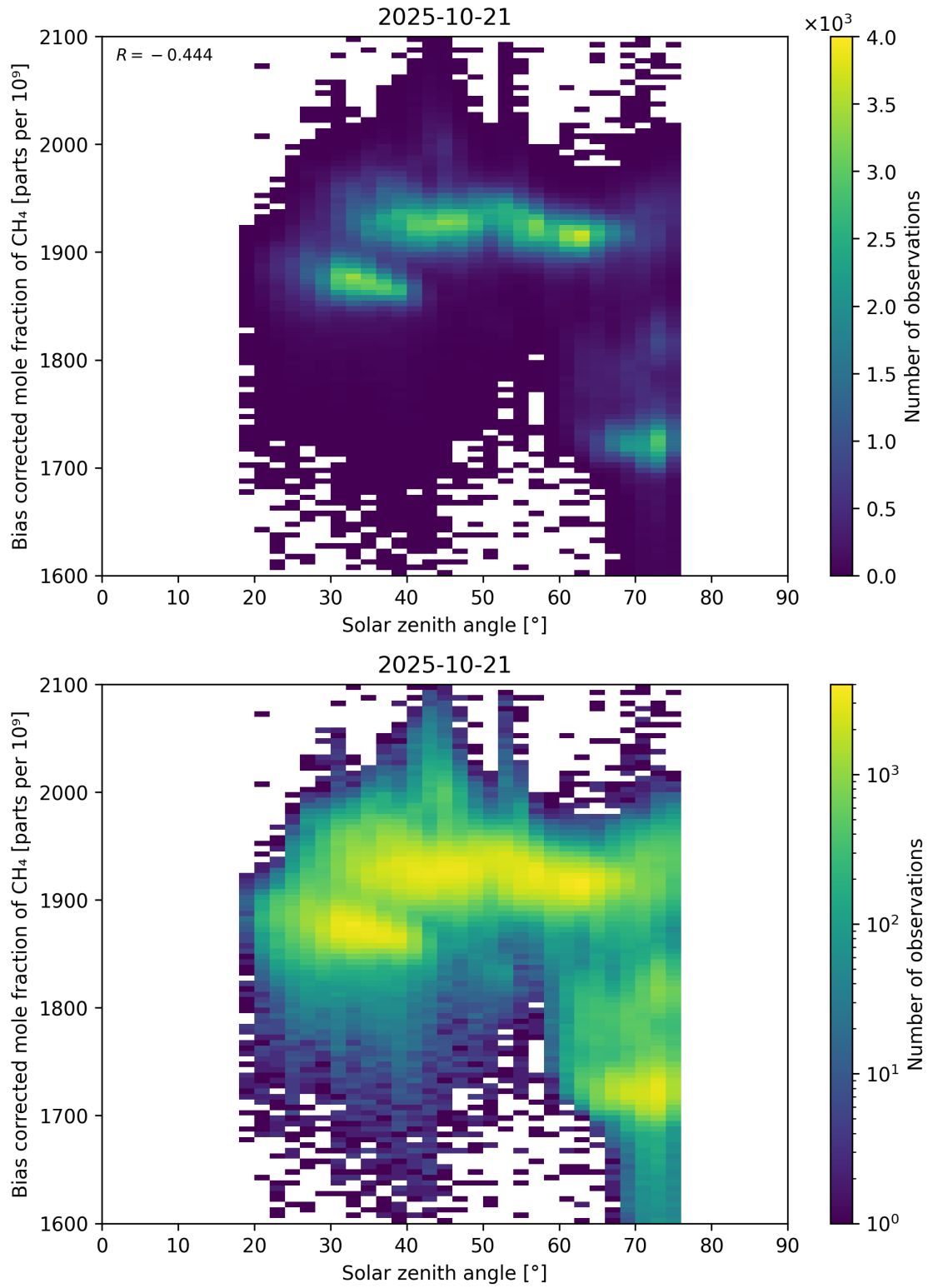
Figure 100: Scatter density plot of “Solar zenith angle” against “Bias corrected mole fraction of \text{CH}_4 ” for 2025-10-20 to 2025-10-22.
