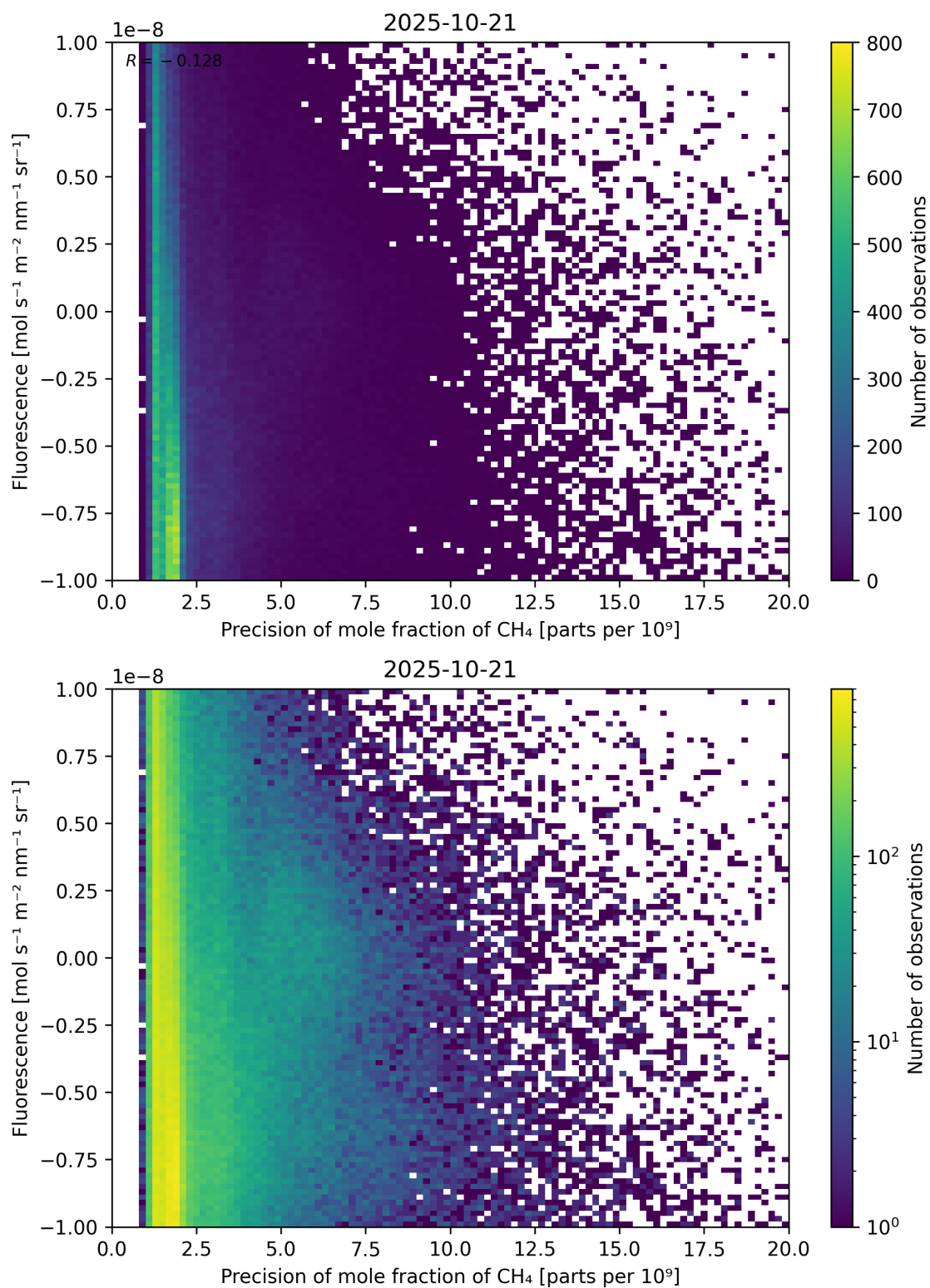
Figure 81: Scatter density plot of “Precision of mole fraction of \text{CH}_4 ” against “Fluorescence” for 2025-10-20 to 2025-10-22.
