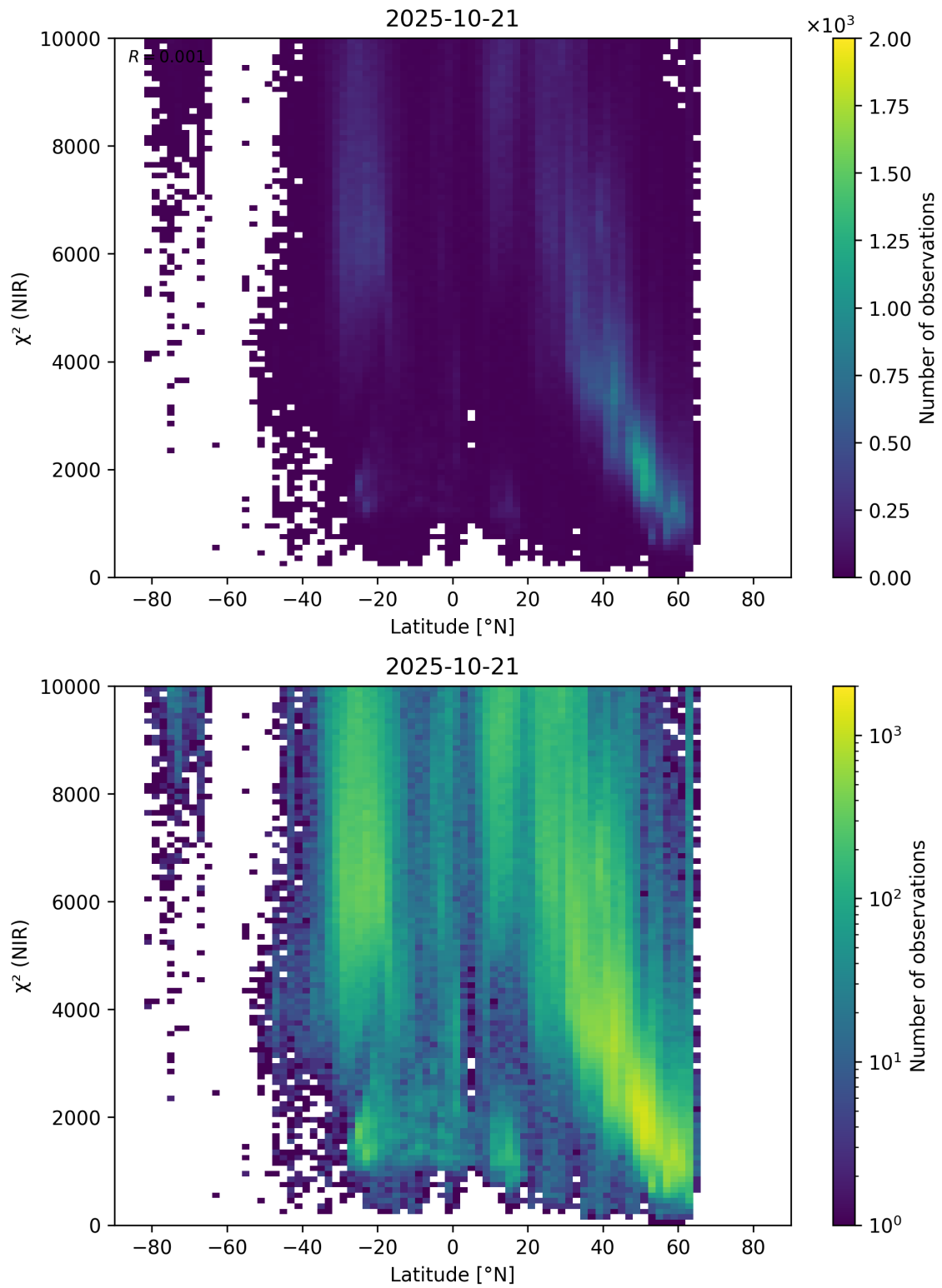
Figure 53: Scatter density plot of “Latitude” against “ \chi^2 (NIR)” for 2025-10-20 to 2025-10-22.
