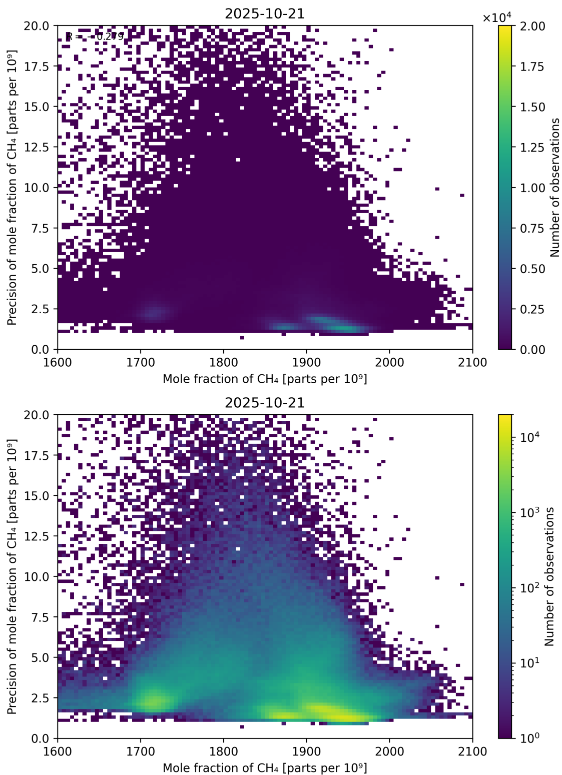
Figure 75: Scatter density plot of “Mole fraction of CH 4 ” against “Precision of mole fraction of CH 4 ” for 2025-10-20 to 2025-10-22.
