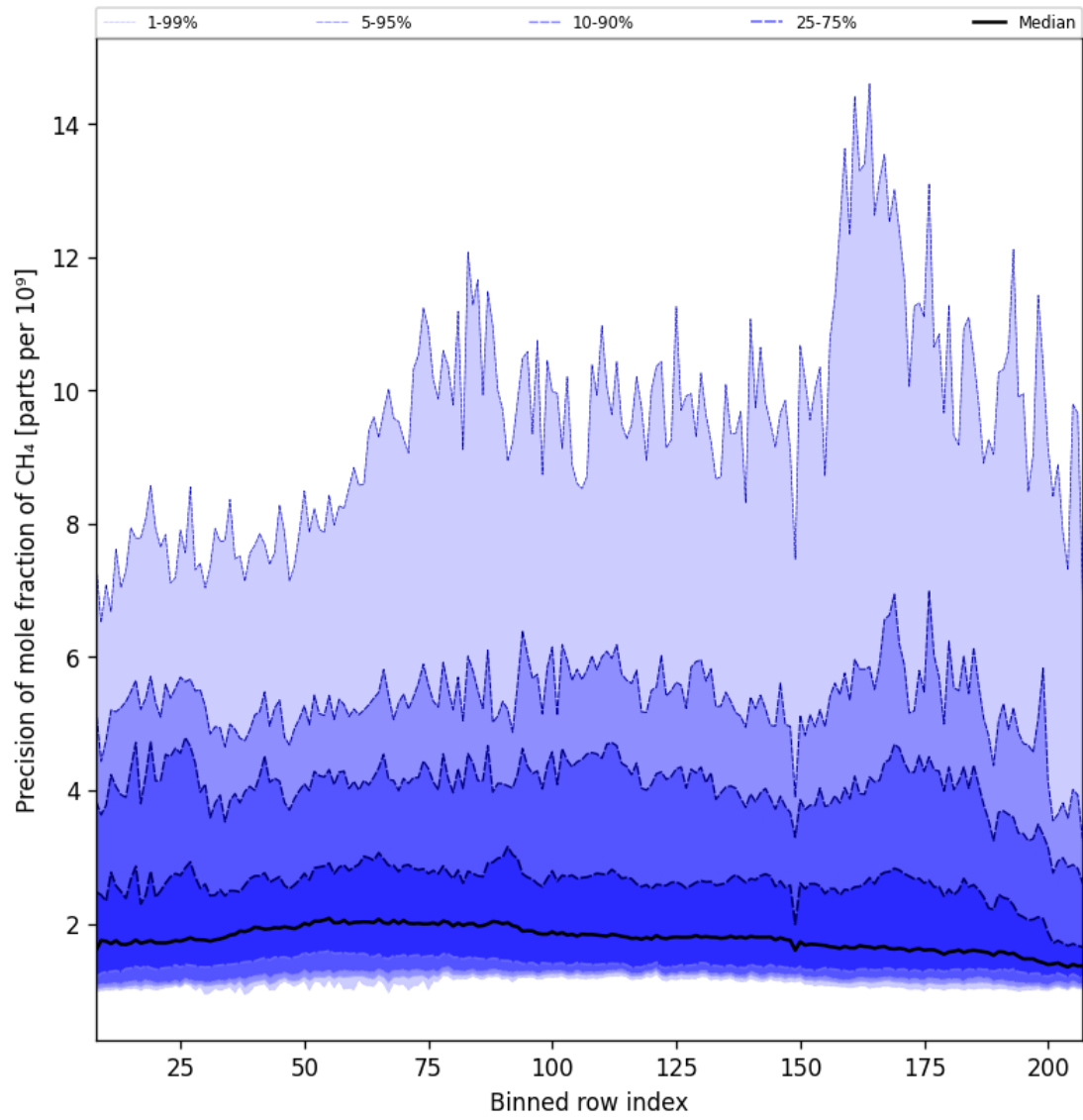
Figure 35: Along track statistics of “Precision of mole fraction of CH 4 ” for 2025-10-20 to 2025-10-22
