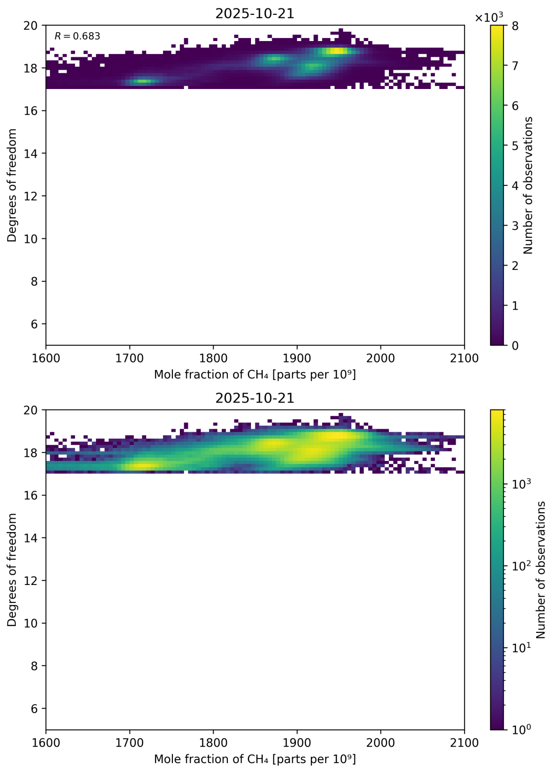
Figure 72: Scatter density plot of “Mole fraction of CH 4 ” against “Degrees of freedom” for 2025-10-20 to 2025-10-22.
