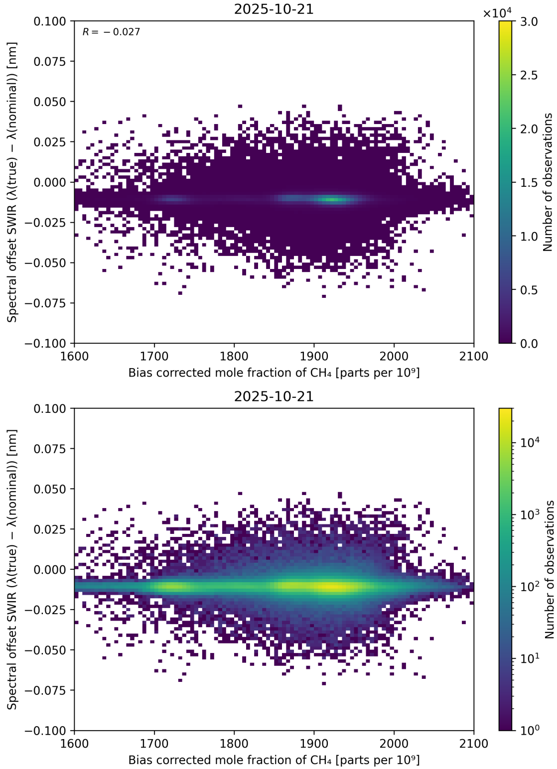
Figure 69: Scatter density plot of “Bias corrected mole fraction of \text{CH}_4 ” against “Spectral offset SWIR ( \lambda_{\text{true}} - \lambda_{\text{nominal}} )” for 2025-10-20 to 2025-10-22.
