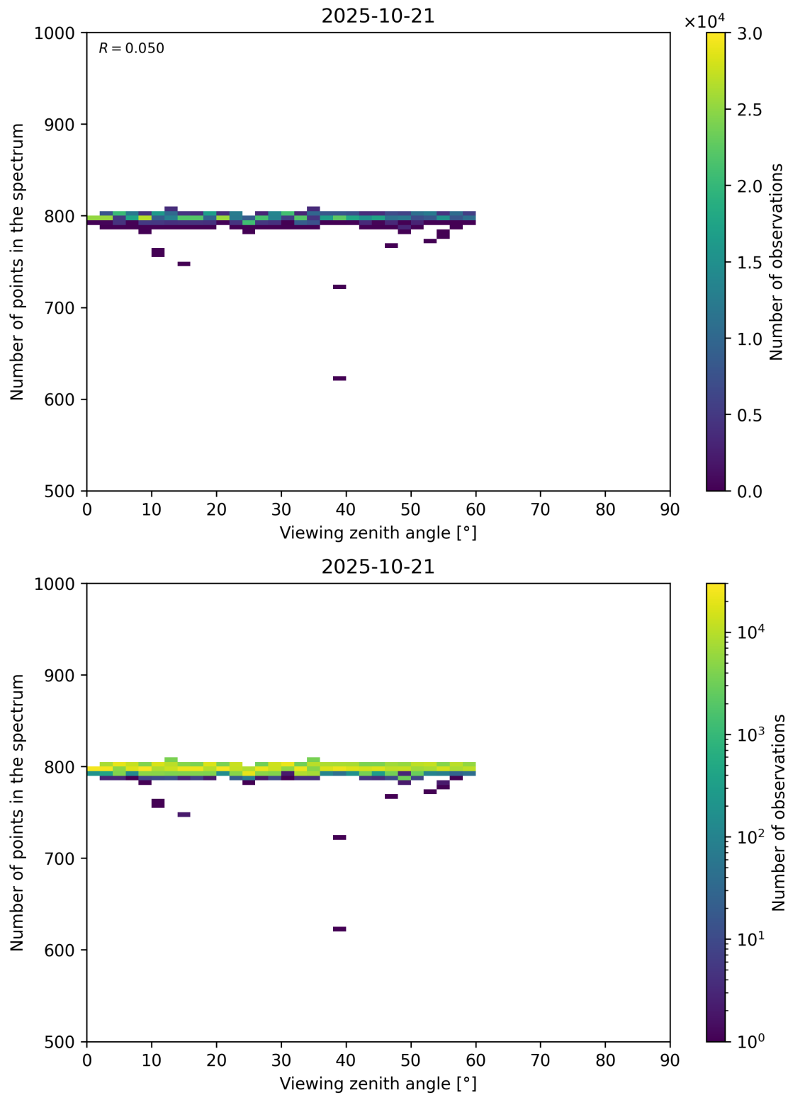
Figure 114: Scatter density plot of “Viewing zenith angle” against “Number of points in the spectrum” for 2025-10-20 to 2025-10-22.
