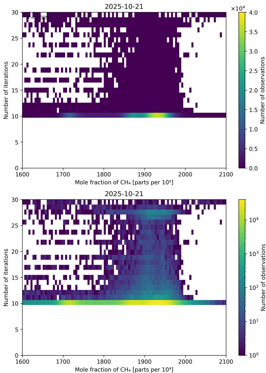
Figure 76: Scatter density plot of “Mole fraction of CH 4 ” against “Number of iterations” for 2025-10-20 to 2025-10-22.
