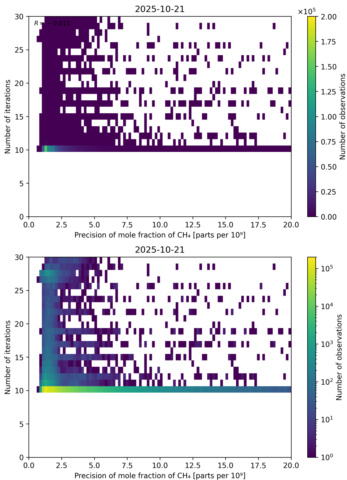
Figure 83: Scatter density plot of “Precision of mole fraction of CH 4 ” against “Number of iterations” for 2025-10-20 to 2025-10-22.
