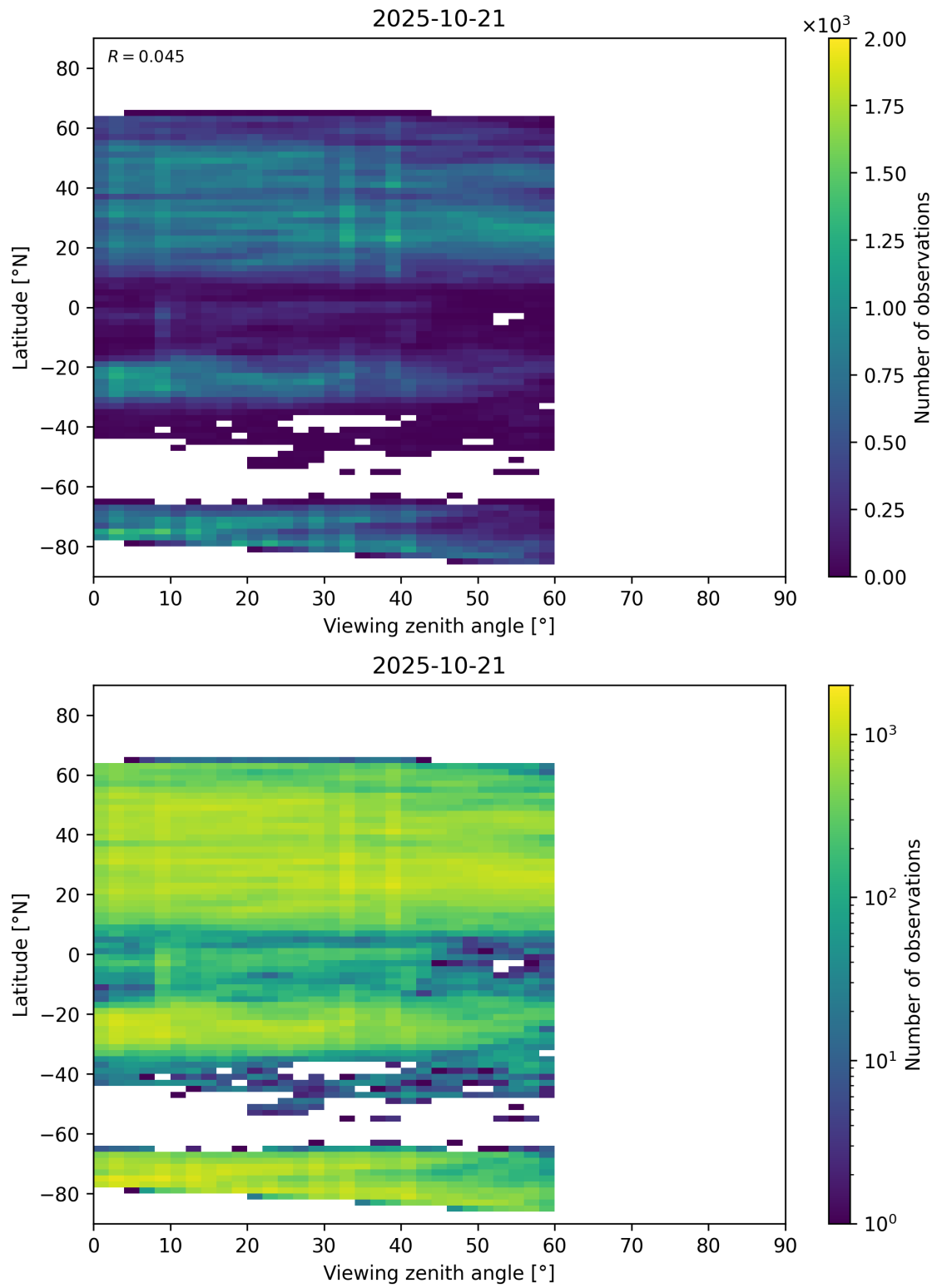
Figure 109: Scatter density plot of “Viewing zenith angle” against “Latitude” for 2025-10-20 to 2025-10-22.
