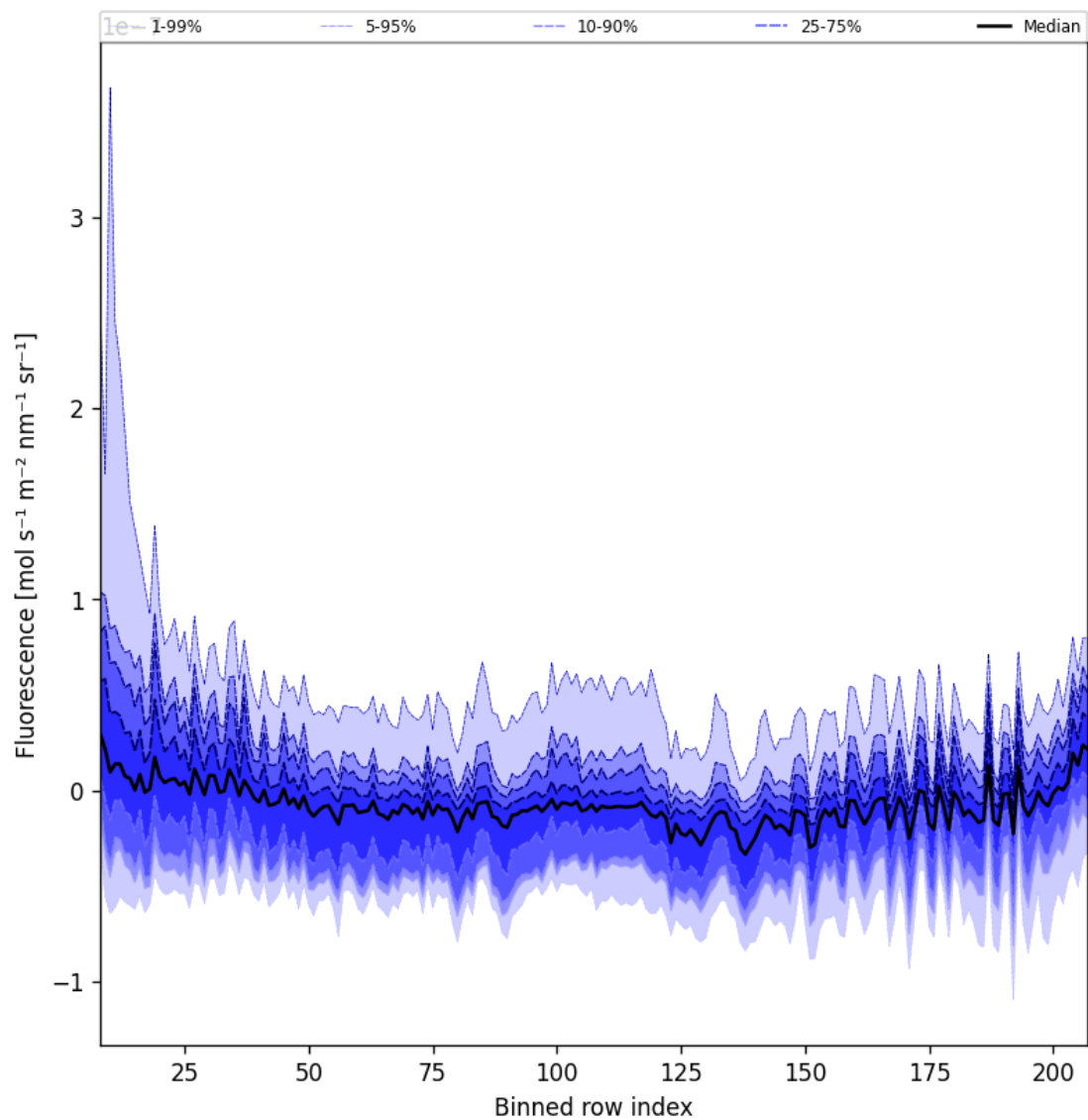
Figure 43: Along track statistics of “Fluorescence” for 2025-10-20 to 2025-10-22
