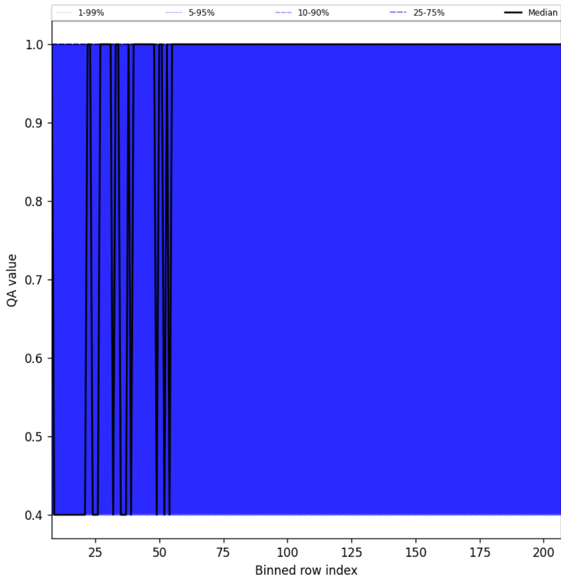
Figure 33: Along track statistics of “QA value” for 2025-10-20 to 2025-10-22
