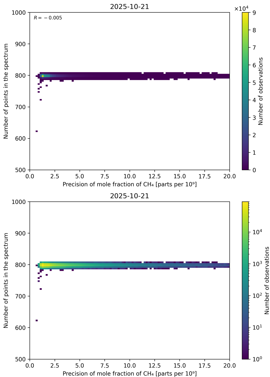
Figure 84: Scatter density plot of “Precision of mole fraction of CH 4 ” against “Number of points in the spectrum” for 2025-10-20 to 2025-10-22.
