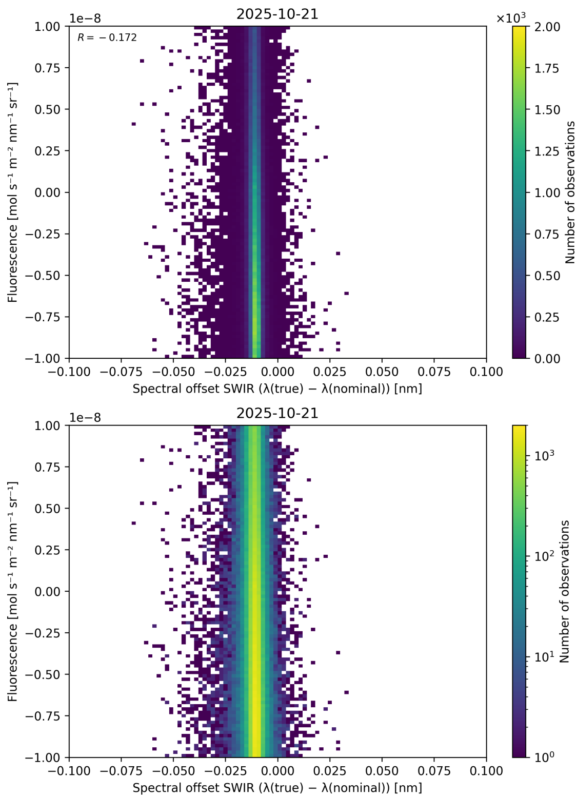
Figure 120: Scatter density plot of “Spectral offset SWIR ( \lambda_{\text{true}} - \lambda_{\text{nominal}} )” against “Fluorescence” for 2025-10-20 to 2025-10-22.
