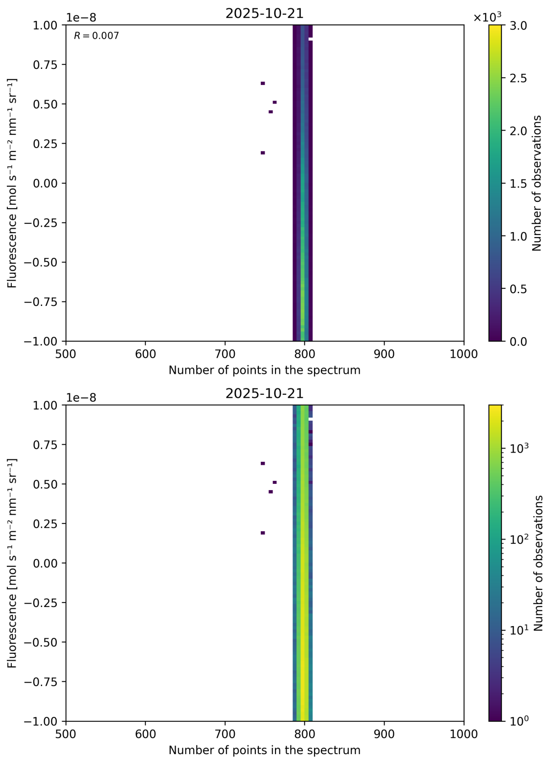
Figure 91: Scatter density plot of “Number of points in the spectrum” against “Fluorescence” for 2025-10-20 to 2025-10-22.
