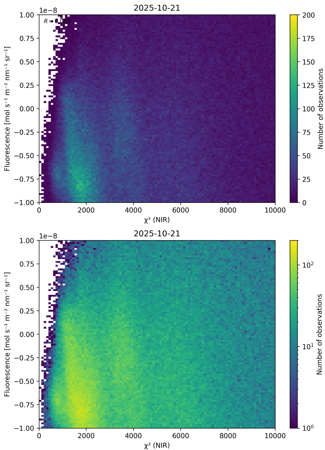
Figure 45: Scatter density plot of “ \chi^2 (NIR)” against “Fluorescence” for 2025-10-20 to 2025-10-22.
