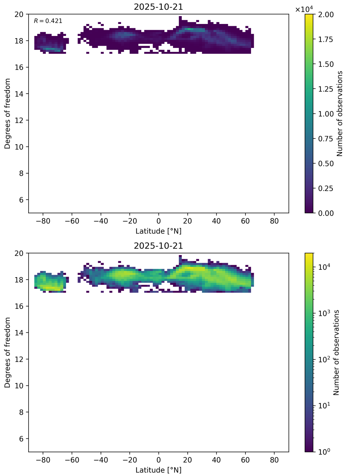
Figure 55: Scatter density plot of “Latitude” against “Degrees of freedom” for 2025-10-20 to 2025-10-22.
