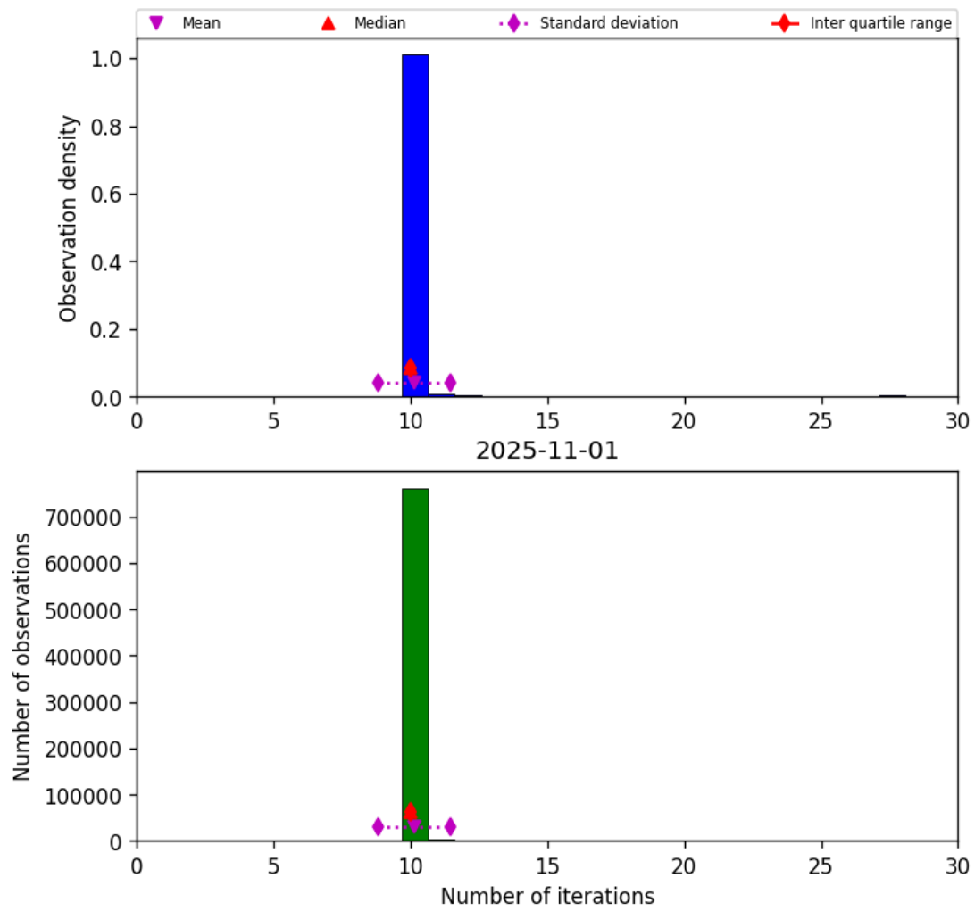
Figure 31: Histogram of “Number of iterations” for 2025-10-31 to 2025-11-02
