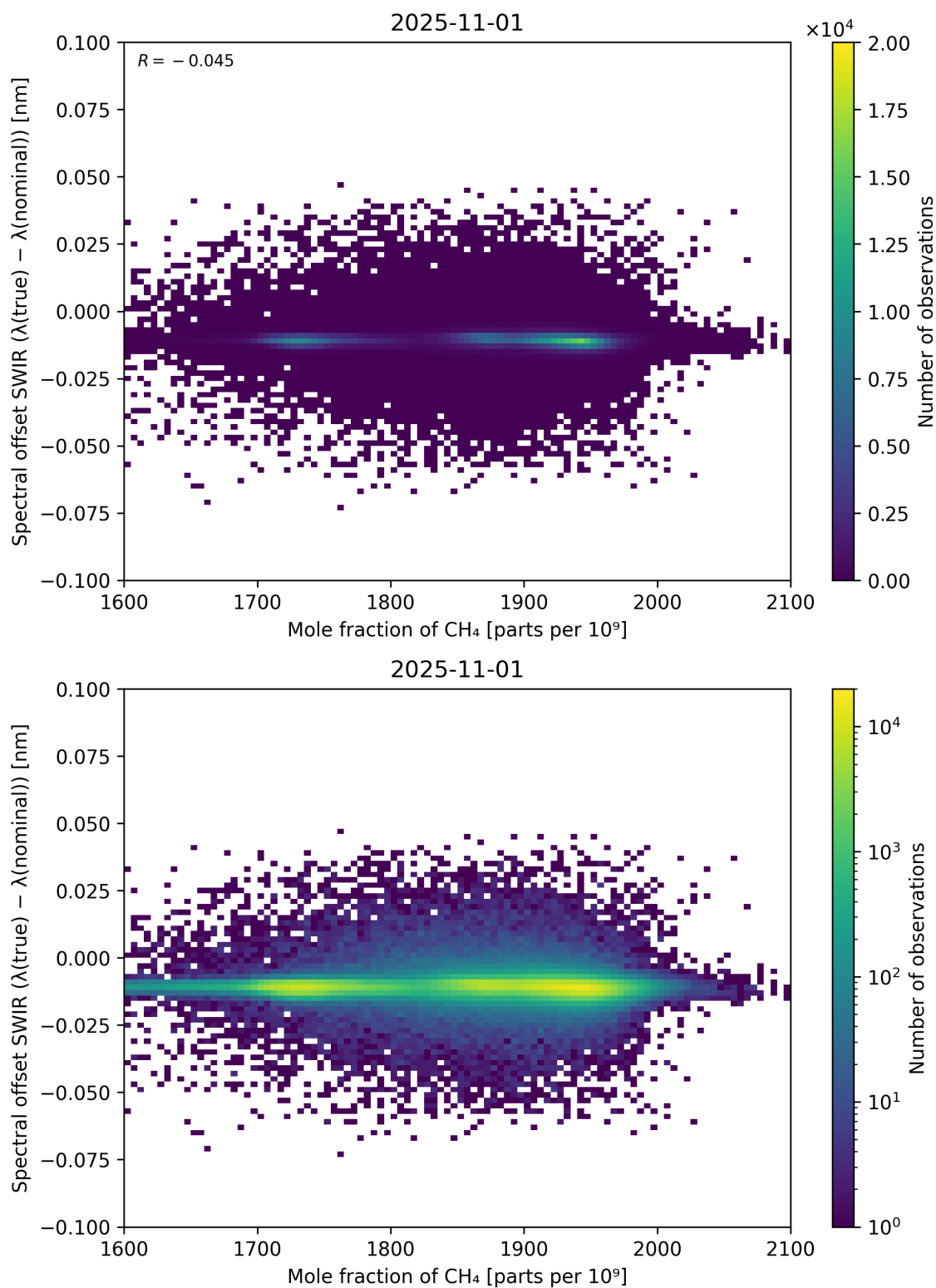
Figure 86: Scatter density plot of “Mole fraction of CH 4 ” against “Spectral offset SWIR ( \lambda_{\text{true}} - \lambda_{\text{nominal}} )” for 2025-10-31 to 2025-11-02.
