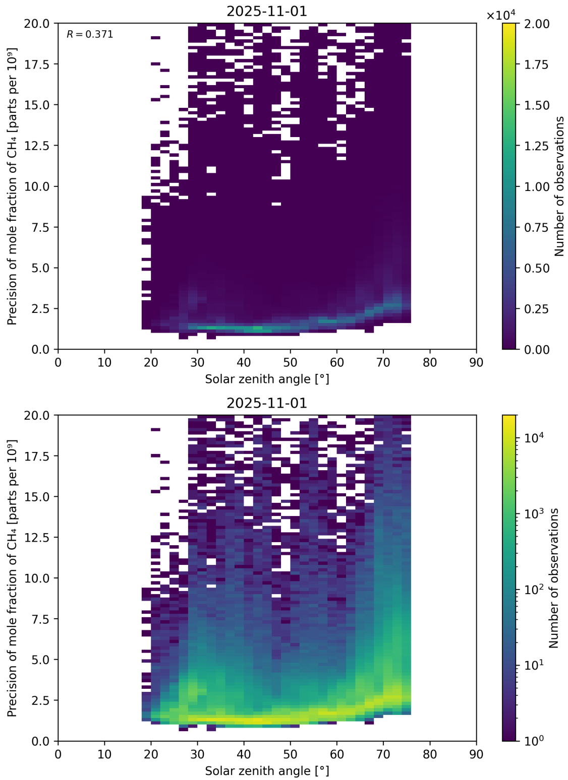
Figure 101: Scatter density plot of “Solar zenith angle” against “Precision of mole fraction of \text{CH}_4 ” for 2025-10-31 to 2025-11-02.
