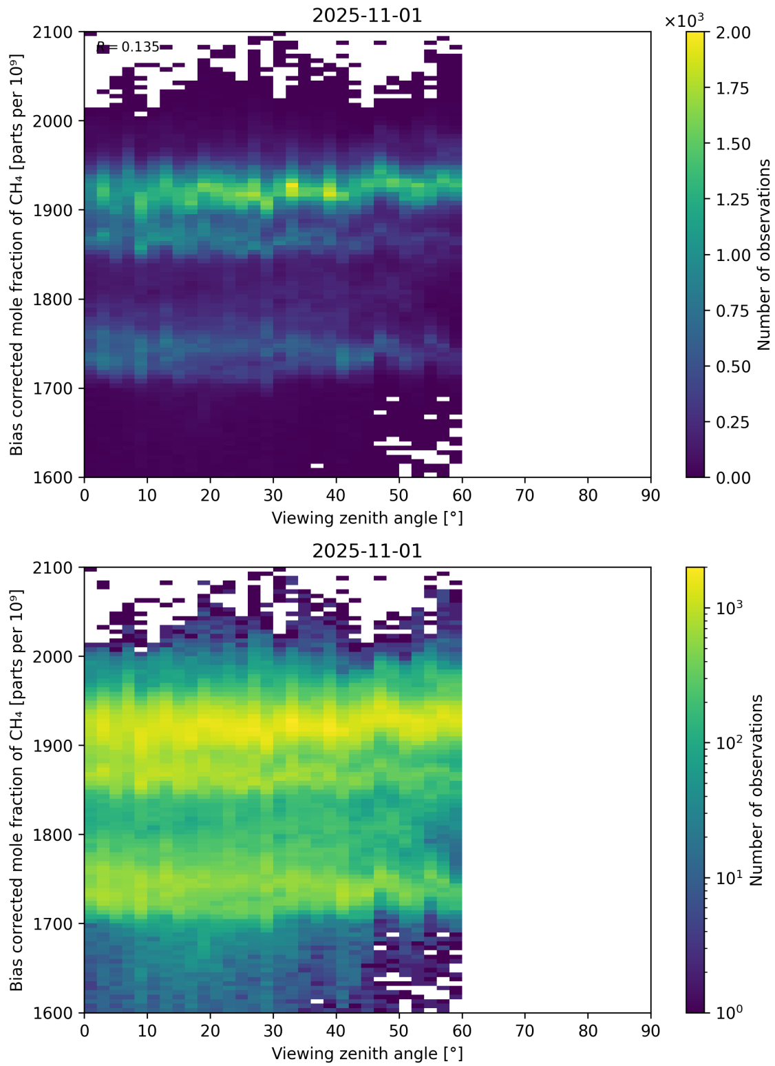
Figure 111: Scatter density plot of “Viewing zenith angle” against “Bias corrected mole fraction of CH 4 ” for 2025-10-31 to 2025-11-02.
