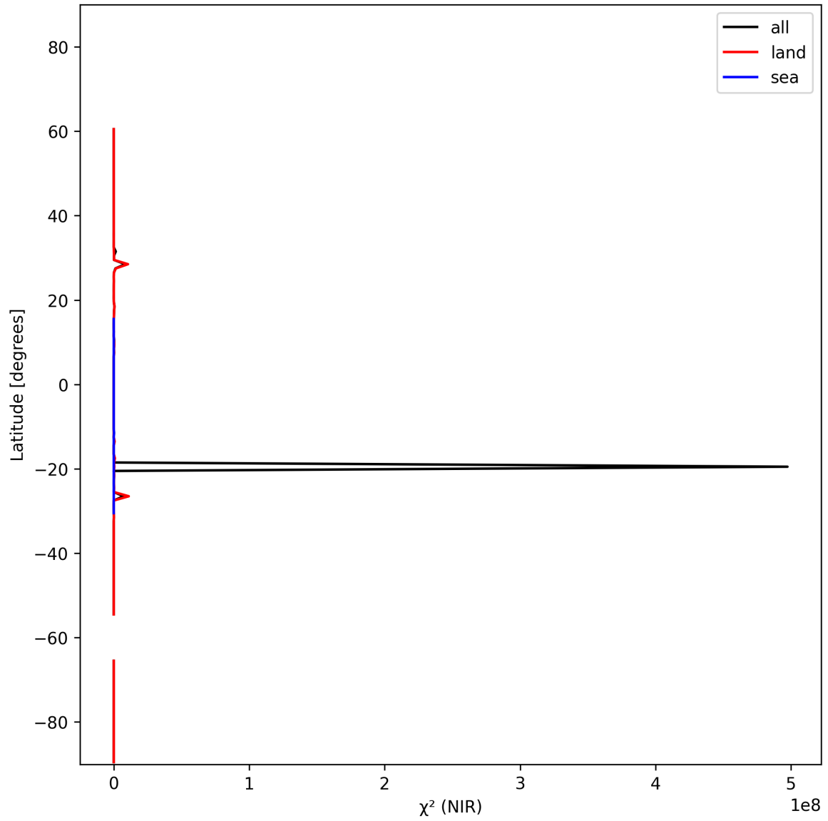
Figure 18: Zonal average of “ \chi^2 (NIR)” for 2025-10-31 to 2025-11-02.
