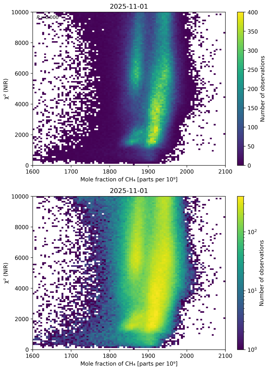
Figure 70: Scatter density plot of “Mole fraction of \text{CH}_4 ” against “ \chi^2 (NIR)” for 2025-10-31 to 2025-11-02.
