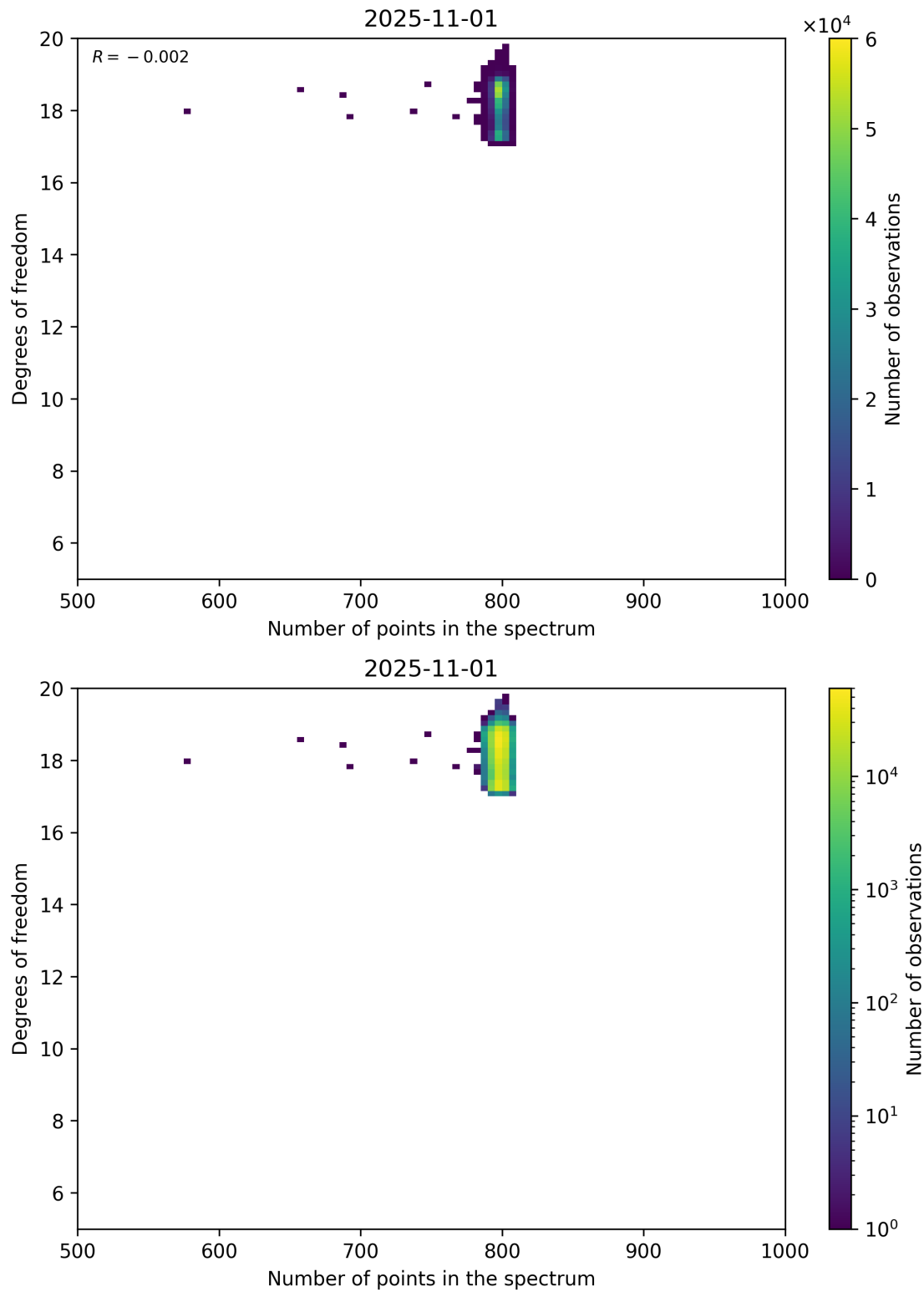
Figure 90: Scatter density plot of “Number of points in the spectrum” against “Degrees of freedom” for 2025-10-31 to 2025-11-02.
