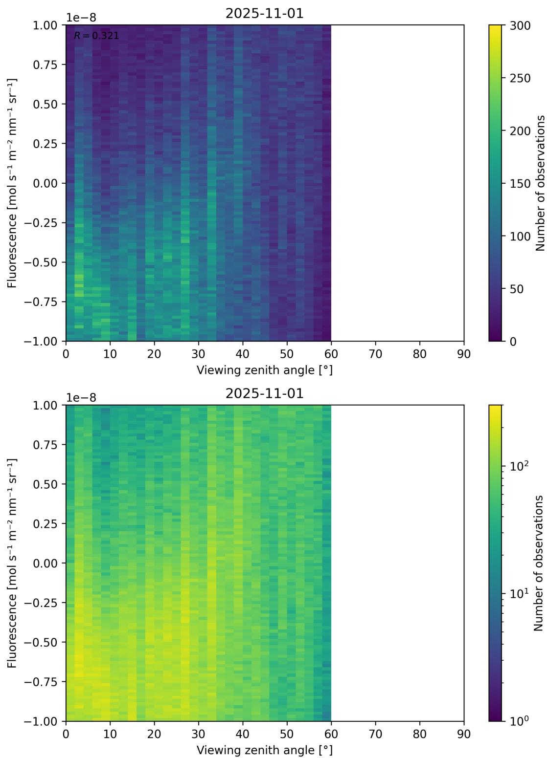
Figure 108: Scatter density plot of “Viewing zenith angle” against “Fluorescence” for 2025-10-31 to 2025-11-02.
