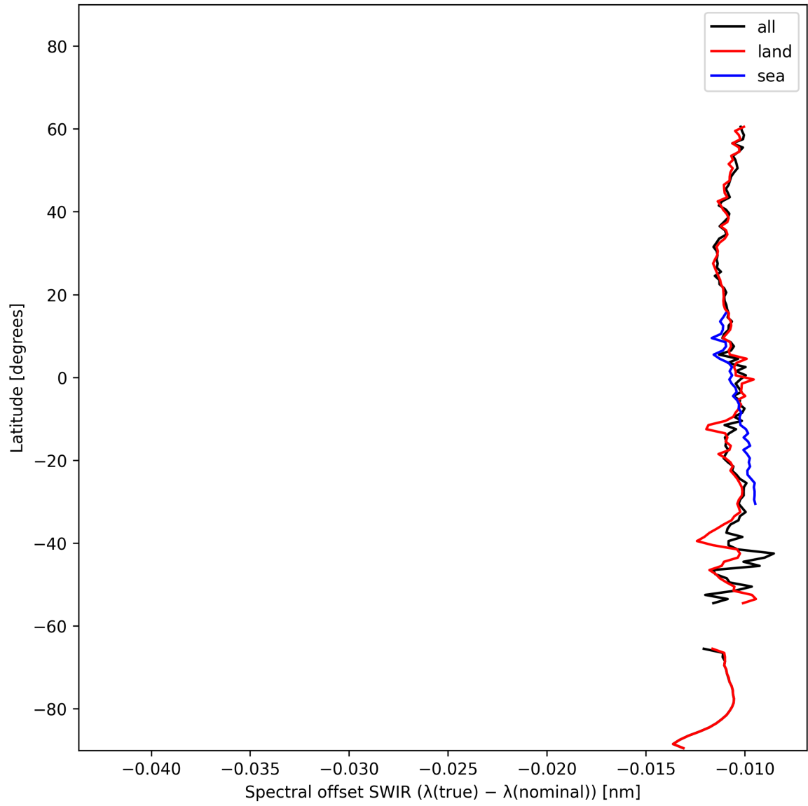
Figure 16: Zonal average of “Spectral offset SWIR ( \lambda_{\text{true}} - \lambda_{\text{nominal}} )” for 2025-10-31 to 2025-11-02.
