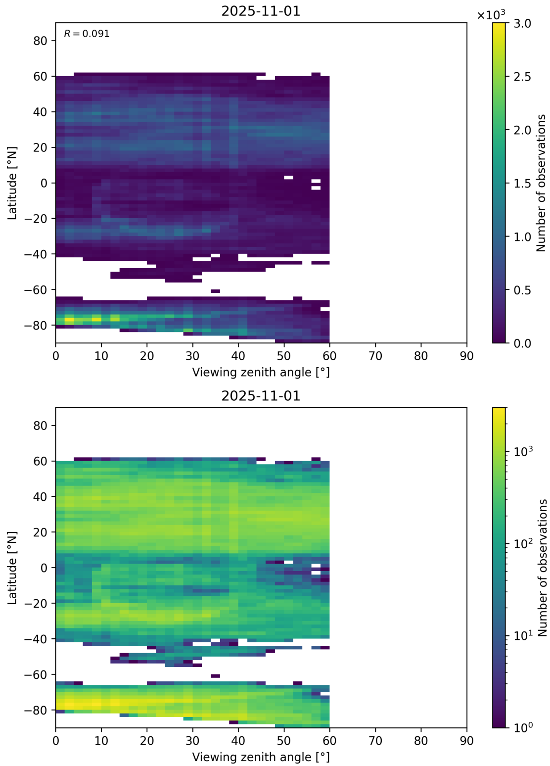
Figure 109: Scatter density plot of “Viewing zenith angle” against “Latitude” for 2025-10-31 to 2025-11-02.
