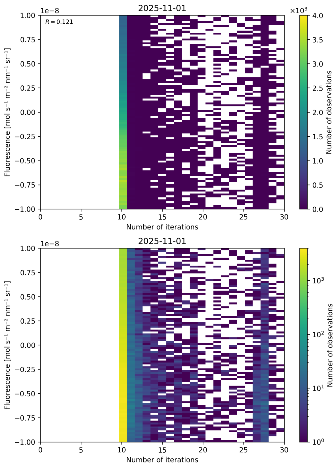
Figure 87: Scatter density plot of "Number of iterations" against "Fluorescence" for 2025-10-31 to 2025-11-02.
