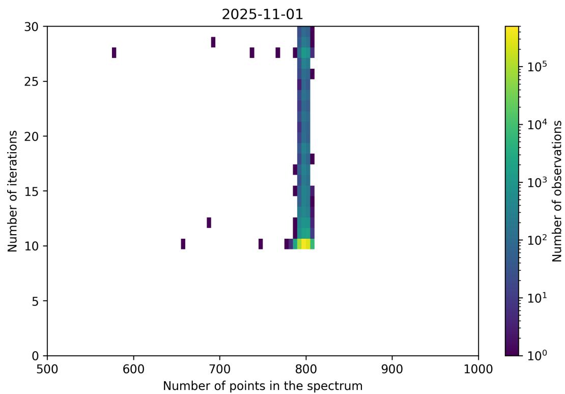
Figure 92: Scatter density plot of “Number of points in the spectrum” against “Number of iterations” for 2025-10-31 to 2025-11-02.
