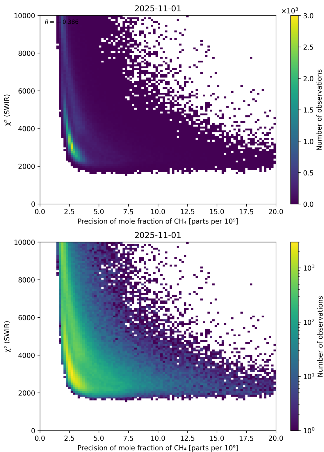
Figure 79: Scatter density plot of “Precision of mole fraction of \text{CH}_4 ” against “ \chi^2 (SWIR)” for 2025-10-31 to 2025-11-02.
