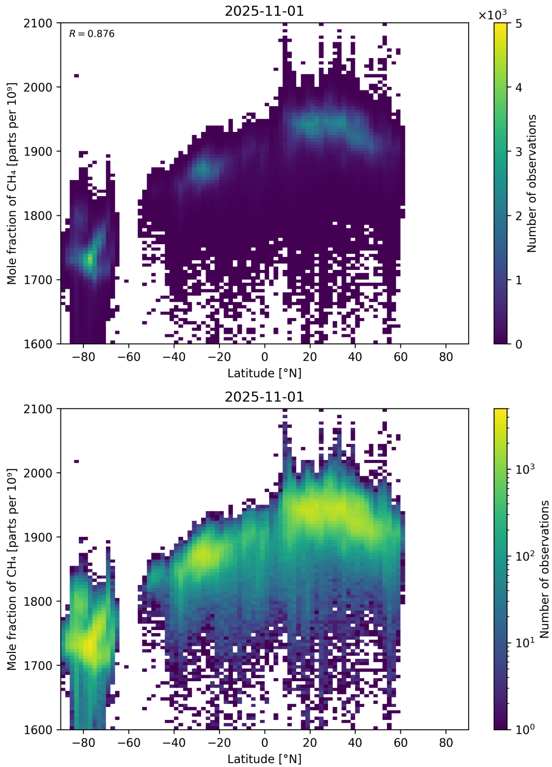
Figure 57: Scatter density plot of “Latitude” against “Mole fraction of CH 4 ” for 2025-10-31 to 2025-11-02.
