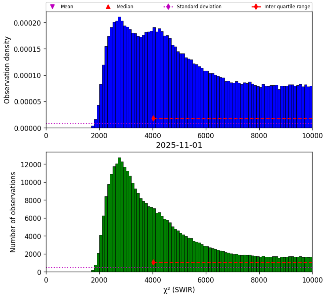
Figure 28: Histogram of “ \chi^2 (SWIR)” for 2025-10-31 to 2025-11-02
