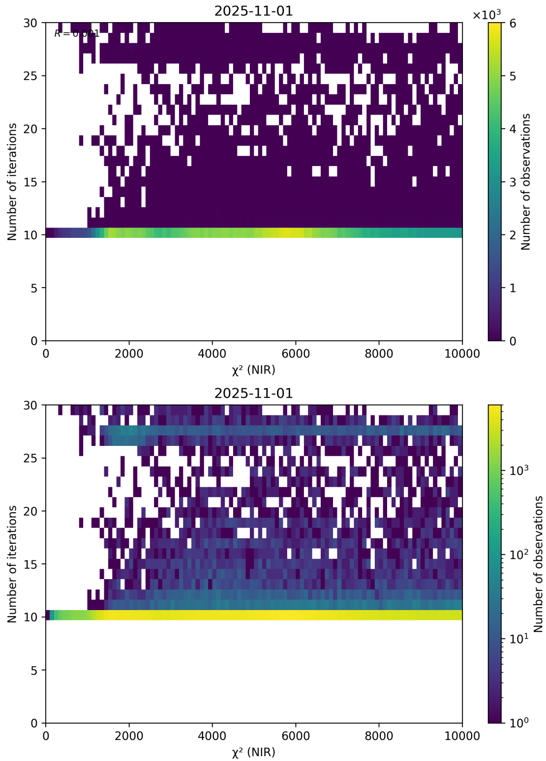
Figure 46: Scatter density plot of “ \chi^2 (NIR)” against “Number of iterations” for 2025-10-31 to 2025-11-02.
