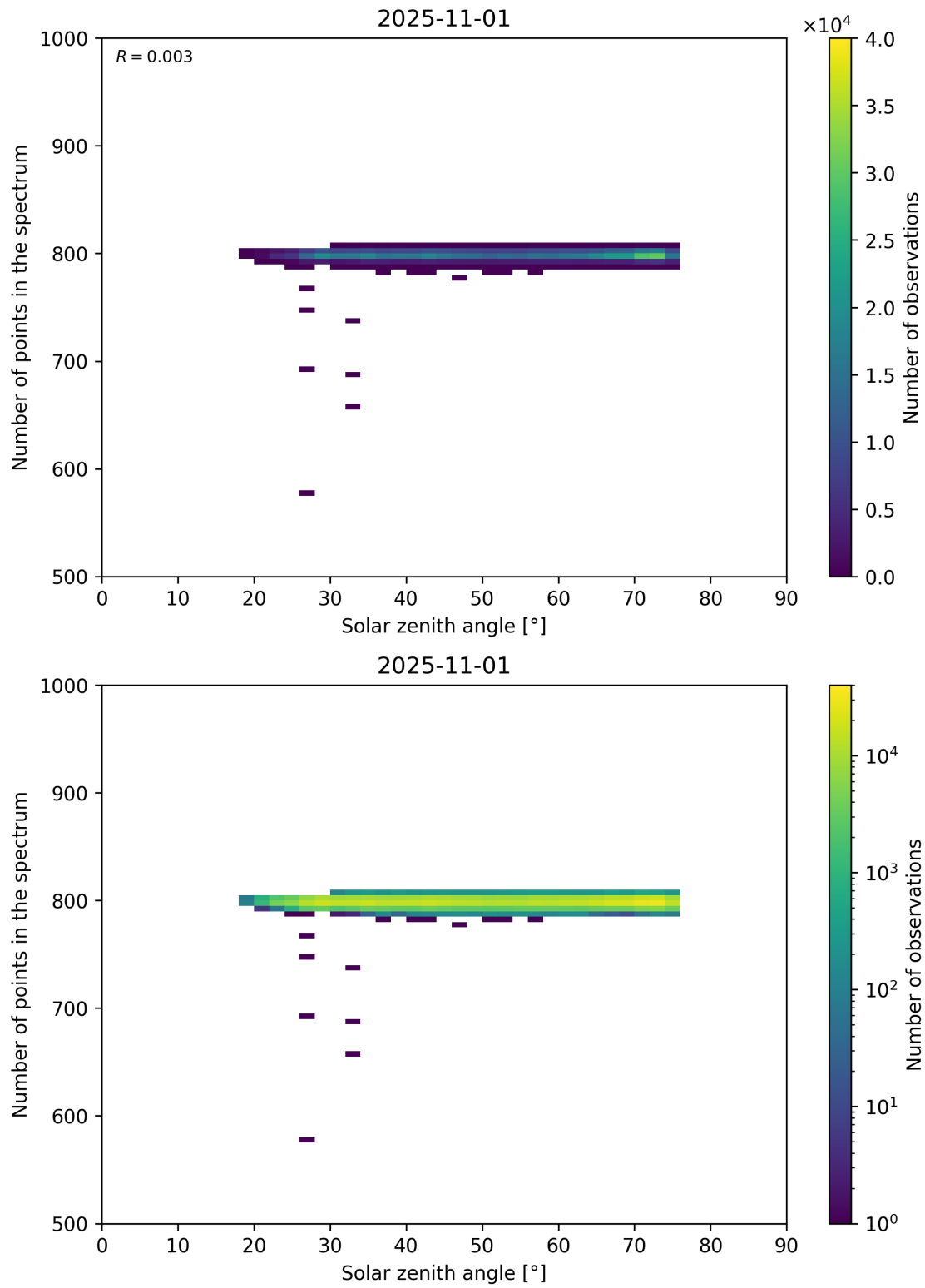
Figure 103: Scatter density plot of “Solar zenith angle” against “Number of points in the spectrum” for 2025-10-31 to 2025-11-02.
