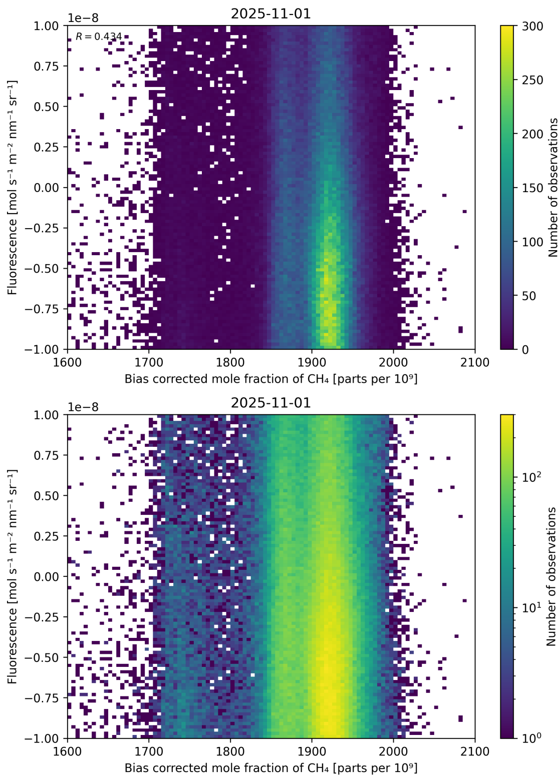
Figure 66: Scatter density plot of “Bias corrected mole fraction of CH 4 ” against “Fluorescence” for 2025-10-31 to 2025-11-02.
