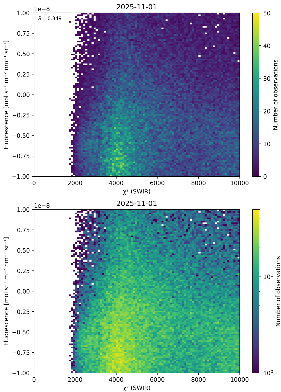
Figure 49: Scatter density plot of “ \chi^2 (SWIR)” against “Fluorescence” for 2025-10-31 to 2025-11-02.
