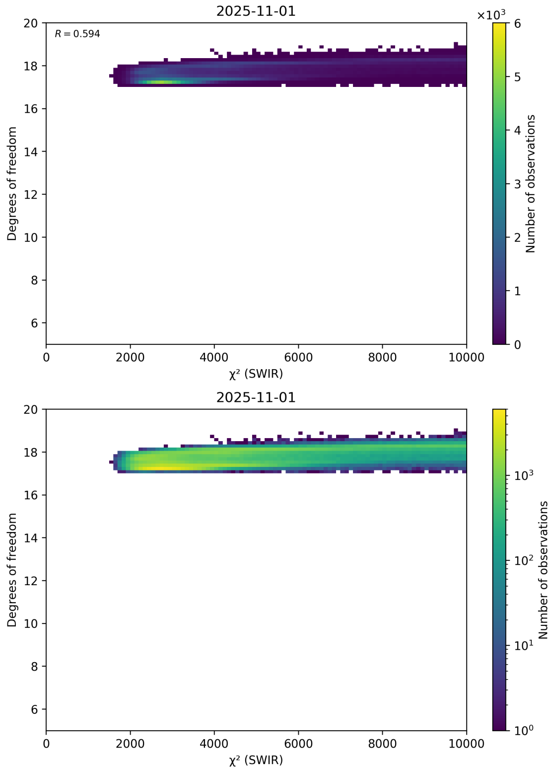
Figure 48: Scatter density plot of “ \chi^2 (SWIR)” against “Degrees of freedom” for 2025-10-31 to 2025-11-02.
