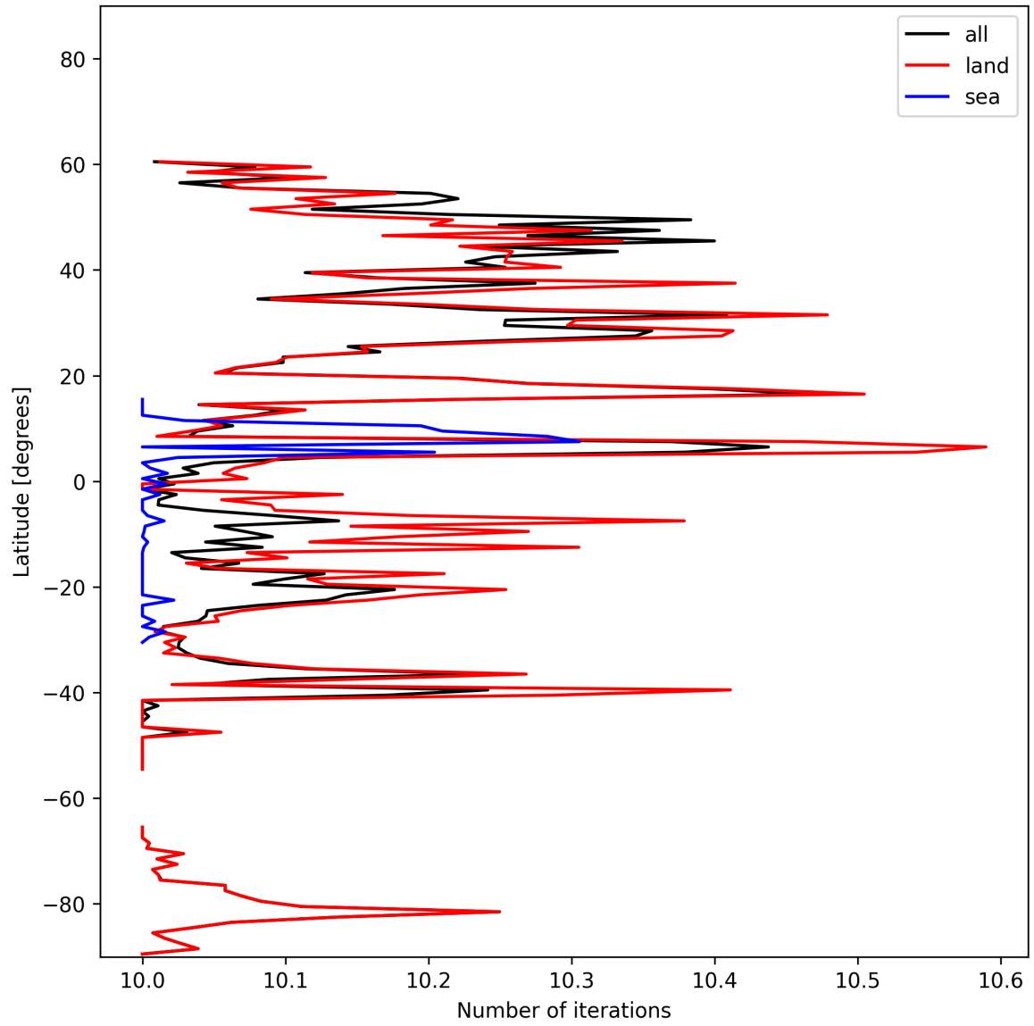
Figure 20: Zonal average of “Number of iterations” for 2025-10-31 to 2025-11-02.
