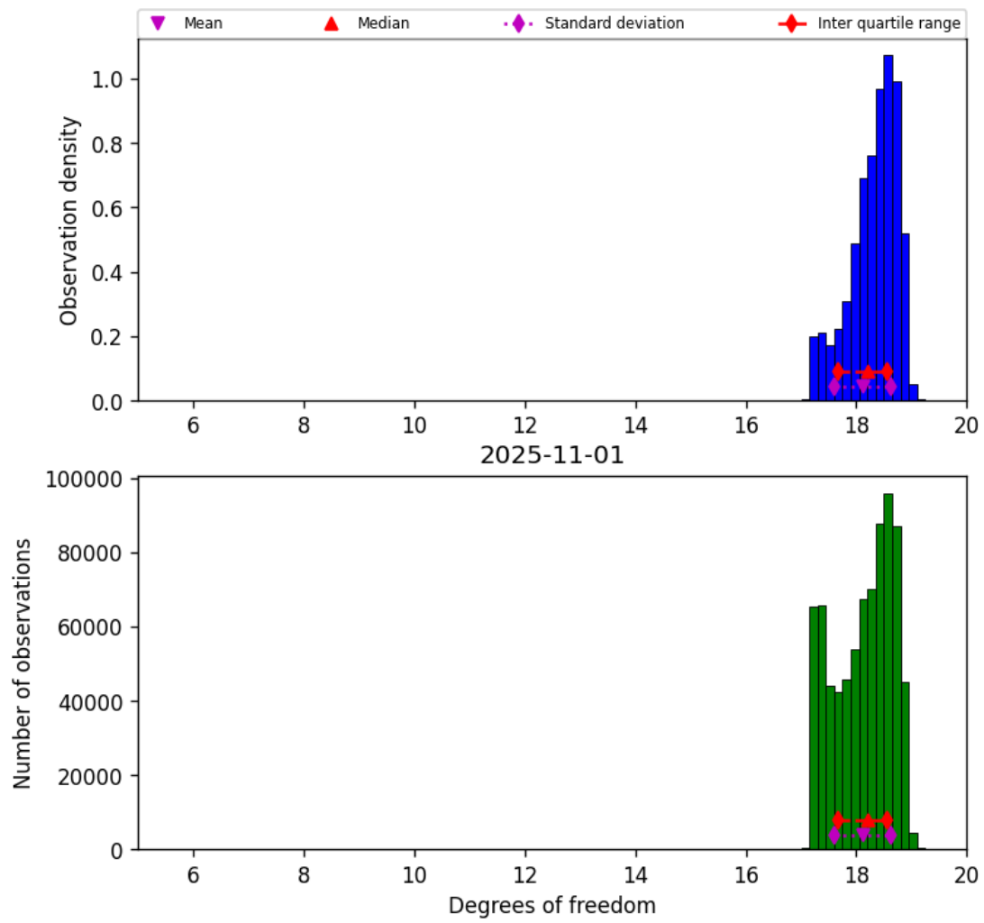
Figure 30: Histogram of “Degrees of freedom” for 2025-10-31 to 2025-11-02
