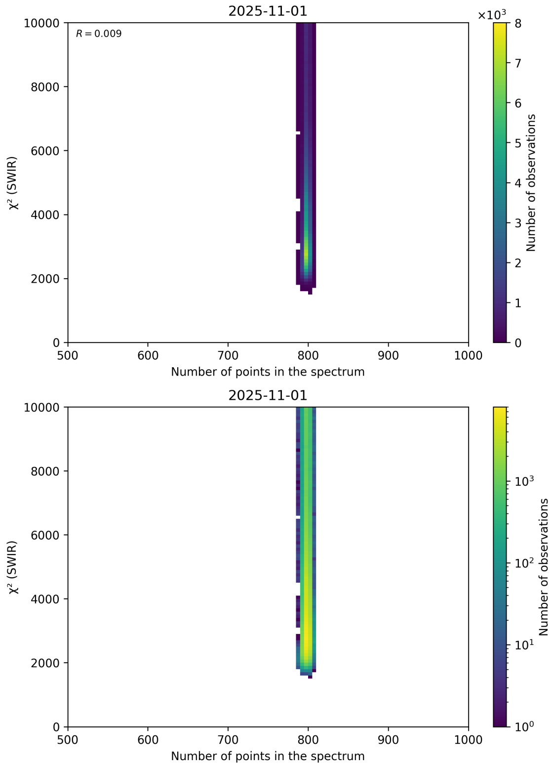
Figure 89: Scatter density plot of “Number of points in the spectrum” against “ \chi^2 (SWIR)” for 2025-10-31 to 2025-11-02.
