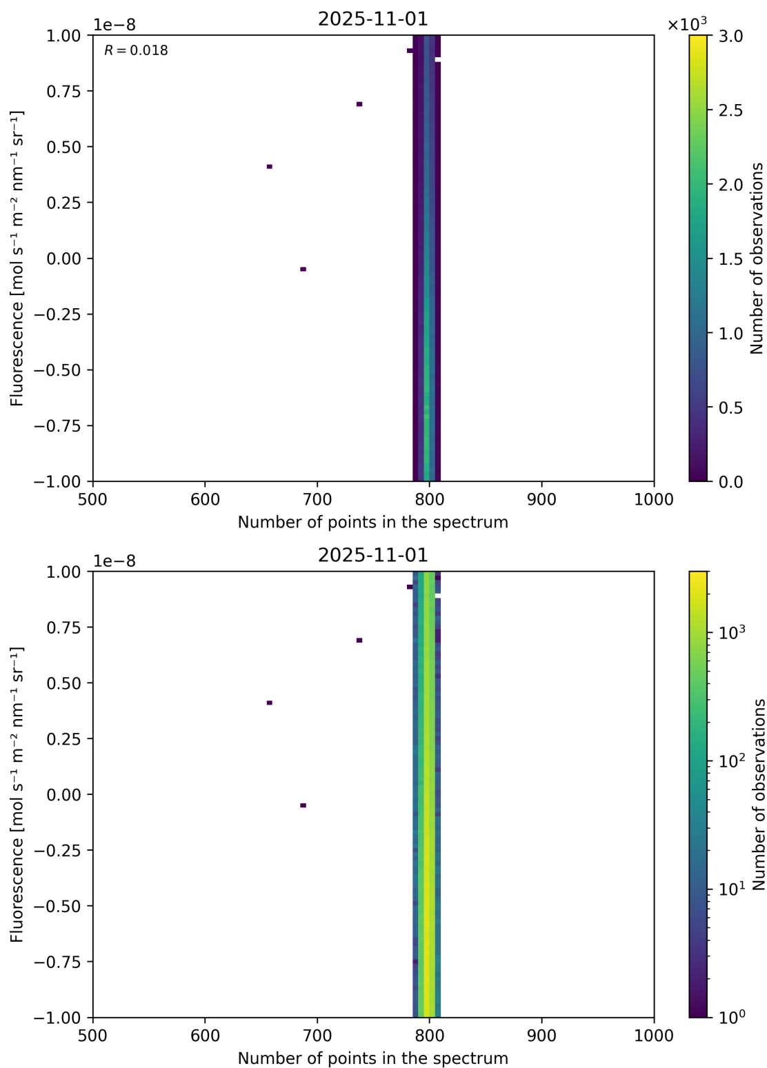
Figure 91: Scatter density plot of “Number of points in the spectrum” against “Fluorescence” for 2025-10-31 to 2025-11-02.
