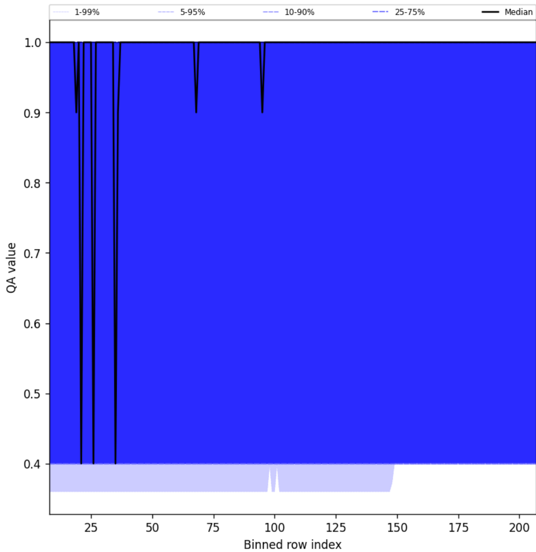
Figure 33: Along track statistics of “QA value” for 2025-10-31 to 2025-11-02
