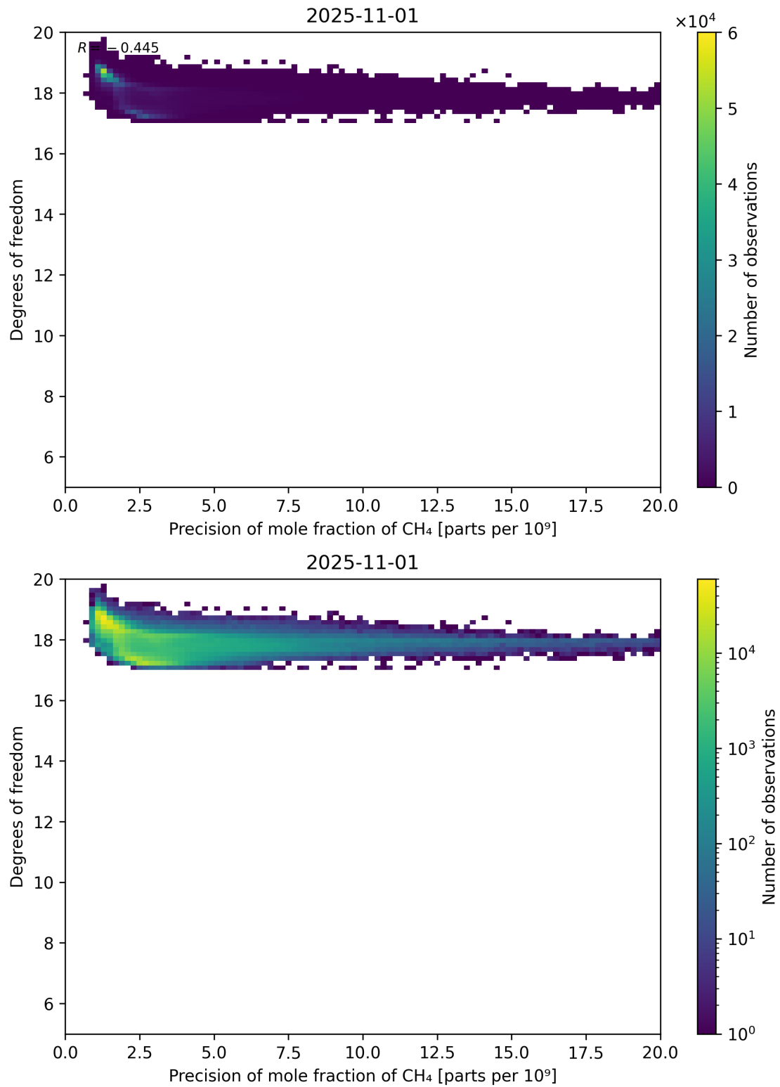
Figure 80: Scatter density plot of “Precision of mole fraction of CH 4 ” against “Degrees of freedom” for 2025-10-31 to 2025-11-02.
