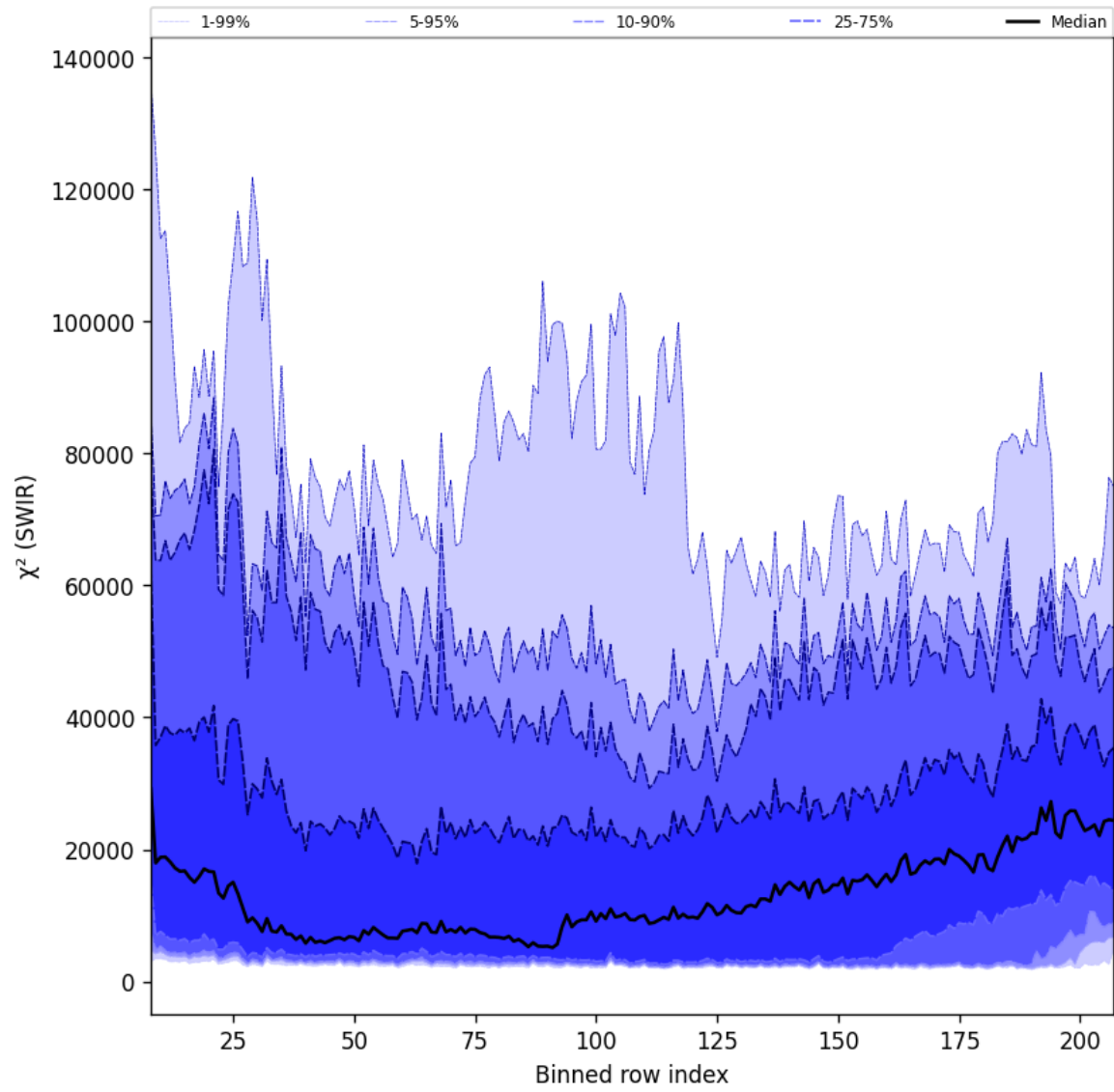
Figure 39: Along track statistics of “ \chi^2 (SWIR)” for 2025-10-31 to 2025-11-02
