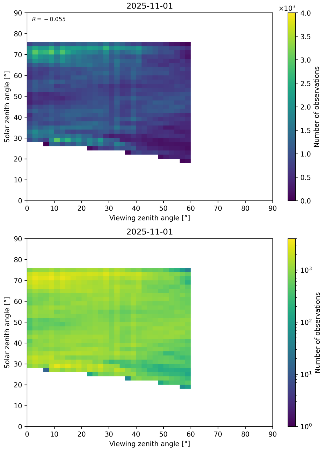
Figure 115: Scatter density plot of “Viewing zenith angle” against “Solar zenith angle” for 2025-10-31 to 2025-11-02.
