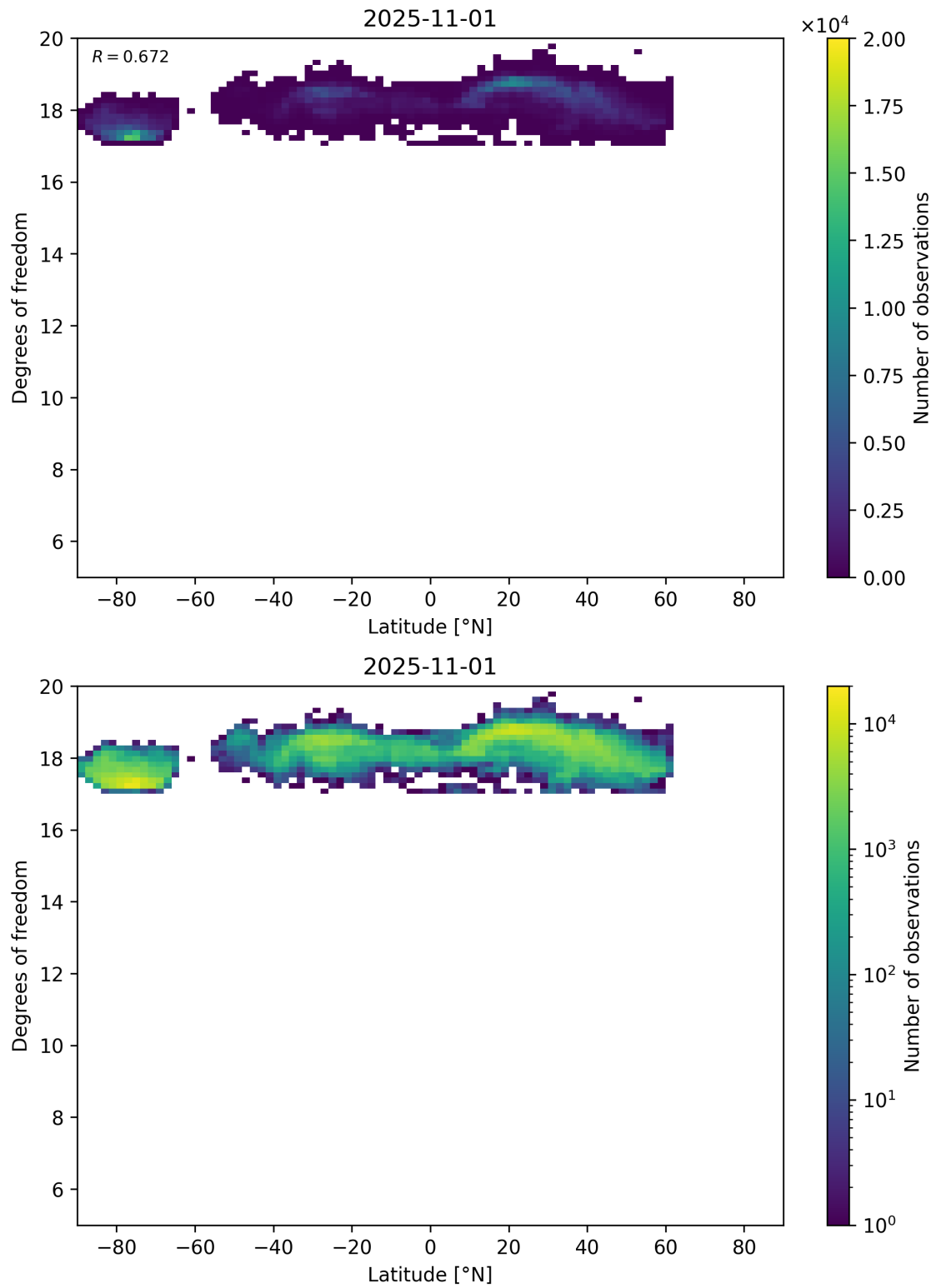
Figure 55: Scatter density plot of “Latitude” against “Degrees of freedom” for 2025-10-31 to 2025-11-02.
