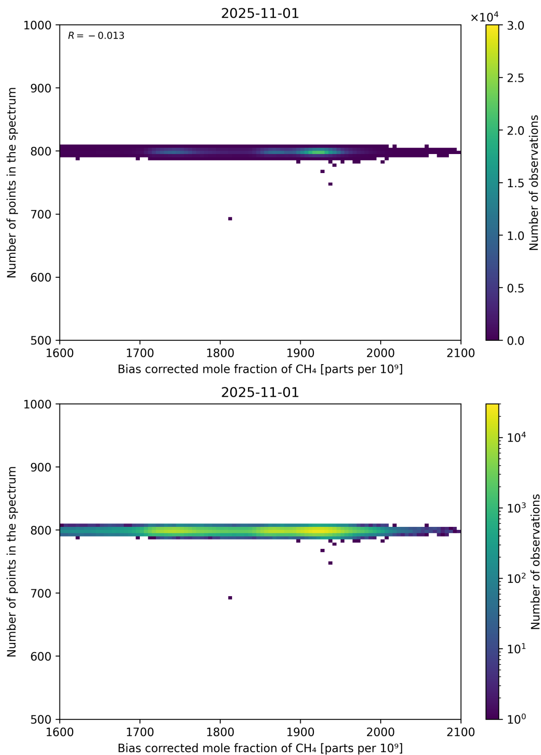
Figure 68: Scatter density plot of “Bias corrected mole fraction of CH 4 ” against “Number of points in the spectrum” for 2025-10-31 to 2025-11-02.
