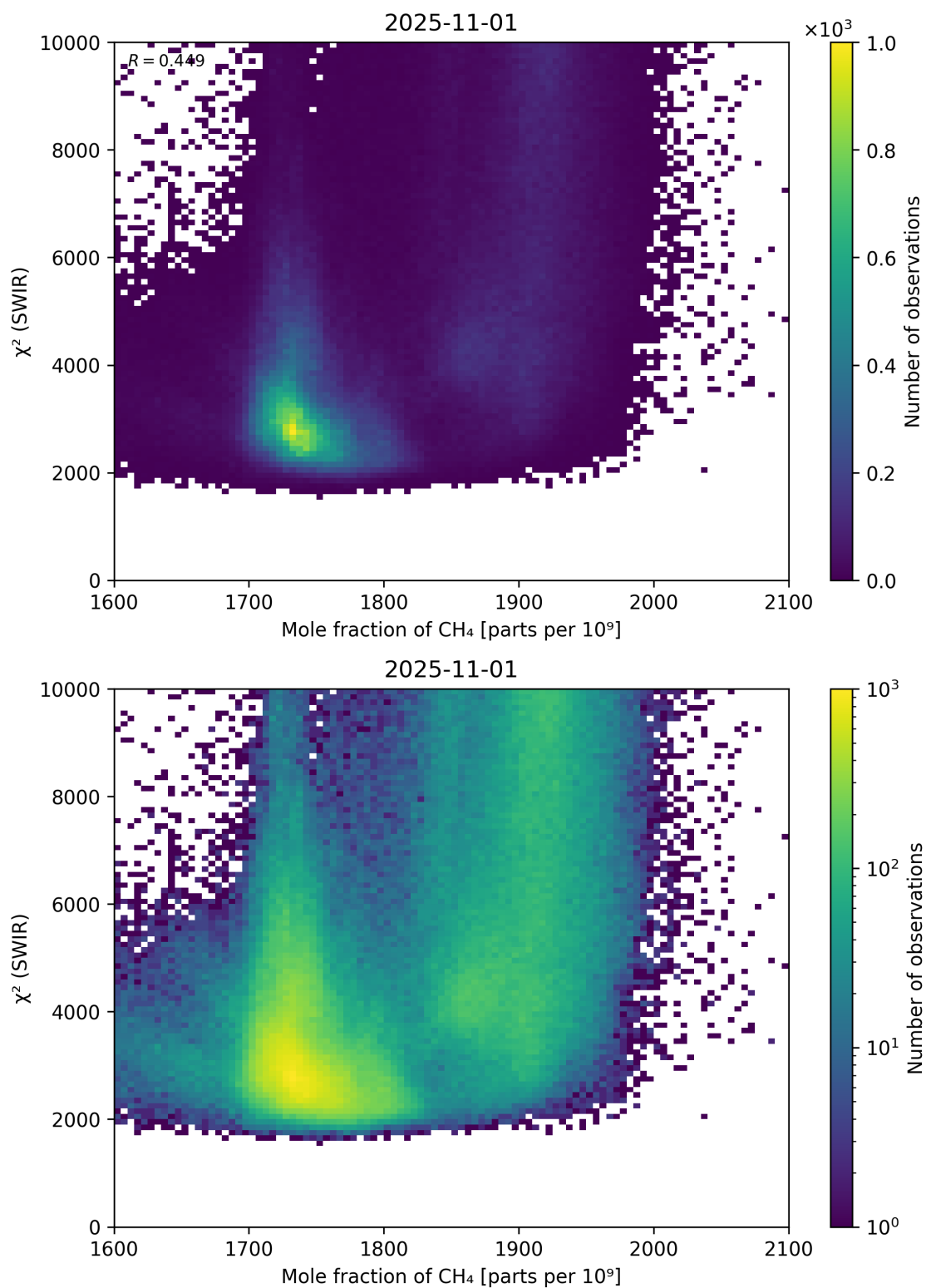
Figure 71: Scatter density plot of “Mole fraction of \text{CH}_4 ” against “ \chi^2 (SWIR)” for 2025-10-31 to 2025-11-02.
