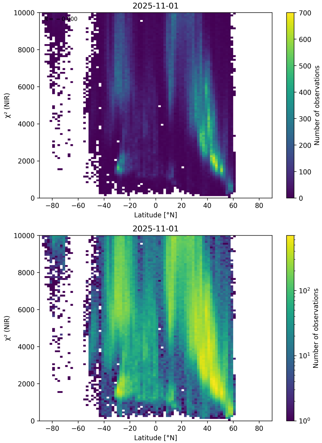
Figure 53: Scatter density plot of “Latitude” against “ \chi^2 (NIR)” for 2025-10-31 to 2025-11-02.
