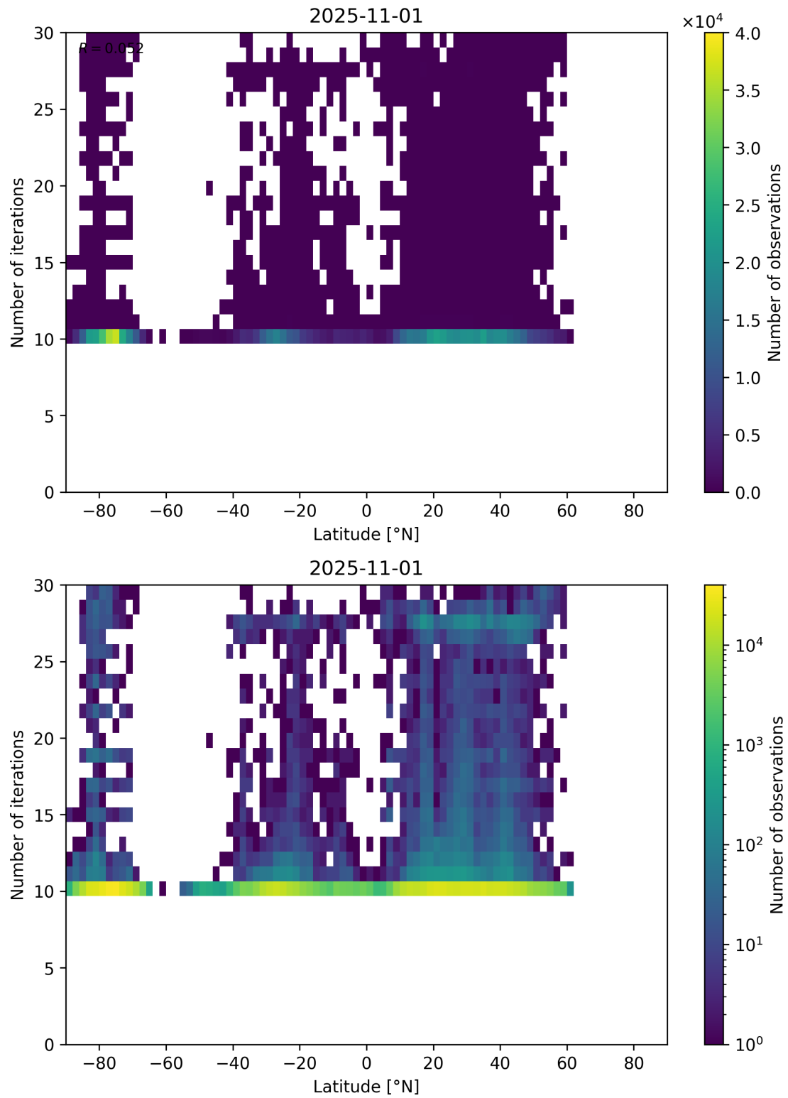
Figure 60: Scatter density plot of “Latitude” against “Number of iterations” for 2025-10-31 to 2025-11-02.
