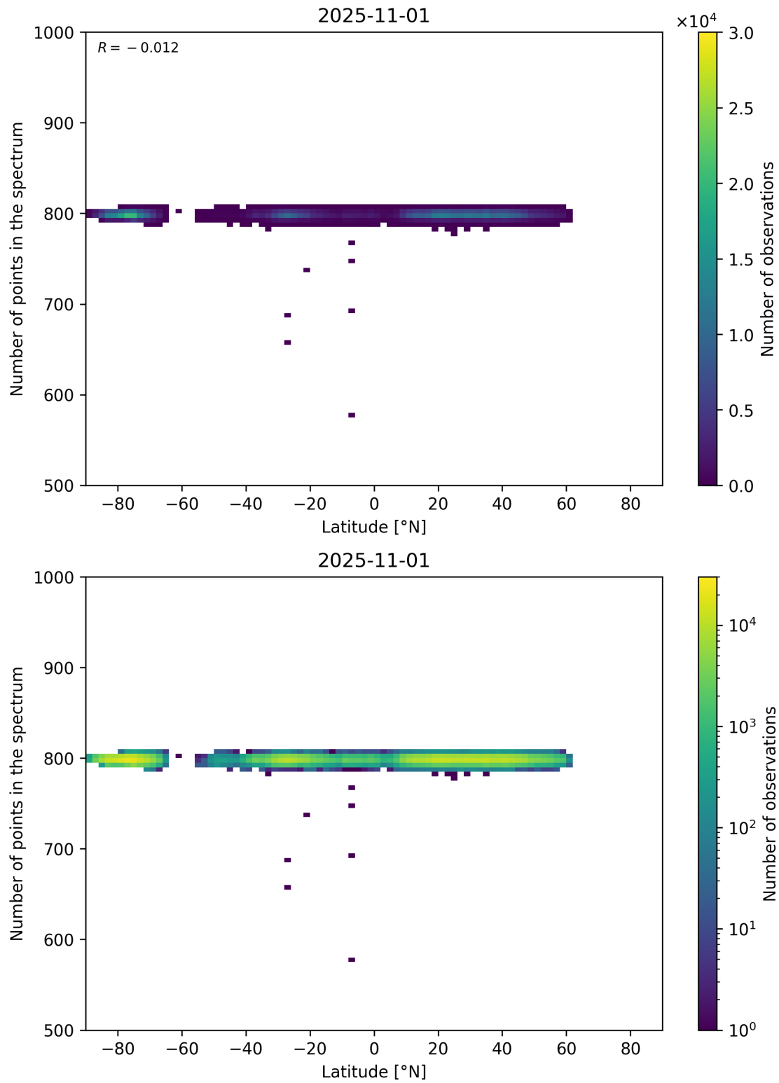
Figure 61: Scatter density plot of “Latitude” against “Number of points in the spectrum” for 2025-10-31 to 2025-11-02.
