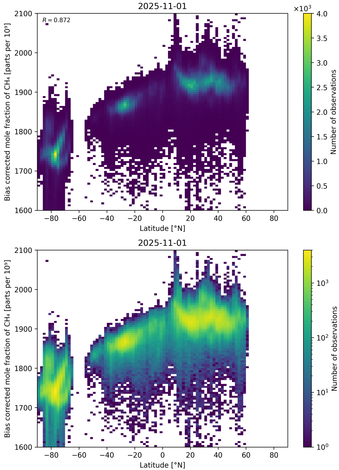
Figure 58: Scatter density plot of “Latitude” against “Bias corrected mole fraction of \text{CH}_4 ” for 2025-10-31 to 2025-11-02.
