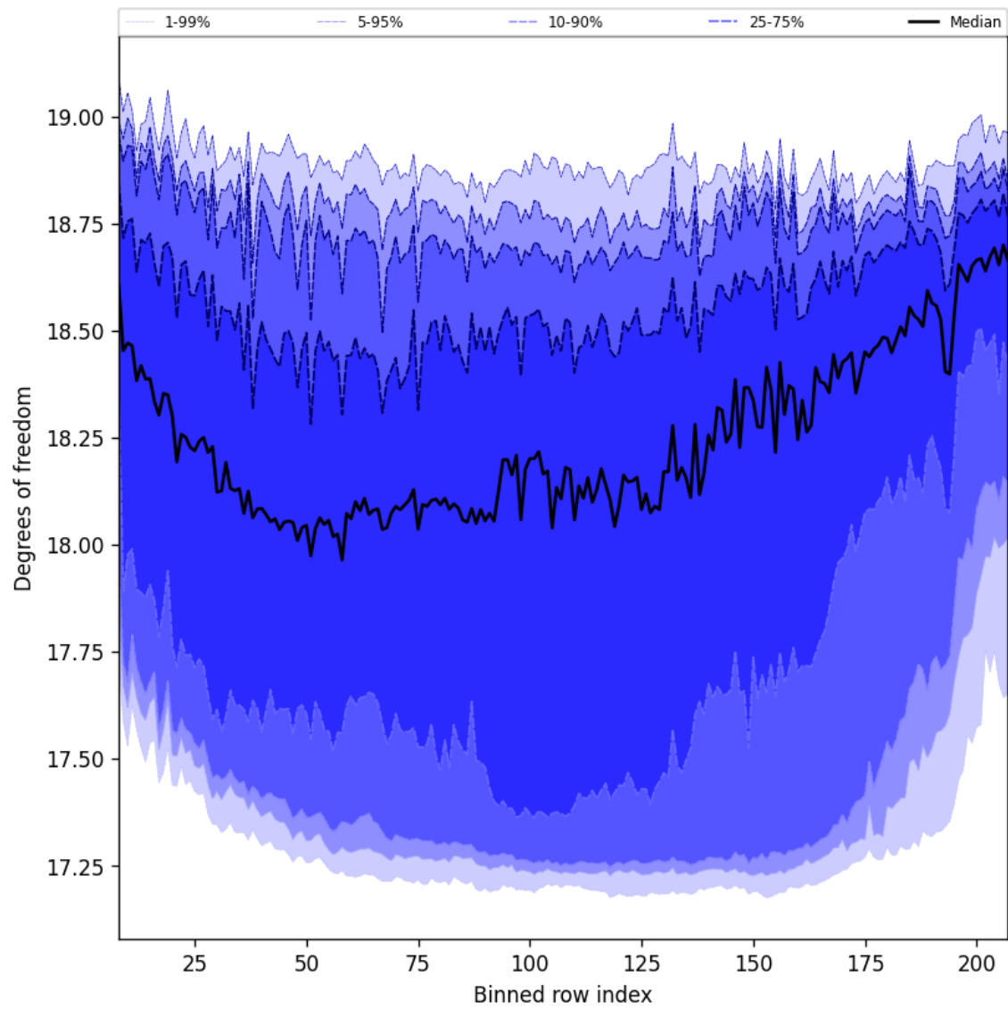
Figure 41: Along track statistics of “Degrees of freedom” for 2025-10-31 to 2025-11-02
