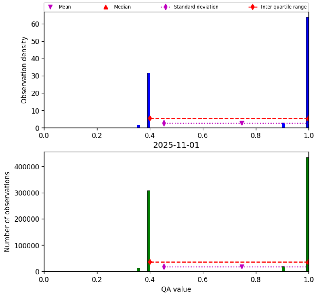
Figure 22: Histogram of “QA value” for 2025-10-31 to 2025-11-02
