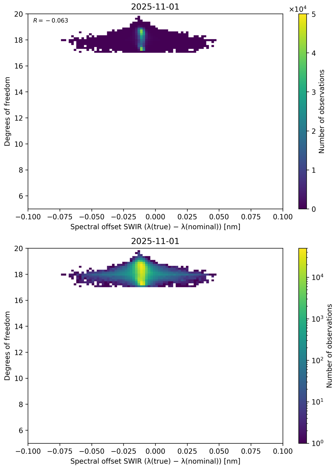
Figure 119: Scatter density plot of “Spectral offset SWIR ( \lambda_{\text{true}} - \lambda_{\text{nominal}} )” against “Degrees of freedom” for 2025-10-31 to 2025-11-02.
