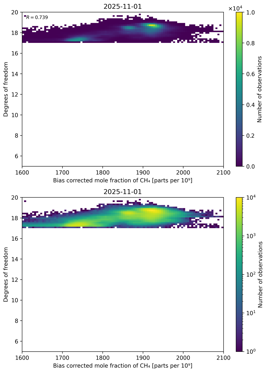
Figure 65: Scatter density plot of “Bias corrected mole fraction of CH 4 ” against “Degrees of freedom” for 2025-10-31 to 2025-11-02.
