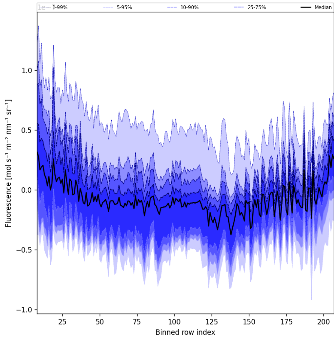
Figure 43: Along track statistics of “Fluorescence” for 2025-10-31 to 2025-11-02
