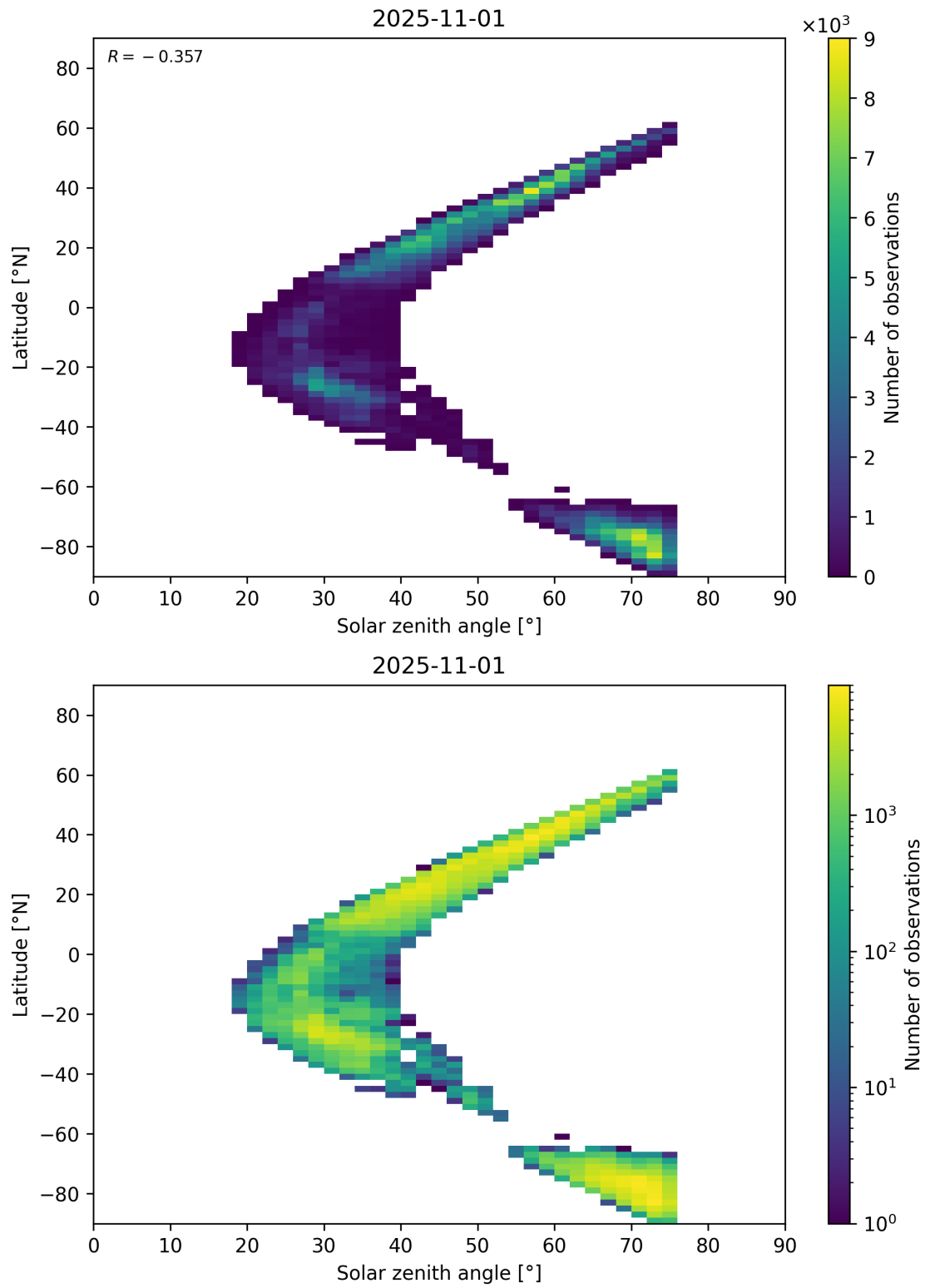
Figure 98: Scatter density plot of “Solar zenith angle” against “Latitude” for 2025-10-31 to 2025-11-02.
