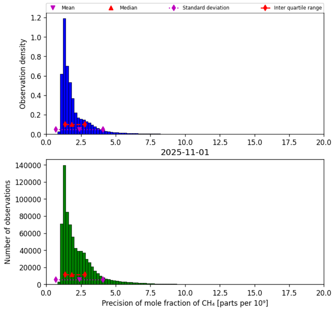
Figure 24: Histogram of “Precision of mole fraction of CH 4 ” for 2025-10-31 to 2025-11-02
