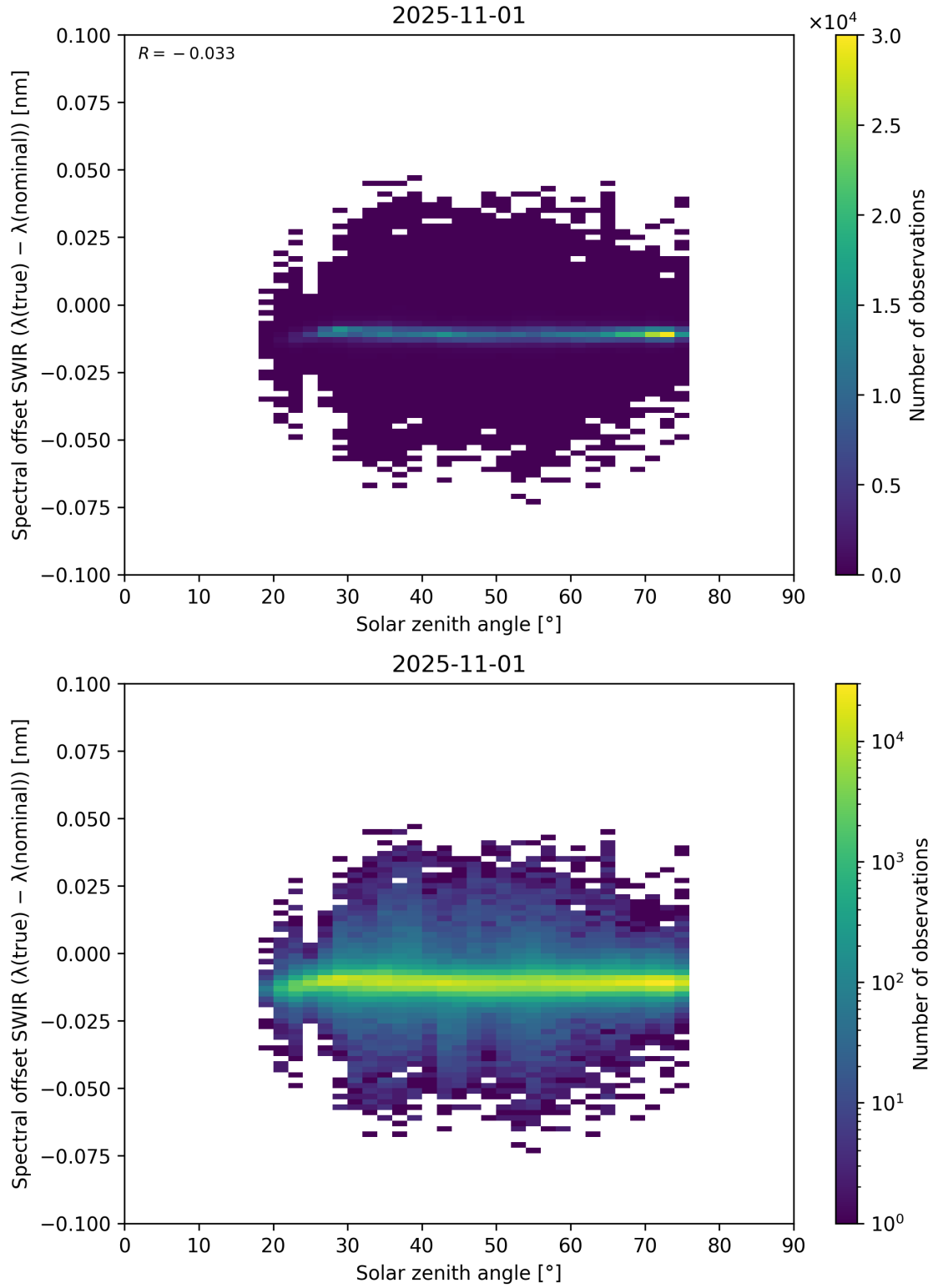
Figure 104: Scatter density plot of “Solar zenith angle” against “Spectral offset SWIR ( \lambda_{\text{true}} - \lambda_{\text{nominal}} )” for 2025-10-31 to 2025-11-02.
