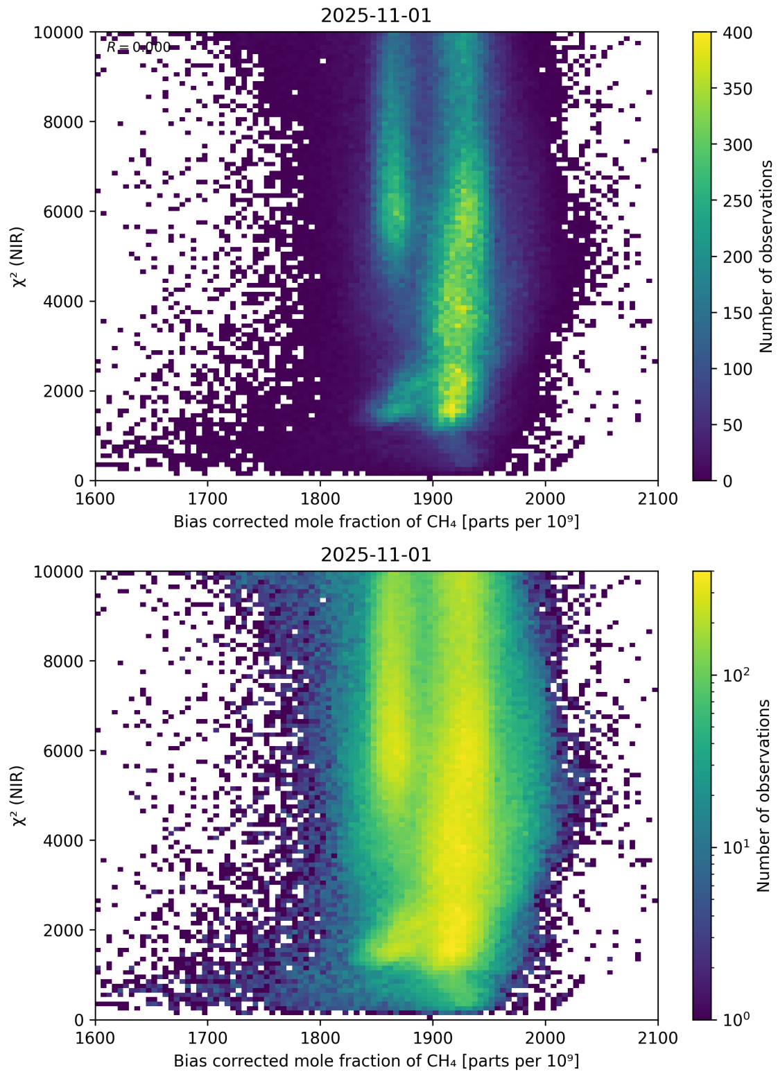
Figure 63: Scatter density plot of “Bias corrected mole fraction of \text{CH}_4 ” against “ \chi^2 (NIR)” for 2025-10-31 to 2025-11-02.
