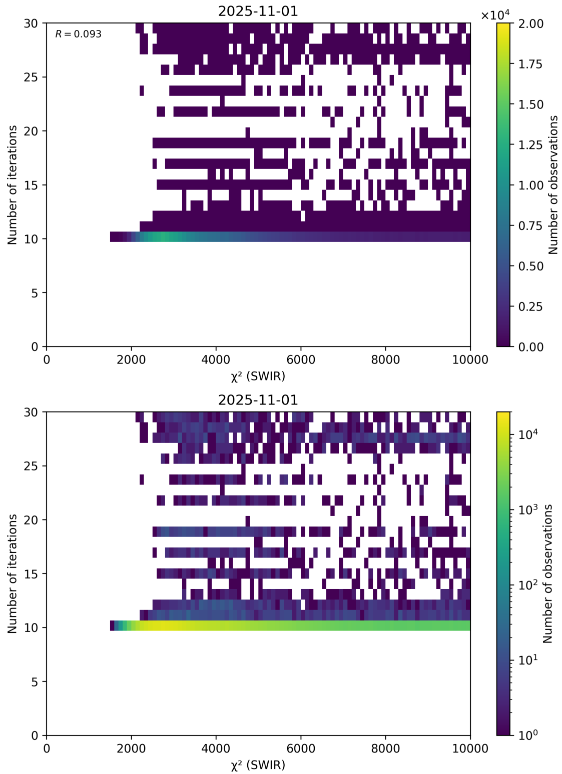
Figure 50: Scatter density plot of “ \chi^2 (SWIR)” against “Number of iterations” for 2025-10-31 to 2025-11-02.
