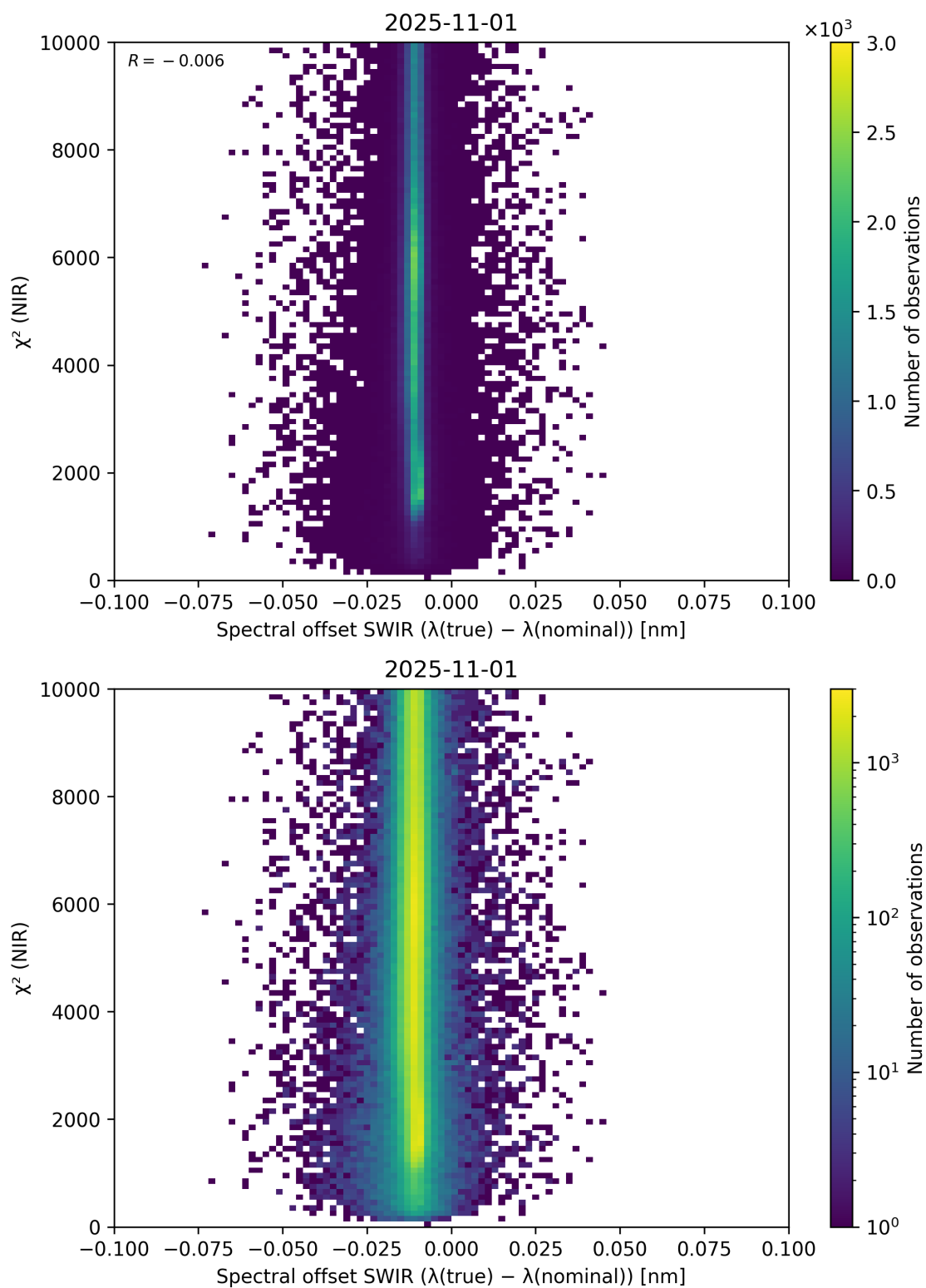
Figure 117: Scatter density plot of “Spectral offset SWIR ( \lambda_{\text{true}} - \lambda_{\text{nominal}} )” against “ \chi^2 (NIR)” for 2025-10-31 to 2025-11-02.
