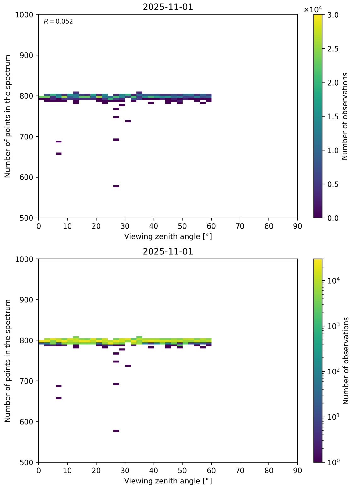
Figure 114: Scatter density plot of “Viewing zenith angle” against “Number of points in the spectrum” for 2025-10-31 to 2025-11-02.
