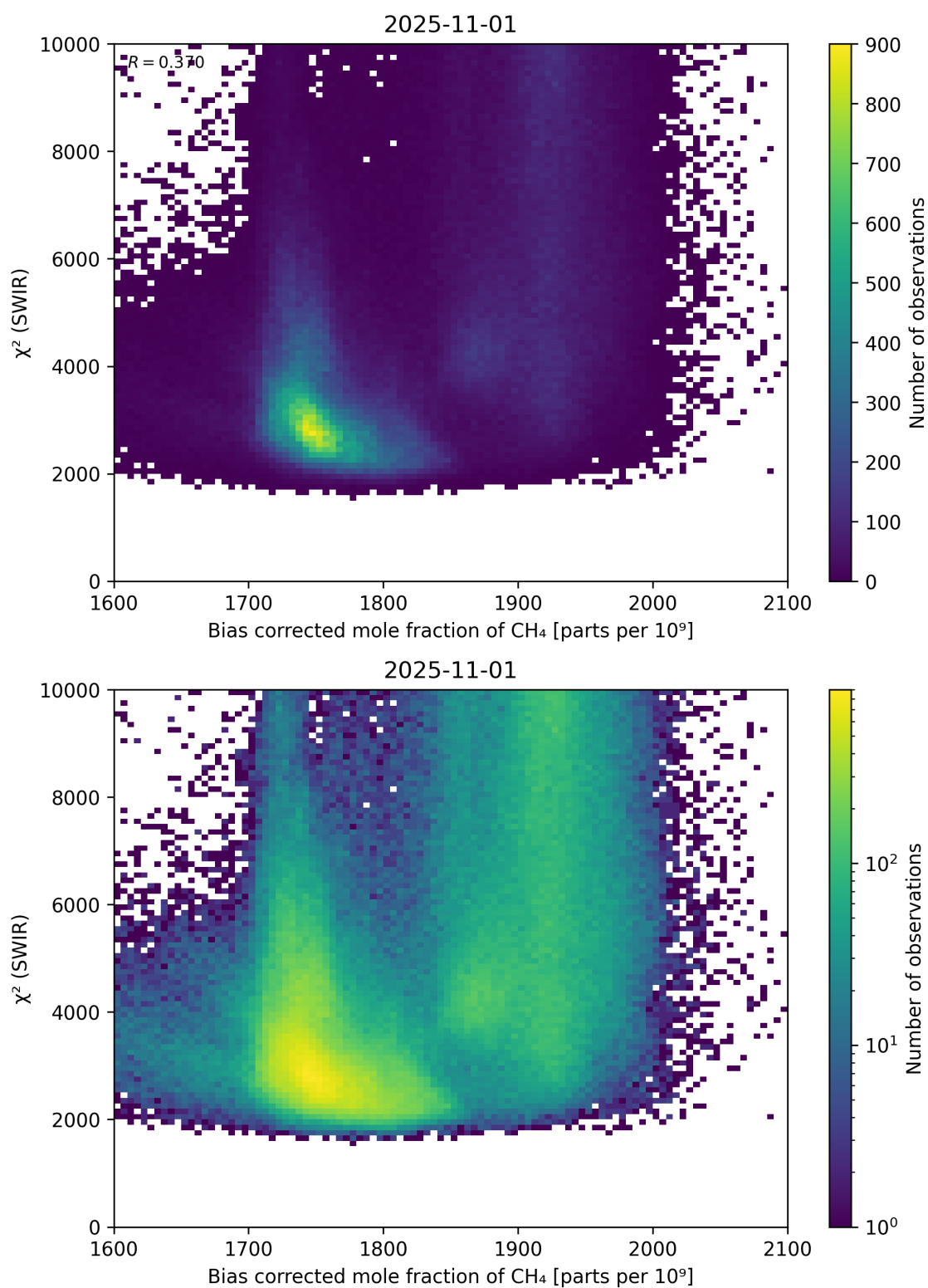
Figure 64: Scatter density plot of “Bias corrected mole fraction of \text{CH}_4 ” against “ \chi^2 (SWIR)” for 2025-10-31 to 2025-11-02.
