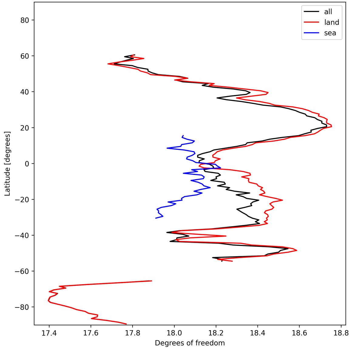
Figure 19: Zonal average of “Degrees of freedom” for 2025-10-31 to 2025-11-02.
