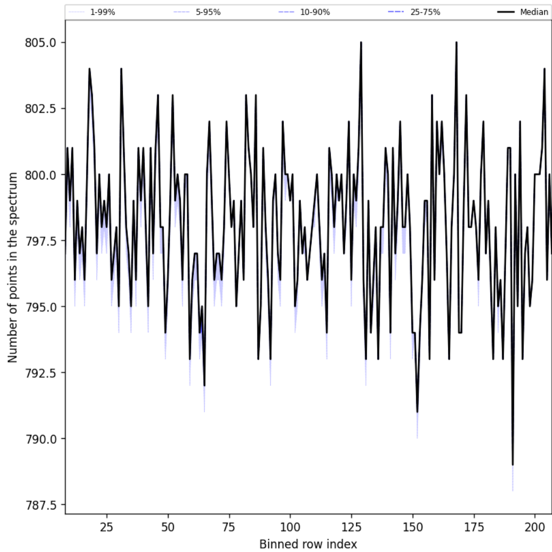
Figure 37: Along track statistics of “Number of points in the spectrum” for 2025-10-31 to 2025-11-02
