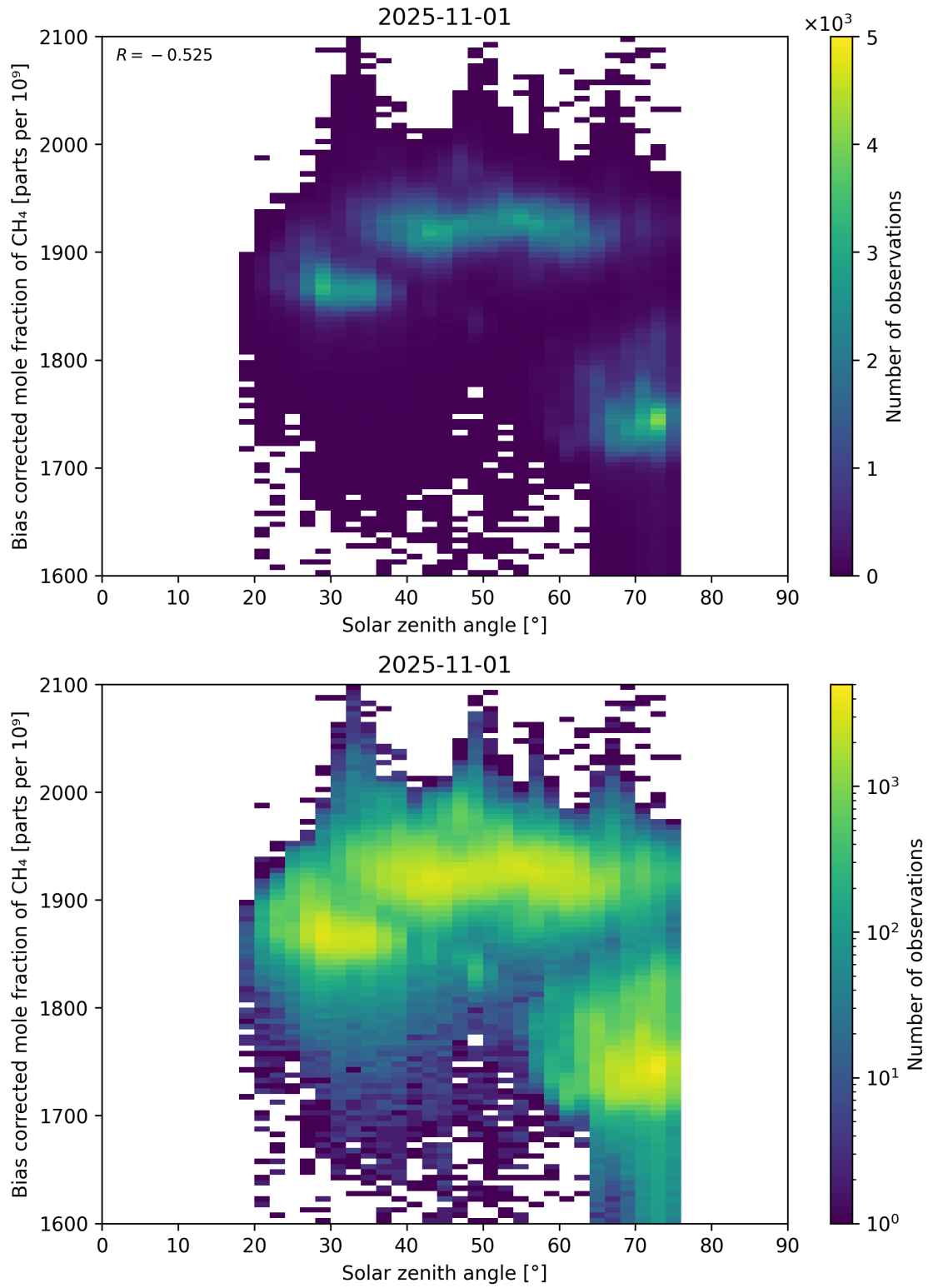
Figure 100: Scatter density plot of “Solar zenith angle” against “Bias corrected mole fraction of CH 4 ” for 2025-10-31 to 2025-11-02.
