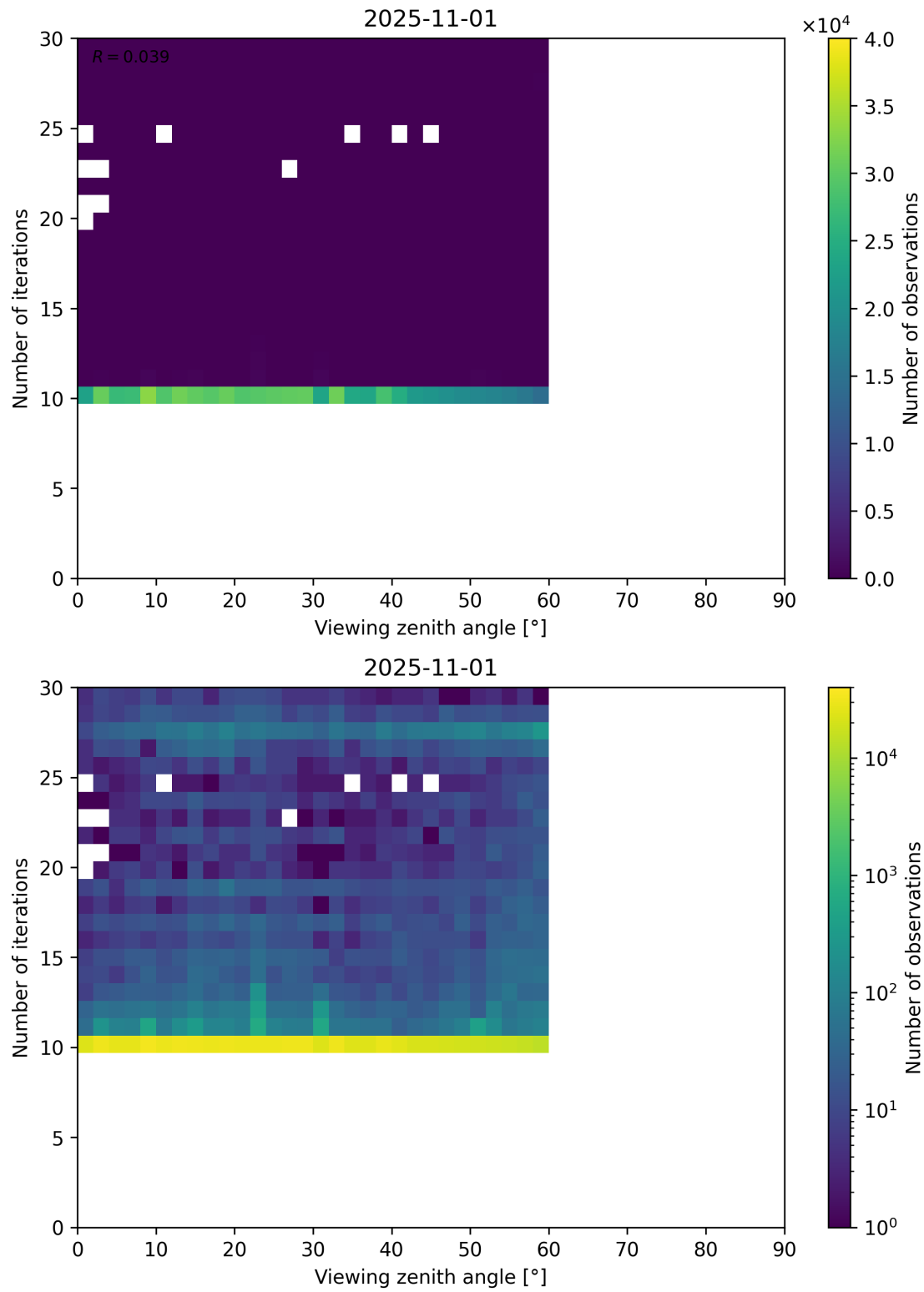
Figure 113: Scatter density plot of “Viewing zenith angle” against “Number of iterations” for 2025-10-31 to 2025-11-02.
