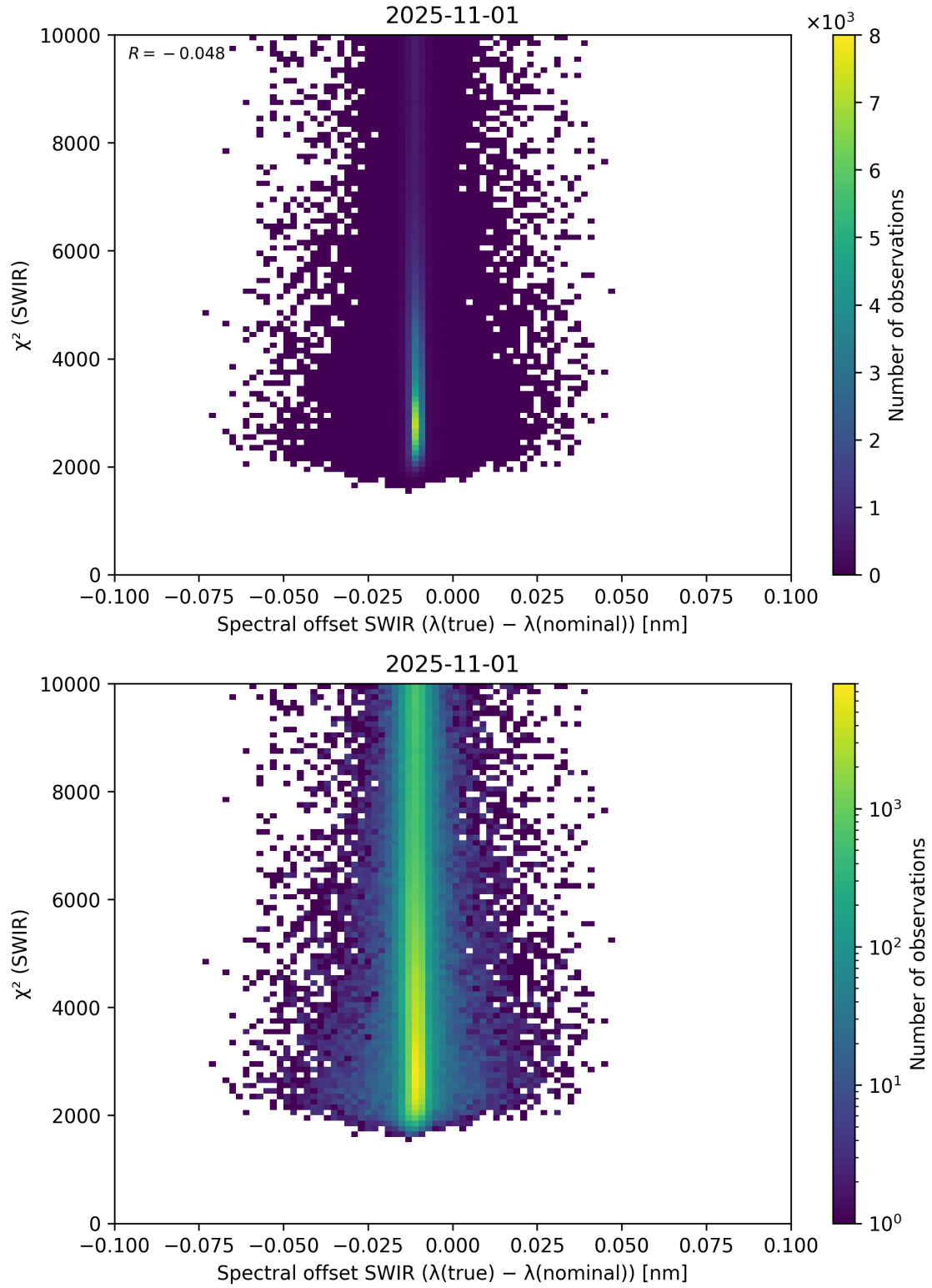
Figure 118: Scatter density plot of “Spectral offset SWIR ( \lambda_{\text{true}} - \lambda_{\text{nominal}} )” against “ \chi^2 (SWIR)” for 2025-10-31 to 2025-11-02.
