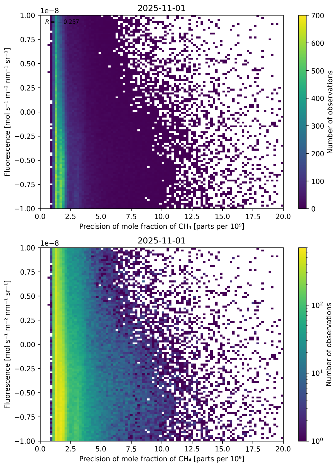
Figure 81: Scatter density plot of “Precision of mole fraction of \text{CH}_4 ” against “Fluorescence” for 2025-10-31 to 2025-11-02.
