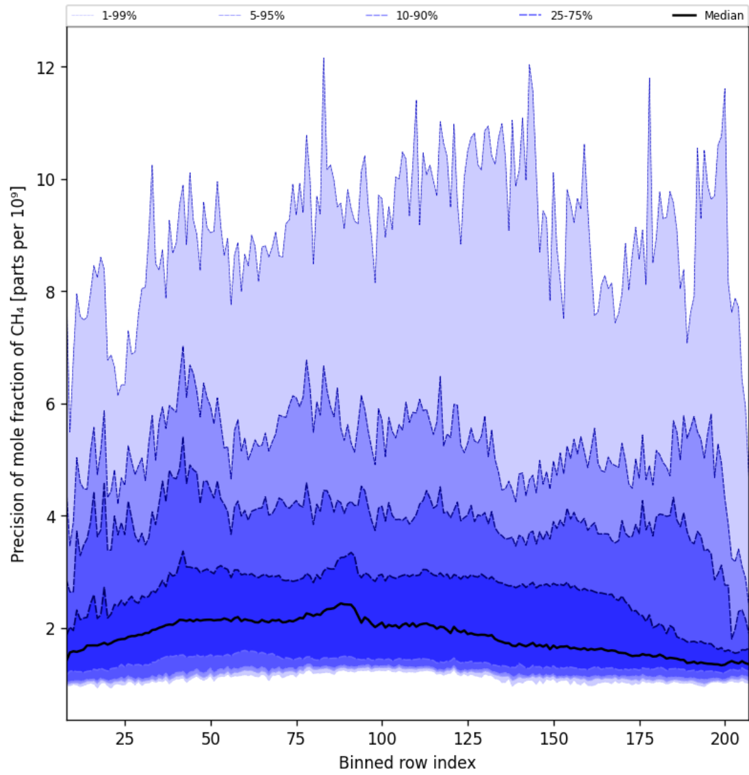
Figure 35: Along track statistics of “Precision of mole fraction of CH 4 ” for 2025-10-31 to 2025-11-02
