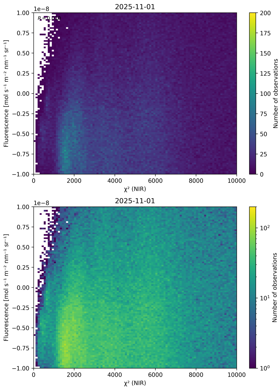
Figure 45: Scatter density plot of “ \chi^2 (NIR)” against “Fluorescence” for 2025-10-31 to 2025-11-02.
