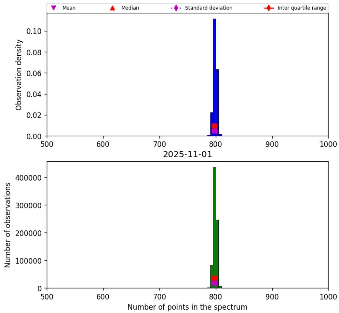
Figure 26: Histogram of “Number of points in the spectrum” for 2025-10-31 to 2025-11-02
