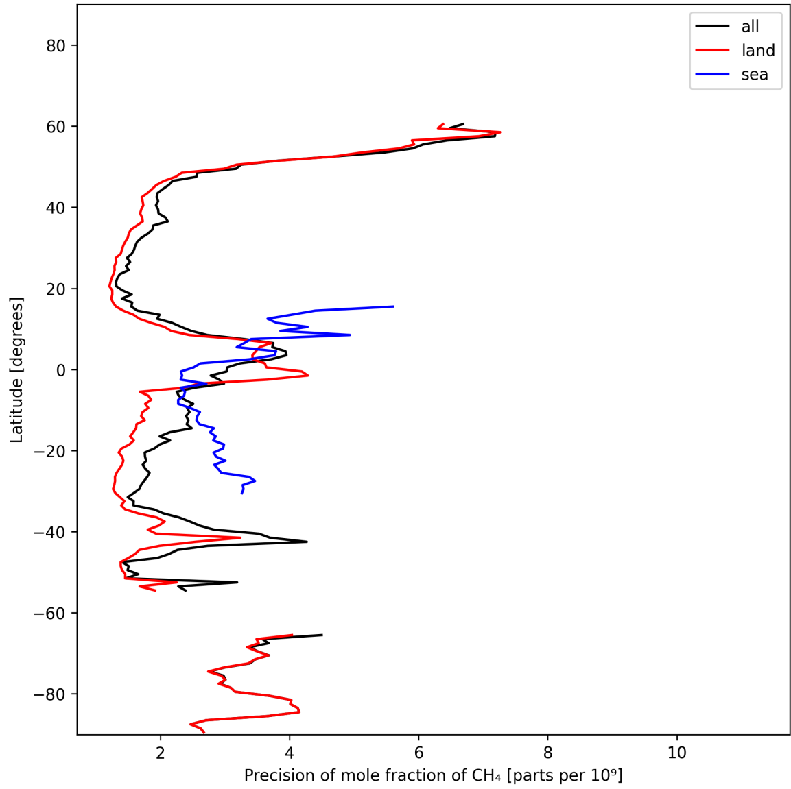
Figure 13: Zonal average of “Precision of mole fraction of CH 4 ” for 2025-10-31 to 2025-11-02.
