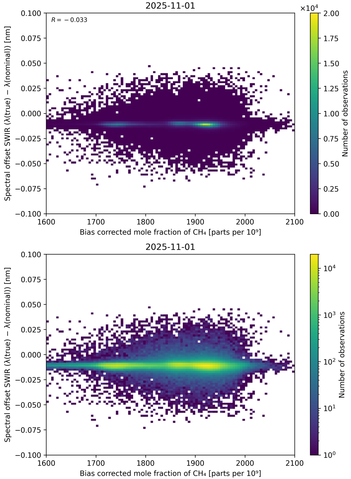
Figure 69: Scatter density plot of “Bias corrected mole fraction of \text{CH}_4 ” against “Spectral offset SWIR ( \lambda_{\text{true}} - \lambda_{\text{nominal}} )” for 2025-10-31 to 2025-11-02.
