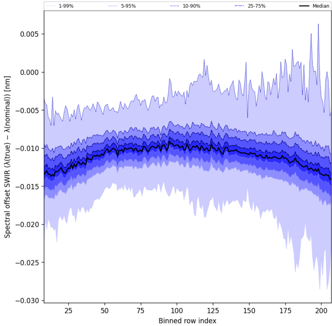
Figure 38: Along track statistics of “Spectral offset SWIR ( \lambda_{\text{true}} - \lambda_{\text{nominal}} )” for 2025-10-31 to 2025-11-02
