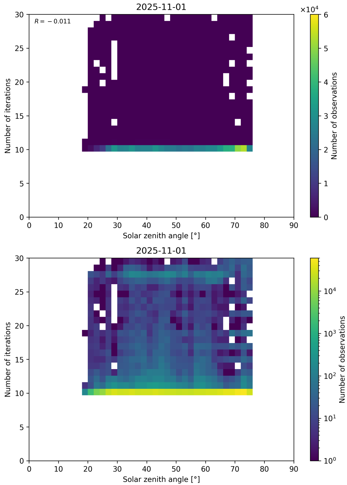
Figure 102: Scatter density plot of “Solar zenith angle” against “Number of iterations” for 2025-10-31 to 2025-11-02.
