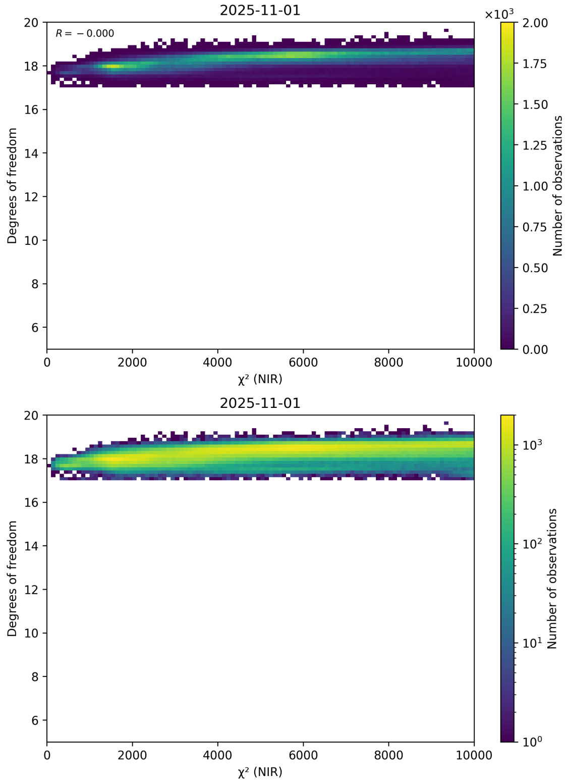
Figure 44: Scatter density plot of “ \chi^2 (NIR)” against “Degrees of freedom” for 2025-10-31 to 2025-11-02.
