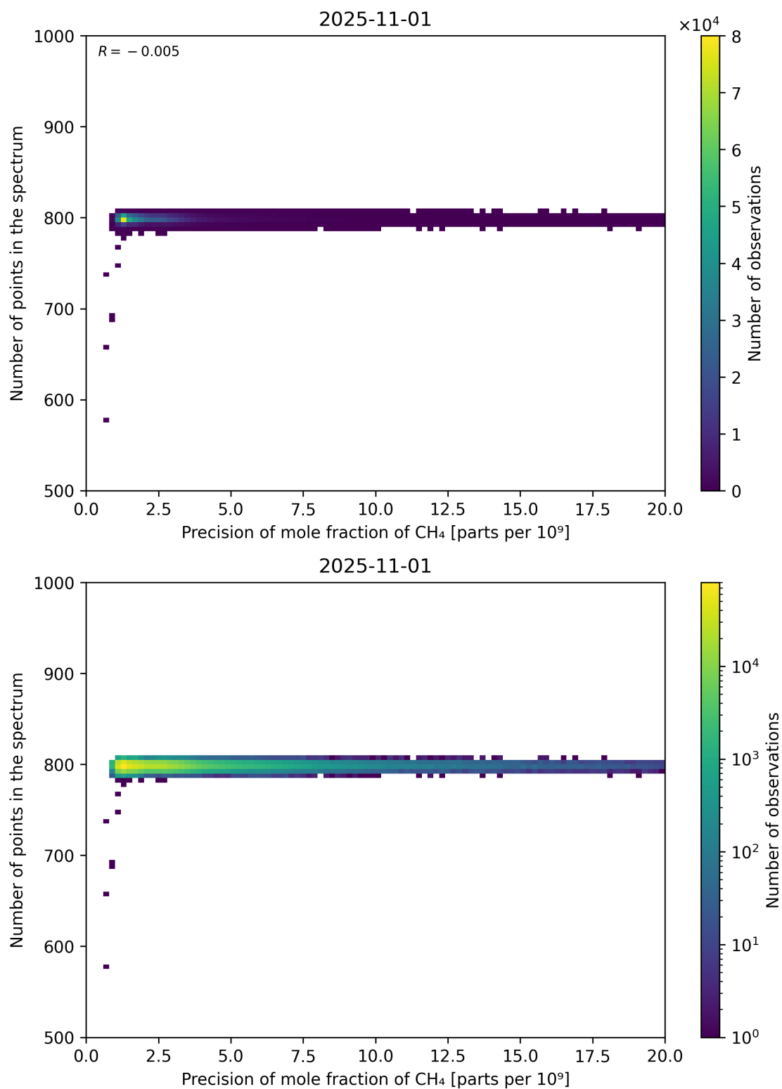
Figure 84: Scatter density plot of “Precision of mole fraction of CH 4 ” against “Number of points in the spectrum” for 2025-10-31 to 2025-11-02.
