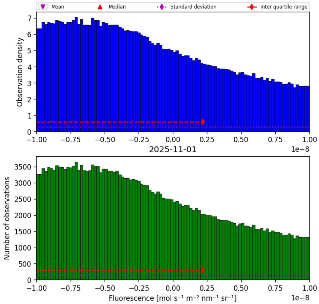
Figure 32: Histogram of “Fluorescence” for 2025-10-31 to 2025-11-02
