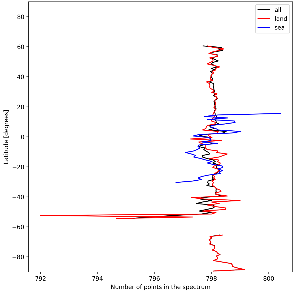
Figure 15: Zonal average of “Number of points in the spectrum” for 2025-10-31 to 2025-11-02.
