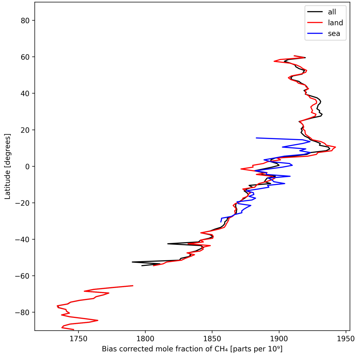
Figure 14: Zonal average of “Bias corrected mole fraction of CH 4 ” for 2025-10-31 to 2025-11-02.
