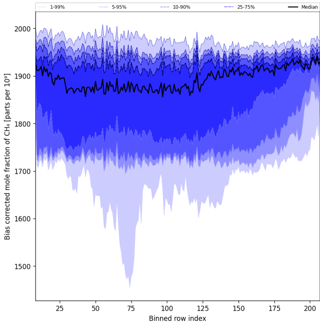
Figure 36: Along track statistics of “Bias corrected mole fraction of CH 4 ” for 2025-10-31 to 2025-11-02
