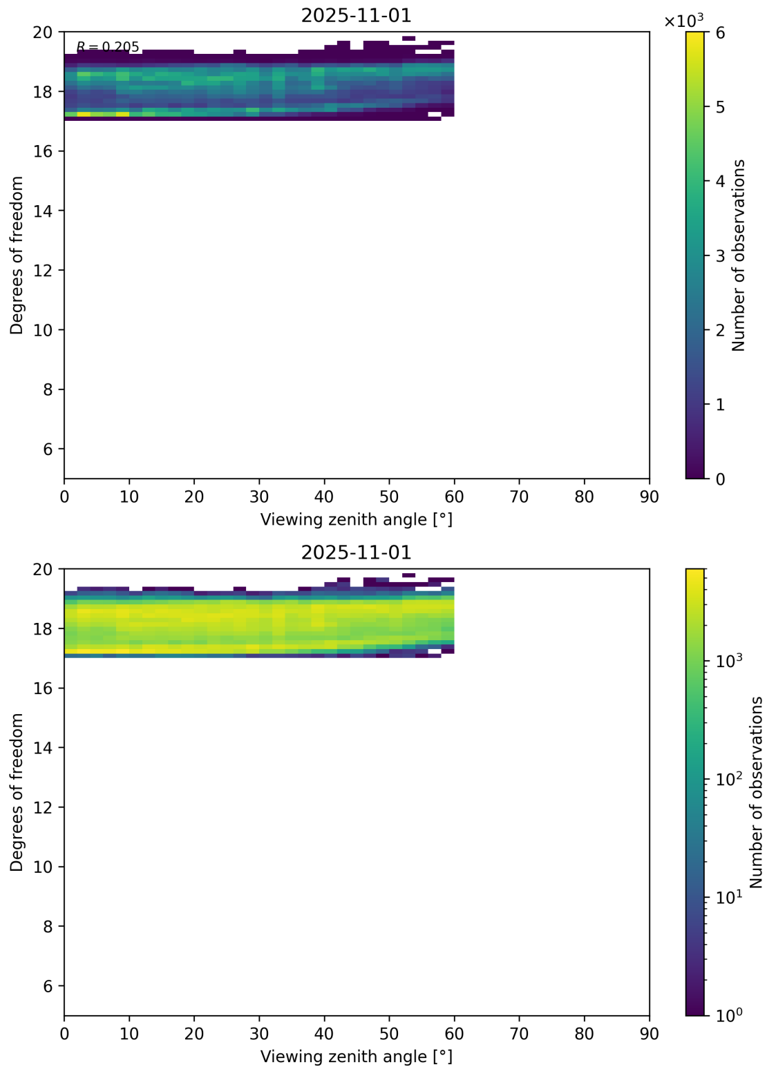
Figure 107: Scatter density plot of “Viewing zenith angle” against “Degrees of freedom” for 2025-10-31 to 2025-11-02.
