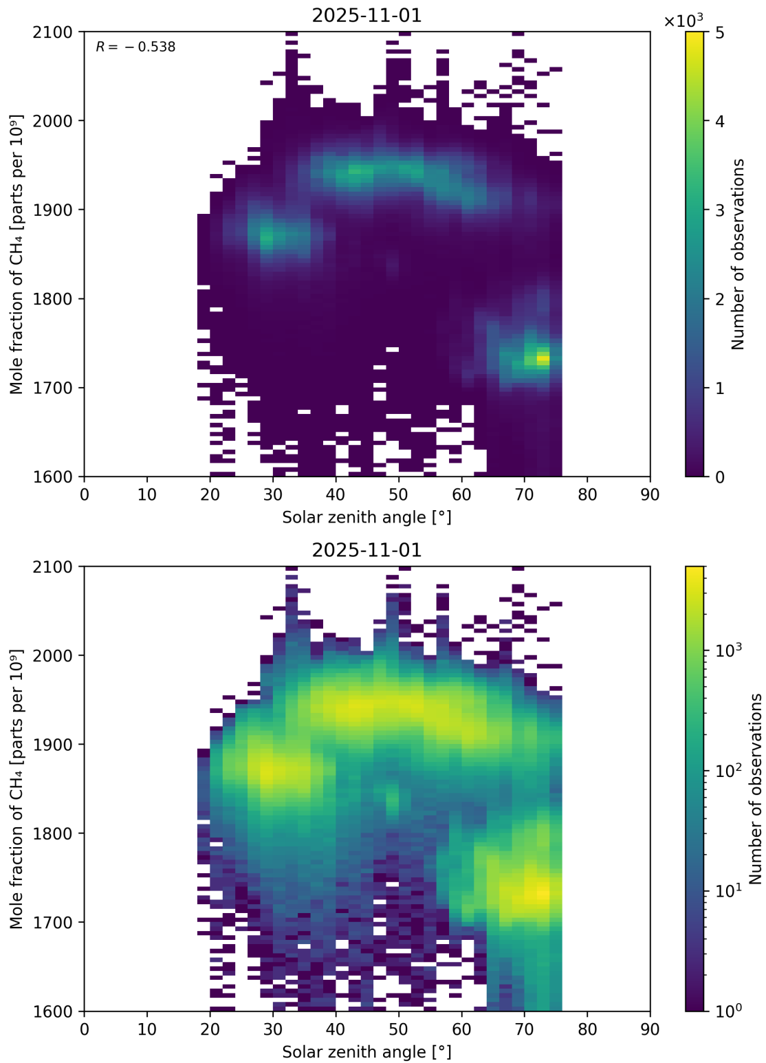
Figure 99: Scatter density plot of “Solar zenith angle” against “Mole fraction of CH 4 ” for 2025-10-31 to 2025-11-02.
