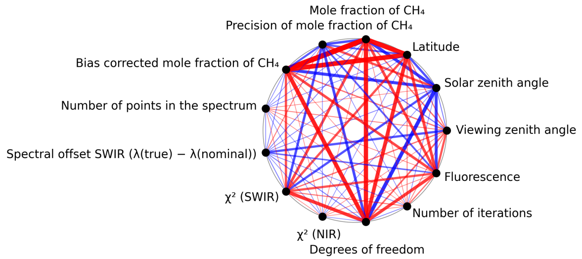
Figure 1: Map of correlation graph for 2025-10-31 to 2025-11-02.
