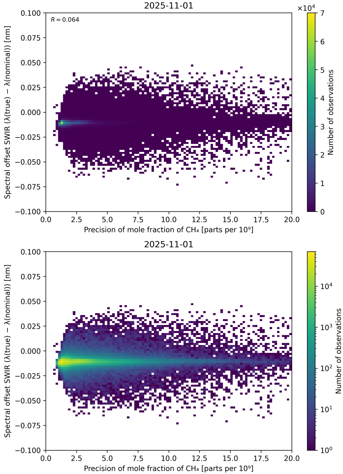
Figure 85: Scatter density plot of “Precision of mole fraction of \text{CH}_4 ” against “Spectral offset SWIR ( \lambda_{\text{true}} - \lambda_{\text{nominal}} )” for 2025-10-31 to 2025-11-02.
