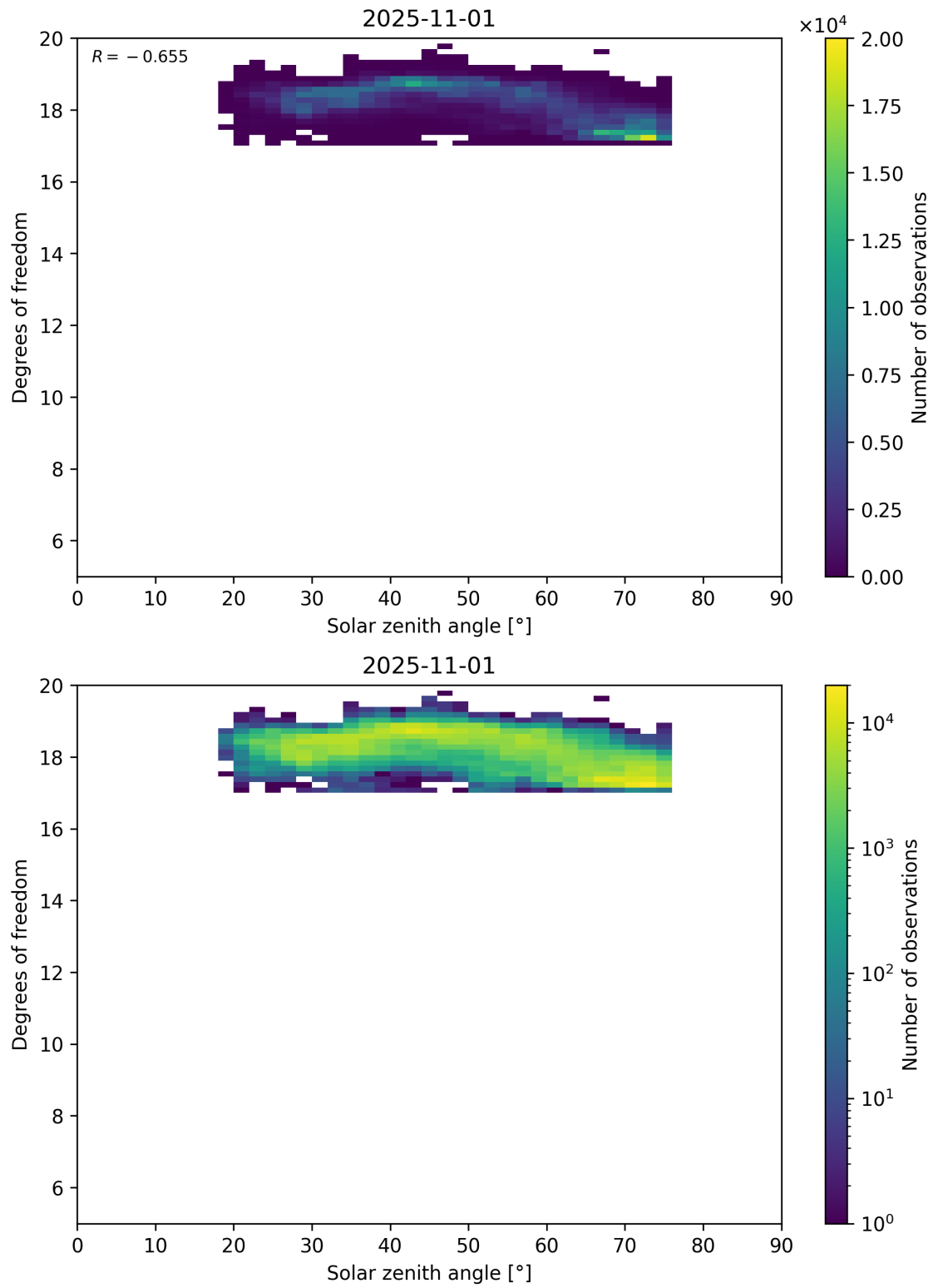
Figure 96: Scatter density plot of “Solar zenith angle” against “Degrees of freedom” for 2025-10-31 to 2025-11-02.
