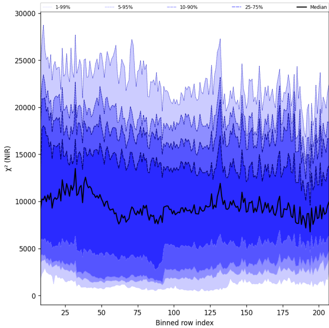
Figure 40: Along track statistics of “ \chi^2 (NIR)” for 2025-10-31 to 2025-11-02
