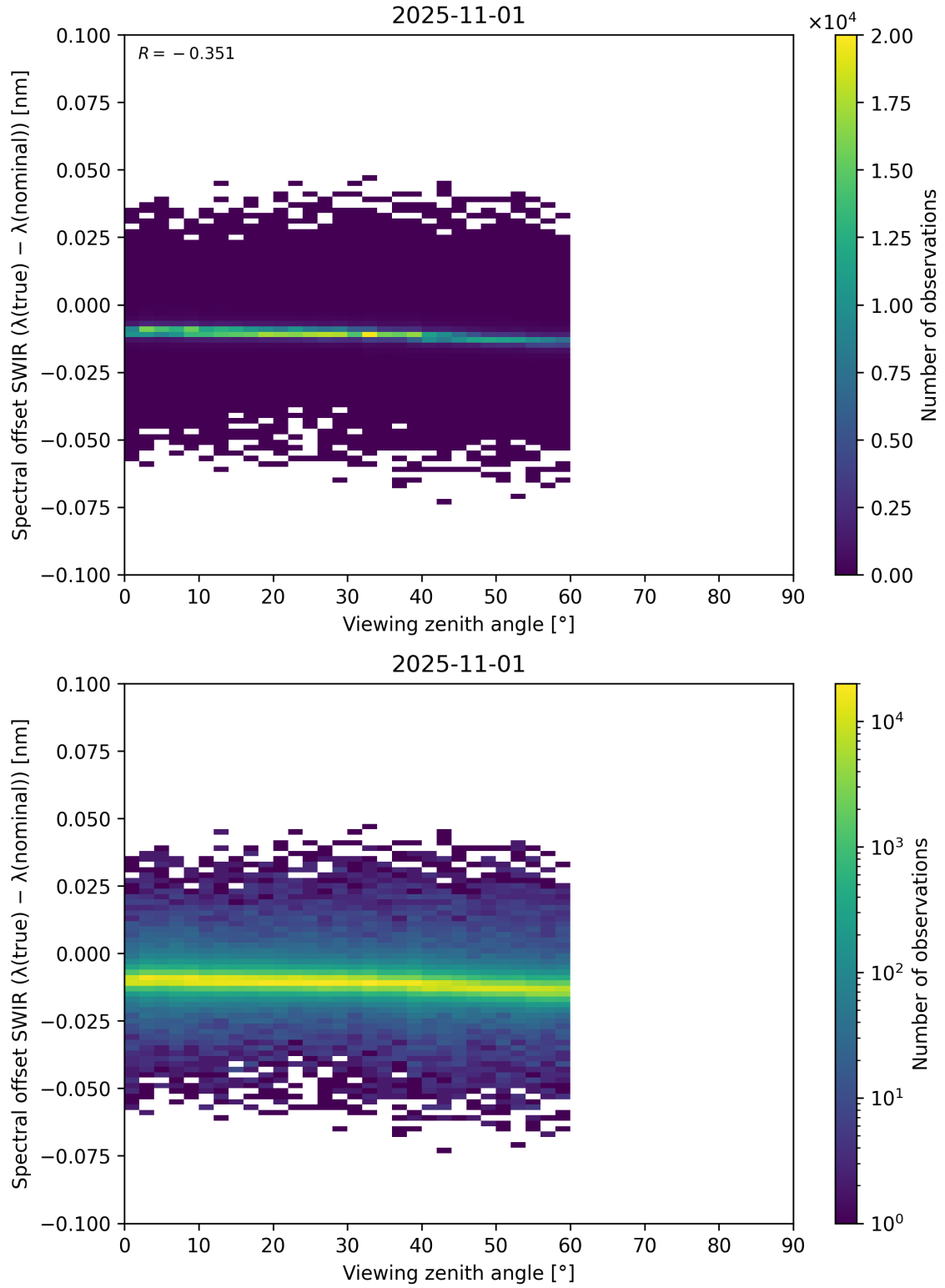
Figure 116: Scatter density plot of “Viewing zenith angle” against “Spectral offset SWIR ( \lambda_{\text{true}} - \lambda_{\text{nominal}} )” for 2025-10-31 to 2025-11-02.
