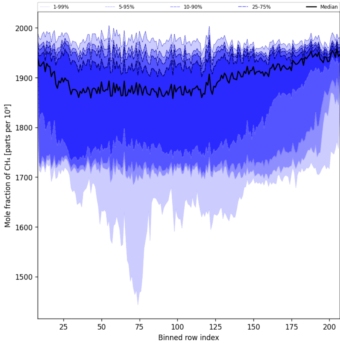
Figure 34: Along track statistics of “Mole fraction of CH 4 ” for 2025-10-31 to 2025-11-02
