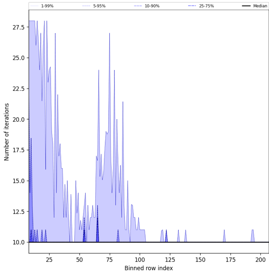
Figure 42: Along track statistics of “Number of iterations” for 2025-10-31 to 2025-11-02
