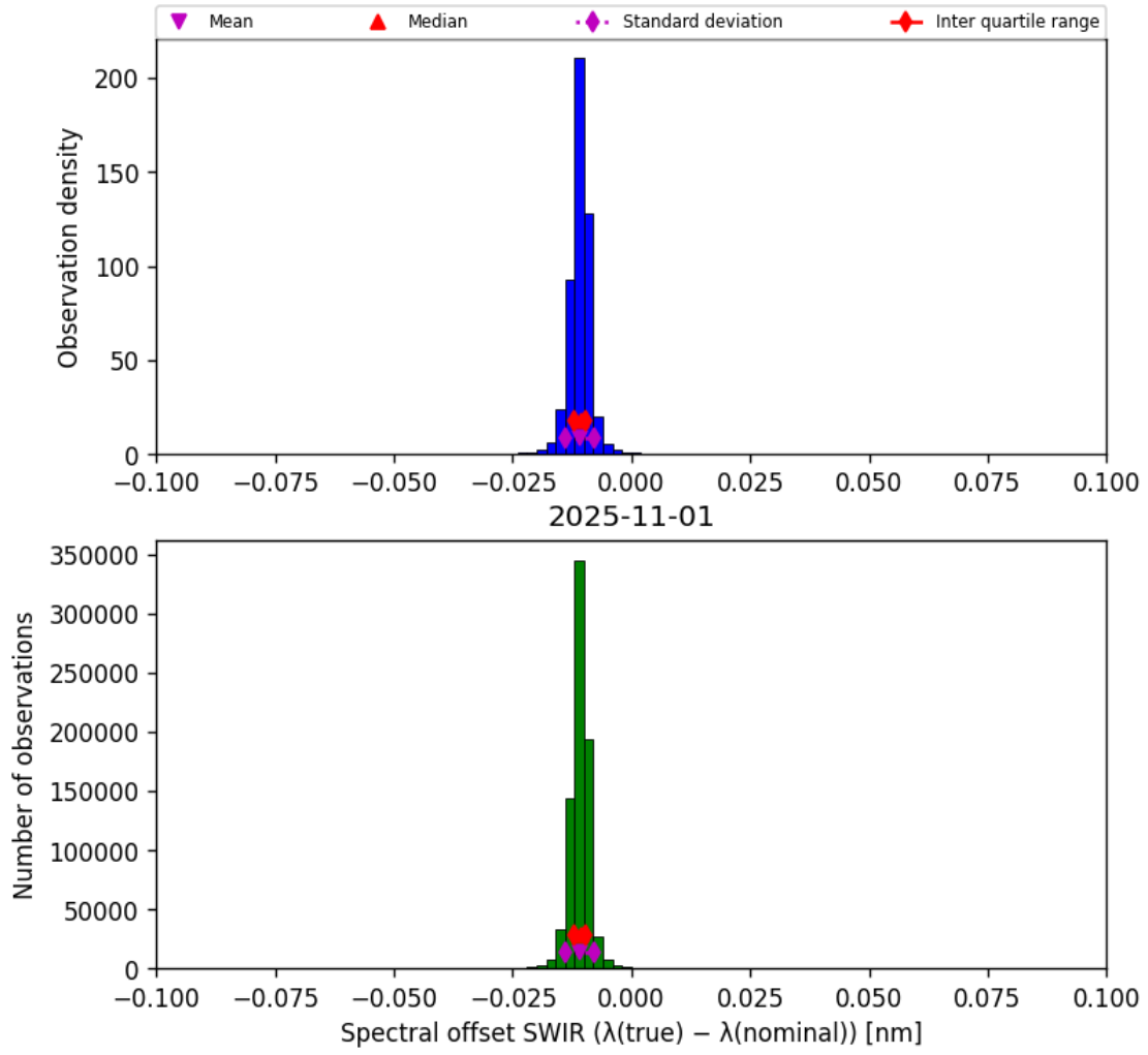
Figure 27: Histogram of “Spectral offset SWIR ( \lambda_{\text{true}} - \lambda_{\text{nominal}} )” for 2025-10-31 to 2025-11-02
