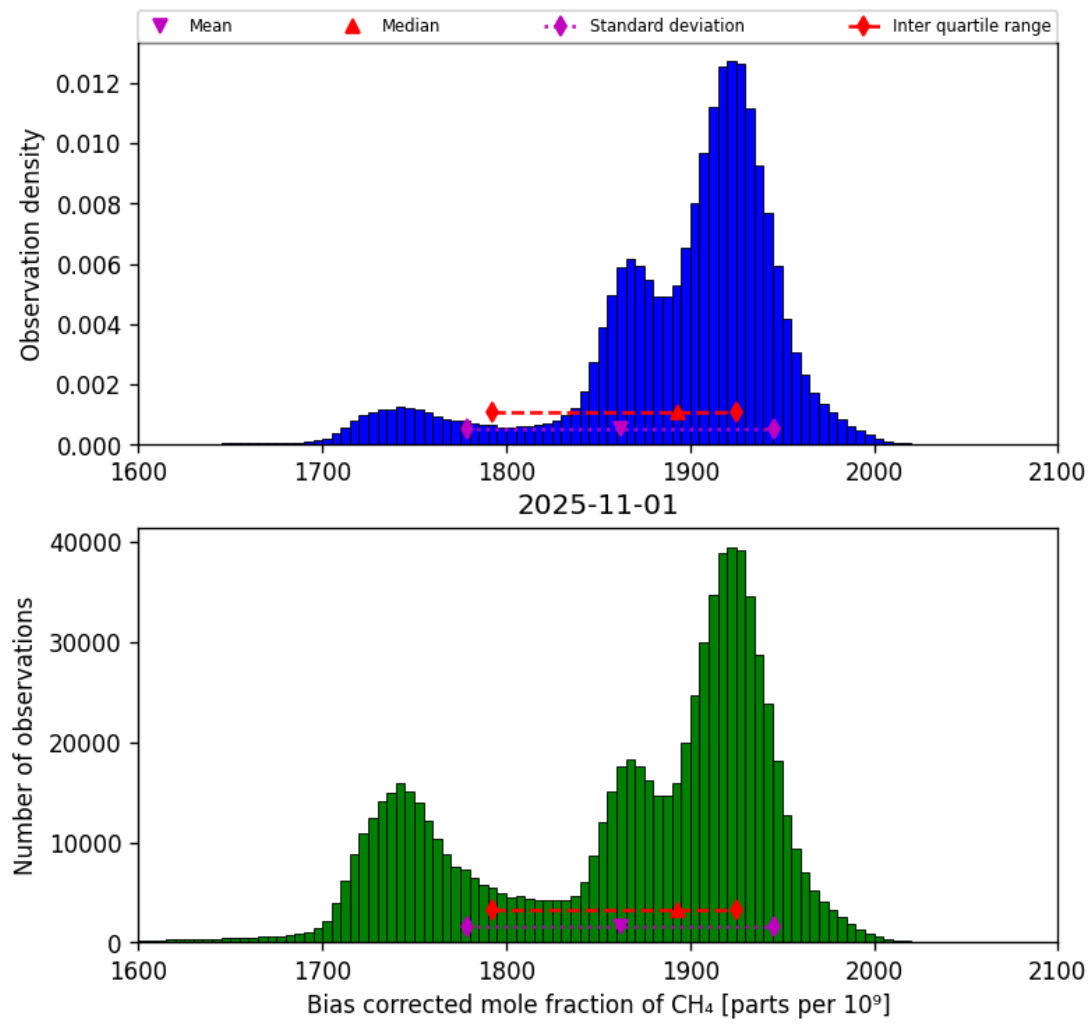
Figure 25: Histogram of “Bias corrected mole fraction of CH 4 ” for 2025-10-31 to 2025-11-02
