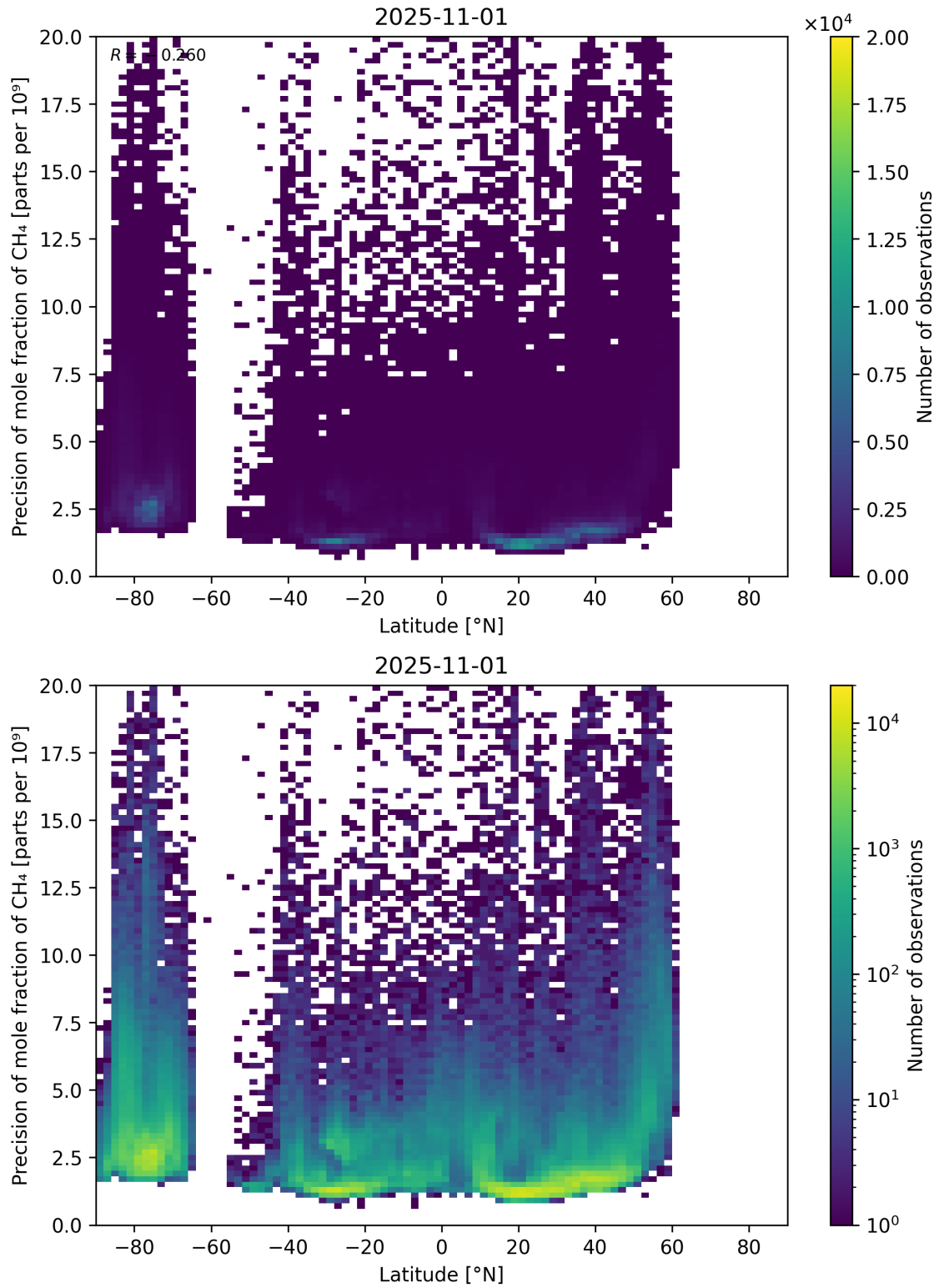
Figure 59: Scatter density plot of “Latitude” against “Precision of mole fraction of CH 4 ” for 2025-10-31 to 2025-11-02.
