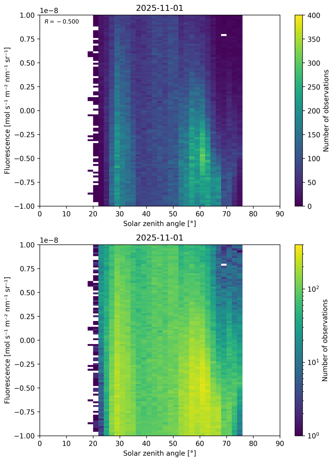
Figure 97: Scatter density plot of “Solar zenith angle” against “Fluorescence” for 2025-10-31 to 2025-11-02.
