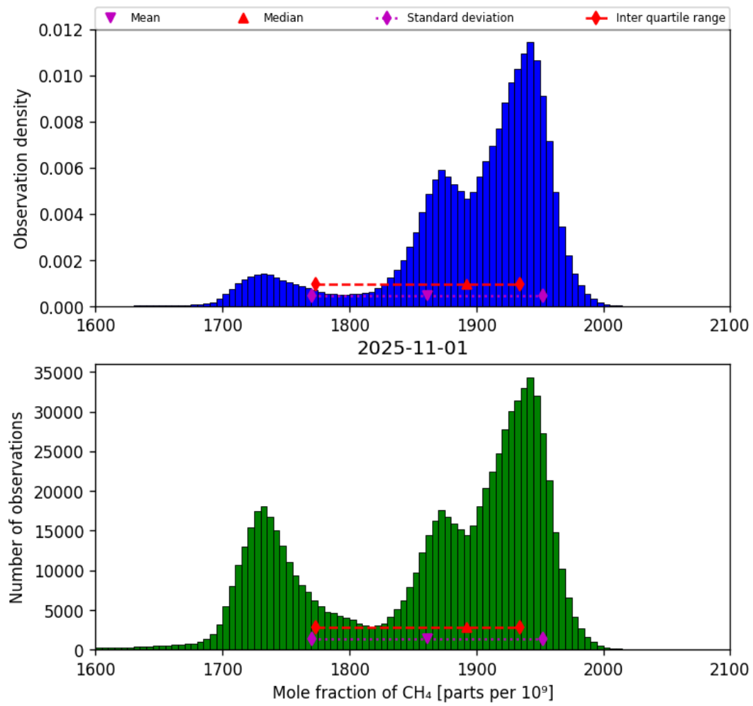
Figure 23: Histogram of “Mole fraction of CH 4 ” for 2025-10-31 to 2025-11-02
