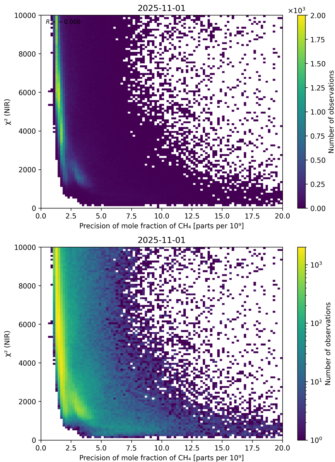
Figure 78: Scatter density plot of “Precision of mole fraction of CH 4 ” against “ \chi^2 (NIR)” for 2025-10-31 to 2025-11-02.
