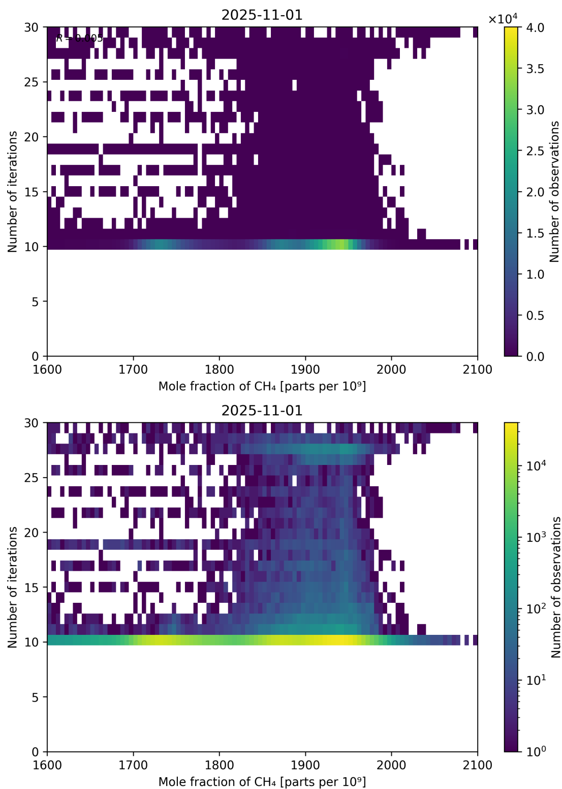
Figure 76: Scatter density plot of “Mole fraction of CH 4 ” against “Number of iterations” for 2025-10-31 to 2025-11-02.
