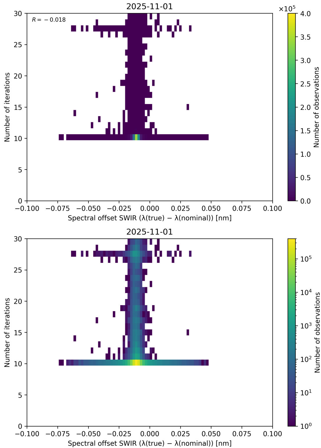
Figure 121: Scatter density plot of “Spectral offset SWIR ( \lambda_{\text{true}} - \lambda_{\text{nominal}} )” against “Number of iterations” for 2025-10-31 to 2025-11-02.
