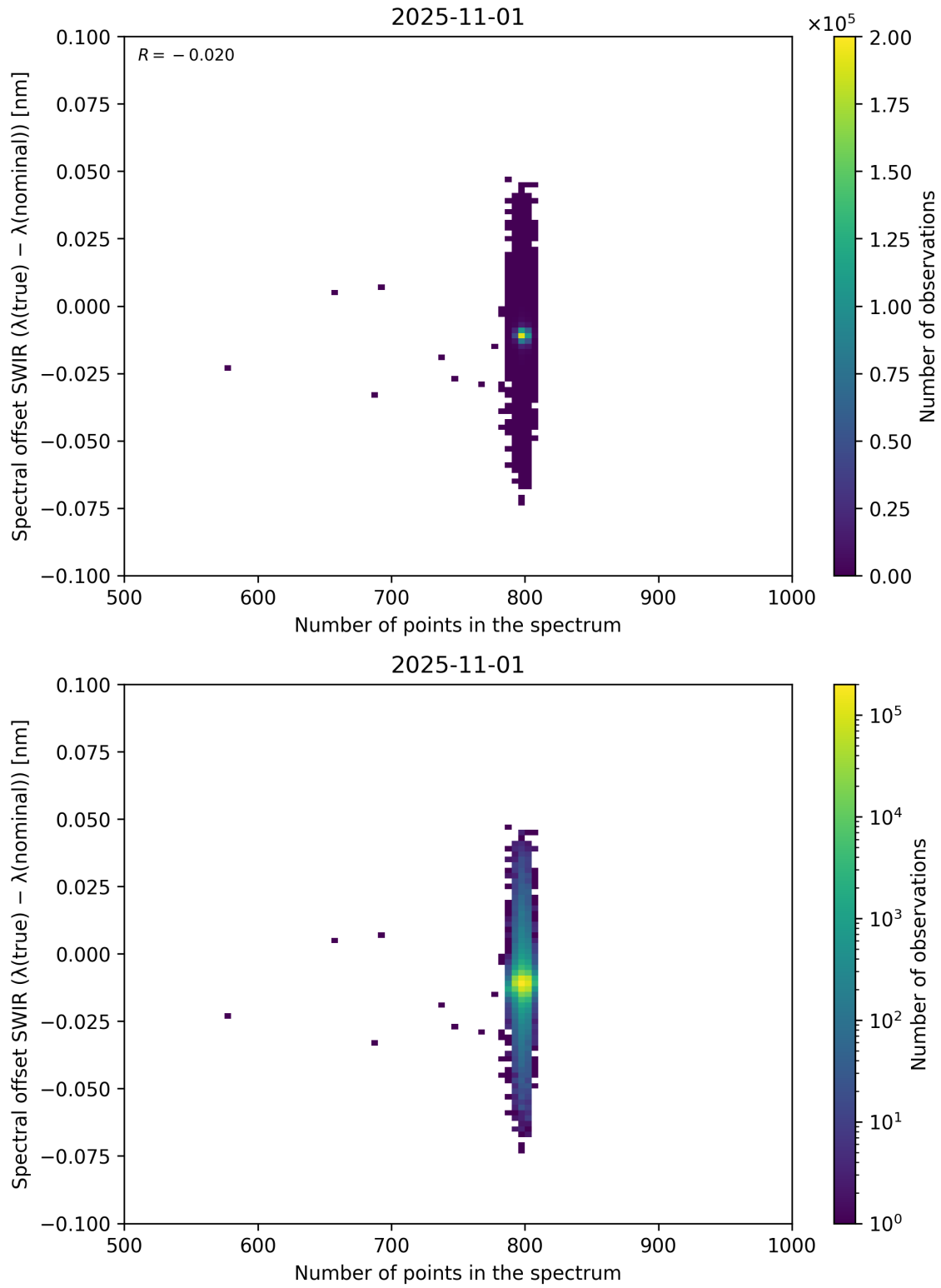
Figure 93: Scatter density plot of “Number of points in the spectrum” against “Spectral offset SWIR ( \lambda_{\text{true}} - \lambda_{\text{nominal}} )” for 2025-10-31 to 2025-11-02.
