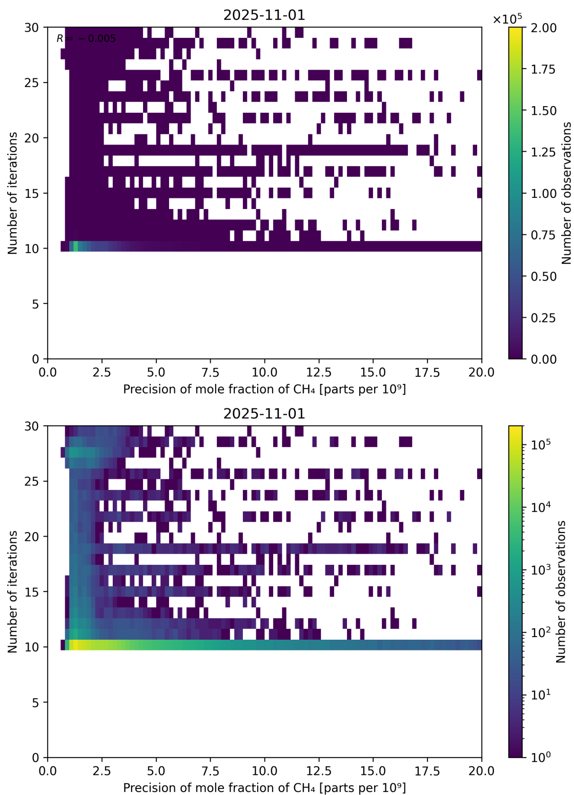
Figure 83: Scatter density plot of “Precision of mole fraction of CH 4 ” against “Number of iterations” for 2025-10-31 to 2025-11-02.
