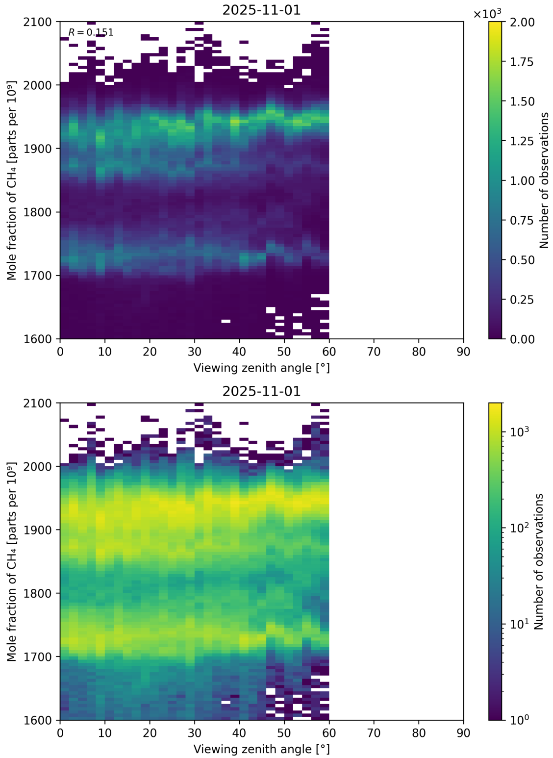
Figure 110: Scatter density plot of “Viewing zenith angle” against “Mole fraction of CH 4 ” for 2025-10-31 to 2025-11-02.
