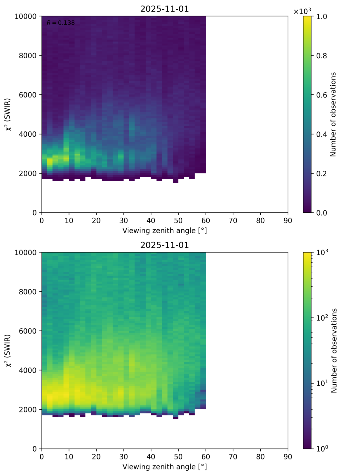
Figure 106: Scatter density plot of “Viewing zenith angle” against “ \chi^2 (SWIR)” for 2025-10-31 to 2025-11-02.
