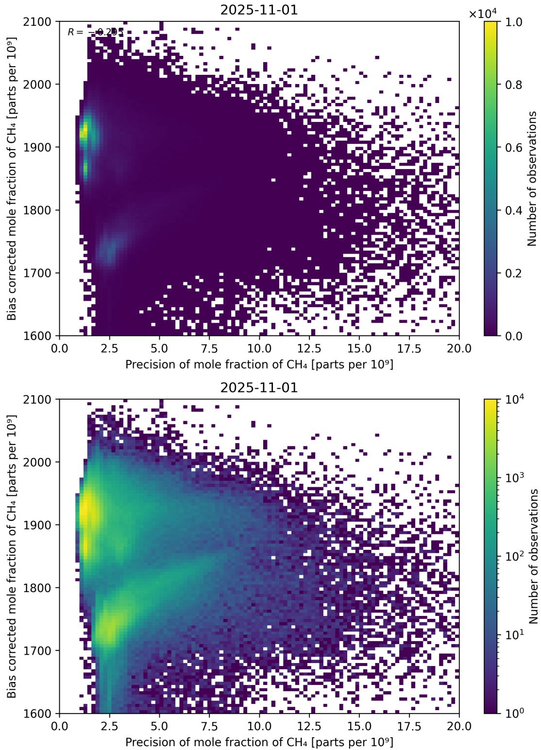
Figure 82: Scatter density plot of “Precision of mole fraction of \text{CH}_4 ” against “Bias corrected mole fraction of \text{CH}_4 ” for 2025-10-31 to 2025-11-02.
