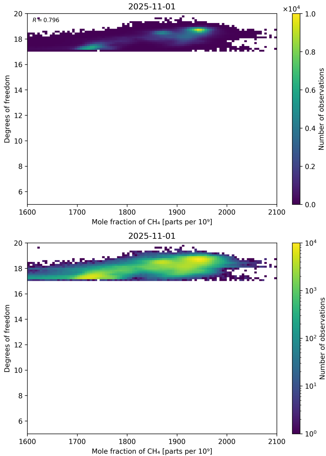
Figure 72: Scatter density plot of “Mole fraction of CH 4 ” against “Degrees of freedom” for 2025-10-31 to 2025-11-02.
