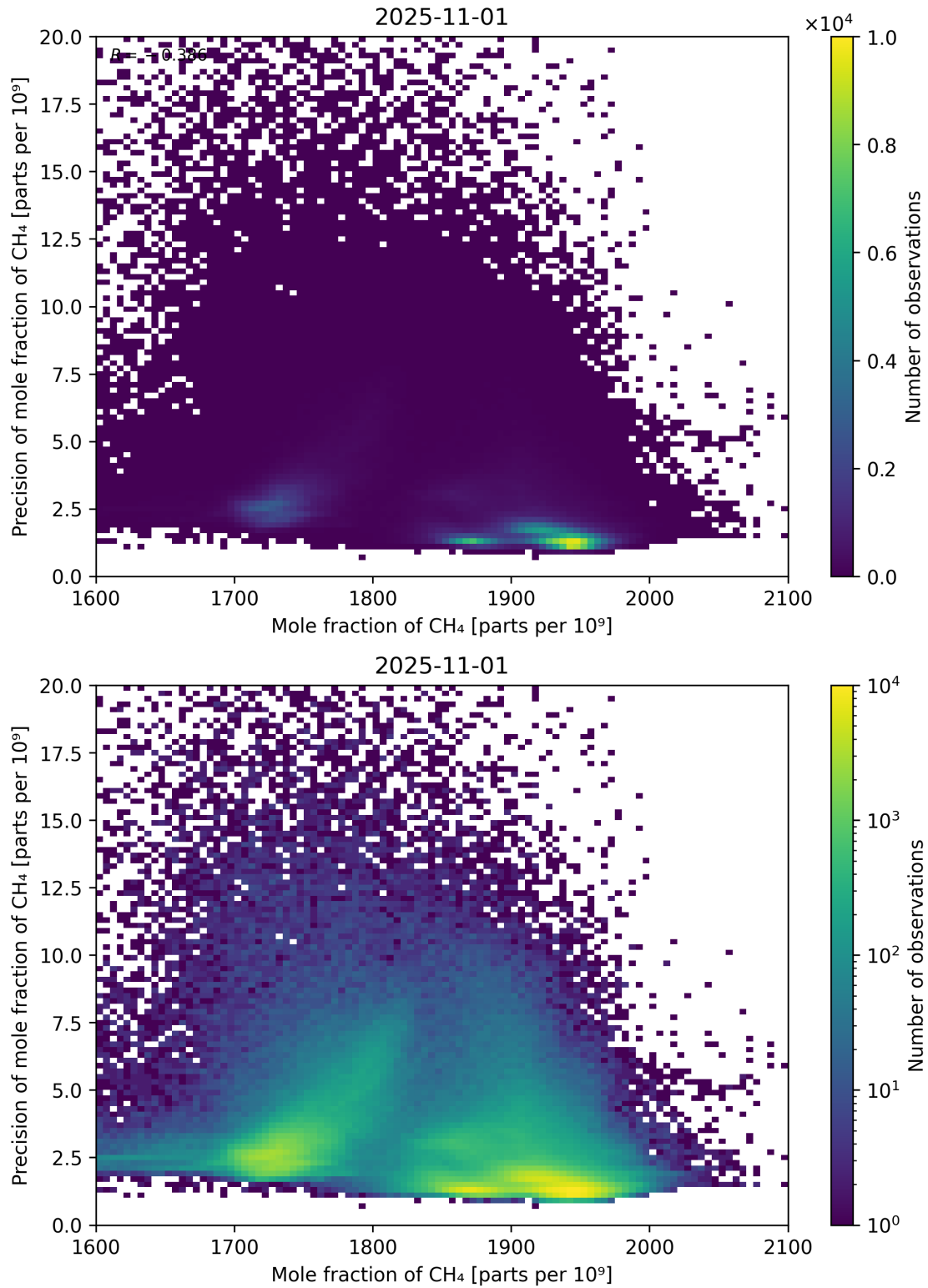
Figure 75: Scatter density plot of “Mole fraction of CH 4 ” against “Precision of mole fraction of CH 4 ” for 2025-10-31 to 2025-11-02.
