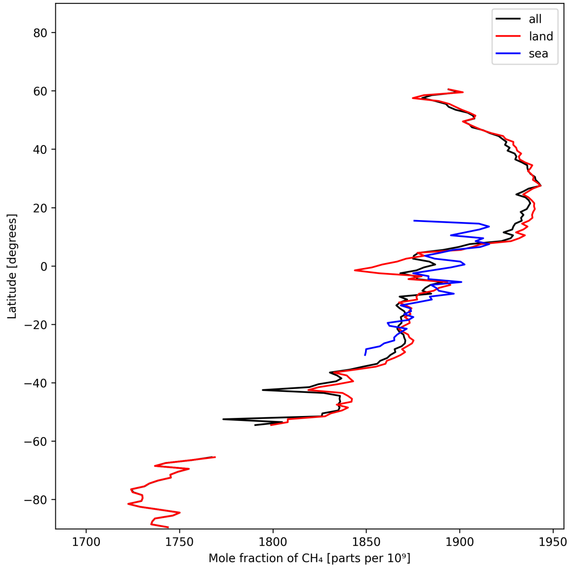
Figure 12: Zonal average of “Mole fraction of CH 4 ” for 2025-10-31 to 2025-11-02.
