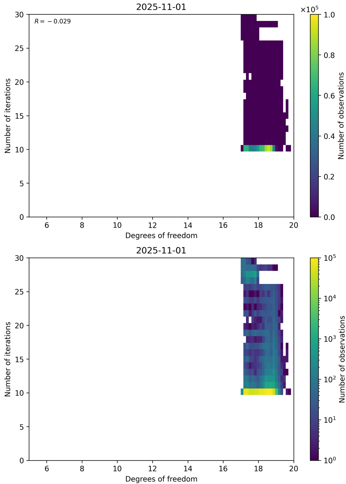
Figure 52: Scatter density plot of “Degrees of freedom” against “Number of iterations” for 2025-10-31 to 2025-11-02.
