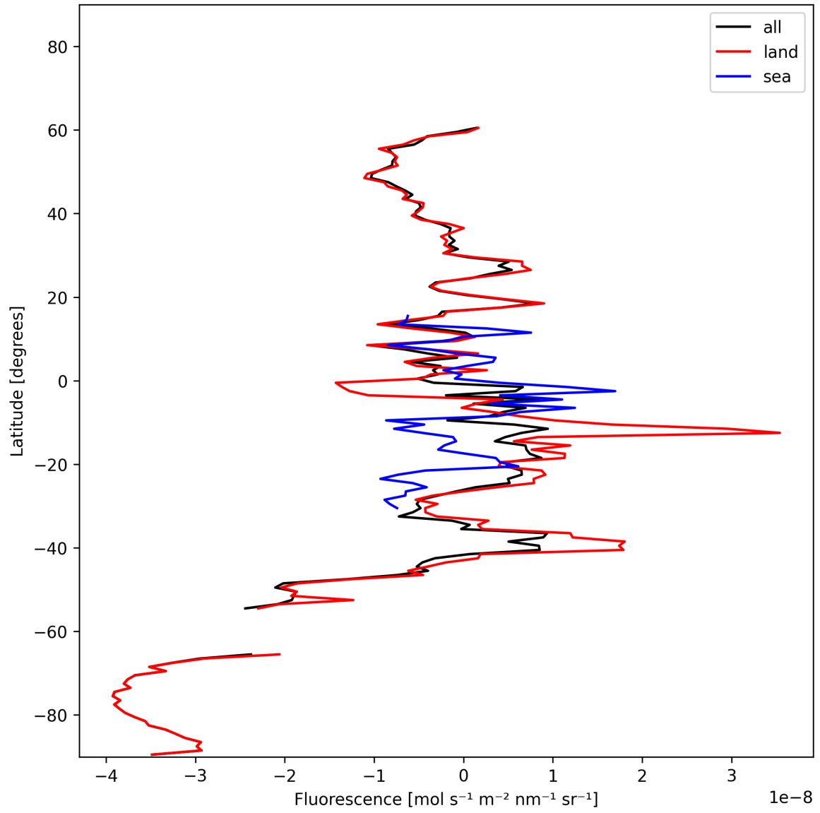
Figure 21: Zonal average of “Fluorescence” for 2025-10-31 to 2025-11-02.
