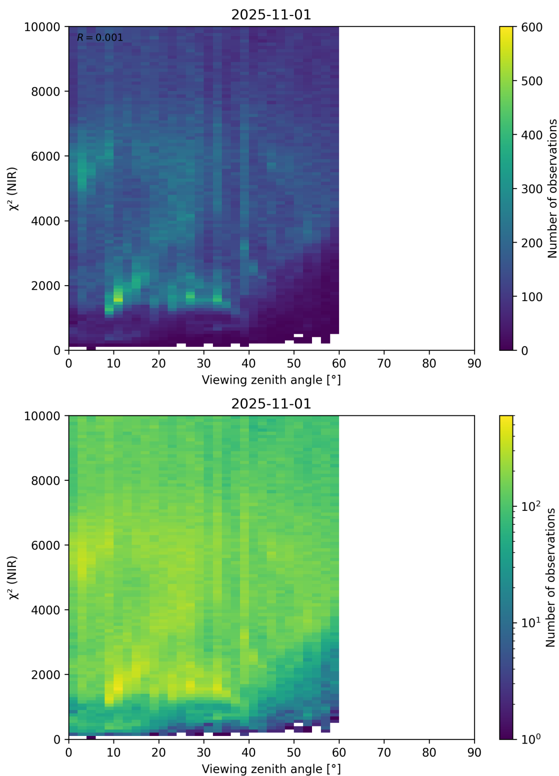
Figure 105: Scatter density plot of “Viewing zenith angle” against “ \chi^2 (NIR)” for 2025-10-31 to 2025-11-02.
