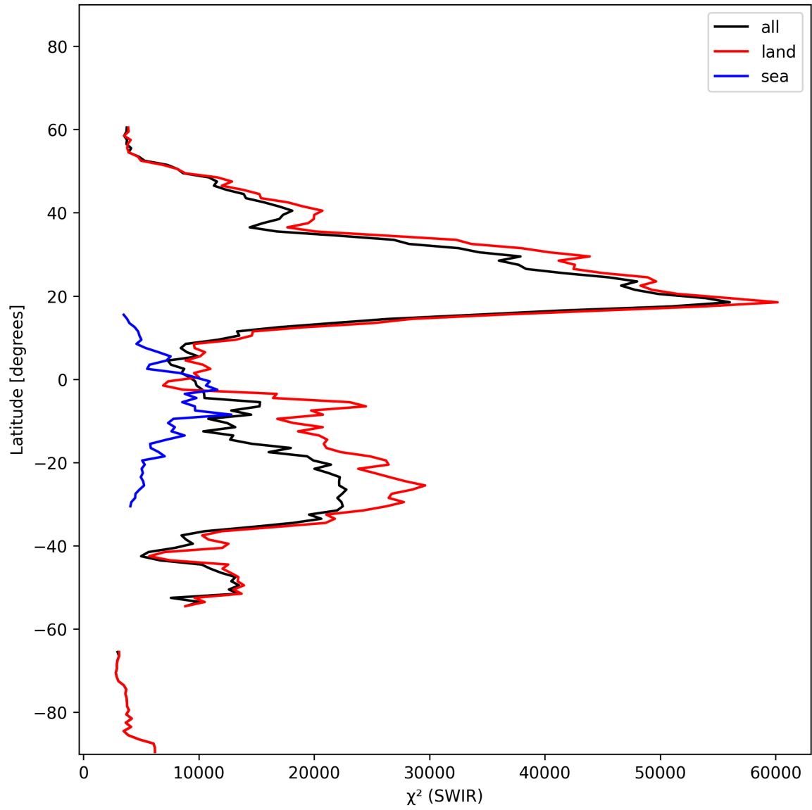
Figure 17: Zonal average of “ \chi^2 (SWIR)” for 2025-10-31 to 2025-11-02.
