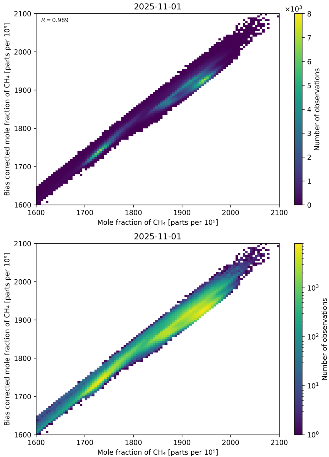
Figure 74: Scatter density plot of “Mole fraction of CH 4 ” against “Bias corrected mole fraction of CH 4 ” for 2025-10-31 to 2025-11-02.
