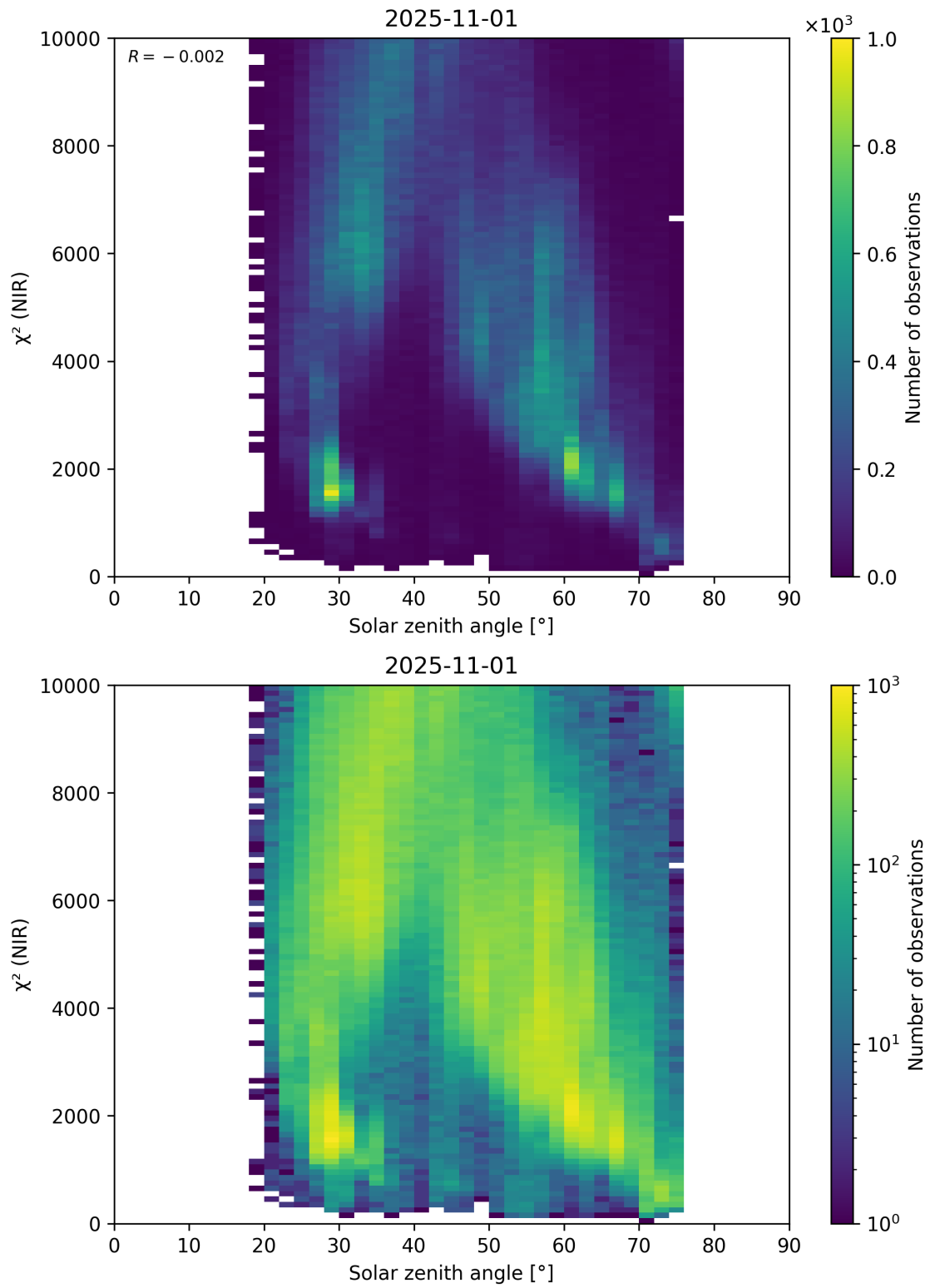
Figure 94: Scatter density plot of “Solar zenith angle” against “ \chi^2 (NIR)” for 2025-10-31 to 2025-11-02.
