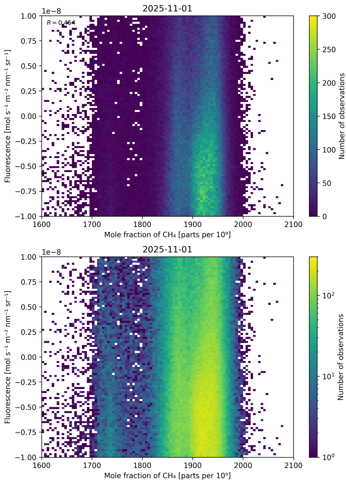
Figure 73: Scatter density plot of “Mole fraction of \text{CH}_4 ” against “Fluorescence” for 2025-10-31 to 2025-11-02.
