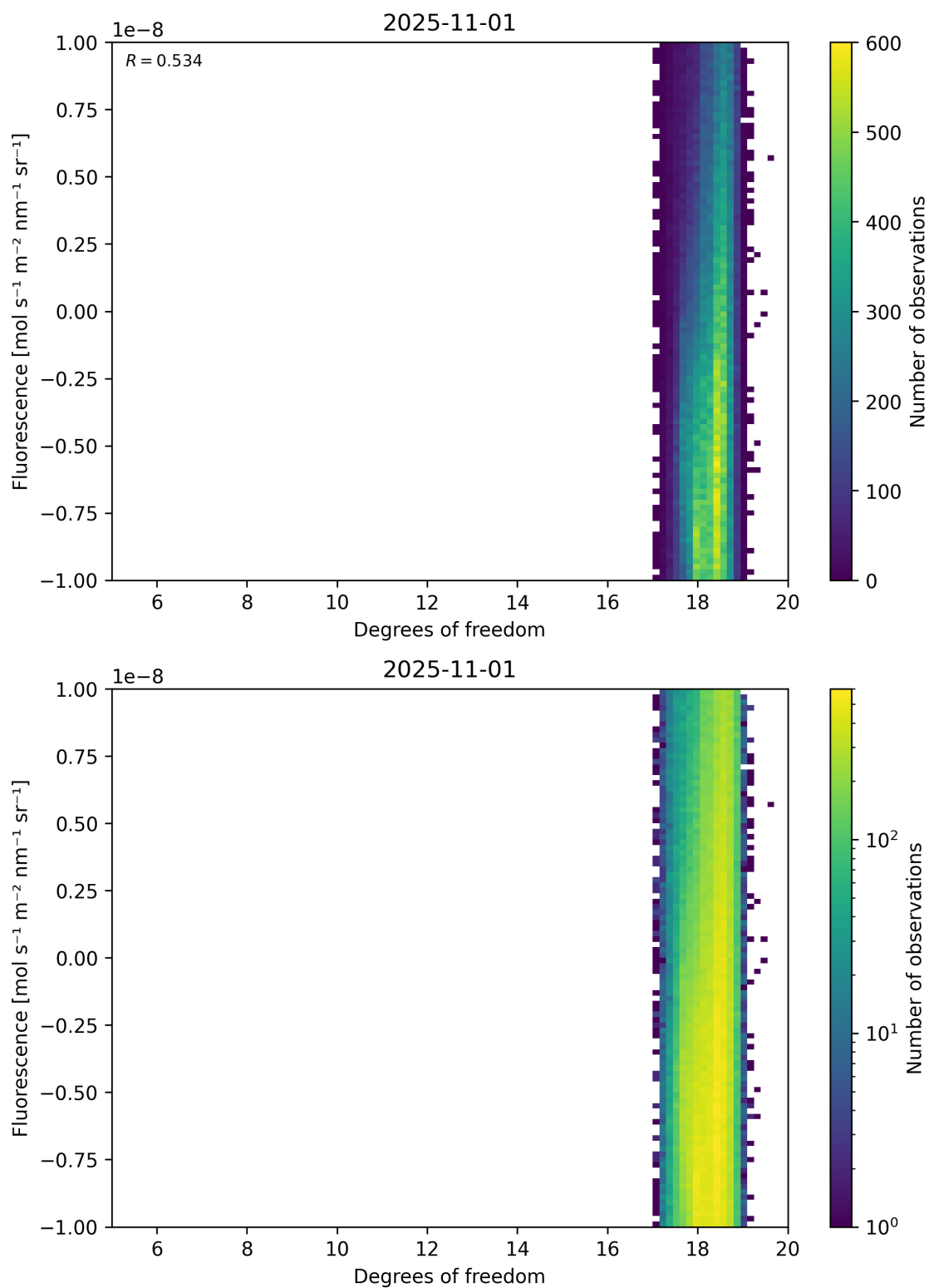
Figure 51: Scatter density plot of “Degrees of freedom” against “Fluorescence” for 2025-10-31 to 2025-11-02.
