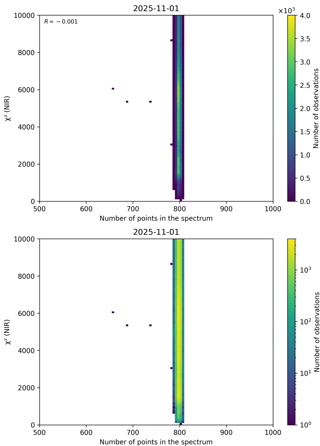
Figure 88: Scatter density plot of “Number of points in the spectrum” against “ \chi^2 (NIR)” for 2025-10-31 to 2025-11-02.
