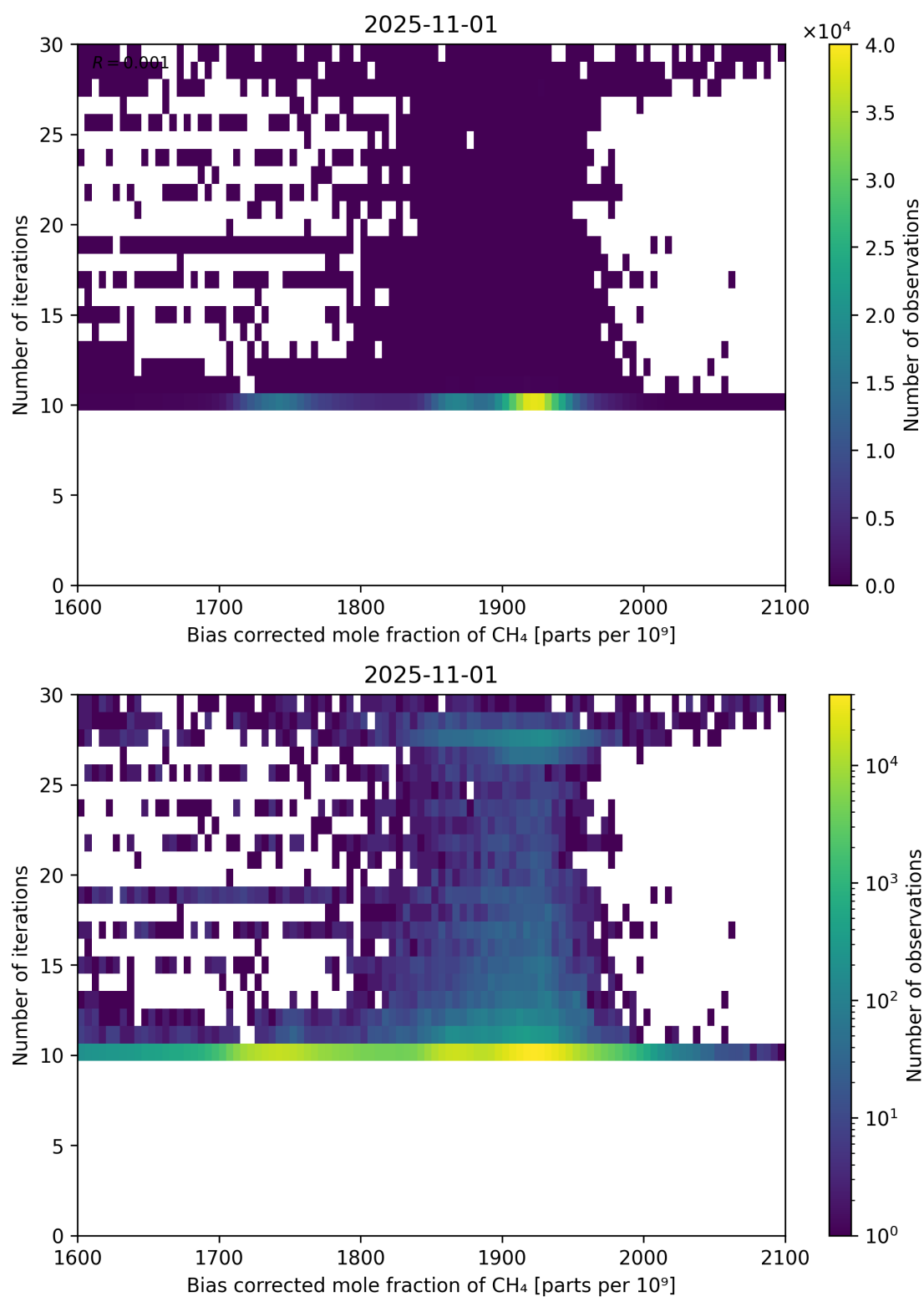
Figure 67: Scatter density plot of “Bias corrected mole fraction of \text{CH}_4 ” against “Number of iterations” for 2025-10-31 to 2025-11-02.
