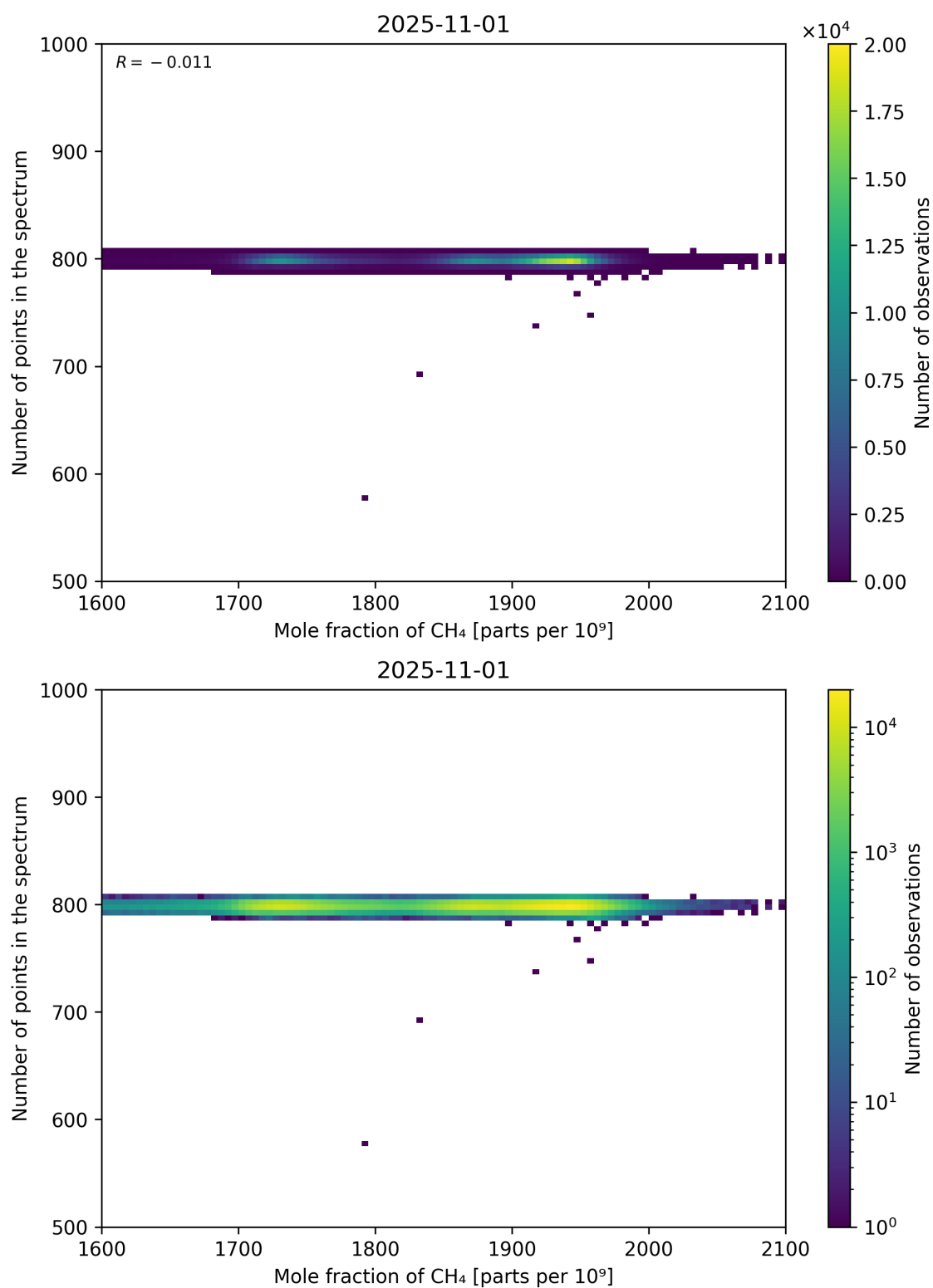
Figure 77: Scatter density plot of “Mole fraction of CH 4 ” against “Number of points in the spectrum” for 2025-10-31 to 2025-11-02.
