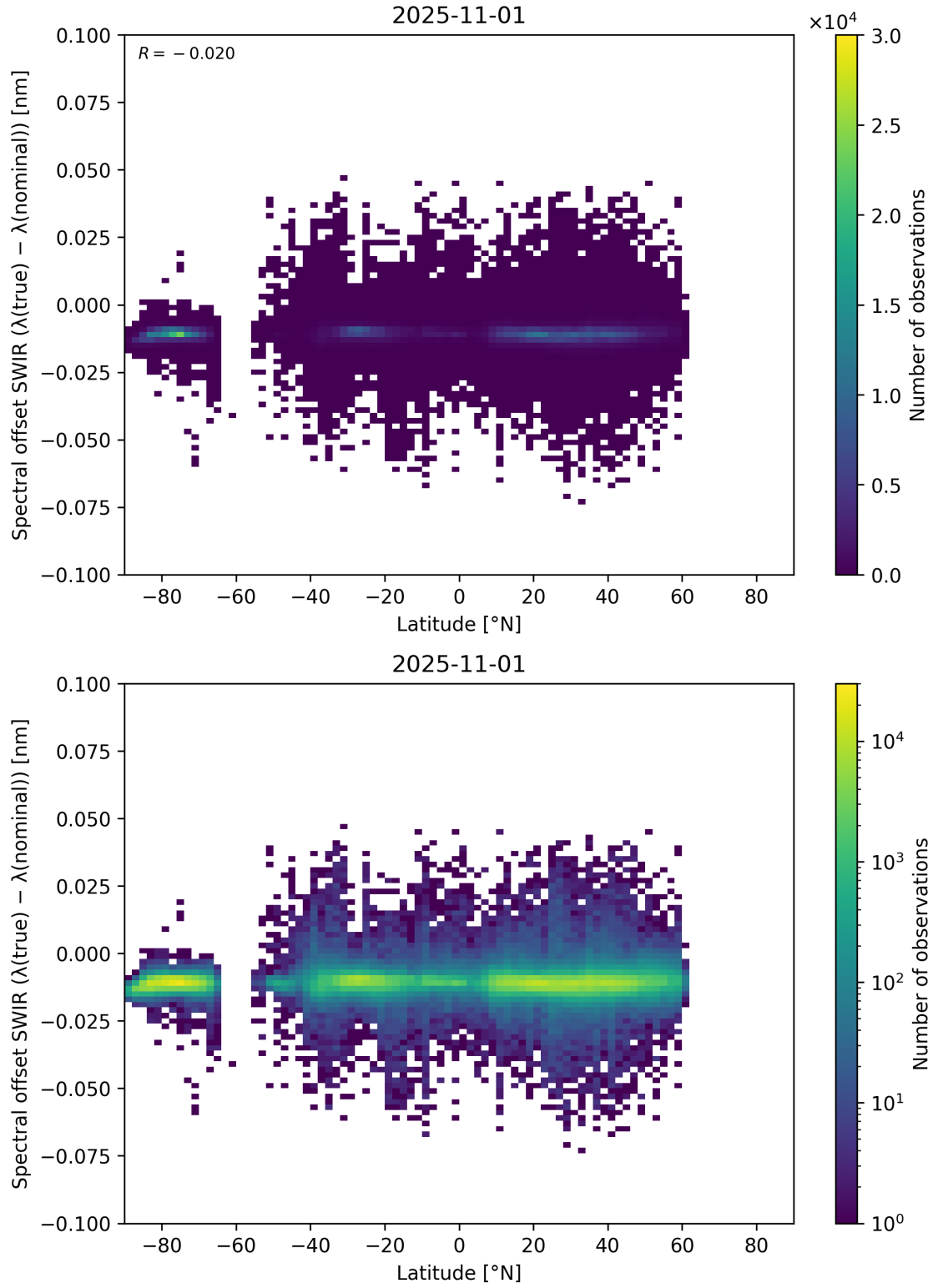
Figure 62: Scatter density plot of “Latitude” against “Spectral offset SWIR ( \lambda_{\text{true}} - \lambda_{\text{nominal}} )” for 2025-10-31 to 2025-11-02.
