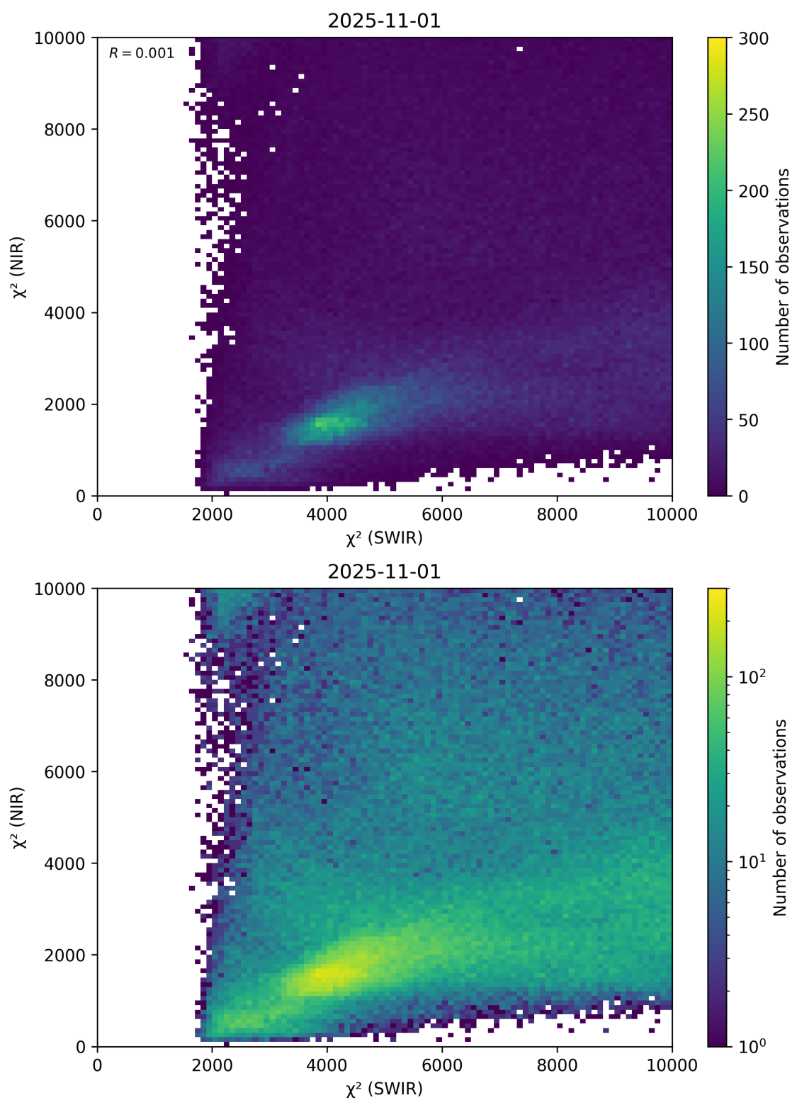
Figure 47: Scatter density plot of “ \chi^2 (SWIR)” against “ \chi^2 (NIR)” for 2025-10-31 to 2025-11-02.
