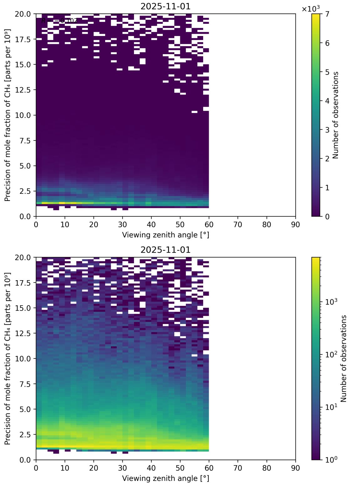
Figure 112: Scatter density plot of “Viewing zenith angle” against “Precision of mole fraction of CH 4 ” for 2025-10-31 to 2025-11-02.
