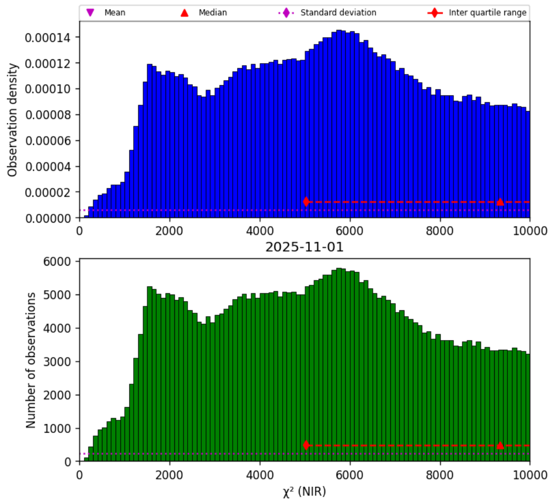
Figure 29: Histogram of “ \chi^2 (NIR)” for 2025-10-31 to 2025-11-02
