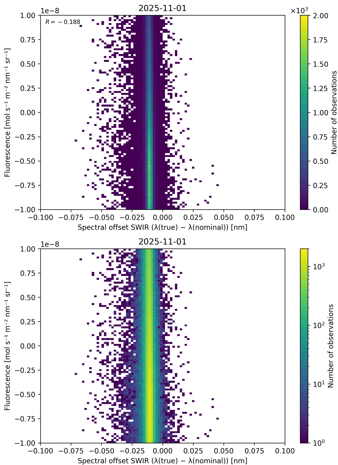
Figure 120: Scatter density plot of “Spectral offset SWIR ( \lambda_{\text{true}} - \lambda_{\text{nominal}} )” against “Fluorescence” for 2025-10-31 to 2025-11-02.
