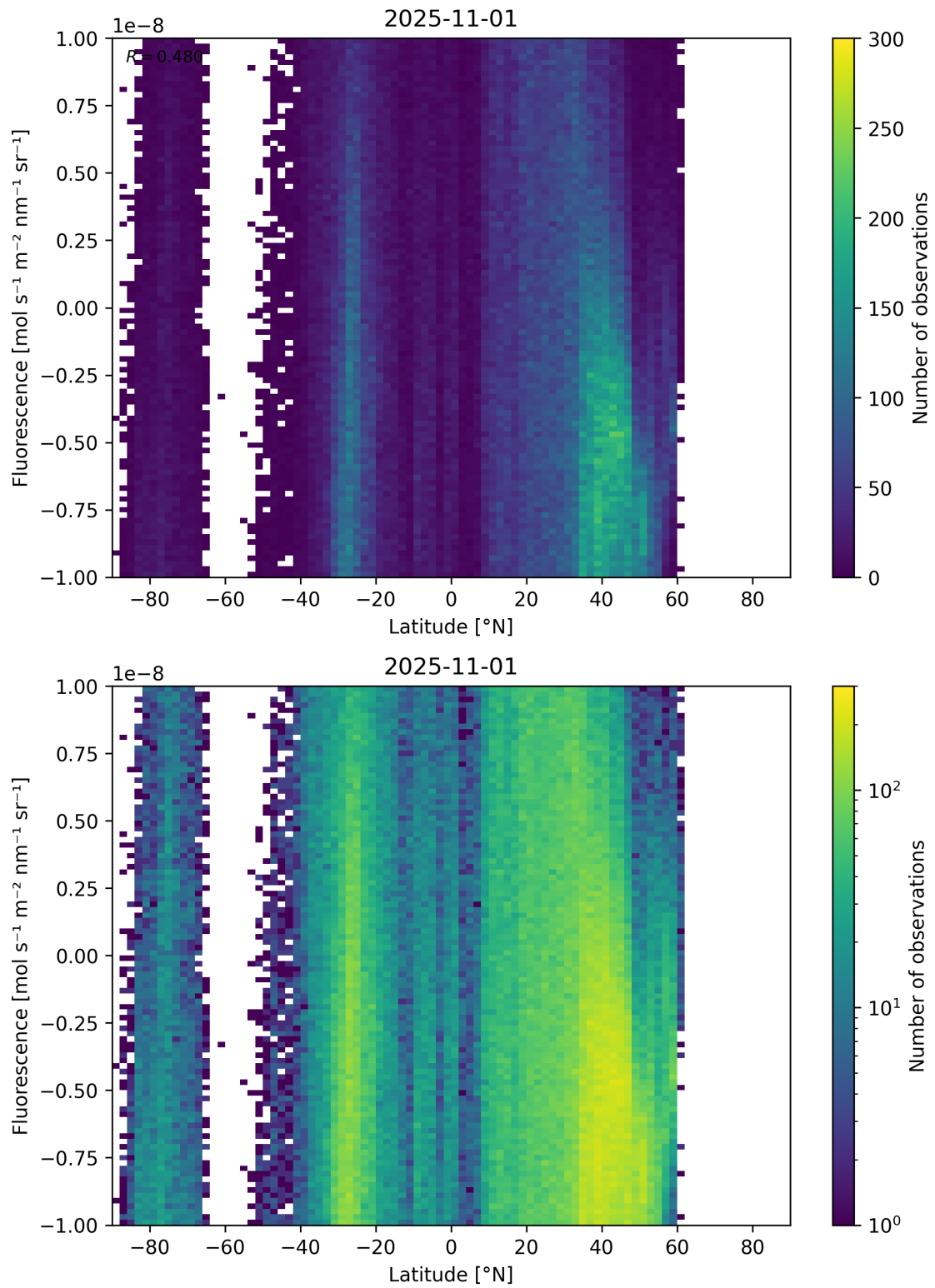
Figure 56: Scatter density plot of “Latitude” against “Fluorescence” for 2025-10-31 to 2025-11-02.
