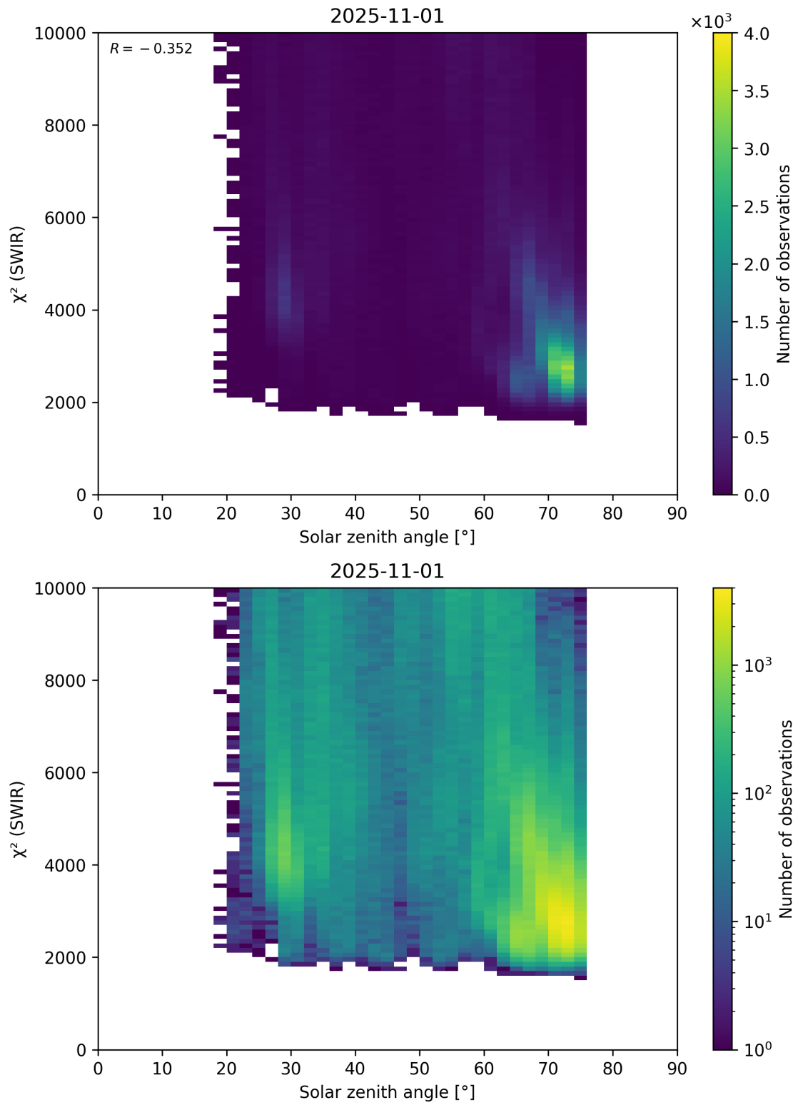
Figure 95: Scatter density plot of “Solar zenith angle” against “ \chi^2 (SWIR)” for 2025-10-31 to 2025-11-02.
