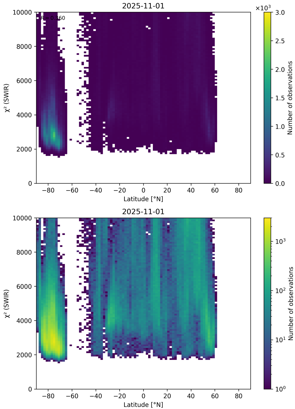
Figure 54: Scatter density plot of “Latitude” against “ \chi^2 (SWIR)” for 2025-10-31 to 2025-11-02.
