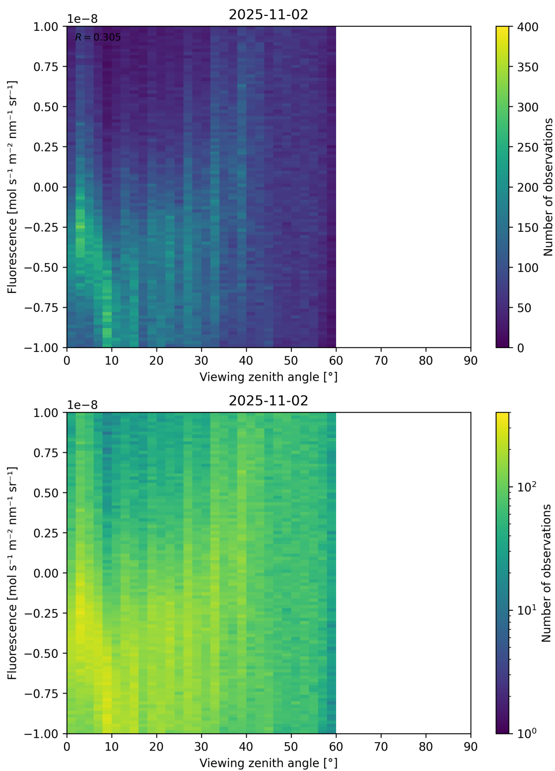
Figure 108: Scatter density plot of “Viewing zenith angle” against “Fluorescence” for 2025-11-02 to 2025-11-03.
