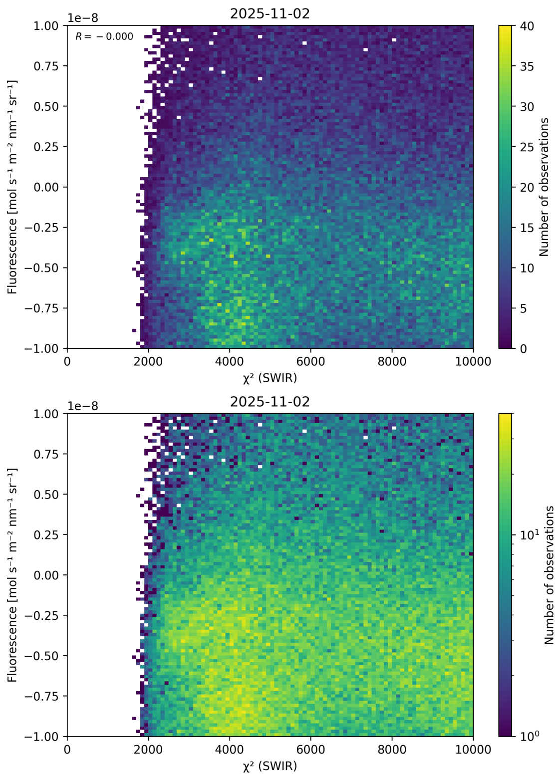
Figure 49: Scatter density plot of “ \chi^2 (SWIR)” against “Fluorescence” for 2025-11-02 to 2025-11-03.
