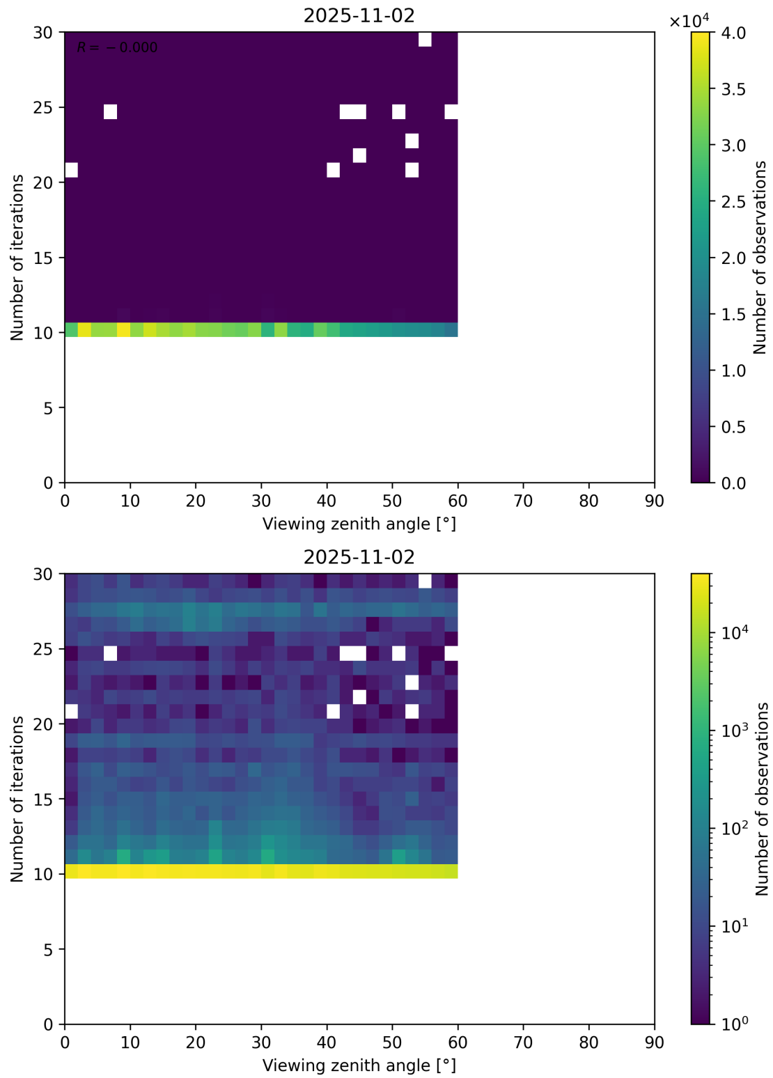
Figure 113: Scatter density plot of “Viewing zenith angle” against “Number of iterations” for 2025-11-02 to 2025-11-03.
