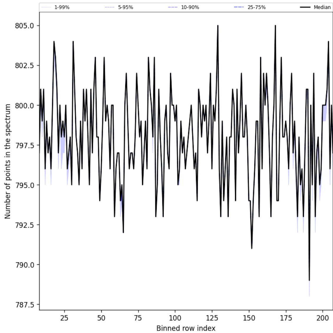
Figure 37: Along track statistics of “Number of points in the spectrum” for 2025-11-02 to 2025-11-03
