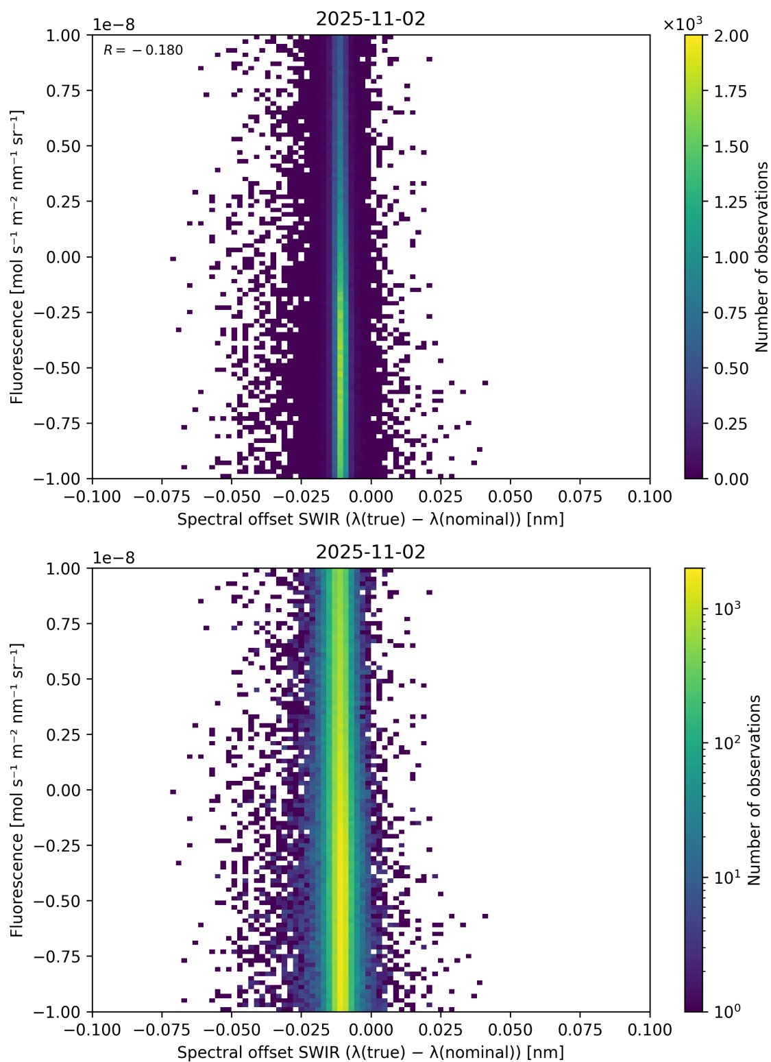
Figure 120: Scatter density plot of “Spectral offset SWIR ( \lambda_{\text{true}} - \lambda_{\text{nominal}} )” against “Fluorescence” for 2025-11-02 to 2025-11-03.
