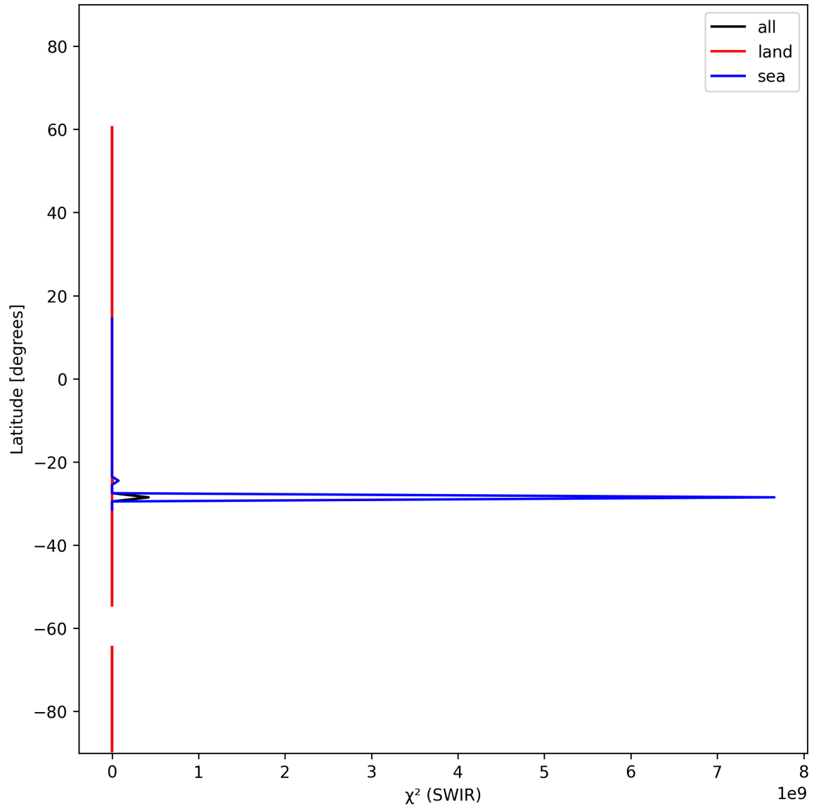
Figure 17: Zonal average of “ \chi^2 (SWIR)” for 2025-11-02 to 2025-11-03.
