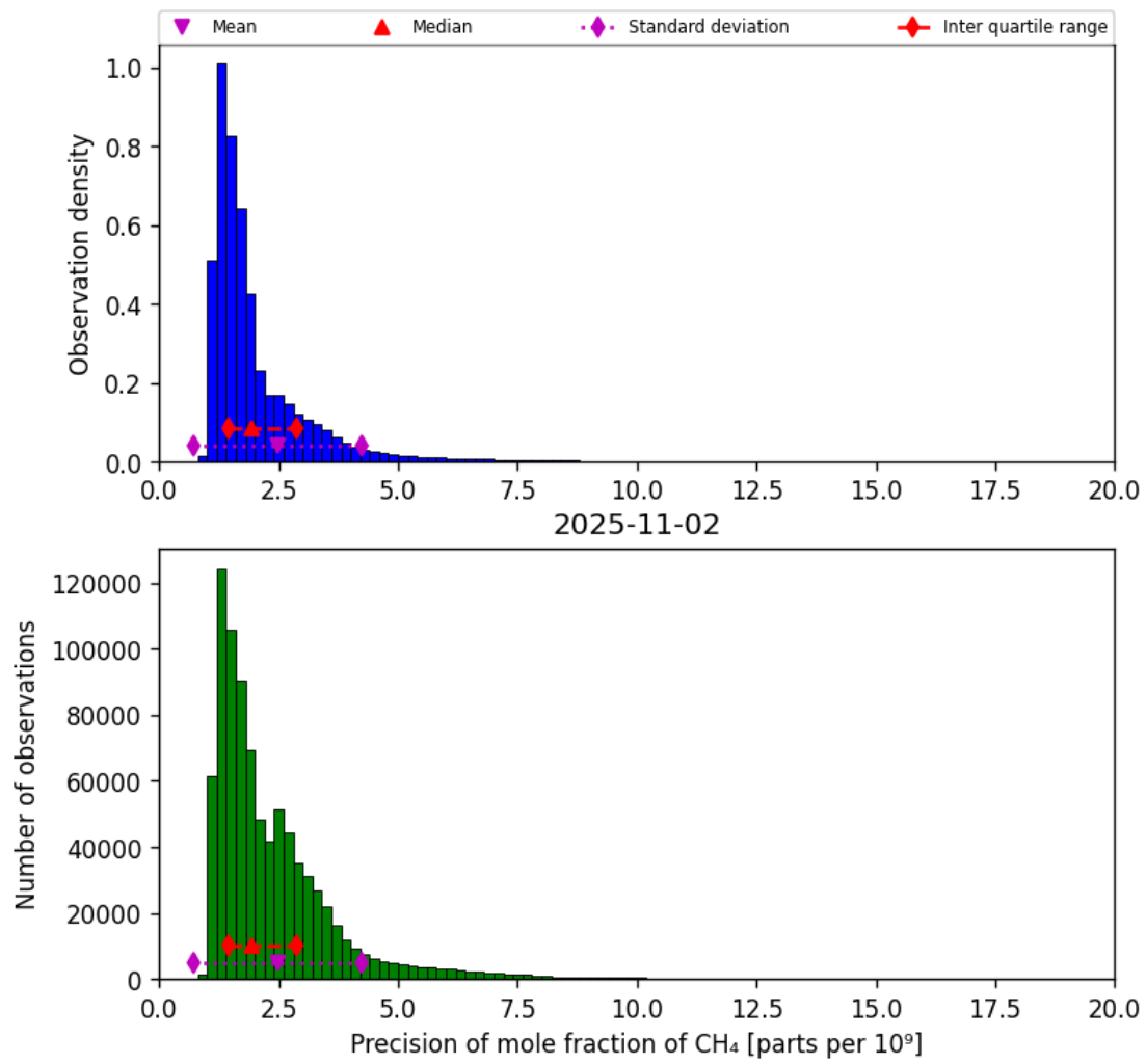
Figure 24: Histogram of “Precision of mole fraction of CH 4 ” for 2025-11-02 to 2025-11-03
