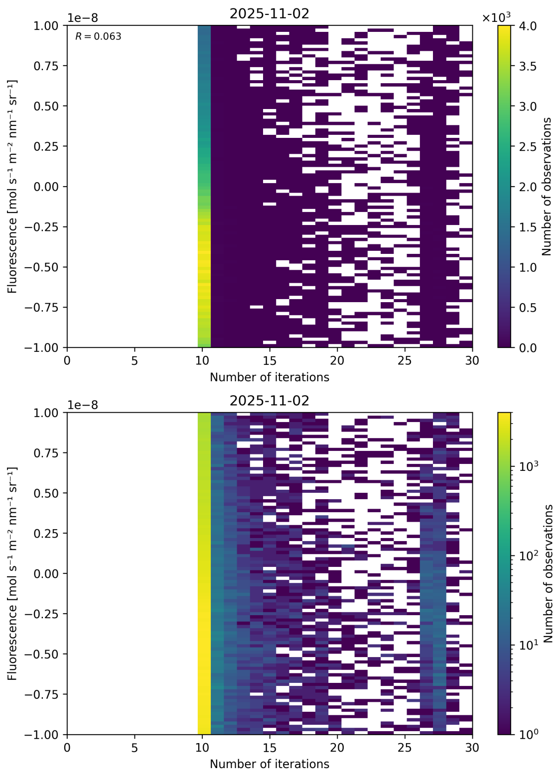
Figure 87: Scatter density plot of “Number of iterations” against “Fluorescence” for 2025-11-02 to 2025-11-03.
