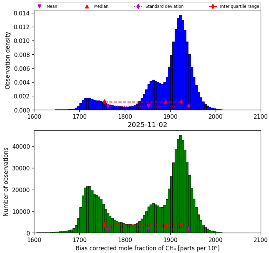
Figure 25: Histogram of “Bias corrected mole fraction of CH 4 ” for 2025-11-02 to 2025-11-03
