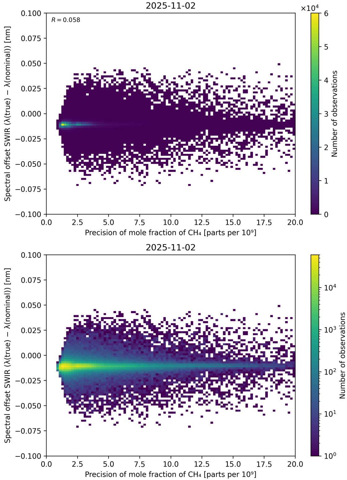
Figure 85: Scatter density plot of “Precision of mole fraction of \text{CH}_4 ” against “Spectral offset SWIR ( \lambda_{\text{true}} - \lambda_{\text{nominal}} )” for 2025-11-02 to 2025-11-03.
