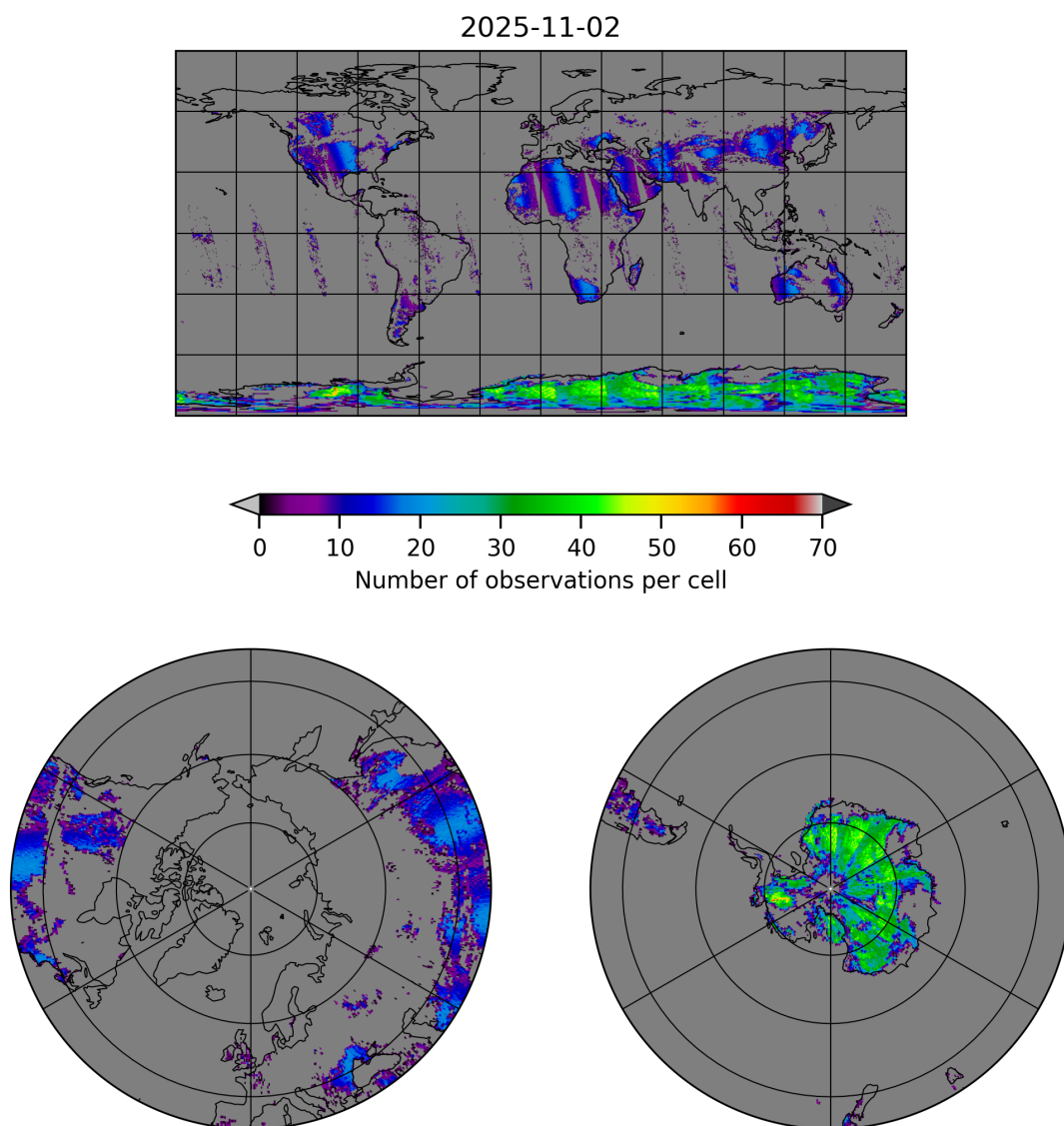
Figure 10: Map of the number of observations for 2025-11-02 to 2025-11-03
