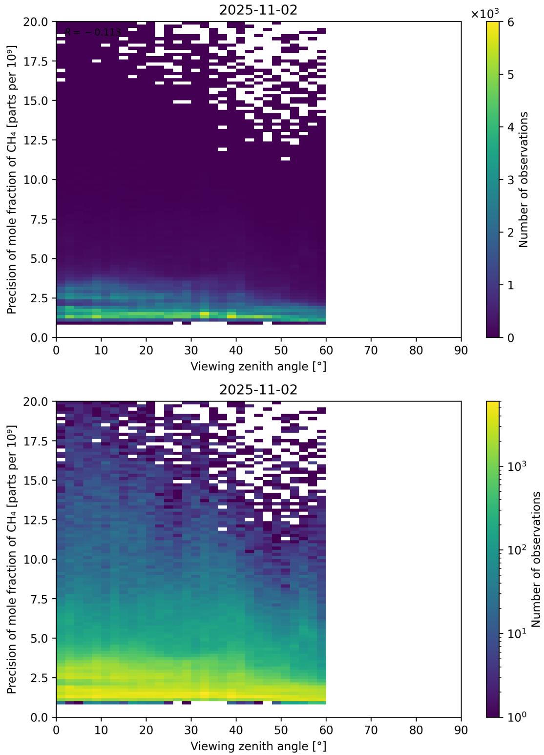
Figure 112: Scatter density plot of “Viewing zenith angle” against “Precision of mole fraction of CH 4 ” for 2025-11-02 to 2025-11-03.
