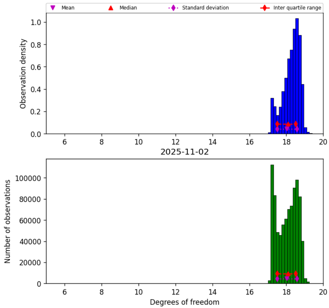
Figure 30: Histogram of “Degrees of freedom” for 2025-11-02 to 2025-11-03
