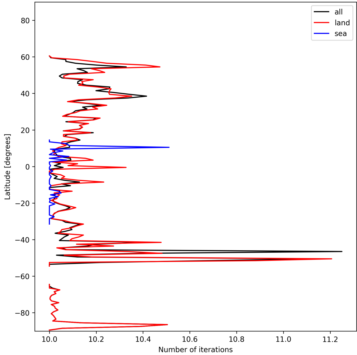
Figure 20: Zonal average of “Number of iterations” for 2025-11-02 to 2025-11-03.
