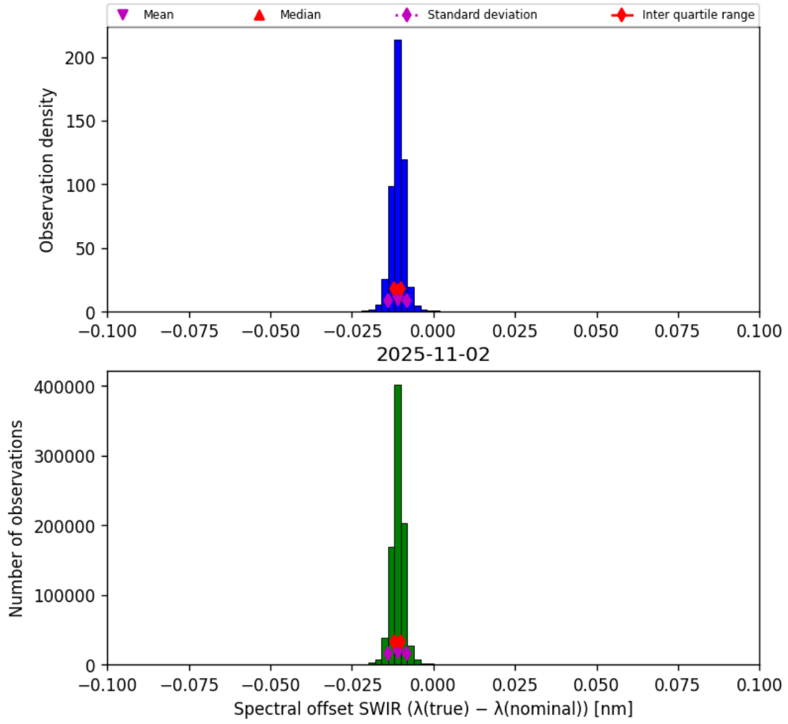
Figure 27: Histogram of “Spectral offset SWIR ( \lambda_{\text{true}} - \lambda_{\text{nominal}} )” for 2025-11-02 to 2025-11-03
