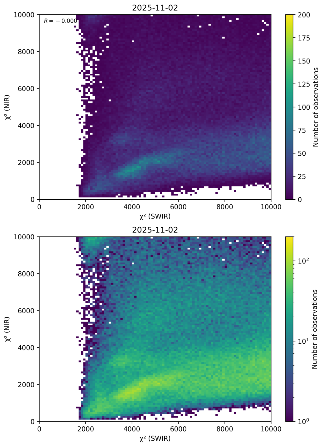
Figure 47: Scatter density plot of “ \chi^2 (SWIR)” against “ \chi^2 (NIR)” for 2025-11-02 to 2025-11-03.
