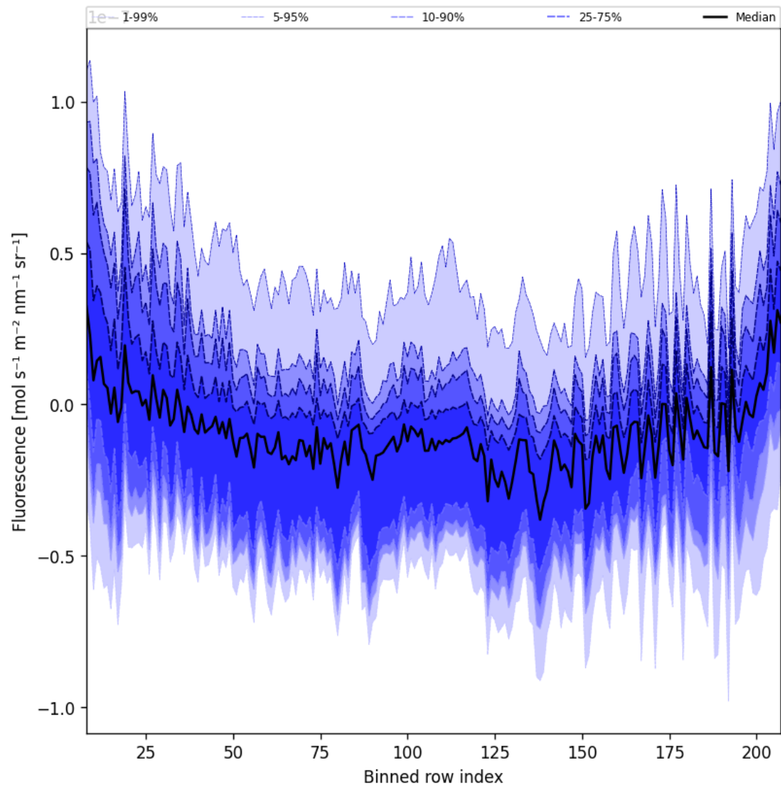
Figure 43: Along track statistics of “Fluorescence” for 2025-11-02 to 2025-11-03
