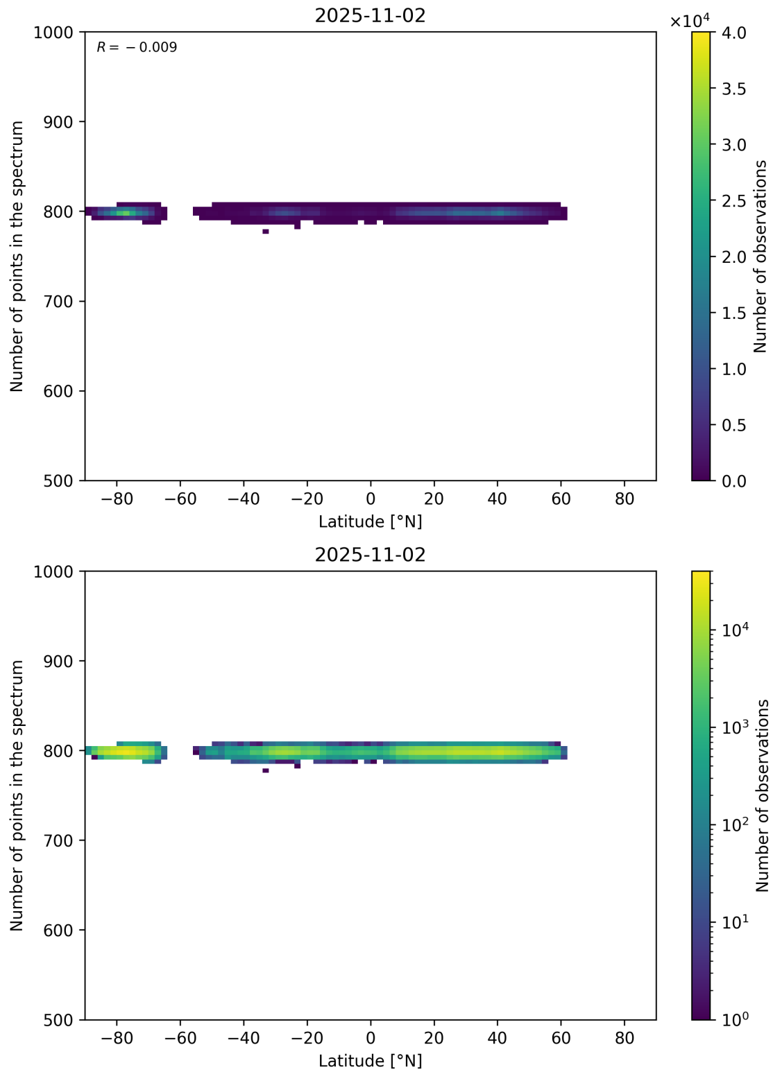
Figure 61: Scatter density plot of “Latitude” against “Number of points in the spectrum” for 2025-11-02 to 2025-11-03.
