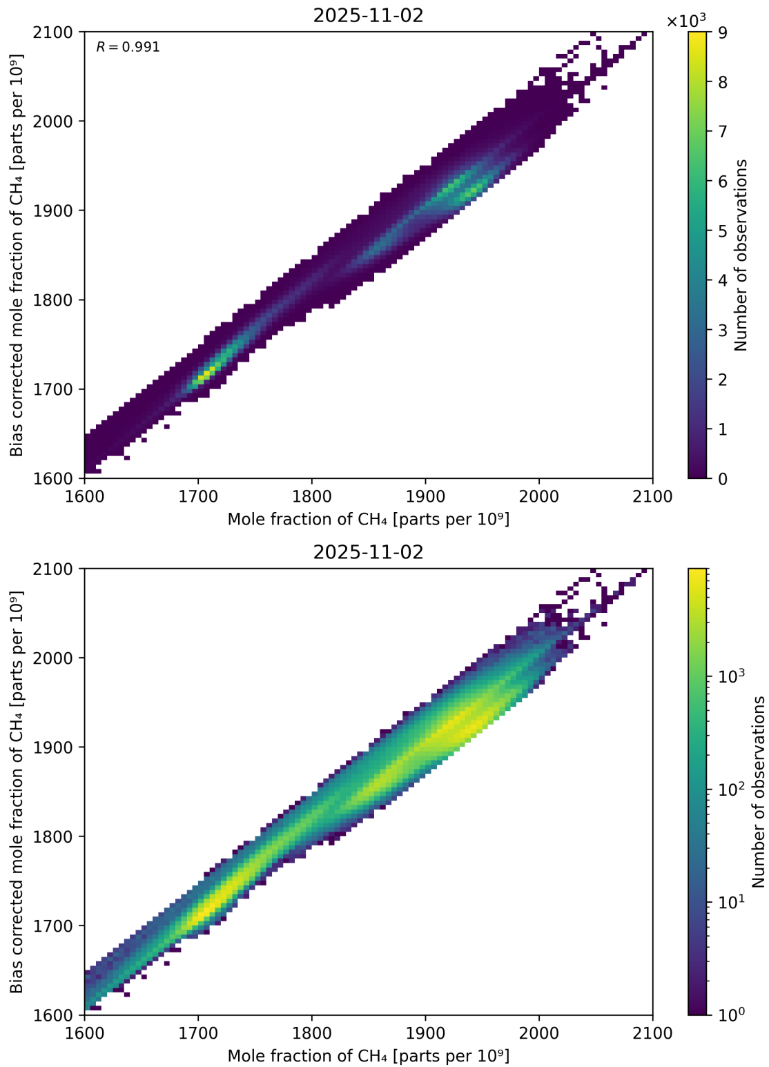
Figure 74: Scatter density plot of “Mole fraction of CH 4 ” against “Bias corrected mole fraction of CH 4 ” for 2025-11-02 to 2025-11-03.
