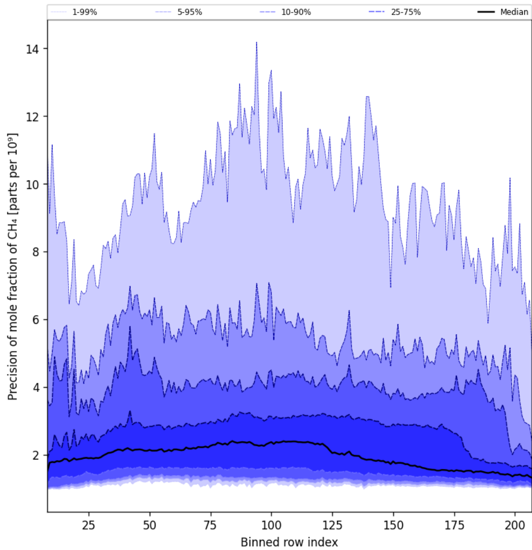
Figure 35: Along track statistics of “Precision of mole fraction of CH 4 ” for 2025-11-02 to 2025-11-03
