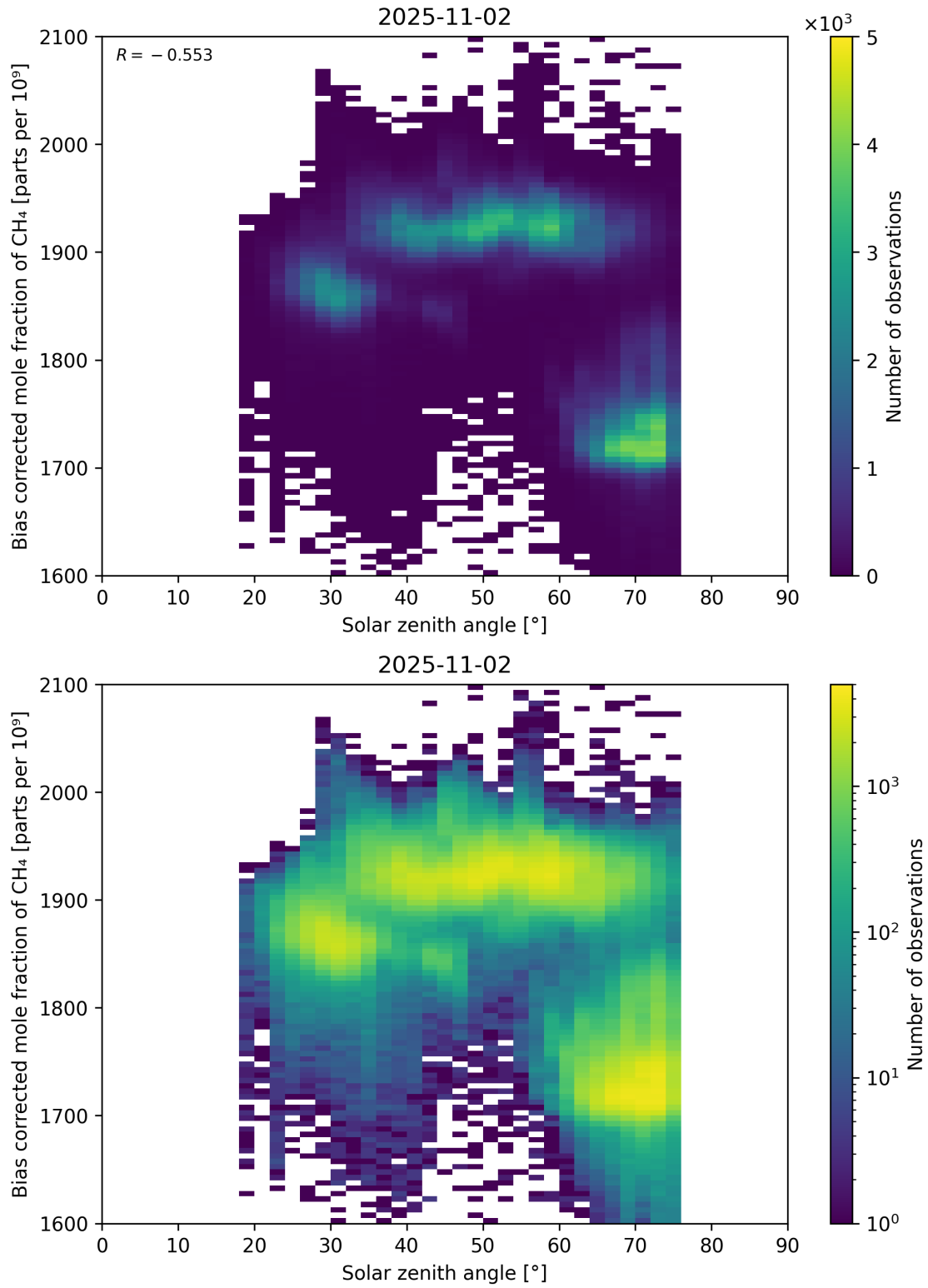
Figure 100: Scatter density plot of “Solar zenith angle” against “Bias corrected mole fraction of CH 4 ” for 2025-11-02 to 2025-11-03.
