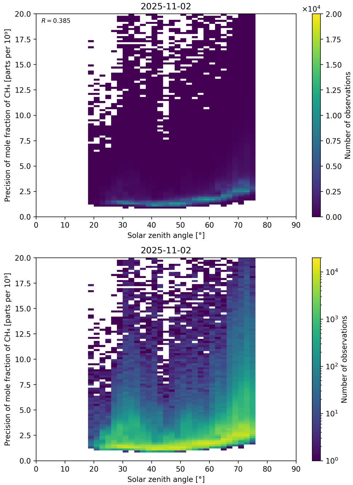
Figure 101: Scatter density plot of “Solar zenith angle” against “Precision of mole fraction of CH 4 ” for 2025-11-02 to 2025-11-03.
