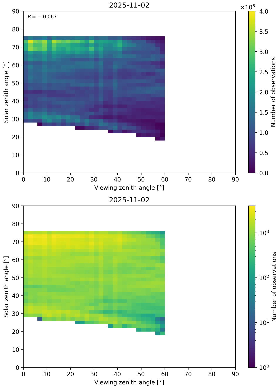
Figure 115: Scatter density plot of “Viewing zenith angle” against “Solar zenith angle” for 2025-11-02 to 2025-11-03.
