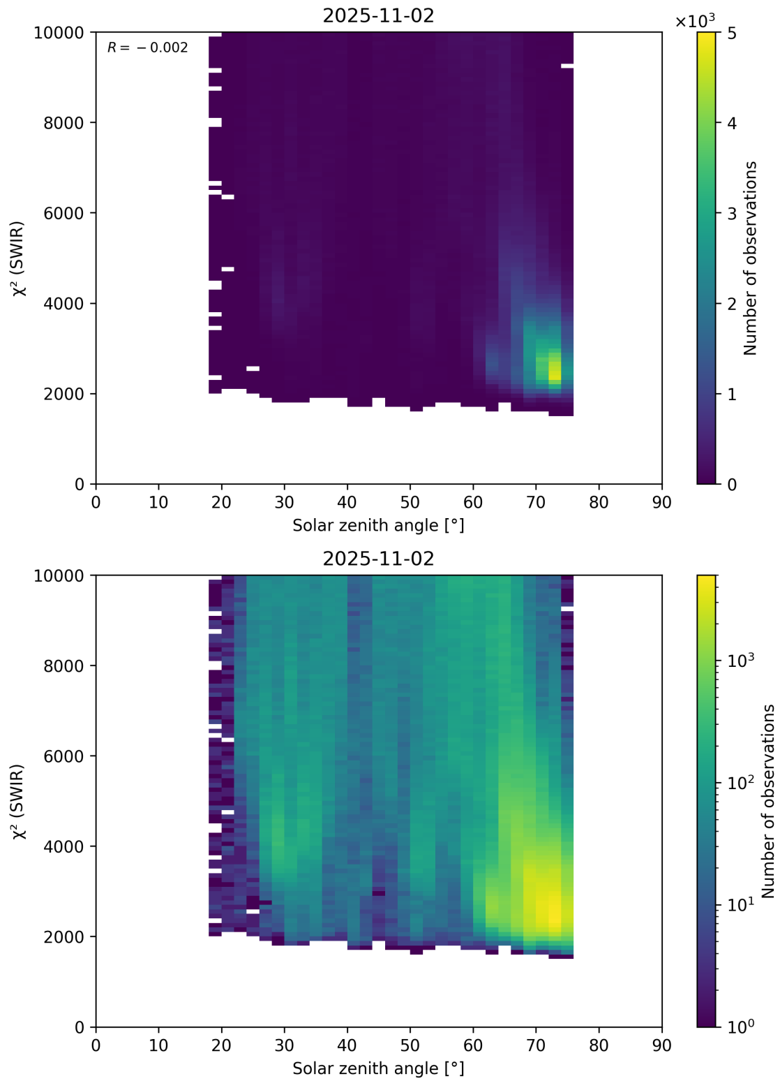
Figure 95: Scatter density plot of “Solar zenith angle” against “ \chi^2 (SWIR)” for 2025-11-02 to 2025-11-03.
