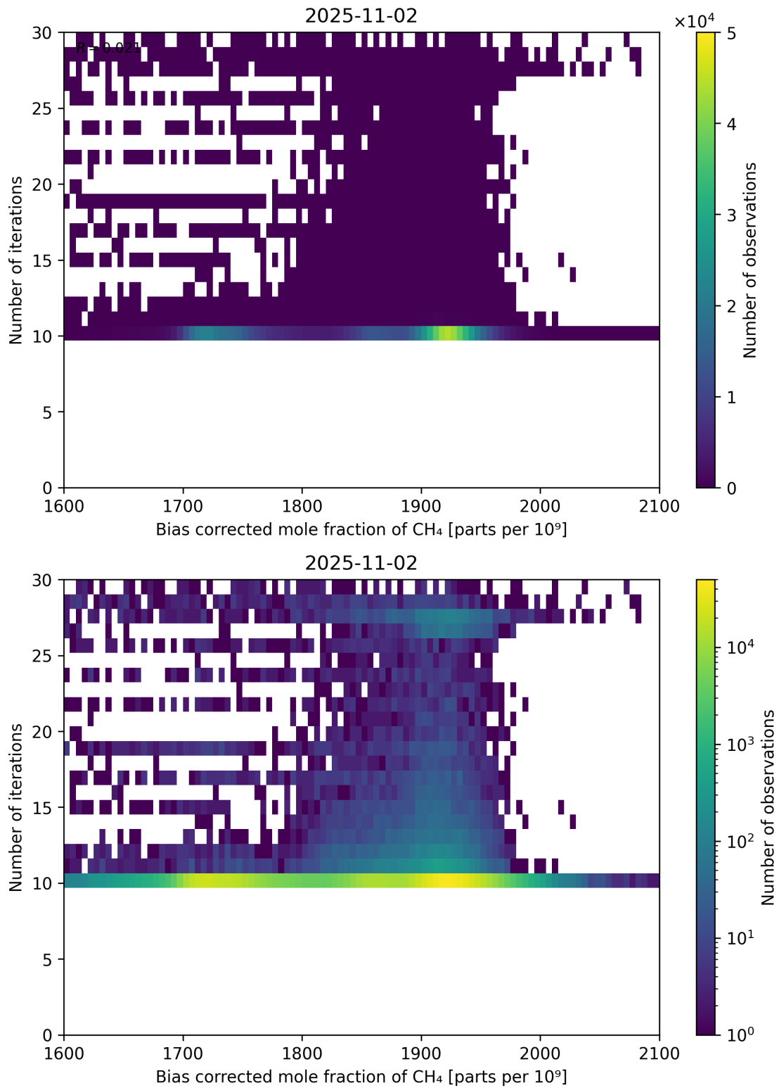
Figure 67: Scatter density plot of “Bias corrected mole fraction of \text{CH}_4 ” against “Number of iterations” for 2025-11-02 to 2025-11-03.
