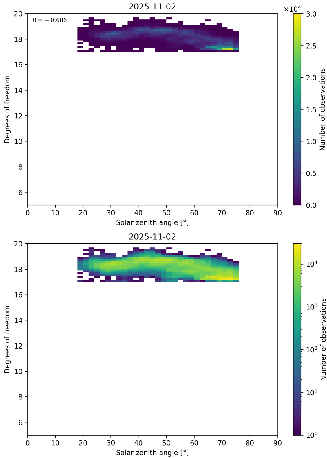
Figure 96: Scatter density plot of “Solar zenith angle” against “Degrees of freedom” for 2025-11-02 to 2025-11-03.
