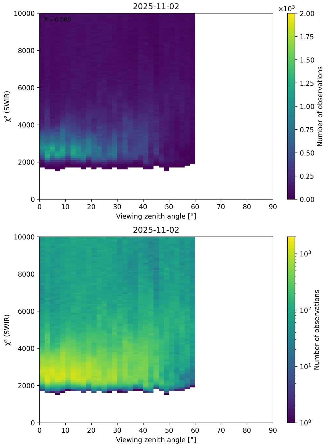
Figure 106: Scatter density plot of “Viewing zenith angle” against “ \chi^2 (SWIR)” for 2025-11-02 to 2025-11-03.
