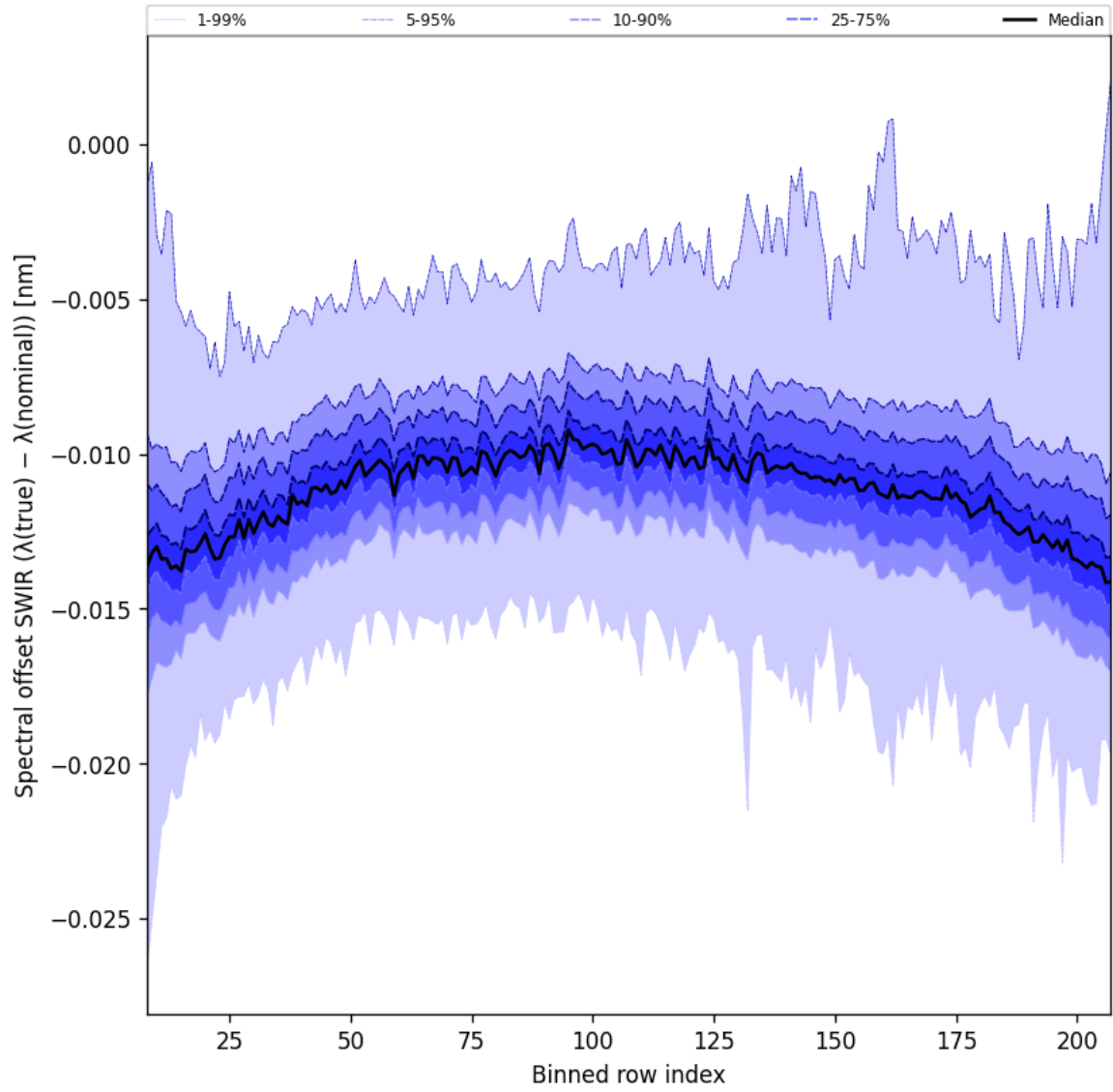
Figure 38: Along track statistics of “Spectral offset SWIR ( \lambda_{\text{true}} - \lambda_{\text{nominal}} )” for 2025-11-02 to 2025-11-03
