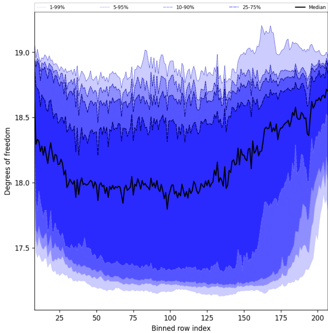
Figure 41: Along track statistics of “Degrees of freedom” for 2025-11-02 to 2025-11-03
