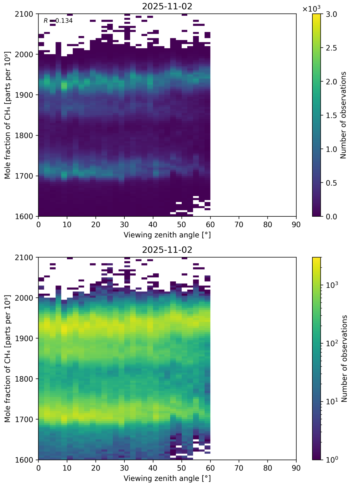
Figure 110: Scatter density plot of “Viewing zenith angle” against “Mole fraction of CH 4 ” for 2025-11-02 to 2025-11-03.
