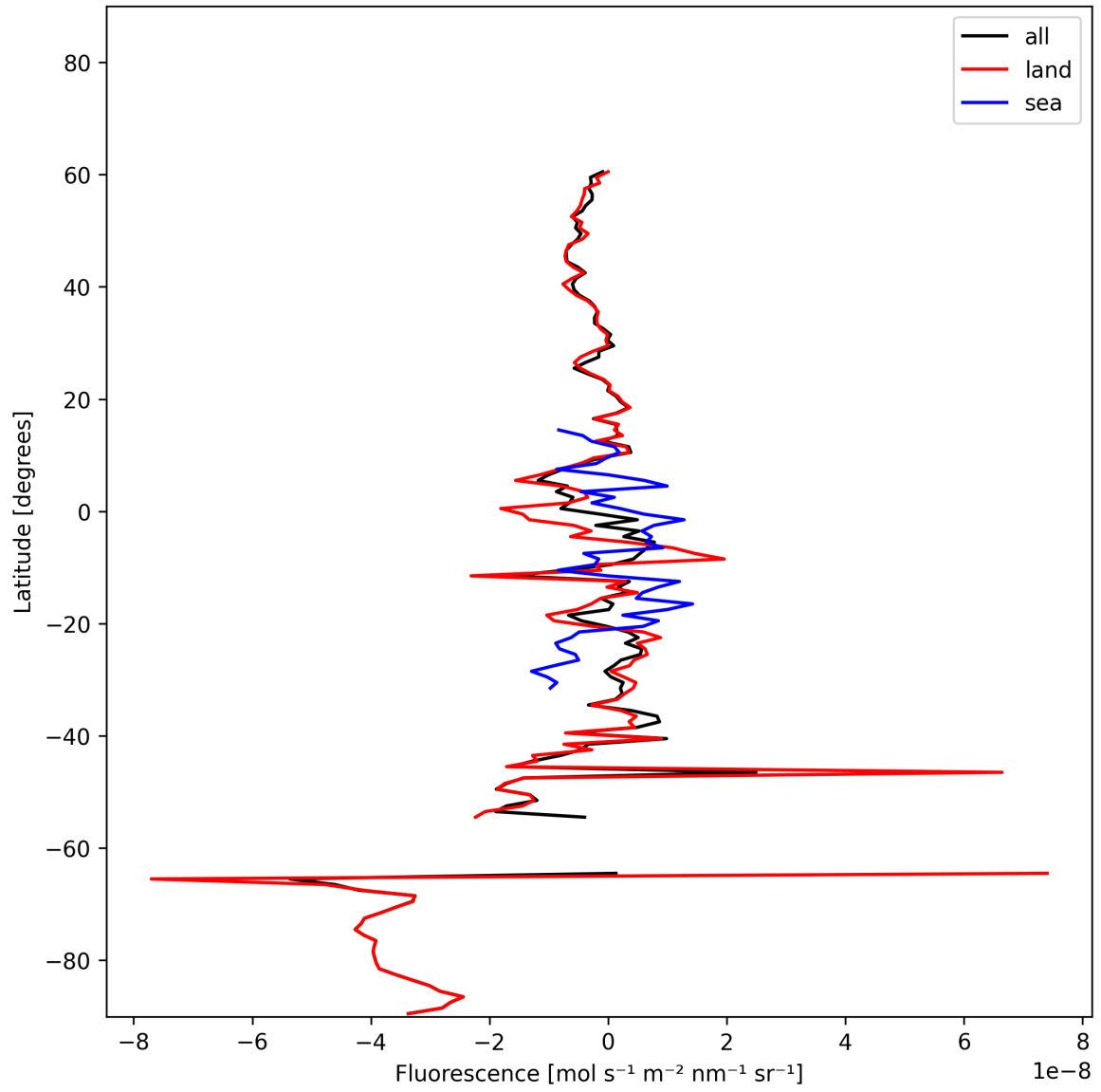
Figure 21: Zonal average of “Fluorescence” for 2025-11-02 to 2025-11-03.
