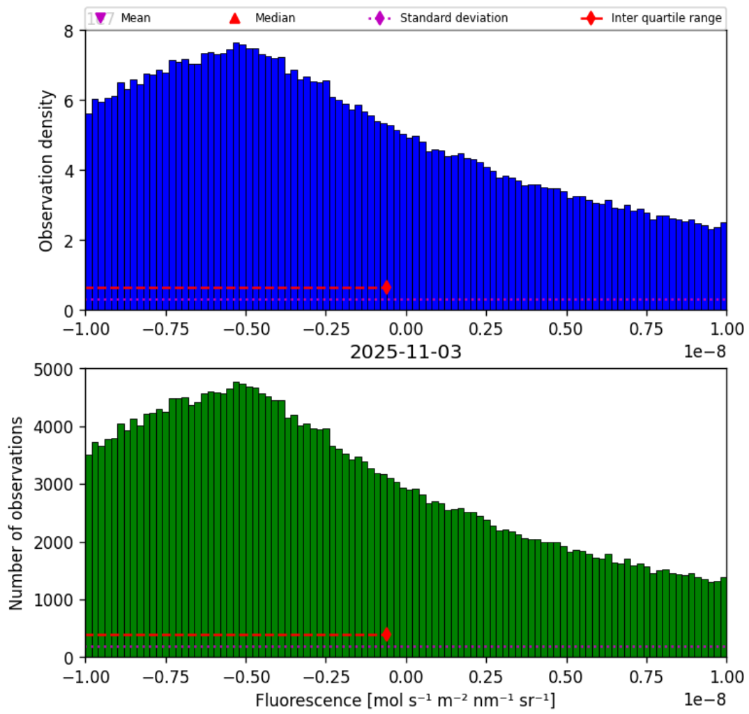
Figure 32: Histogram of “Fluorescence” for 2025-11-02 to 2025-11-04
