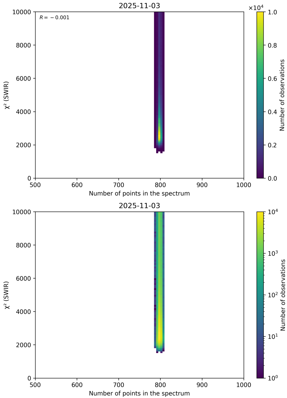
Figure 89: Scatter density plot of “Number of points in the spectrum” against “ \chi^2 (SWIR)” for 2025-11-02 to 2025-11-04.
