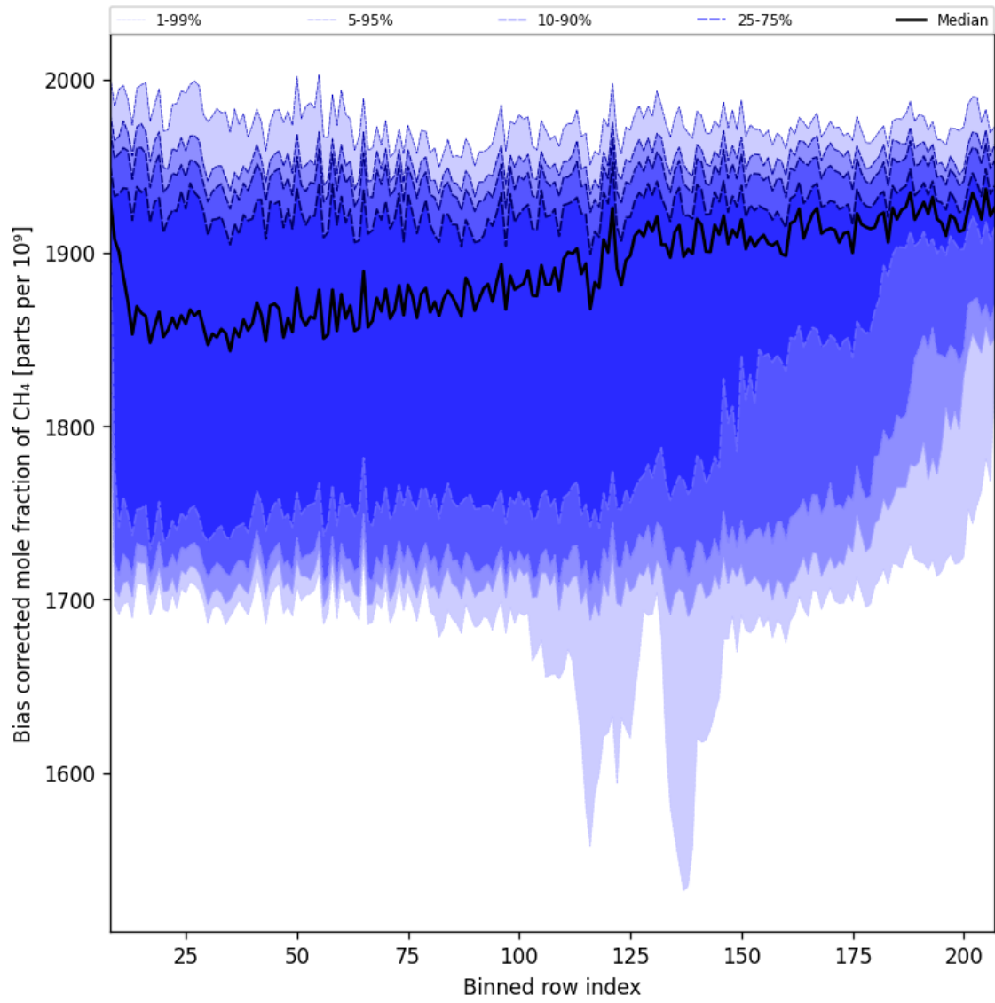
Figure 36: Along track statistics of “Bias corrected mole fraction of CH 4 ” for 2025-11-02 to 2025-11-04
