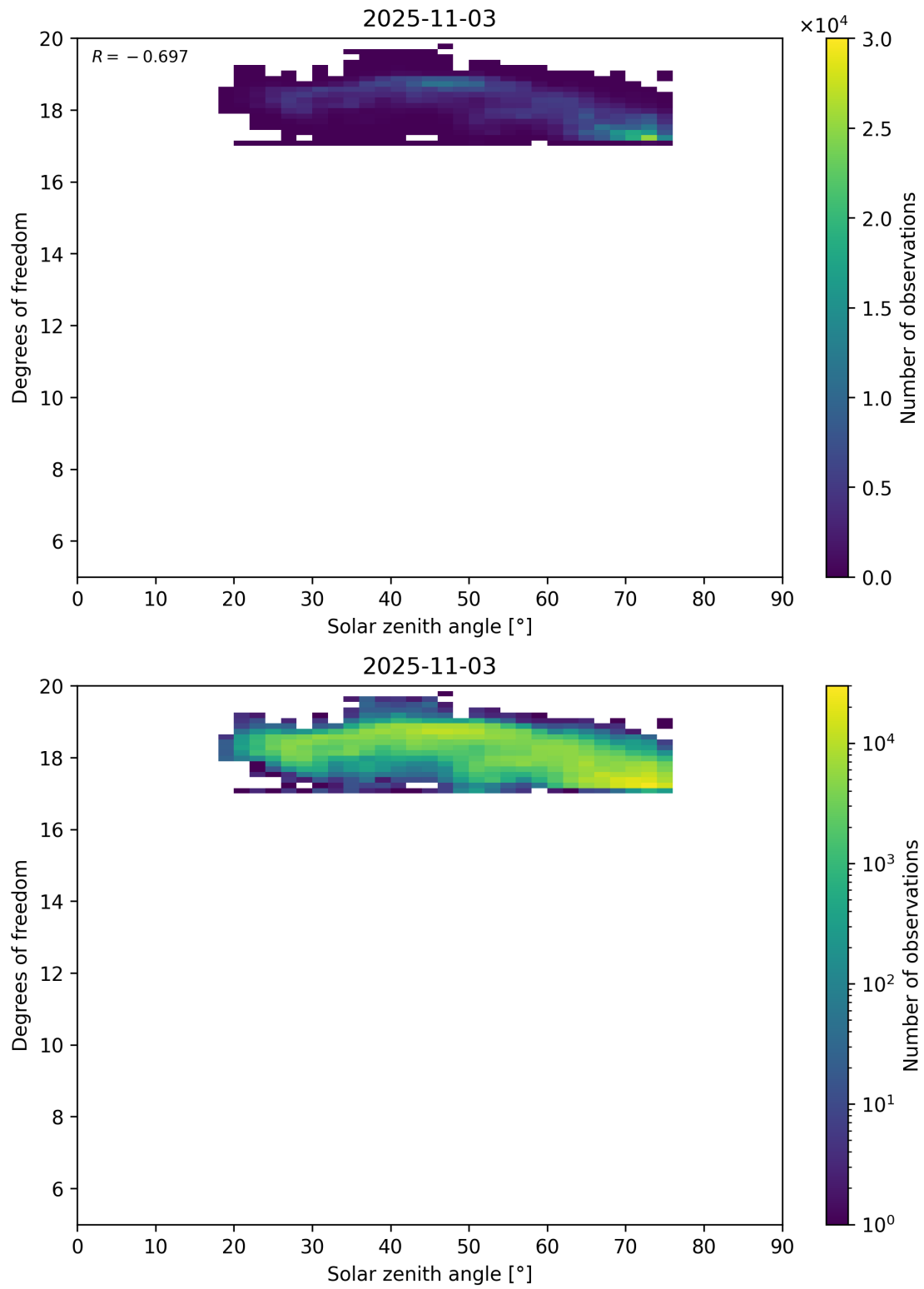
Figure 96: Scatter density plot of “Solar zenith angle” against “Degrees of freedom” for 2025-11-02 to 2025-11-04.
