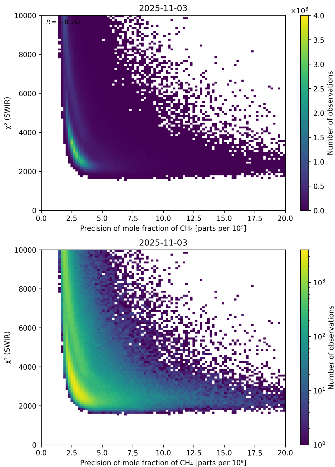
Figure 79: Scatter density plot of “Precision of mole fraction of \text{CH}_4 ” against “ \chi^2 (SWIR)” for 2025-11-02 to 2025-11-04.
