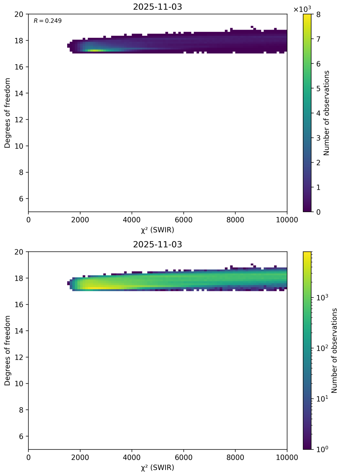
Figure 48: Scatter density plot of “ \chi^2 (SWIR)” against “Degrees of freedom” for 2025-11-02 to 2025-11-04.
