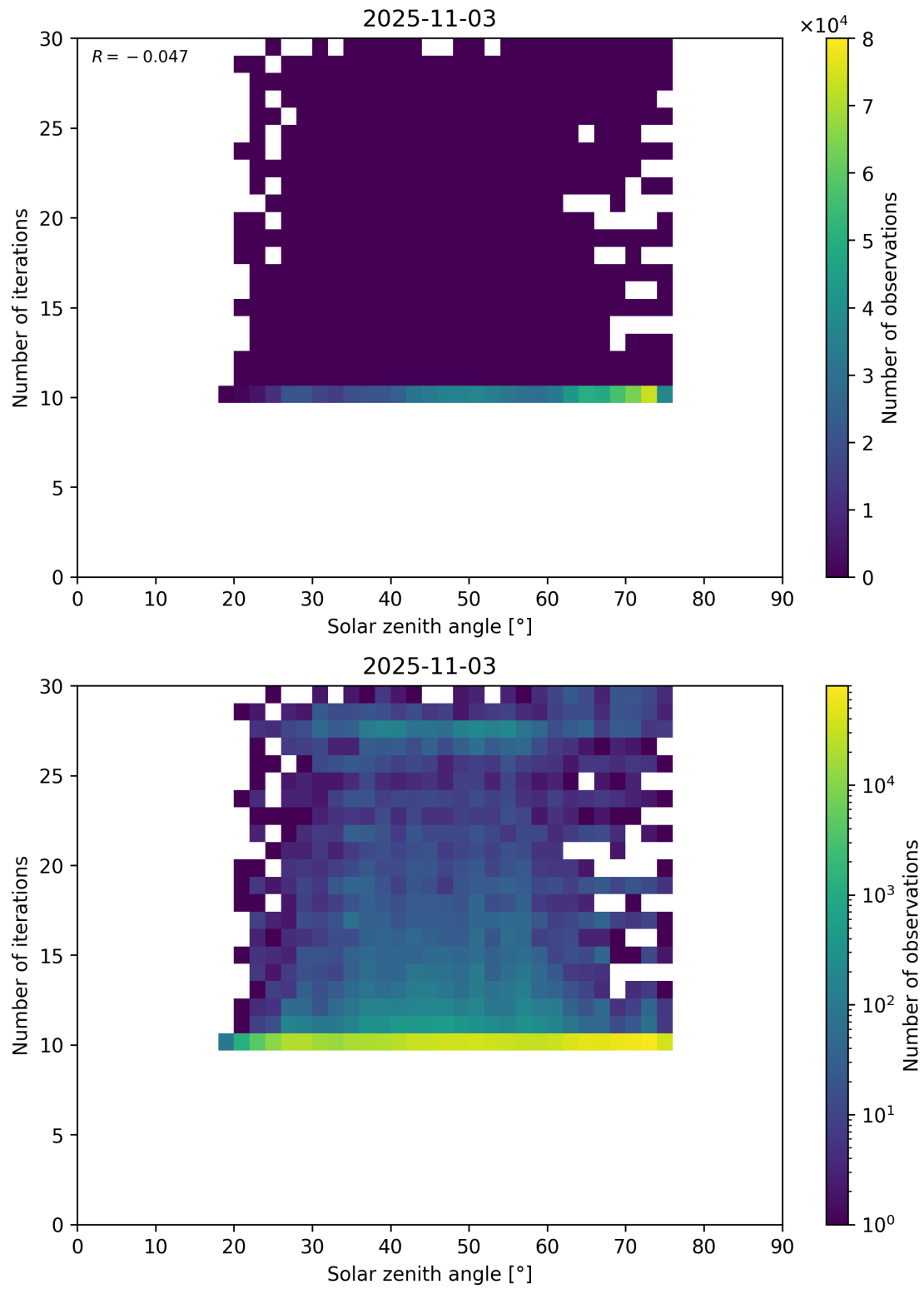
Figure 102: Scatter density plot of “Solar zenith angle” against “Number of iterations” for 2025-11-02 to 2025-11-04.
