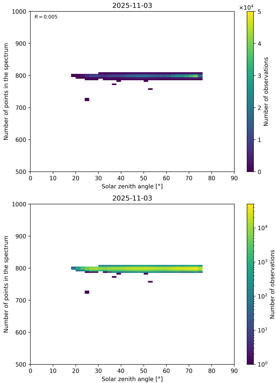
Figure 103: Scatter density plot of “Solar zenith angle” against “Number of points in the spectrum” for 2025-11-02 to 2025-11-04.
