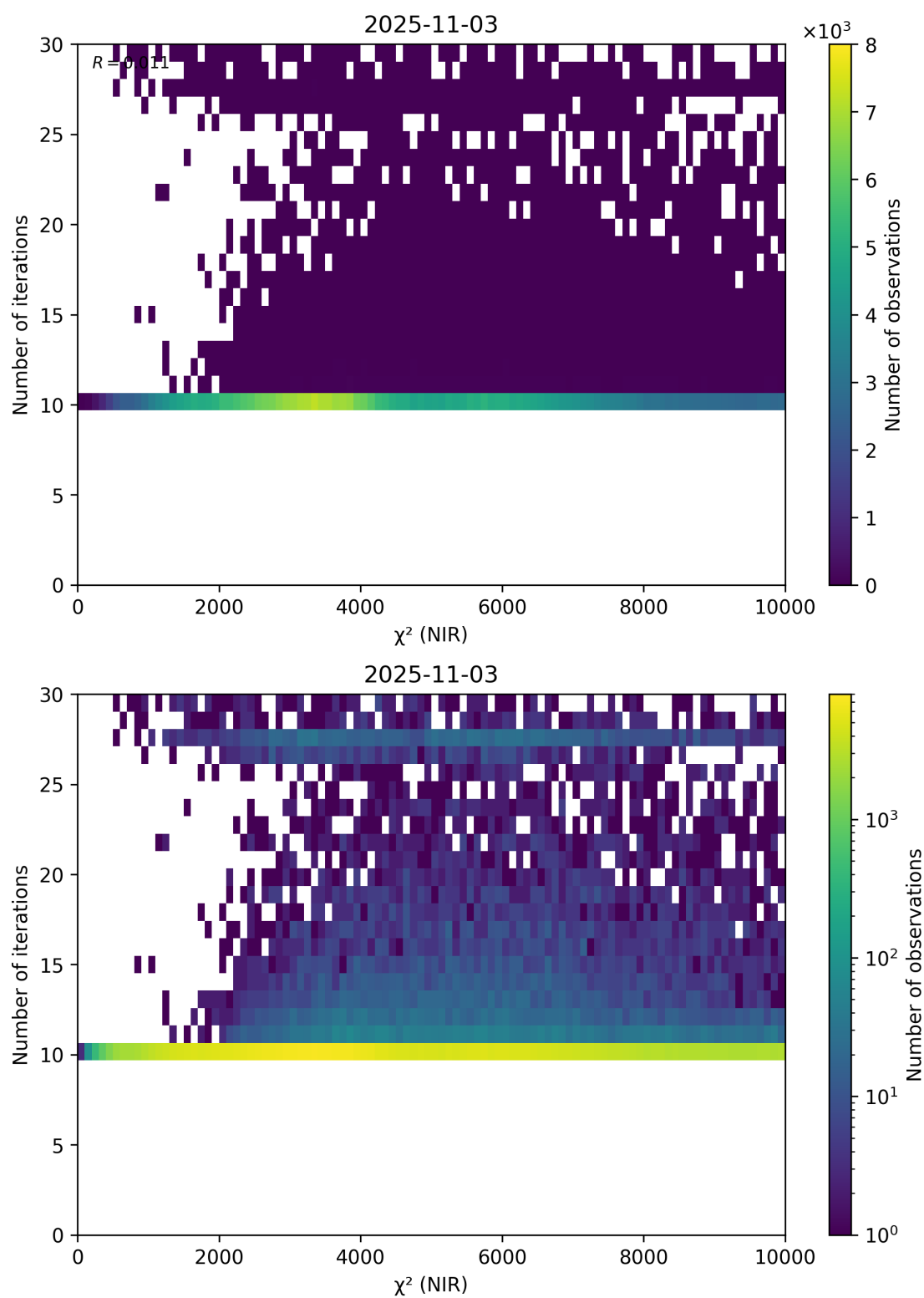
Figure 46: Scatter density plot of “ \chi^2 (NIR)” against “Number of iterations” for 2025-11-02 to 2025-11-04.
