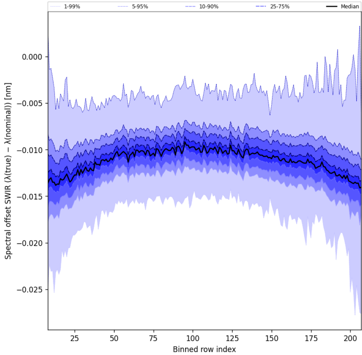
Figure 38: Along track statistics of “Spectral offset SWIR ( \lambda_{\text{true}} - \lambda_{\text{nominal}} )” for 2025-11-02 to 2025-11-04
