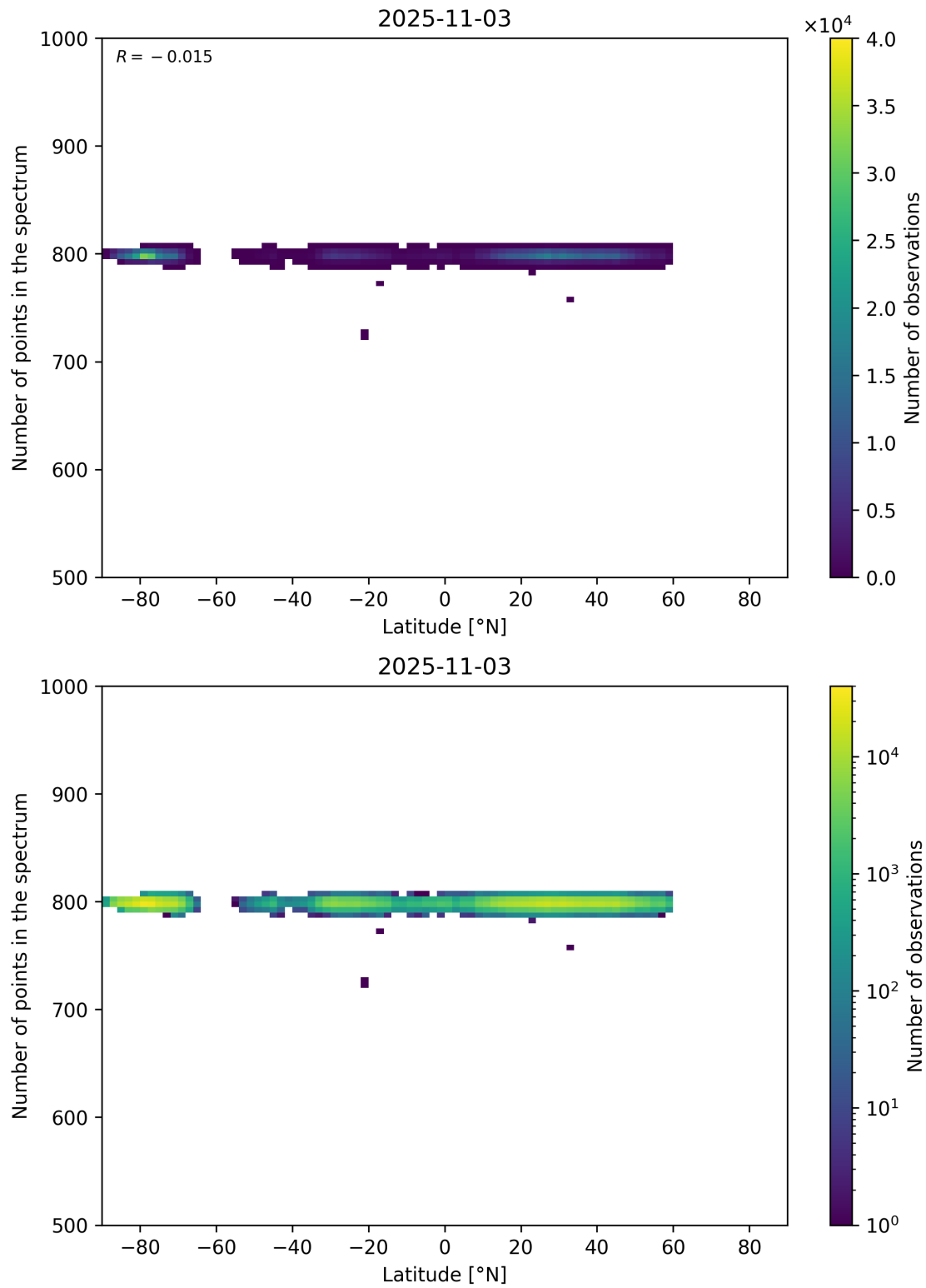
Figure 61: Scatter density plot of “Latitude” against “Number of points in the spectrum” for 2025-11-02 to 2025-11-04.
