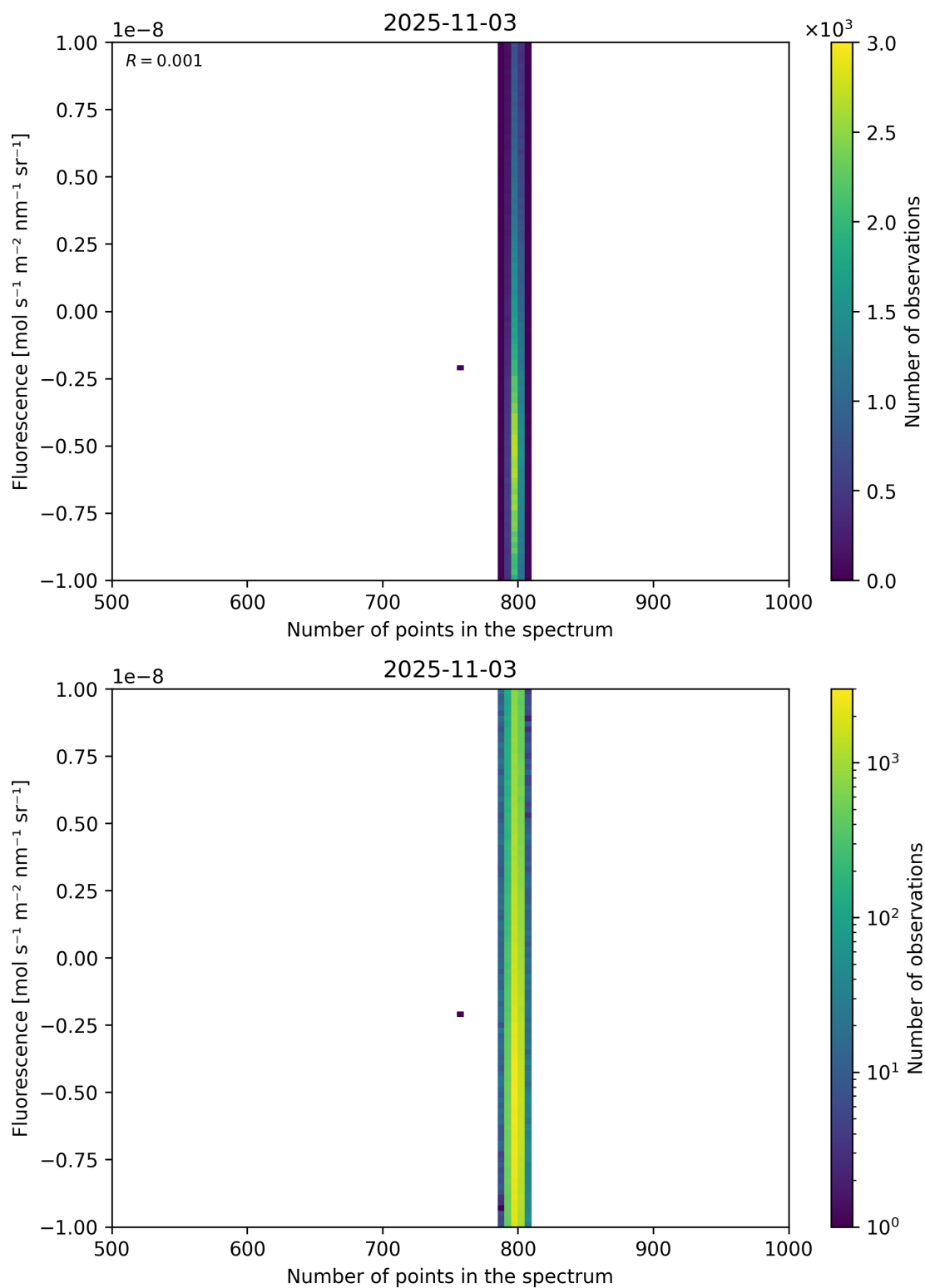
Figure 91: Scatter density plot of “Number of points in the spectrum” against “Fluorescence” for 2025-11-02 to 2025-11-04.
