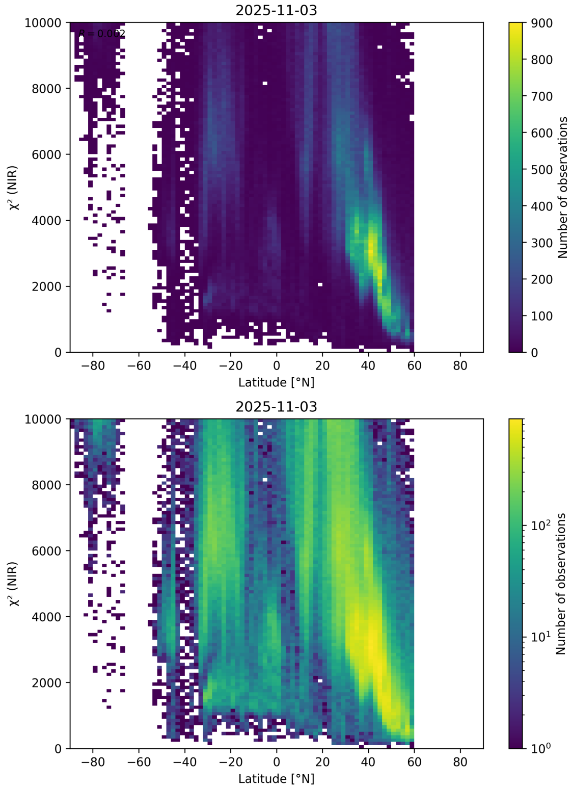
Figure 53: Scatter density plot of “Latitude” against “ \chi^2 (NIR)” for 2025-11-02 to 2025-11-04.
