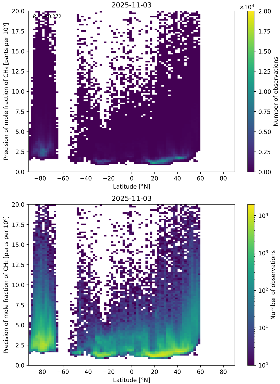
Figure 59: Scatter density plot of “Latitude” against “Precision of mole fraction of CH 4 ” for 2025-11-02 to 2025-11-04.
