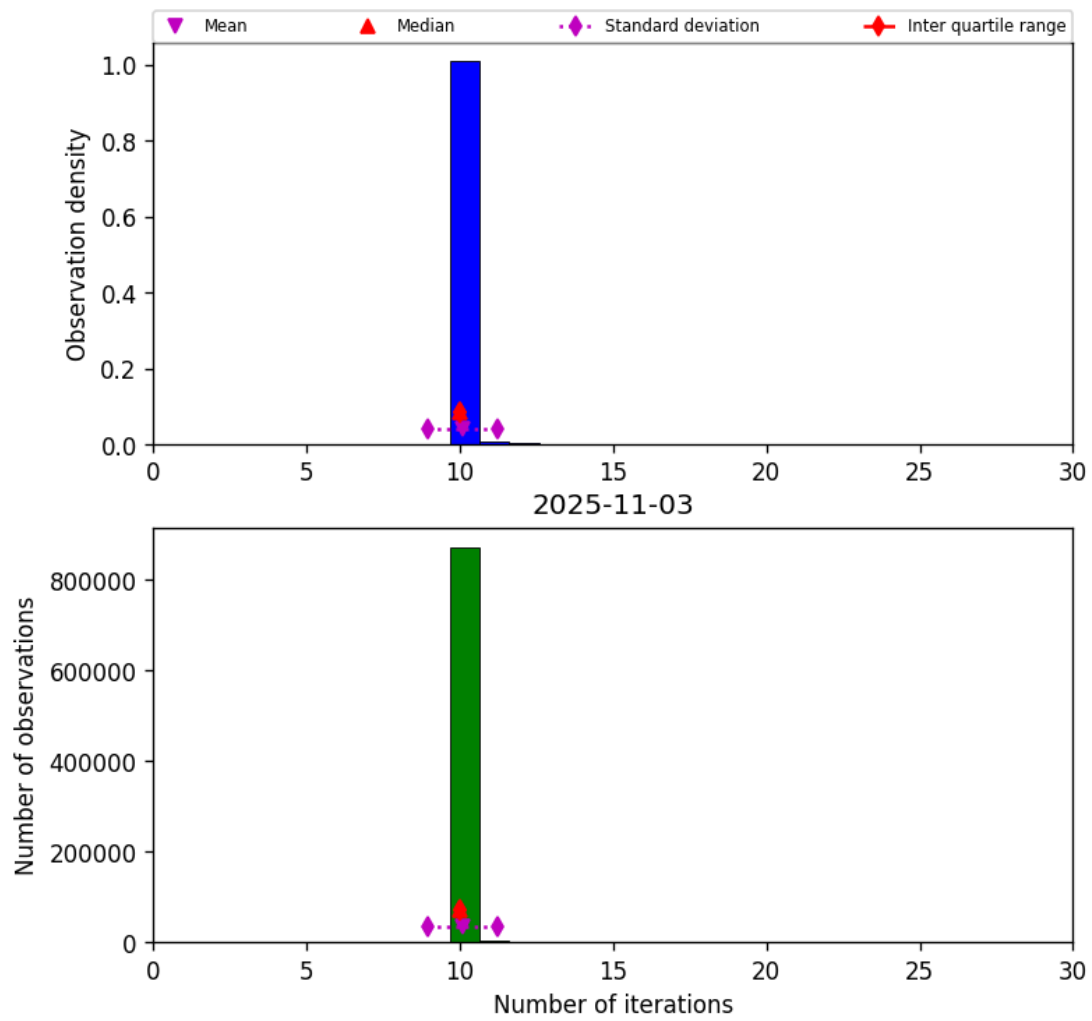
Figure 31: Histogram of “Number of iterations” for 2025-11-02 to 2025-11-04
