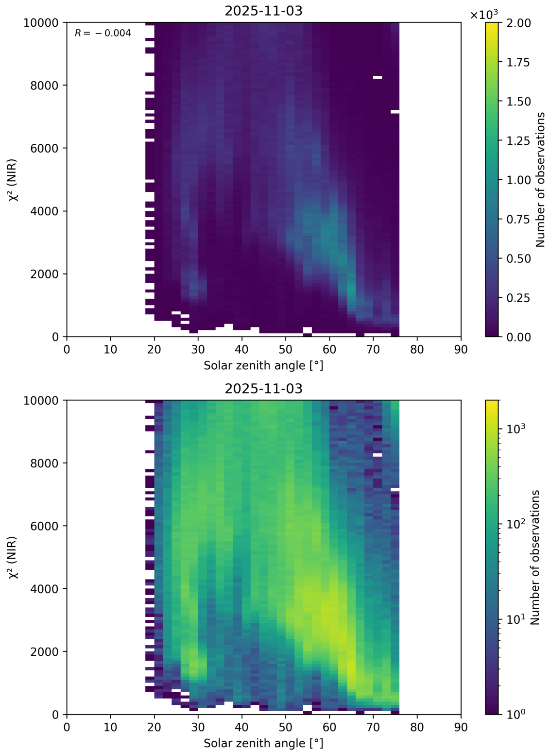
Figure 94: Scatter density plot of “Solar zenith angle” against “ \chi^2 (NIR)” for 2025-11-02 to 2025-11-04.
