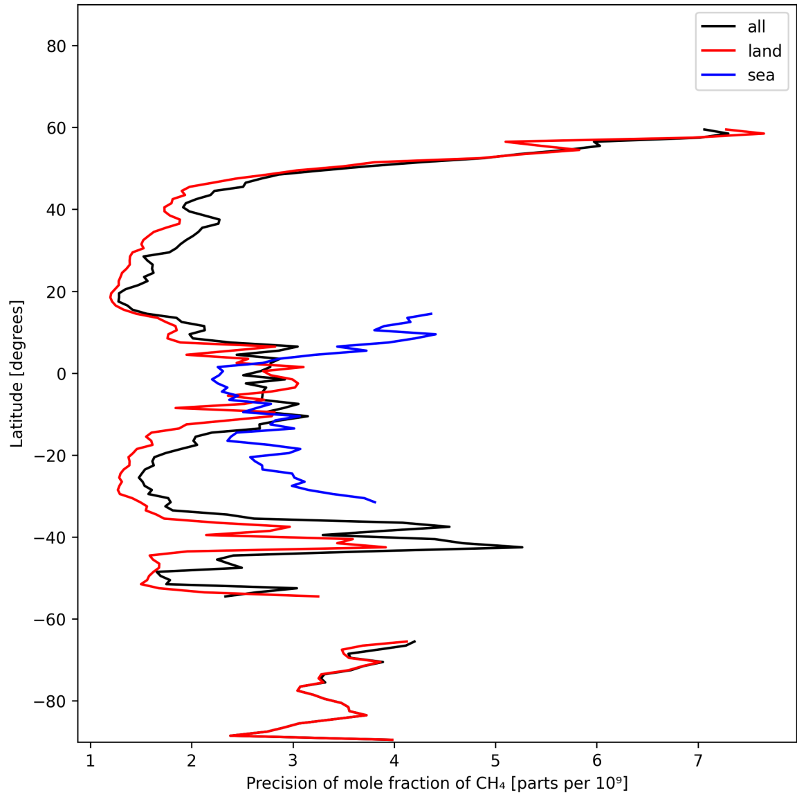
Figure 13: Zonal average of “Precision of mole fraction of CH 4 ” for 2025-11-02 to 2025-11-04.
