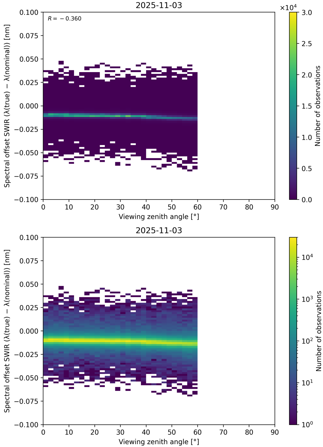
Figure 116: Scatter density plot of “Viewing zenith angle” against “Spectral offset SWIR ( \lambda_{\text{true}} - \lambda_{\text{nominal}} )” for 2025-11-02 to 2025-11-04.
