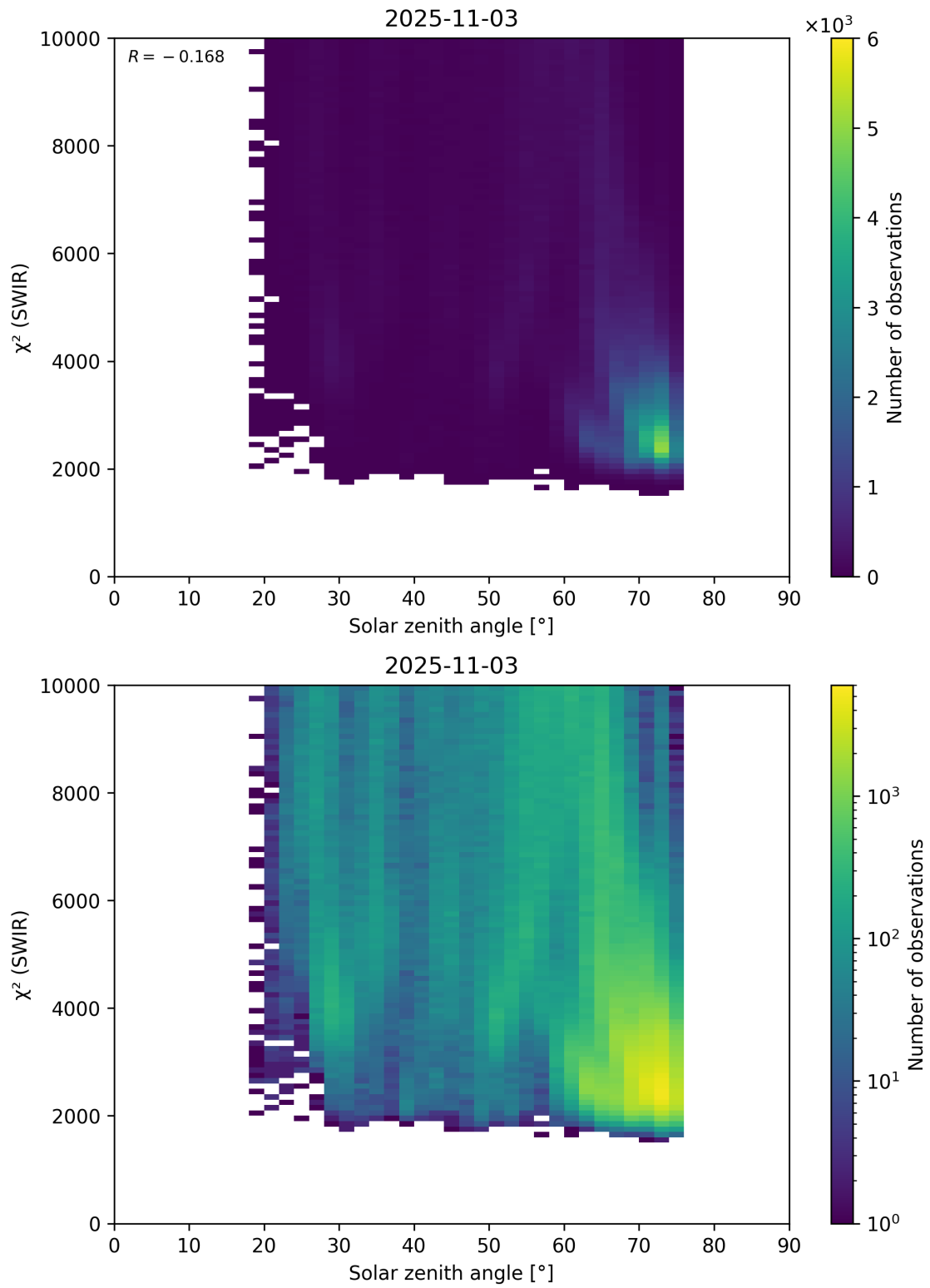
Figure 95: Scatter density plot of “Solar zenith angle” against “ \chi^2 (SWIR)” for 2025-11-02 to 2025-11-04.
