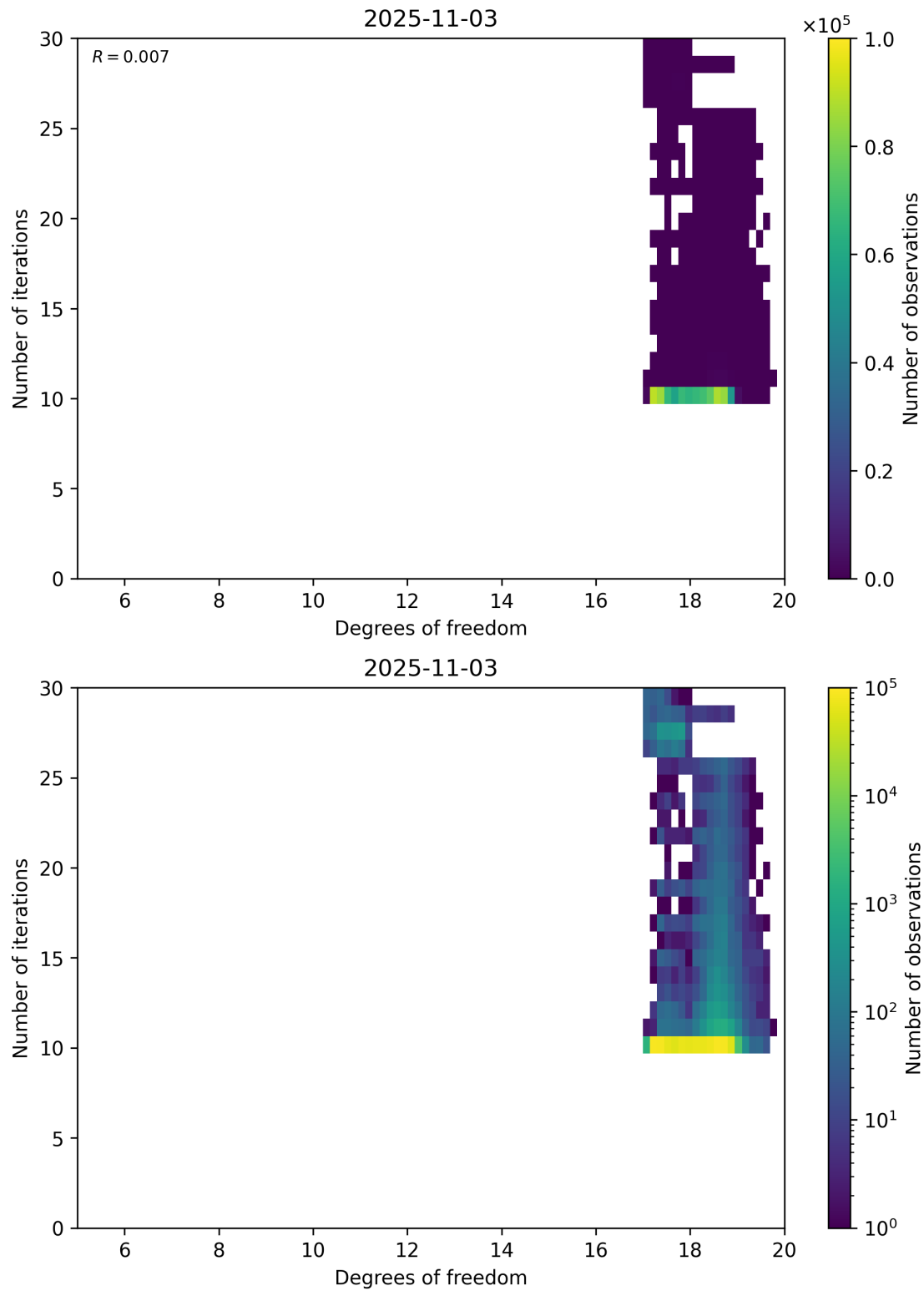
Figure 52: Scatter density plot of “Degrees of freedom” against “Number of iterations” for 2025-11-02 to 2025-11-04.
