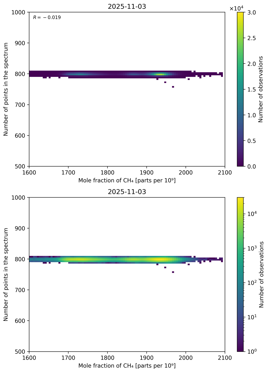
Figure 77: Scatter density plot of “Mole fraction of CH 4 ” against “Number of points in the spectrum” for 2025-11-02 to 2025-11-04.
