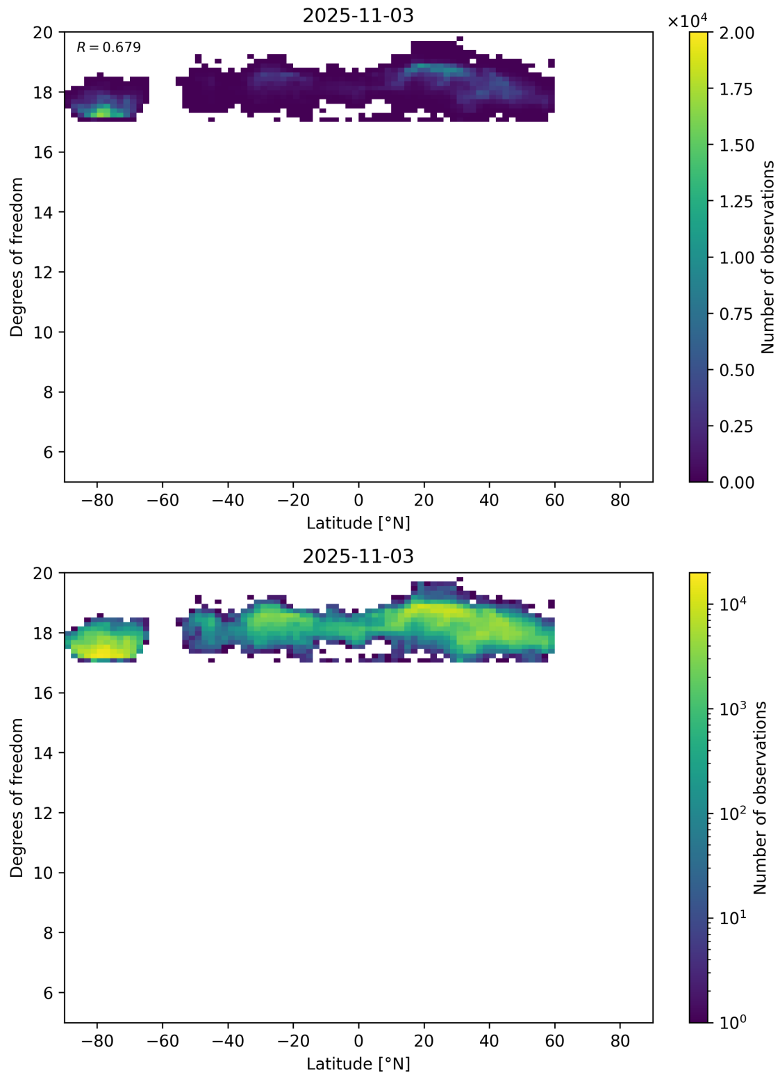
Figure 55: Scatter density plot of “Latitude” against “Degrees of freedom” for 2025-11-02 to 2025-11-04.
