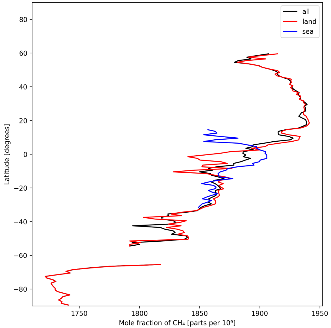
Figure 12: Zonal average of “Mole fraction of CH 4 ” for 2025-11-02 to 2025-11-04.
