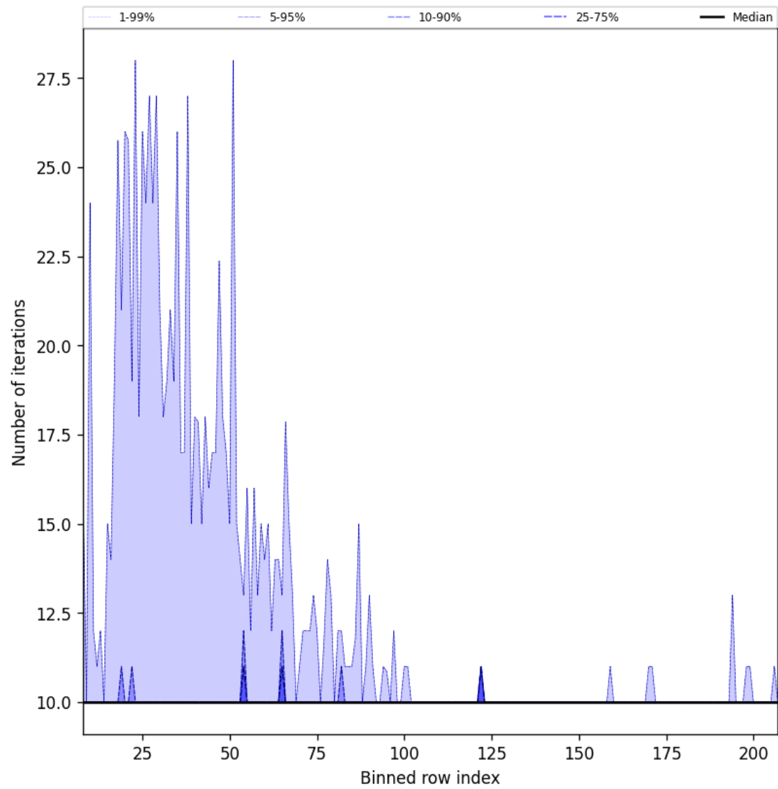
Figure 42: Along track statistics of “Number of iterations” for 2025-11-02 to 2025-11-04
