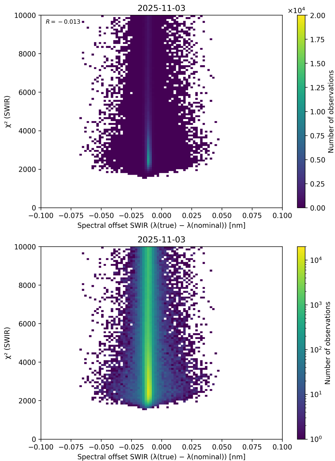
Figure 118: Scatter density plot of “Spectral offset SWIR ( \lambda_{\text{true}} - \lambda_{\text{nominal}} )” against “ \chi^2 (SWIR)” for 2025-11-02 to 2025-11-04.
