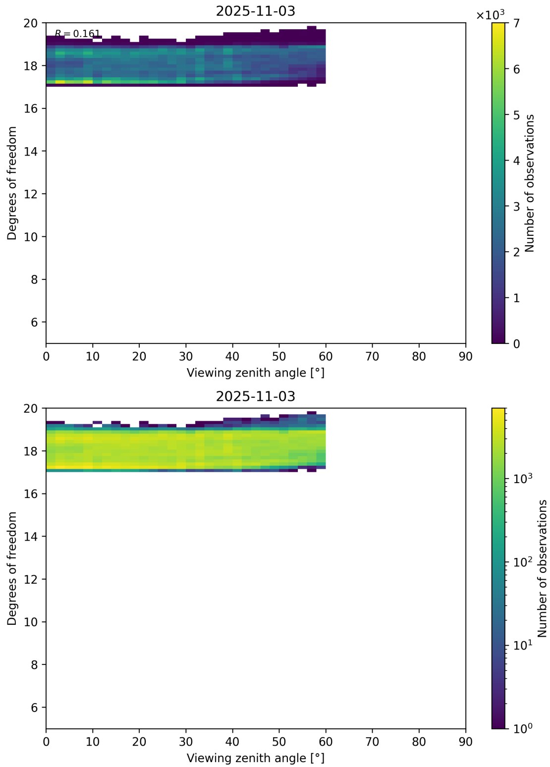
Figure 107: Scatter density plot of “Viewing zenith angle” against “Degrees of freedom” for 2025-11-02 to 2025-11-04.
