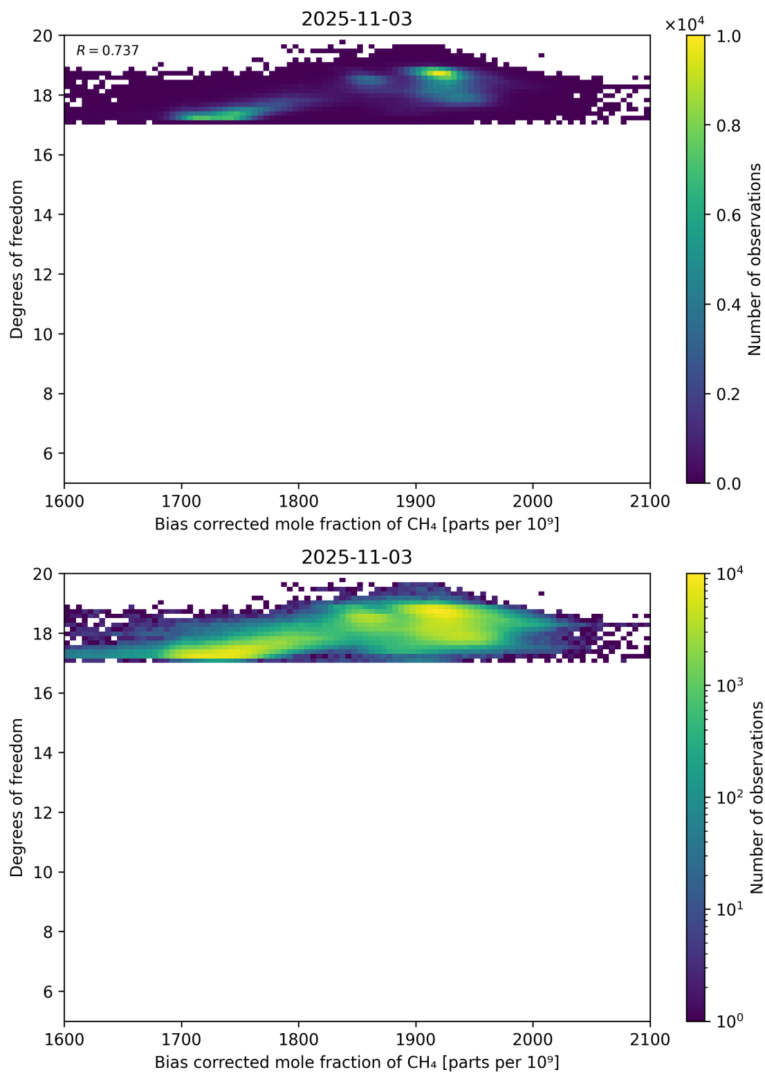
Figure 65: Scatter density plot of “Bias corrected mole fraction of CH 4 ” against “Degrees of freedom” for 2025-11-02 to 2025-11-04.
