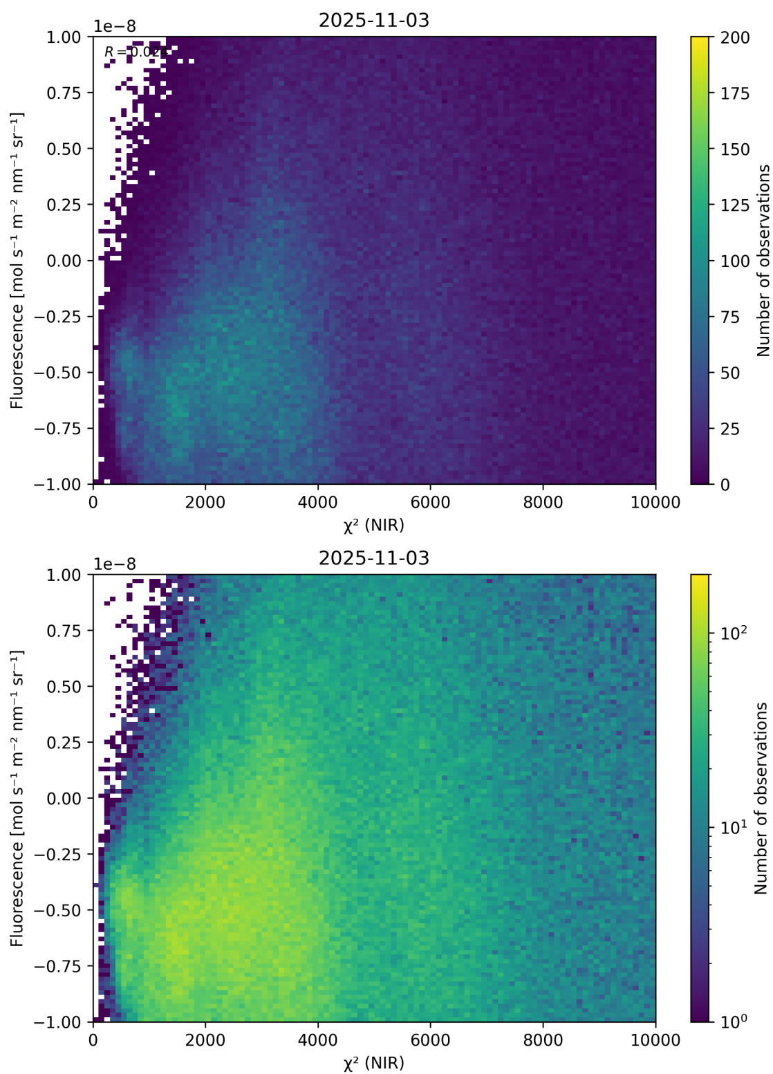
Figure 45: Scatter density plot of “ \chi^2 (NIR)” against “Fluorescence” for 2025-11-02 to 2025-11-04.
