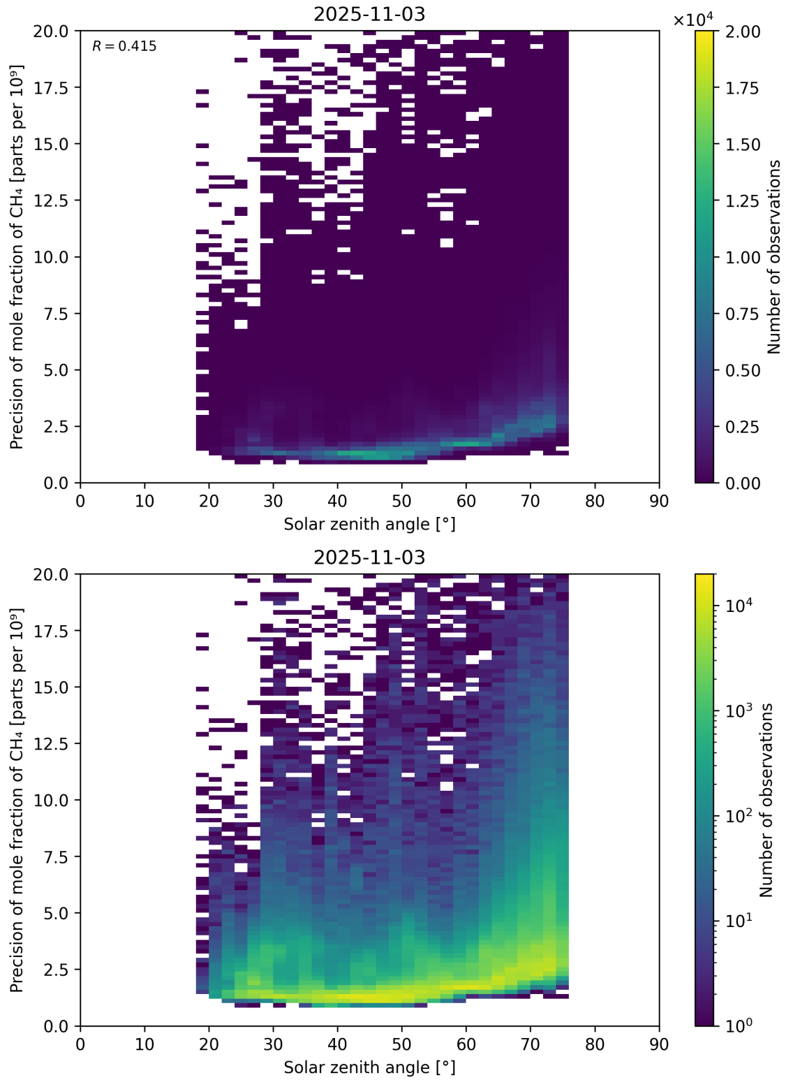
Figure 101: Scatter density plot of “Solar zenith angle” against “Precision of mole fraction of \text{CH}_4 ” for 2025-11-02 to 2025-11-04.
