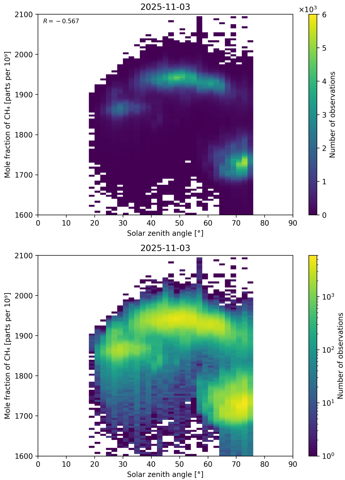
Figure 99: Scatter density plot of “Solar zenith angle” against “Mole fraction of CH 4 ” for 2025-11-02 to 2025-11-04.
