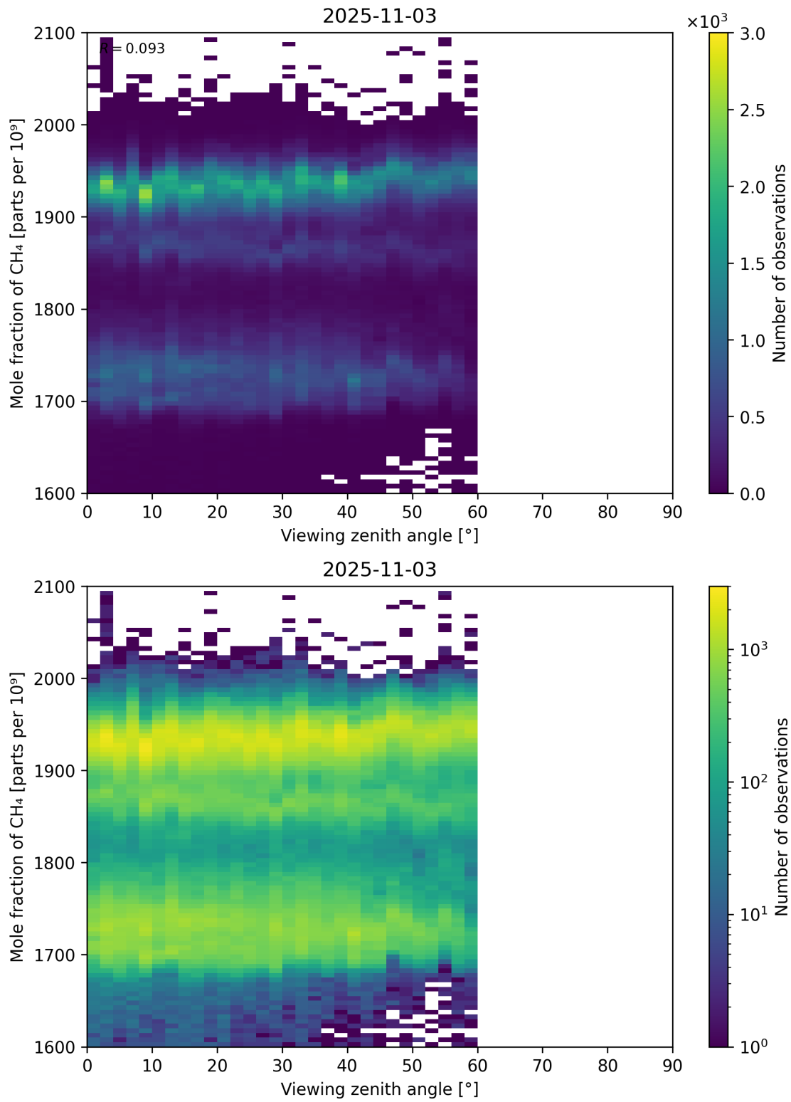
Figure 110: Scatter density plot of “Viewing zenith angle” against “Mole fraction of CH 4 ” for 2025-11-02 to 2025-11-04.
