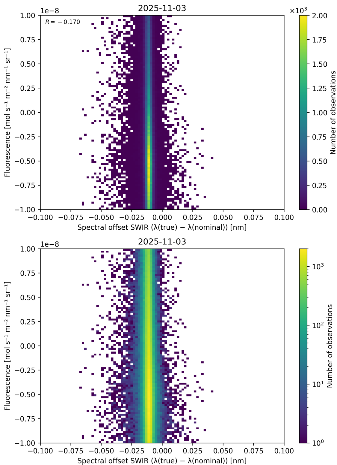
Figure 120: Scatter density plot of “Spectral offset SWIR ( \lambda_{\text{true}} - \lambda_{\text{nominal}} )” against “Fluorescence” for 2025-11-02 to 2025-11-04.
