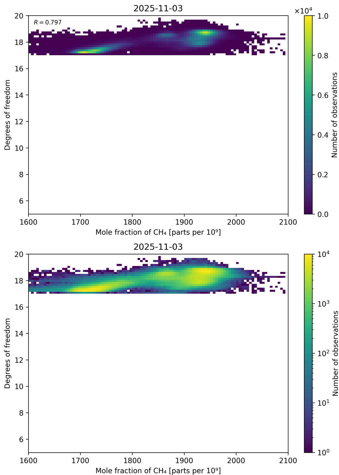
Figure 72: Scatter density plot of “Mole fraction of CH 4 ” against “Degrees of freedom” for 2025-11-02 to 2025-11-04.
