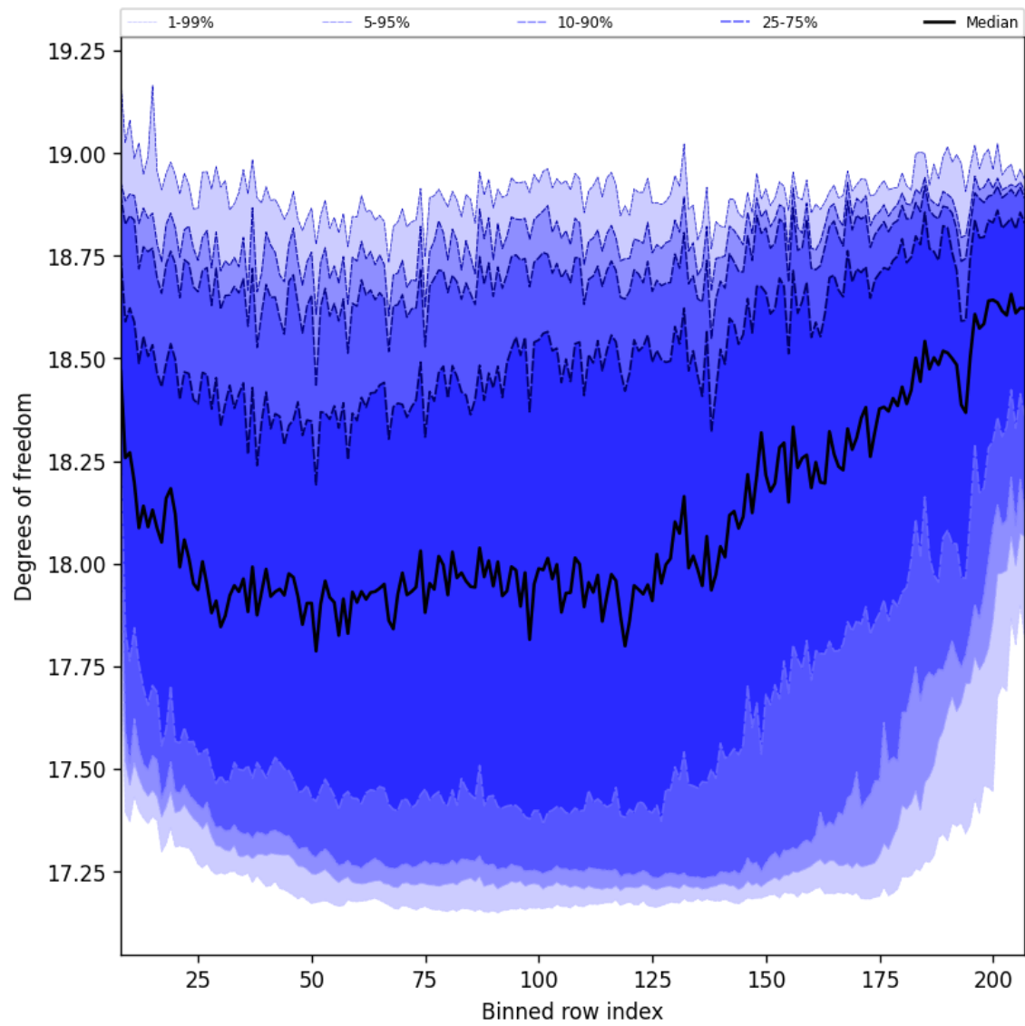
Figure 41: Along track statistics of “Degrees of freedom” for 2025-11-02 to 2025-11-04
