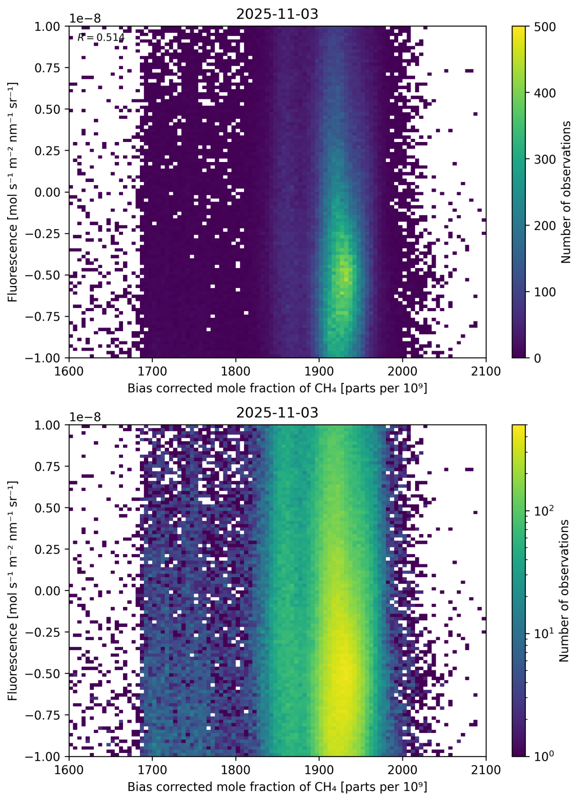
Figure 66: Scatter density plot of “Bias corrected mole fraction of \text{CH}_4 ” against “Fluorescence” for 2025-11-02 to 2025-11-04.
