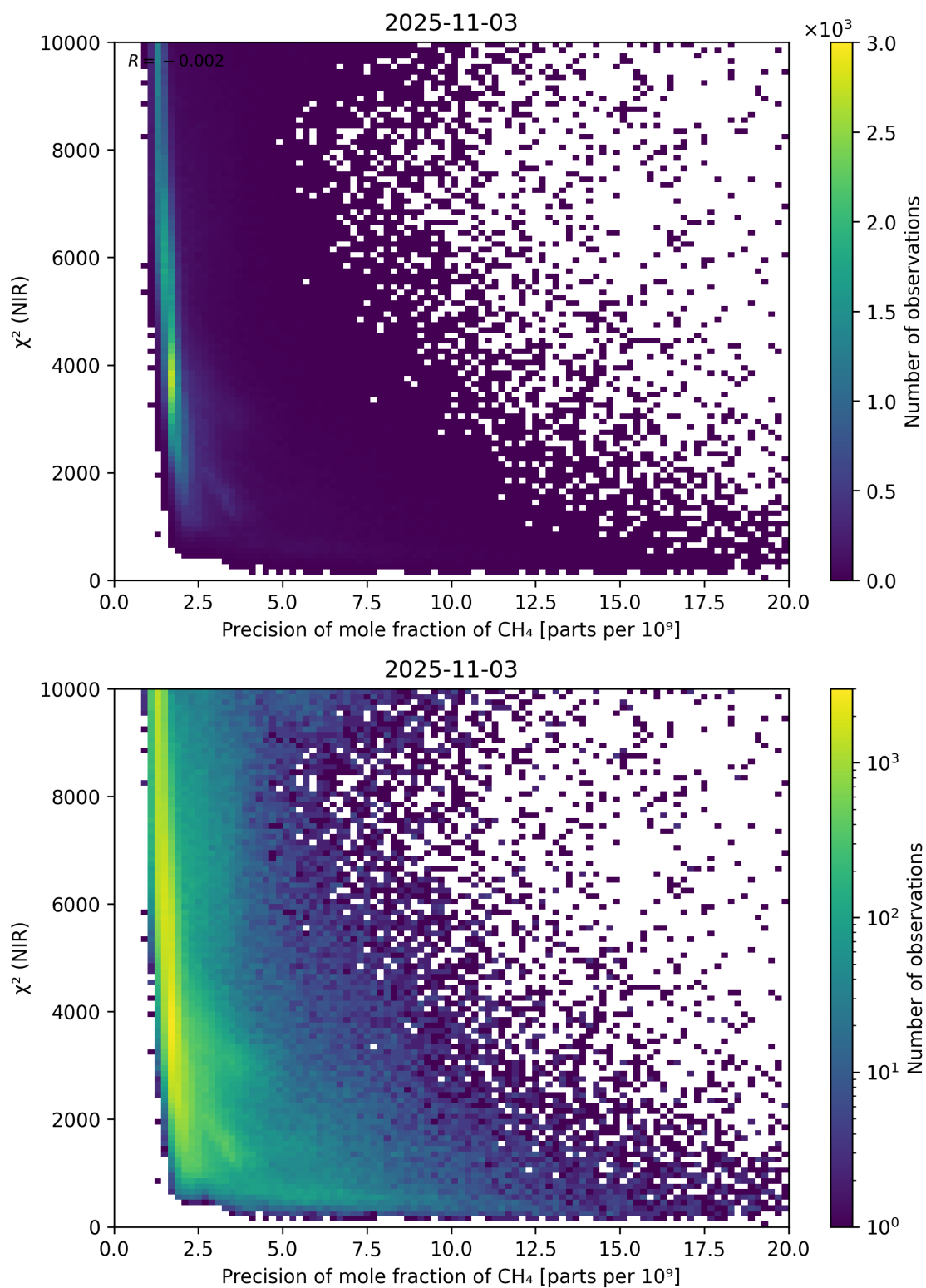
Figure 78: Scatter density plot of “Precision of mole fraction of CH 4 ” against “ \chi^2 (NIR)” for 2025-11-02 to 2025-11-04.
