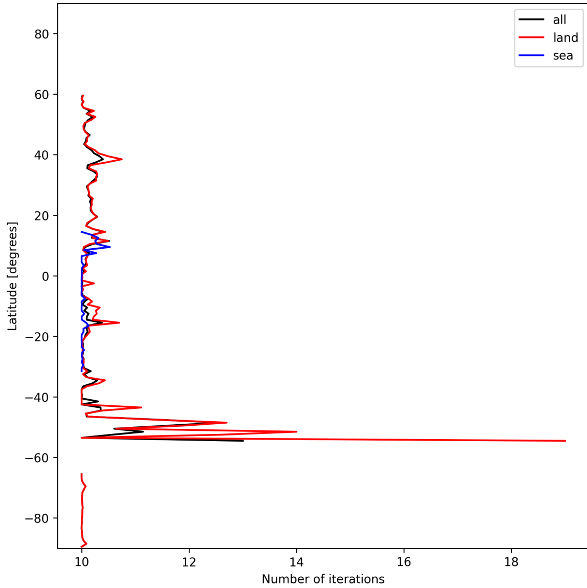
Figure 20: Zonal average of “Number of iterations” for 2025-11-02 to 2025-11-04.
