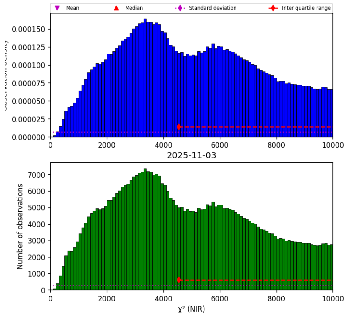
Figure 29: Histogram of “ \chi^2 (NIR)” for 2025-11-02 to 2025-11-04
