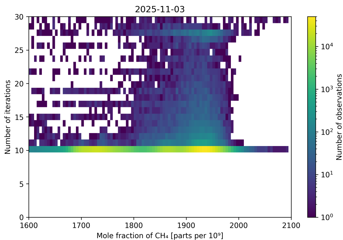
Figure 76: Scatter density plot of “Mole fraction of CH 4 ” against “Number of iterations” for 2025-11-02 to 2025-11-04.
