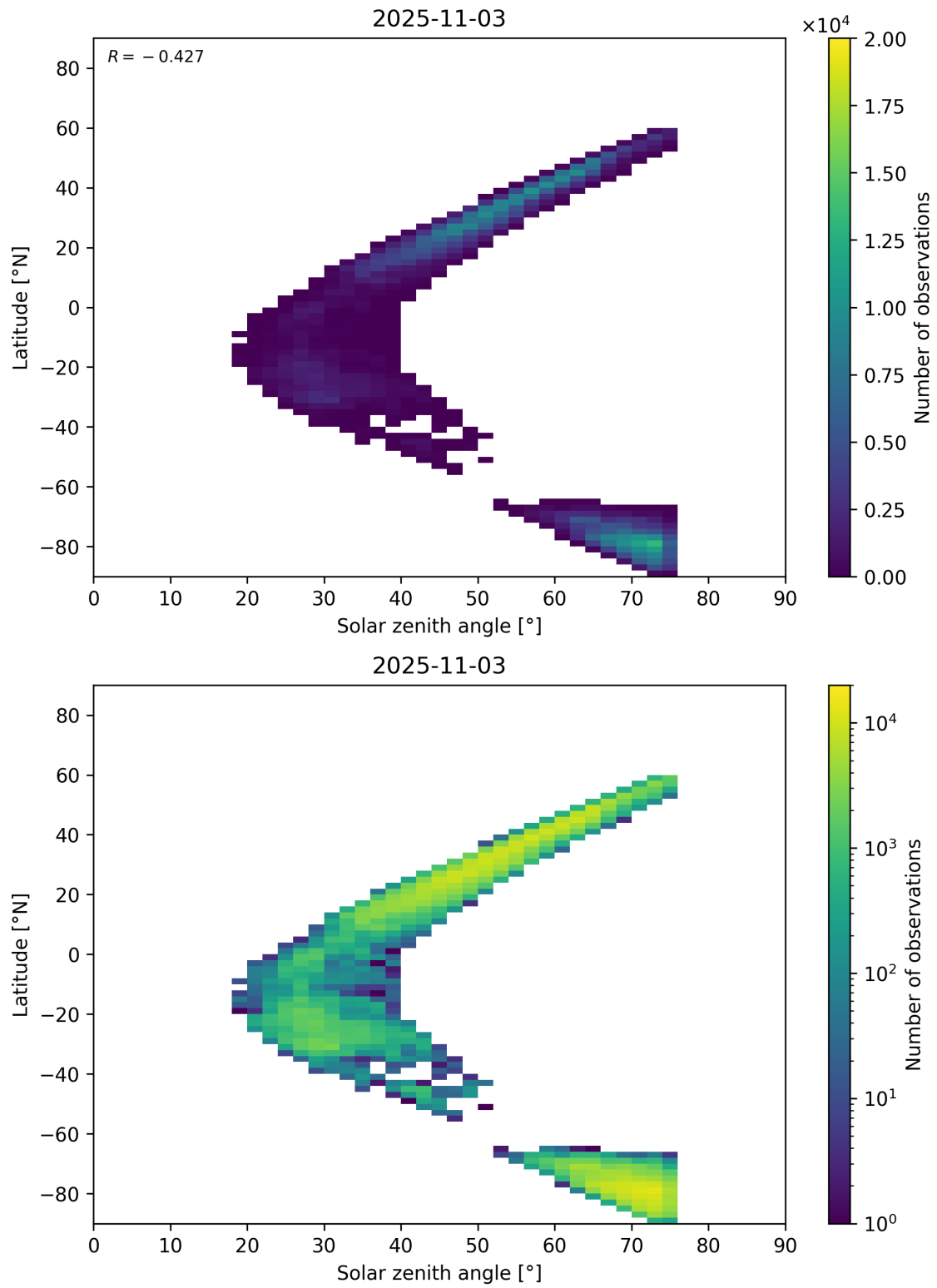
Figure 98: Scatter density plot of “Solar zenith angle” against “Latitude” for 2025-11-02 to 2025-11-04.
