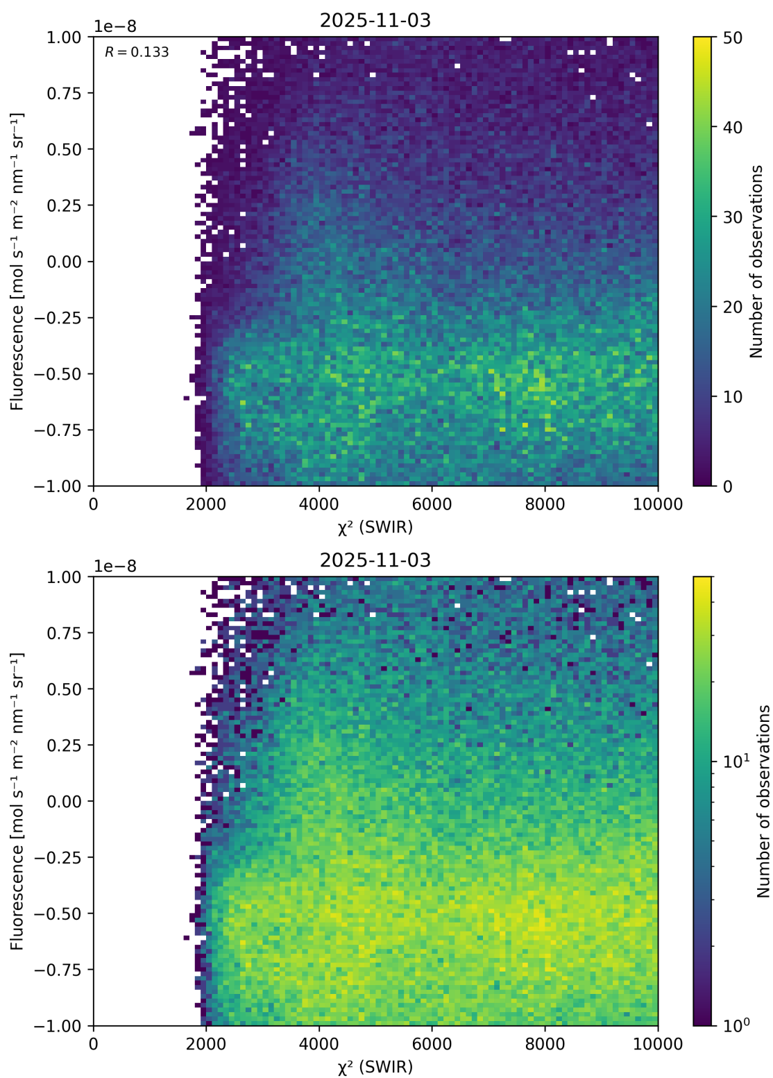
Figure 49: Scatter density plot of “ \chi^2 (SWIR)” against “Fluorescence” for 2025-11-02 to 2025-11-04.
