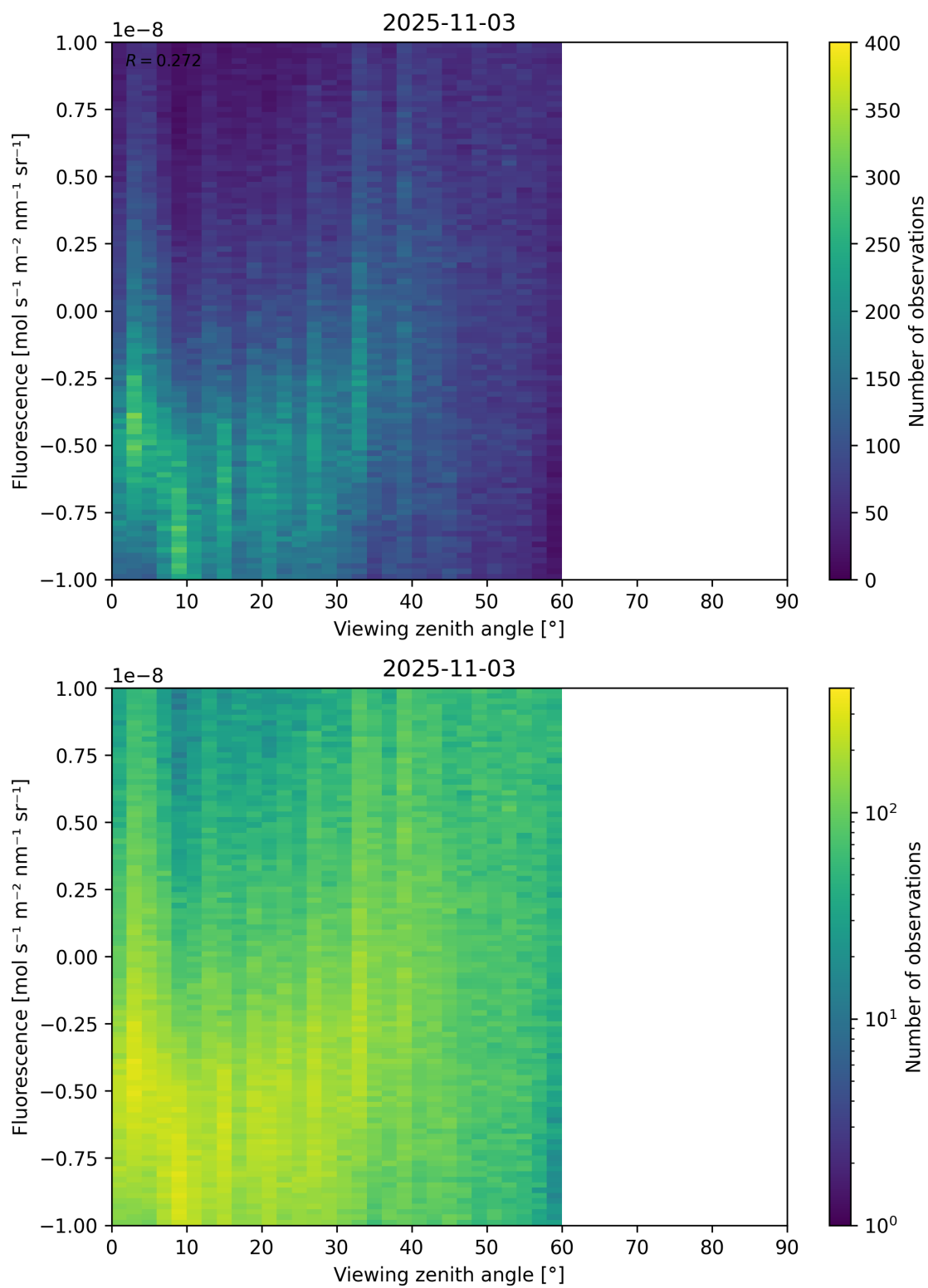
Figure 108: Scatter density plot of “Viewing zenith angle” against “Fluorescence” for 2025-11-02 to 2025-11-04.
