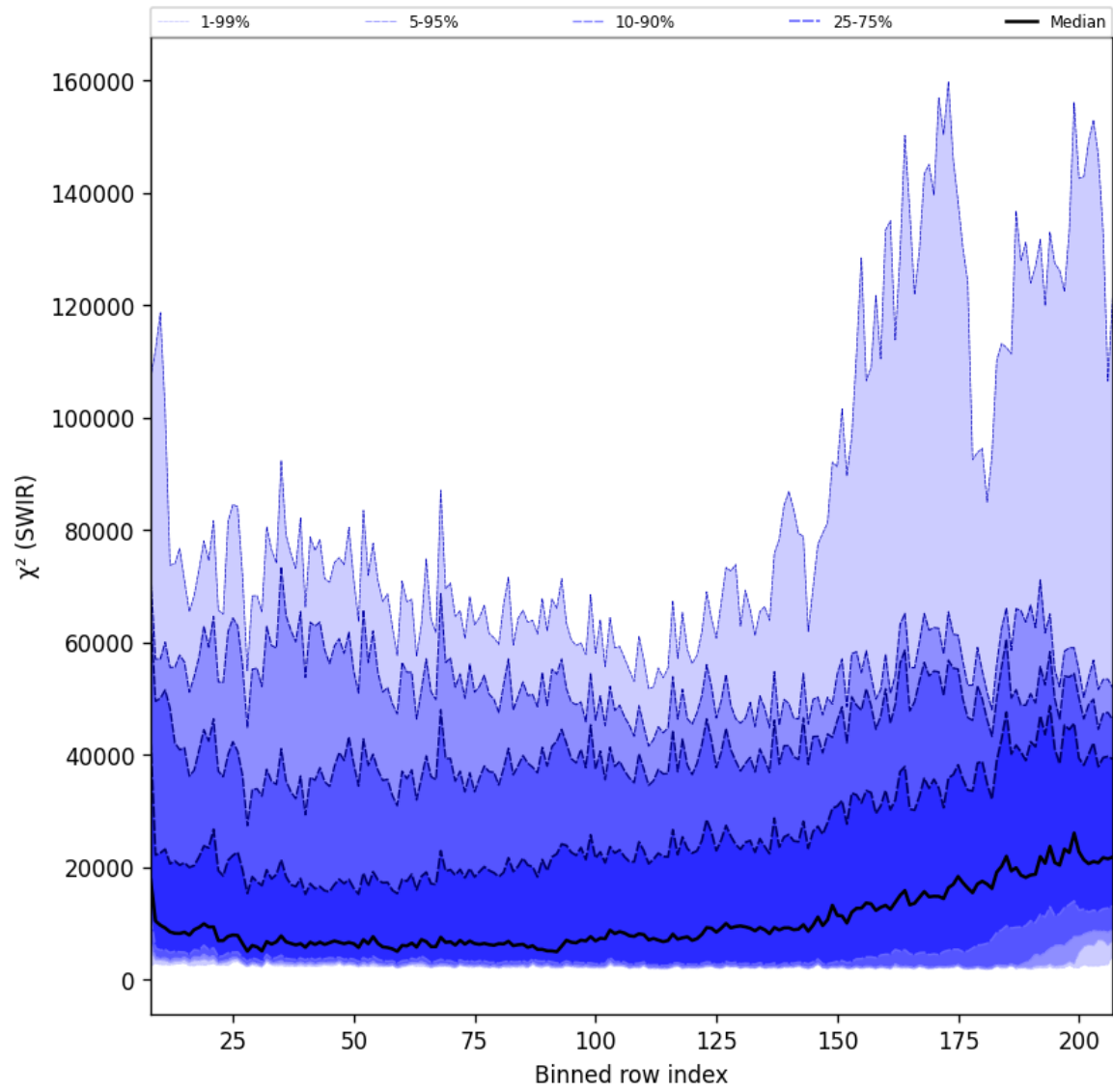
Figure 39: Along track statistics of " \chi^2 (SWIR)" for 2025-11-02 to 2025-11-04
