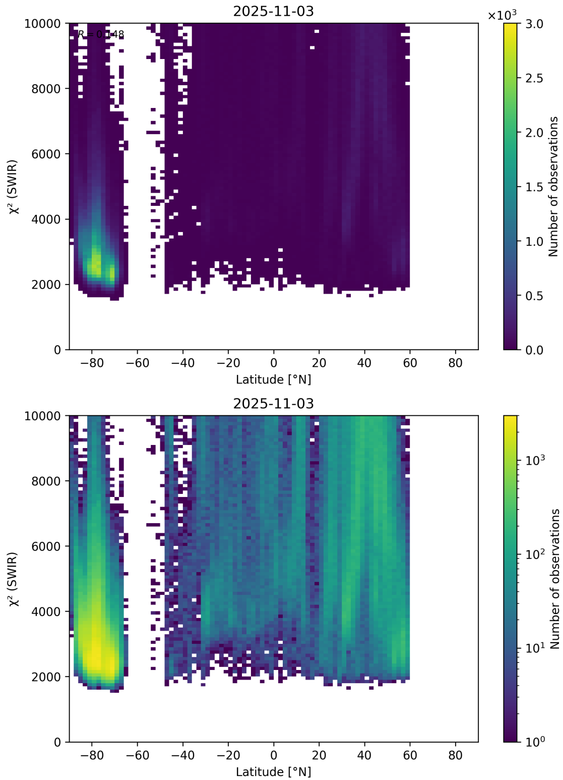
Figure 54: Scatter density plot of “Latitude” against “ \chi^2 (SWIR)” for 2025-11-02 to 2025-11-04.
