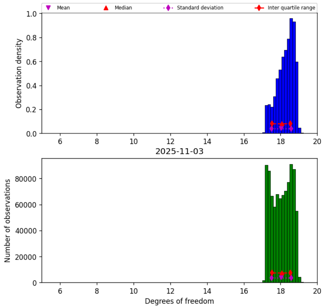
Figure 30: Histogram of “Degrees of freedom” for 2025-11-02 to 2025-11-04
