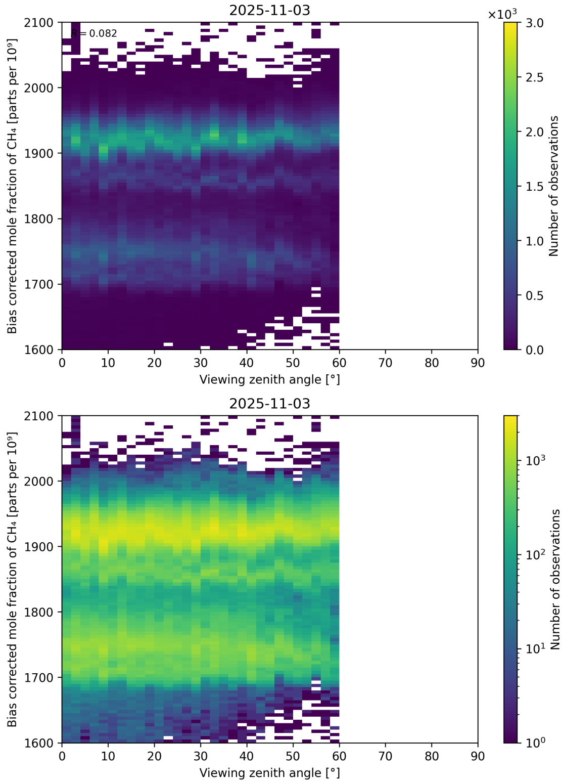
Figure 111: Scatter density plot of “Viewing zenith angle” against “Bias corrected mole fraction of CH 4 ” for 2025-11-02 to 2025-11-04.
