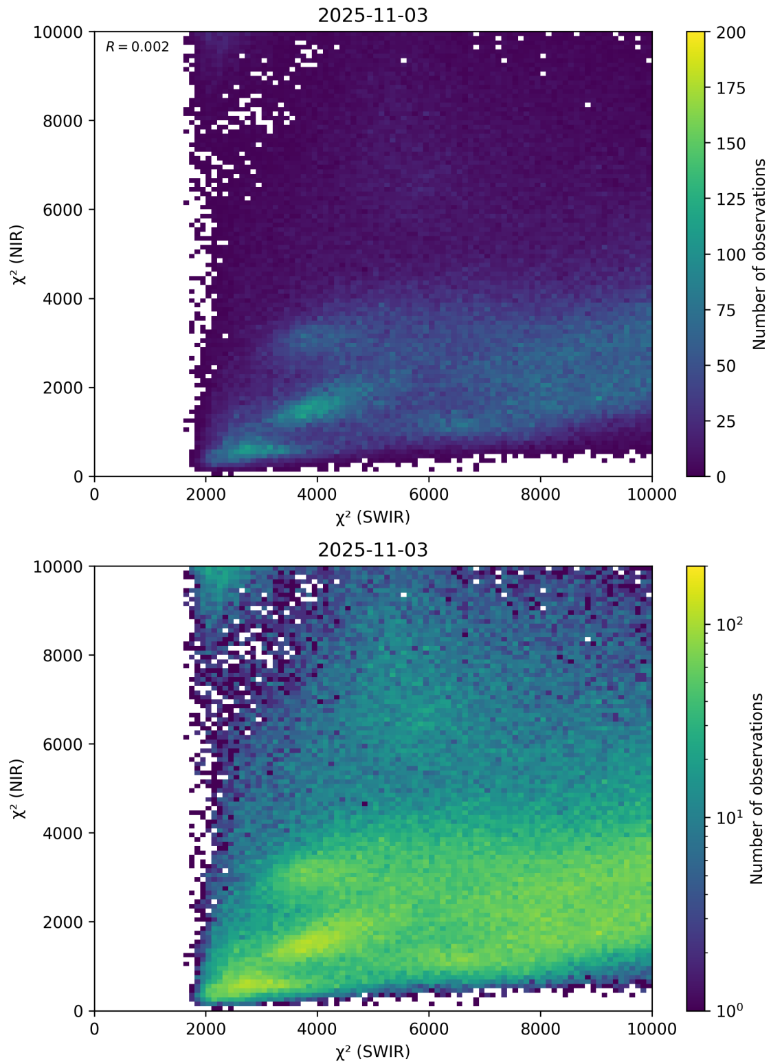
Figure 47: Scatter density plot of “ \chi^2 (SWIR)” against “ \chi^2 (NIR)” for 2025-11-02 to 2025-11-04.
