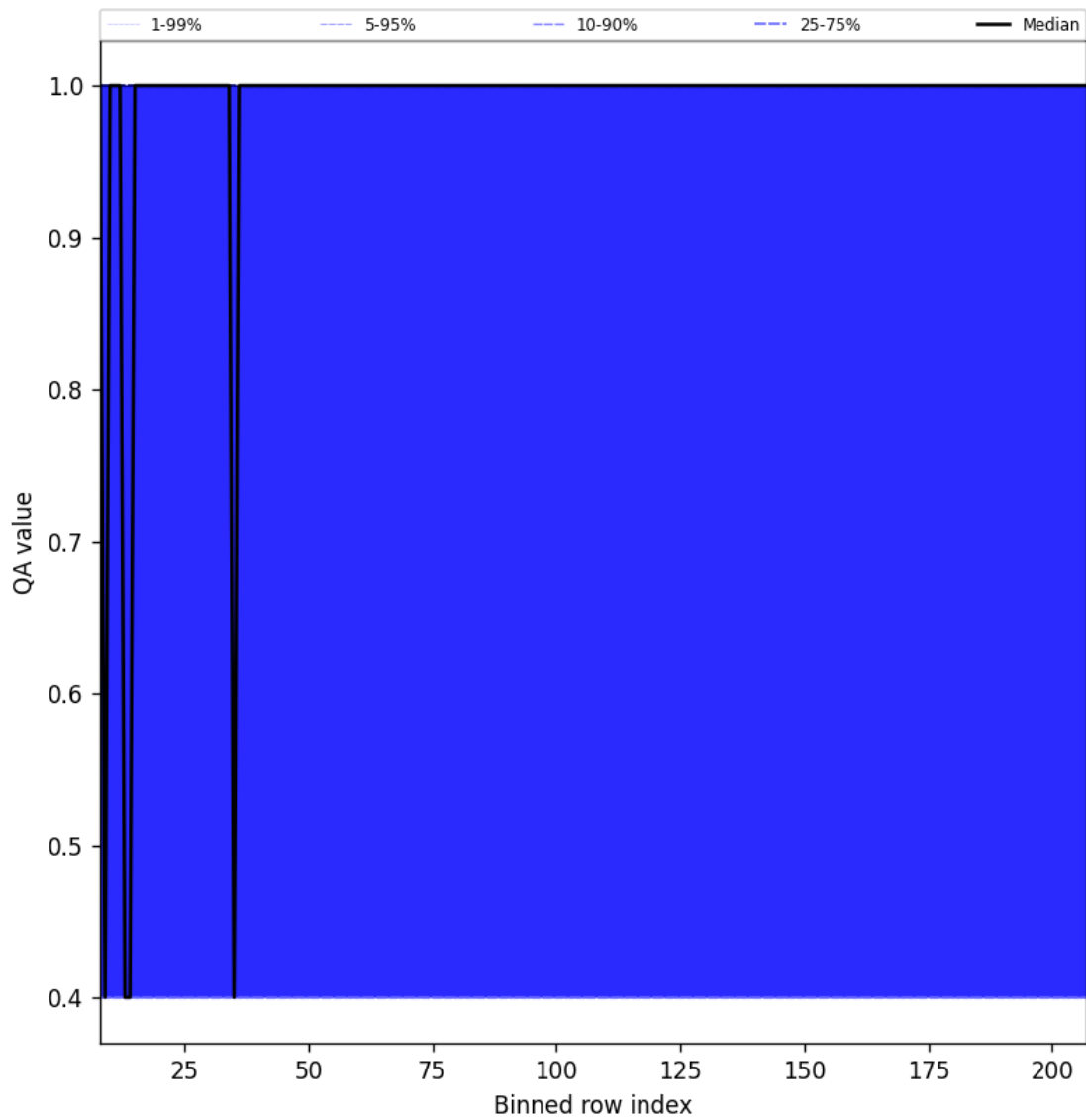
Figure 33: Along track statistics of “QA value” for 2025-11-02 to 2025-11-04
