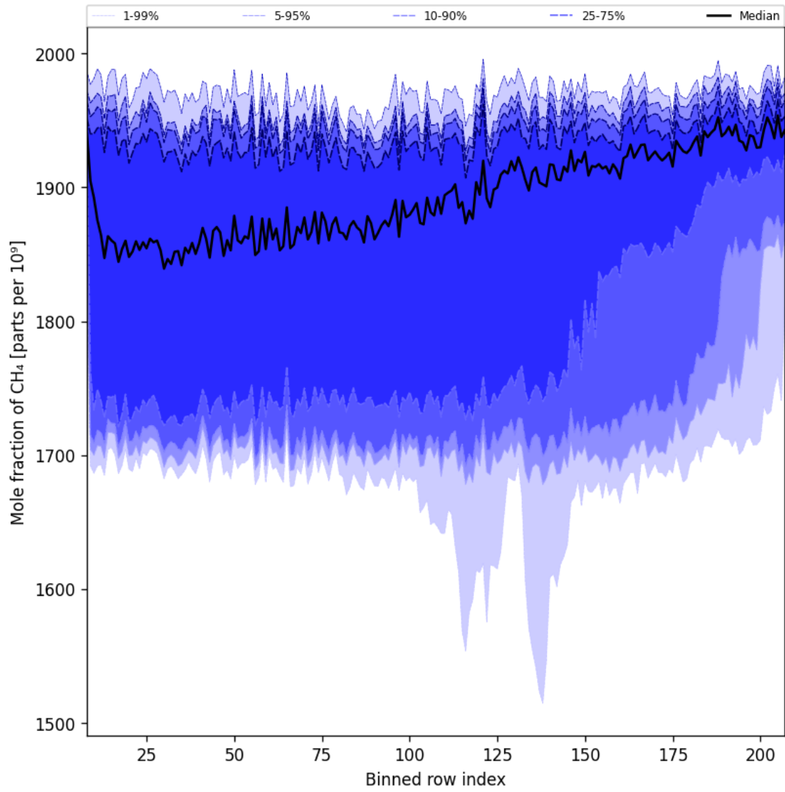
Figure 34: Along track statistics of “Mole fraction of CH 4 ” for 2025-11-02 to 2025-11-04
