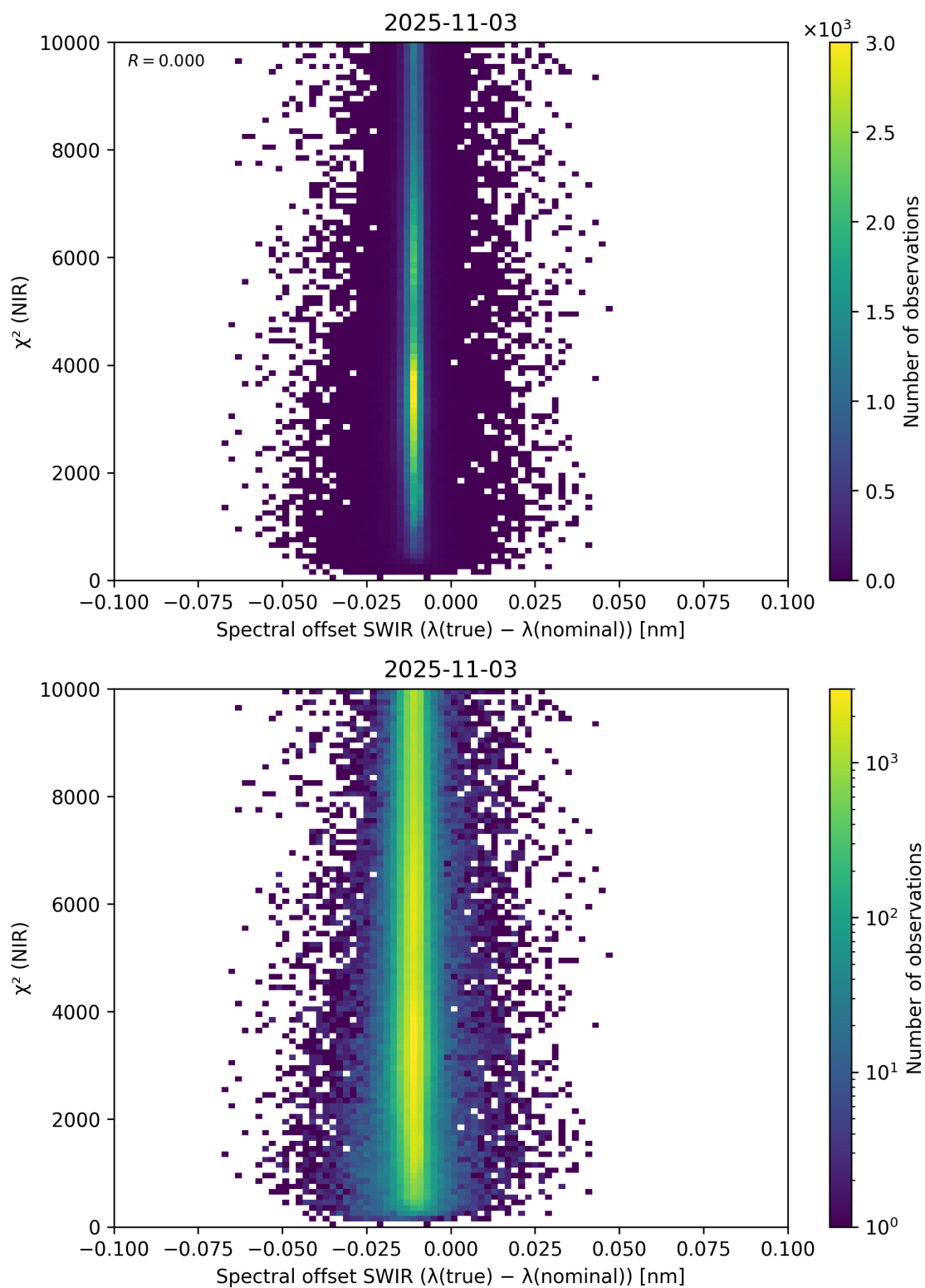
Figure 117: Scatter density plot of “Spectral offset SWIR ( \lambda_{\text{true}} - \lambda_{\text{nominal}} )” against “ \chi^2 (NIR)” for 2025-11-02 to 2025-11-04.
