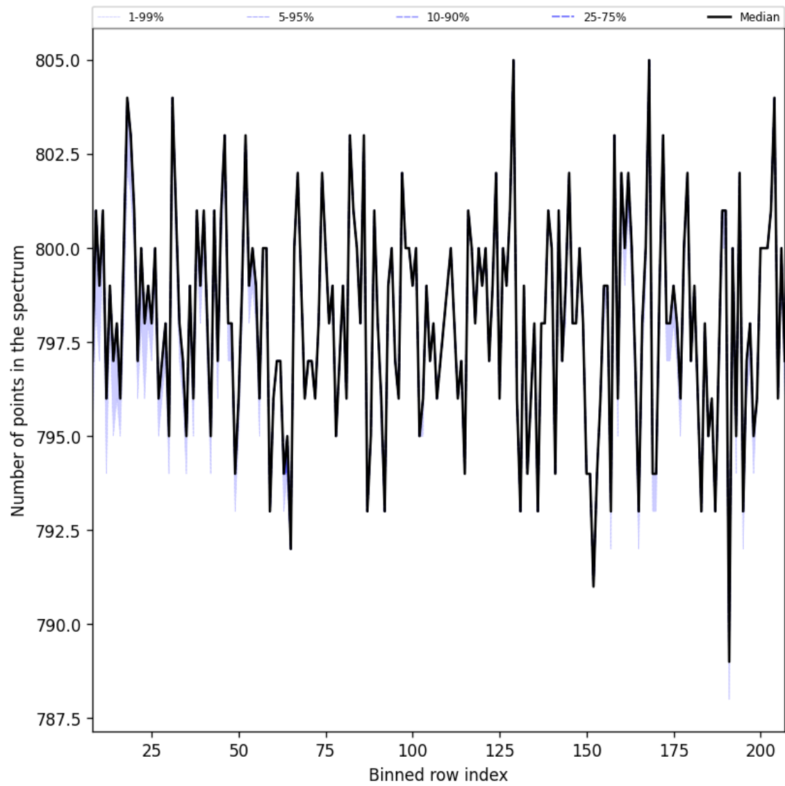
Figure 37: Along track statistics of “Number of points in the spectrum” for 2025-11-02 to 2025-11-04
