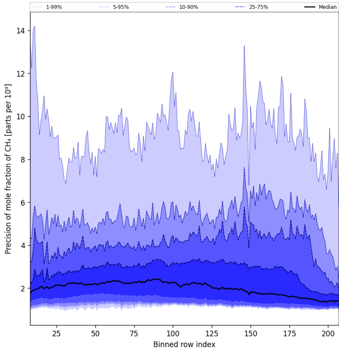
Figure 35: Along track statistics of “Precision of mole fraction of CH 4 ” for 2025-11-02 to 2025-11-04
