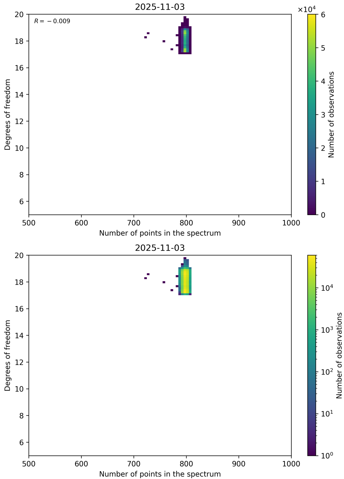
Figure 90: Scatter density plot of “Number of points in the spectrum” against “Degrees of freedom” for 2025-11-02 to 2025-11-04.
