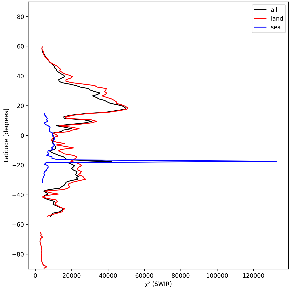
Figure 17: Zonal average of “ \chi^2 (SWIR)” for 2025-11-02 to 2025-11-04.
