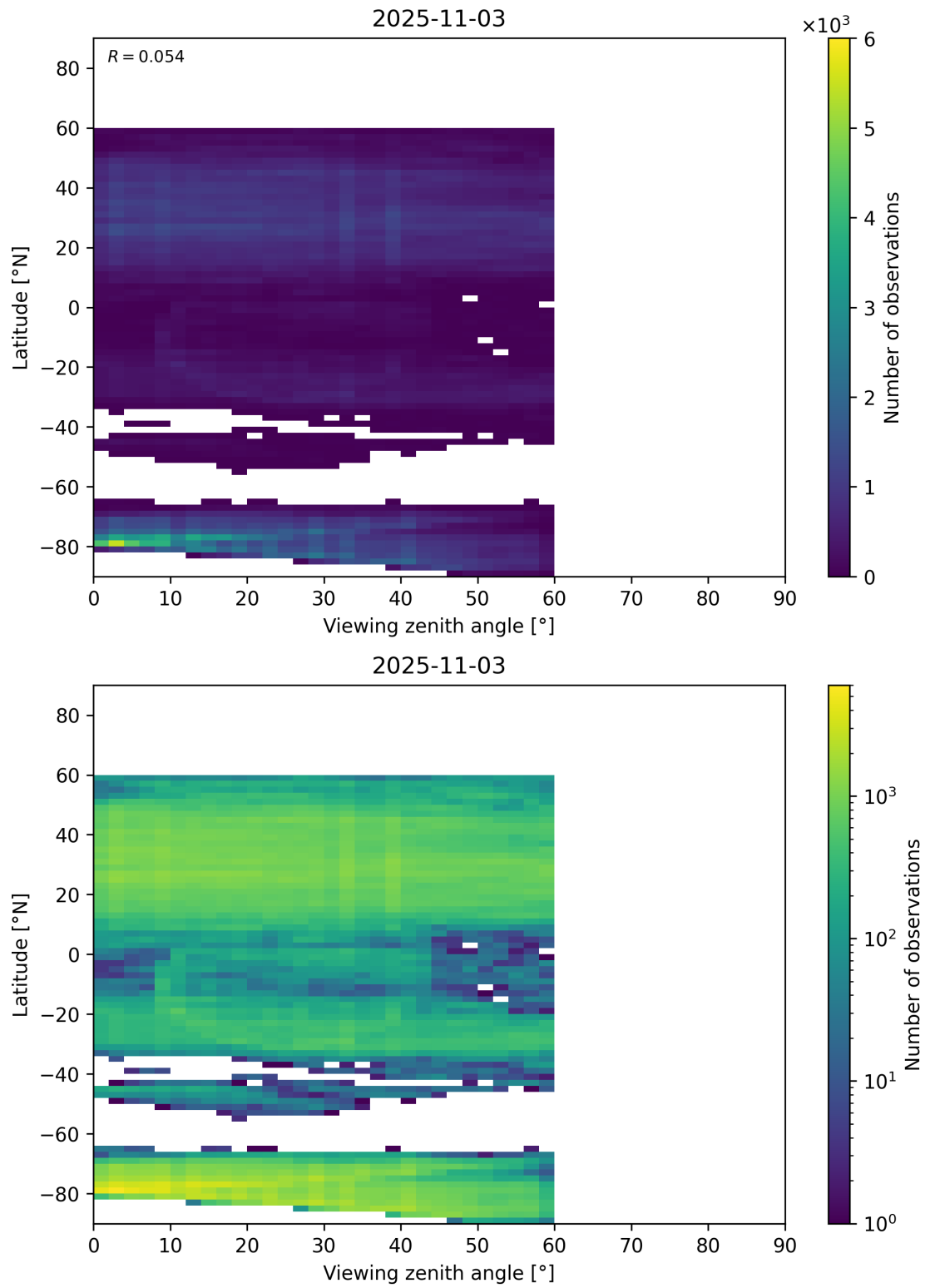
Figure 109: Scatter density plot of “Viewing zenith angle” against “Latitude” for 2025-11-02 to 2025-11-04.
