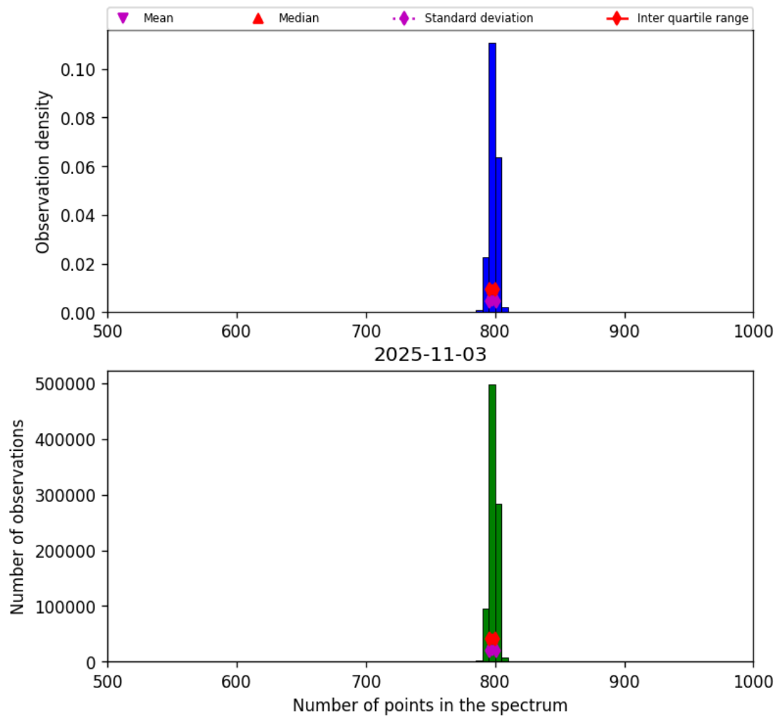
Figure 26: Histogram of “Number of points in the spectrum” for 2025-11-02 to 2025-11-04
