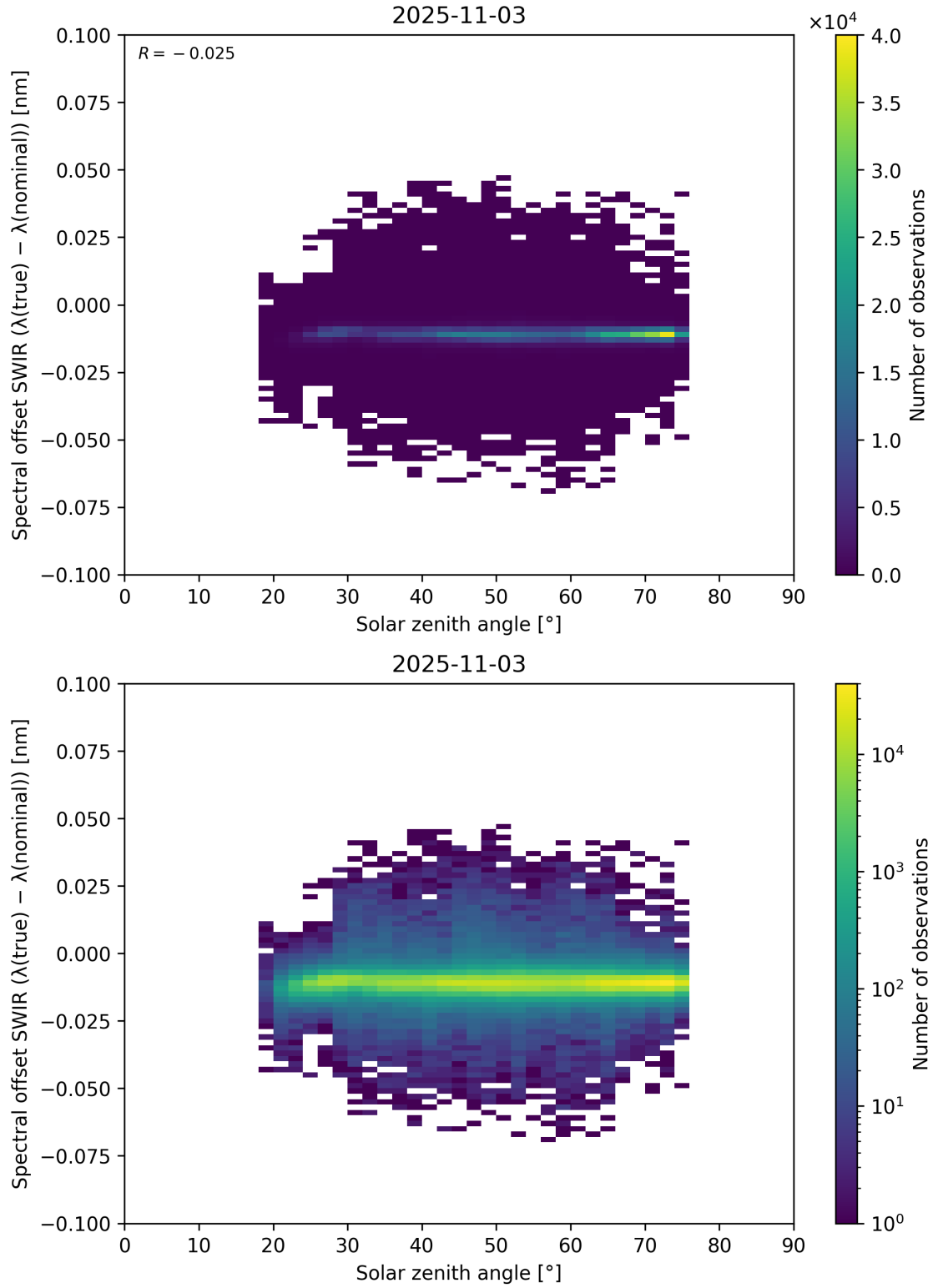
Figure 104: Scatter density plot of “Solar zenith angle” against “Spectral offset SWIR ( \lambda_{\text{true}} - \lambda_{\text{nominal}} )” for 2025-11-02 to 2025-11-04.
