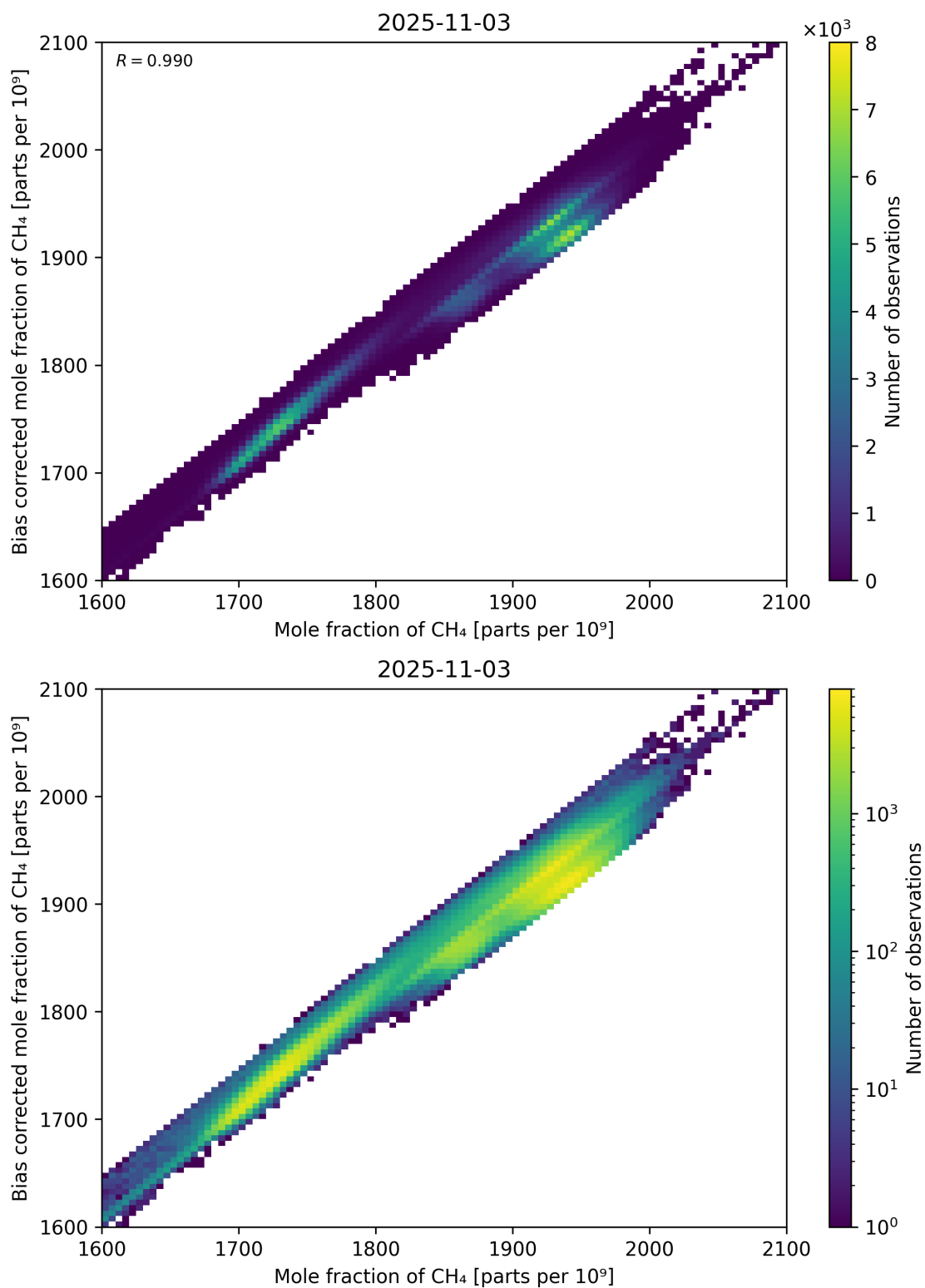
Figure 74: Scatter density plot of “Mole fraction of CH 4 ” against “Bias corrected mole fraction of CH 4 ” for 2025-11-02 to 2025-11-04.
