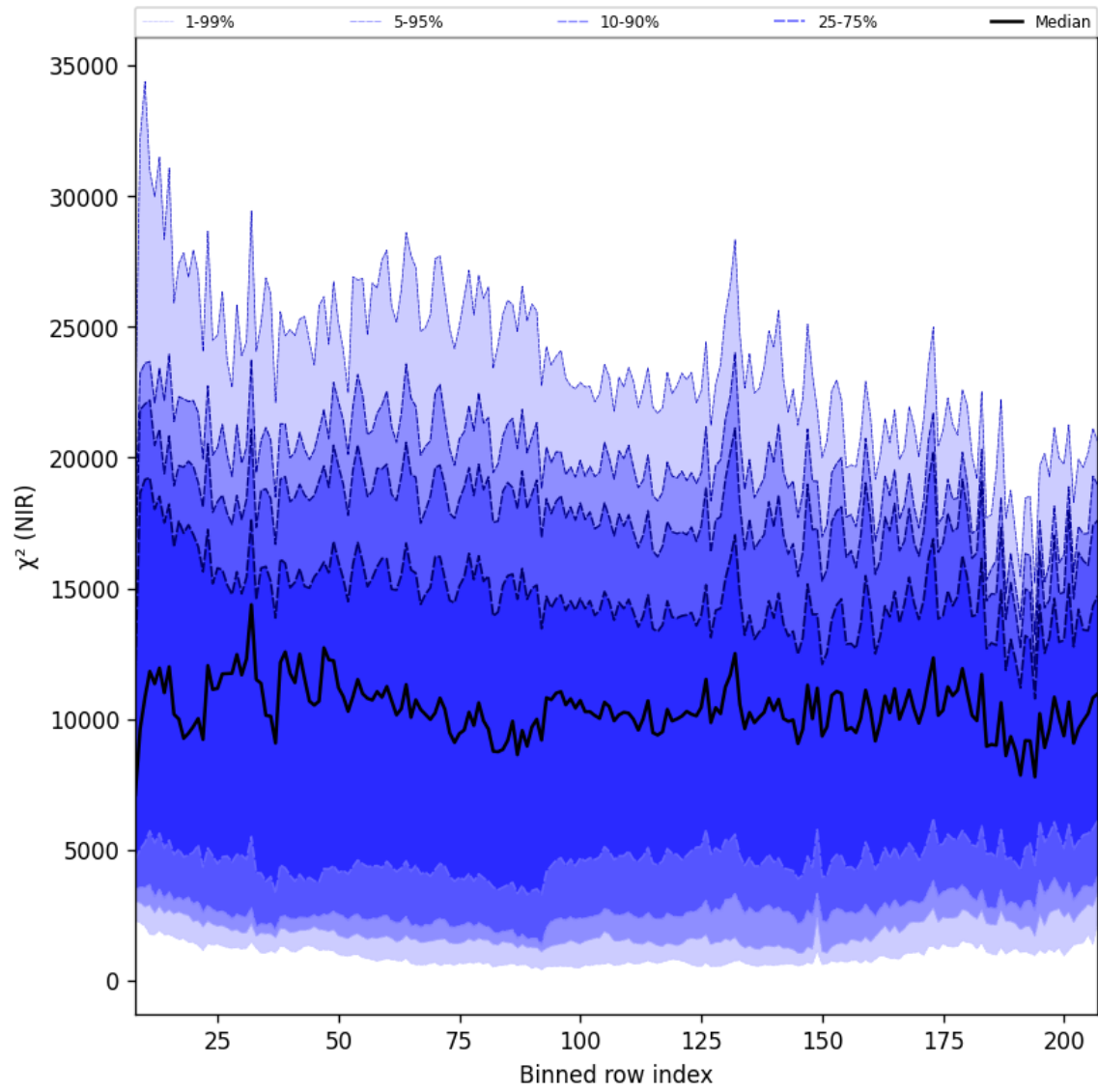
Figure 40: Along track statistics of “ \chi^2 (NIR)” for 2025-11-02 to 2025-11-04
