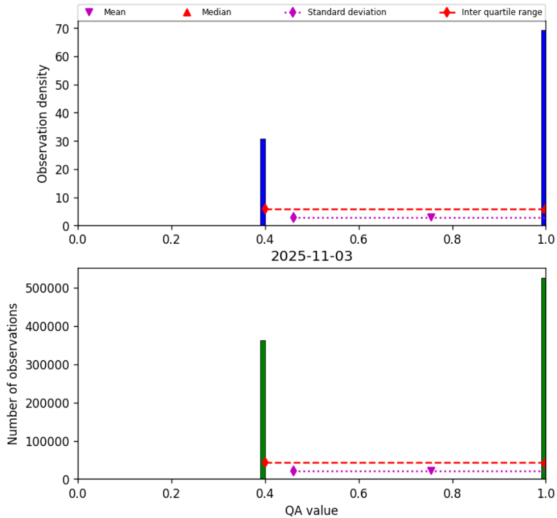
Figure 22: Histogram of “QA value” for 2025-11-02 to 2025-11-04
