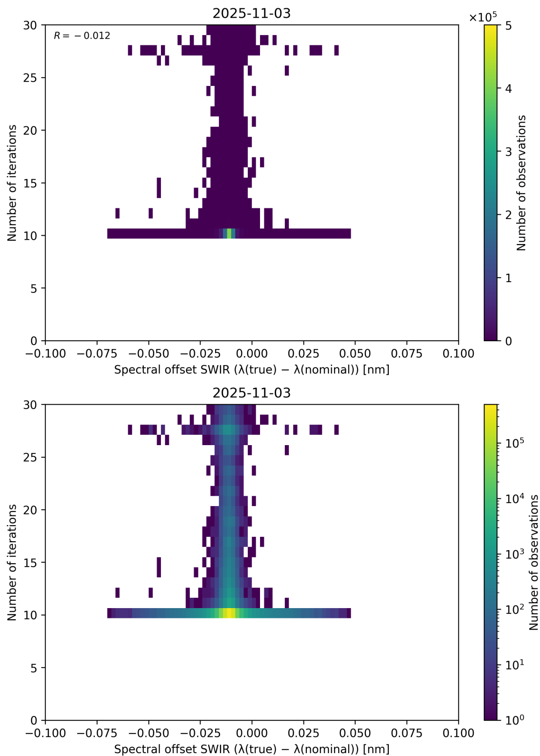
Figure 121: Scatter density plot of “Spectral offset SWIR ( \lambda_{\text{true}} - \lambda_{\text{nominal}} )” against “Number of iterations” for 2025-11-02 to 2025-11-04.
