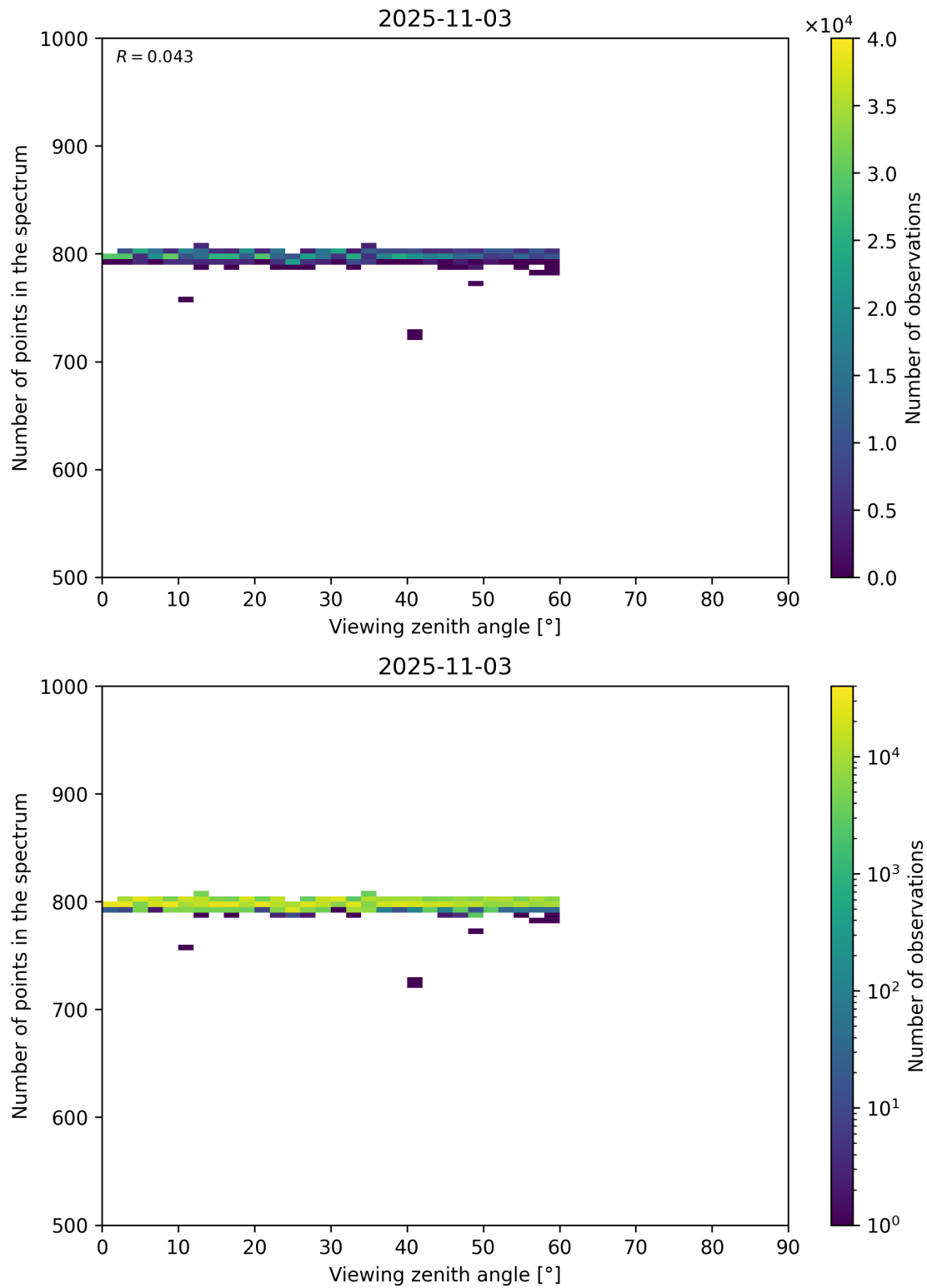
Figure 114: Scatter density plot of “Viewing zenith angle” against “Number of points in the spectrum” for 2025-11-02 to 2025-11-04.
