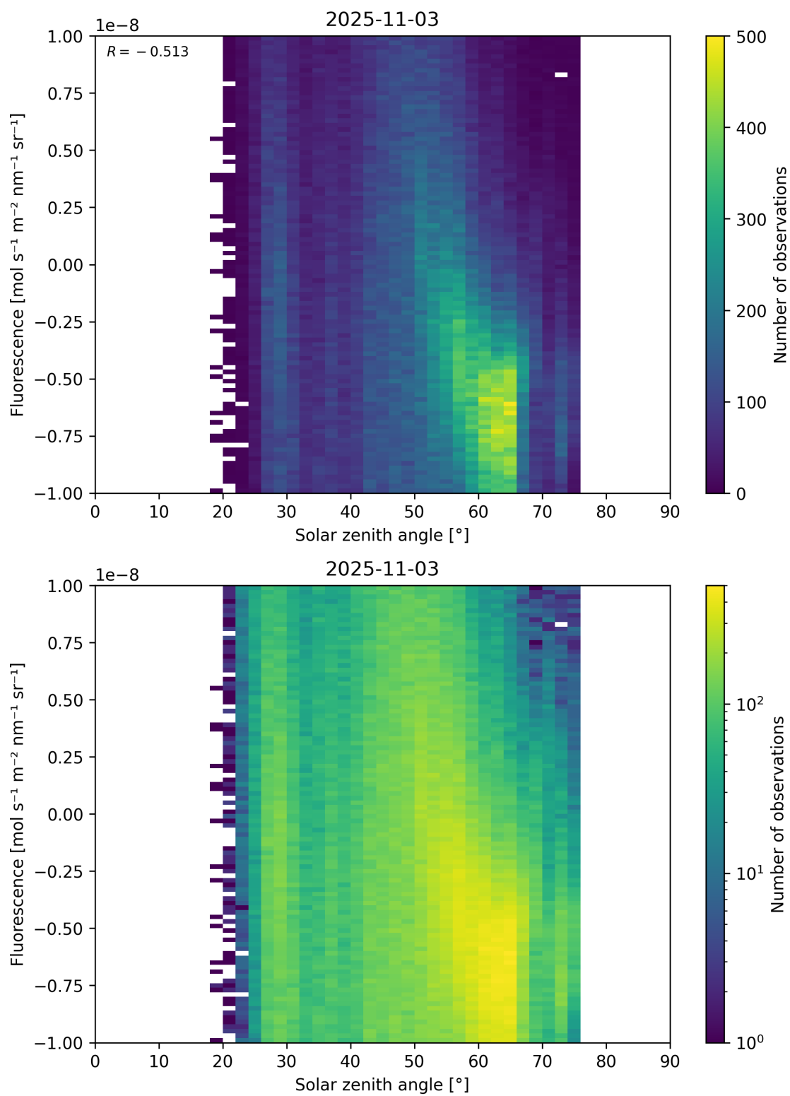
Figure 97: Scatter density plot of “Solar zenith angle” against “Fluorescence” for 2025-11-02 to 2025-11-04.
