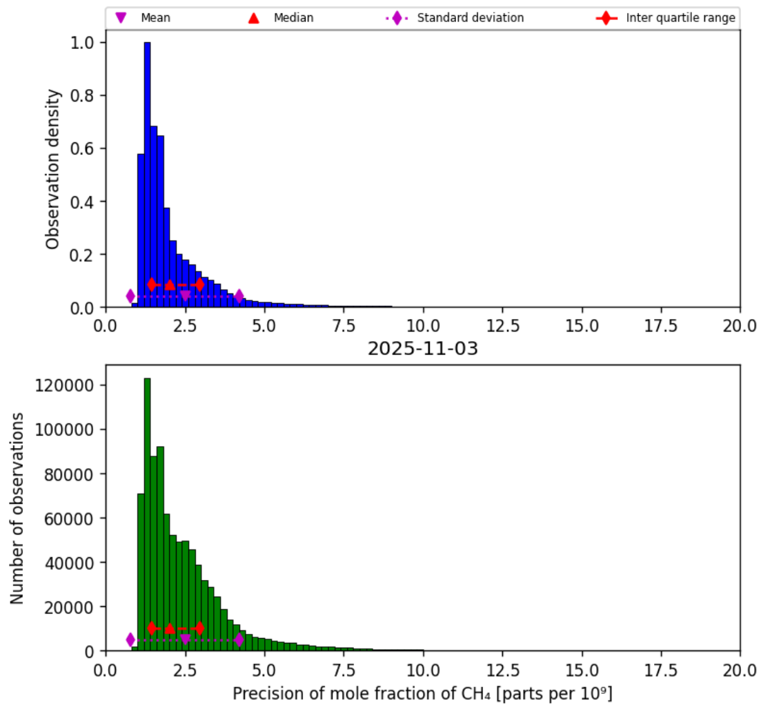
Figure 24: Histogram of “Precision of mole fraction of CH 4 ” for 2025-11-02 to 2025-11-04
