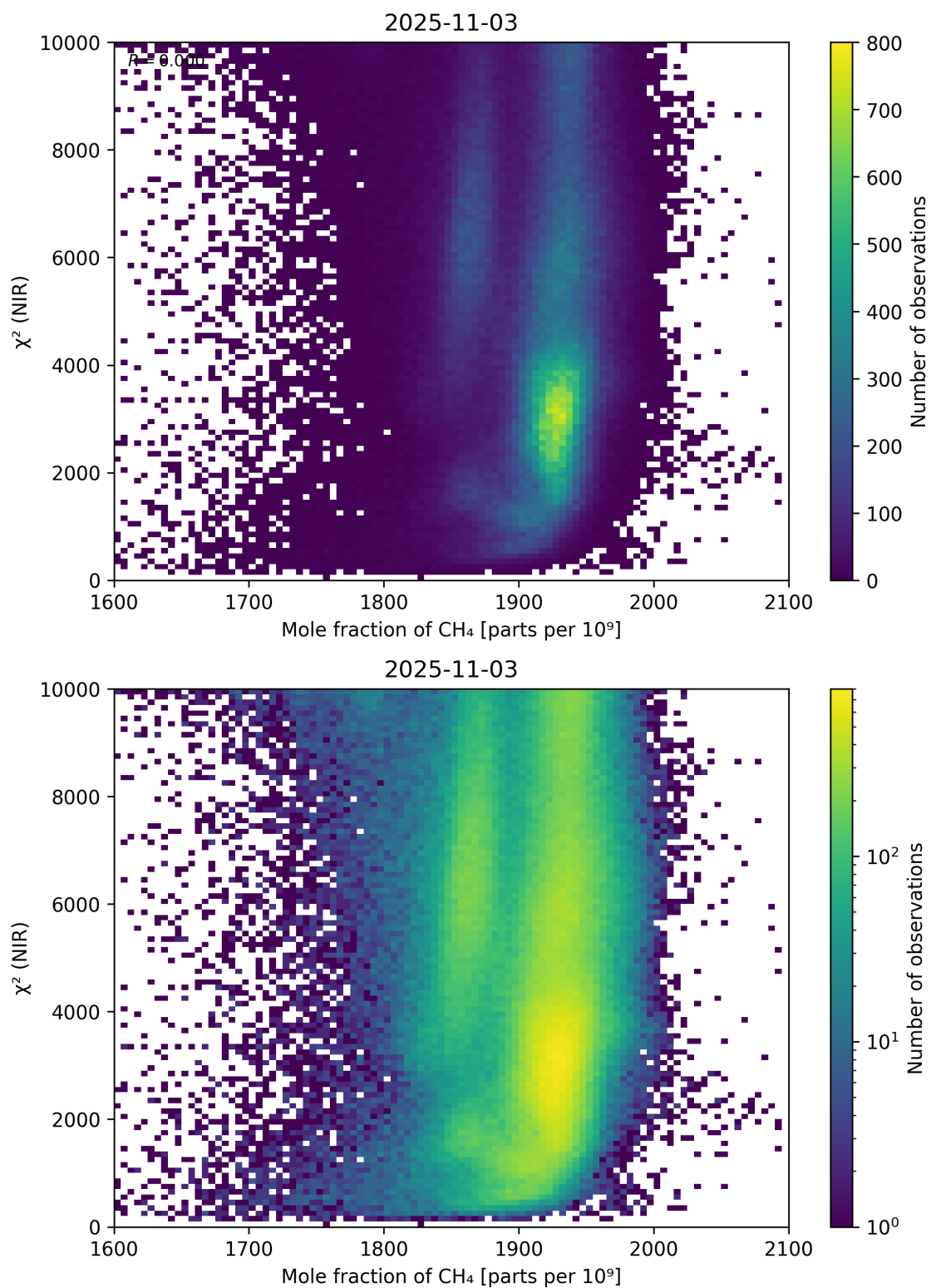
Figure 70: Scatter density plot of “Mole fraction of CH 4 ” against “ \chi^2 (NIR)” for 2025-11-02 to 2025-11-04.
