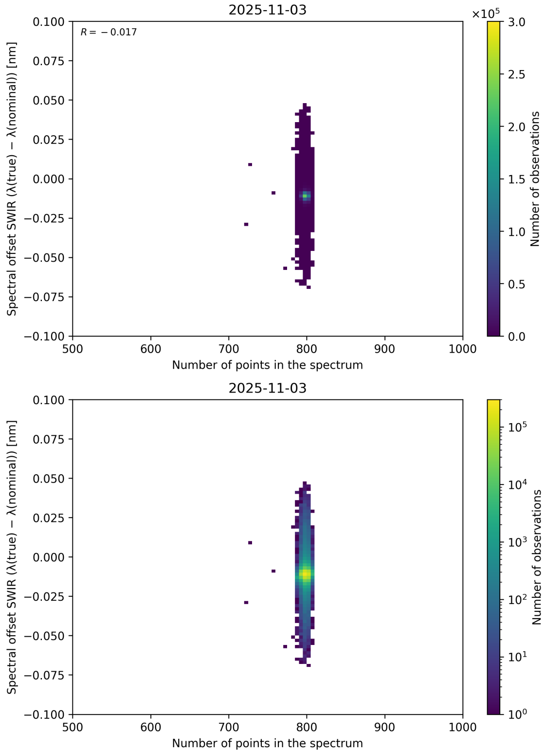
Figure 93: Scatter density plot of “Number of points in the spectrum” against “Spectral offset SWIR ( \lambda_{\text{true}} - \lambda_{\text{nominal}} )” for 2025-11-02 to 2025-11-04.
