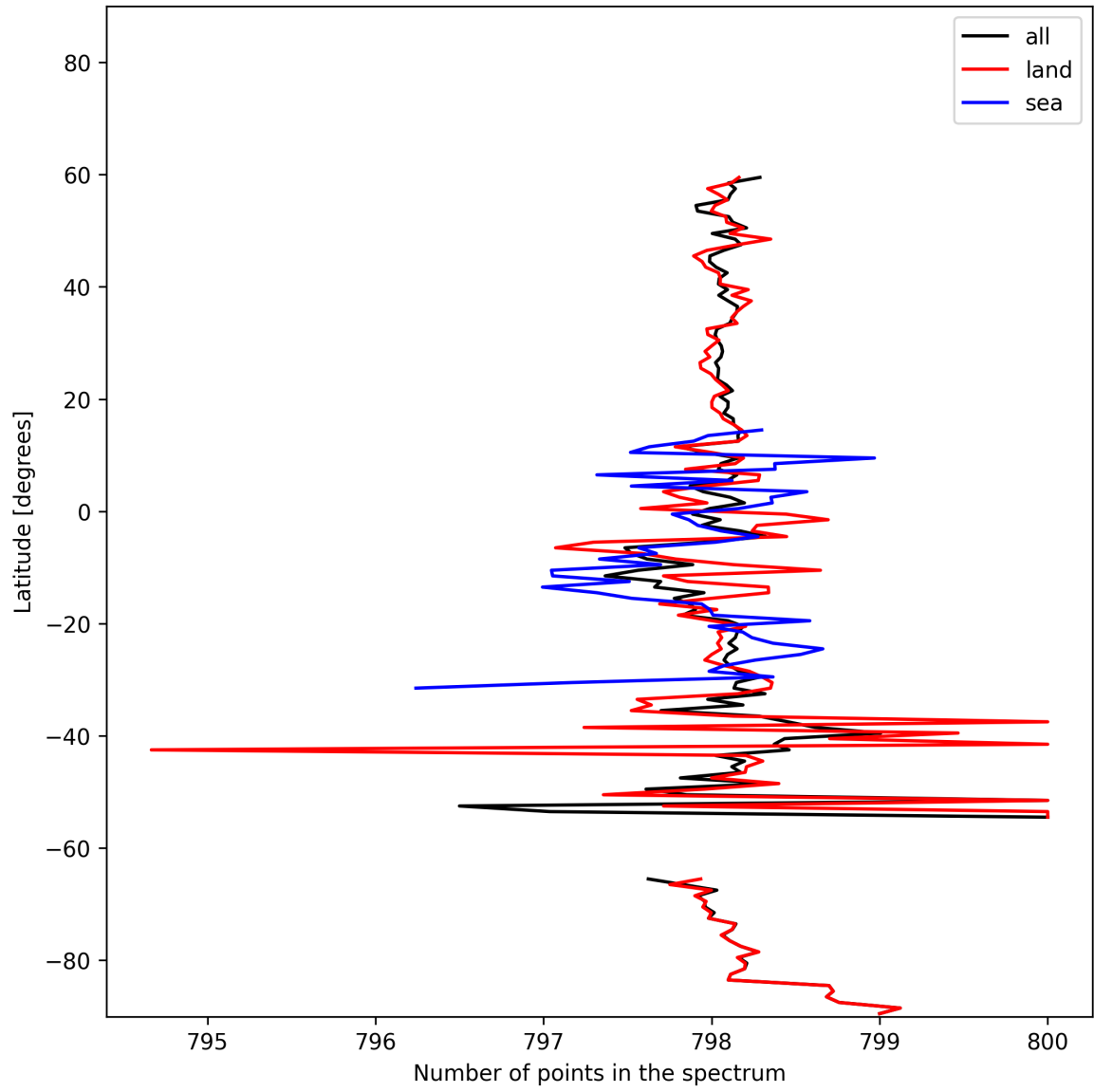
Figure 15: Zonal average of “Number of points in the spectrum” for 2025-11-02 to 2025-11-04.
