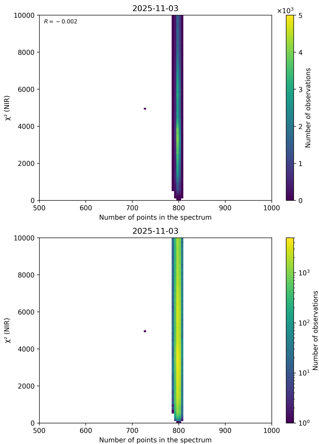
Figure 88: Scatter density plot of “Number of points in the spectrum” against “ \chi^2 (NIR)” for 2025-11-02 to 2025-11-04.
