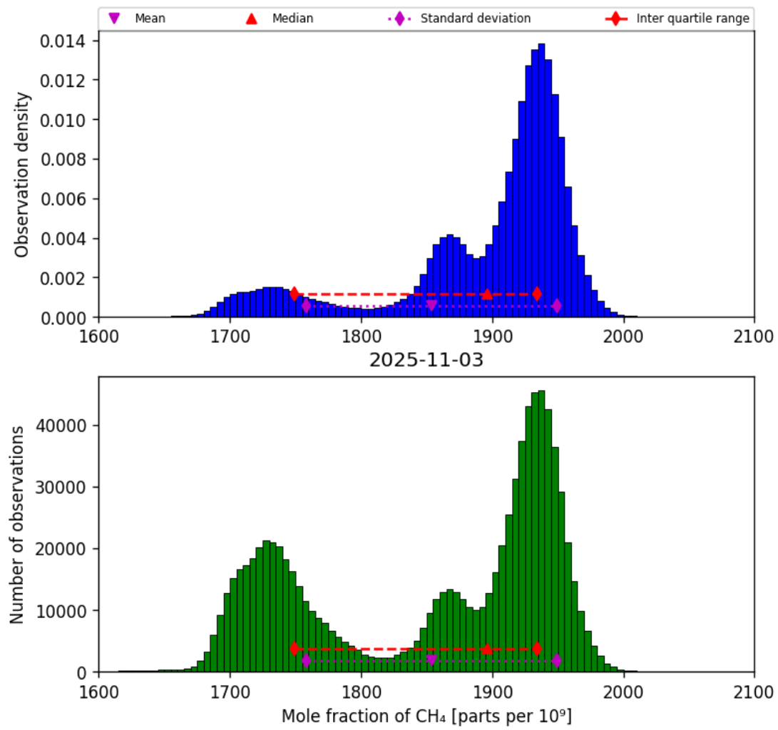
Figure 23: Histogram of “Mole fraction of CH 4 ” for 2025-11-02 to 2025-11-04
