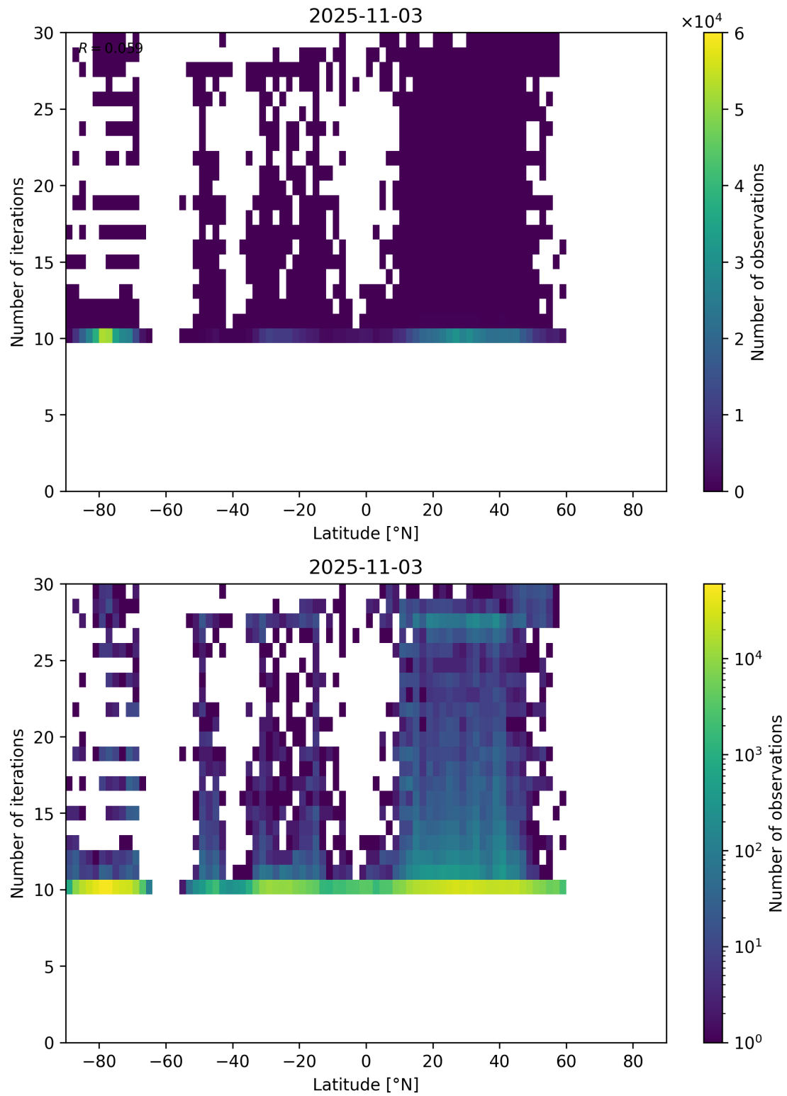
Figure 60: Scatter density plot of “Latitude” against “Number of iterations” for 2025-11-02 to 2025-11-04.
