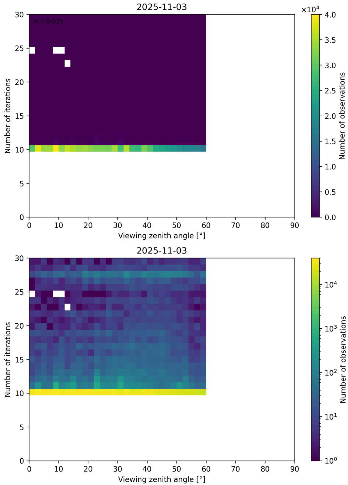
Figure 113: Scatter density plot of “Viewing zenith angle” against “Number of iterations” for 2025-11-02 to 2025-11-04.
