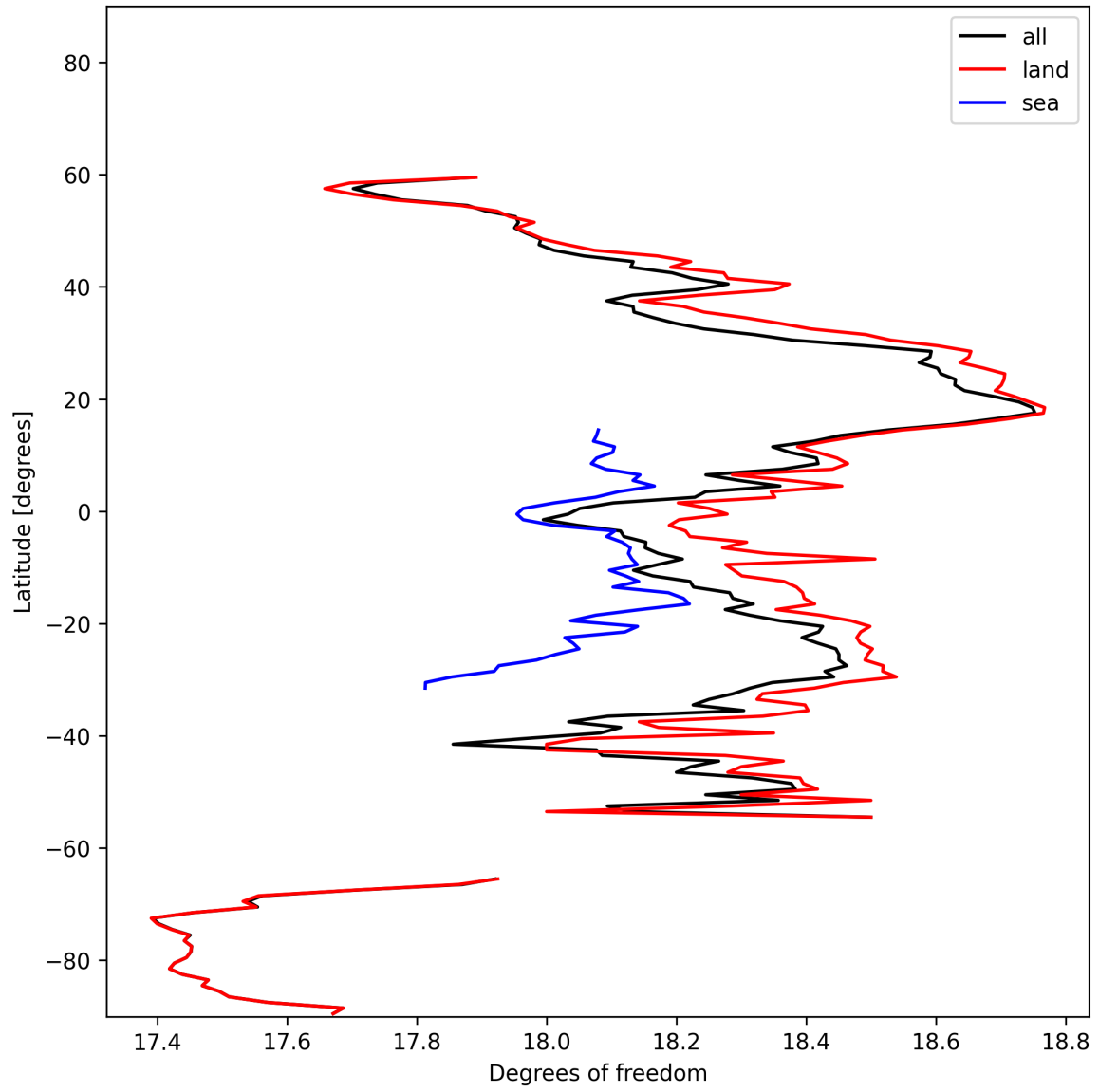
Figure 19: Zonal average of “Degrees of freedom” for 2025-11-02 to 2025-11-04.
