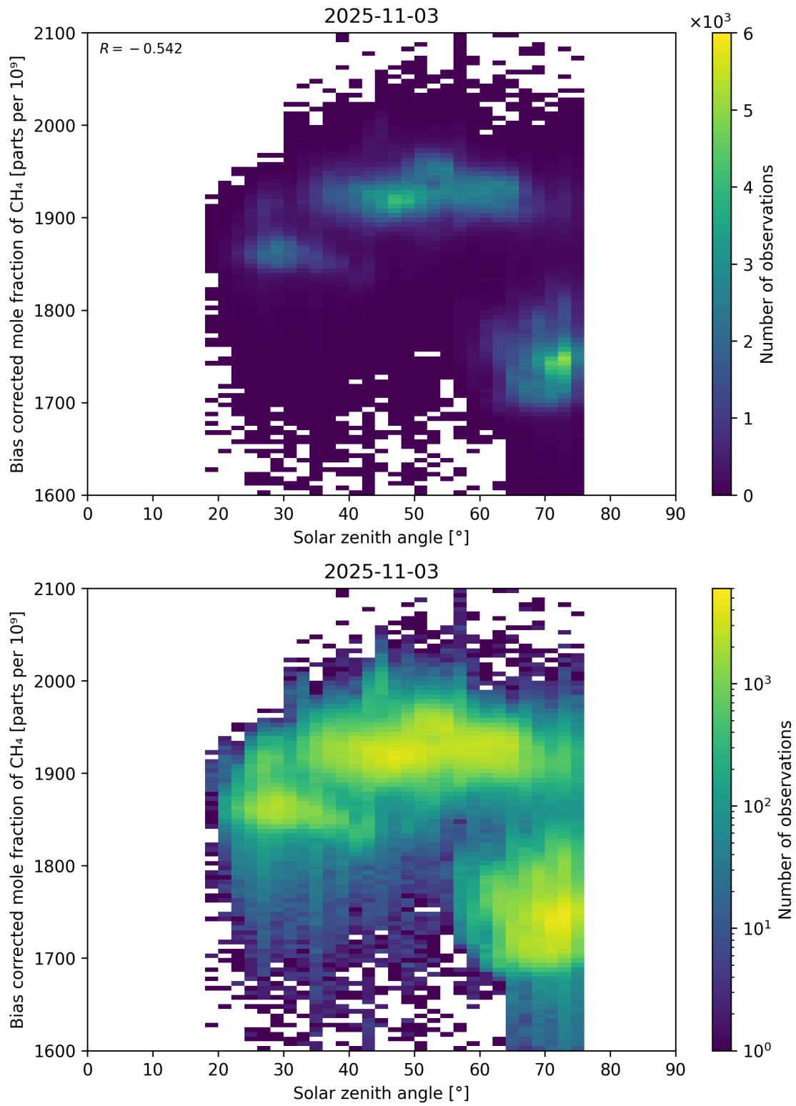
Figure 100: Scatter density plot of “Solar zenith angle” against “Bias corrected mole fraction of CH 4 ” for 2025-11-02 to 2025-11-04.
