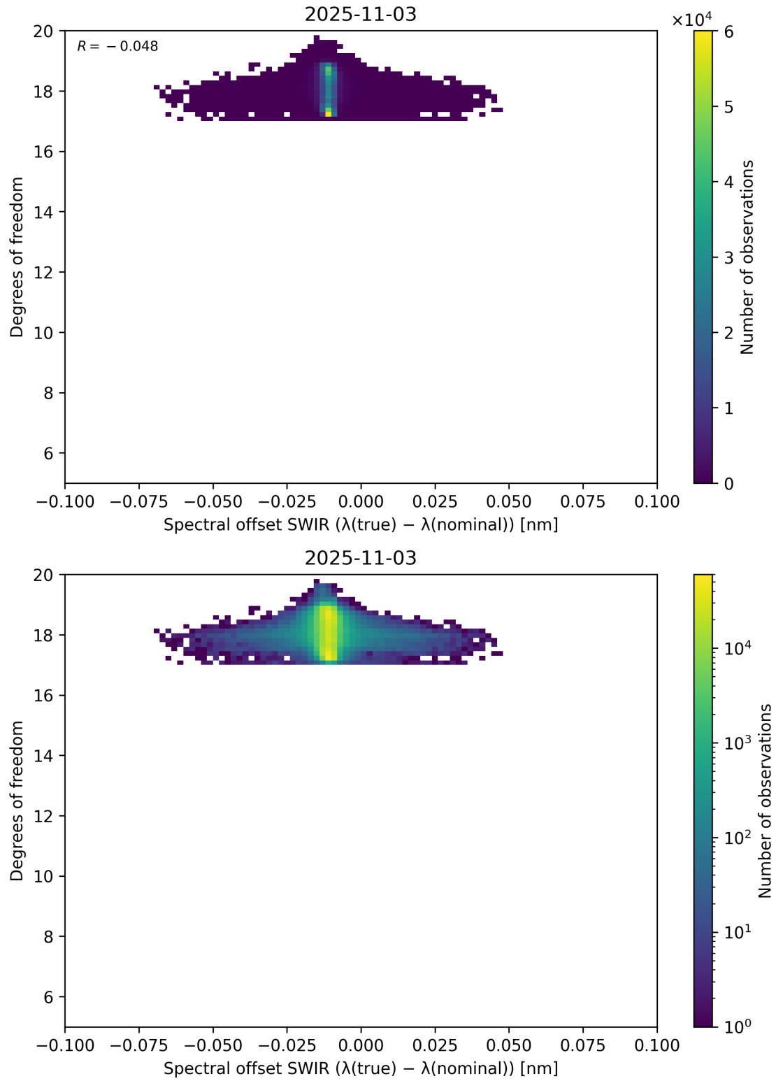
Figure 119: Scatter density plot of “Spectral offset SWIR ( \lambda_{\text{true}} - \lambda_{\text{nominal}} )” against “Degrees of freedom” for 2025-11-02 to 2025-11-04.
