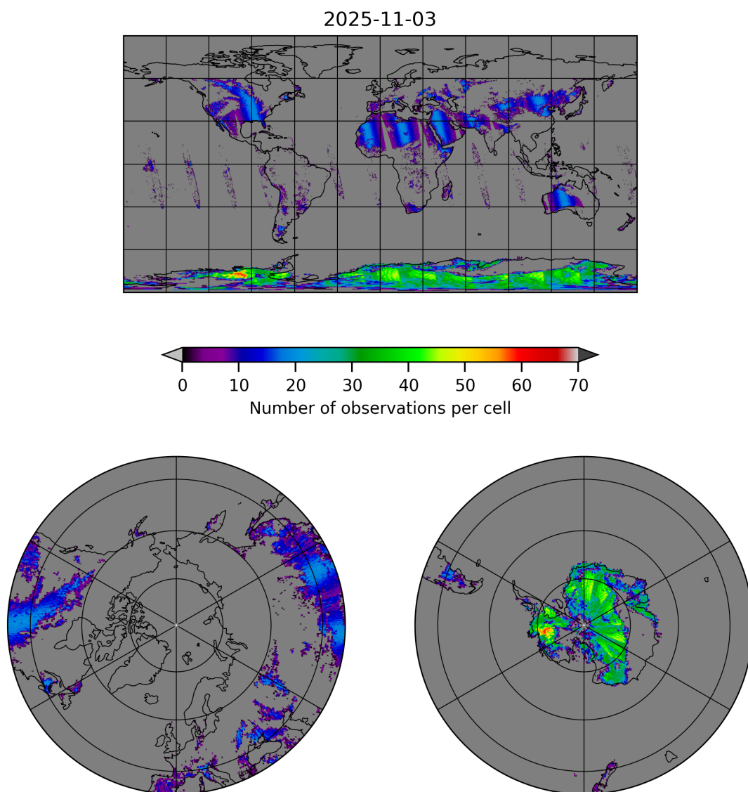
Figure 10: Map of the number of observations for 2025-11-02 to 2025-11-04
