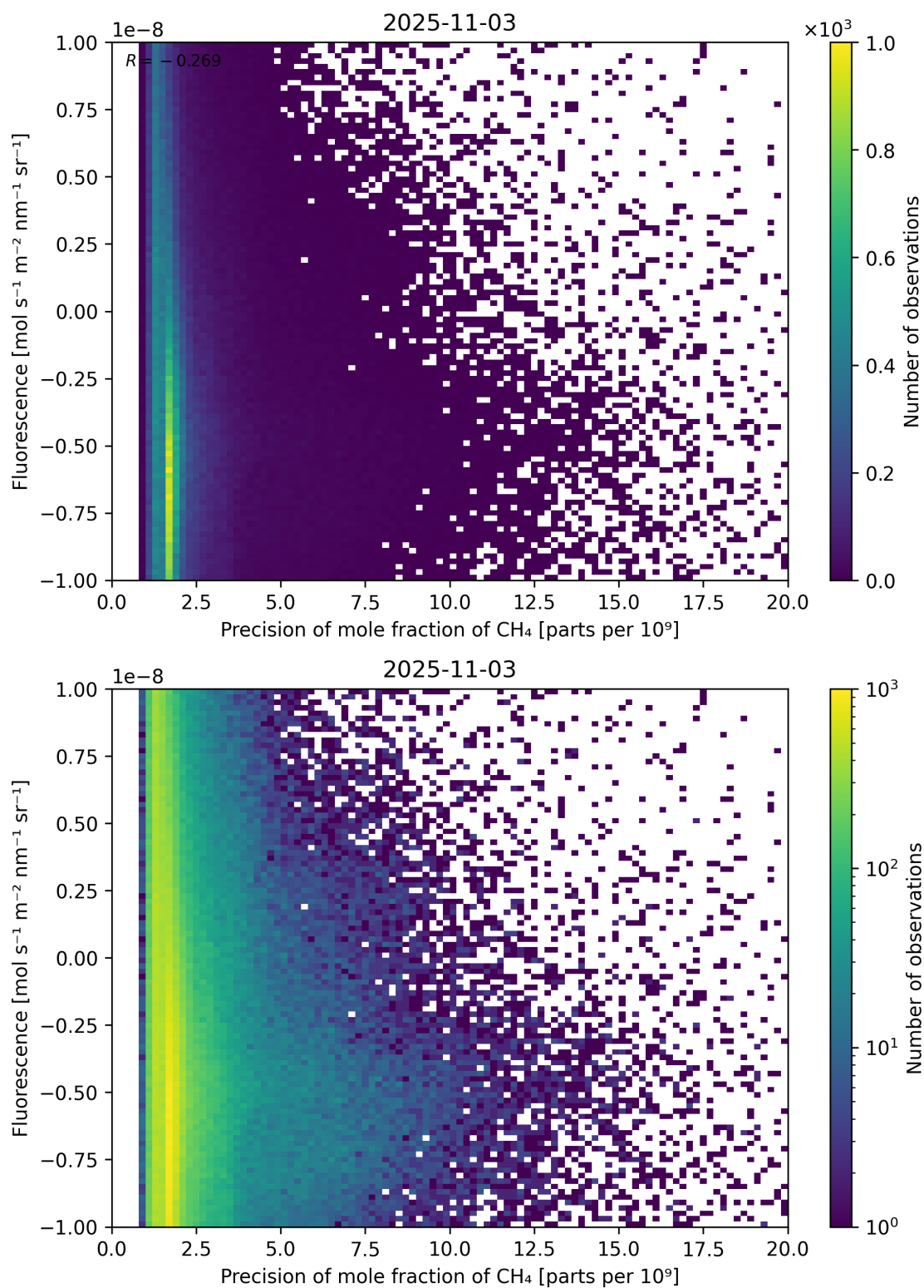
Figure 81: Scatter density plot of “Precision of mole fraction of CH 4 ” against “Fluorescence” for 2025-11-02 to 2025-11-04.
