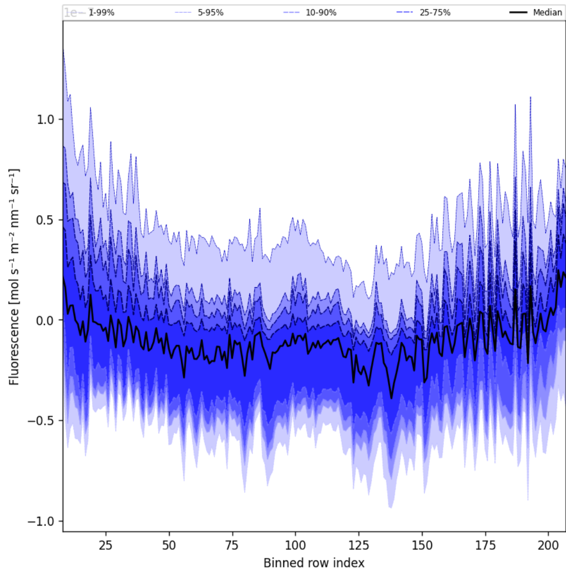
Figure 43: Along track statistics of “Fluorescence” for 2025-11-02 to 2025-11-04
