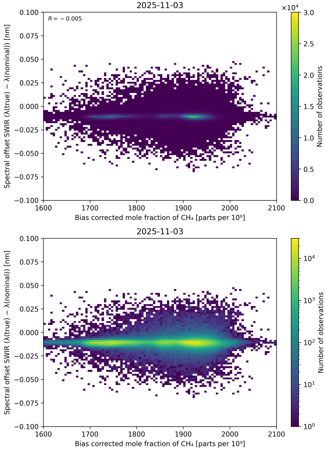
Figure 69: Scatter density plot of “Bias corrected mole fraction of \text{CH}_4 ” against “Spectral offset SWIR ( \lambda_{\text{true}} - \lambda_{\text{nominal}} )” for 2025-11-02 to 2025-11-04.
