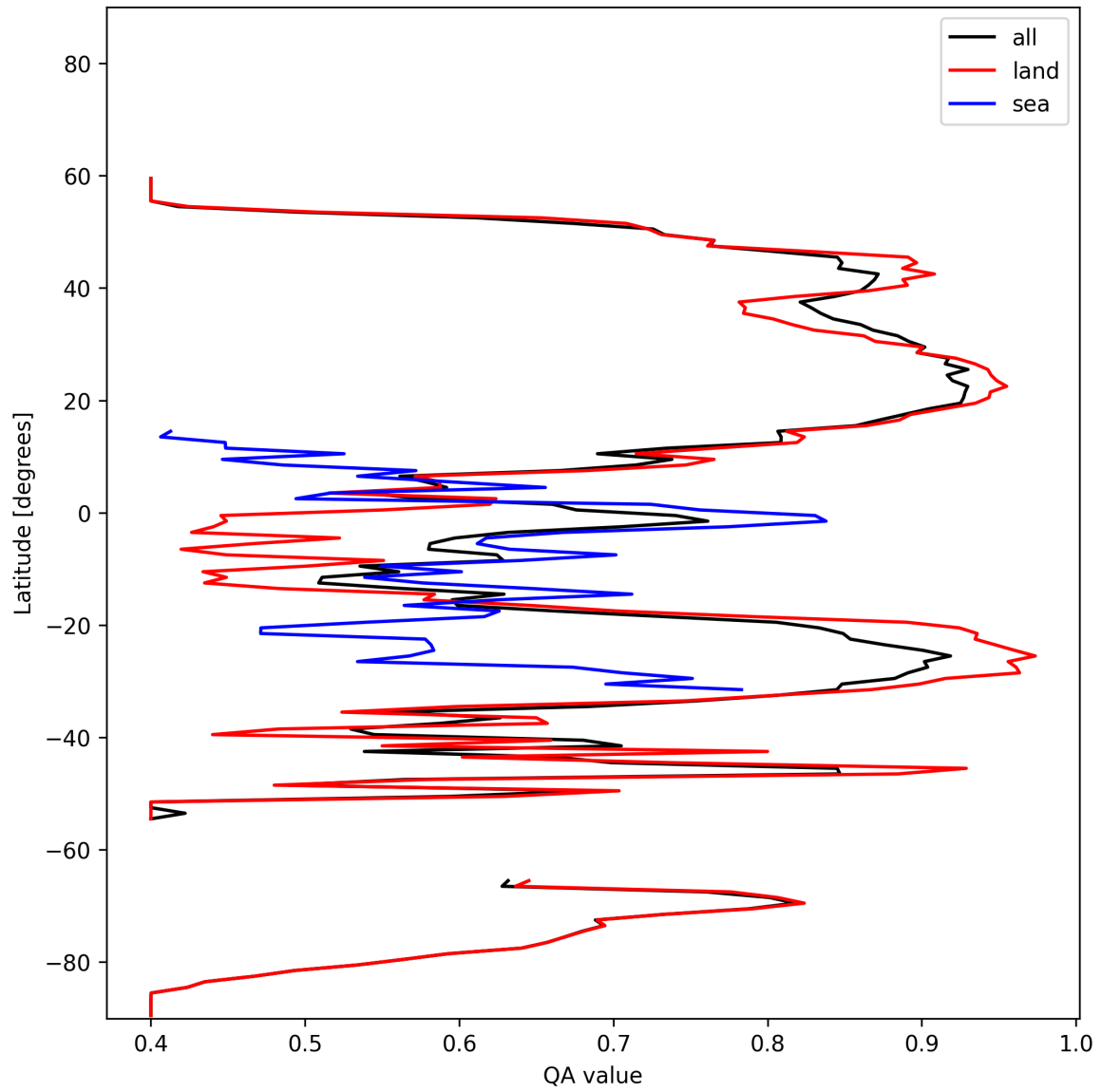
Figure 11: Zonal average of “QA value” for 2025-11-02 to 2025-11-04.
