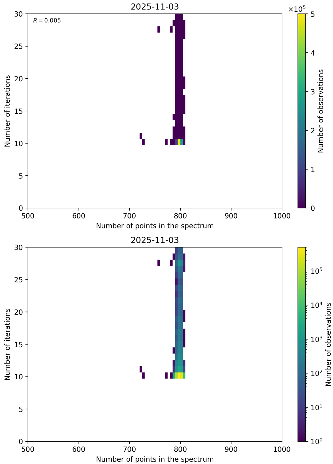
Figure 92: Scatter density plot of “Number of points in the spectrum” against “Number of iterations” for 2025-11-02 to 2025-11-04.
