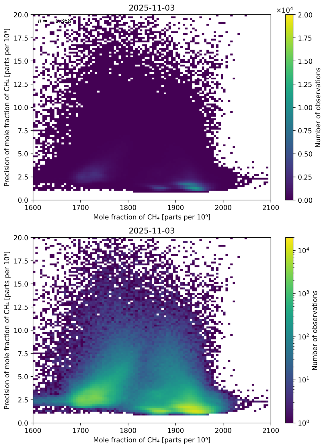
Figure 75: Scatter density plot of “Mole fraction of CH 4 ” against “Precision of mole fraction of CH 4 ” for 2025-11-02 to 2025-11-04.
