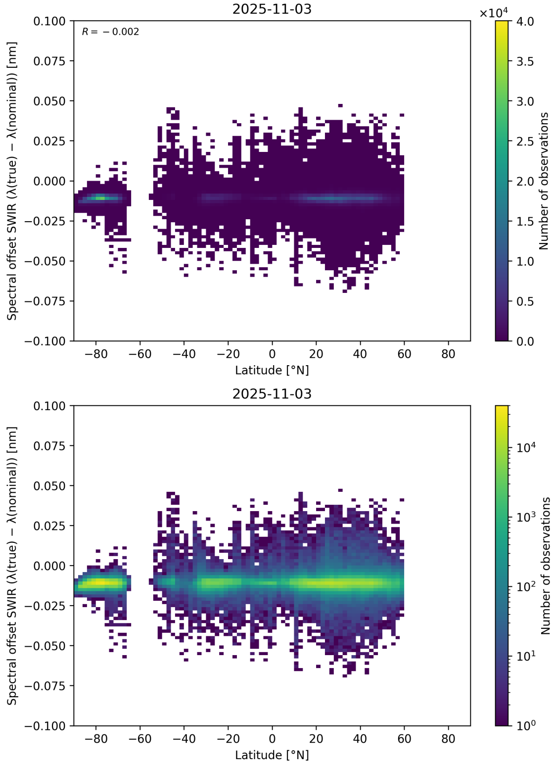
Figure 62: Scatter density plot of “Latitude” against “Spectral offset SWIR ( \lambda_{\text{true}} - \lambda_{\text{nominal}} )” for 2025-11-02 to 2025-11-04.
