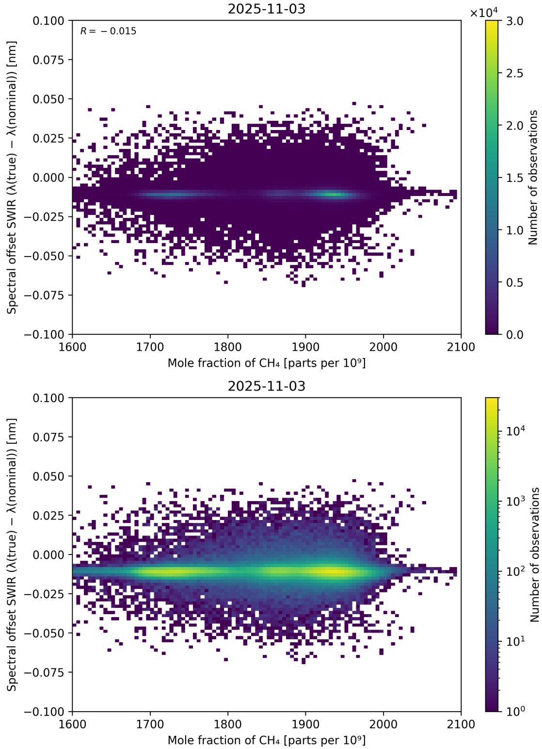
Figure 86: Scatter density plot of “Mole fraction of CH 4 ” against “Spectral offset SWIR ( \lambda_{\text{true}} - \lambda_{\text{nominal}} )” for 2025-11-02 to 2025-11-04.
