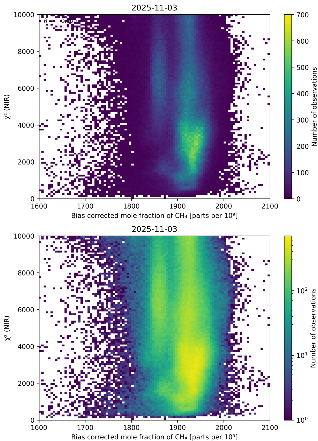
Figure 63: Scatter density plot of “Bias corrected mole fraction of \text{CH}_4 ” against “ \chi^2 (NIR)” for 2025-11-02 to 2025-11-04.
