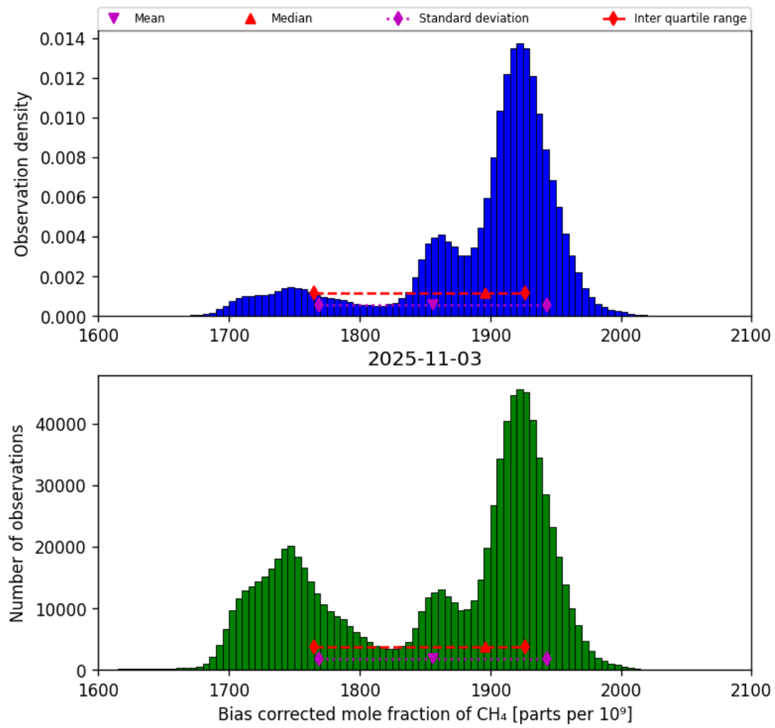
Figure 25: Histogram of “Bias corrected mole fraction of CH 4 ” for 2025-11-02 to 2025-11-04
