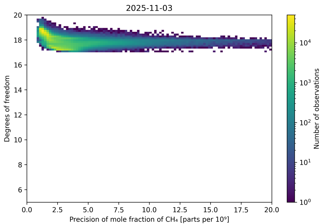
Figure 80: Scatter density plot of “Precision of mole fraction of CH 4 ” against “Degrees of freedom” for 2025-11-02 to 2025-11-04.
