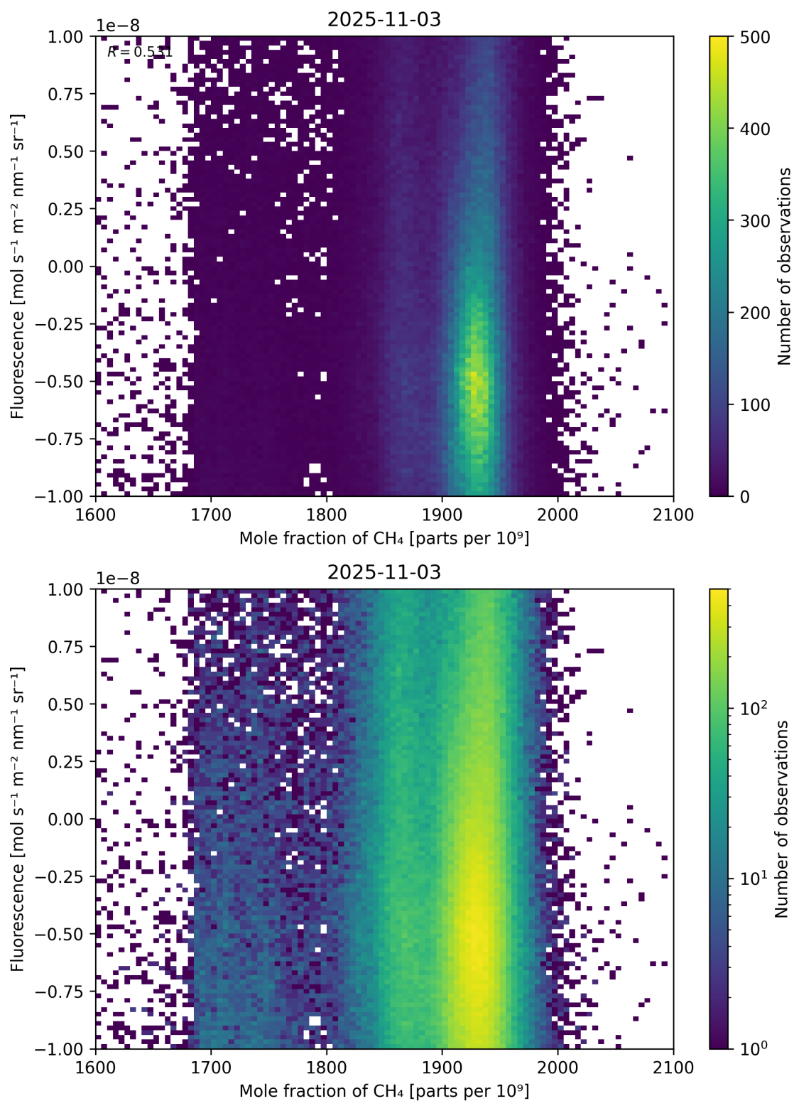
Figure 73: Scatter density plot of “Mole fraction of \text{CH}_4 ” against “Fluorescence” for 2025-11-02 to 2025-11-04.
