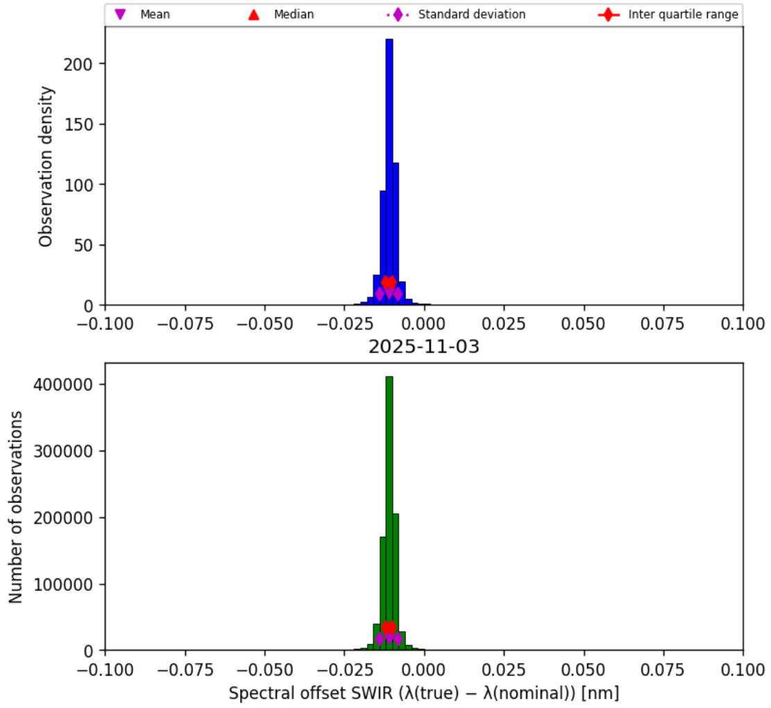
Figure 27: Histogram of “Spectral offset SWIR ( \lambda_{\text{true}} - \lambda_{\text{nominal}} )” for 2025-11-02 to 2025-11-04
