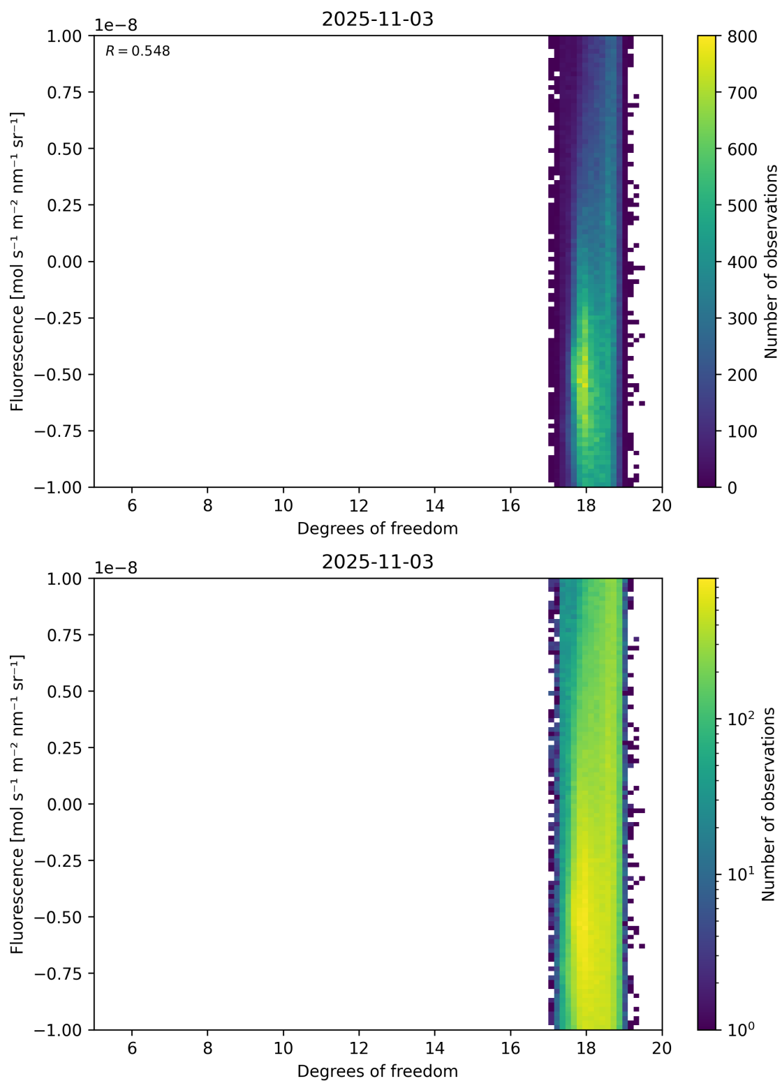
Figure 51: Scatter density plot of “Degrees of freedom” against “Fluorescence” for 2025-11-02 to 2025-11-04.
