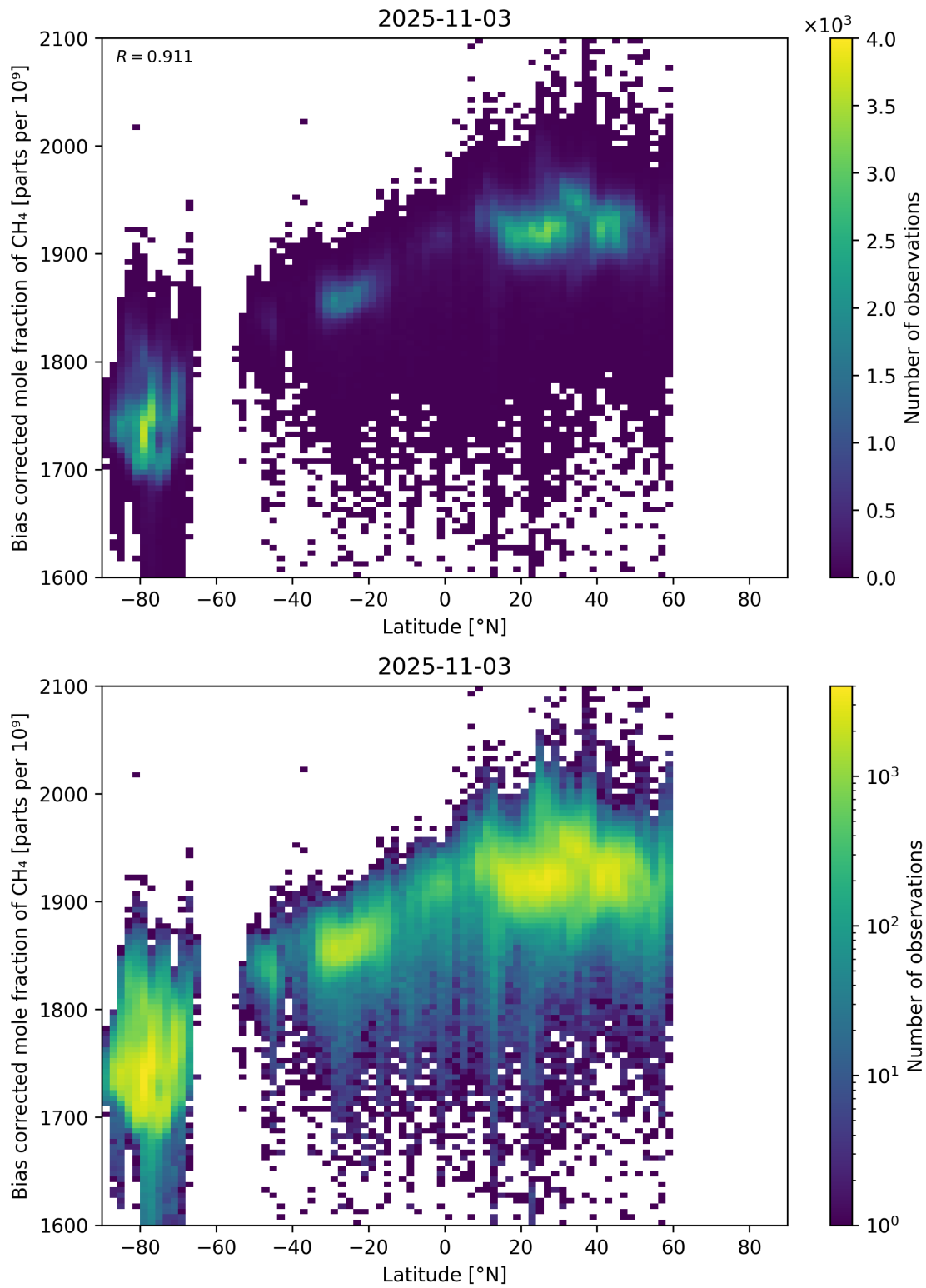
Figure 58: Scatter density plot of “Latitude” against “Bias corrected mole fraction of CH 4 ” for 2025-11-02 to 2025-11-04.
