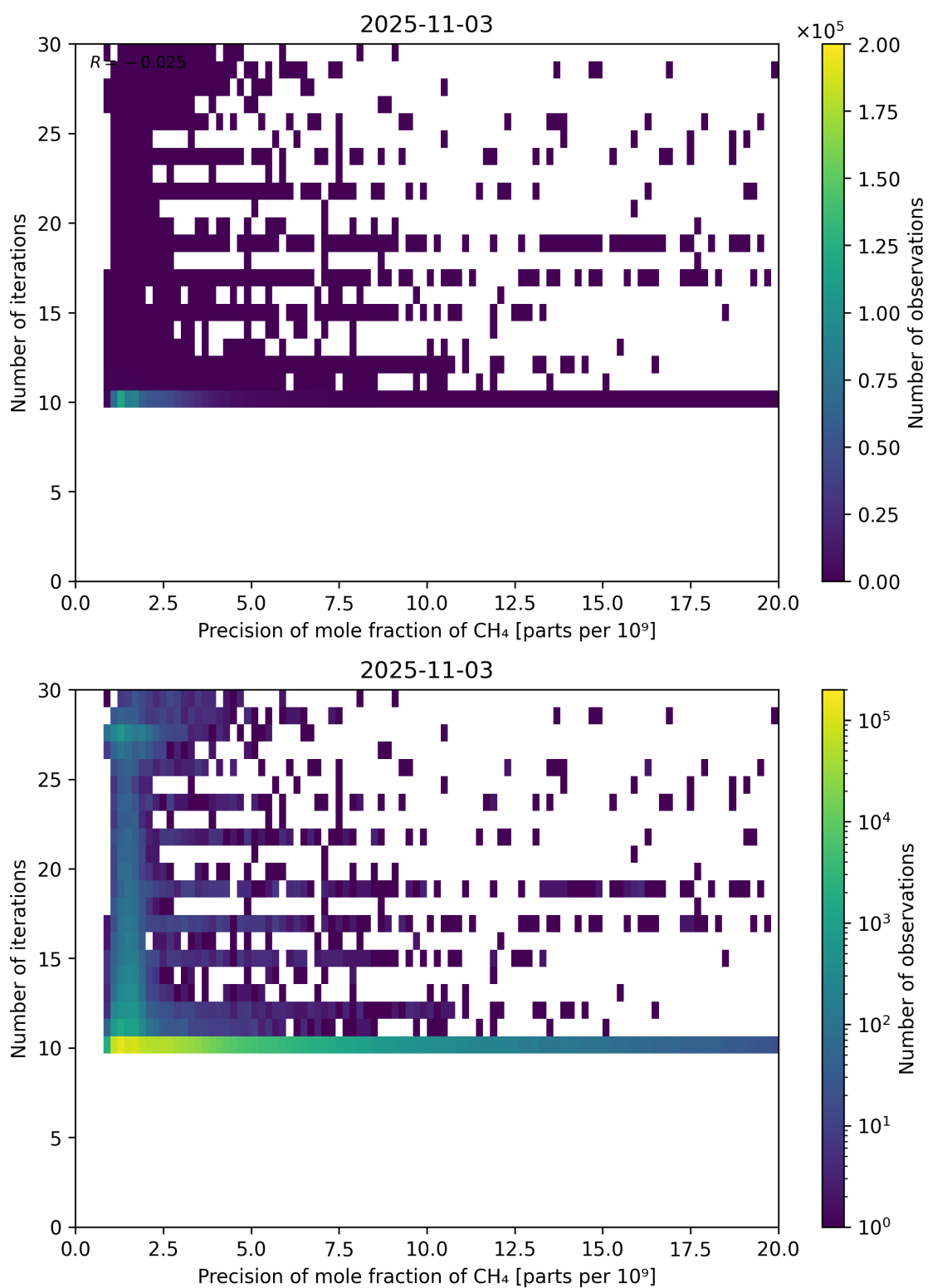
Figure 83: Scatter density plot of “Precision of mole fraction of CH 4 ” against “Number of iterations” for 2025-11-02 to 2025-11-04.
