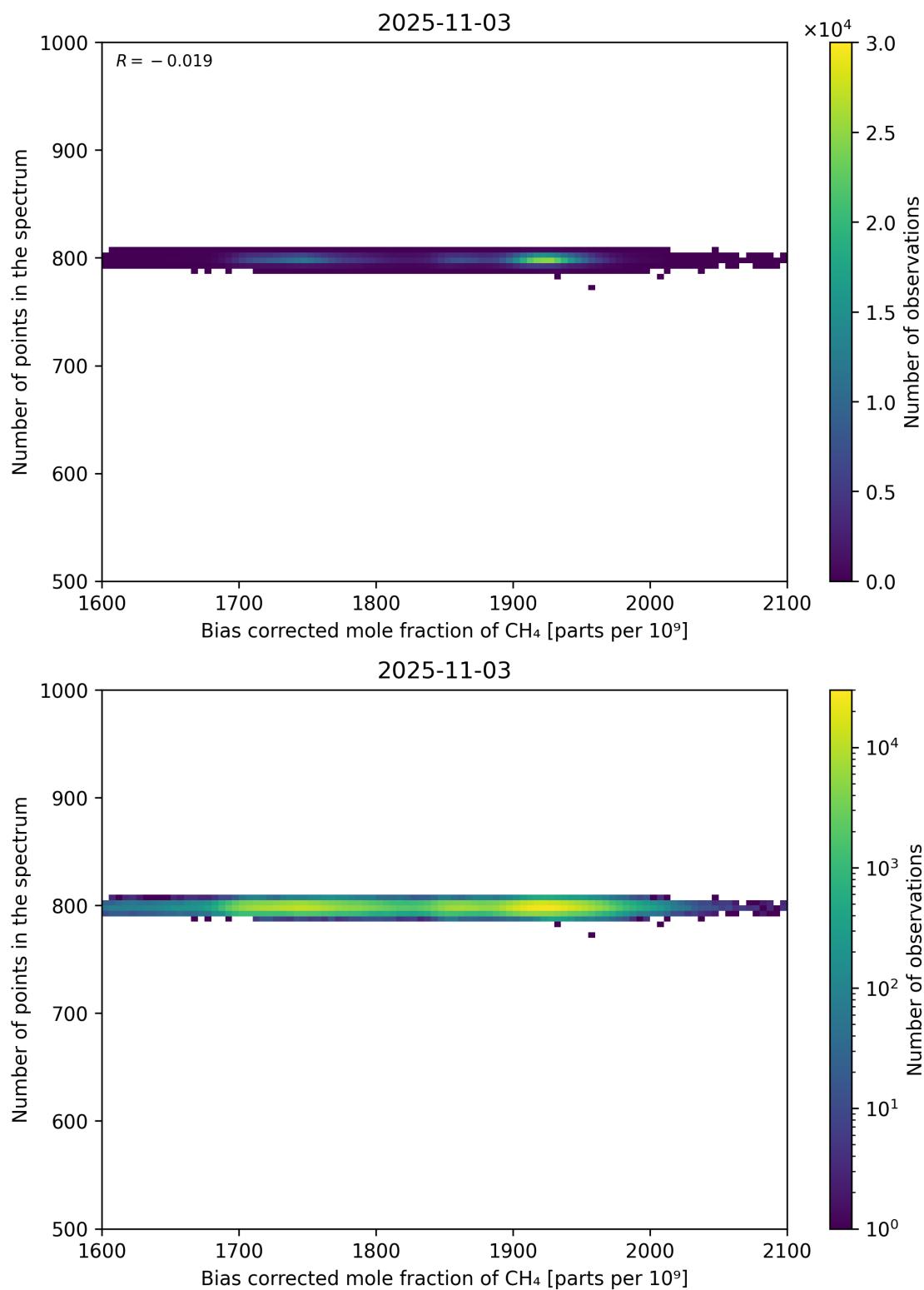
Figure 68: Scatter density plot of “Bias corrected mole fraction of CH 4 ” against “Number of points in the spectrum” for 2025-11-02 to 2025-11-04.
