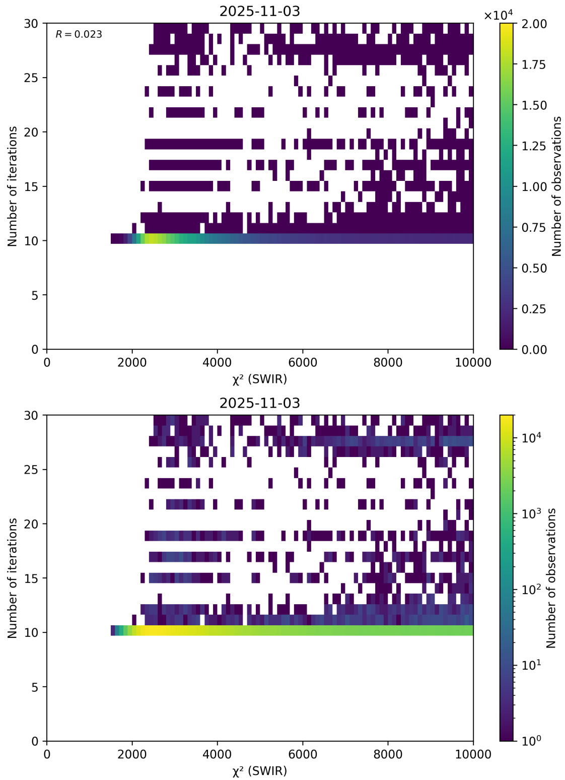
Figure 50: Scatter density plot of “ \chi^2 (SWIR)” against “Number of iterations” for 2025-11-02 to 2025-11-04.
