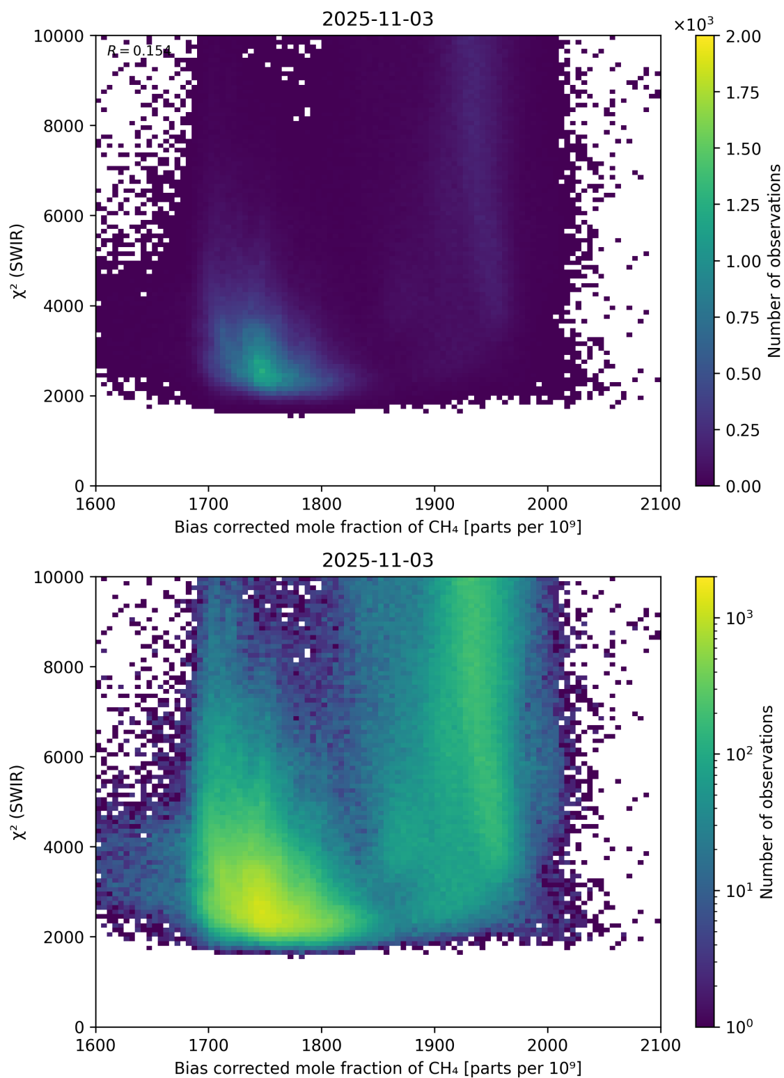
Figure 64: Scatter density plot of “Bias corrected mole fraction of \text{CH}_4 ” against “ \chi^2 (SWIR)” for 2025-11-02 to 2025-11-04.
