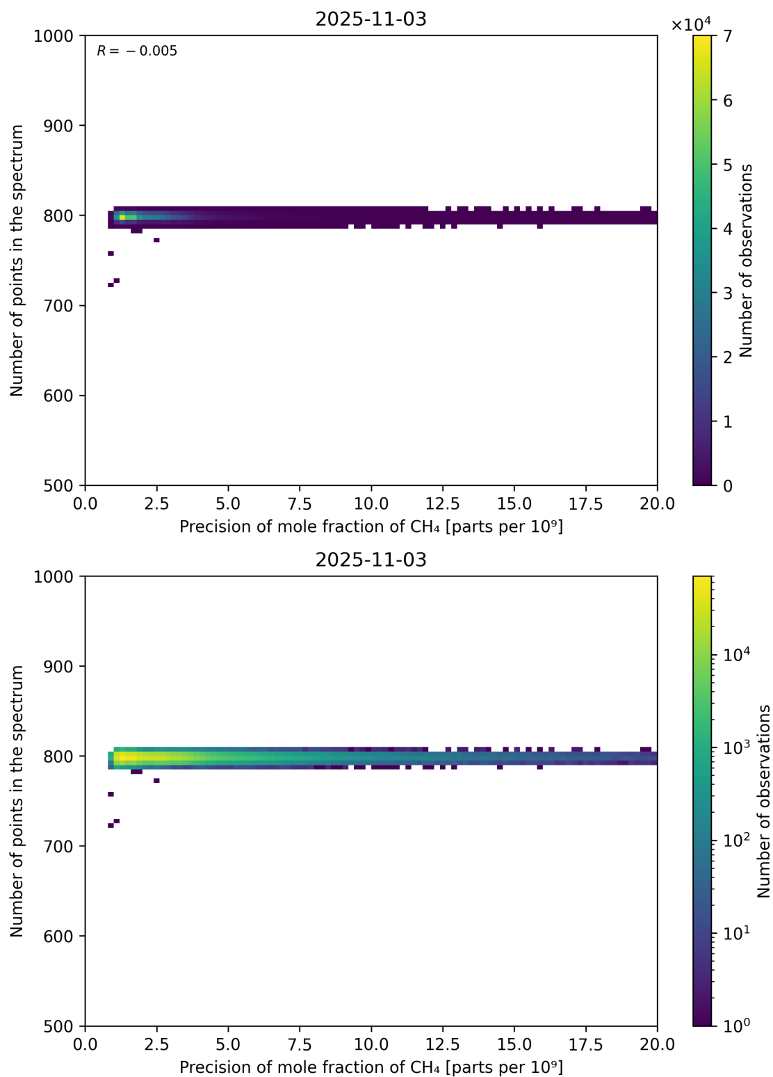
Figure 84: Scatter density plot of “Precision of mole fraction of CH 4 ” against “Number of points in the spectrum” for 2025-11-02 to 2025-11-04.
