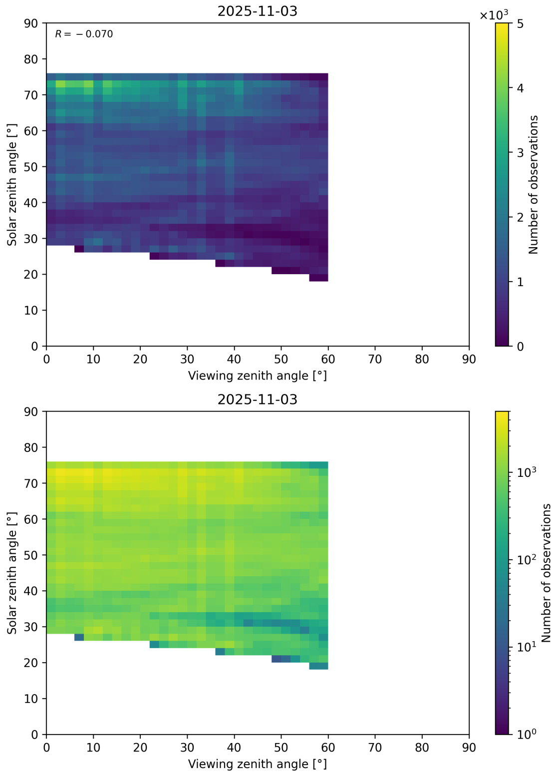
Figure 115: Scatter density plot of “Viewing zenith angle” against “Solar zenith angle” for 2025-11-02 to 2025-11-04.
