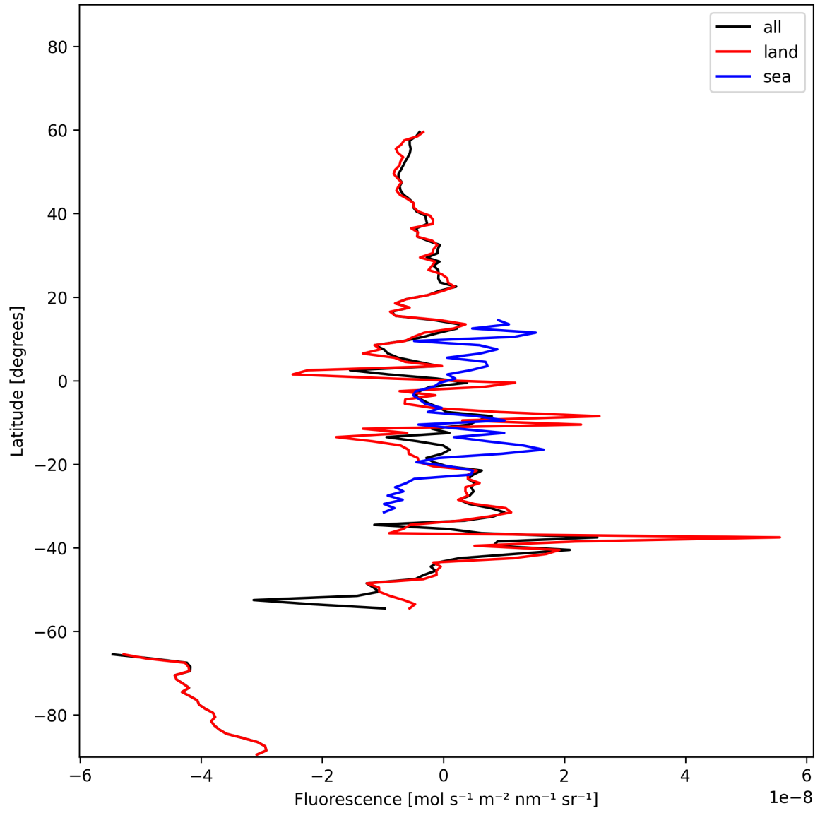
Figure 21: Zonal average of “Fluorescence” for 2025-11-02 to 2025-11-04.
