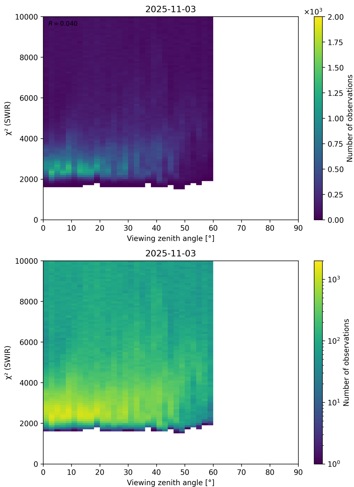
Figure 106: Scatter density plot of “Viewing zenith angle” against “ \chi^2 (SWIR)” for 2025-11-02 to 2025-11-04.
