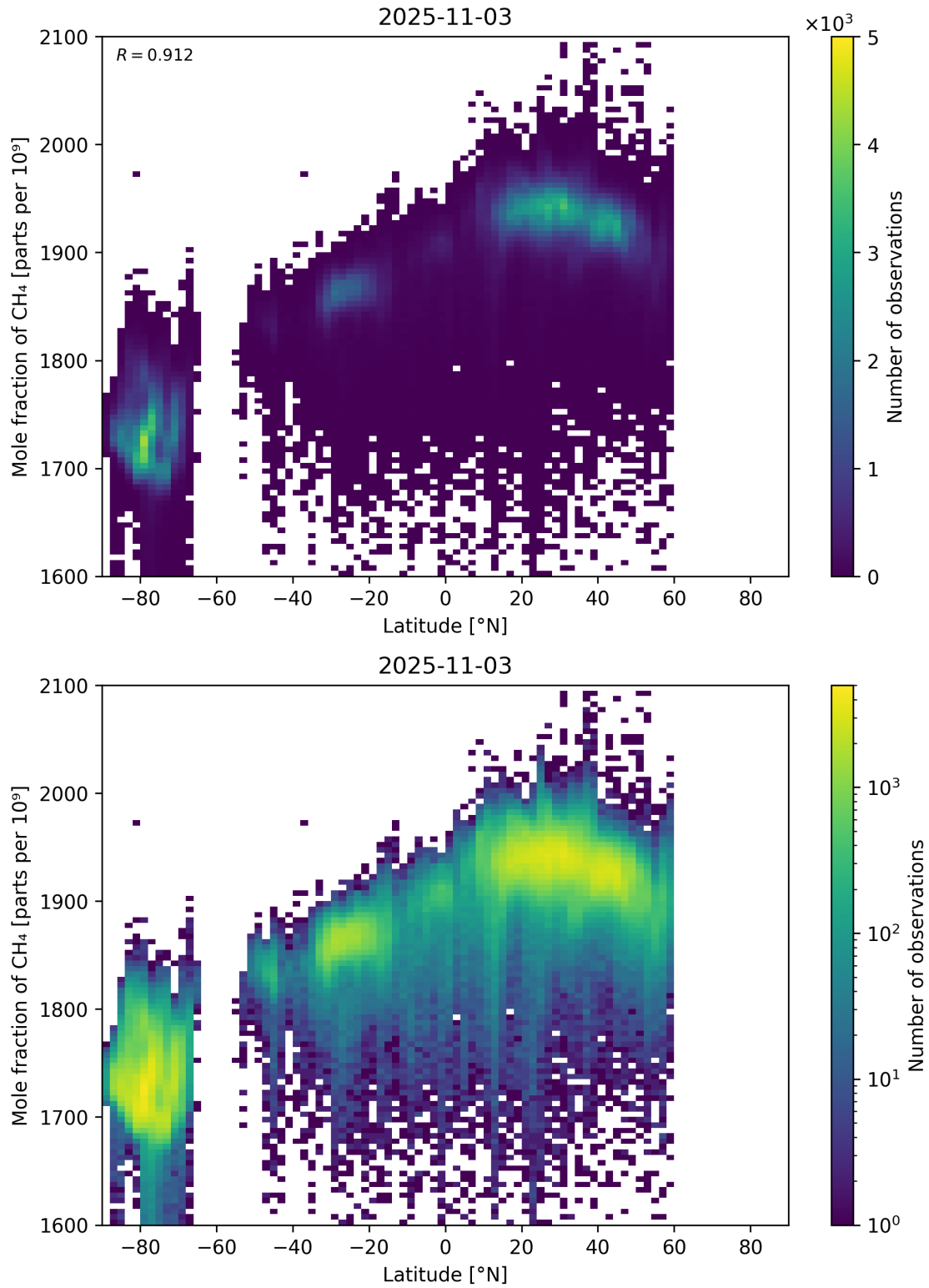
Figure 57: Scatter density plot of “Latitude” against “Mole fraction of CH 4 ” for 2025-11-02 to 2025-11-04.
