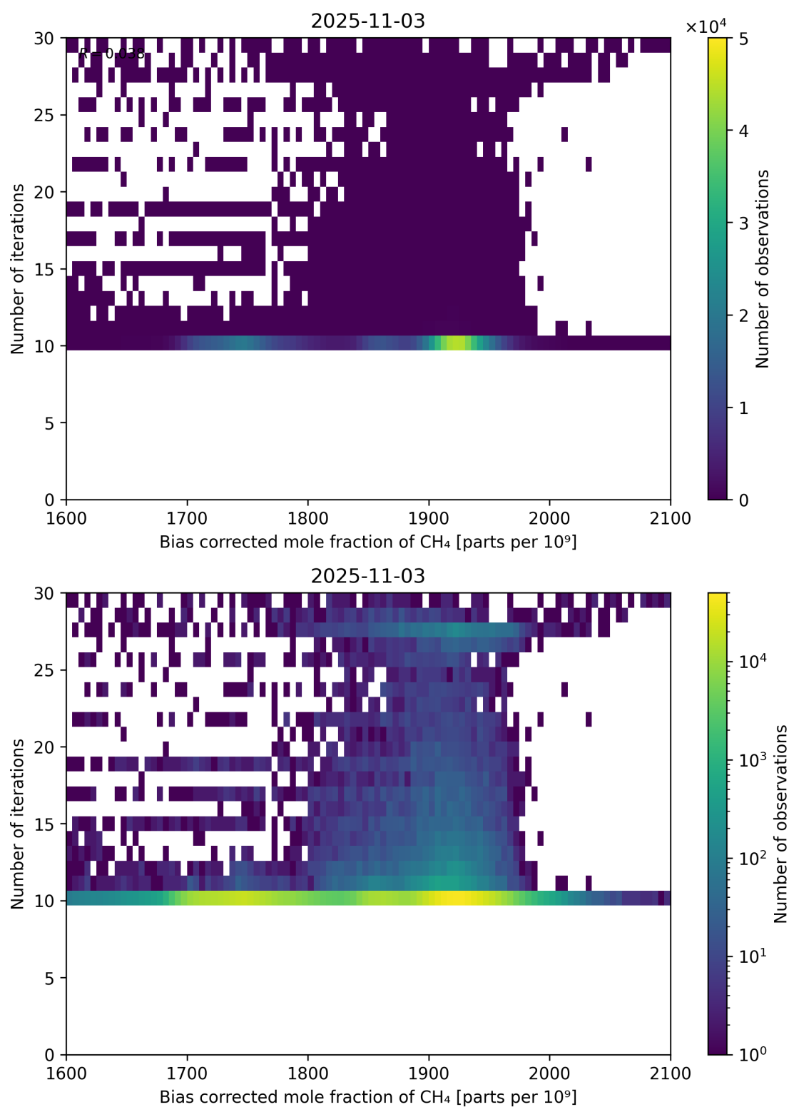
Figure 67: Scatter density plot of “Bias corrected mole fraction of \text{CH}_4 ” against “Number of iterations” for 2025-11-02 to 2025-11-04.
