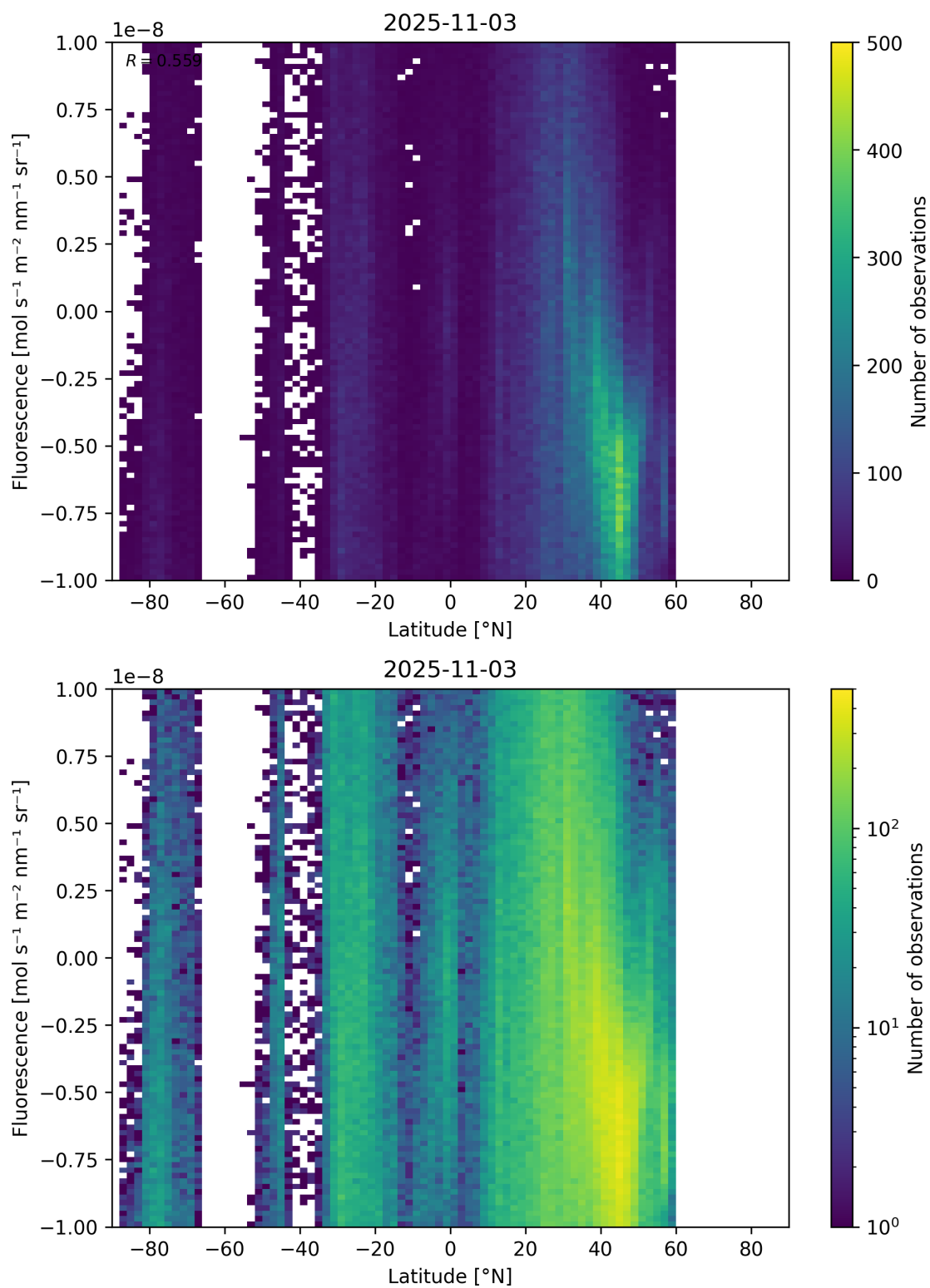
Figure 56: Scatter density plot of “Latitude” against “Fluorescence” for 2025-11-02 to 2025-11-04.
