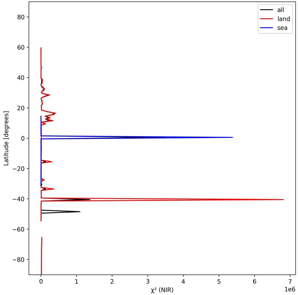
Figure 18: Zonal average of “ \chi^2 (NIR)” for 2025-11-02 to 2025-11-04.
