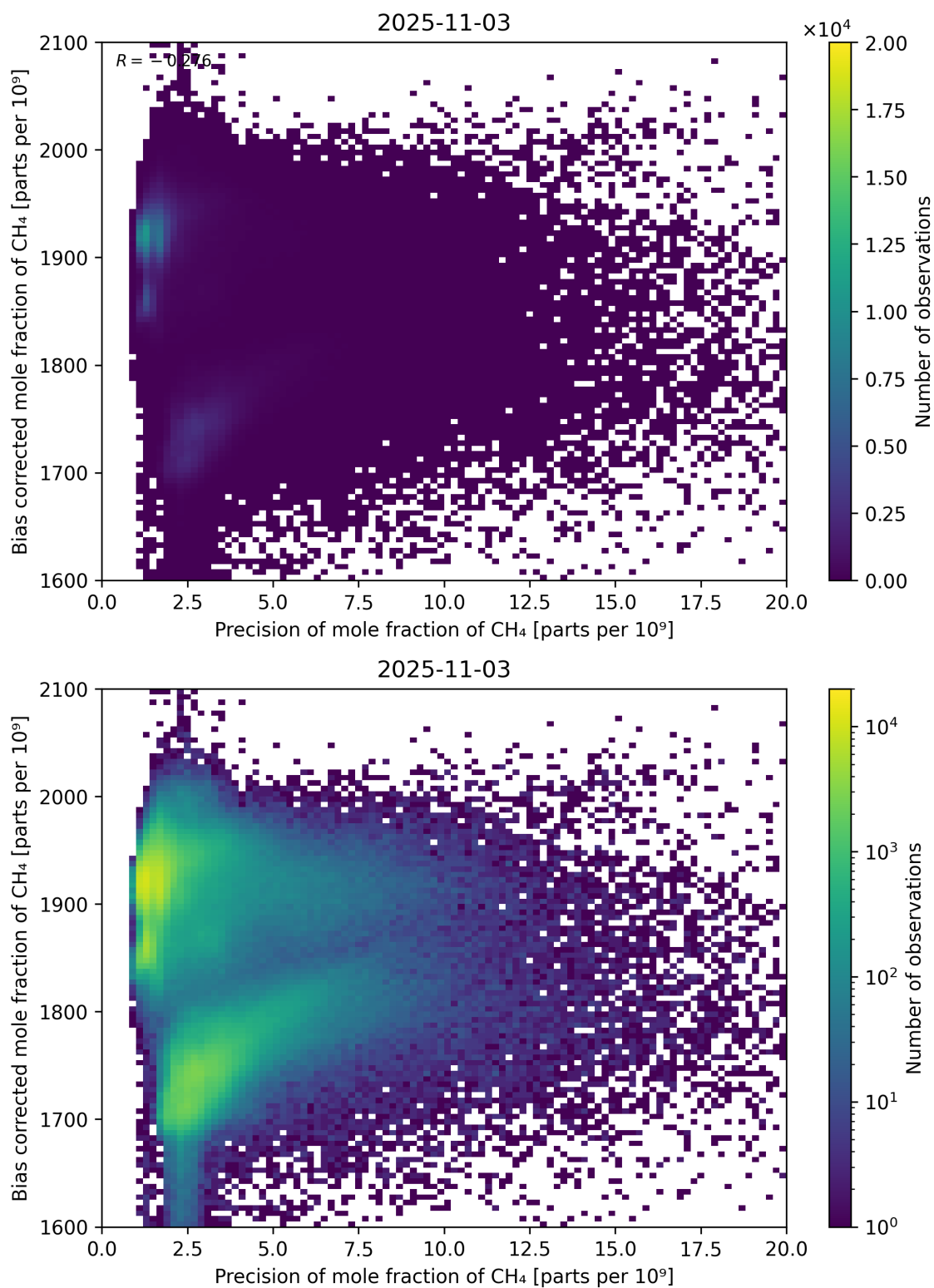
Figure 82: Scatter density plot of “Precision of mole fraction of CH 4 ” against “Bias corrected mole fraction of CH 4 ” for 2025-11-02 to 2025-11-04.
