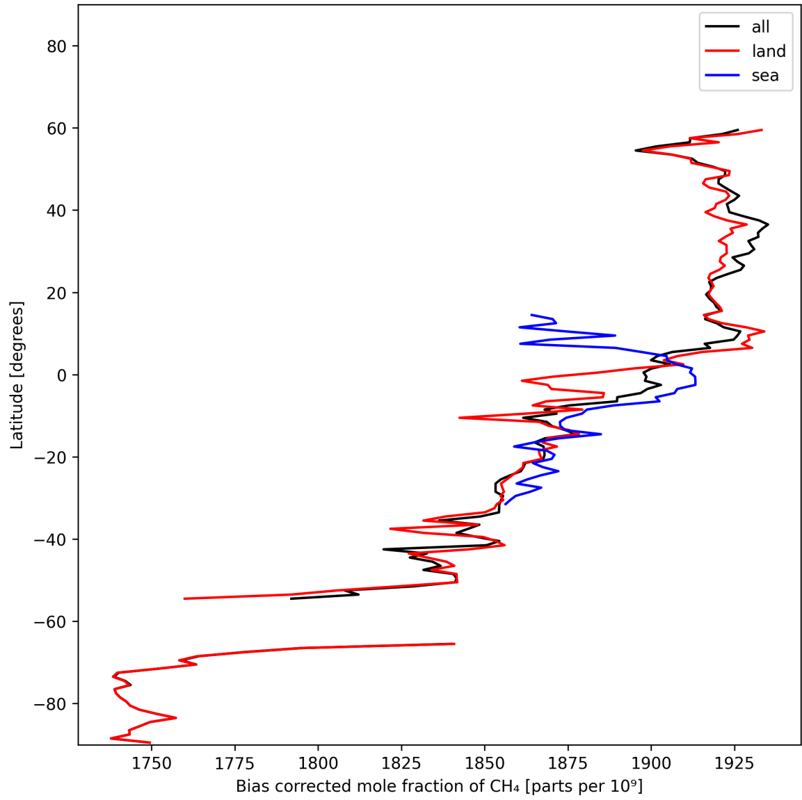
Figure 14: Zonal average of “Bias corrected mole fraction of CH 4 ” for 2025-11-02 to 2025-11-04.
