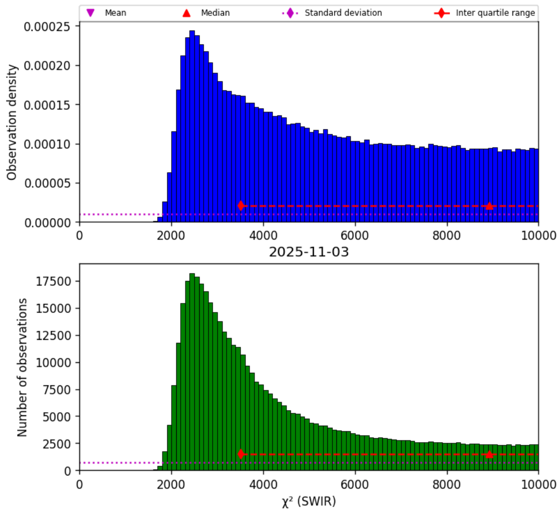
Figure 28: Histogram of “ \chi^2 (SWIR)” for 2025-11-02 to 2025-11-04
