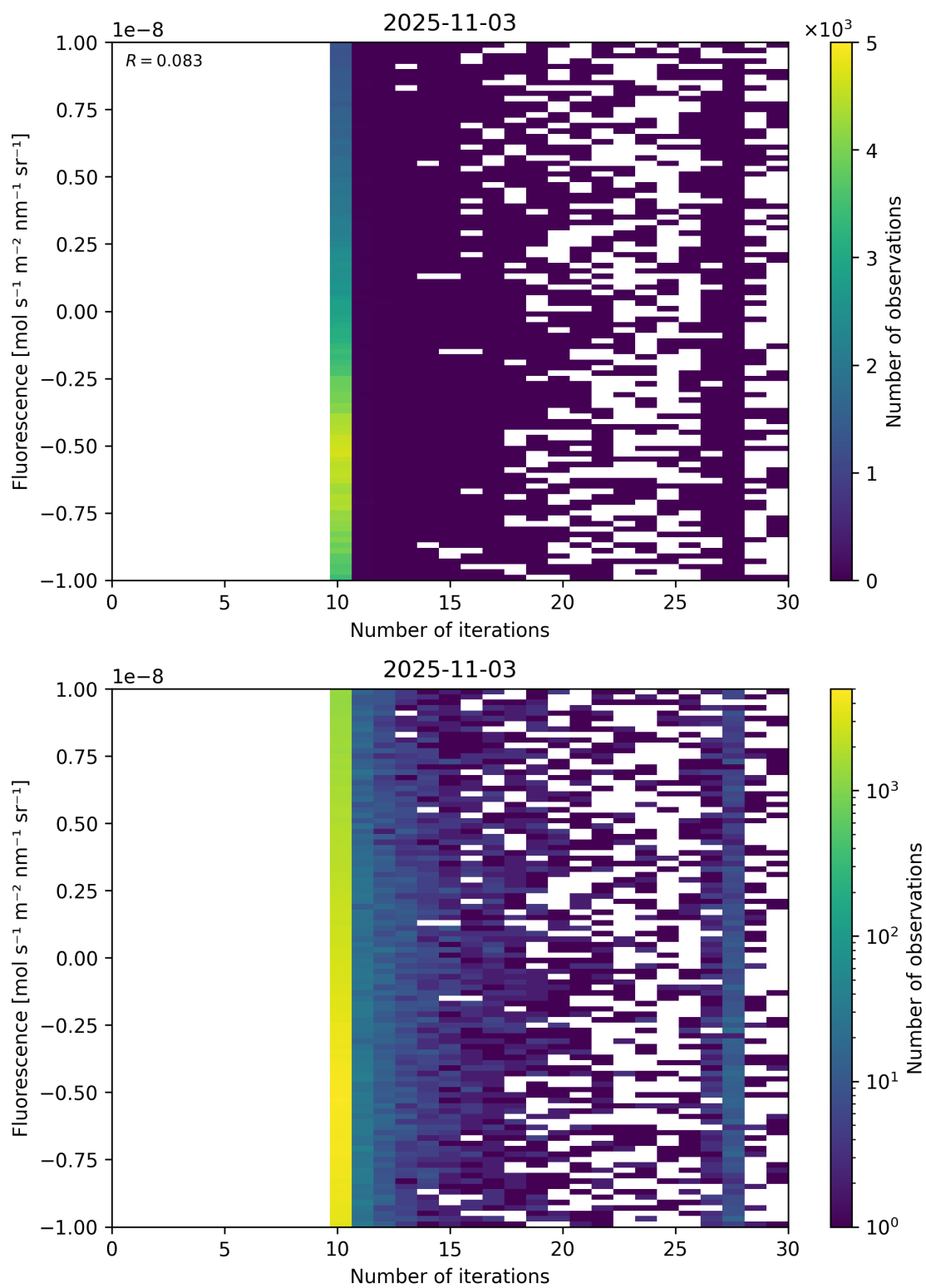
Figure 87: Scatter density plot of “Number of iterations” against “Fluorescence” for 2025-11-02 to 2025-11-04.
