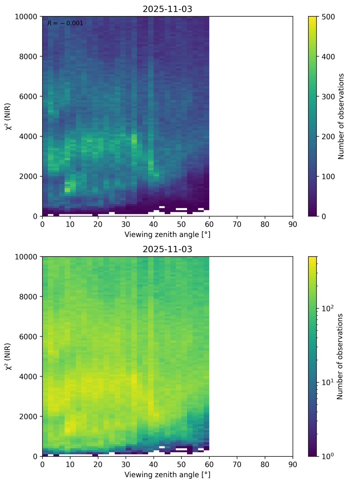
Figure 105: Scatter density plot of “Viewing zenith angle” against “ \chi^2 (NIR)” for 2025-11-02 to 2025-11-04.
