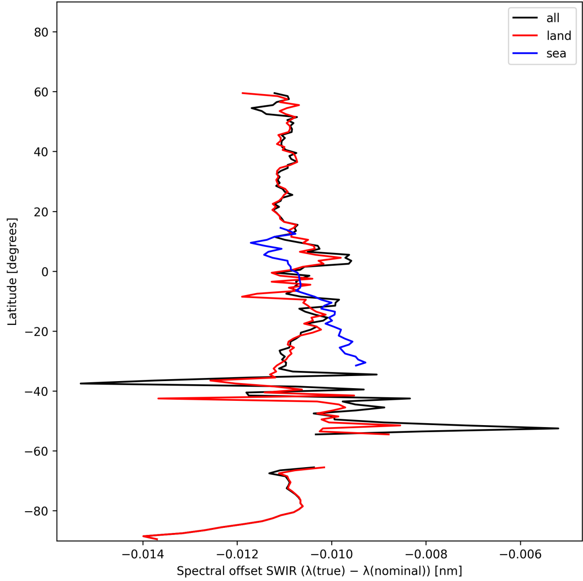
Figure 16: Zonal average of “Spectral offset SWIR ( \lambda_{\text{true}} - \lambda_{\text{nominal}} )” for 2025-11-02 to 2025-11-04.
