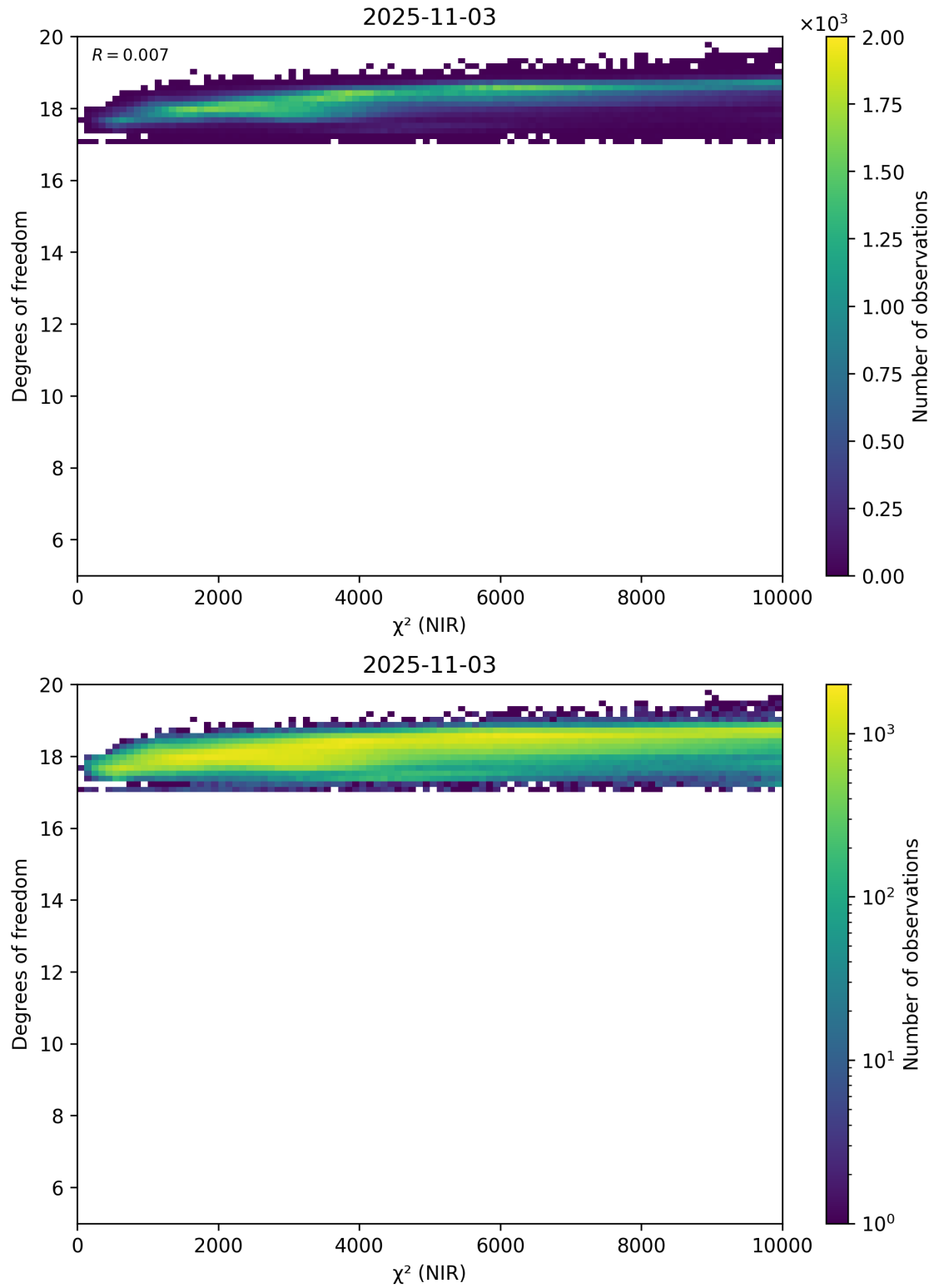
Figure 44: Scatter density plot of “ \chi^2 (NIR)” against “Degrees of freedom” for 2025-11-02 to 2025-11-04.
