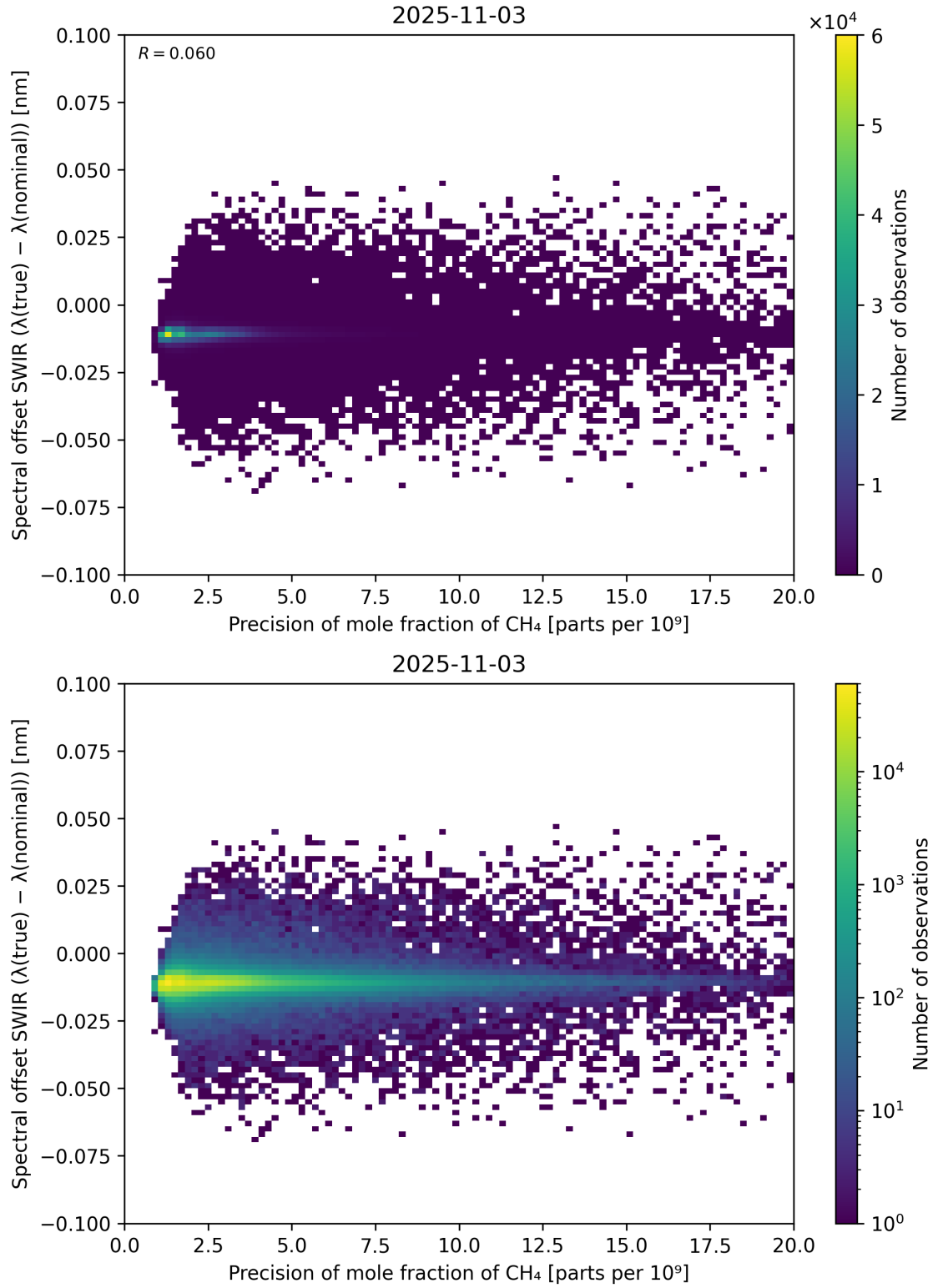
Figure 85: Scatter density plot of “Precision of mole fraction of CH 4 ” against “Spectral offset SWIR ( \lambda_{\text{true}} - \lambda_{\text{nominal}} )” for 2025-11-02 to 2025-11-04.
