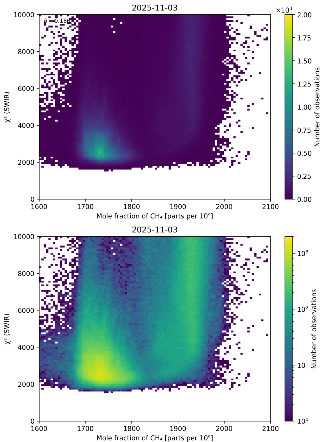
Figure 71: Scatter density plot of “Mole fraction of \text{CH}_4 ” against “ \chi^2 (SWIR)” for 2025-11-02 to 2025-11-04.
