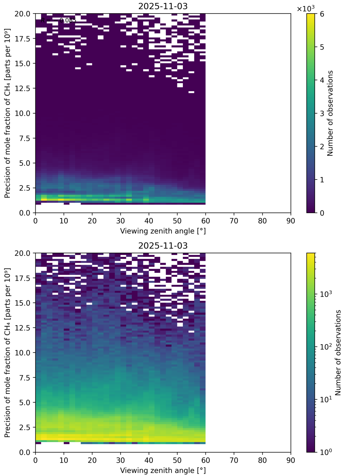
Figure 112: Scatter density plot of “Viewing zenith angle” against “Precision of mole fraction of CH 4 ” for 2025-11-02 to 2025-11-04.
