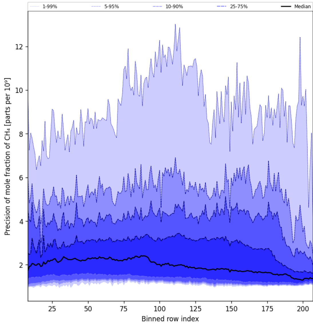
Figure 35: Along track statistics of “Precision of mole fraction of CH 4 ” for 2025-11-03 to 2025-11-05
