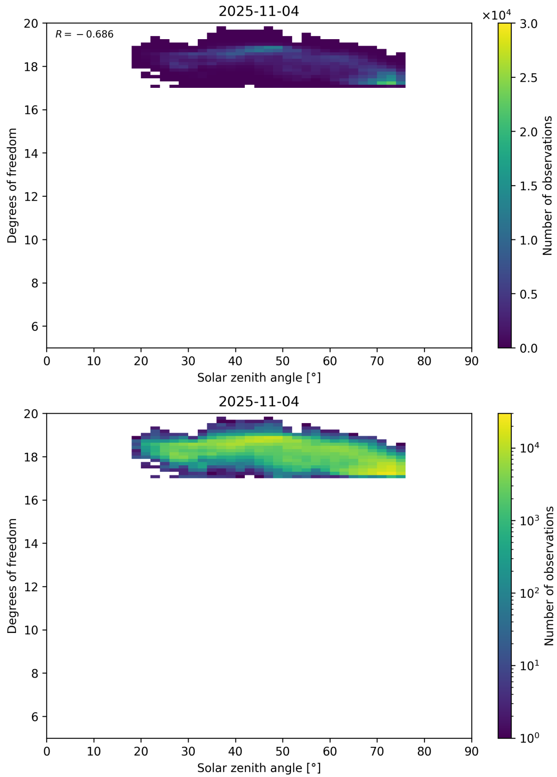
Figure 96: Scatter density plot of “Solar zenith angle” against “Degrees of freedom” for 2025-11-03 to 2025-11-05.
