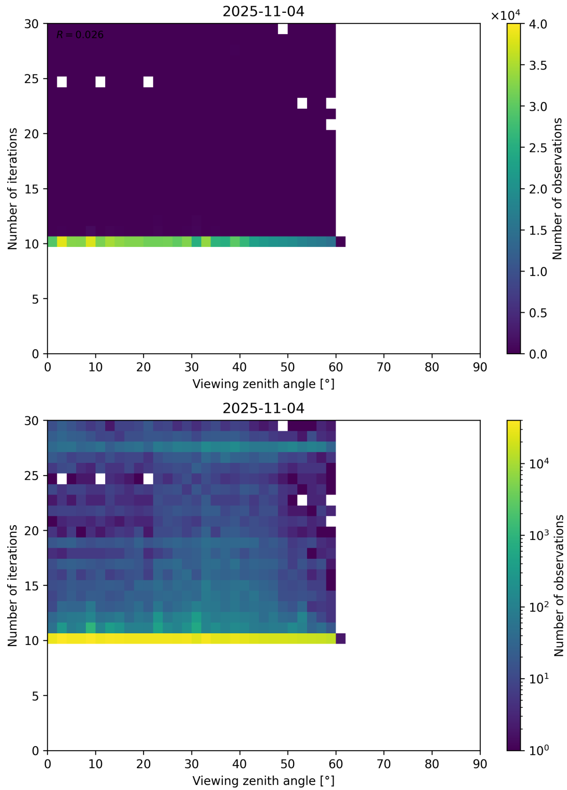
Figure 113: Scatter density plot of “Viewing zenith angle” against “Number of iterations” for 2025-11-03 to 2025-11-05.
