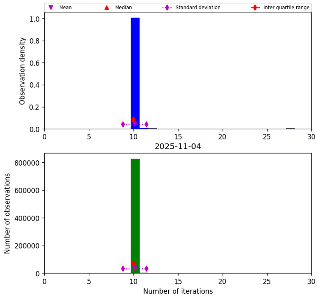
Figure 31: Histogram of “Number of iterations” for 2025-11-03 to 2025-11-05
