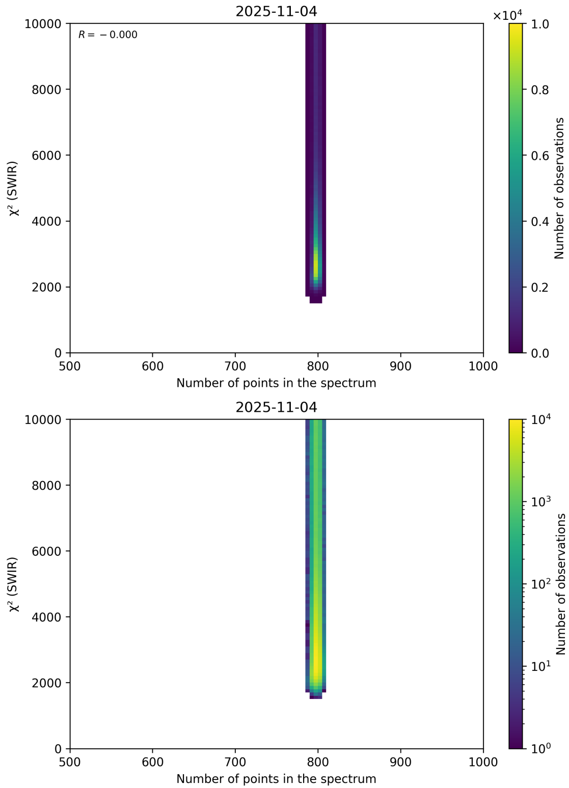
Figure 89: Scatter density plot of “Number of points in the spectrum” against “ \chi^2 (SWIR)” for 2025-11-03 to 2025-11-05.
