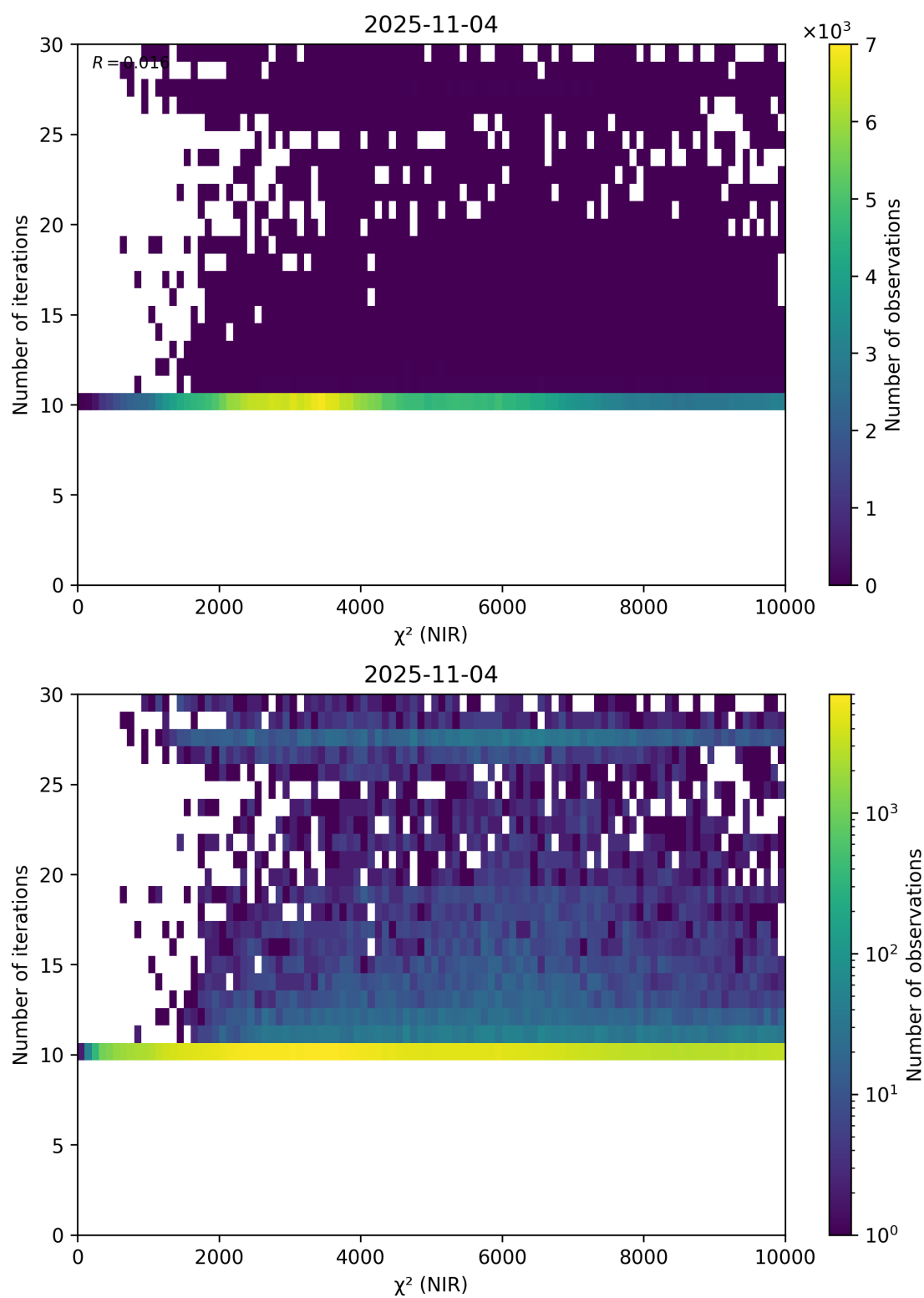
Figure 46: Scatter density plot of “ \chi^2 (NIR)” against “Number of iterations” for 2025-11-03 to 2025-11-05.
