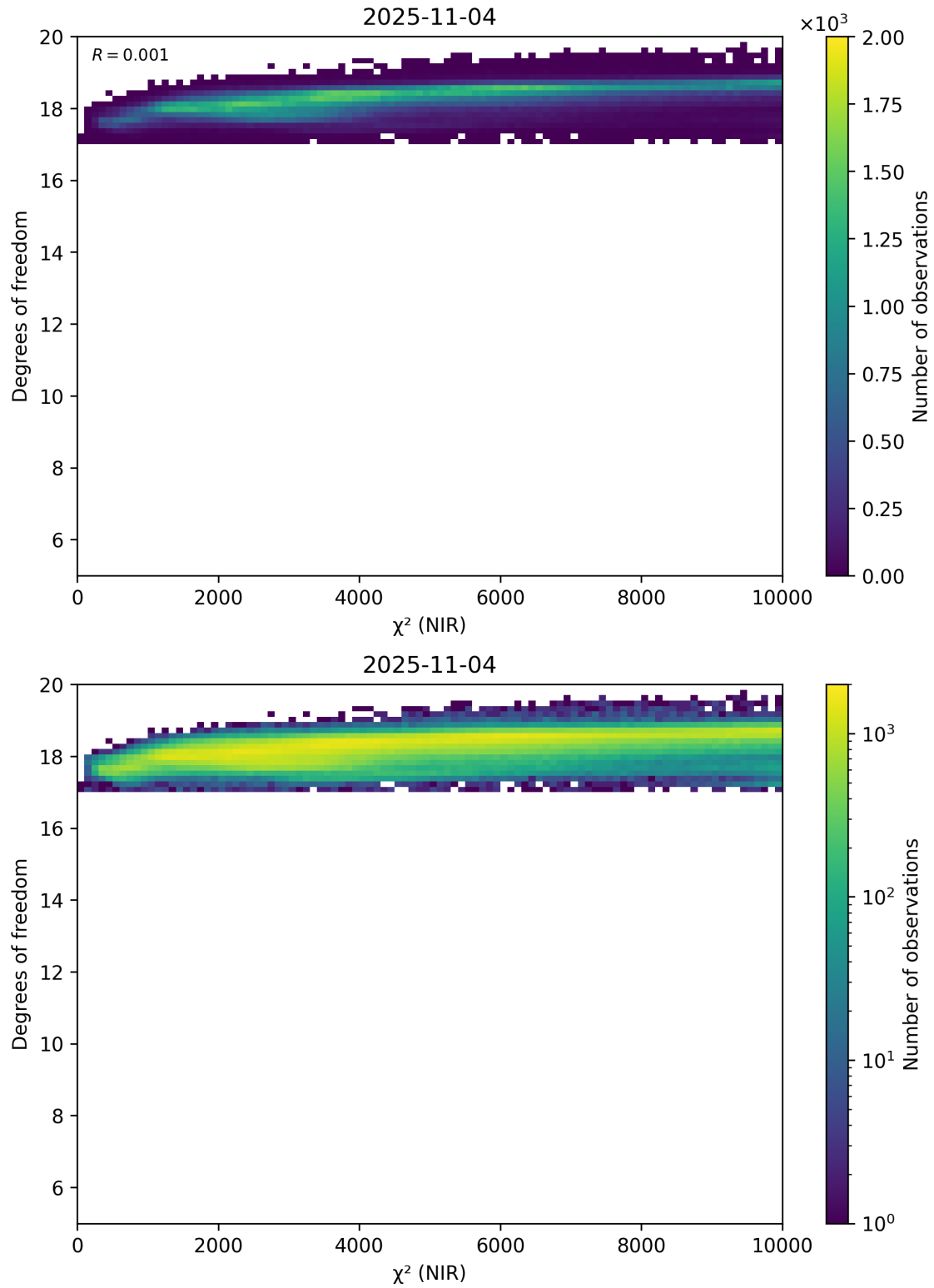
Figure 44: Scatter density plot of “ \chi^2 (NIR)” against “Degrees of freedom” for 2025-11-03 to 2025-11-05.
