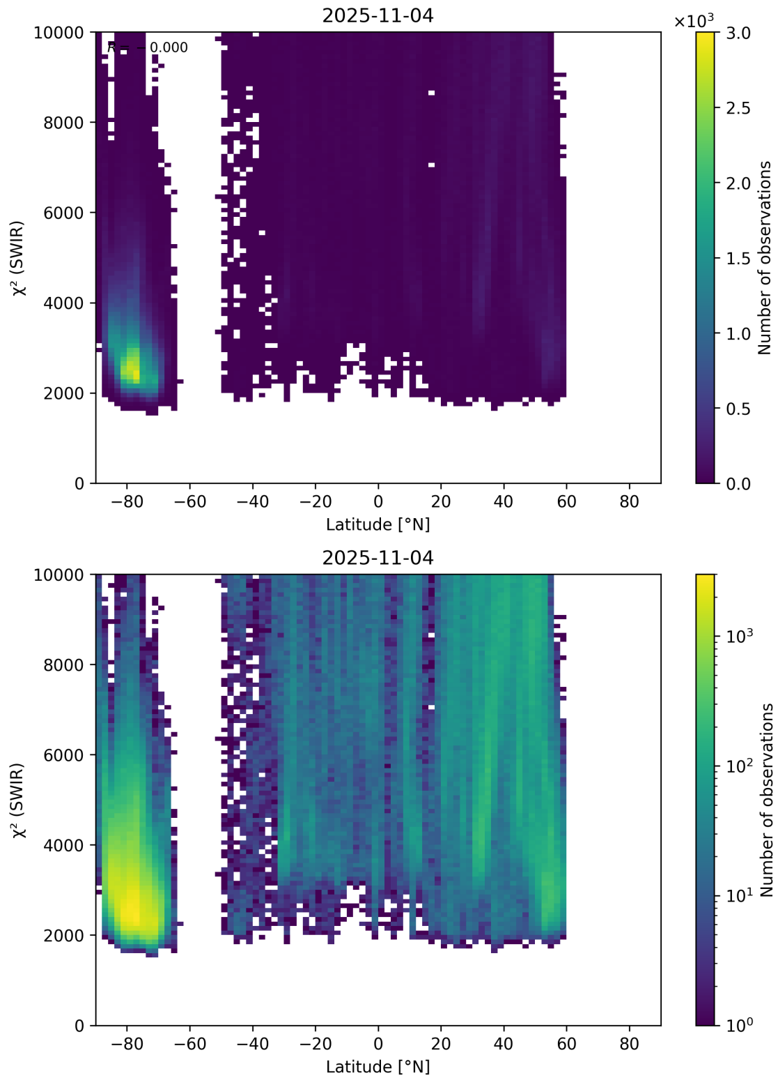
Figure 54: Scatter density plot of “Latitude” against “ \chi^2 (SWIR)” for 2025-11-03 to 2025-11-05.
