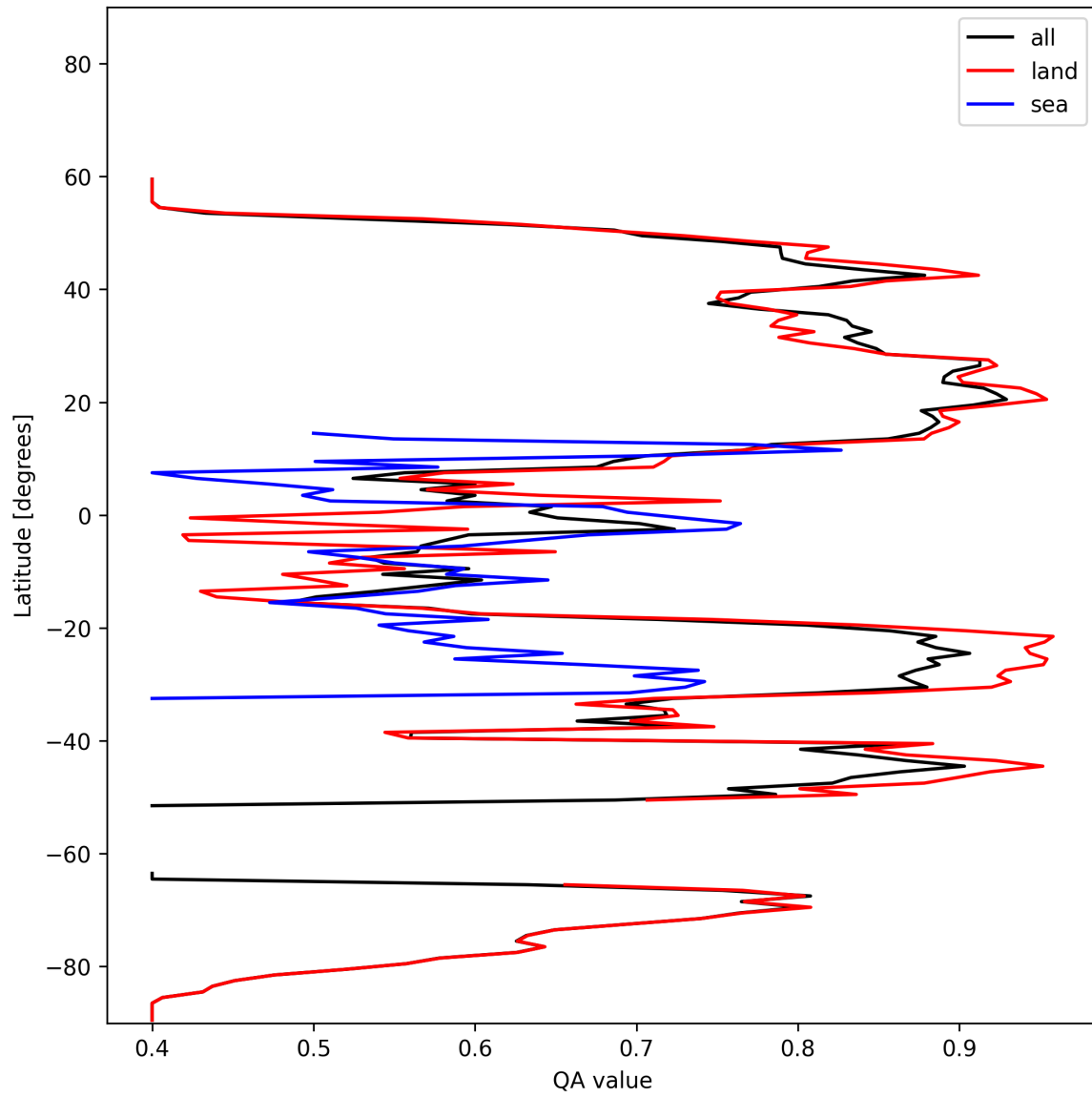
Figure 11: Zonal average of “QA value” for 2025-11-03 to 2025-11-05.
