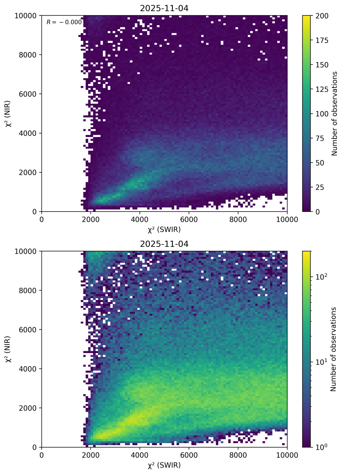
Figure 47: Scatter density plot of “ \chi^2 (SWIR)” against “ \chi^2 (NIR)” for 2025-11-03 to 2025-11-05.
