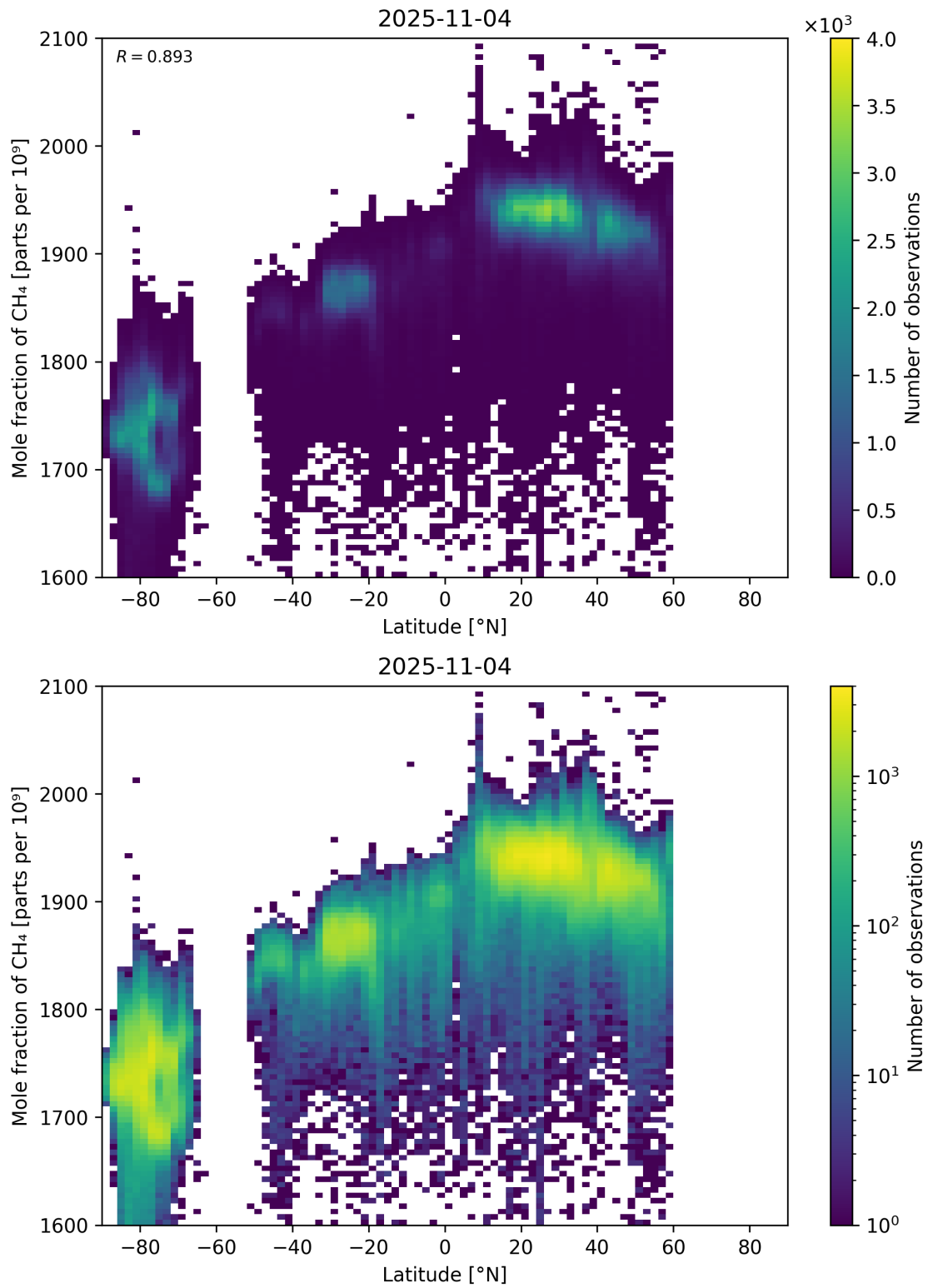
Figure 57: Scatter density plot of “Latitude” against “Mole fraction of CH 4 ” for 2025-11-03 to 2025-11-05.
