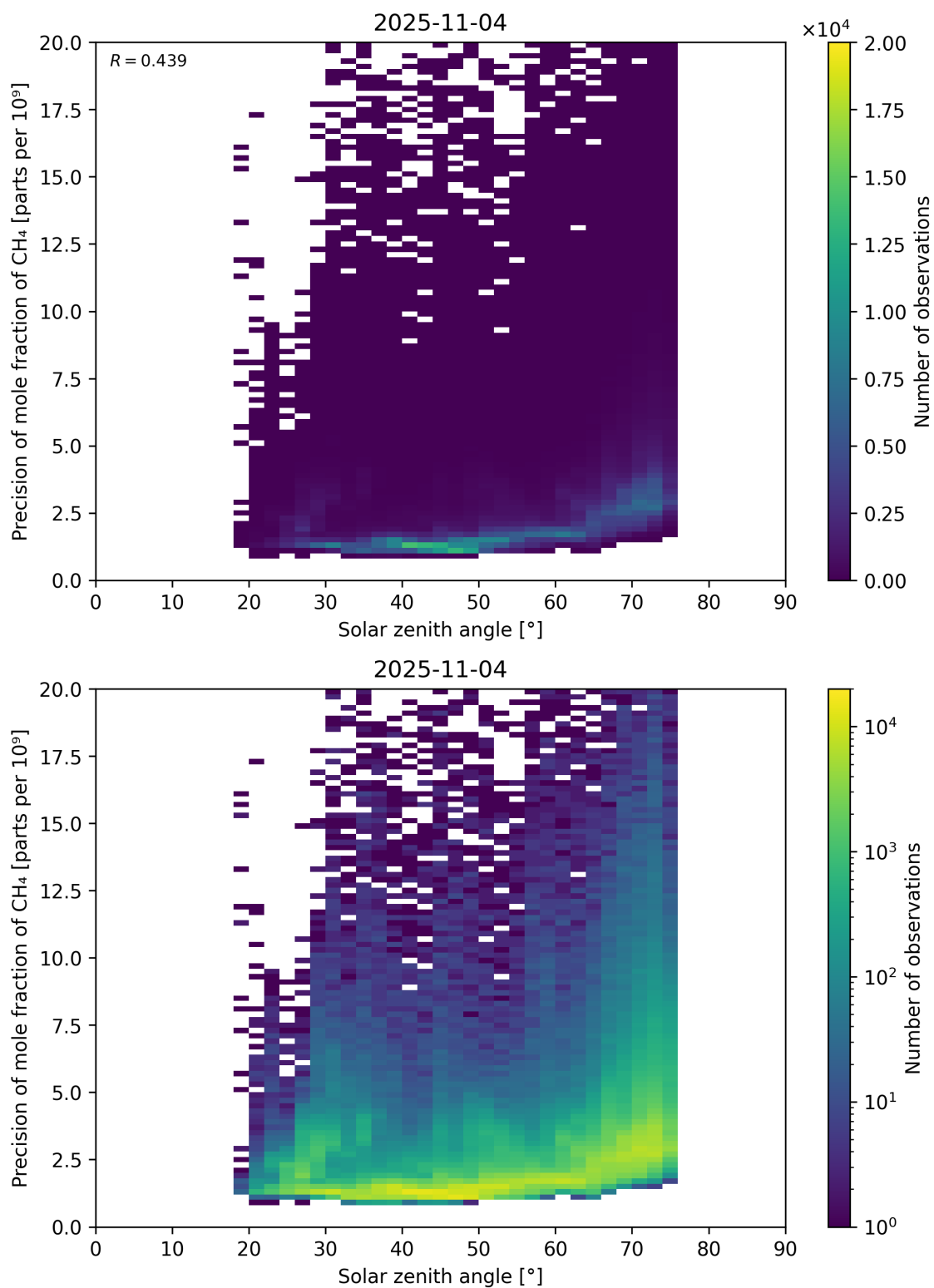
Figure 101: Scatter density plot of “Solar zenith angle” against “Precision of mole fraction of \text{CH}_4 ” for 2025-11-03 to 2025-11-05.
