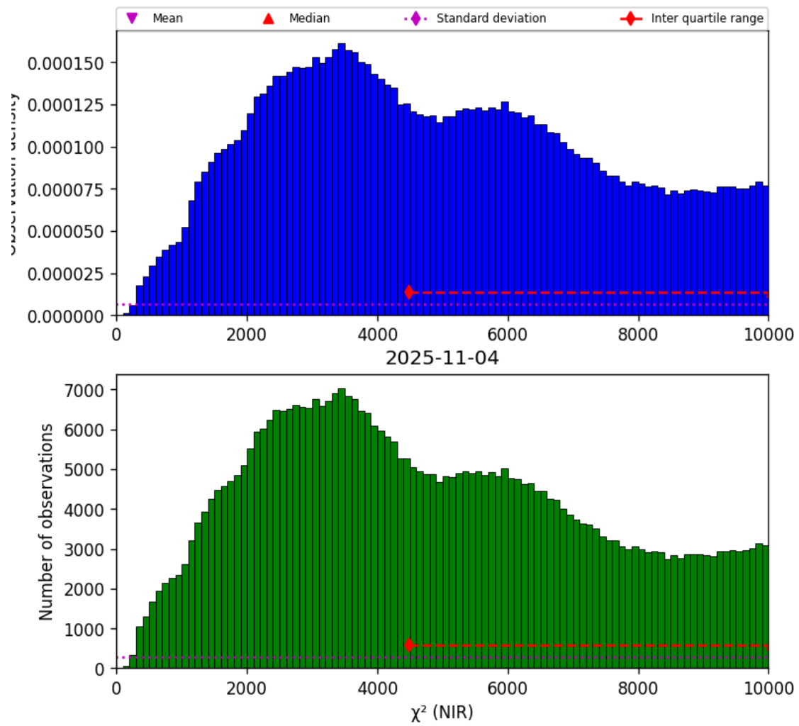
Figure 29: Histogram of “ \chi^2 (NIR)” for 2025-11-03 to 2025-11-05
