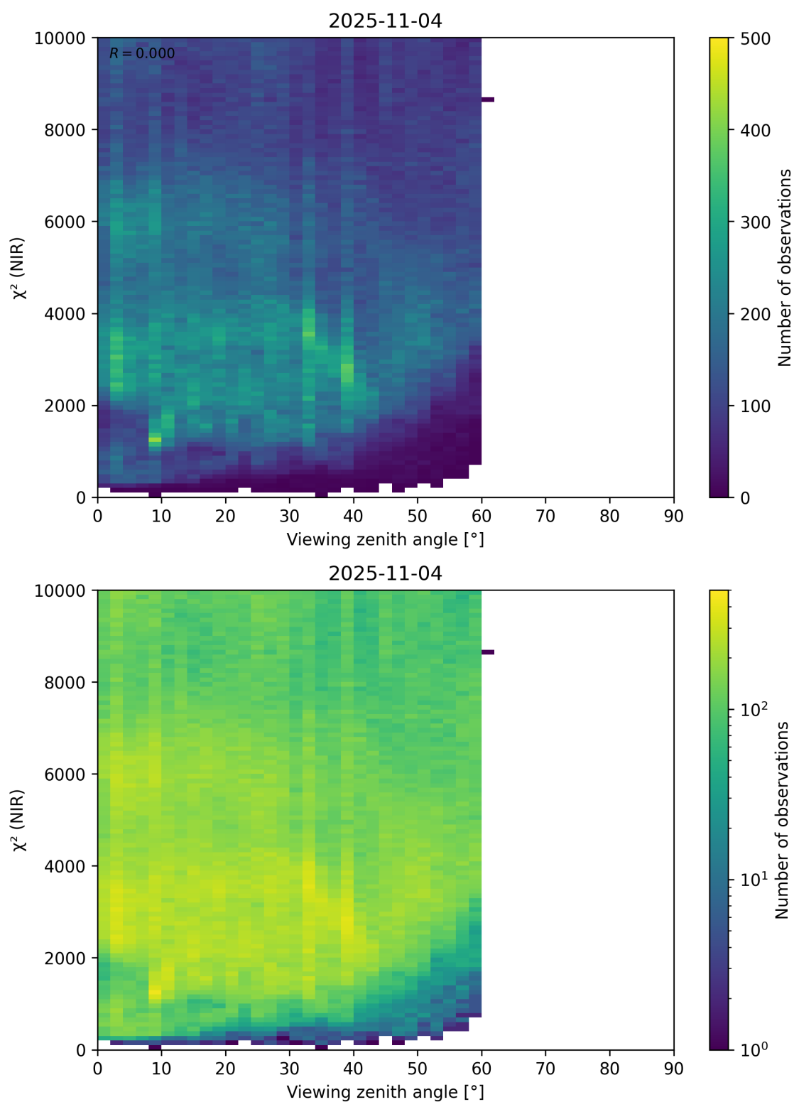
Figure 105: Scatter density plot of “Viewing zenith angle” against “ \chi^2 (NIR)” for 2025-11-03 to 2025-11-05.
