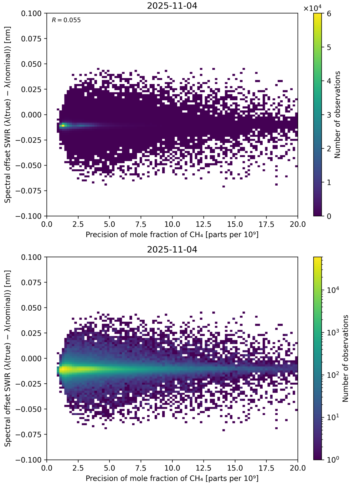
Figure 85: Scatter density plot of “Precision of mole fraction of CH 4 ” against “Spectral offset SWIR ( \lambda_{\text{true}} - \lambda_{\text{nominal}} )” for 2025-11-03 to 2025-11-05.
