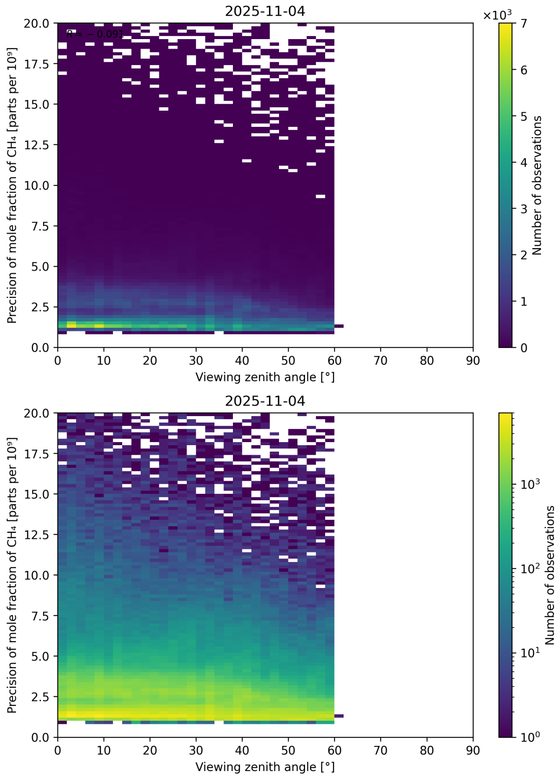
Figure 112: Scatter density plot of “Viewing zenith angle” against “Precision of mole fraction of CH 4 ” for 2025-11-03 to 2025-11-05.
