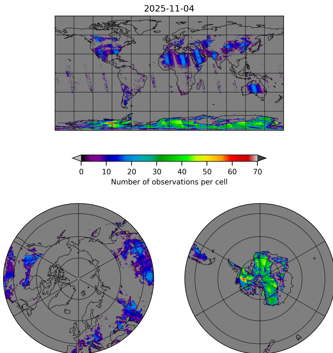
Figure 10: Map of the number of observations for 2025-11-03 to 2025-11-05
