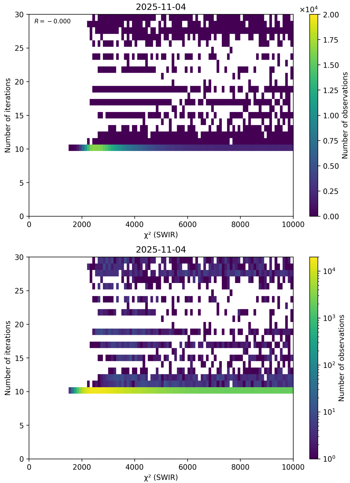
Figure 50: Scatter density plot of “ \chi^2 (SWIR)” against “Number of iterations” for 2025-11-03 to 2025-11-05.
