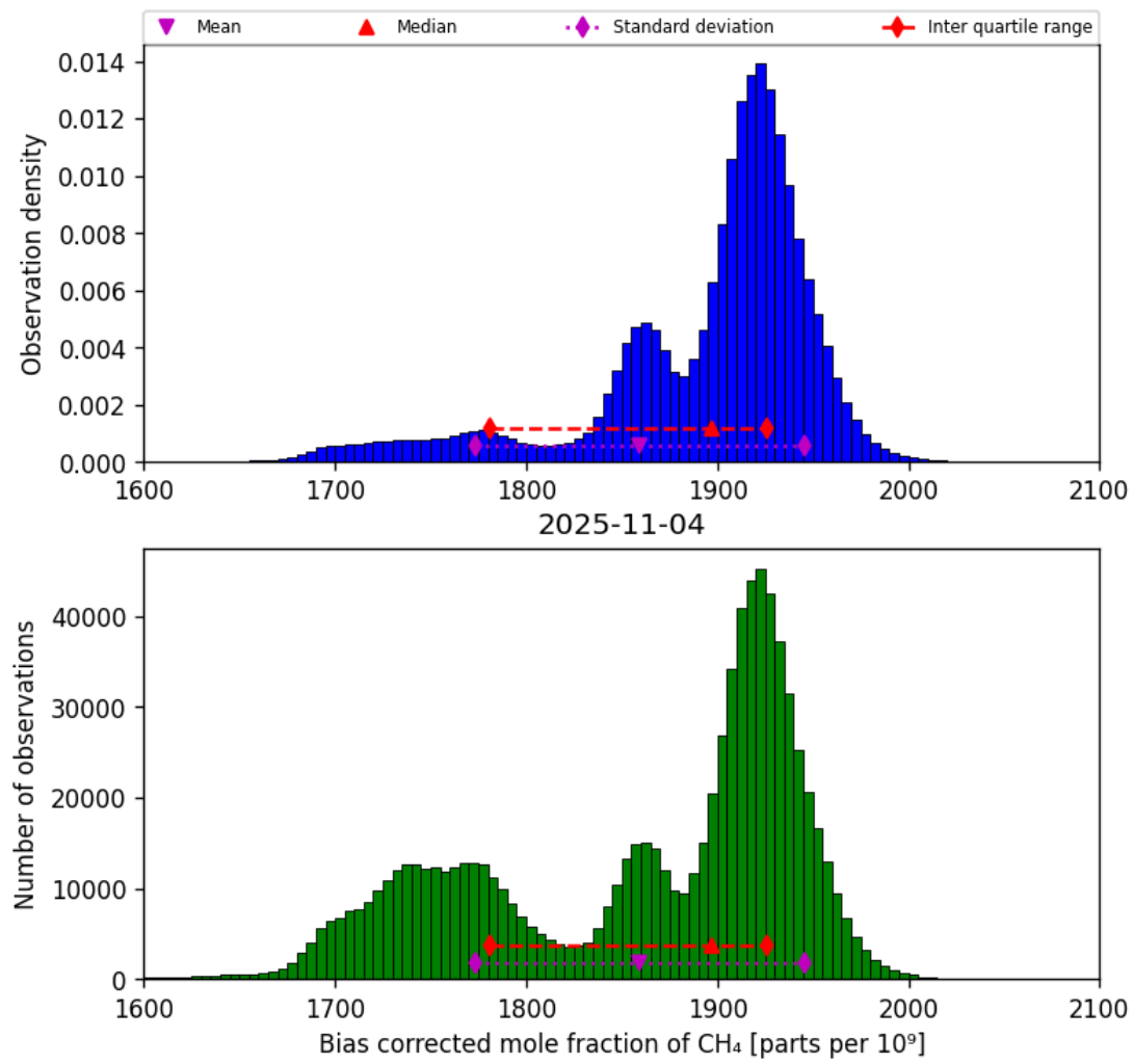
Figure 25: Histogram of “Bias corrected mole fraction of CH 4 ” for 2025-11-03 to 2025-11-05
