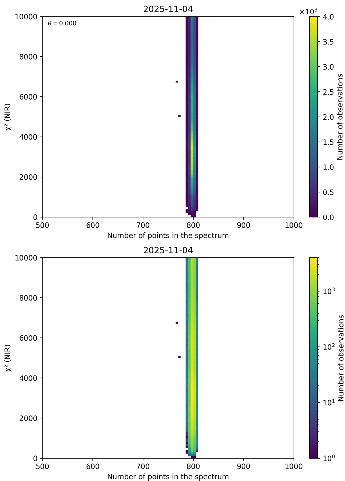
Figure 88: Scatter density plot of “Number of points in the spectrum” against “ \chi^2 (NIR)” for 2025-11-03 to 2025-11-05.
