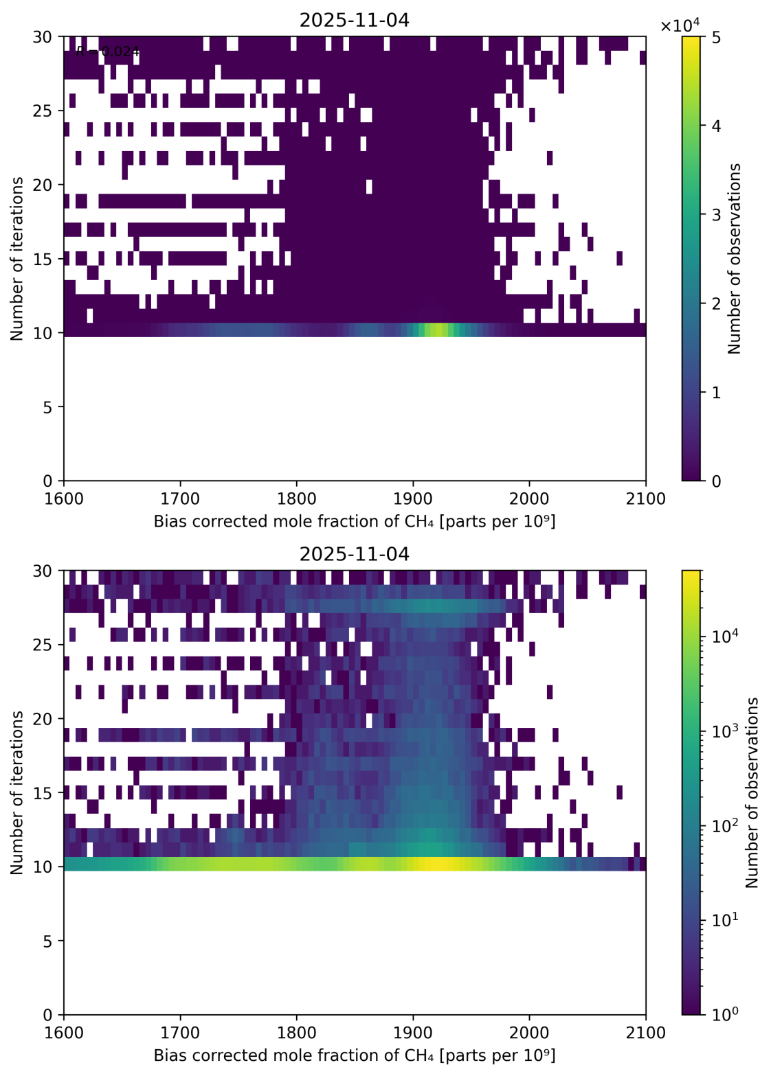
Figure 67: Scatter density plot of “Bias corrected mole fraction of \text{CH}_4 ” against “Number of iterations” for 2025-11-03 to 2025-11-05.
