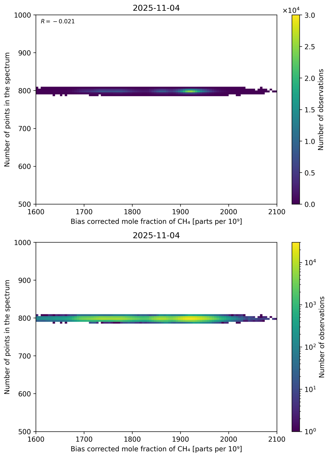
Figure 68: Scatter density plot of “Bias corrected mole fraction of CH 4 ” against “Number of points in the spectrum” for 2025-11-03 to 2025-11-05.
