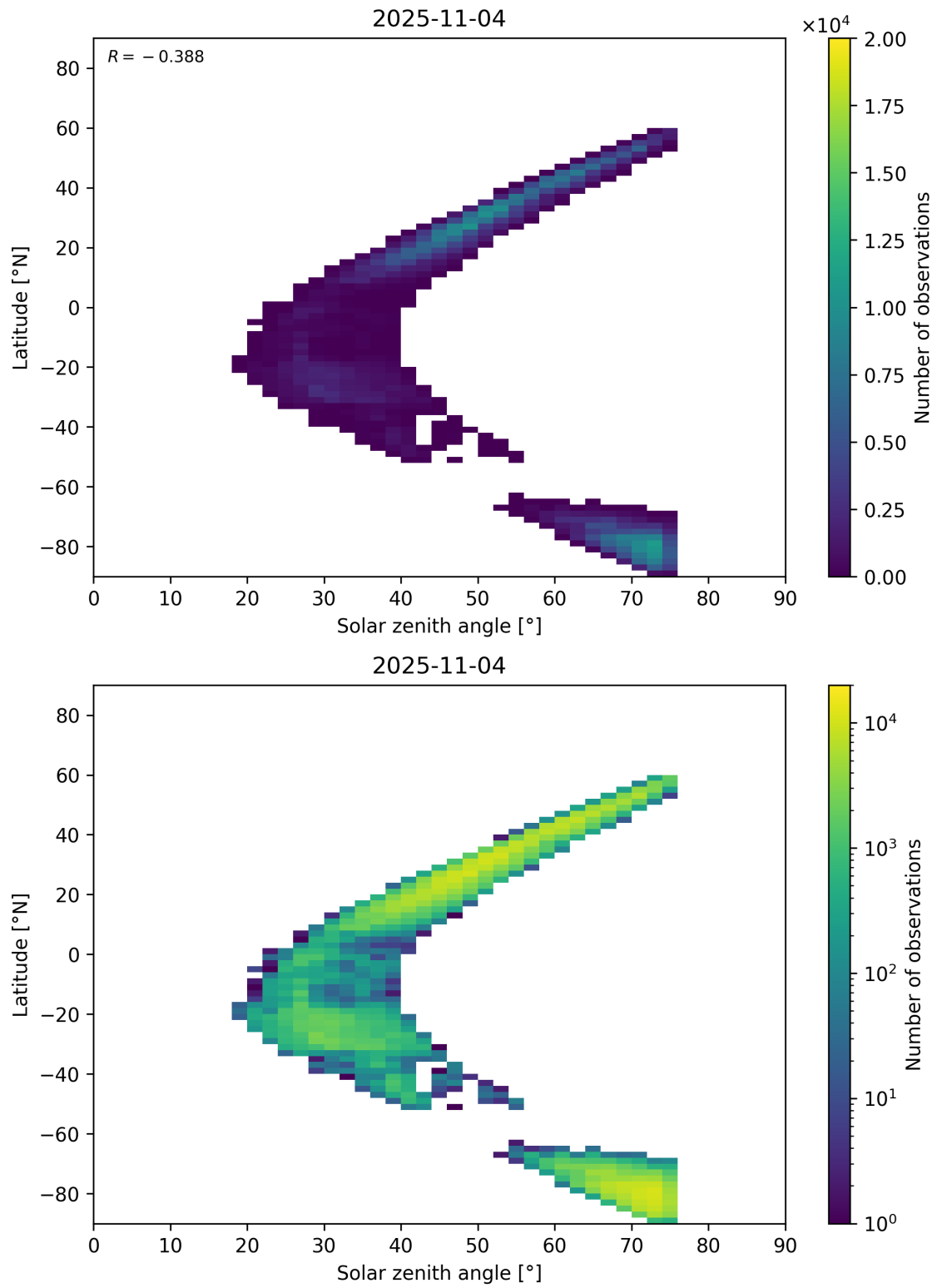
Figure 98: Scatter density plot of “Solar zenith angle” against “Latitude” for 2025-11-03 to 2025-11-05.
