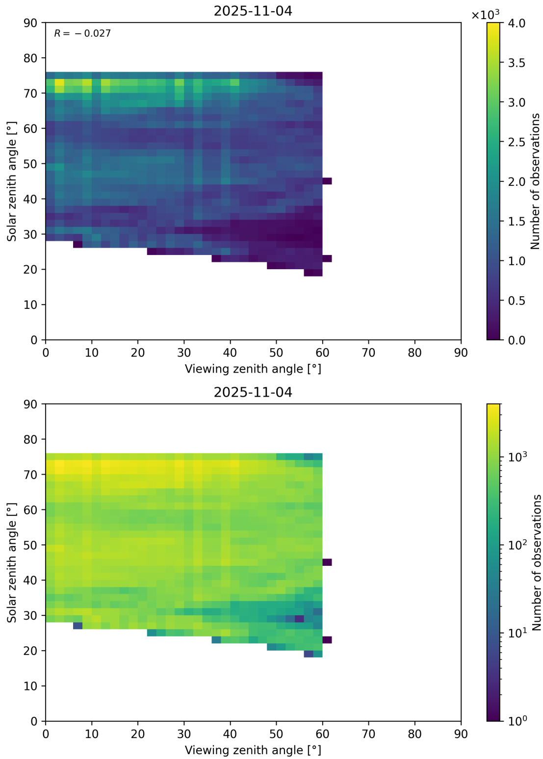
Figure 115: Scatter density plot of “Viewing zenith angle” against “Solar zenith angle” for 2025-11-03 to 2025-11-05.
