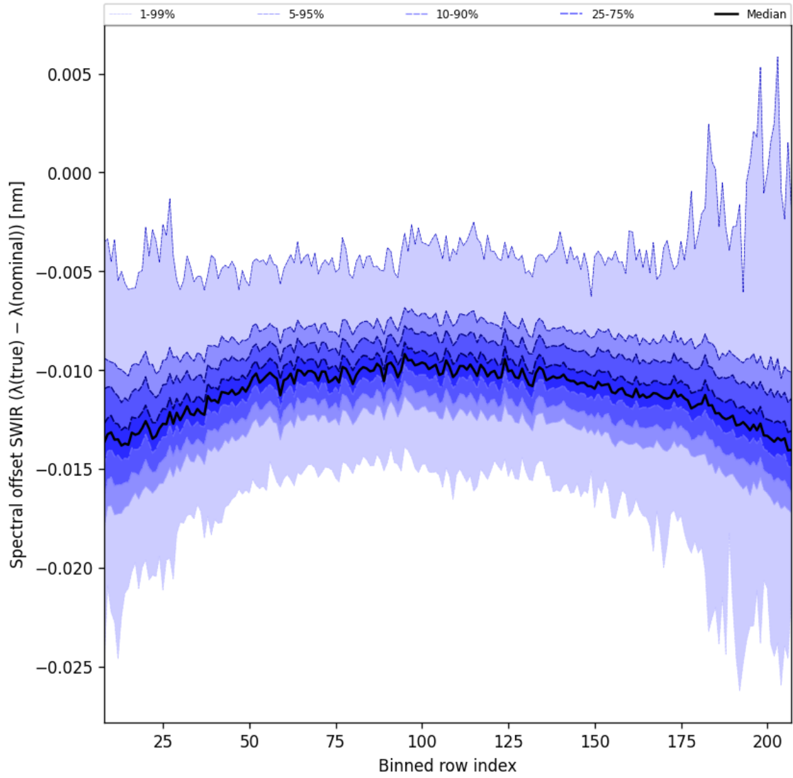
Figure 38: Along track statistics of “Spectral offset SWIR ( \lambda_{\text{true}} - \lambda_{\text{nominal}} )” for 2025-11-03 to 2025-11-05
