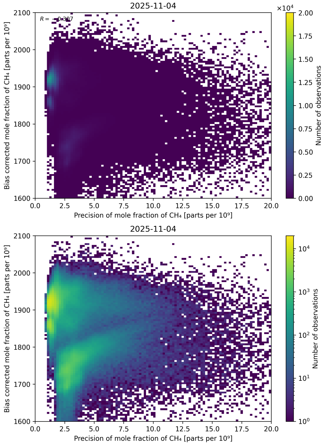
Figure 82: Scatter density plot of “Precision of mole fraction of CH 4 ” against “Bias corrected mole fraction of CH 4 ” for 2025-11-03 to 2025-11-05.
