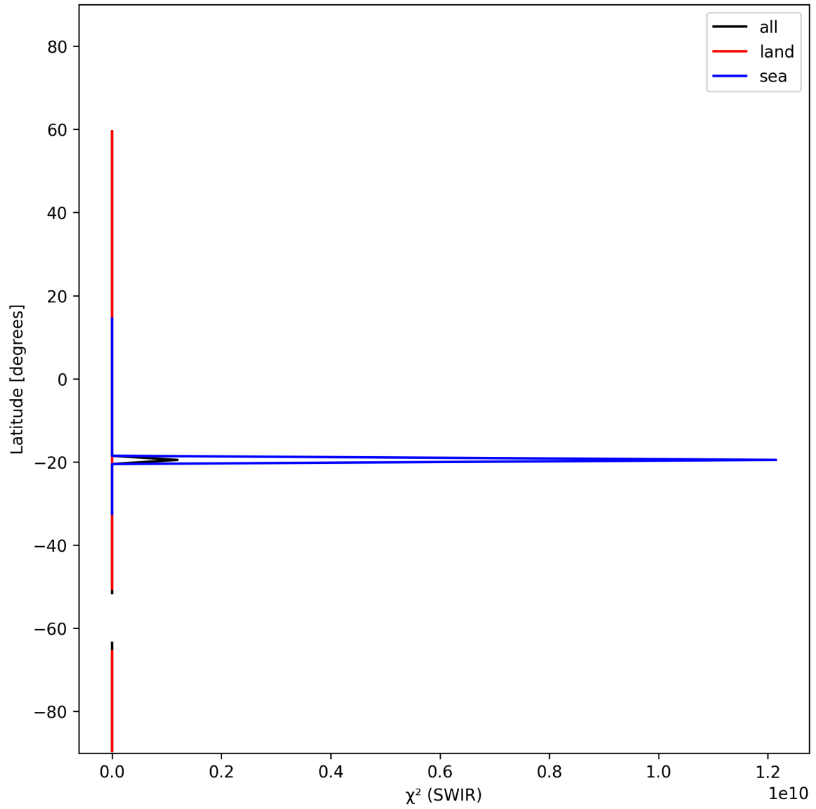
Figure 17: Zonal average of “ \chi^2 (SWIR)” for 2025-11-03 to 2025-11-05.
