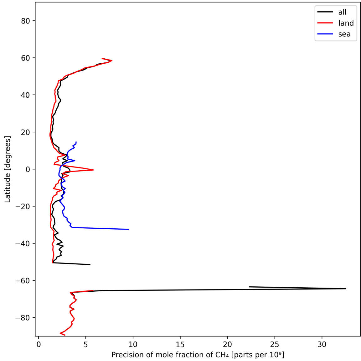
Figure 13: Zonal average of “Precision of mole fraction of CH 4 ” for 2025-11-03 to 2025-11-05.
