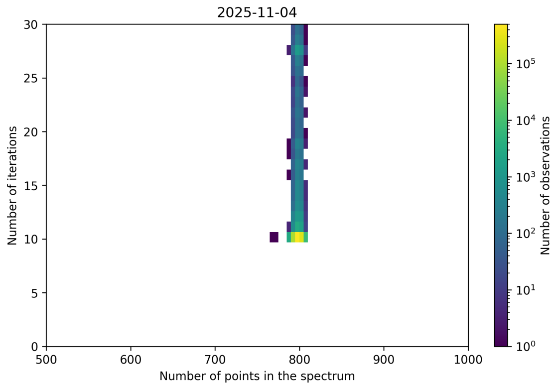
Figure 92: Scatter density plot of “Number of points in the spectrum” against “Number of iterations” for 2025-11-03 to 2025-11-05.
