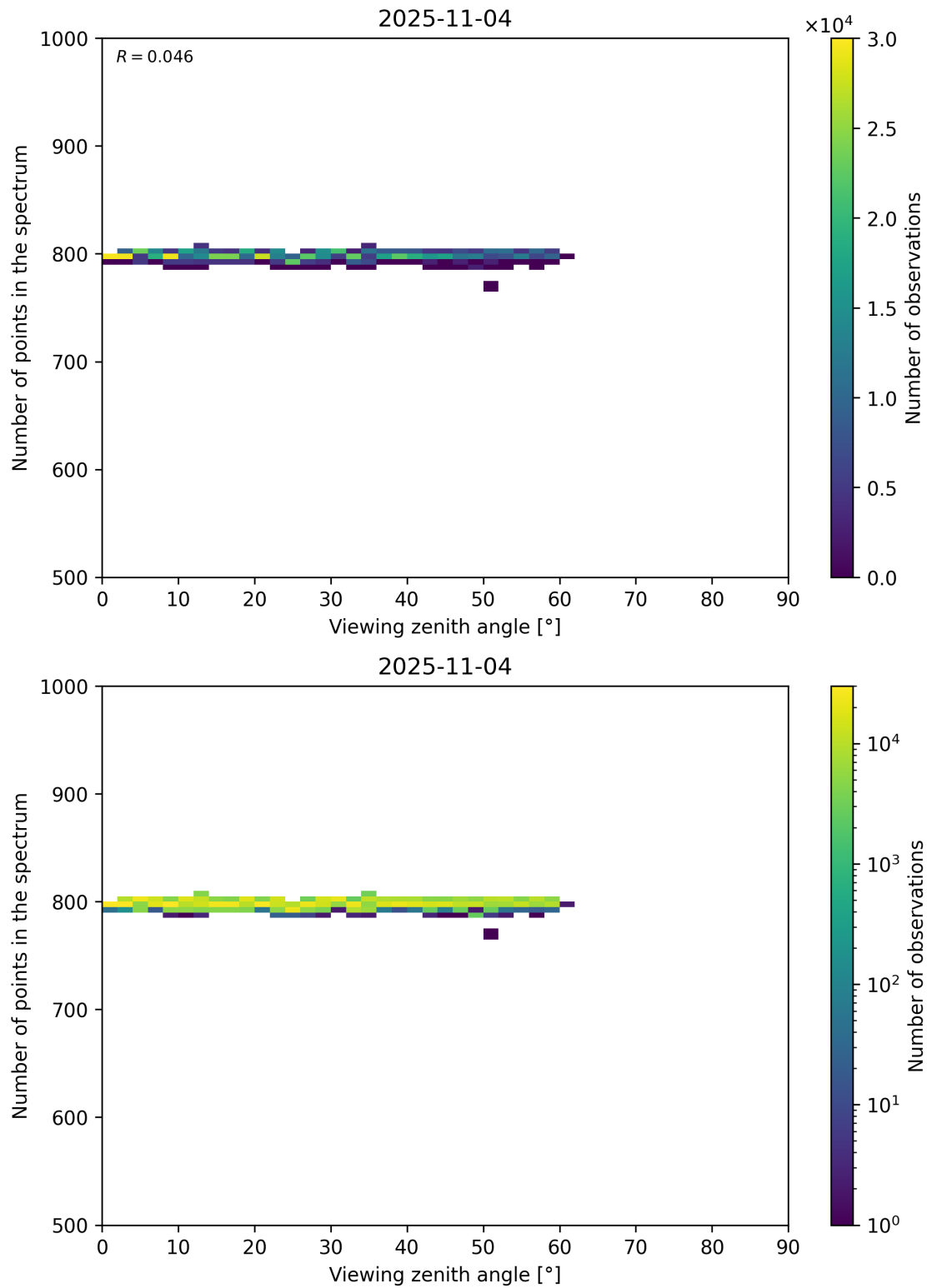
Figure 114: Scatter density plot of “Viewing zenith angle” against “Number of points in the spectrum” for 2025-11-03 to 2025-11-05.
