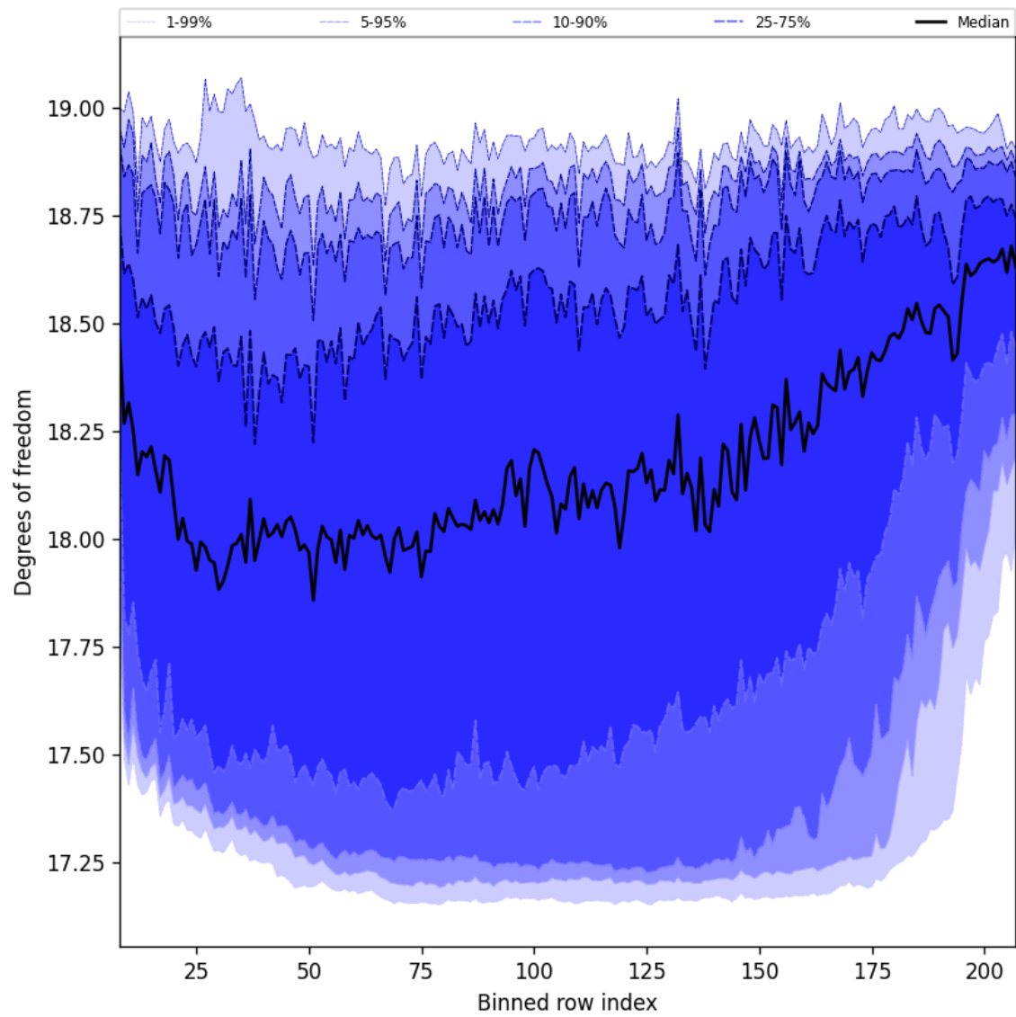
Figure 41: Along track statistics of “Degrees of freedom” for 2025-11-03 to 2025-11-05
