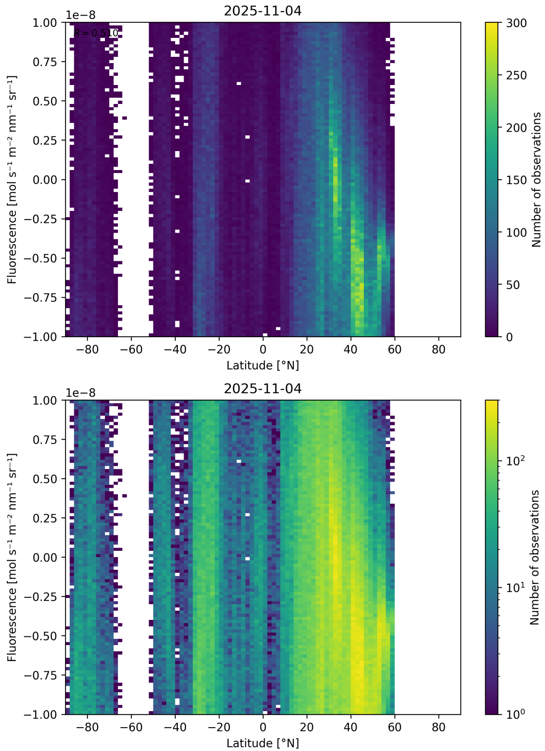
Figure 56: Scatter density plot of “Latitude” against “Fluorescence” for 2025-11-03 to 2025-11-05.
