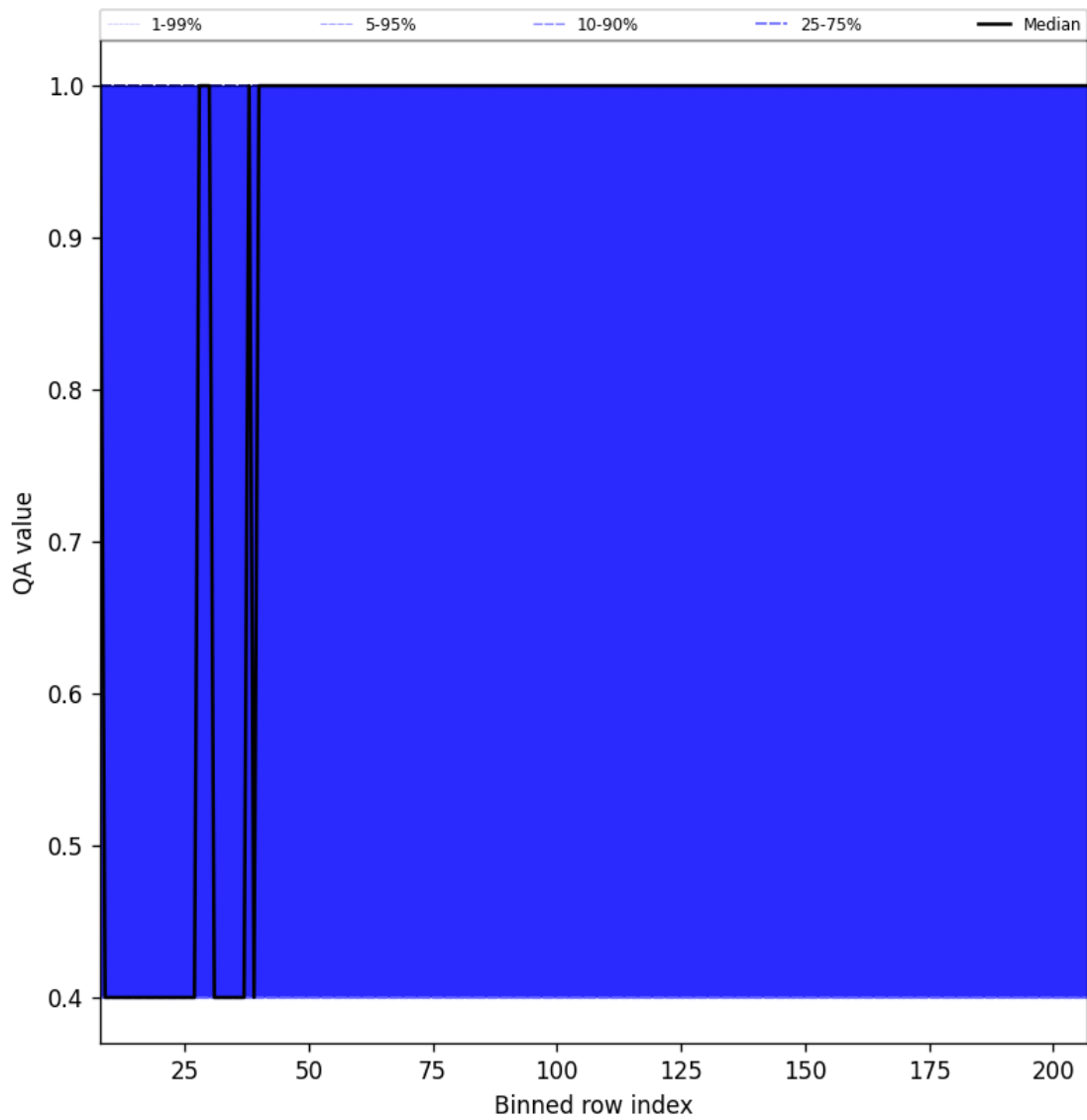
Figure 33: Along track statistics of “QA value” for 2025-11-03 to 2025-11-05
