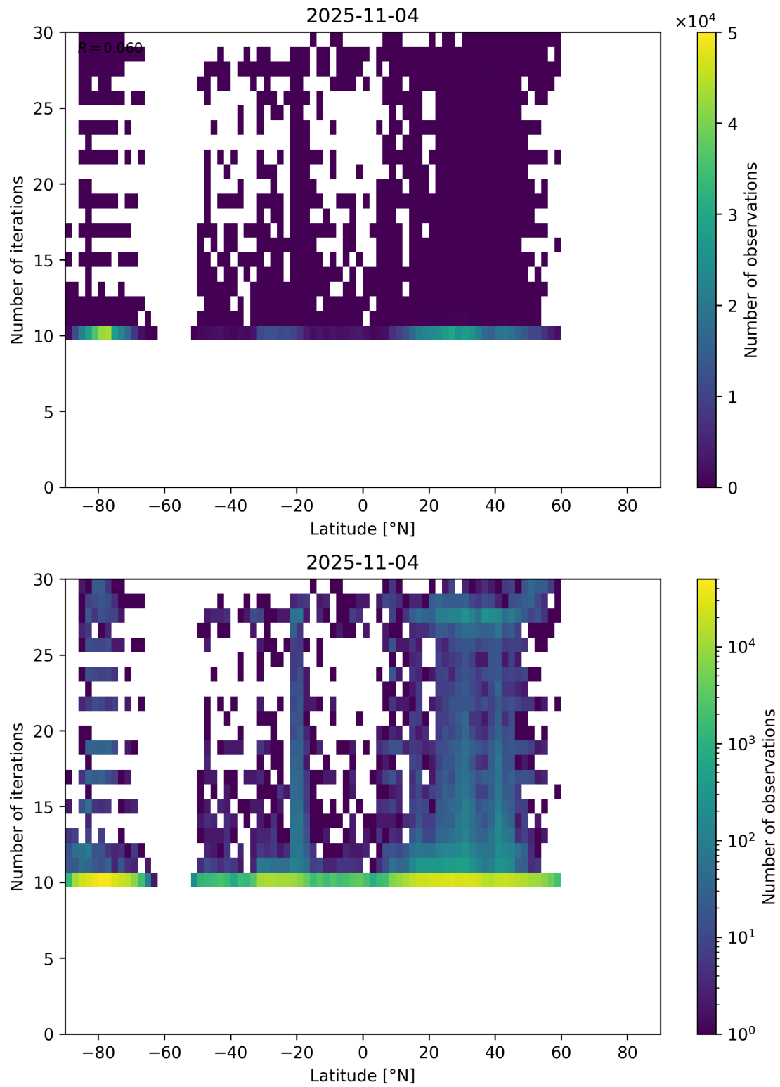
Figure 60: Scatter density plot of “Latitude” against “Number of iterations” for 2025-11-03 to 2025-11-05.
