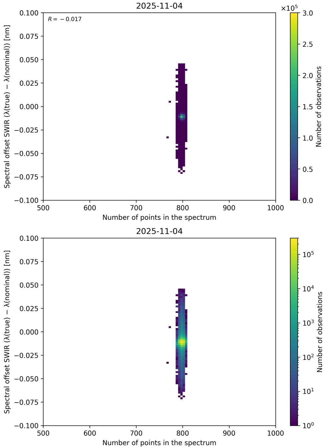
Figure 93: Scatter density plot of “Number of points in the spectrum” against “Spectral offset SWIR ( \lambda_{\text{true}} - \lambda_{\text{nominal}} )” for 2025-11-03 to 2025-11-05.
