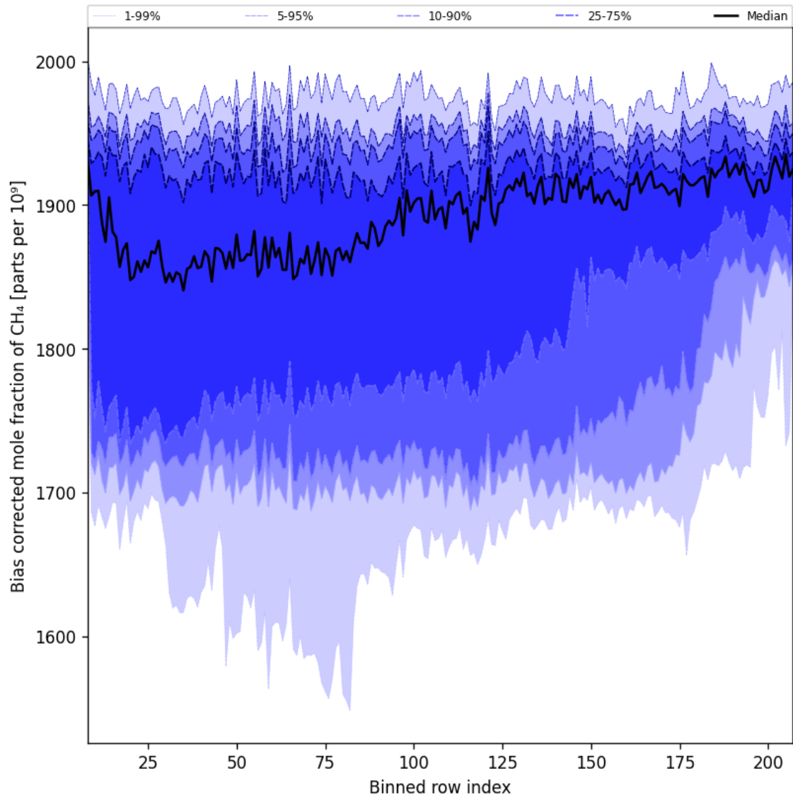
Figure 36: Along track statistics of “Bias corrected mole fraction of CH 4 ” for 2025-11-03 to 2025-11-05
