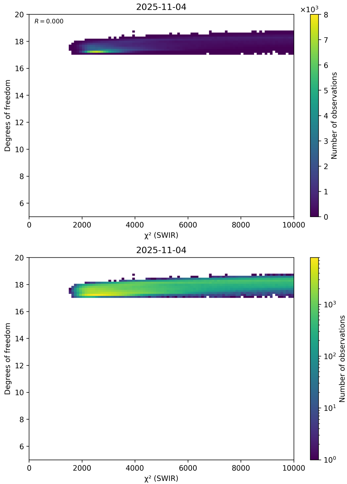
Figure 48: Scatter density plot of “ \chi^2 (SWIR)” against “Degrees of freedom” for 2025-11-03 to 2025-11-05.
