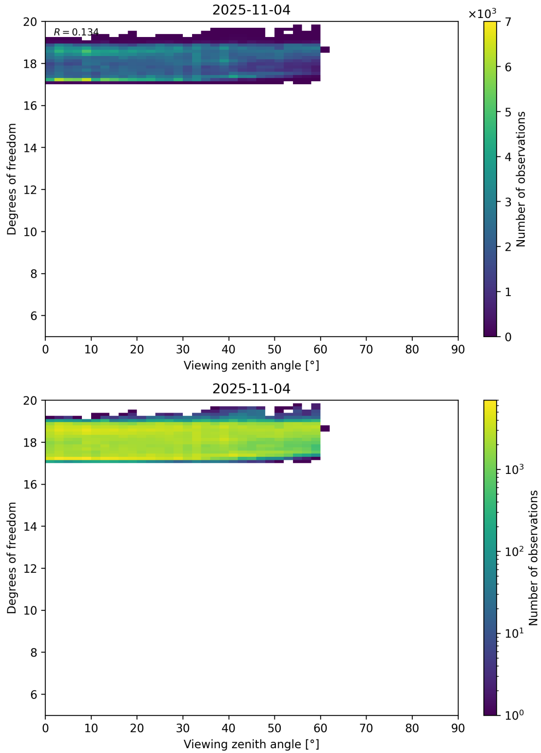
Figure 107: Scatter density plot of “Viewing zenith angle” against “Degrees of freedom” for 2025-11-03 to 2025-11-05.
