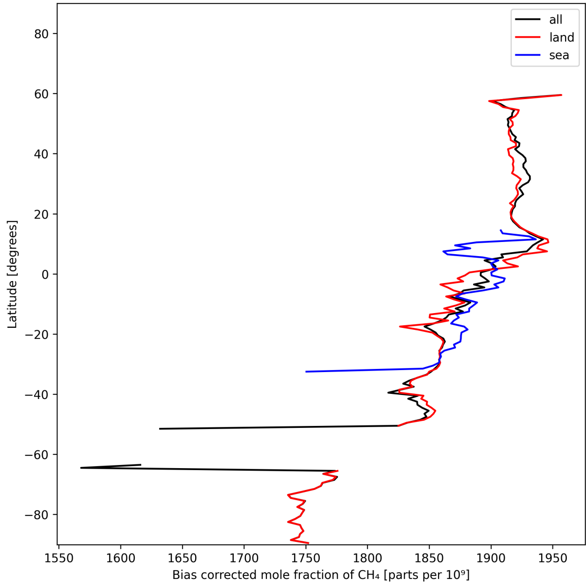
Figure 14: Zonal average of “Bias corrected mole fraction of \text{CH}_4 ” for 2025-11-03 to 2025-11-05.
