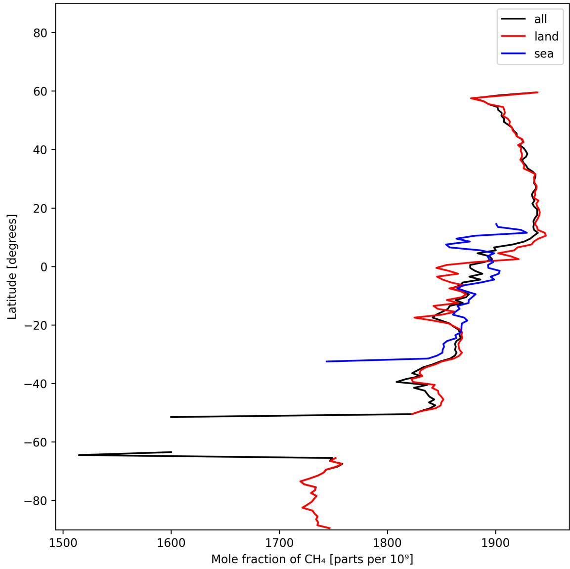
Figure 12: Zonal average of “Mole fraction of \text{CH}_4 ” for 2025-11-03 to 2025-11-05.
