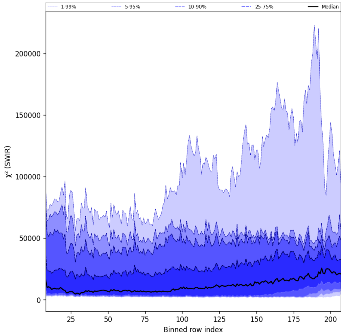
Figure 39: Along track statistics of “ \chi^2 (SWIR)” for 2025-11-03 to 2025-11-05
