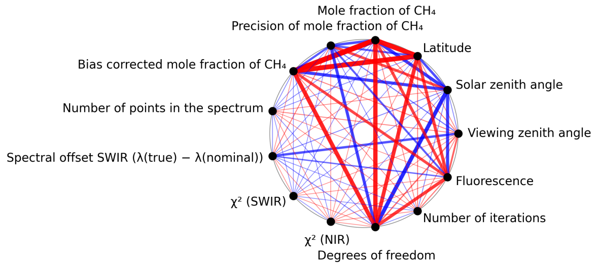
Figure 1: Map of correlation graph for 2025-11-03 to 2025-11-05.
