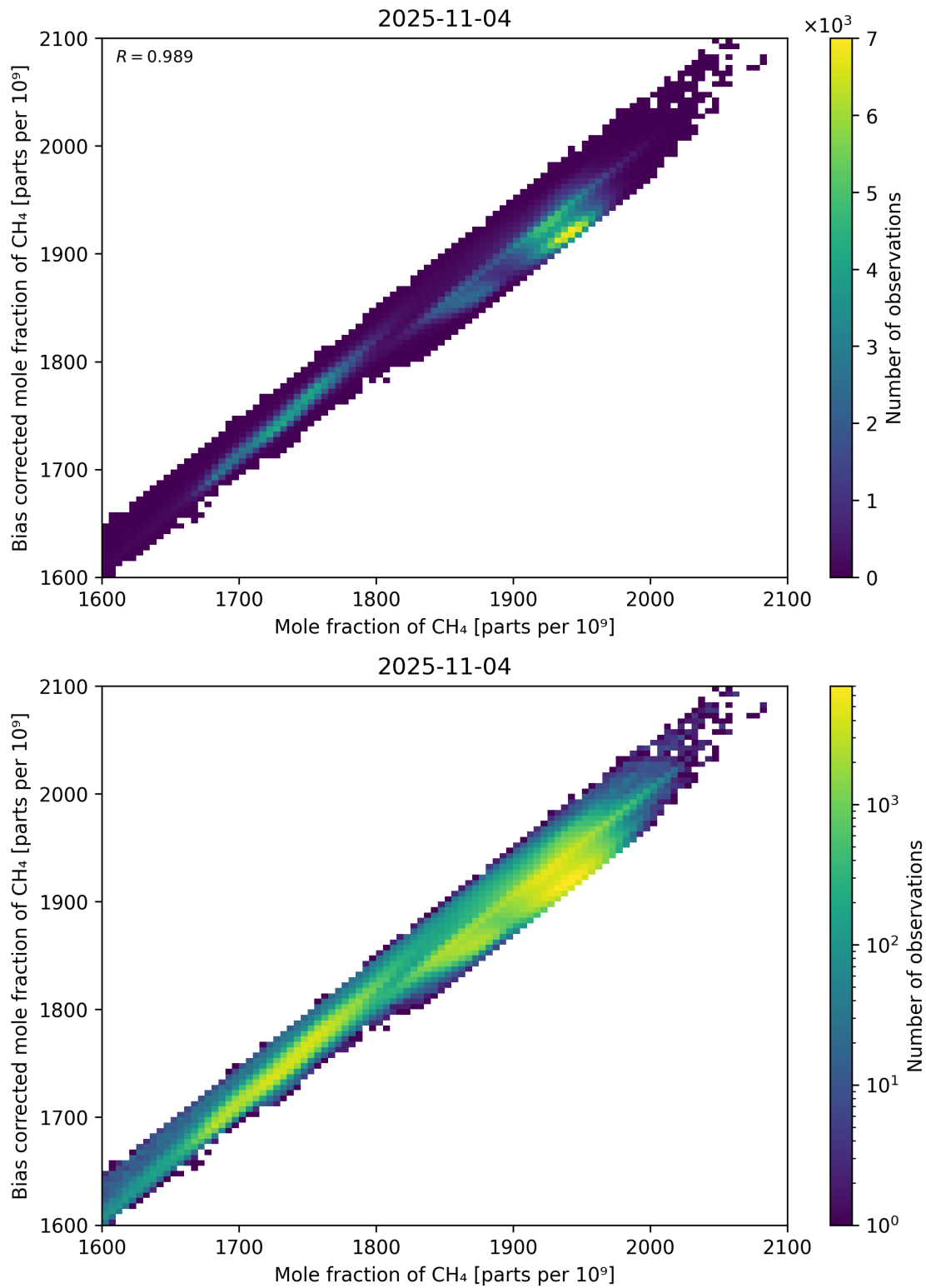
Figure 74: Scatter density plot of “Mole fraction of CH 4 ” against “Bias corrected mole fraction of CH 4 ” for 2025-11-03 to 2025-11-05.
