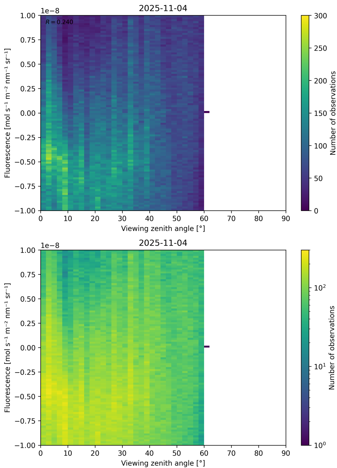
Figure 108: Scatter density plot of “Viewing zenith angle” against “Fluorescence” for 2025-11-03 to 2025-11-05.
