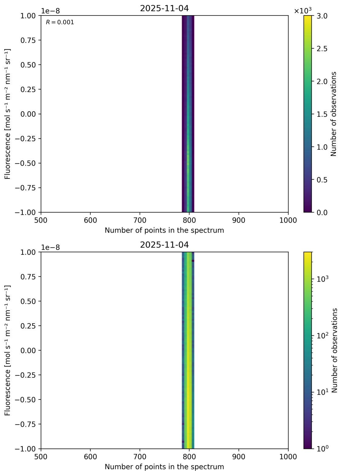
Figure 91: Scatter density plot of “Number of points in the spectrum” against “Fluorescence” for 2025-11-03 to 2025-11-05.
