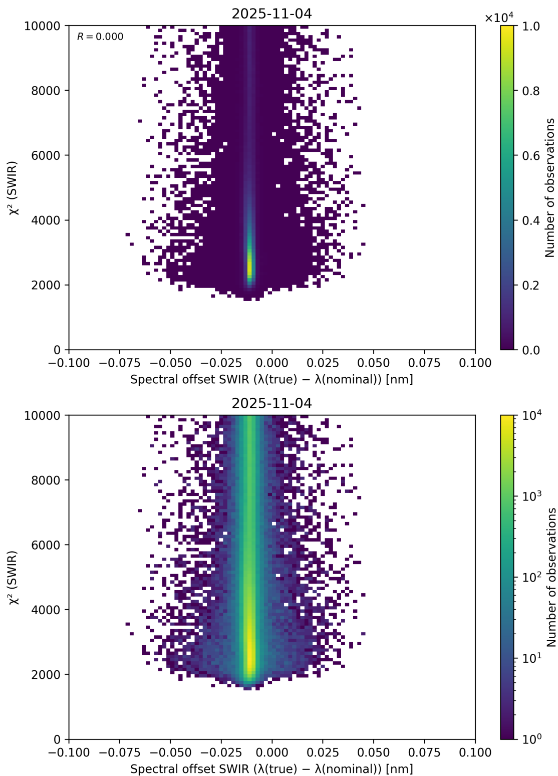
Figure 118: Scatter density plot of “Spectral offset SWIR ( \lambda_{\text{true}} - \lambda_{\text{nominal}} )” against “ \chi^2 (SWIR)” for 2025-11-03 to 2025-11-05.
