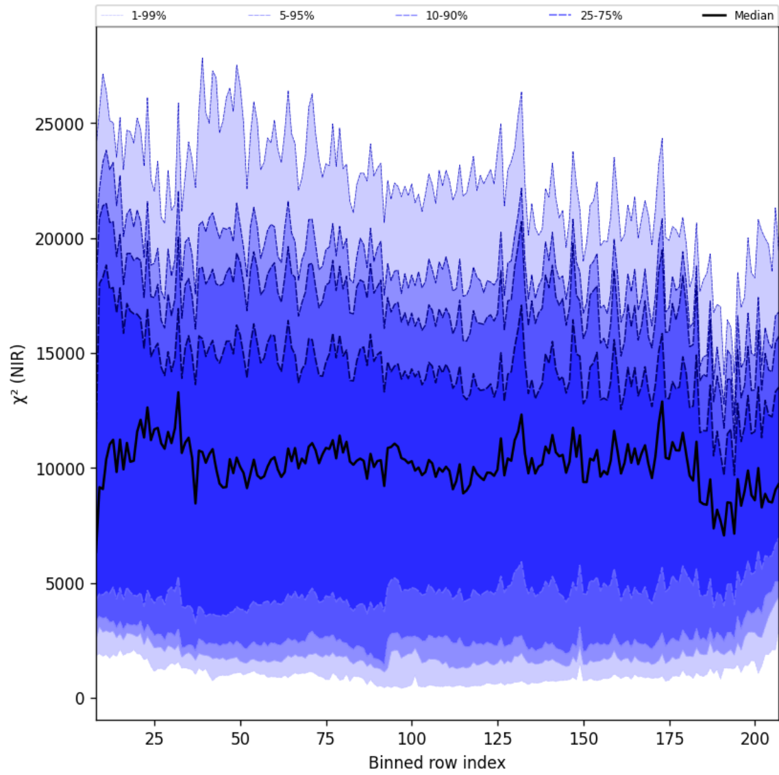
Figure 40: Along track statistics of " \chi^2 (NIR)" for 2025-11-03 to 2025-11-05
