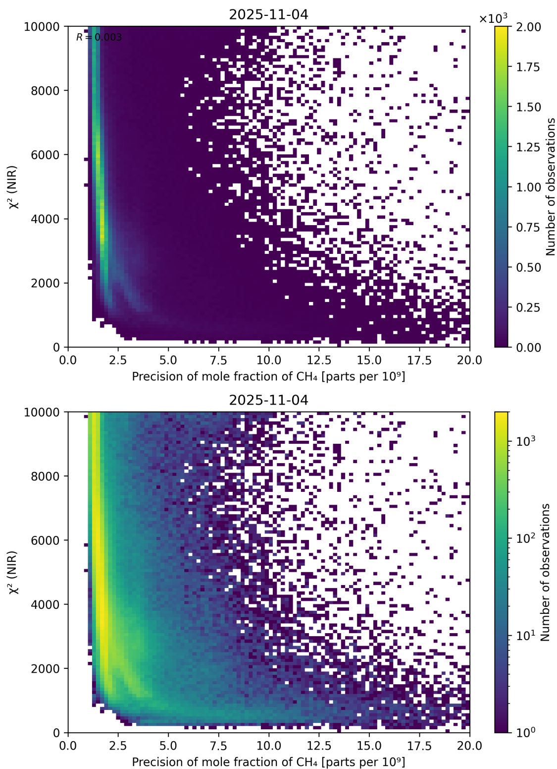
Figure 78: Scatter density plot of “Precision of mole fraction of CH 4 ” against “ \chi^2 (NIR)” for 2025-11-03 to 2025-11-05.
