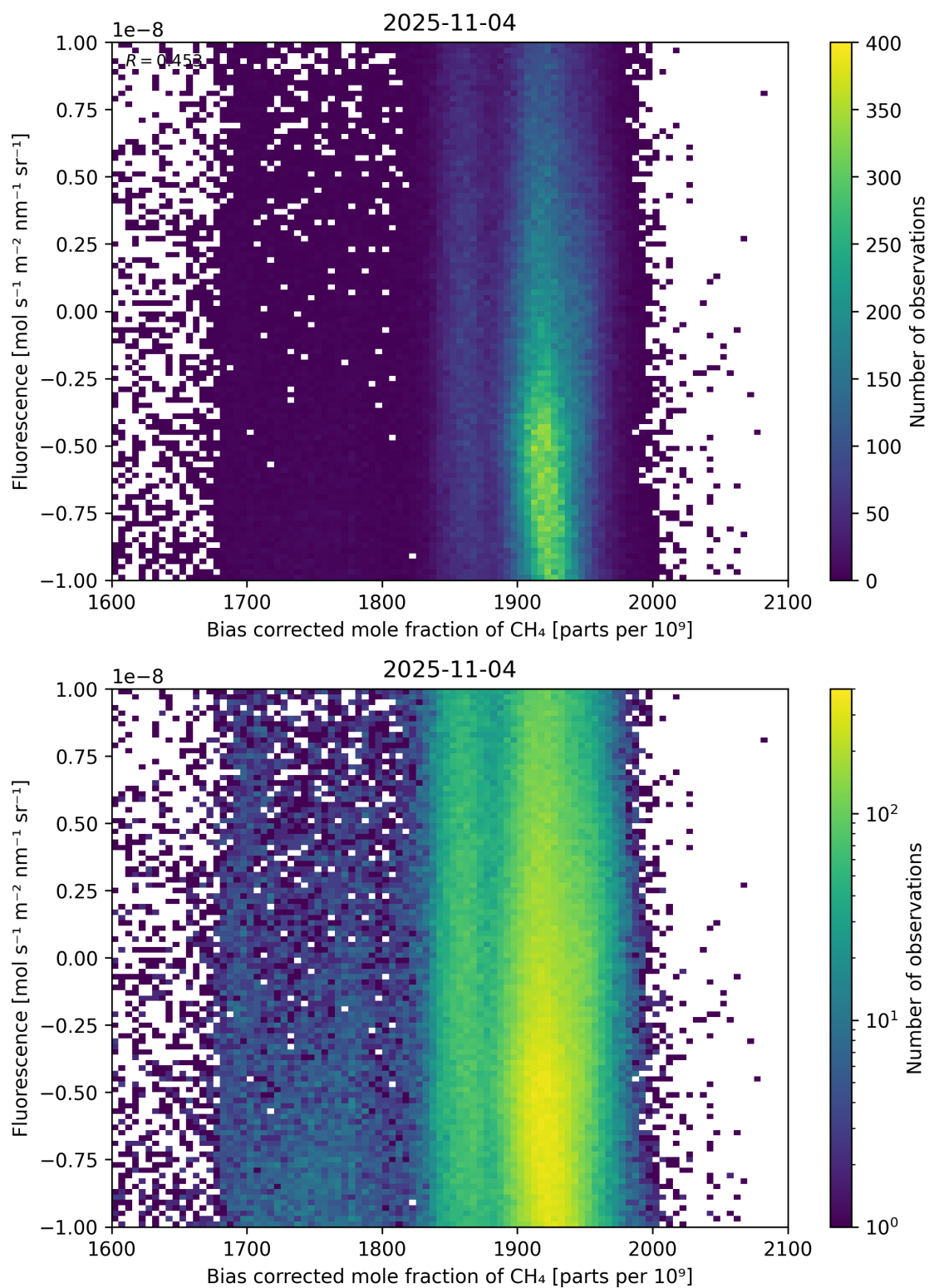
Figure 66: Scatter density plot of “Bias corrected mole fraction of \text{CH}_4 ” against “Fluorescence” for 2025-11-03 to 2025-11-05.
