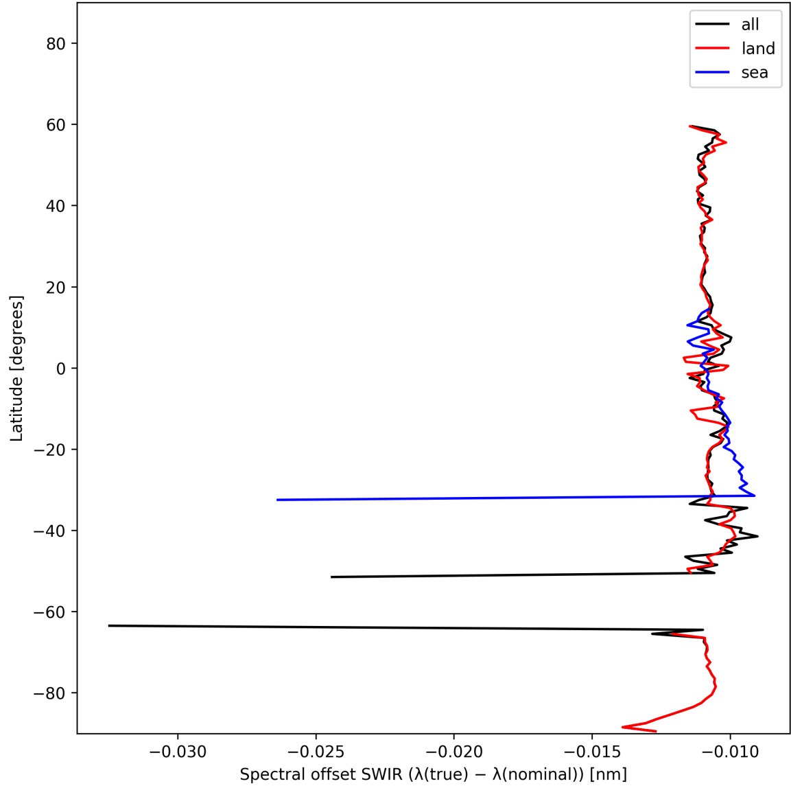
Figure 16: Zonal average of “Spectral offset SWIR ( \lambda_{\text{true}} - \lambda_{\text{nominal}} )” for 2025-11-03 to 2025-11-05.
