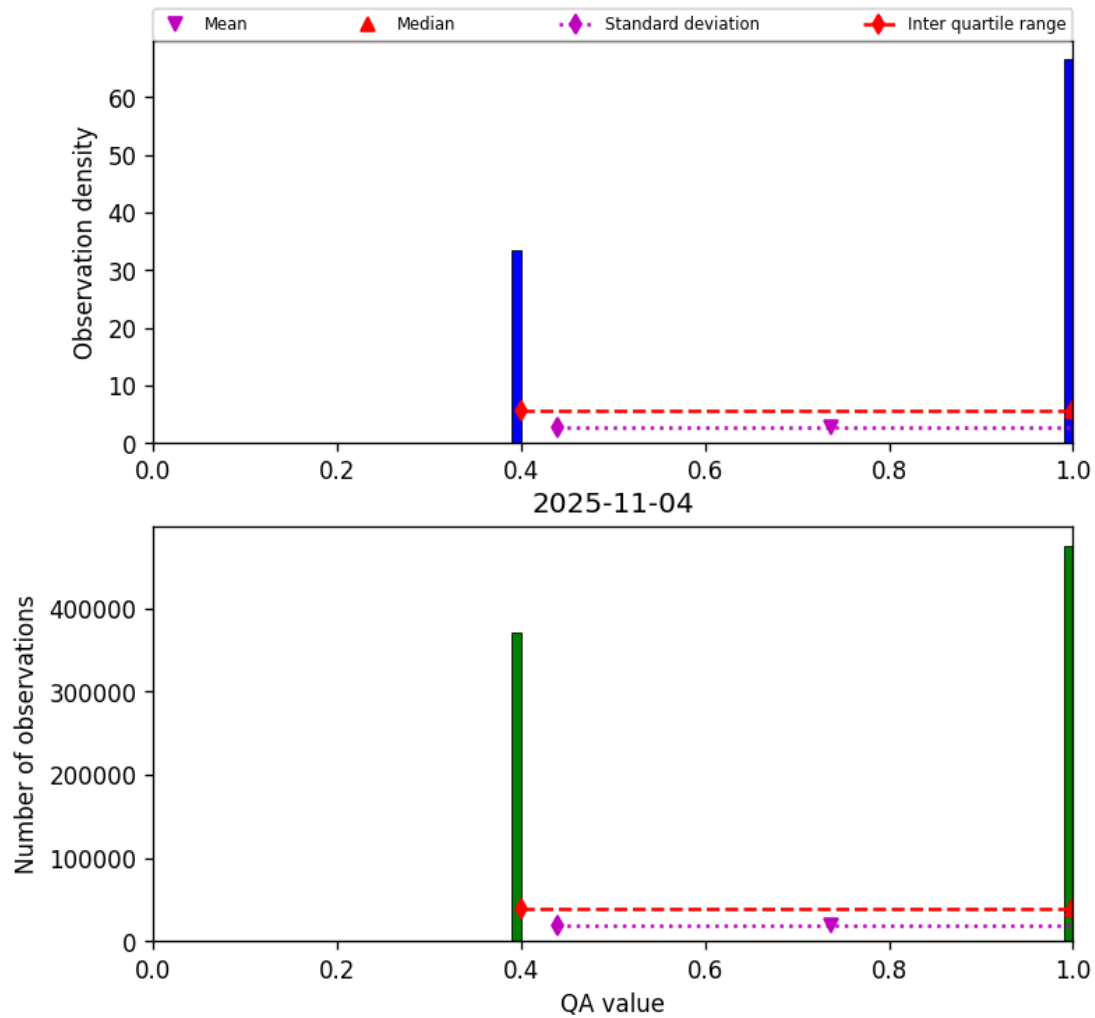
Figure 22: Histogram of “QA value” for 2025-11-03 to 2025-11-05
