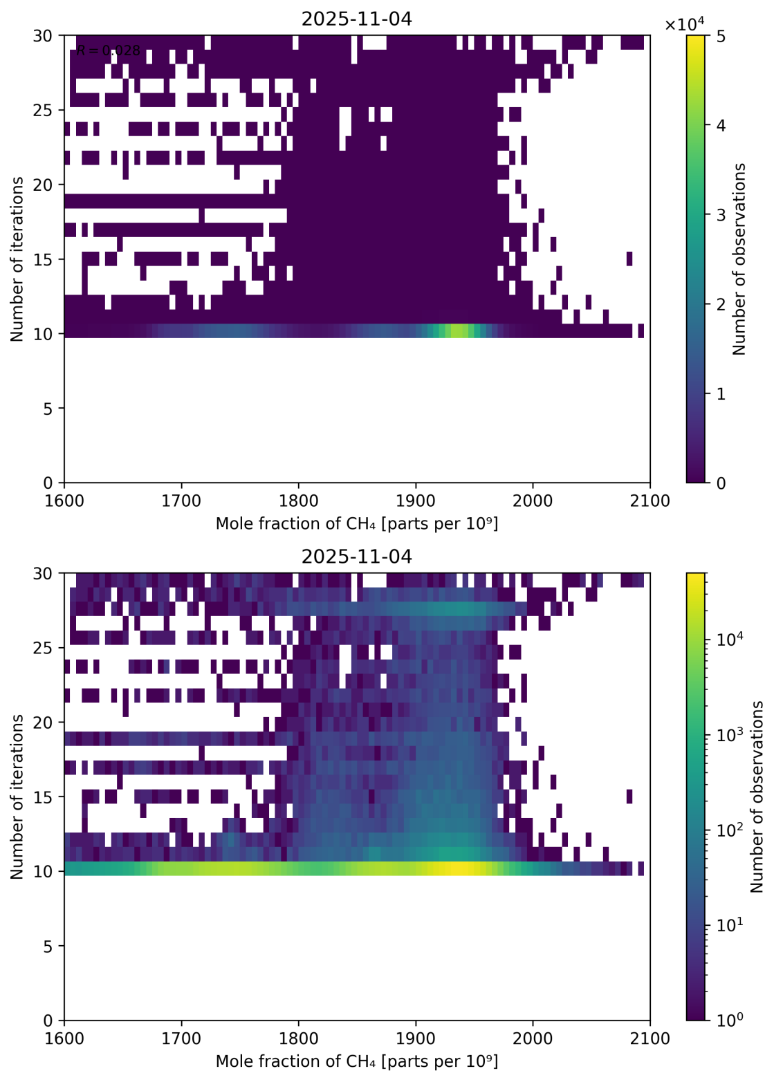
Figure 76: Scatter density plot of “Mole fraction of CH 4 ” against “Number of iterations” for 2025-11-03 to 2025-11-05.
