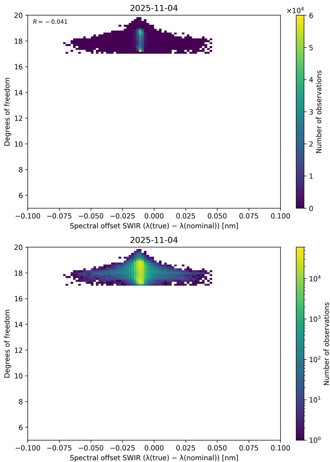
Figure 119: Scatter density plot of “Spectral offset SWIR ( \lambda_{\text{true}} - \lambda_{\text{nominal}} )” against “Degrees of freedom” for 2025-11-03 to 2025-11-05.
