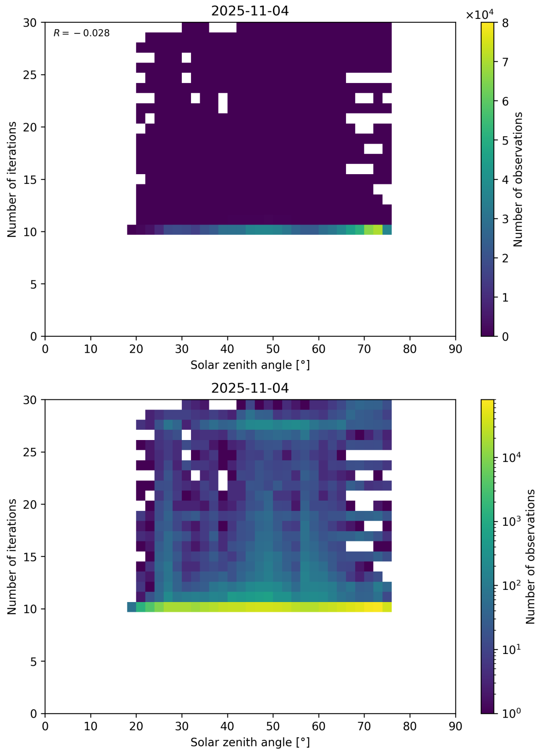
Figure 102: Scatter density plot of “Solar zenith angle” against “Number of iterations” for 2025-11-03 to 2025-11-05.
