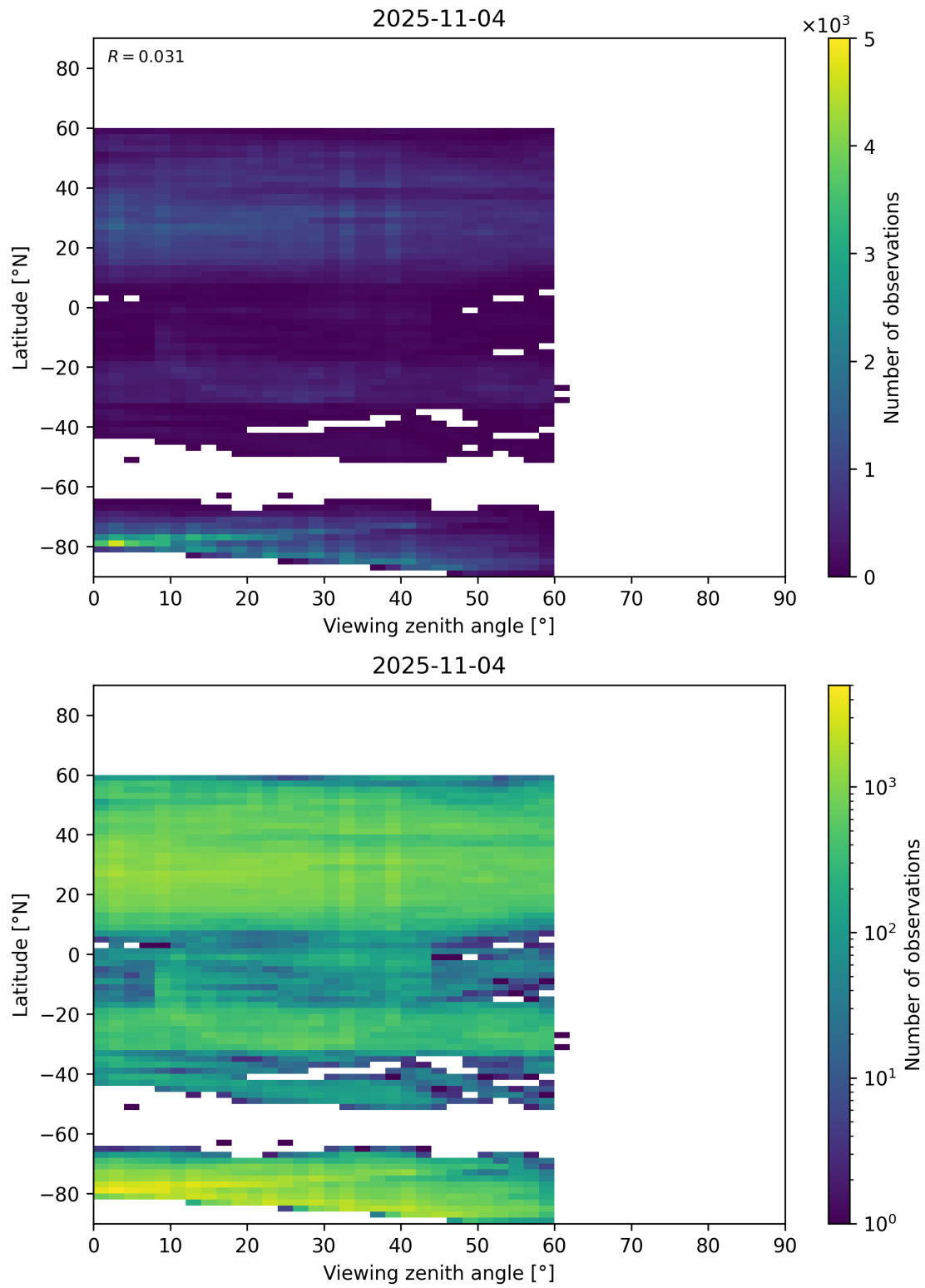
Figure 109: Scatter density plot of “Viewing zenith angle” against “Latitude” for 2025-11-03 to 2025-11-05.
