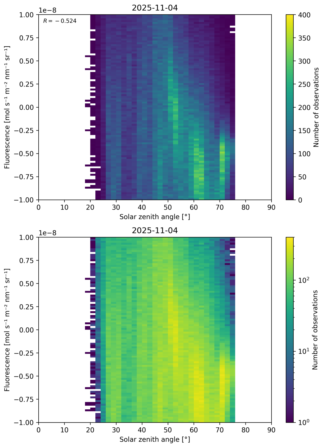
Figure 97: Scatter density plot of “Solar zenith angle” against “Fluorescence” for 2025-11-03 to 2025-11-05.
