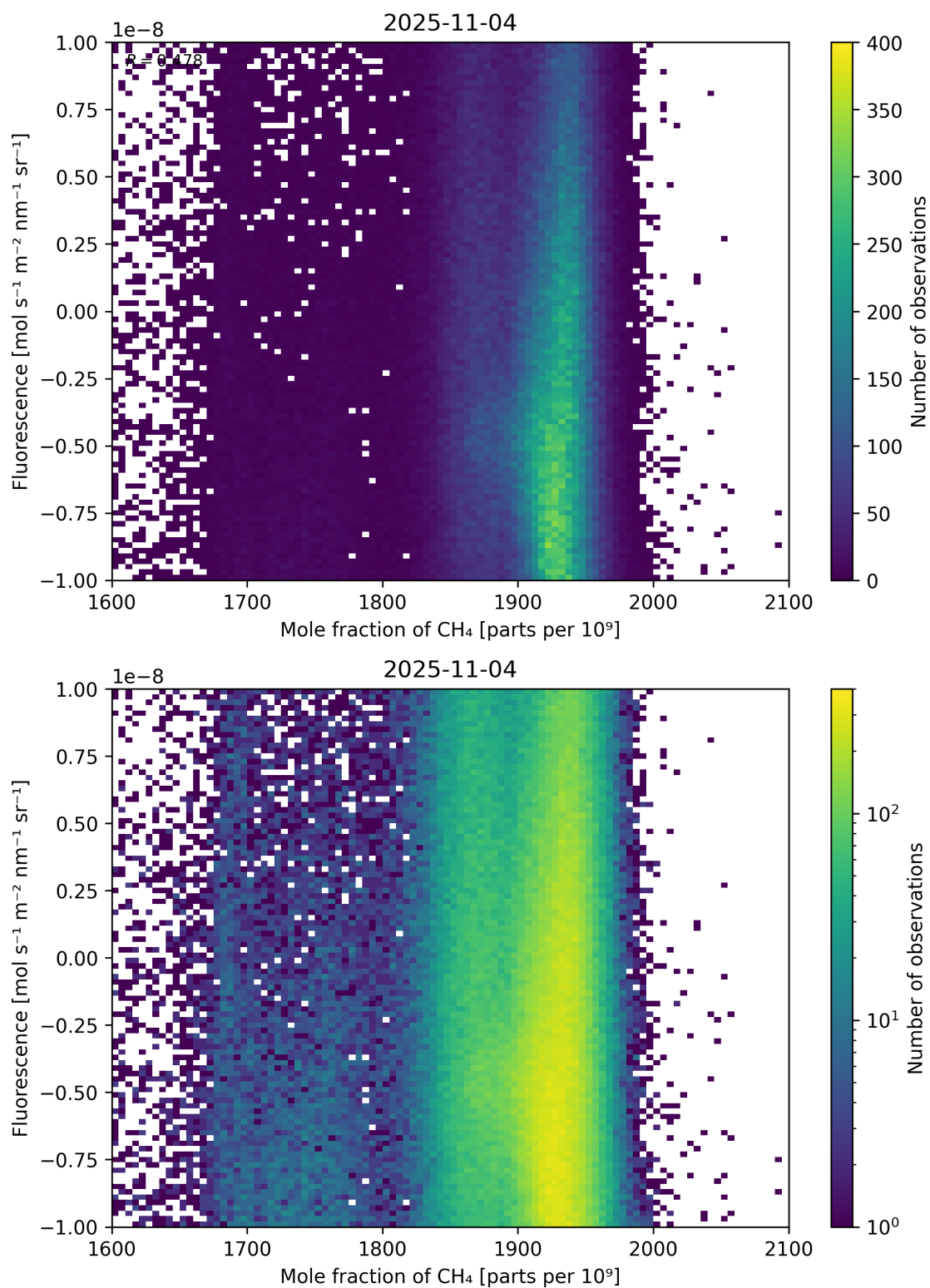
Figure 73: Scatter density plot of “Mole fraction of \text{CH}_4 ” against “Fluorescence” for 2025-11-03 to 2025-11-05.
