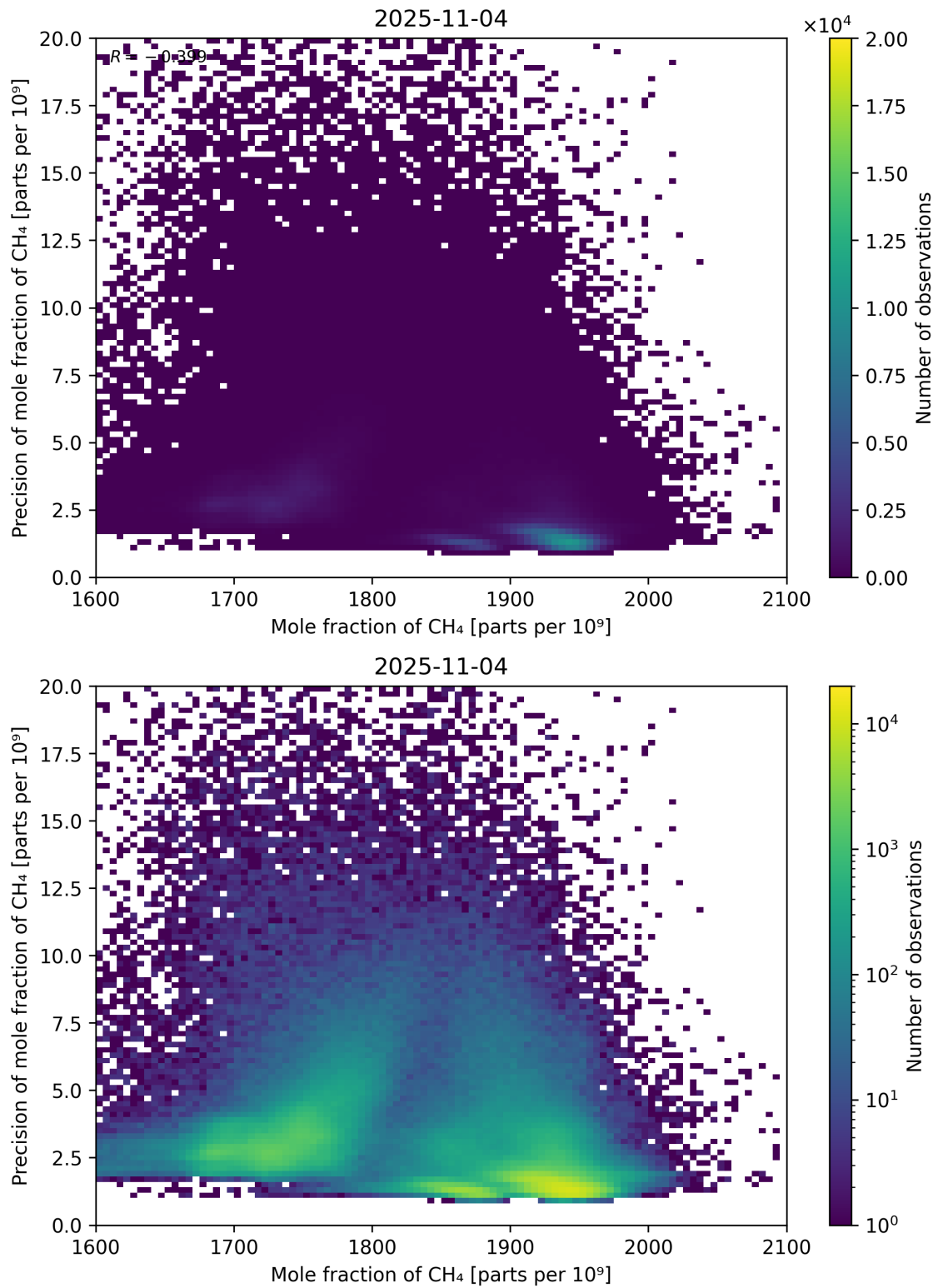
Figure 75: Scatter density plot of “Mole fraction of CH 4 ” against “Precision of mole fraction of CH 4 ” for 2025-11-03 to 2025-11-05.
