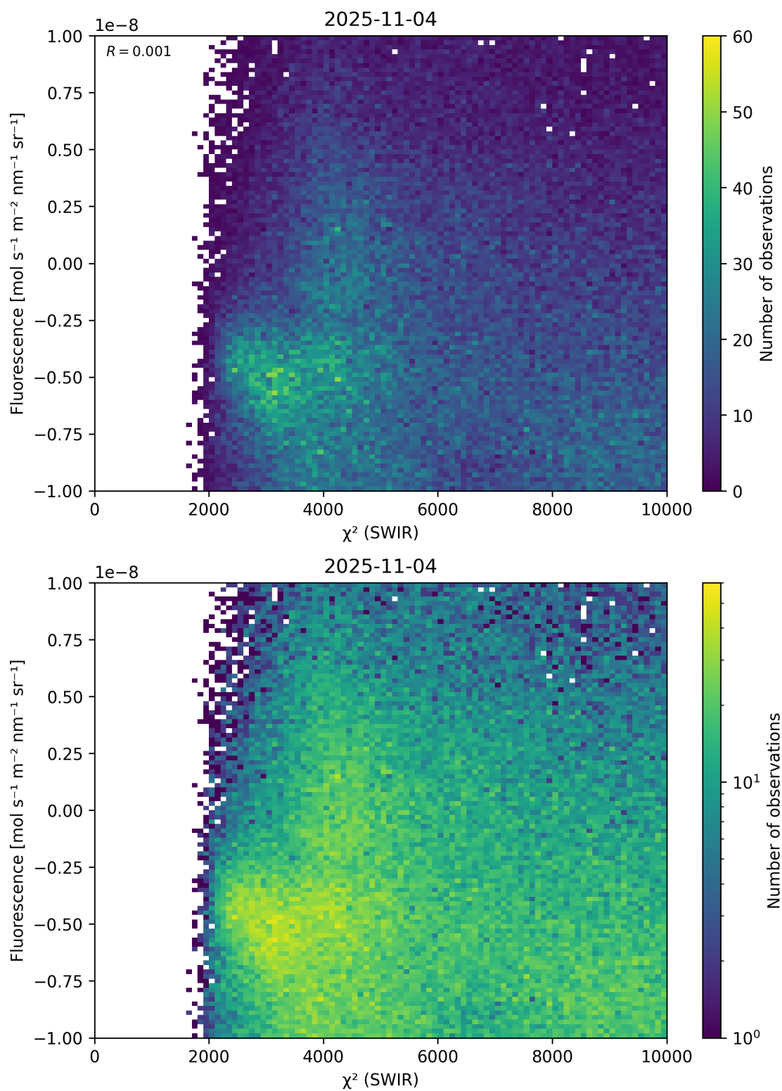
Figure 49: Scatter density plot of “ \chi^2 (SWIR)” against “Fluorescence” for 2025-11-03 to 2025-11-05.
