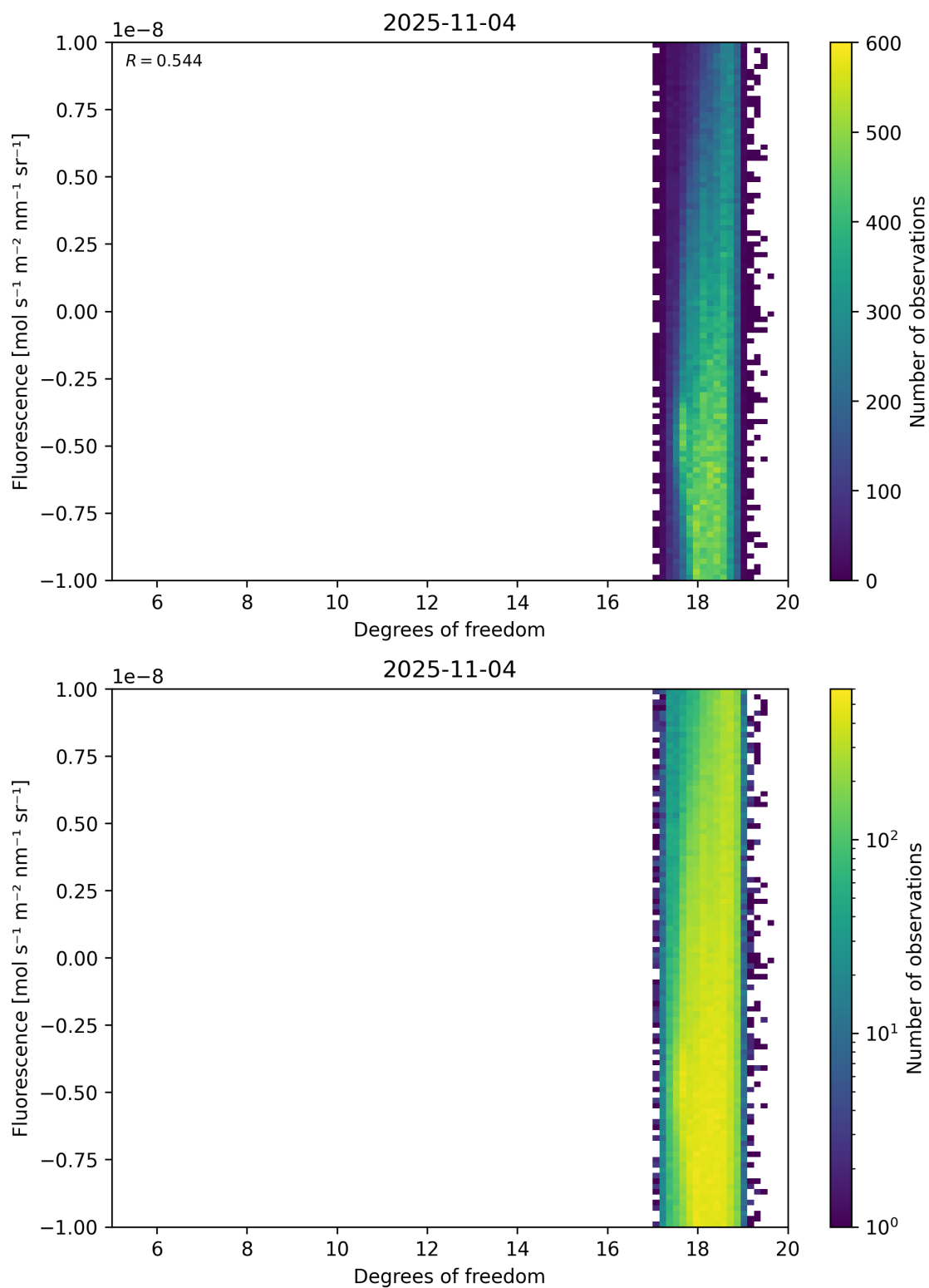
Figure 51: Scatter density plot of “Degrees of freedom” against “Fluorescence” for 2025-11-03 to 2025-11-05.
