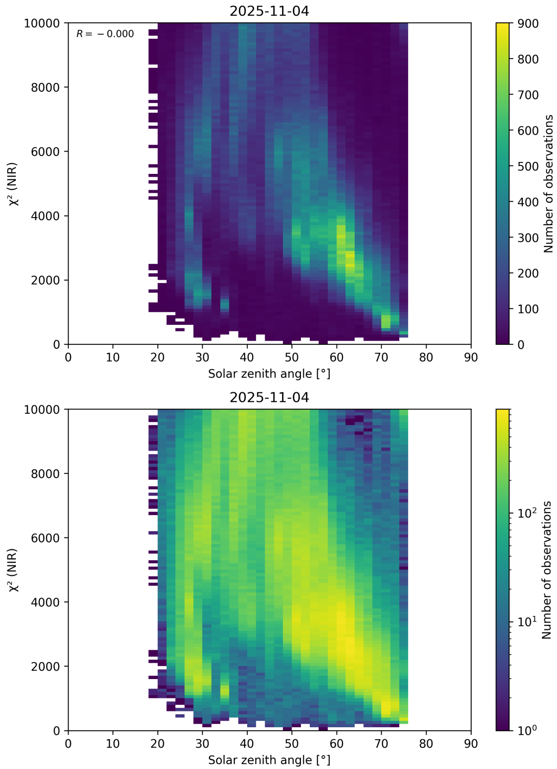
Figure 94: Scatter density plot of “Solar zenith angle” against “ \chi^2 (NIR)” for 2025-11-03 to 2025-11-05.
