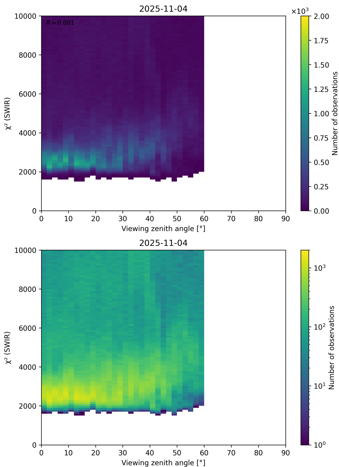
Figure 106: Scatter density plot of “Viewing zenith angle” against “ \chi^2 (SWIR)” for 2025-11-03 to 2025-11-05.
