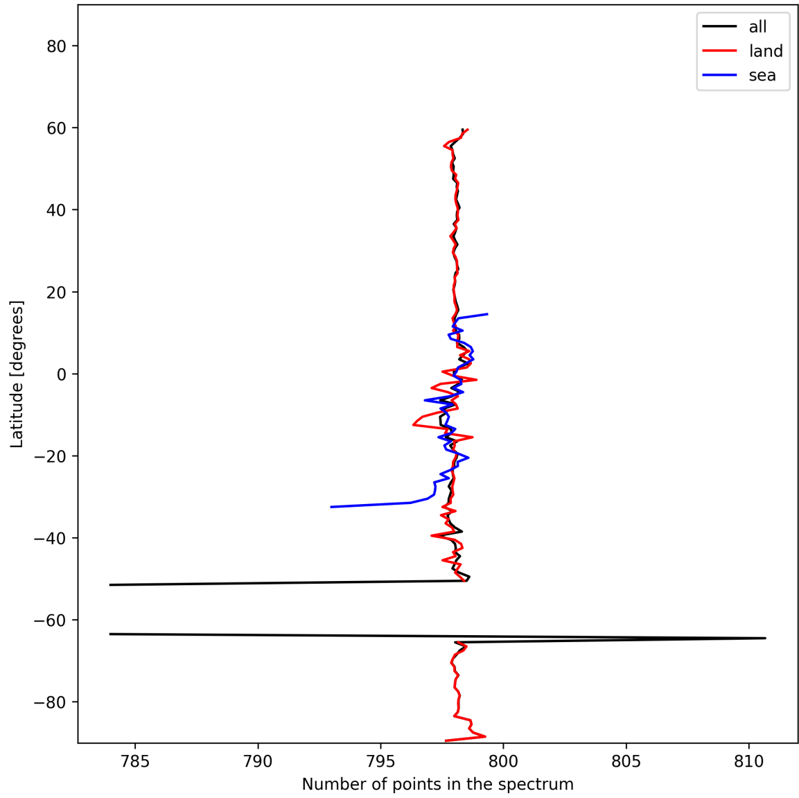
Figure 15: Zonal average of “Number of points in the spectrum” for 2025-11-03 to 2025-11-05.
