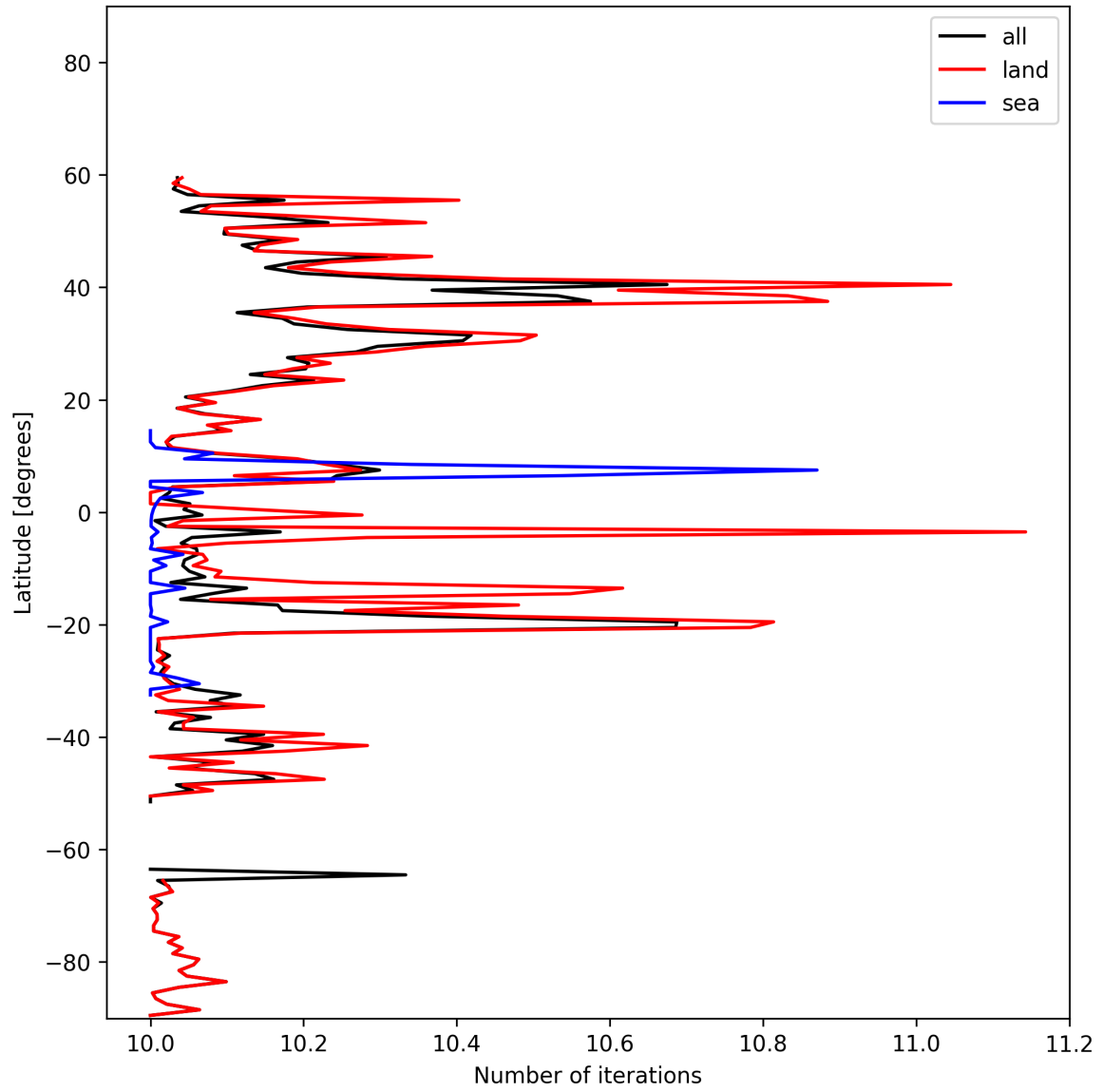
Figure 20: Zonal average of “Number of iterations” for 2025-11-03 to 2025-11-05.
