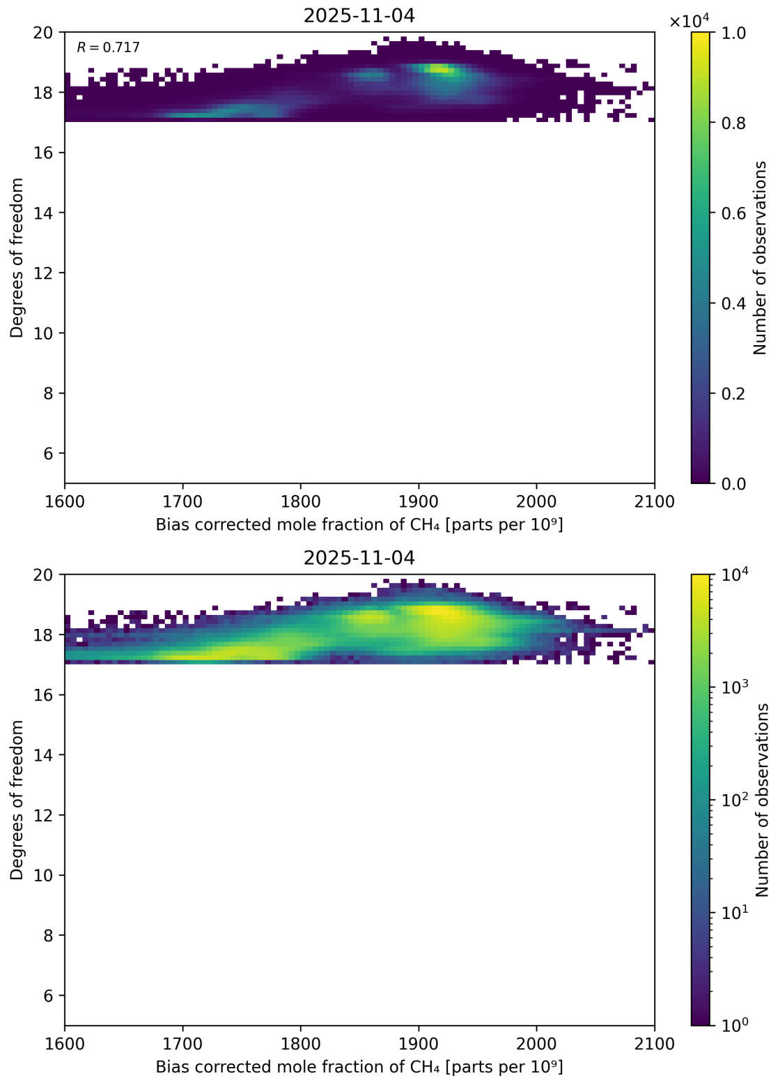
Figure 65: Scatter density plot of “Bias corrected mole fraction of CH 4 ” against “Degrees of freedom” for 2025-11-03 to 2025-11-05.
