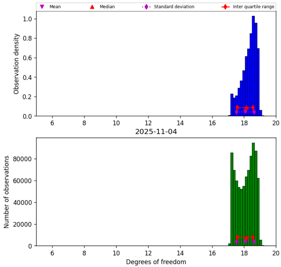
Figure 30: Histogram of “Degrees of freedom” for 2025-11-03 to 2025-11-05
