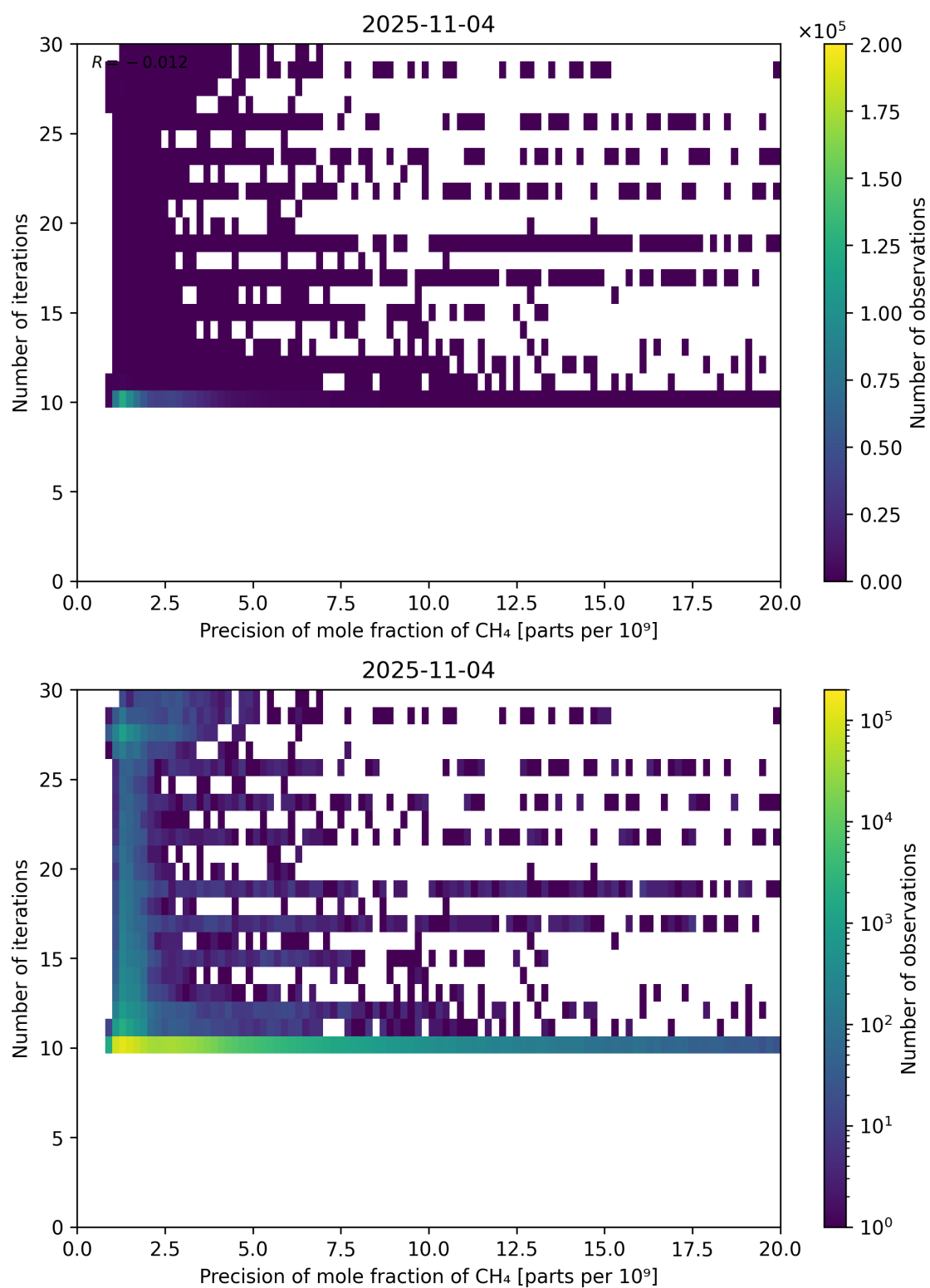
Figure 83: Scatter density plot of “Precision of mole fraction of CH 4 ” against “Number of iterations” for 2025-11-03 to 2025-11-05.
