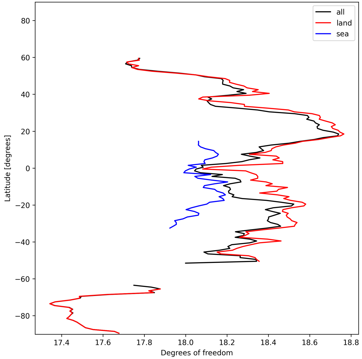
Figure 19: Zonal average of “Degrees of freedom” for 2025-11-03 to 2025-11-05.
