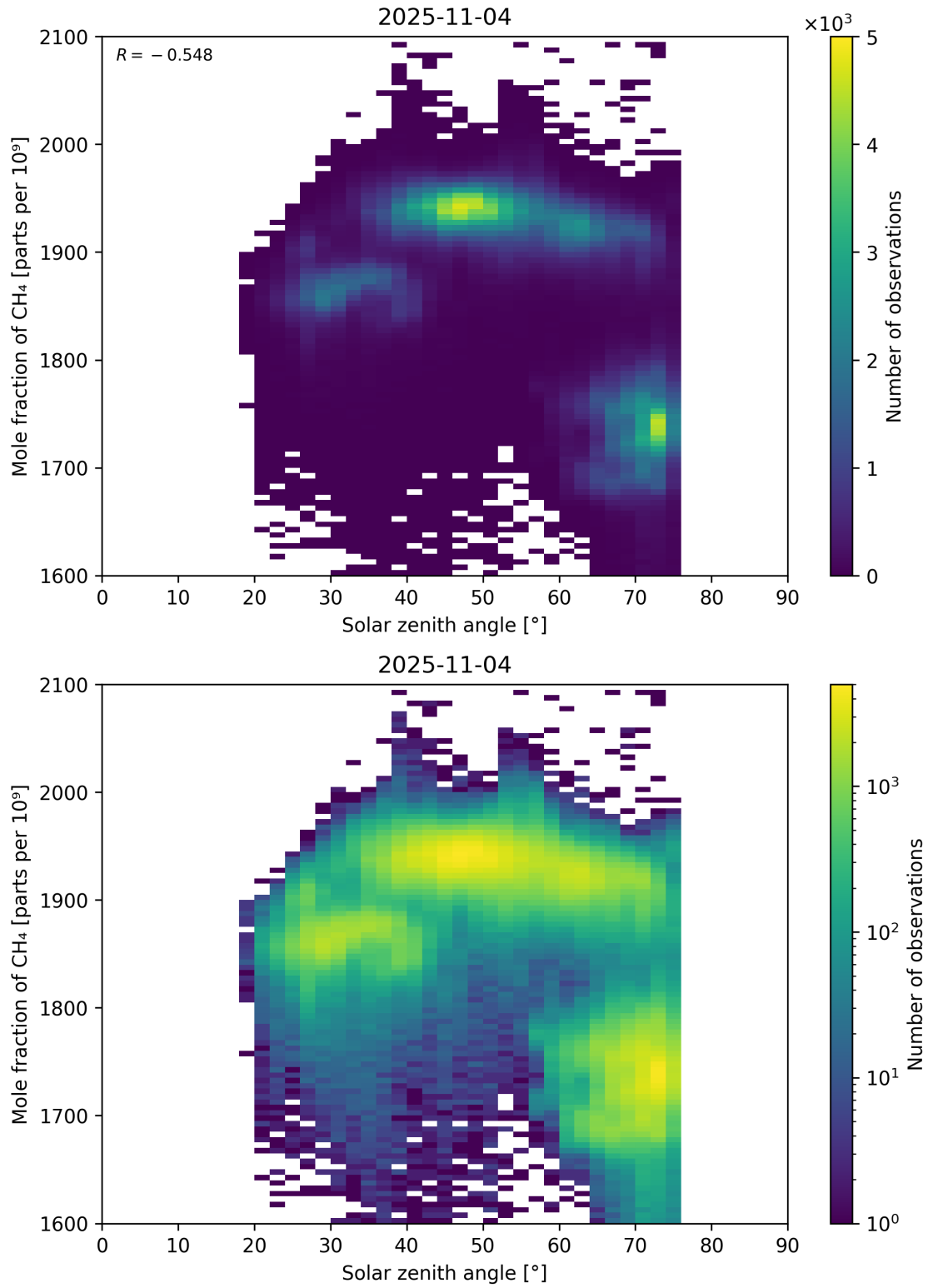
Figure 99: Scatter density plot of “Solar zenith angle” against “Mole fraction of CH 4 ” for 2025-11-03 to 2025-11-05.
