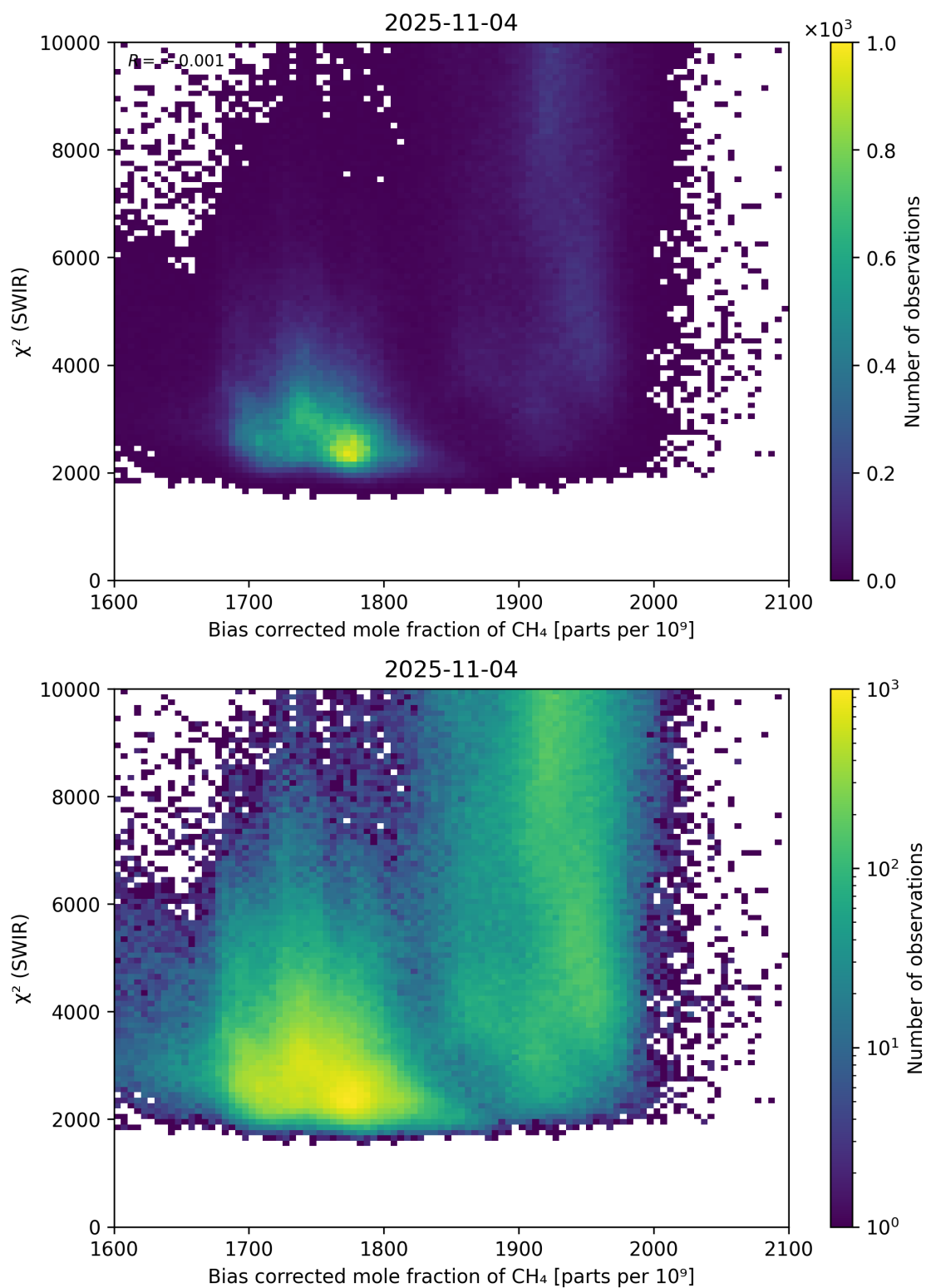
Figure 64: Scatter density plot of “Bias corrected mole fraction of \text{CH}_4 ” against “ \chi^2 (SWIR)” for 2025-11-03 to 2025-11-05.
