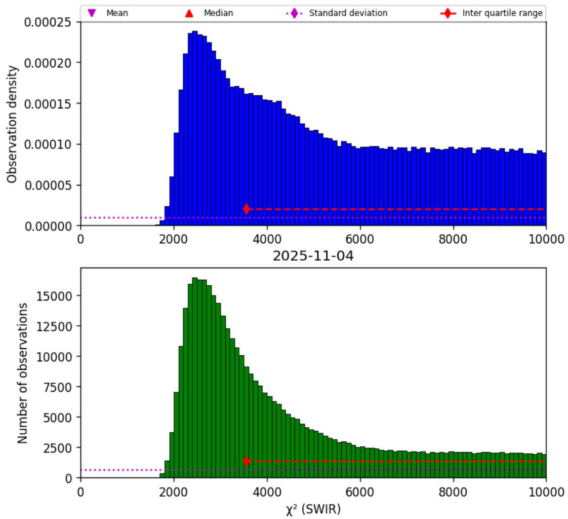
Figure 28: Histogram of “ \chi^2 (SWIR)” for 2025-11-03 to 2025-11-05
