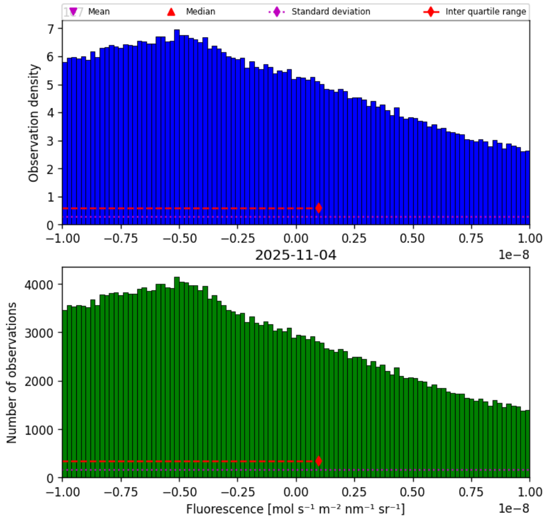
Figure 32: Histogram of “Fluorescence” for 2025-11-03 to 2025-11-05
