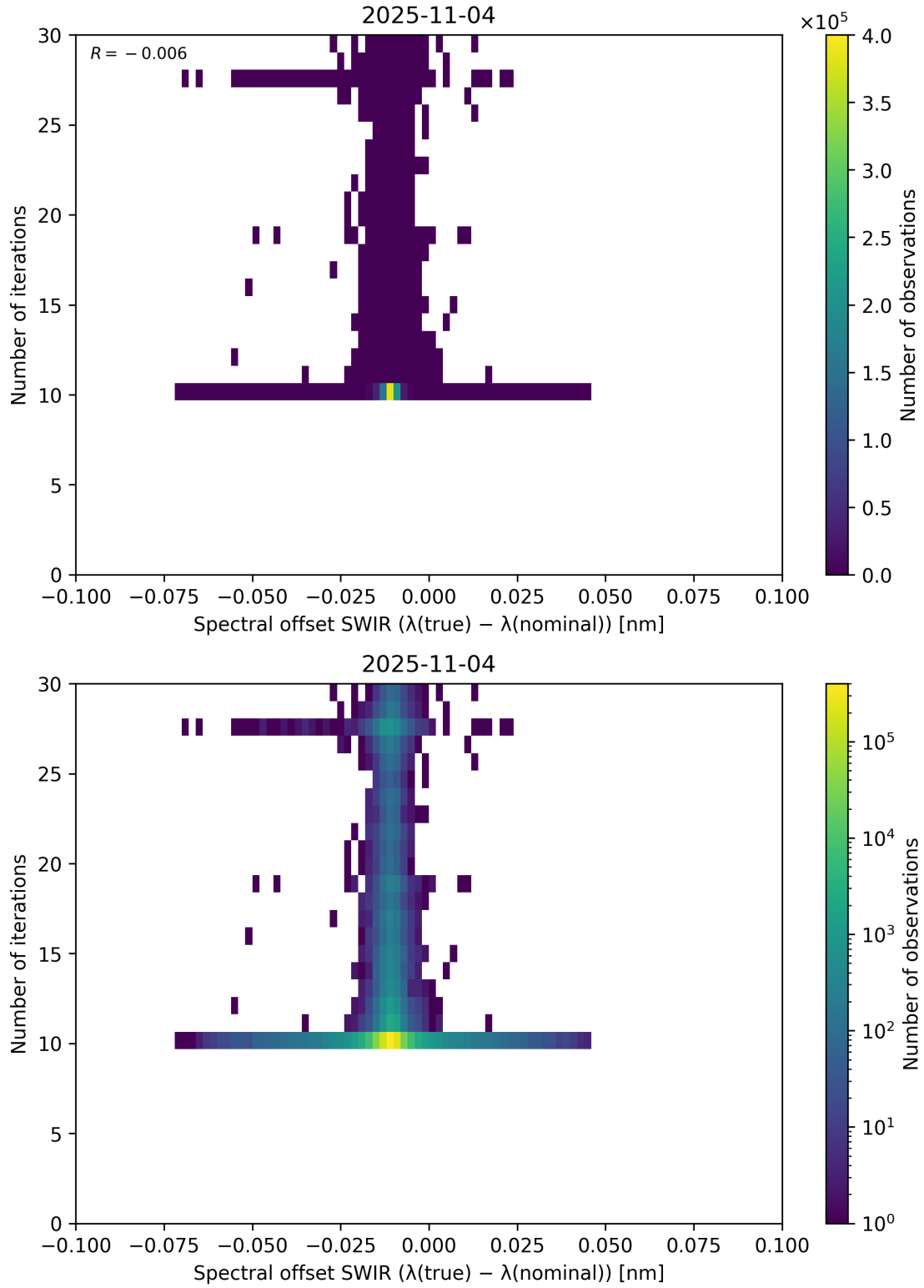
Figure 121: Scatter density plot of “Spectral offset SWIR ( \lambda_{\text{true}} - \lambda_{\text{nominal}} )” against “Number of iterations” for 2025-11-03 to 2025-11-05.
