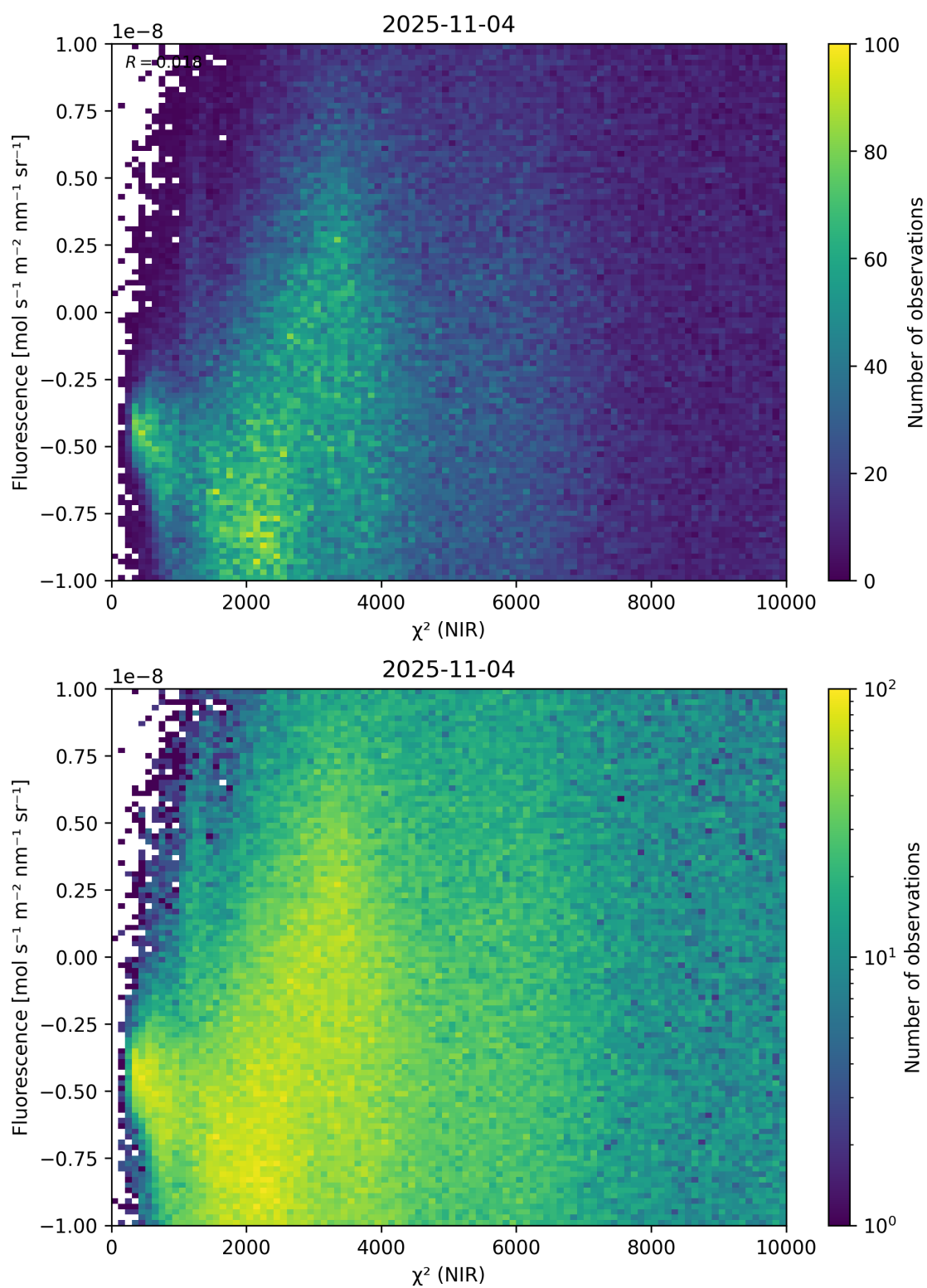
Figure 45: Scatter density plot of “ \chi^2 (NIR)” against “Fluorescence” for 2025-11-03 to 2025-11-05.
