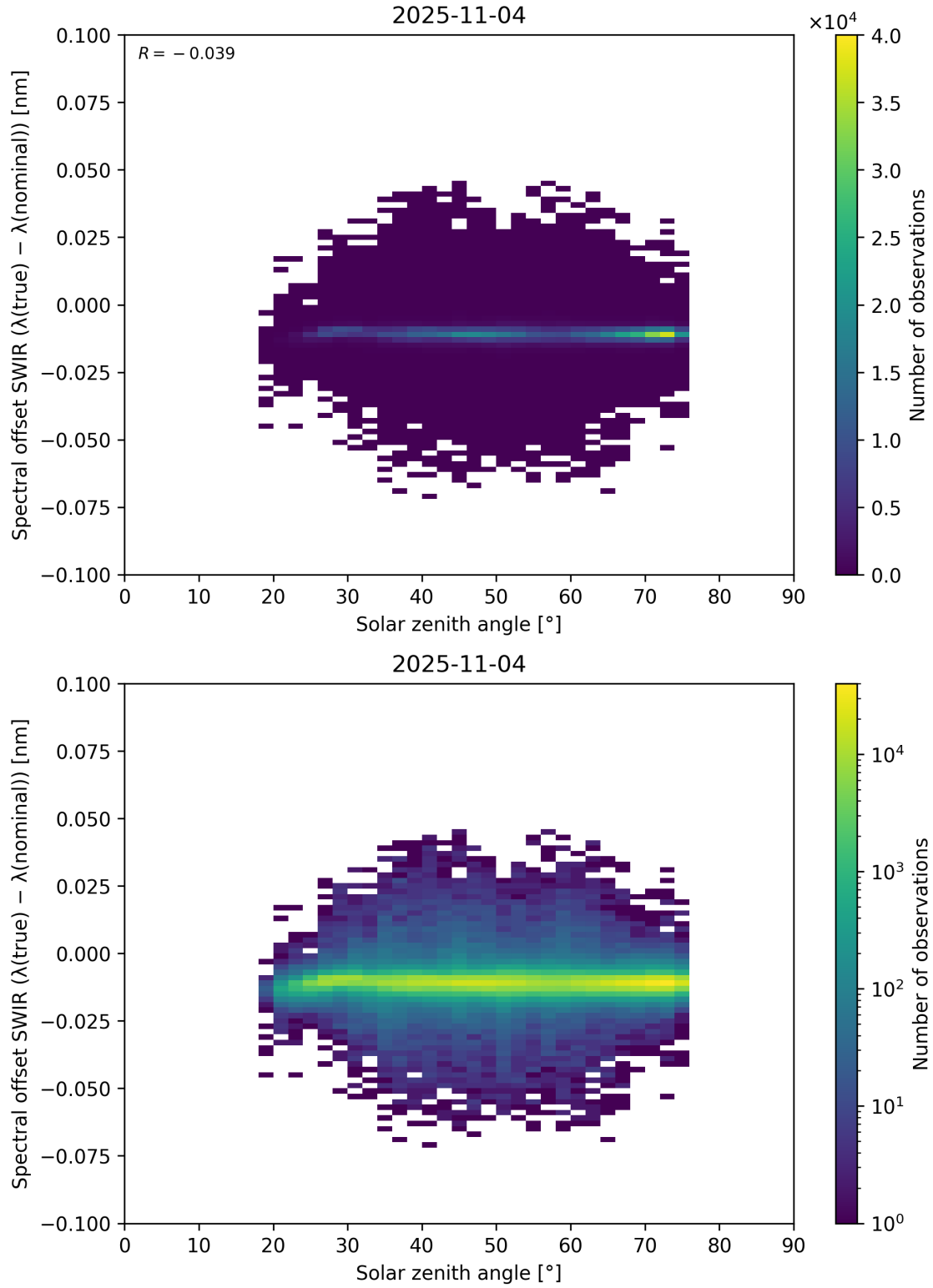
Figure 104: Scatter density plot of “Solar zenith angle” against “Spectral offset SWIR ( \lambda_{\text{true}} - \lambda_{\text{nominal}} )” for 2025-11-03 to 2025-11-05.
