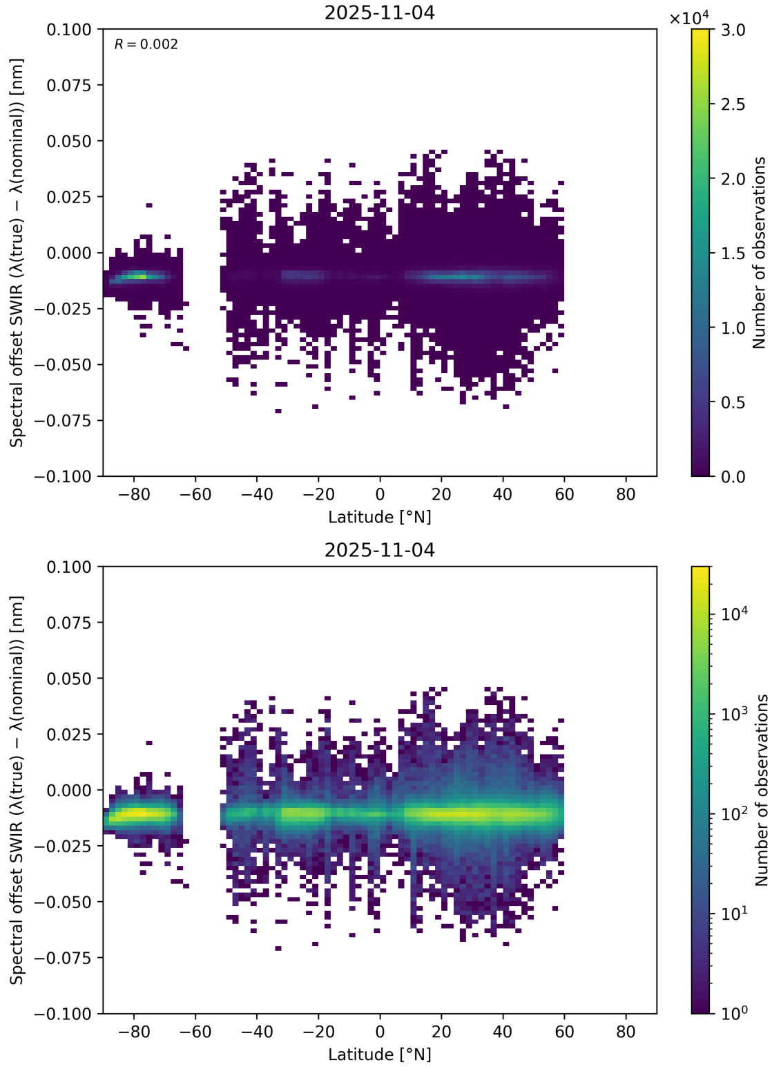
Figure 62: Scatter density plot of “Latitude” against “Spectral offset SWIR ( \lambda_{\text{true}} - \lambda_{\text{nominal}} )” for 2025-11-03 to 2025-11-05.
