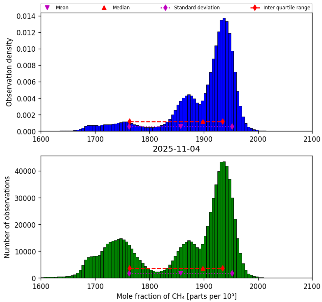
Figure 23: Histogram of “Mole fraction of CH 4 ” for 2025-11-03 to 2025-11-05
