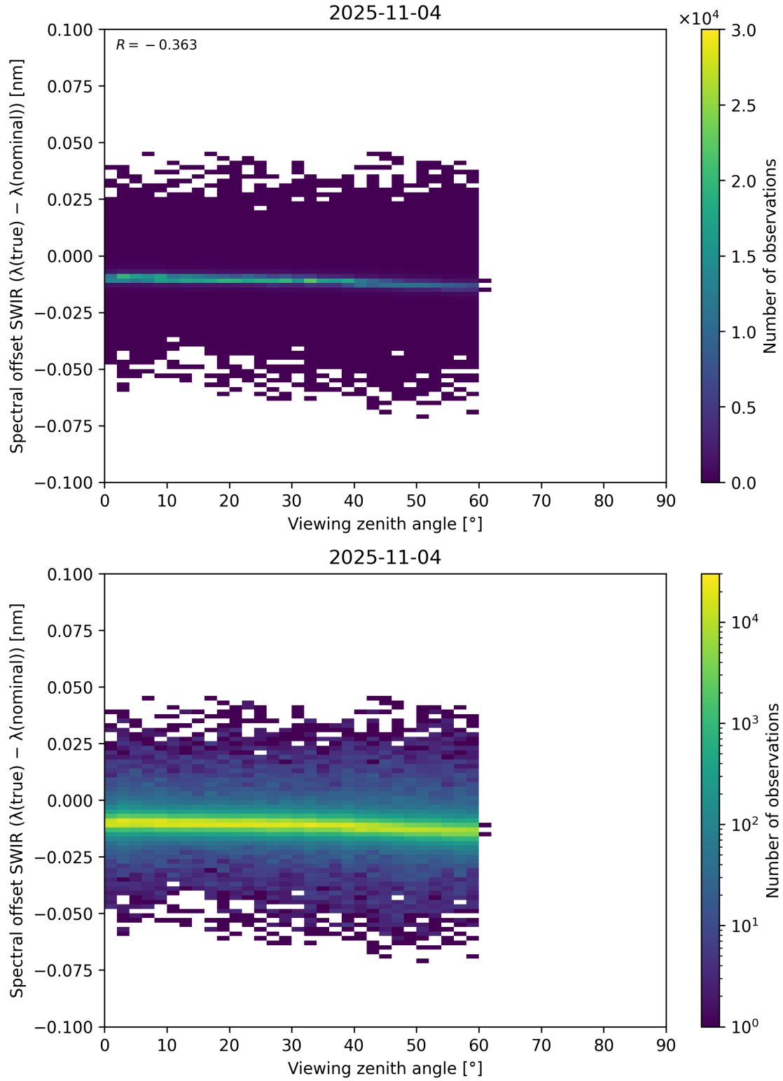
Figure 116: Scatter density plot of “Viewing zenith angle” against “Spectral offset SWIR ( \lambda_{\text{true}} - \lambda_{\text{nominal}} )” for 2025-11-03 to 2025-11-05.
