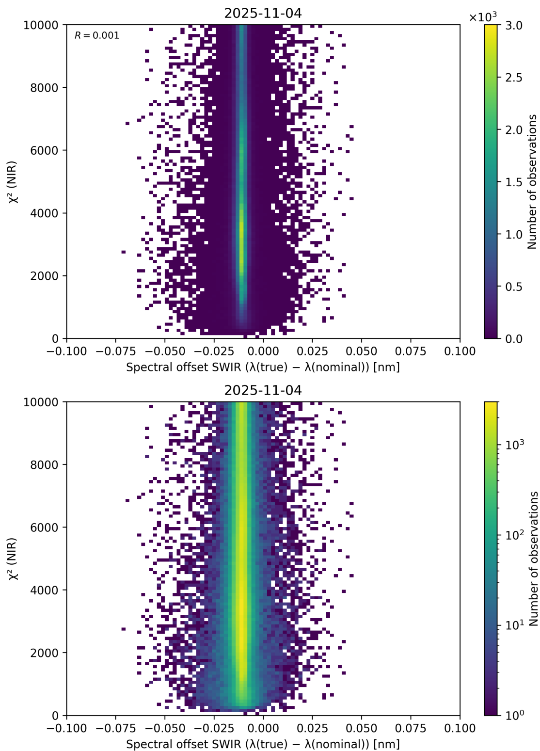
Figure 117: Scatter density plot of “Spectral offset SWIR ( \lambda_{\text{true}} - \lambda_{\text{nominal}} )” against “ \chi^2 (NIR)” for 2025-11-03 to 2025-11-05.
