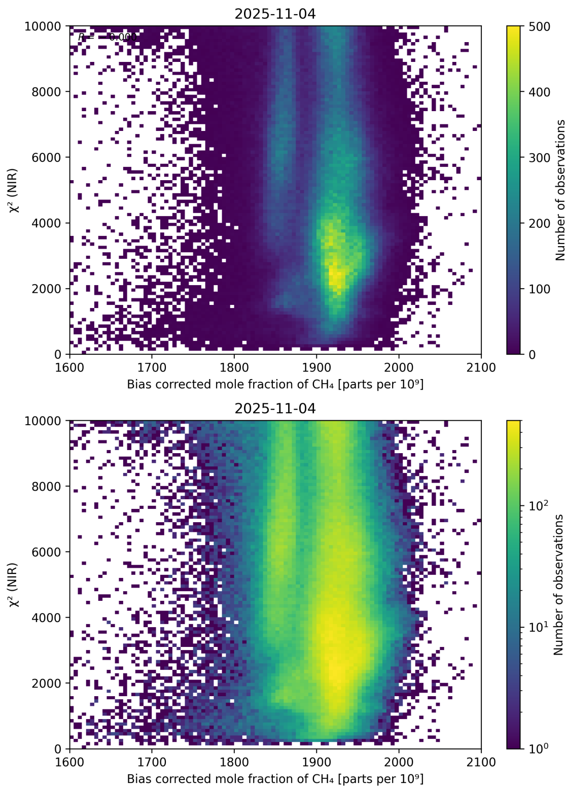
Figure 63: Scatter density plot of “Bias corrected mole fraction of \text{CH}_4 ” against “ \chi^2 (NIR)” for 2025-11-03 to 2025-11-05.
