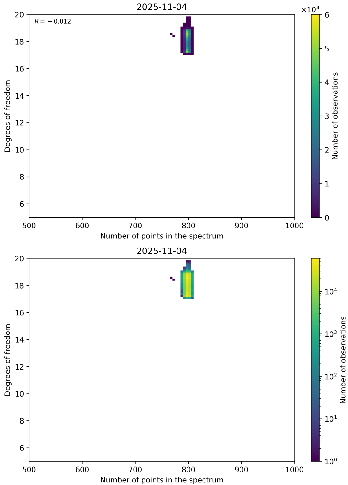
Figure 90: Scatter density plot of “Number of points in the spectrum” against “Degrees of freedom” for 2025-11-03 to 2025-11-05.
