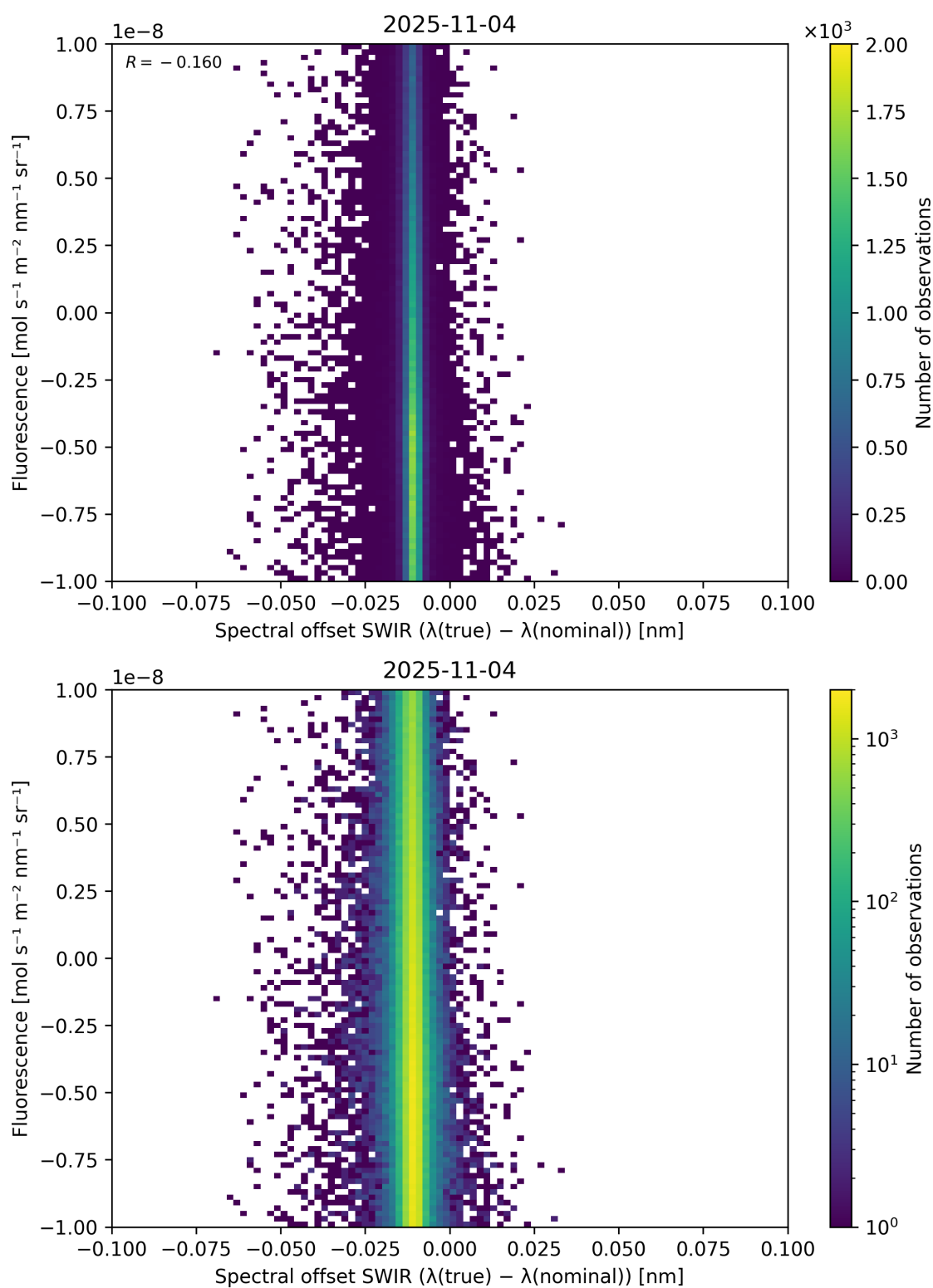
Figure 120: Scatter density plot of “Spectral offset SWIR ( \lambda_{\text{true}} - \lambda_{\text{nominal}} )” against “Fluorescence” for 2025-11-03 to 2025-11-05.
