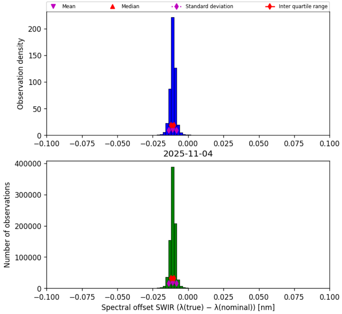
Figure 27: Histogram of “Spectral offset SWIR ( \lambda_{\text{true}} - \lambda_{\text{nominal}} )” for 2025-11-03 to 2025-11-05
