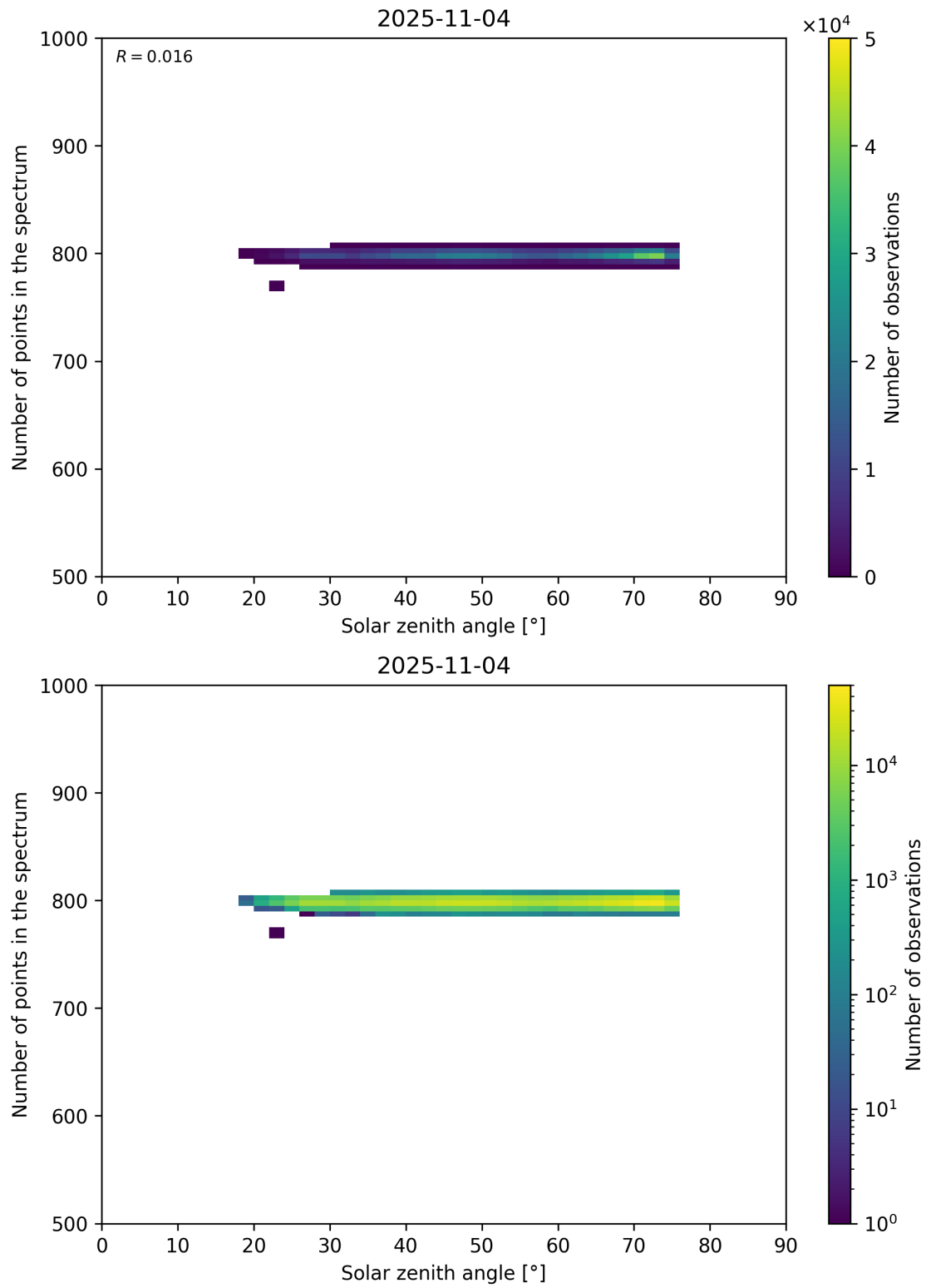
Figure 103: Scatter density plot of “Solar zenith angle” against “Number of points in the spectrum” for 2025-11-03 to 2025-11-05.
