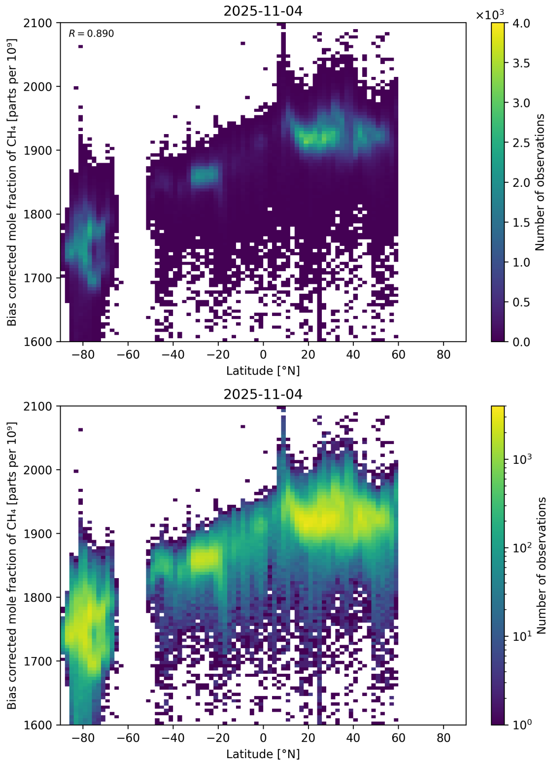
Figure 58: Scatter density plot of “Latitude” against “Bias corrected mole fraction of \text{CH}_4 ” for 2025-11-03 to 2025-11-05.
