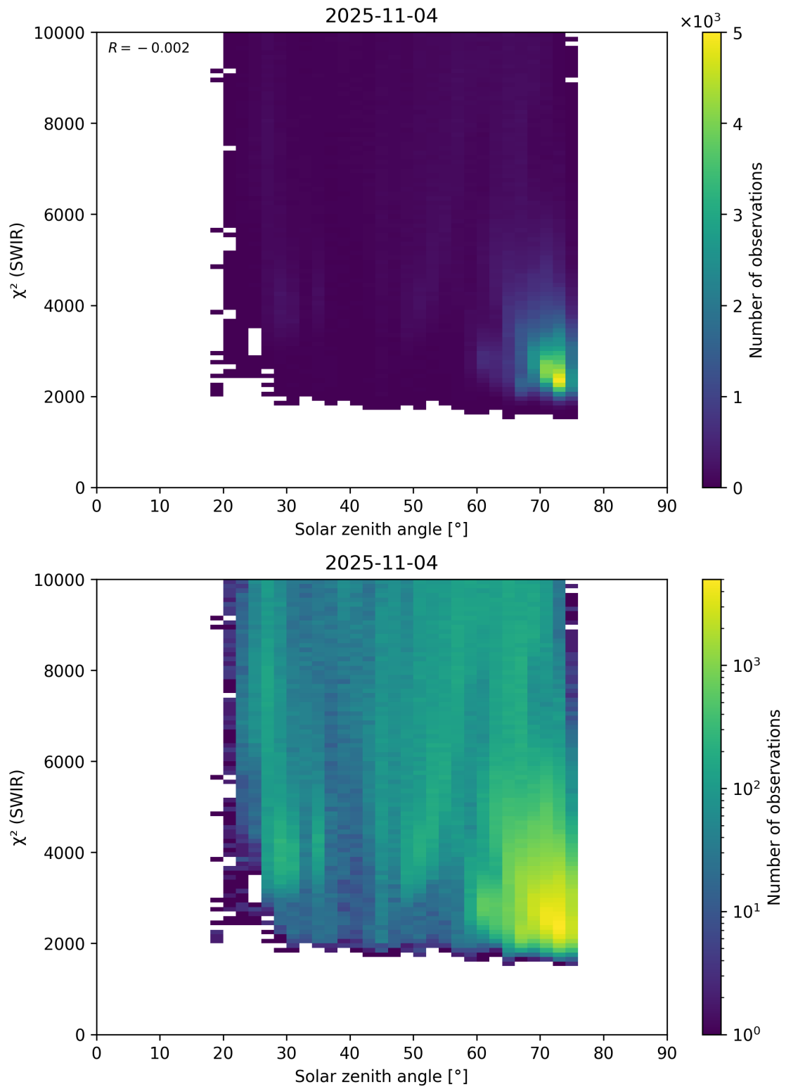
Figure 95: Scatter density plot of “Solar zenith angle” against “ \chi^2 (SWIR)” for 2025-11-03 to 2025-11-05.
