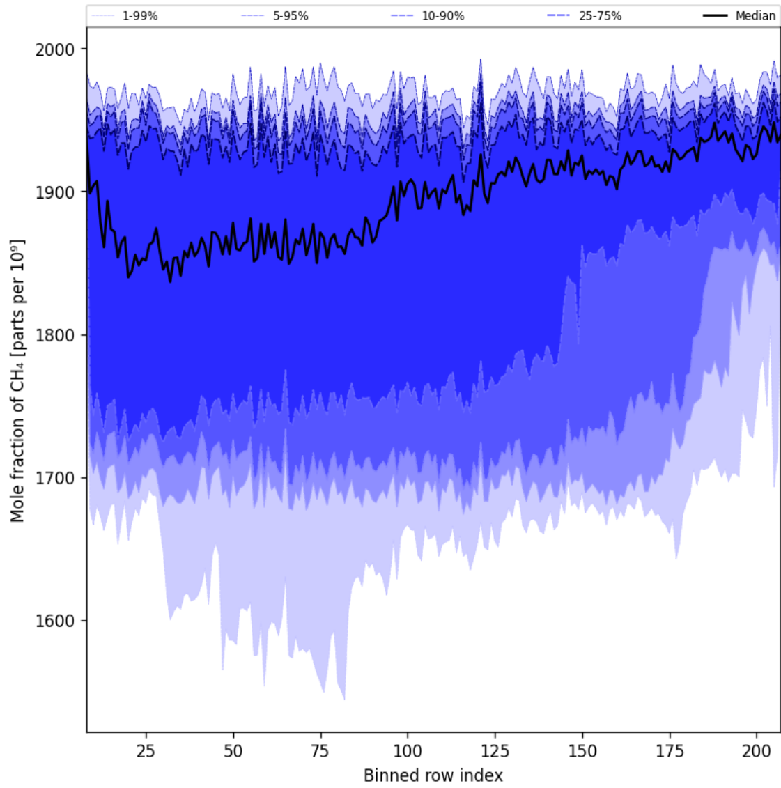
Figure 34: Along track statistics of “Mole fraction of CH 4 ” for 2025-11-03 to 2025-11-05
