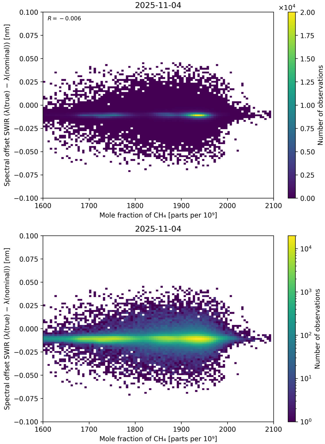
Figure 86: Scatter density plot of “Mole fraction of \text{CH}_4 ” against “Spectral offset SWIR ( \lambda_{\text{true}} - \lambda_{\text{nominal}} )” for 2025-11-03 to 2025-11-05.
