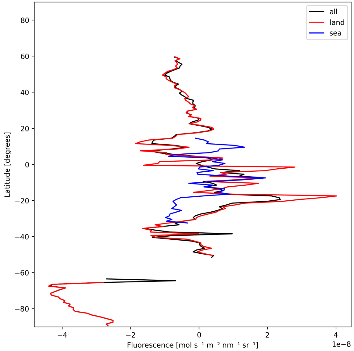
Figure 21: Zonal average of “Fluorescence” for 2025-11-03 to 2025-11-05.
