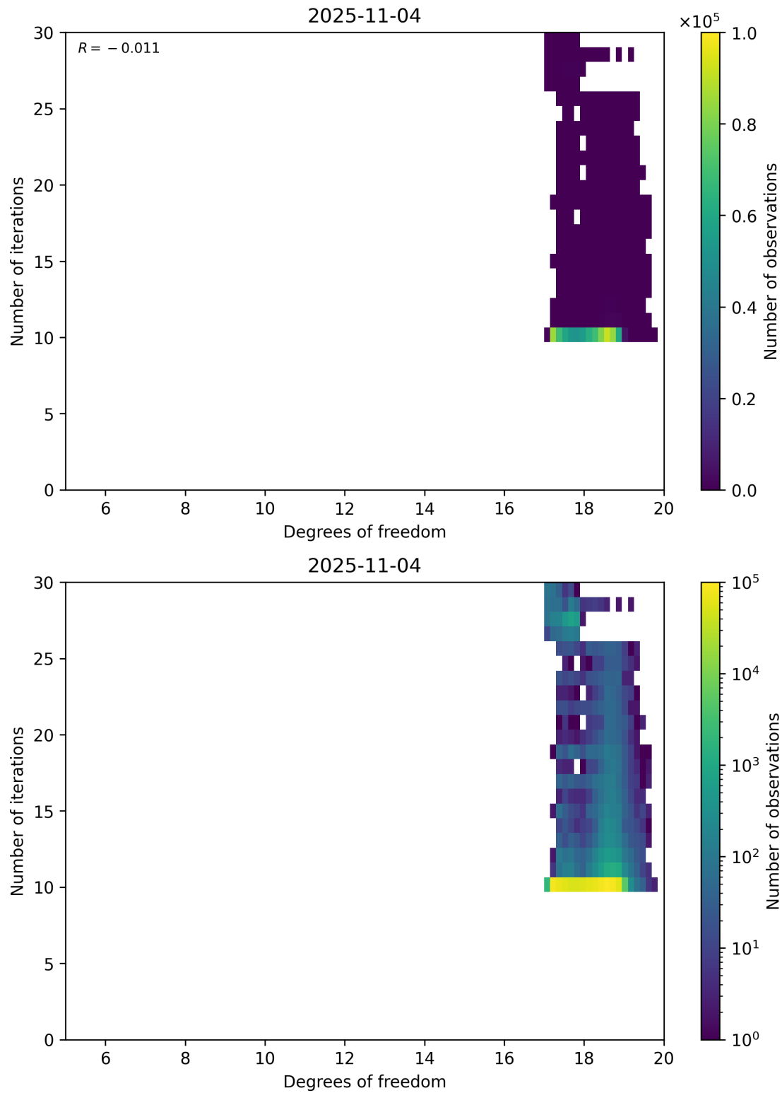
Figure 52: Scatter density plot of “Degrees of freedom” against “Number of iterations” for 2025-11-03 to 2025-11-05.
