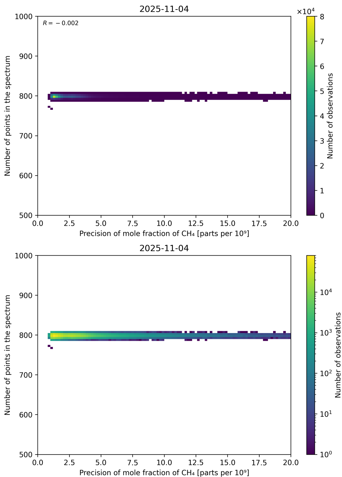
Figure 84: Scatter density plot of “Precision of mole fraction of CH 4 ” against “Number of points in the spectrum” for 2025-11-03 to 2025-11-05.
