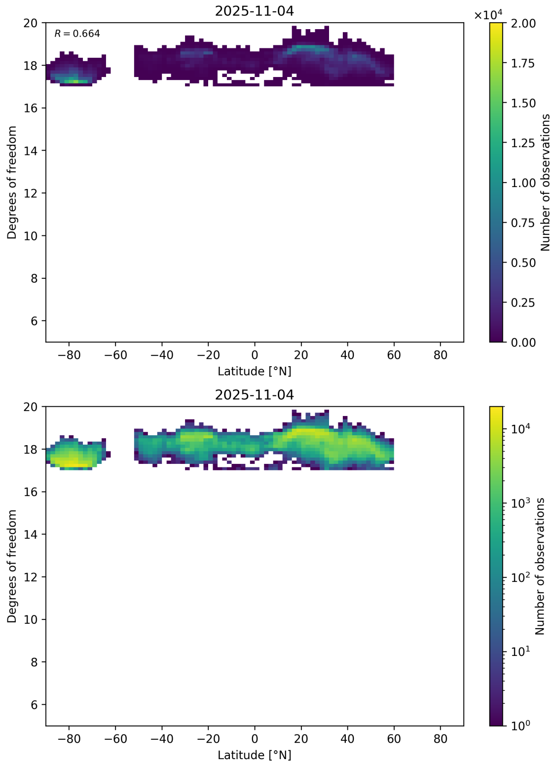
Figure 55: Scatter density plot of “Latitude” against “Degrees of freedom” for 2025-11-03 to 2025-11-05.
