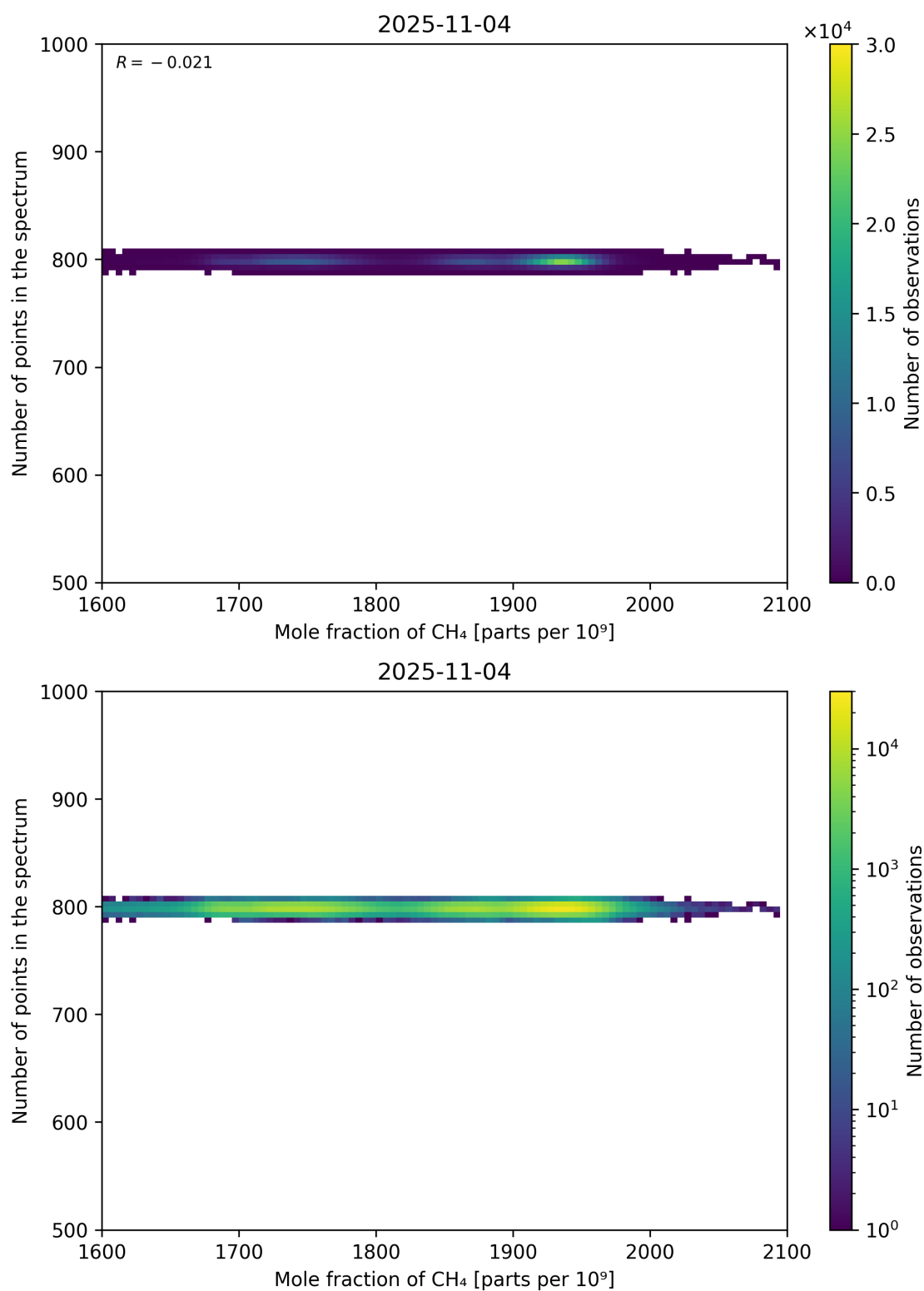
Figure 77: Scatter density plot of “Mole fraction of CH 4 ” against “Number of points in the spectrum” for 2025-11-03 to 2025-11-05.
