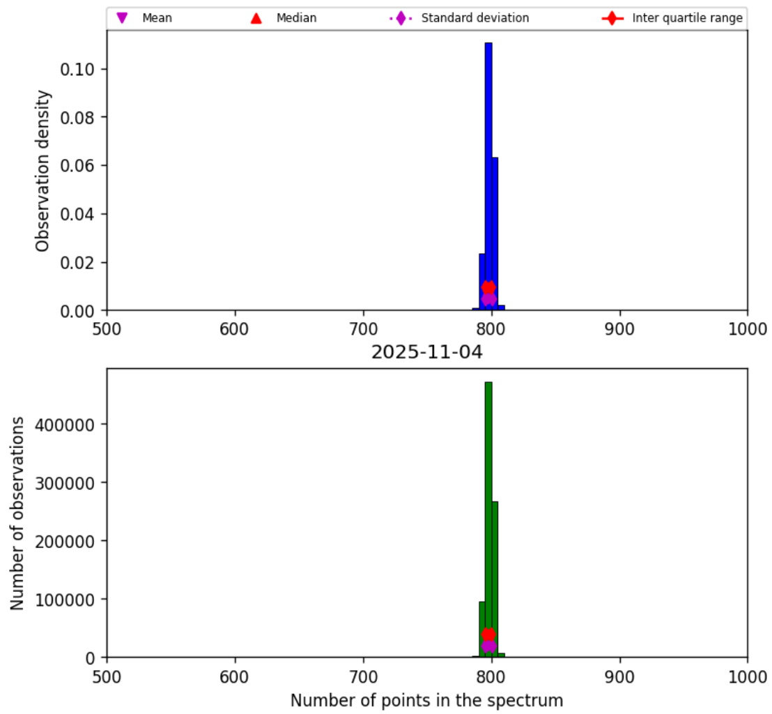
Figure 26: Histogram of “Number of points in the spectrum” for 2025-11-03 to 2025-11-05
