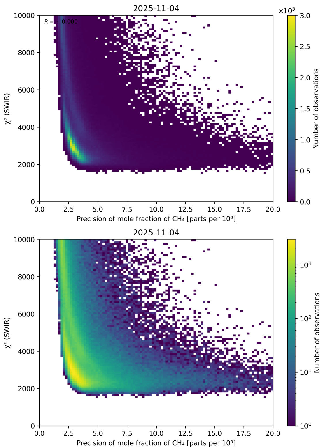
Figure 79: Scatter density plot of “Precision of mole fraction of \text{CH}_4 ” against “ \chi^2 (SWIR)” for 2025-11-03 to 2025-11-05.
