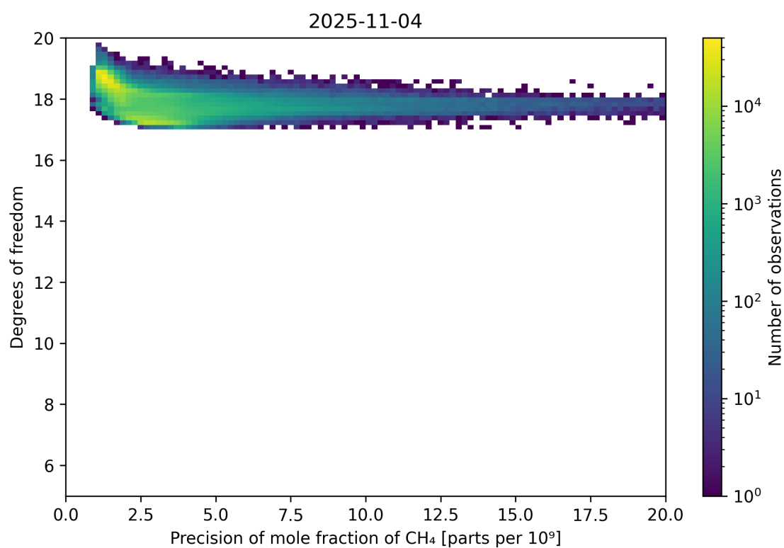
Figure 80: Scatter density plot of “Precision of mole fraction of CH 4 ” against “Degrees of freedom” for 2025-11-03 to 2025-11-05.
