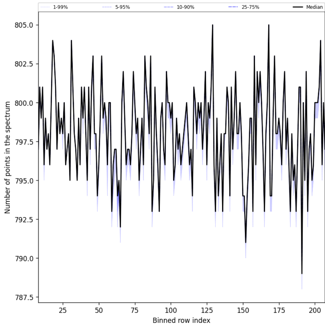
Figure 37: Along track statistics of “Number of points in the spectrum” for 2025-11-03 to 2025-11-05
