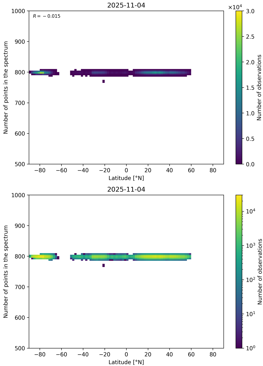
Figure 61: Scatter density plot of “Latitude” against “Number of points in the spectrum” for 2025-11-03 to 2025-11-05.
