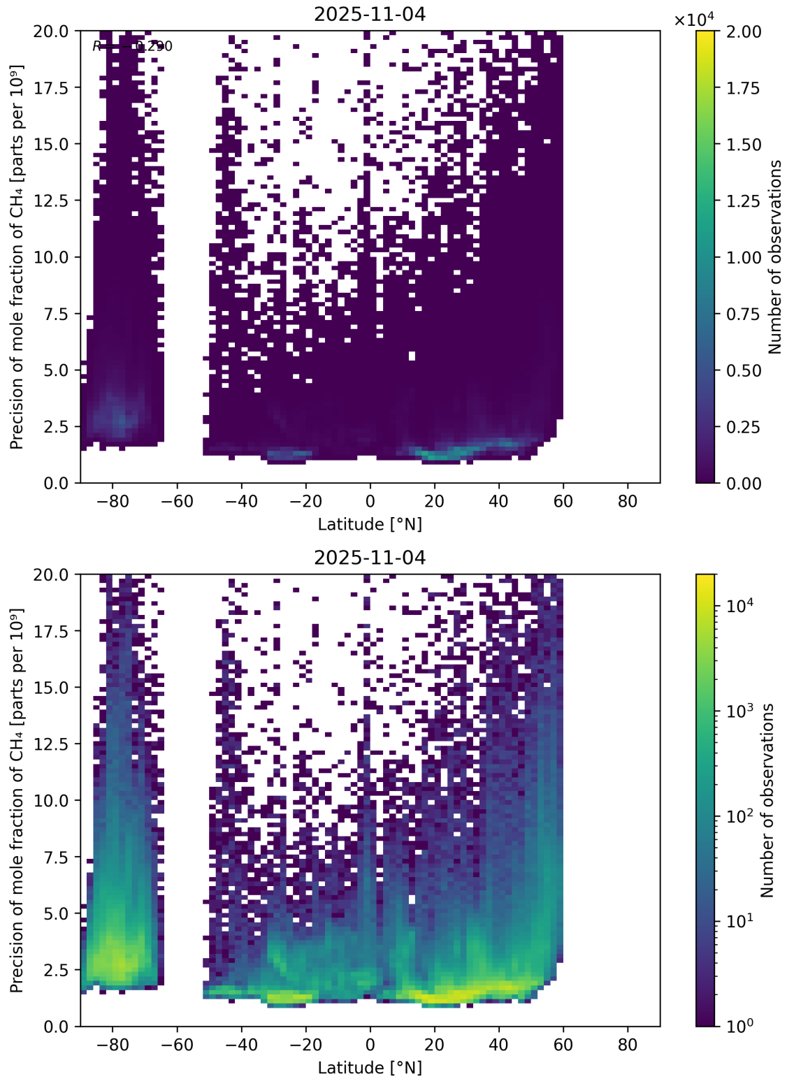
Figure 59: Scatter density plot of “Latitude” against “Precision of mole fraction of CH 4 ” for 2025-11-03 to 2025-11-05.
