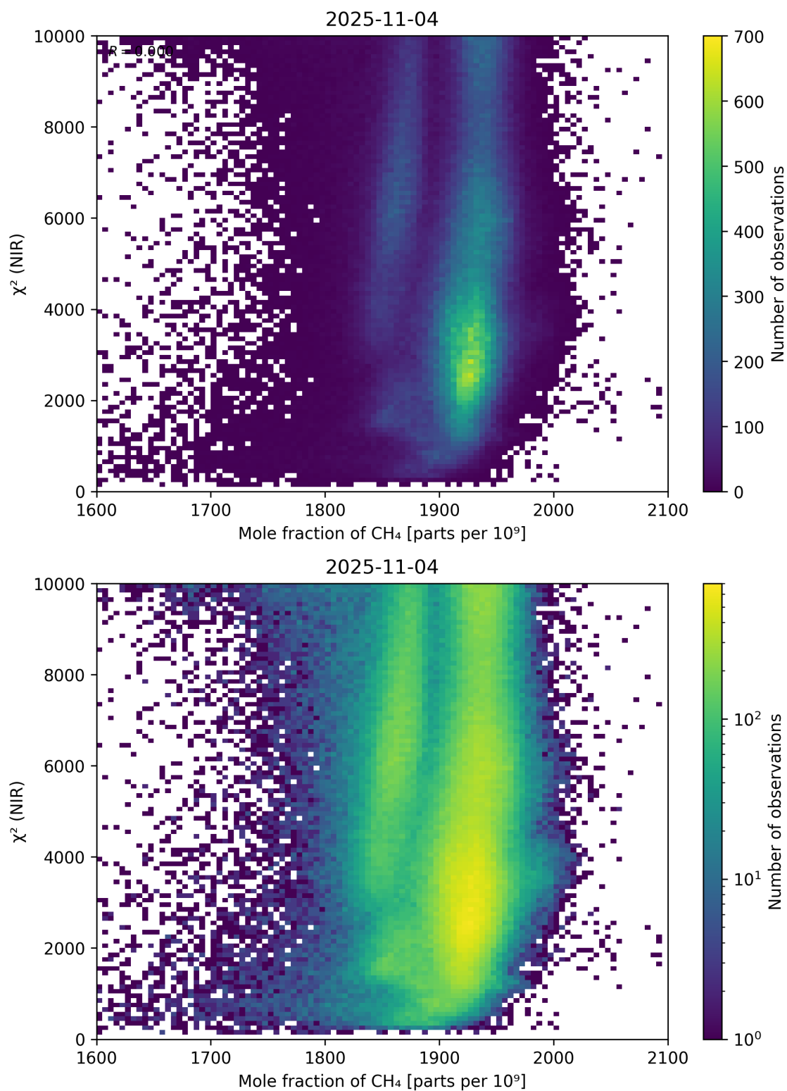
Figure 70: Scatter density plot of “Mole fraction of \text{CH}_4 ” against “ \chi^2 (NIR)” for 2025-11-03 to 2025-11-05.
