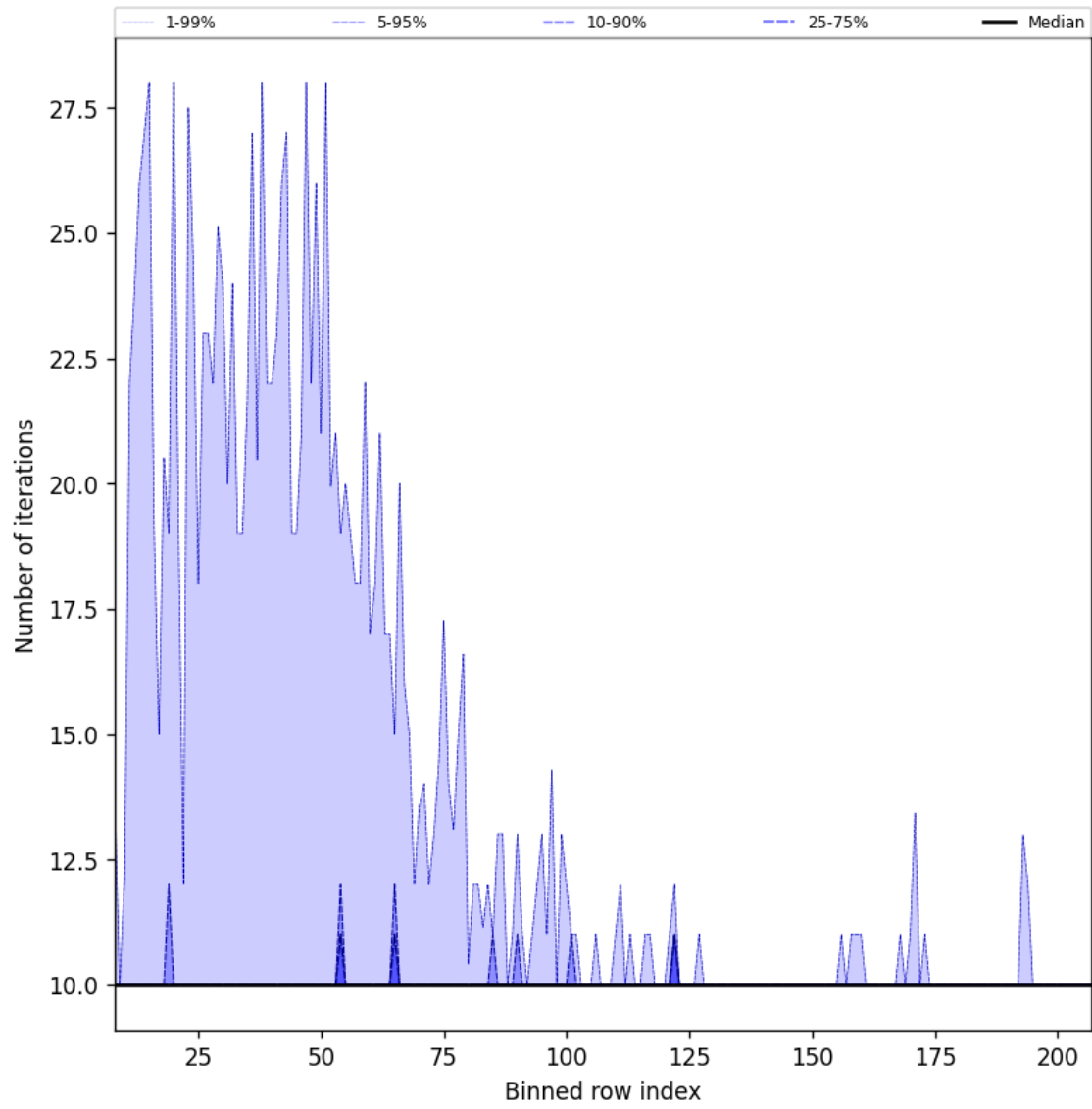
Figure 42: Along track statistics of “Number of iterations” for 2025-11-03 to 2025-11-05
