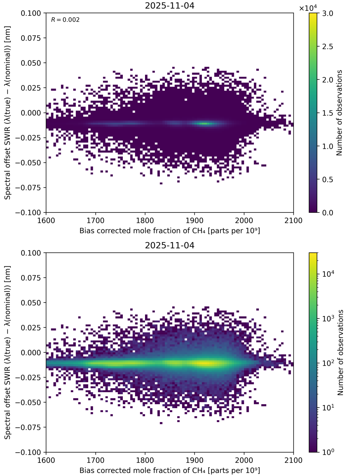
Figure 69: Scatter density plot of “Bias corrected mole fraction of \text{CH}_4 ” against “Spectral offset SWIR ( \lambda_{\text{true}} - \lambda_{\text{nominal}} )” for 2025-11-03 to 2025-11-05.
