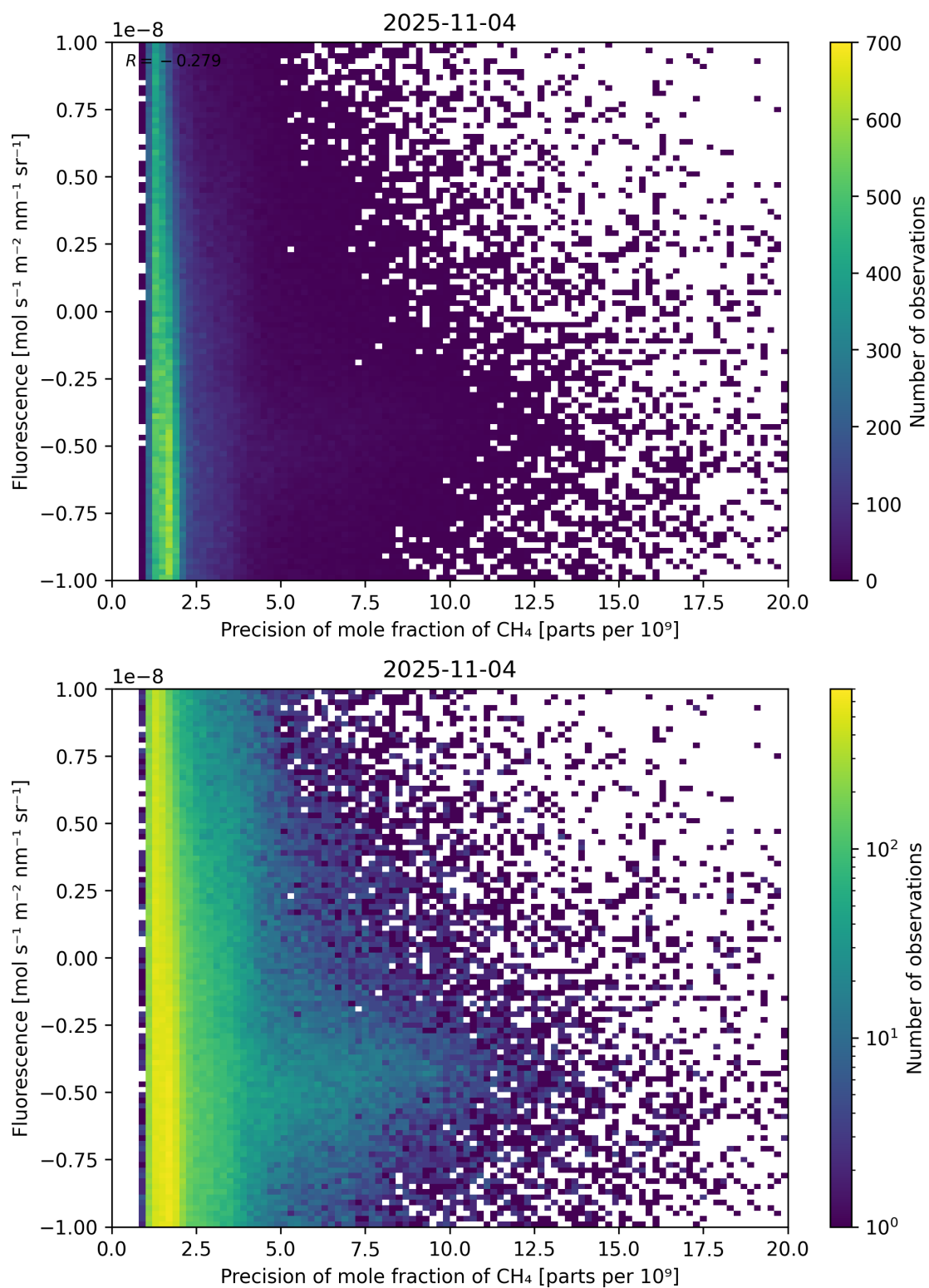
Figure 81: Scatter density plot of “Precision of mole fraction of \text{CH}_4 ” against “Fluorescence” for 2025-11-03 to 2025-11-05.
