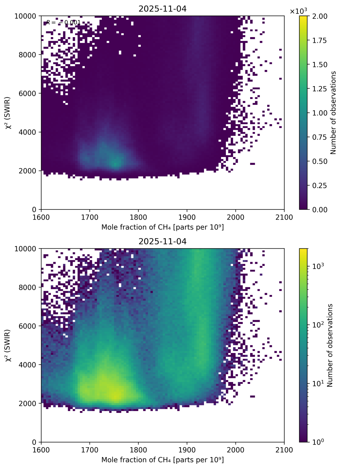
Figure 71: Scatter density plot of “Mole fraction of CH 4 ” against “ \chi^2 (SWIR)” for 2025-11-03 to 2025-11-05.
