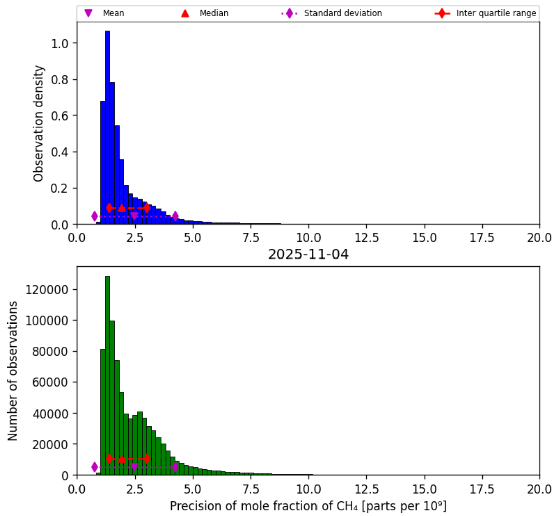
Figure 24: Histogram of “Precision of mole fraction of CH 4 ” for 2025-11-03 to 2025-11-05
