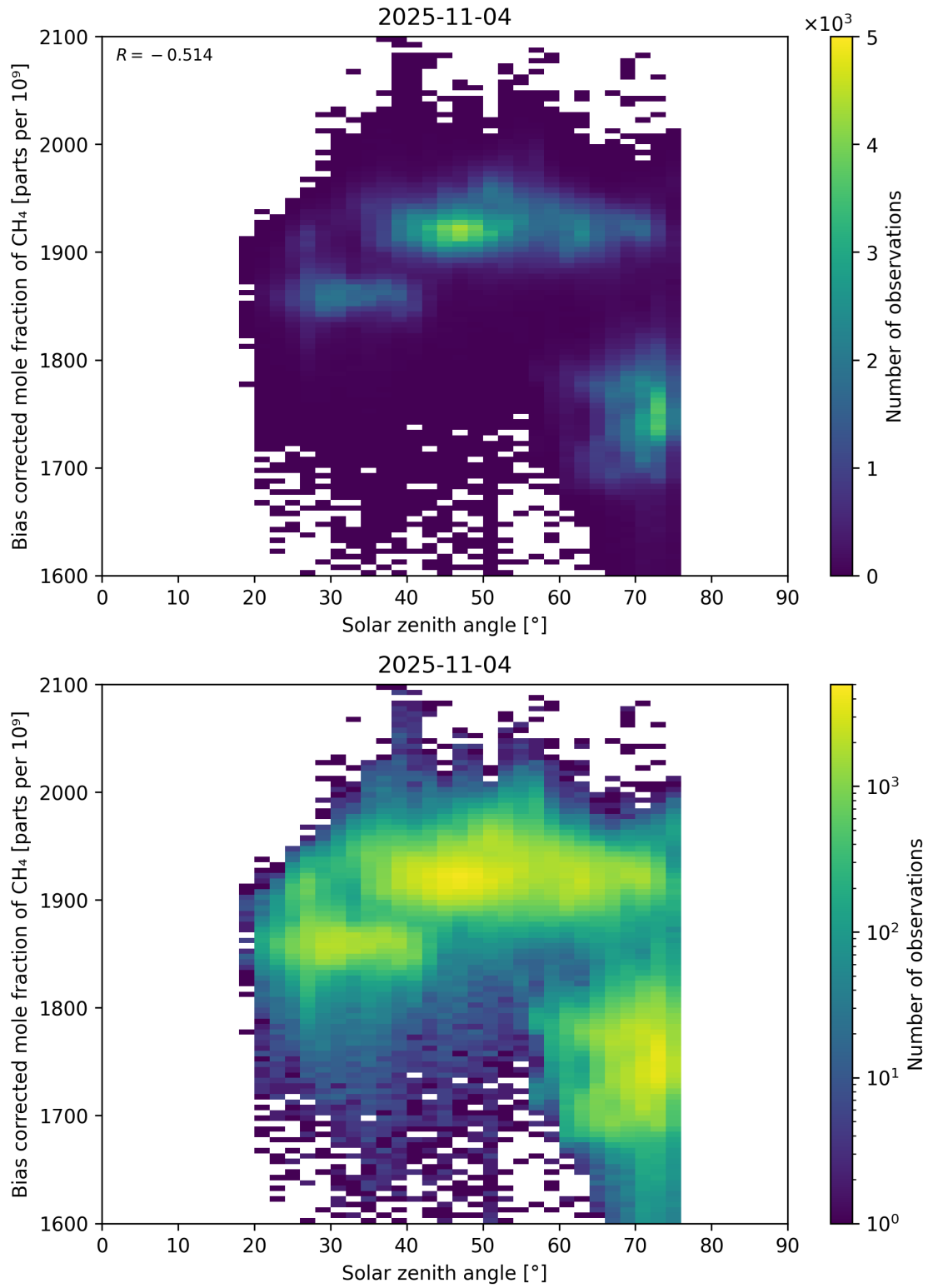
Figure 100: Scatter density plot of “Solar zenith angle” against “Bias corrected mole fraction of \text{CH}_4 ” for 2025-11-03 to 2025-11-05.
