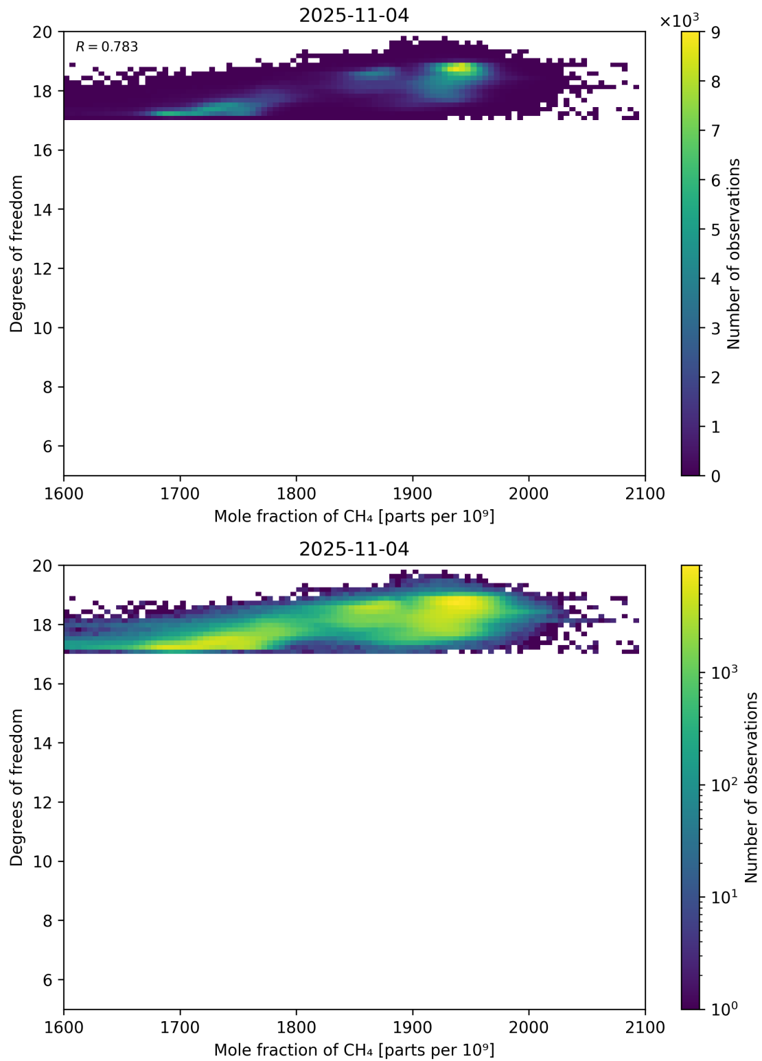
Figure 72: Scatter density plot of “Mole fraction of CH 4 ” against “Degrees of freedom” for 2025-11-03 to 2025-11-05.
