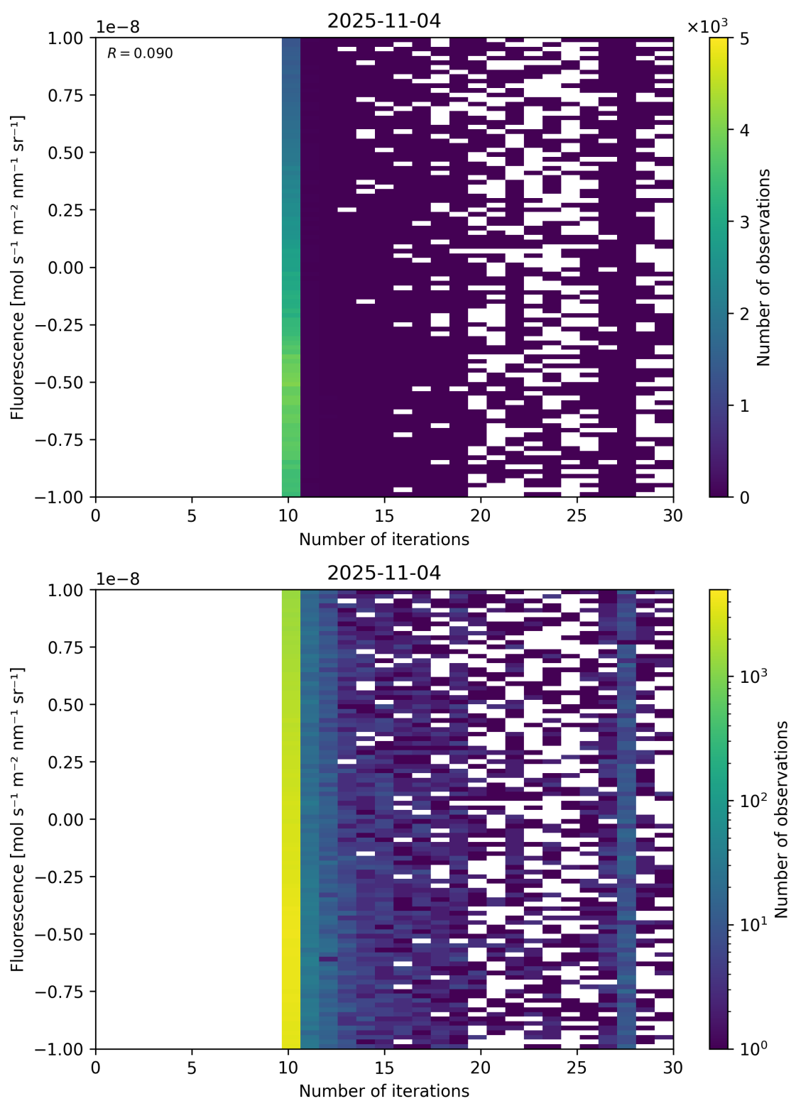
Figure 87: Scatter density plot of “Number of iterations” against “Fluorescence” for 2025-11-03 to 2025-11-05.
