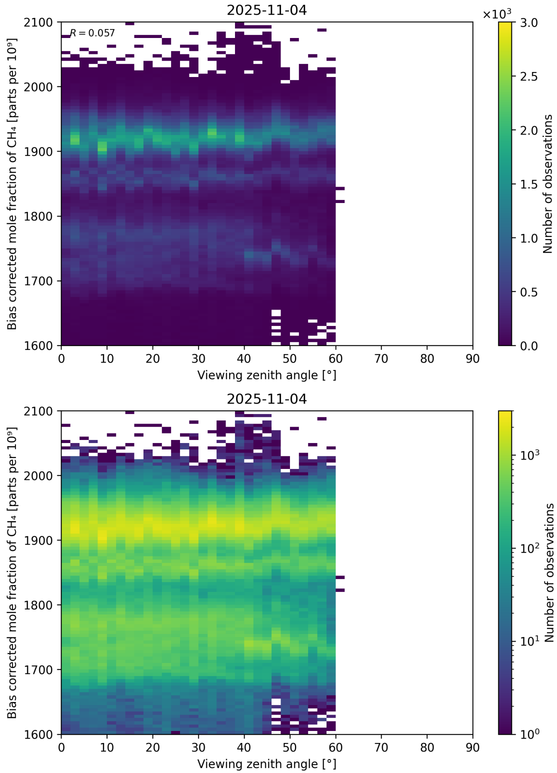
Figure 111: Scatter density plot of “Viewing zenith angle” against “Bias corrected mole fraction of CH 4 ” for 2025-11-03 to 2025-11-05.
