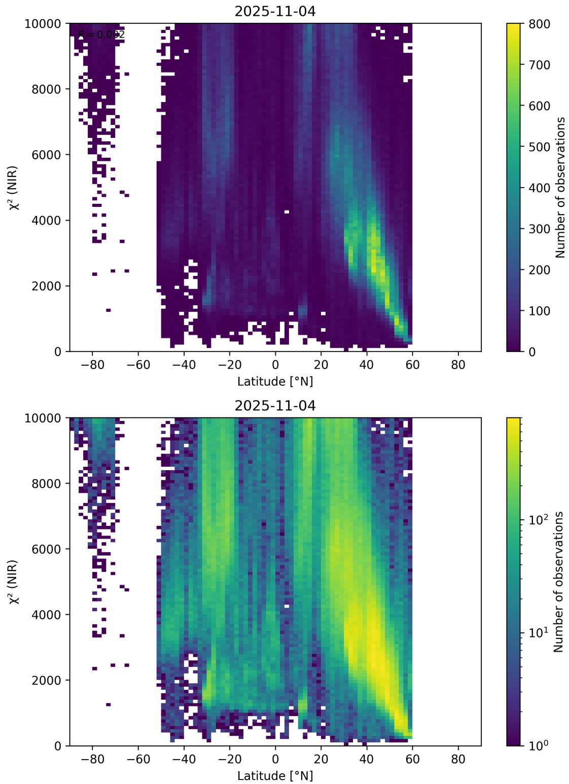
Figure 53: Scatter density plot of “Latitude” against “ \chi^2 (NIR)” for 2025-11-03 to 2025-11-05.
