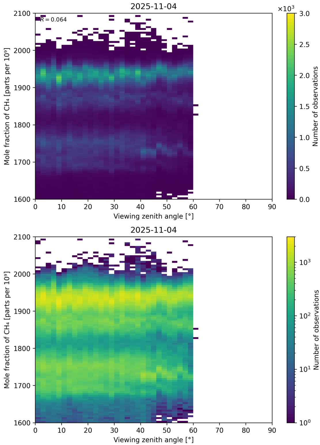
Figure 110: Scatter density plot of “Viewing zenith angle” against “Mole fraction of CH 4 ” for 2025-11-03 to 2025-11-05.
