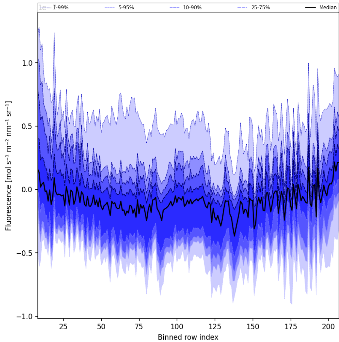
Figure 43: Along track statistics of “Fluorescence” for 2025-11-03 to 2025-11-05
