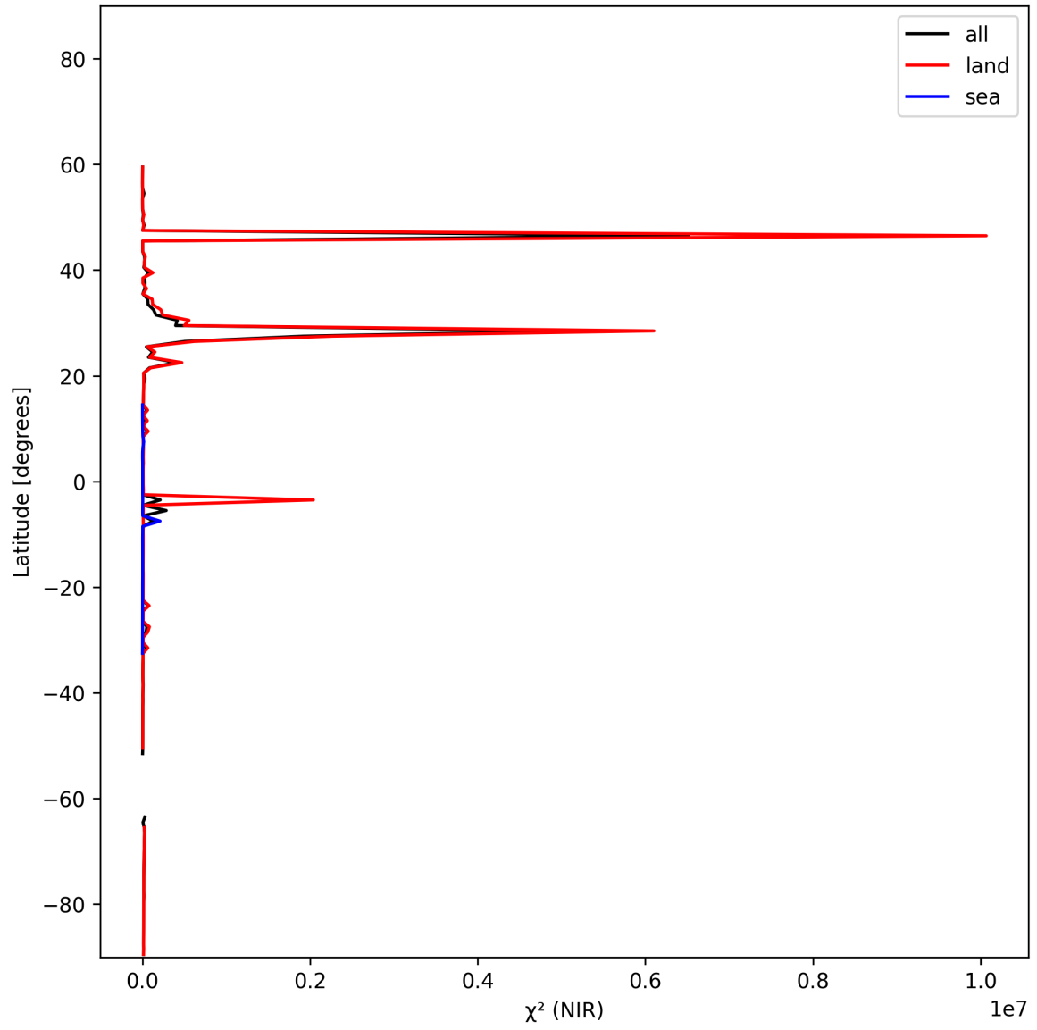
Figure 18: Zonal average of “ \chi^2 (NIR)” for 2025-11-03 to 2025-11-05.
