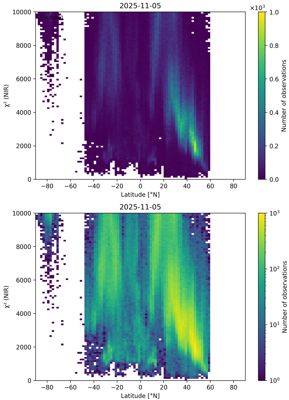
Figure 53: Scatter density plot of “Latitude” against “ \chi^2 (NIR)” for 2025-11-04 to 2025-11-06.
