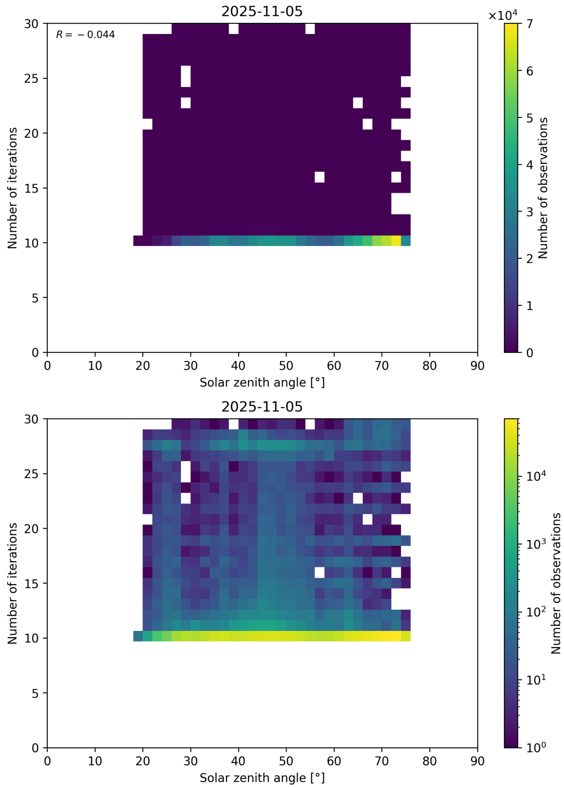
Figure 102: Scatter density plot of “Solar zenith angle” against “Number of iterations” for 2025-11-04 to 2025-11-06.
