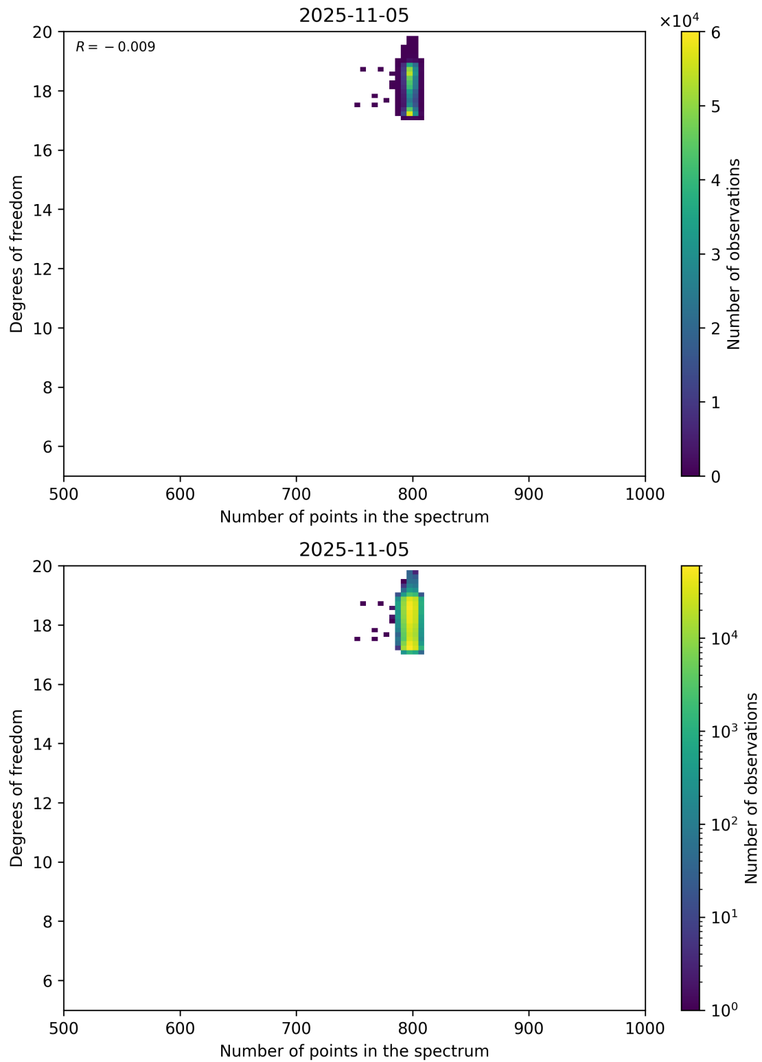
Figure 90: Scatter density plot of “Number of points in the spectrum” against “Degrees of freedom” for 2025-11-04 to 2025-11-06.
