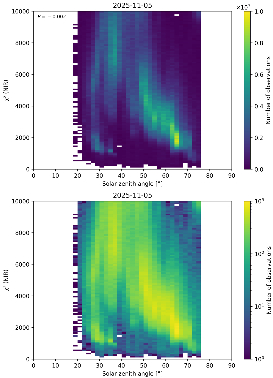
Figure 94: Scatter density plot of “Solar zenith angle” against “ \chi^2 (NIR)” for 2025-11-04 to 2025-11-06.
