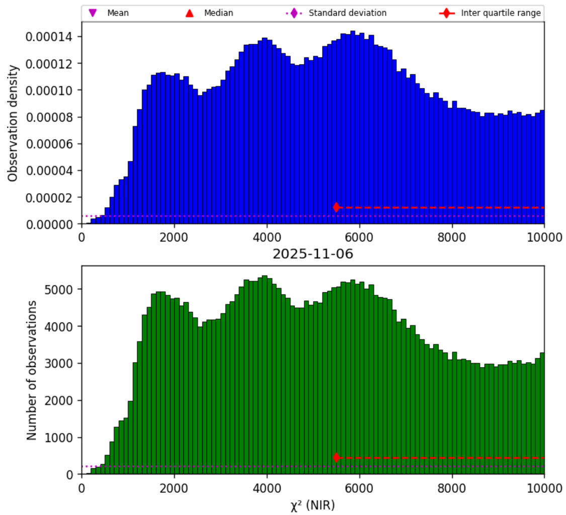
Figure 29: Histogram of “ \chi^2 (NIR)” for 2025-11-05 to 2025-11-07
