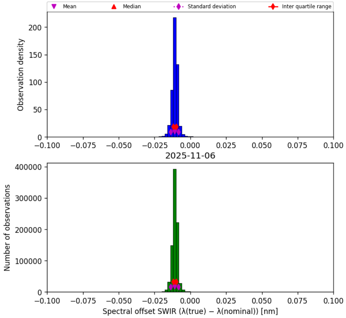
Figure 27: Histogram of “Spectral offset SWIR ( \lambda_{\text{true}} - \lambda_{\text{nominal}} )” for 2025-11-05 to 2025-11-07
