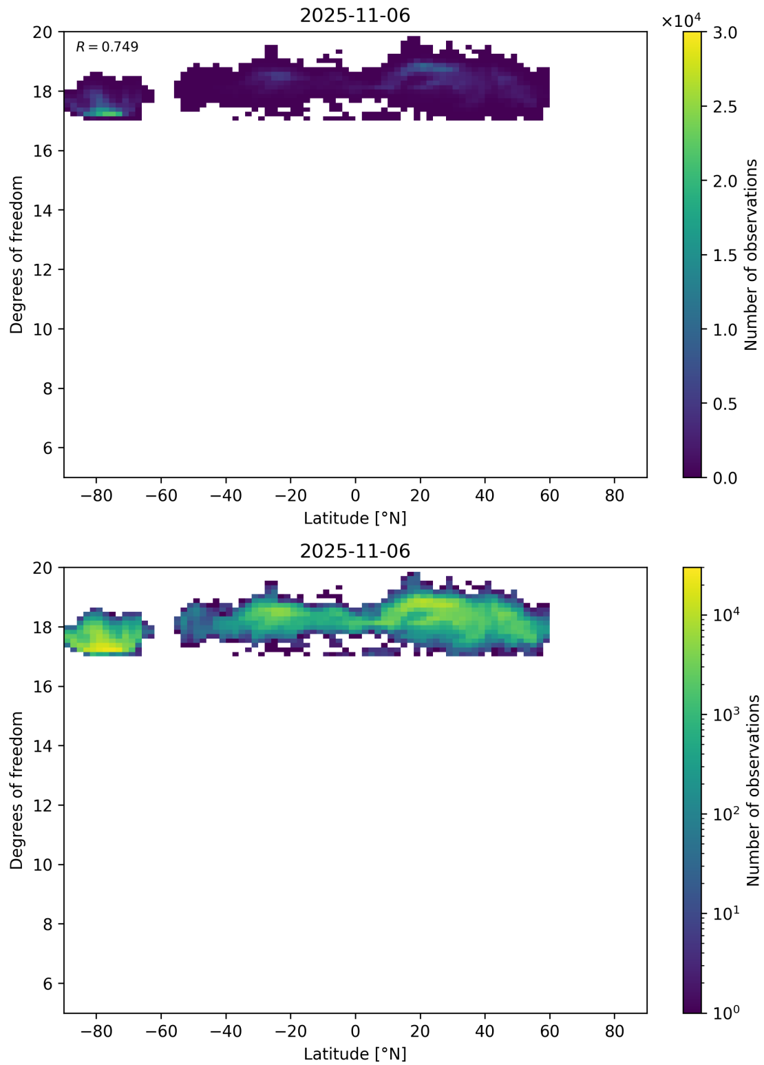
Figure 55: Scatter density plot of “Latitude” against “Degrees of freedom” for 2025-11-05 to 2025-11-07.
