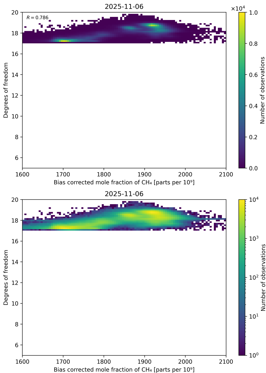
Figure 65: Scatter density plot of “Bias corrected mole fraction of \text{CH}_4 ” against “Degrees of freedom” for 2025-11-05 to 2025-11-07.
