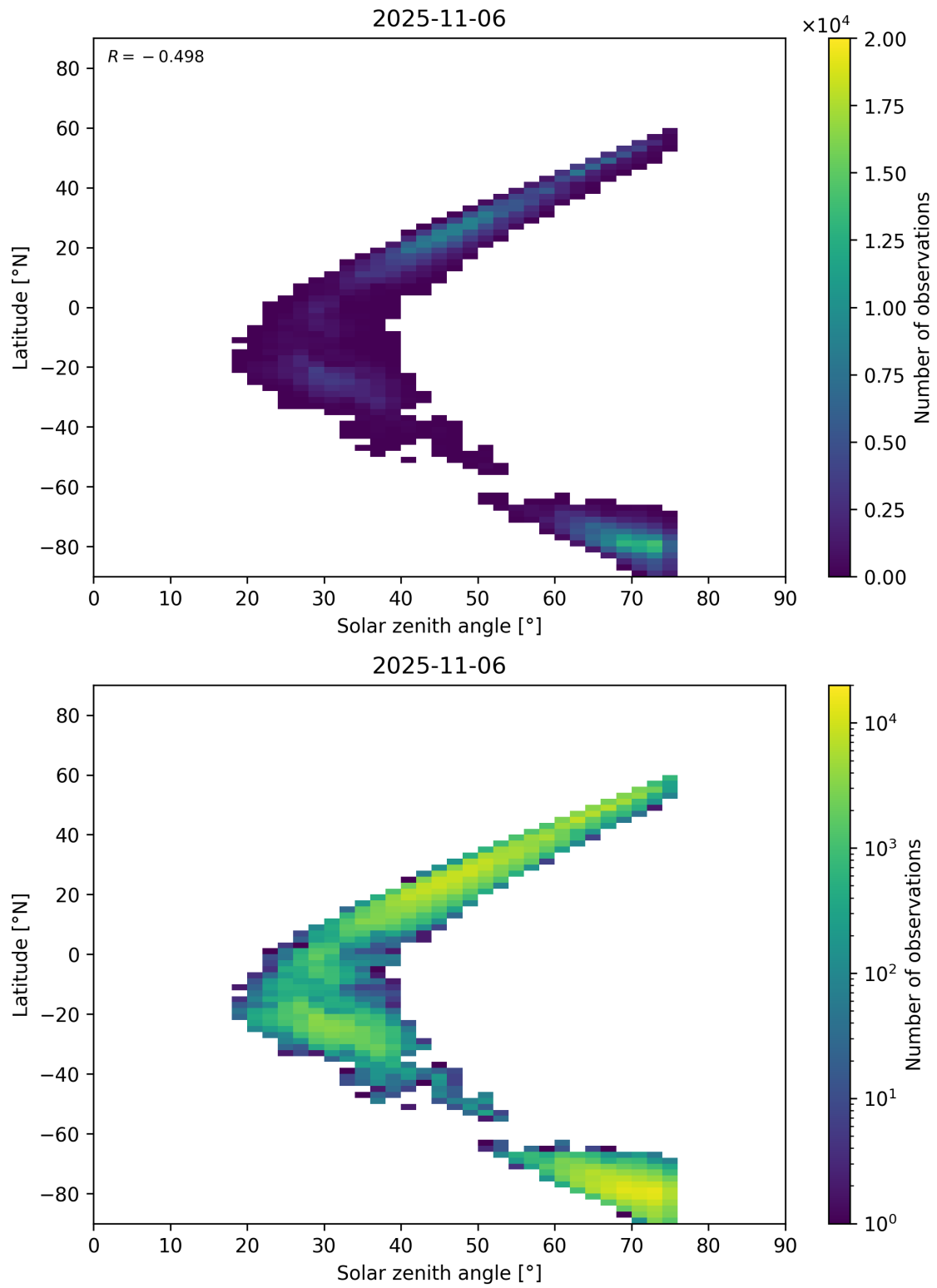
Figure 98: Scatter density plot of “Solar zenith angle” against “Latitude” for 2025-11-05 to 2025-11-07.
