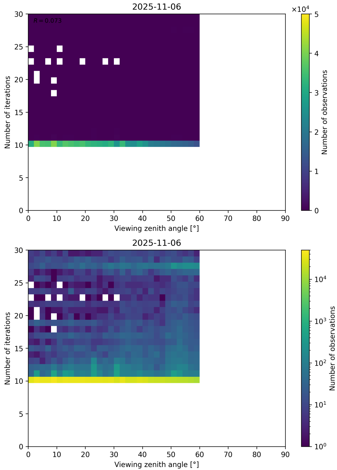
Figure 113: Scatter density plot of “Viewing zenith angle” against “Number of iterations” for 2025-11-05 to 2025-11-07.
