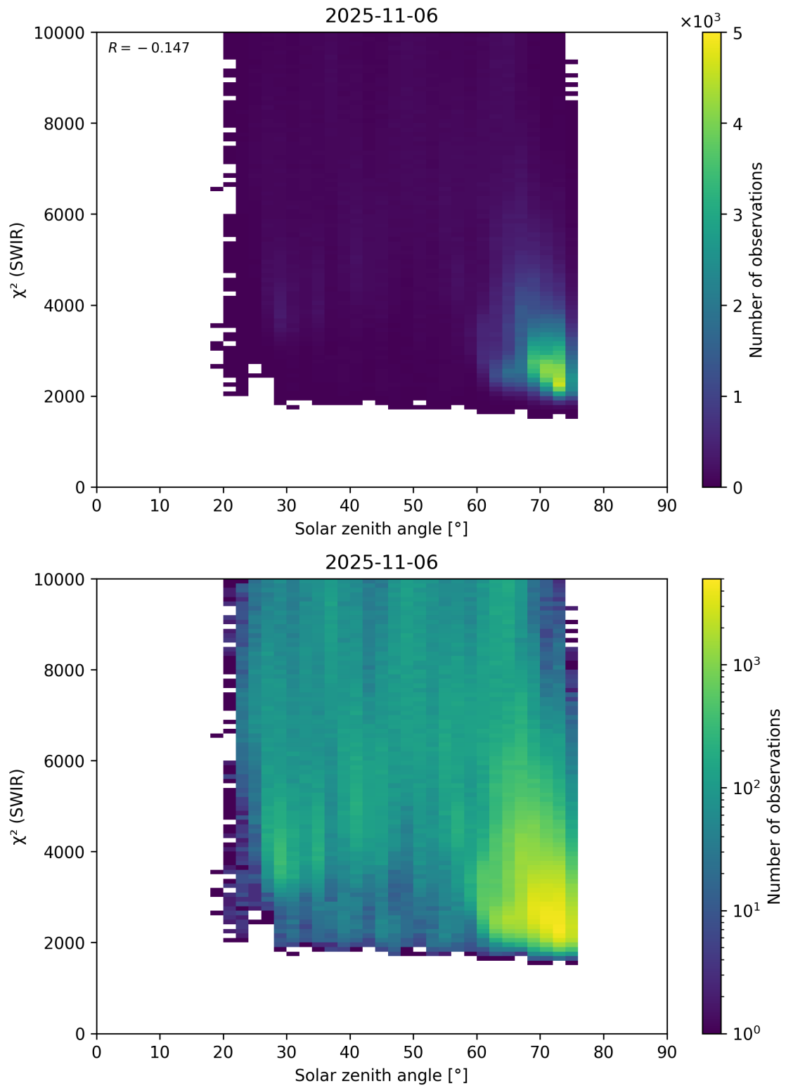
Figure 95: Scatter density plot of “Solar zenith angle” against “ \chi^2 (SWIR)” for 2025-11-05 to 2025-11-07.
