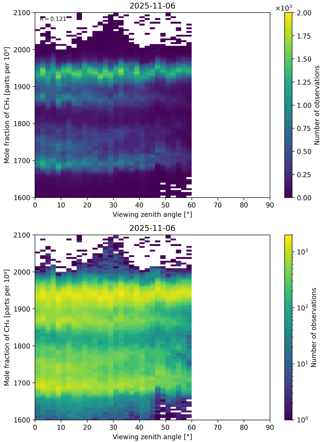
Figure 110: Scatter density plot of “Viewing zenith angle” against “Mole fraction of CH 4 ” for 2025-11-05 to 2025-11-07.
