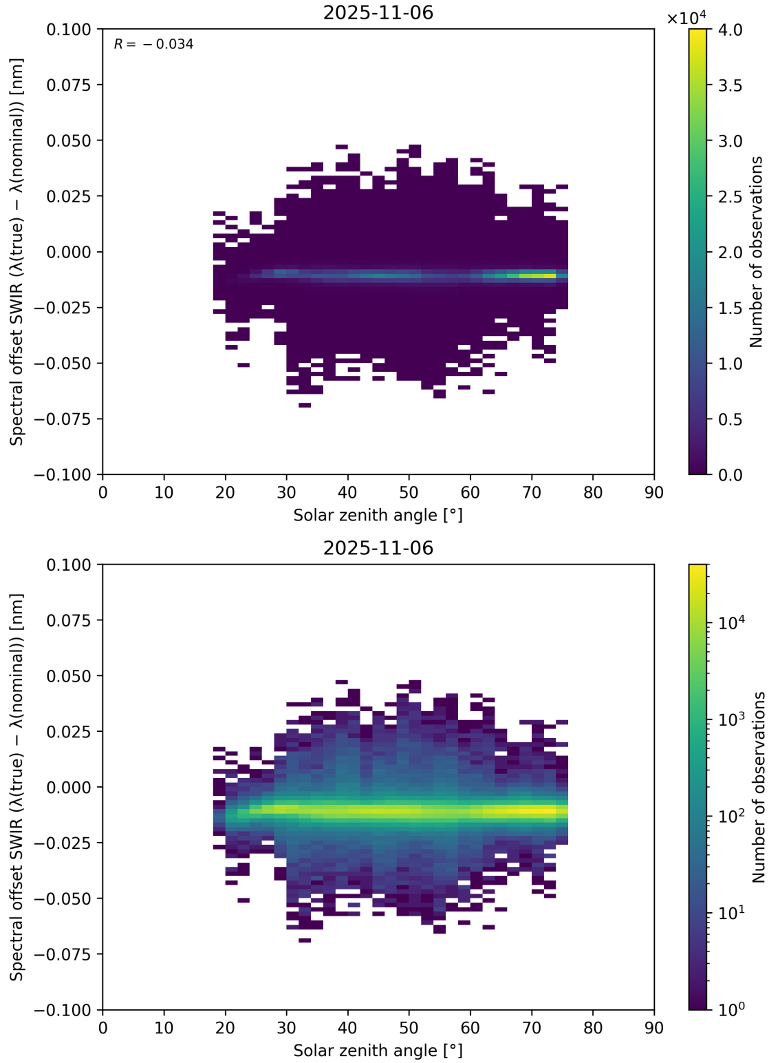
Figure 104: Scatter density plot of “Solar zenith angle” against “Spectral offset SWIR ( \lambda_{\text{true}} - \lambda_{\text{nominal}} )” for 2025-11-05 to 2025-11-07.
