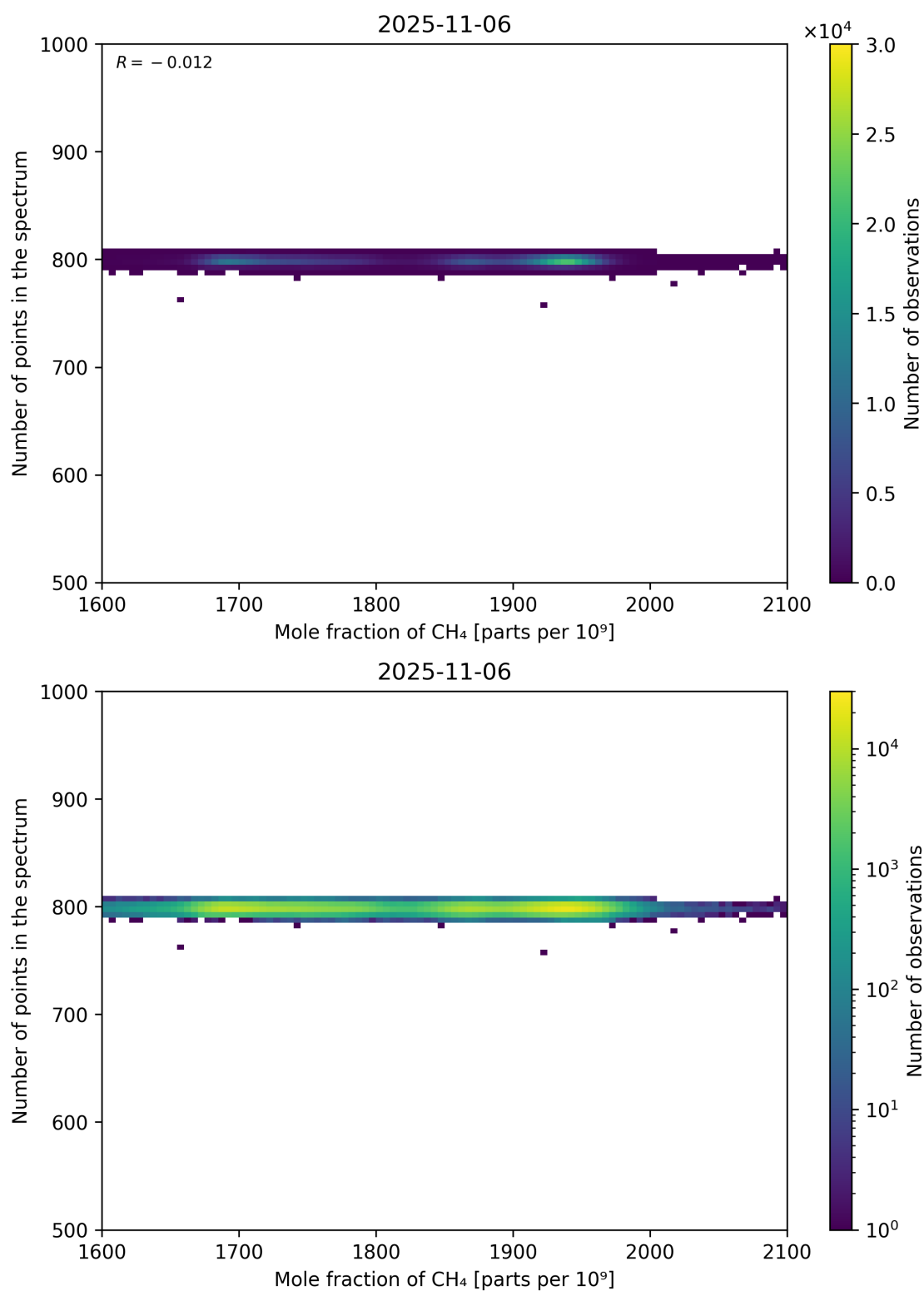
Figure 77: Scatter density plot of “Mole fraction of CH 4 ” against “Number of points in the spectrum” for 2025-11-05 to 2025-11-07.
