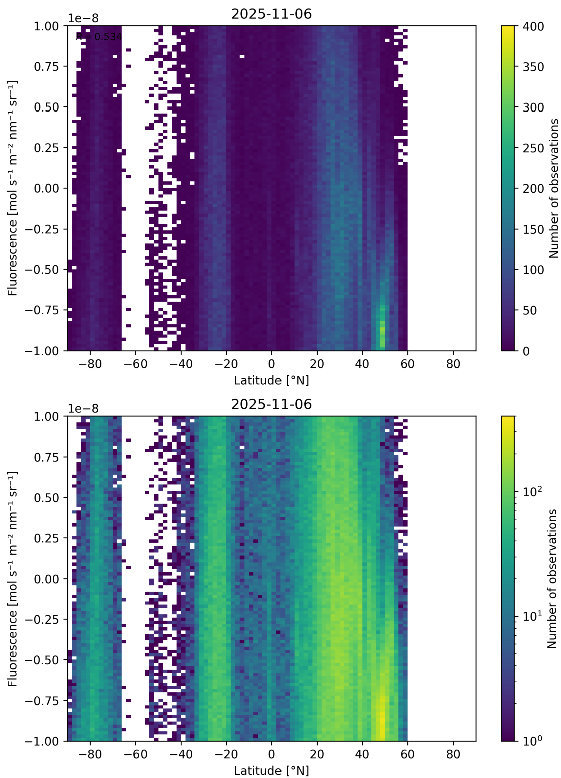
Figure 56: Scatter density plot of “Latitude” against “Fluorescence” for 2025-11-05 to 2025-11-07.
