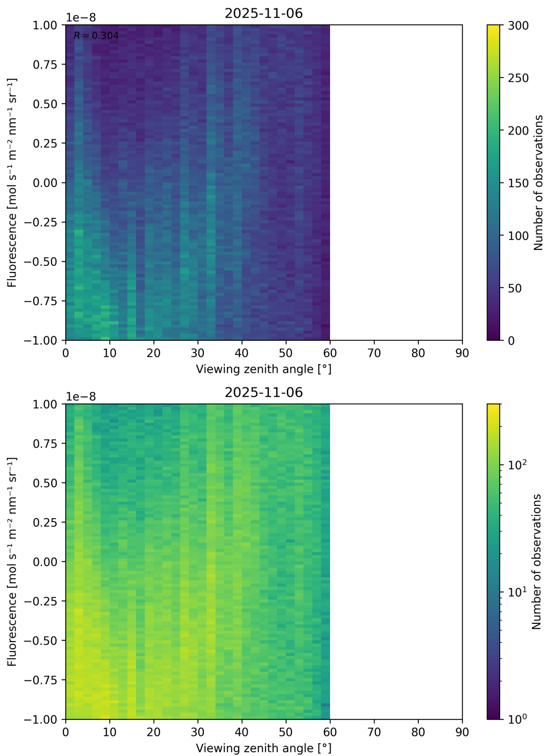
Figure 108: Scatter density plot of “Viewing zenith angle” against “Fluorescence” for 2025-11-05 to 2025-11-07.
