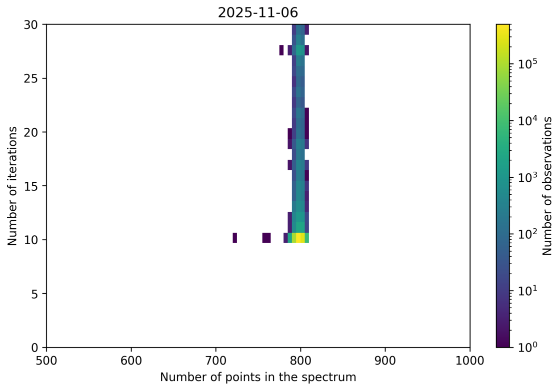
Figure 92: Scatter density plot of “Number of points in the spectrum” against “Number of iterations” for 2025-11-05 to 2025-11-07.
