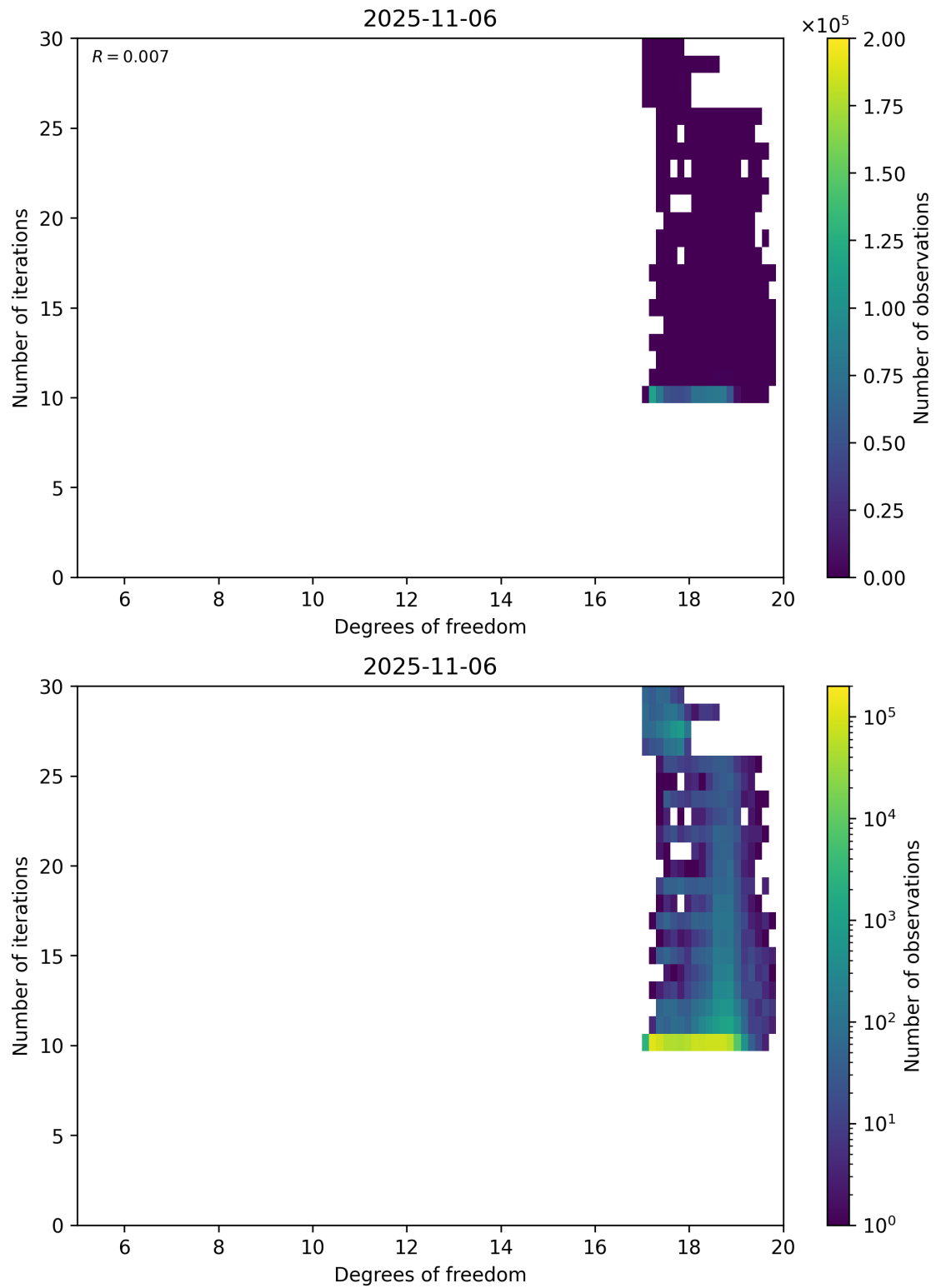
Figure 52: Scatter density plot of “Degrees of freedom” against “Number of iterations” for 2025-11-05 to 2025-11-07.
