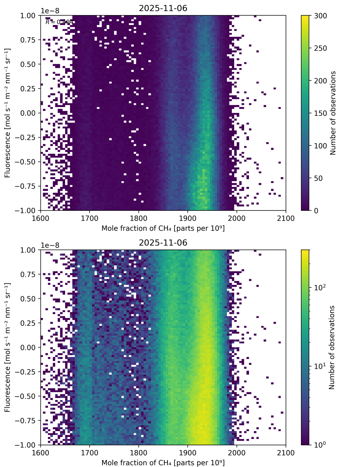
Figure 73: Scatter density plot of “Mole fraction of \text{CH}_4 ” against “Fluorescence” for 2025-11-05 to 2025-11-07.
