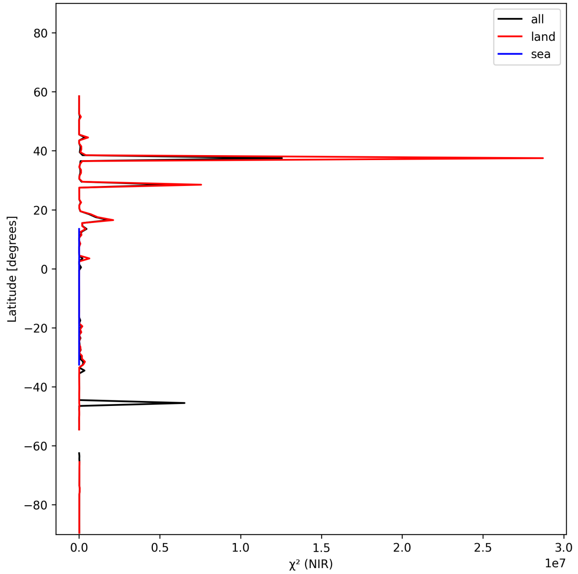
Figure 18: Zonal average of “ \chi^2 (NIR)” for 2025-11-05 to 2025-11-07.
