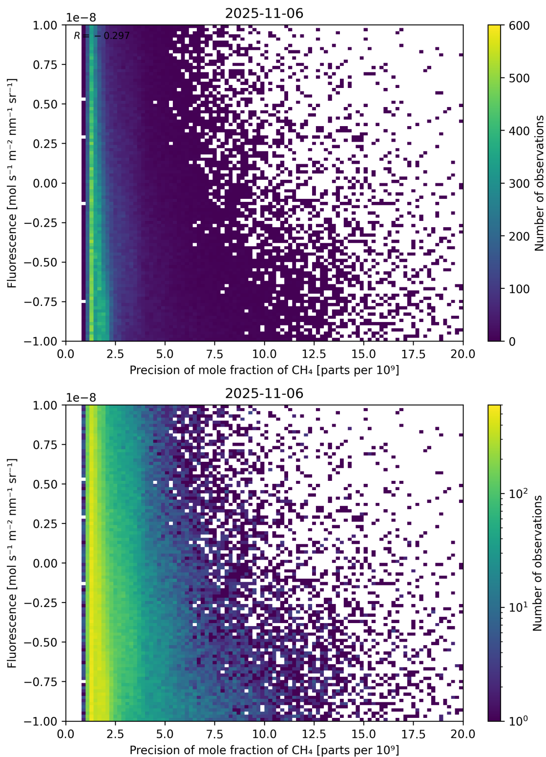
Figure 81: Scatter density plot of “Precision of mole fraction of CH 4 ” against “Fluorescence” for 2025-11-05 to 2025-11-07.
