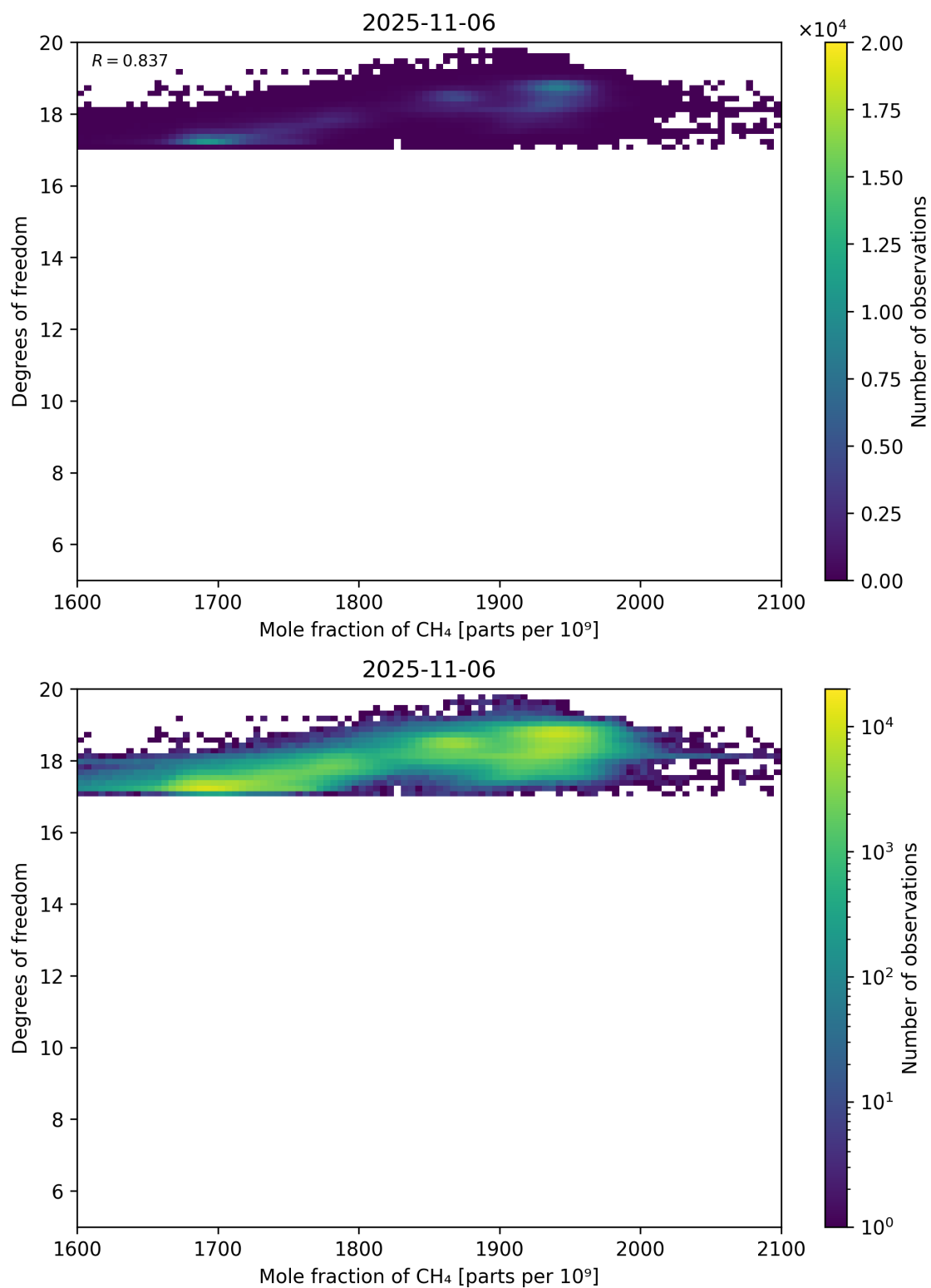
Figure 72: Scatter density plot of “Mole fraction of CH 4 ” against “Degrees of freedom” for 2025-11-05 to 2025-11-07.
