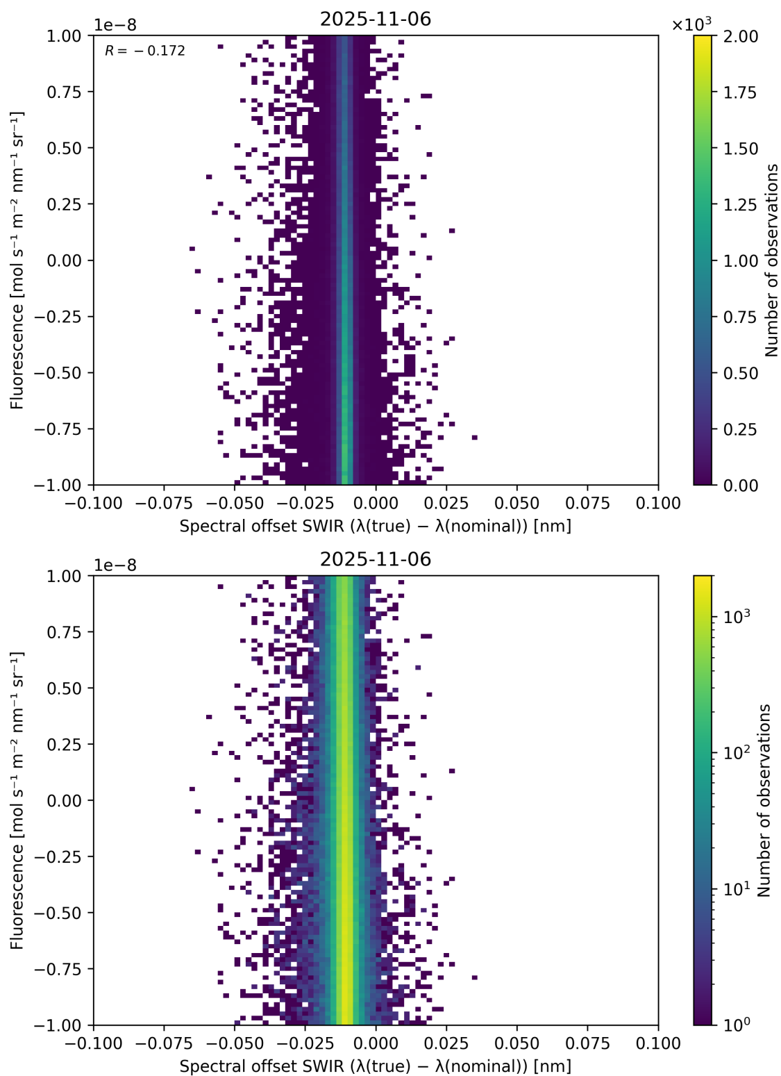
Figure 120: Scatter density plot of “Spectral offset SWIR ( \lambda_{\text{true}} - \lambda_{\text{nominal}} )” against “Fluorescence” for 2025-11-05 to 2025-11-07.
