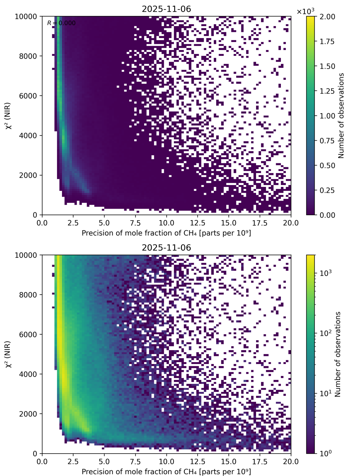
Figure 78: Scatter density plot of “Precision of mole fraction of CH 4 ” against “ \chi^2 (NIR)” for 2025-11-05 to 2025-11-07.
