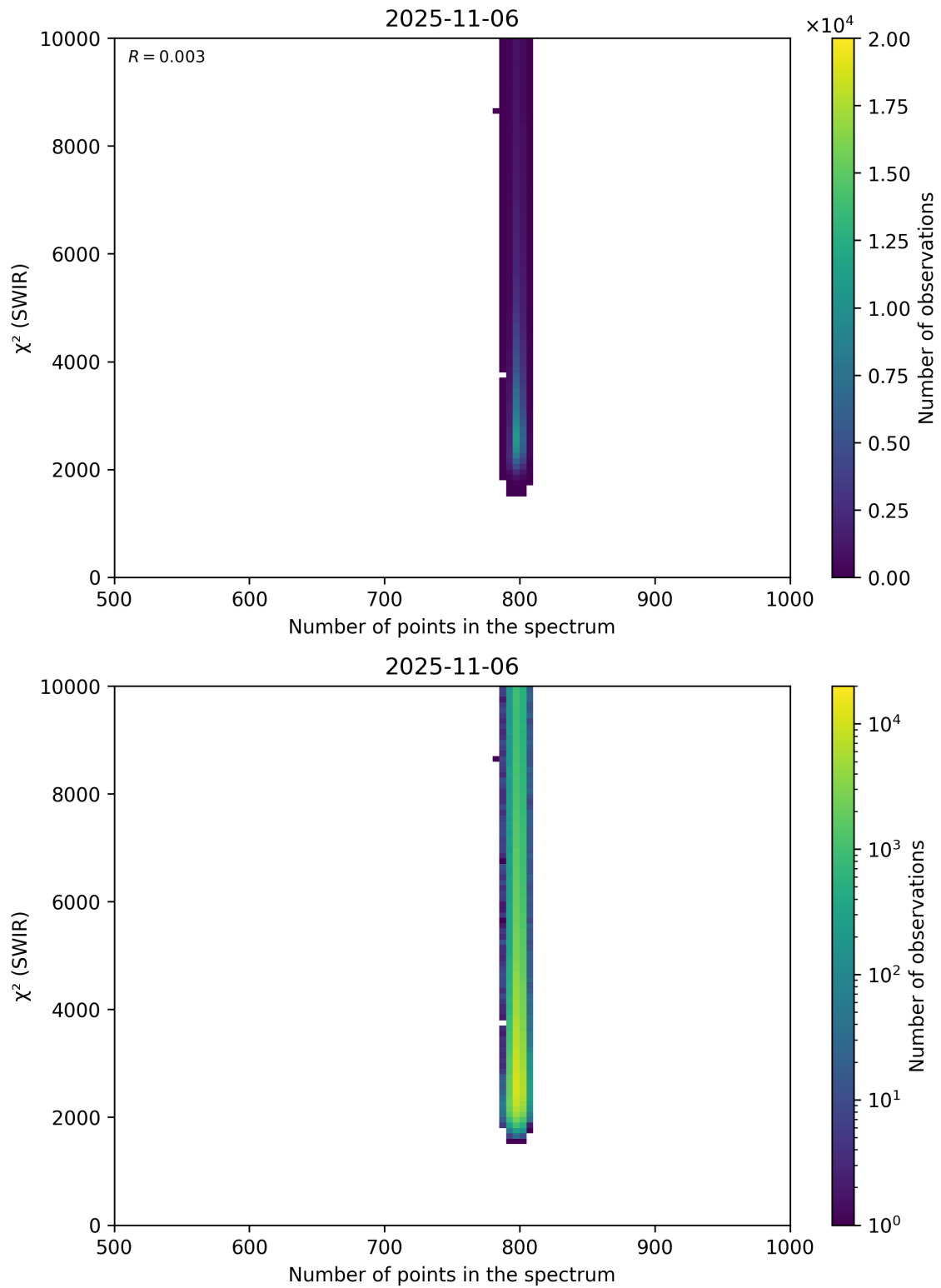
Figure 89: Scatter density plot of “Number of points in the spectrum” against “ \chi^2 (SWIR)” for 2025-11-05 to 2025-11-07.
