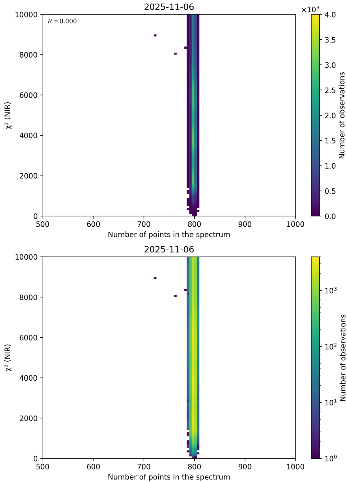
Figure 88: Scatter density plot of “Number of points in the spectrum” against “ \chi^2 (NIR)” for 2025-11-05 to 2025-11-07.
