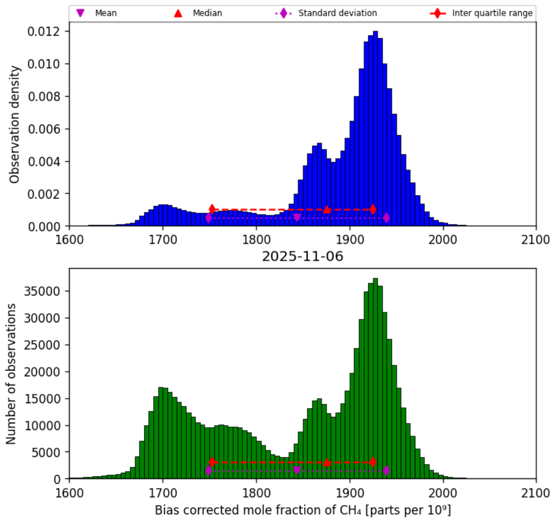
Figure 25: Histogram of “Bias corrected mole fraction of CH 4 ” for 2025-11-05 to 2025-11-07
