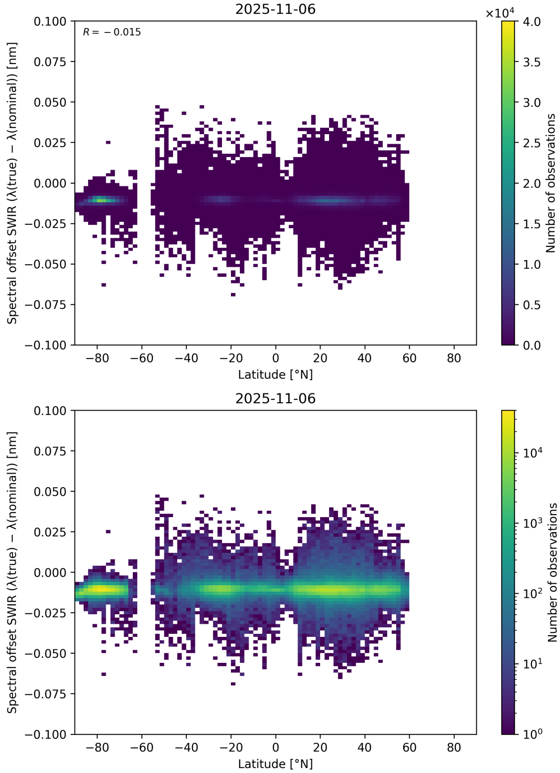
Figure 62: Scatter density plot of “Latitude” against “Spectral offset SWIR ( \lambda_{\text{true}} - \lambda_{\text{nominal}} )” for 2025-11-05 to 2025-11-07.
