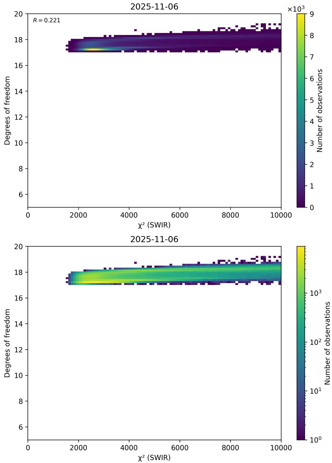
Figure 48: Scatter density plot of “ \chi^2 (SWIR)” against “Degrees of freedom” for 2025-11-05 to 2025-11-07.
