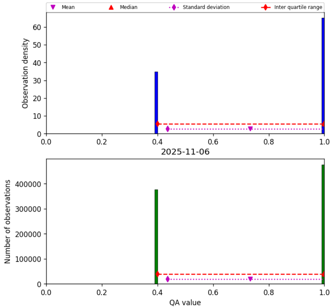
Figure 22: Histogram of “QA value” for 2025-11-05 to 2025-11-07
