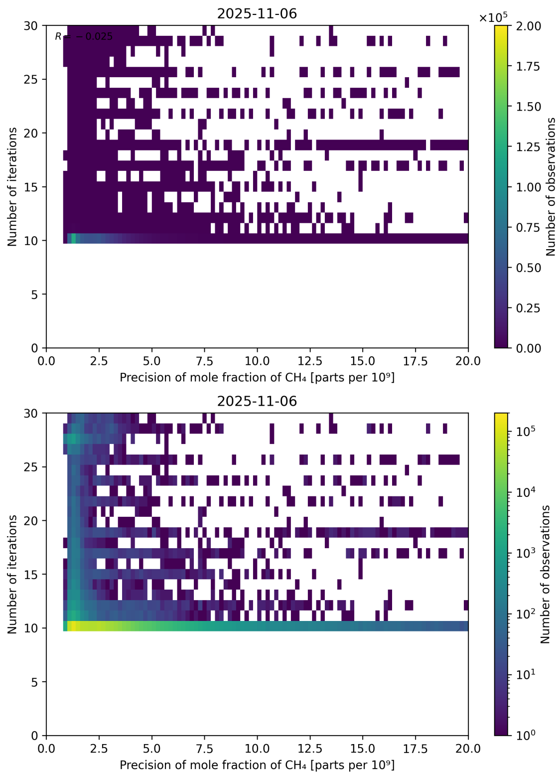
Figure 83: Scatter density plot of “Precision of mole fraction of CH 4 ” against “Number of iterations” for 2025-11-05 to 2025-11-07.
