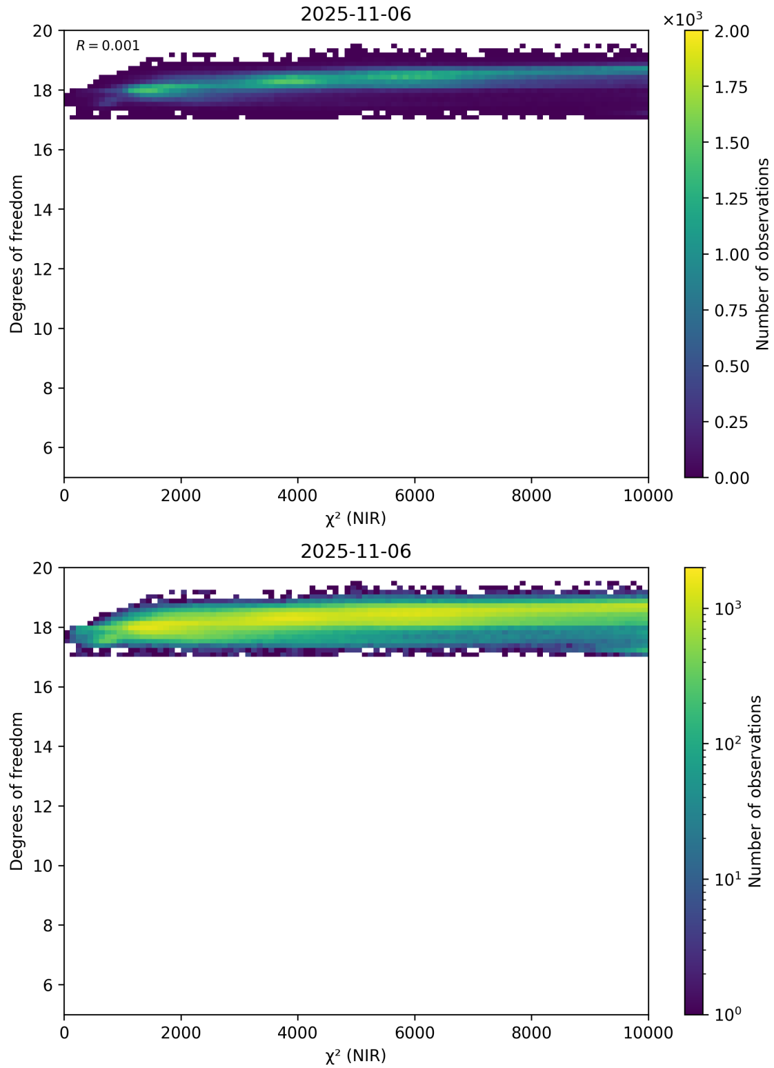
Figure 44: Scatter density plot of “ \chi^2 (NIR)” against “Degrees of freedom” for 2025-11-05 to 2025-11-07.
