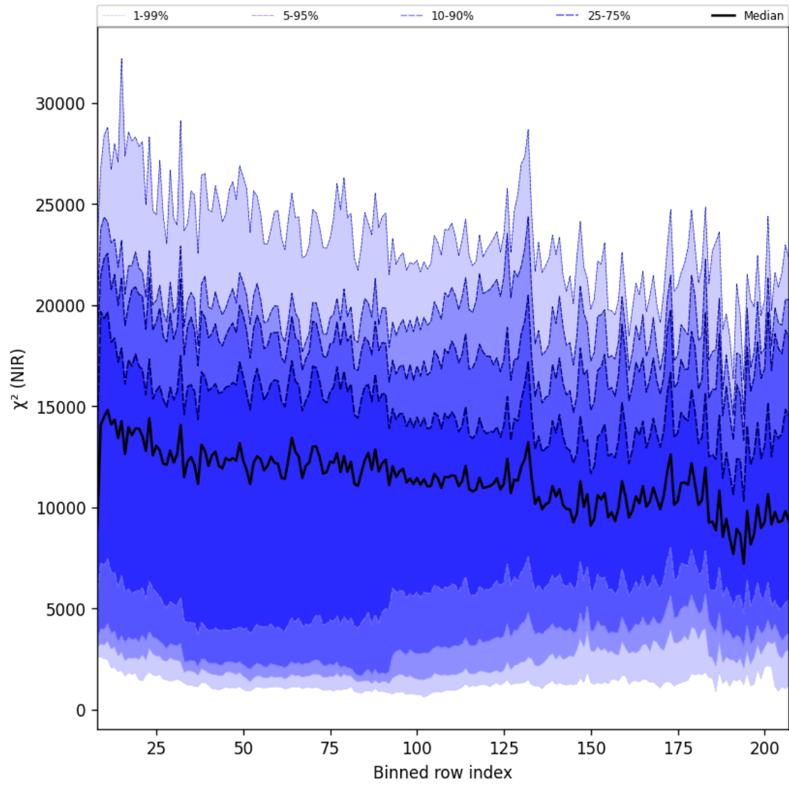
Figure 40: Along track statistics of “ \chi^2 (NIR)” for 2025-11-05 to 2025-11-07
