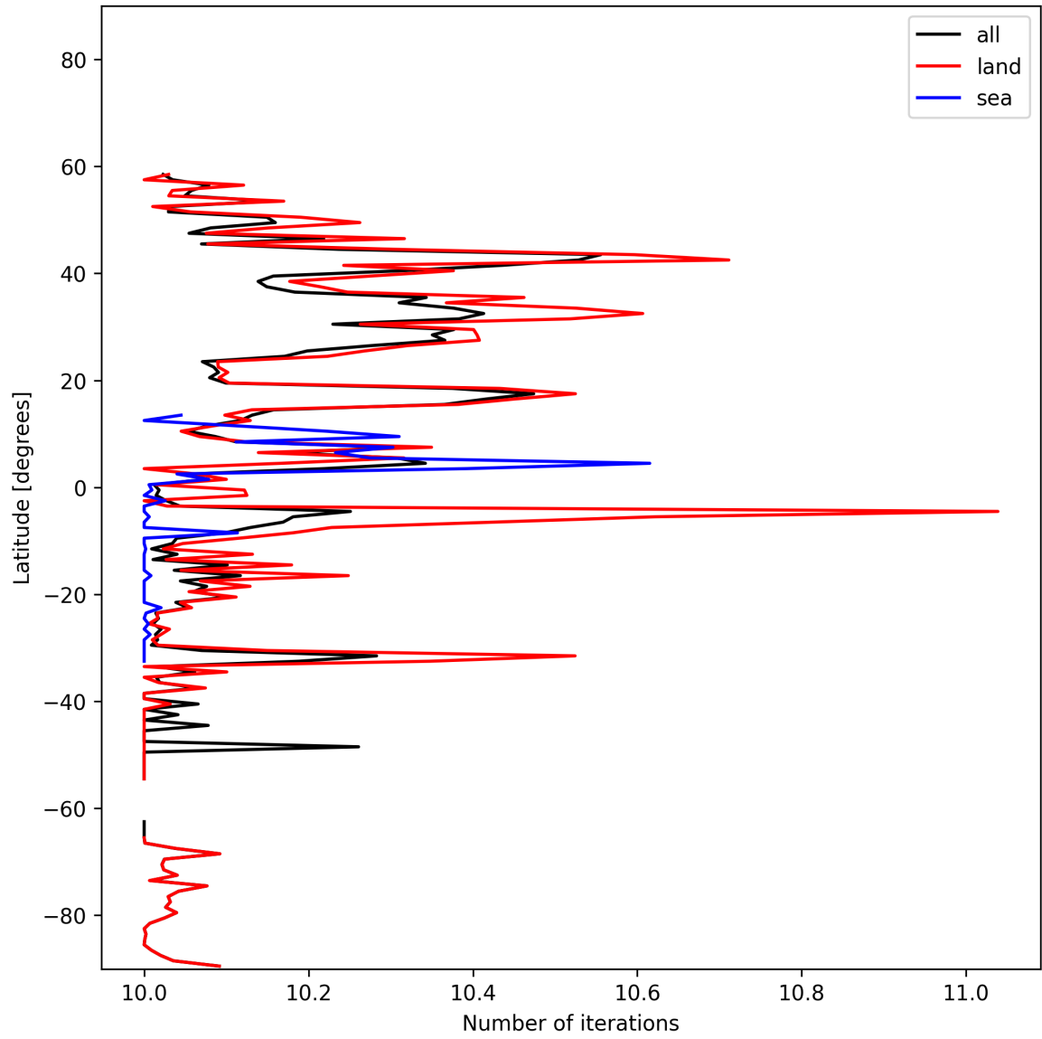
Figure 20: Zonal average of “Number of iterations” for 2025-11-05 to 2025-11-07.
