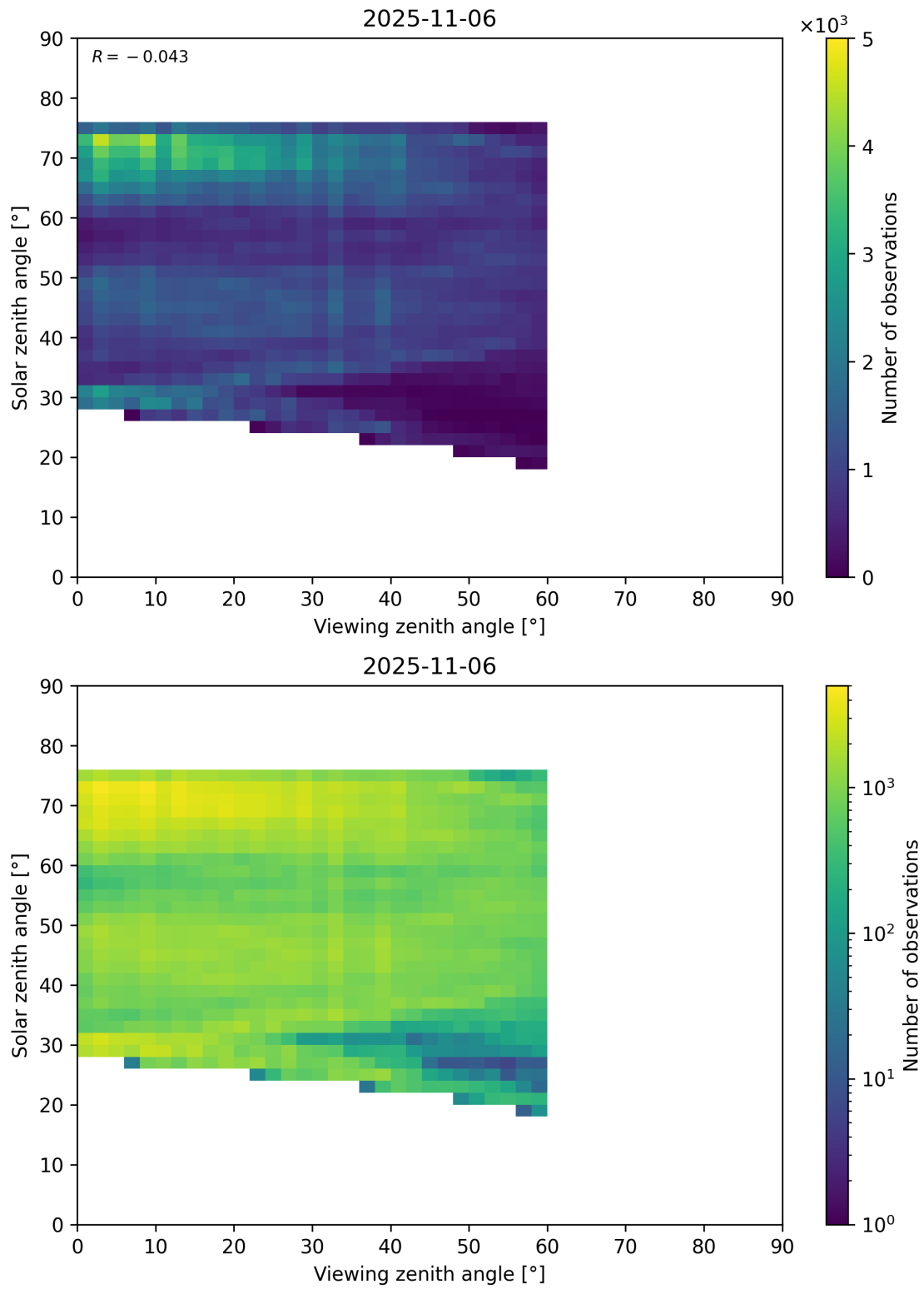
Figure 115: Scatter density plot of “Viewing zenith angle” against “Solar zenith angle” for 2025-11-05 to 2025-11-07.
