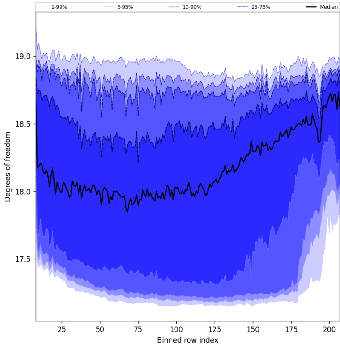
Figure 41: Along track statistics of “Degrees of freedom” for 2025-11-05 to 2025-11-07
