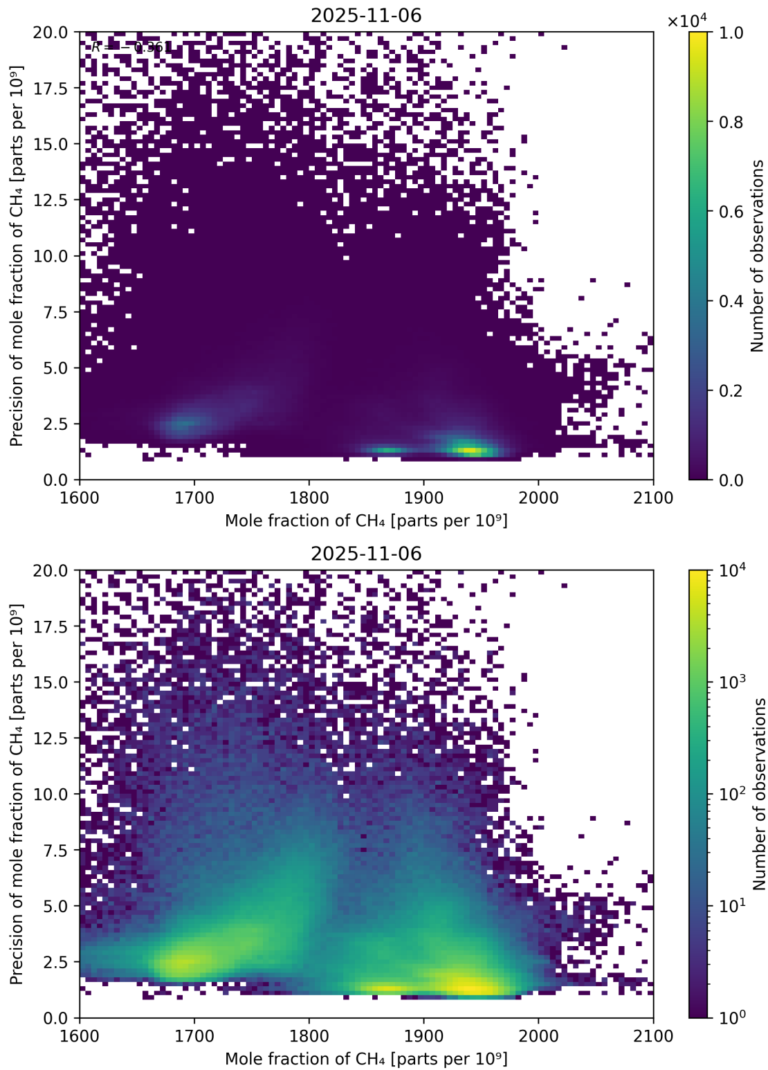
Figure 75: Scatter density plot of “Mole fraction of CH 4 ” against “Precision of mole fraction of CH 4 ” for 2025-11-05 to 2025-11-07.
