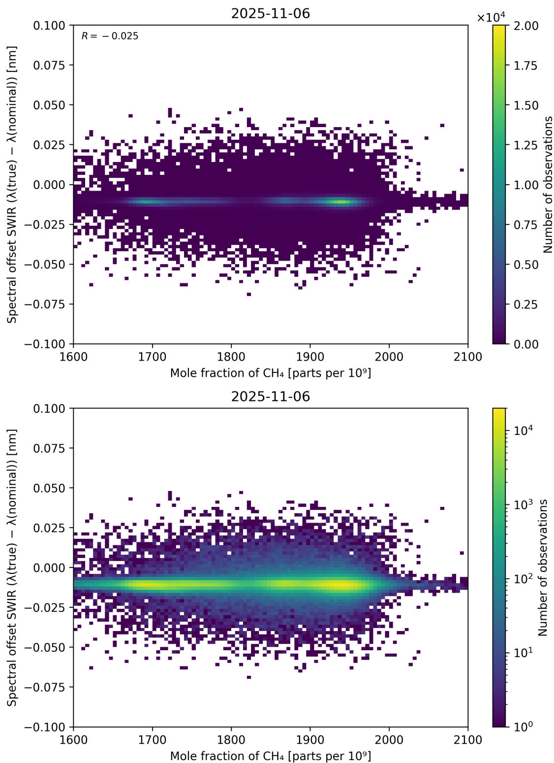
Figure 86: Scatter density plot of “Mole fraction of \text{CH}_4 ” against “Spectral offset SWIR ( \lambda_{\text{true}} - \lambda_{\text{nominal}} )” for 2025-11-05 to 2025-11-07.
