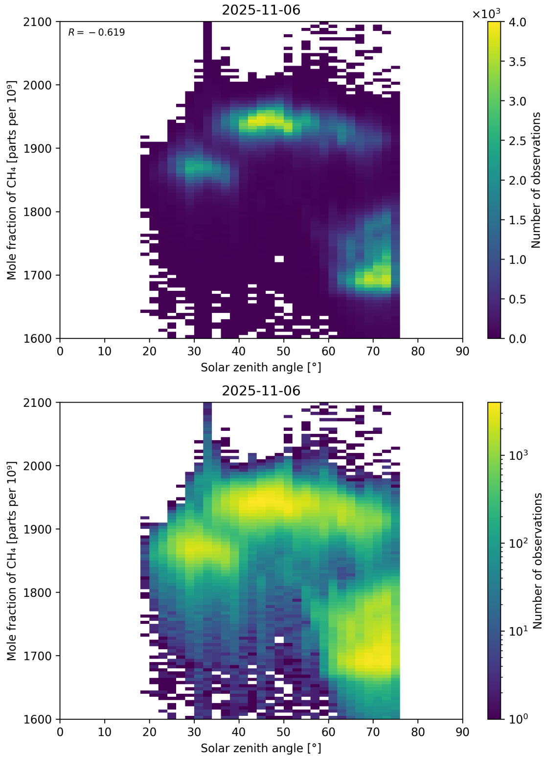
Figure 99: Scatter density plot of “Solar zenith angle” against “Mole fraction of CH 4 ” for 2025-11-05 to 2025-11-07.
