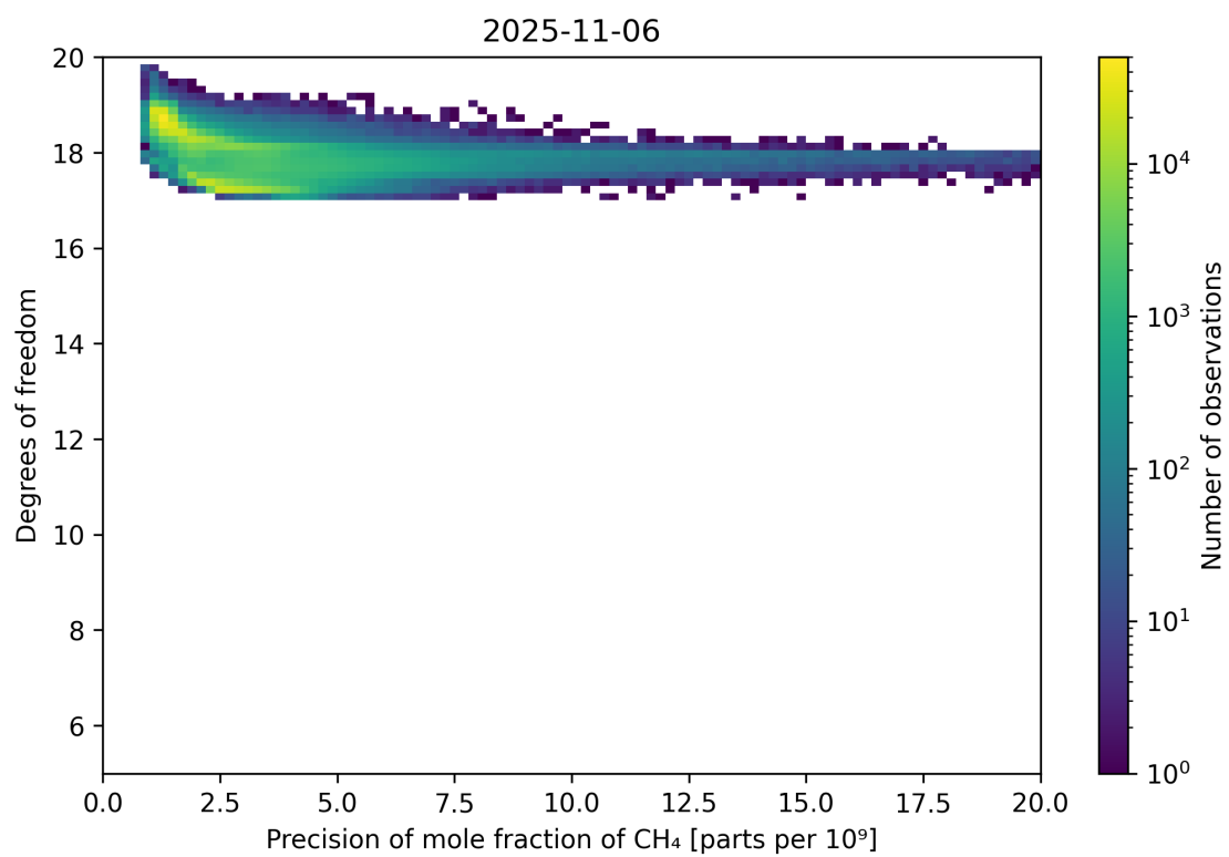
Figure 80: Scatter density plot of “Precision of mole fraction of CH 4 ” against “Degrees of freedom” for 2025-11-05 to 2025-11-07.
