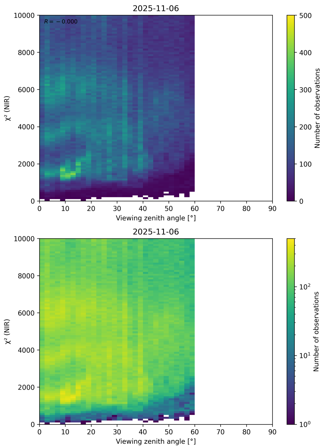
Figure 105: Scatter density plot of “Viewing zenith angle” against “ \chi^2 (NIR)” for 2025-11-05 to 2025-11-07.
