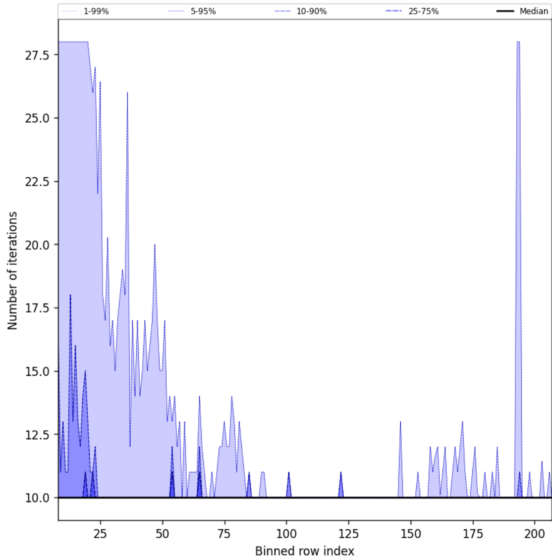
Figure 42: Along track statistics of “Number of iterations” for 2025-11-05 to 2025-11-07
