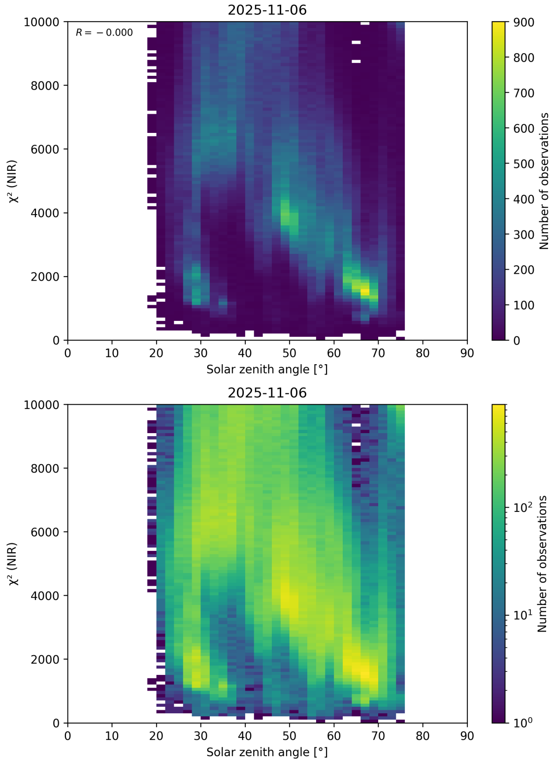
Figure 94: Scatter density plot of “Solar zenith angle” against “ \chi^2 (NIR)” for 2025-11-05 to 2025-11-07.
