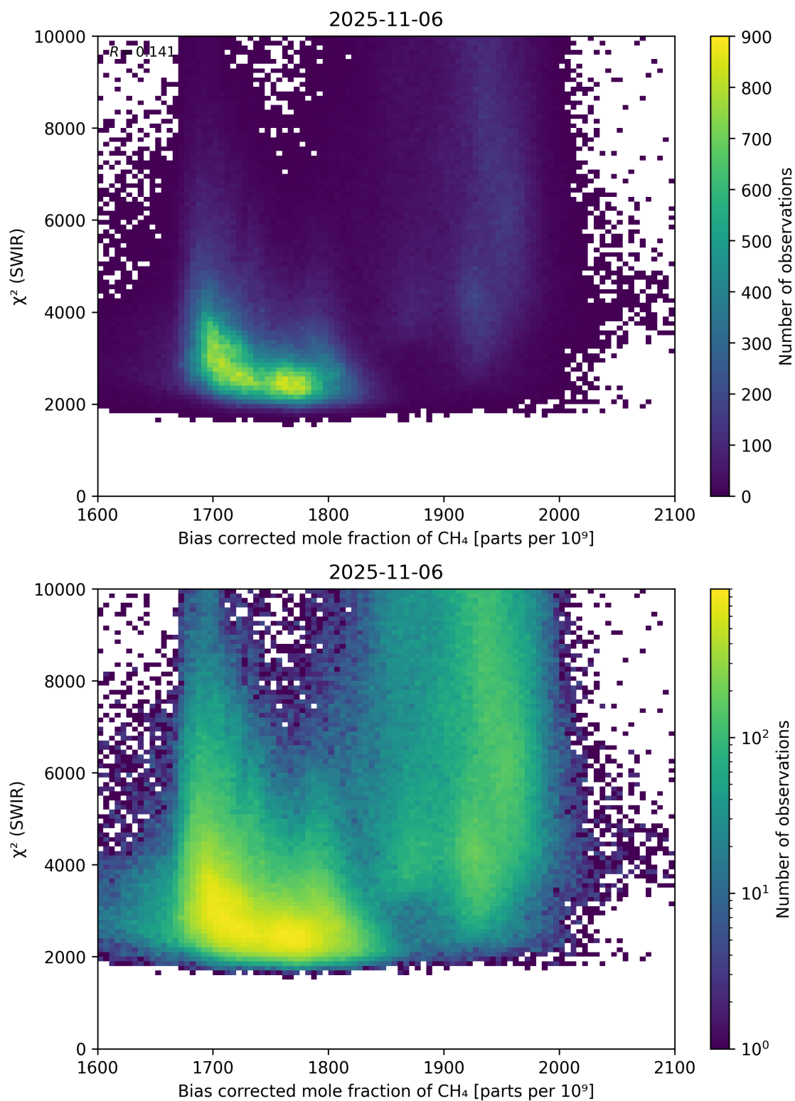
Figure 64: Scatter density plot of “Bias corrected mole fraction of \text{CH}_4 ” against “ \chi^2 (SWIR)” for 2025-11-05 to 2025-11-07.
