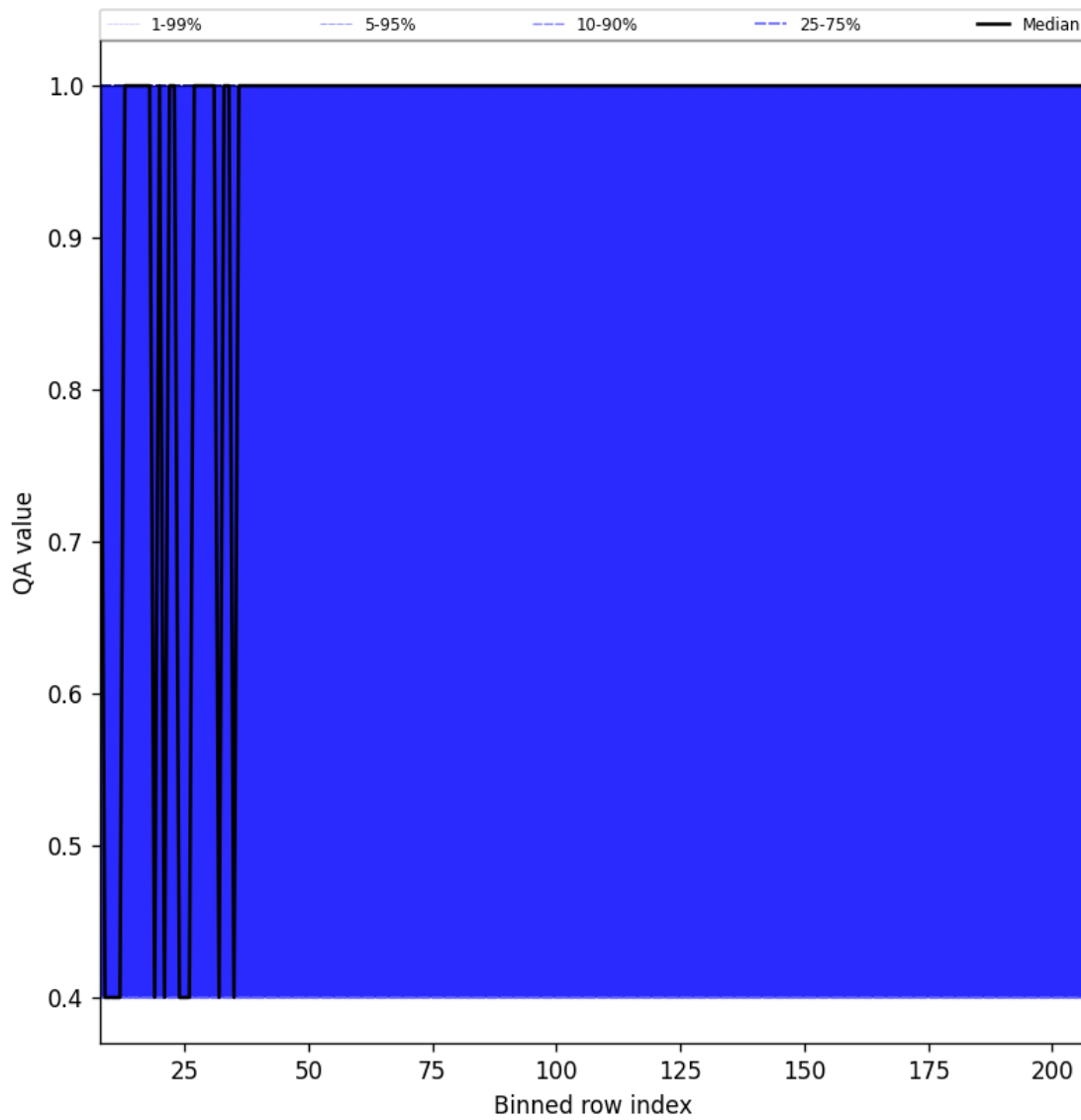
Figure 33: Along track statistics of “QA value” for 2025-11-05 to 2025-11-07
