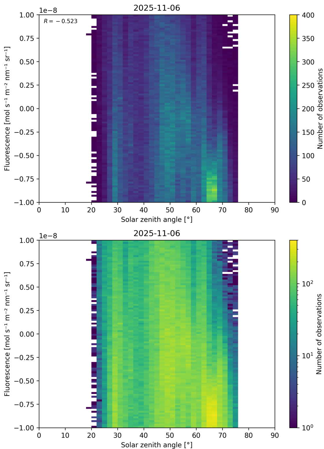
Figure 97: Scatter density plot of “Solar zenith angle” against “Fluorescence” for 2025-11-05 to 2025-11-07.
