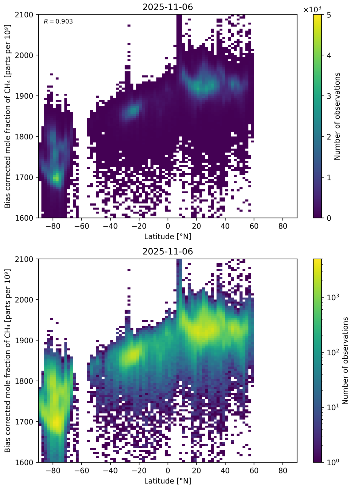
Figure 58: Scatter density plot of “Latitude” against “Bias corrected mole fraction of CH 4 ” for 2025-11-05 to 2025-11-07.
