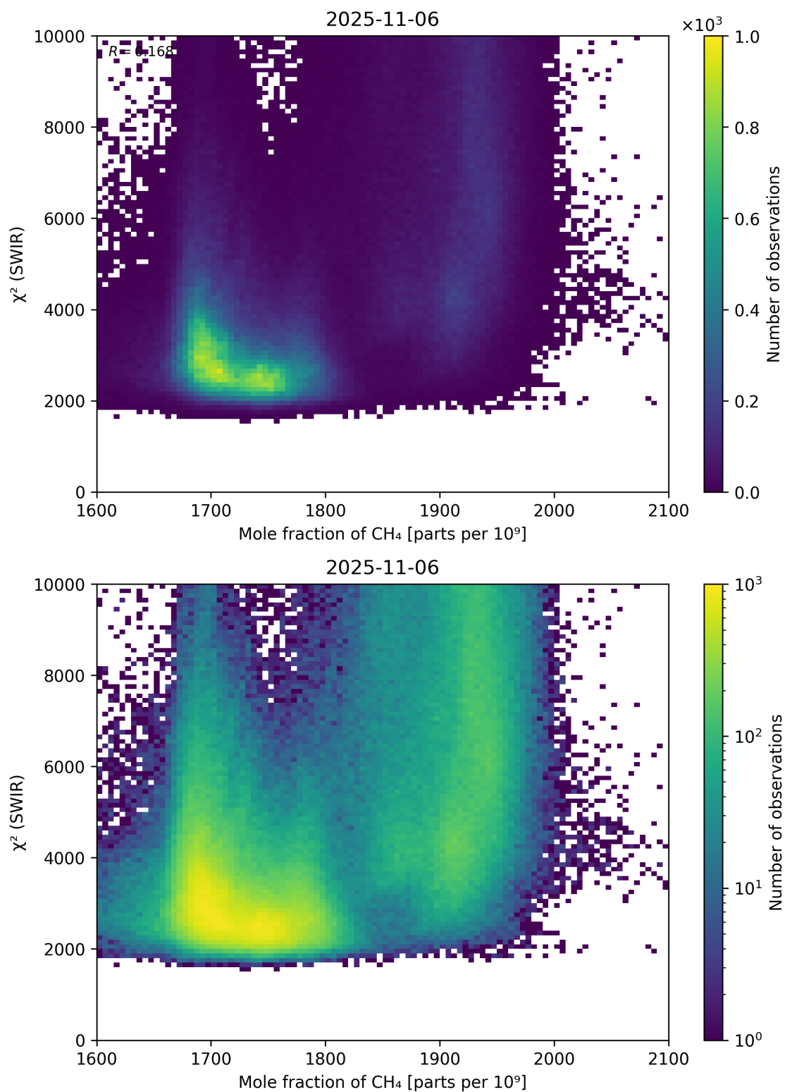
Figure 71: Scatter density plot of “Mole fraction of \text{CH}_4 ” against “ \chi^2 (SWIR)” for 2025-11-05 to 2025-11-07.
