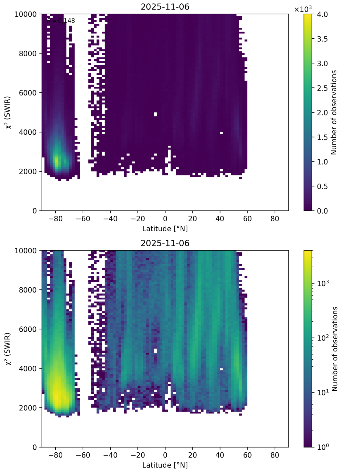
Figure 54: Scatter density plot of “Latitude” against “ \chi^2 (SWIR)” for 2025-11-05 to 2025-11-07.
