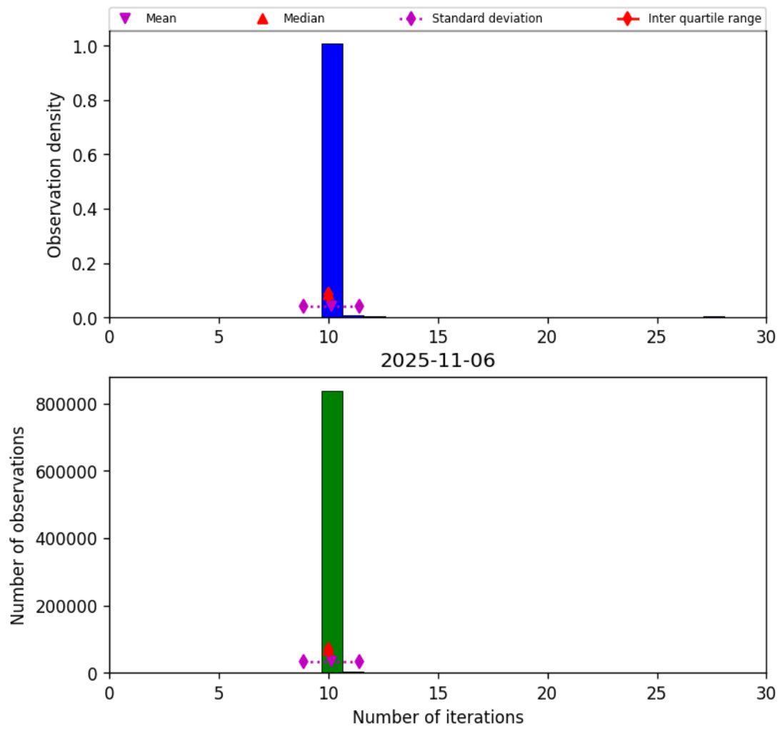
Figure 31: Histogram of “Number of iterations” for 2025-11-05 to 2025-11-07
