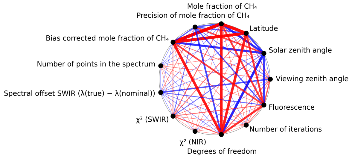
Figure 1: Map of correlation graph for 2025-11-05 to 2025-11-07.
