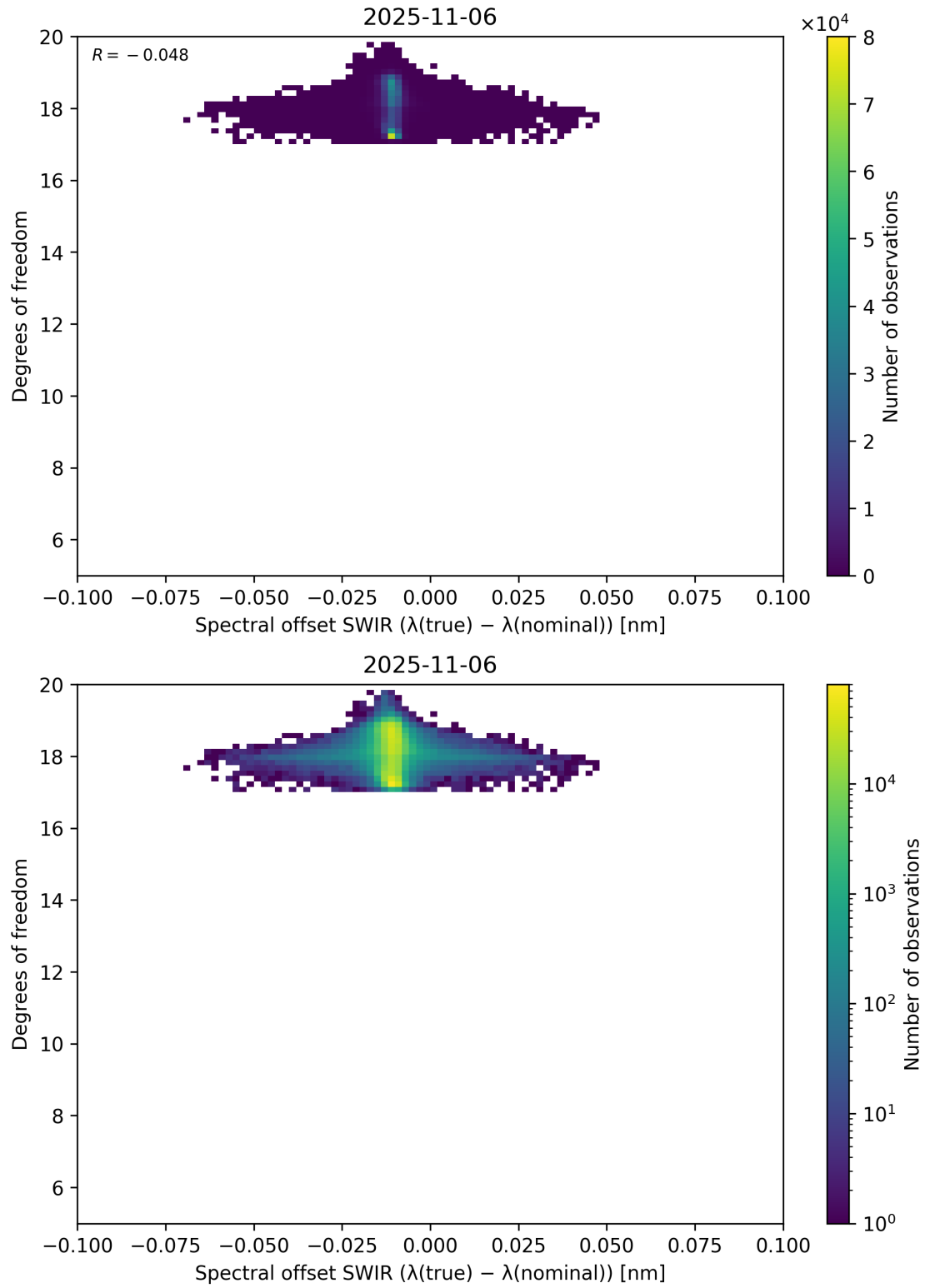
Figure 119: Scatter density plot of “Spectral offset SWIR ( \lambda_{\text{true}} - \lambda_{\text{nominal}} )” against “Degrees of freedom” for 2025-11-05 to 2025-11-07.
