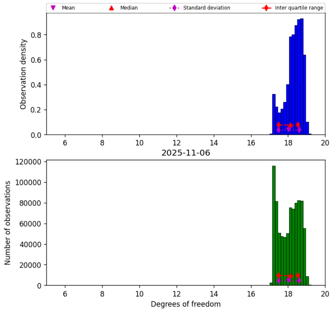
Figure 30: Histogram of “Degrees of freedom” for 2025-11-05 to 2025-11-07
