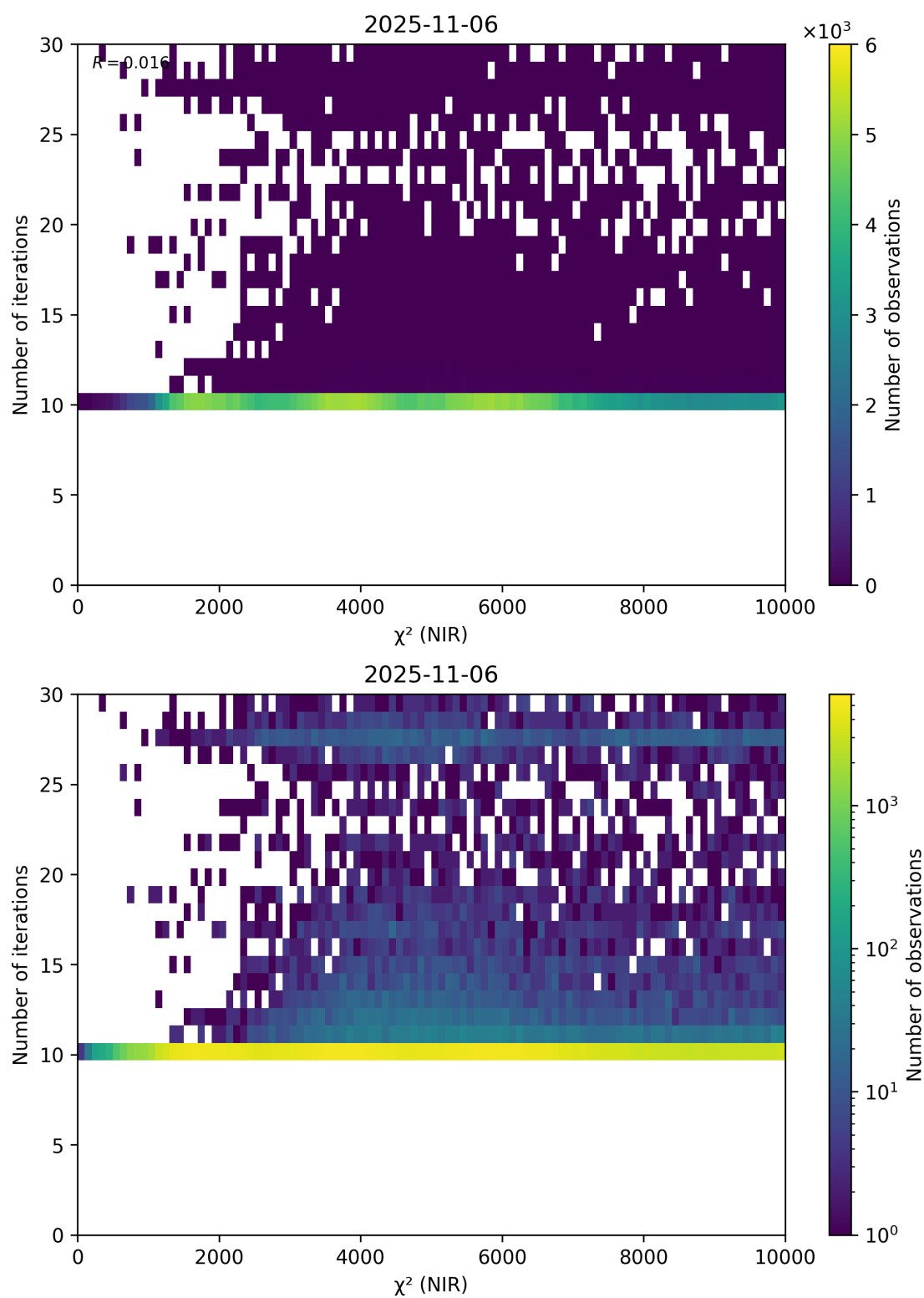
Figure 46: Scatter density plot of “ \chi^2 (NIR)” against “Number of iterations” for 2025-11-05 to 2025-11-07.
