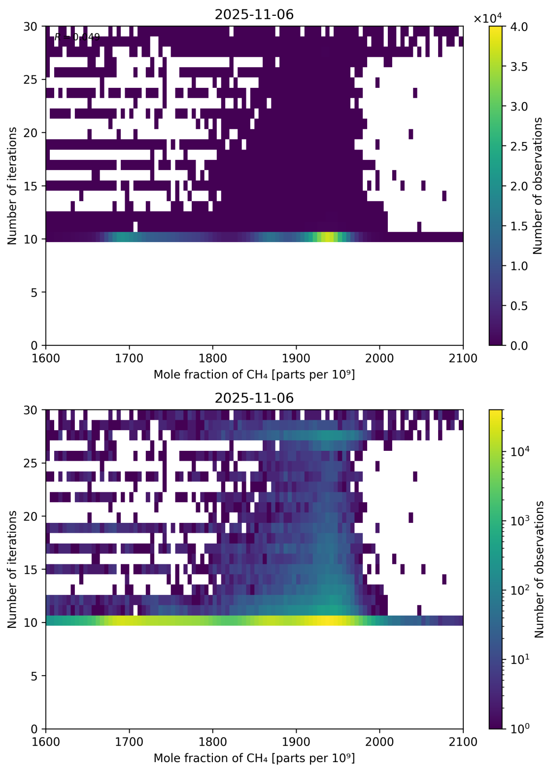
Figure 76: Scatter density plot of “Mole fraction of CH 4 ” against “Number of iterations” for 2025-11-05 to 2025-11-07.
