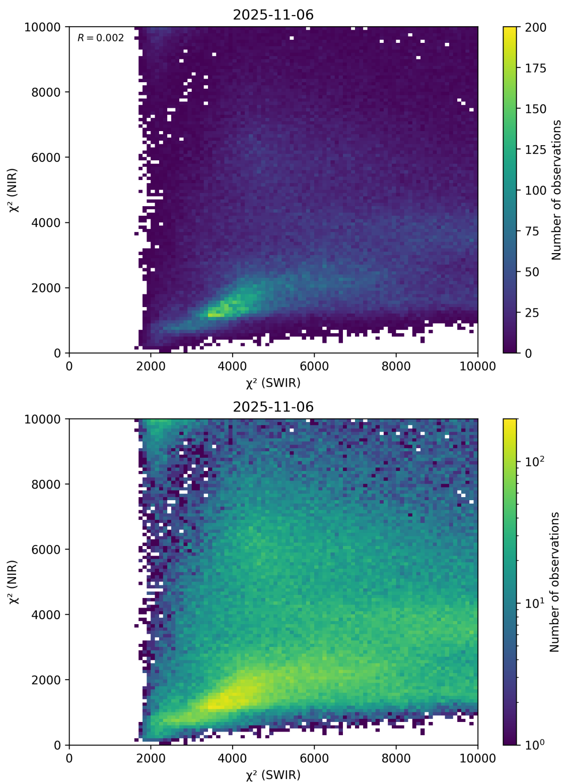
Figure 47: Scatter density plot of “ \chi^2 (SWIR)” against “ \chi^2 (NIR)” for 2025-11-05 to 2025-11-07.
