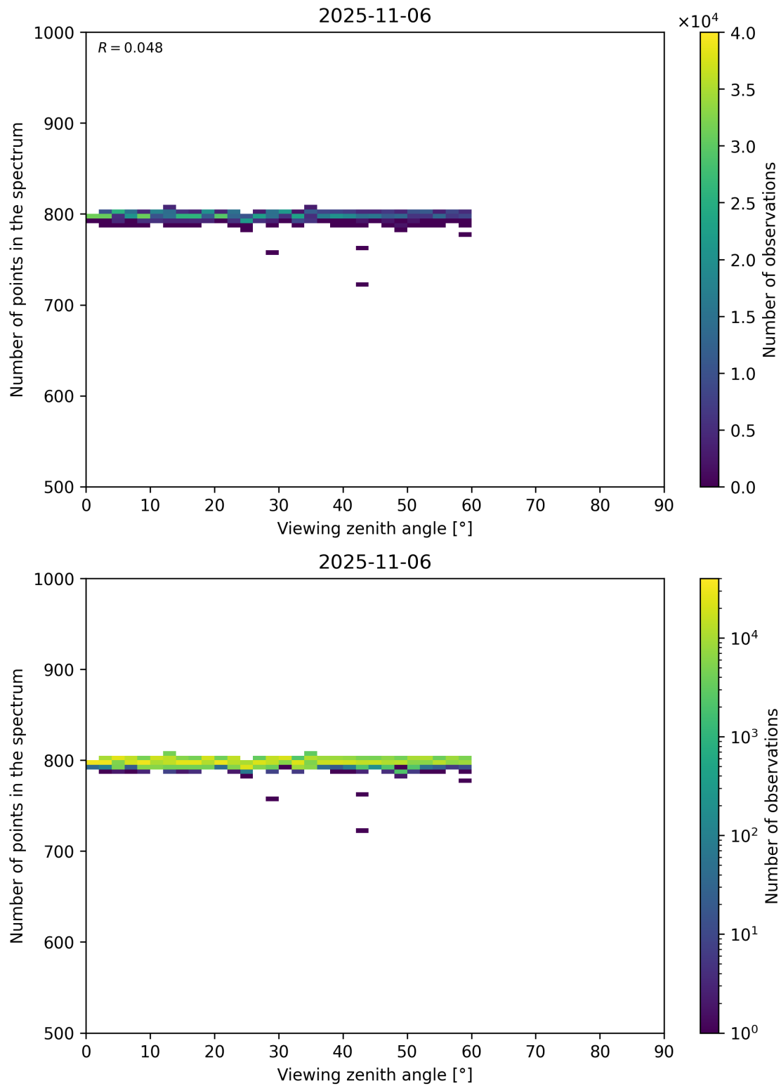
Figure 114: Scatter density plot of “Viewing zenith angle” against “Number of points in the spectrum” for 2025-11-05 to 2025-11-07.
