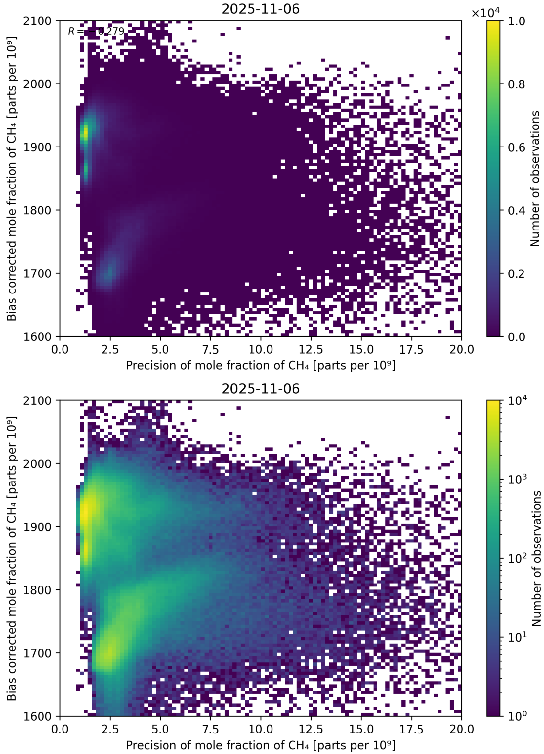
Figure 82: Scatter density plot of “Precision of mole fraction of CH 4 ” against “Bias corrected mole fraction of CH 4 ” for 2025-11-05 to 2025-11-07.
