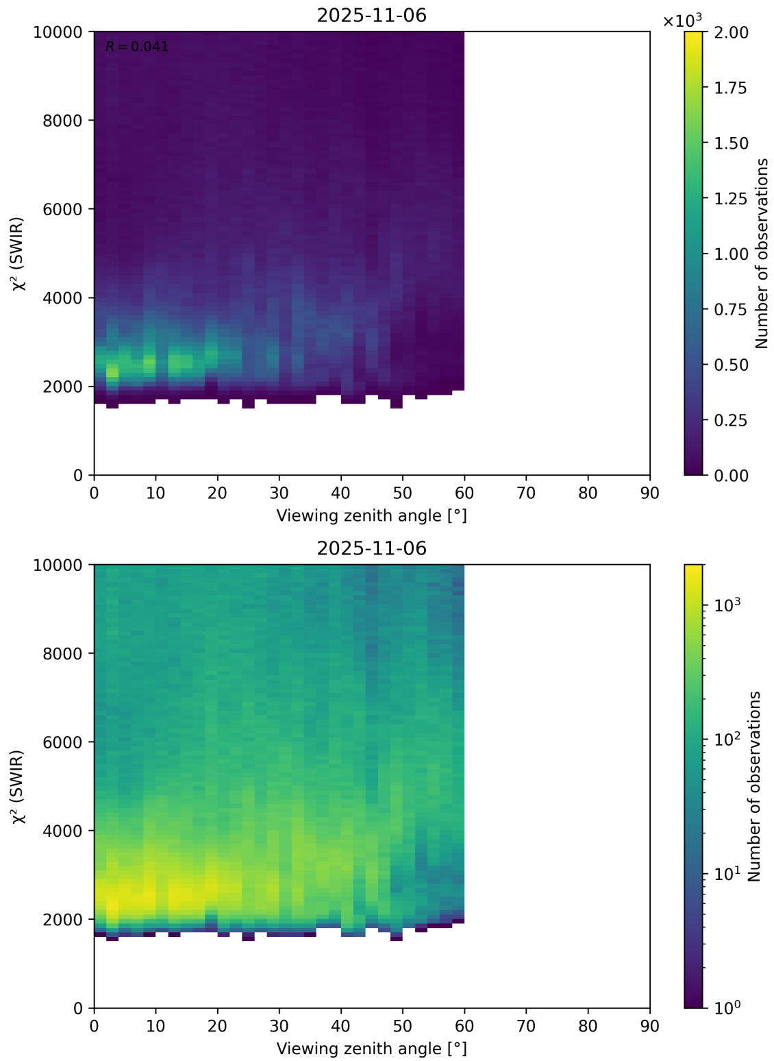
Figure 106: Scatter density plot of “Viewing zenith angle” against “ \chi^2 (SWIR)” for 2025-11-05 to 2025-11-07.
