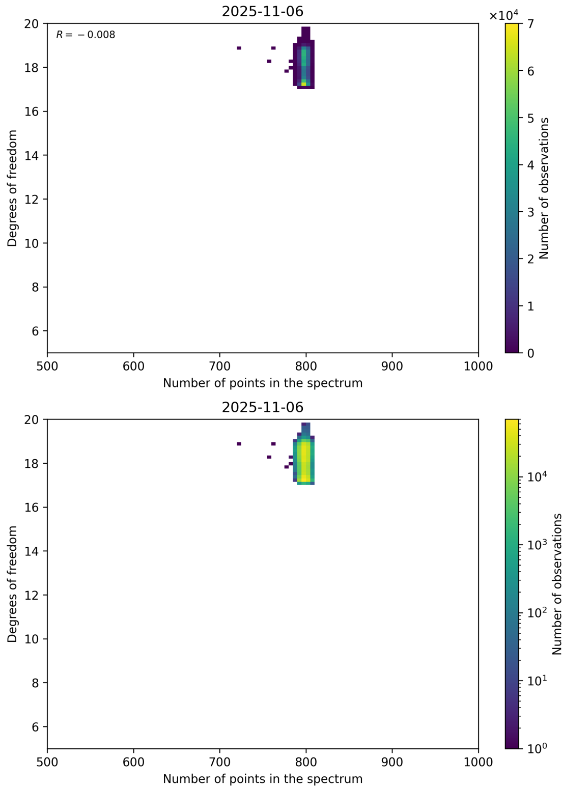
Figure 90: Scatter density plot of “Number of points in the spectrum” against “Degrees of freedom” for 2025-11-05 to 2025-11-07.
