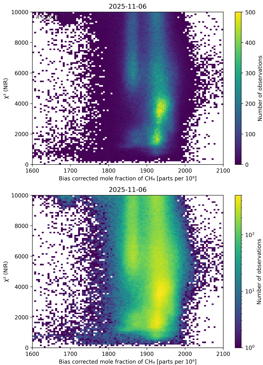
Figure 63: Scatter density plot of “Bias corrected mole fraction of CH 4 ” against “ \chi^2 (NIR)” for 2025-11-05 to 2025-11-07.
