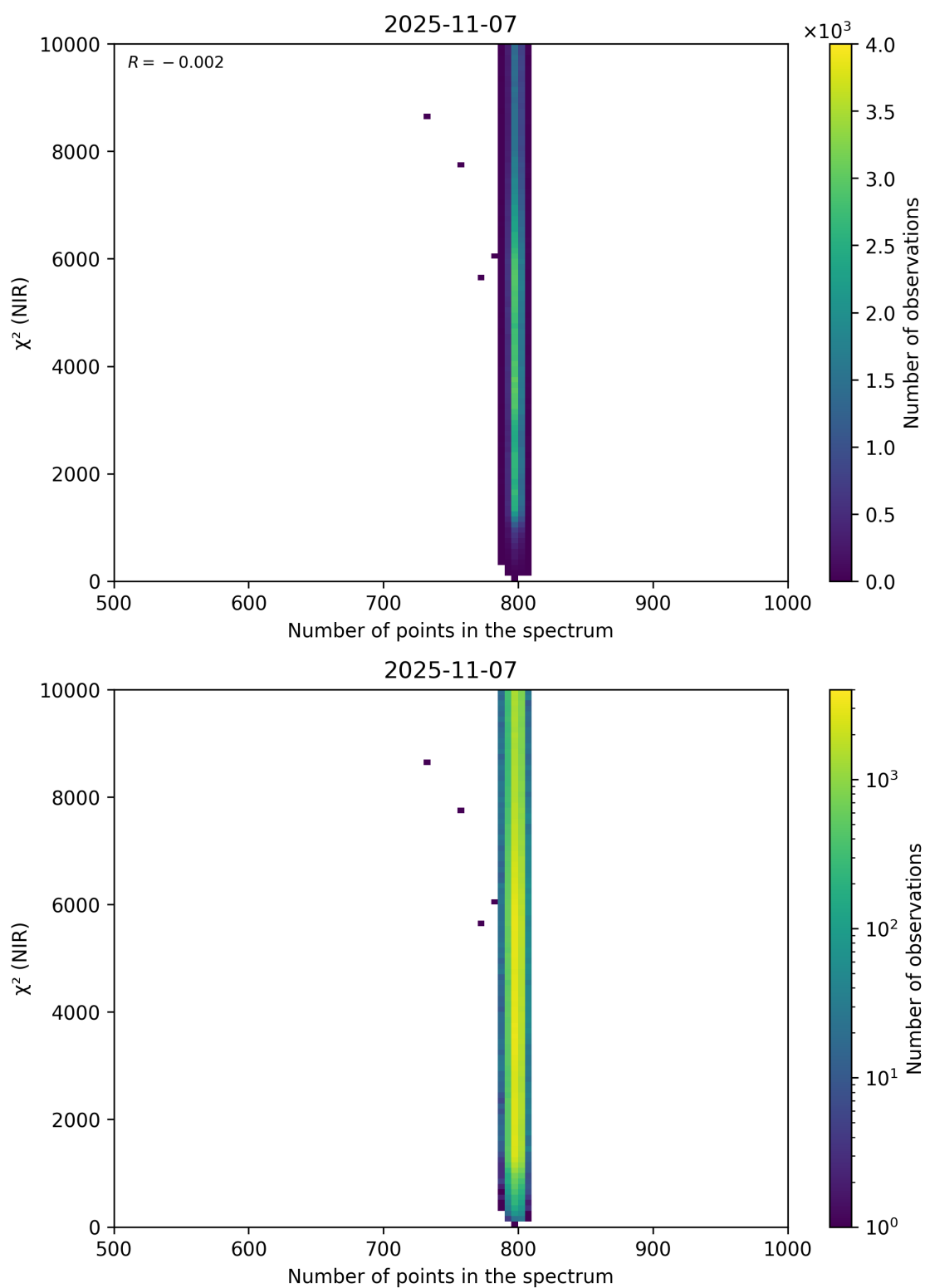
Figure 88: Scatter density plot of “Number of points in the spectrum” against “ \chi^2 (NIR)” for 2025-11-07 to 2025-11-08.
