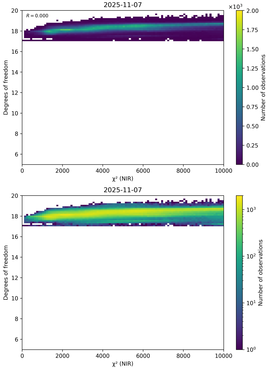
Figure 44: Scatter density plot of “ \chi^2 (NIR)” against “Degrees of freedom” for 2025-11-07 to 2025-11-08.
