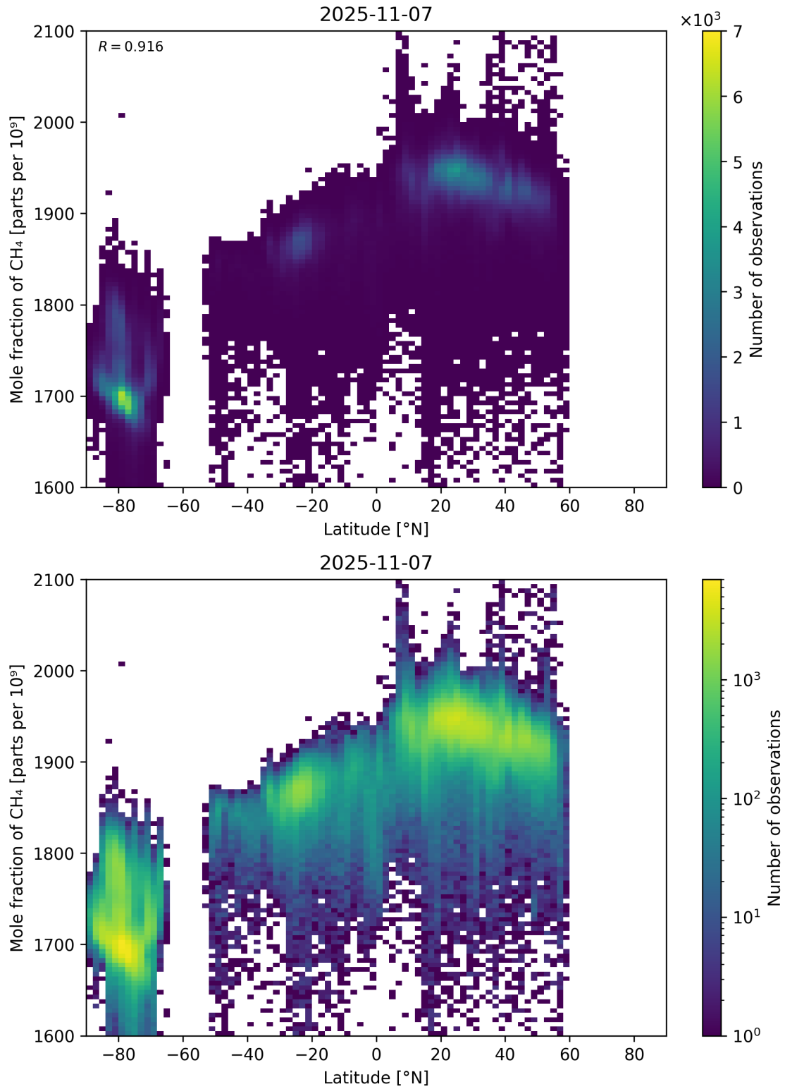
Figure 57: Scatter density plot of “Latitude” against “Mole fraction of CH 4 ” for 2025-11-07 to 2025-11-08.
