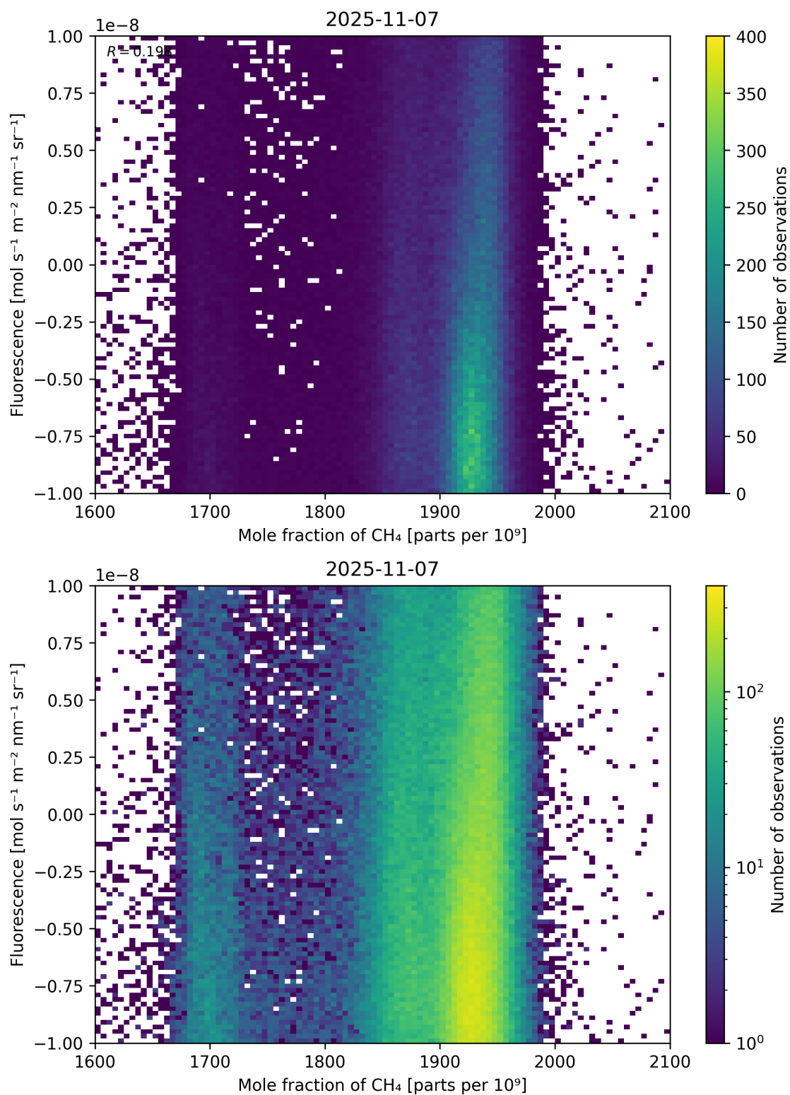
Figure 73: Scatter density plot of “Mole fraction of \text{CH}_4 ” against “Fluorescence” for 2025-11-07 to 2025-11-08.
