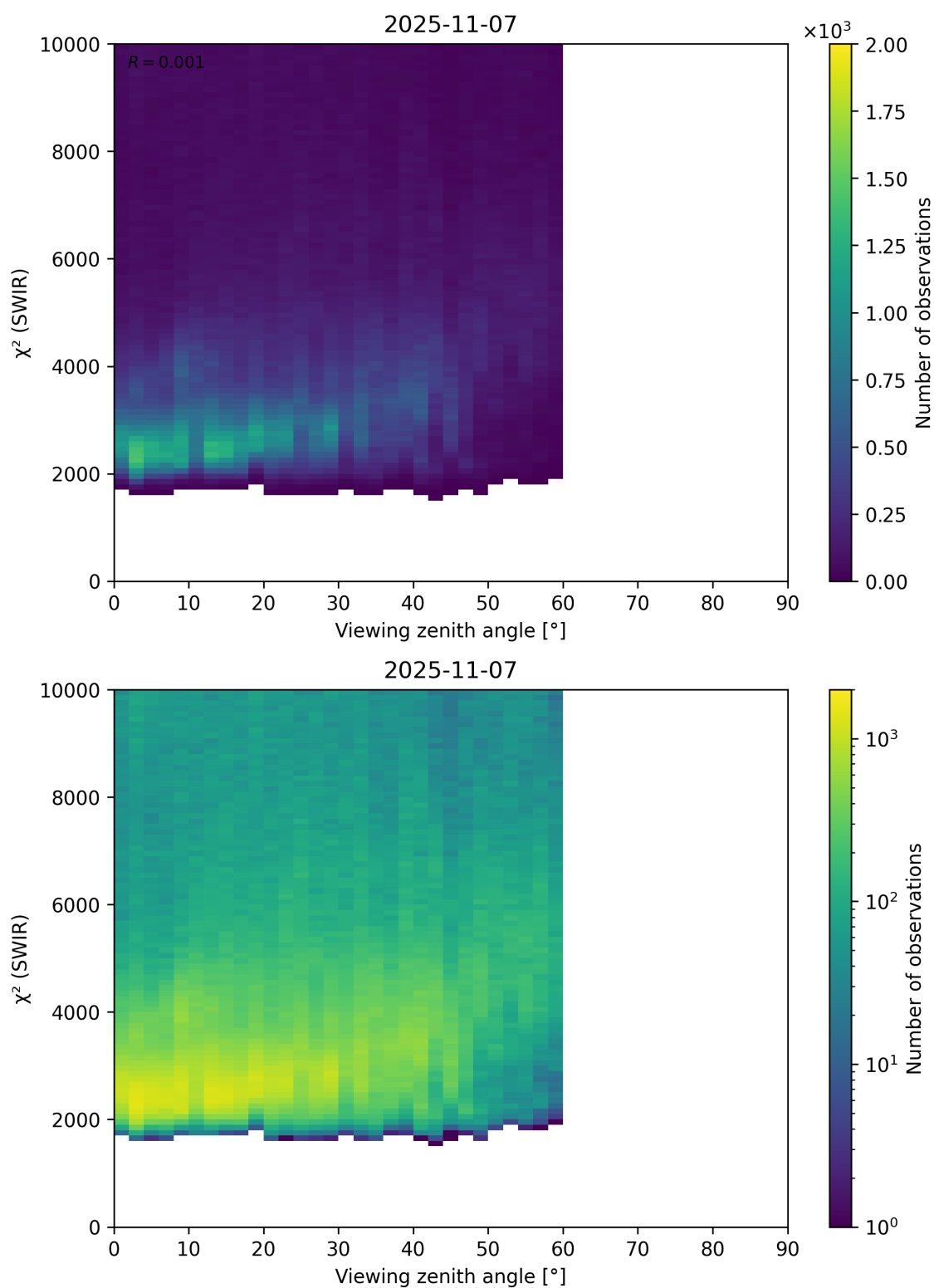
Figure 106: Scatter density plot of “Viewing zenith angle” against “ \chi^2 (SWIR)” for 2025-11-07 to 2025-11-08.
