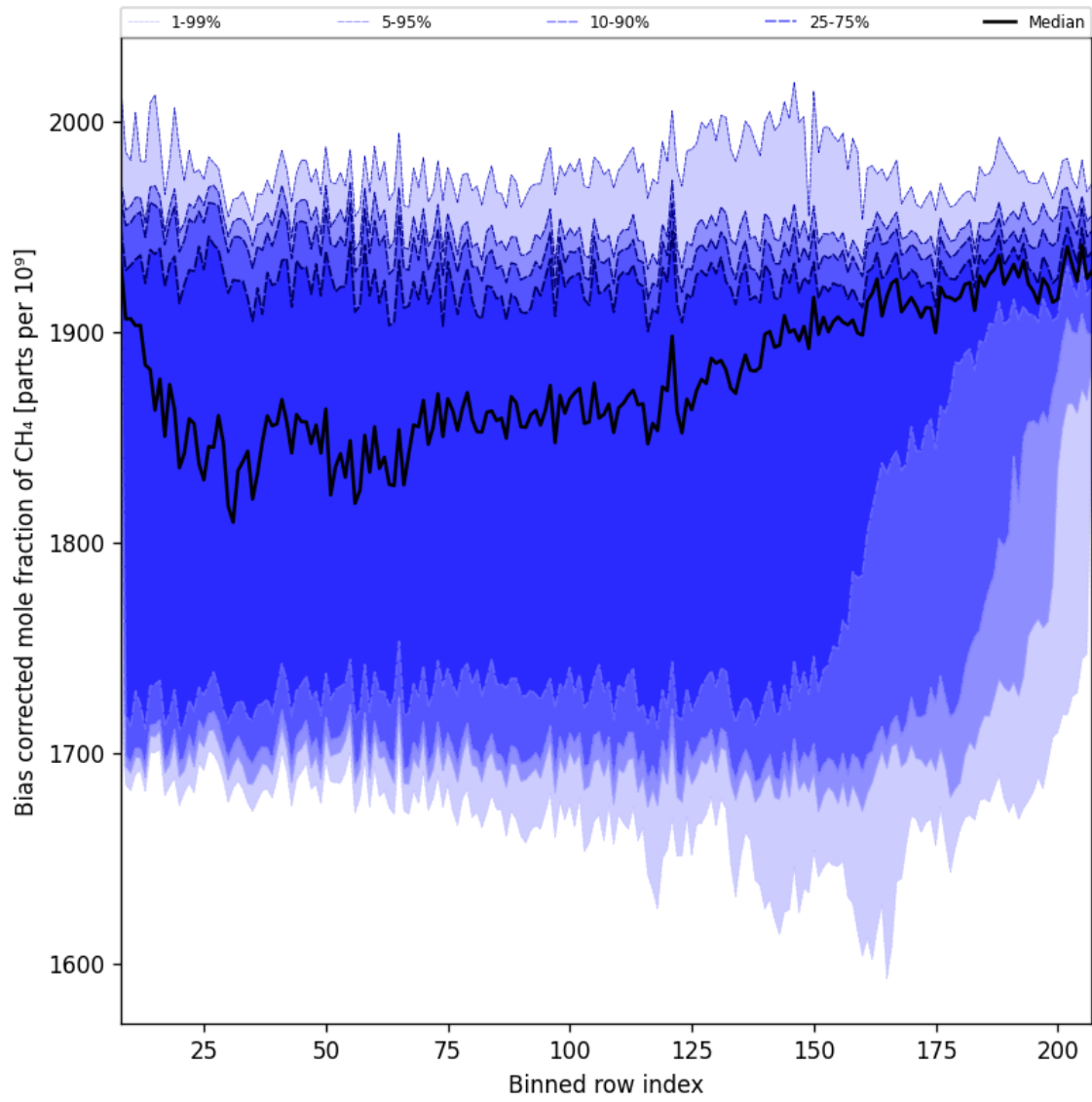
Figure 36: Along track statistics of “Bias corrected mole fraction of CH 4 ” for 2025-11-07 to 2025-11-08
