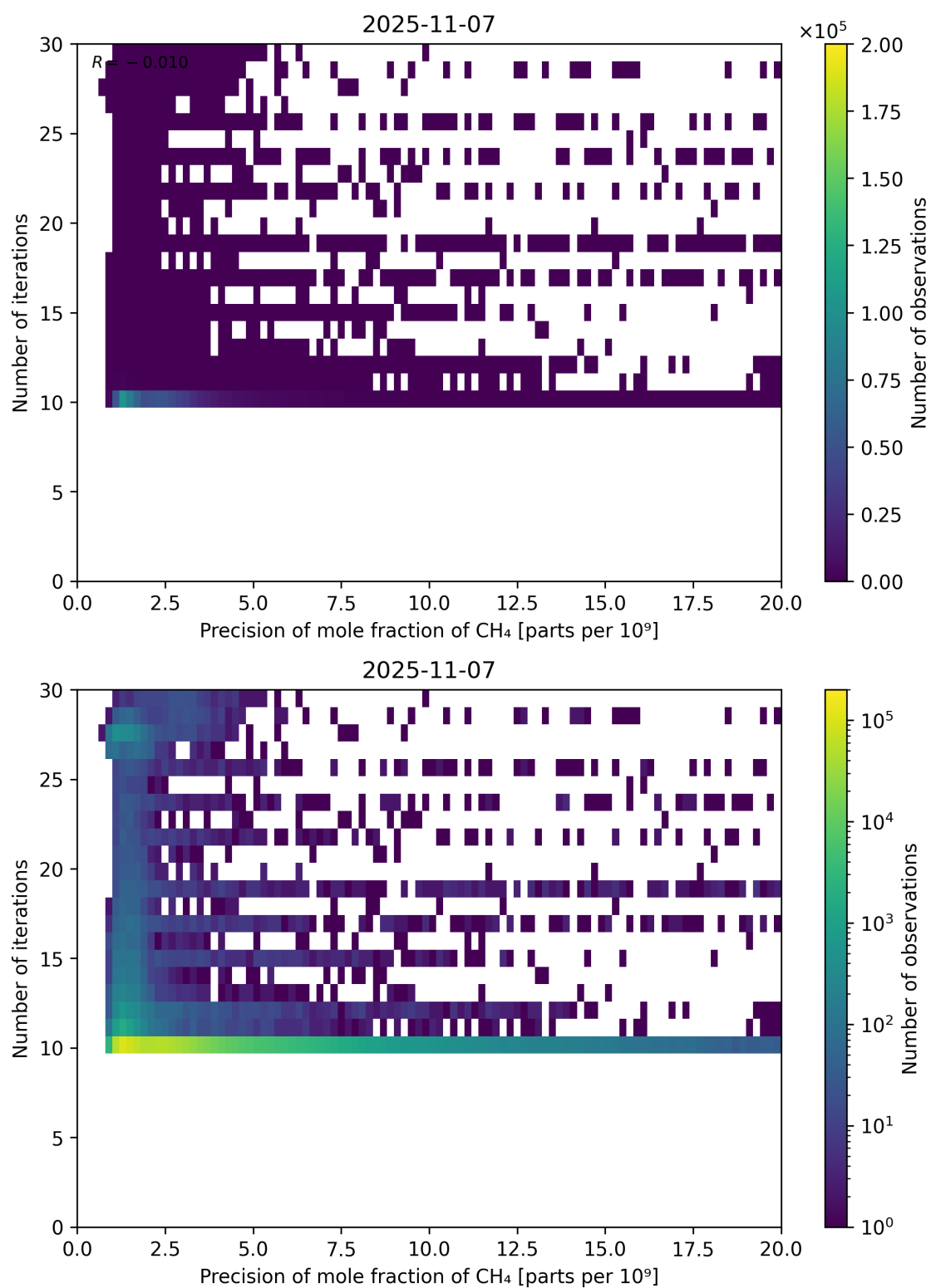
Figure 83: Scatter density plot of “Precision of mole fraction of CH 4 ” against “Number of iterations” for 2025-11-07 to 2025-11-08.
