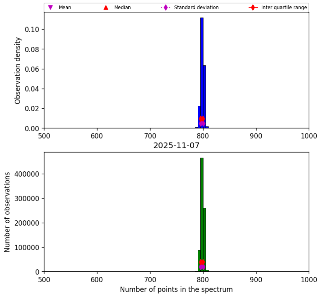
Figure 26: Histogram of “Number of points in the spectrum” for 2025-11-07 to 2025-11-08
