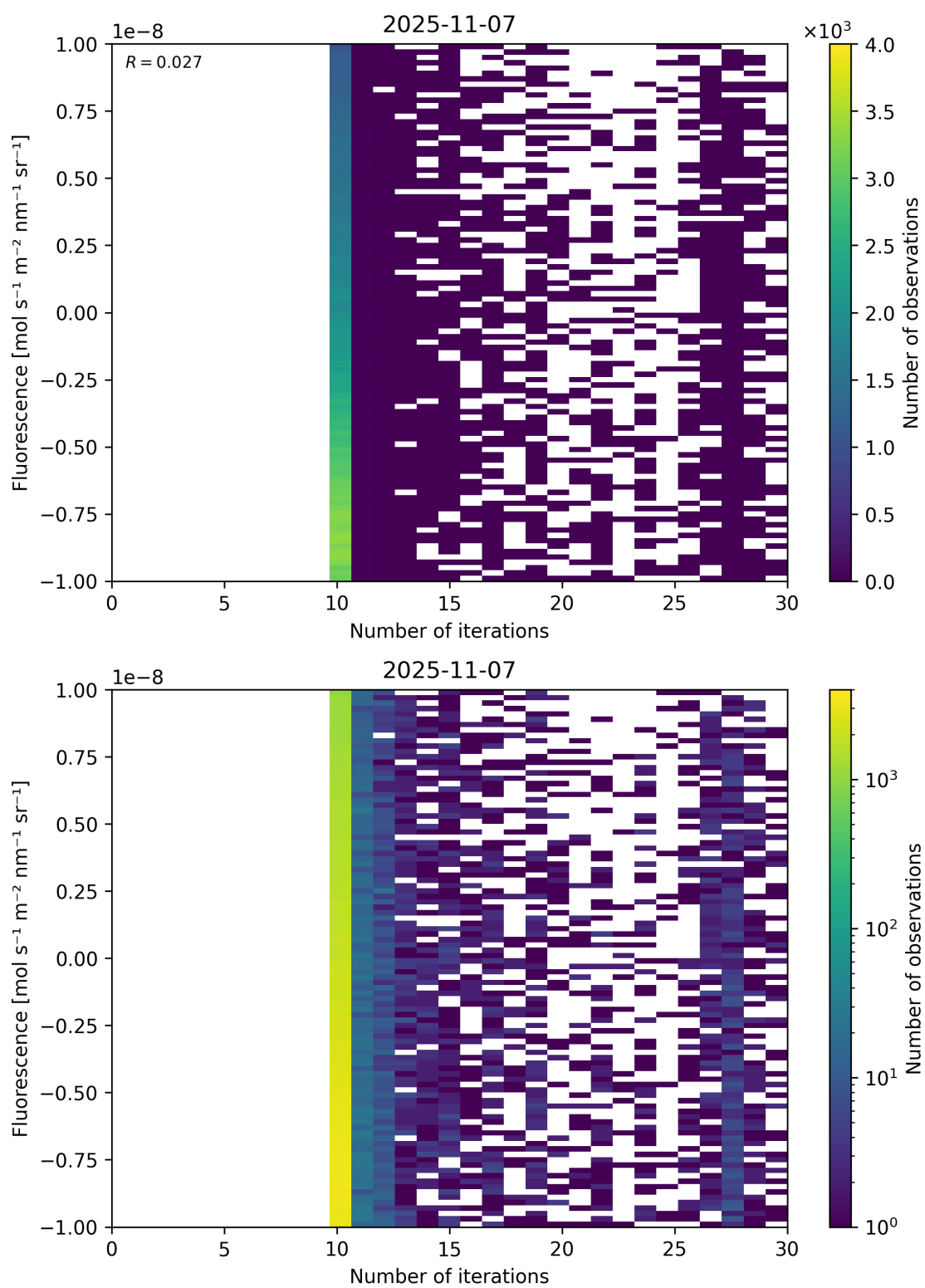
Figure 87: Scatter density plot of “Number of iterations” against “Fluorescence” for 2025-11-07 to 2025-11-08.
