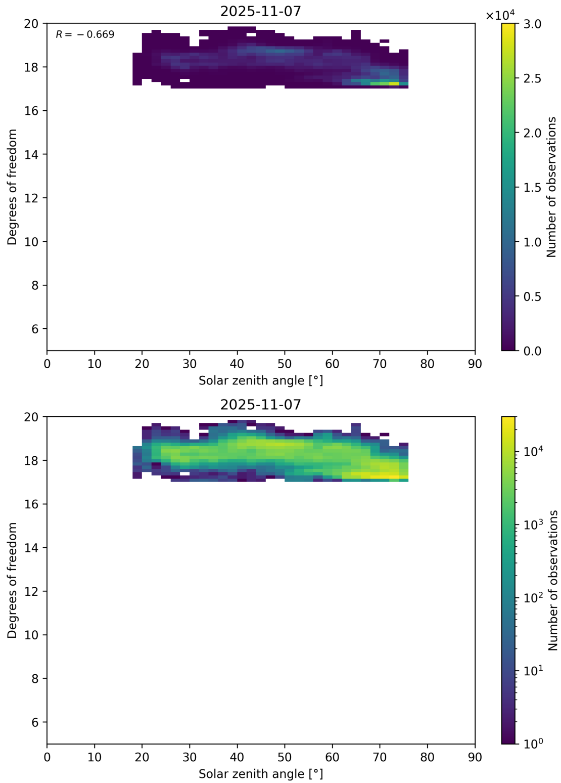
Figure 96: Scatter density plot of “Solar zenith angle” against “Degrees of freedom” for 2025-11-07 to 2025-11-08.
