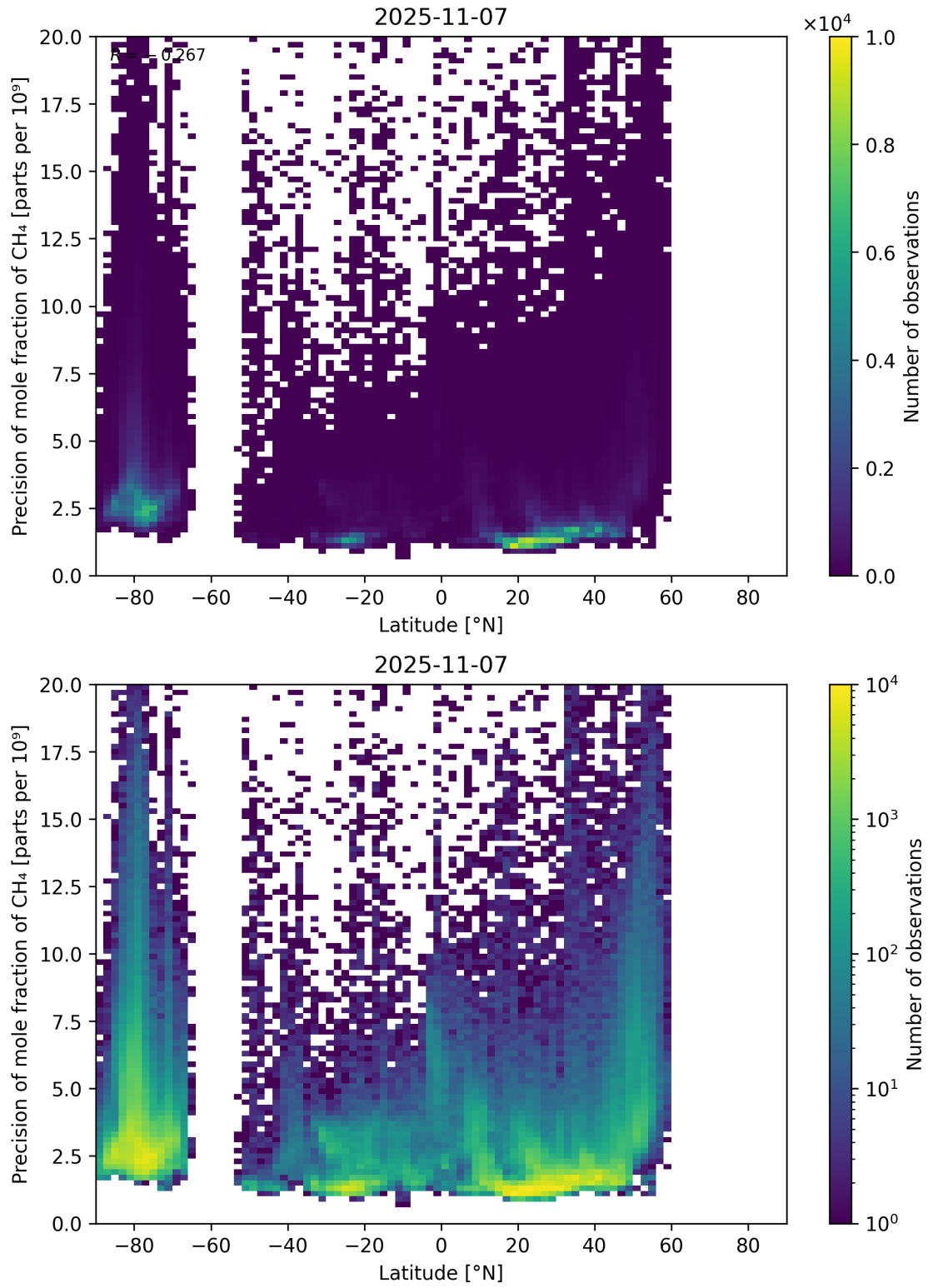
Figure 59: Scatter density plot of “Latitude” against “Precision of mole fraction of CH 4 ” for 2025-11-07 to 2025-11-08.
