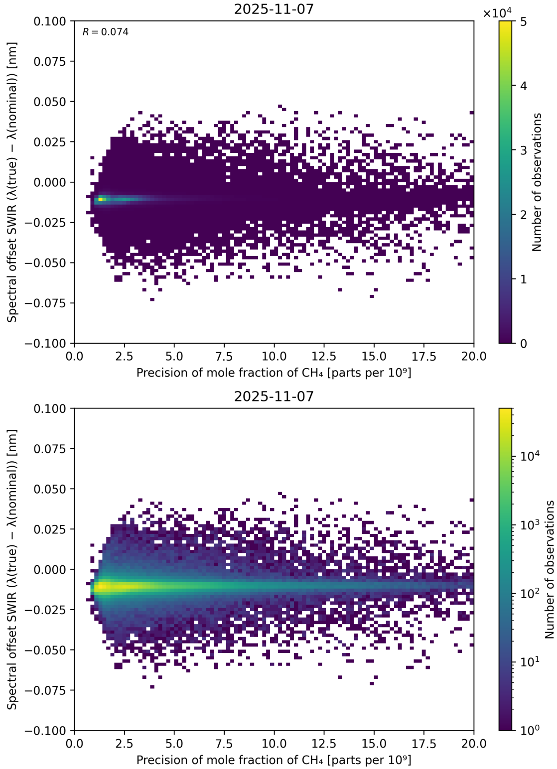
Figure 85: Scatter density plot of “Precision of mole fraction of \text{CH}_4 ” against “Spectral offset SWIR ( \lambda_{\text{true}} - \lambda_{\text{nominal}} )” for 2025-11-07 to 2025-11-08.
