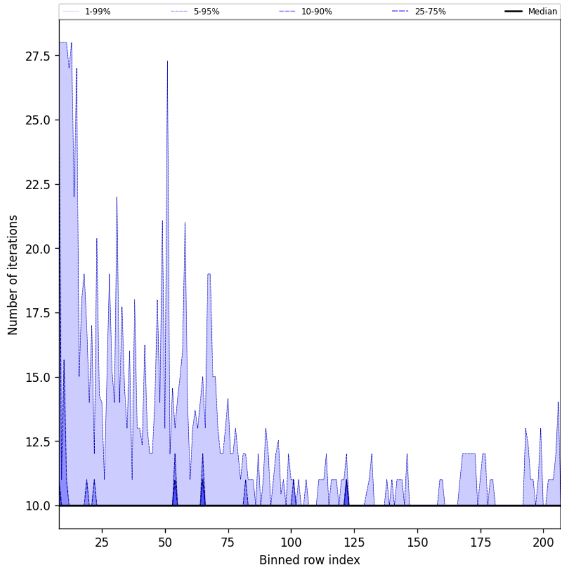
Figure 42: Along track statistics of “Number of iterations” for 2025-11-07 to 2025-11-08
