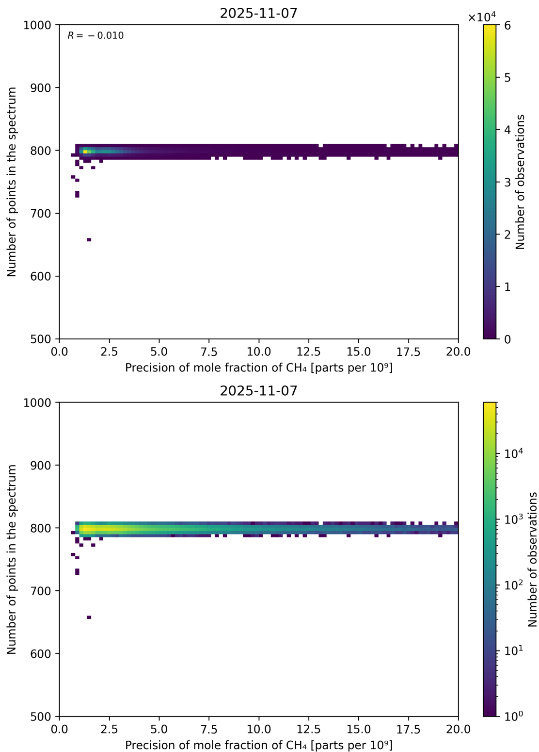
Figure 84: Scatter density plot of “Precision of mole fraction of CH 4 ” against “Number of points in the spectrum” for 2025-11-07 to 2025-11-08.
