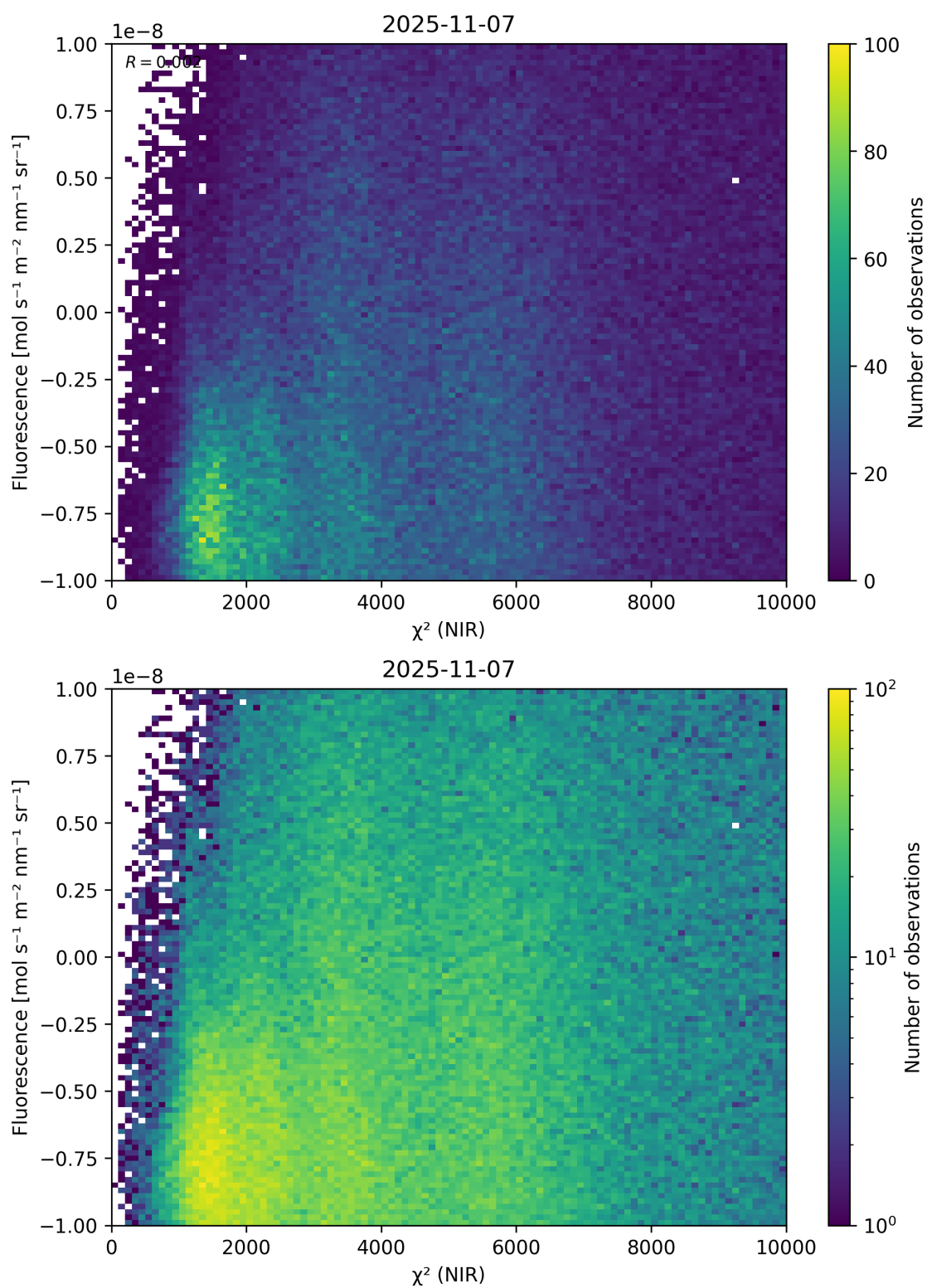
Figure 45: Scatter density plot of “ \chi^2 (NIR)” against “Fluorescence” for 2025-11-07 to 2025-11-08.
