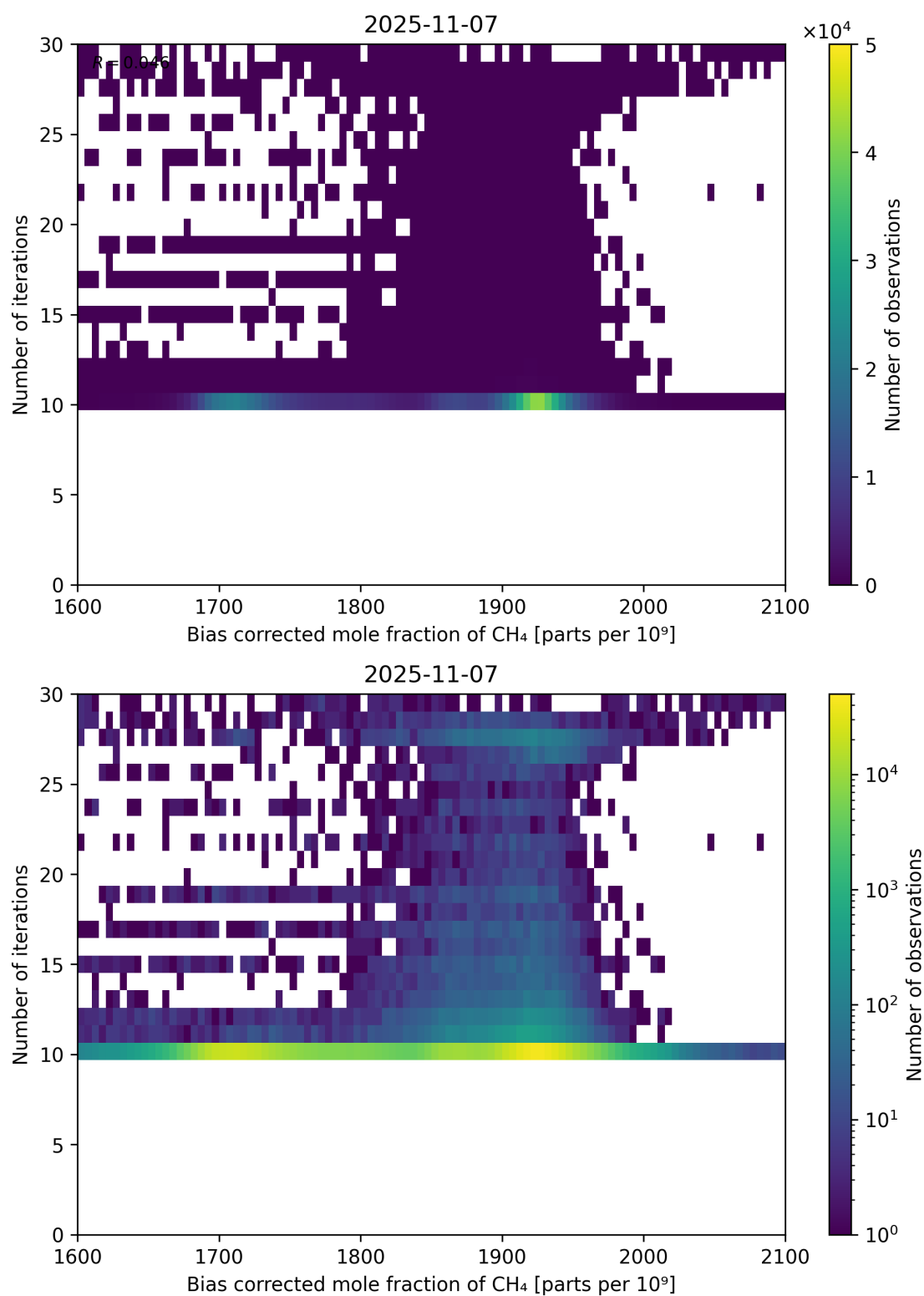
Figure 67: Scatter density plot of “Bias corrected mole fraction of \text{CH}_4 ” against “Number of iterations” for 2025-11-07 to 2025-11-08.
