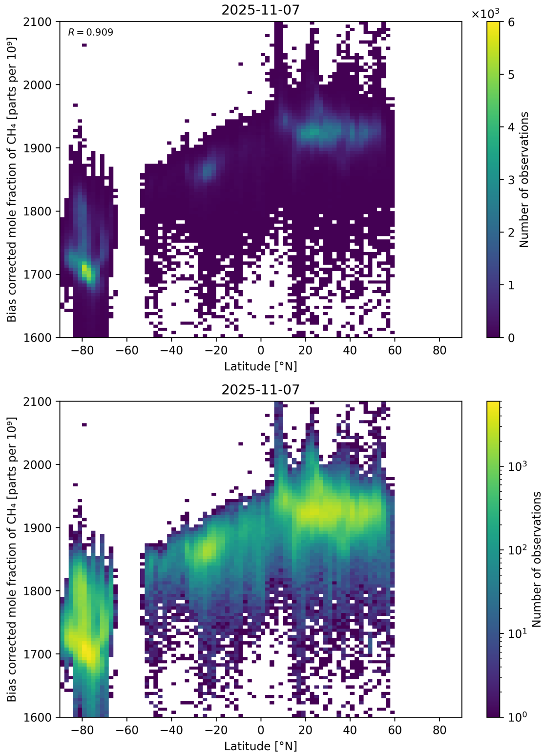
Figure 58: Scatter density plot of “Latitude” against “Bias corrected mole fraction of CH 4 ” for 2025-11-07 to 2025-11-08.
