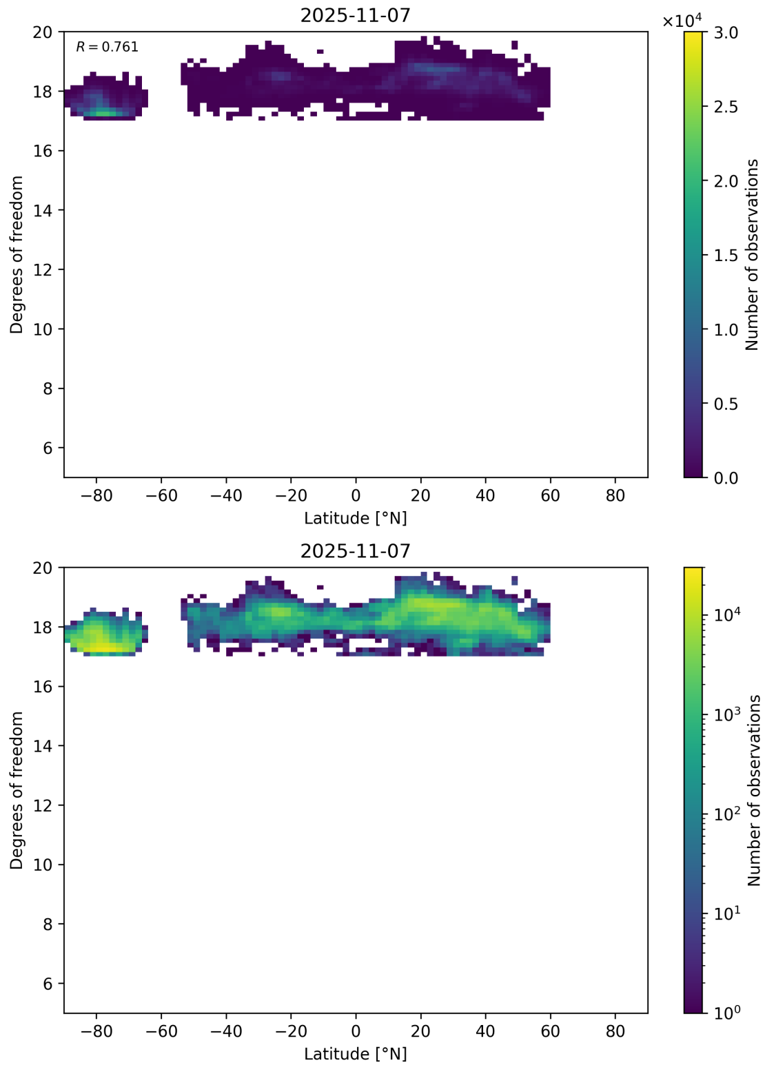
Figure 55: Scatter density plot of “Latitude” against “Degrees of freedom” for 2025-11-07 to 2025-11-08.
