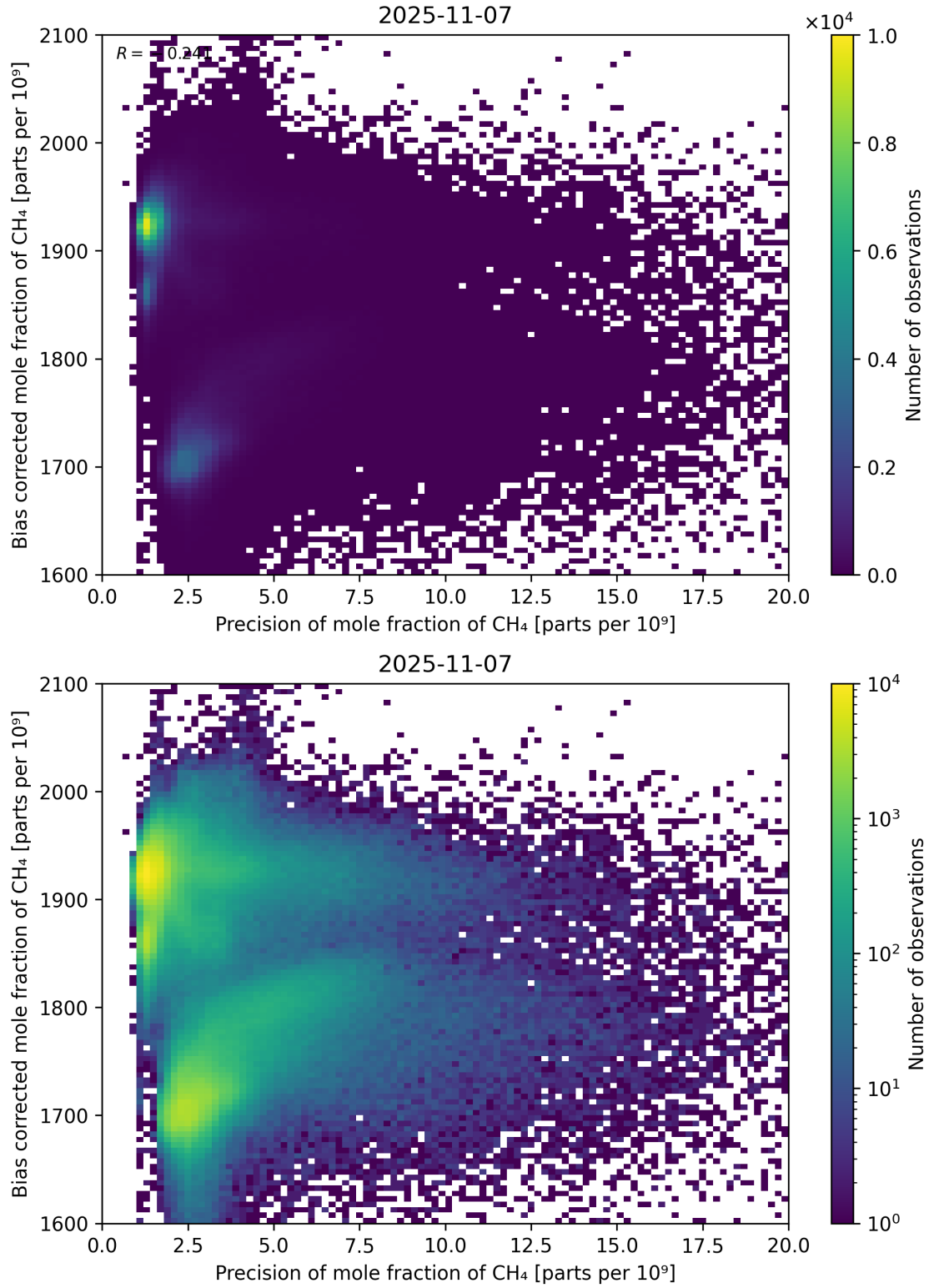
Figure 82: Scatter density plot of “Precision of mole fraction of CH 4 ” against “Bias corrected mole fraction of CH 4 ” for 2025-11-07 to 2025-11-08.
