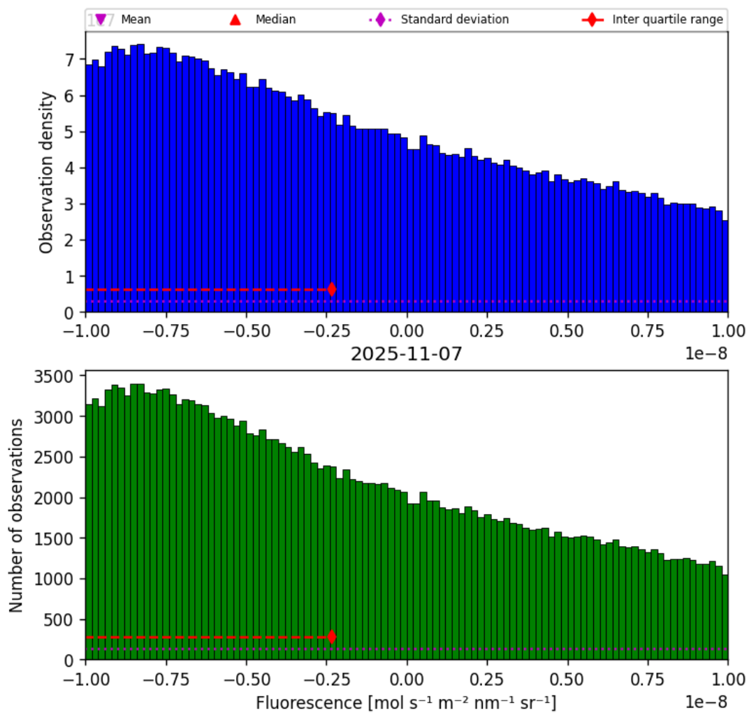
Figure 32: Histogram of “Fluorescence” for 2025-11-07 to 2025-11-08
