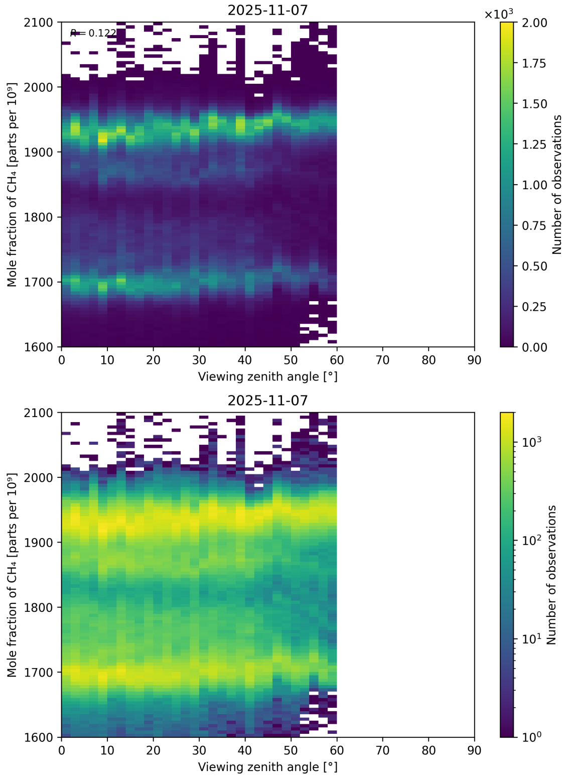
Figure 110: Scatter density plot of “Viewing zenith angle” against “Mole fraction of CH 4 ” for 2025-11-07 to 2025-11-08.
