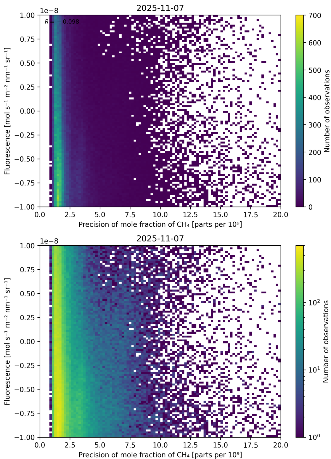
Figure 81: Scatter density plot of “Precision of mole fraction of \text{CH}_4 ” against “Fluorescence” for 2025-11-07 to 2025-11-08.
