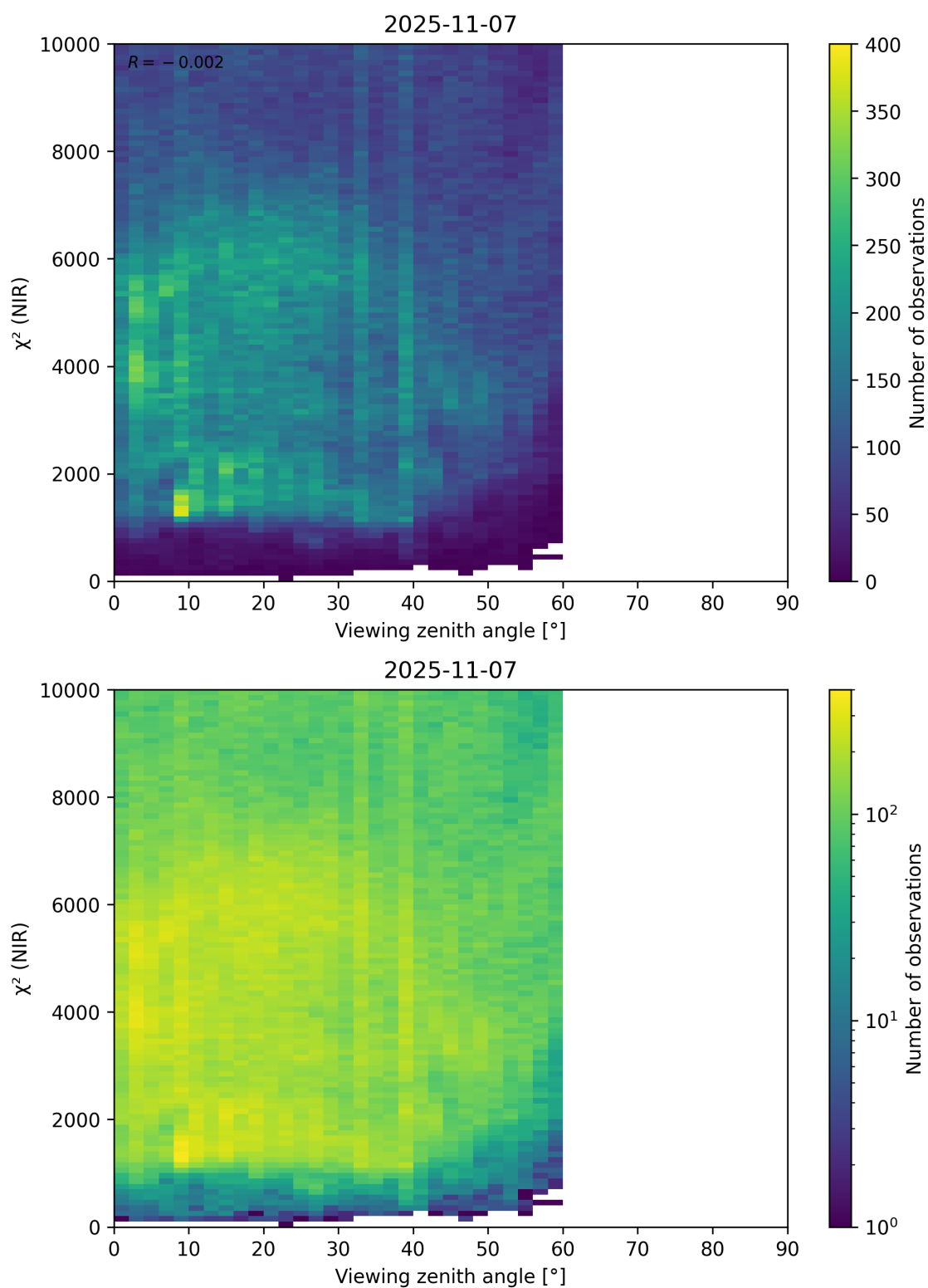
Figure 105: Scatter density plot of “Viewing zenith angle” against “ \chi^2 (NIR)” for 2025-11-07 to 2025-11-08.
