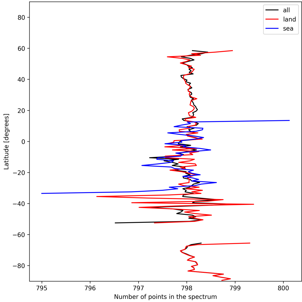
Figure 15: Zonal average of “Number of points in the spectrum” for 2025-11-07 to 2025-11-08.
