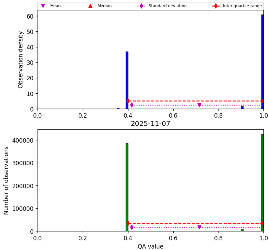
Figure 22: Histogram of “QA value” for 2025-11-07 to 2025-11-08
