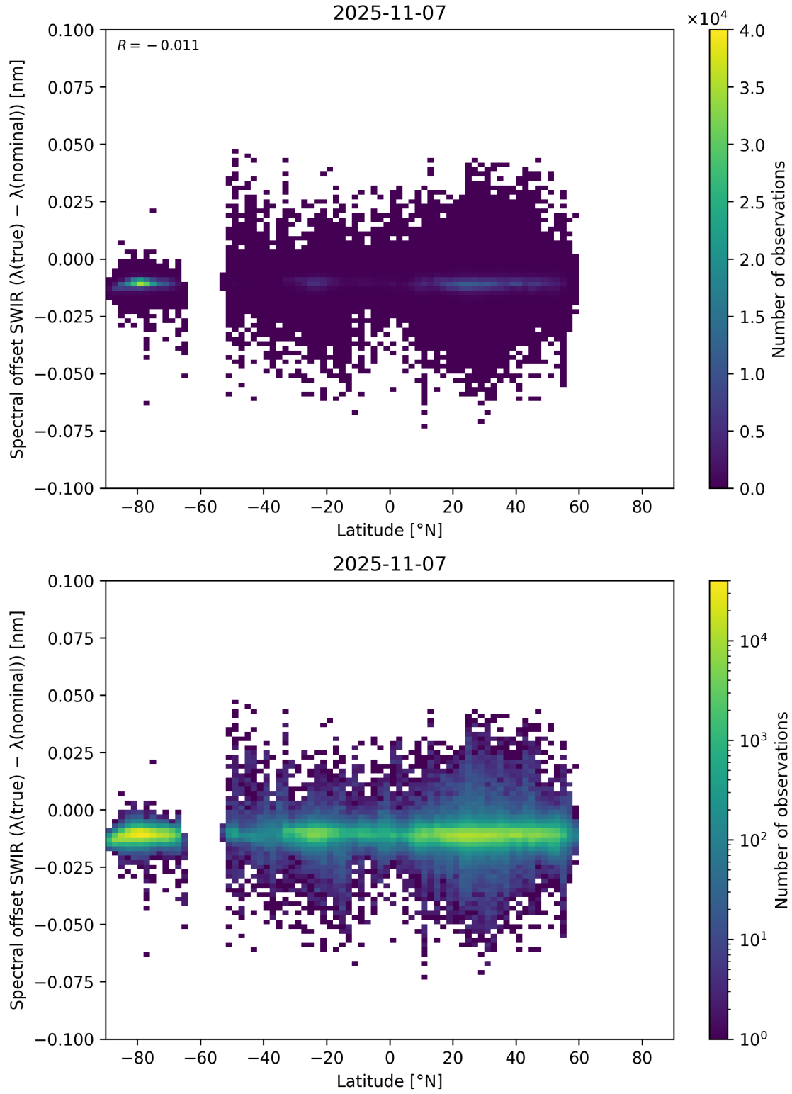
Figure 62: Scatter density plot of “Latitude” against “Spectral offset SWIR ( \lambda_{\text{true}} - \lambda_{\text{nominal}} )” for 2025-11-07 to 2025-11-08.
