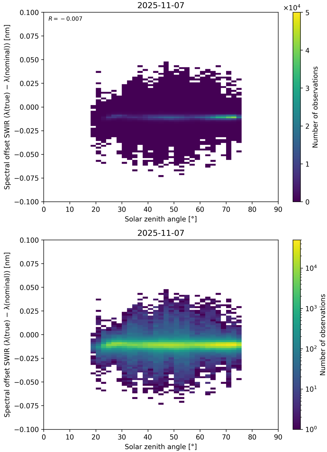
Figure 104: Scatter density plot of “Solar zenith angle” against “Spectral offset SWIR ( \lambda_{\text{true}} - \lambda_{\text{nominal}} )” for 2025-11-07 to 2025-11-08.
