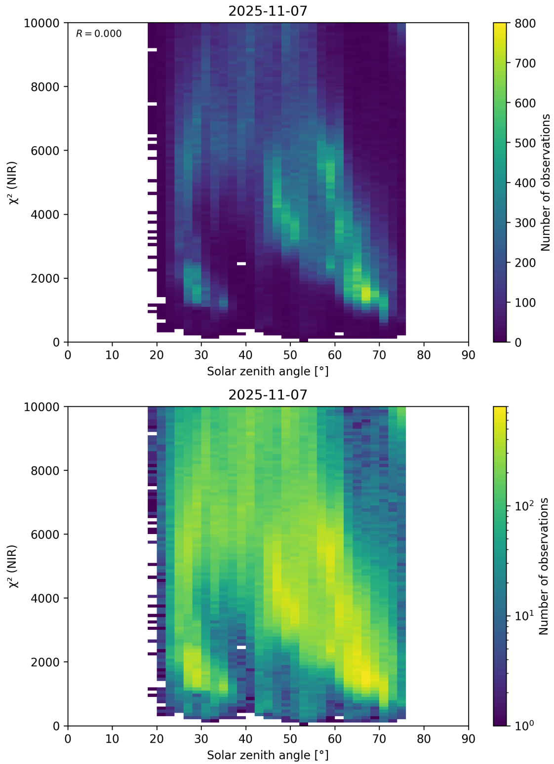
Figure 94: Scatter density plot of “Solar zenith angle” against “ \chi^2 (NIR)” for 2025-11-07 to 2025-11-08.
