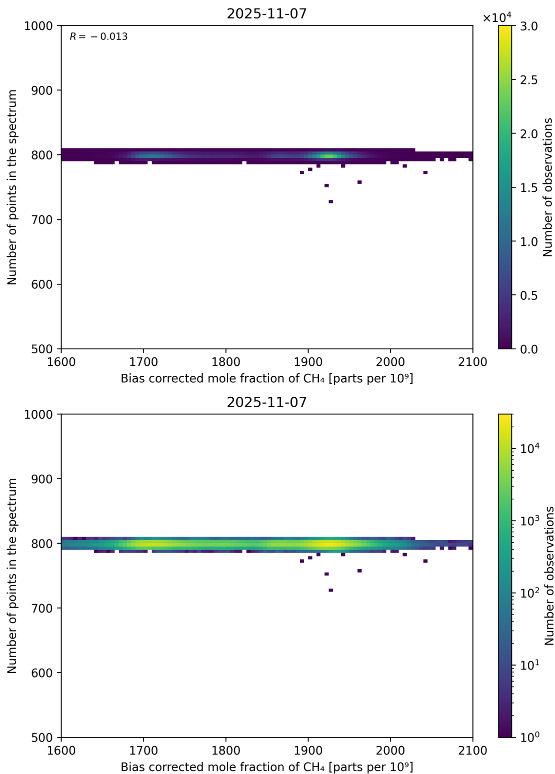
Figure 68: Scatter density plot of “Bias corrected mole fraction of CH 4 ” against “Number of points in the spectrum” for 2025-11-07 to 2025-11-08.
