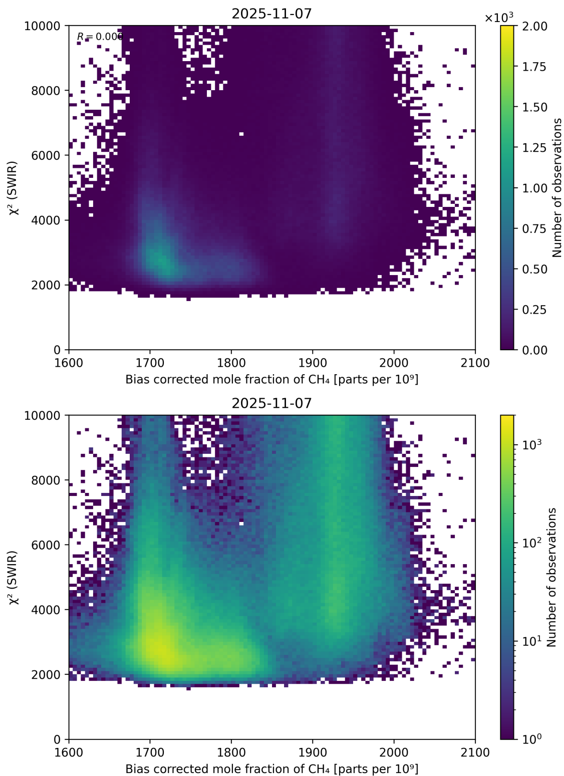
Figure 64: Scatter density plot of “Bias corrected mole fraction of \text{CH}_4 ” against “ \chi^2 (SWIR)” for 2025-11-07 to 2025-11-08.
