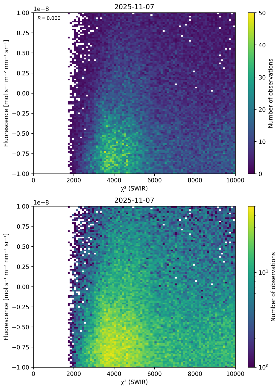
Figure 49: Scatter density plot of “ \chi^2 (SWIR)” against “Fluorescence” for 2025-11-07 to 2025-11-08.
