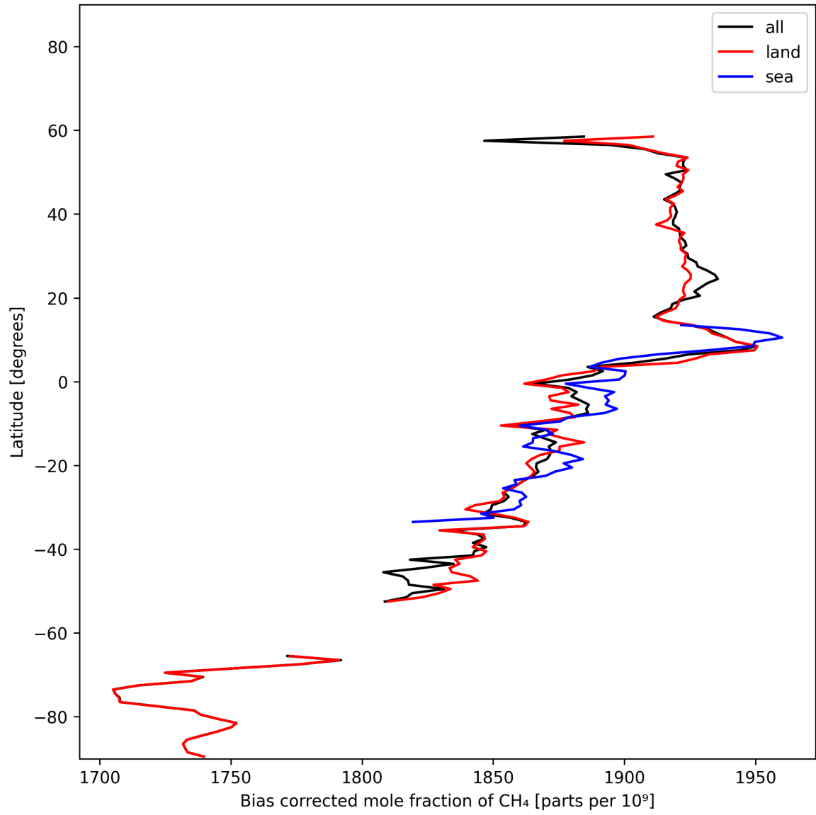
Figure 14: Zonal average of “Bias corrected mole fraction of CH 4 ” for 2025-11-07 to 2025-11-08.
