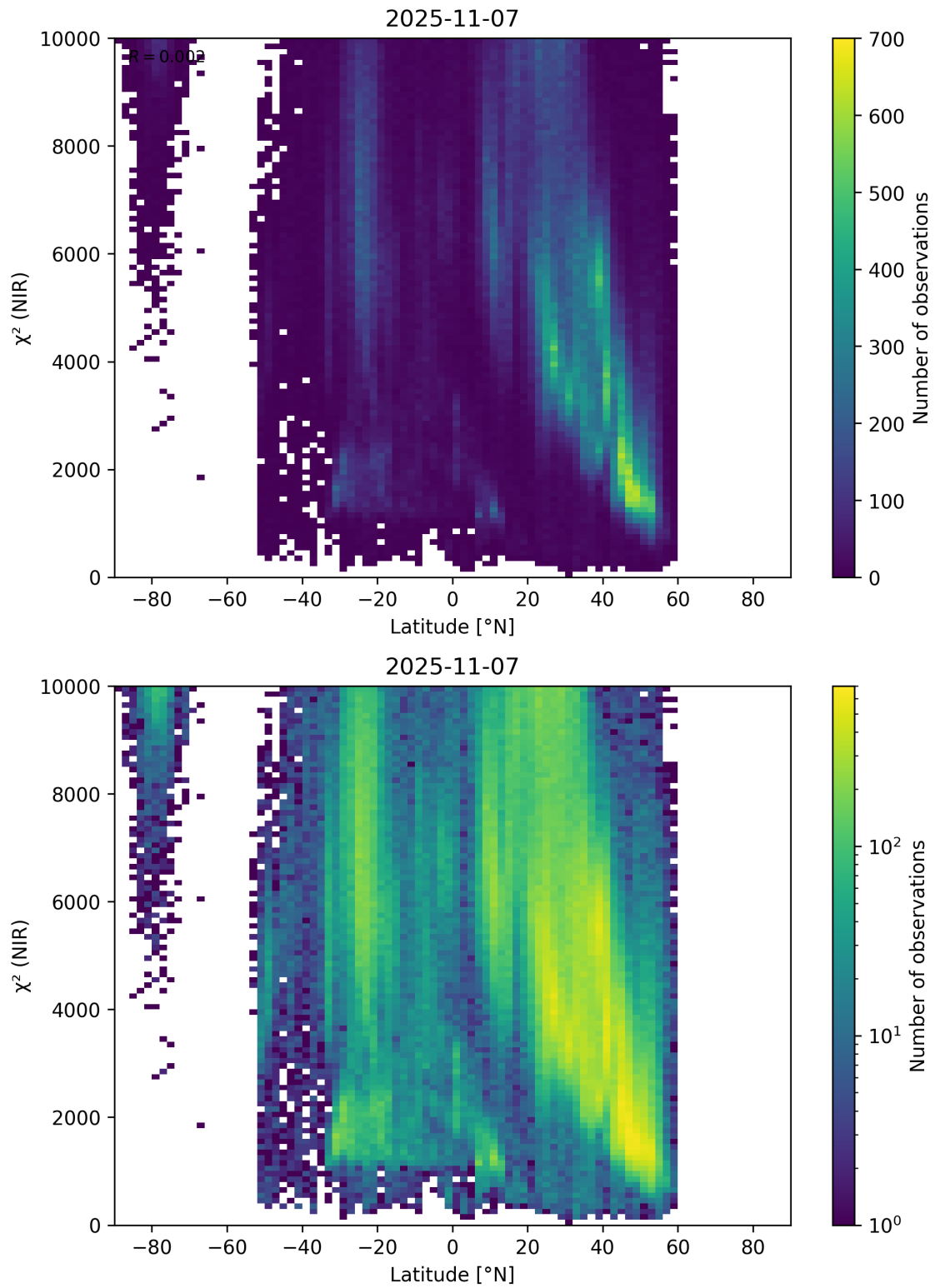
Figure 53: Scatter density plot of “Latitude” against “ \chi^2 (NIR)” for 2025-11-07 to 2025-11-08.
