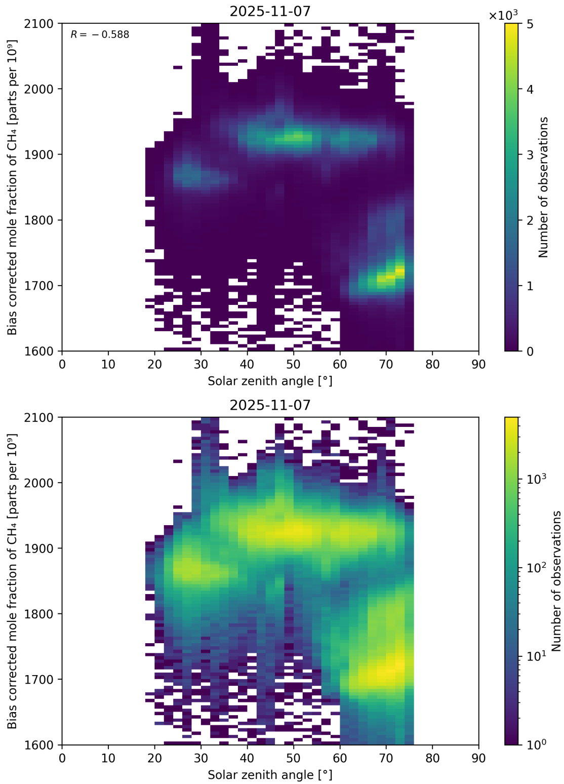
Figure 100: Scatter density plot of “Solar zenith angle” against “Bias corrected mole fraction of CH 4 ” for 2025-11-07 to 2025-11-08.
