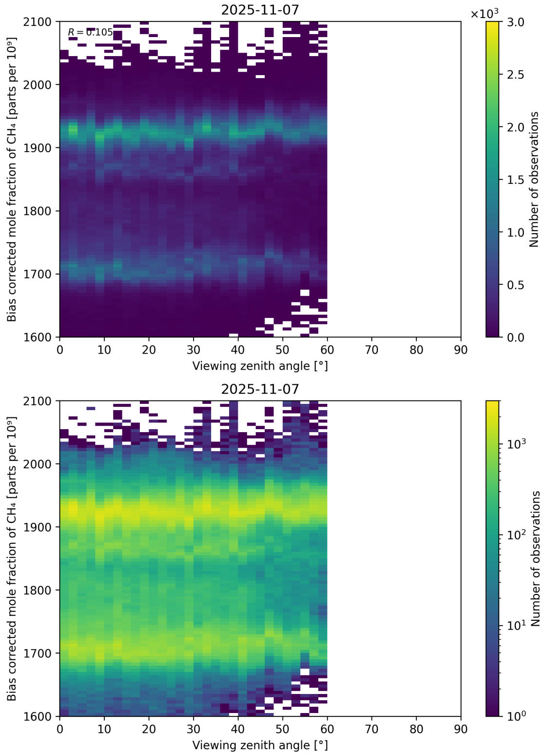
Figure 111: Scatter density plot of “Viewing zenith angle” against “Bias corrected mole fraction of CH 4 ” for 2025-11-07 to 2025-11-08.
