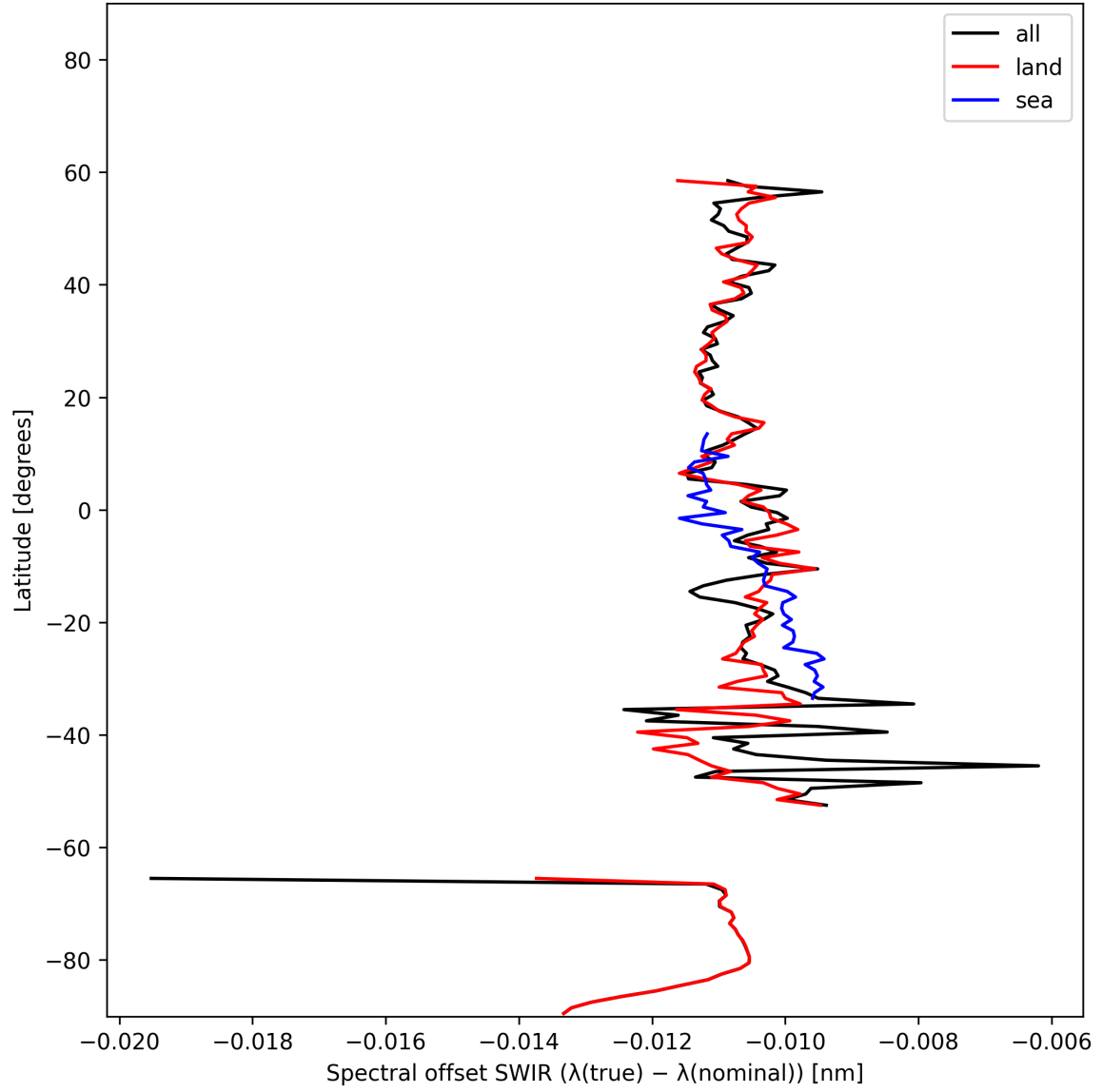
Figure 16: Zonal average of “Spectral offset SWIR ( \lambda_{\text{true}} - \lambda_{\text{nominal}} )” for 2025-11-07 to 2025-11-08.
