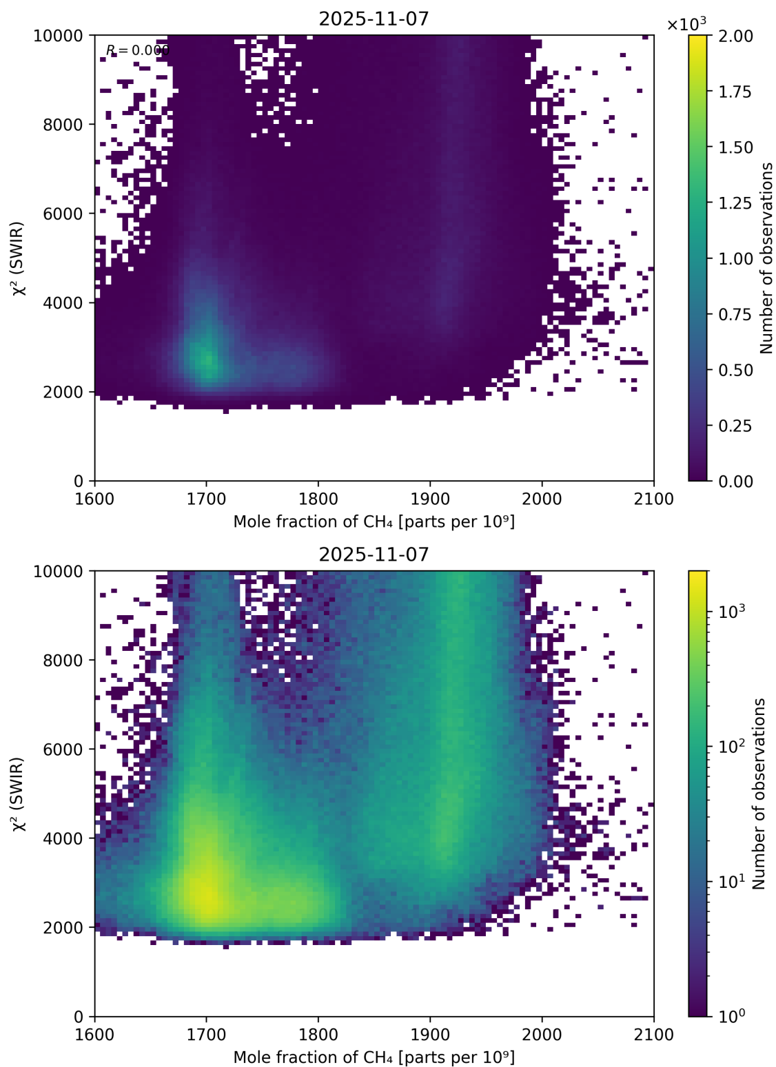
Figure 71: Scatter density plot of “Mole fraction of \text{CH}_4 ” against “ \chi^2 (SWIR)” for 2025-11-07 to 2025-11-08.
