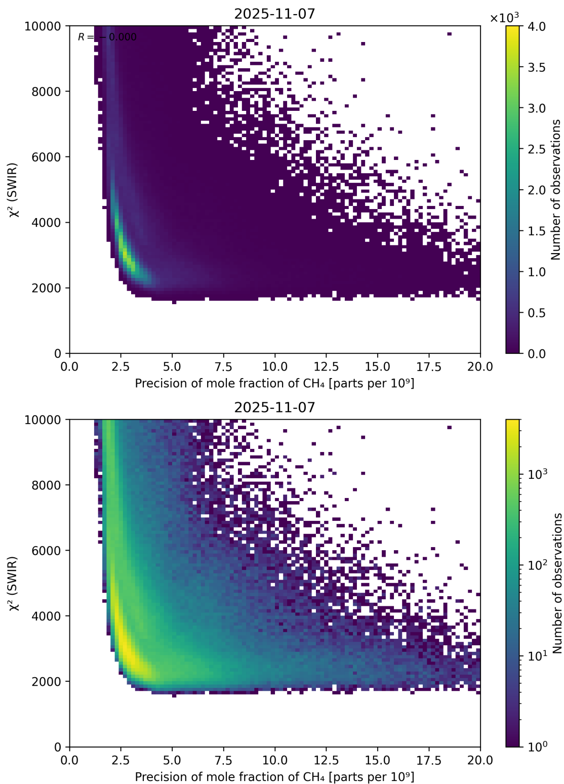
Figure 79: Scatter density plot of “Precision of mole fraction of \text{CH}_4 ” against “ \chi^2 (SWIR)” for 2025-11-07 to 2025-11-08.
