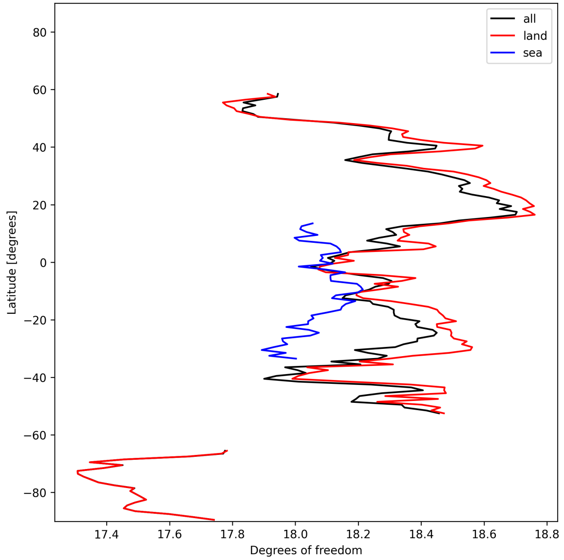
Figure 19: Zonal average of “Degrees of freedom” for 2025-11-07 to 2025-11-08.
