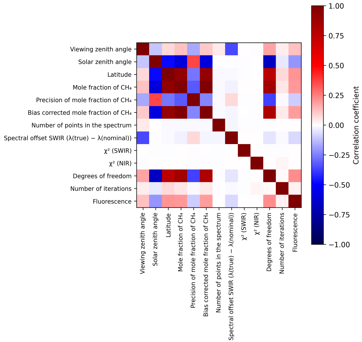
Figure 2: Map of correlation matrix for 2025-11-07 to 2025-11-08.
