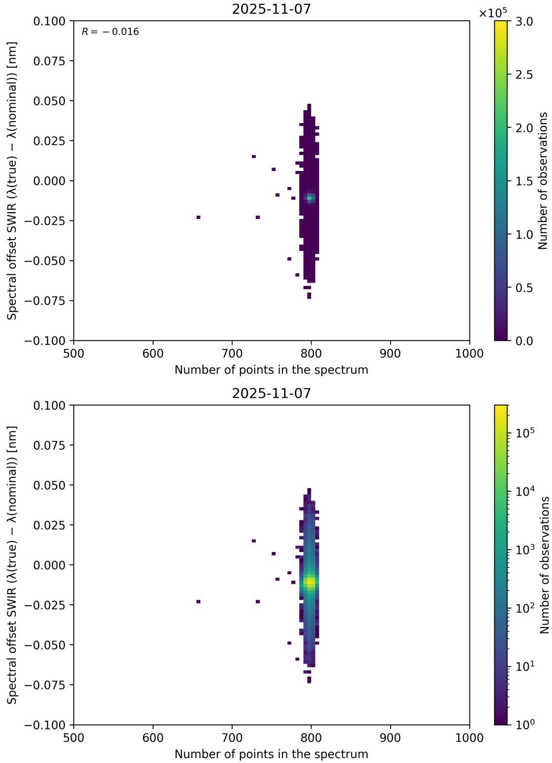
Figure 93: Scatter density plot of “Number of points in the spectrum” against “Spectral offset SWIR ( \lambda_{\text{true}} - \lambda_{\text{nominal}} )” for 2025-11-07 to 2025-11-08.
