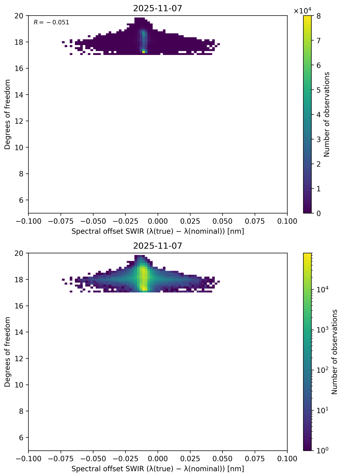
Figure 119: Scatter density plot of “Spectral offset SWIR ( \lambda_{\text{true}} - \lambda_{\text{nominal}} )” against “Degrees of freedom” for 2025-11-07 to 2025-11-08.
