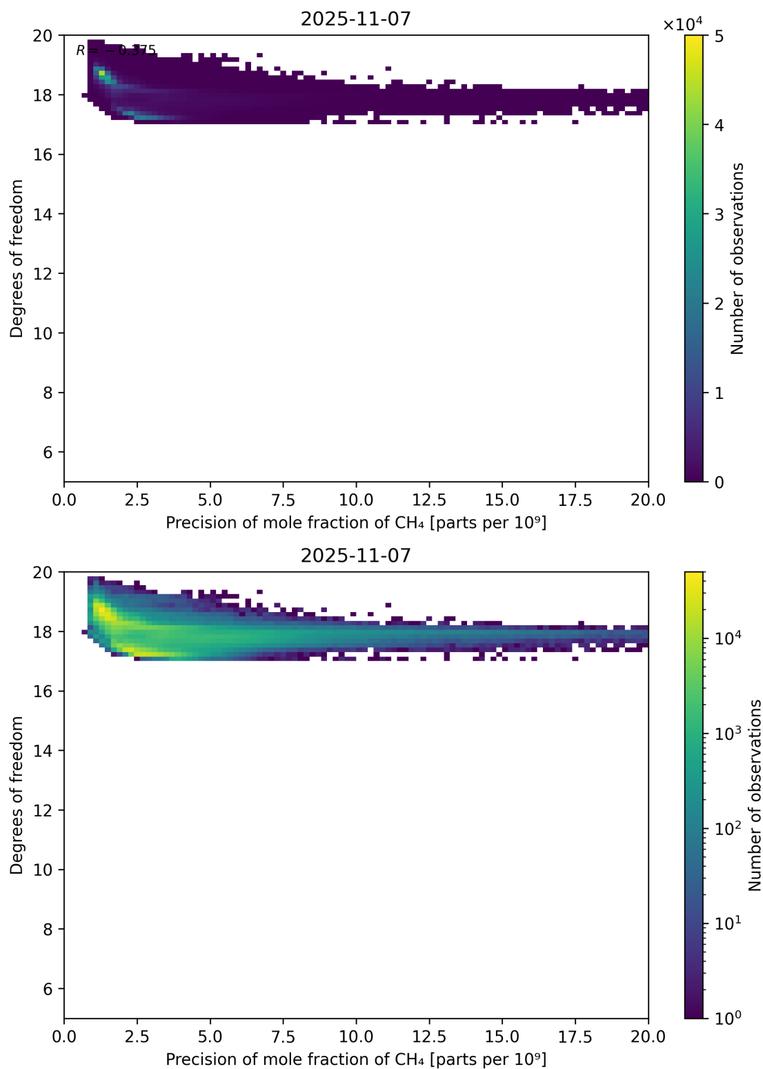
Figure 80: Scatter density plot of “Precision of mole fraction of CH 4 ” against “Degrees of freedom” for 2025-11-07 to 2025-11-08.
