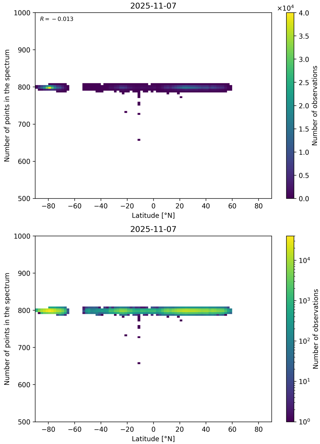
Figure 61: Scatter density plot of “Latitude” against “Number of points in the spectrum” for 2025-11-07 to 2025-11-08.
