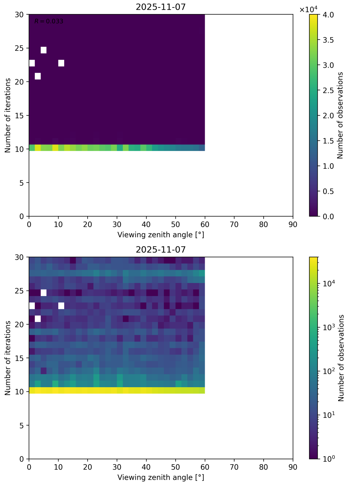
Figure 113: Scatter density plot of “Viewing zenith angle” against “Number of iterations” for 2025-11-07 to 2025-11-08.
