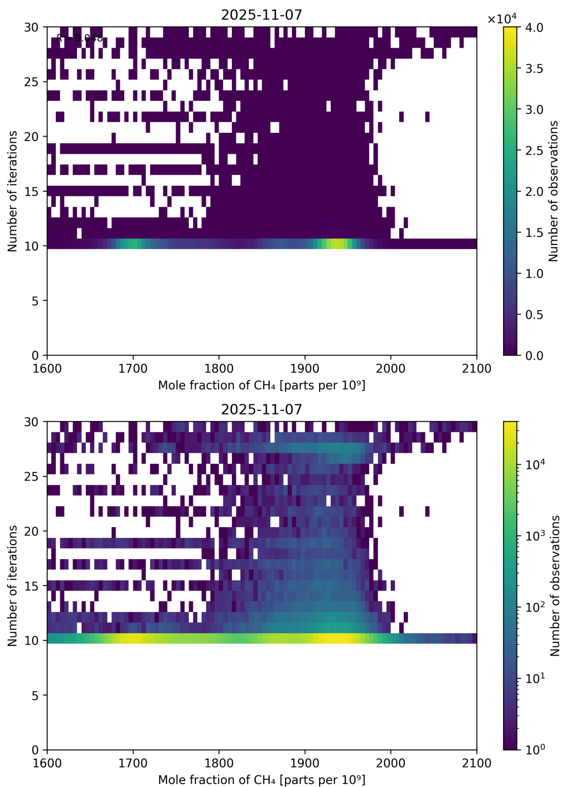
Figure 76: Scatter density plot of “Mole fraction of CH 4 ” against “Number of iterations” for 2025-11-07 to 2025-11-08.
