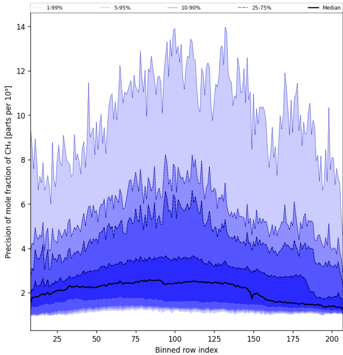
Figure 35: Along track statistics of “Precision of mole fraction of CH 4 ” for 2025-11-07 to 2025-11-08
