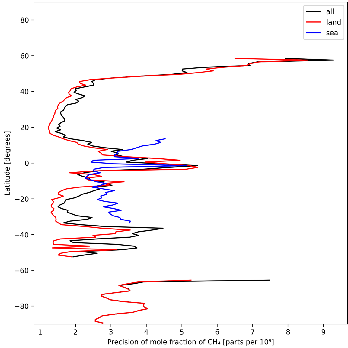
Figure 13: Zonal average of “Precision of mole fraction of CH 4 ” for 2025-11-07 to 2025-11-08.
