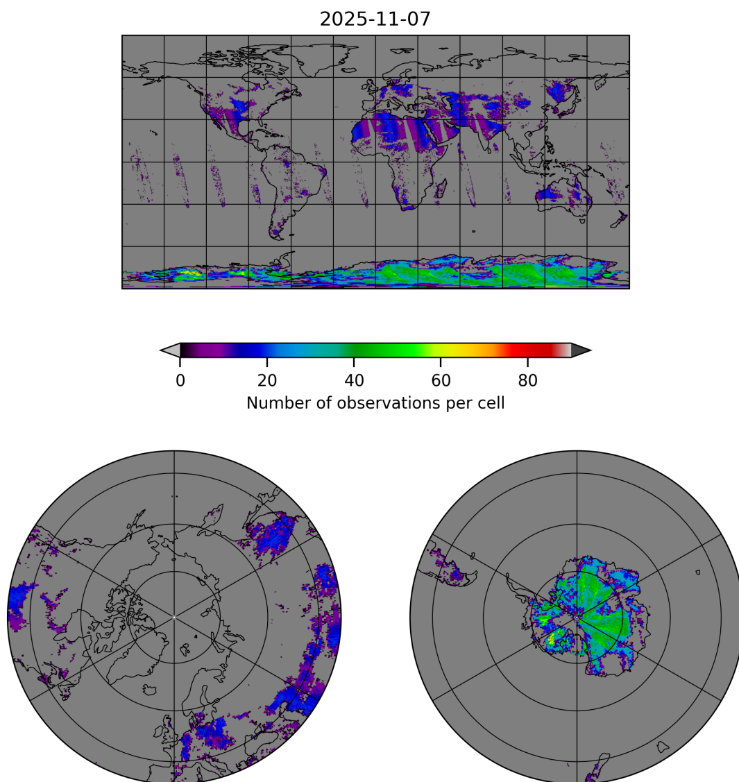
Figure 10: Map of the number of observations for 2025-11-07 to 2025-11-08
