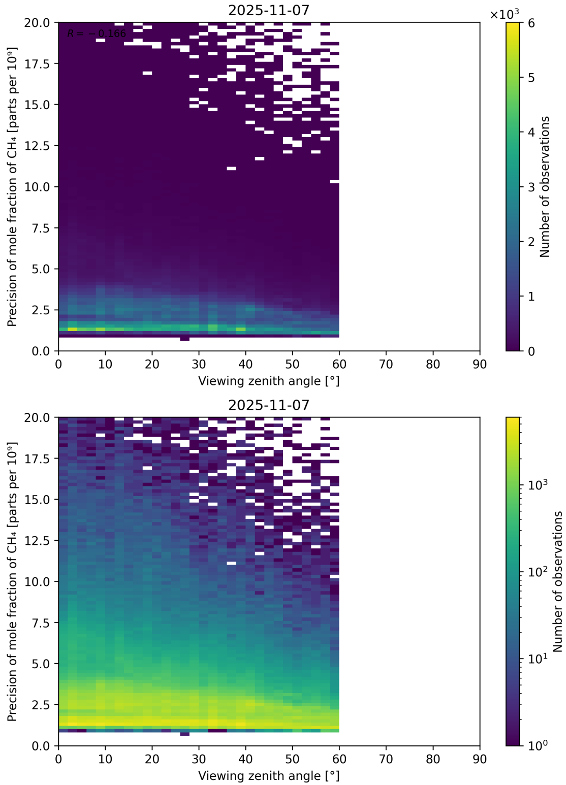
Figure 112: Scatter density plot of “Viewing zenith angle” against “Precision of mole fraction of CH 4 ” for 2025-11-07 to 2025-11-08.
