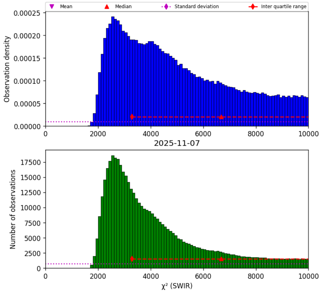
Figure 28: Histogram of “ \chi^2 (SWIR)” for 2025-11-07 to 2025-11-08
