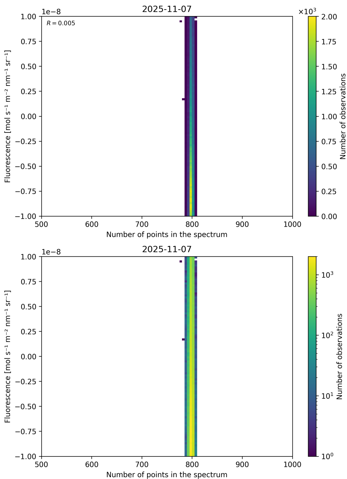
Figure 91: Scatter density plot of “Number of points in the spectrum” against “Fluorescence” for 2025-11-07 to 2025-11-08.
