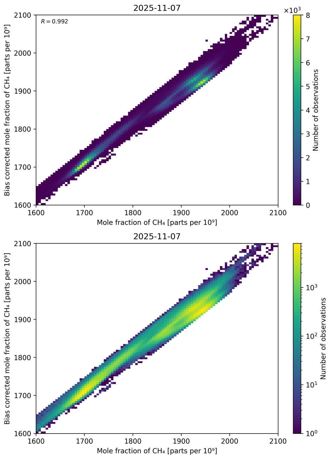
Figure 74: Scatter density plot of “Mole fraction of CH 4 ” against “Bias corrected mole fraction of CH 4 ” for 2025-11-07 to 2025-11-08.
