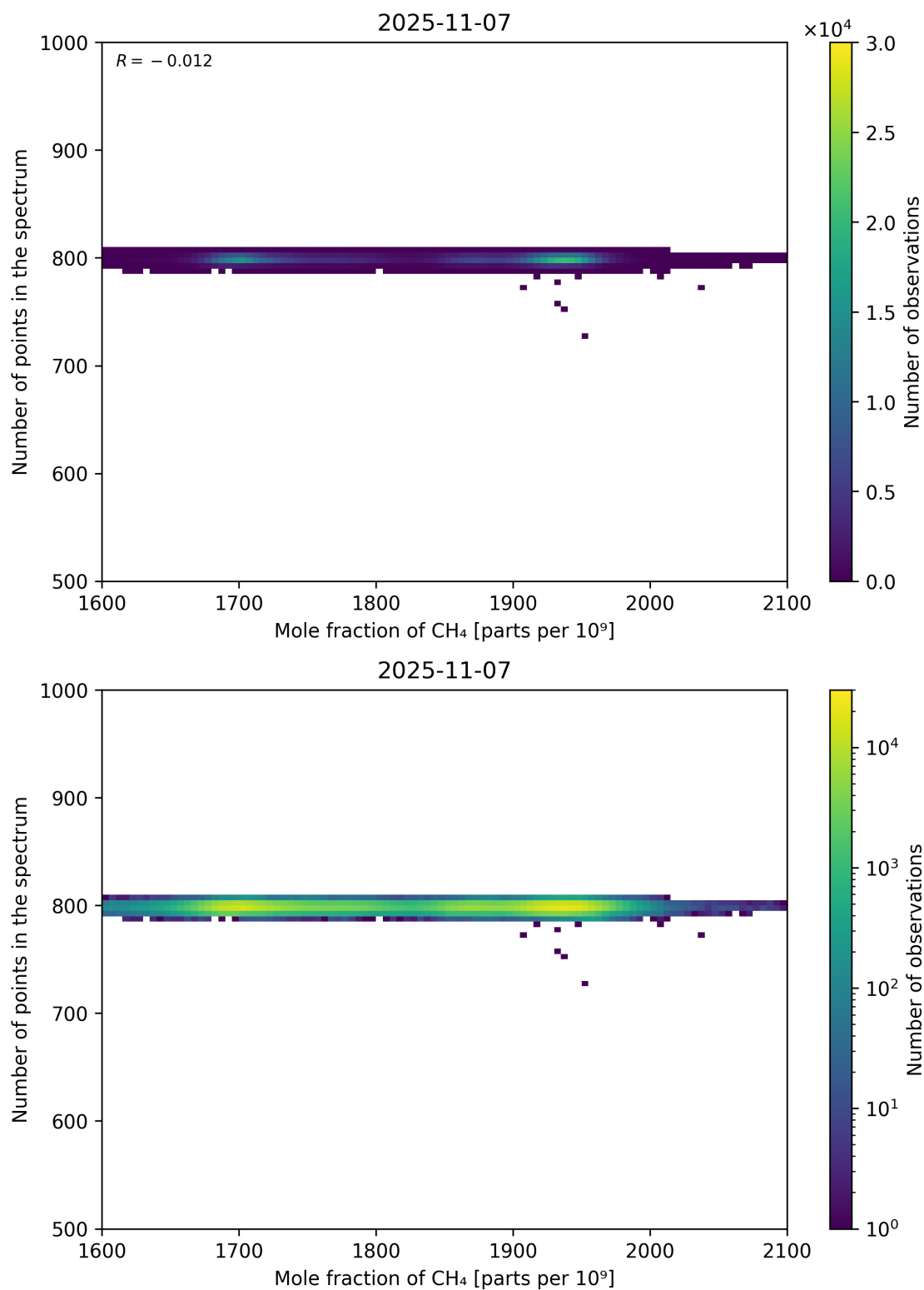
Figure 77: Scatter density plot of “Mole fraction of CH 4 ” against “Number of points in the spectrum” for 2025-11-07 to 2025-11-08.
