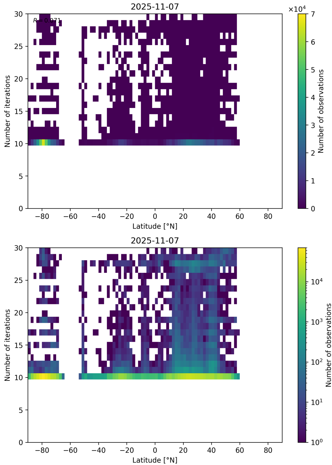
Figure 60: Scatter density plot of “Latitude” against “Number of iterations” for 2025-11-07 to 2025-11-08.
