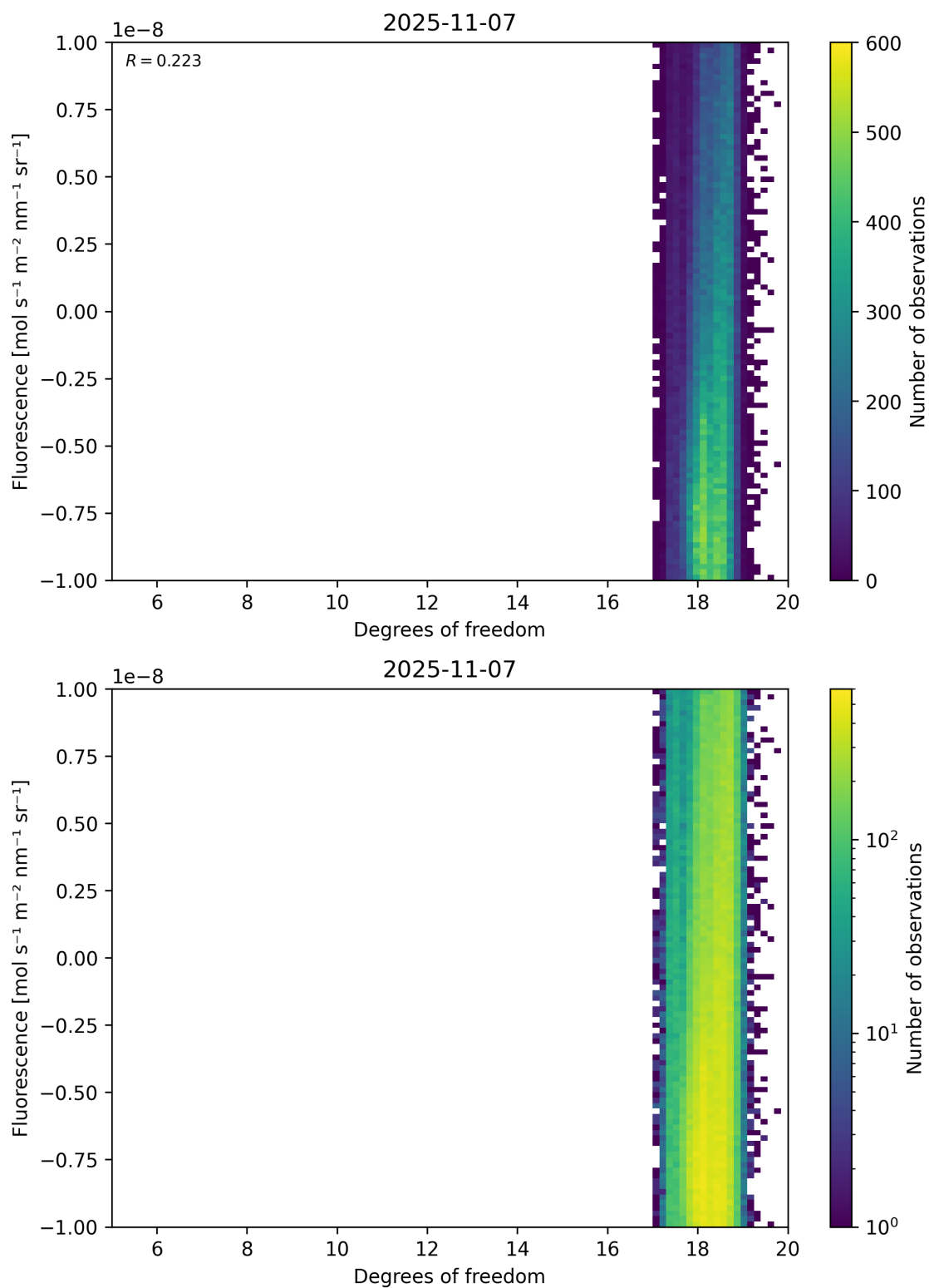
Figure 51: Scatter density plot of “Degrees of freedom” against “Fluorescence” for 2025-11-07 to 2025-11-08.
