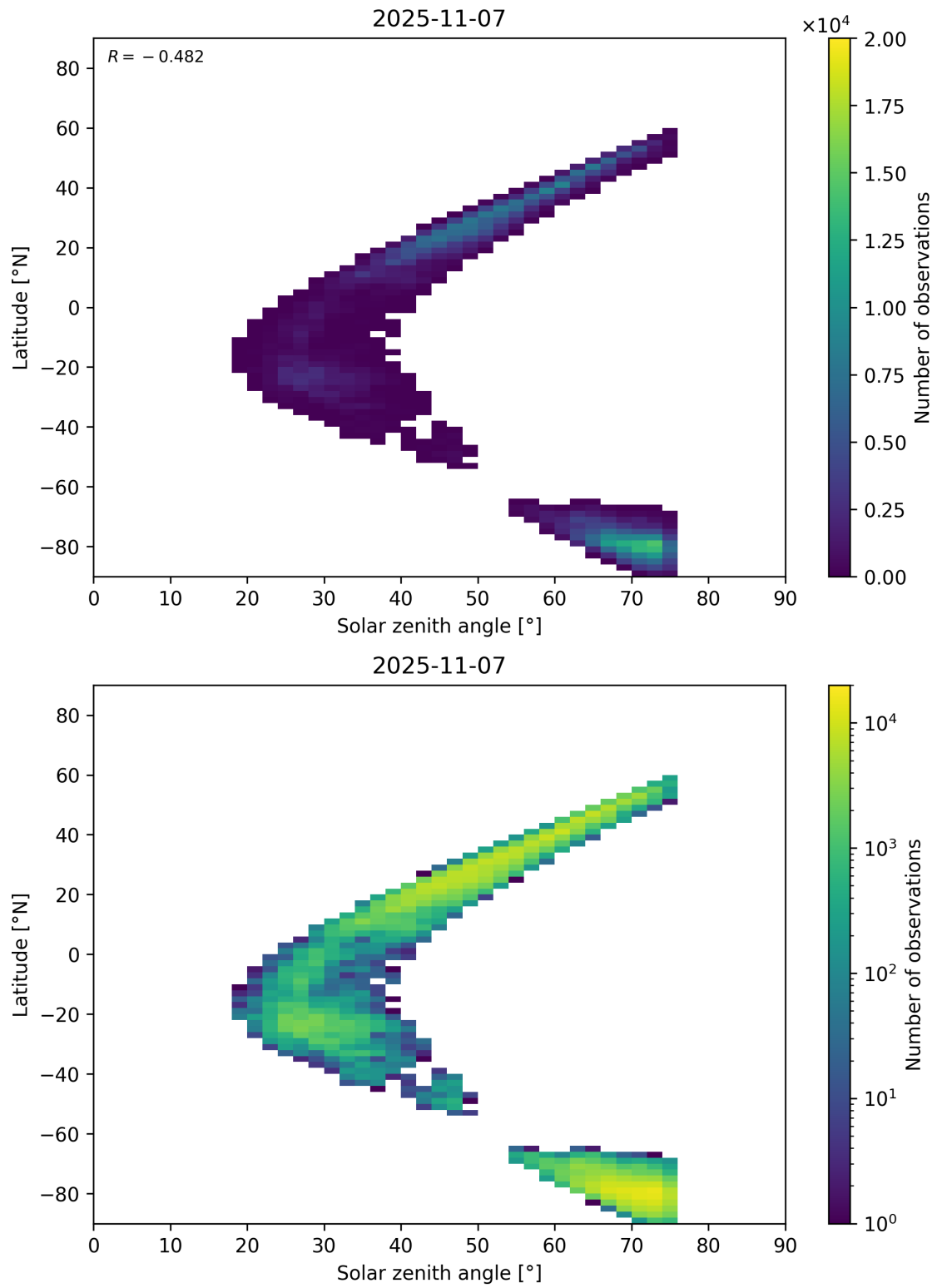
Figure 98: Scatter density plot of “Solar zenith angle” against “Latitude” for 2025-11-07 to 2025-11-08.
