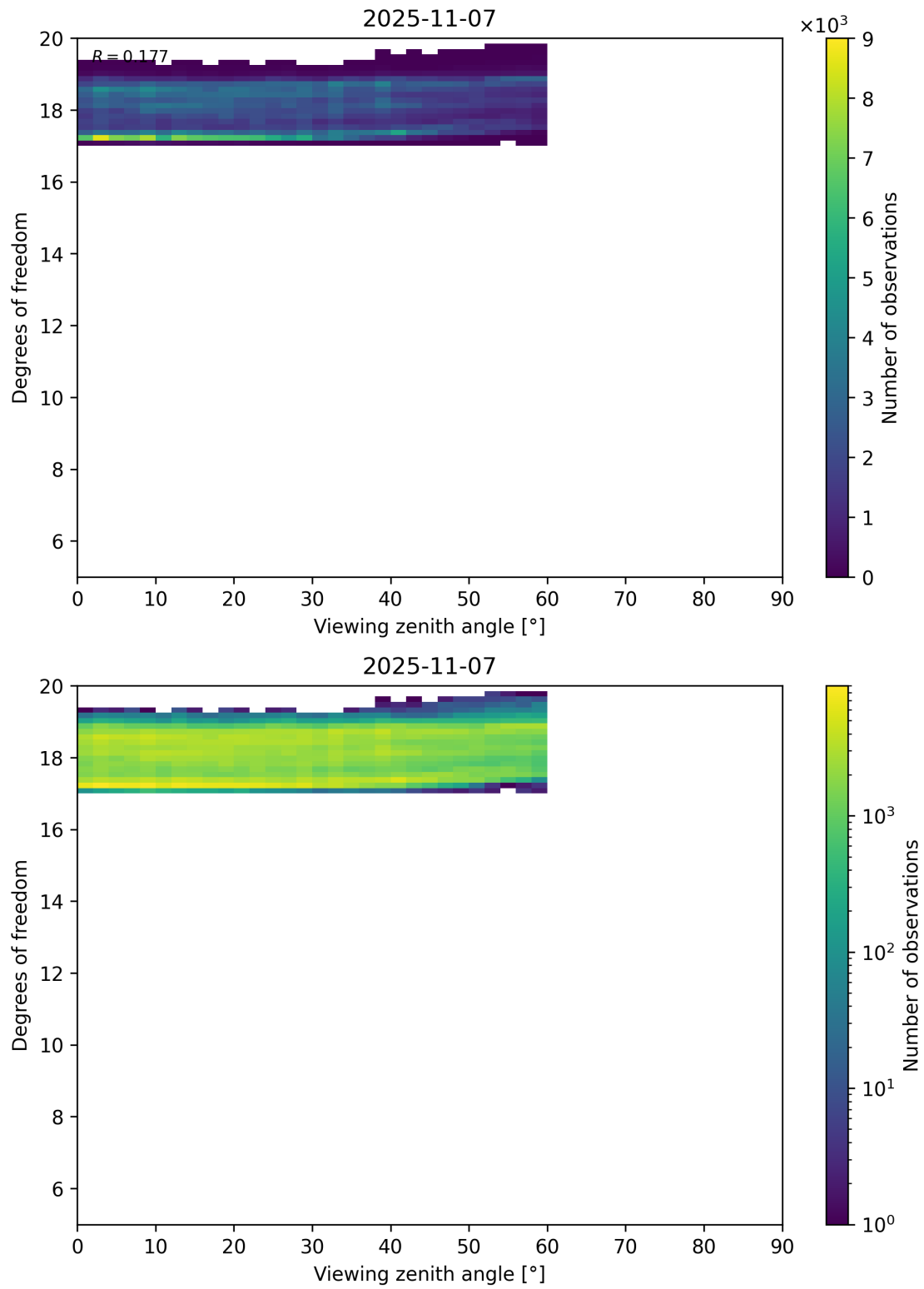
Figure 107: Scatter density plot of “Viewing zenith angle” against “Degrees of freedom” for 2025-11-07 to 2025-11-08.
