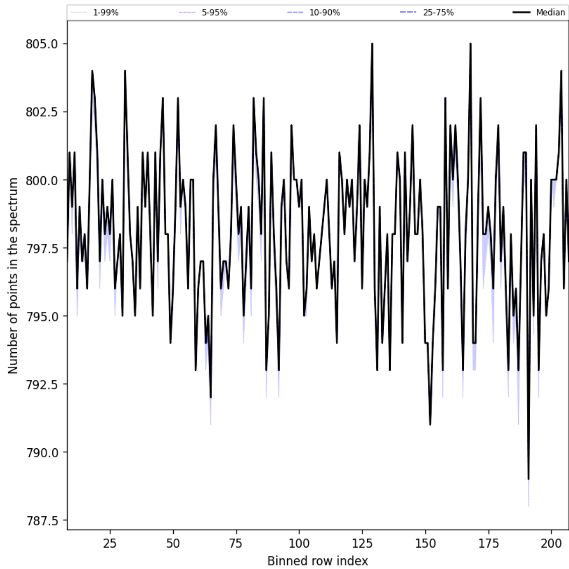
Figure 37: Along track statistics of “Number of points in the spectrum” for 2025-11-07 to 2025-11-08
