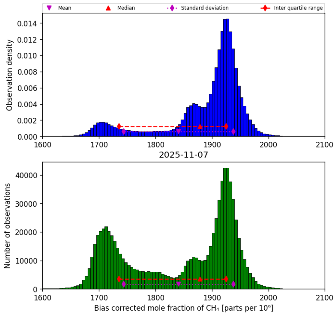
Figure 25: Histogram of “Bias corrected mole fraction of CH 4 ” for 2025-11-07 to 2025-11-08
