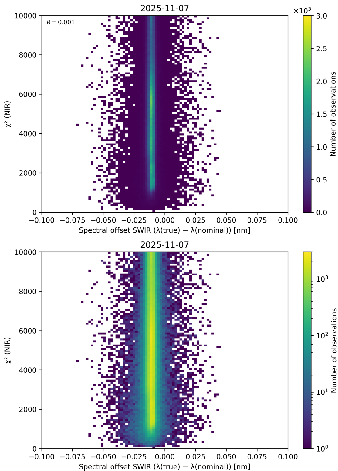
Figure 117: Scatter density plot of “Spectral offset SWIR ( \lambda_{\text{true}} - \lambda_{\text{nominal}} )” against “ \chi^2 (NIR)” for 2025-11-07 to 2025-11-08.
