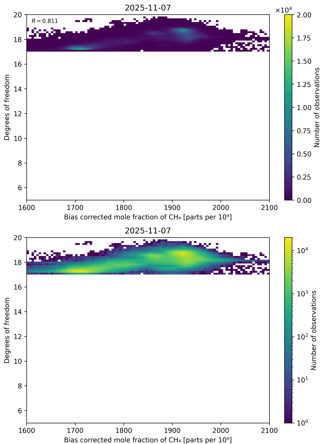
Figure 65: Scatter density plot of “Bias corrected mole fraction of \text{CH}_4 ” against “Degrees of freedom” for 2025-11-07 to 2025-11-08.
