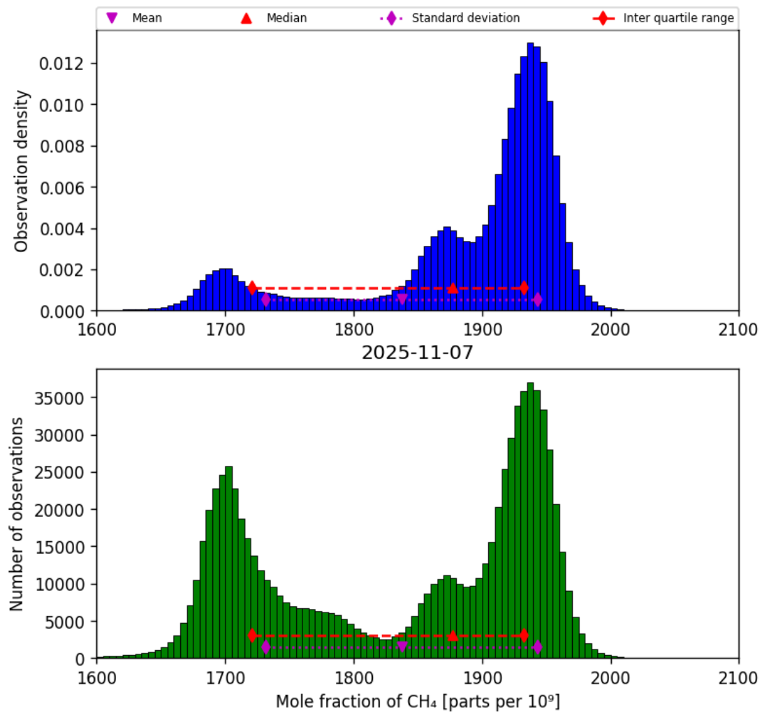
Figure 23: Histogram of “Mole fraction of CH 4 ” for 2025-11-07 to 2025-11-08
