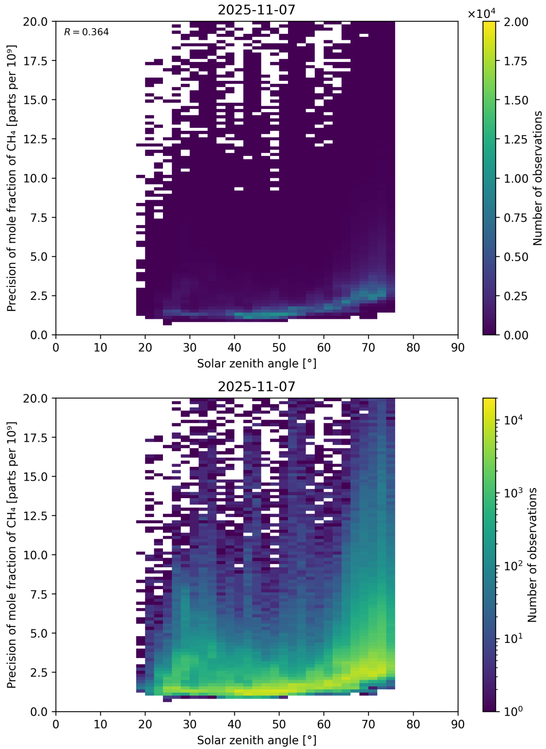
Figure 101: Scatter density plot of “Solar zenith angle” against “Precision of mole fraction of CH 4 ” for 2025-11-07 to 2025-11-08.
