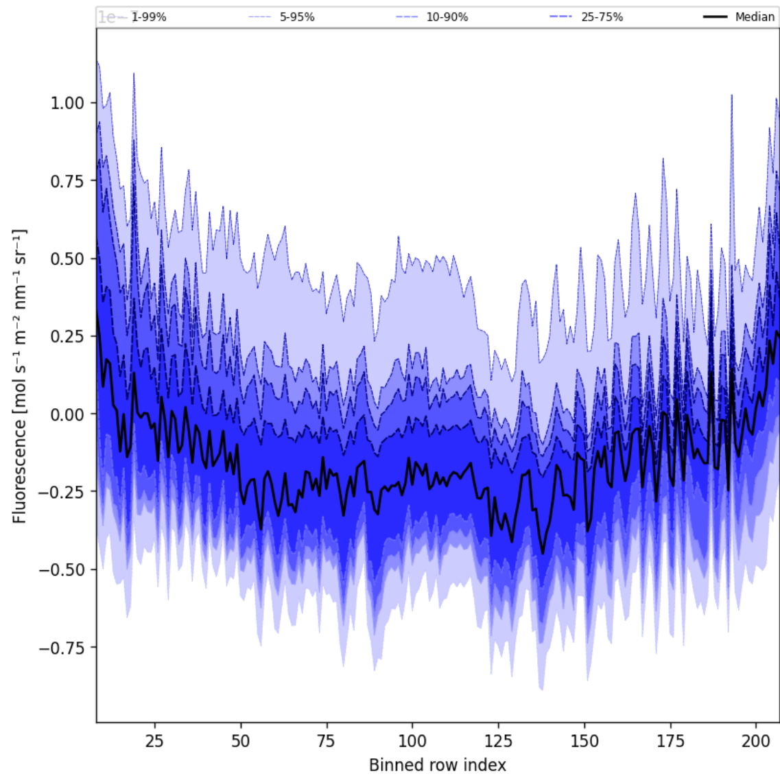
Figure 43: Along track statistics of “Fluorescence” for 2025-11-07 to 2025-11-08
