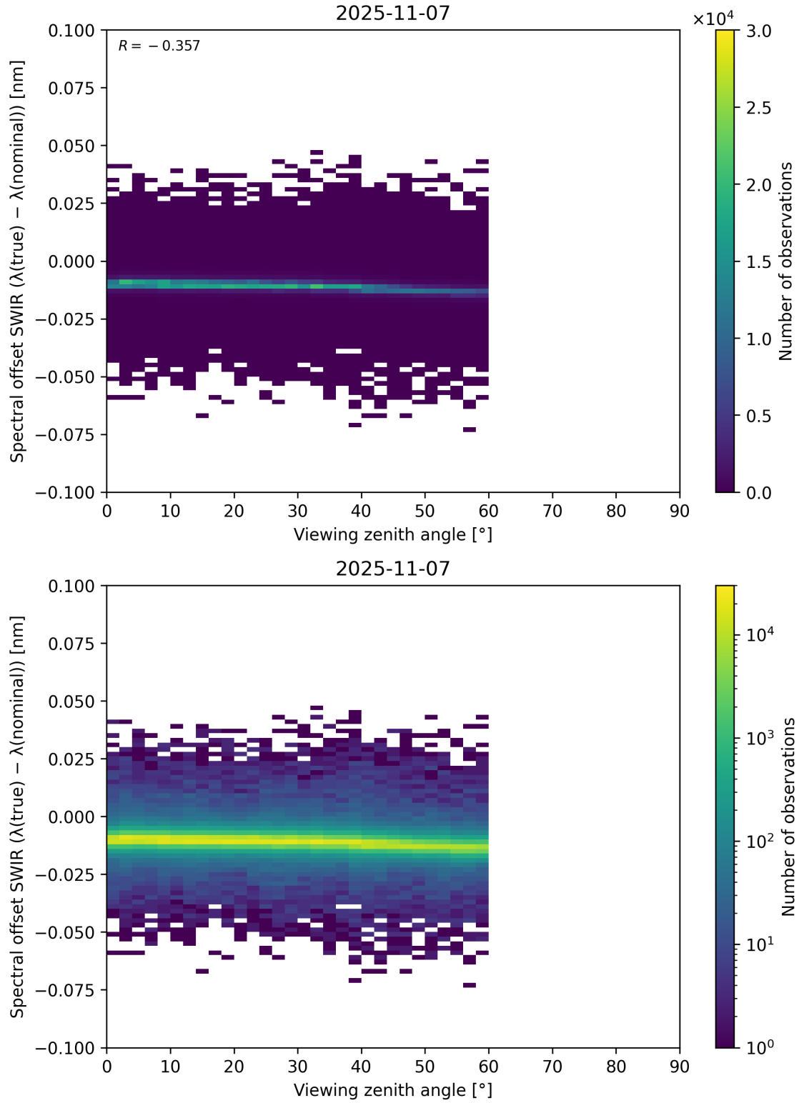
Figure 116: Scatter density plot of “Viewing zenith angle” against “Spectral offset SWIR ( \lambda_{\text{true}} - \lambda_{\text{nominal}} )” for 2025-11-07 to 2025-11-08.
