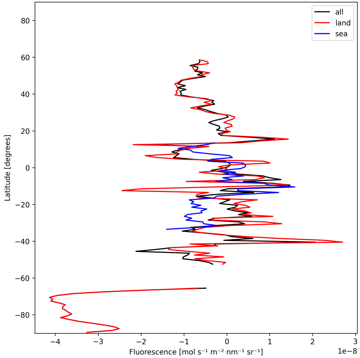
Figure 21: Zonal average of “Fluorescence” for 2025-11-07 to 2025-11-08.
