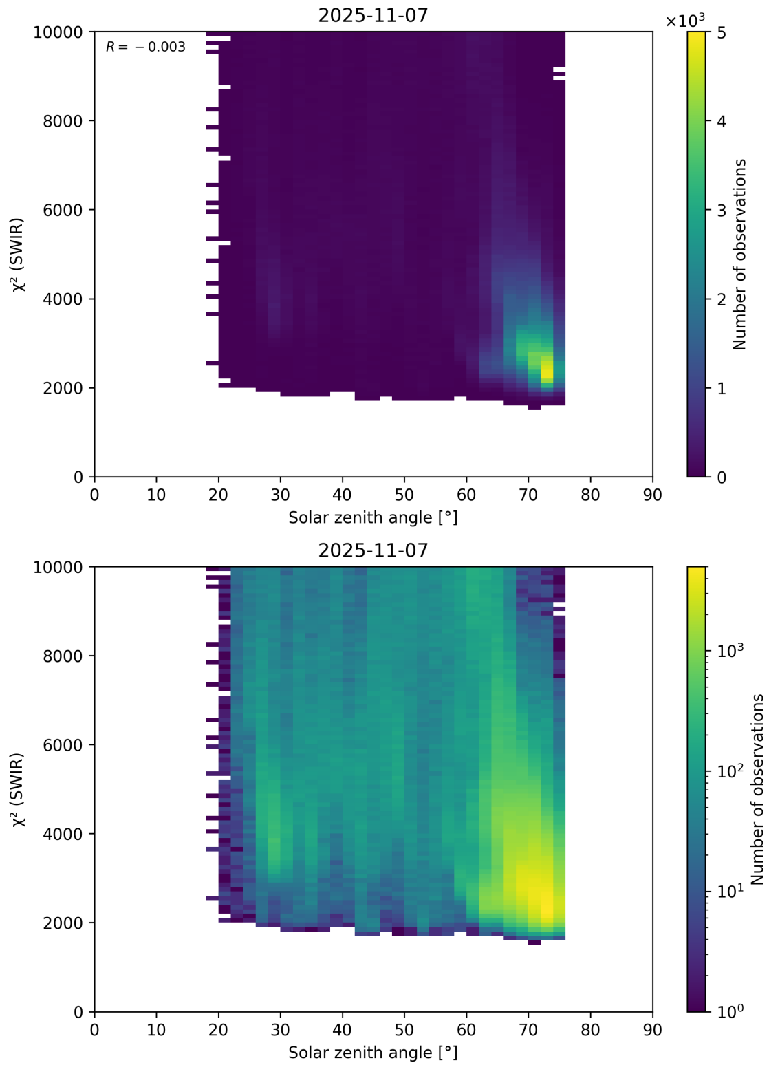
Figure 95: Scatter density plot of “Solar zenith angle” against “ \chi^2 (SWIR)” for 2025-11-07 to 2025-11-08.
