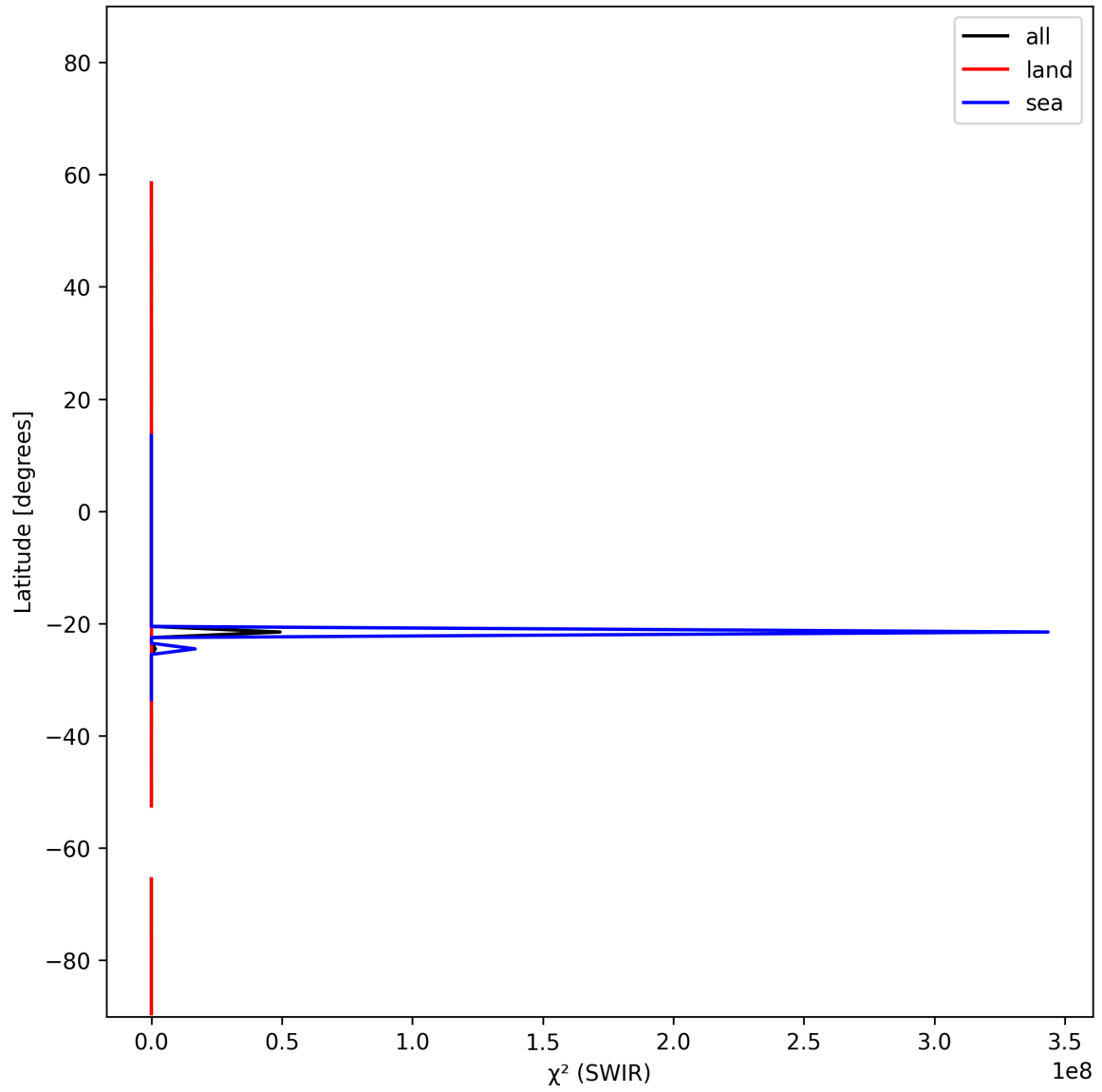
Figure 17: Zonal average of “ \chi^2 (SWIR)” for 2025-11-07 to 2025-11-08.
