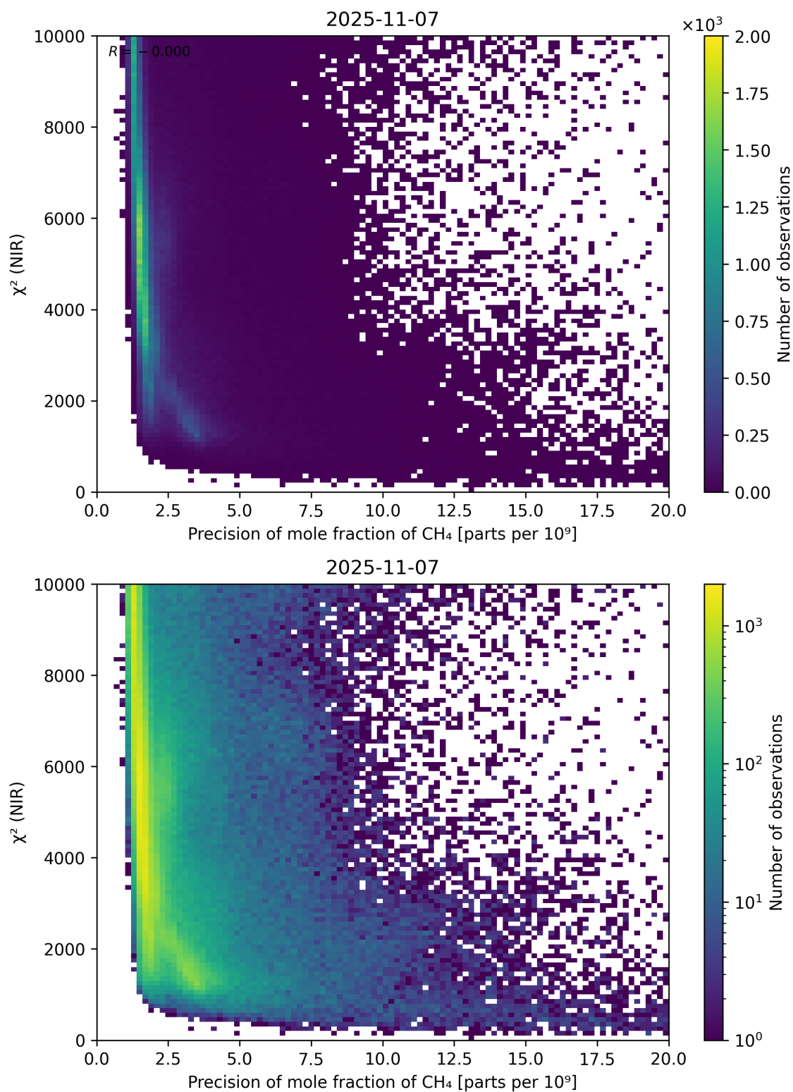
Figure 78: Scatter density plot of “Precision of mole fraction of \text{CH}_4 ” against “ \chi^2 (NIR)” for 2025-11-07 to 2025-11-08.
