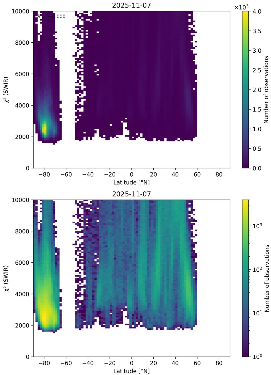
Figure 54: Scatter density plot of “Latitude” against “ \chi^2 (SWIR)” for 2025-11-07 to 2025-11-08.
