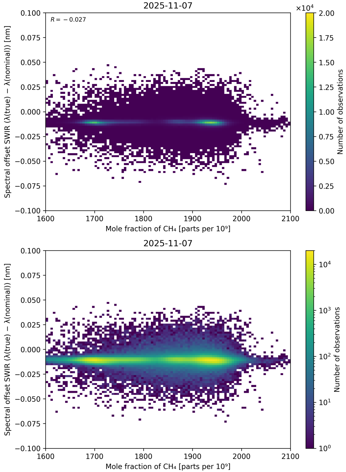
Figure 86: Scatter density plot of “Mole fraction of \text{CH}_4 ” against “Spectral offset SWIR ( \lambda_{\text{true}} - \lambda_{\text{nominal}} )” for 2025-11-07 to 2025-11-08.
