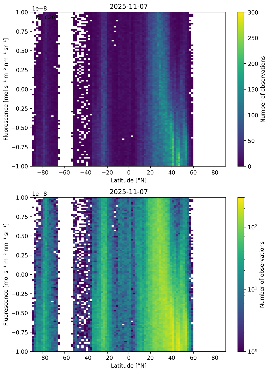
Figure 56: Scatter density plot of “Latitude” against “Fluorescence” for 2025-11-07 to 2025-11-08.
