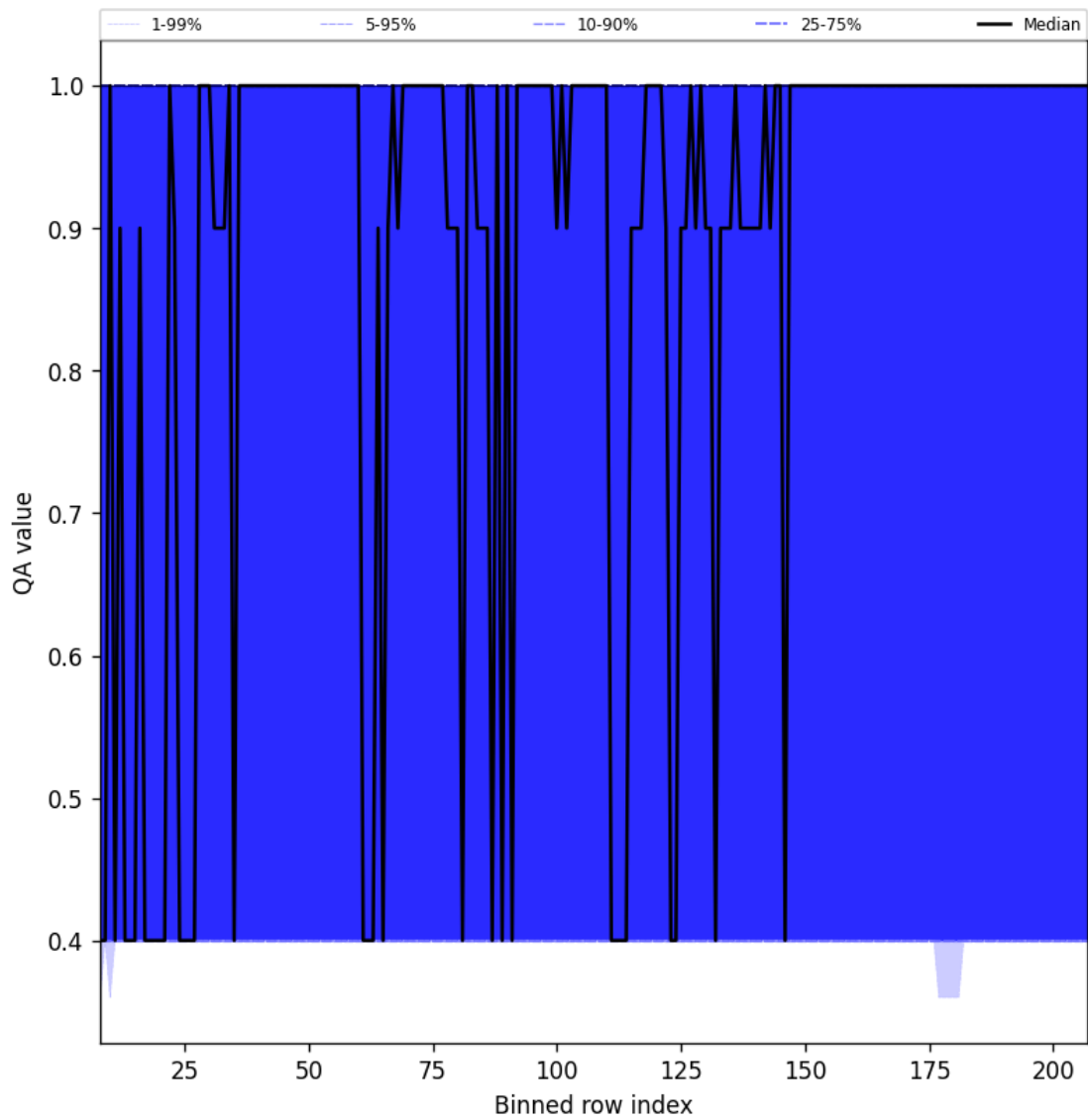
Figure 33: Along track statistics of “QA value” for 2025-11-07 to 2025-11-08
