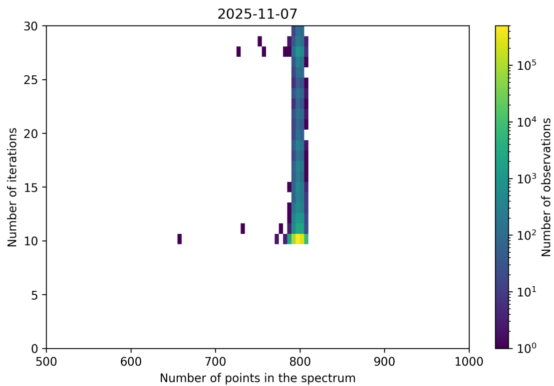
Figure 92: Scatter density plot of “Number of points in the spectrum” against “Number of iterations” for 2025-11-07 to 2025-11-08.
