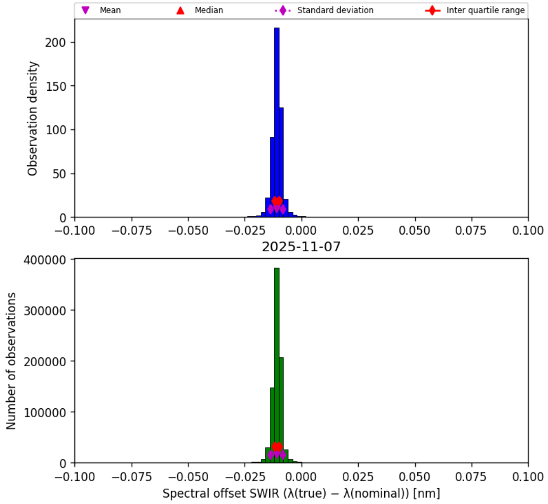
Figure 27: Histogram of “Spectral offset SWIR ( \lambda_{\text{true}} - \lambda_{\text{nominal}} )” for 2025-11-07 to 2025-11-08
