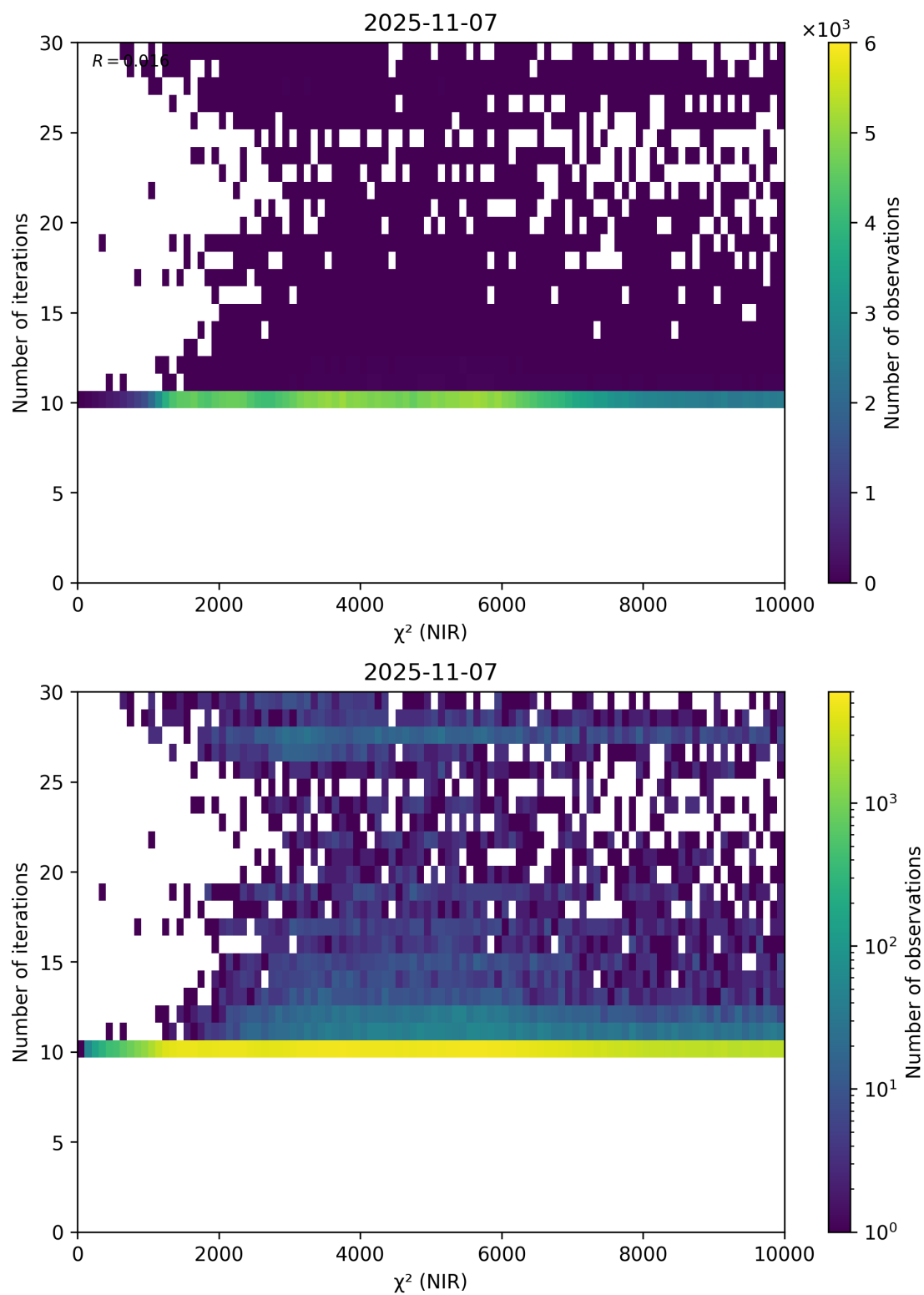
Figure 46: Scatter density plot of “ \chi^2 (NIR)” against “Number of iterations” for 2025-11-07 to 2025-11-08.
