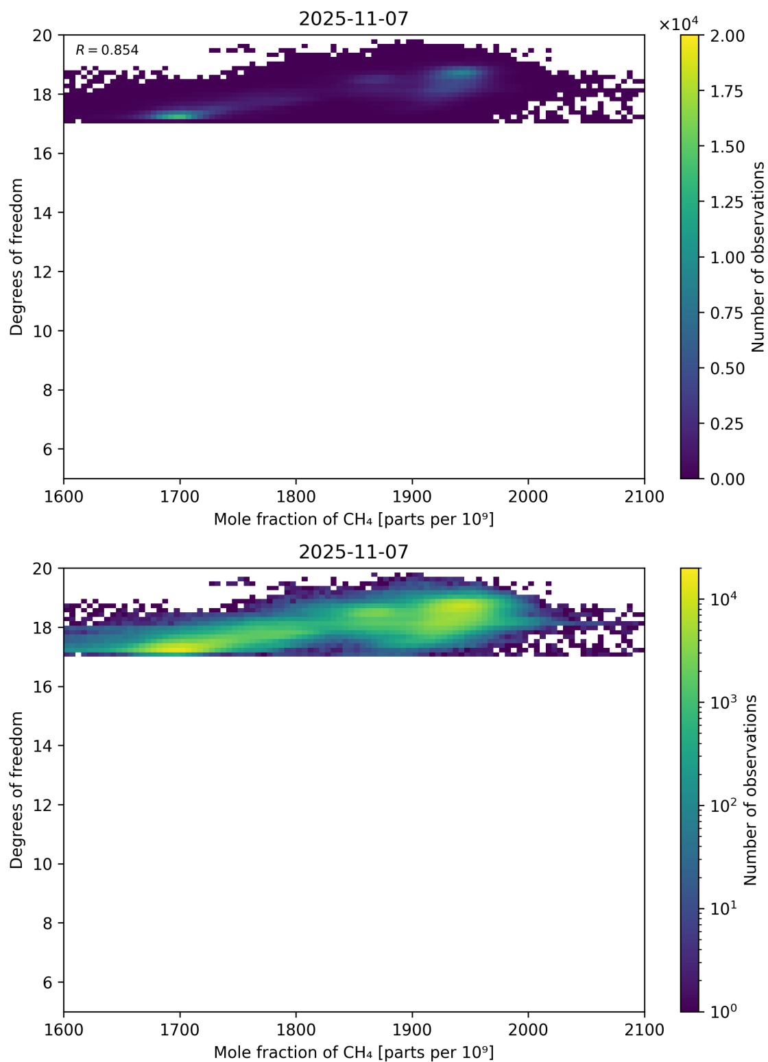
Figure 72: Scatter density plot of “Mole fraction of CH 4 ” against “Degrees of freedom” for 2025-11-07 to 2025-11-08.
