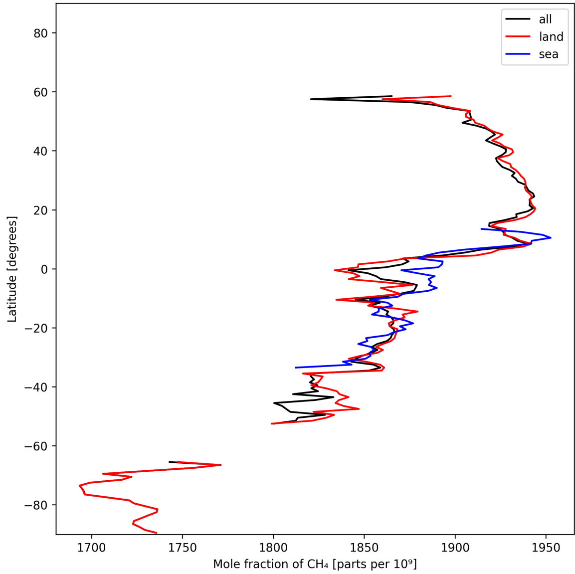
Figure 12: Zonal average of “Mole fraction of CH 4 ” for 2025-11-07 to 2025-11-08.
