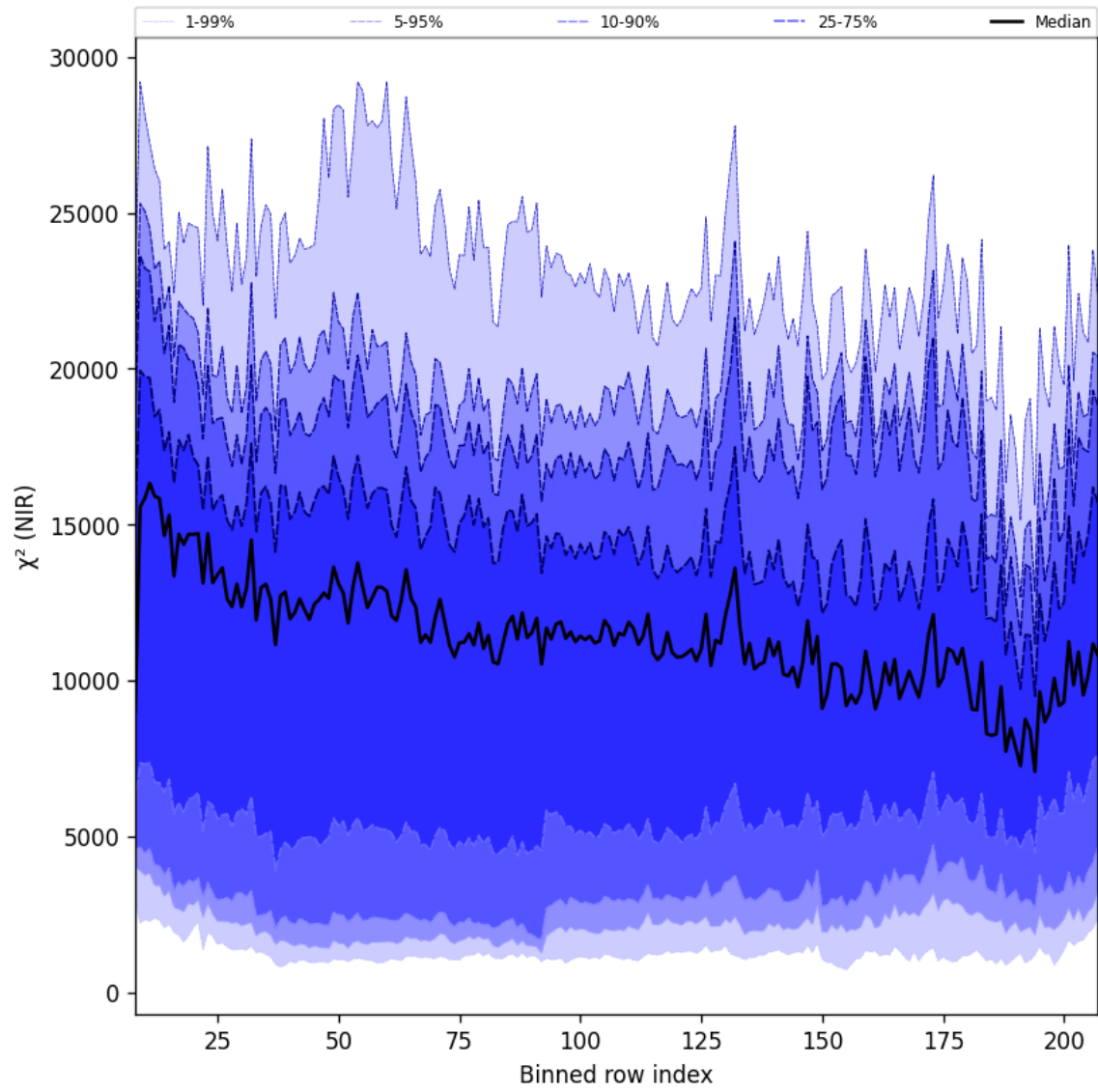
Figure 40: Along track statistics of “ \chi^2 (NIR)” for 2025-11-07 to 2025-11-08
