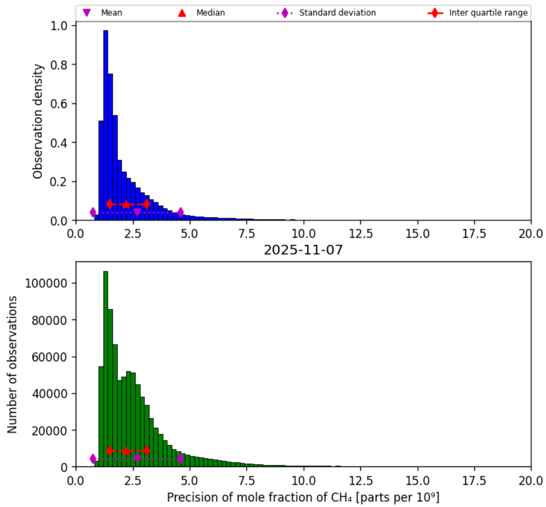
Figure 24: Histogram of “Precision of mole fraction of CH 4 ” for 2025-11-07 to 2025-11-08
