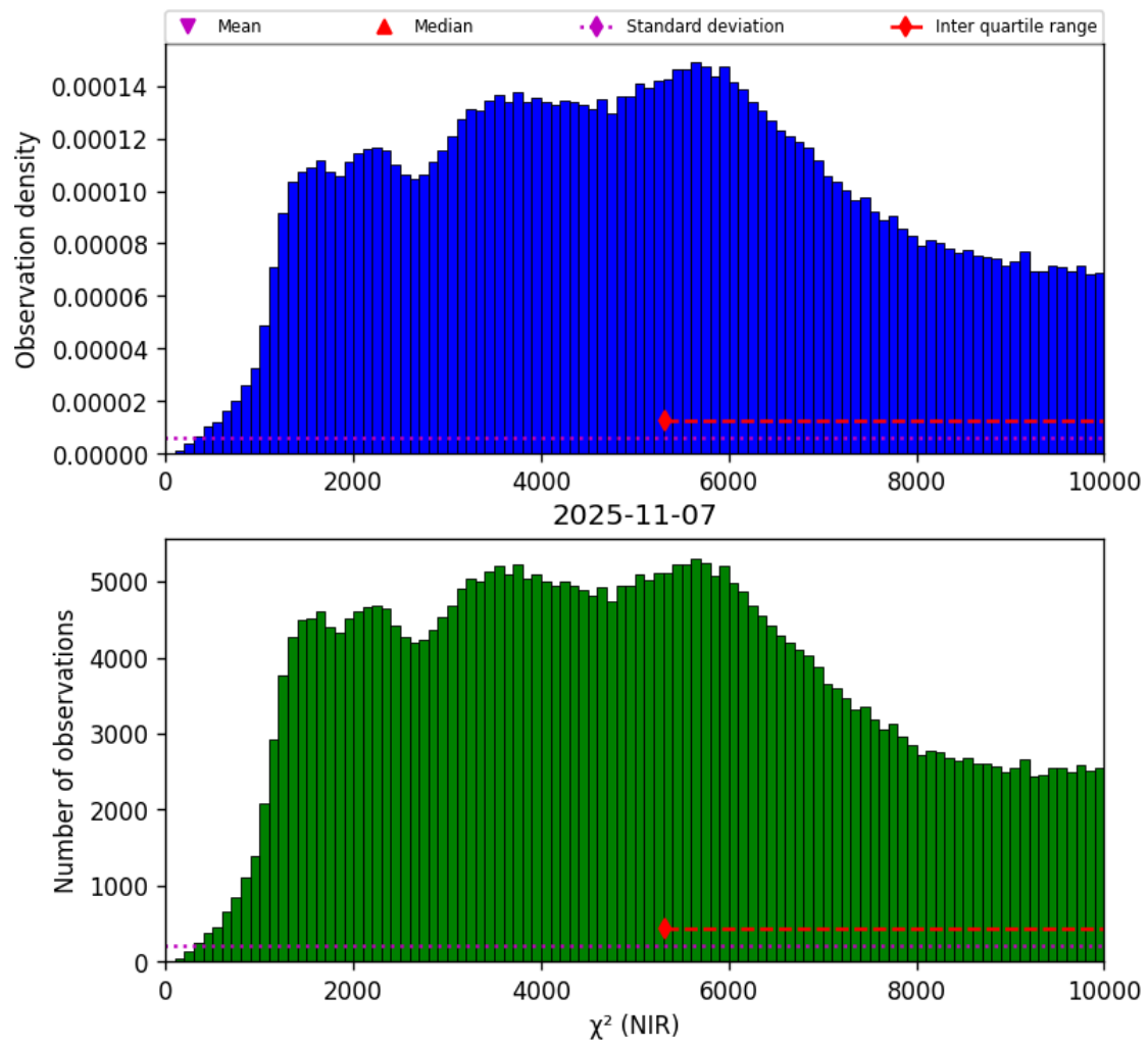
Figure 29: Histogram of “ \chi^2 (NIR)” for 2025-11-07 to 2025-11-08
