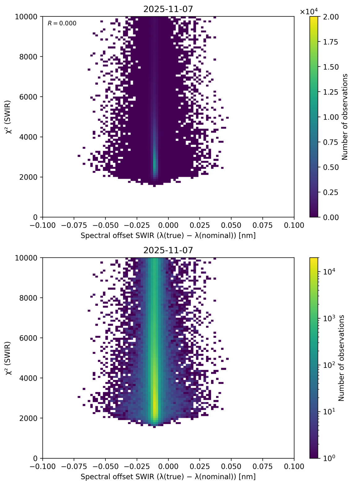
Figure 118: Scatter density plot of “Spectral offset SWIR ( \lambda_{\text{true}} - \lambda_{\text{nominal}} )” against “ \chi^2 (SWIR)” for 2025-11-07 to 2025-11-08.
