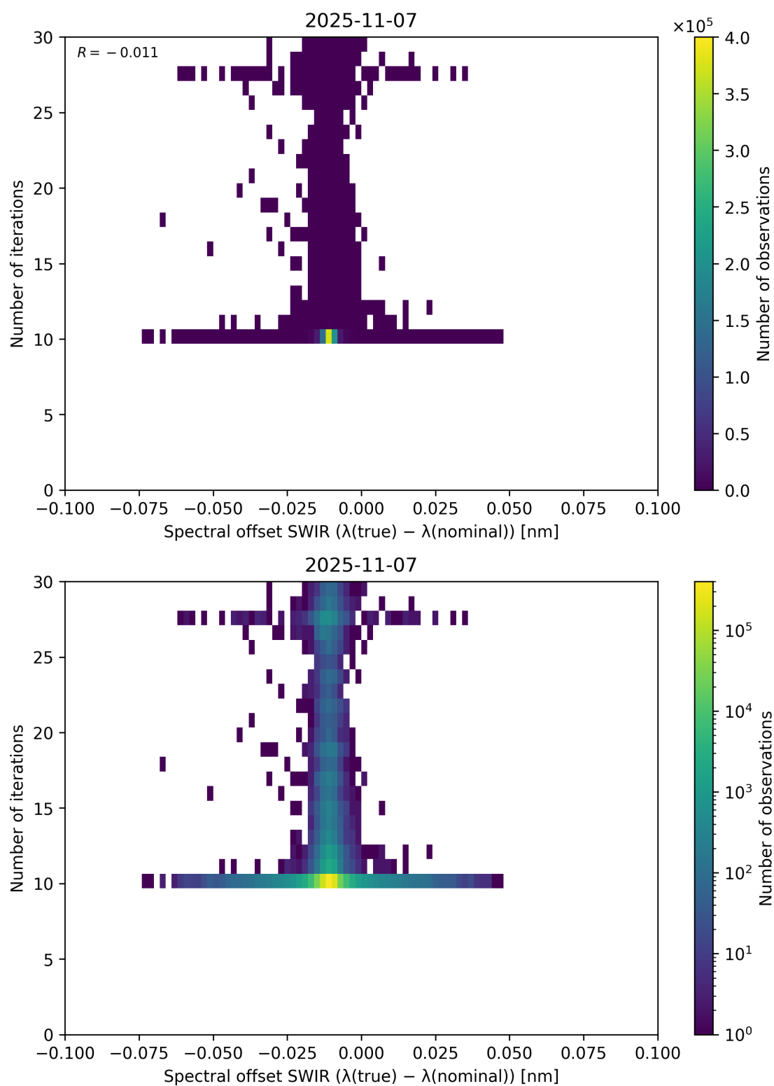
Figure 121: Scatter density plot of “Spectral offset SWIR ( \lambda_{\text{true}} - \lambda_{\text{nominal}} )” against “Number of iterations” for 2025-11-07 to 2025-11-08.
