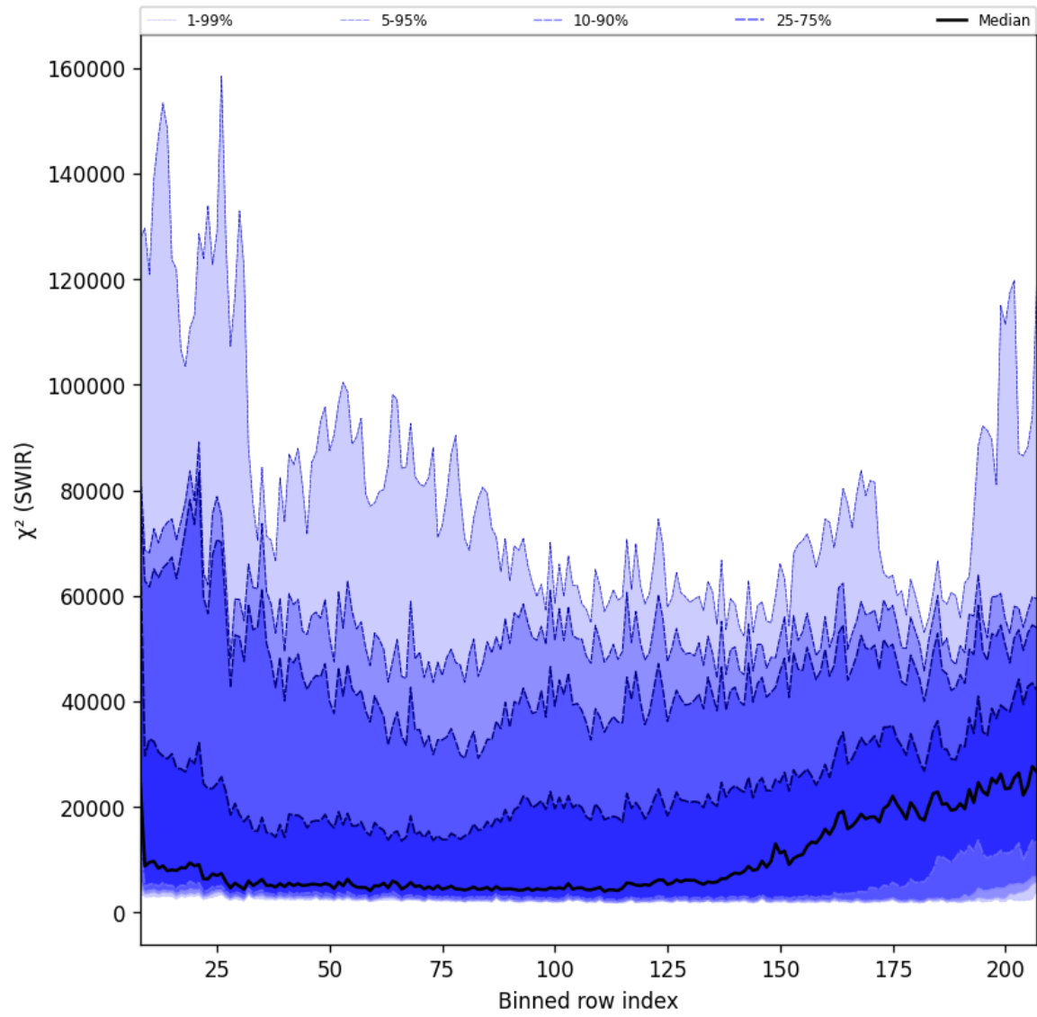
Figure 39: Along track statistics of “ \chi^2 (SWIR)” for 2025-11-07 to 2025-11-08
