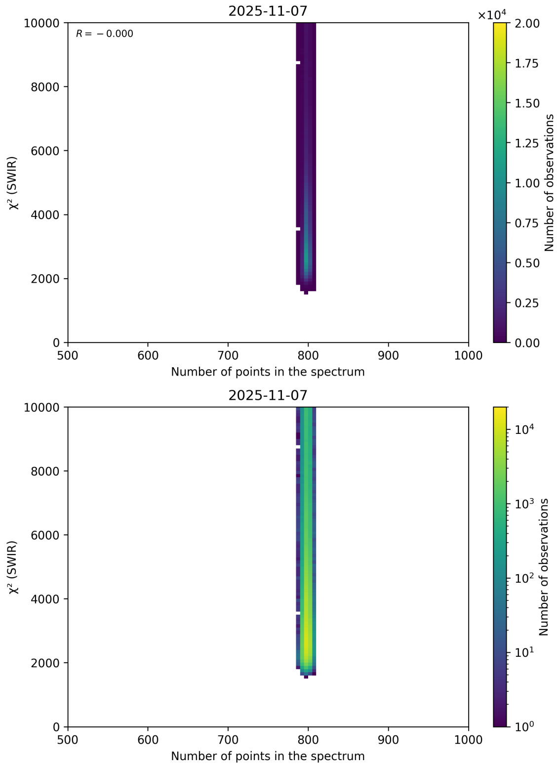
Figure 89: Scatter density plot of “Number of points in the spectrum” against “ \chi^2 (SWIR)” for 2025-11-07 to 2025-11-08.
