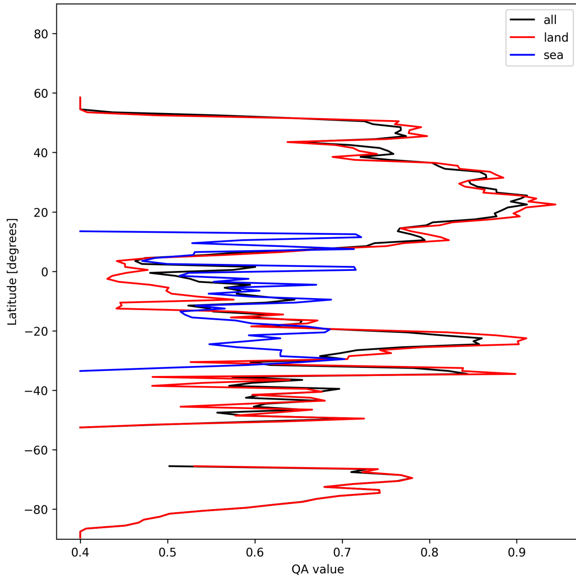
Figure 11: Zonal average of “QA value” for 2025-11-07 to 2025-11-08.
