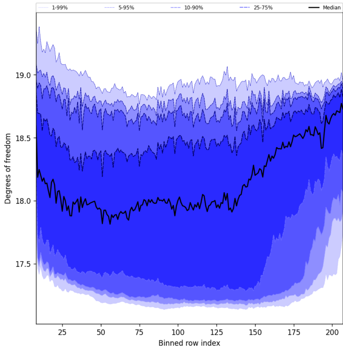
Figure 41: Along track statistics of “Degrees of freedom” for 2025-11-07 to 2025-11-08
