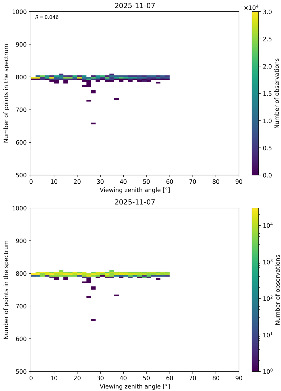
Figure 114: Scatter density plot of “Viewing zenith angle” against “Number of points in the spectrum” for 2025-11-07 to 2025-11-08.
