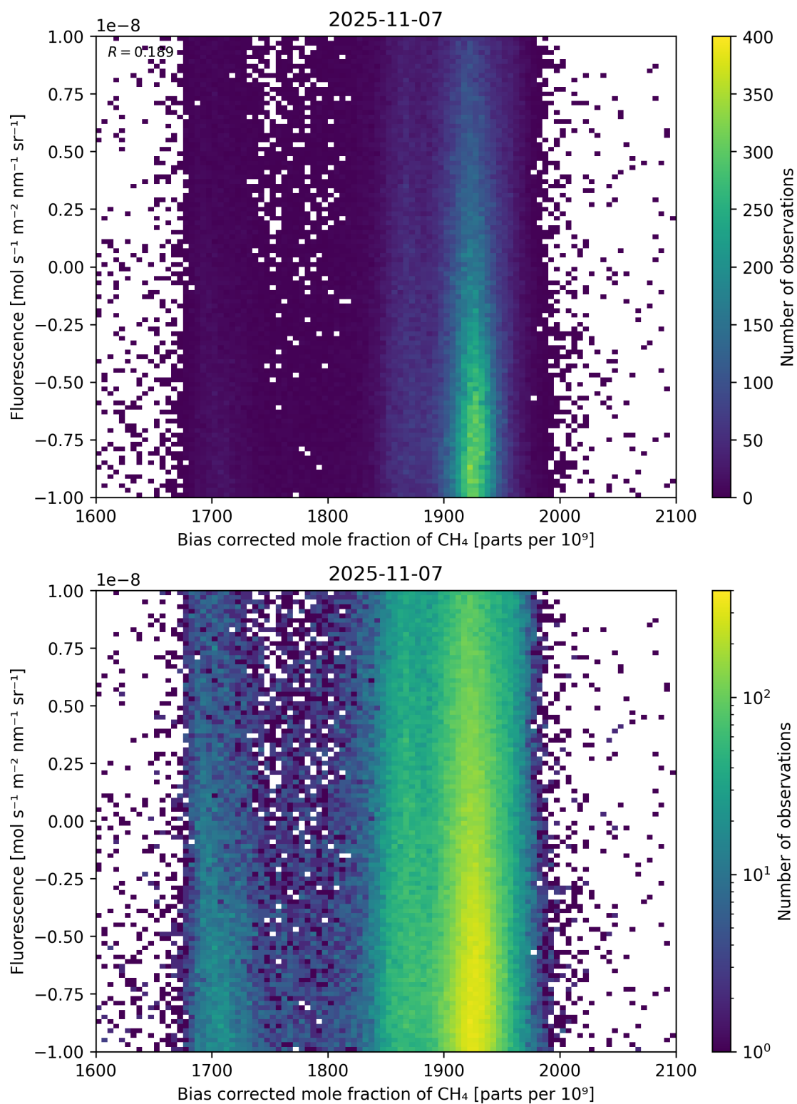
Figure 66: Scatter density plot of “Bias corrected mole fraction of \text{CH}_4 ” against “Fluorescence” for 2025-11-07 to 2025-11-08.
