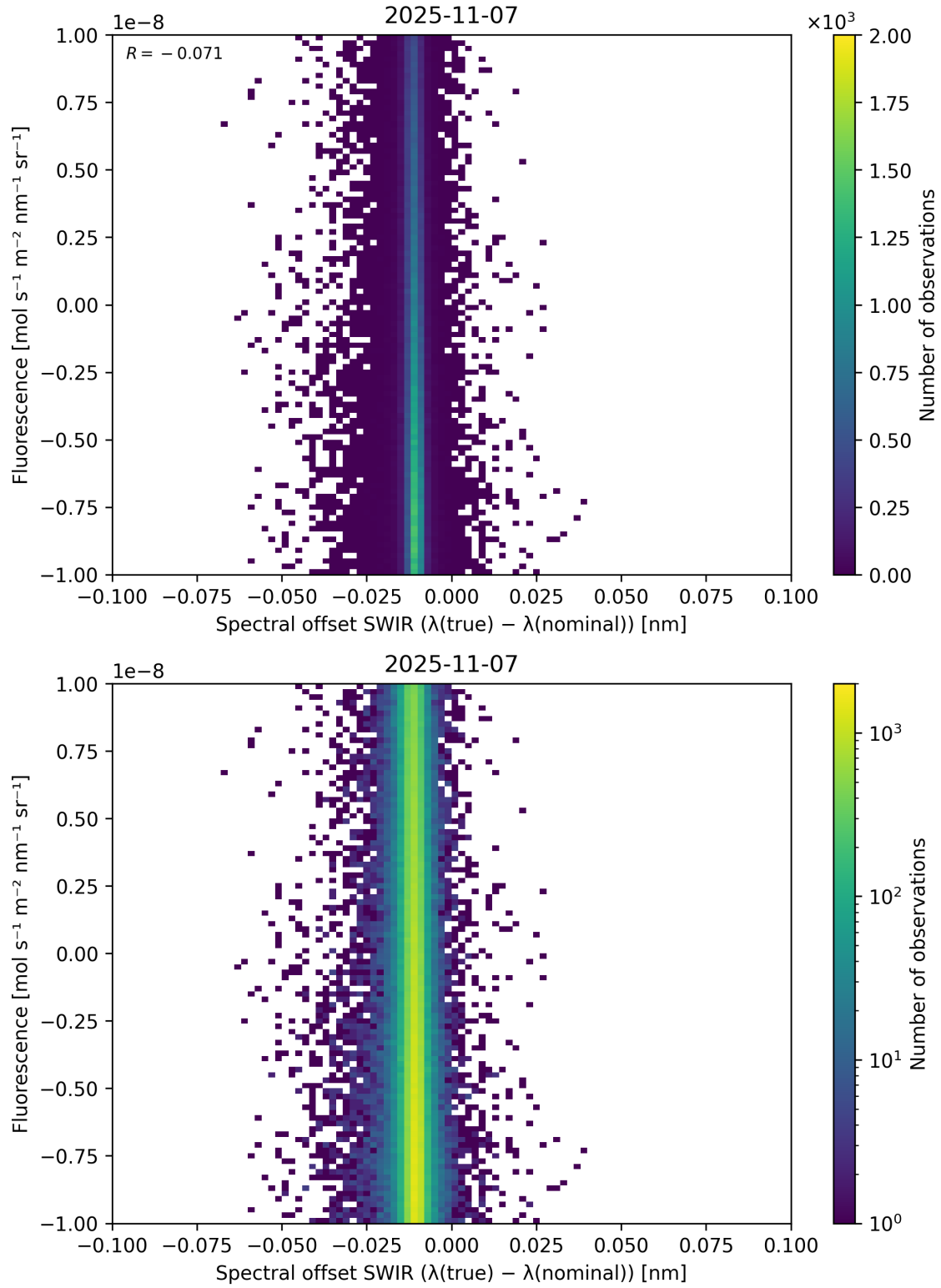
Figure 120: Scatter density plot of “Spectral offset SWIR ( \lambda_{\text{true}} - \lambda_{\text{nominal}} )” against “Fluorescence” for 2025-11-07 to 2025-11-08.
