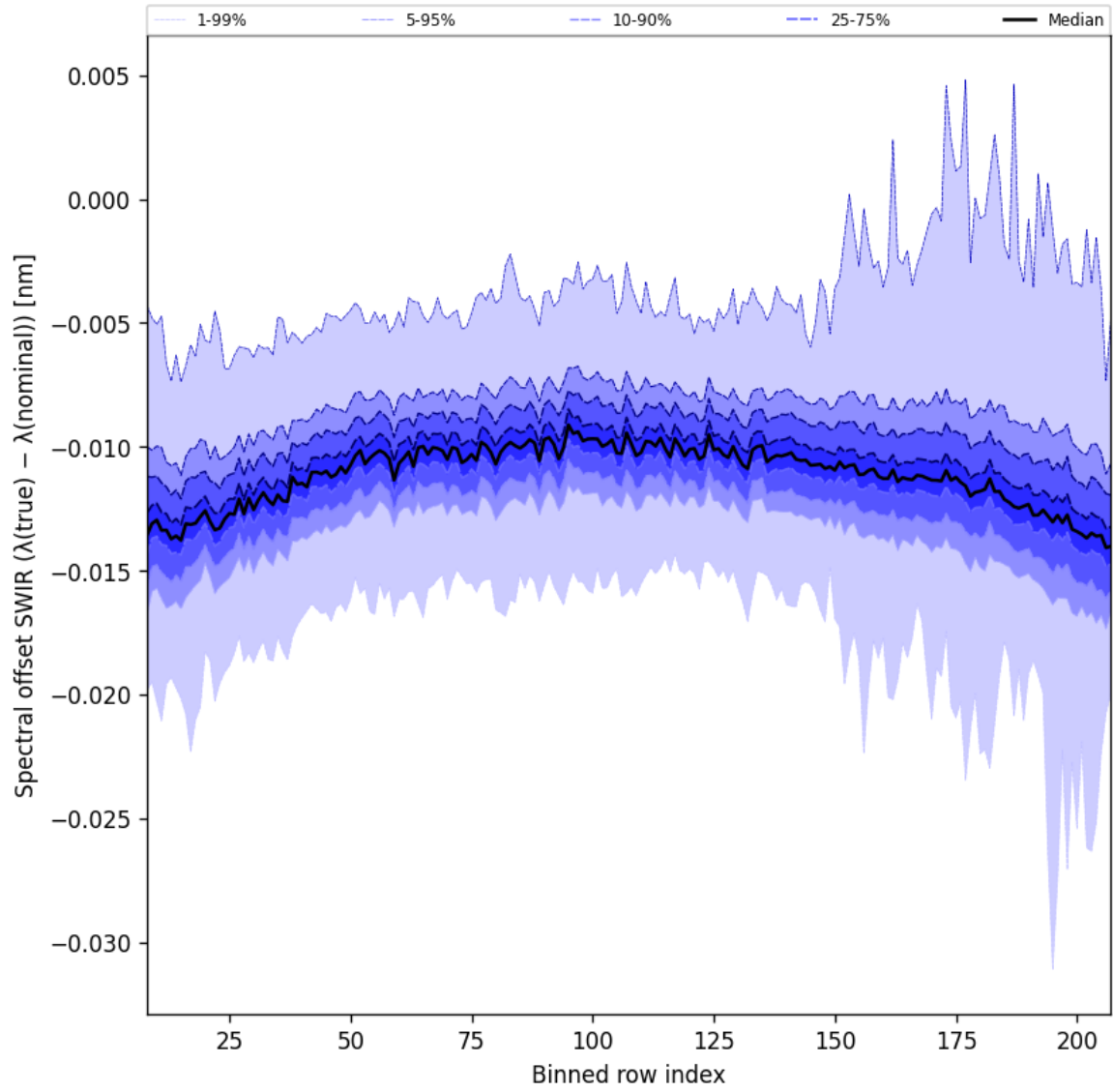
Figure 38: Along track statistics of “Spectral offset SWIR ( \lambda_{\text{true}} - \lambda_{\text{nominal}} )” for 2025-11-07 to 2025-11-08
