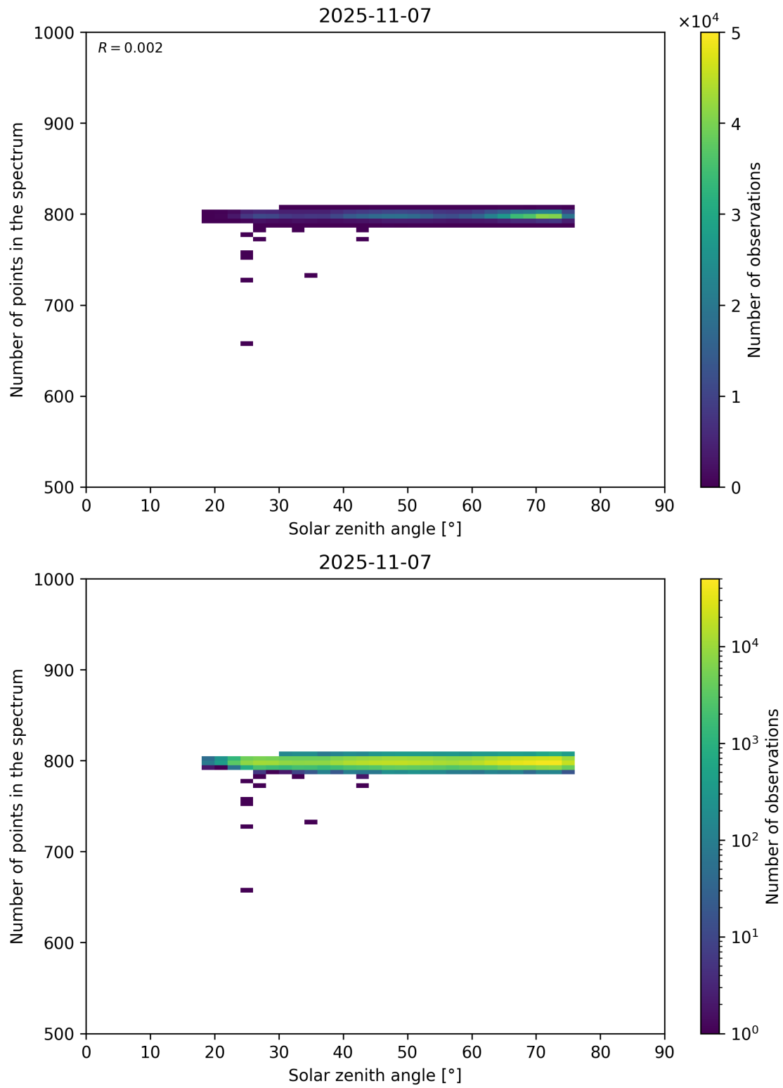
Figure 103: Scatter density plot of “Solar zenith angle” against “Number of points in the spectrum” for 2025-11-07 to 2025-11-08.
