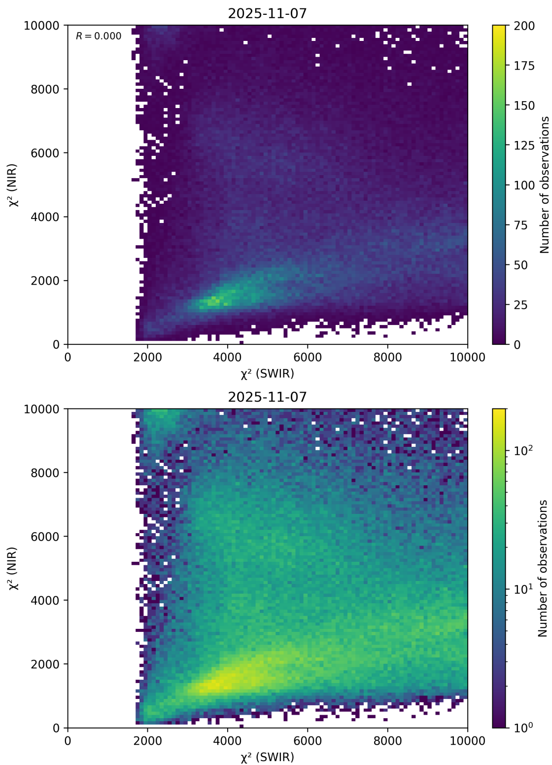
Figure 47: Scatter density plot of “ \chi^2 (SWIR)” against “ \chi^2 (NIR)” for 2025-11-07 to 2025-11-08.
