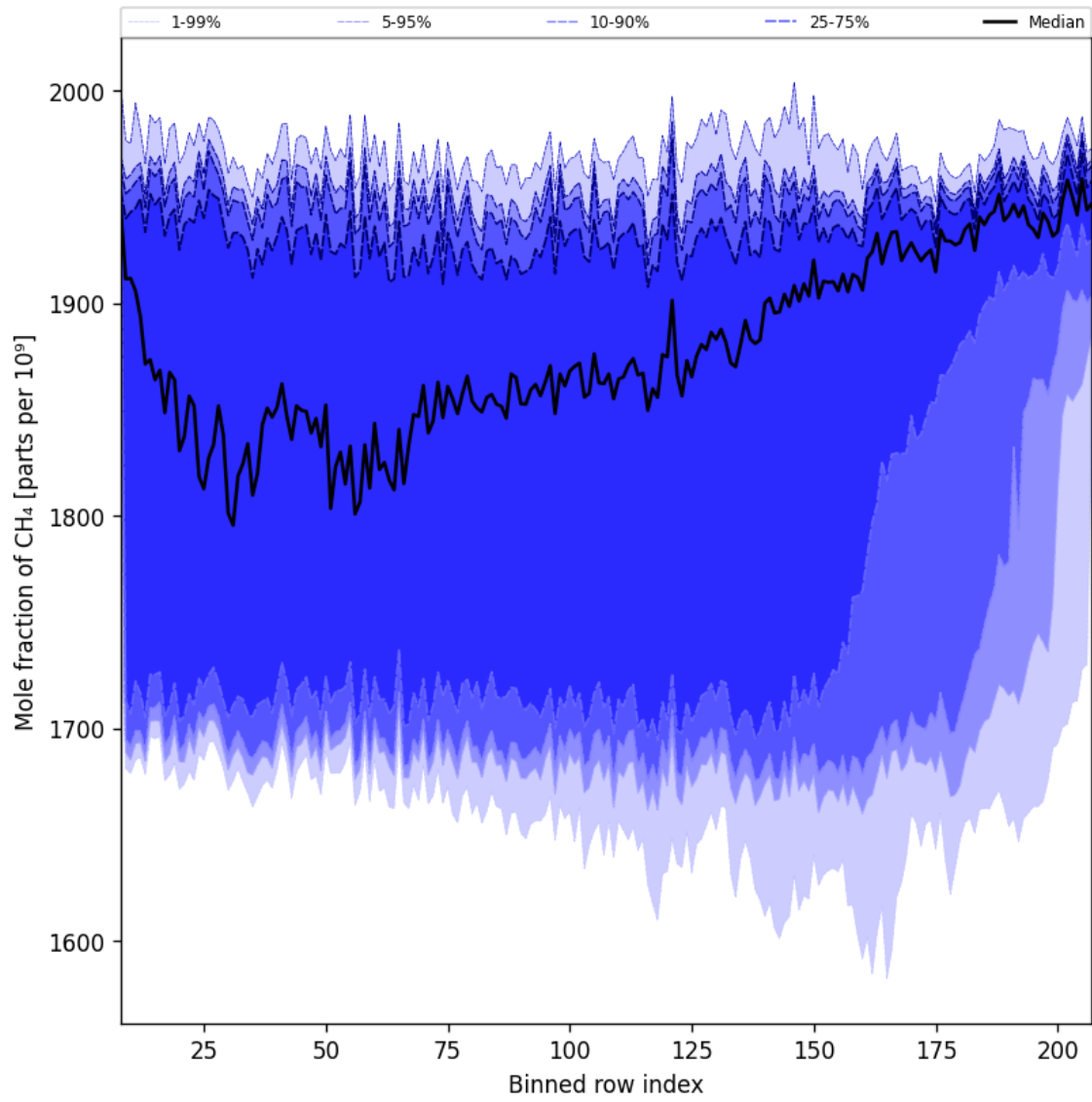
Figure 34: Along track statistics of “Mole fraction of CH 4 ” for 2025-11-07 to 2025-11-08
