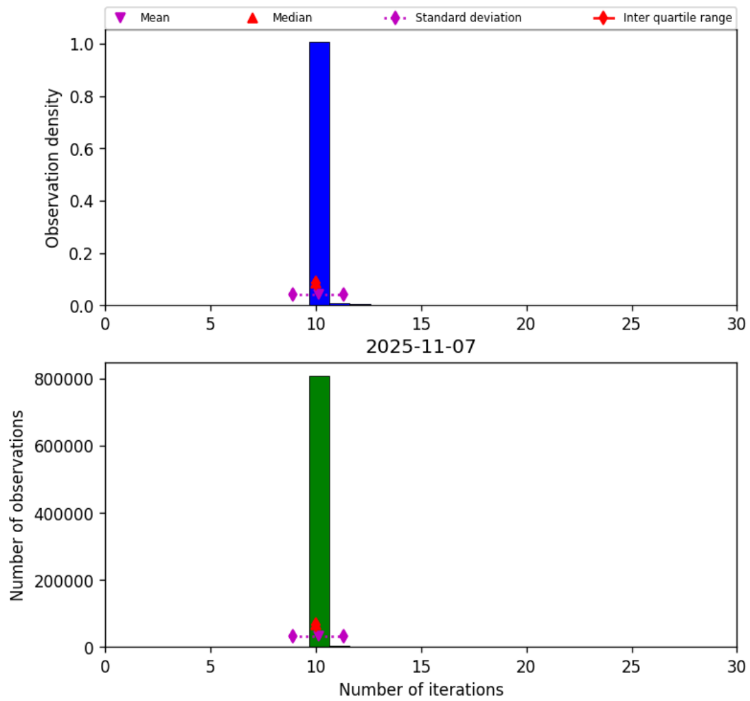
Figure 31: Histogram of “Number of iterations” for 2025-11-07 to 2025-11-08
