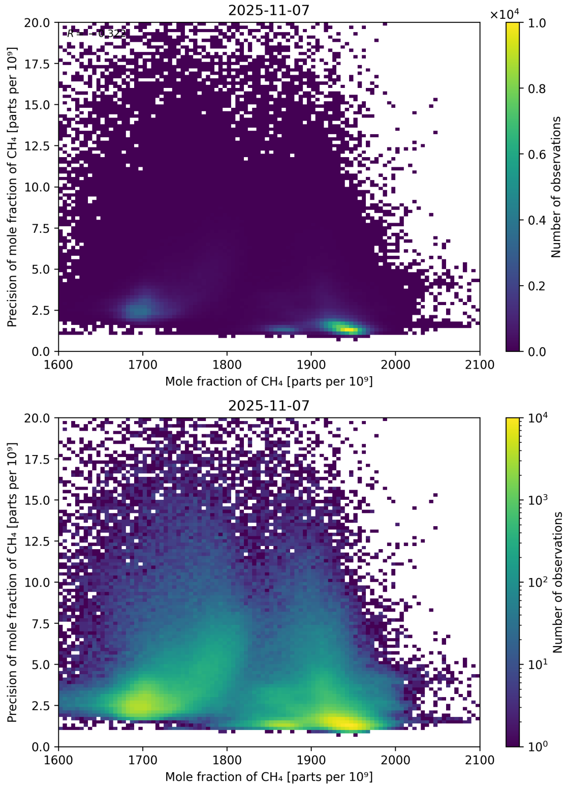
Figure 75: Scatter density plot of “Mole fraction of CH 4 ” against “Precision of mole fraction of CH 4 ” for 2025-11-07 to 2025-11-08.
