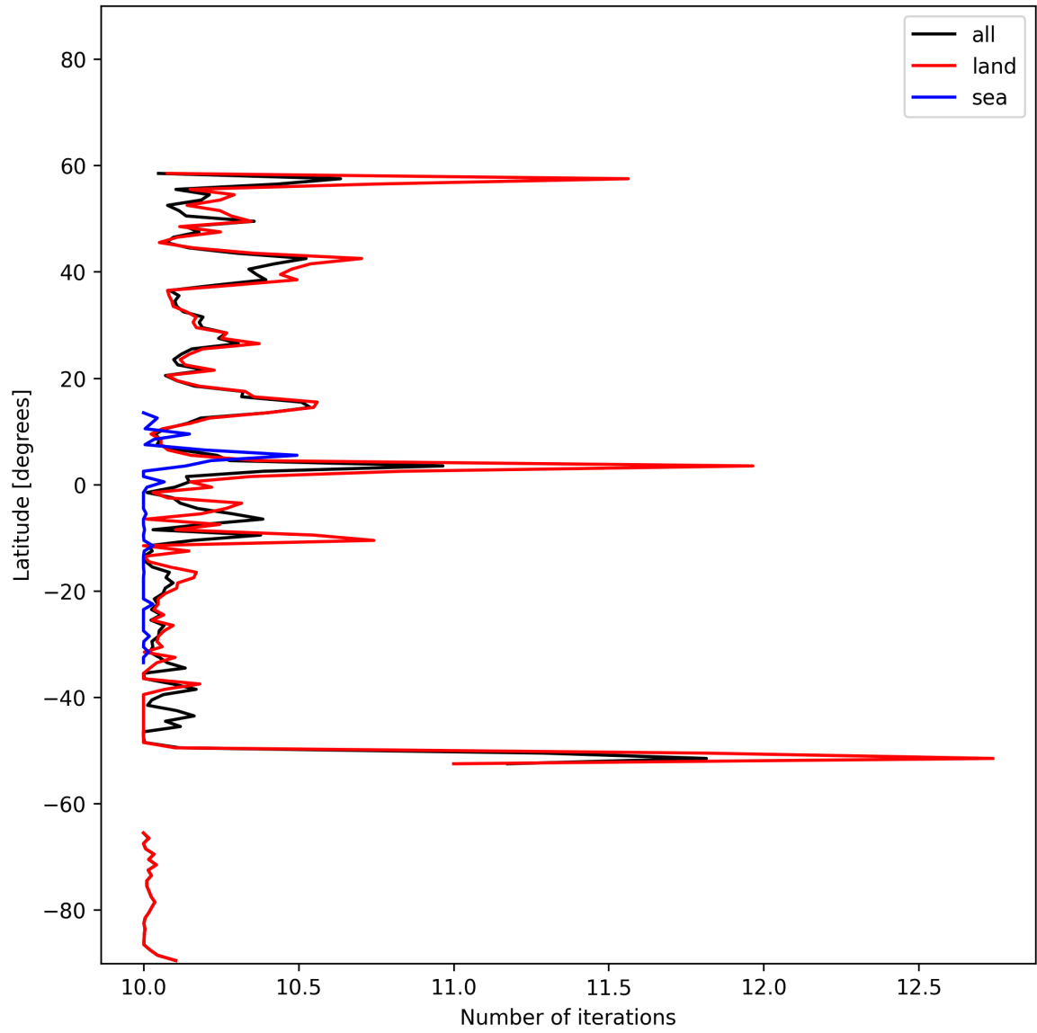
Figure 20: Zonal average of “Number of iterations” for 2025-11-07 to 2025-11-08.
