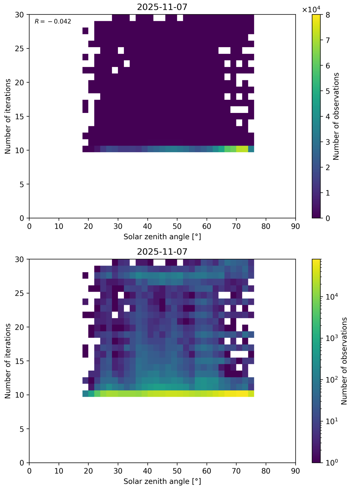
Figure 102: Scatter density plot of “Solar zenith angle” against “Number of iterations” for 2025-11-07 to 2025-11-08.
