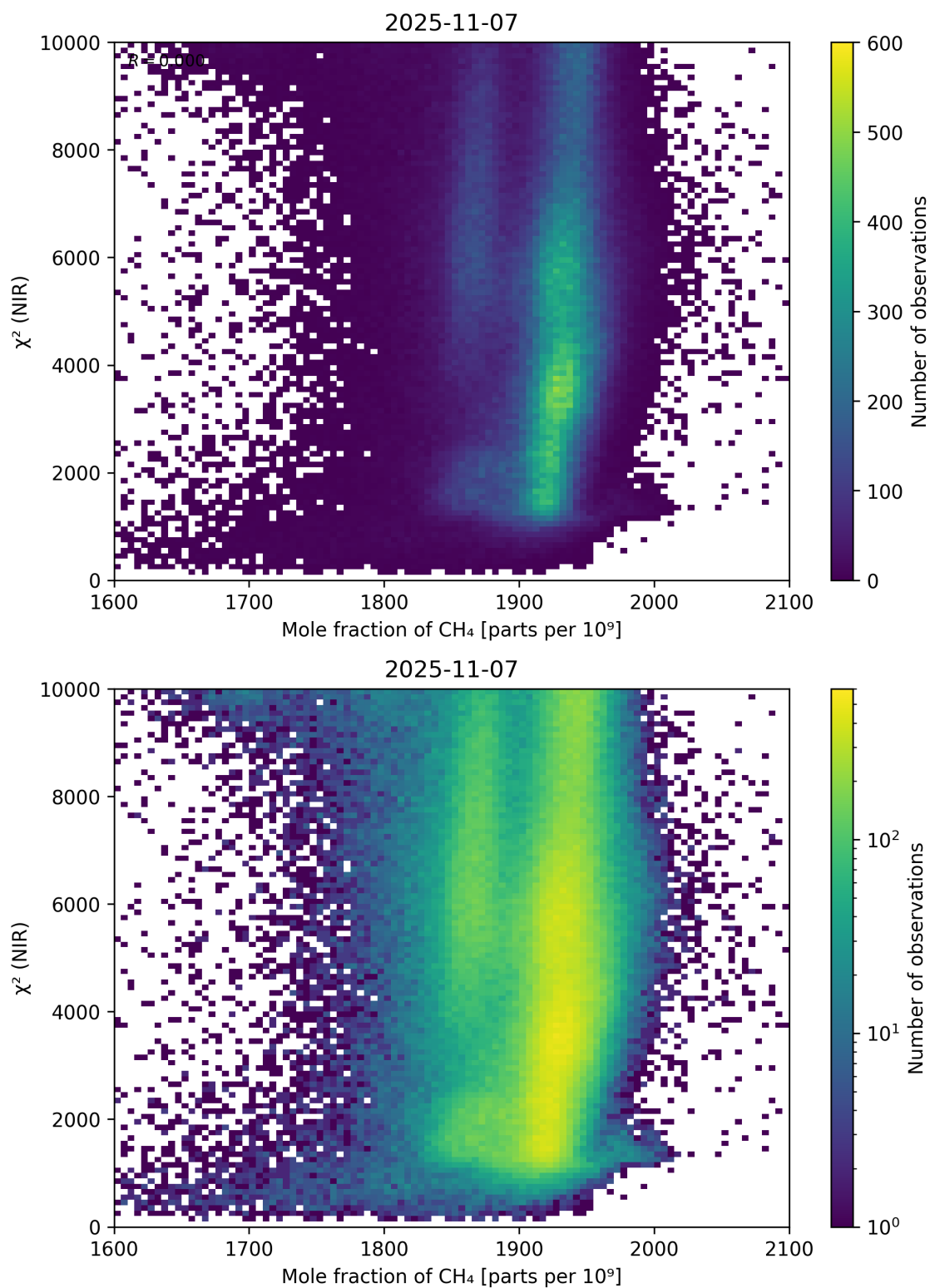
Figure 70: Scatter density plot of “Mole fraction of \text{CH}_4 ” against “ \chi^2 (NIR)” for 2025-11-07 to 2025-11-08.
