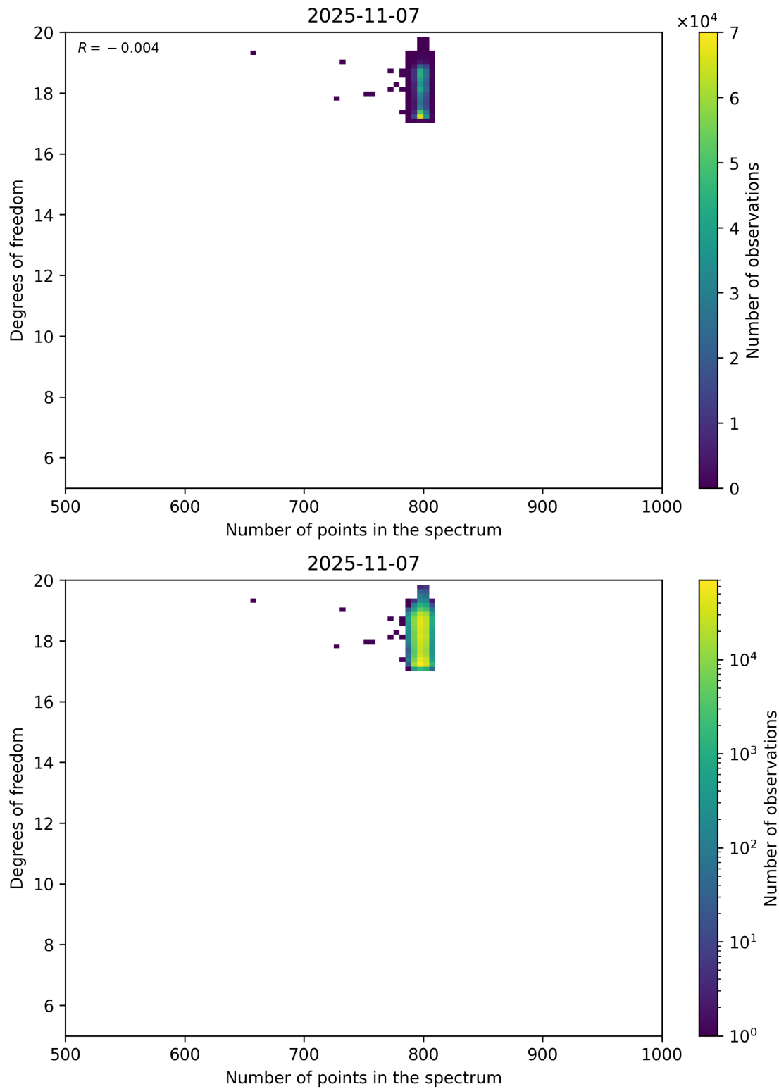
Figure 90: Scatter density plot of “Number of points in the spectrum” against “Degrees of freedom” for 2025-11-07 to 2025-11-08.
