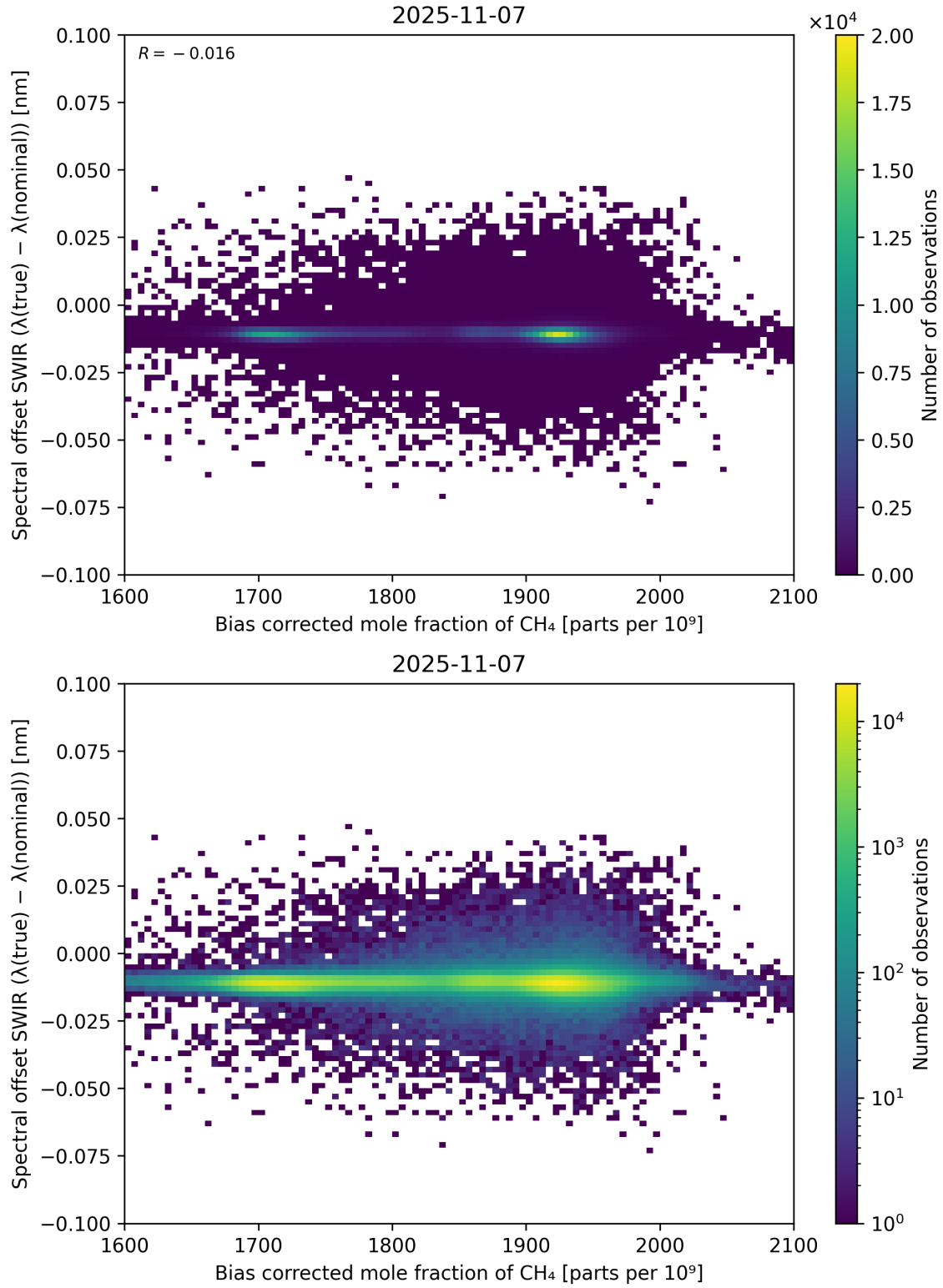
Figure 69: Scatter density plot of “Bias corrected mole fraction of \text{CH}_4 ” against “Spectral offset SWIR ( \lambda_{\text{true}} - \lambda_{\text{nominal}} )” for 2025-11-07 to 2025-11-08.
