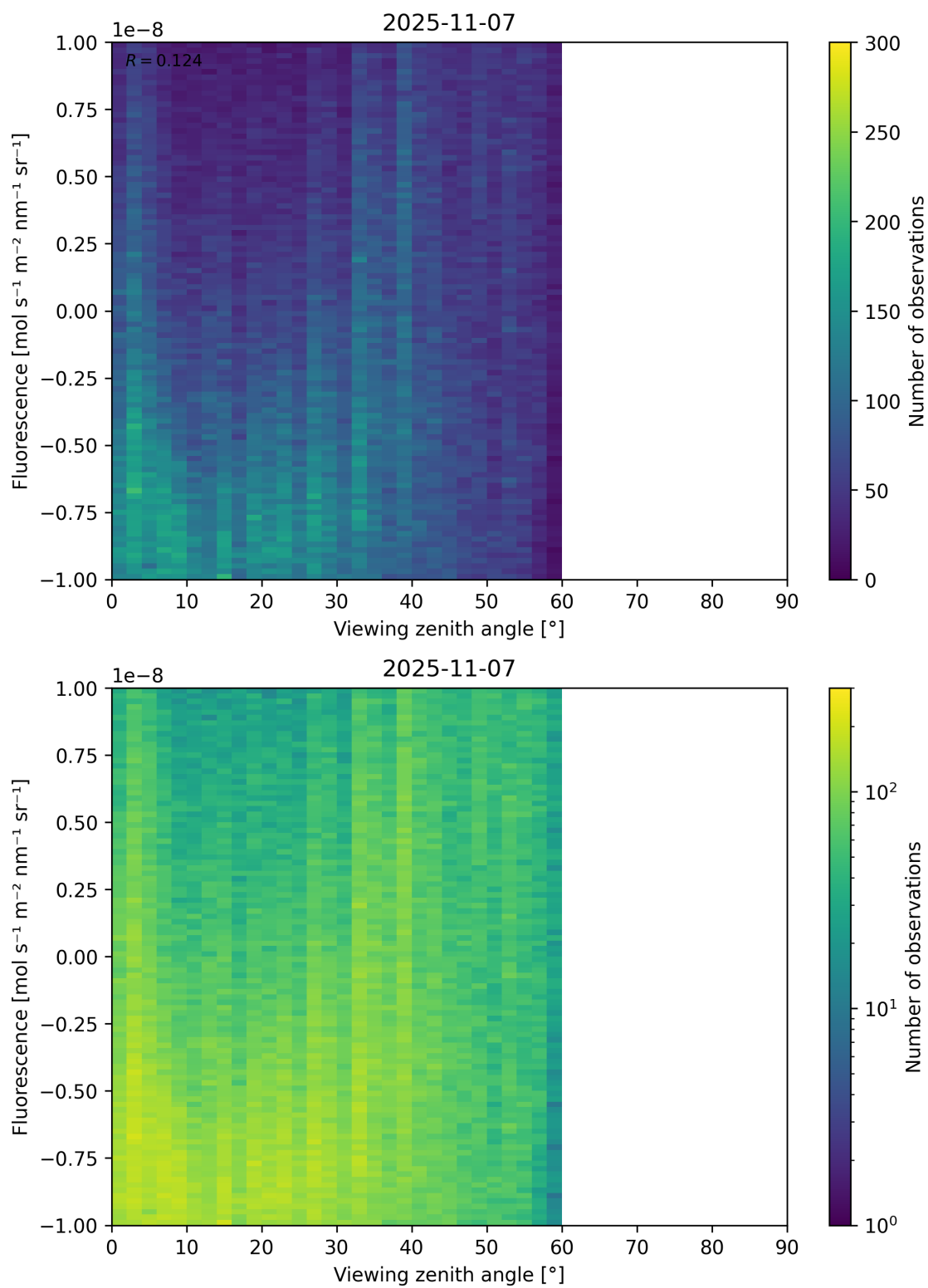
Figure 108: Scatter density plot of “Viewing zenith angle” against “Fluorescence” for 2025-11-07 to 2025-11-08.
