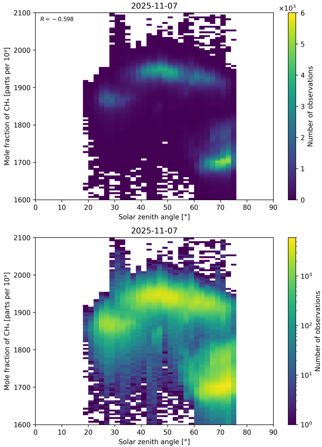
Figure 99: Scatter density plot of “Solar zenith angle” against “Mole fraction of CH 4 ” for 2025-11-07 to 2025-11-08.
