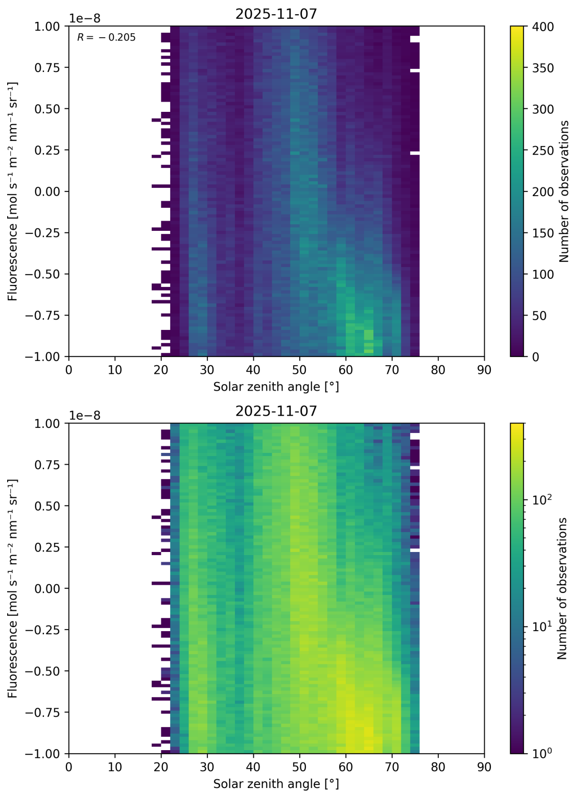
Figure 97: Scatter density plot of “Solar zenith angle” against “Fluorescence” for 2025-11-07 to 2025-11-08.
