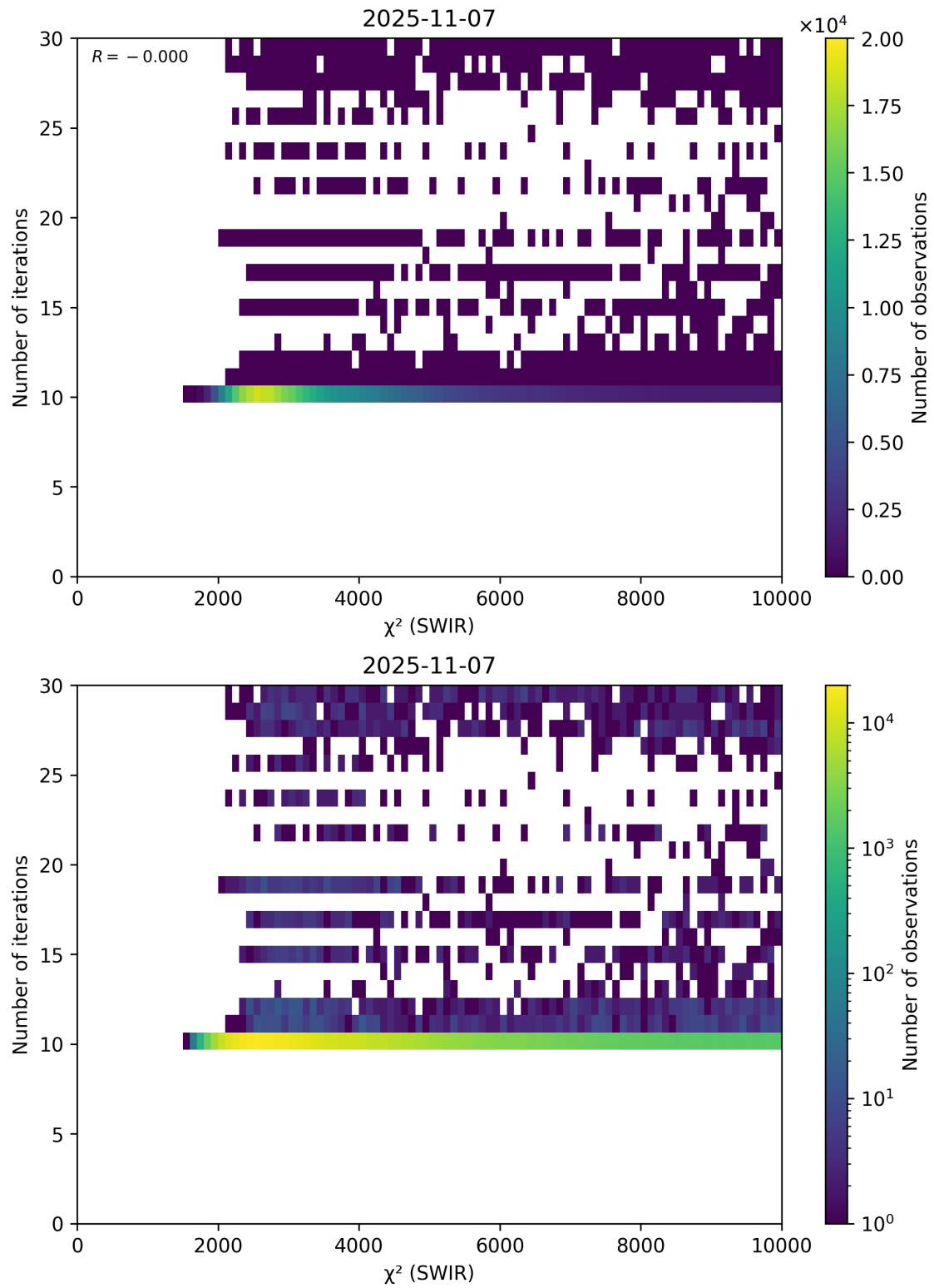
Figure 50: Scatter density plot of “ \chi^2 (SWIR)” against “Number of iterations” for 2025-11-07 to 2025-11-08.
