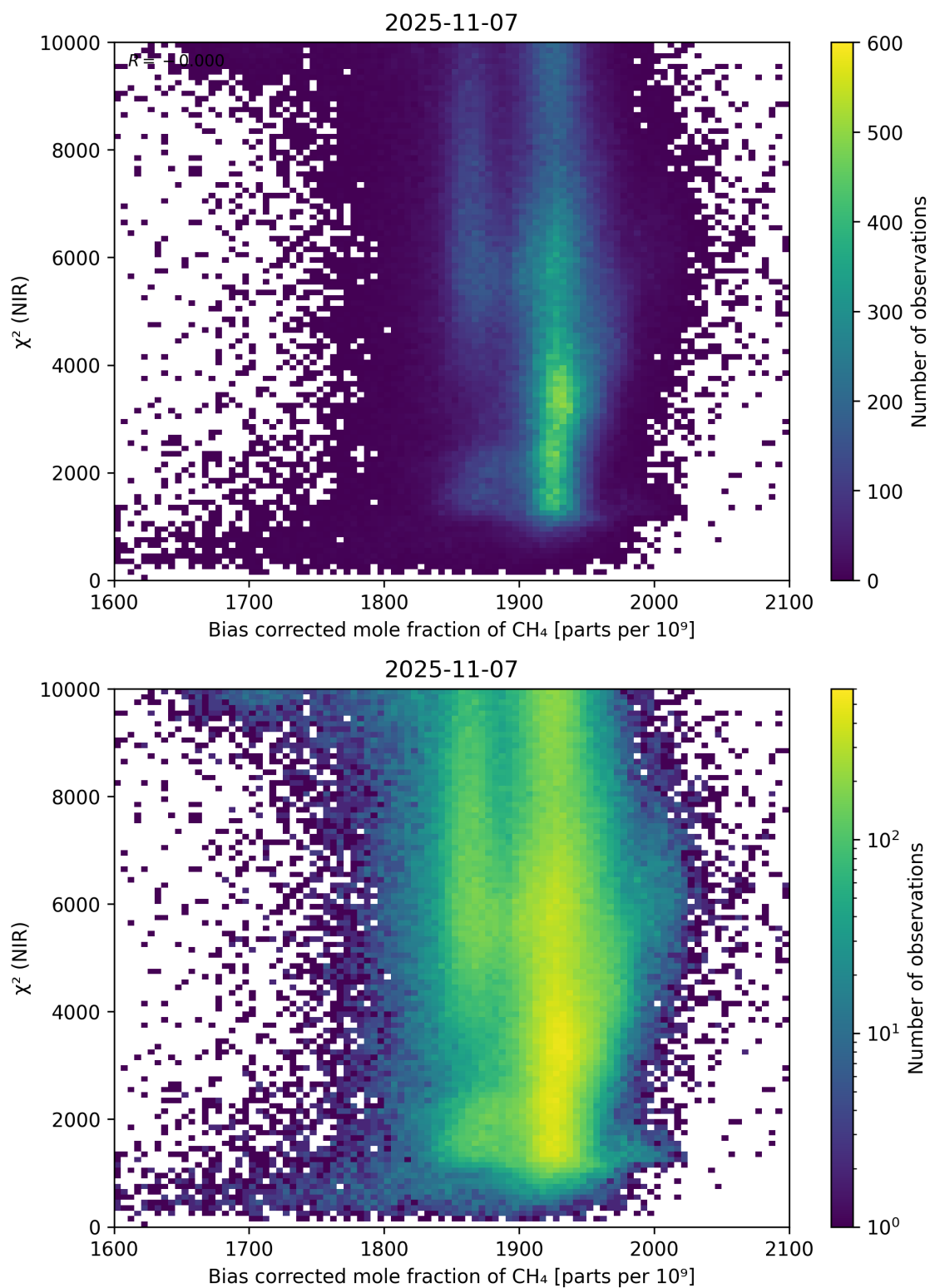
Figure 63: Scatter density plot of “Bias corrected mole fraction of CH 4 ” against “ \chi^2 (NIR)” for 2025-11-07 to 2025-11-08.
