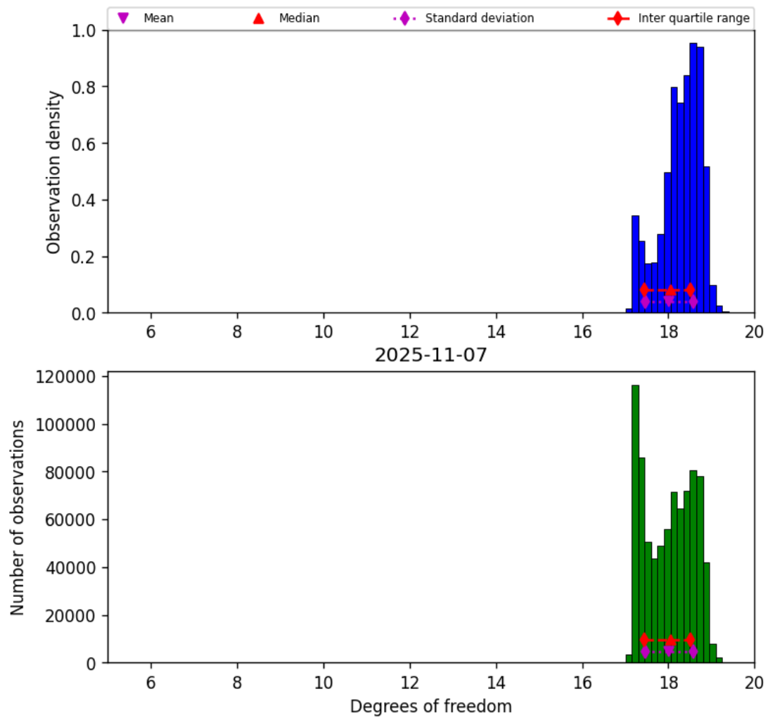
Figure 30: Histogram of “Degrees of freedom” for 2025-11-07 to 2025-11-08
