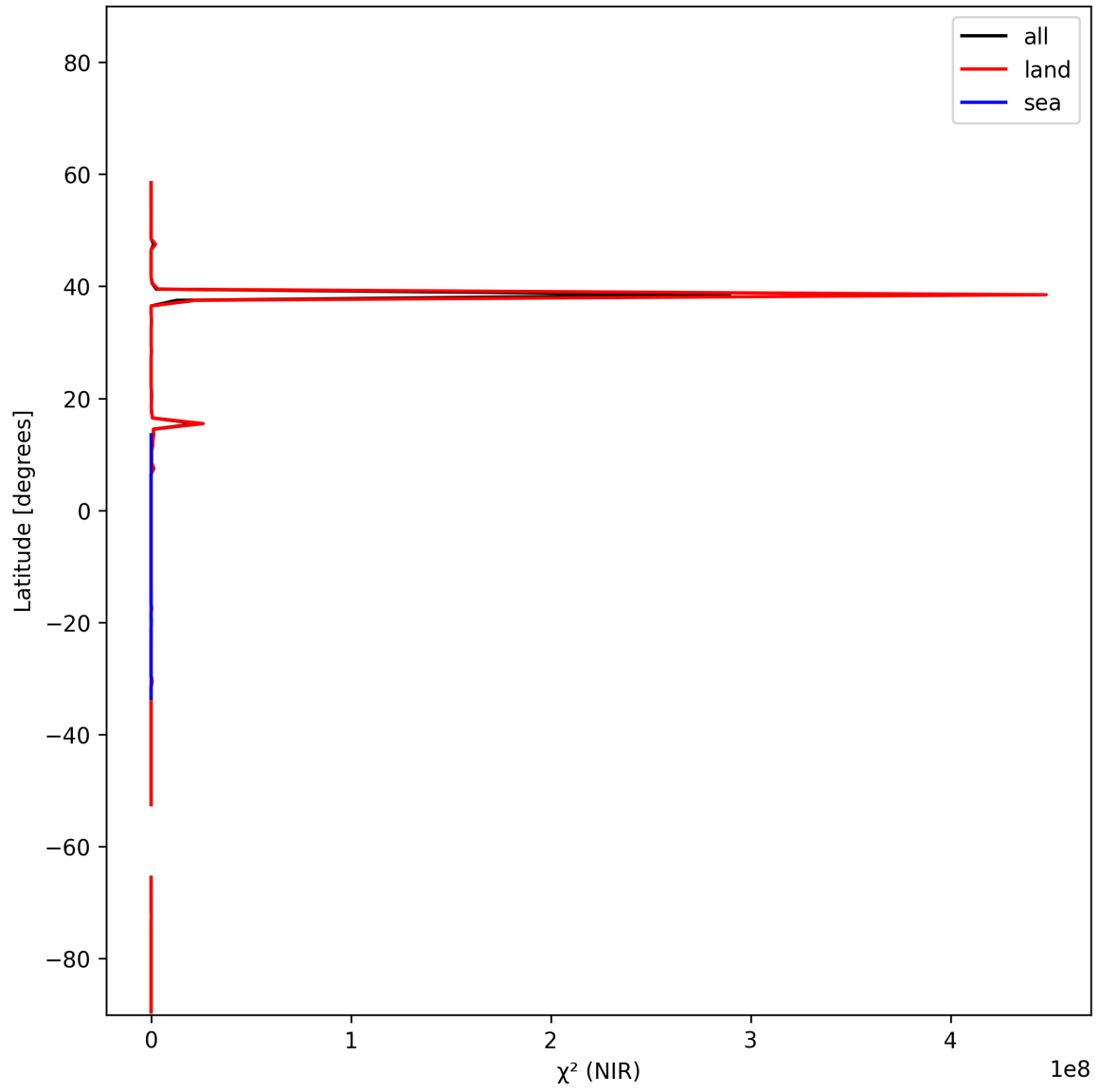
Figure 18: Zonal average of “ \chi^2 (NIR)” for 2025-11-07 to 2025-11-08.
