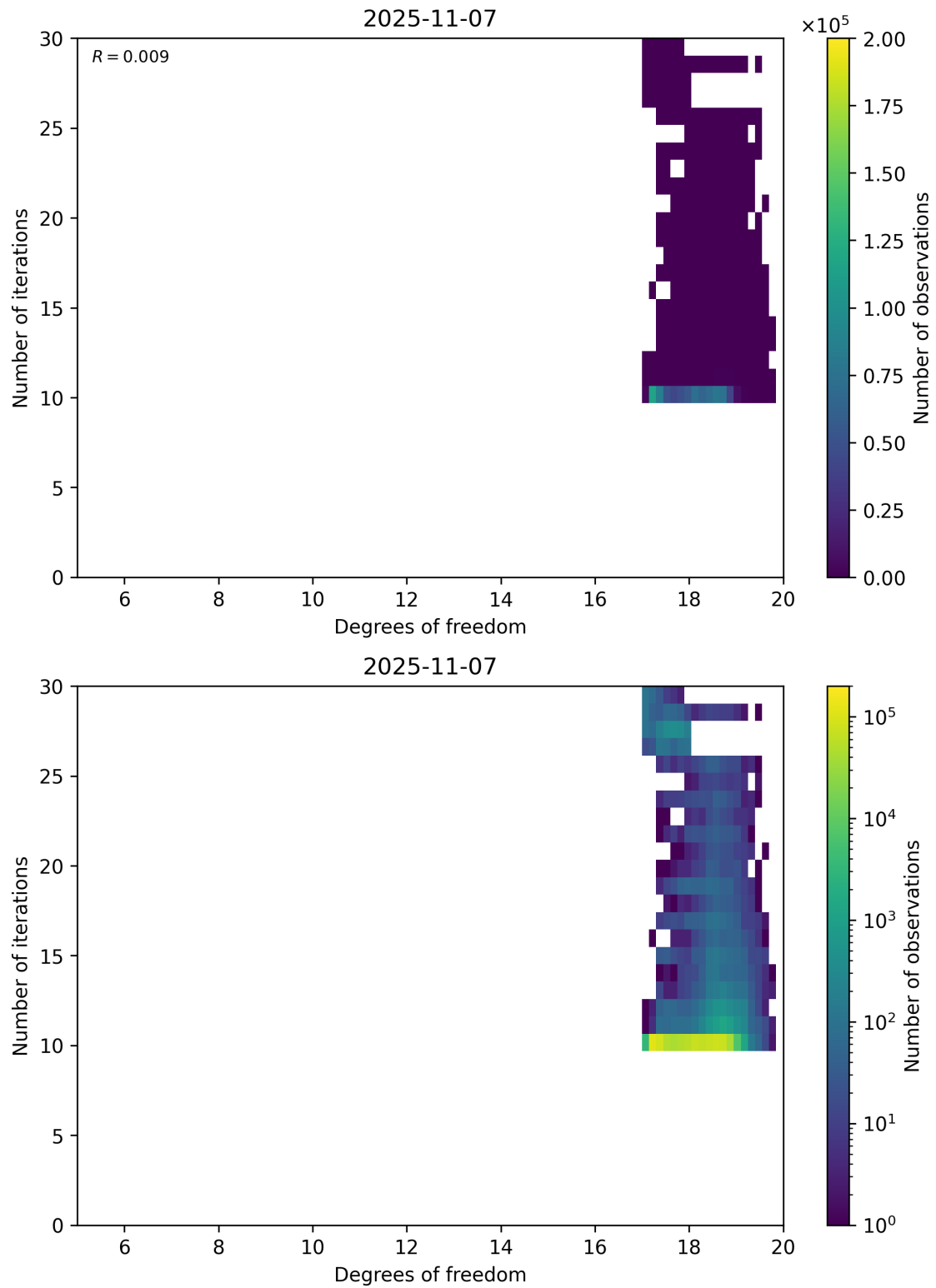
Figure 52: Scatter density plot of “Degrees of freedom” against “Number of iterations” for 2025-11-07 to 2025-11-08.
