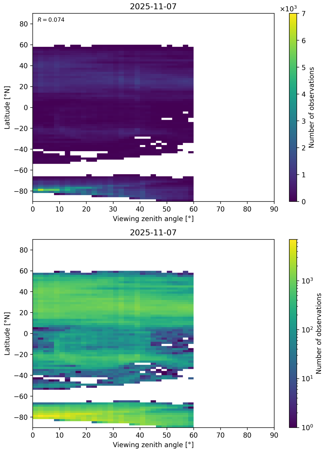
Figure 109: Scatter density plot of “Viewing zenith angle” against “Latitude” for 2025-11-07 to 2025-11-08.
