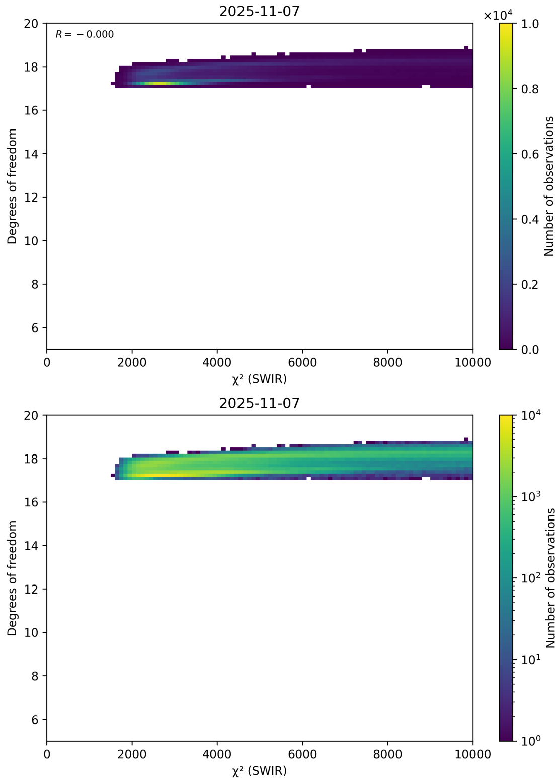
Figure 48: Scatter density plot of “ \chi^2 (SWIR)” against “Degrees of freedom” for 2025-11-07 to 2025-11-08.
