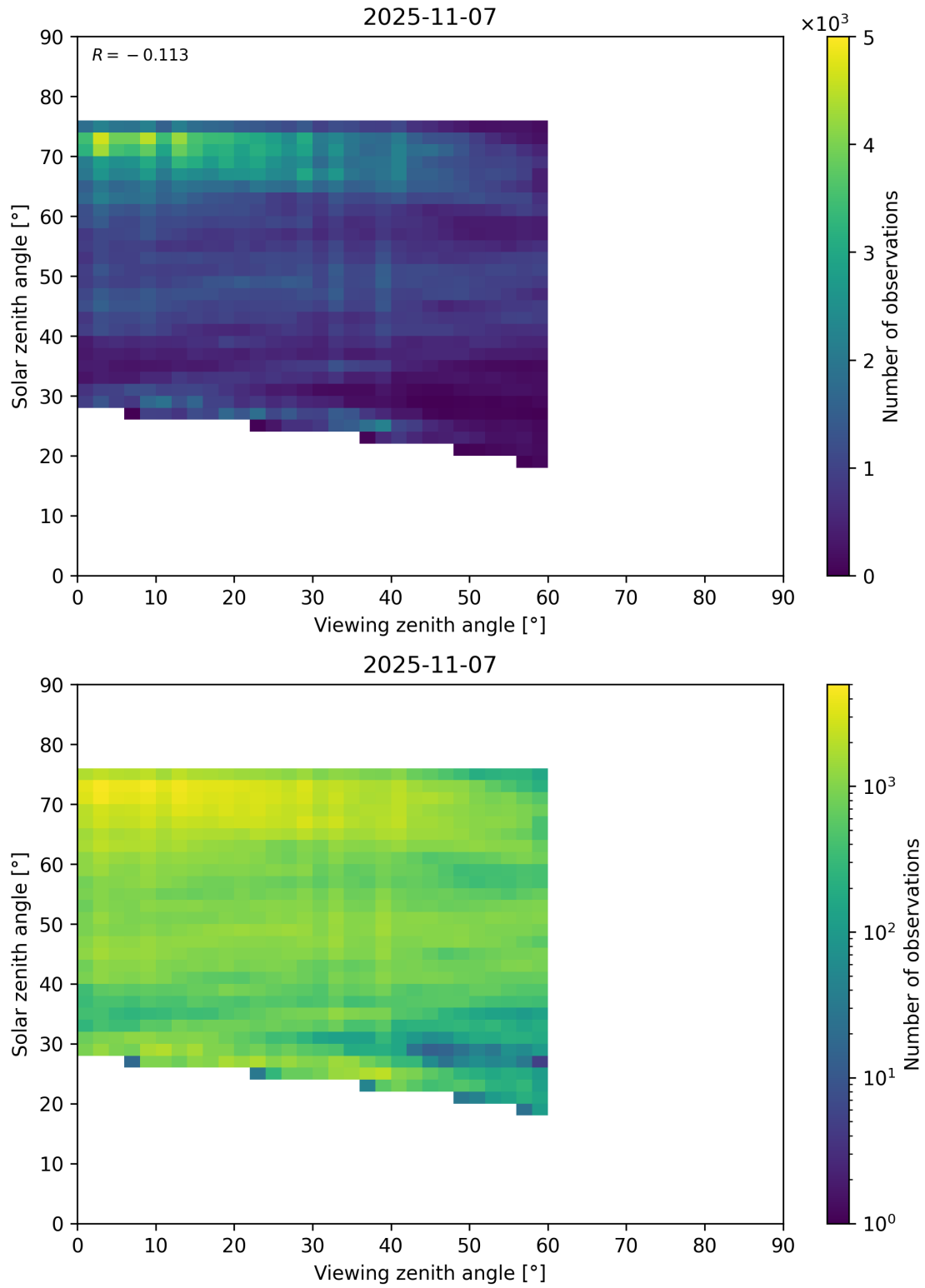
Figure 115: Scatter density plot of “Viewing zenith angle” against “Solar zenith angle” for 2025-11-07 to 2025-11-08.
