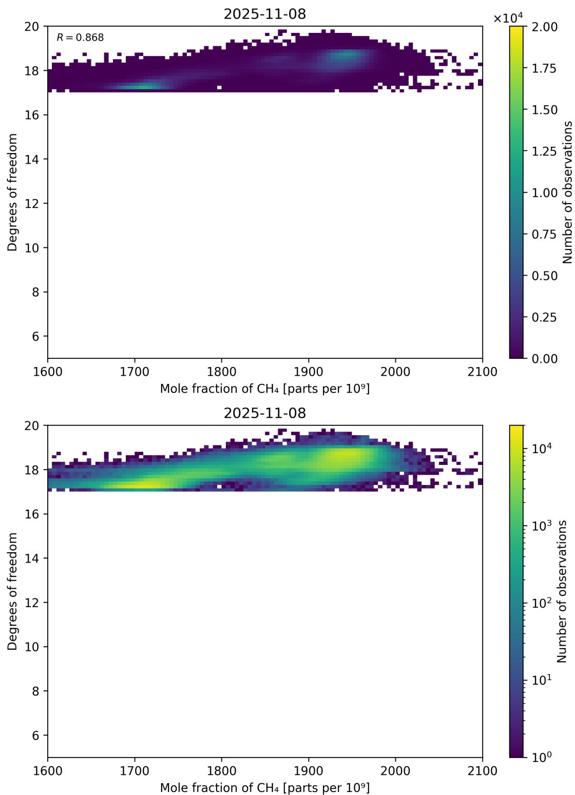
Figure 72: Scatter density plot of “Mole fraction of CH 4 ” against “Degrees of freedom” for 2025-11-07 to 2025-11-09.
