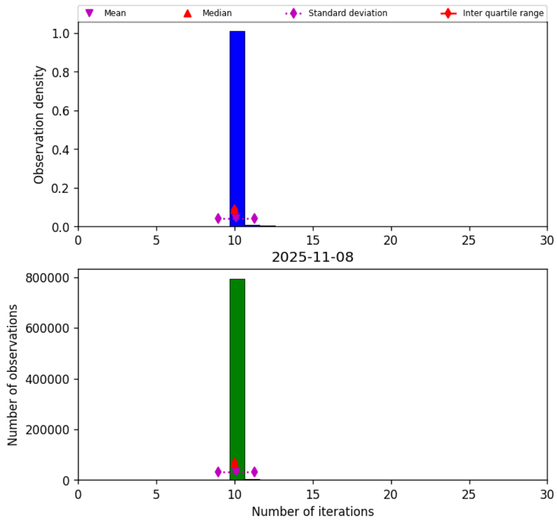
Figure 31: Histogram of “Number of iterations” for 2025-11-07 to 2025-11-09
