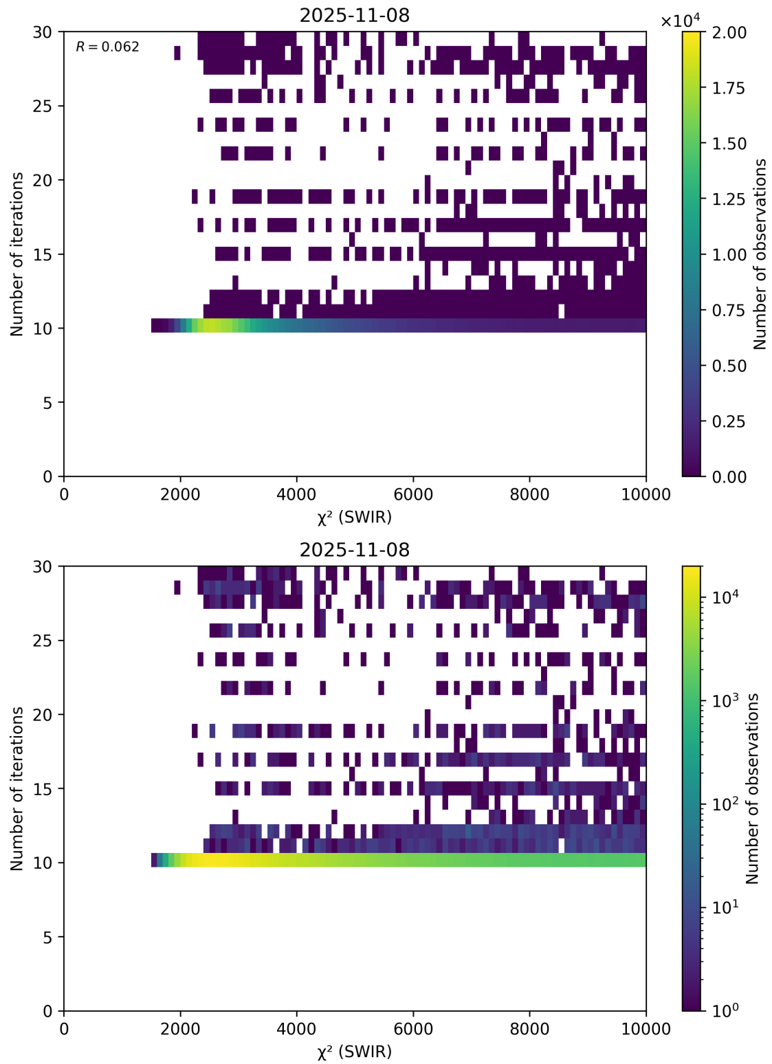
Figure 50: Scatter density plot of “ \chi^2 (SWIR)” against “Number of iterations” for 2025-11-07 to 2025-11-09.
