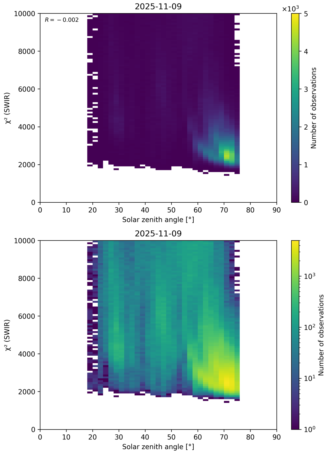
Figure 95: Scatter density plot of “Solar zenith angle” against “ \chi^2 (SWIR)” for 2025-11-08 to 2025-11-10.
