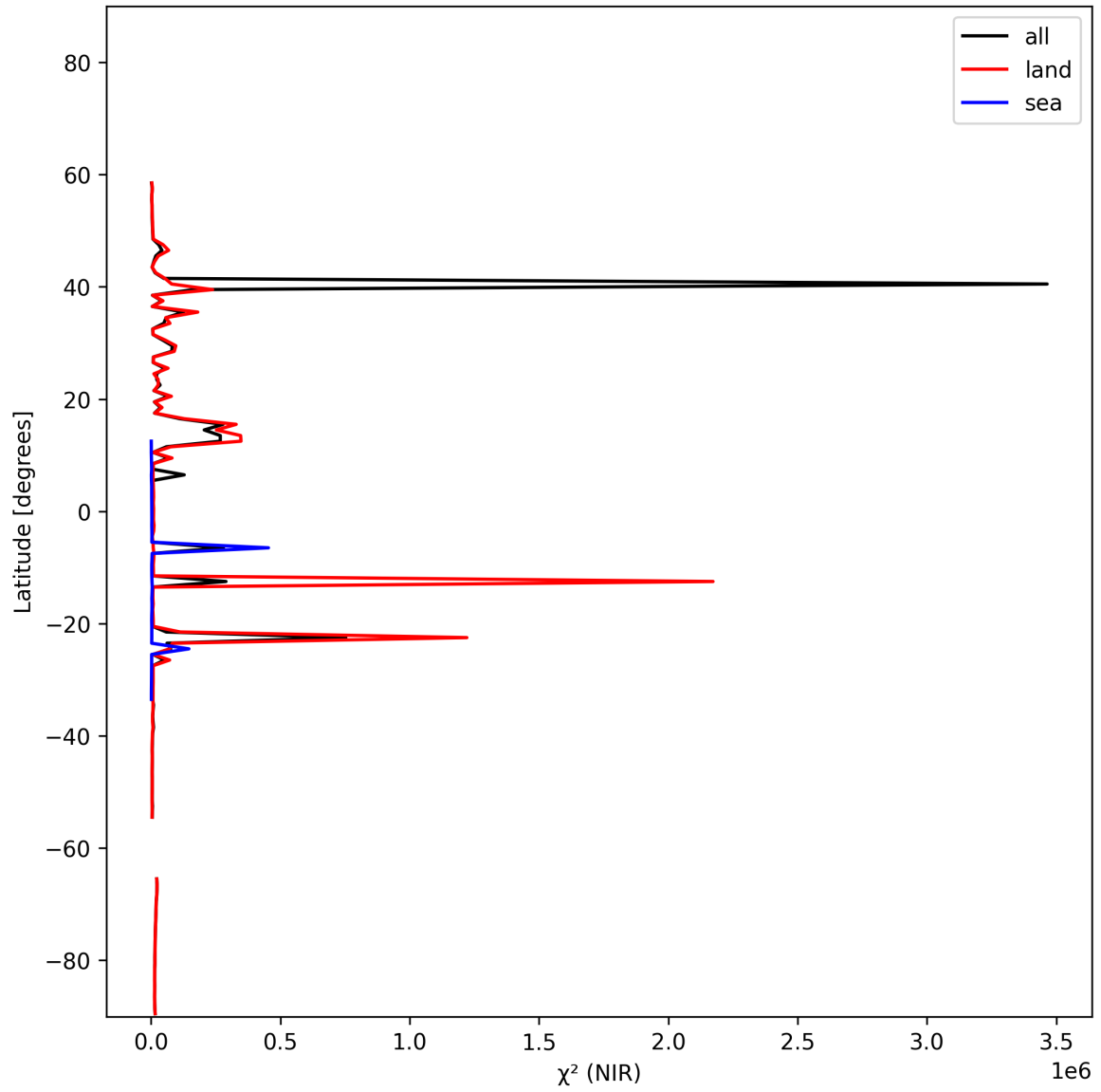
Figure 18: Zonal average of “ \chi^2 (NIR)” for 2025-11-08 to 2025-11-10.
