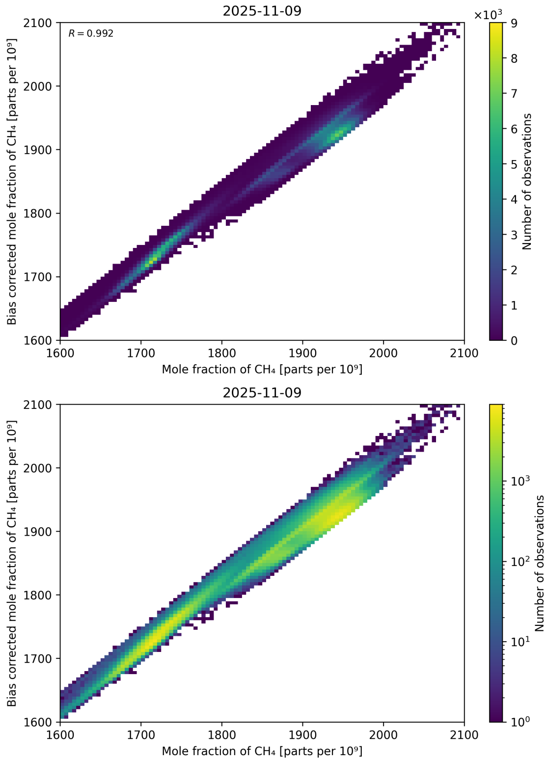
Figure 74: Scatter density plot of “Mole fraction of CH 4 ” against “Bias corrected mole fraction of CH 4 ” for 2025-11-08 to 2025-11-10.
