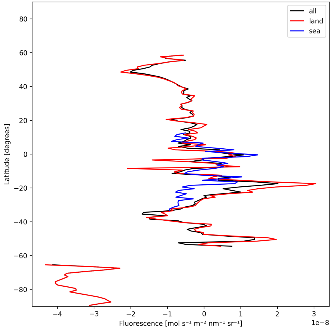
Figure 21: Zonal average of “Fluorescence” for 2025-11-08 to 2025-11-10.
