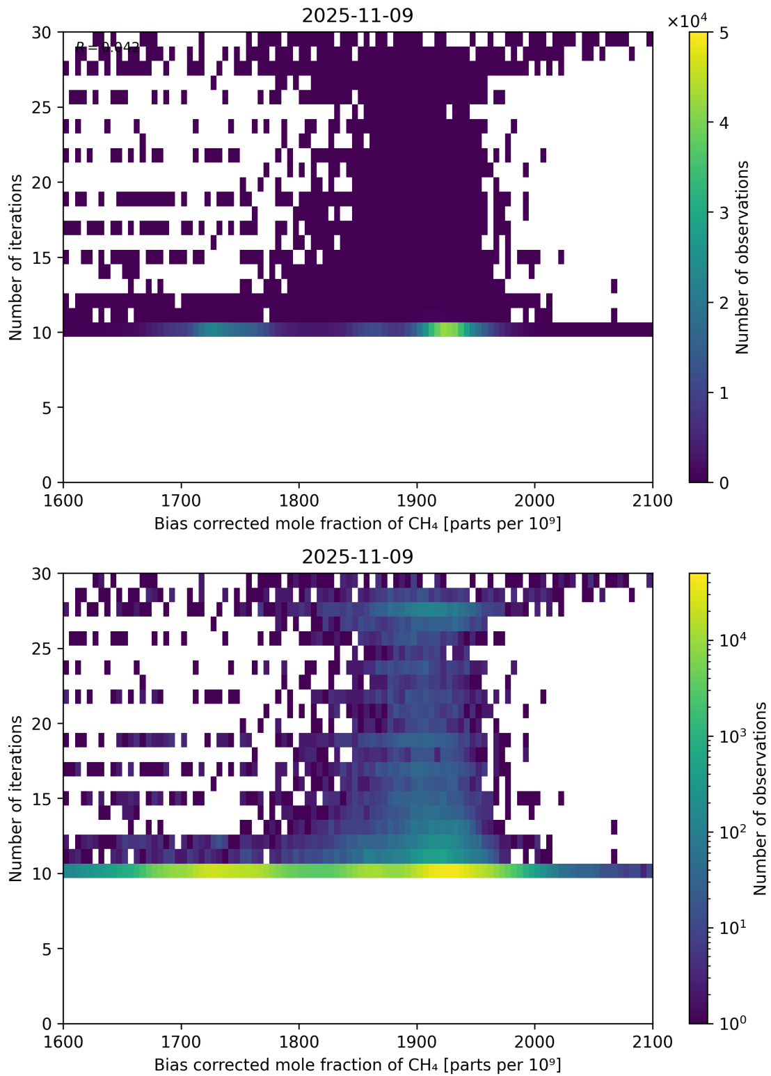
Figure 67: Scatter density plot of “Bias corrected mole fraction of CH 4 ” against “Number of iterations” for 2025-11-08 to 2025-11-10.
