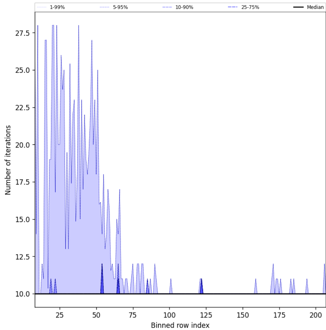
Figure 42: Along track statistics of “Number of iterations” for 2025-11-08 to 2025-11-10
