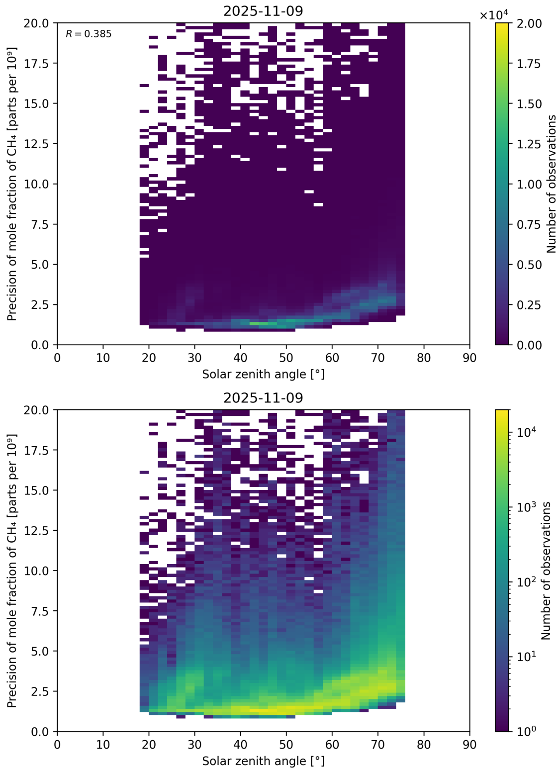
Figure 101: Scatter density plot of “Solar zenith angle” against “Precision of mole fraction of CH 4 ” for 2025-11-08 to 2025-11-10.
