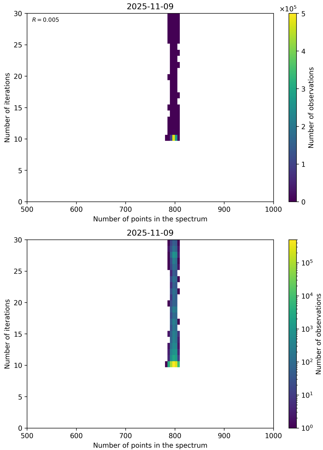
Figure 92: Scatter density plot of “Number of points in the spectrum” against “Number of iterations” for 2025-11-08 to 2025-11-10.
