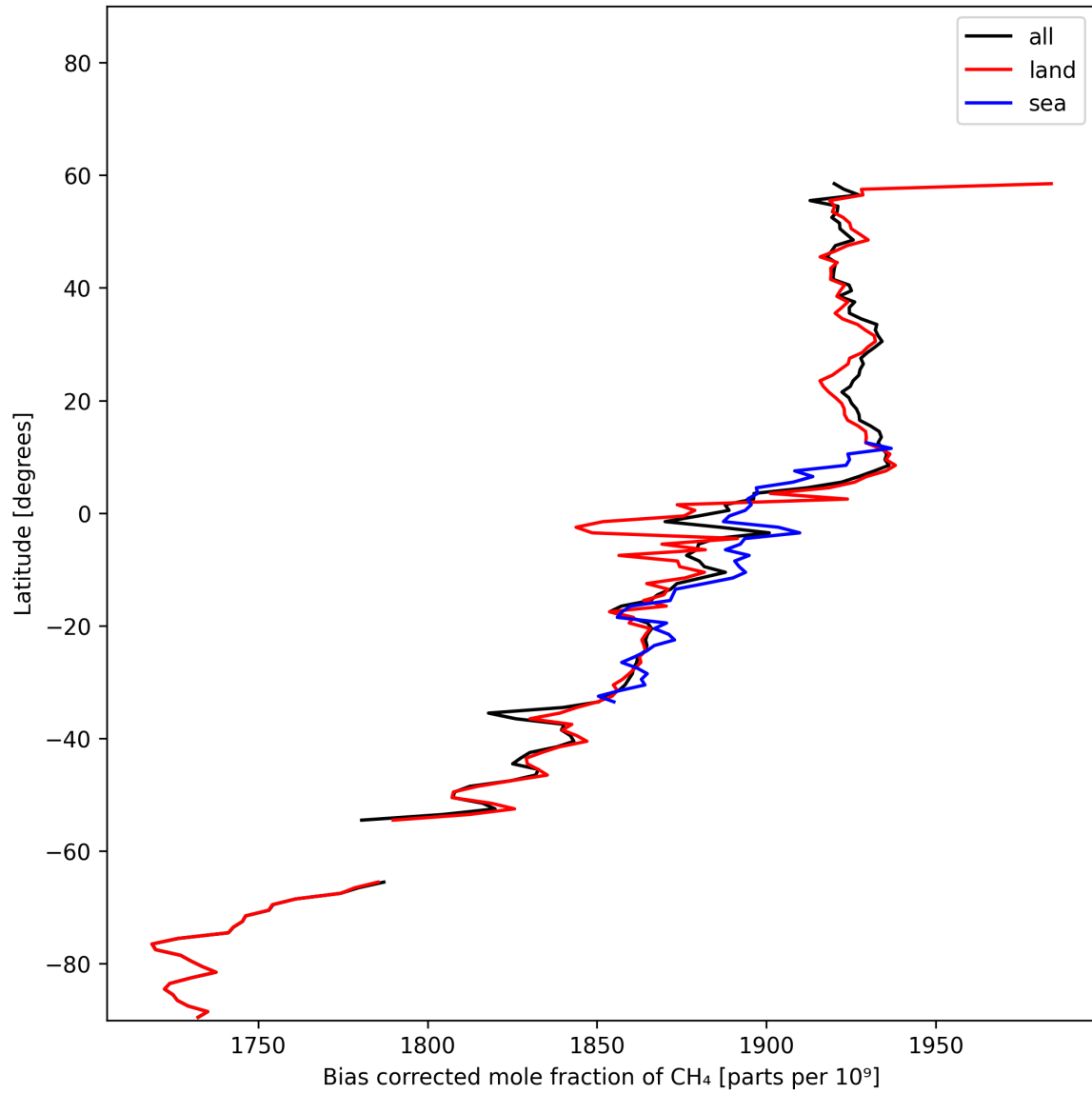
Figure 14: Zonal average of “Bias corrected mole fraction of CH 4 ” for 2025-11-08 to 2025-11-10.
