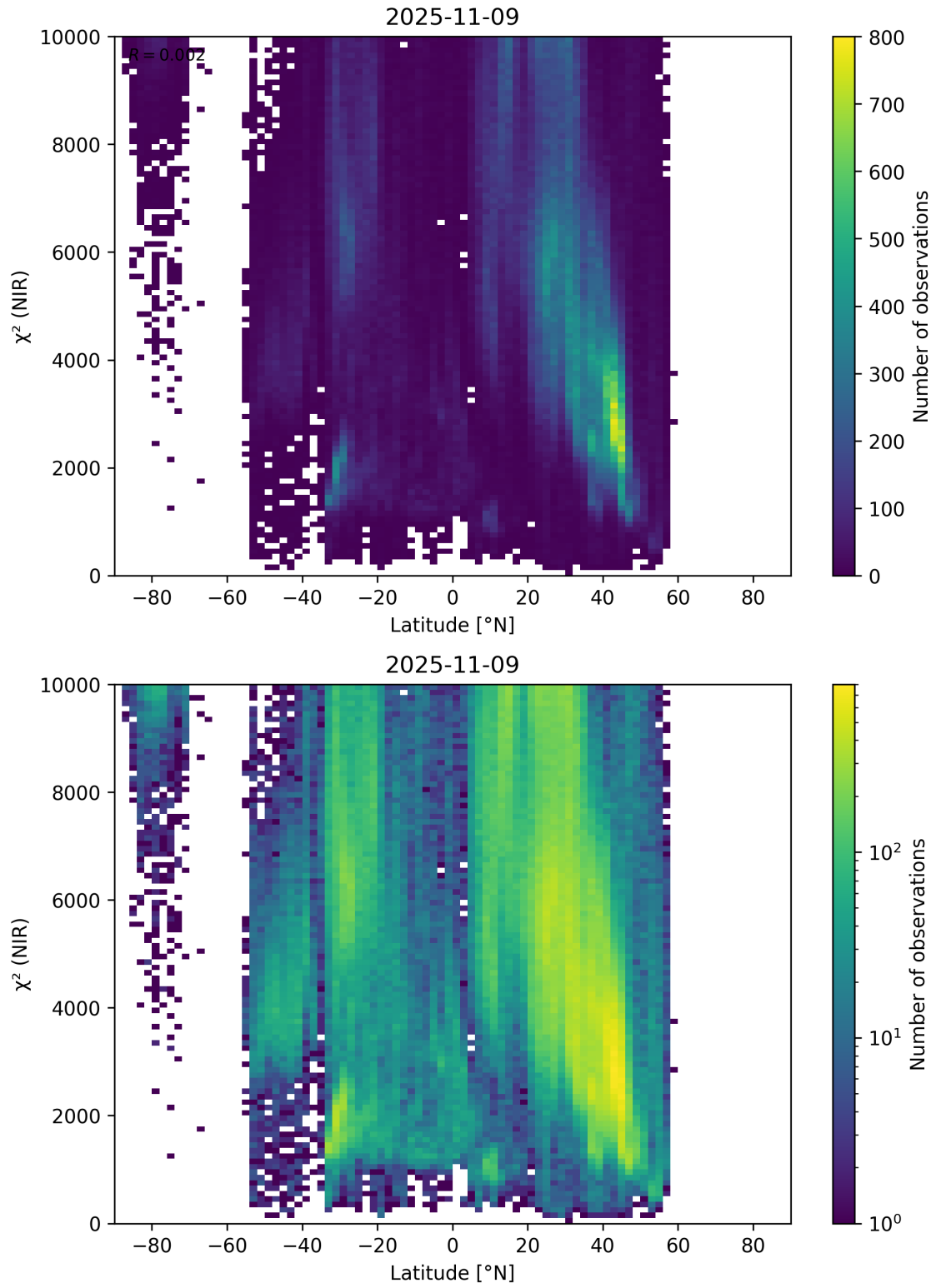
Figure 53: Scatter density plot of “Latitude” against “ \chi^2 (NIR)” for 2025-11-08 to 2025-11-10.
