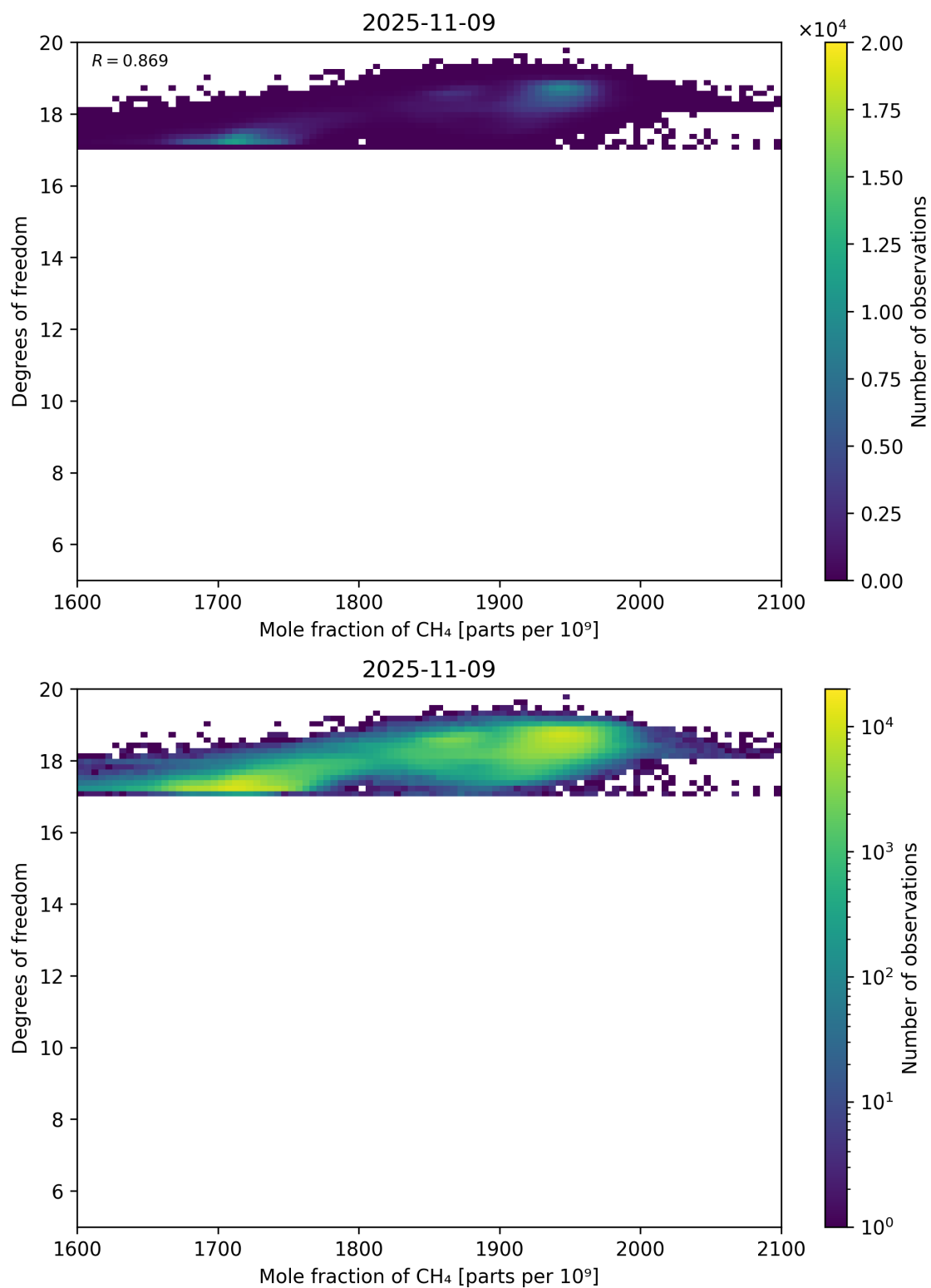
Figure 72: Scatter density plot of “Mole fraction of CH 4 ” against “Degrees of freedom” for 2025-11-08 to 2025-11-10.
