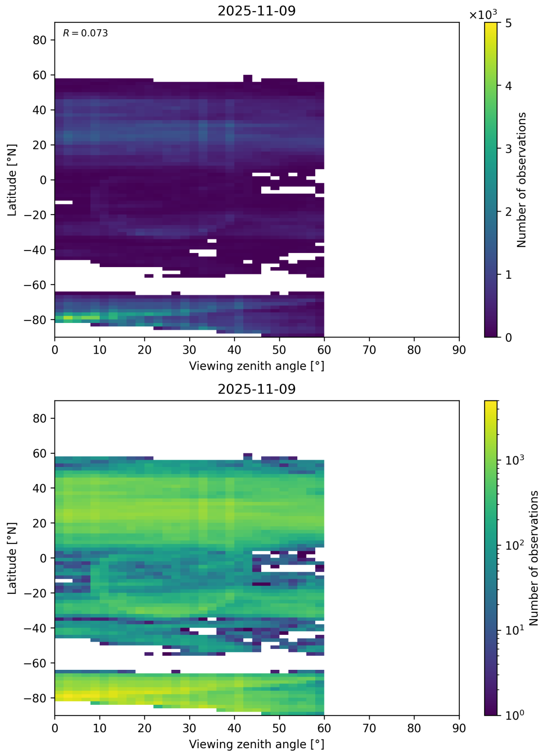
Figure 109: Scatter density plot of “Viewing zenith angle” against “Latitude” for 2025-11-08 to 2025-11-10.
