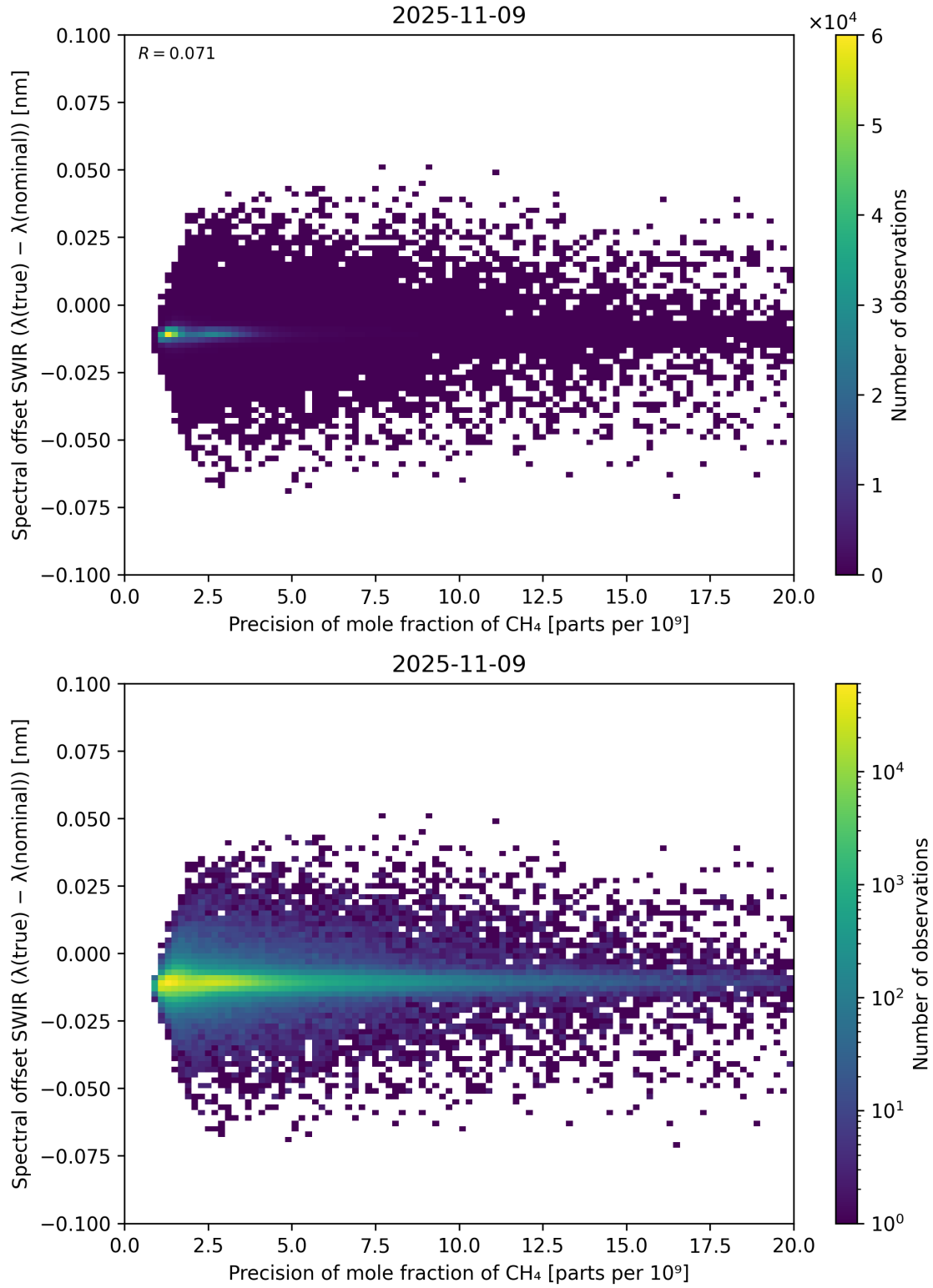
Figure 85: Scatter density plot of “Precision of mole fraction of \text{CH}_4 ” against “Spectral offset SWIR ( \lambda_{\text{true}} - \lambda_{\text{nominal}} )” for 2025-11-08 to 2025-11-10.
