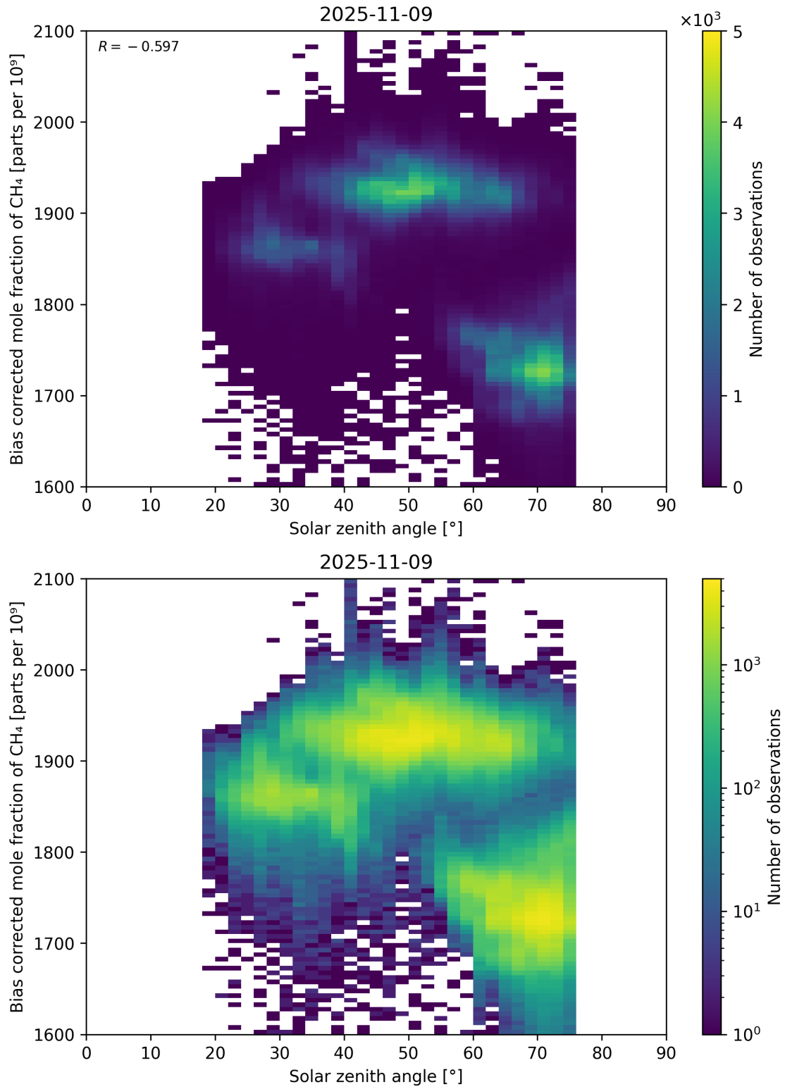
Figure 100: Scatter density plot of “Solar zenith angle” against “Bias corrected mole fraction of CH 4 ” for 2025-11-08 to 2025-11-10.
