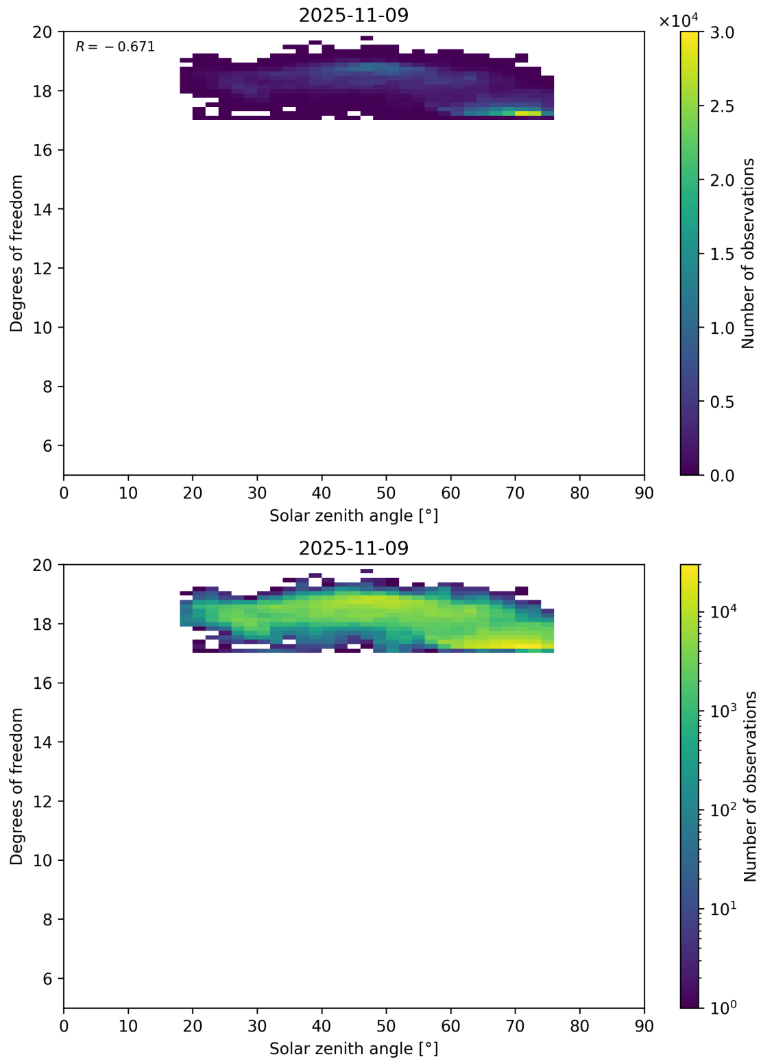
Figure 96: Scatter density plot of “Solar zenith angle” against “Degrees of freedom” for 2025-11-08 to 2025-11-10.
