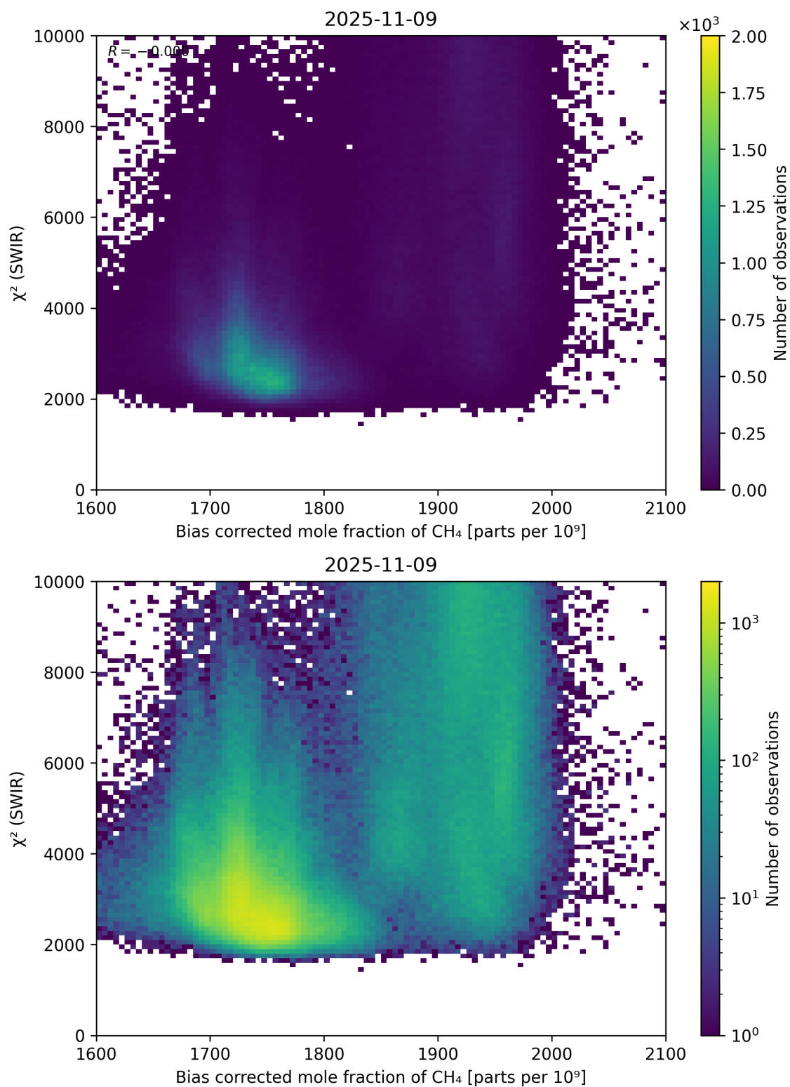
Figure 64: Scatter density plot of “Bias corrected mole fraction of CH 4 ” against “ \chi^2 (SWIR)” for 2025-11-08 to 2025-11-10.
