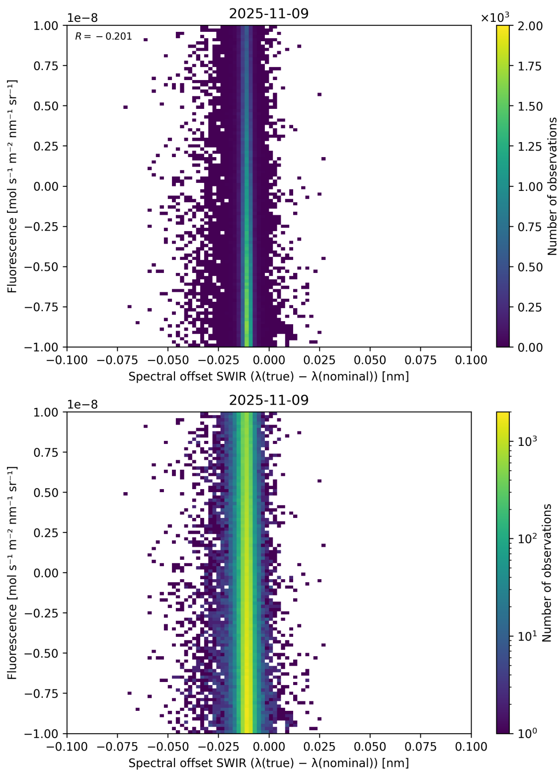
Figure 120: Scatter density plot of “Spectral offset SWIR ( \lambda_{\text{true}} - \lambda_{\text{nominal}} )” against “Fluorescence” for 2025-11-08 to 2025-11-10.
