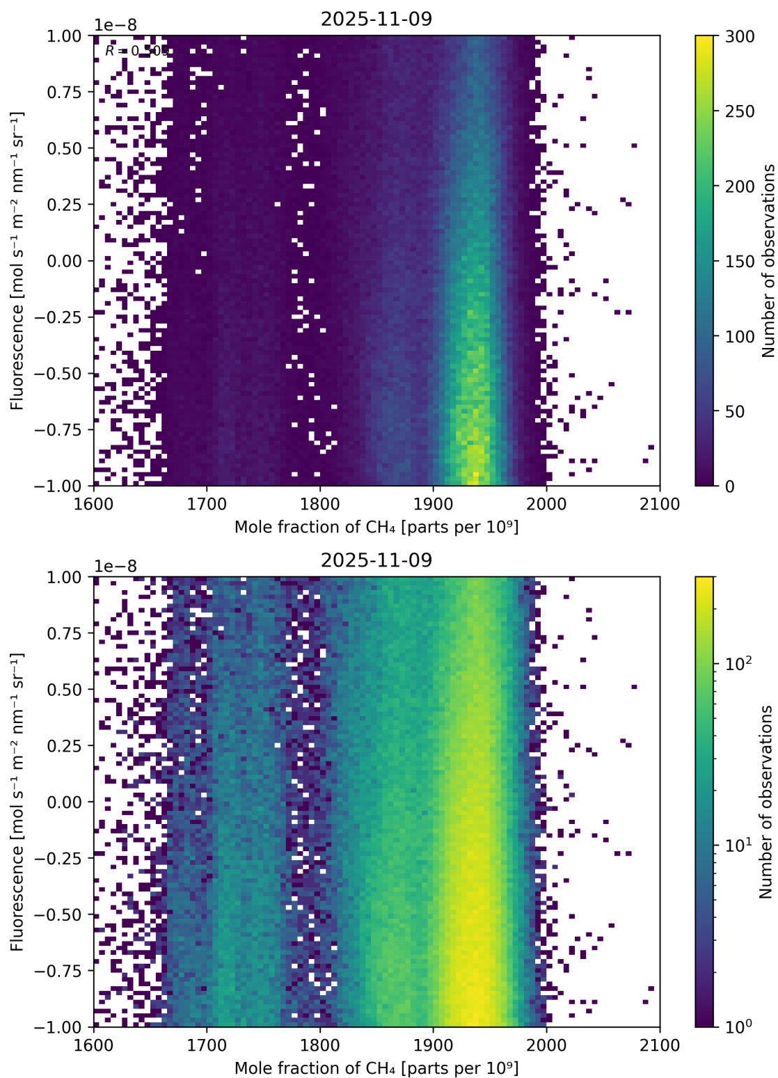
Figure 73: Scatter density plot of “Mole fraction of CH 4 ” against “Fluorescence” for 2025-11-08 to 2025-11-10.
