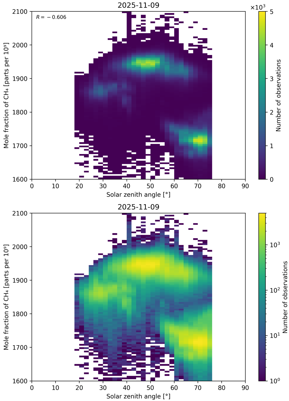
Figure 99: Scatter density plot of “Solar zenith angle” against “Mole fraction of CH 4 ” for 2025-11-08 to 2025-11-10.
