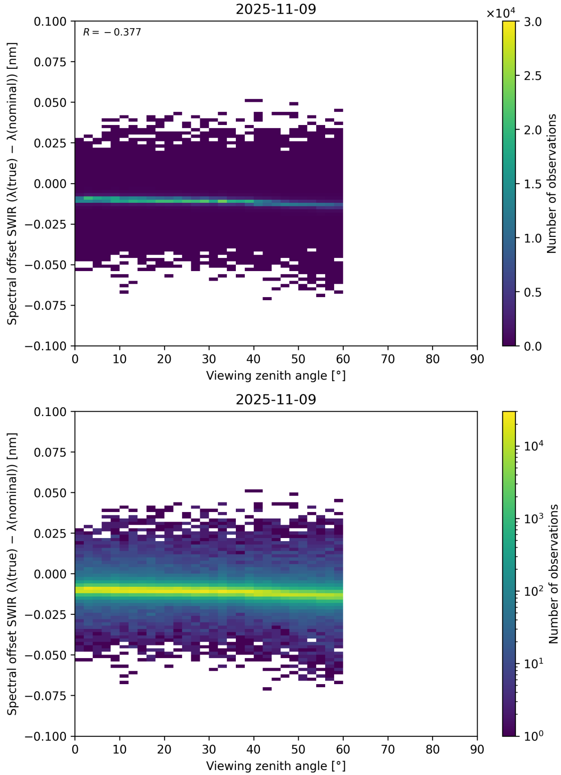
Figure 116: Scatter density plot of “Viewing zenith angle” against “Spectral offset SWIR ( \lambda_{\text{true}} - \lambda_{\text{nominal}} )” for 2025-11-08 to 2025-11-10.
