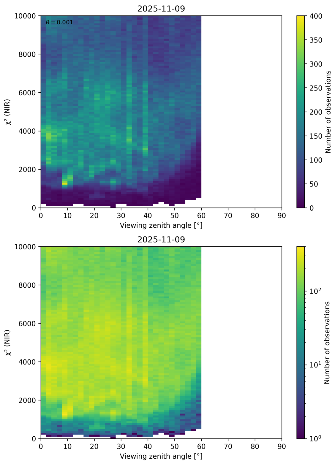
Figure 105: Scatter density plot of “Viewing zenith angle” against “ \chi^2 (NIR)” for 2025-11-08 to 2025-11-10.
