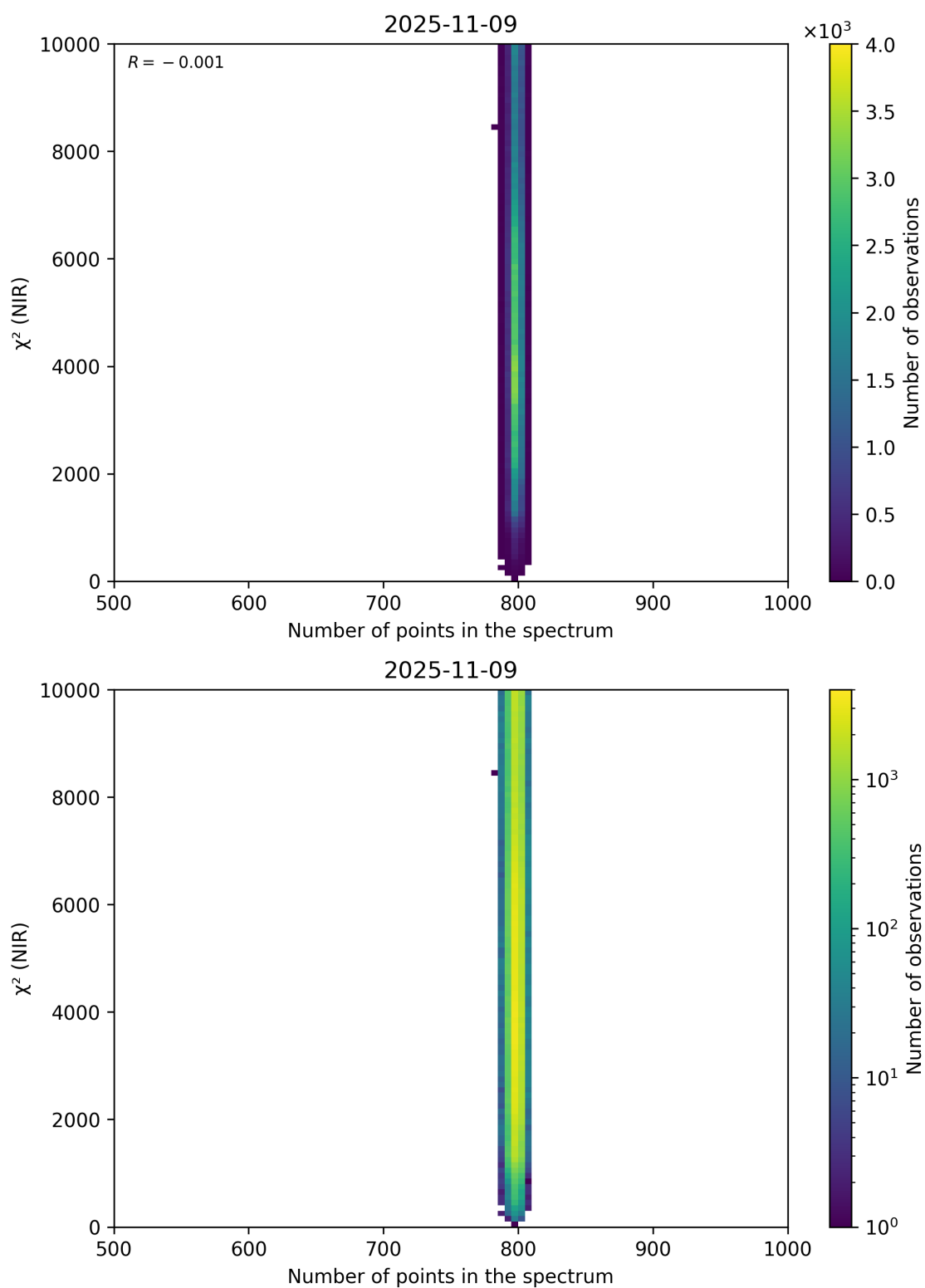
Figure 88: Scatter density plot of “Number of points in the spectrum” against “ \chi^2 (NIR)” for 2025-11-08 to 2025-11-10.
