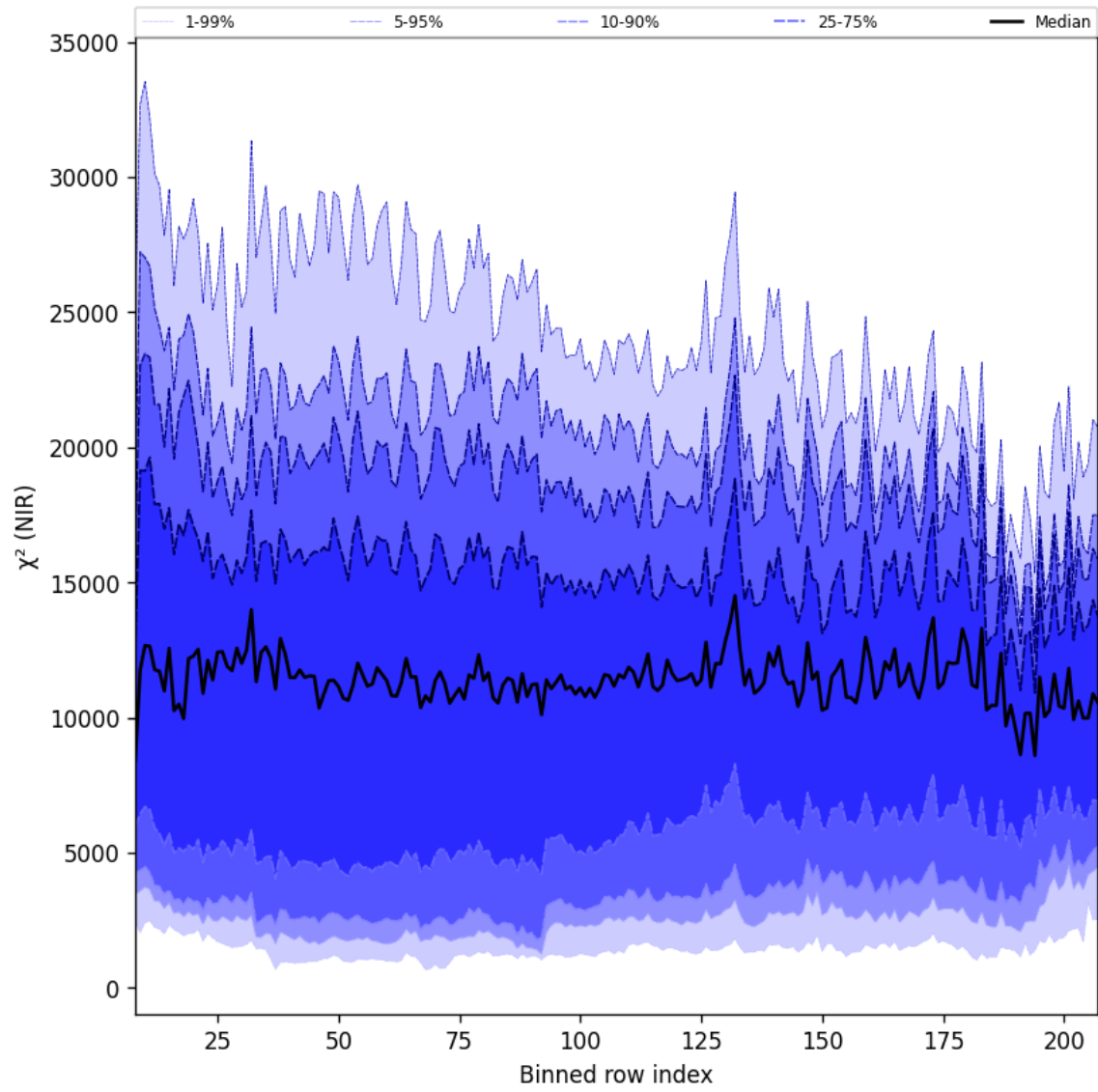
Figure 40: Along track statistics of " \chi^2 (NIR)" for 2025-11-08 to 2025-11-10
