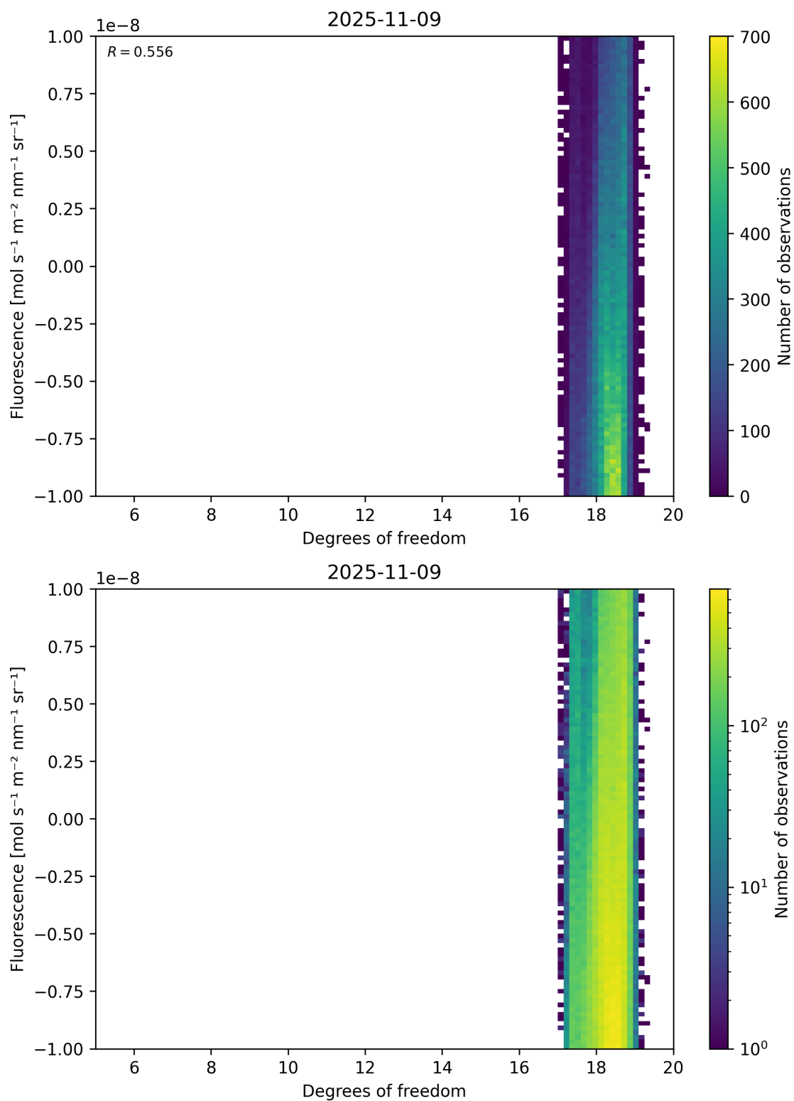
Figure 51: Scatter density plot of “Degrees of freedom” against “Fluorescence” for 2025-11-08 to 2025-11-10.
