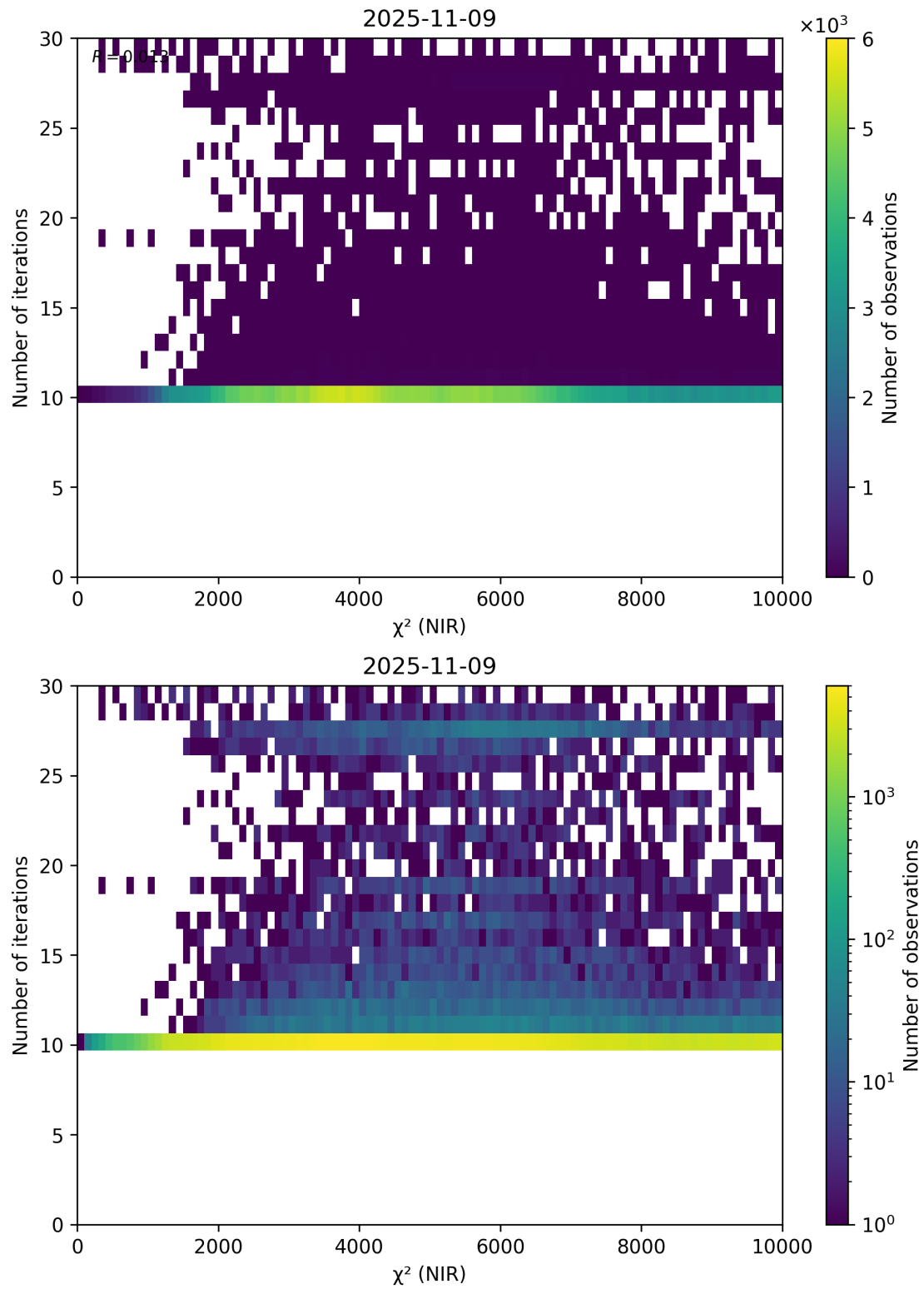
Figure 46: Scatter density plot of “ \chi^2 (NIR)” against “Number of iterations” for 2025-11-08 to 2025-11-10.
