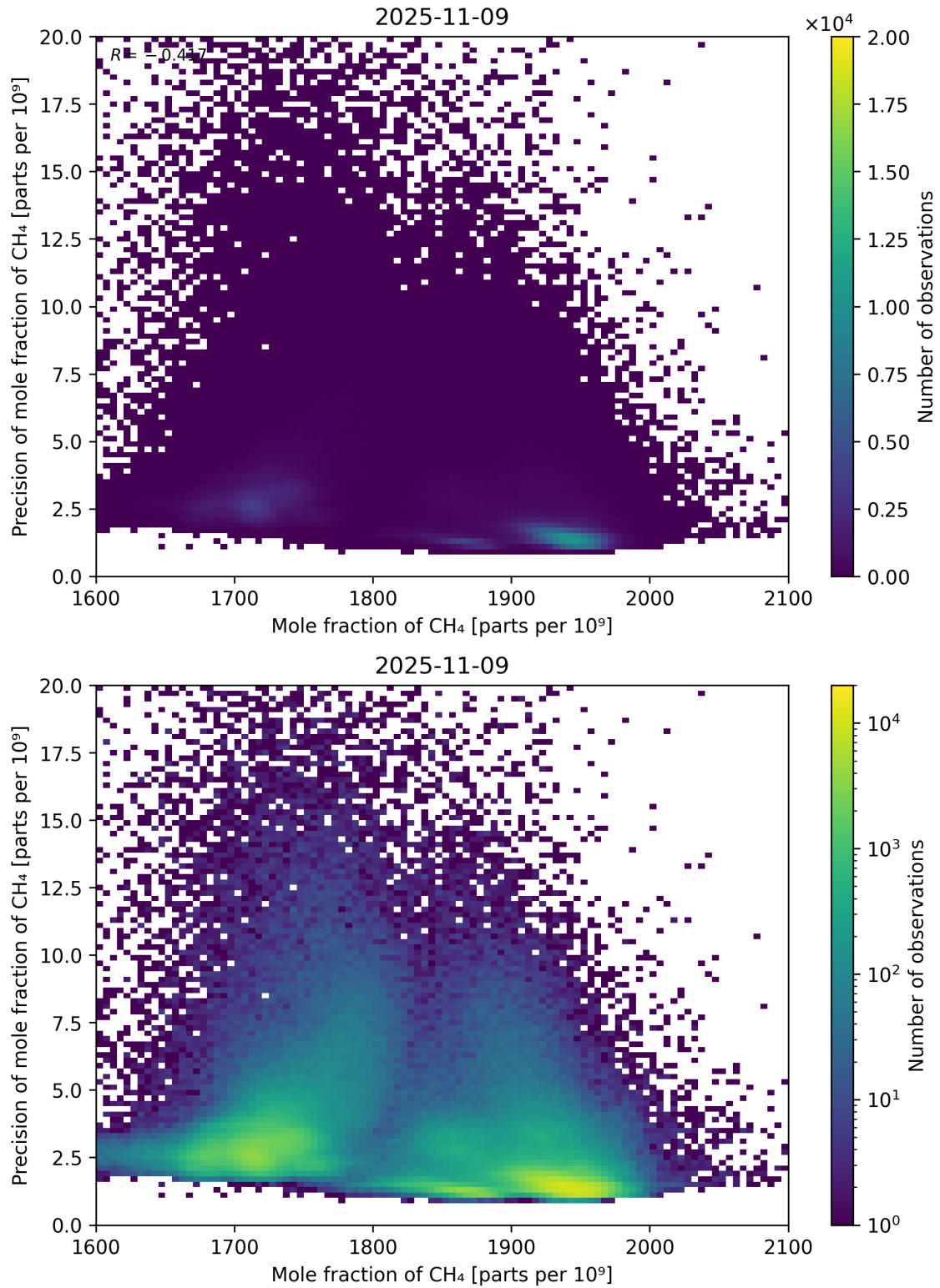
Figure 75: Scatter density plot of “Mole fraction of CH 4 ” against “Precision of mole fraction of CH 4 ” for 2025-11-08 to 2025-11-10.
