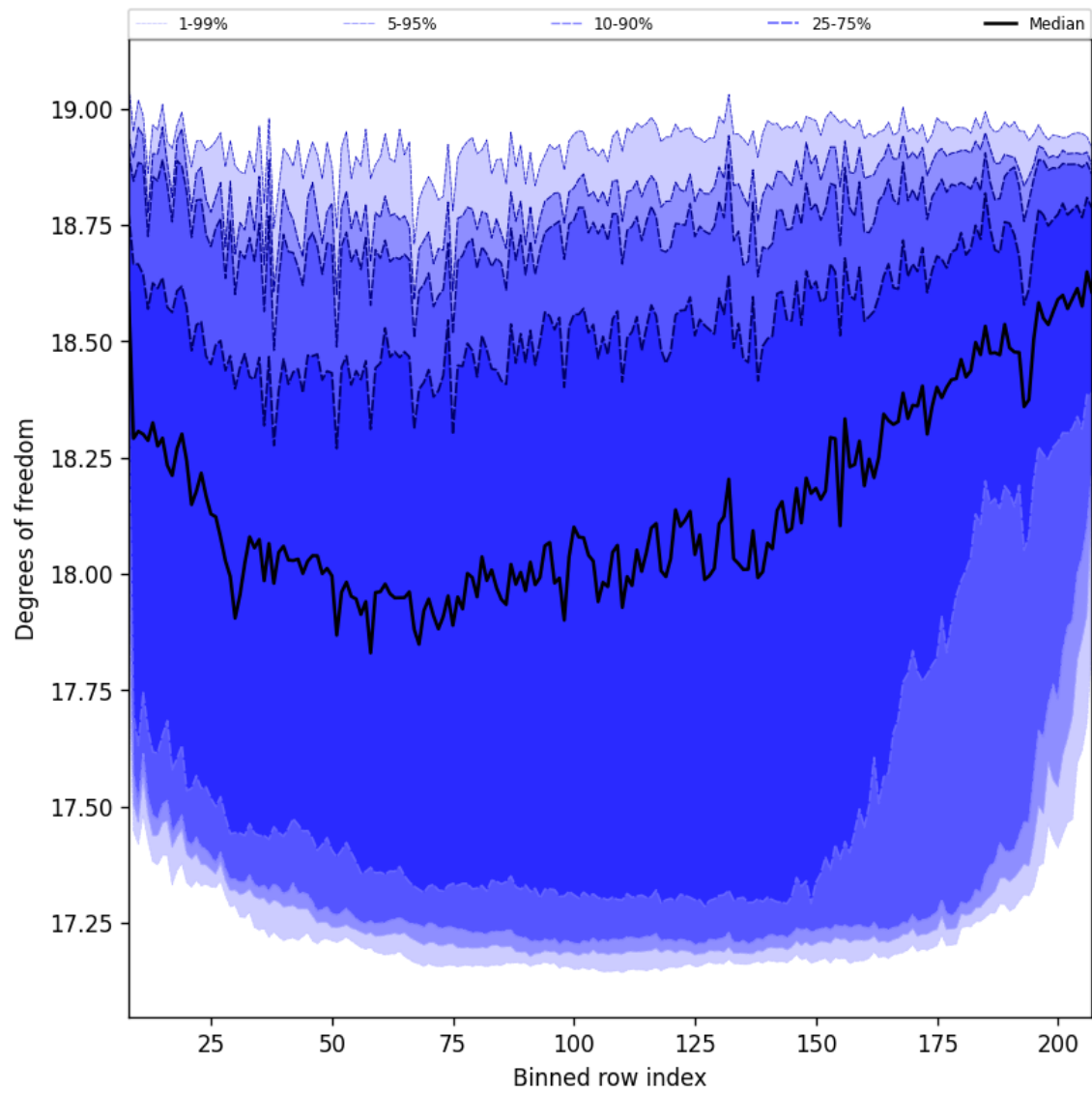
Figure 41: Along track statistics of “Degrees of freedom” for 2025-11-08 to 2025-11-10
