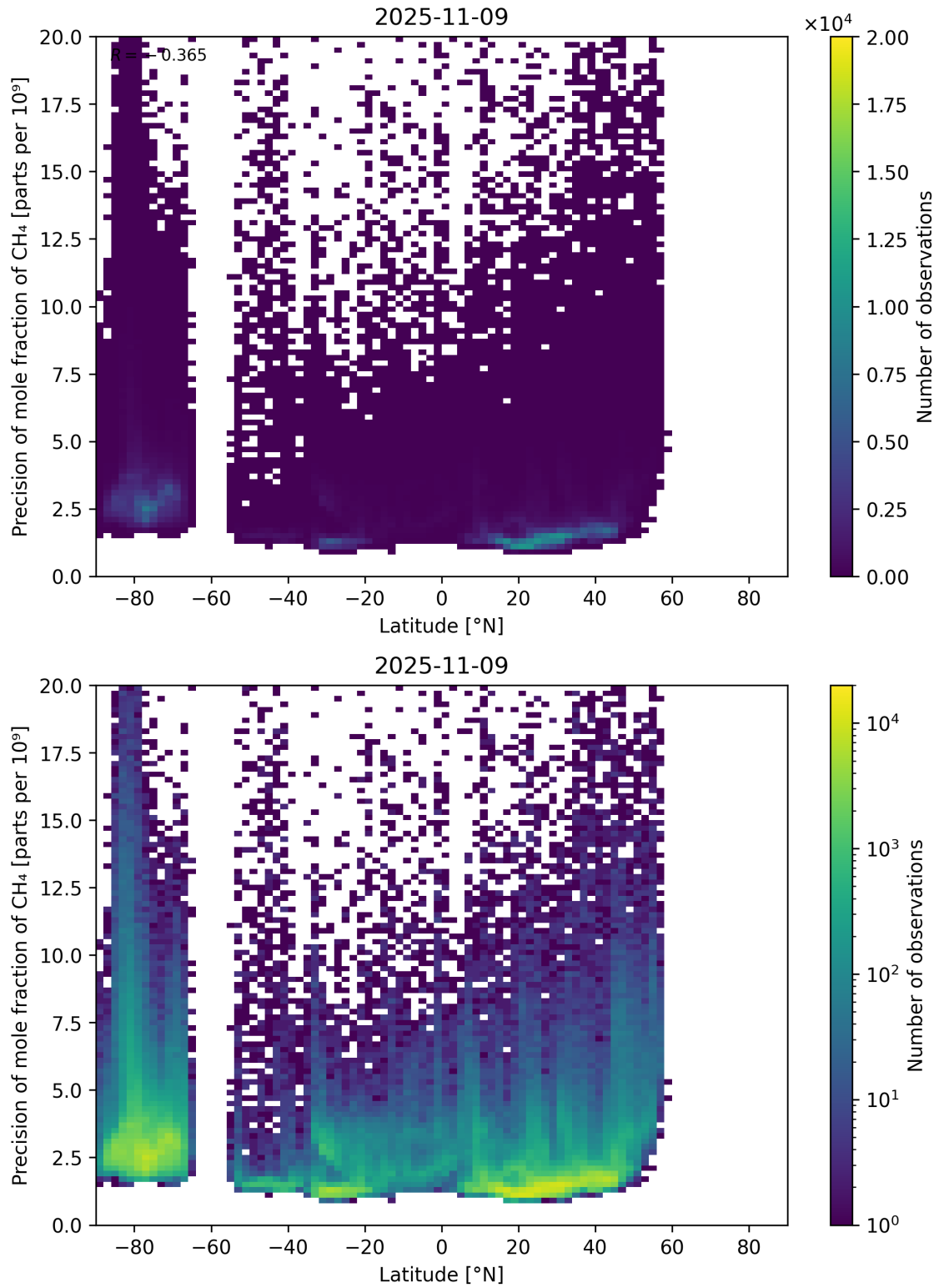
Figure 59: Scatter density plot of “Latitude” against “Precision of mole fraction of CH 4 ” for 2025-11-08 to 2025-11-10.
