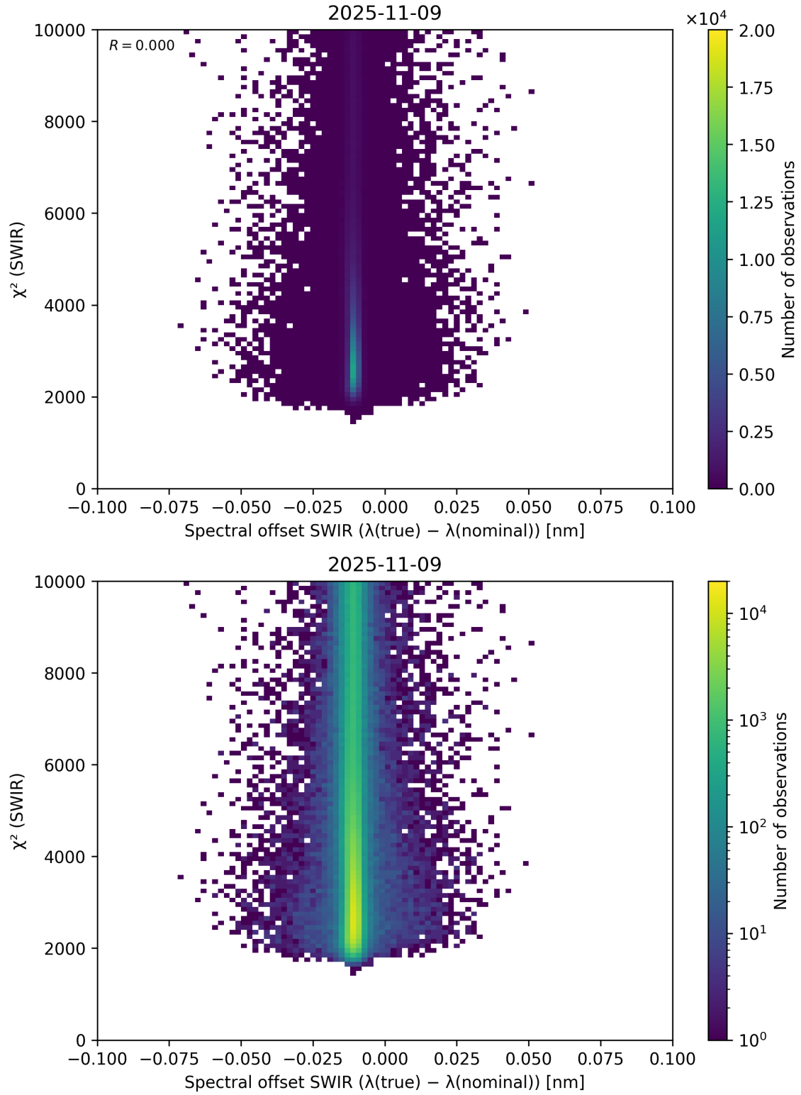
Figure 118: Scatter density plot of “Spectral offset SWIR ( \lambda_{\text{true}} - \lambda_{\text{nominal}} )” against “ \chi^2 (SWIR)” for 2025-11-08 to 2025-11-10.
