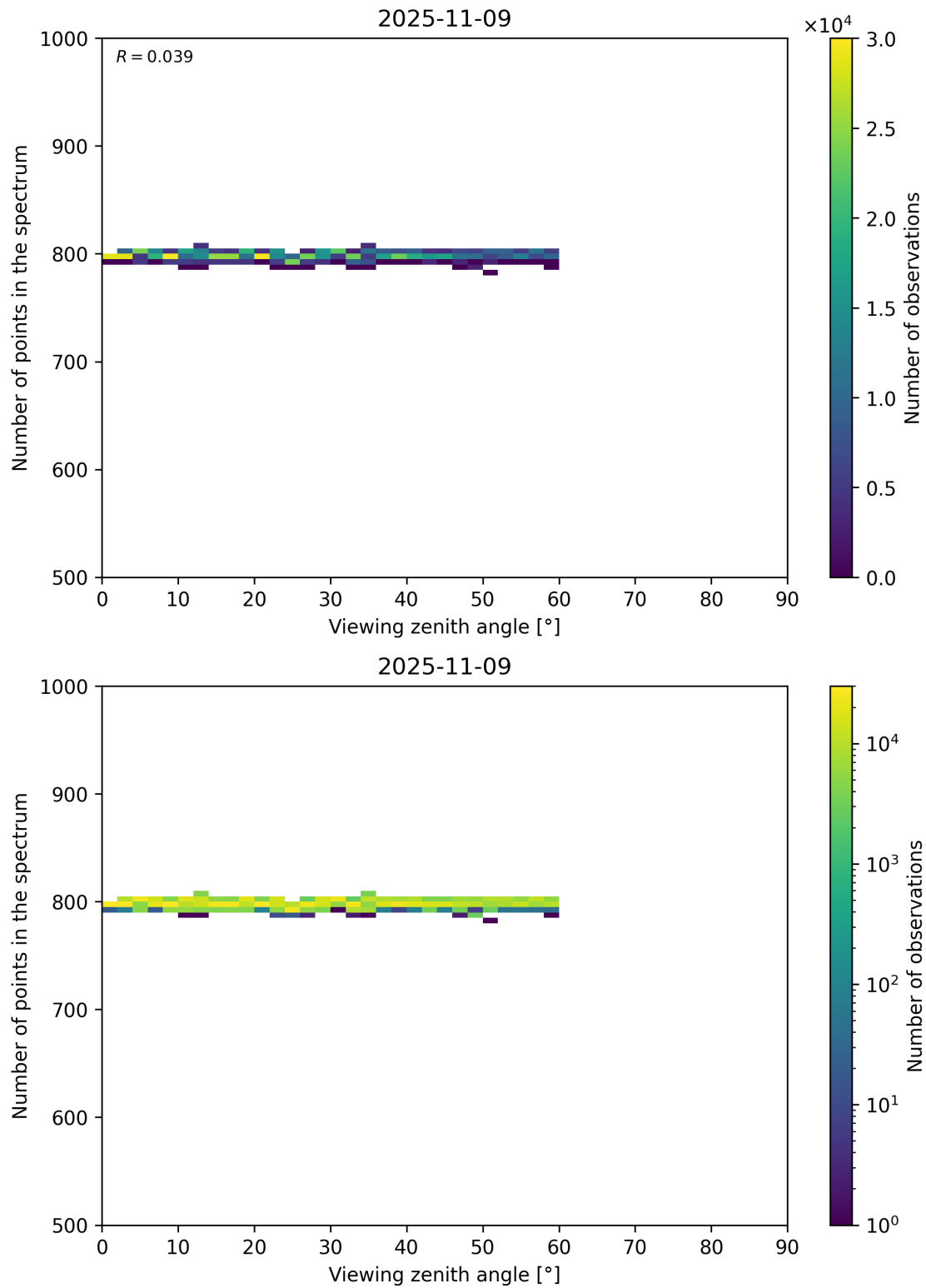
Figure 114: Scatter density plot of “Viewing zenith angle” against “Number of points in the spectrum” for 2025-11-08 to 2025-11-10.
