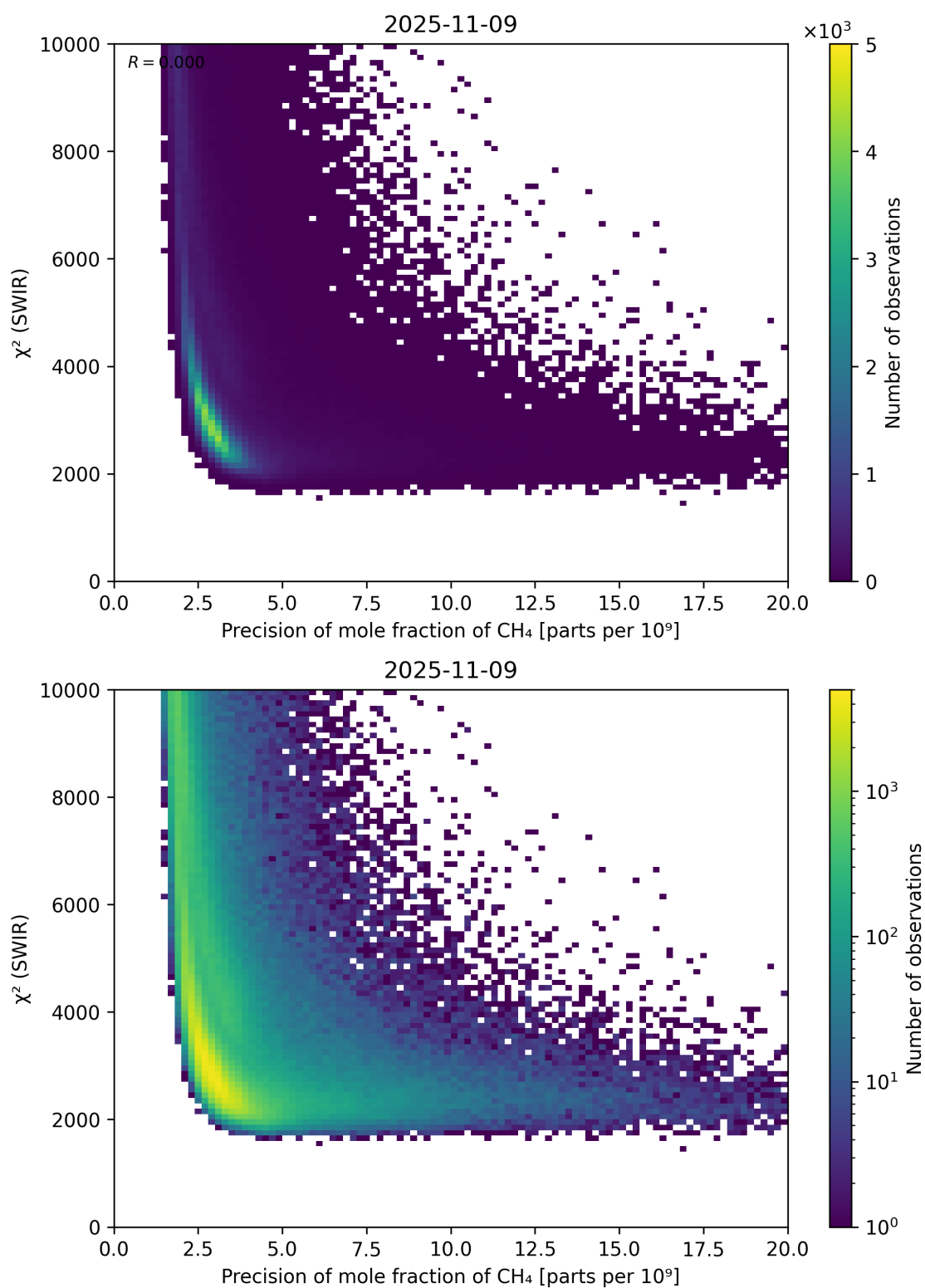
Figure 79: Scatter density plot of “Precision of mole fraction of \text{CH}_4 ” against “ \chi^2 (SWIR)” for 2025-11-08 to 2025-11-10.
