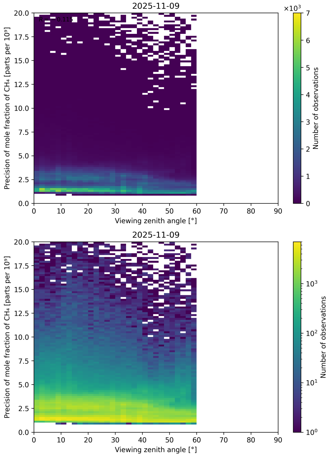
Figure 112: Scatter density plot of “Viewing zenith angle” against “Precision of mole fraction of CH 4 ” for 2025-11-08 to 2025-11-10.
