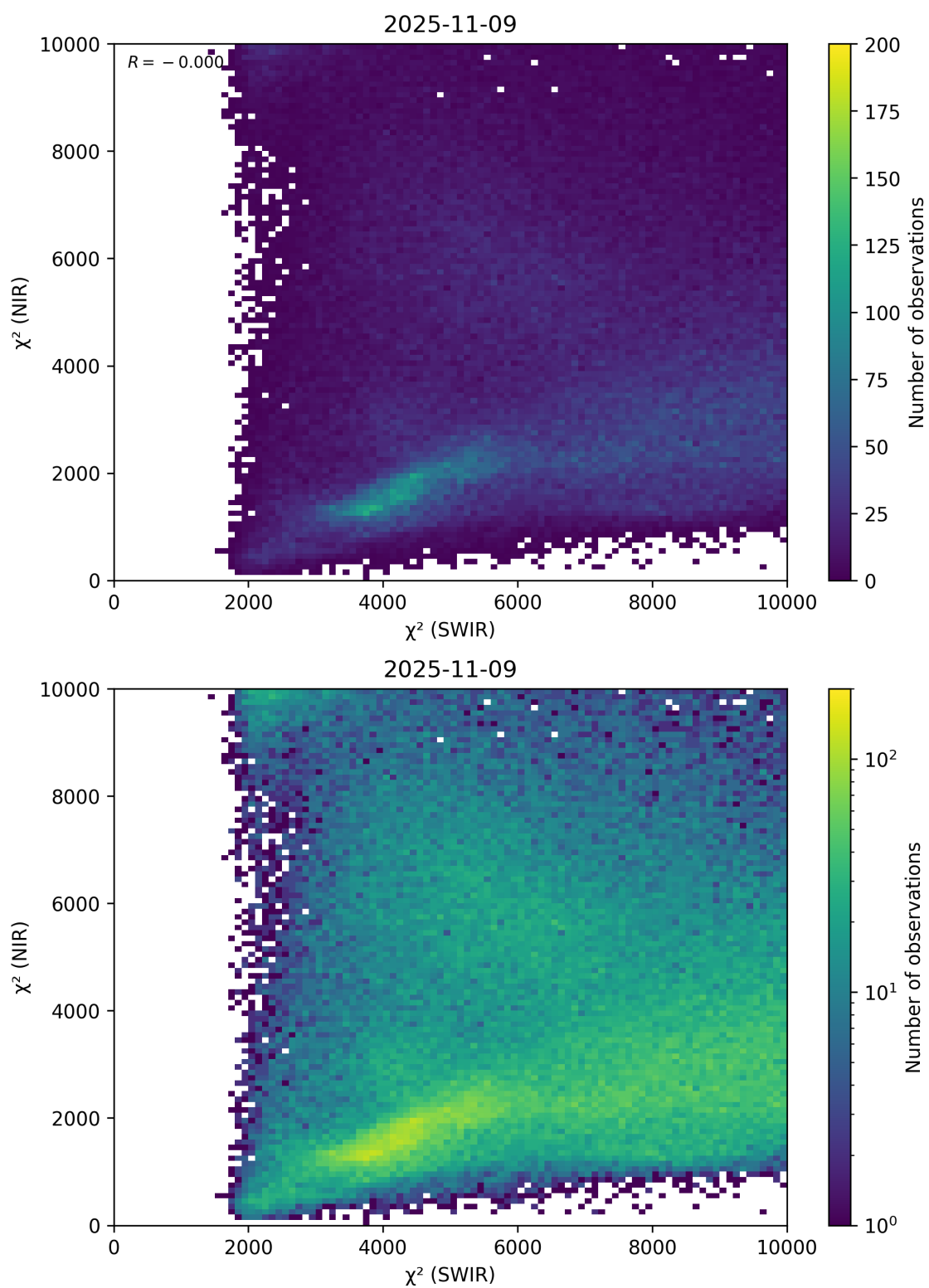
Figure 47: Scatter density plot of “ \chi^2 (SWIR)” against “ \chi^2 (NIR)” for 2025-11-08 to 2025-11-10.
