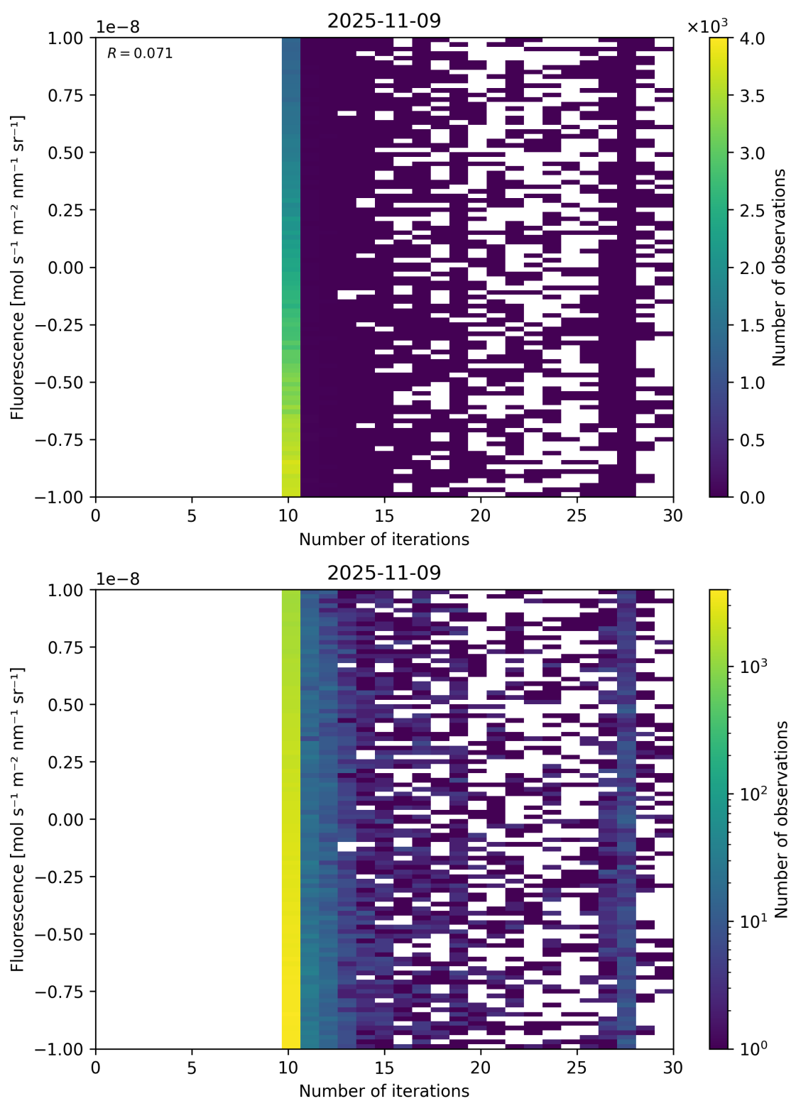
Figure 87: Scatter density plot of “Number of iterations” against “Fluorescence” for 2025-11-08 to 2025-11-10.
