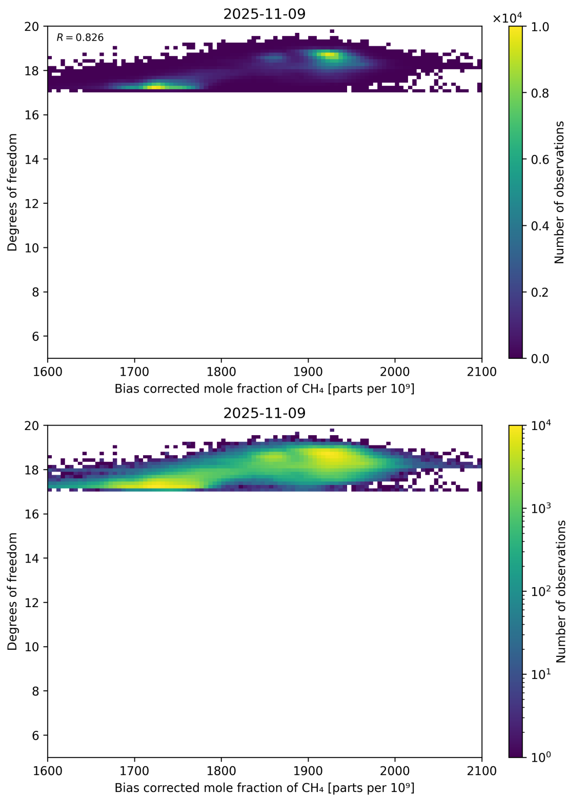
Figure 65: Scatter density plot of “Bias corrected mole fraction of CH 4 ” against “Degrees of freedom” for 2025-11-08 to 2025-11-10.
