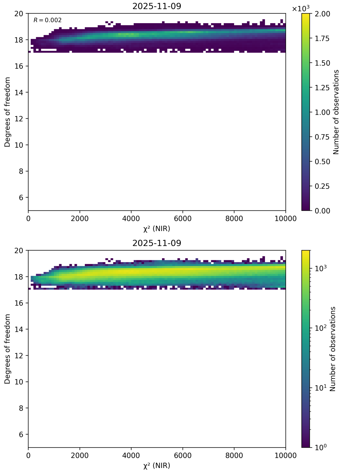
Figure 44: Scatter density plot of “ \chi^2 (NIR)” against “Degrees of freedom” for 2025-11-08 to 2025-11-10.
