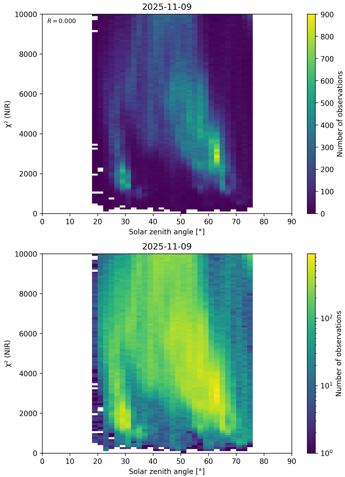
Figure 94: Scatter density plot of “Solar zenith angle” against “ \chi^2 (NIR)” for 2025-11-08 to 2025-11-10.
