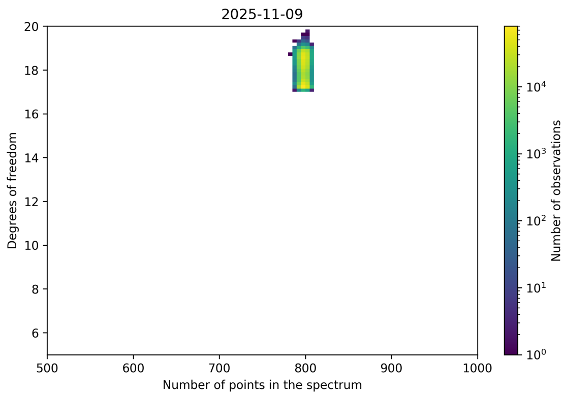
Figure 90: Scatter density plot of “Number of points in the spectrum” against “Degrees of freedom” for 2025-11-08 to 2025-11-10.
