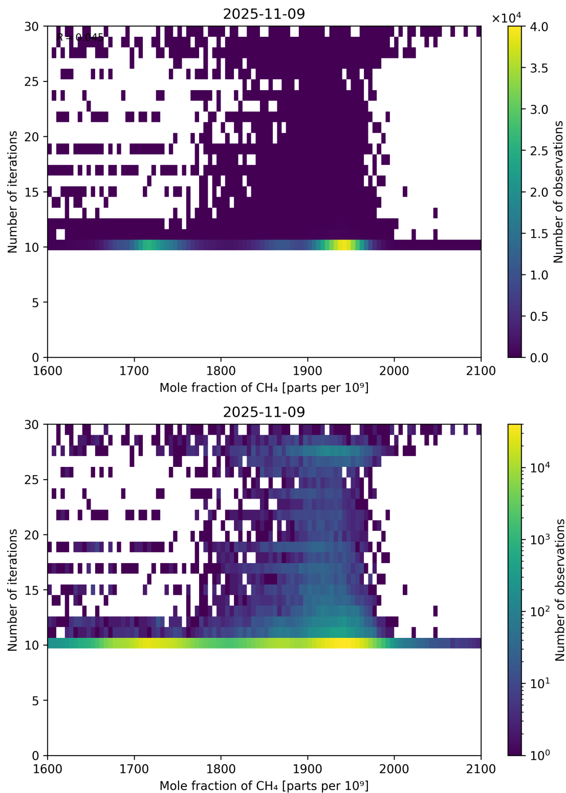
Figure 76: Scatter density plot of “Mole fraction of CH 4 ” against “Number of iterations” for 2025-11-08 to 2025-11-10.
