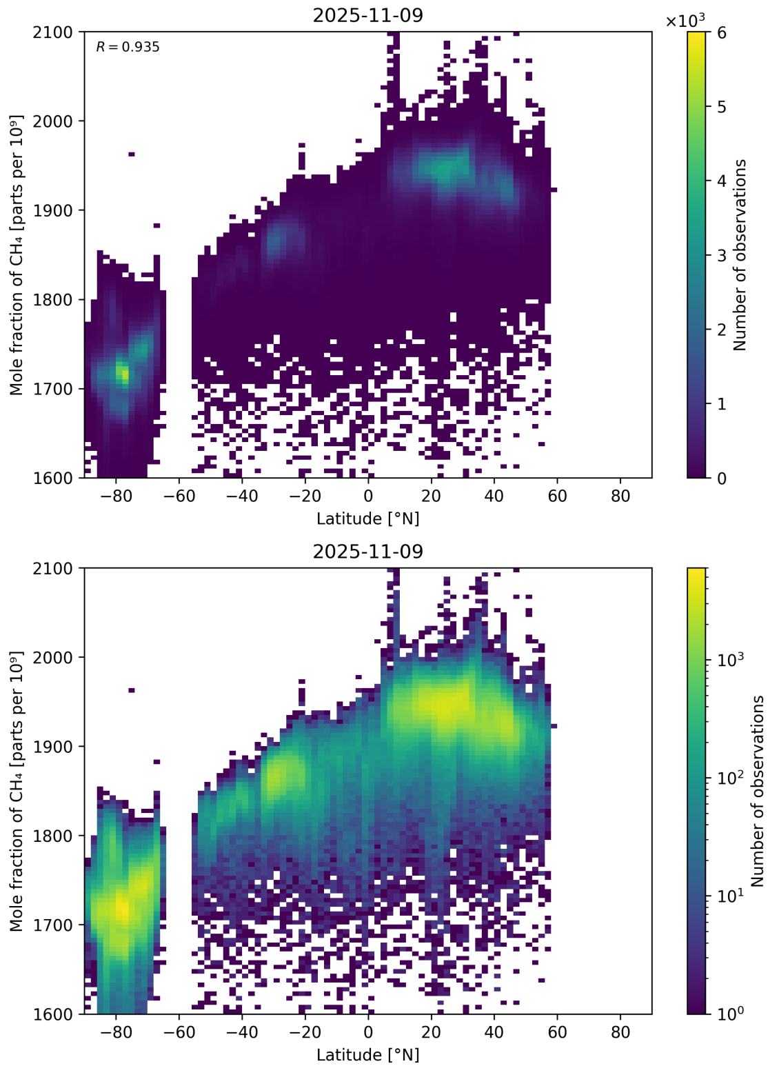
Figure 57: Scatter density plot of “Latitude” against “Mole fraction of CH 4 ” for 2025-11-08 to 2025-11-10.
