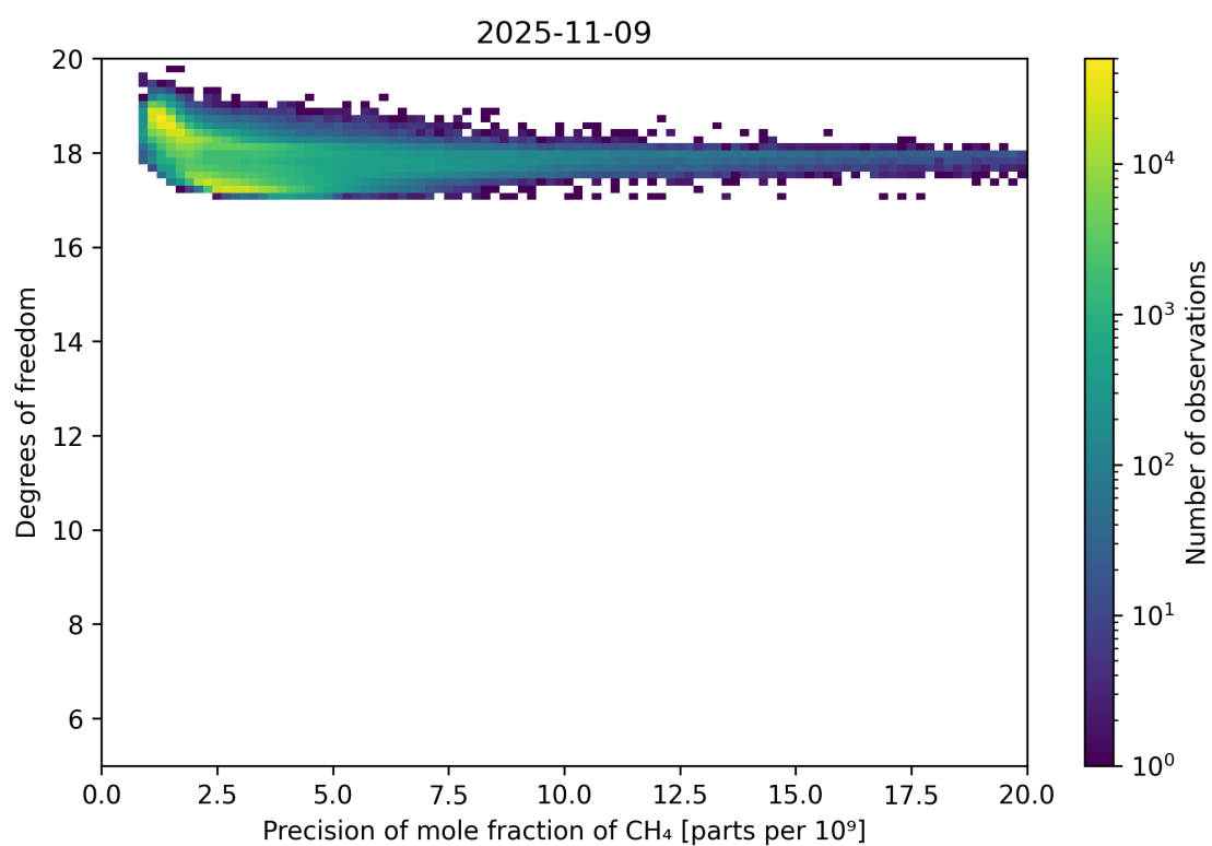
Figure 80: Scatter density plot of “Precision of mole fraction of CH 4 ” against “Degrees of freedom” for 2025-11-08 to 2025-11-10.
