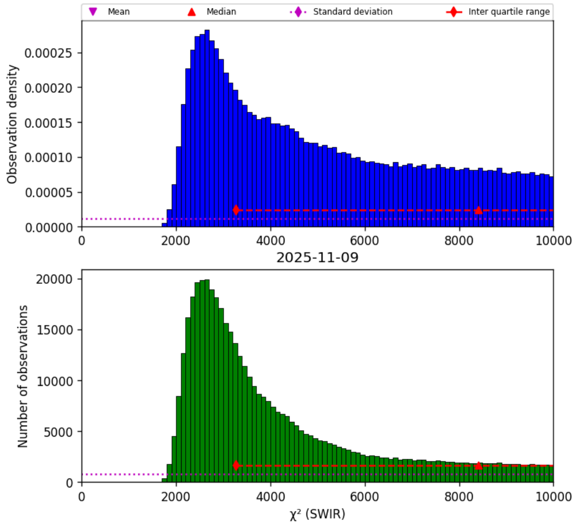
Figure 28: Histogram of " \chi^2 (SWIR)" for 2025-11-08 to 2025-11-10
