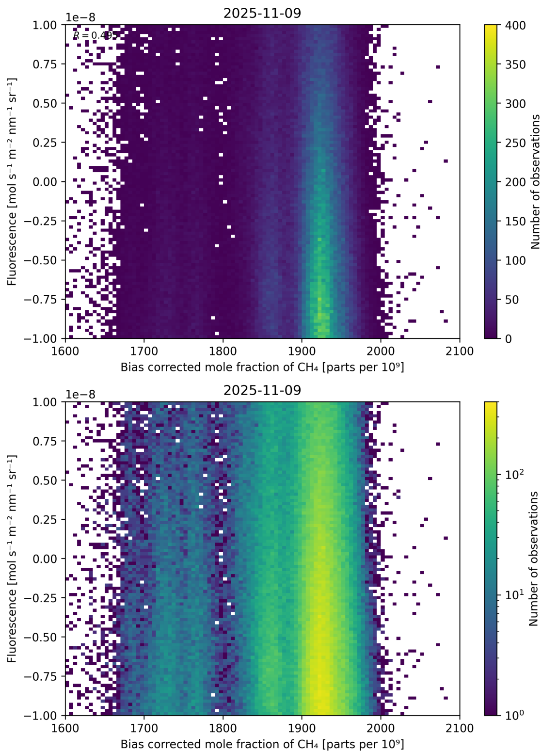
Figure 66: Scatter density plot of “Bias corrected mole fraction of \text{CH}_4 ” against “Fluorescence” for 2025-11-08 to 2025-11-10.
