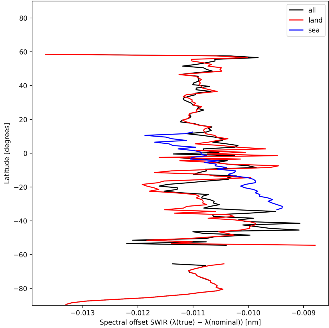
Figure 16: Zonal average of “Spectral offset SWIR ( \lambda_{\text{true}} - \lambda_{\text{nominal}} )” for 2025-11-08 to 2025-11-10.
