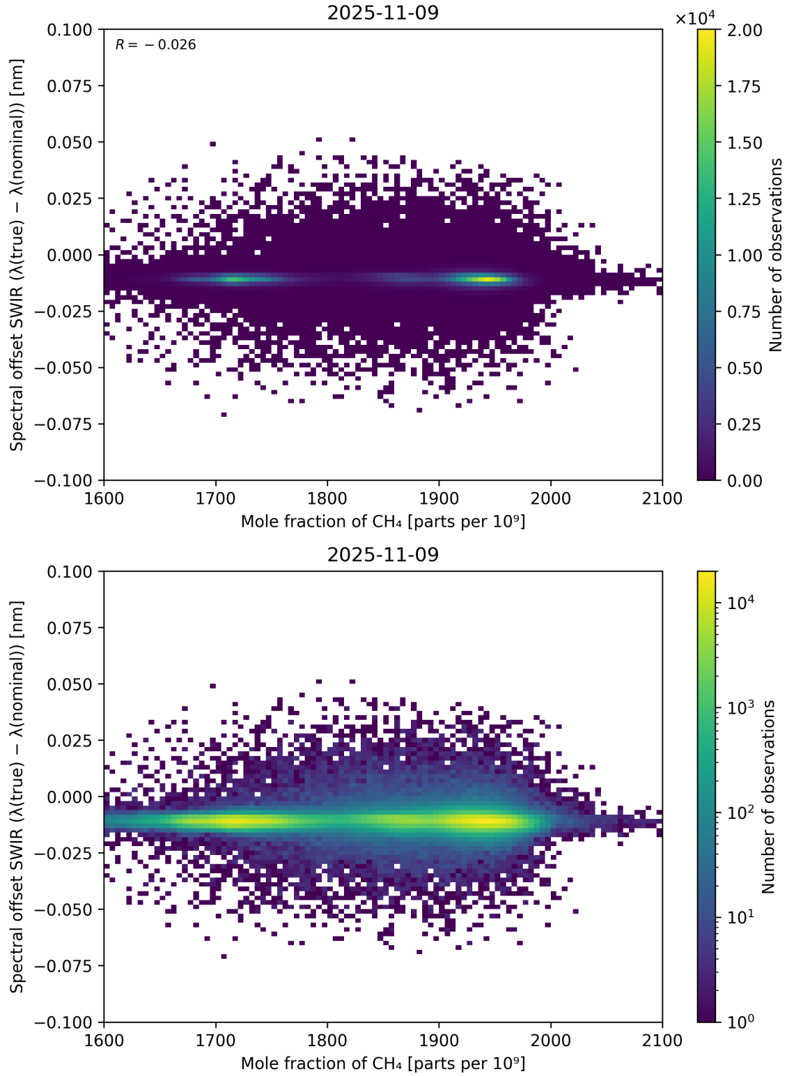
Figure 86: Scatter density plot of “Mole fraction of CH 4 ” against “Spectral offset SWIR ( \lambda_{\text{true}} - \lambda_{\text{nominal}} )” for 2025-11-08 to 2025-11-10.
