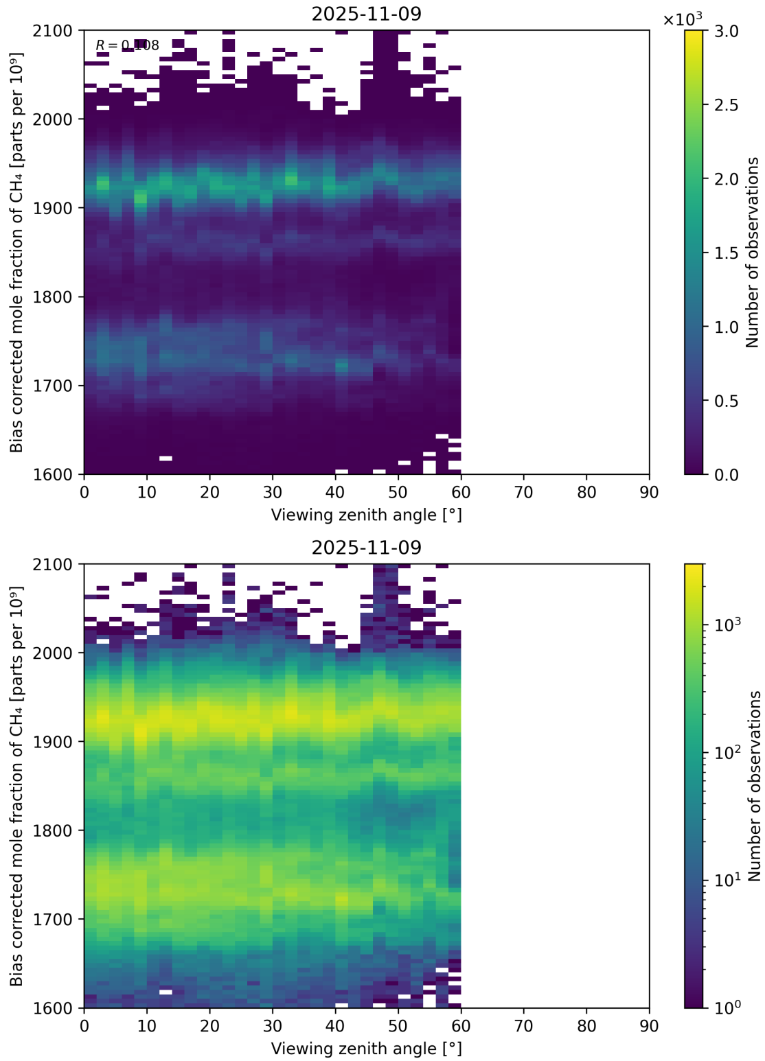
Figure 111: Scatter density plot of “Viewing zenith angle” against “Bias corrected mole fraction of CH 4 ” for 2025-11-08 to 2025-11-10.
