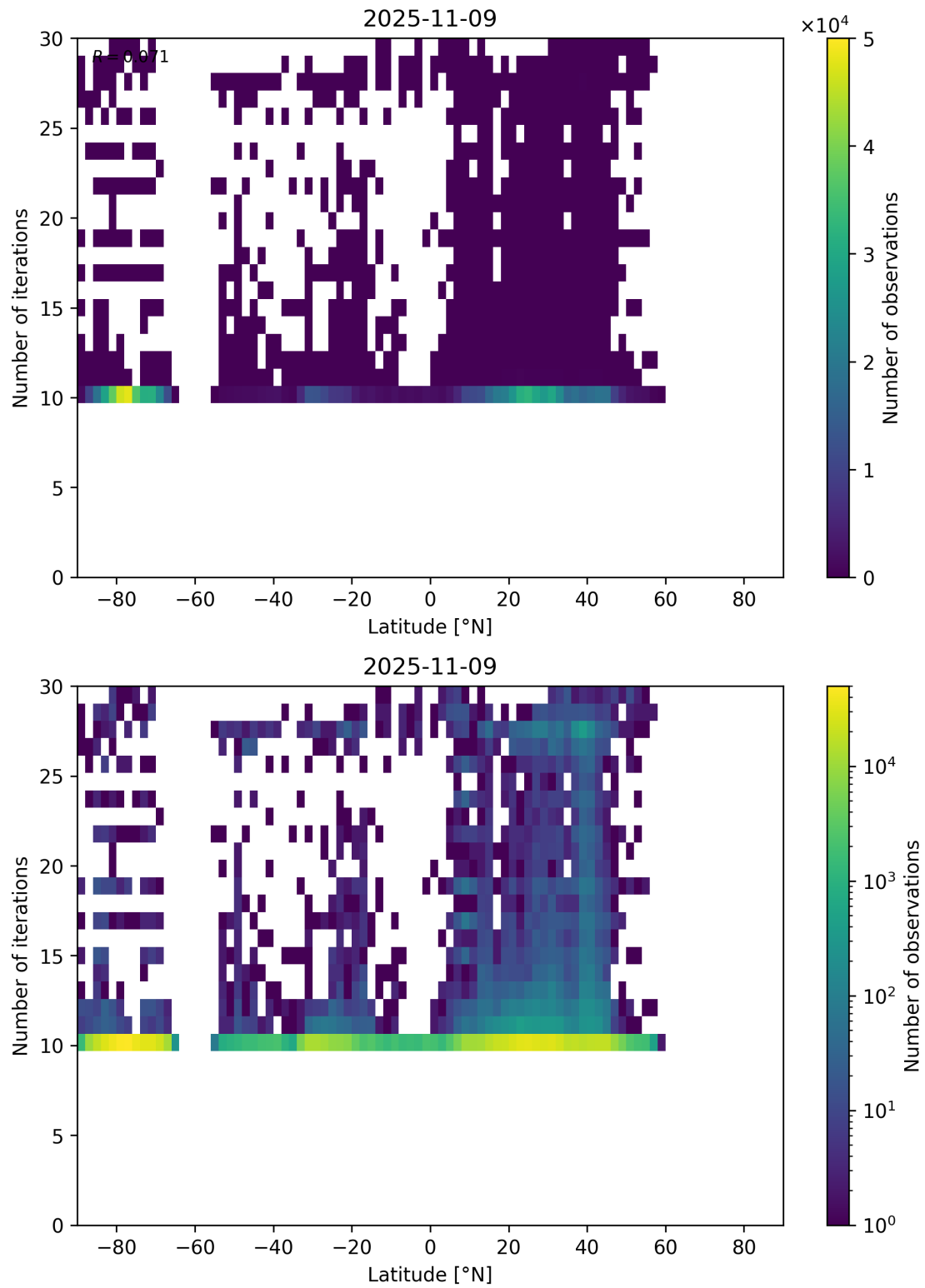
Figure 60: Scatter density plot of “Latitude” against “Number of iterations” for 2025-11-08 to 2025-11-10.
