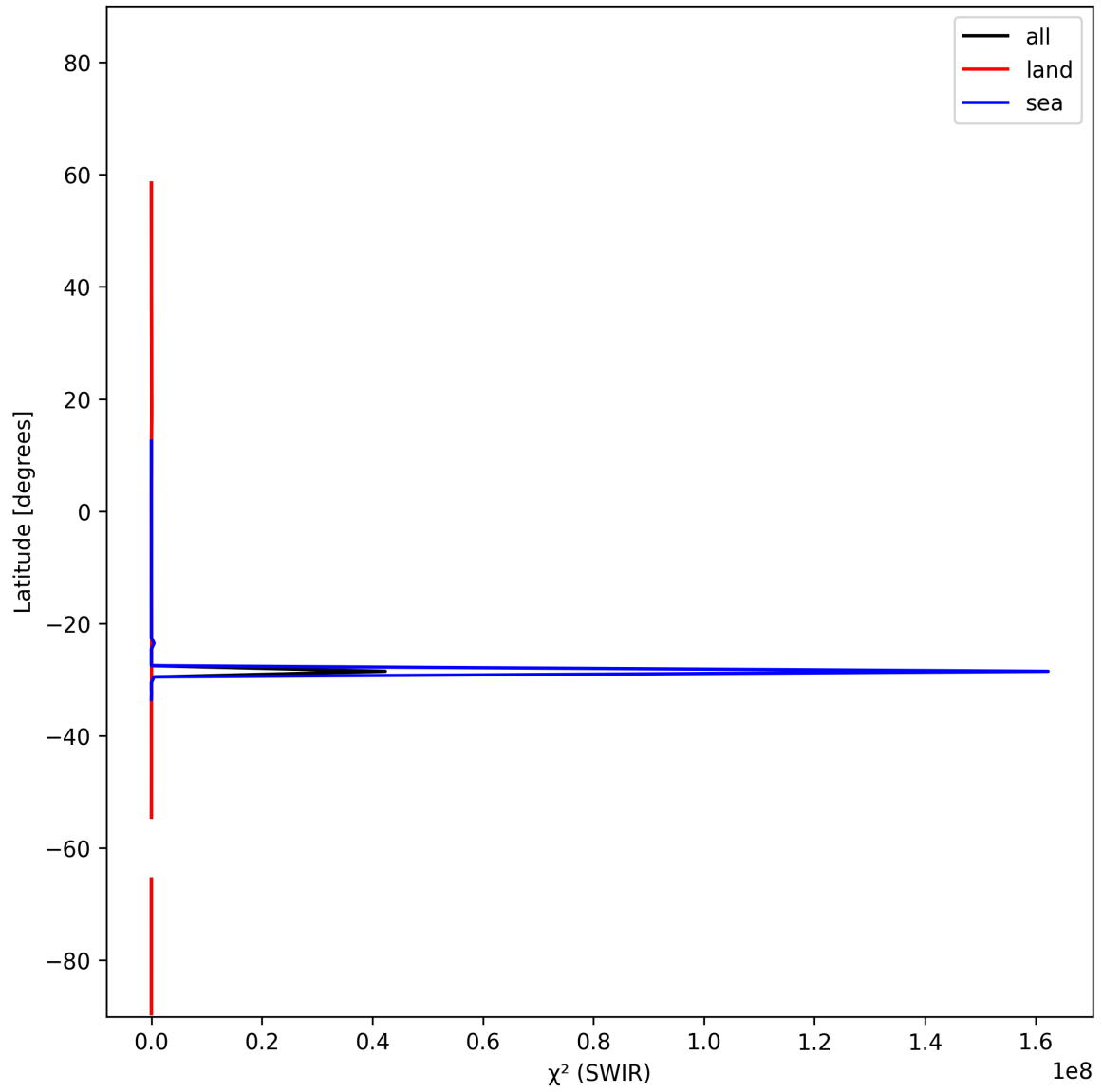
Figure 17: Zonal average of “ \chi^2 (SWIR)” for 2025-11-08 to 2025-11-10.
