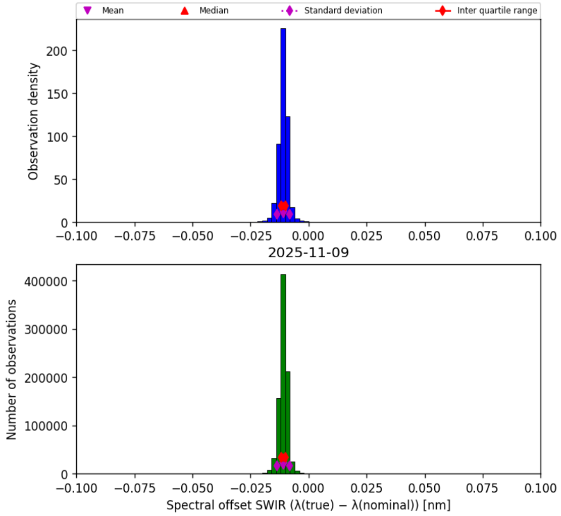
Figure 27: Histogram of “Spectral offset SWIR ( \lambda_{\text{true}} - \lambda_{\text{nominal}} )” for 2025-11-08 to 2025-11-10
