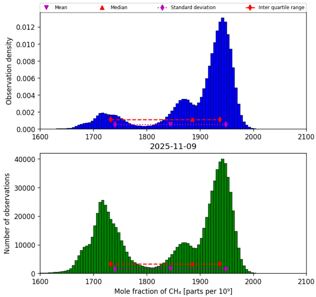
Figure 23: Histogram of “Mole fraction of CH 4 ” for 2025-11-08 to 2025-11-10
