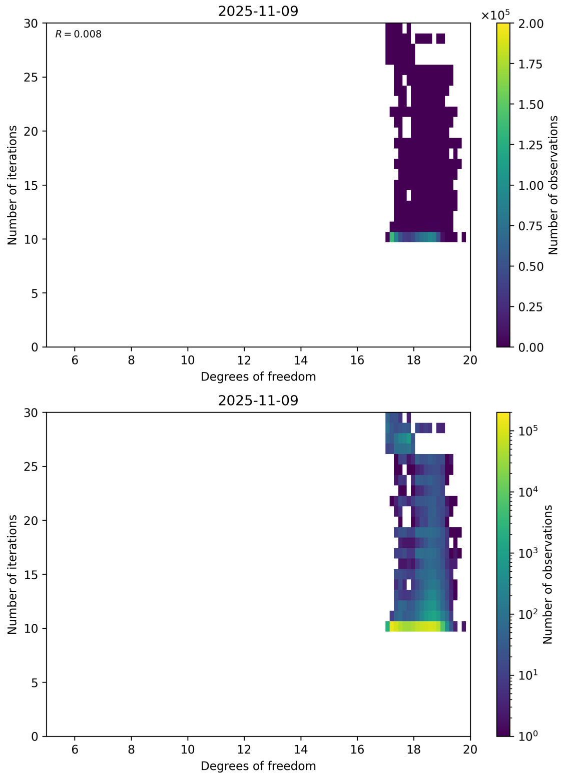
Figure 52: Scatter density plot of “Degrees of freedom” against “Number of iterations” for 2025-11-08 to 2025-11-10.
