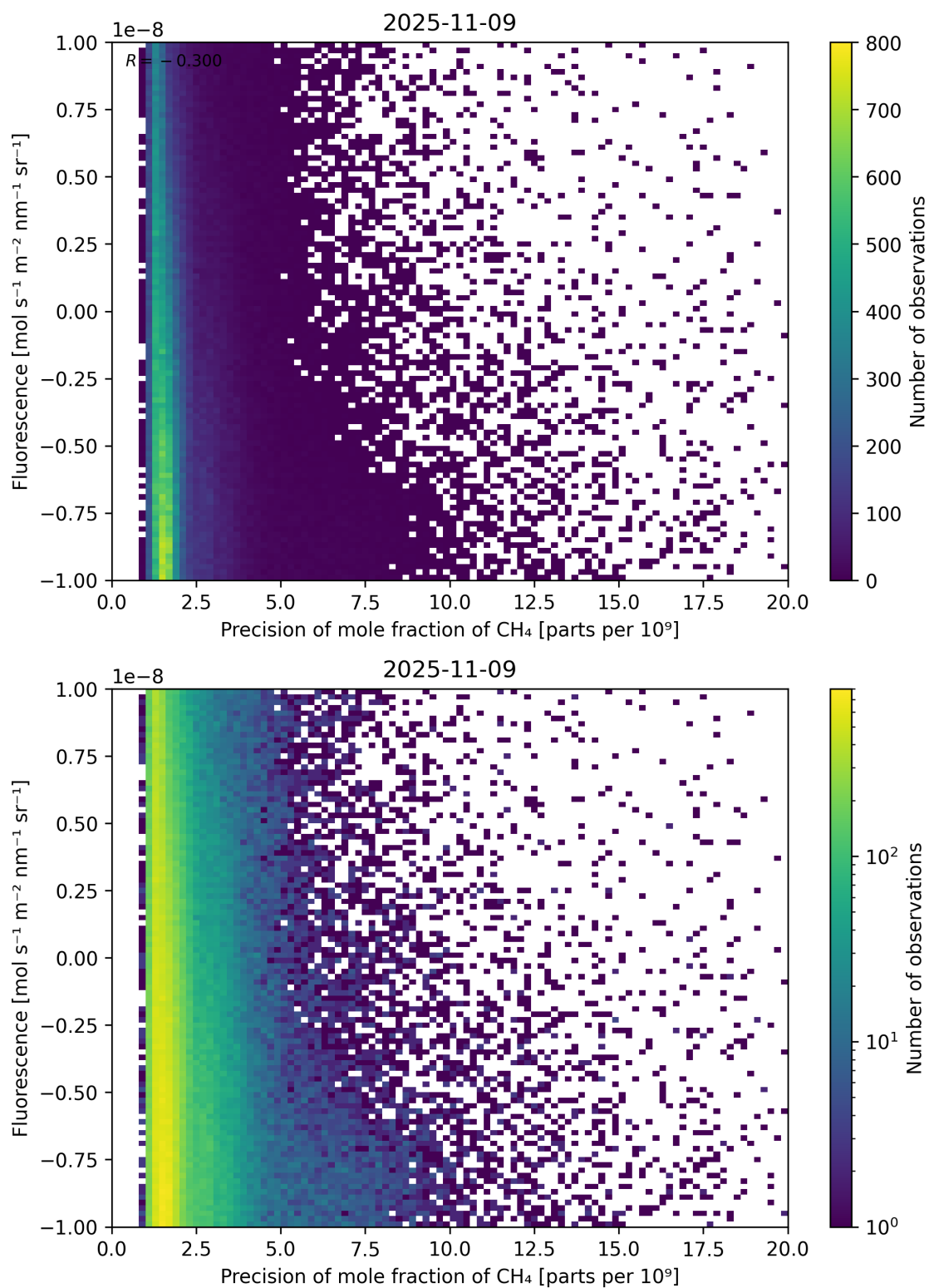
Figure 81: Scatter density plot of “Precision of mole fraction of \text{CH}_4 ” against “Fluorescence” for 2025-11-08 to 2025-11-10.
