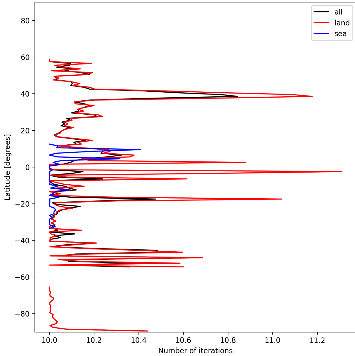
Figure 20: Zonal average of “Number of iterations” for 2025-11-08 to 2025-11-10.
