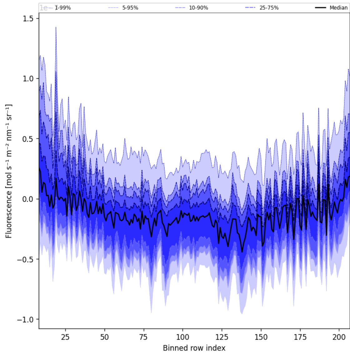
Figure 43: Along track statistics of “Fluorescence” for 2025-11-08 to 2025-11-10
