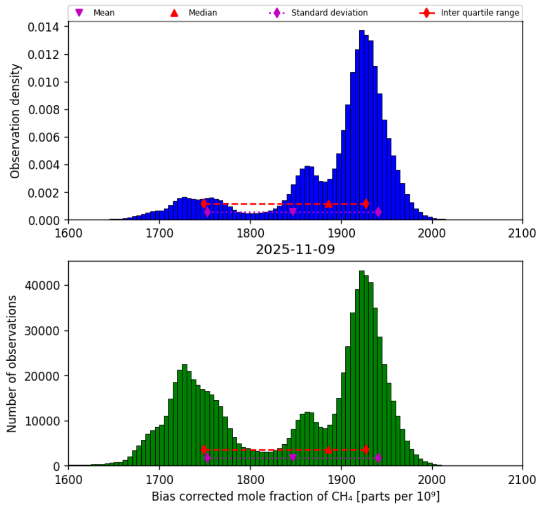
Figure 25: Histogram of “Bias corrected mole fraction of CH 4 ” for 2025-11-08 to 2025-11-10
