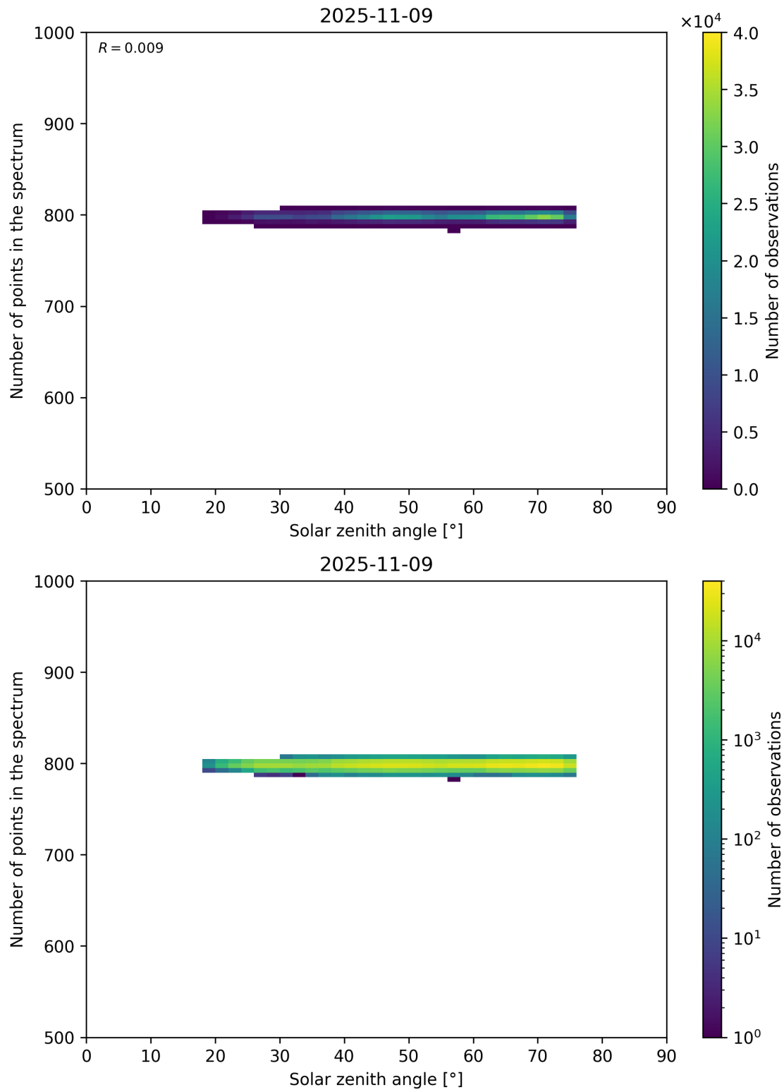
Figure 103: Scatter density plot of “Solar zenith angle” against “Number of points in the spectrum” for 2025-11-08 to 2025-11-10.
