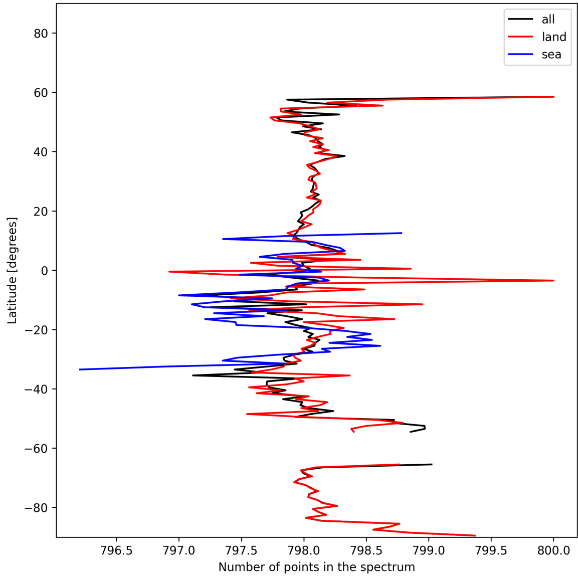
Figure 15: Zonal average of “Number of points in the spectrum” for 2025-11-08 to 2025-11-10.
