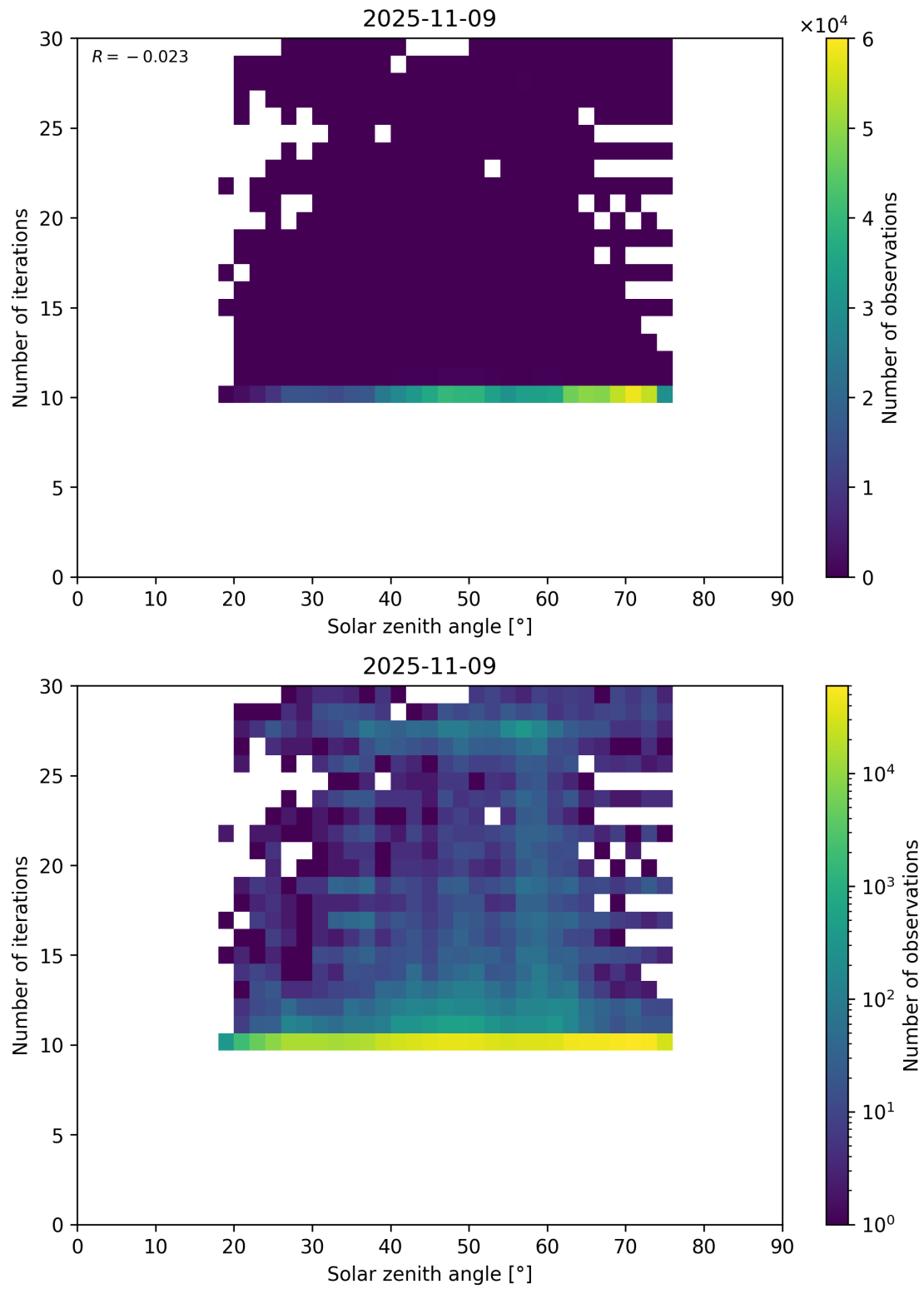
Figure 102: Scatter density plot of “Solar zenith angle” against “Number of iterations” for 2025-11-08 to 2025-11-10.
