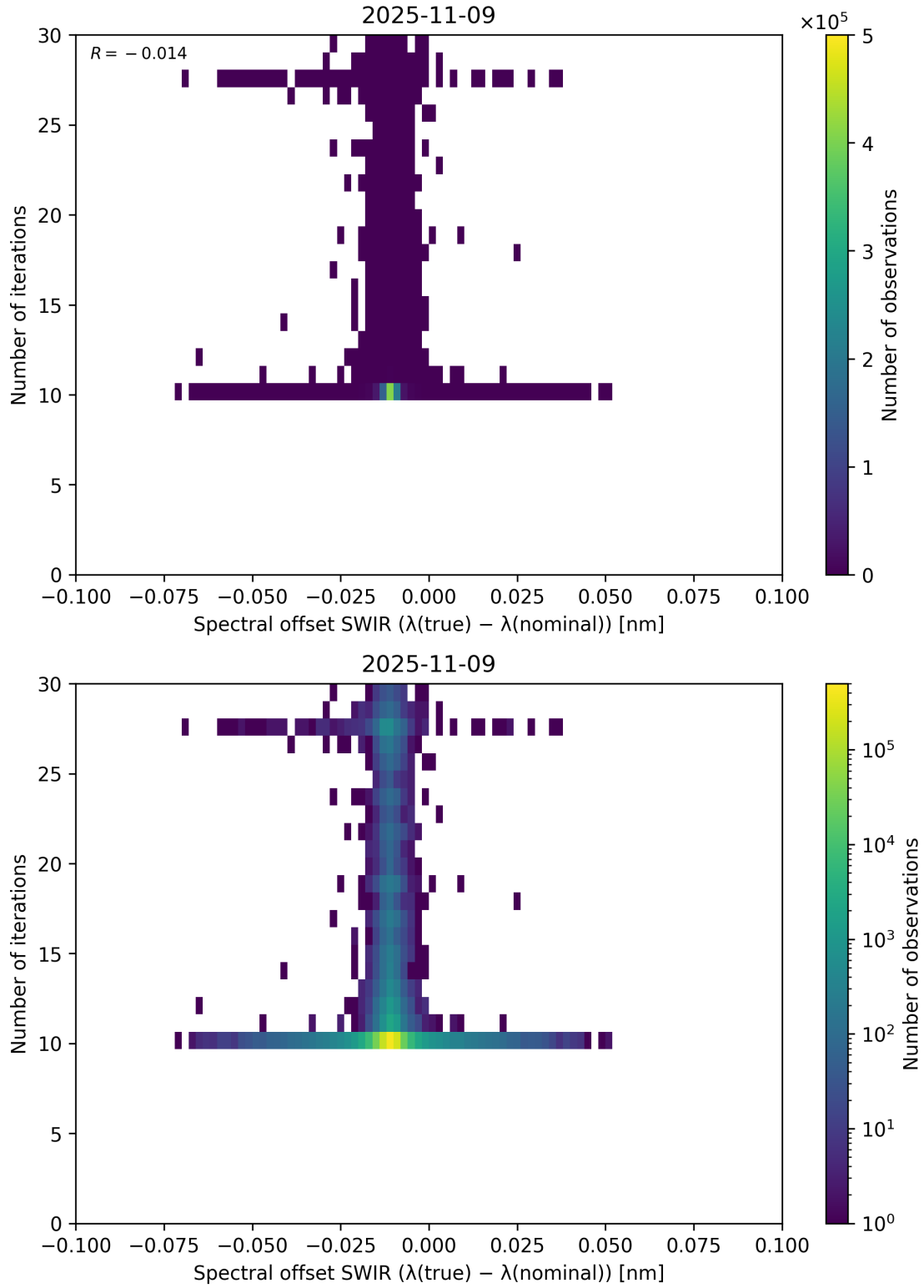
Figure 121: Scatter density plot of “Spectral offset SWIR ( \lambda_{\text{true}} - \lambda_{\text{nominal}} )” against “Number of iterations” for 2025-11-08 to 2025-11-10.
