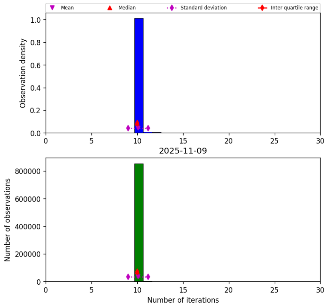
Figure 31: Histogram of “Number of iterations” for 2025-11-08 to 2025-11-10
