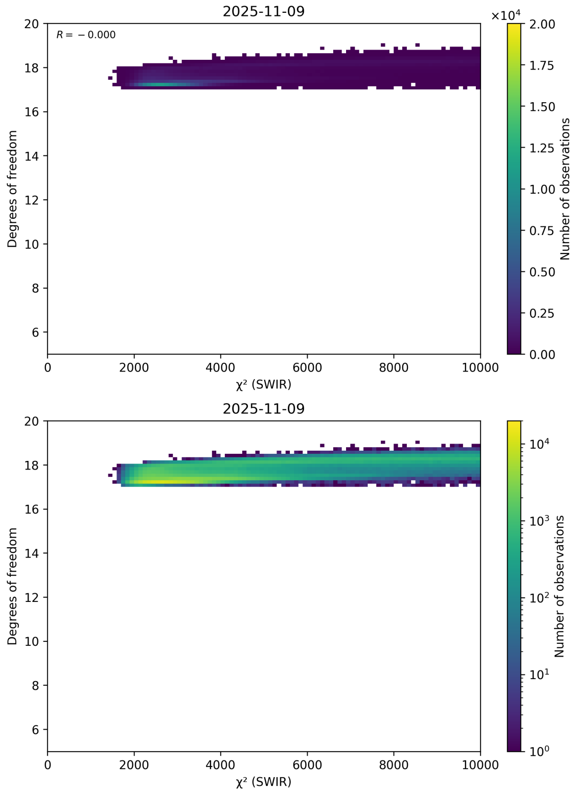
Figure 48: Scatter density plot of “ \chi^2 (SWIR)” against “Degrees of freedom” for 2025-11-08 to 2025-11-10.
