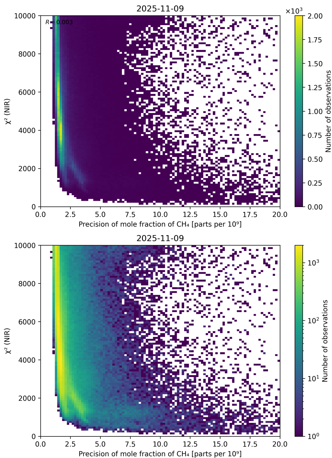
Figure 78: Scatter density plot of “Precision of mole fraction of \text{CH}_4 ” against “ \chi^2 (NIR)” for 2025-11-08 to 2025-11-10.
