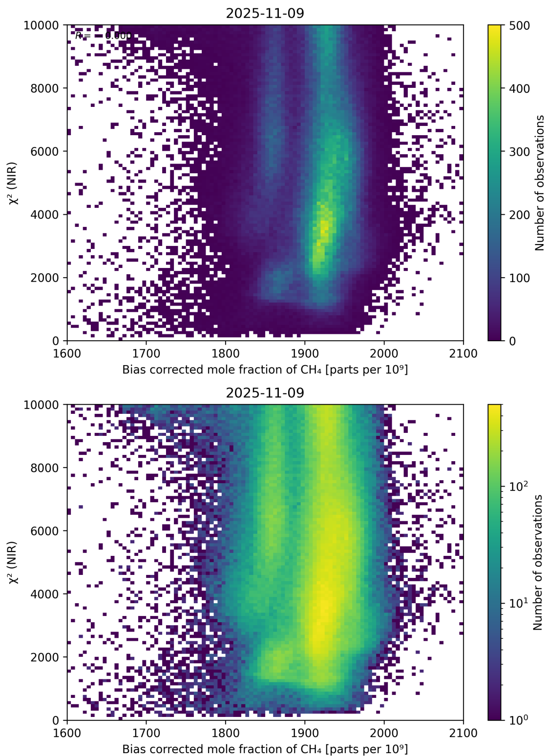
Figure 63: Scatter density plot of “Bias corrected mole fraction of \text{CH}_4 ” against “ \chi^2 (NIR)” for 2025-11-08 to 2025-11-10.
