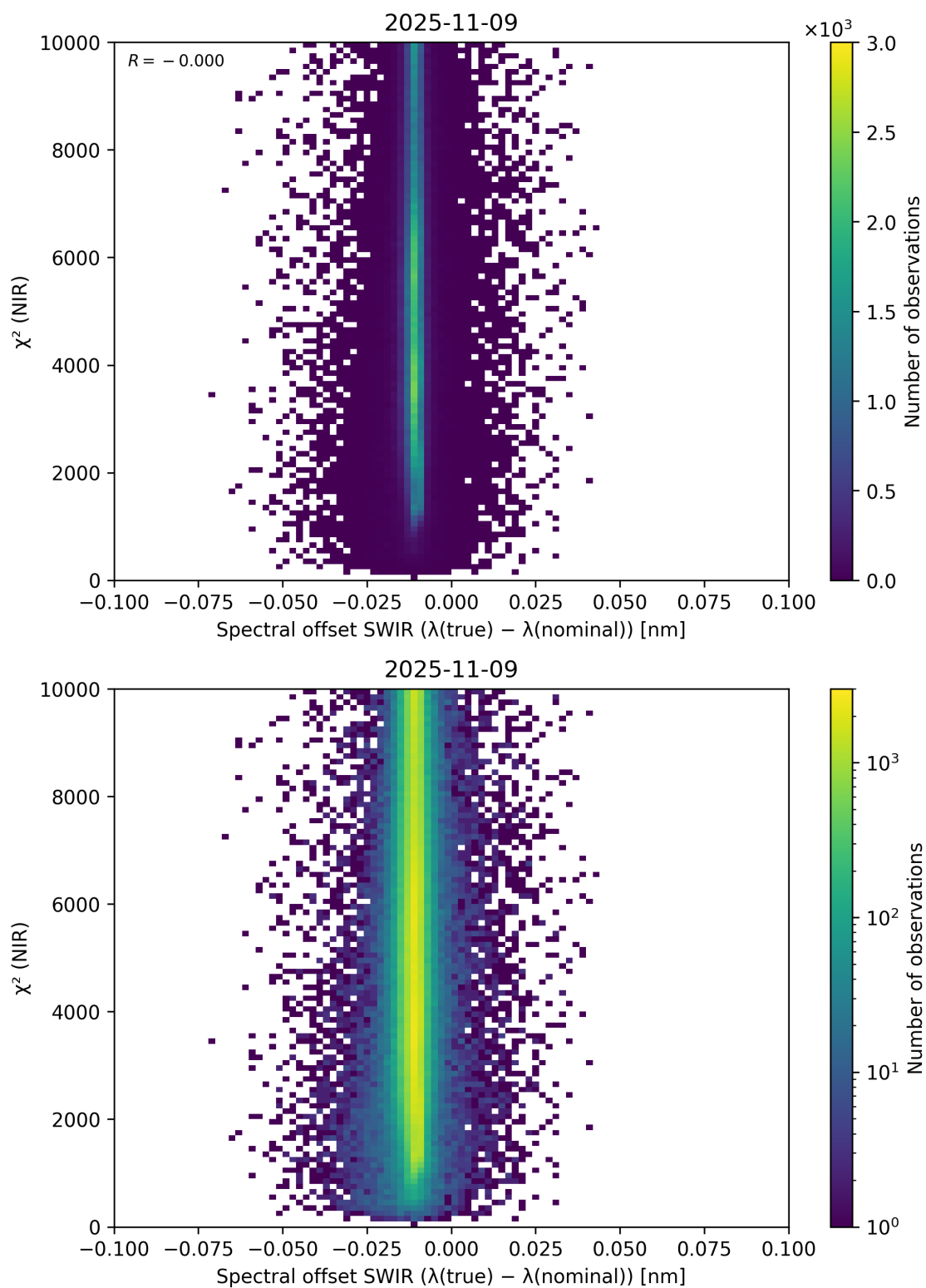
Figure 117: Scatter density plot of “Spectral offset SWIR ( \lambda_{\text{true}} - \lambda_{\text{nominal}} )” against “ \chi^2 (NIR)” for 2025-11-08 to 2025-11-10.
