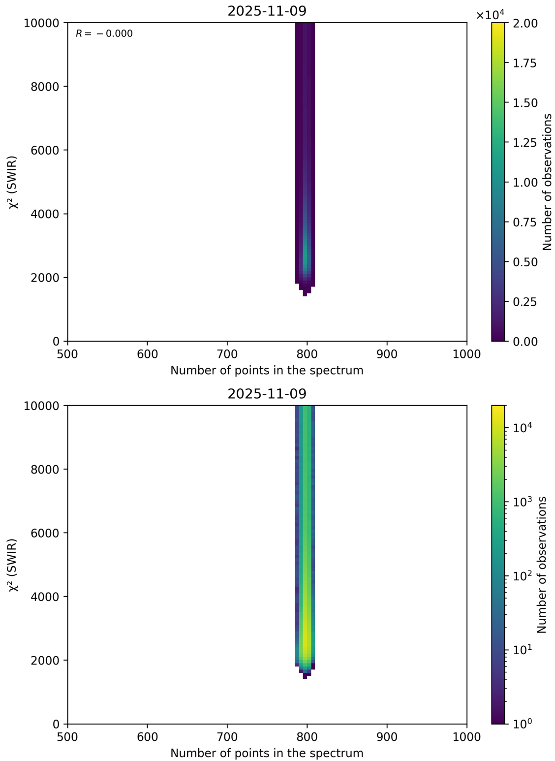
Figure 89: Scatter density plot of “Number of points in the spectrum” against “ \chi^2 (SWIR)” for 2025-11-08 to 2025-11-10.
