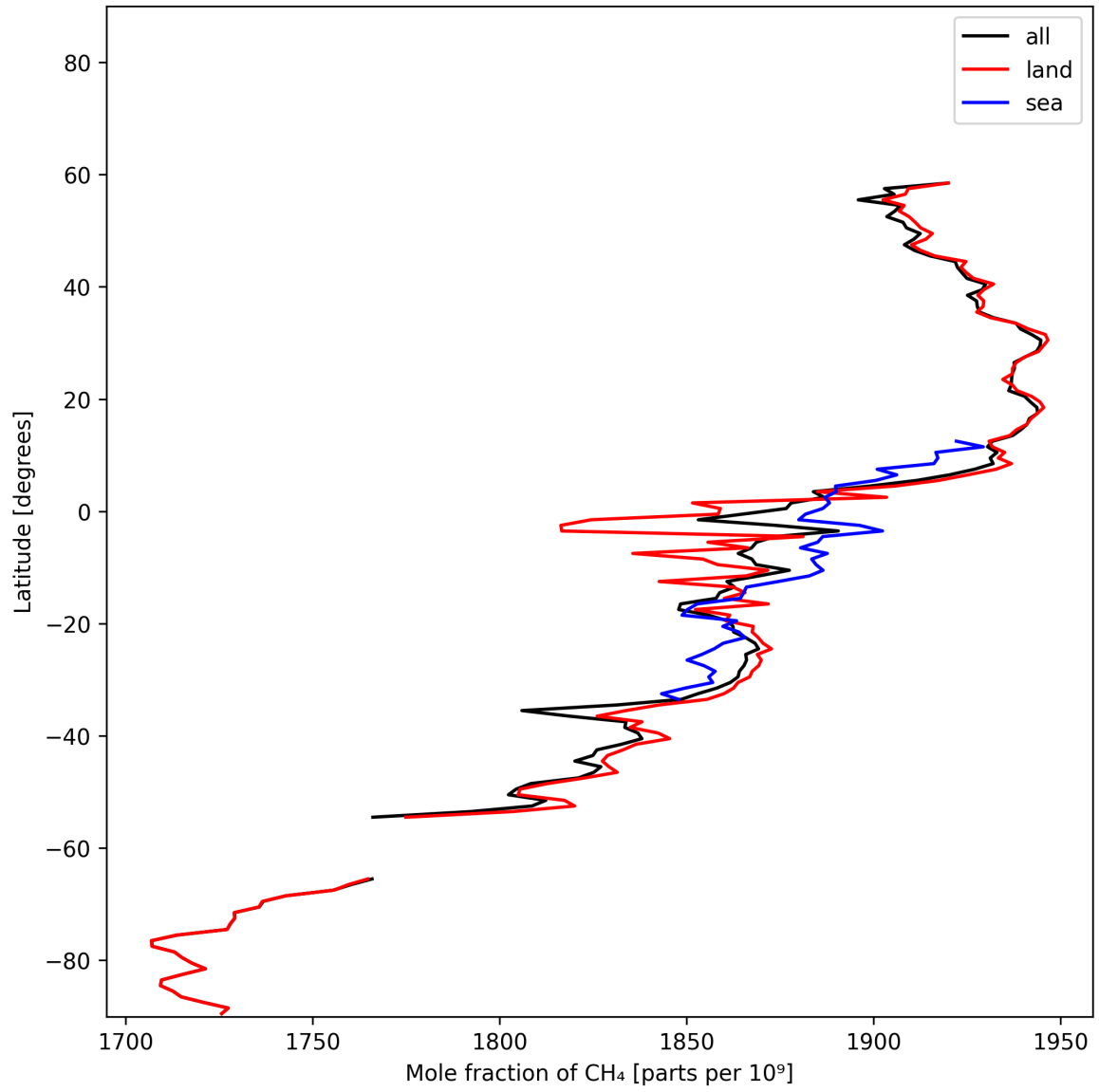
Figure 12: Zonal average of “Mole fraction of \text{CH}_4 ” for 2025-11-08 to 2025-11-10.
