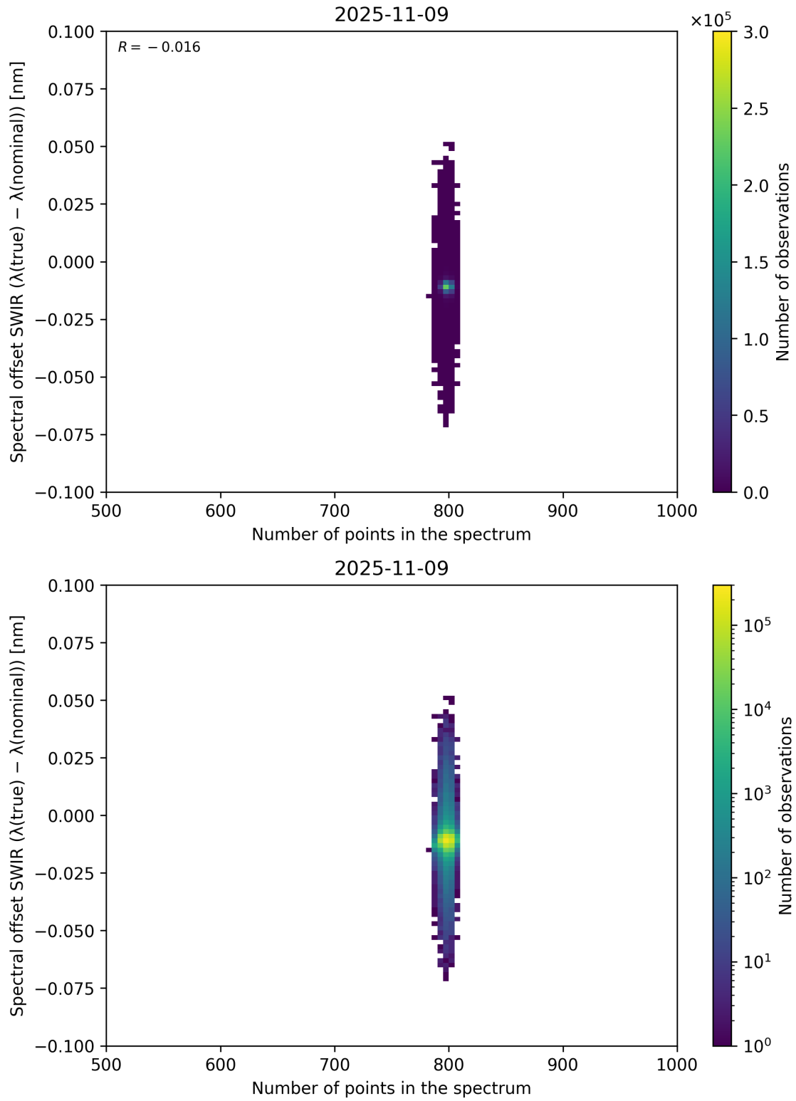
Figure 93: Scatter density plot of “Number of points in the spectrum” against “Spectral offset SWIR ( \lambda_{\text{true}} - \lambda_{\text{nominal}} )” for 2025-11-08 to 2025-11-10.
