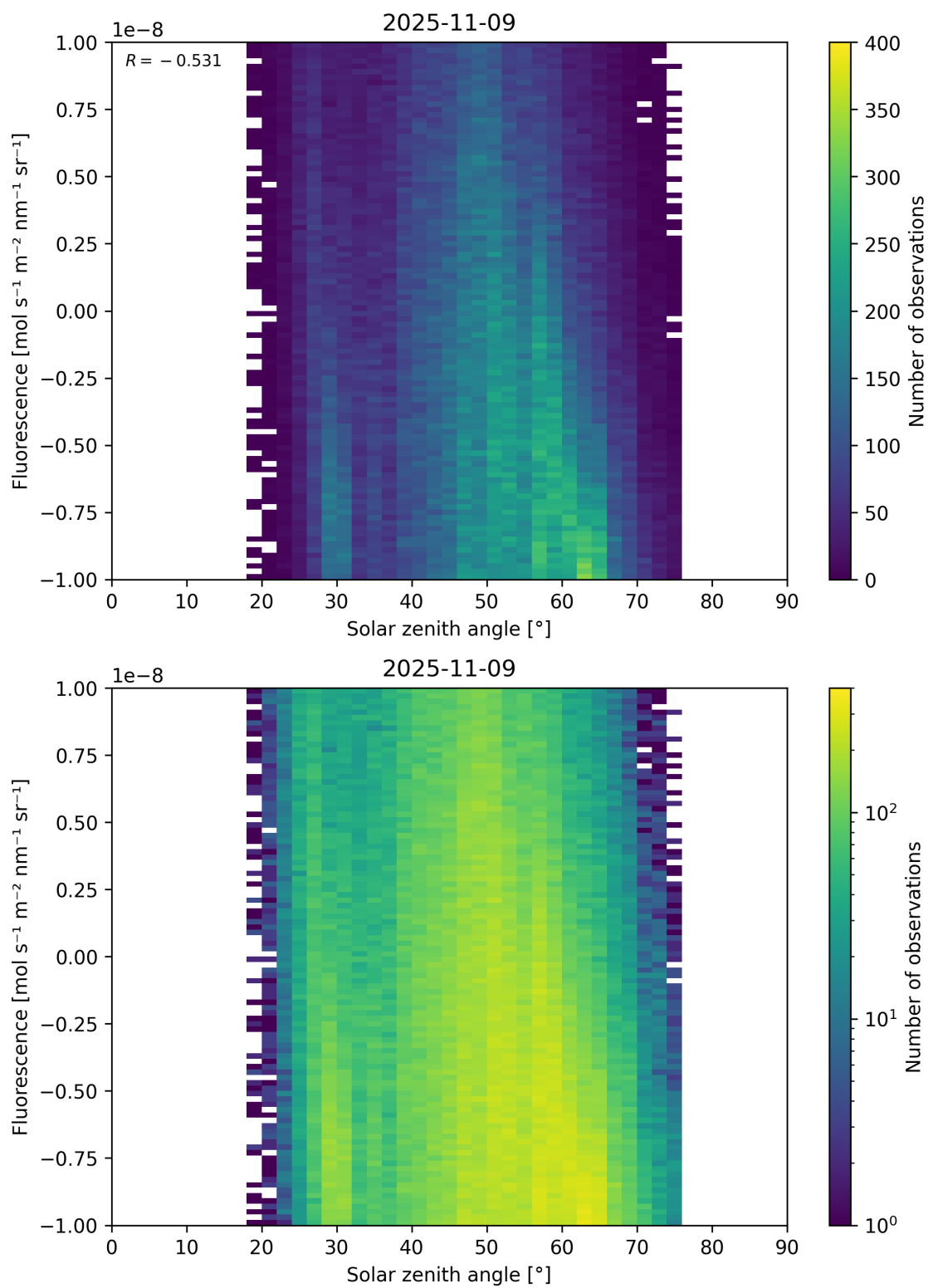
Figure 97: Scatter density plot of “Solar zenith angle” against “Fluorescence” for 2025-11-08 to 2025-11-10.
