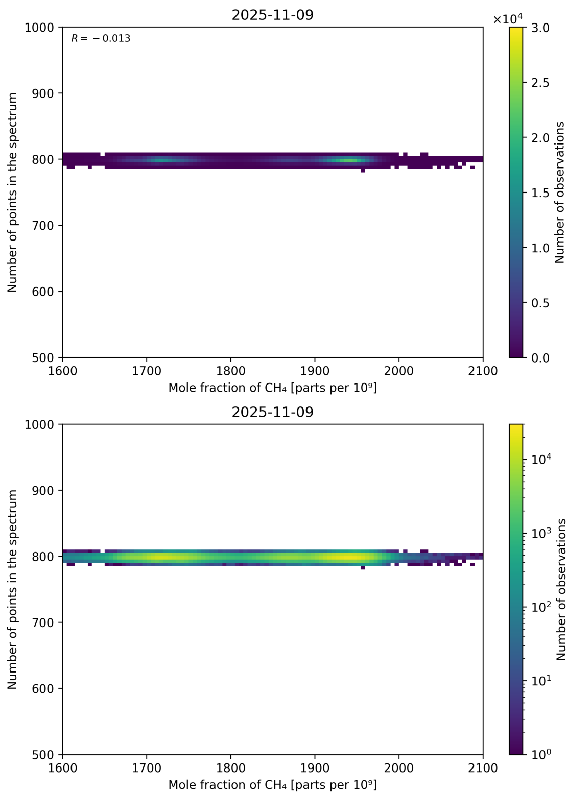
Figure 77: Scatter density plot of “Mole fraction of CH 4 ” against “Number of points in the spectrum” for 2025-11-08 to 2025-11-10.
