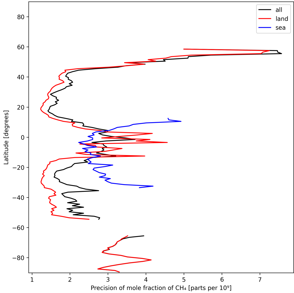
Figure 13: Zonal average of “Precision of mole fraction of CH 4 ” for 2025-11-08 to 2025-11-10.
