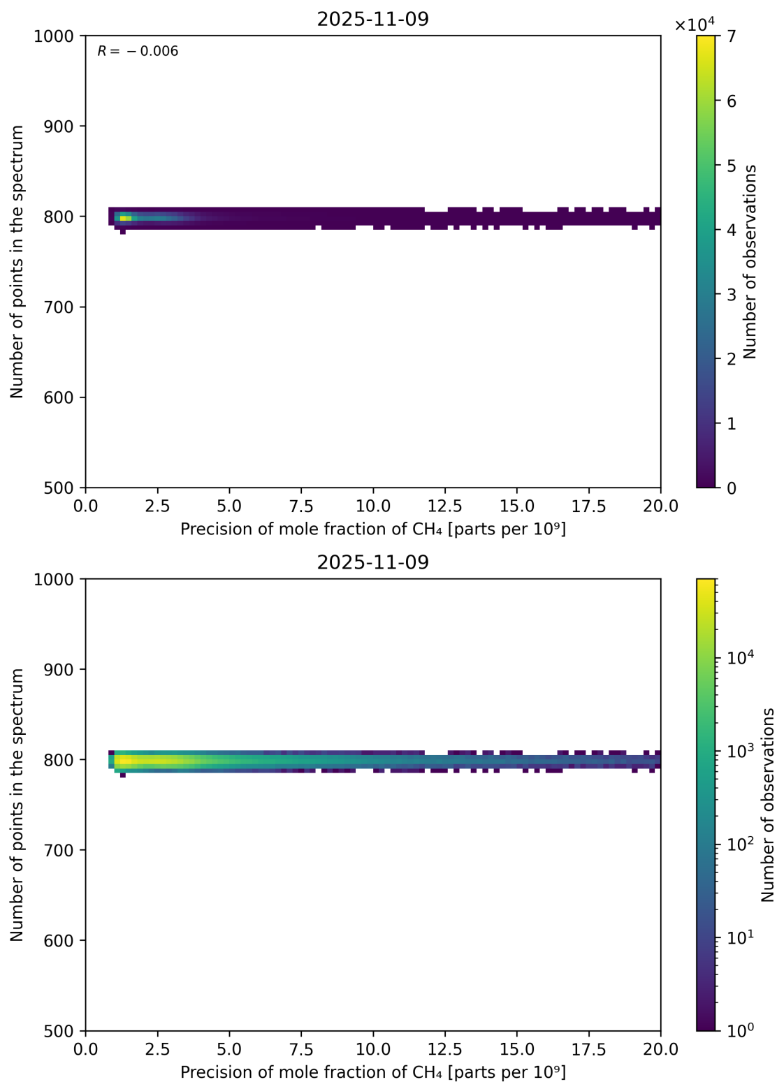
Figure 84: Scatter density plot of “Precision of mole fraction of CH 4 ” against “Number of points in the spectrum” for 2025-11-08 to 2025-11-10.
