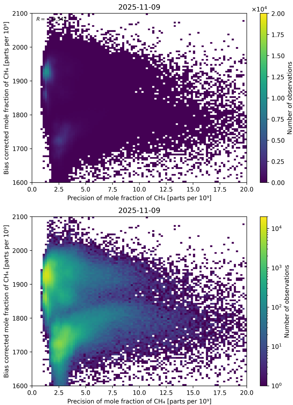
Figure 82: Scatter density plot of “Precision of mole fraction of CH 4 ” against “Bias corrected mole fraction of CH 4 ” for 2025-11-08 to 2025-11-10.
