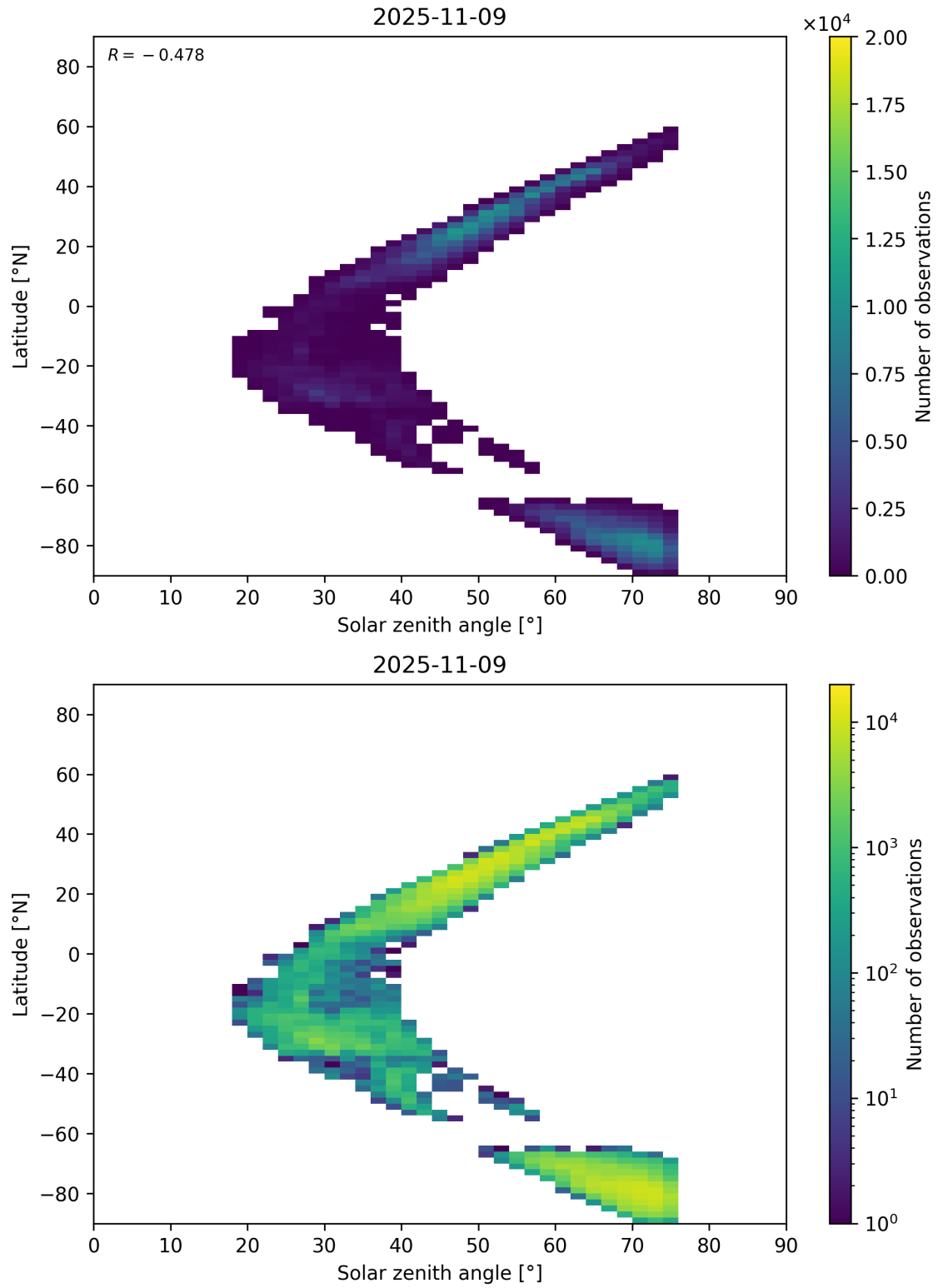
Figure 98: Scatter density plot of “Solar zenith angle” against “Latitude” for 2025-11-08 to 2025-11-10.
