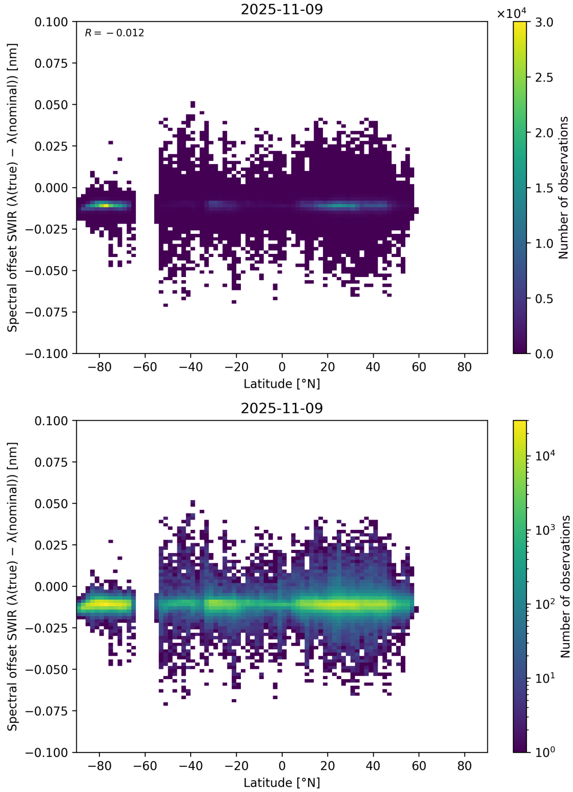
Figure 62: Scatter density plot of “Latitude” against “Spectral offset SWIR ( \lambda_{\text{true}} - \lambda_{\text{nominal}} )” for 2025-11-08 to 2025-11-10.
