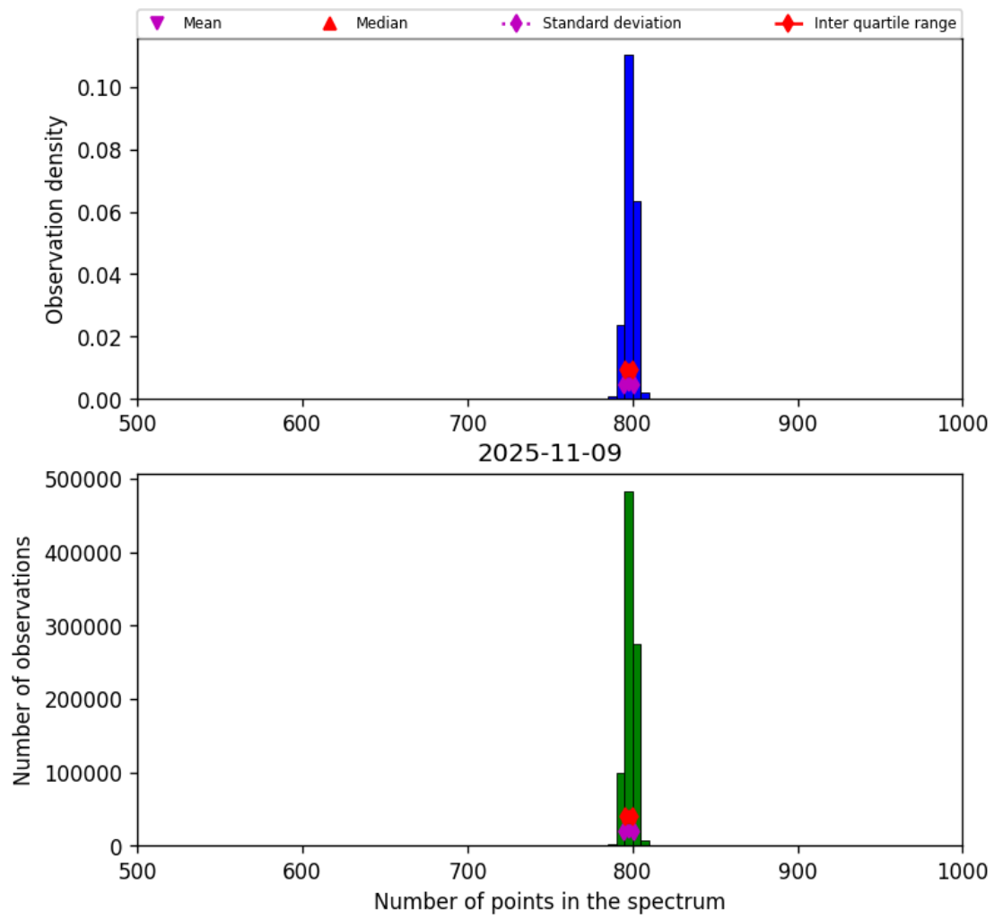
Figure 26: Histogram of “Number of points in the spectrum” for 2025-11-08 to 2025-11-10
