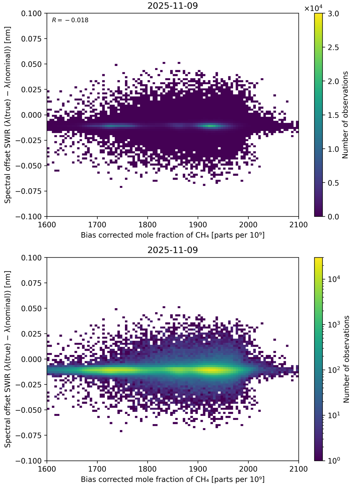
Figure 69: Scatter density plot of “Bias corrected mole fraction of \text{CH}_4 ” against “Spectral offset SWIR ( \lambda_{\text{true}} - \lambda_{\text{nominal}} )” for 2025-11-08 to 2025-11-10.
