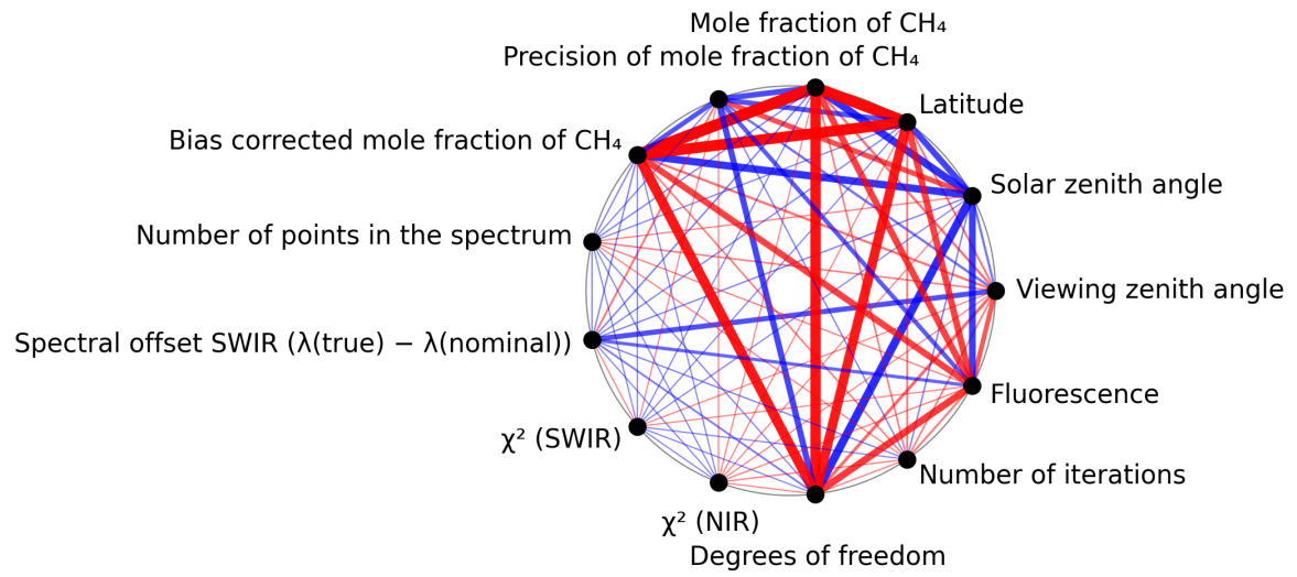
Figure 1: Map of correlation graph for 2025-11-08 to 2025-11-10.
