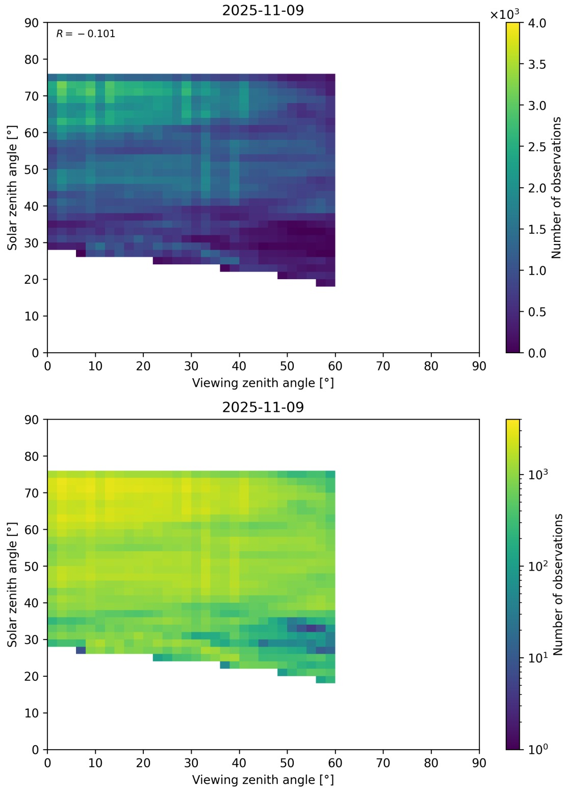
Figure 115: Scatter density plot of “Viewing zenith angle” against “Solar zenith angle” for 2025-11-08 to 2025-11-10.
