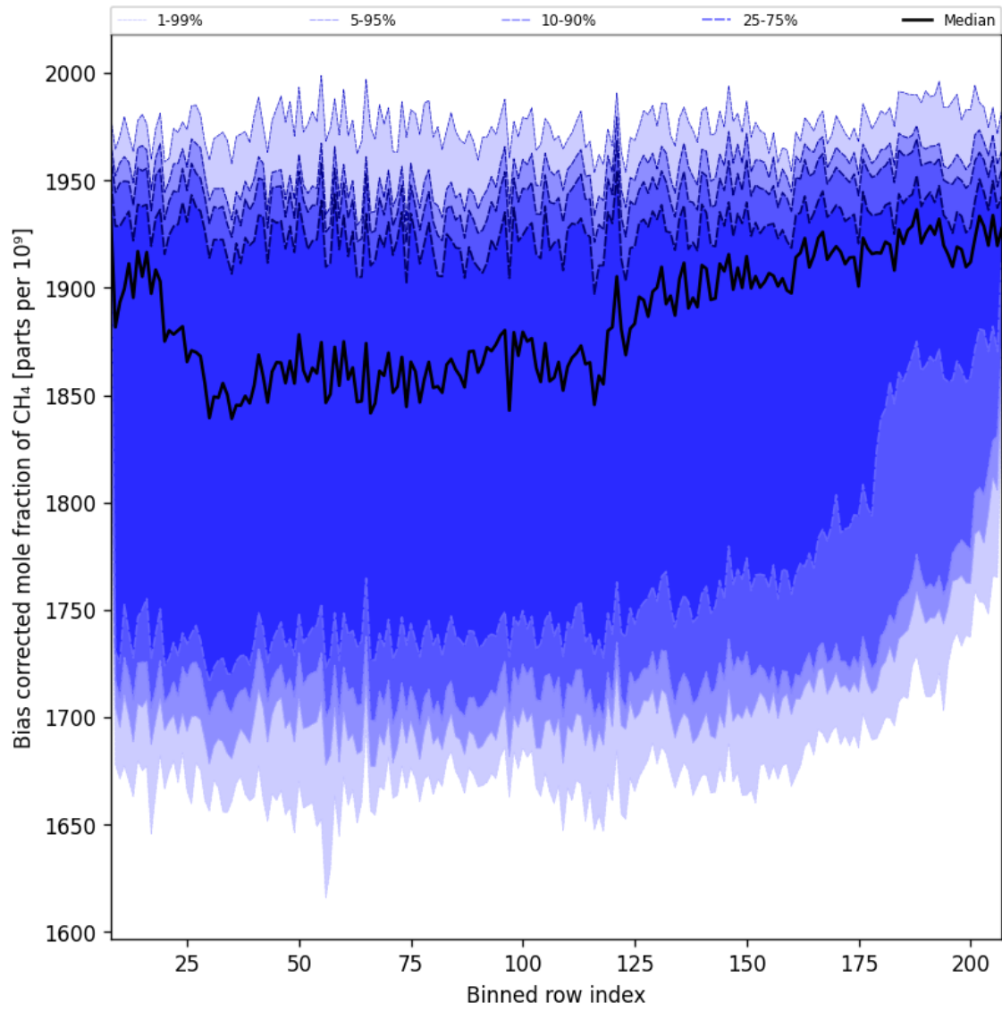
Figure 36: Along track statistics of “Bias corrected mole fraction of CH 4 ” for 2025-11-08 to 2025-11-10
