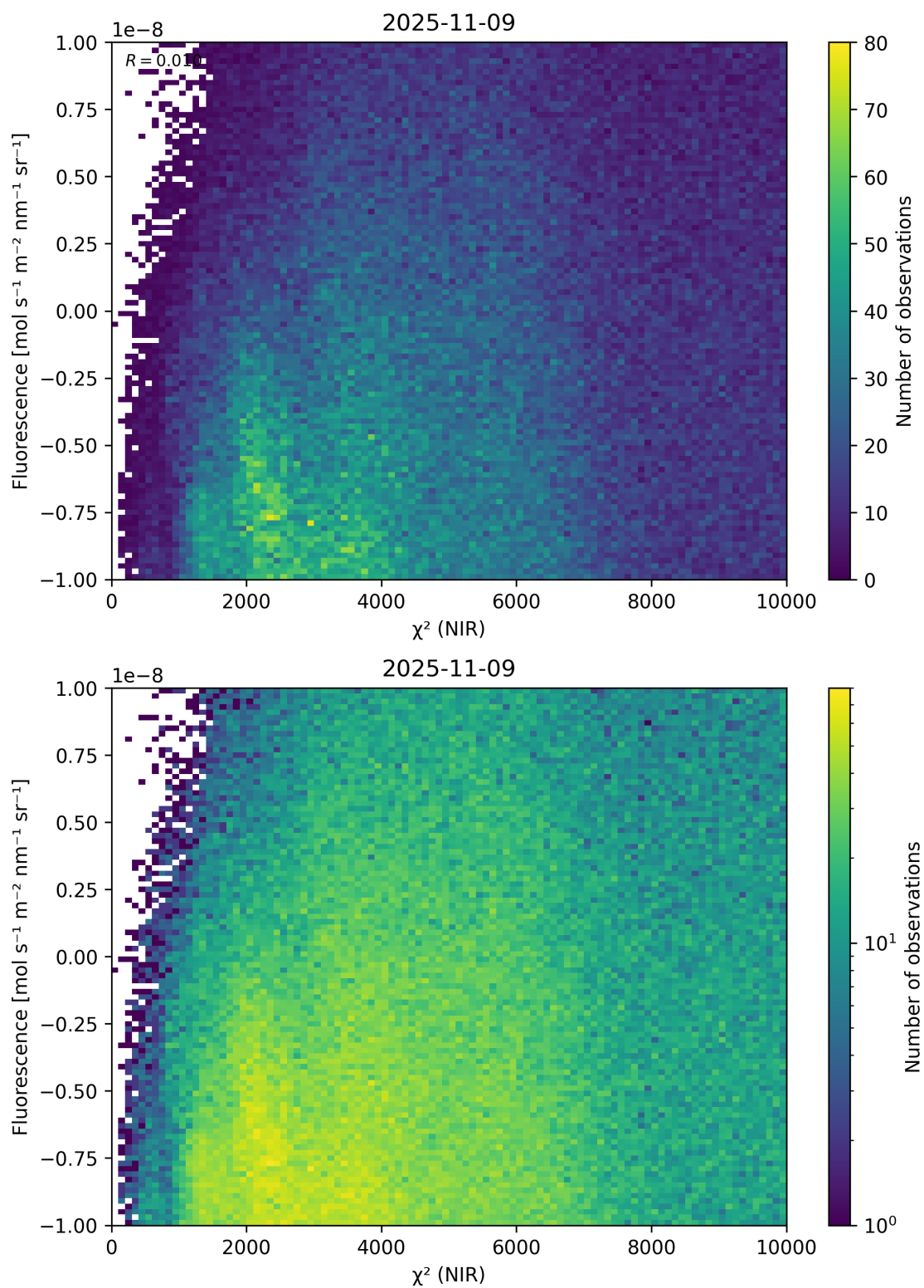
Figure 45: Scatter density plot of “ \chi^2 (NIR)” against “Fluorescence” for 2025-11-08 to 2025-11-10.
