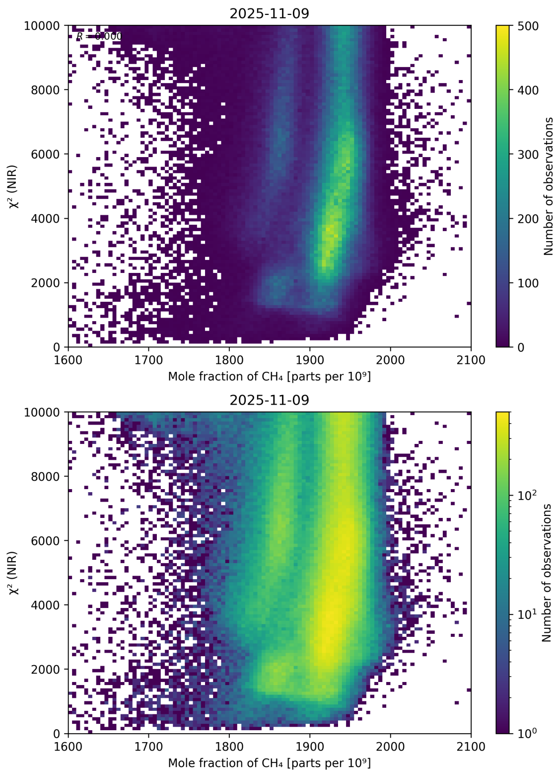
Figure 70: Scatter density plot of “Mole fraction of \text{CH}_4 ” against “ \chi^2 (NIR)” for 2025-11-08 to 2025-11-10.
