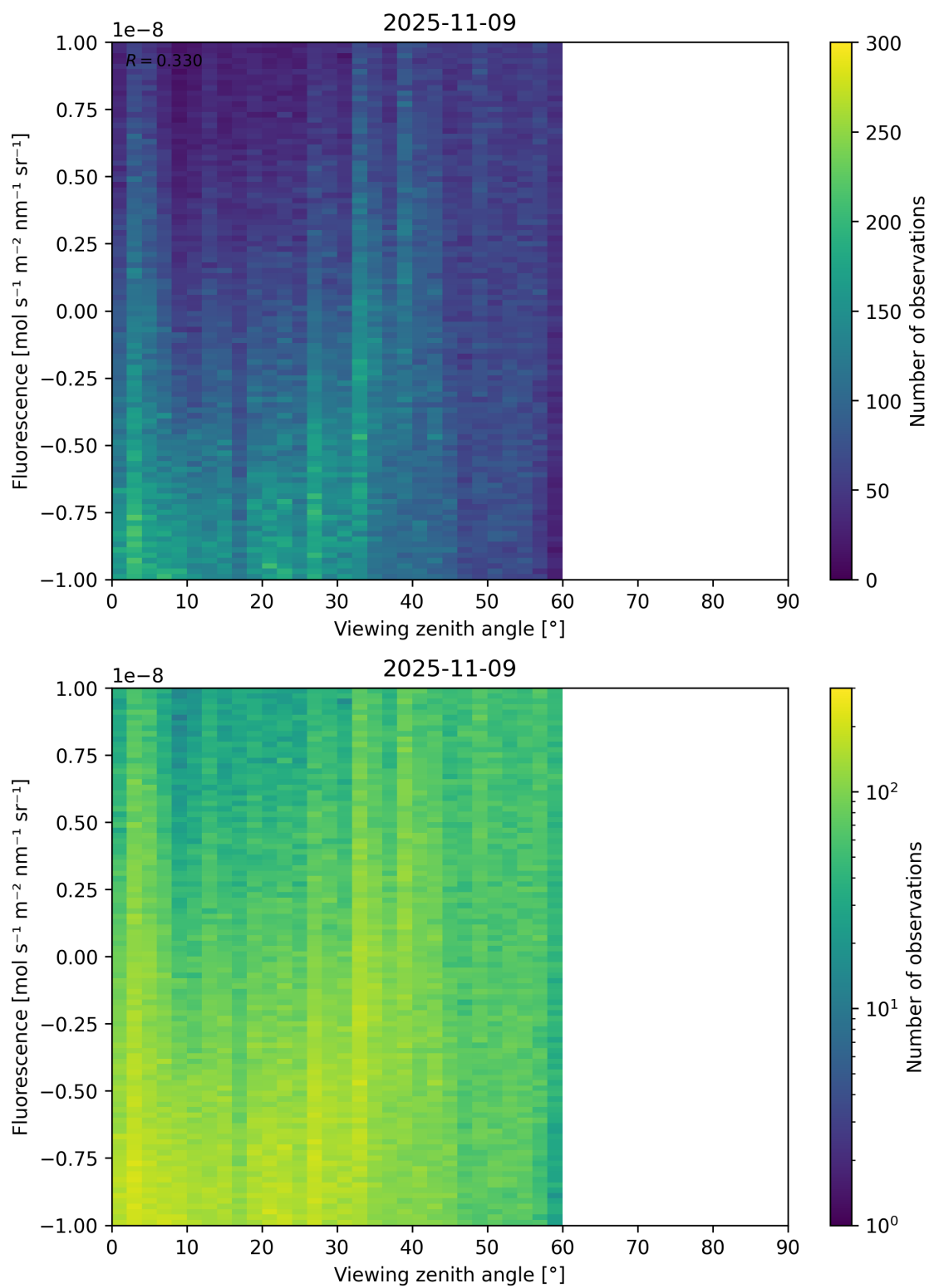
Figure 108: Scatter density plot of “Viewing zenith angle” against “Fluorescence” for 2025-11-08 to 2025-11-10.
