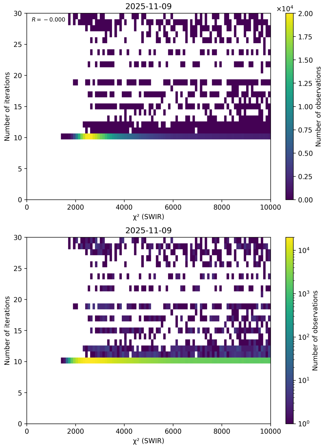
Figure 50: Scatter density plot of “ \chi^2 (SWIR)” against “Number of iterations” for 2025-11-08 to 2025-11-10.
