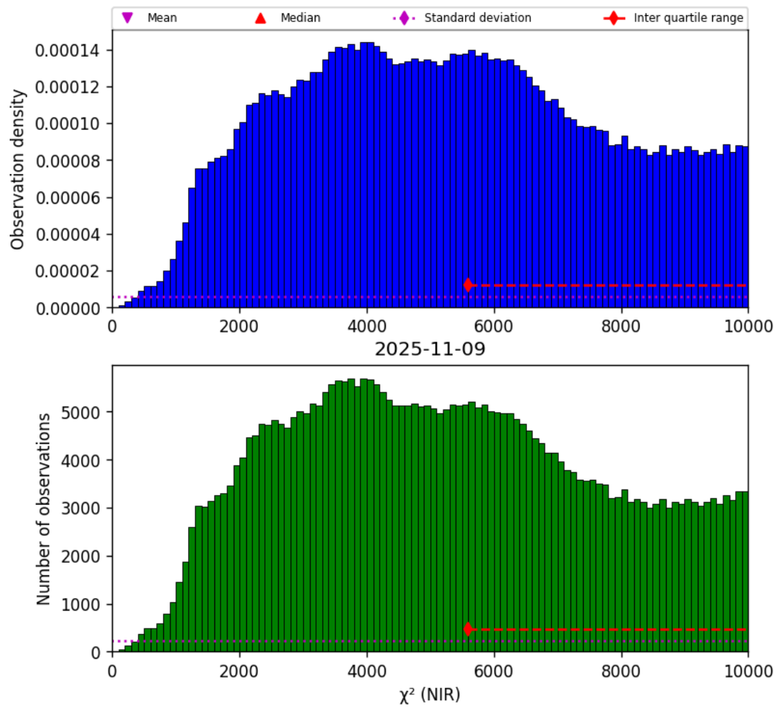
Figure 29: Histogram of " \chi^2 (NIR)" for 2025-11-08 to 2025-11-10
