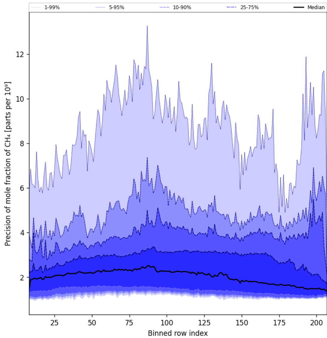
Figure 35: Along track statistics of “Precision of mole fraction of CH 4 ” for 2025-11-08 to 2025-11-10
