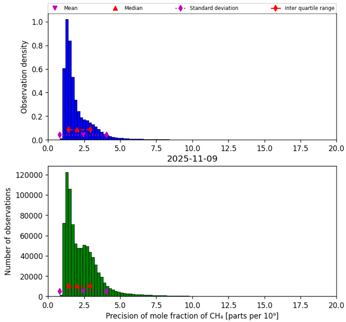
Figure 24: Histogram of “Precision of mole fraction of CH 4 ” for 2025-11-08 to 2025-11-10
