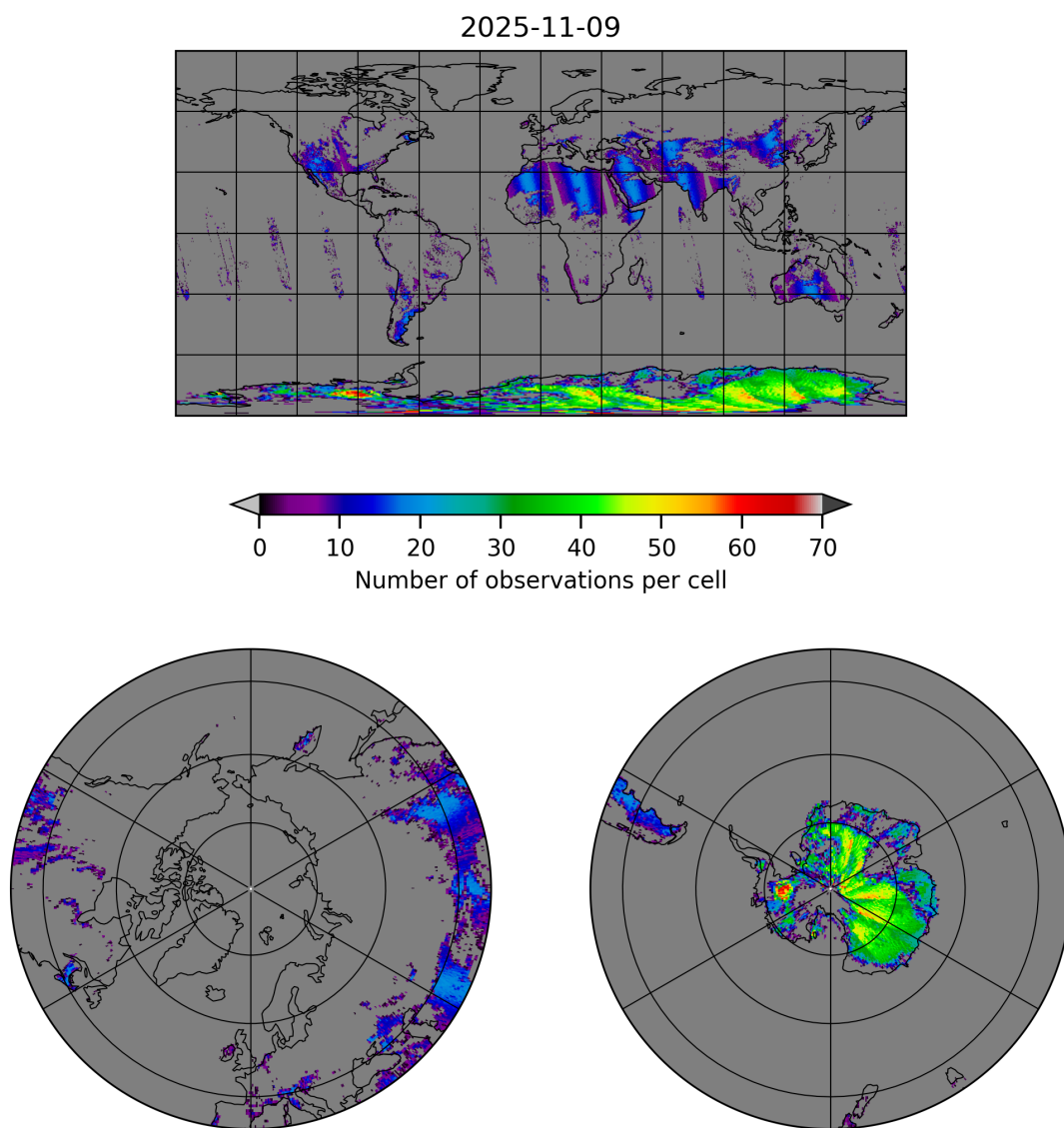
Figure 10: Map of the number of observations for 2025-11-08 to 2025-11-10
