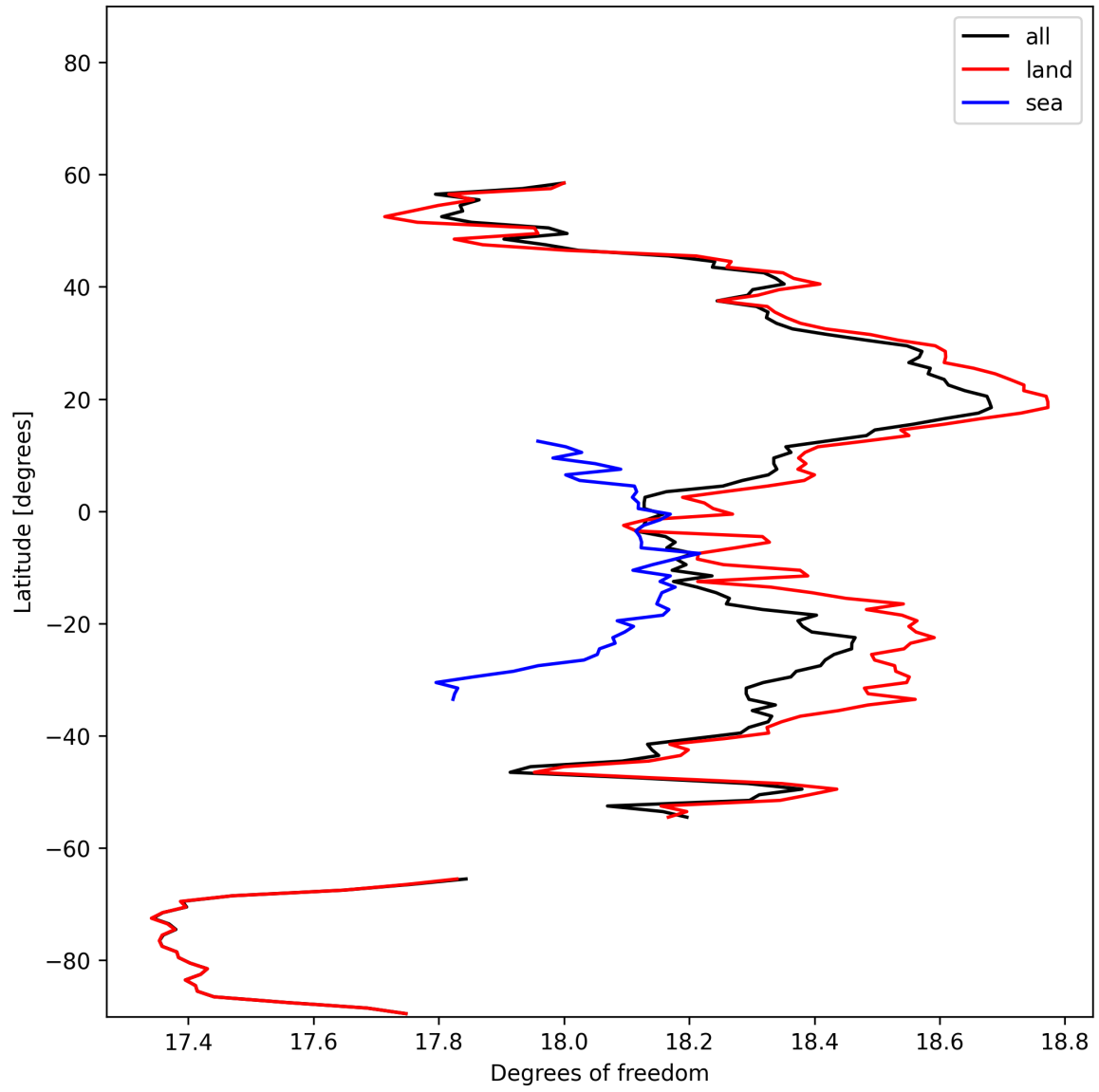
Figure 19: Zonal average of “Degrees of freedom” for 2025-11-08 to 2025-11-10.
