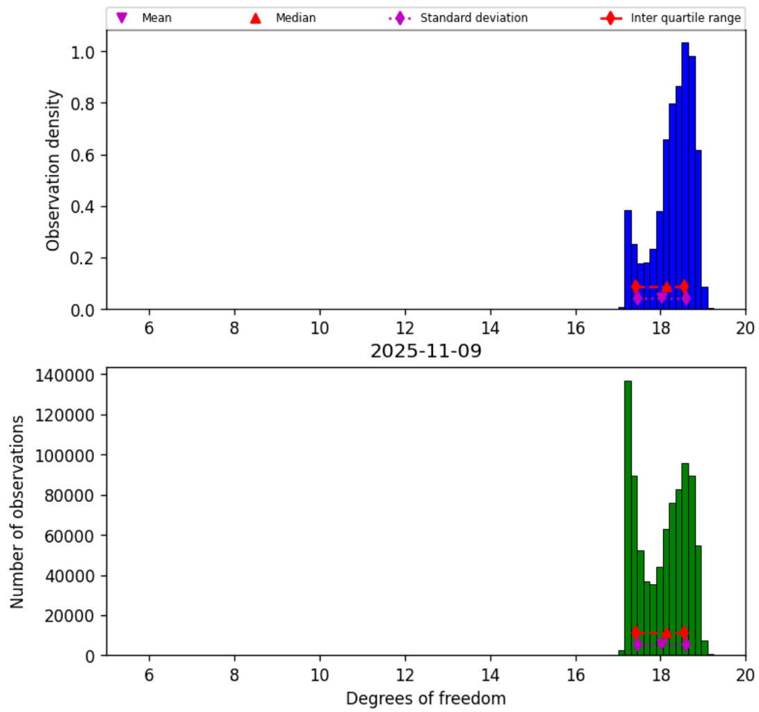
Figure 30: Histogram of "Degrees of freedom" for 2025-11-08 to 2025-11-10
