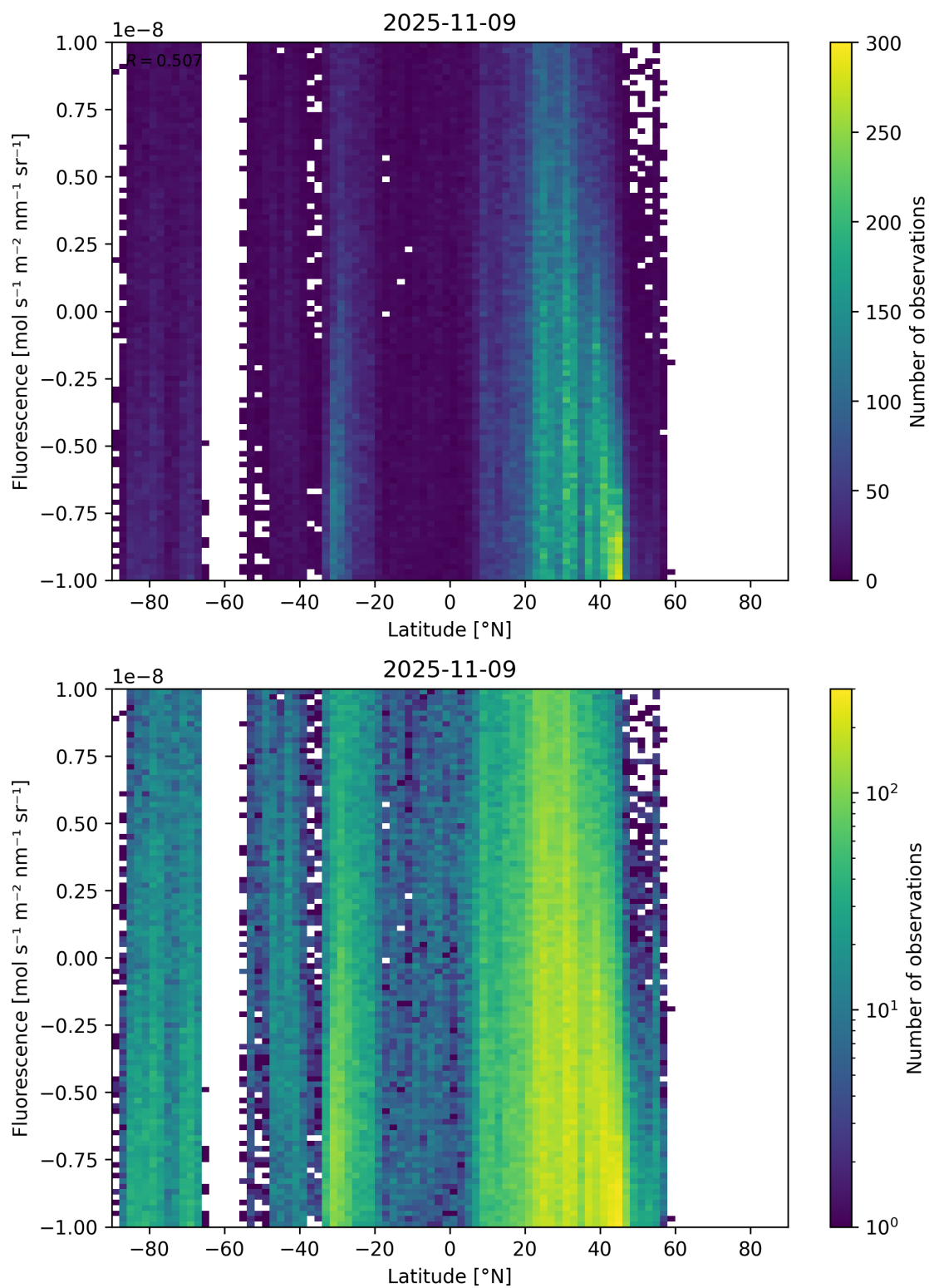
Figure 56: Scatter density plot of “Latitude” against “Fluorescence” for 2025-11-08 to 2025-11-10.
