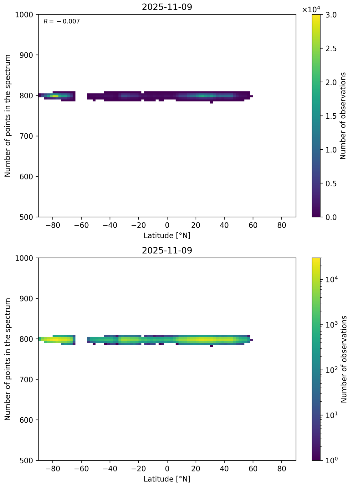
Figure 61: Scatter density plot of “Latitude” against “Number of points in the spectrum” for 2025-11-08 to 2025-11-10.
