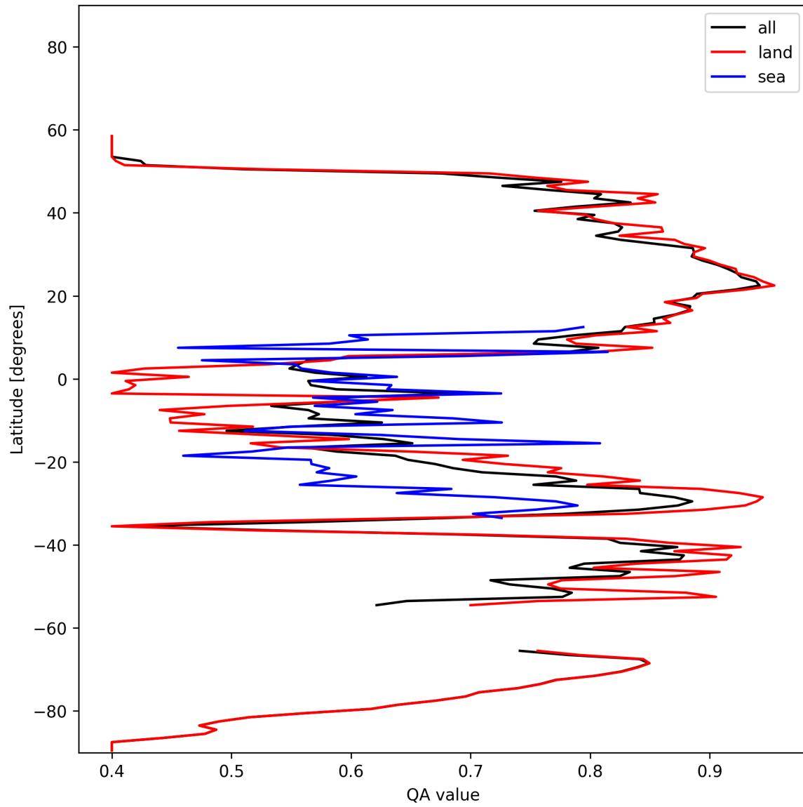
Figure 11: Zonal average of “QA value” for 2025-11-08 to 2025-11-10.
