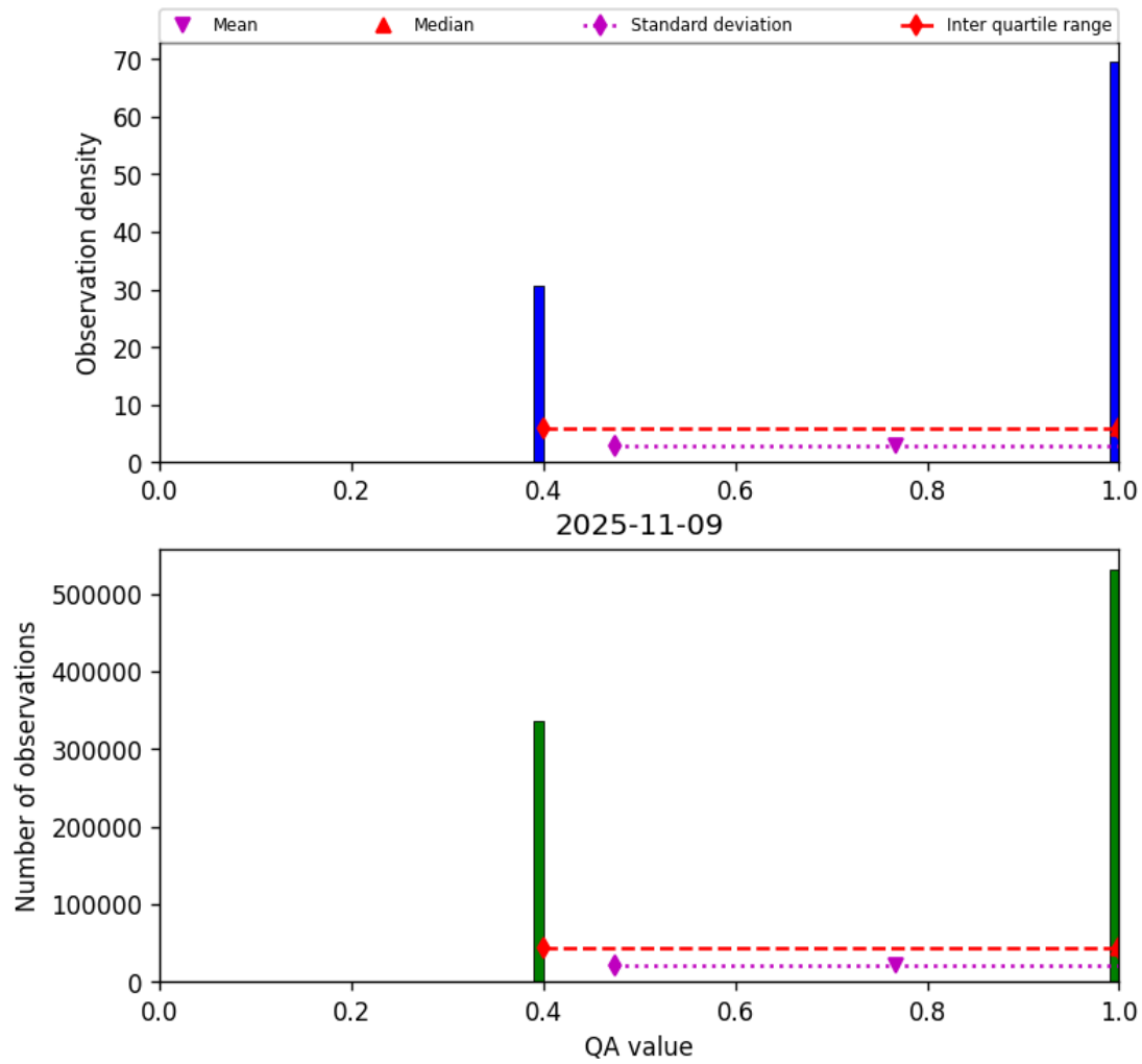
Figure 22: Histogram of “QA value” for 2025-11-08 to 2025-11-10
