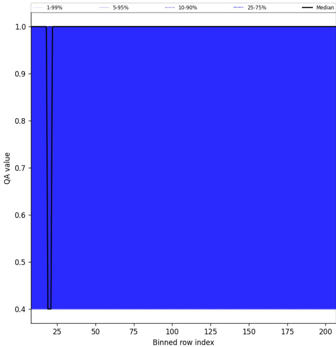
Figure 33: Along track statistics of “QA value” for 2025-11-08 to 2025-11-10
