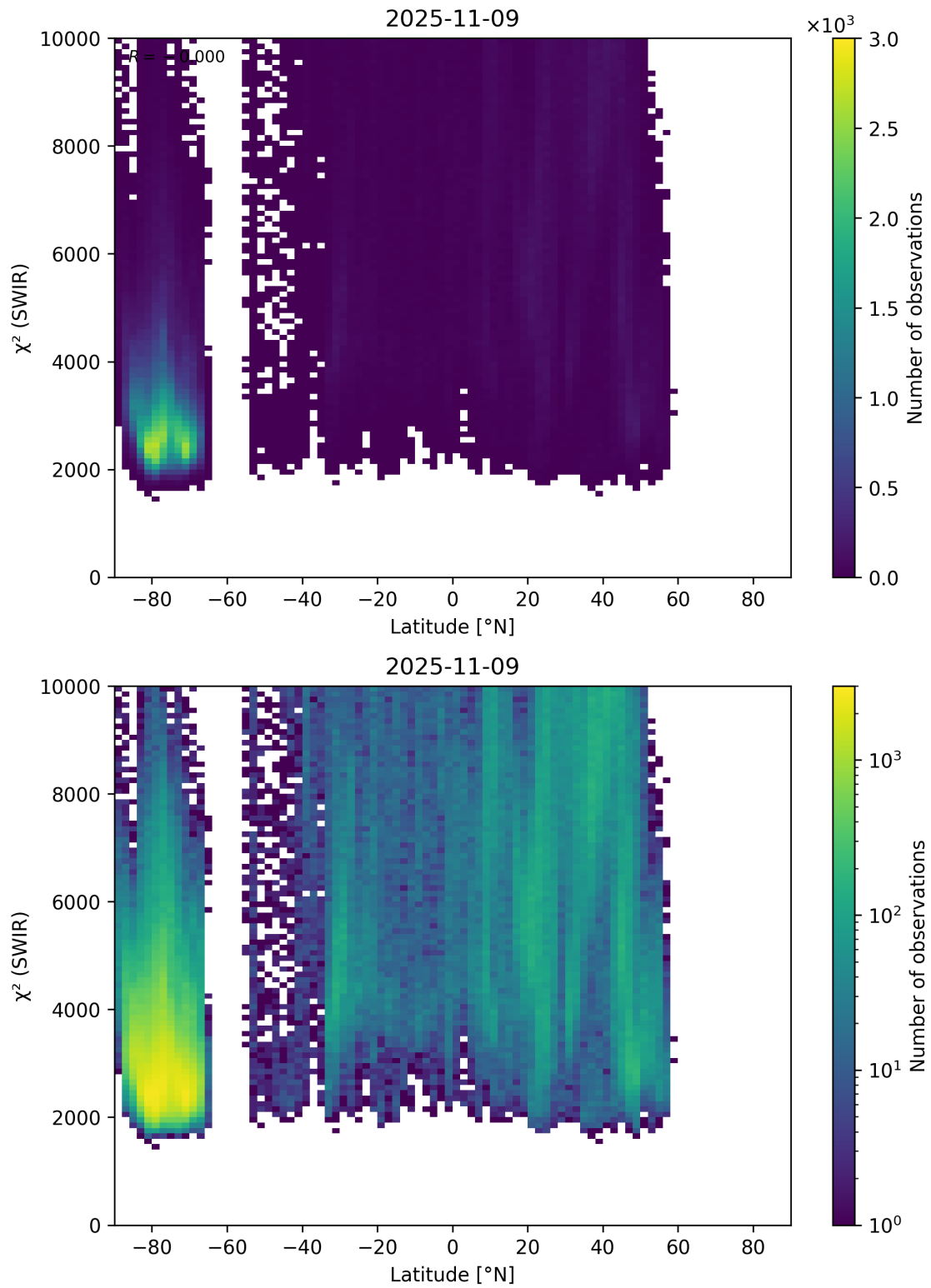
Figure 54: Scatter density plot of “Latitude” against “ \chi^2 (SWIR)” for 2025-11-08 to 2025-11-10.
