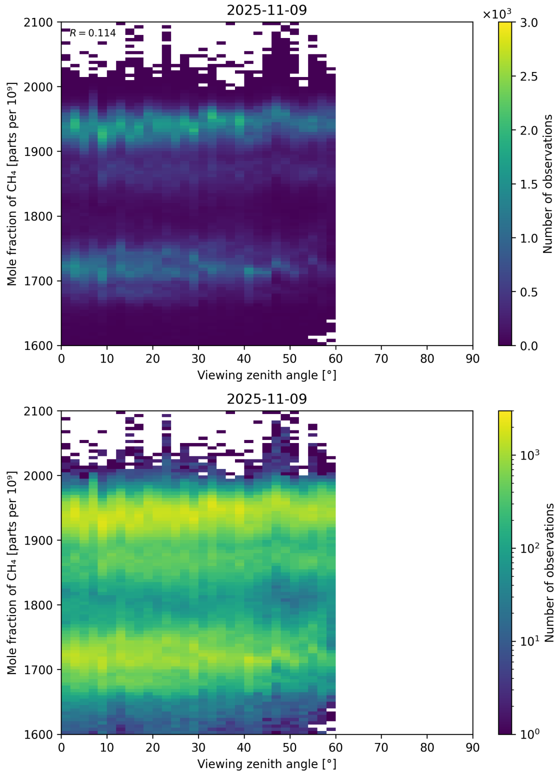
Figure 110: Scatter density plot of “Viewing zenith angle” against “Mole fraction of CH 4 ” for 2025-11-08 to 2025-11-10.
