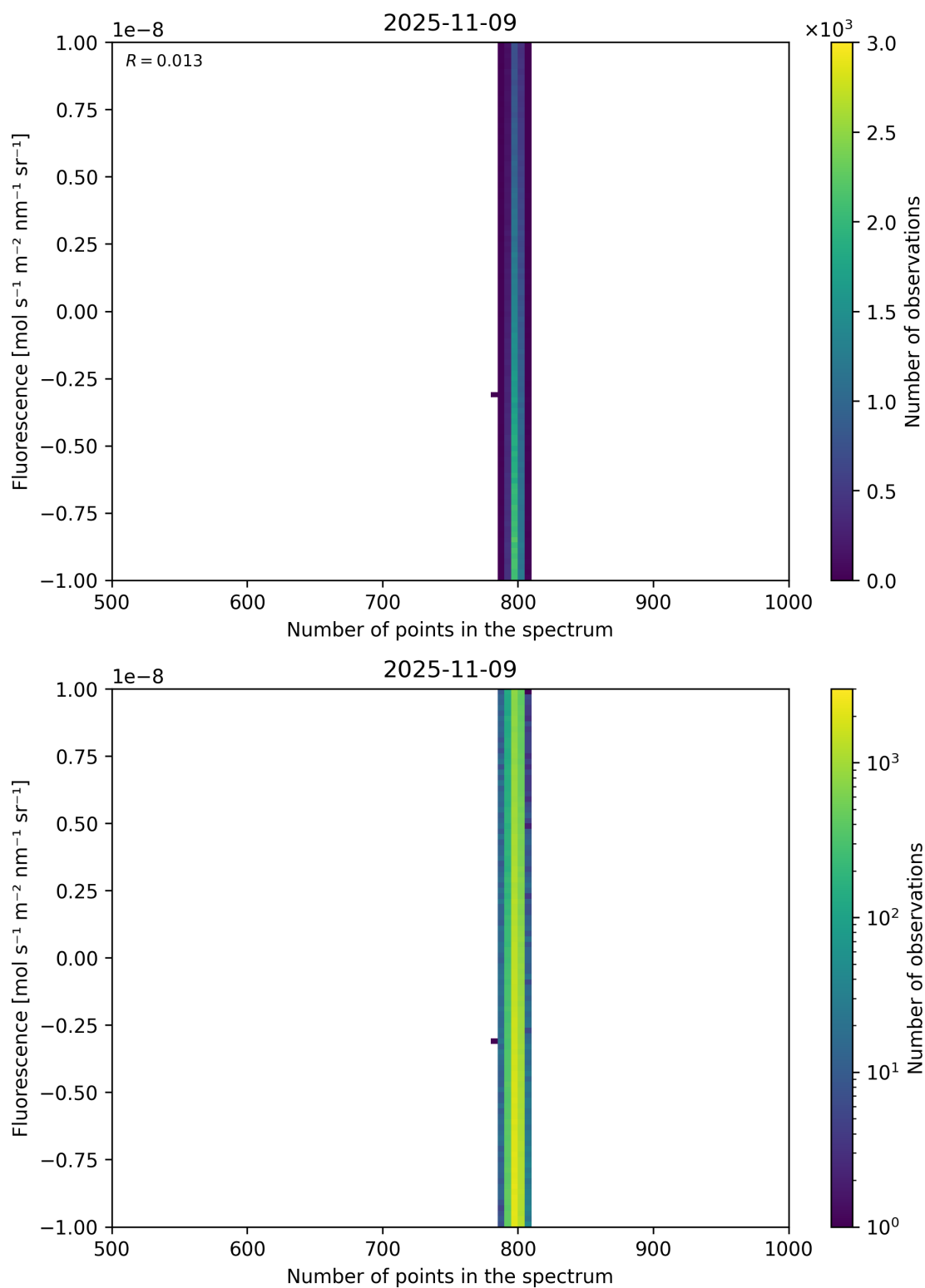
Figure 91: Scatter density plot of “Number of points in the spectrum” against “Fluorescence” for 2025-11-08 to 2025-11-10.
