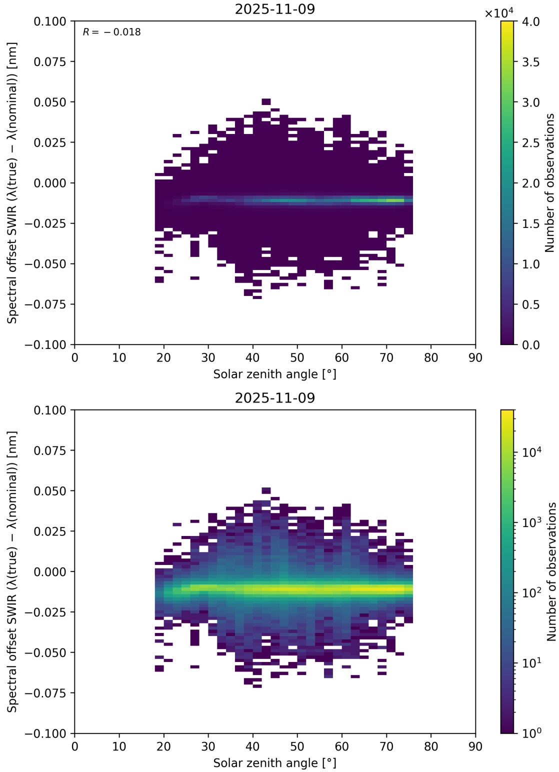
Figure 104: Scatter density plot of “Solar zenith angle” against “Spectral offset SWIR ( \lambda_{\text{true}} - \lambda_{\text{nominal}} )” for 2025-11-08 to 2025-11-10.
