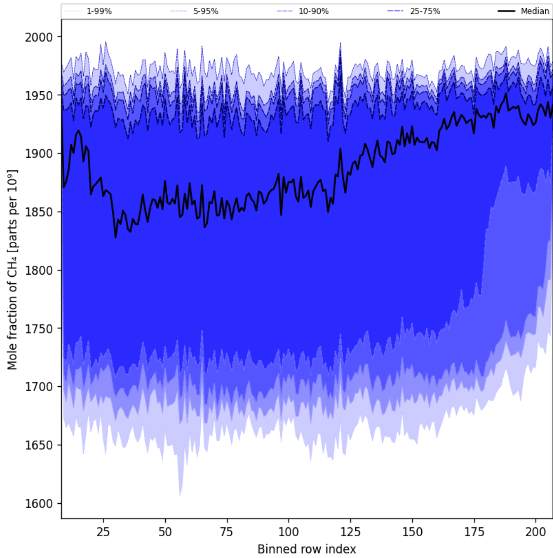
Figure 34: Along track statistics of “Mole fraction of CH 4 ” for 2025-11-08 to 2025-11-10
