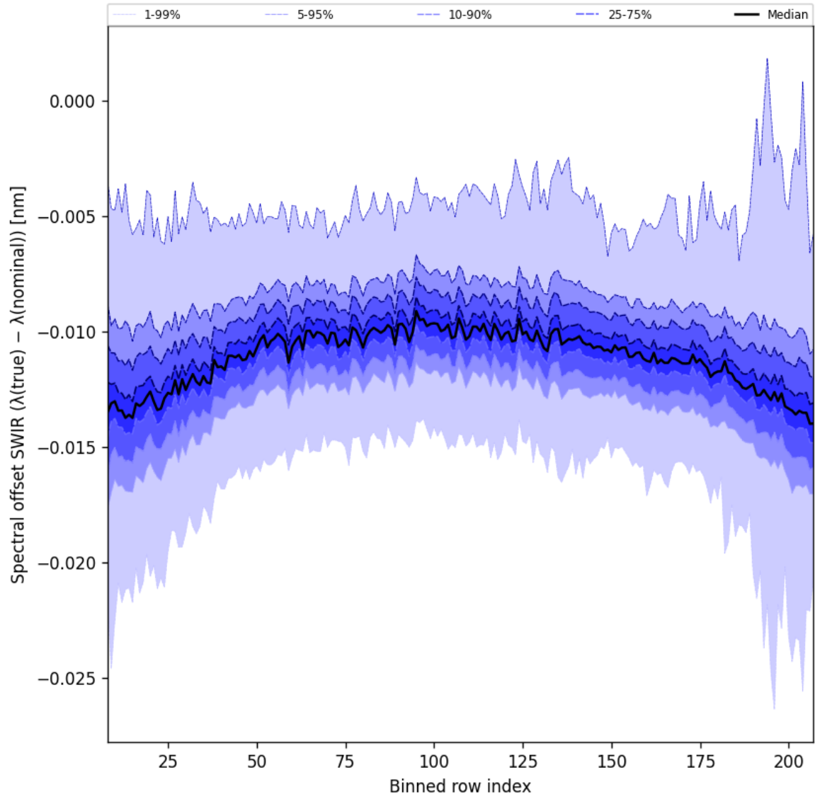
Figure 38: Along track statistics of “Spectral offset SWIR ( \lambda_{\text{true}} - \lambda_{\text{nominal}} )” for 2025-11-08 to 2025-11-10
