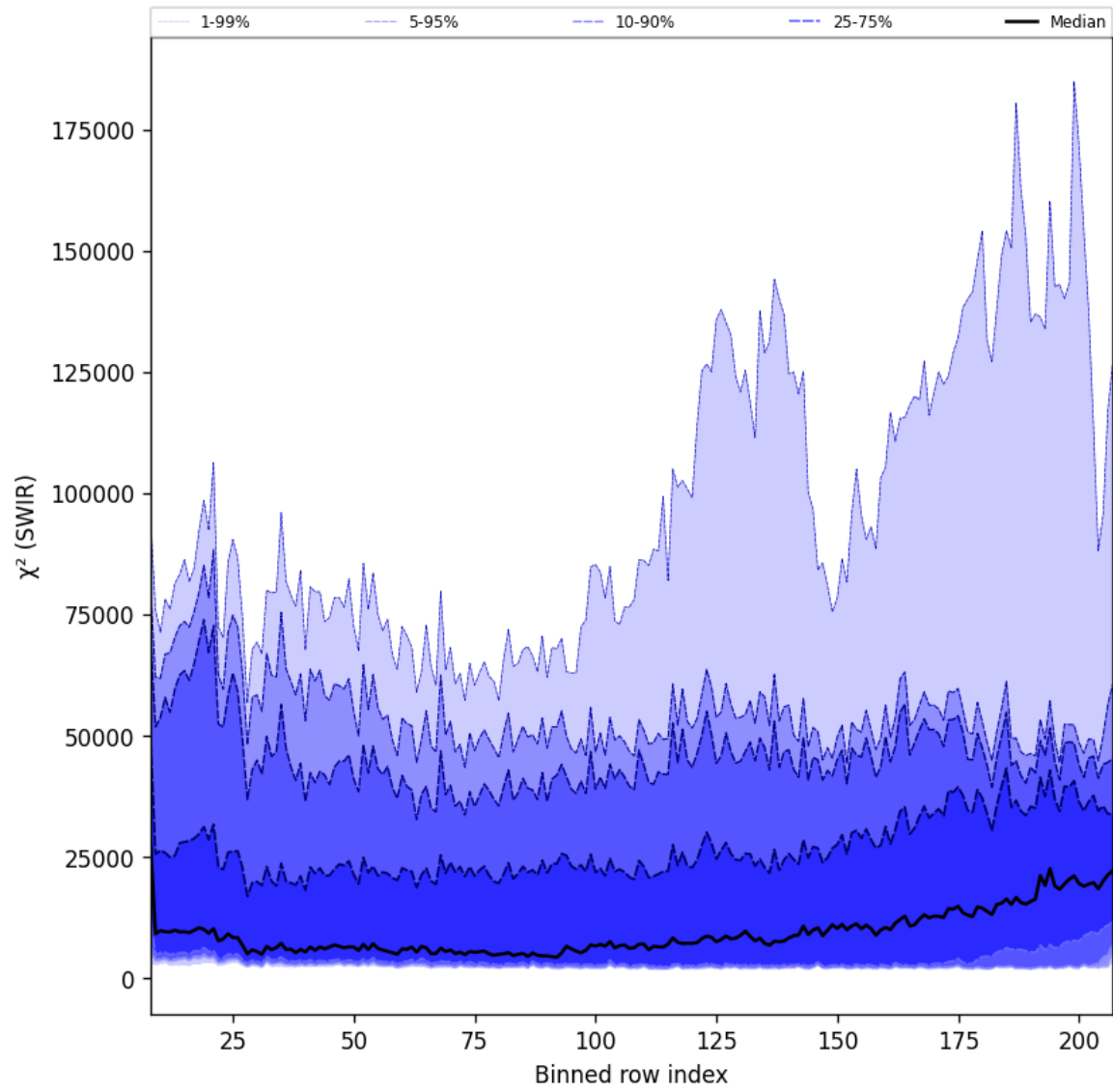
Figure 39: Along track statistics of “ \chi^2 (SWIR)” for 2025-11-08 to 2025-11-10
