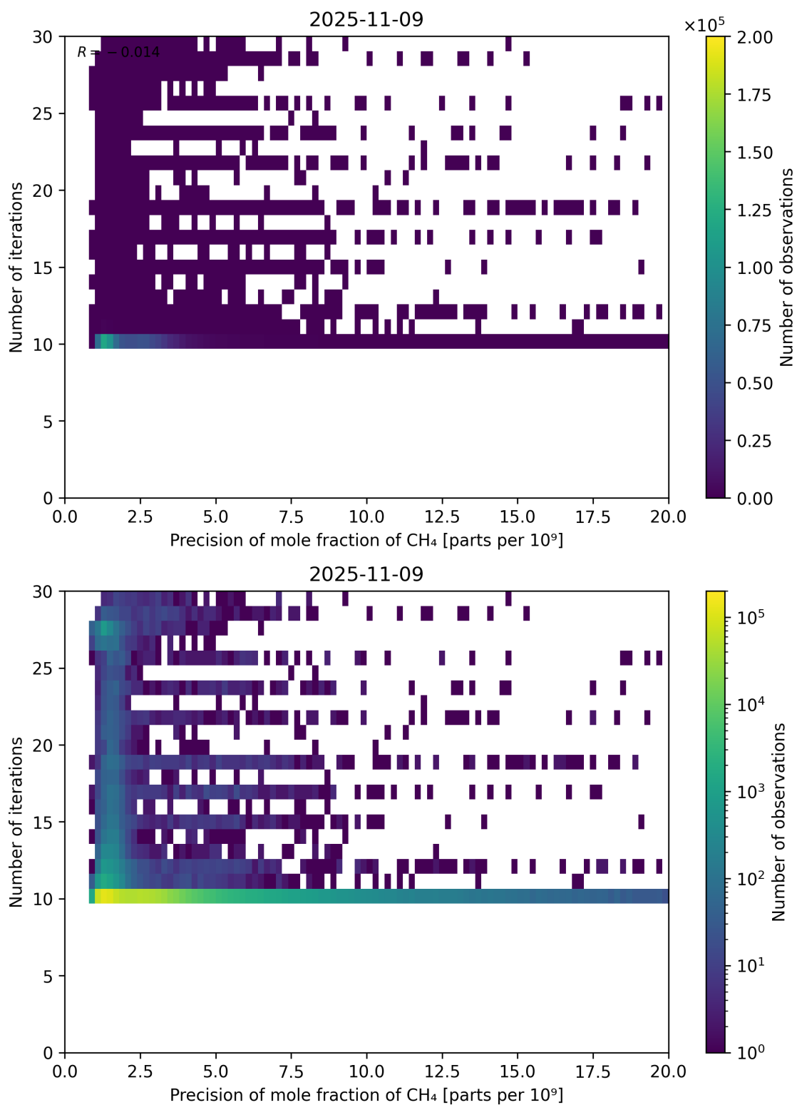
Figure 83: Scatter density plot of “Precision of mole fraction of \text{CH}_4 ” against “Number of iterations” for 2025-11-08 to 2025-11-10.
