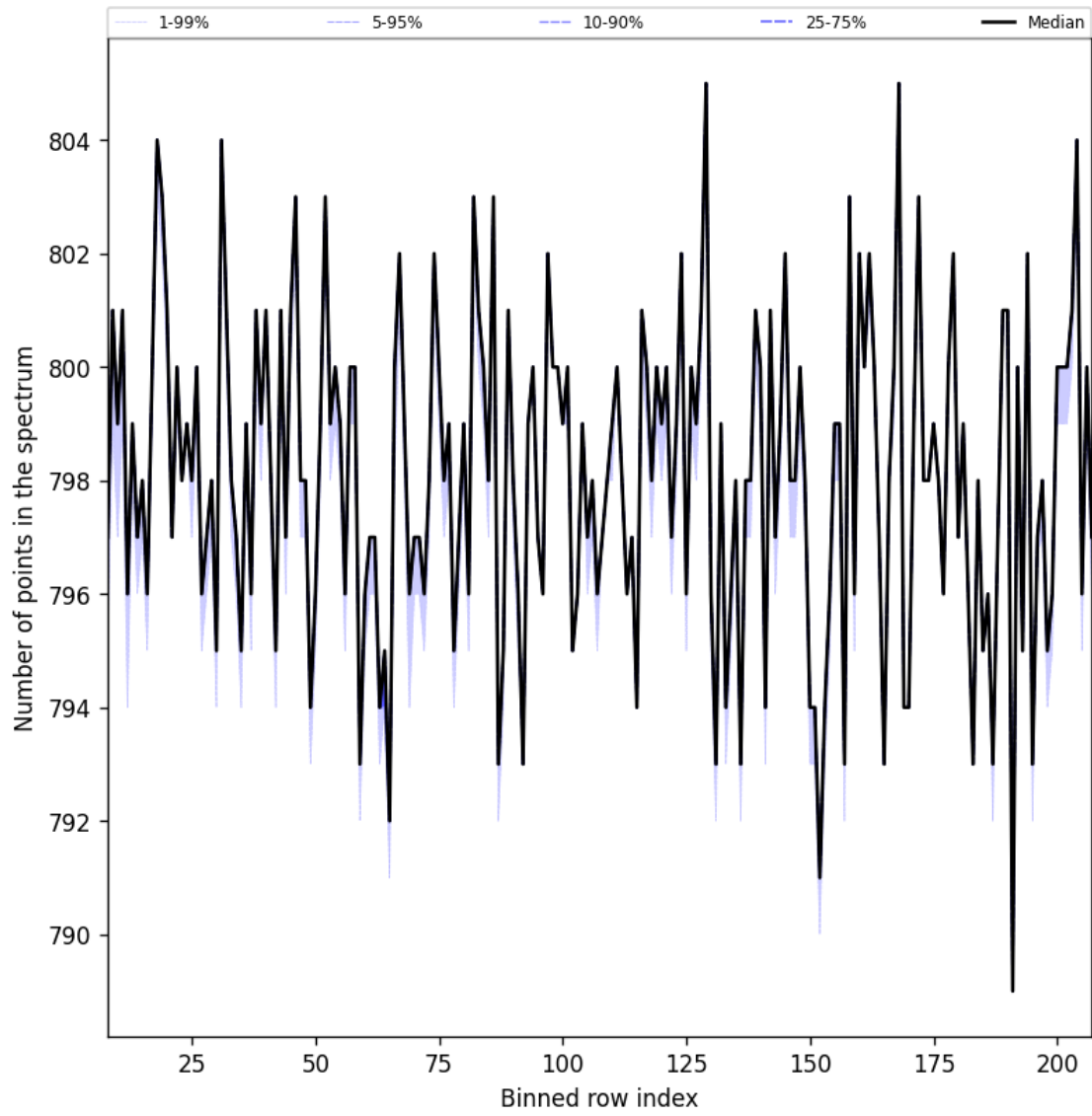
Figure 37: Along track statistics of “Number of points in the spectrum” for 2025-11-08 to 2025-11-10
