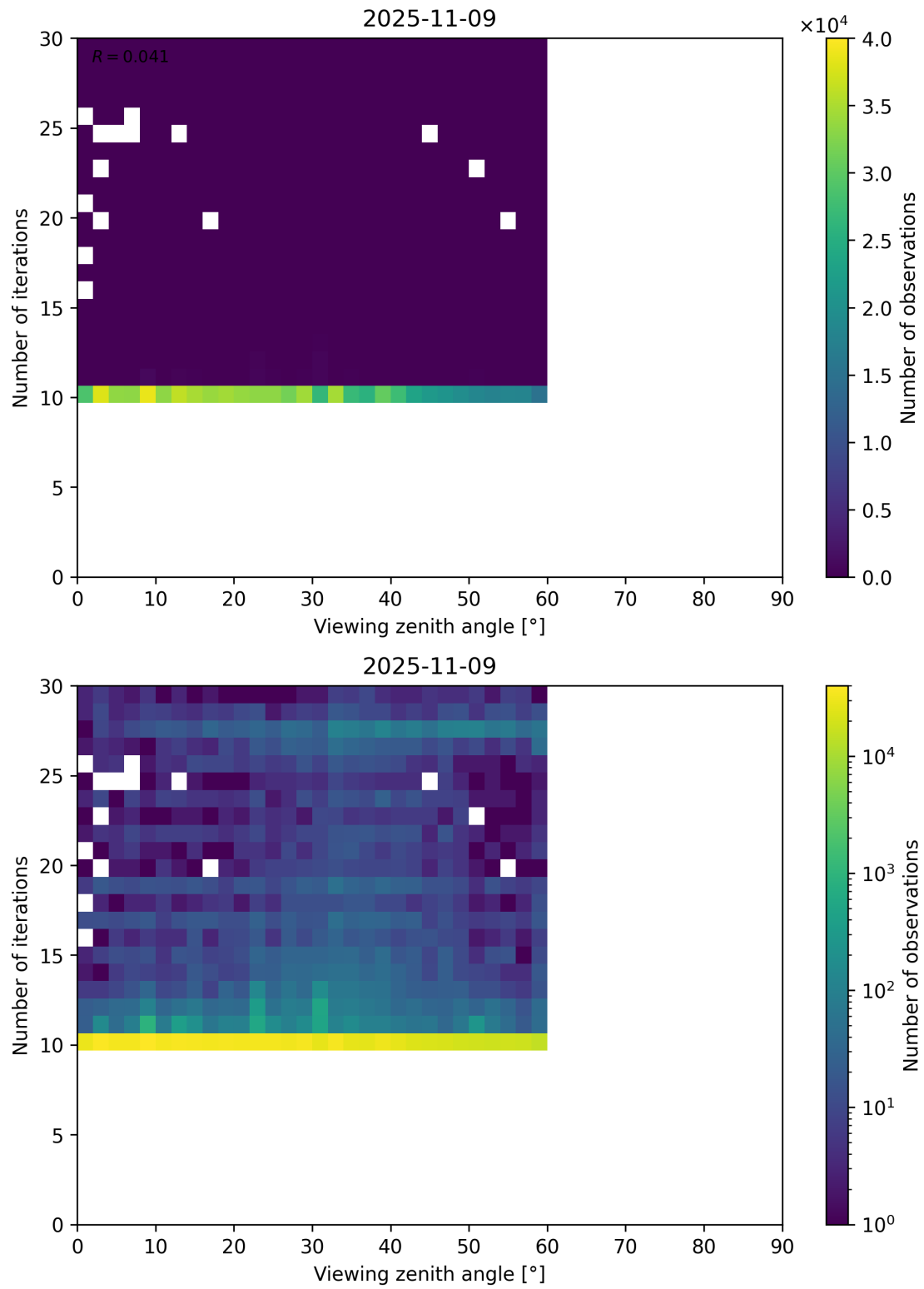
Figure 113: Scatter density plot of “Viewing zenith angle” against “Number of iterations” for 2025-11-08 to 2025-11-10.
