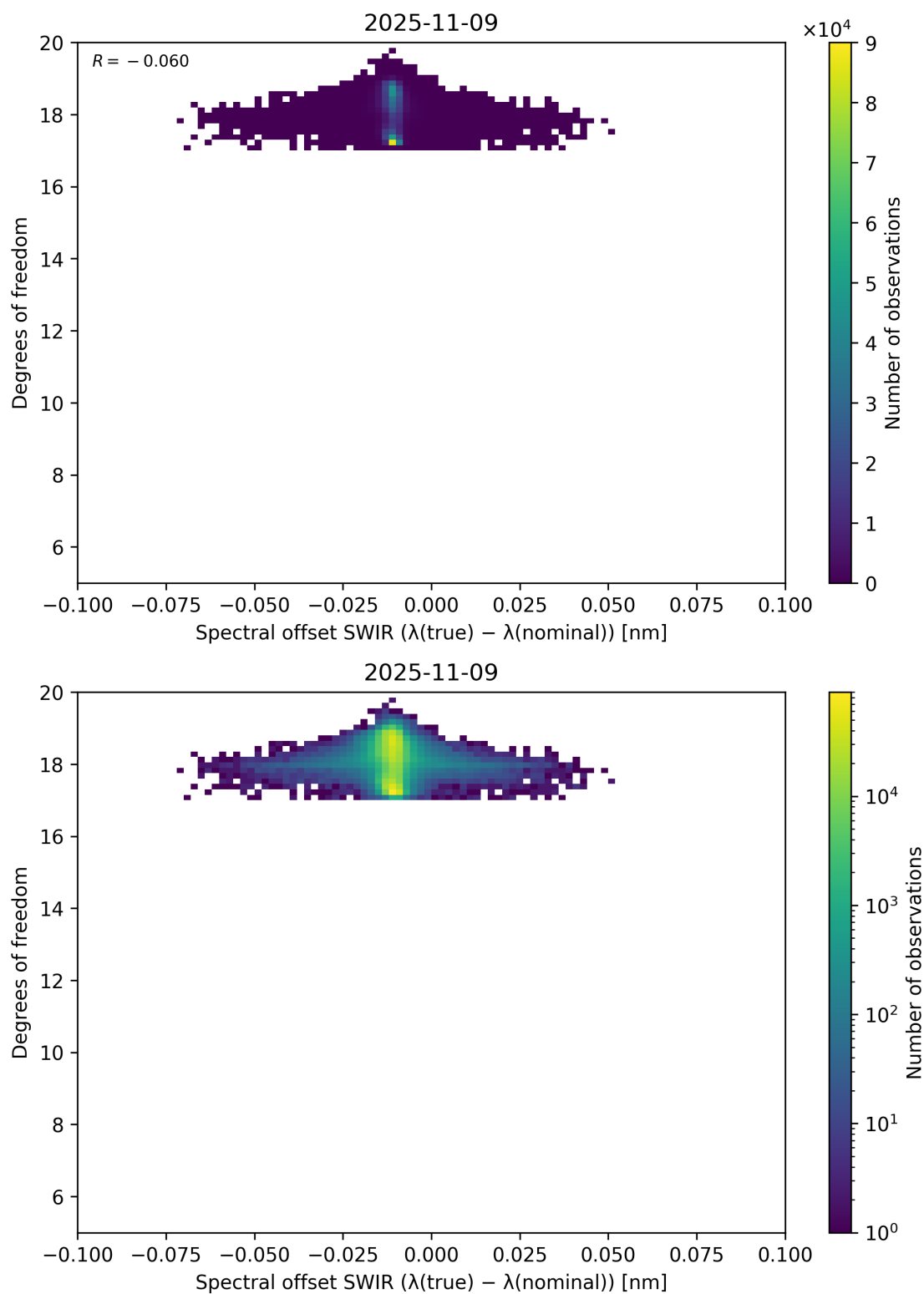
Figure 119: Scatter density plot of “Spectral offset SWIR ( \lambda_{\text{true}} - \lambda_{\text{nominal}} )” against “Degrees of freedom” for 2025-11-08 to 2025-11-10.
