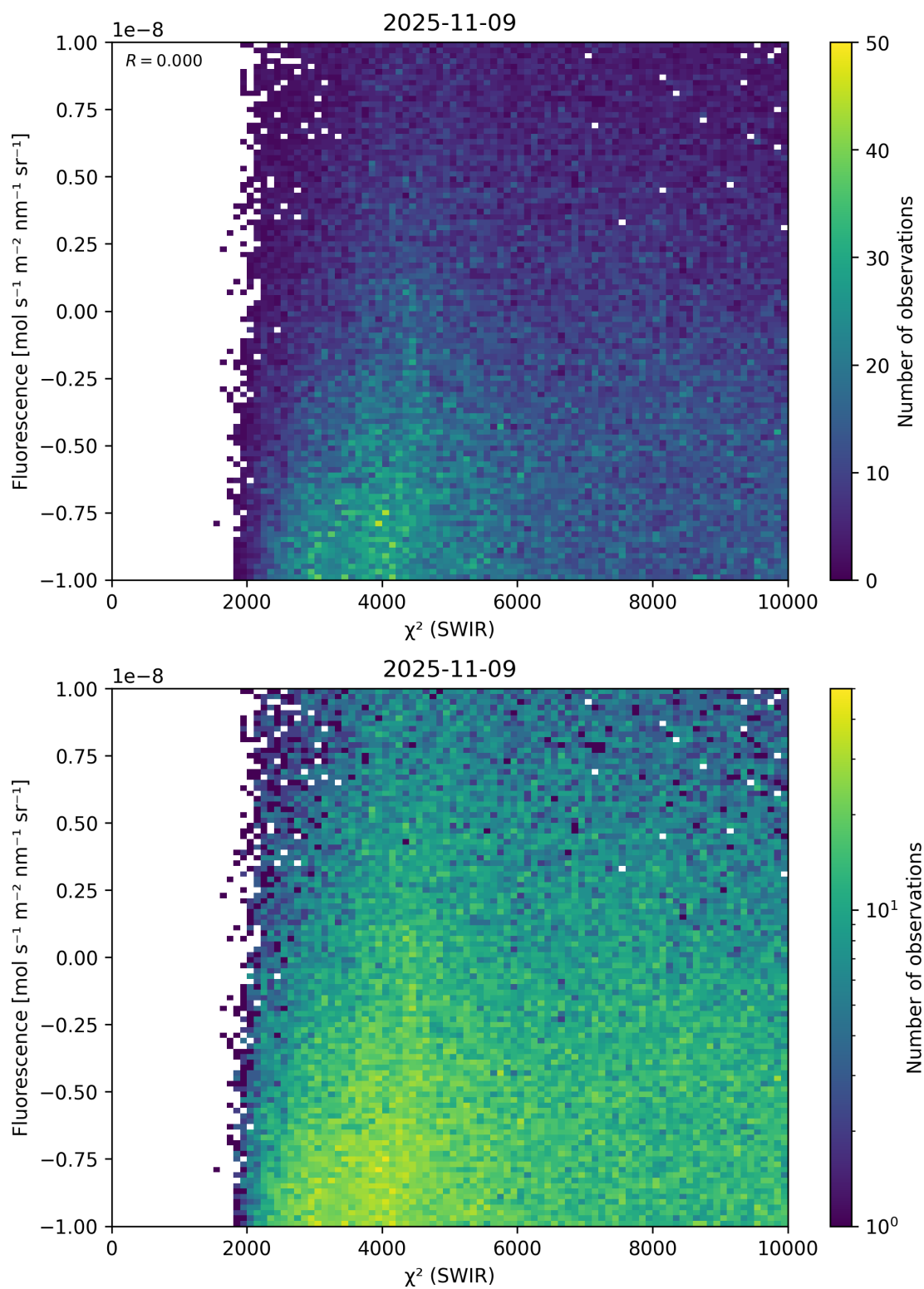
Figure 49: Scatter density plot of “ \chi^2 (SWIR)” against “Fluorescence” for 2025-11-08 to 2025-11-10.
