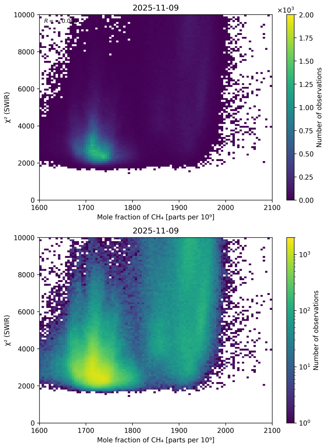
Figure 71: Scatter density plot of “Mole fraction of CH 4 ” against “ \chi^2 (SWIR)” for 2025-11-08 to 2025-11-10.
