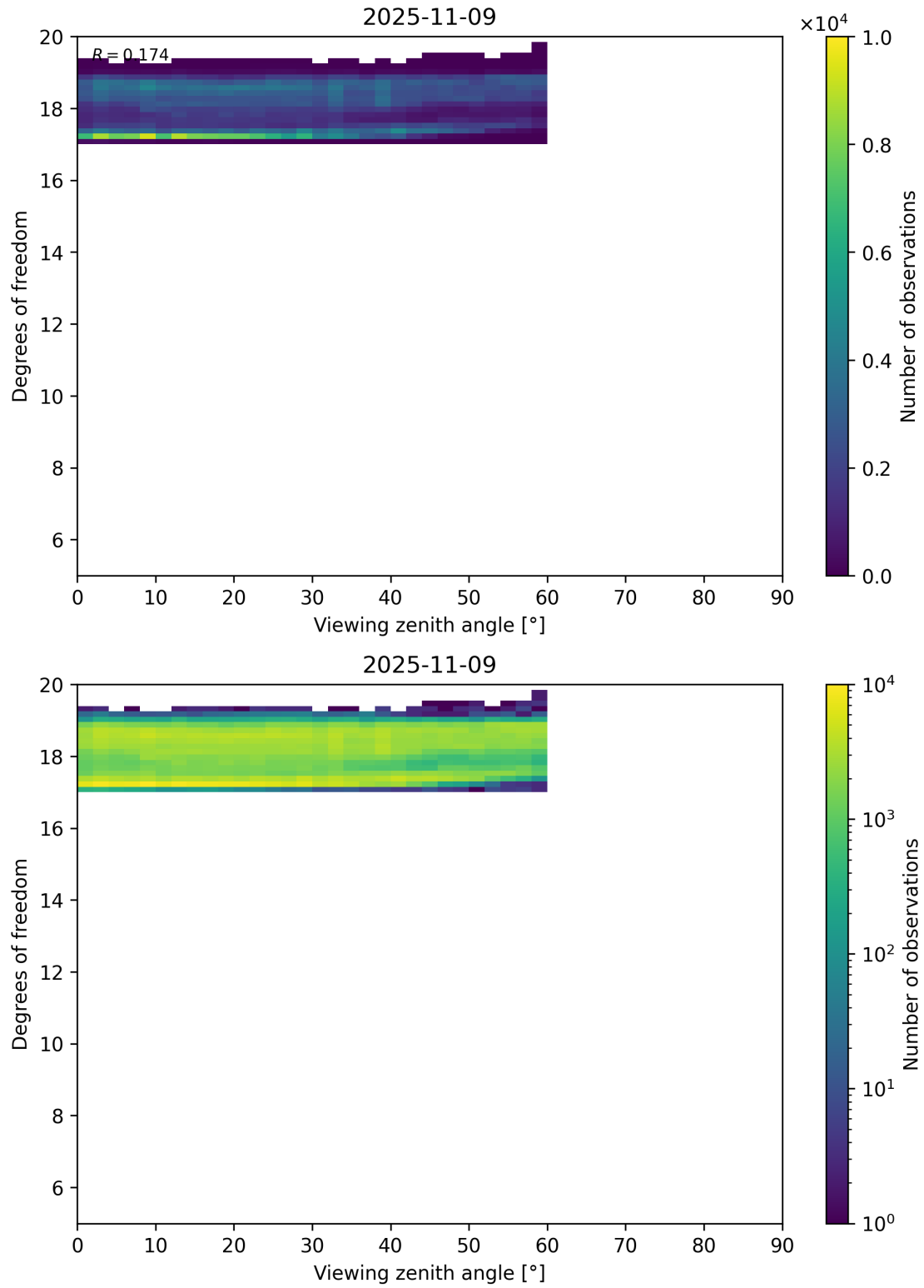
Figure 107: Scatter density plot of “Viewing zenith angle” against “Degrees of freedom” for 2025-11-08 to 2025-11-10.
