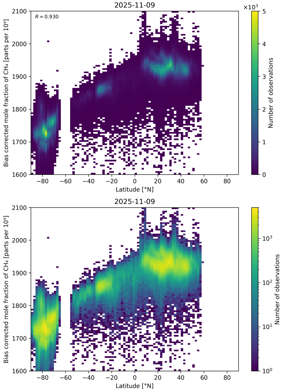
Figure 58: Scatter density plot of “Latitude” against “Bias corrected mole fraction of \text{CH}_4 ” for 2025-11-08 to 2025-11-10.
