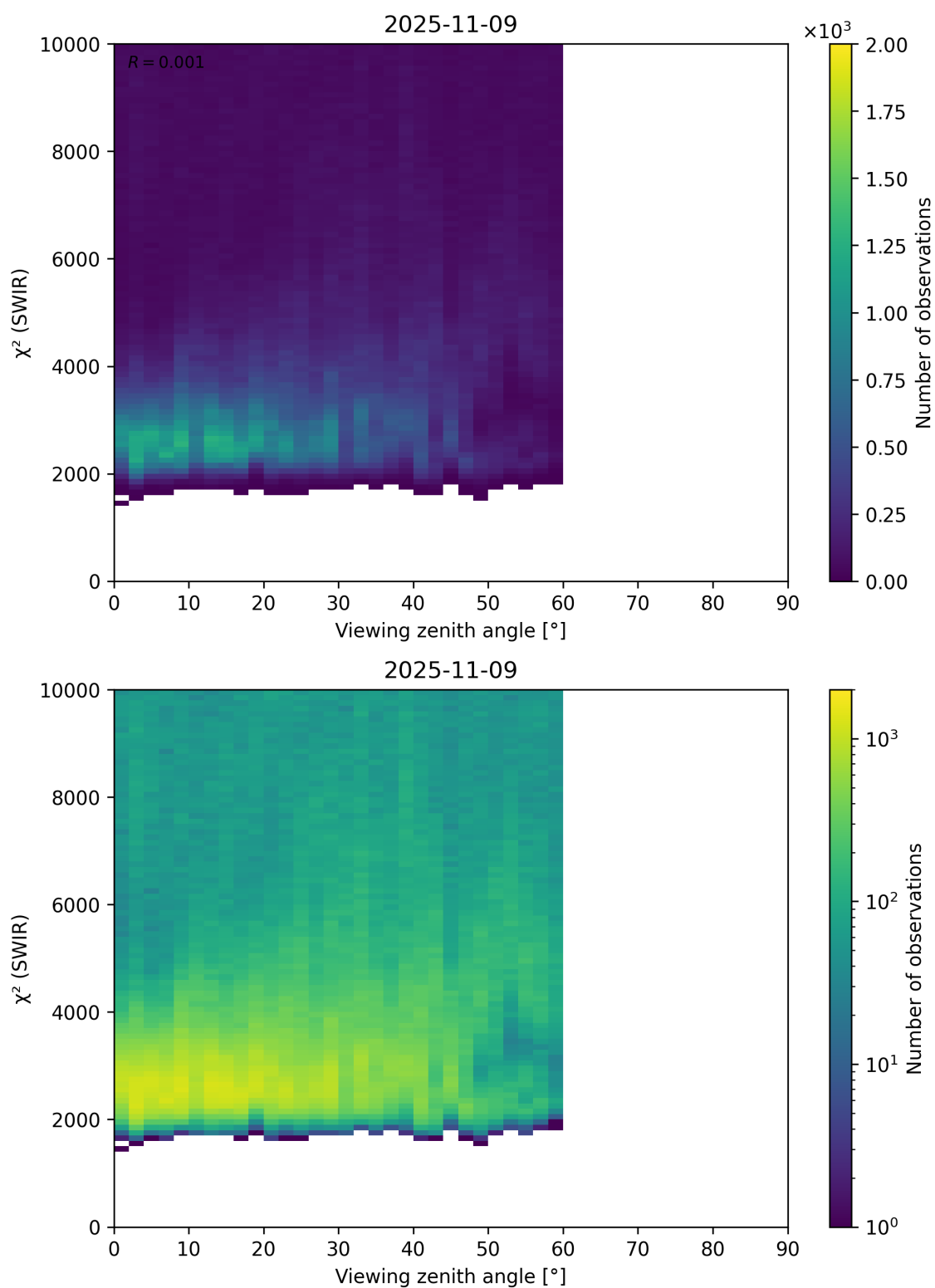
Figure 106: Scatter density plot of “Viewing zenith angle” against “ \chi^2 (SWIR)” for 2025-11-08 to 2025-11-10.
