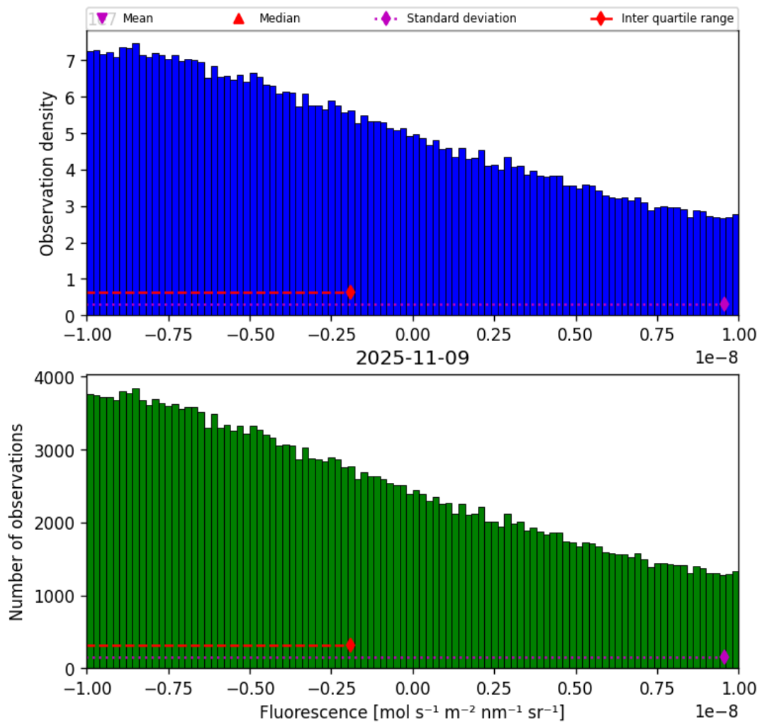
Figure 32: Histogram of “Fluorescence” for 2025-11-08 to 2025-11-10
