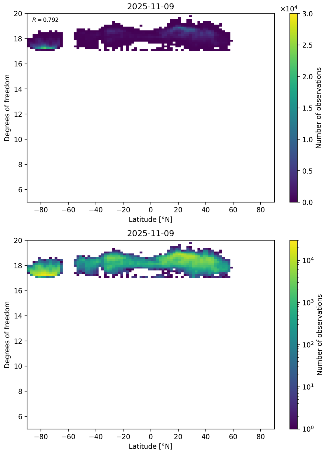
Figure 55: Scatter density plot of “Latitude” against “Degrees of freedom” for 2025-11-08 to 2025-11-10.
