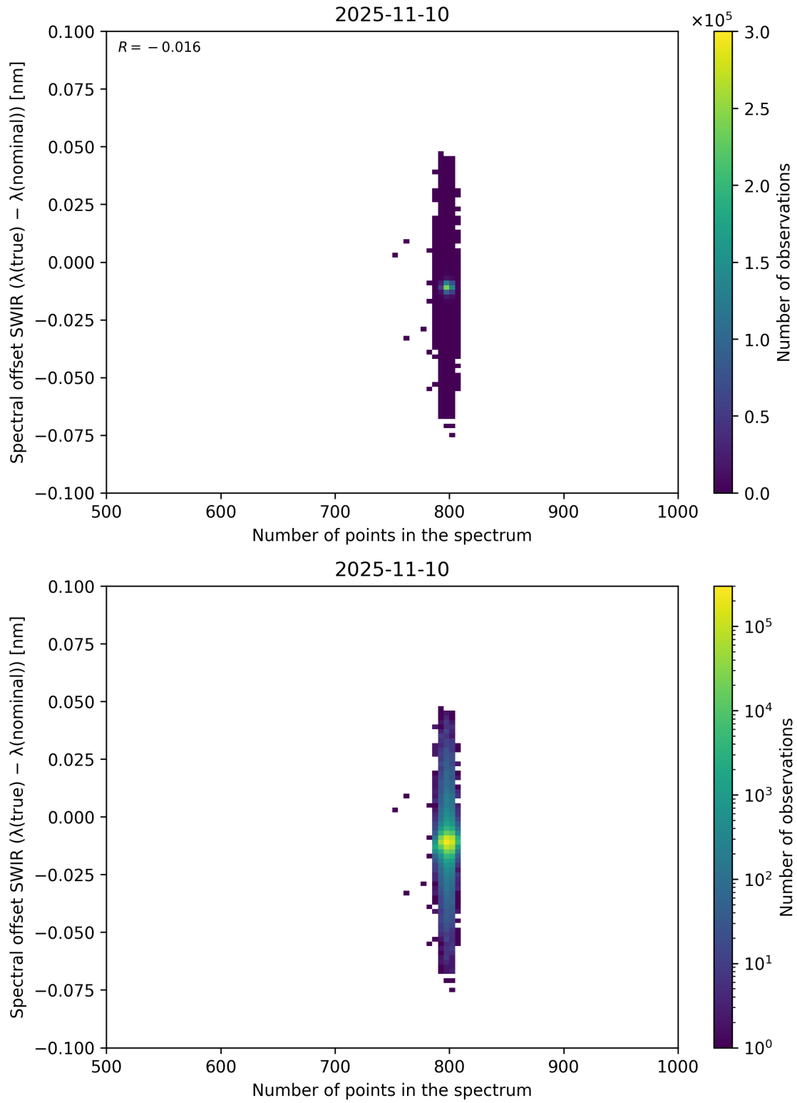
Figure 93: Scatter density plot of “Number of points in the spectrum” against “Spectral offset SWIR ( \lambda_{\text{true}} - \lambda_{\text{nominal}} )” for 2025-11-09 to 2025-11-11.
