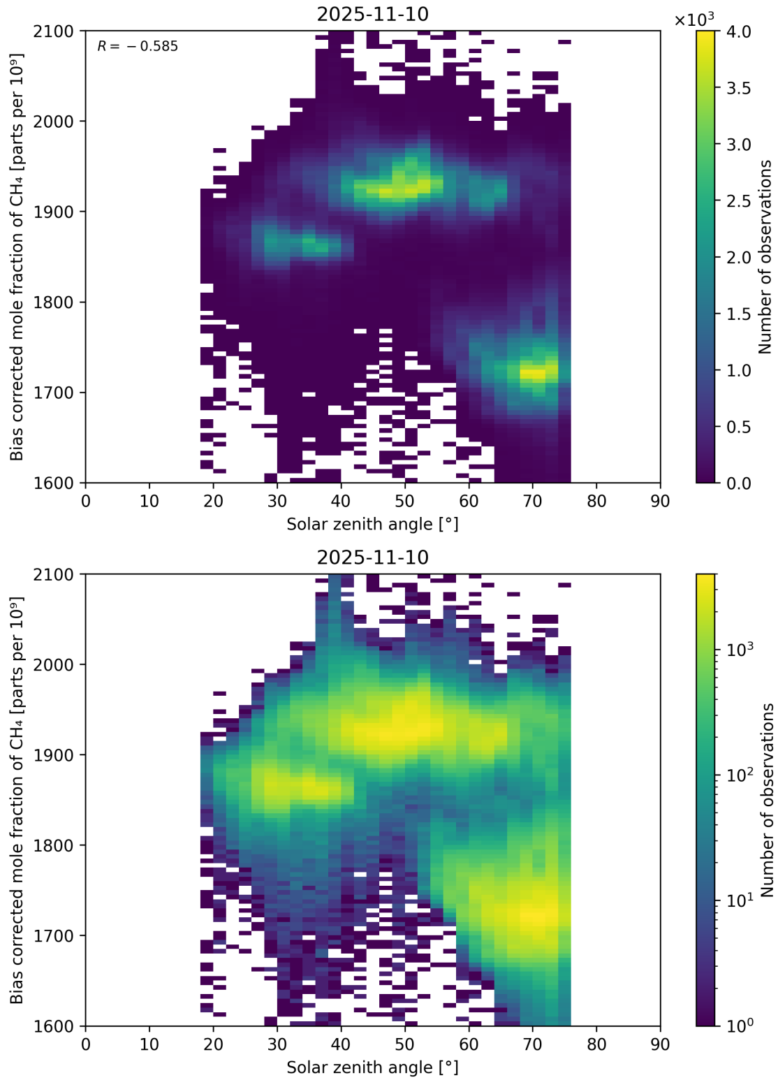
Figure 100: Scatter density plot of “Solar zenith angle” against “Bias corrected mole fraction of \text{CH}_4 ” for 2025-11-09 to 2025-11-11.
