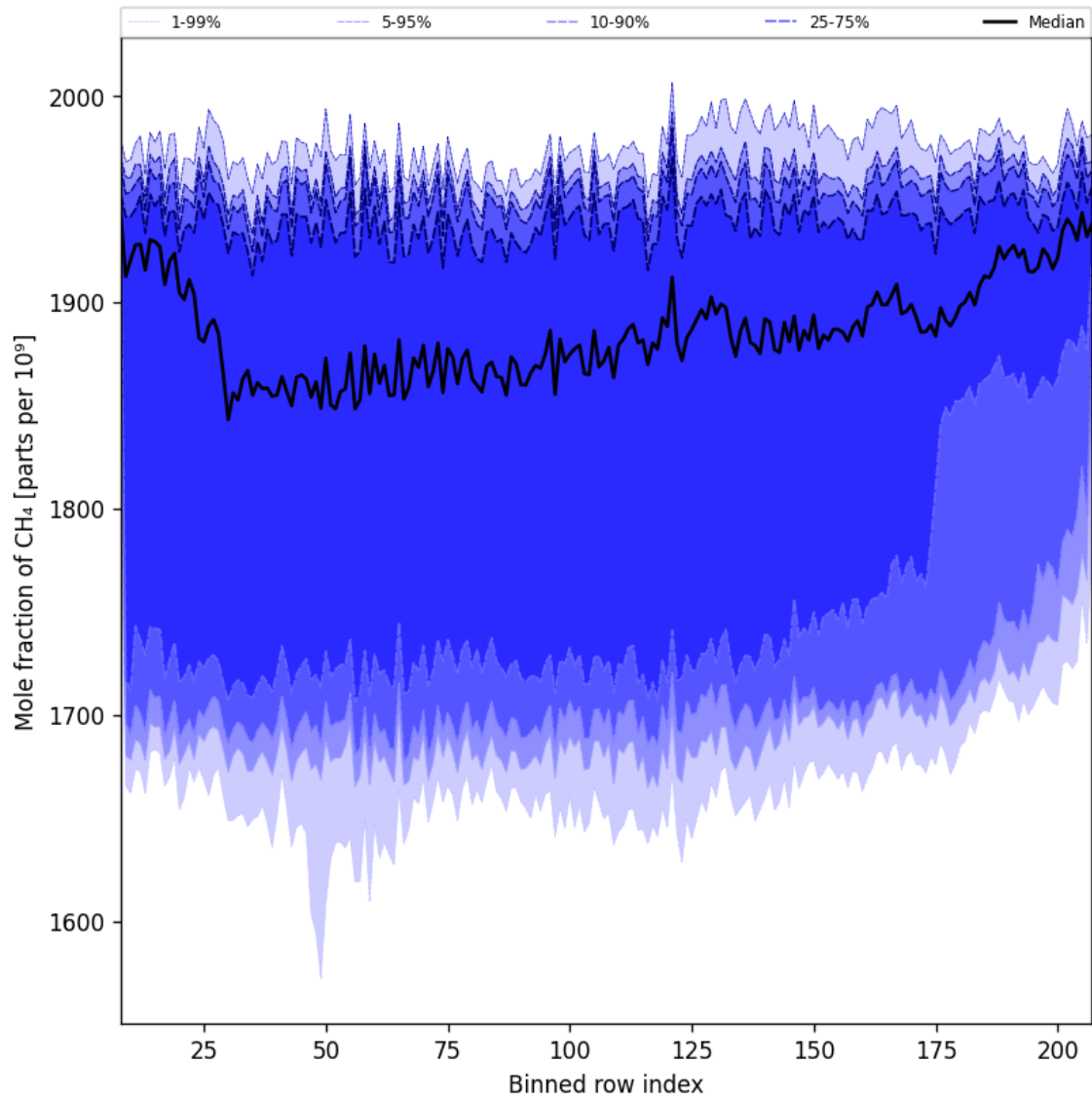
Figure 34: Along track statistics of “Mole fraction of CH 4 ” for 2025-11-09 to 2025-11-11
