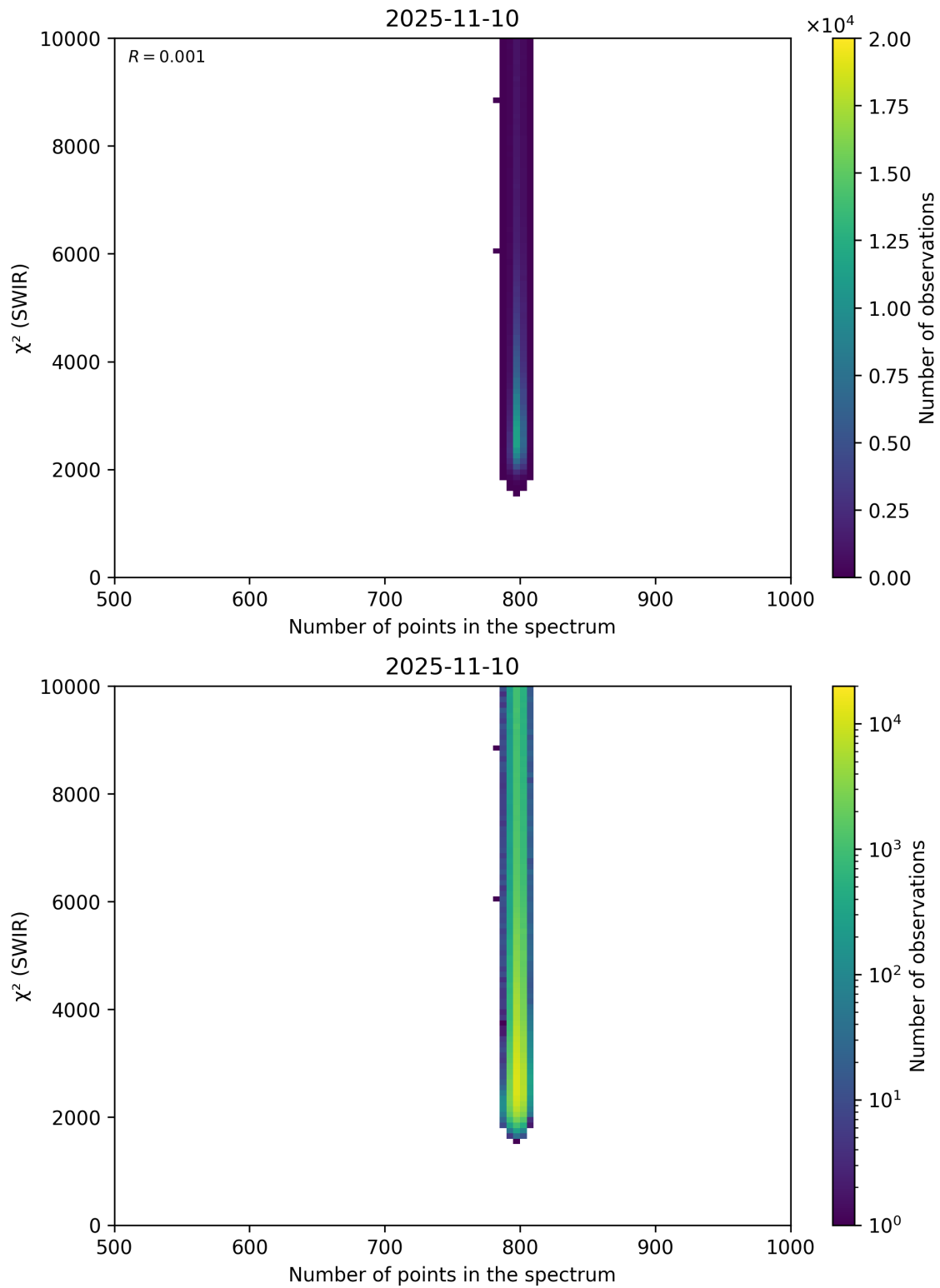
Figure 89: Scatter density plot of “Number of points in the spectrum” against “ \chi^2 (SWIR)” for 2025-11-09 to 2025-11-11.
