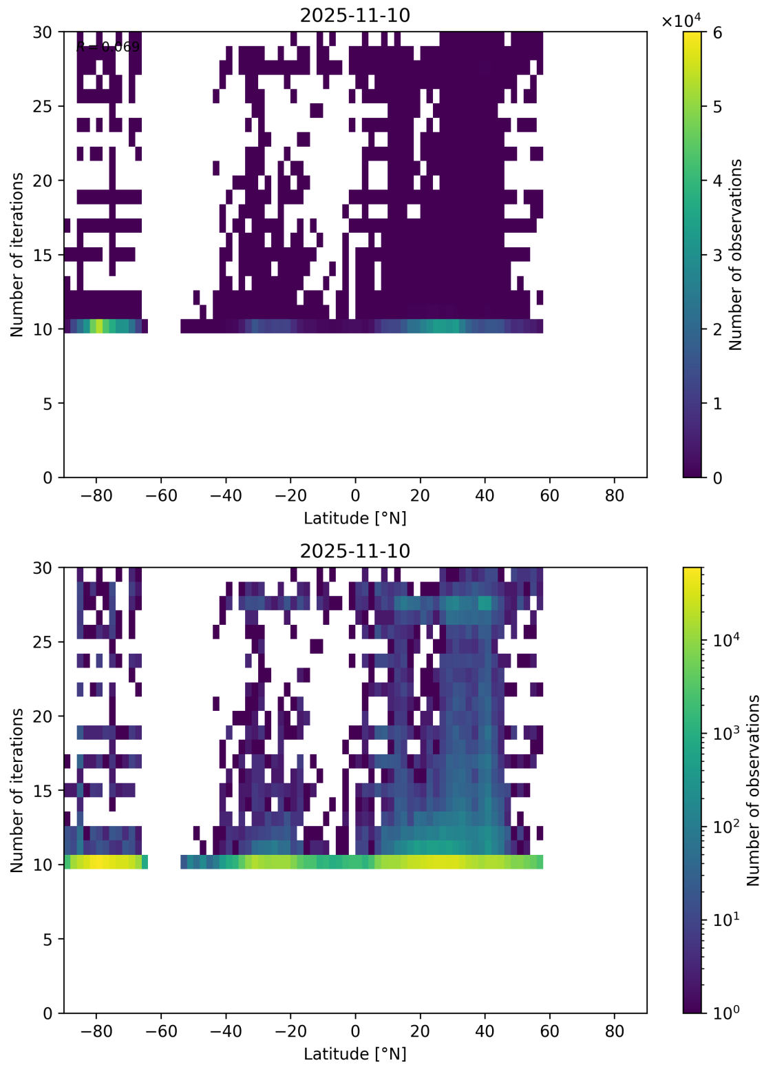
Figure 60: Scatter density plot of “Latitude” against “Number of iterations” for 2025-11-09 to 2025-11-11.
