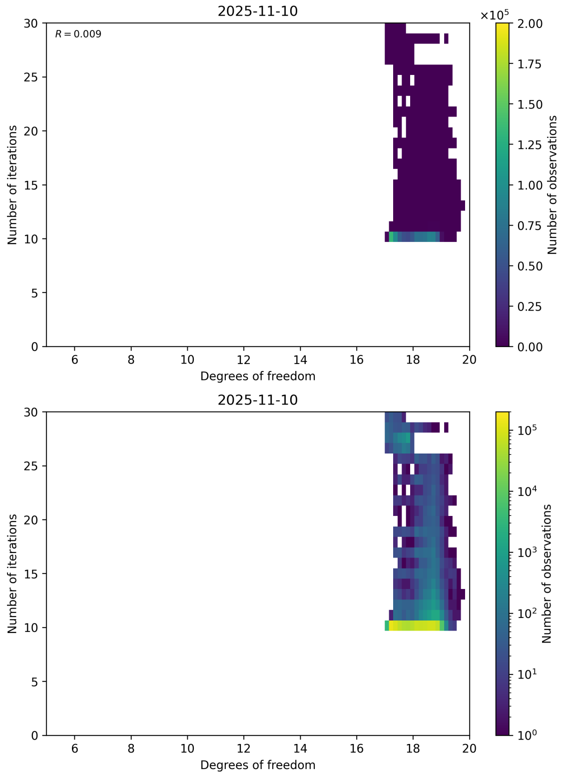
Figure 52: Scatter density plot of “Degrees of freedom” against “Number of iterations” for 2025-11-09 to 2025-11-11.
