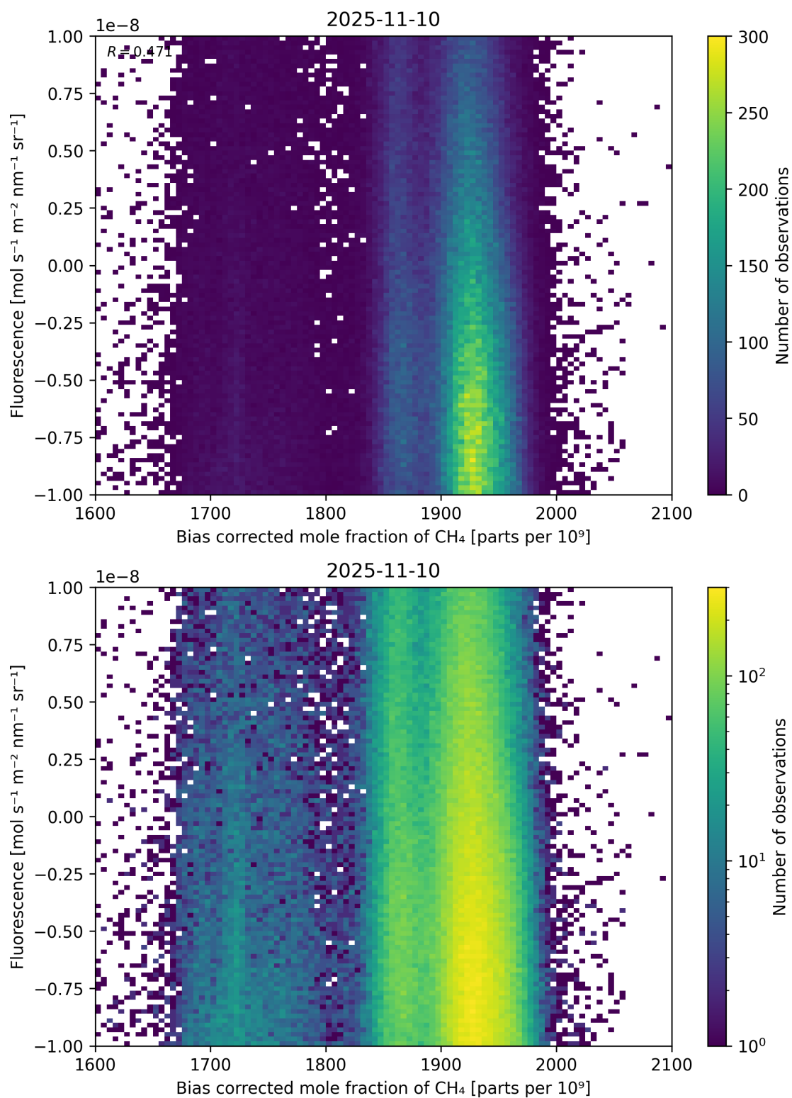
Figure 66: Scatter density plot of “Bias corrected mole fraction of CH 4 ” against “Fluorescence” for 2025-11-09 to 2025-11-11.
