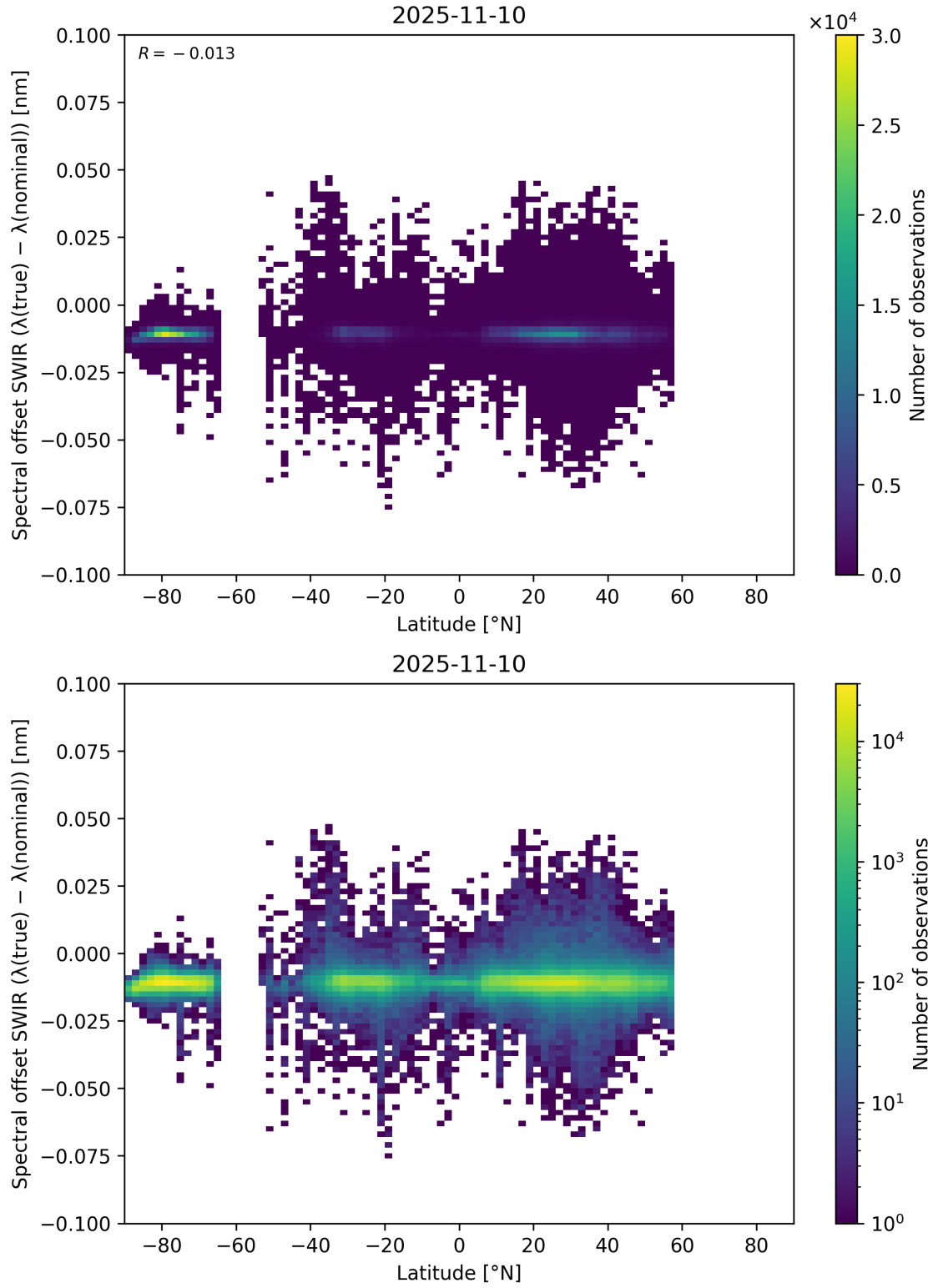
Figure 62: Scatter density plot of “Latitude” against “Spectral offset SWIR ( \lambda_{\text{true}} - \lambda_{\text{nominal}} )” for 2025-11-09 to 2025-11-11.
