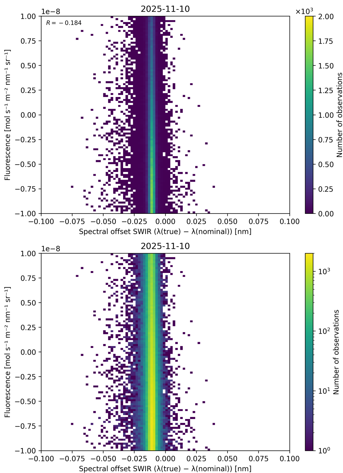
Figure 120: Scatter density plot of “Spectral offset SWIR ( \lambda_{\text{true}} - \lambda_{\text{nominal}} )” against “Fluorescence” for 2025-11-09 to 2025-11-11.
