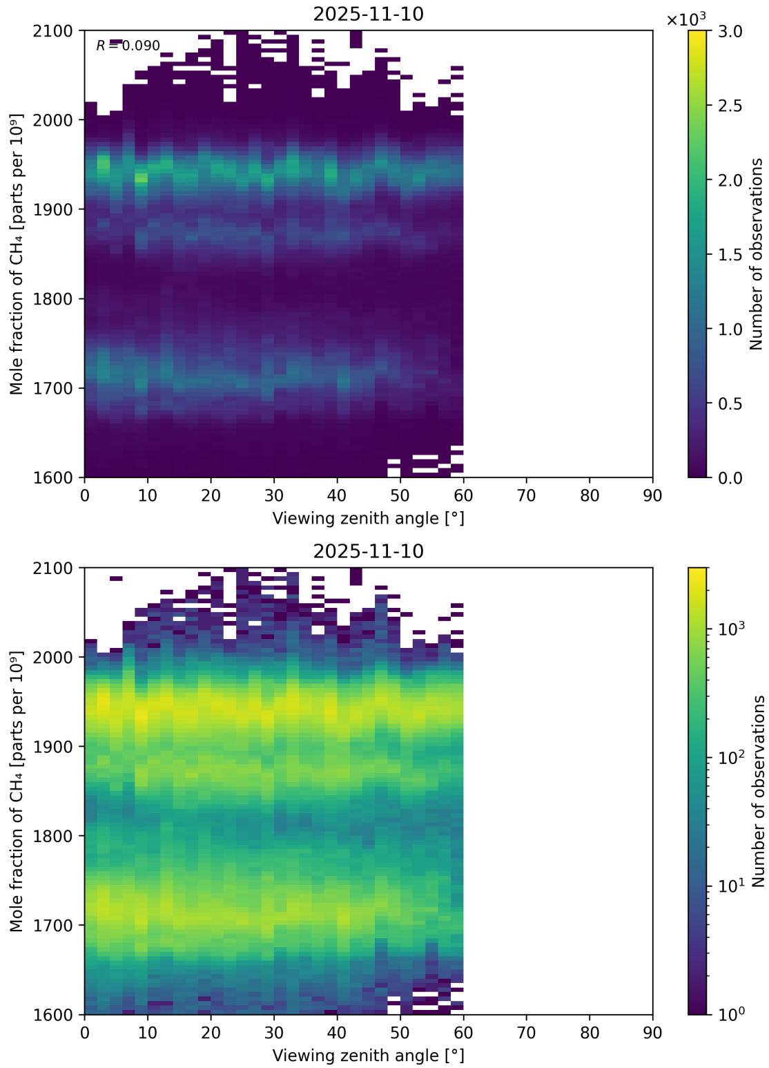
Figure 110: Scatter density plot of “Viewing zenith angle” against “Mole fraction of CH 4 ” for 2025-11-09 to 2025-11-11.
