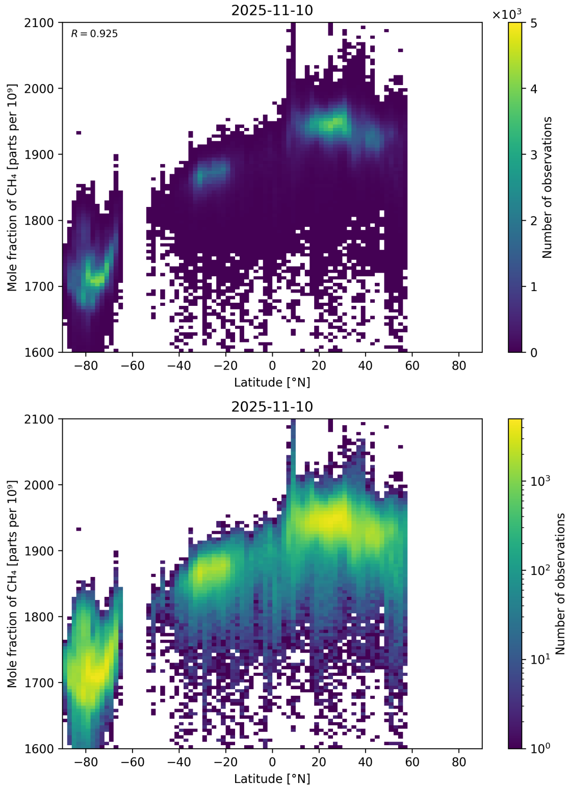
Figure 57: Scatter density plot of “Latitude” against “Mole fraction of CH 4 ” for 2025-11-09 to 2025-11-11.
