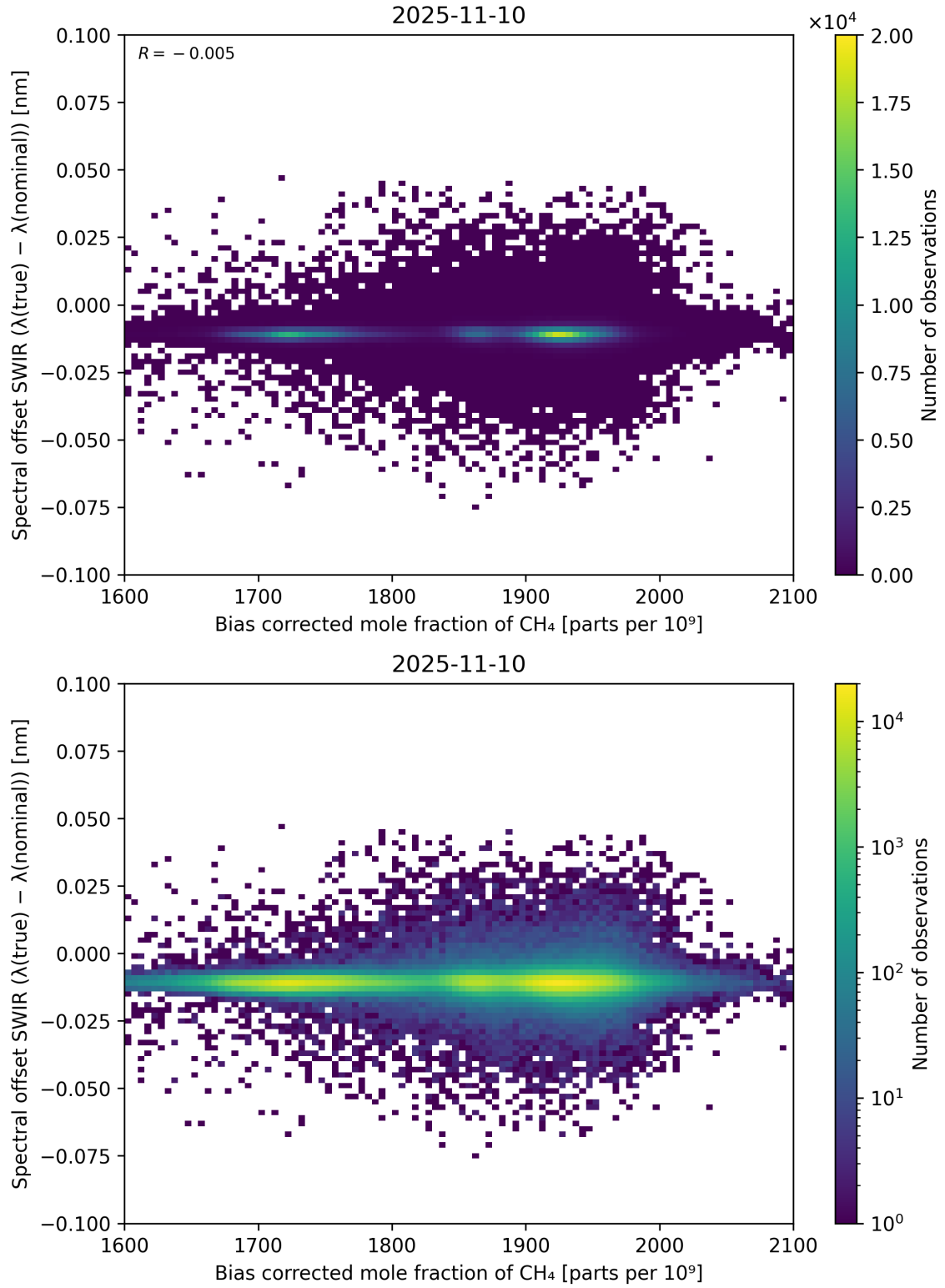
Figure 69: Scatter density plot of “Bias corrected mole fraction of \text{CH}_4 ” against “Spectral offset SWIR ( \lambda_{\text{true}} - \lambda_{\text{nominal}} )” for 2025-11-09 to 2025-11-11.
