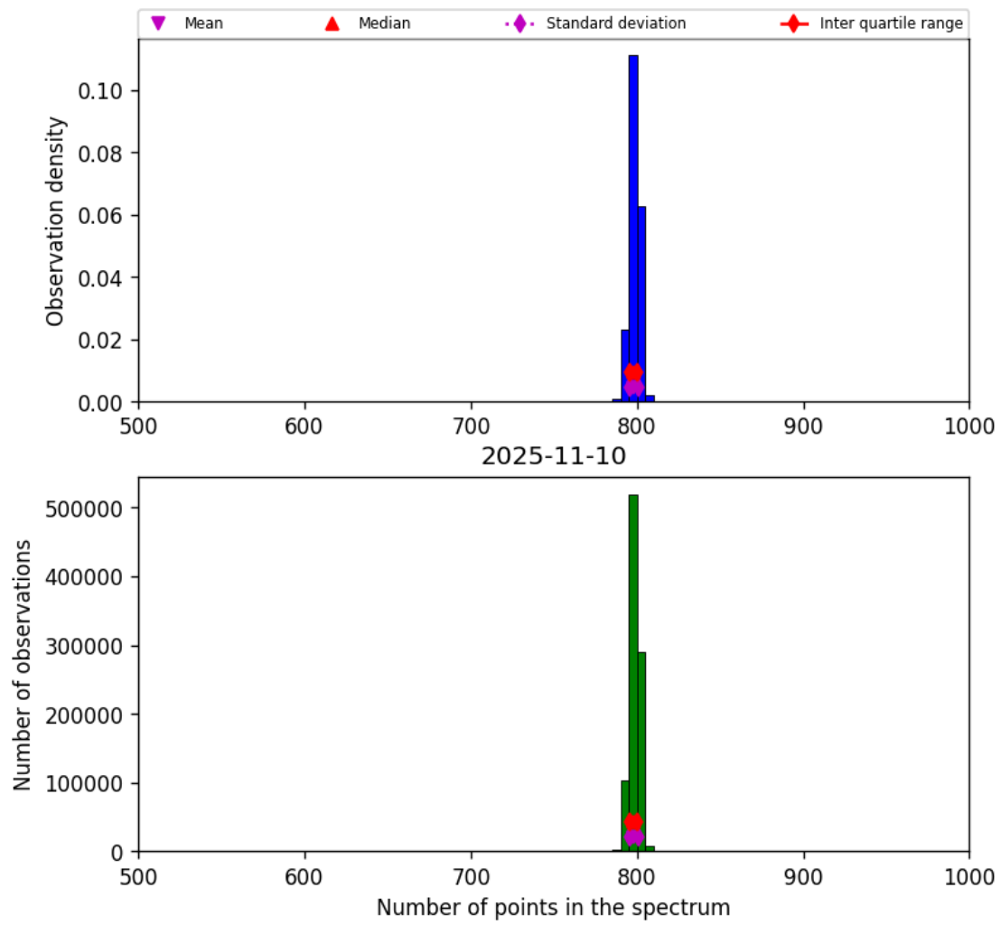
Figure 26: Histogram of “Number of points in the spectrum” for 2025-11-09 to 2025-11-11
