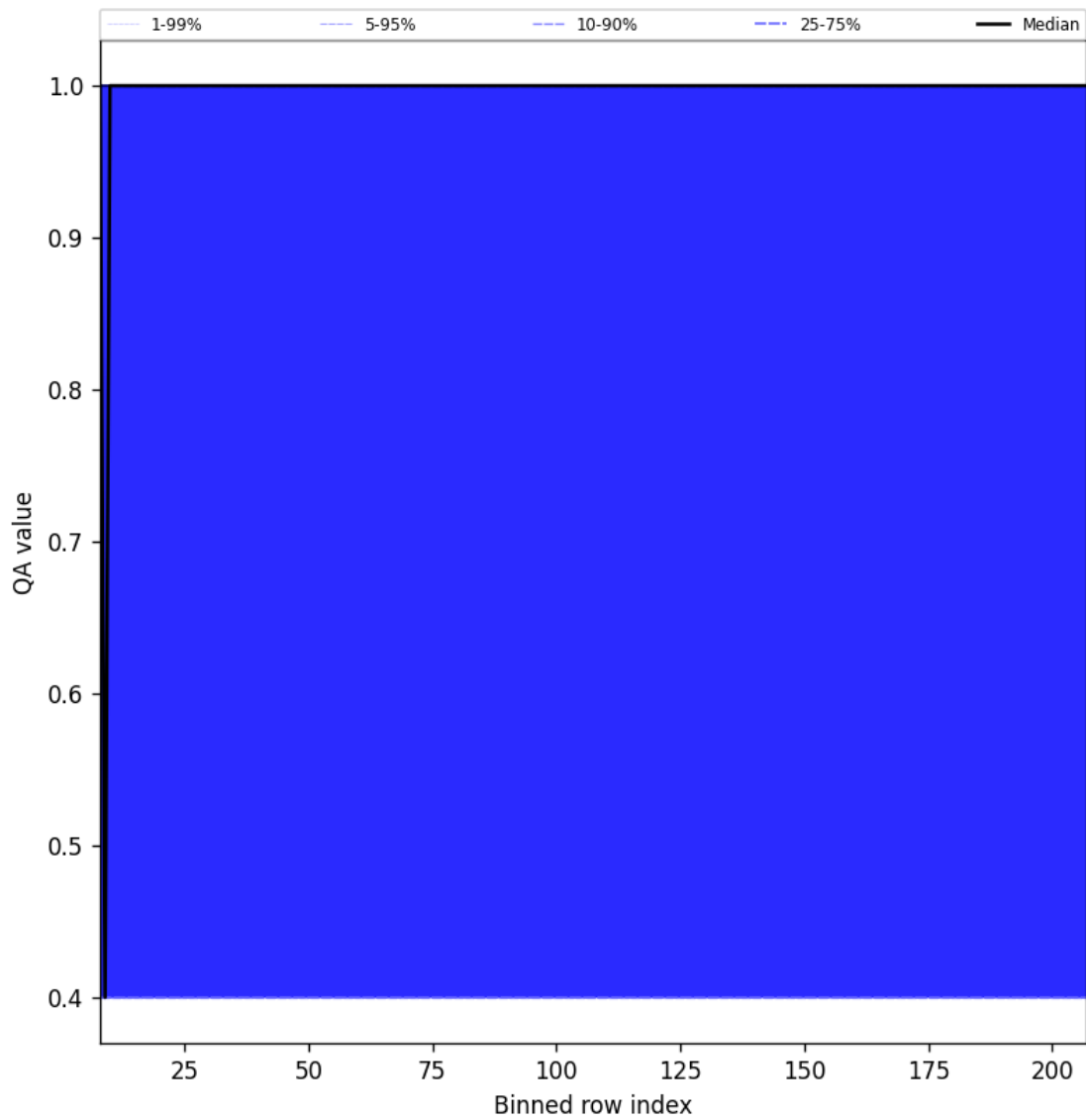
Figure 33: Along track statistics of “QA value” for 2025-11-09 to 2025-11-11
