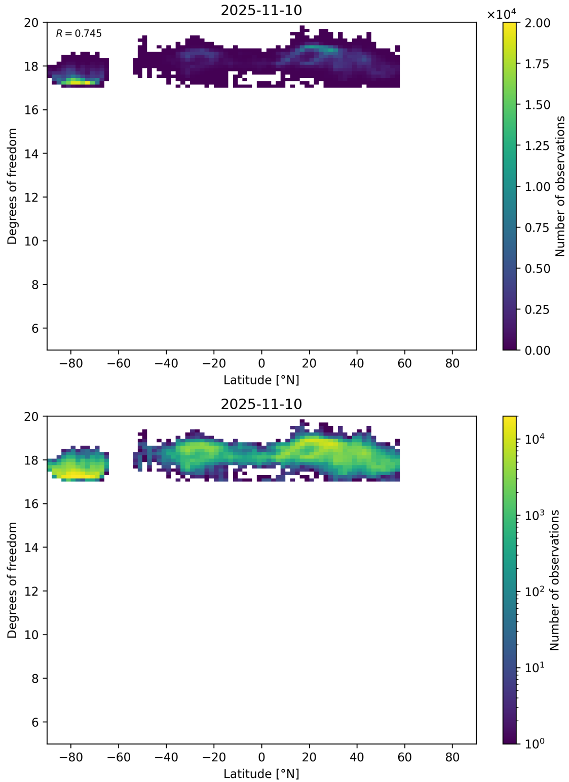
Figure 55: Scatter density plot of “Latitude” against “Degrees of freedom” for 2025-11-09 to 2025-11-11.
