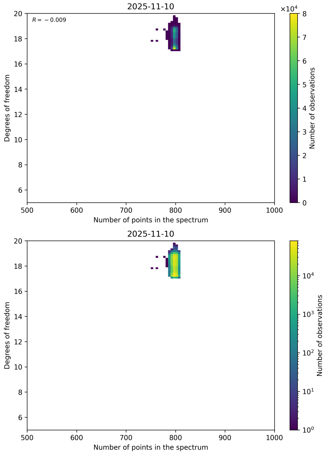
Figure 90: Scatter density plot of “Number of points in the spectrum” against “Degrees of freedom” for 2025-11-09 to 2025-11-11.
