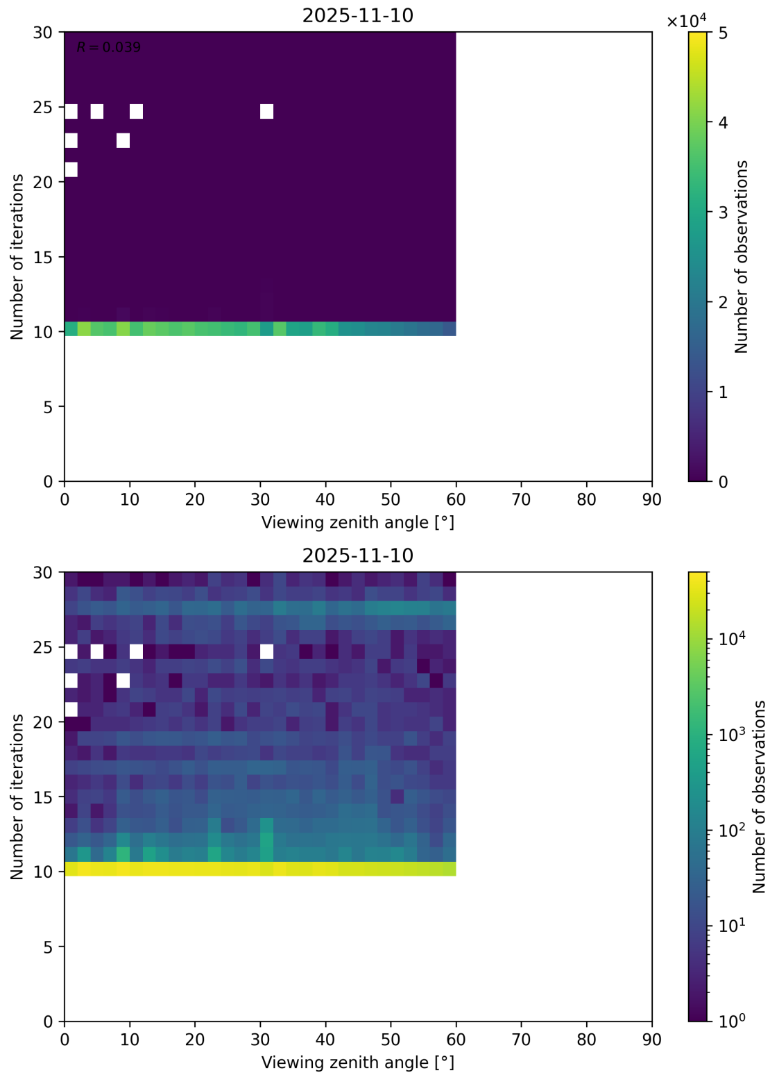
Figure 113: Scatter density plot of “Viewing zenith angle” against “Number of iterations” for 2025-11-09 to 2025-11-11.
