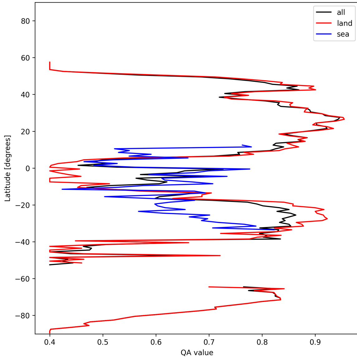
Figure 11: Zonal average of “QA value” for 2025-11-09 to 2025-11-11.
