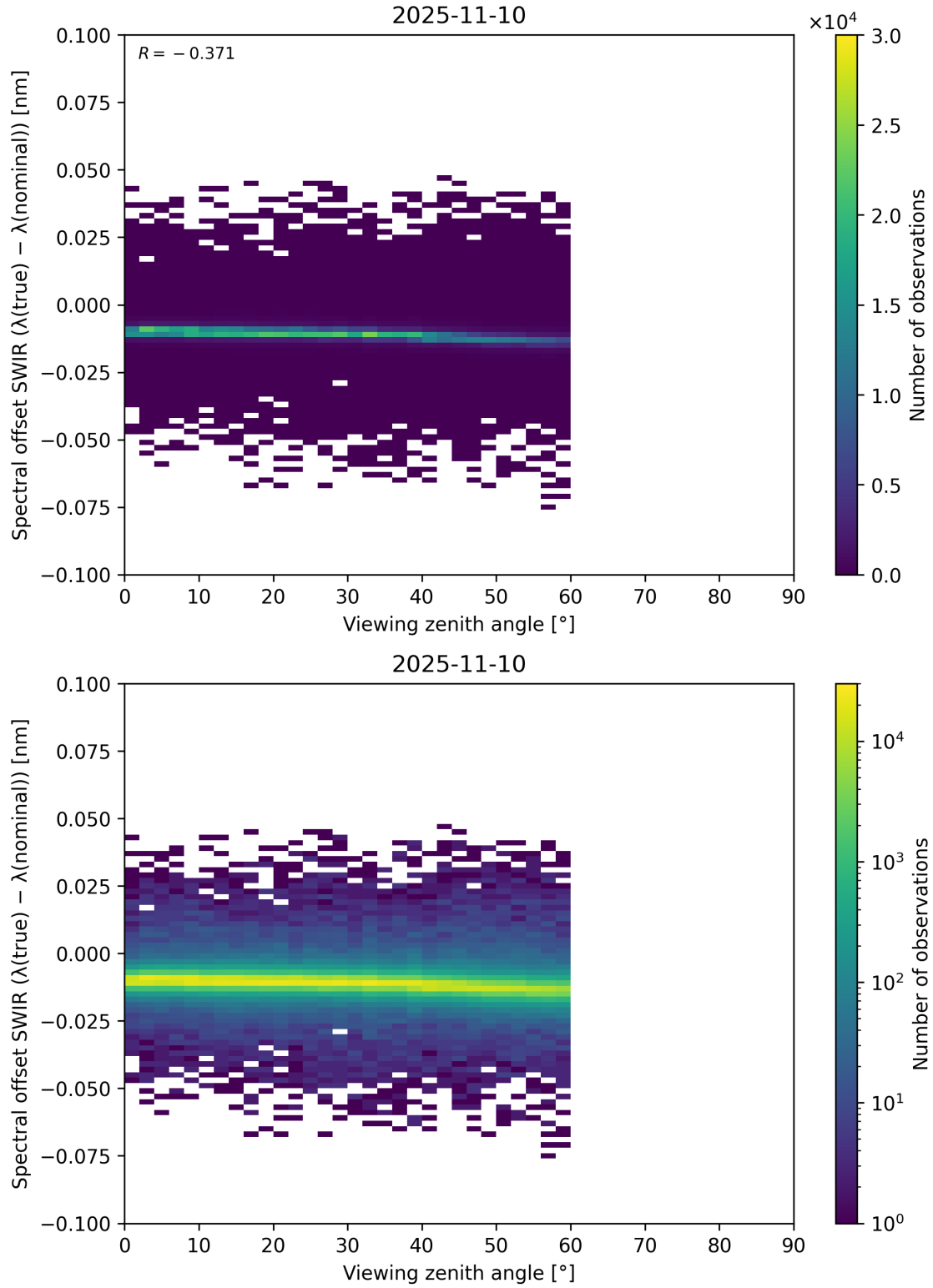
Figure 116: Scatter density plot of “Viewing zenith angle” against “Spectral offset SWIR ( \lambda_{\text{true}} - \lambda_{\text{nominal}} )” for 2025-11-09 to 2025-11-11.
