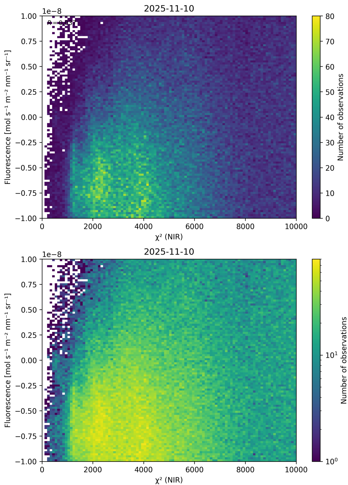
Figure 45: Scatter density plot of “ \chi^2 (NIR)” against “Fluorescence” for 2025-11-09 to 2025-11-11.
