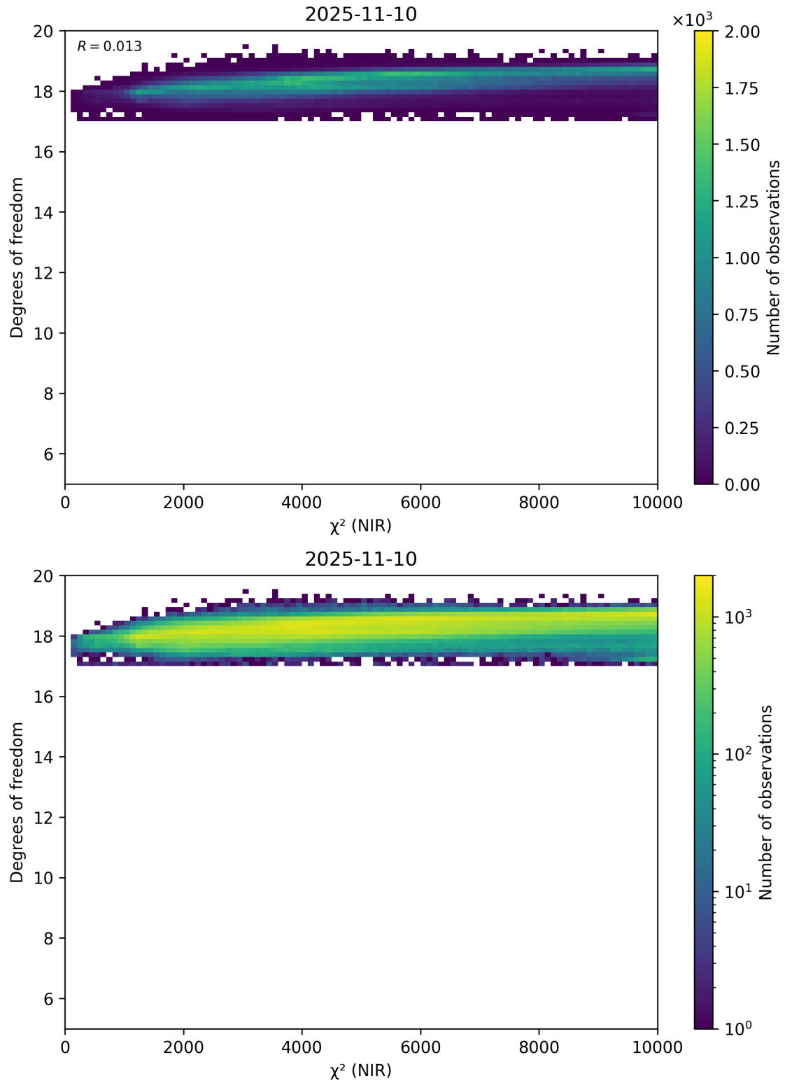
Figure 44: Scatter density plot of “ \chi^2 (NIR)” against “Degrees of freedom” for 2025-11-09 to 2025-11-11.
