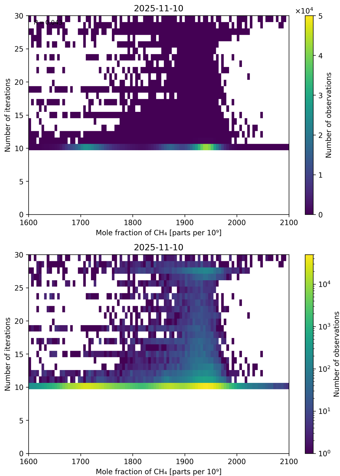
Figure 76: Scatter density plot of “Mole fraction of CH 4 ” against “Number of iterations” for 2025-11-09 to 2025-11-11.
