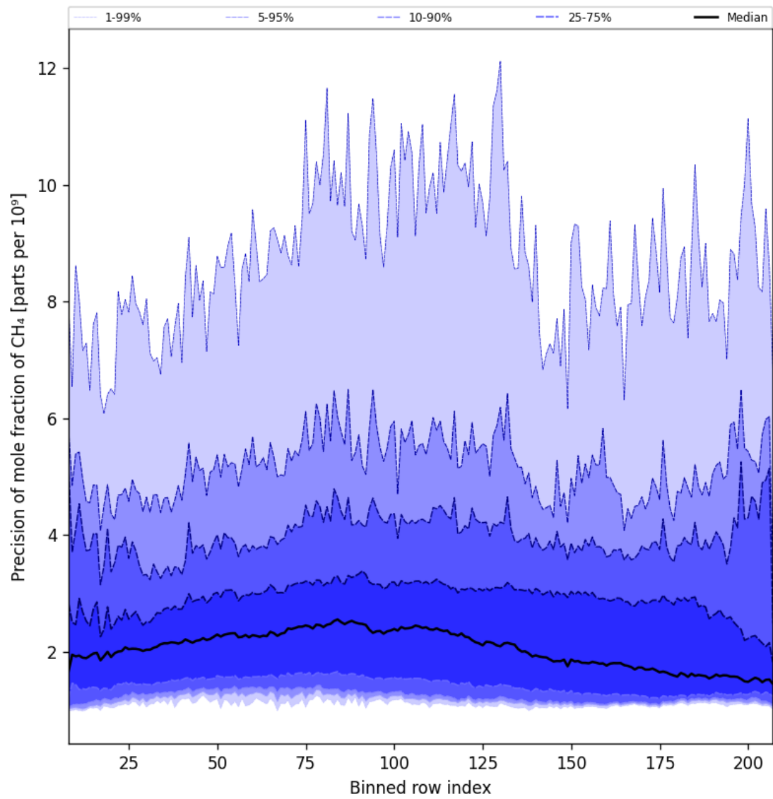
Figure 35: Along track statistics of “Precision of mole fraction of CH 4 ” for 2025-11-09 to 2025-11-11
