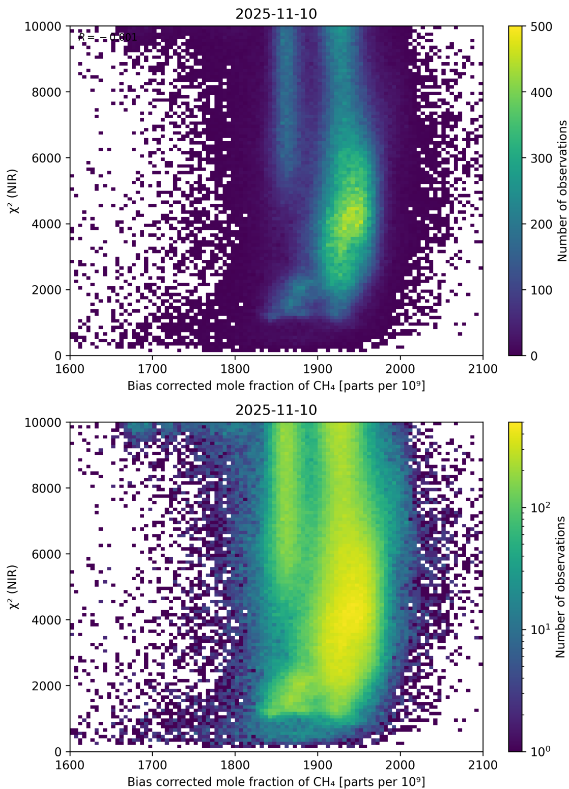
Figure 63: Scatter density plot of “Bias corrected mole fraction of \text{CH}_4 ” against “ \chi^2 (NIR)” for 2025-11-09 to 2025-11-11.
