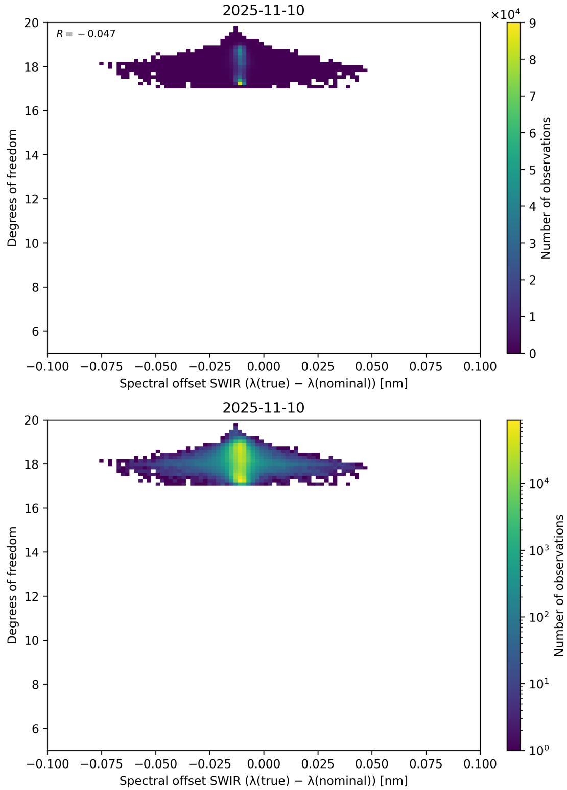
Figure 119: Scatter density plot of “Spectral offset SWIR ( \lambda_{\text{true}} - \lambda_{\text{nominal}} )” against “Degrees of freedom” for 2025-11-09 to 2025-11-11.
