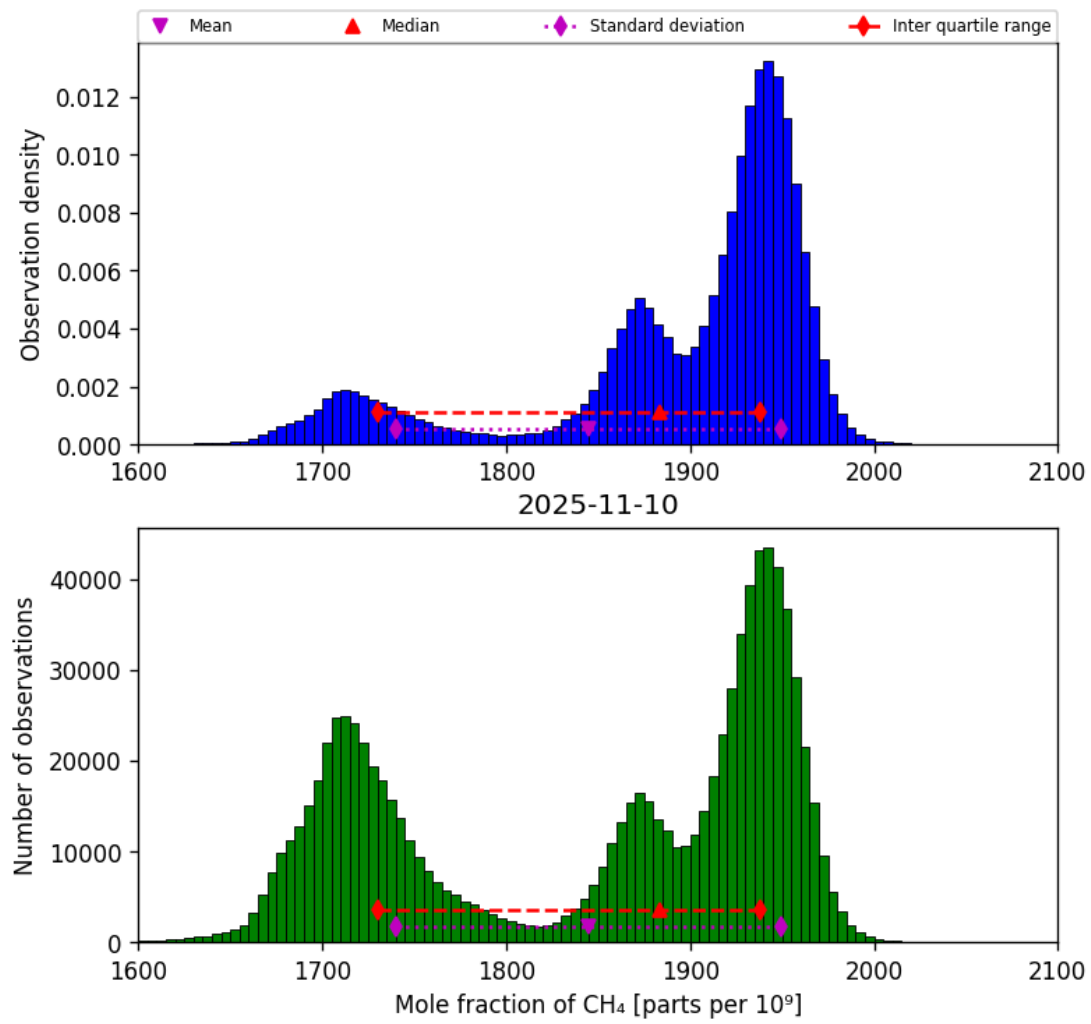
Figure 23: Histogram of “Mole fraction of CH 4 ” for 2025-11-09 to 2025-11-11
