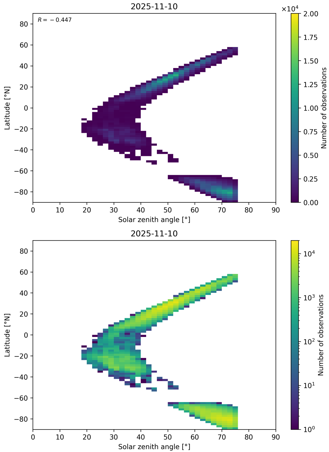
Figure 98: Scatter density plot of “Solar zenith angle” against “Latitude” for 2025-11-09 to 2025-11-11.
