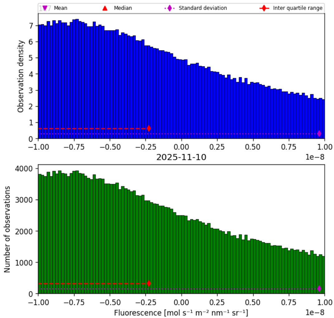
Figure 32: Histogram of “Fluorescence” for 2025-11-09 to 2025-11-11
