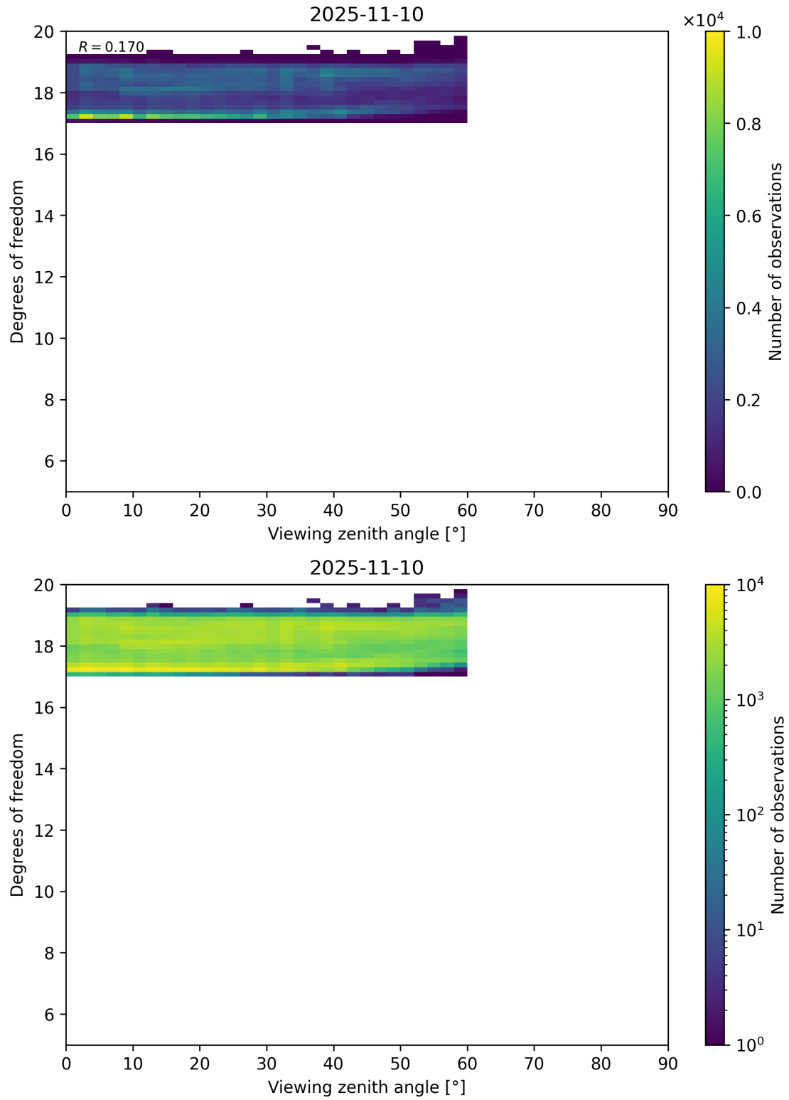
Figure 107: Scatter density plot of “Viewing zenith angle” against “Degrees of freedom” for 2025-11-09 to 2025-11-11.
