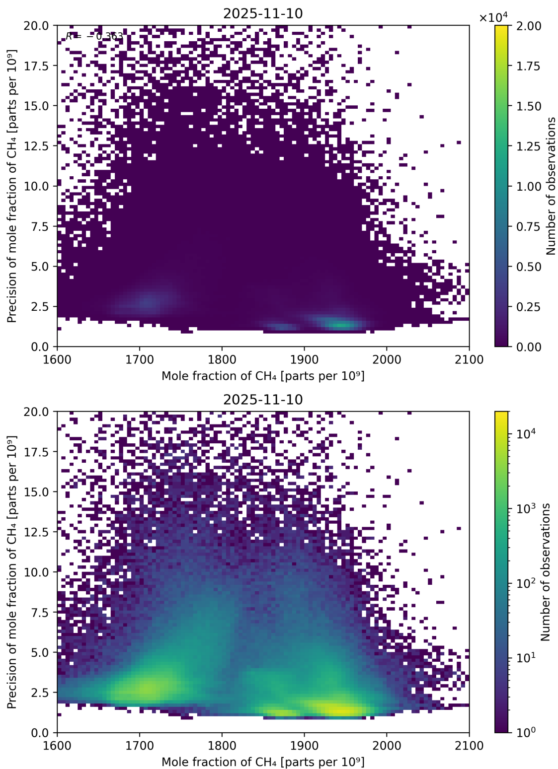
Figure 75: Scatter density plot of “Mole fraction of CH 4 ” against “Precision of mole fraction of CH 4 ” for 2025-11-09 to 2025-11-11.
