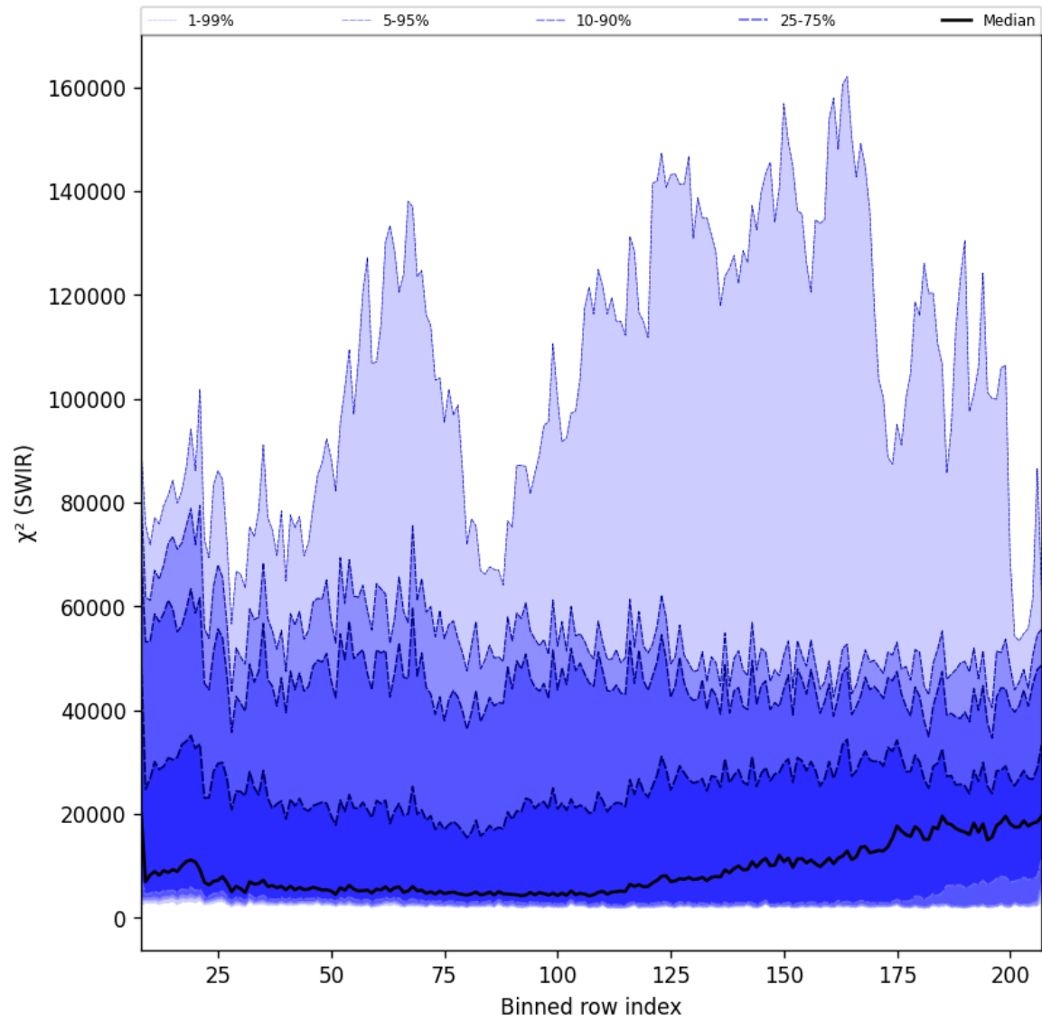
Figure 39: Along track statistics of " \chi^2 (SWIR)" for 2025-11-09 to 2025-11-11
