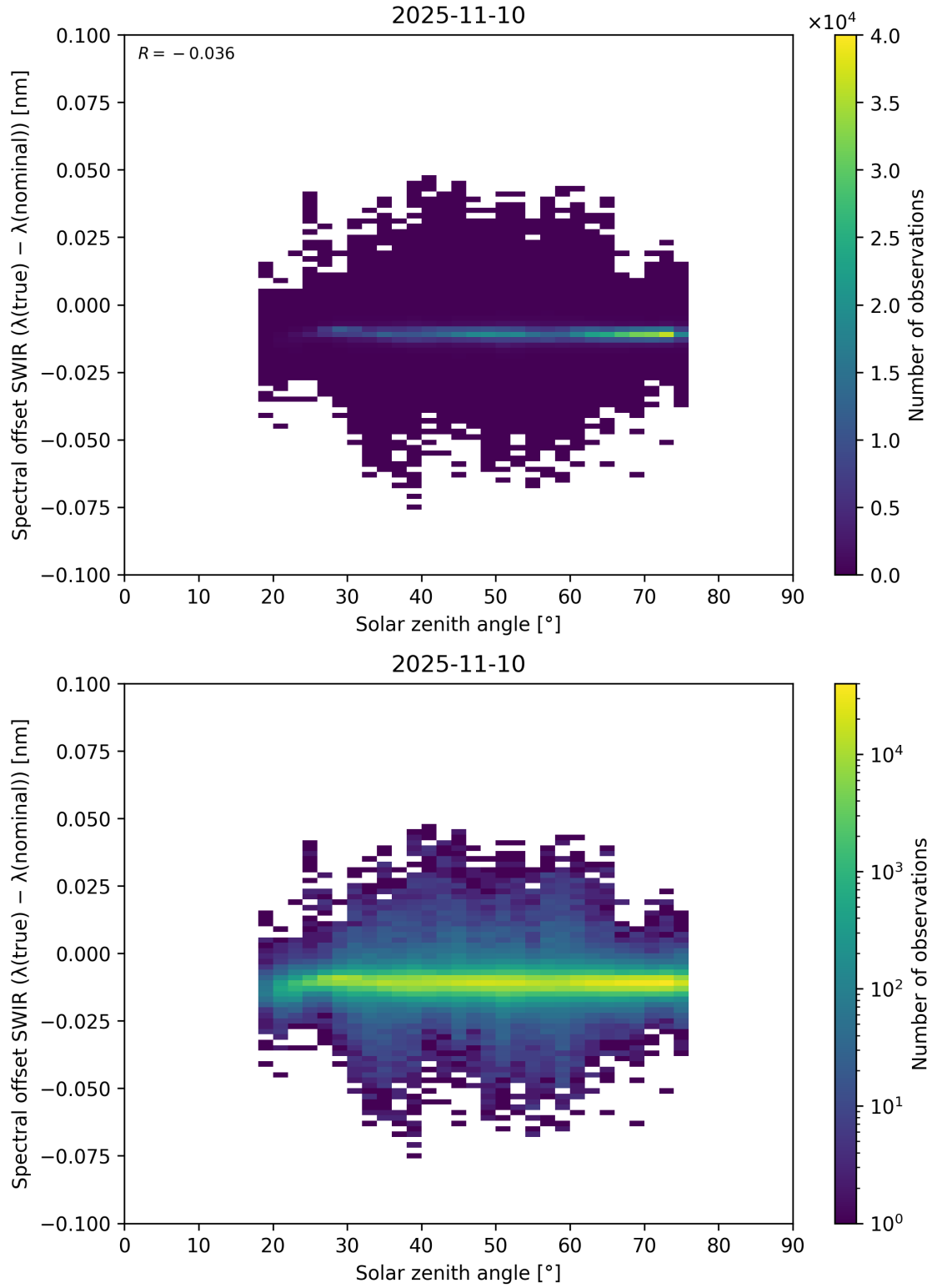
Figure 104: Scatter density plot of “Solar zenith angle” against “Spectral offset SWIR ( \lambda_{\text{true}} - \lambda_{\text{nominal}} )” for 2025-11-09 to 2025-11-11.
