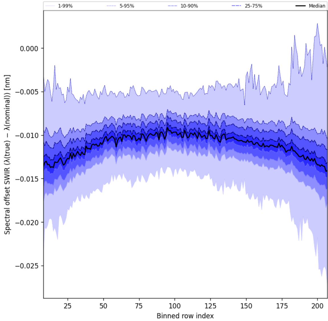
Figure 38: Along track statistics of “Spectral offset SWIR ( \lambda_{\text{true}} - \lambda_{\text{nominal}} )” for 2025-11-09 to 2025-11-11
