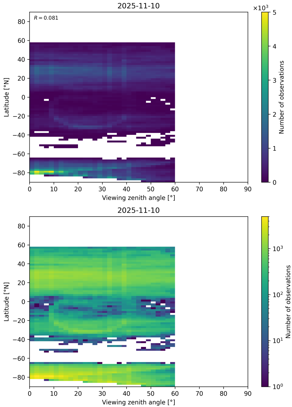
Figure 109: Scatter density plot of “Viewing zenith angle” against “Latitude” for 2025-11-09 to 2025-11-11.
