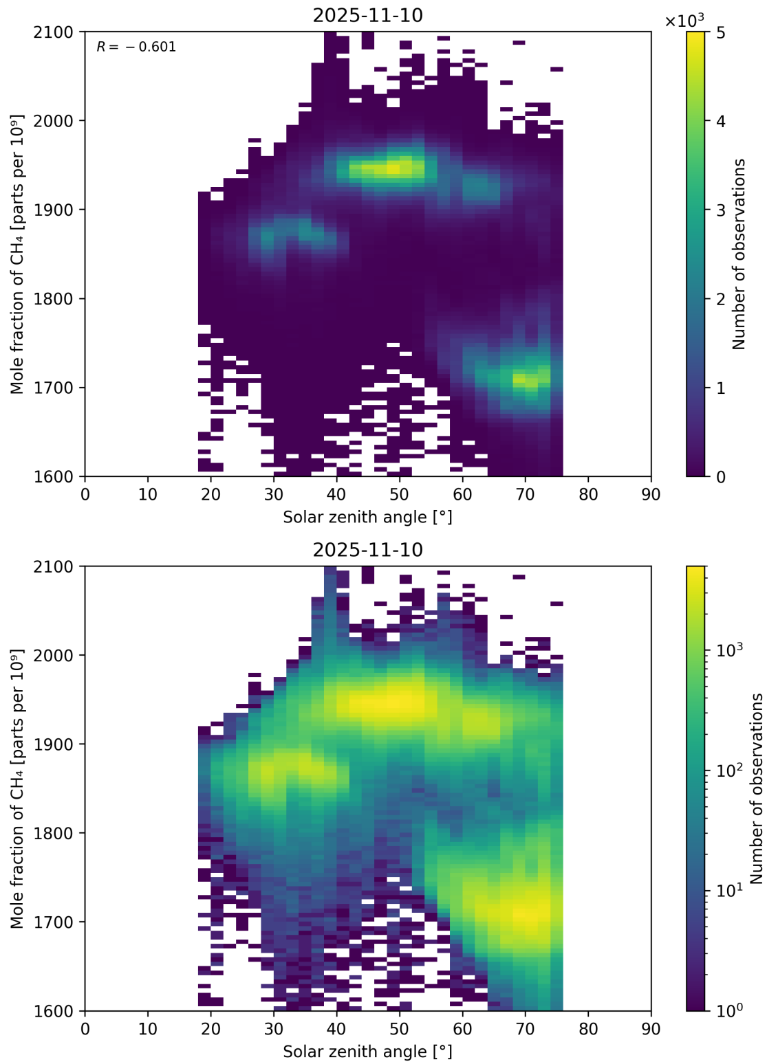
Figure 99: Scatter density plot of “Solar zenith angle” against “Mole fraction of CH 4 ” for 2025-11-09 to 2025-11-11.
