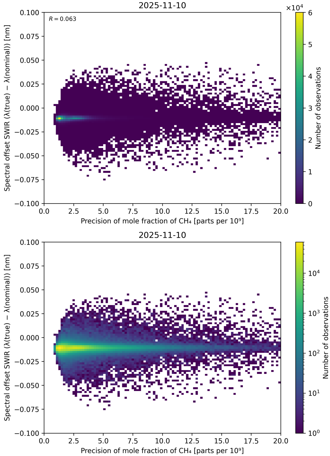
Figure 85: Scatter density plot of “Precision of mole fraction of CH 4 ” against “Spectral offset SWIR ( \lambda_{\text{true}} - \lambda_{\text{nominal}} )” for 2025-11-09 to 2025-11-11.
