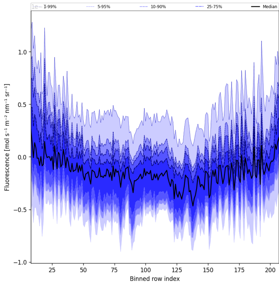
Figure 43: Along track statistics of “Fluorescence” for 2025-11-09 to 2025-11-11
