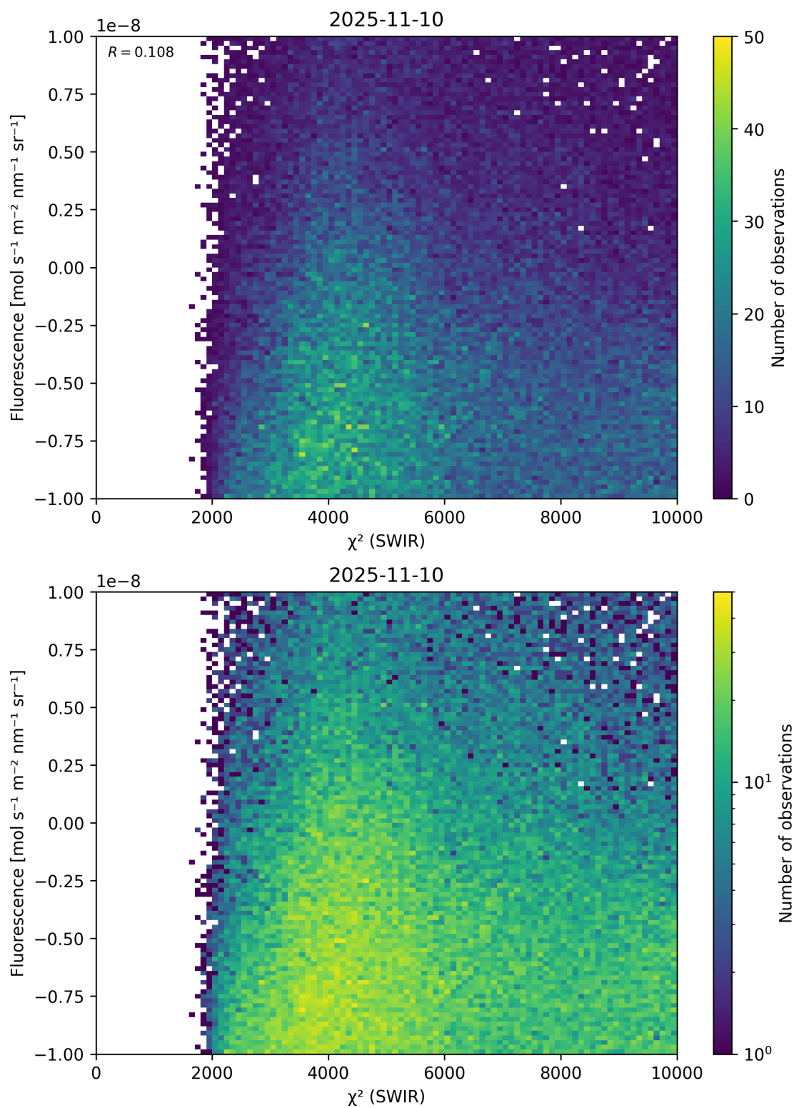
Figure 49: Scatter density plot of “ \chi^2 (SWIR)” against “Fluorescence” for 2025-11-09 to 2025-11-11.
