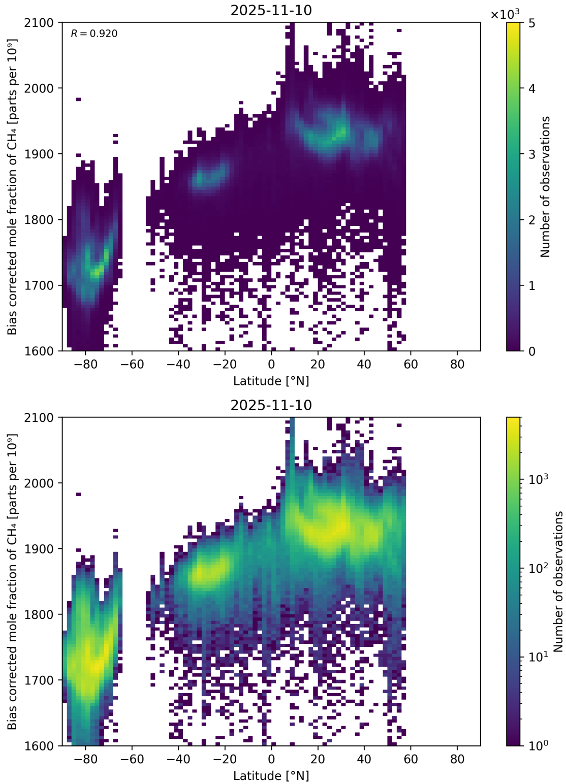
Figure 58: Scatter density plot of “Latitude” against “Bias corrected mole fraction of \text{CH}_4 ” for 2025-11-09 to 2025-11-11.
