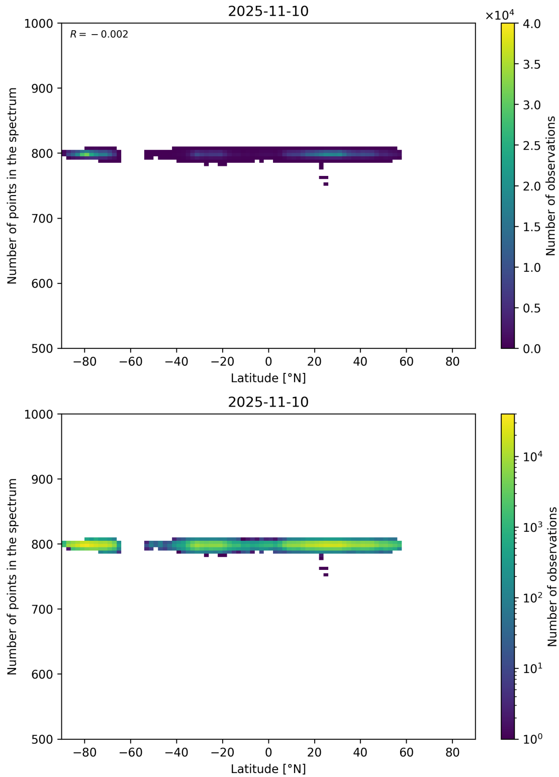
Figure 61: Scatter density plot of “Latitude” against “Number of points in the spectrum” for 2025-11-09 to 2025-11-11.
