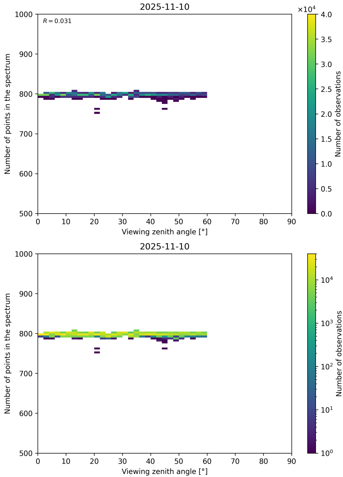
Figure 114: Scatter density plot of “Viewing zenith angle” against “Number of points in the spectrum” for 2025-11-09 to 2025-11-11.
