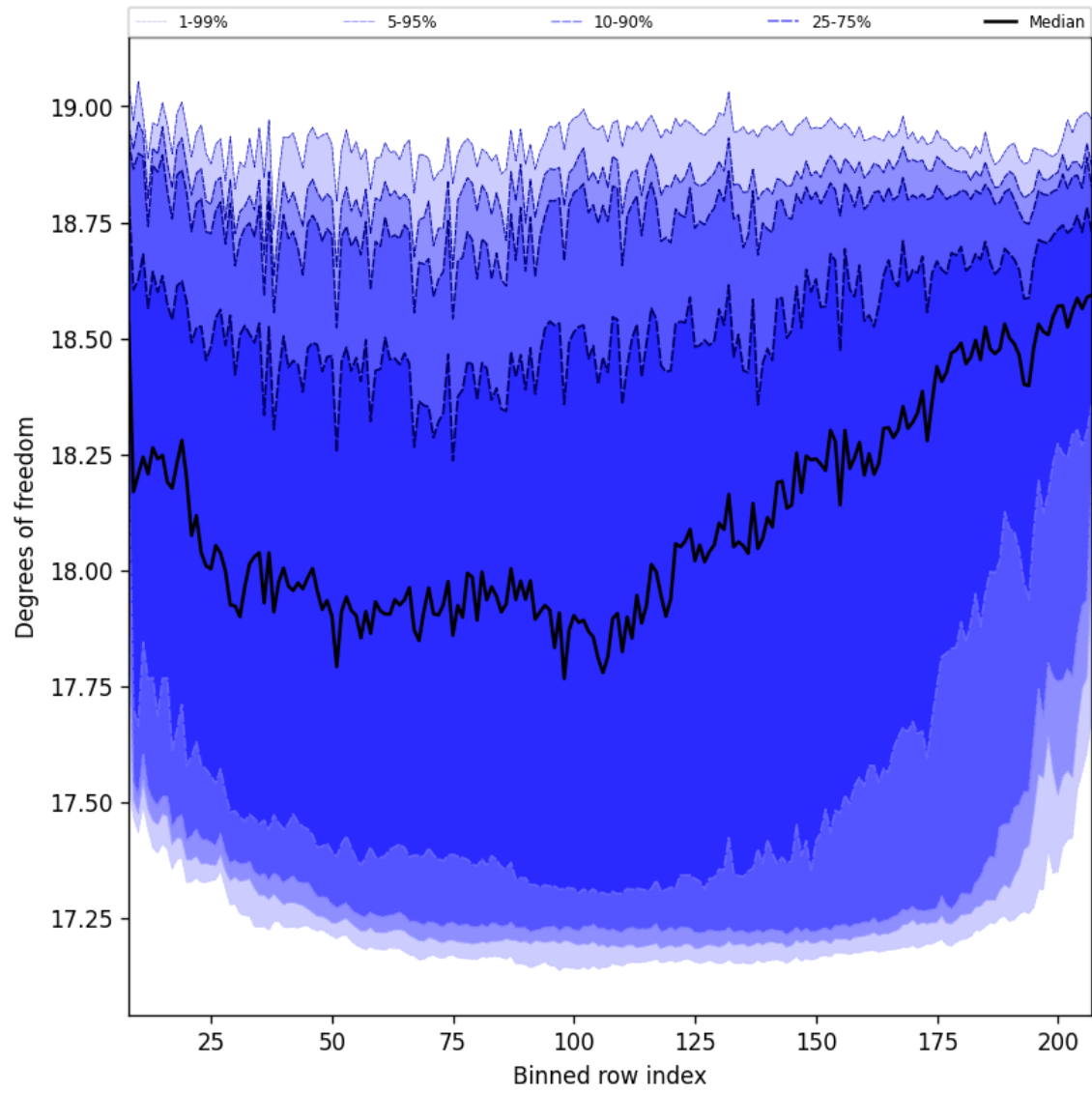
Figure 41: Along track statistics of “Degrees of freedom” for 2025-11-09 to 2025-11-11
