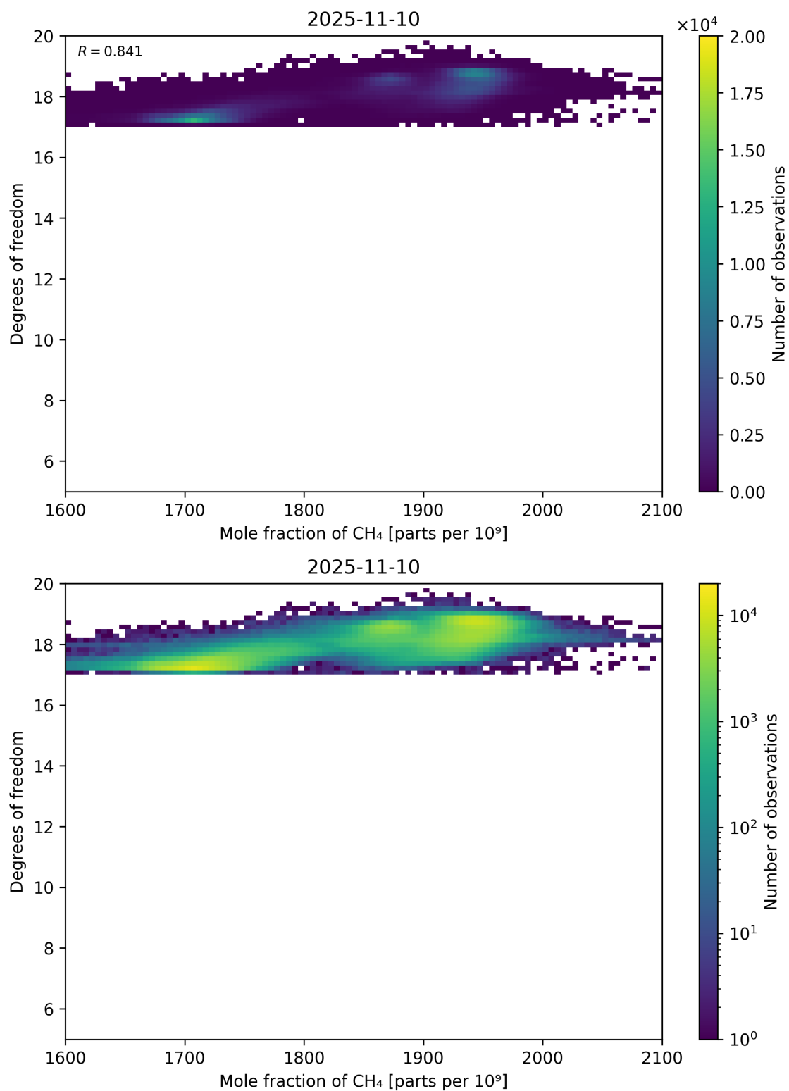
Figure 72: Scatter density plot of “Mole fraction of CH 4 ” against “Degrees of freedom” for 2025-11-09 to 2025-11-11.
