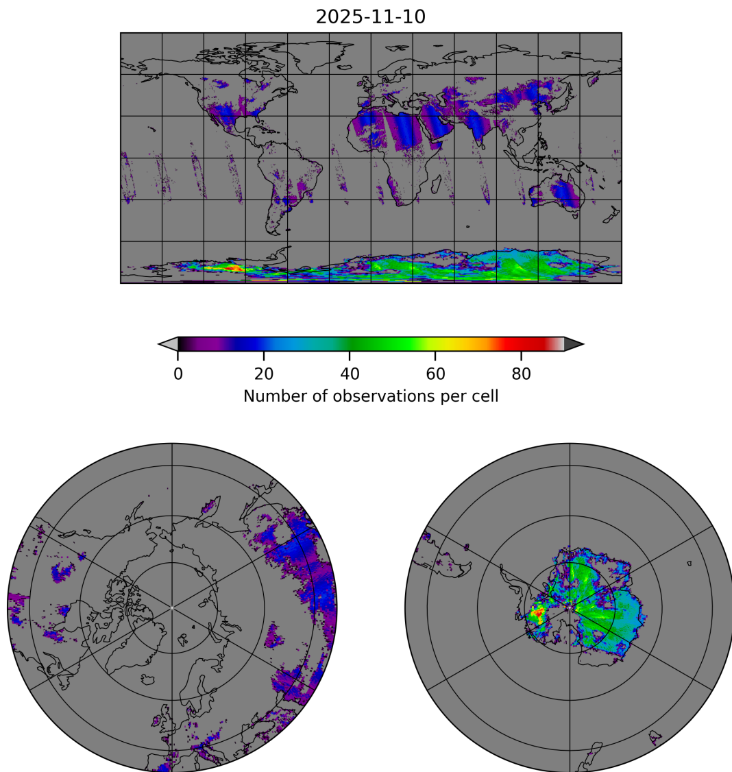
Figure 10: Map of the number of observations for 2025-11-09 to 2025-11-11
