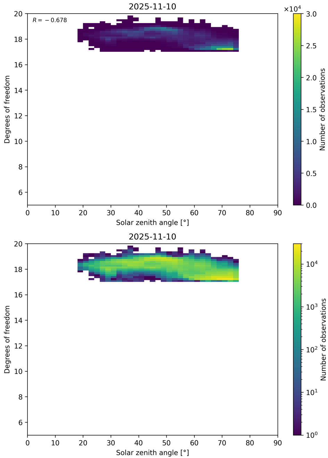
Figure 96: Scatter density plot of “Solar zenith angle” against “Degrees of freedom” for 2025-11-09 to 2025-11-11.
