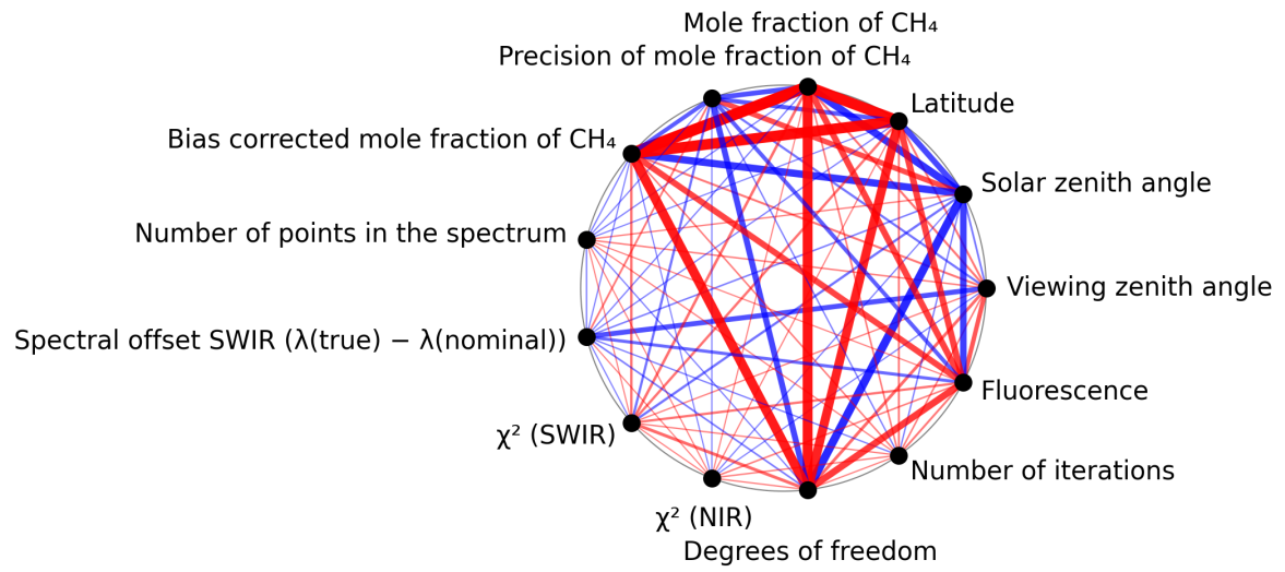
Figure 1: Map of correlation graph for 2025-11-09 to 2025-11-11.
