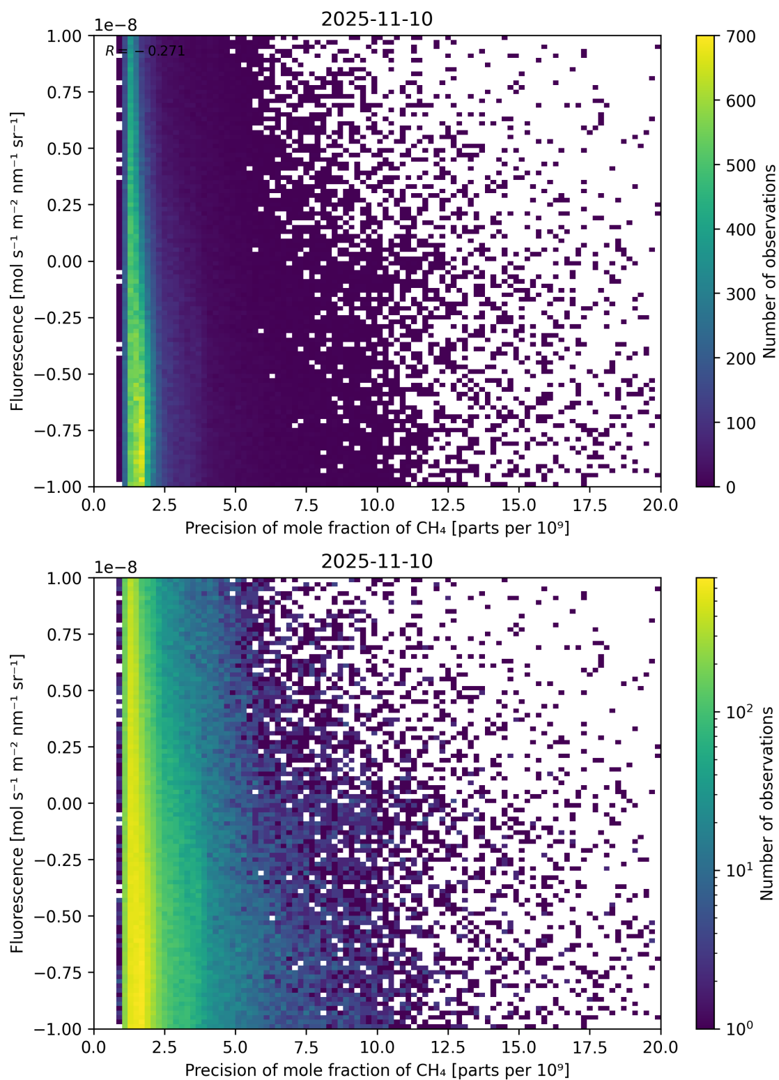
Figure 81: Scatter density plot of “Precision of mole fraction of CH 4 ” against “Fluorescence” for 2025-11-09 to 2025-11-11.
