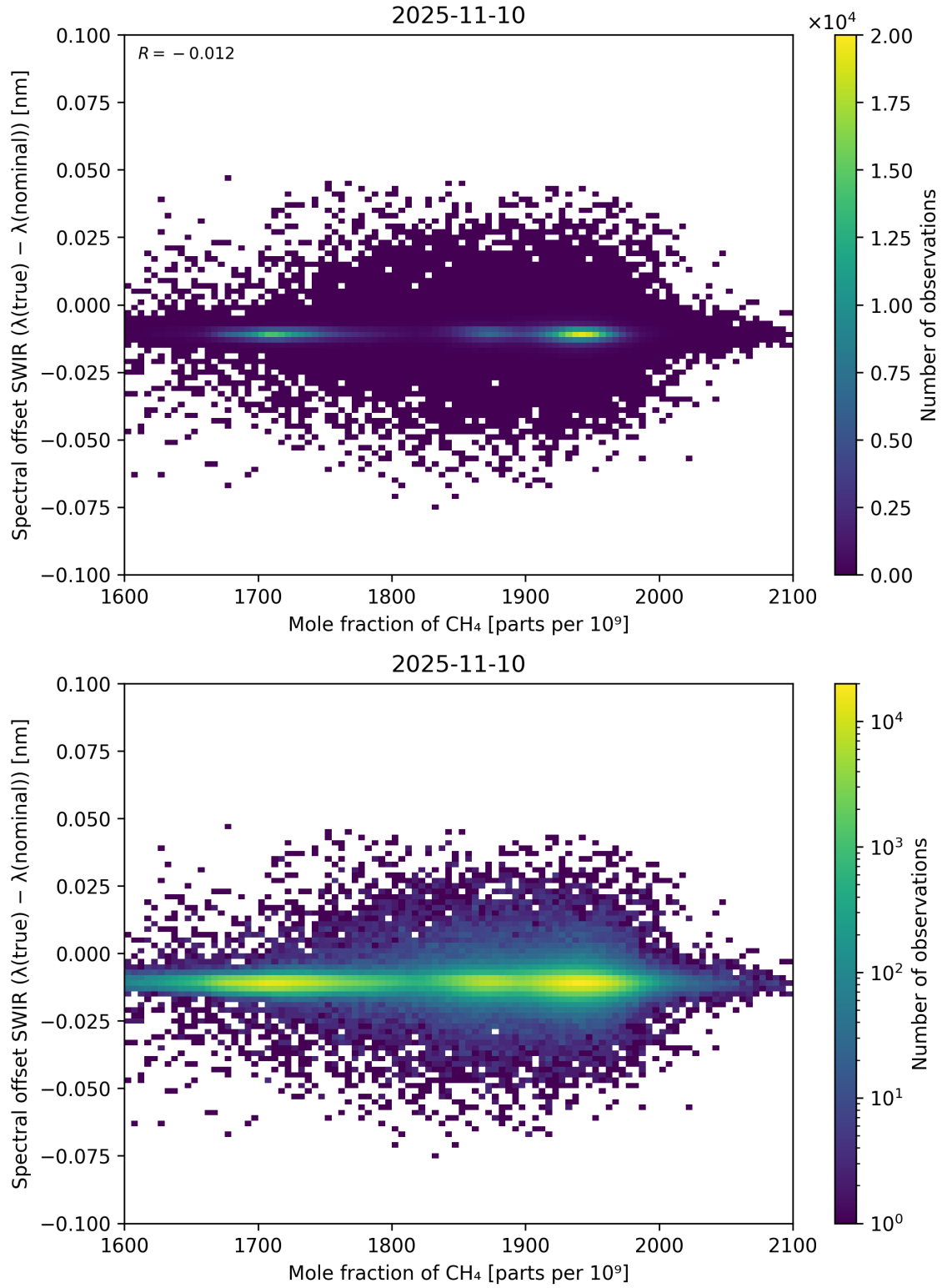
Figure 86: Scatter density plot of “Mole fraction of CH 4 ” against “Spectral offset SWIR ( \lambda_{\text{true}} - \lambda_{\text{nominal}} )” for 2025-11-09 to 2025-11-11.
