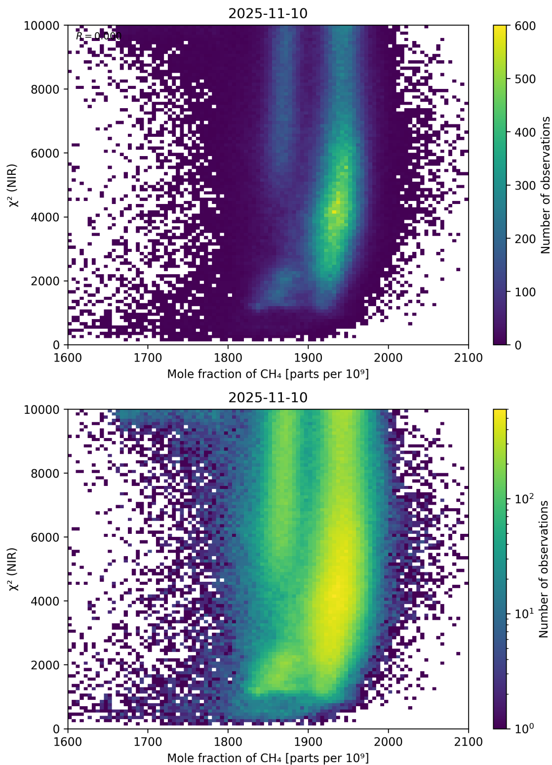
Figure 70: Scatter density plot of “Mole fraction of CH 4 ” against “ \chi^2 (NIR)” for 2025-11-09 to 2025-11-11.
