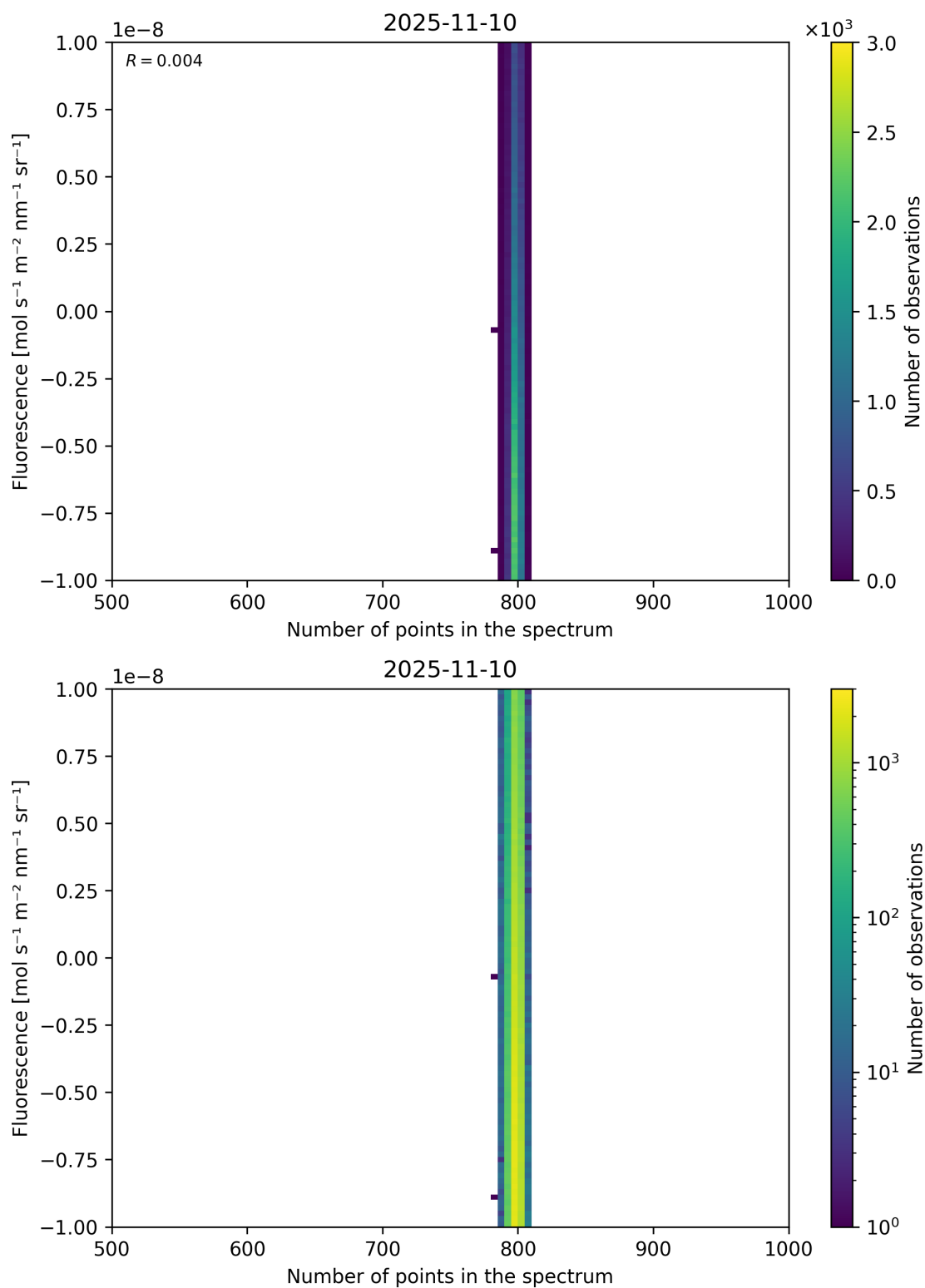
Figure 91: Scatter density plot of “Number of points in the spectrum” against “Fluorescence” for 2025-11-09 to 2025-11-11.
