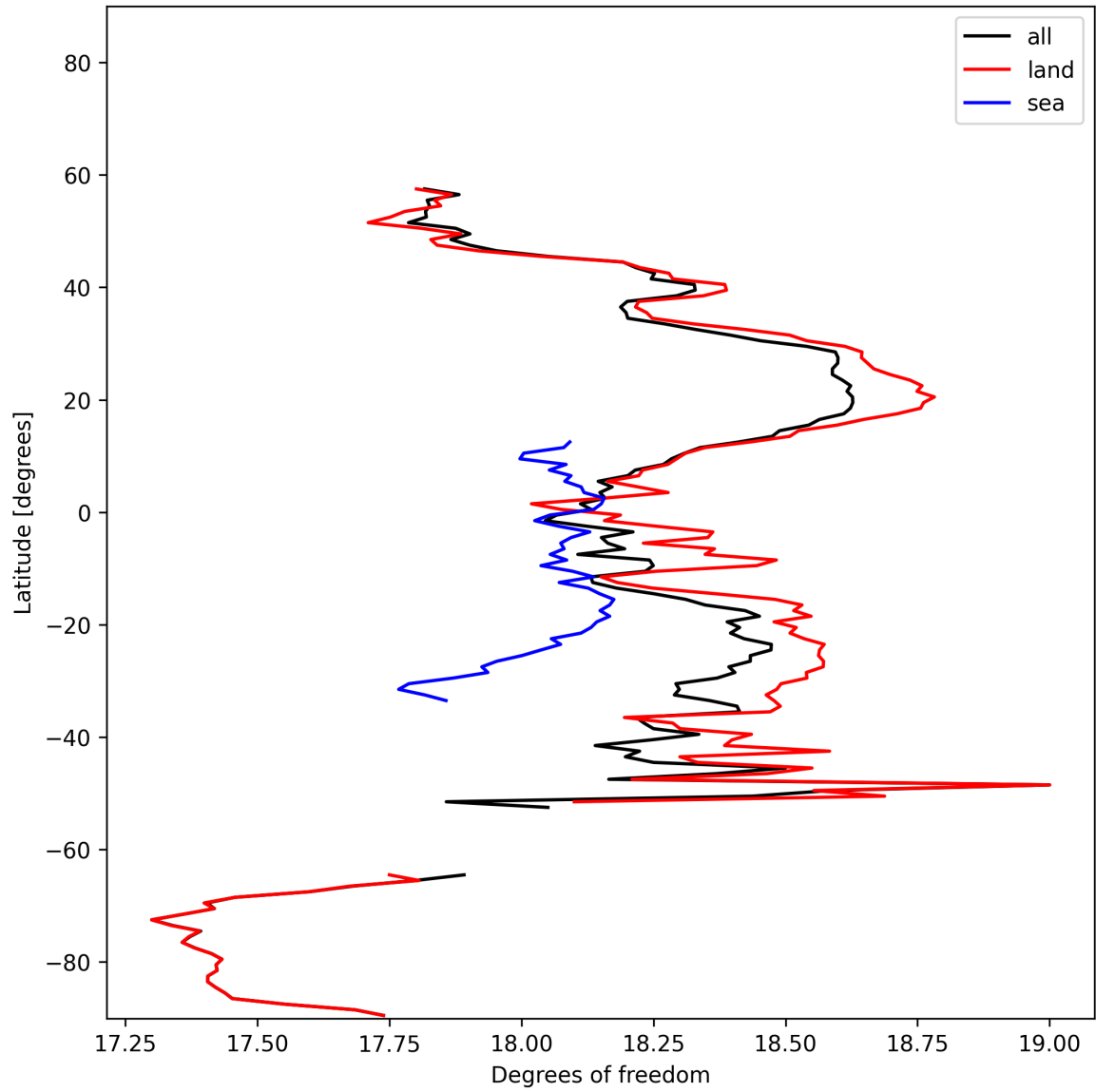
Figure 19: Zonal average of “Degrees of freedom” for 2025-11-09 to 2025-11-11.
