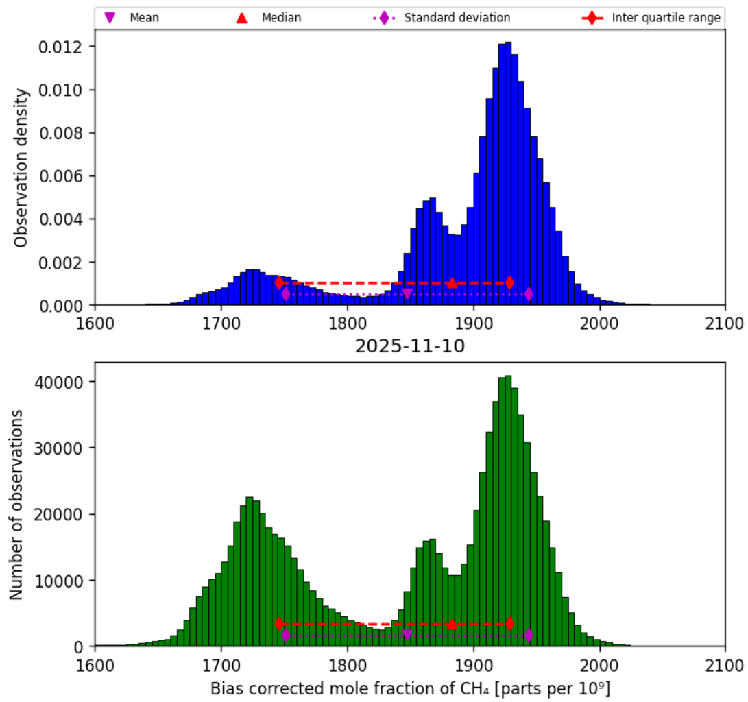
Figure 25: Histogram of “Bias corrected mole fraction of CH 4 ” for 2025-11-09 to 2025-11-11
