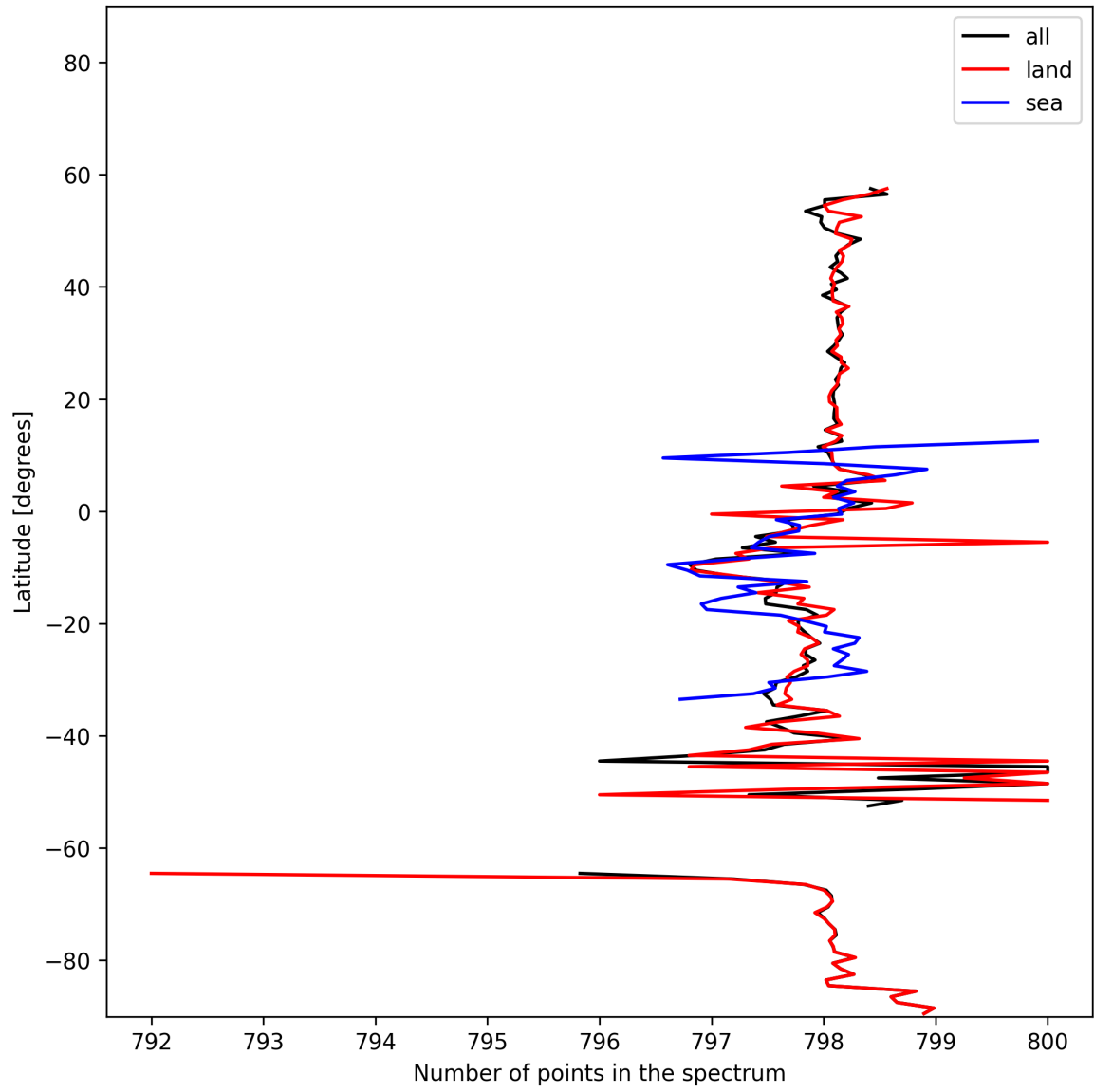
Figure 15: Zonal average of “Number of points in the spectrum” for 2025-11-09 to 2025-11-11.
