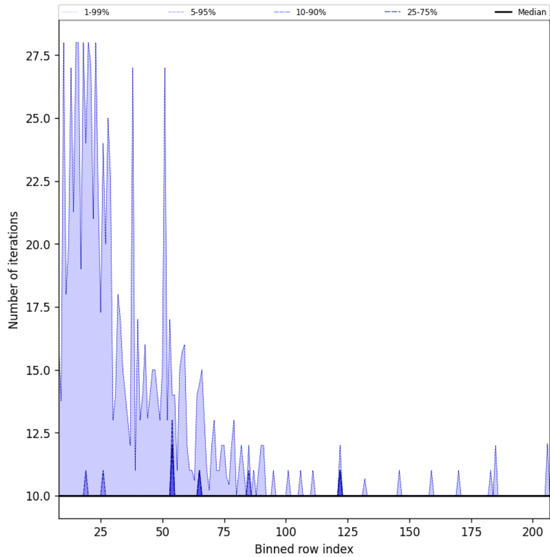
Figure 42: Along track statistics of “Number of iterations” for 2025-11-09 to 2025-11-11
