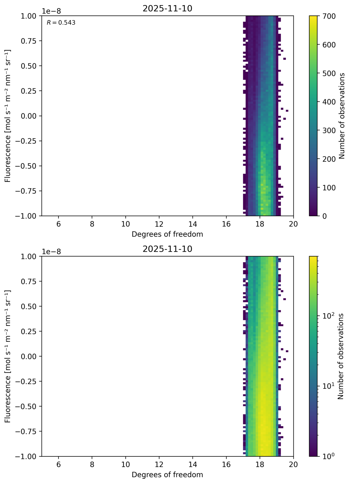
Figure 51: Scatter density plot of “Degrees of freedom” against “Fluorescence” for 2025-11-09 to 2025-11-11.
