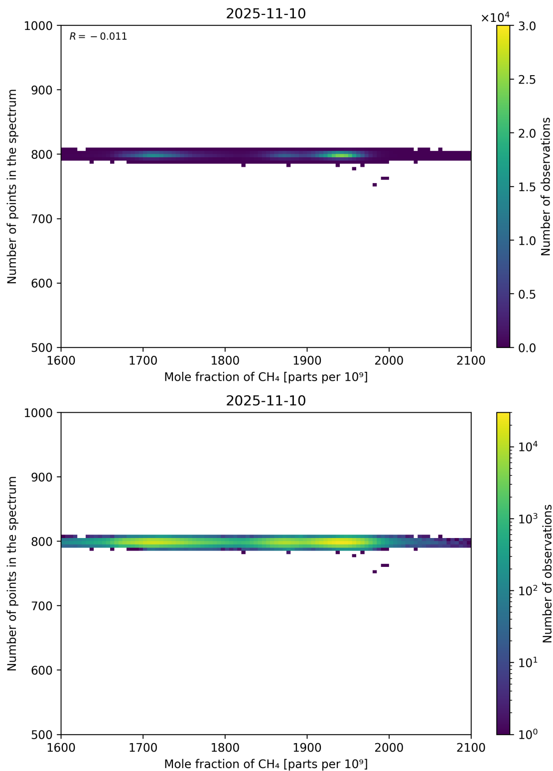
Figure 77: Scatter density plot of “Mole fraction of CH 4 ” against “Number of points in the spectrum” for 2025-11-09 to 2025-11-11.
