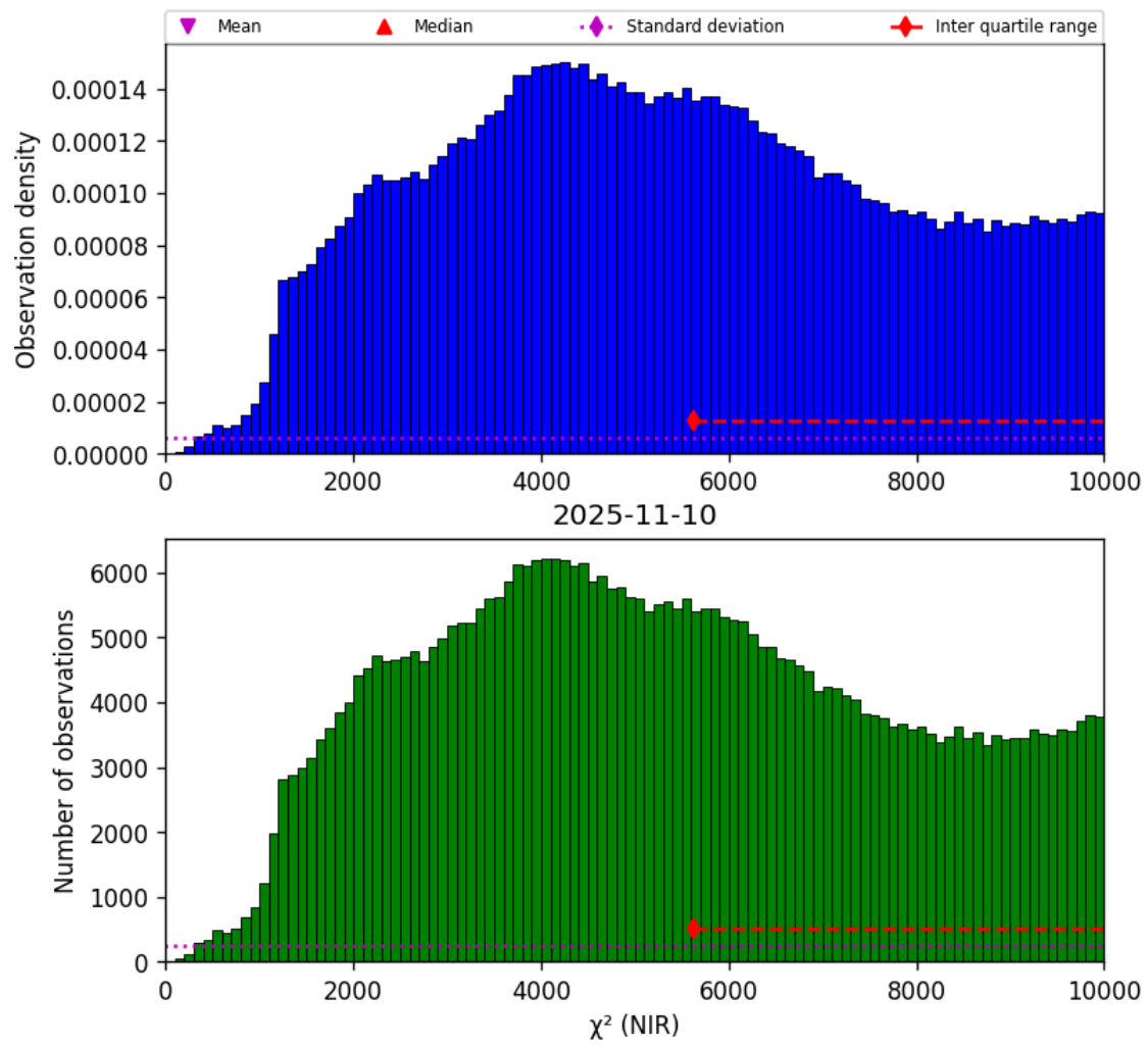
Figure 29: Histogram of " \chi^2 (NIR)" for 2025-11-09 to 2025-11-11
