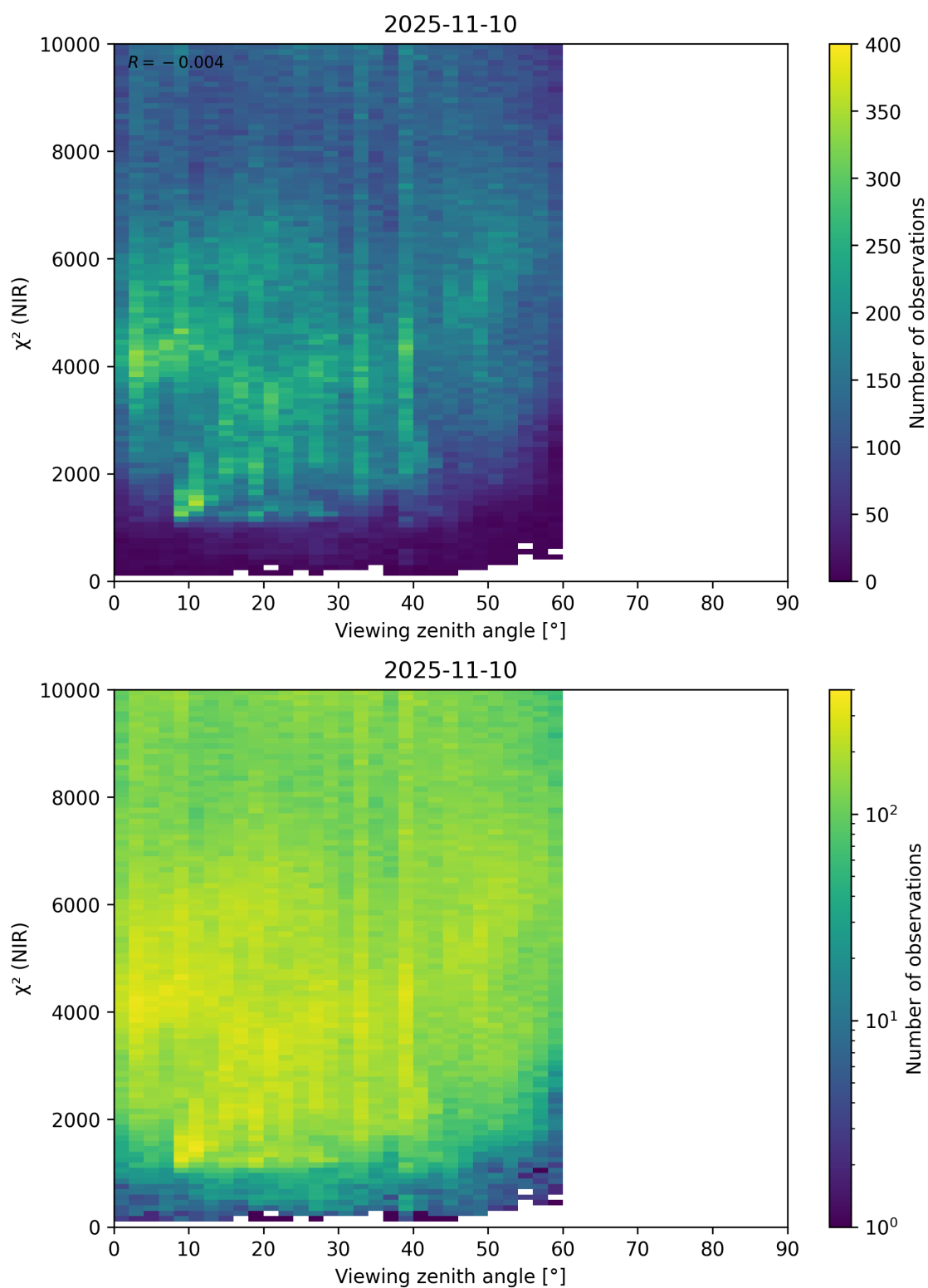
Figure 105: Scatter density plot of “Viewing zenith angle” against “ \chi^2 (NIR)” for 2025-11-09 to 2025-11-11.
