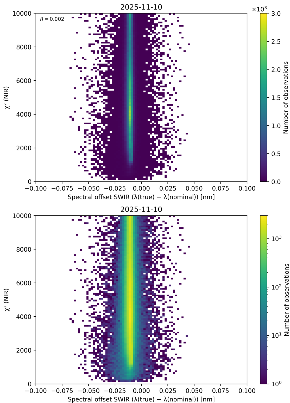
Figure 117: Scatter density plot of “Spectral offset SWIR ( \lambda_{\text{true}} - \lambda_{\text{nominal}} )” against “ \chi^2 (NIR)” for 2025-11-09 to 2025-11-11.
