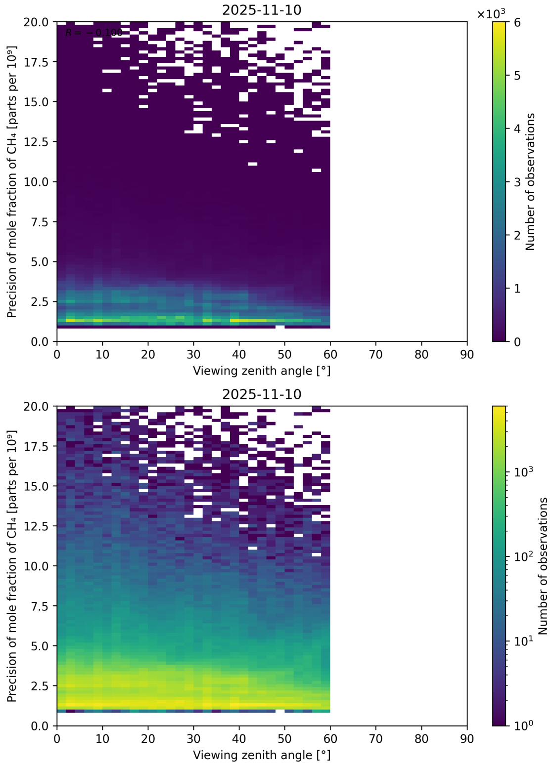
Figure 112: Scatter density plot of “Viewing zenith angle” against “Precision of mole fraction of CH 4 ” for 2025-11-09 to 2025-11-11.
