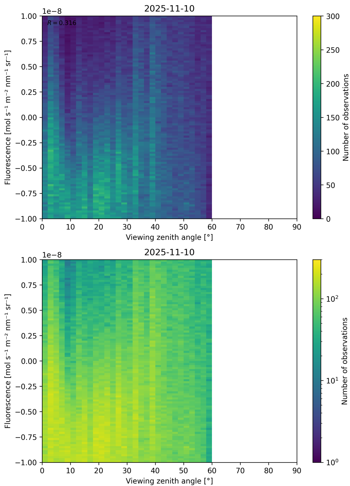
Figure 108: Scatter density plot of “Viewing zenith angle” against “Fluorescence” for 2025-11-09 to 2025-11-11.
