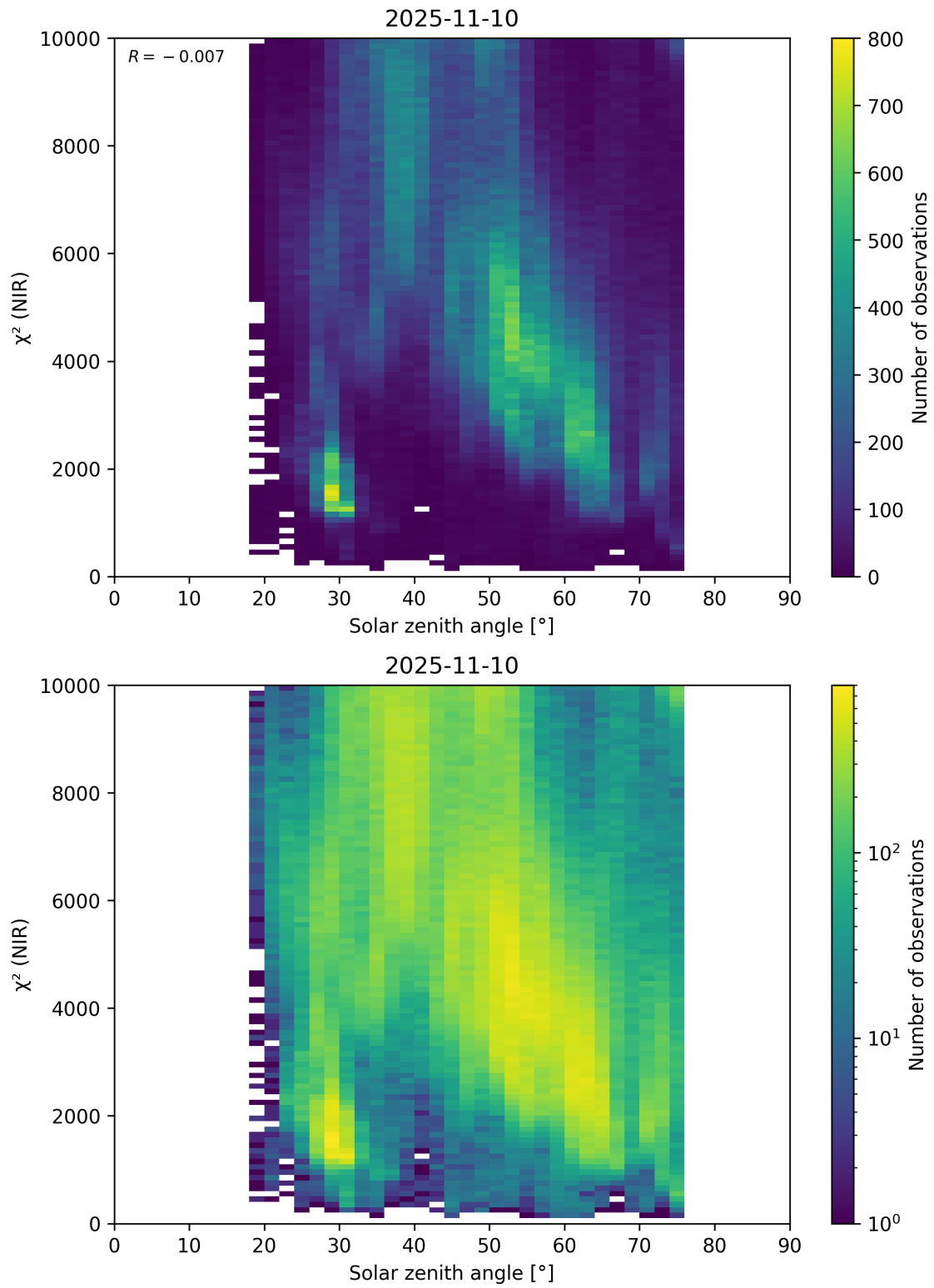
Figure 94: Scatter density plot of “Solar zenith angle” against “ \chi^2 (NIR)” for 2025-11-09 to 2025-11-11.
