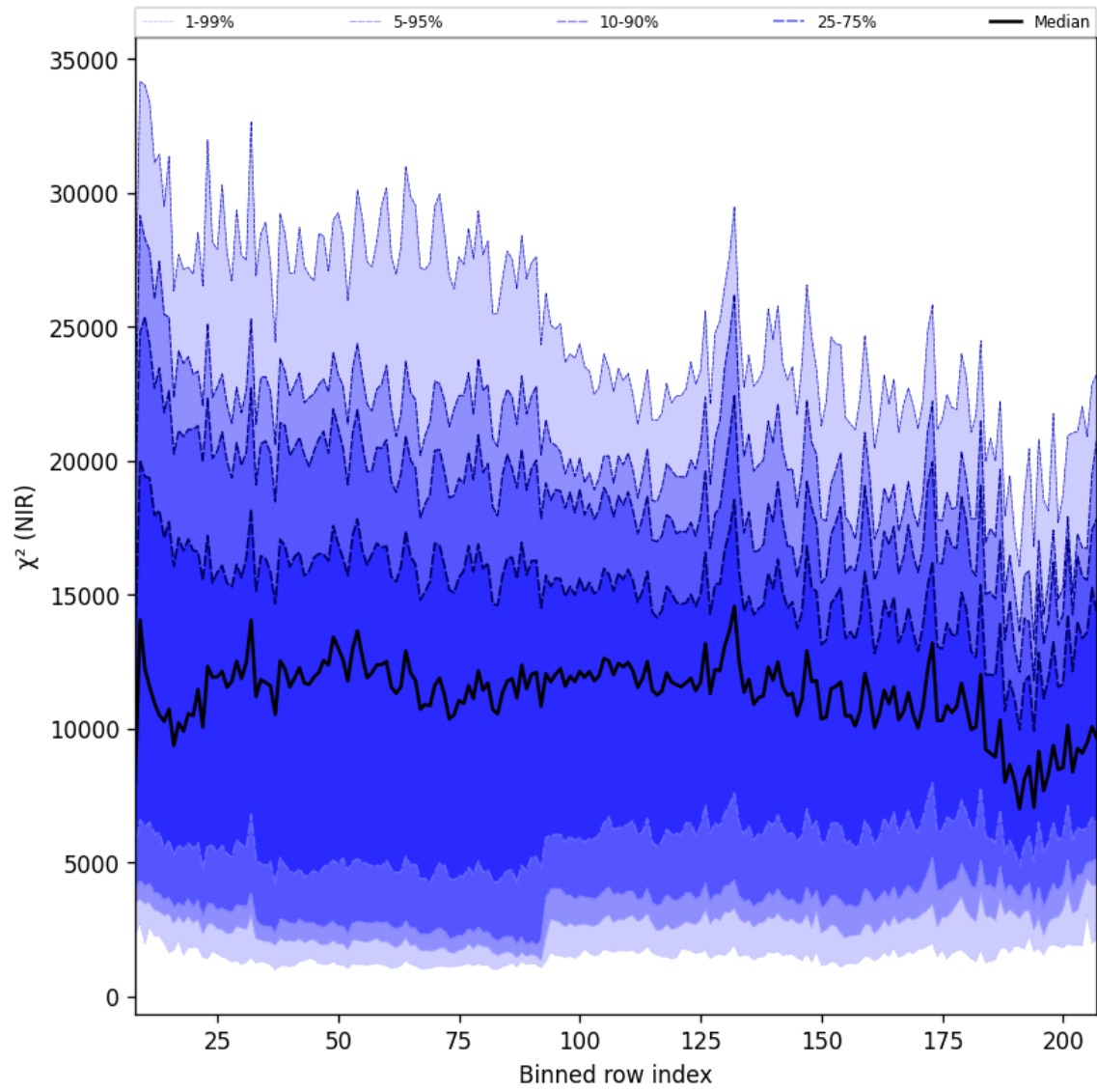
Figure 40: Along track statistics of “ \chi^2 (NIR)” for 2025-11-09 to 2025-11-11
