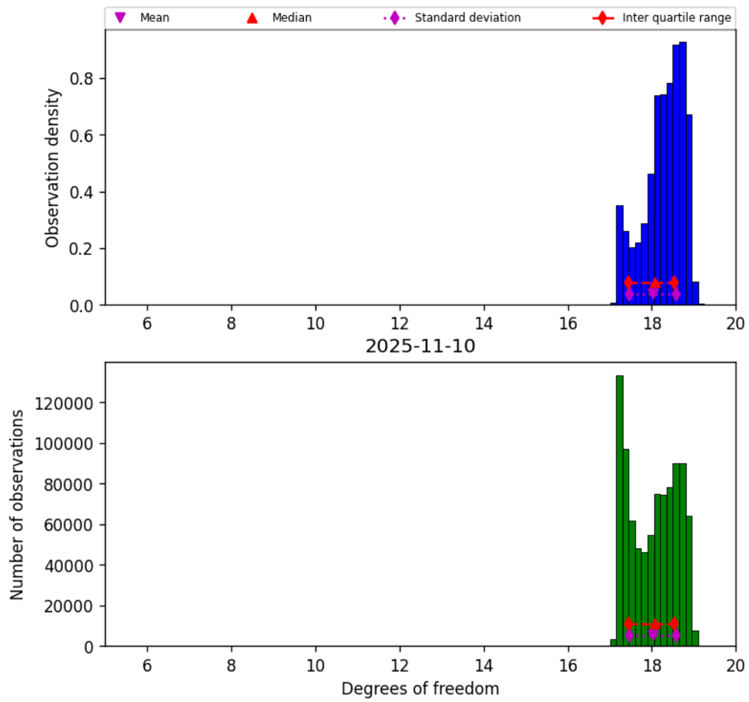
Figure 30: Histogram of “Degrees of freedom” for 2025-11-09 to 2025-11-11
