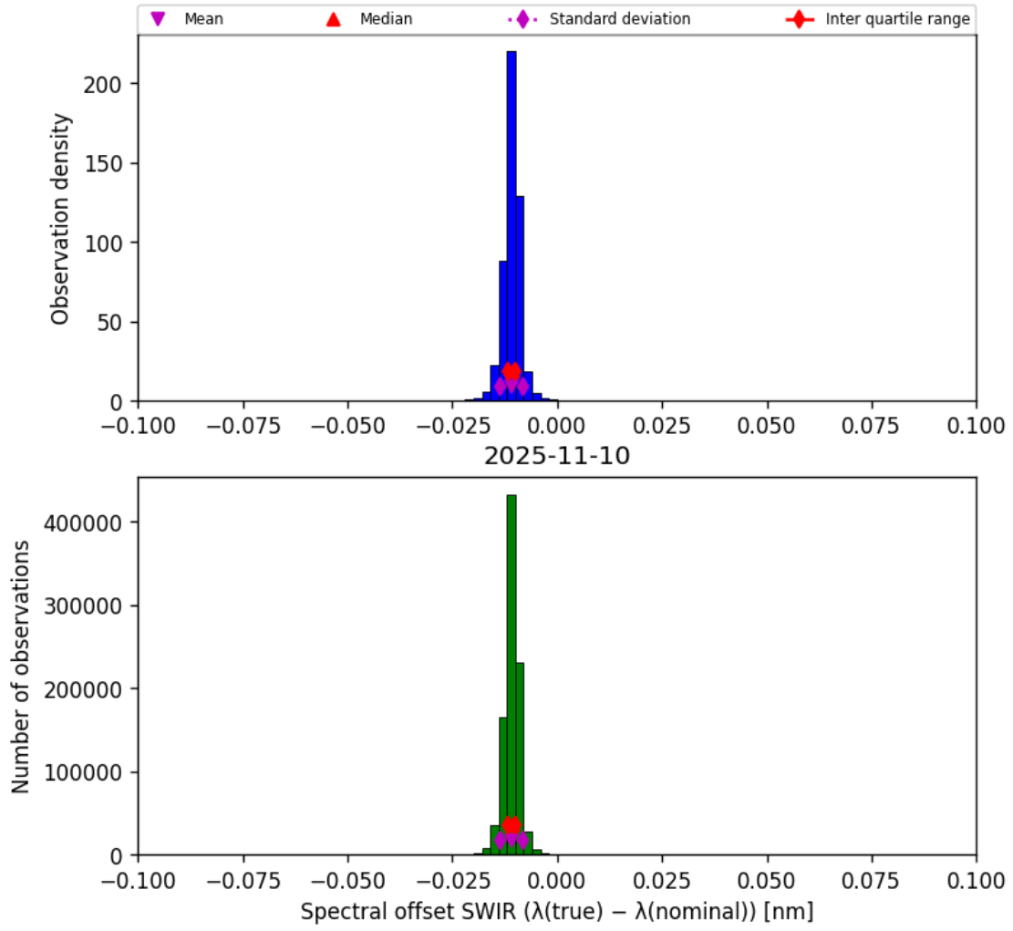
Figure 27: Histogram of “Spectral offset SWIR ( \lambda_{\text{true}} - \lambda_{\text{nominal}} )” for 2025-11-09 to 2025-11-11
