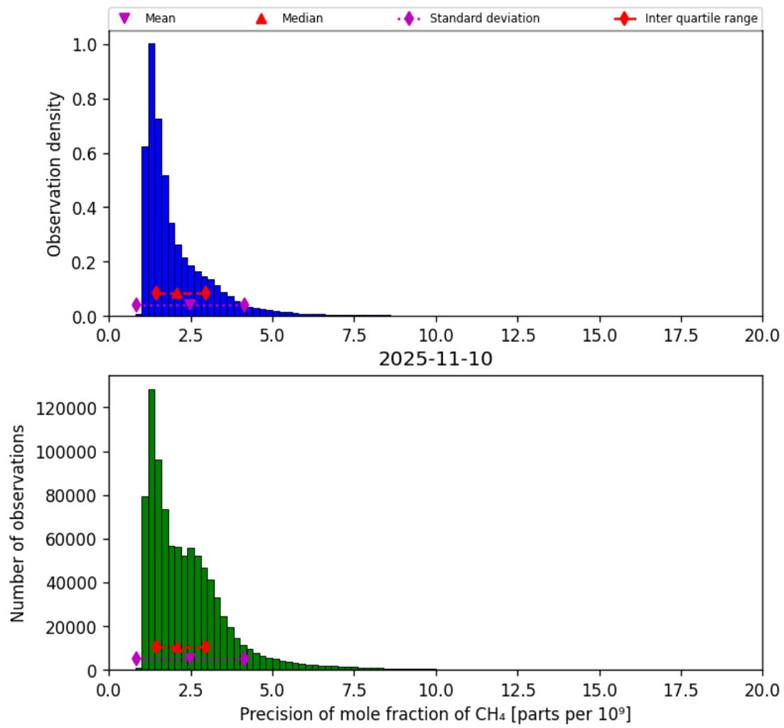
Figure 24: Histogram of “Precision of mole fraction of CH 4 ” for 2025-11-09 to 2025-11-11
