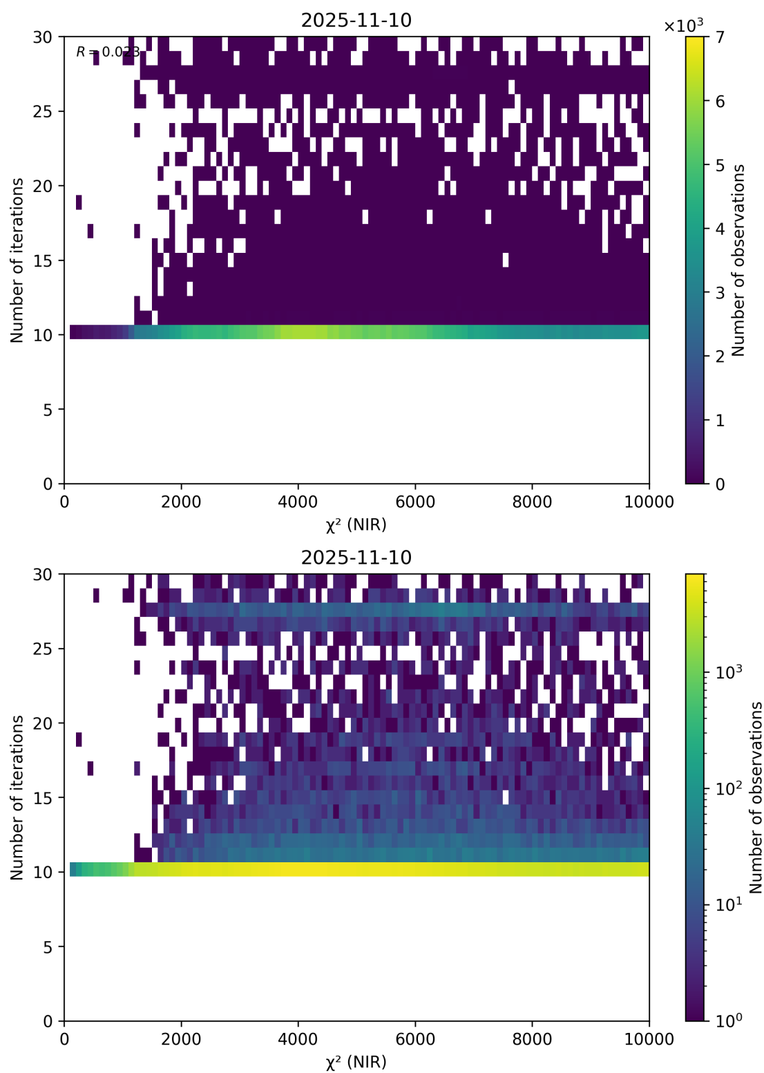
Figure 46: Scatter density plot of “ \chi^2 (NIR)” against “Number of iterations” for 2025-11-09 to 2025-11-11.
