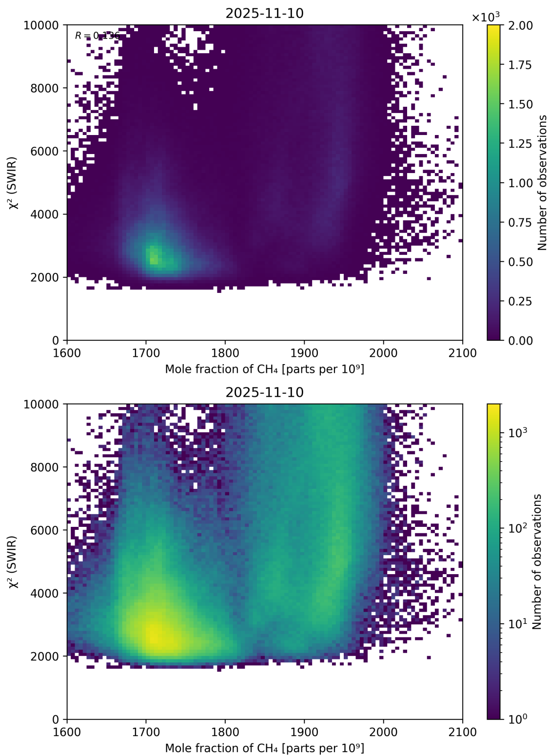
Figure 71: Scatter density plot of “Mole fraction of \text{CH}_4 ” against “ \chi^2 (SWIR)” for 2025-11-09 to 2025-11-11.
