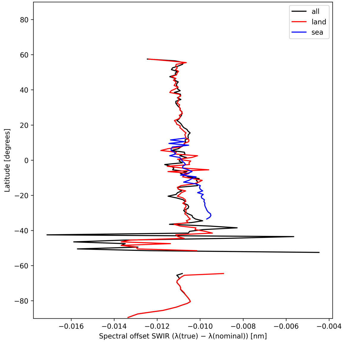
Figure 16: Zonal average of “Spectral offset SWIR ( \lambda_{\text{true}} - \lambda_{\text{nominal}} )” for 2025-11-09 to 2025-11-11.
