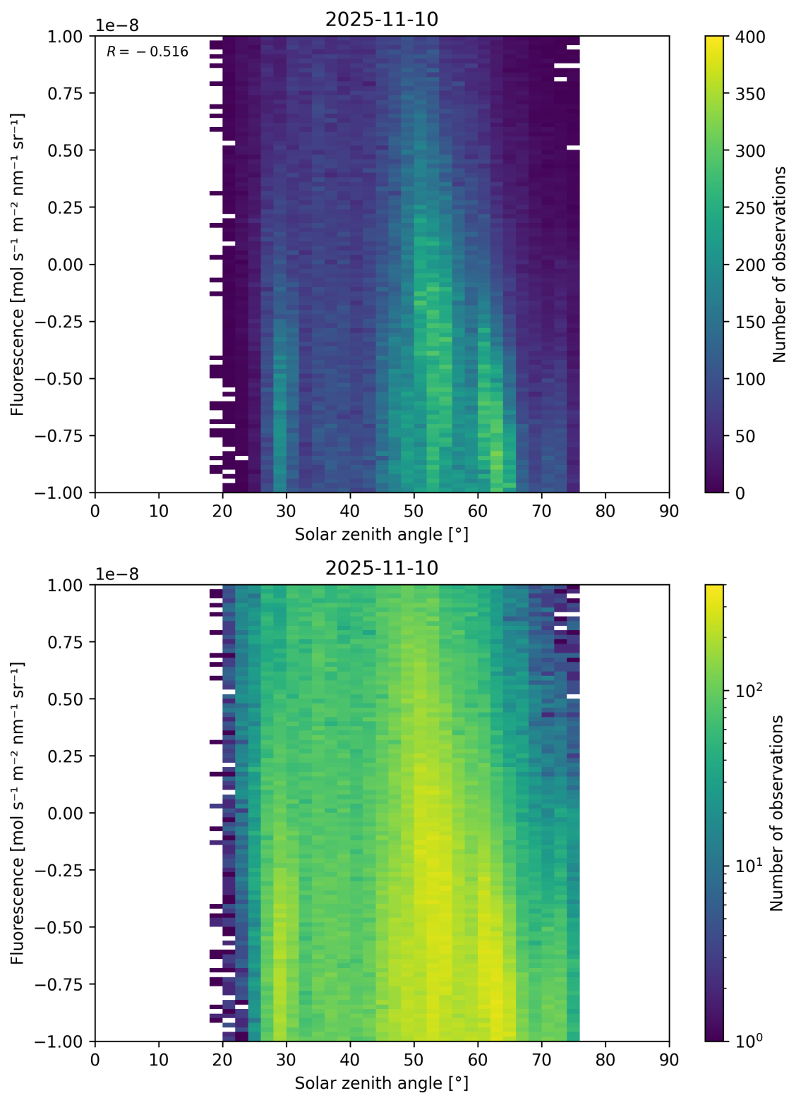
Figure 97: Scatter density plot of “Solar zenith angle” against “Fluorescence” for 2025-11-09 to 2025-11-11.
