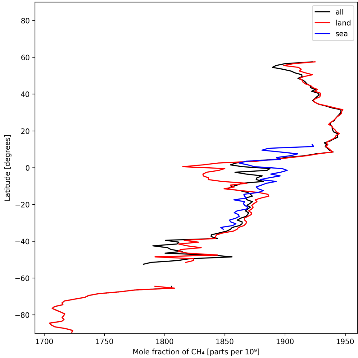
Figure 12: Zonal average of “Mole fraction of \text{CH}_4 ” for 2025-11-09 to 2025-11-11.
