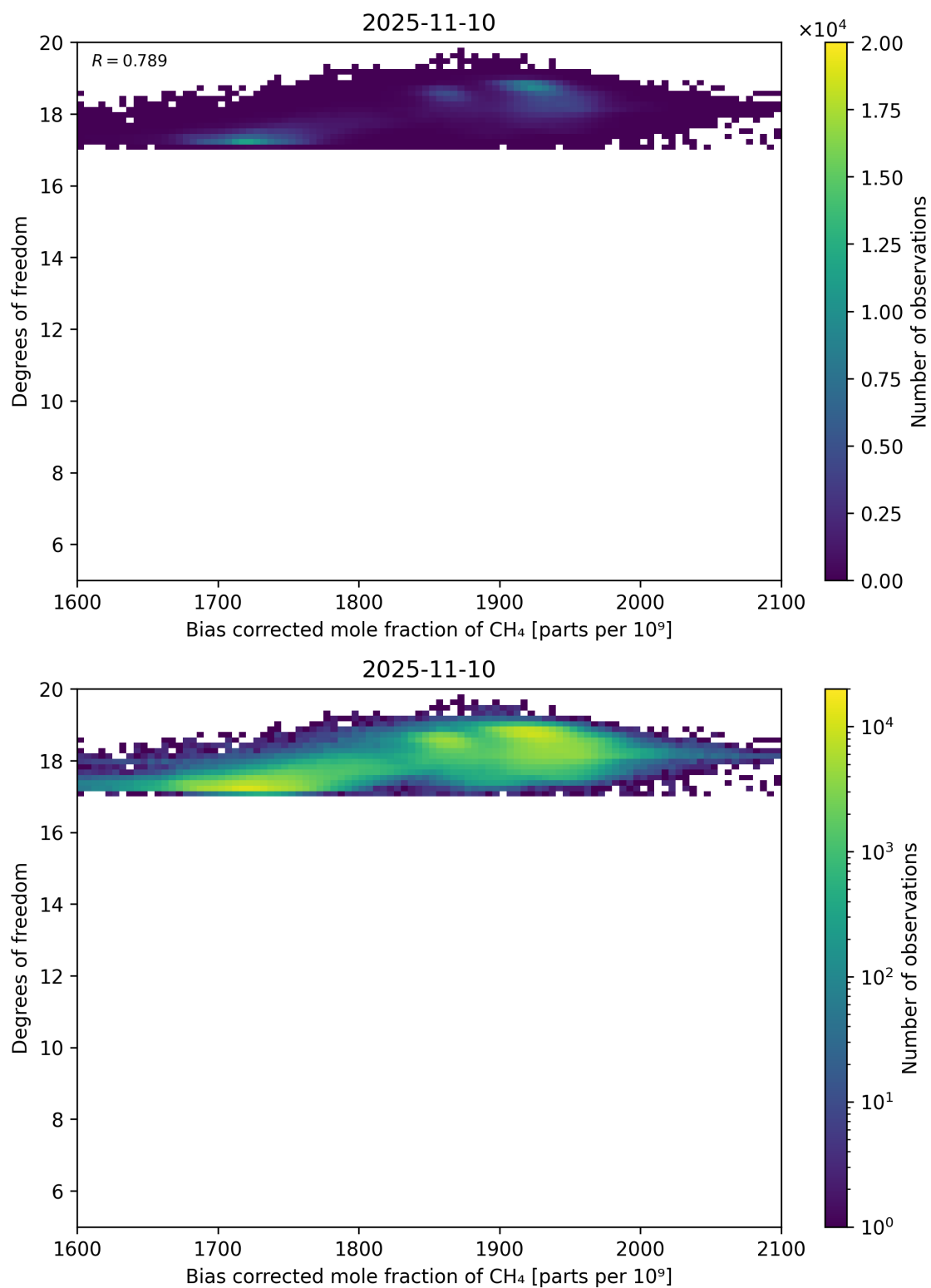
Figure 65: Scatter density plot of “Bias corrected mole fraction of CH 4 ” against “Degrees of freedom” for 2025-11-09 to 2025-11-11.
