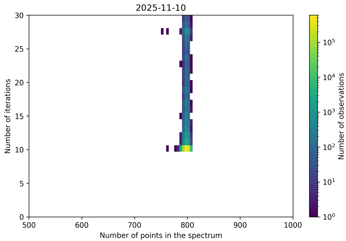
Figure 92: Scatter density plot of “Number of points in the spectrum” against “Number of iterations” for 2025-11-09 to 2025-11-11.
