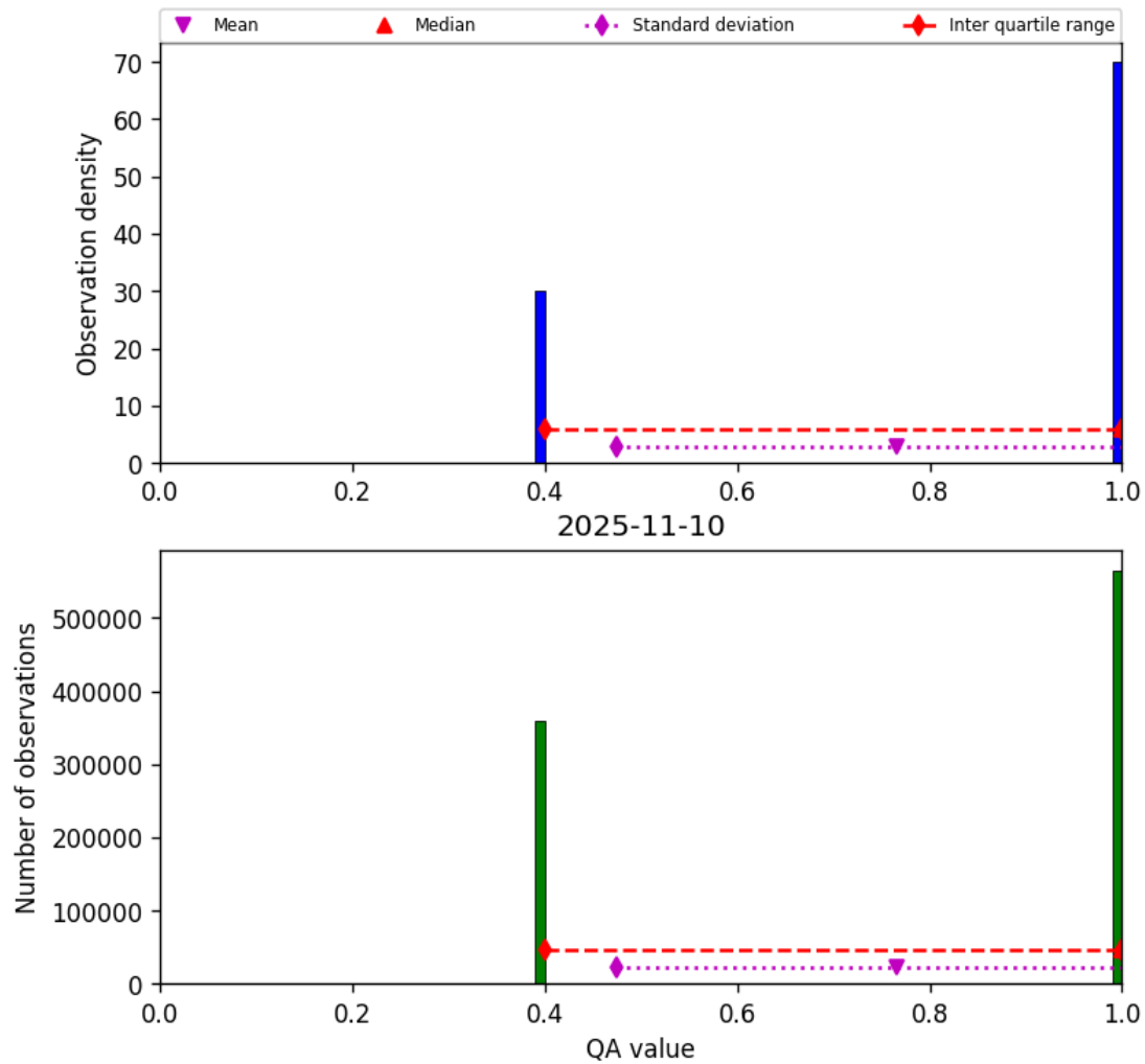
Figure 22: Histogram of “QA value” for 2025-11-09 to 2025-11-11
