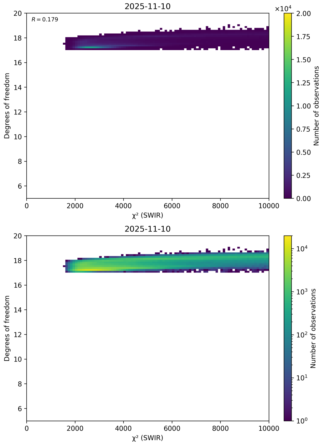
Figure 48: Scatter density plot of “ \chi^2 (SWIR)” against “Degrees of freedom” for 2025-11-09 to 2025-11-11.
