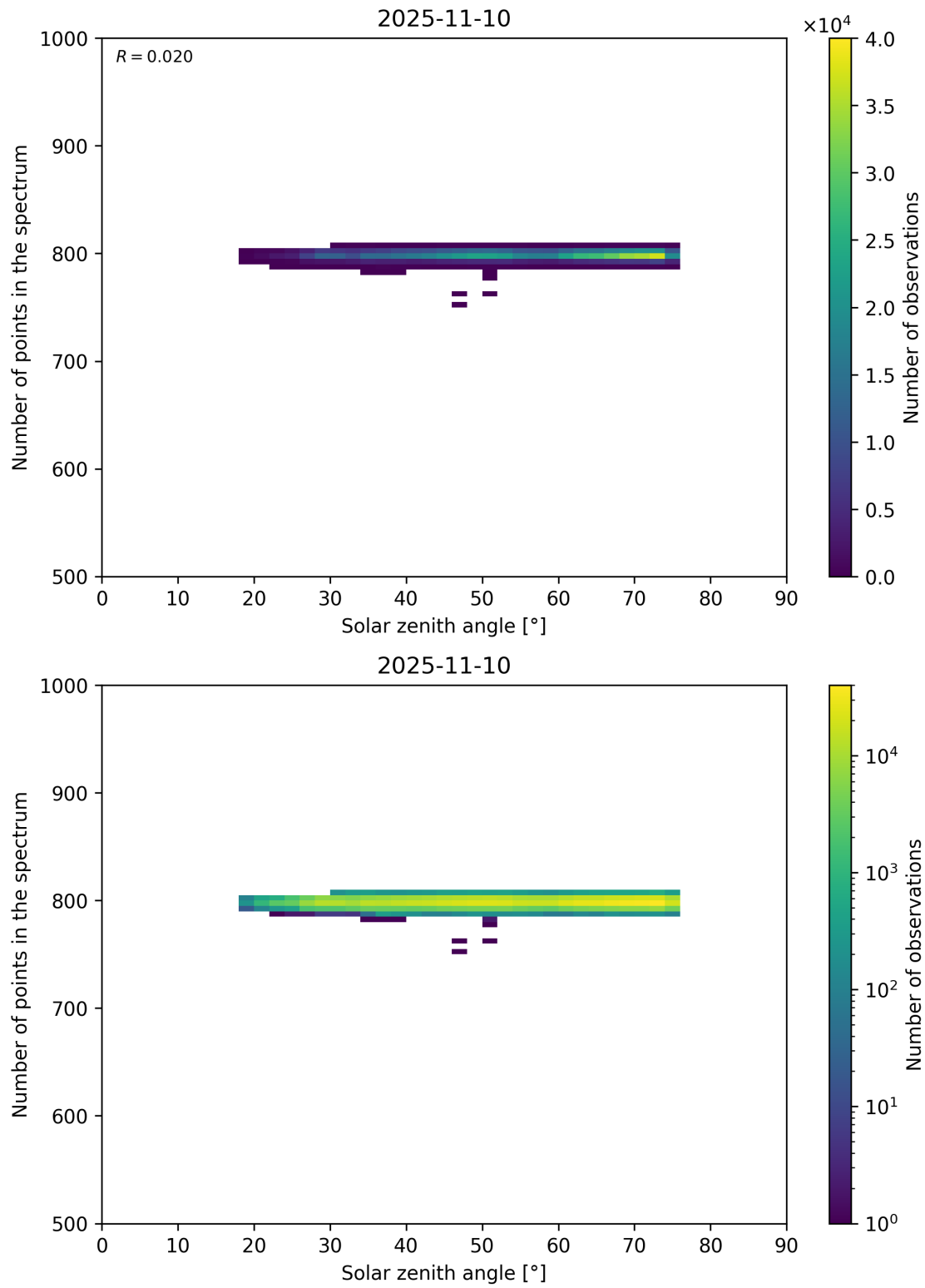
Figure 103: Scatter density plot of “Solar zenith angle” against “Number of points in the spectrum” for 2025-11-09 to 2025-11-11.
