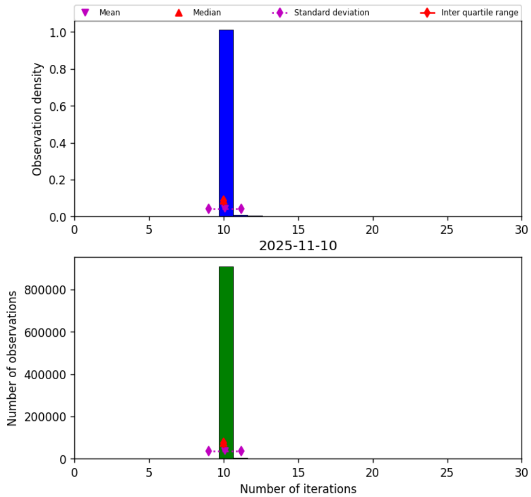
Figure 31: Histogram of “Number of iterations” for 2025-11-09 to 2025-11-11
