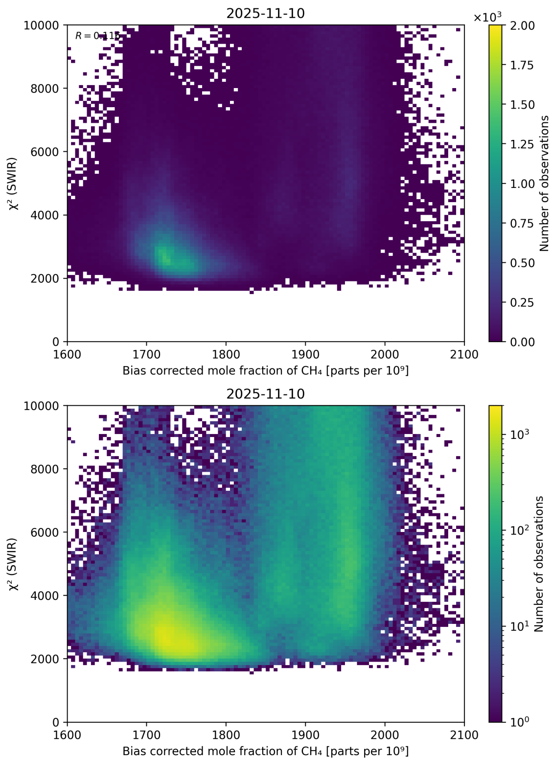
Figure 64: Scatter density plot of “Bias corrected mole fraction of \text{CH}_4 ” against “ \chi^2 (SWIR)” for 2025-11-09 to 2025-11-11.
