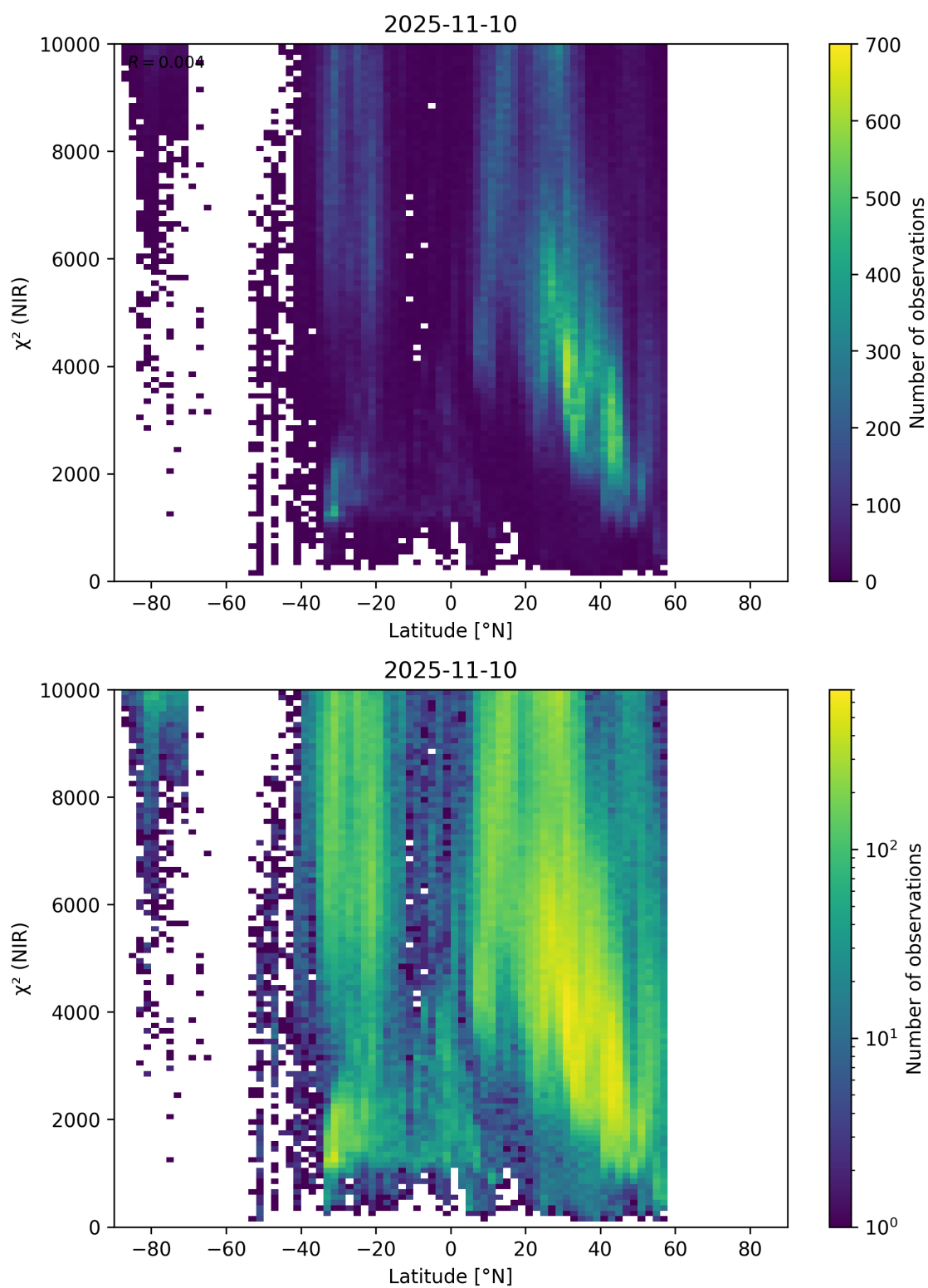
Figure 53: Scatter density plot of “Latitude” against “ \chi^2 (NIR)” for 2025-11-09 to 2025-11-11.
