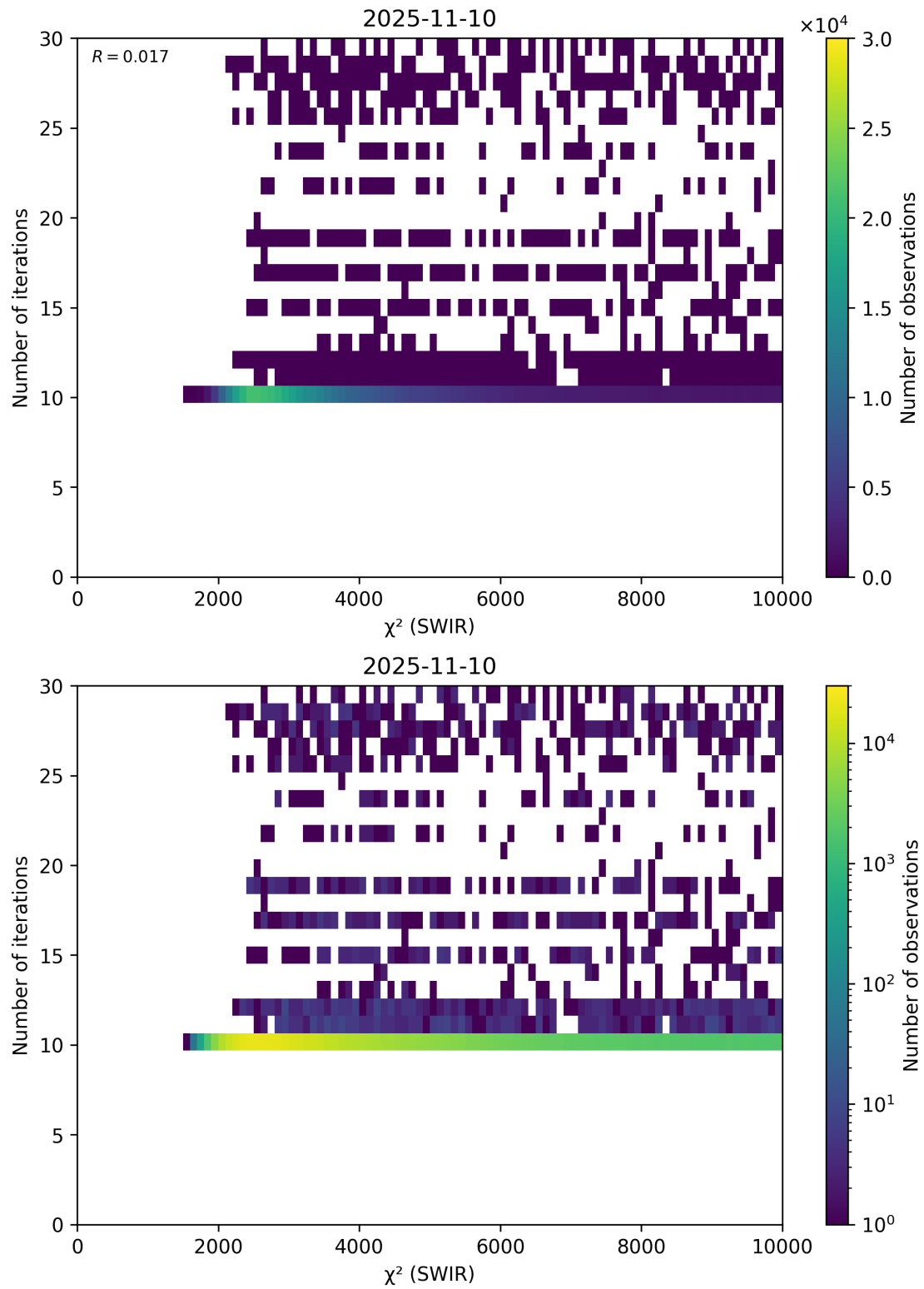
Figure 50: Scatter density plot of “ \chi^2 (SWIR)” against “Number of iterations” for 2025-11-09 to 2025-11-11.
