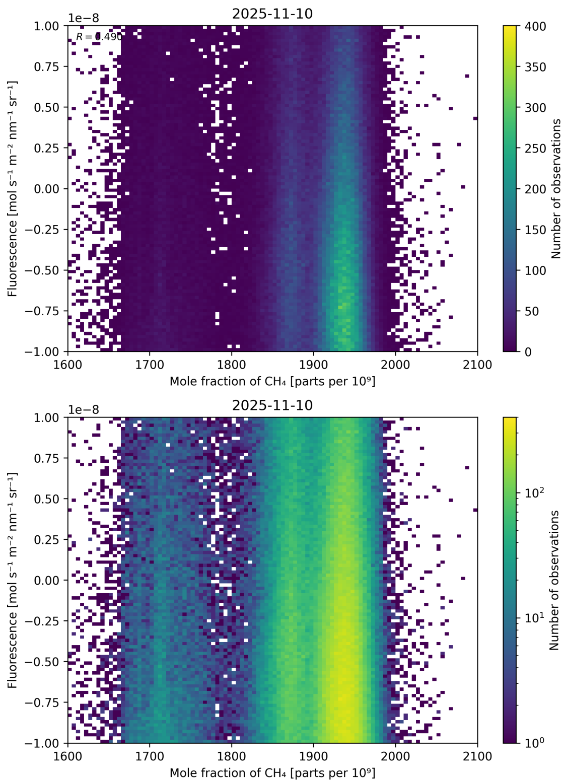
Figure 73: Scatter density plot of “Mole fraction of CH 4 ” against “Fluorescence” for 2025-11-09 to 2025-11-11.
