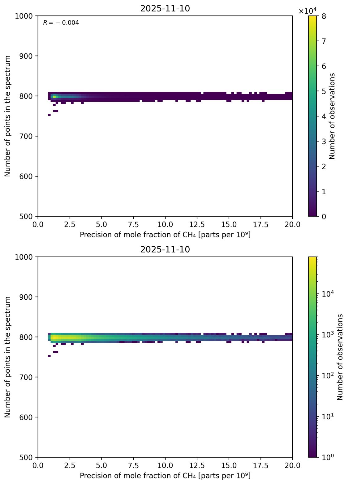
Figure 84: Scatter density plot of “Precision of mole fraction of CH 4 ” against “Number of points in the spectrum” for 2025-11-09 to 2025-11-11.
