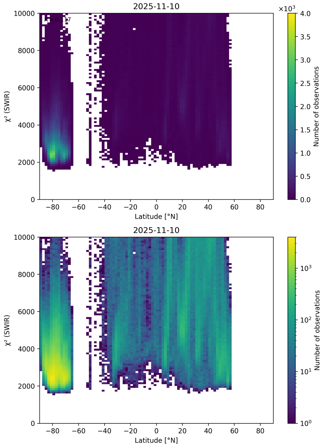
Figure 54: Scatter density plot of “Latitude” against “ \chi^2 (SWIR)” for 2025-11-09 to 2025-11-11.
