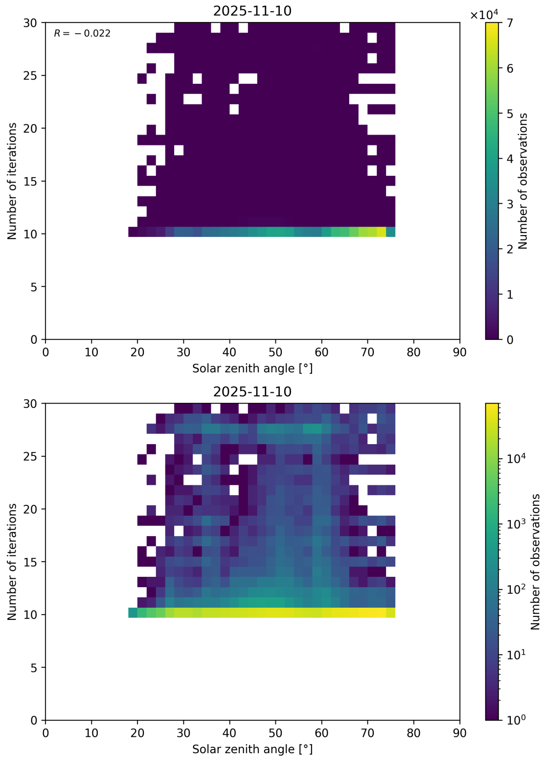
Figure 102: Scatter density plot of “Solar zenith angle” against “Number of iterations” for 2025-11-09 to 2025-11-11.
