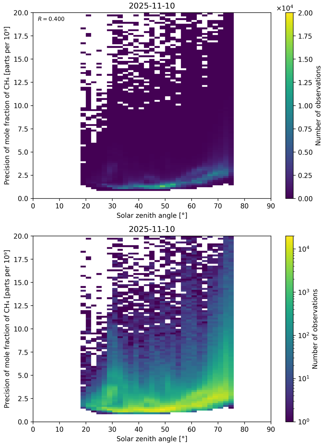
Figure 101: Scatter density plot of “Solar zenith angle” against “Precision of mole fraction of \text{CH}_4 ” for 2025-11-09 to 2025-11-11.
