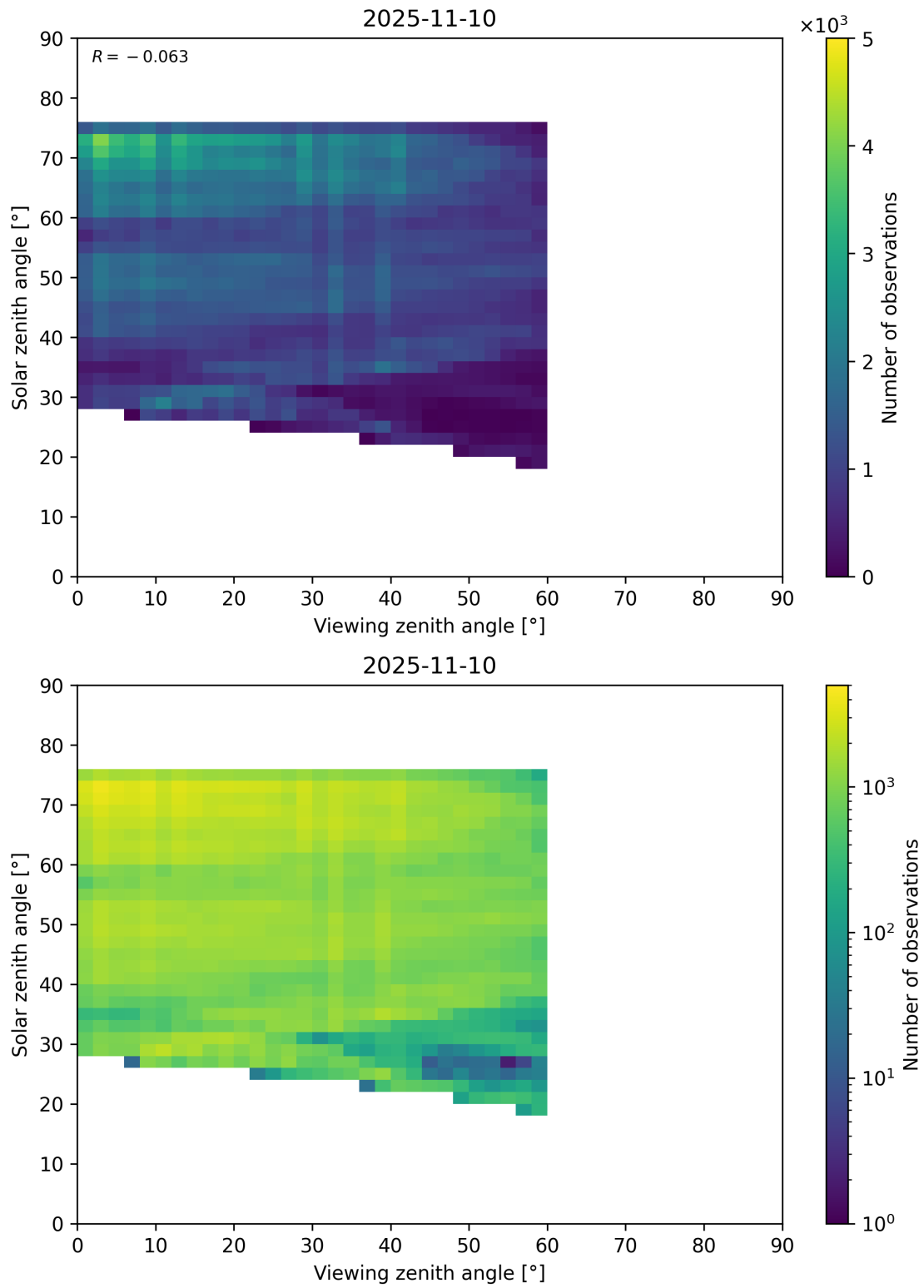
Figure 115: Scatter density plot of “Viewing zenith angle” against “Solar zenith angle” for 2025-11-09 to 2025-11-11.
