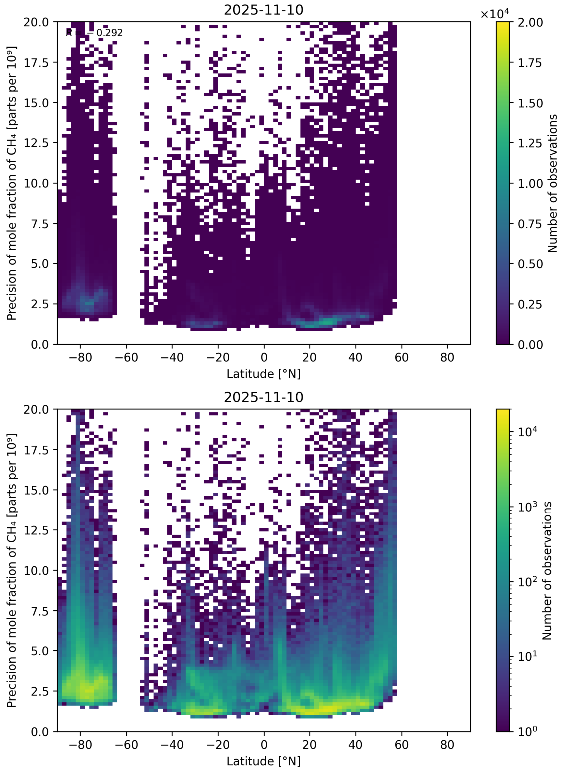
Figure 59: Scatter density plot of “Latitude” against “Precision of mole fraction of CH 4 ” for 2025-11-09 to 2025-11-11.
