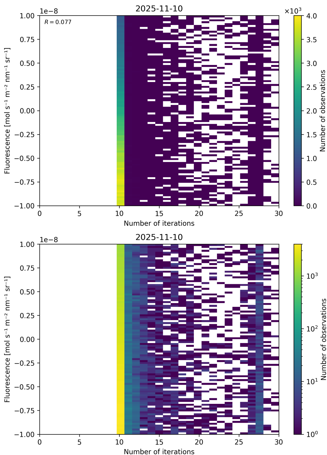
Figure 87: Scatter density plot of “Number of iterations” against “Fluorescence” for 2025-11-09 to 2025-11-11.
