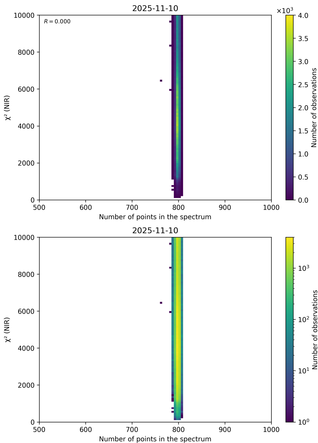
Figure 88: Scatter density plot of “Number of points in the spectrum” against “ \chi^2 (NIR)” for 2025-11-09 to 2025-11-11.
