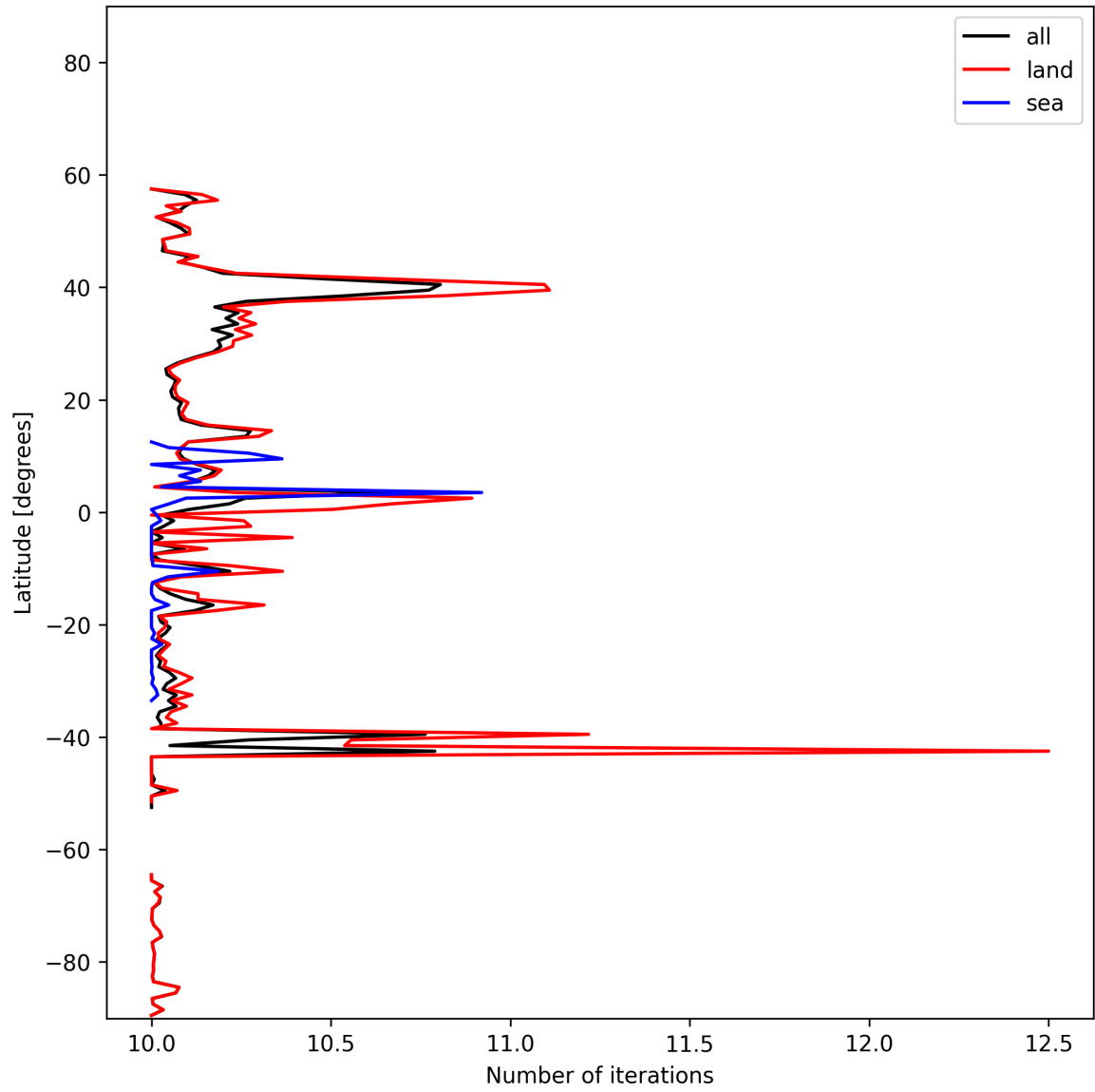
Figure 20: Zonal average of “Number of iterations” for 2025-11-09 to 2025-11-11.
