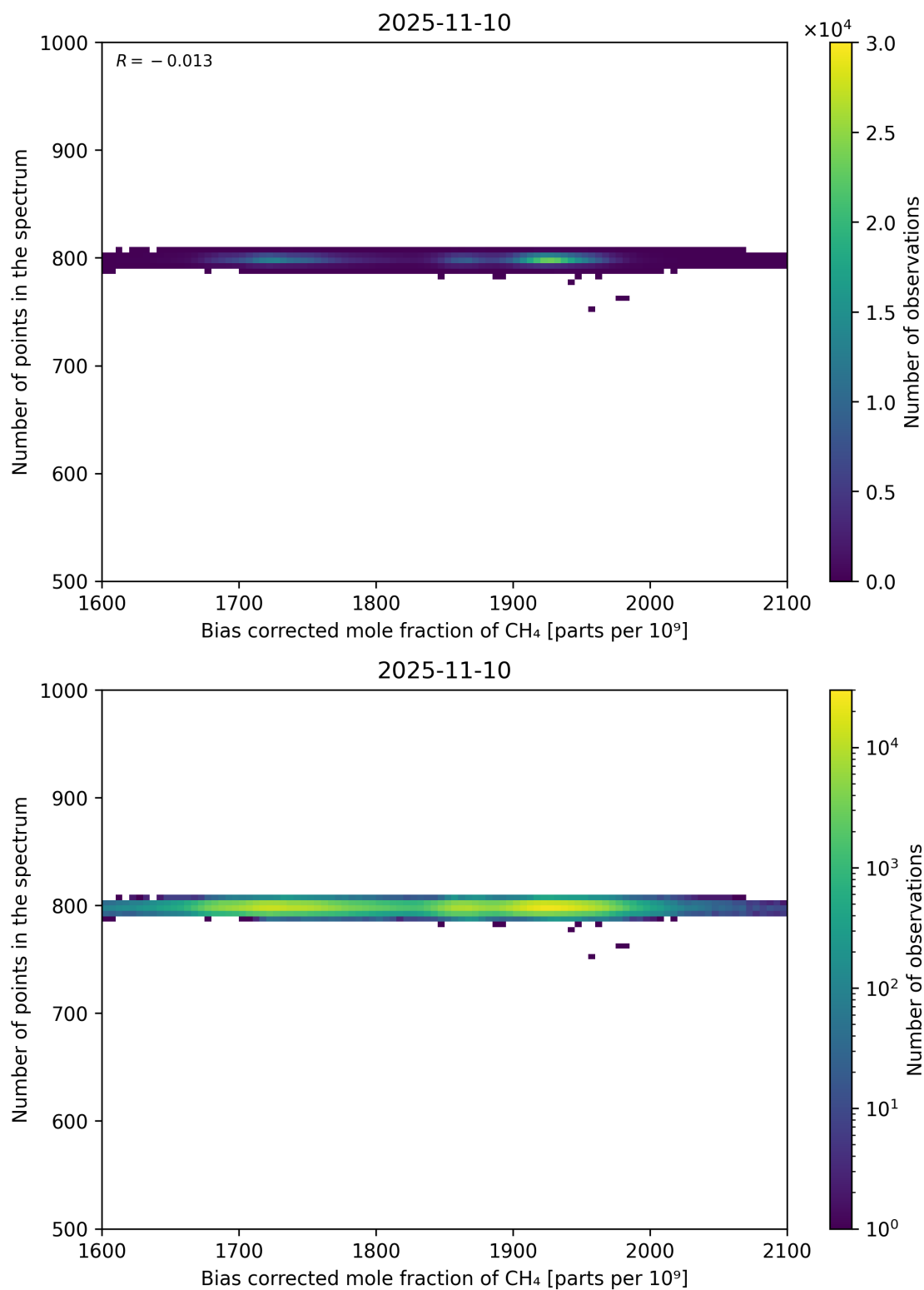
Figure 68: Scatter density plot of “Bias corrected mole fraction of CH 4 ” against “Number of points in the spectrum” for 2025-11-09 to 2025-11-11.
