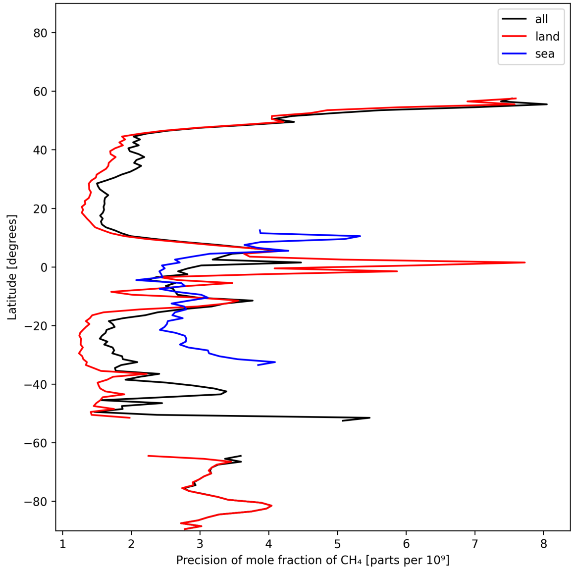
Figure 13: Zonal average of “Precision of mole fraction of CH 4 ” for 2025-11-09 to 2025-11-11.
