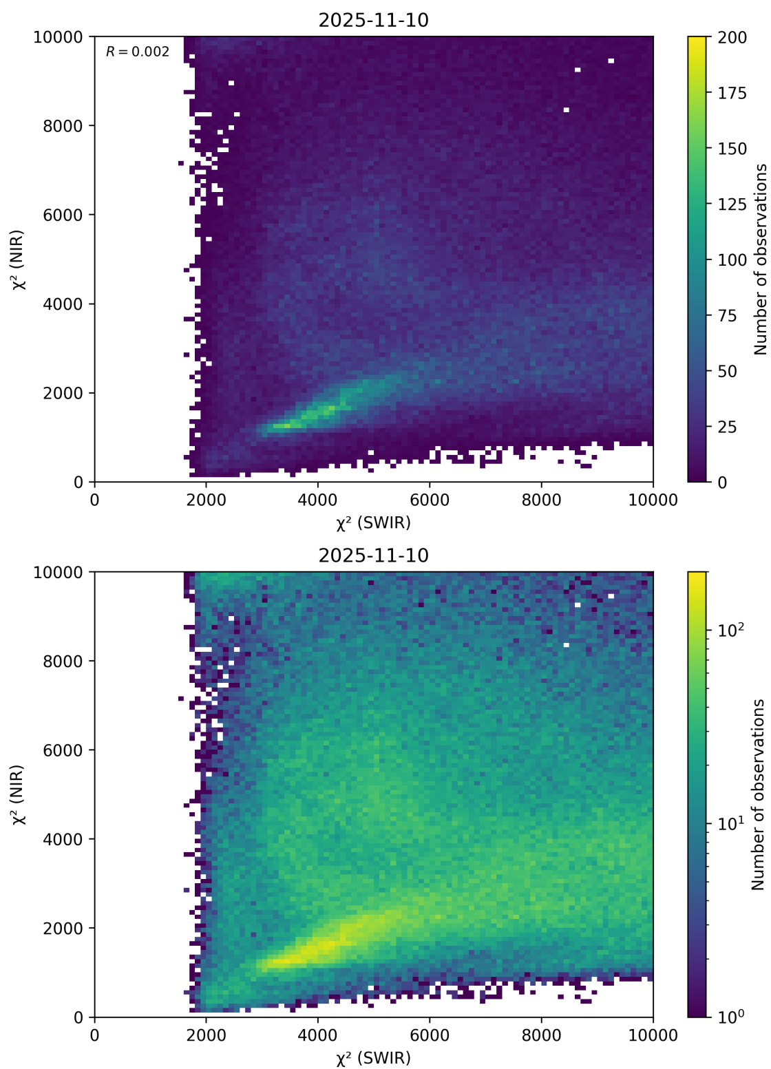
Figure 47: Scatter density plot of “ \chi^2 (SWIR)” against “ \chi^2 (NIR)” for 2025-11-09 to 2025-11-11.
