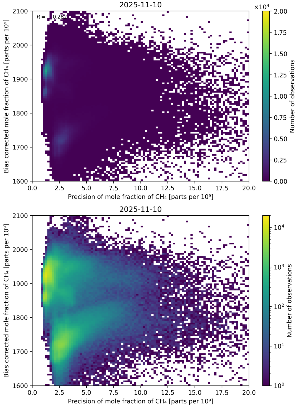
Figure 82: Scatter density plot of “Precision of mole fraction of CH 4 ” against “Bias corrected mole fraction of CH 4 ” for 2025-11-09 to 2025-11-11.
