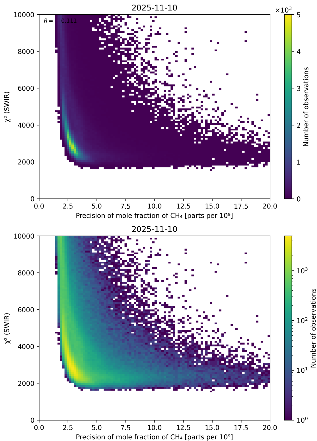
Figure 79: Scatter density plot of “Precision of mole fraction of \text{CH}_4 ” against “ \chi^2 (SWIR)” for 2025-11-09 to 2025-11-11.
