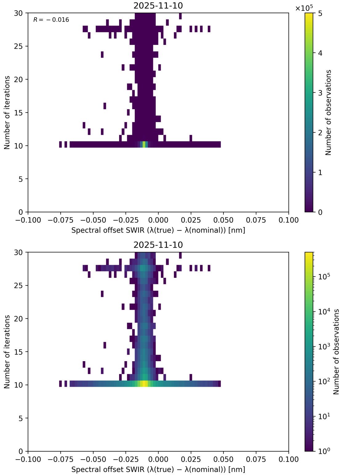
Figure 121: Scatter density plot of “Spectral offset SWIR ( \lambda_{\text{true}} - \lambda_{\text{nominal}} )” against “Number of iterations” for 2025-11-09 to 2025-11-11.
