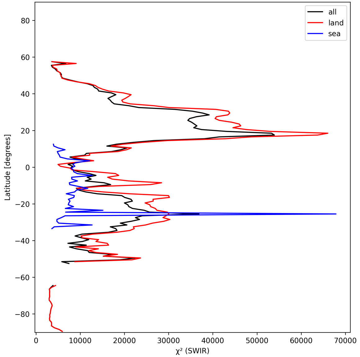
Figure 17: Zonal average of “ \chi^2 (SWIR)” for 2025-11-09 to 2025-11-11.
