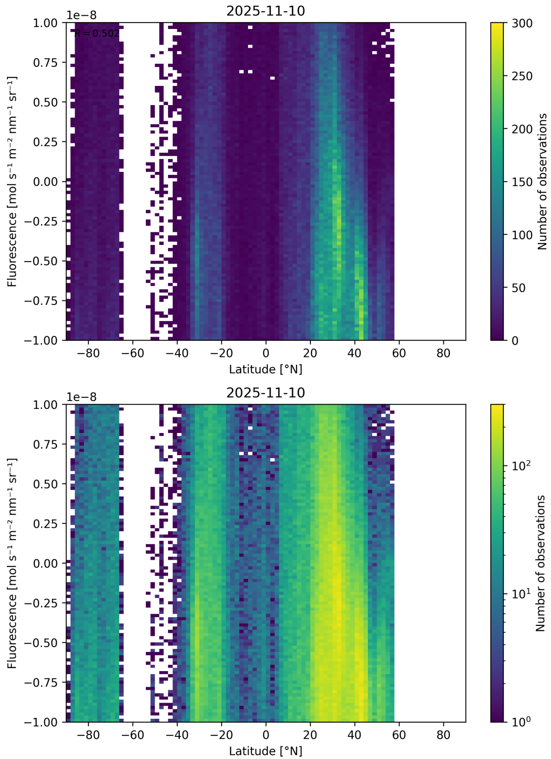
Figure 56: Scatter density plot of “Latitude” against “Fluorescence” for 2025-11-09 to 2025-11-11.
