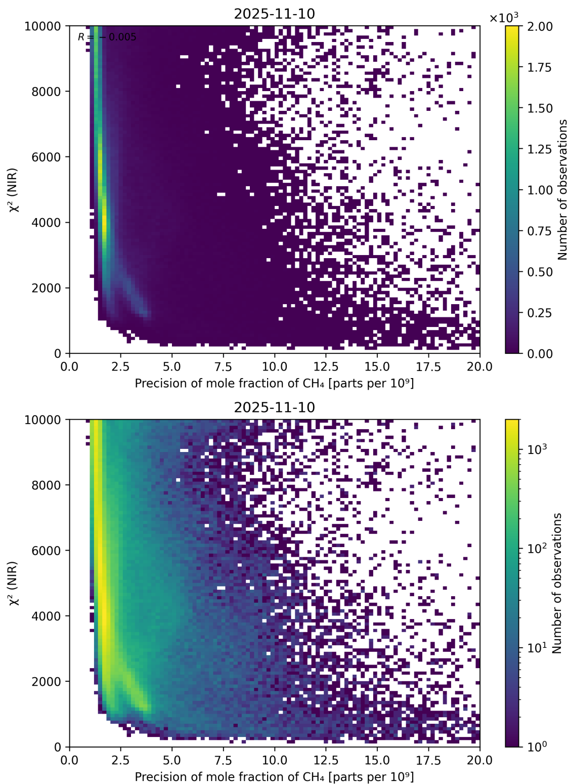
Figure 78: Scatter density plot of “Precision of mole fraction of CH 4 ” against “ \chi^2 (NIR)” for 2025-11-09 to 2025-11-11.
