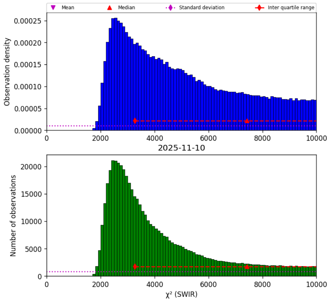
Figure 28: Histogram of “ \chi^2 (SWIR)” for 2025-11-09 to 2025-11-11
