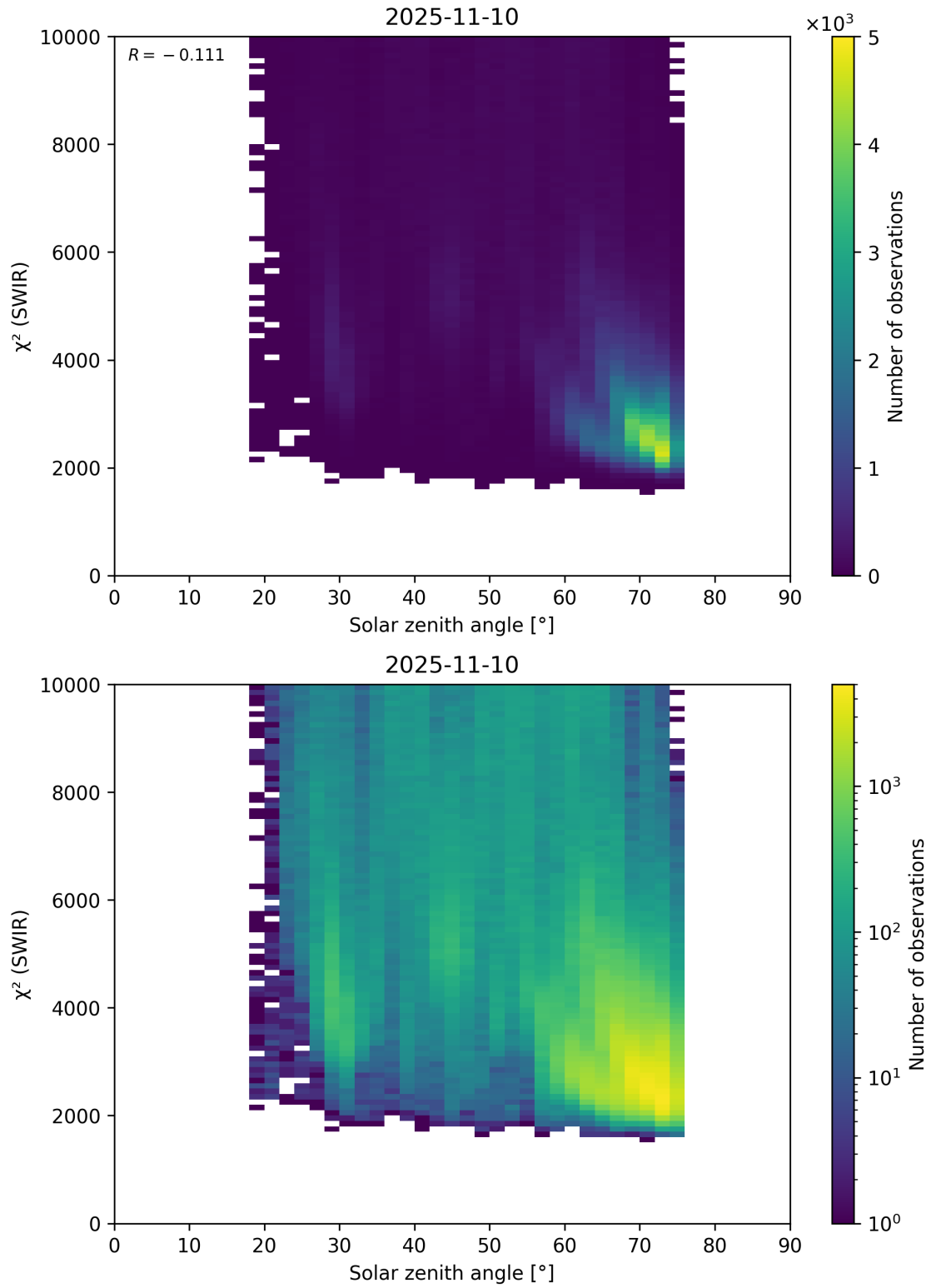
Figure 95: Scatter density plot of “Solar zenith angle” against “ \chi^2 (SWIR)” for 2025-11-09 to 2025-11-11.
