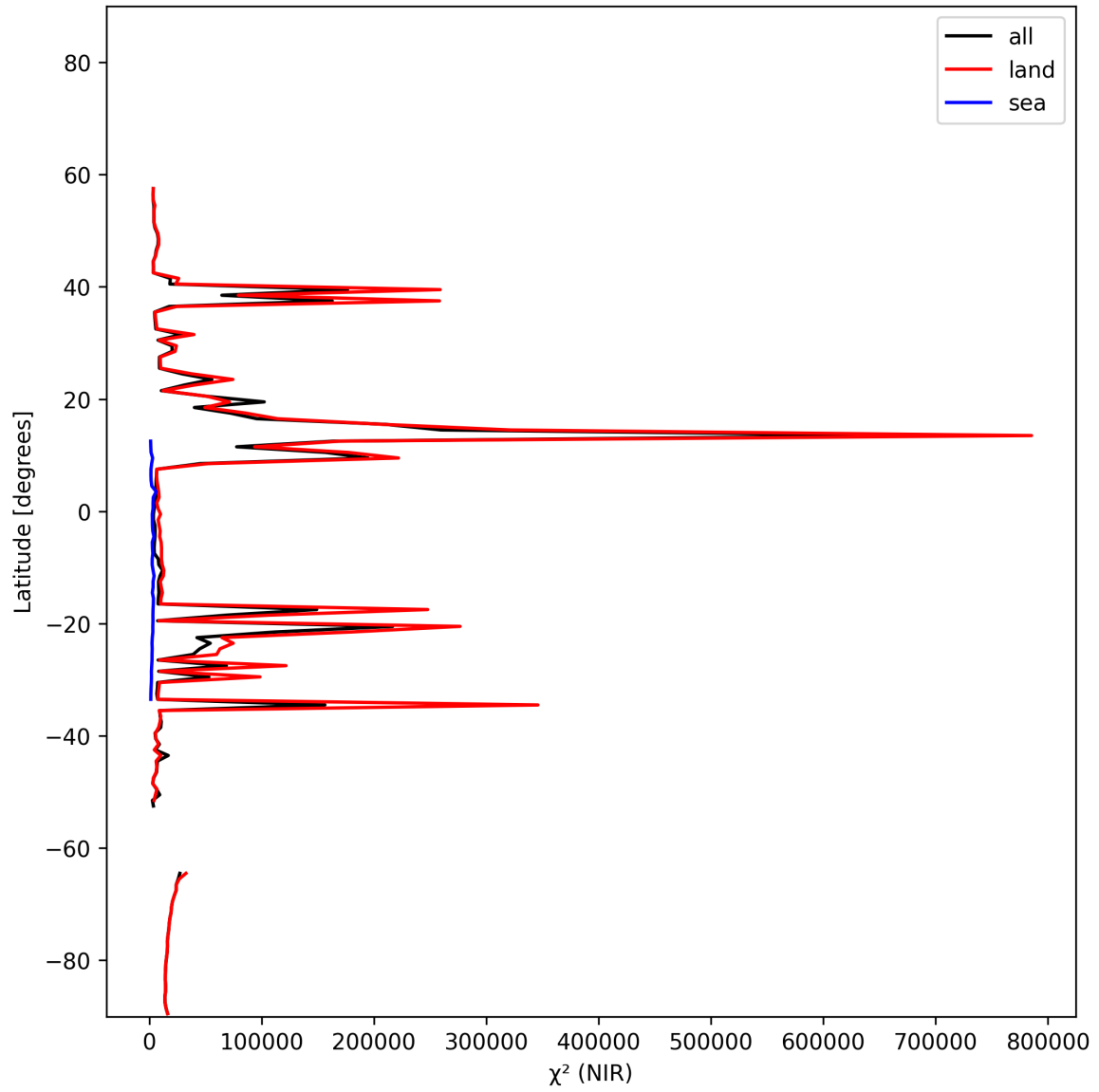
Figure 18: Zonal average of “ \chi^2 (NIR)” for 2025-11-09 to 2025-11-11.
