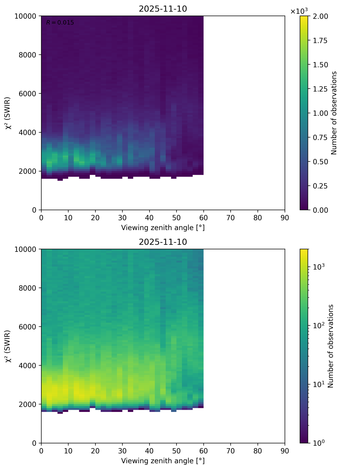
Figure 106: Scatter density plot of “Viewing zenith angle” against “ \chi^2 (SWIR)” for 2025-11-09 to 2025-11-11.
