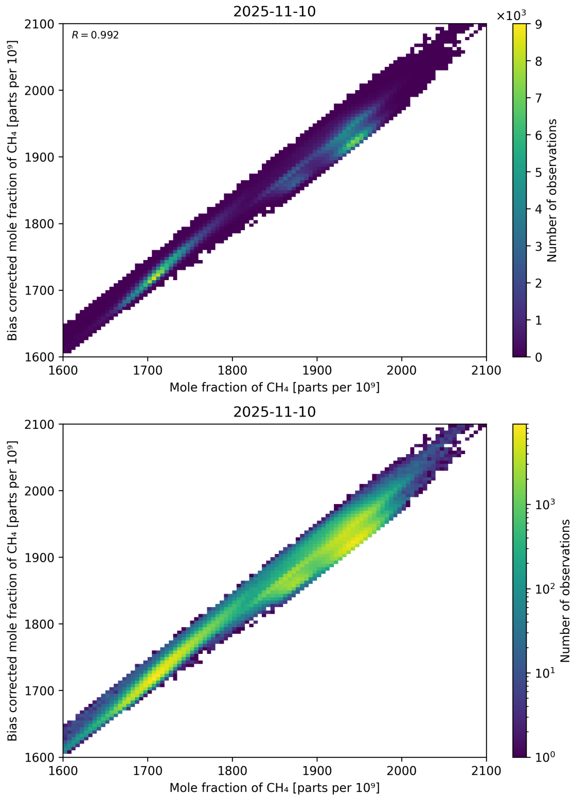
Figure 74: Scatter density plot of “Mole fraction of CH 4 ” against “Bias corrected mole fraction of CH 4 ” for 2025-11-09 to 2025-11-11.
