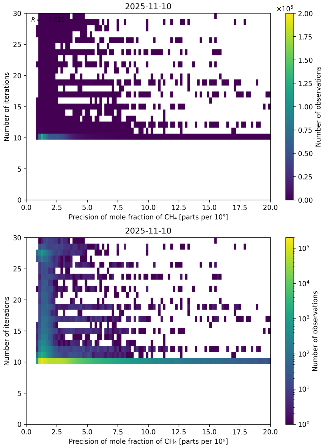
Figure 83: Scatter density plot of “Precision of mole fraction of \text{CH}_4 ” against “Number of iterations” for 2025-11-09 to 2025-11-11.
