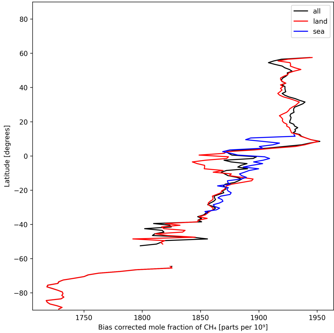
Figure 14: Zonal average of “Bias corrected mole fraction of CH 4 ” for 2025-11-09 to 2025-11-11.
