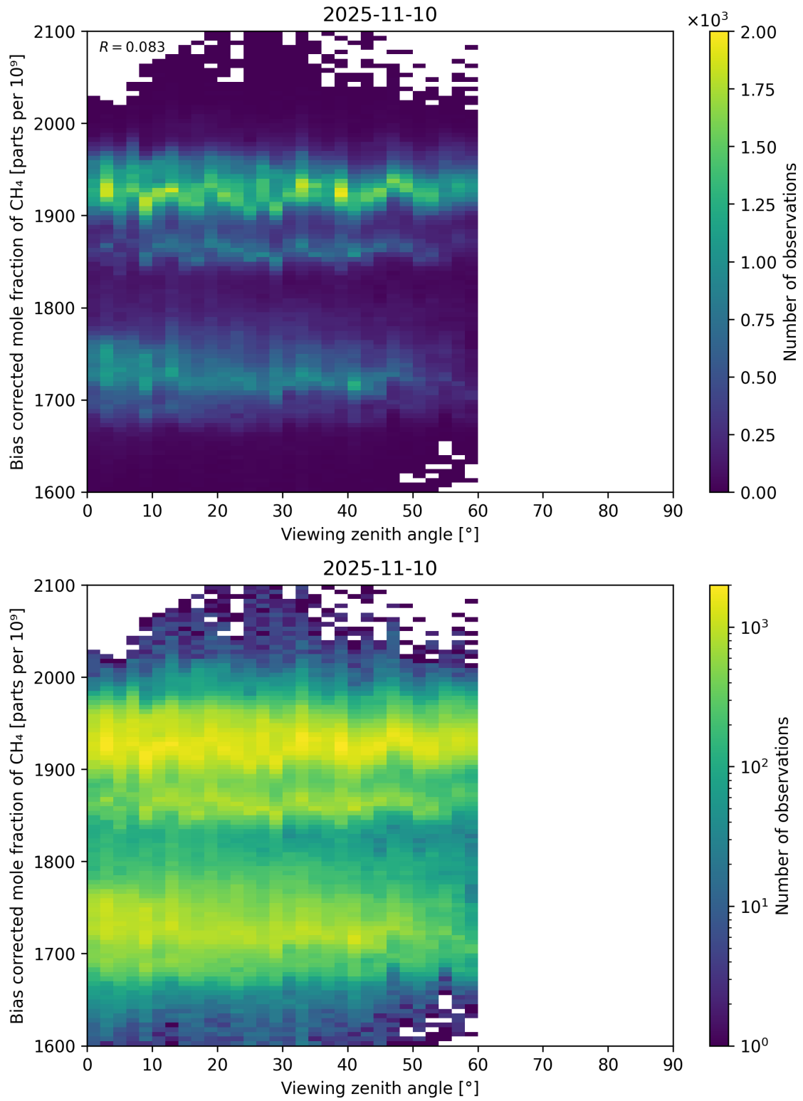
Figure 111: Scatter density plot of “Viewing zenith angle” against “Bias corrected mole fraction of CH 4 ” for 2025-11-09 to 2025-11-11.
