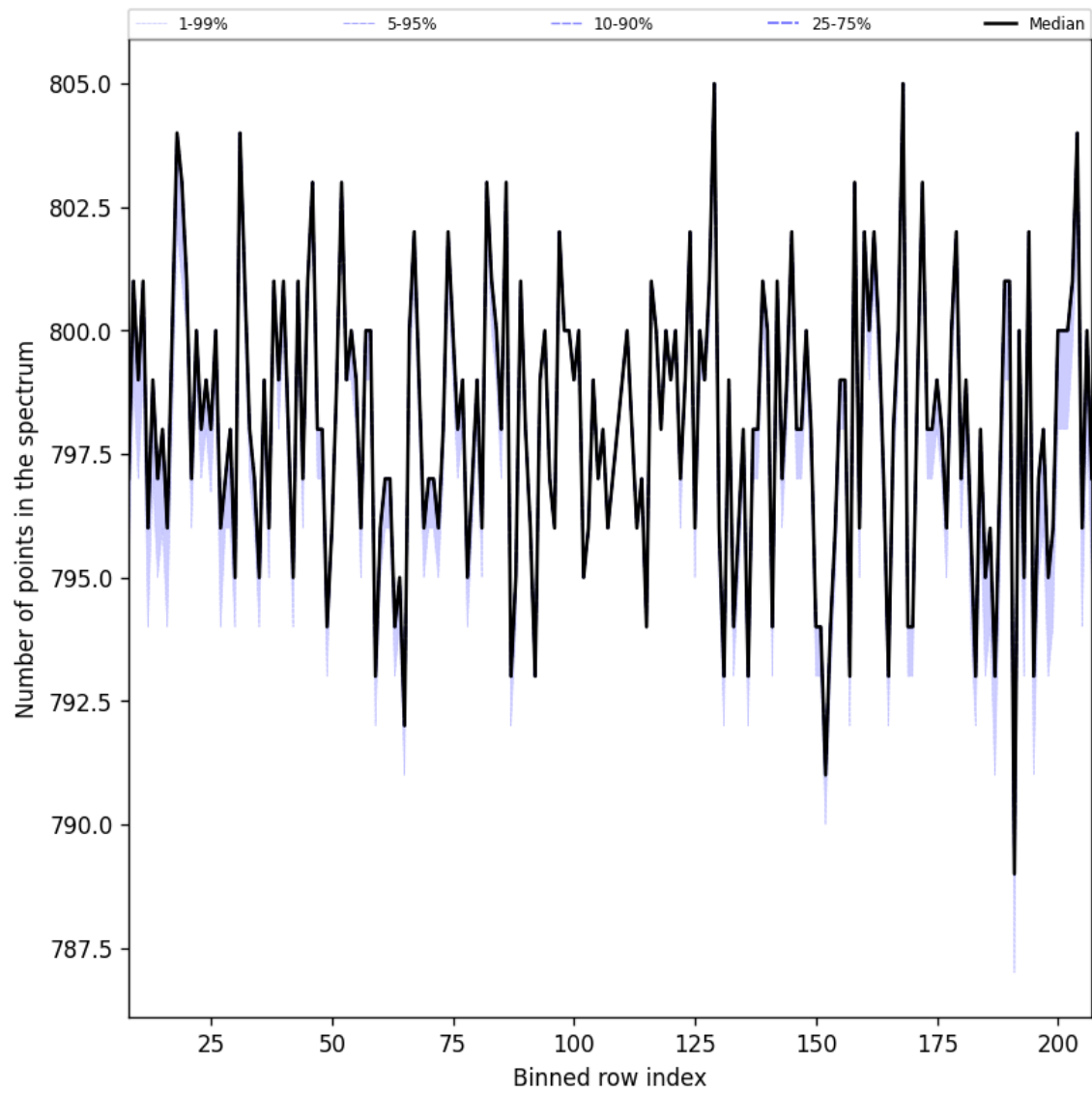
Figure 37: Along track statistics of “Number of points in the spectrum” for 2025-11-09 to 2025-11-11
