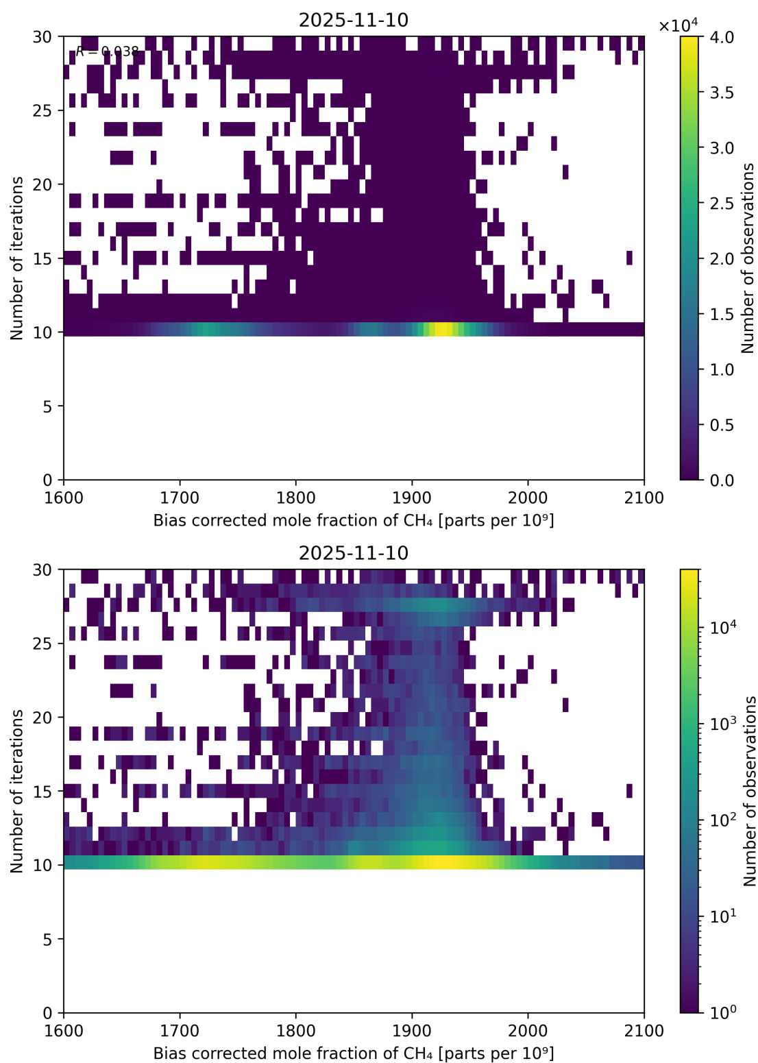
Figure 67: Scatter density plot of “Bias corrected mole fraction of \text{CH}_4 ” against “Number of iterations” for 2025-11-09 to 2025-11-11.
