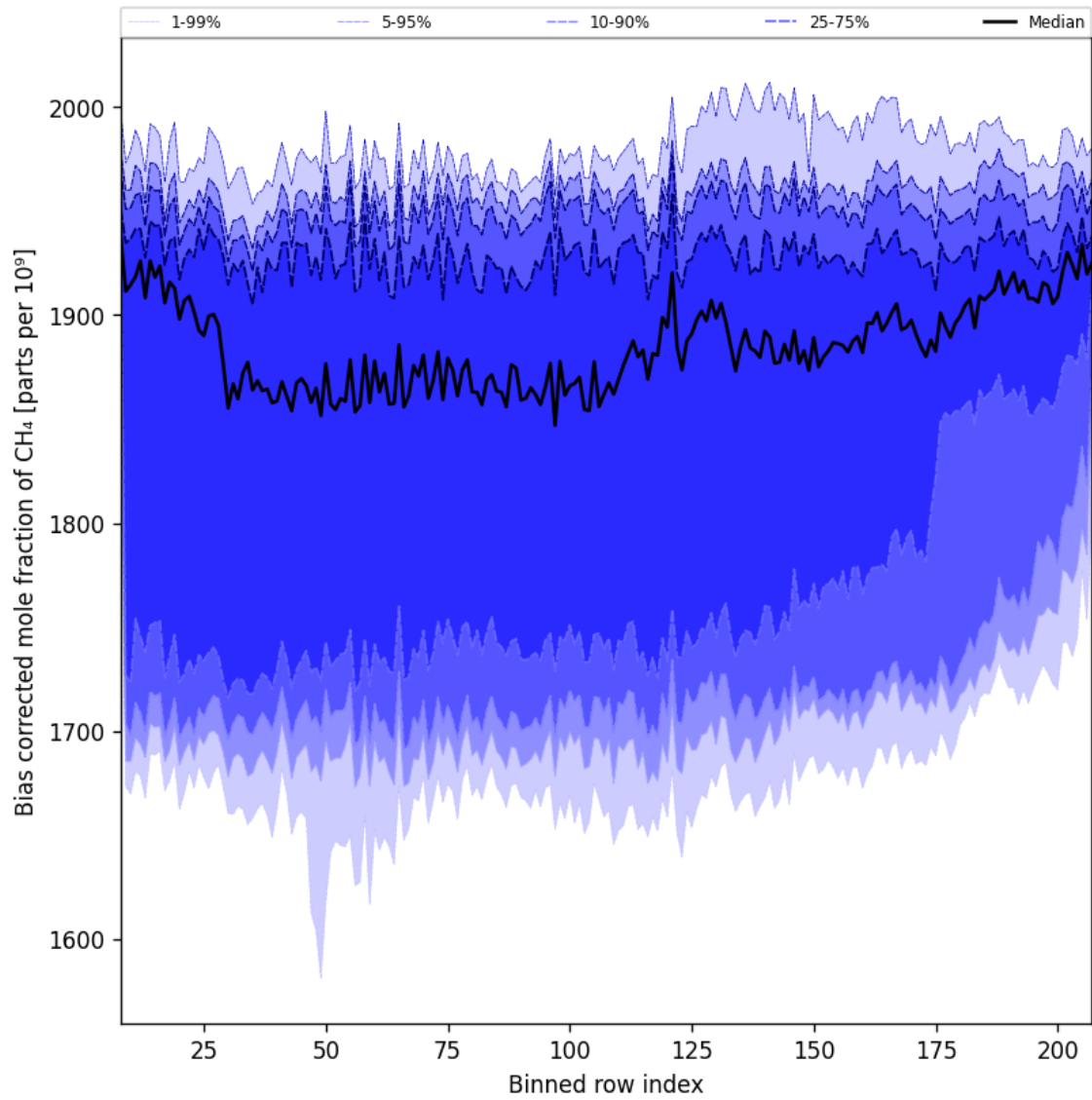
Figure 36: Along track statistics of “Bias corrected mole fraction of CH 4 ” for 2025-11-09 to 2025-11-11
