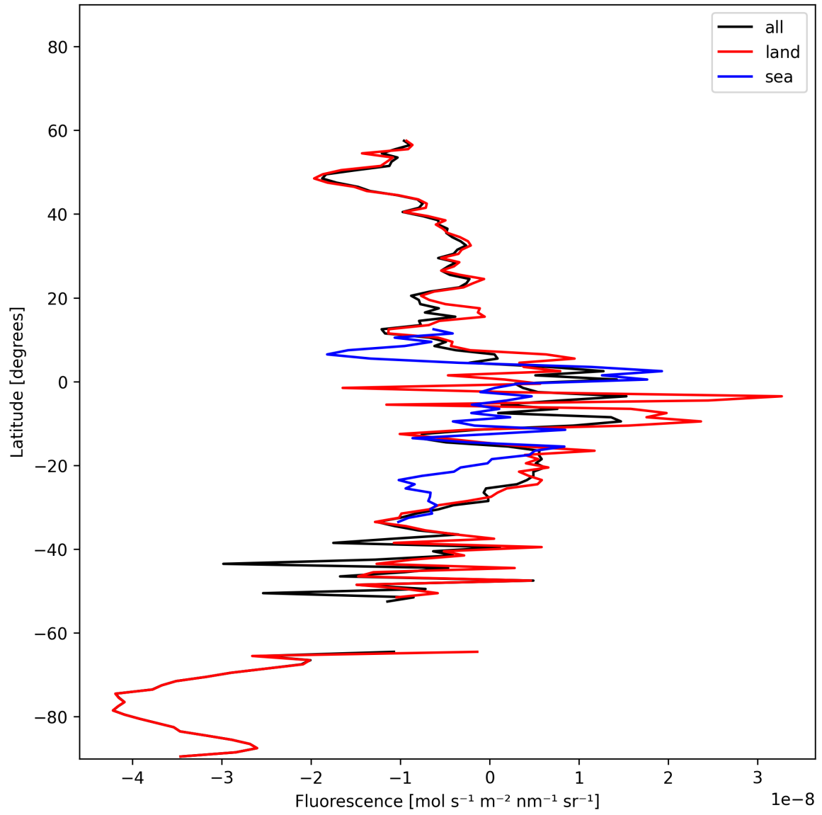
Figure 21: Zonal average of “Fluorescence” for 2025-11-09 to 2025-11-11.
