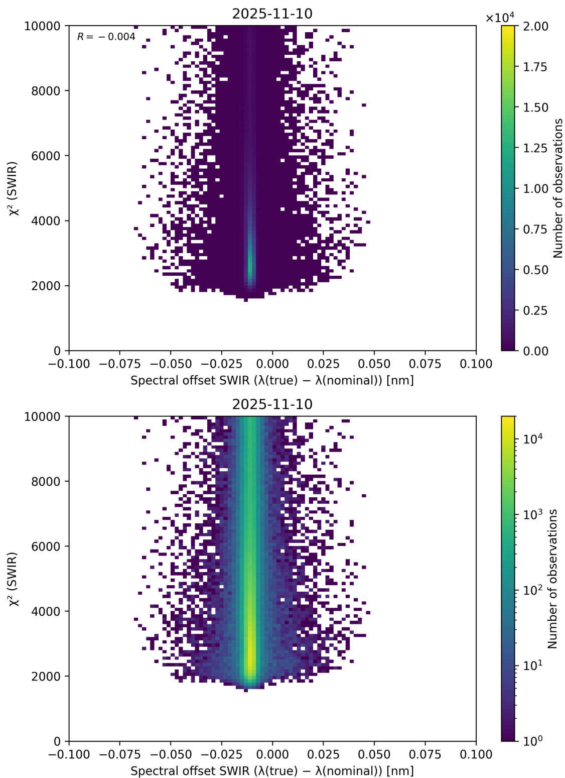
Figure 118: Scatter density plot of “Spectral offset SWIR ( \lambda_{\text{true}} - \lambda_{\text{nominal}} )” against “ \chi^2 (SWIR)” for 2025-11-09 to 2025-11-11.
