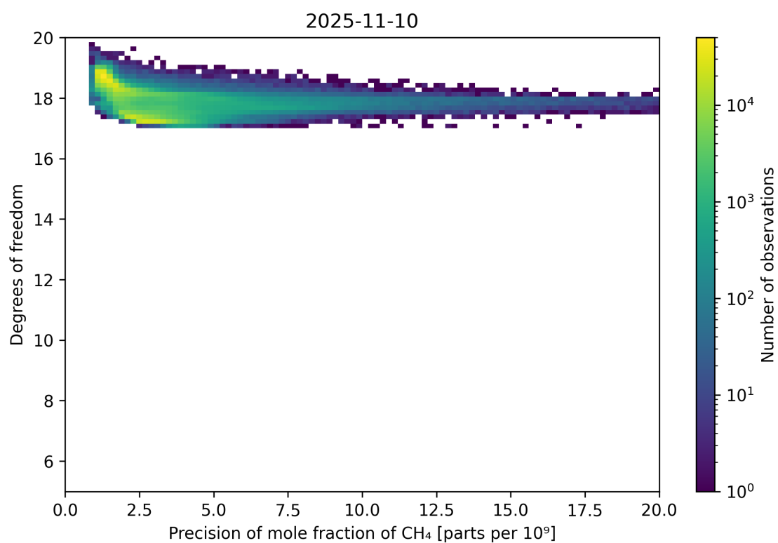
Figure 80: Scatter density plot of “Precision of mole fraction of CH 4 ” against “Degrees of freedom” for 2025-11-09 to 2025-11-11.
