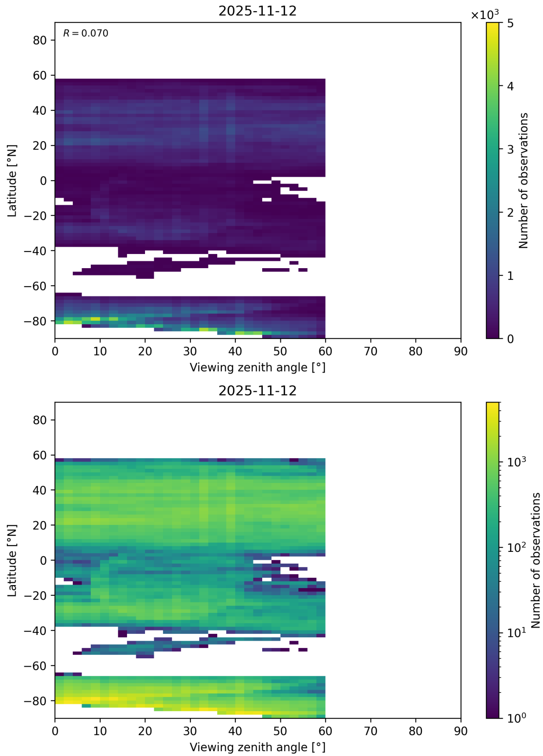
Figure 109: Scatter density plot of “Viewing zenith angle” against “Latitude” for 2025-11-12 to 2025-11-13.
