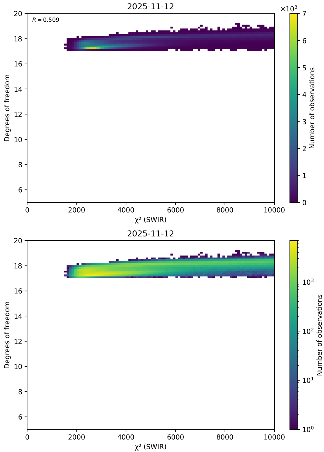
Figure 48: Scatter density plot of “ \chi^2 (SWIR)” against “Degrees of freedom” for 2025-11-12 to 2025-11-13.
