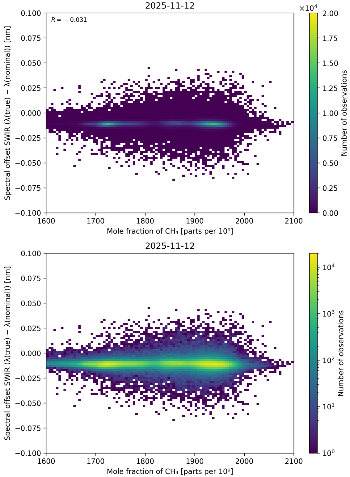
Figure 86: Scatter density plot of “Mole fraction of CH 4 ” against “Spectral offset SWIR ( \lambda_{\text{true}} - \lambda_{\text{nominal}} )” for 2025-11-12 to 2025-11-13.
