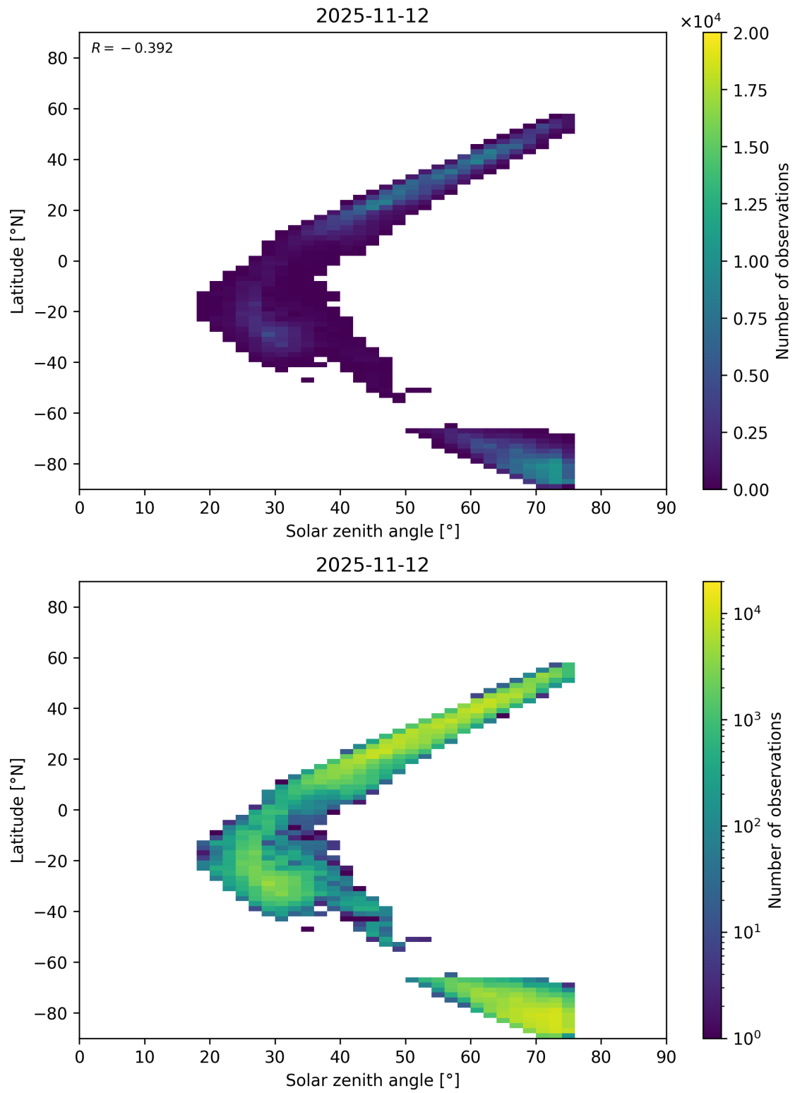
Figure 98: Scatter density plot of “Solar zenith angle” against “Latitude” for 2025-11-12 to 2025-11-13.
