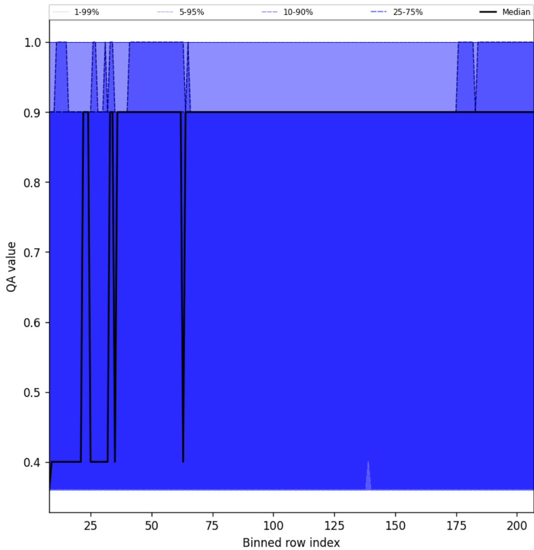
Figure 33: Along track statistics of “QA value” for 2025-11-12 to 2025-11-13
