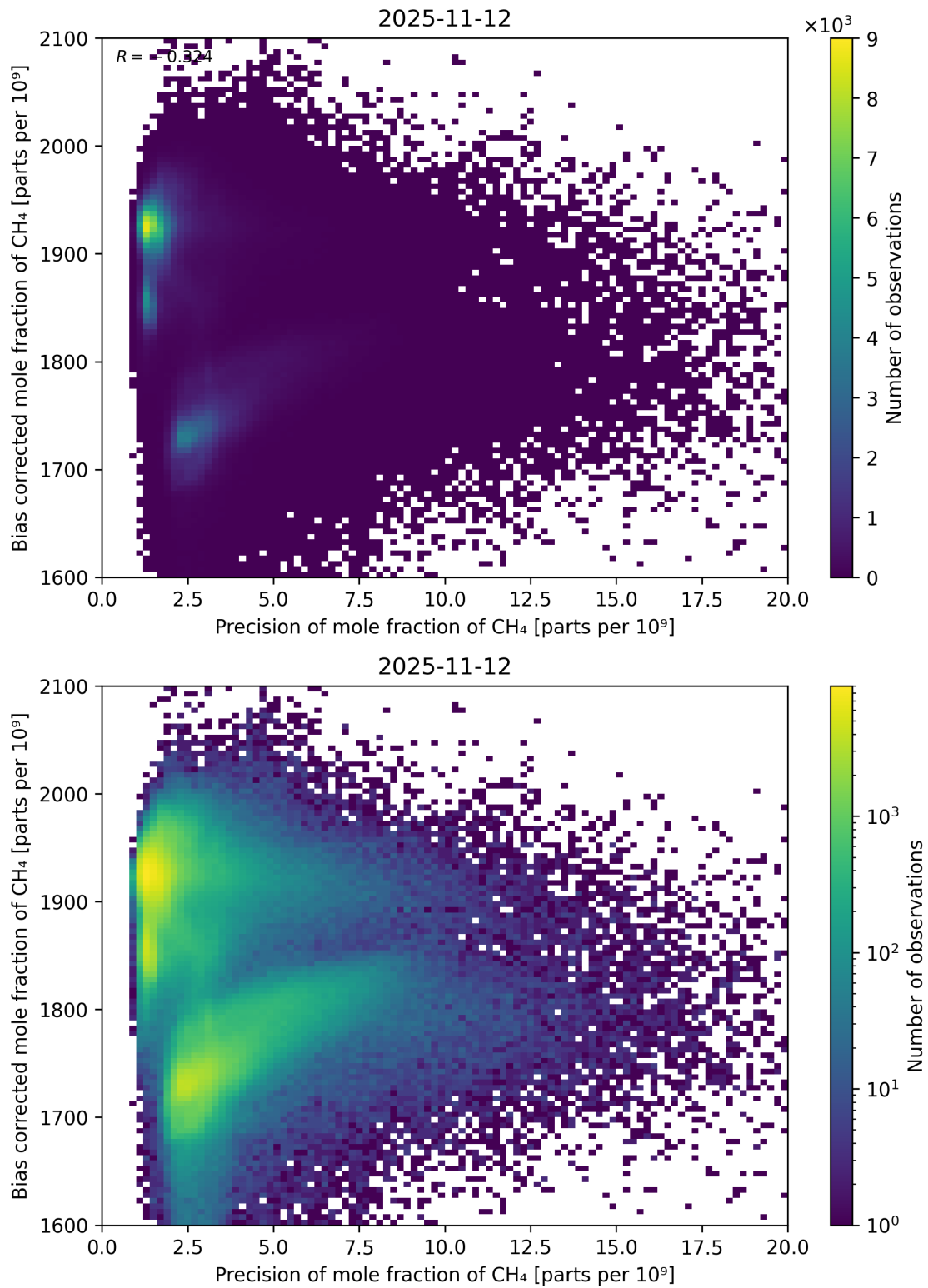
Figure 82: Scatter density plot of “Precision of mole fraction of \text{CH}_4 ” against “Bias corrected mole fraction of \text{CH}_4 ” for 2025-11-12 to 2025-11-13.
