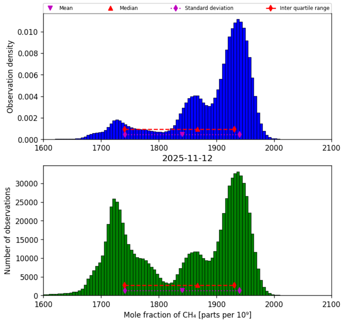
Figure 23: Histogram of “Mole fraction of CH 4 ” for 2025-11-12 to 2025-11-13
