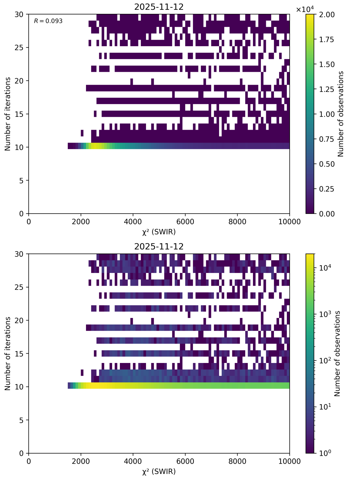
Figure 50: Scatter density plot of “ \chi^2 (SWIR)” against “Number of iterations” for 2025-11-12 to 2025-11-13.
