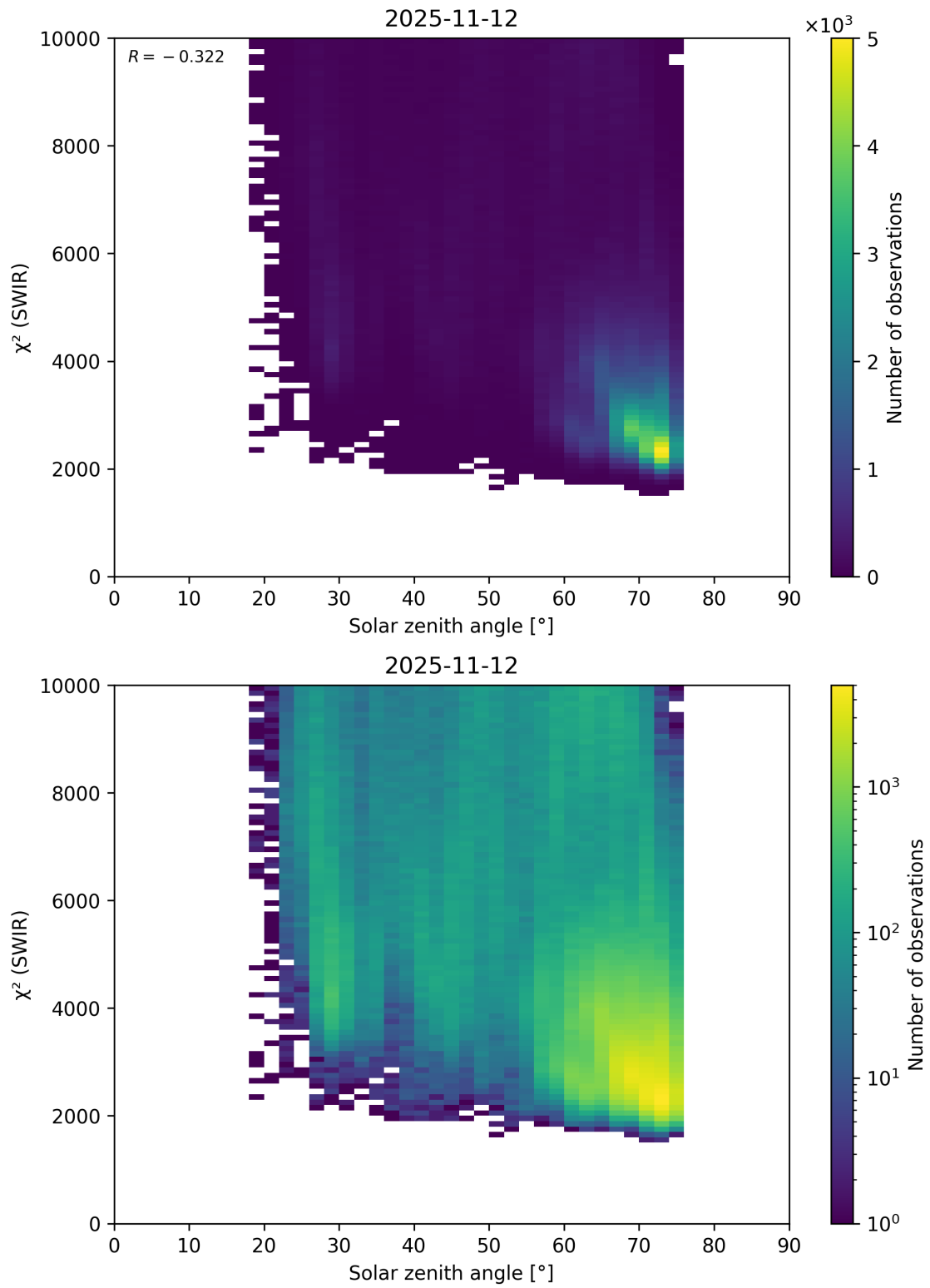
Figure 95: Scatter density plot of “Solar zenith angle” against “ \chi^2 (SWIR)” for 2025-11-12 to 2025-11-13.
