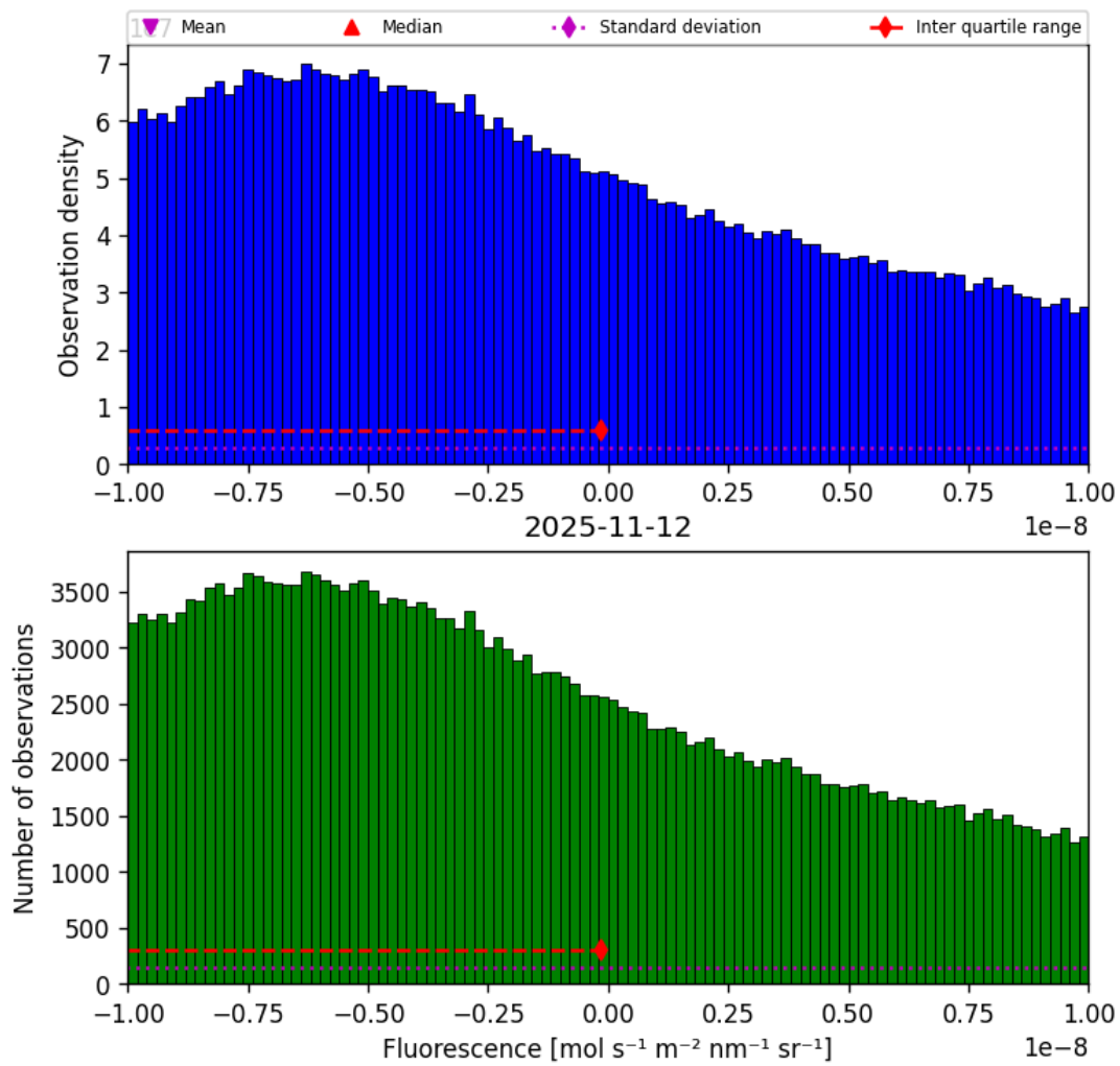
Figure 32: Histogram of “Fluorescence” for 2025-11-12 to 2025-11-13
