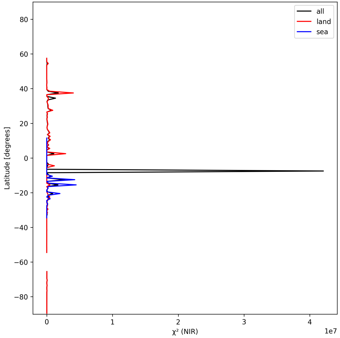
Figure 18: Zonal average of “ \chi^2 (NIR)” for 2025-11-12 to 2025-11-13.
