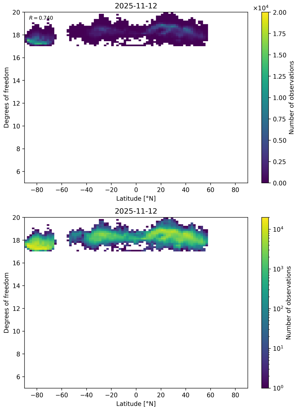
Figure 55: Scatter density plot of “Latitude” against “Degrees of freedom” for 2025-11-12 to 2025-11-13.
