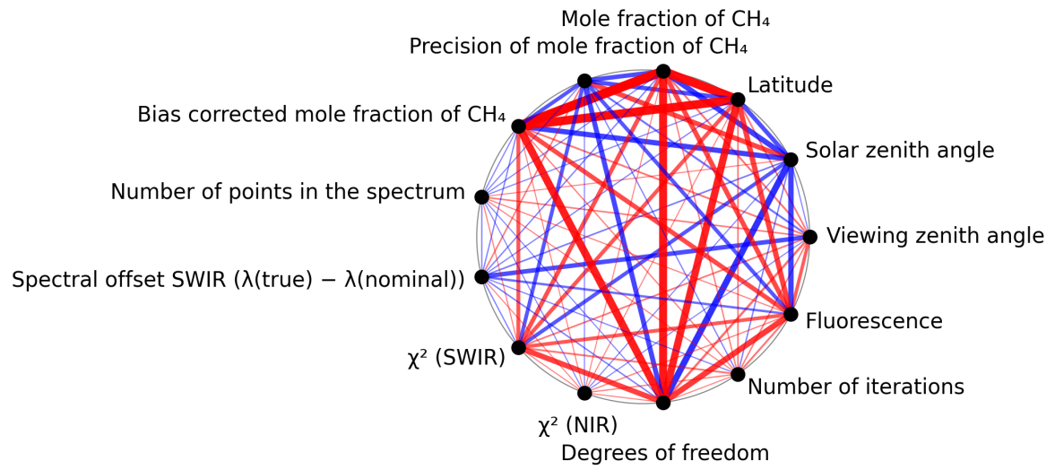
Figure 1: Map of correlation graph for 2025-11-12 to 2025-11-13.
