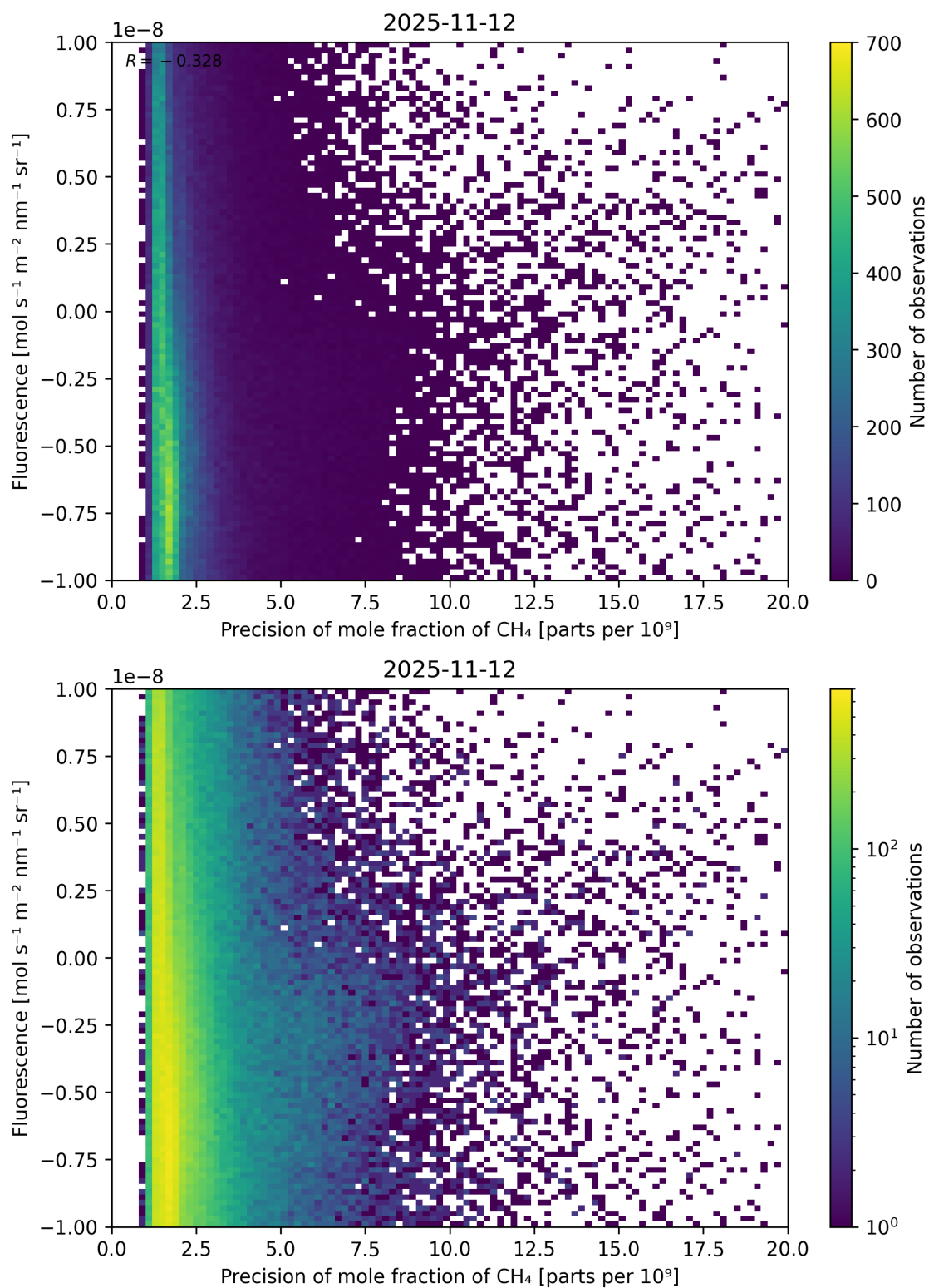
Figure 81: Scatter density plot of “Precision of mole fraction of CH 4 ” against “Fluorescence” for 2025-11-12 to 2025-11-13.
