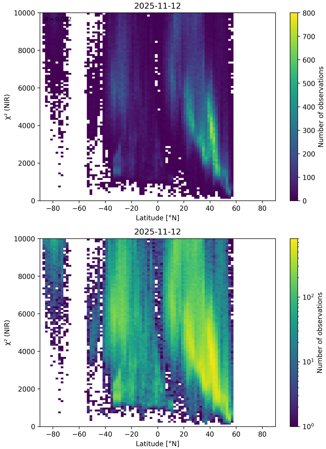
Figure 53: Scatter density plot of “Latitude” against “ \chi^2 (NIR)” for 2025-11-12 to 2025-11-13.
