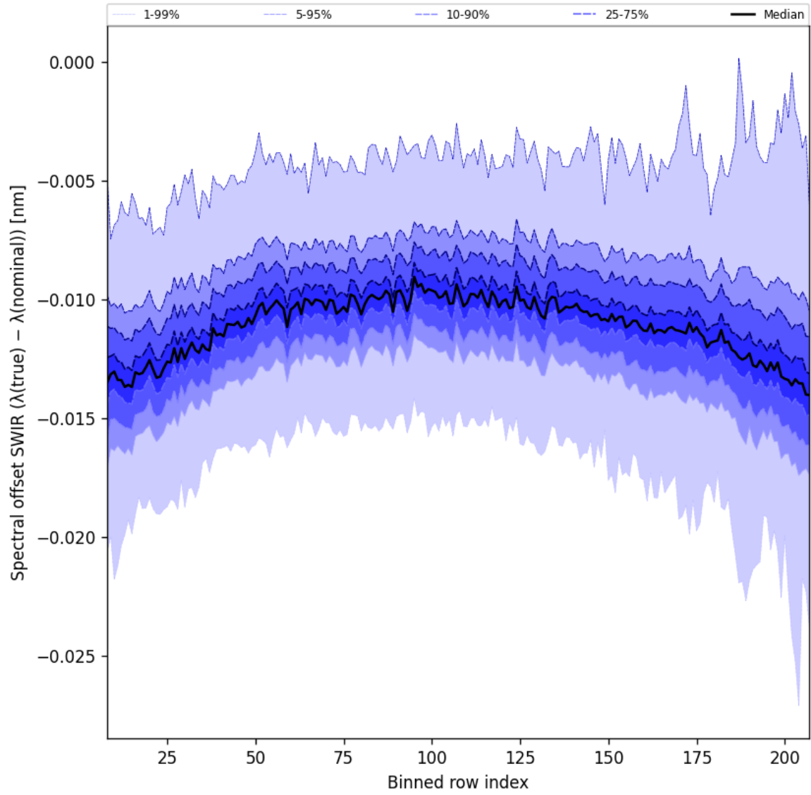
Figure 38: Along track statistics of “Spectral offset SWIR ( \lambda_{\text{true}} - \lambda_{\text{nominal}} )” for 2025-11-12 to 2025-11-13
