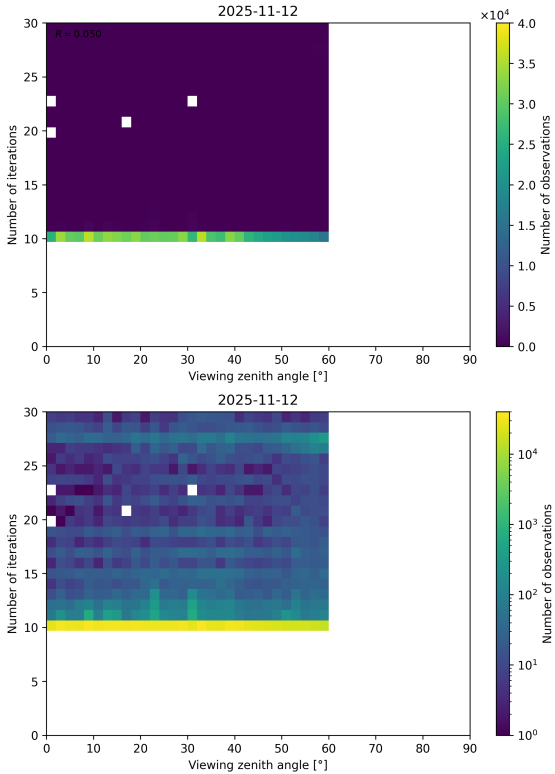
Figure 113: Scatter density plot of “Viewing zenith angle” against “Number of iterations” for 2025-11-12 to 2025-11-13.
