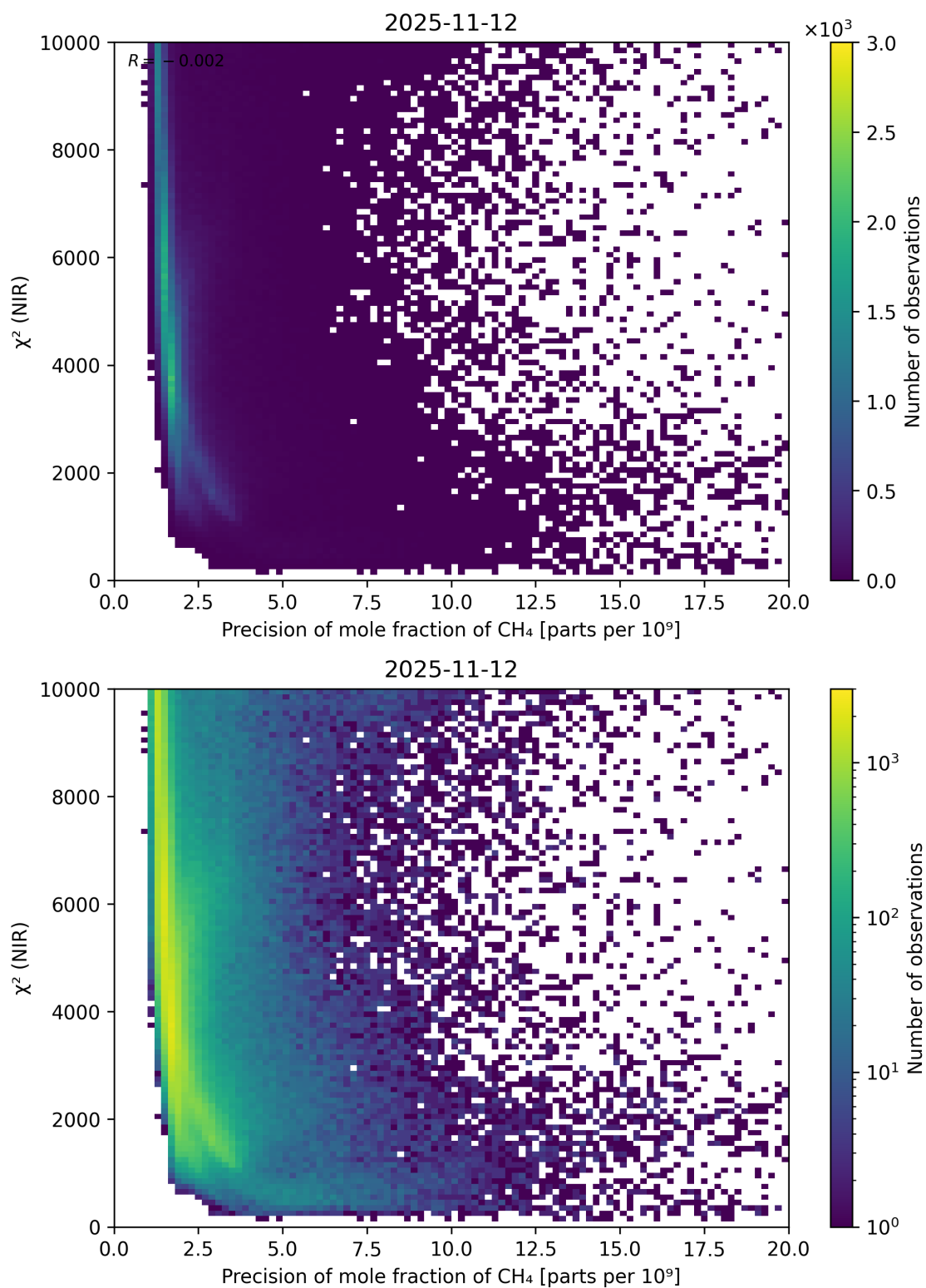
Figure 78: Scatter density plot of “Precision of mole fraction of CH 4 ” against “ \chi^2 (NIR)” for 2025-11-12 to 2025-11-13.
