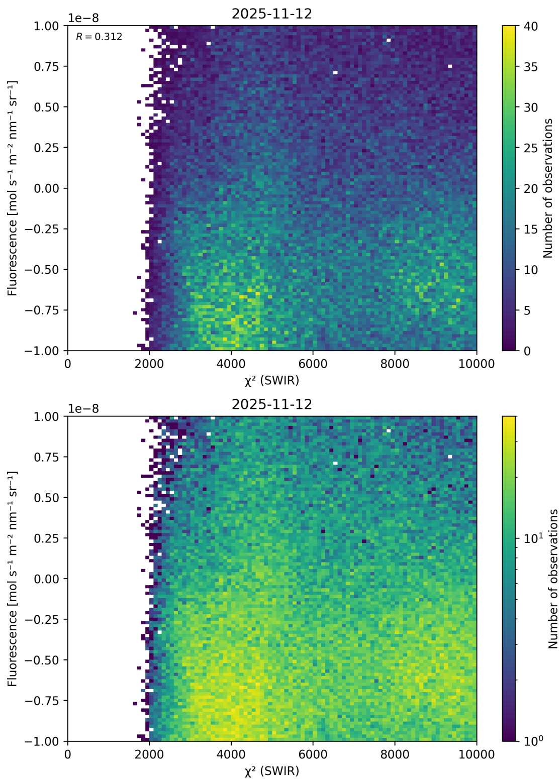
Figure 49: Scatter density plot of “ \chi^2 (SWIR)” against “Fluorescence” for 2025-11-12 to 2025-11-13.
