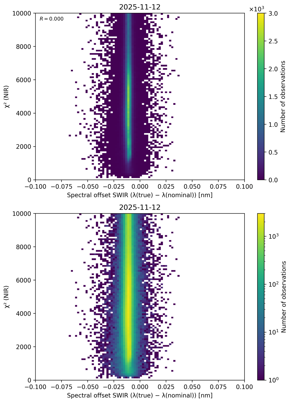
Figure 117: Scatter density plot of “Spectral offset SWIR ( \lambda_{\text{true}} - \lambda_{\text{nominal}} )” against “ \chi^2 (NIR)” for 2025-11-12 to 2025-11-13.
