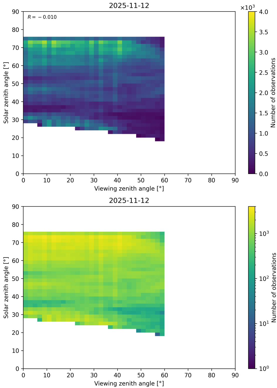
Figure 115: Scatter density plot of “Viewing zenith angle” against “Solar zenith angle” for 2025-11-12 to 2025-11-13.
