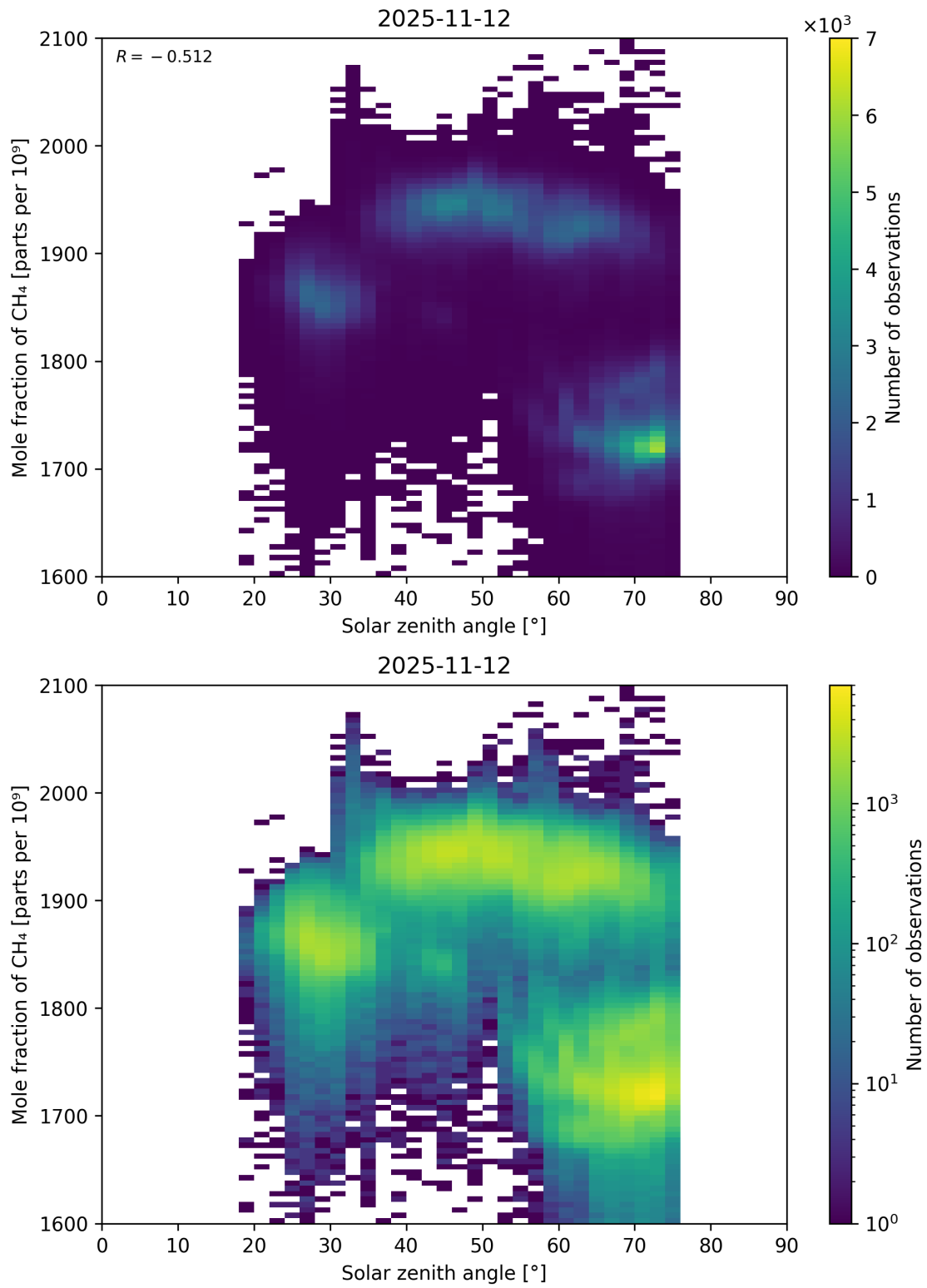
Figure 99: Scatter density plot of “Solar zenith angle” against “Mole fraction of CH 4 ” for 2025-11-12 to 2025-11-13.
