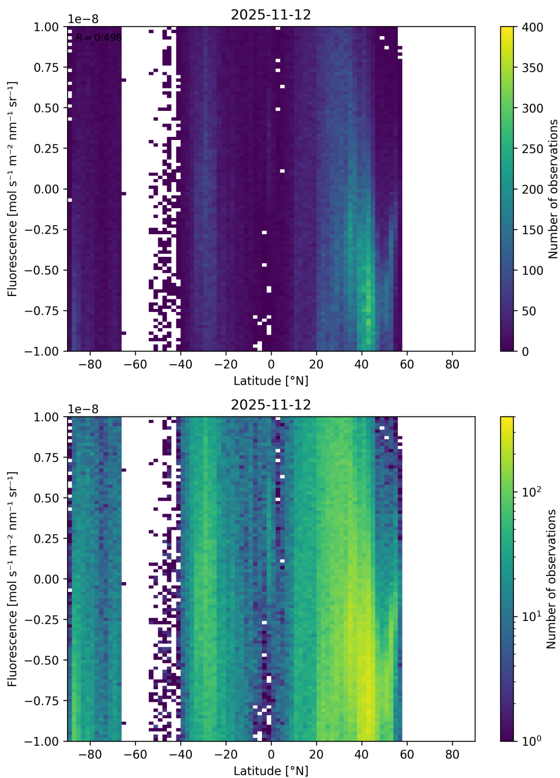
Figure 56: Scatter density plot of “Latitude” against “Fluorescence” for 2025-11-12 to 2025-11-13.
