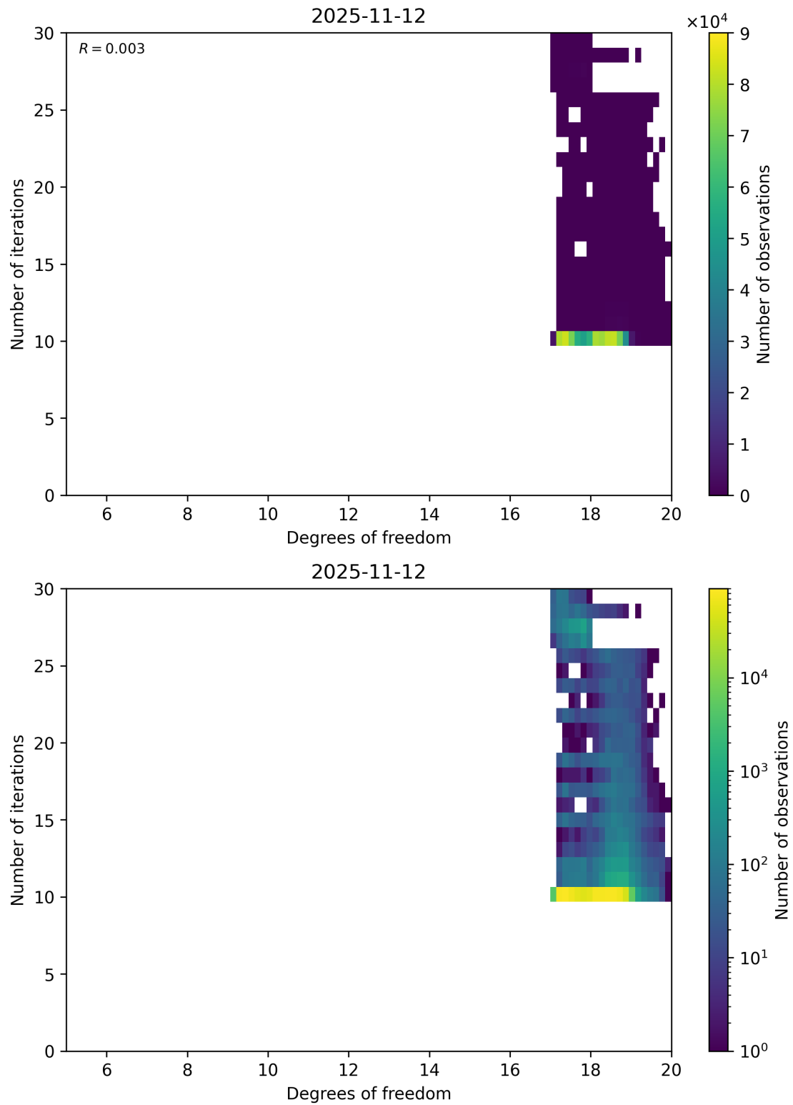
Figure 52: Scatter density plot of “Degrees of freedom” against “Number of iterations” for 2025-11-12 to 2025-11-13.
