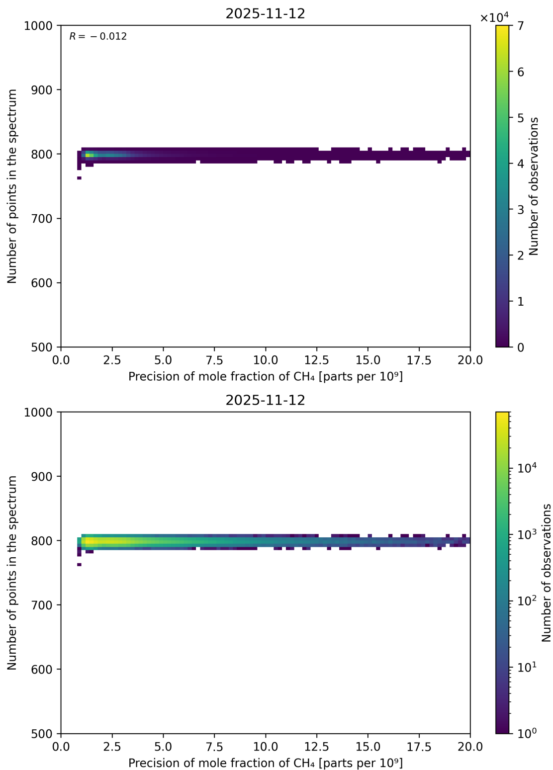
Figure 84: Scatter density plot of “Precision of mole fraction of CH 4 ” against “Number of points in the spectrum” for 2025-11-12 to 2025-11-13.
