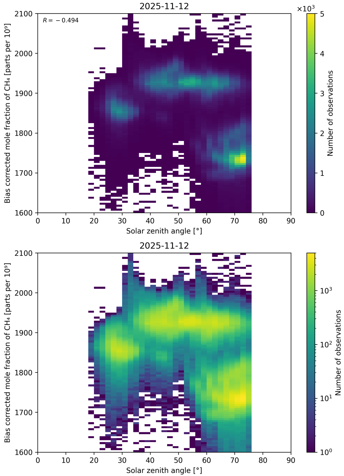
Figure 100: Scatter density plot of “Solar zenith angle” against “Bias corrected mole fraction of CH 4 ” for 2025-11-12 to 2025-11-13.
