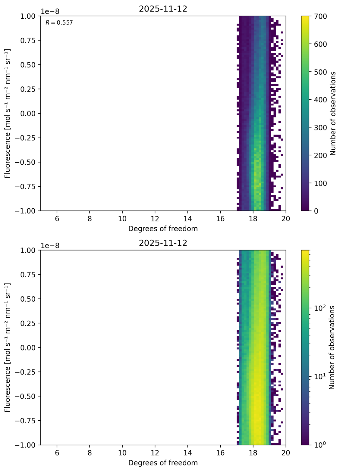
Figure 51: Scatter density plot of “Degrees of freedom” against “Fluorescence” for 2025-11-12 to 2025-11-13.
