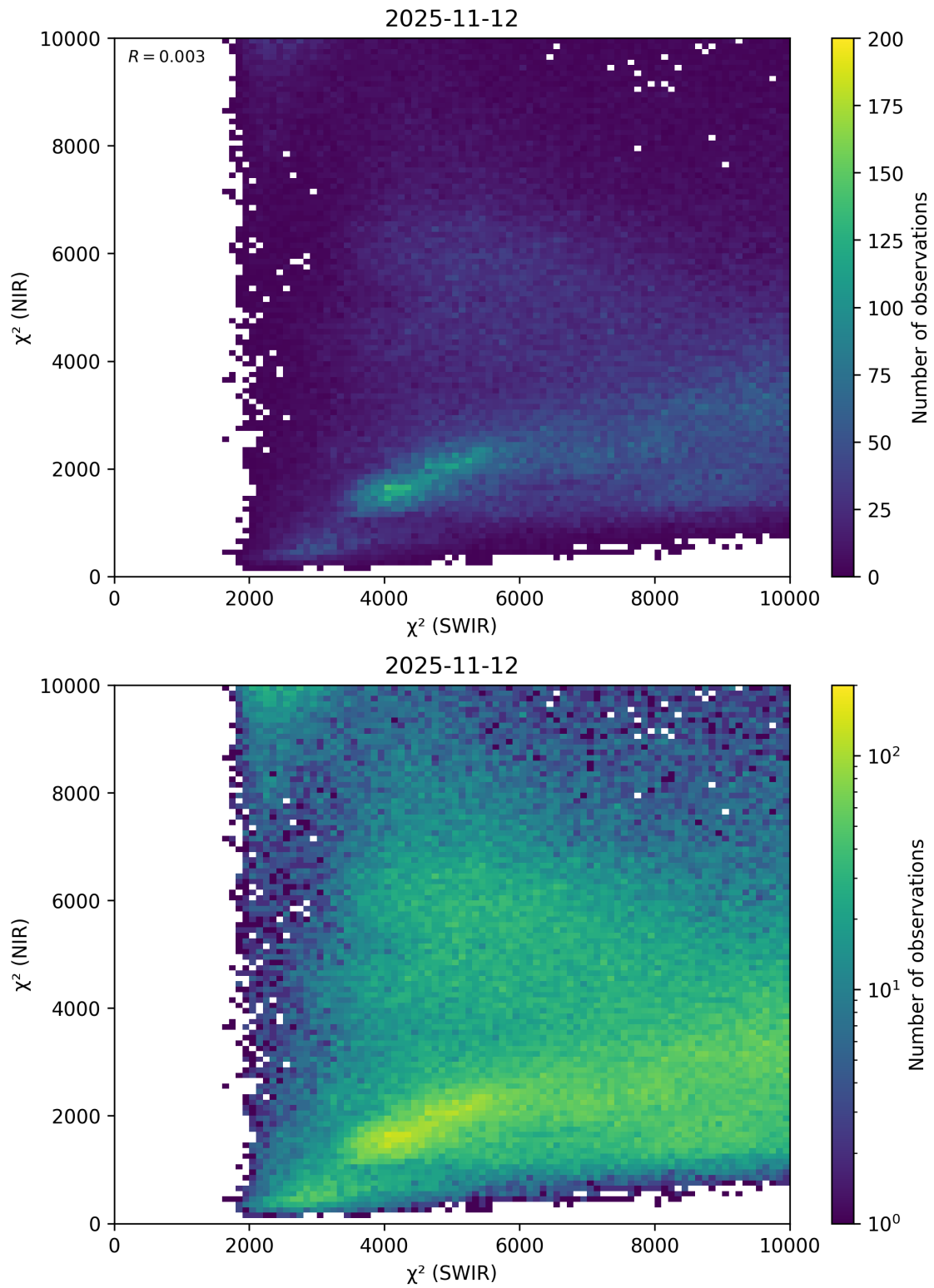
Figure 47: Scatter density plot of “ \chi^2 (SWIR)” against “ \chi^2 (NIR)” for 2025-11-12 to 2025-11-13.
