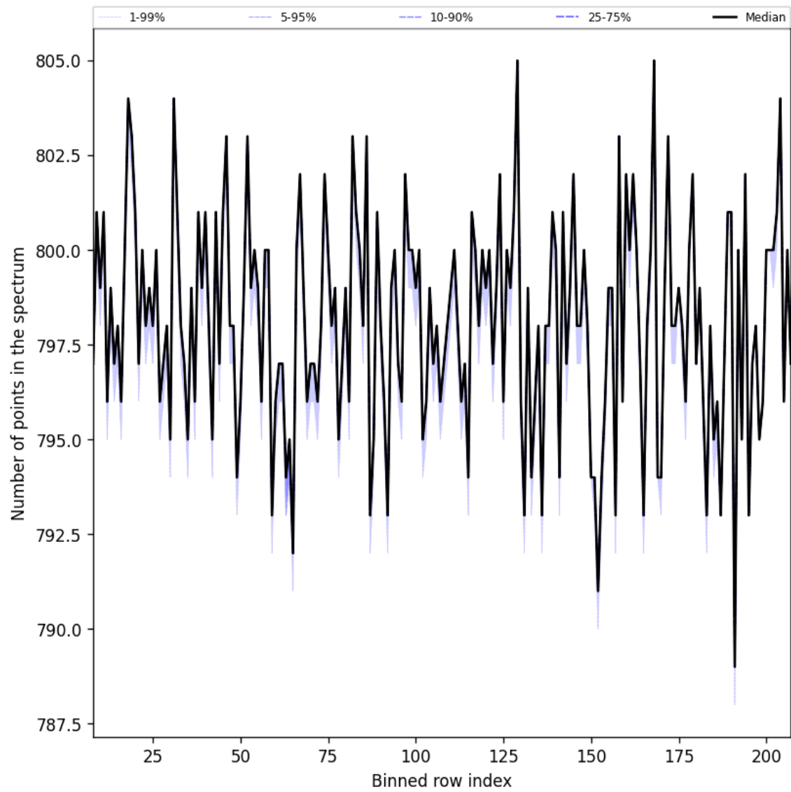
Figure 37: Along track statistics of “Number of points in the spectrum” for 2025-11-12 to 2025-11-13
