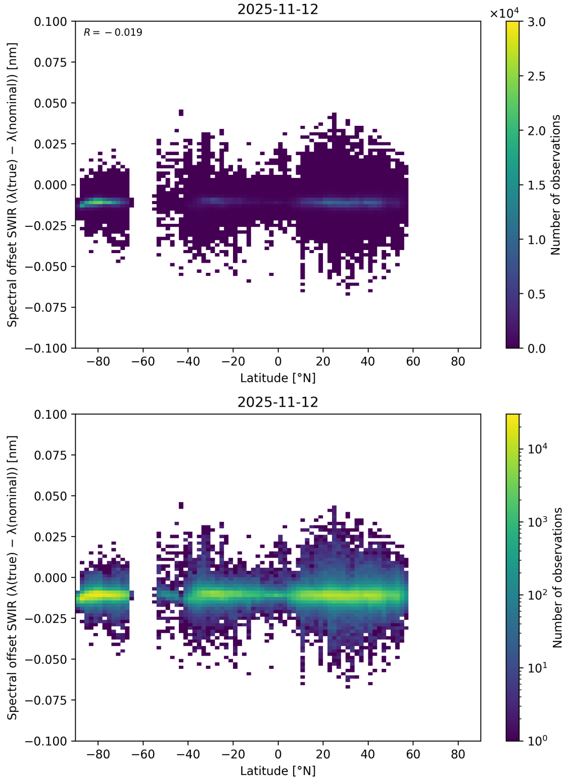
Figure 62: Scatter density plot of “Latitude” against “Spectral offset SWIR ( \lambda_{\text{true}} - \lambda_{\text{nominal}} )” for 2025-11-12 to 2025-11-13.
