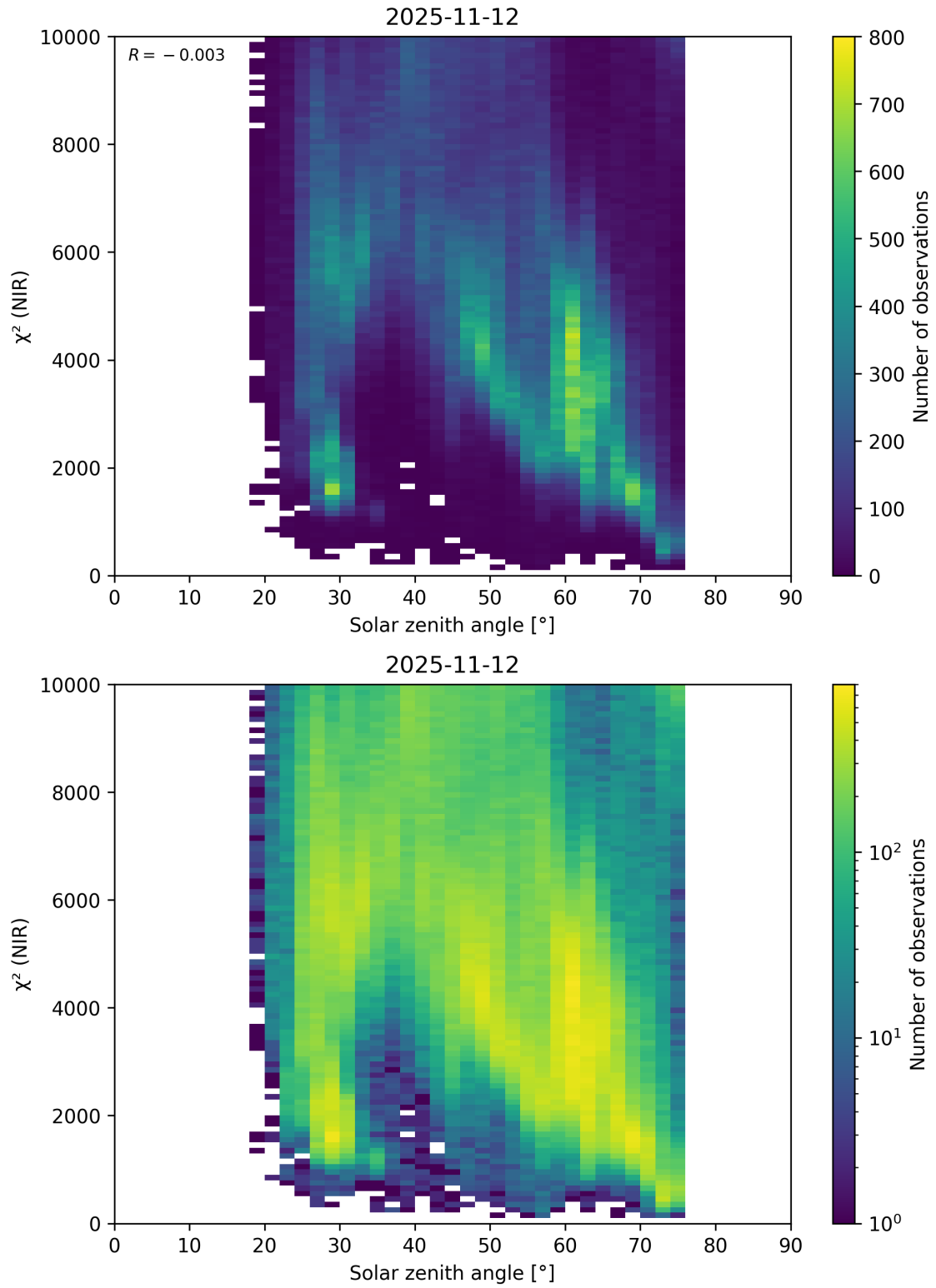
Figure 94: Scatter density plot of “Solar zenith angle” against “ \chi^2 (NIR)” for 2025-11-12 to 2025-11-13.
