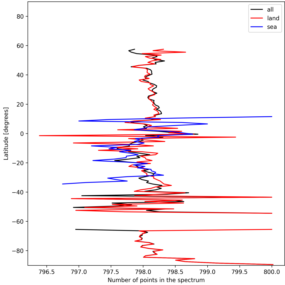
Figure 15: Zonal average of “Number of points in the spectrum” for 2025-11-12 to 2025-11-13.
