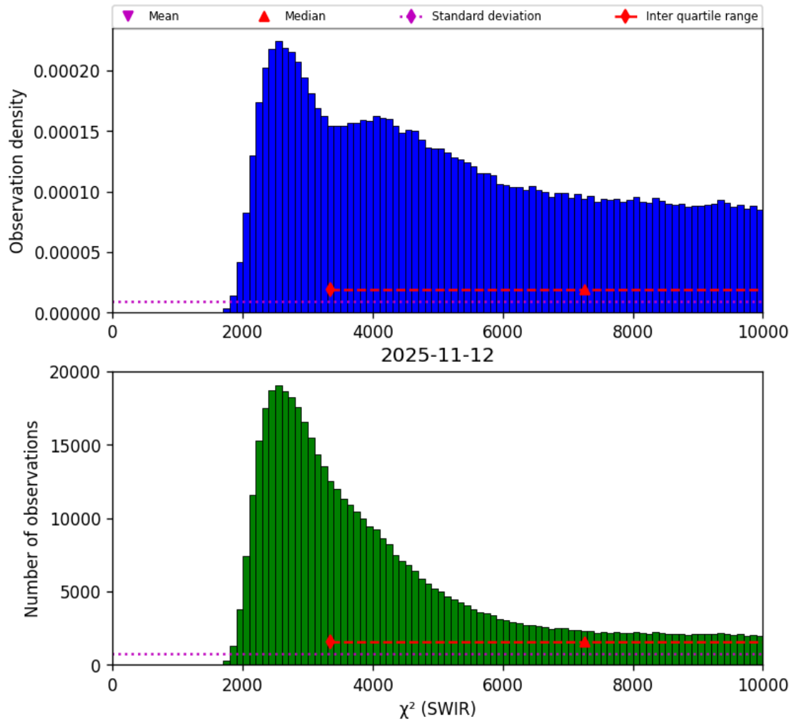
Figure 28: Histogram of “ \chi^2 (SWIR)” for 2025-11-12 to 2025-11-13
