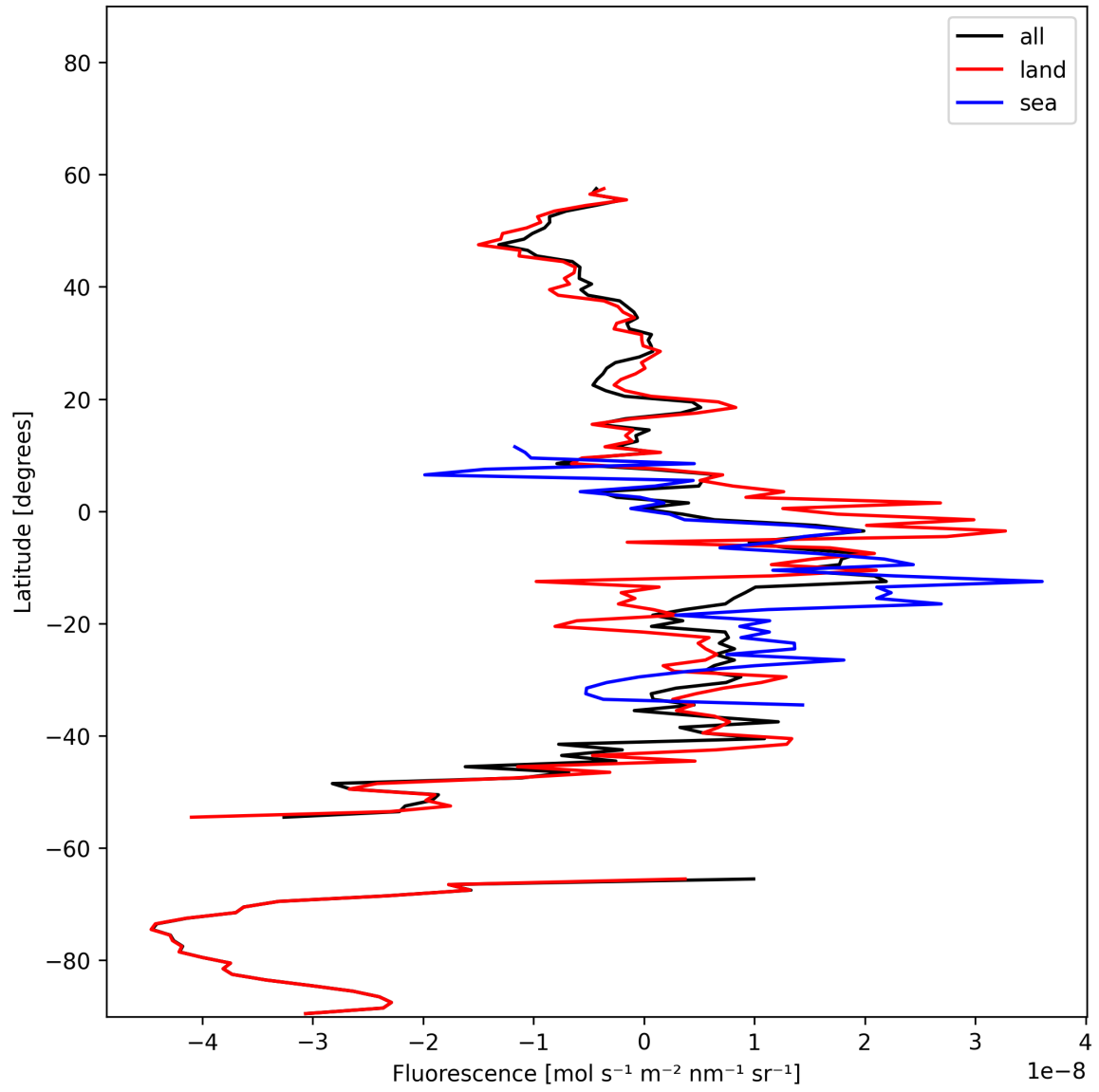
Figure 21: Zonal average of “Fluorescence” for 2025-11-12 to 2025-11-13.
