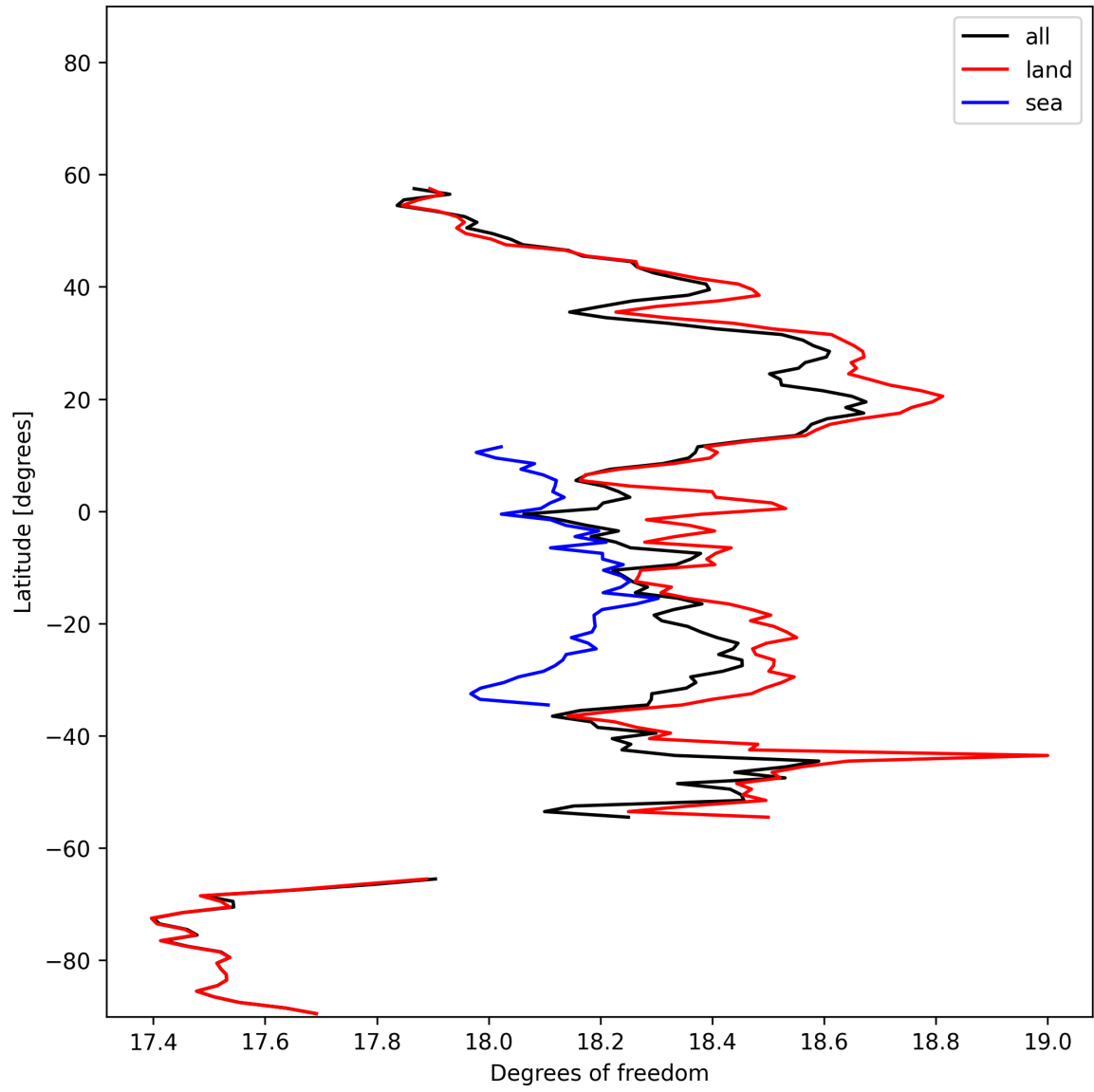
Figure 19: Zonal average of “Degrees of freedom” for 2025-11-12 to 2025-11-13.
