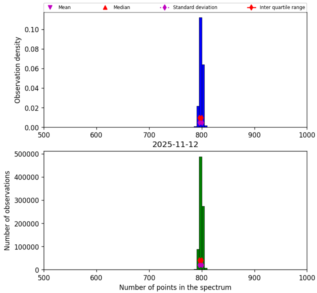
Figure 26: Histogram of “Number of points in the spectrum” for 2025-11-12 to 2025-11-13
