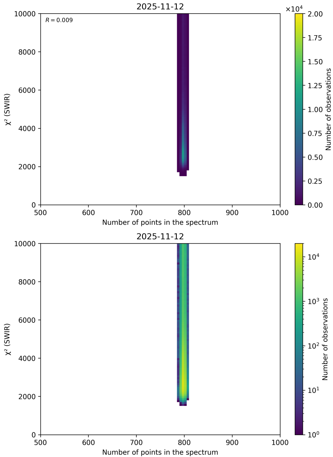
Figure 89: Scatter density plot of “Number of points in the spectrum” against “ \chi^2 (SWIR)” for 2025-11-12 to 2025-11-13.
