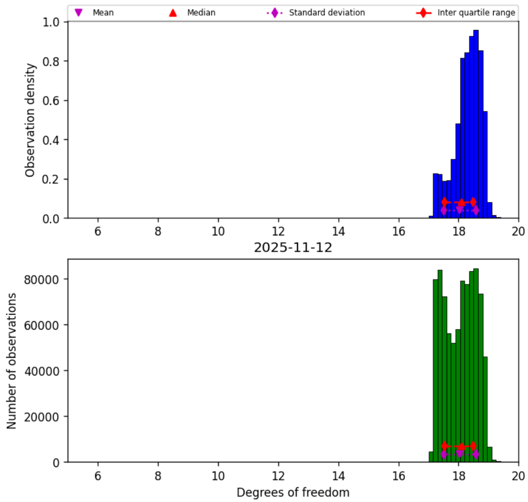
Figure 30: Histogram of “Degrees of freedom” for 2025-11-12 to 2025-11-13
