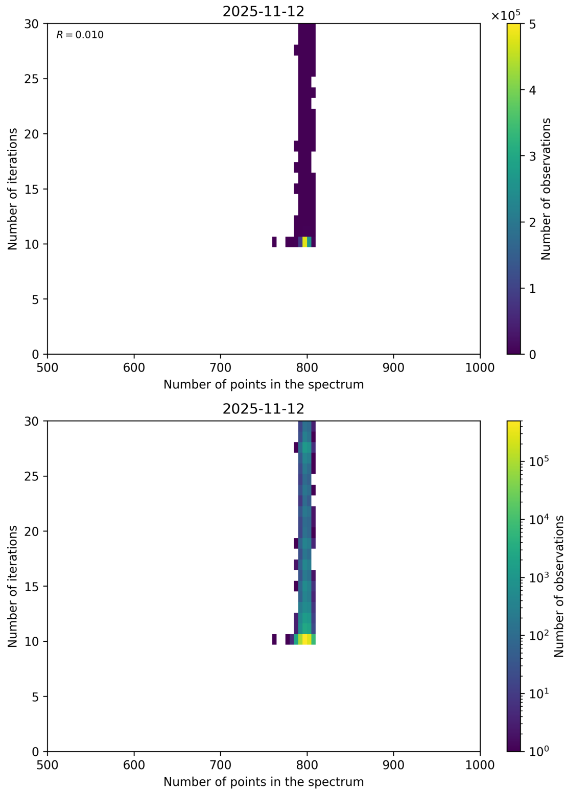
Figure 92: Scatter density plot of “Number of points in the spectrum” against “Number of iterations” for 2025-11-12 to 2025-11-13.
