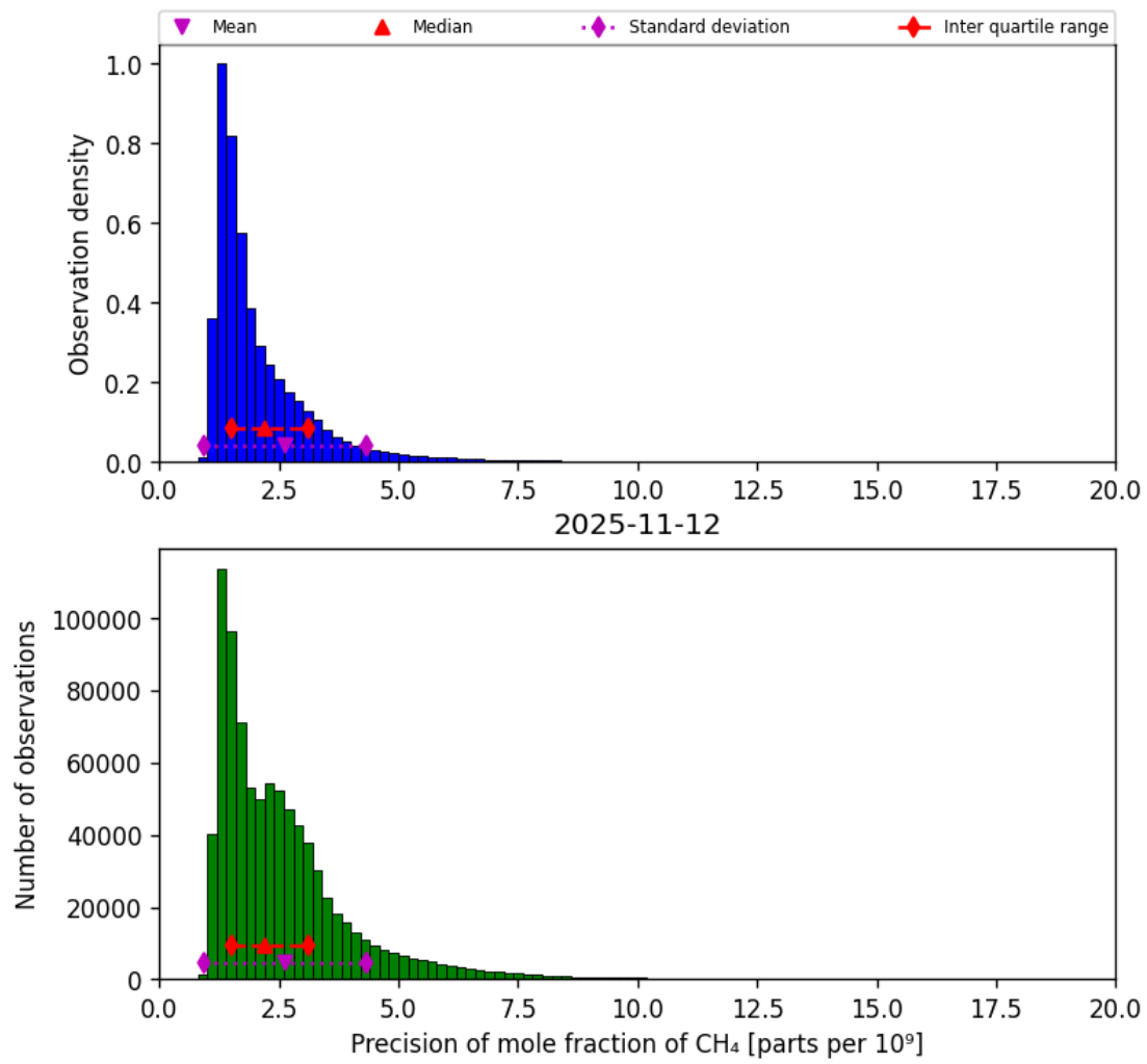
Figure 24: Histogram of “Precision of mole fraction of CH 4 ” for 2025-11-12 to 2025-11-13
