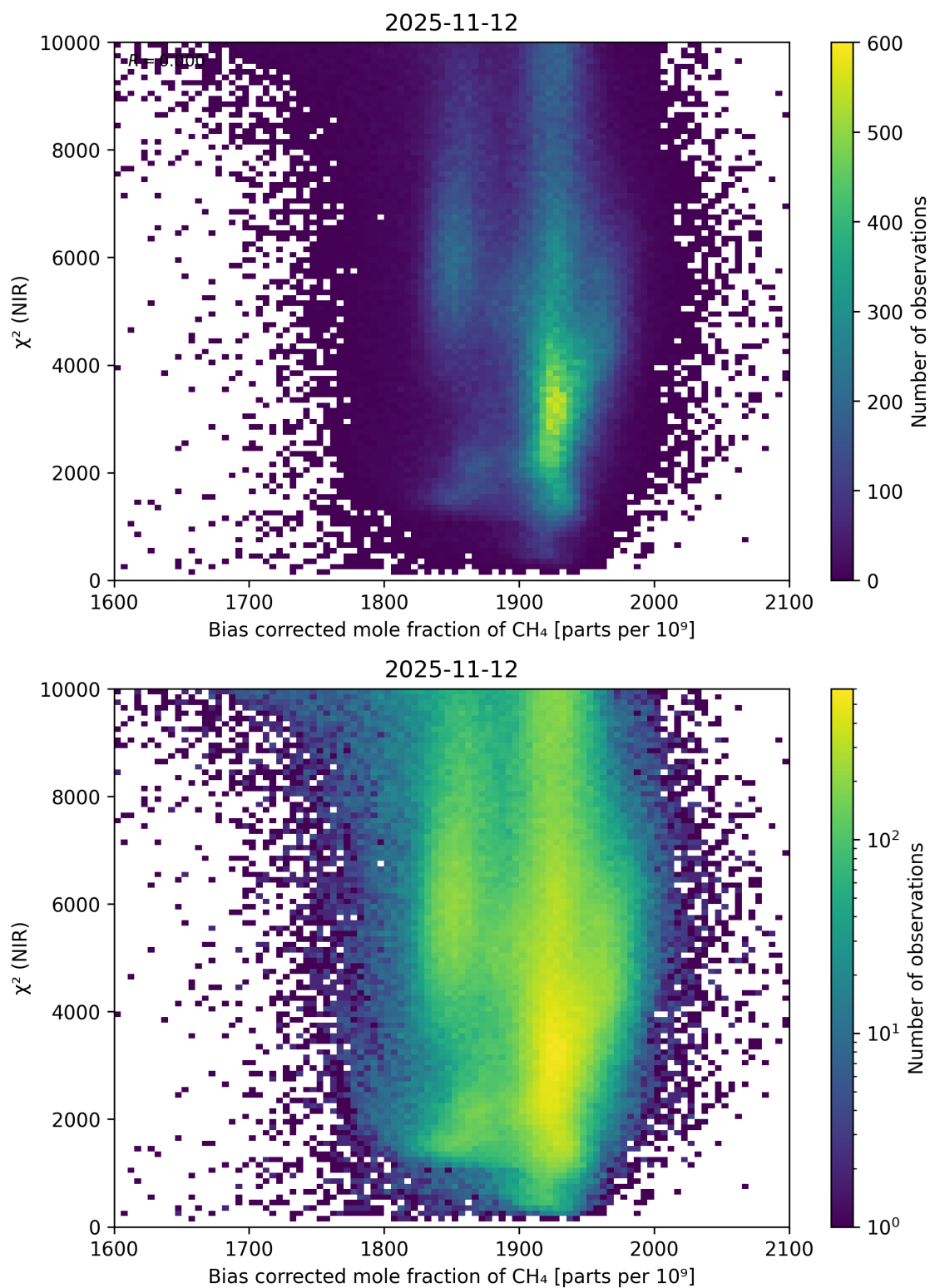
Figure 63: Scatter density plot of “Bias corrected mole fraction of \text{CH}_4 ” against “ \chi^2 (NIR)” for 2025-11-12 to 2025-11-13.
