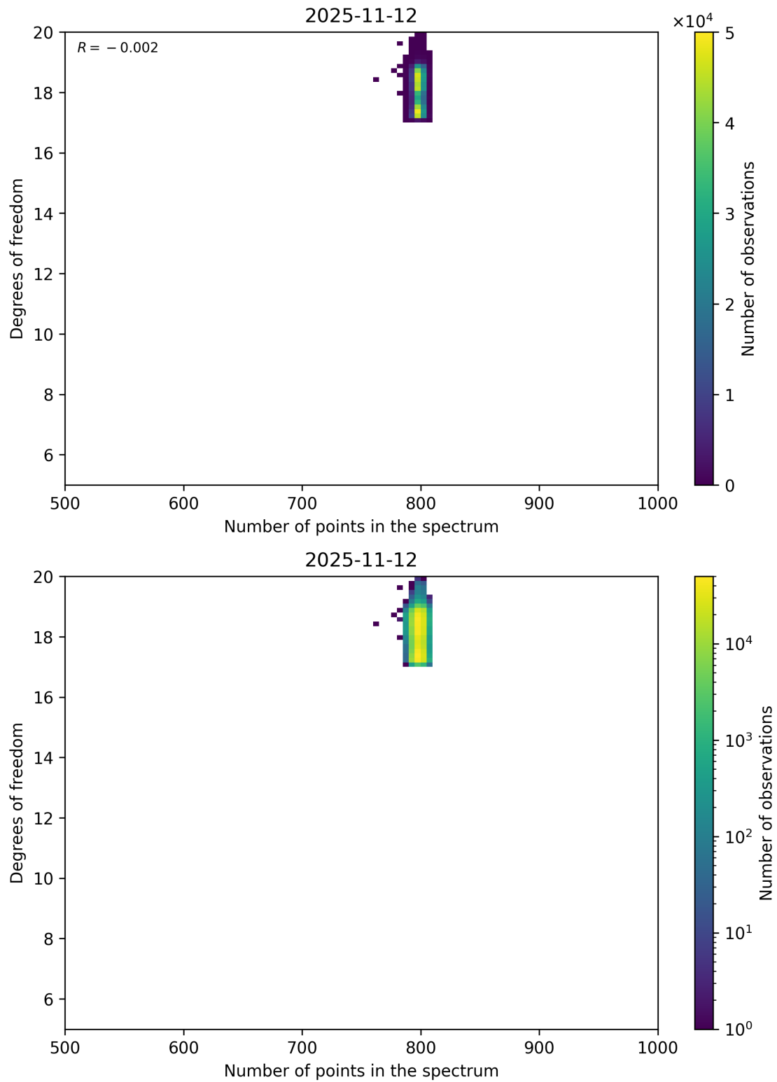
Figure 90: Scatter density plot of “Number of points in the spectrum” against “Degrees of freedom” for 2025-11-12 to 2025-11-13.
