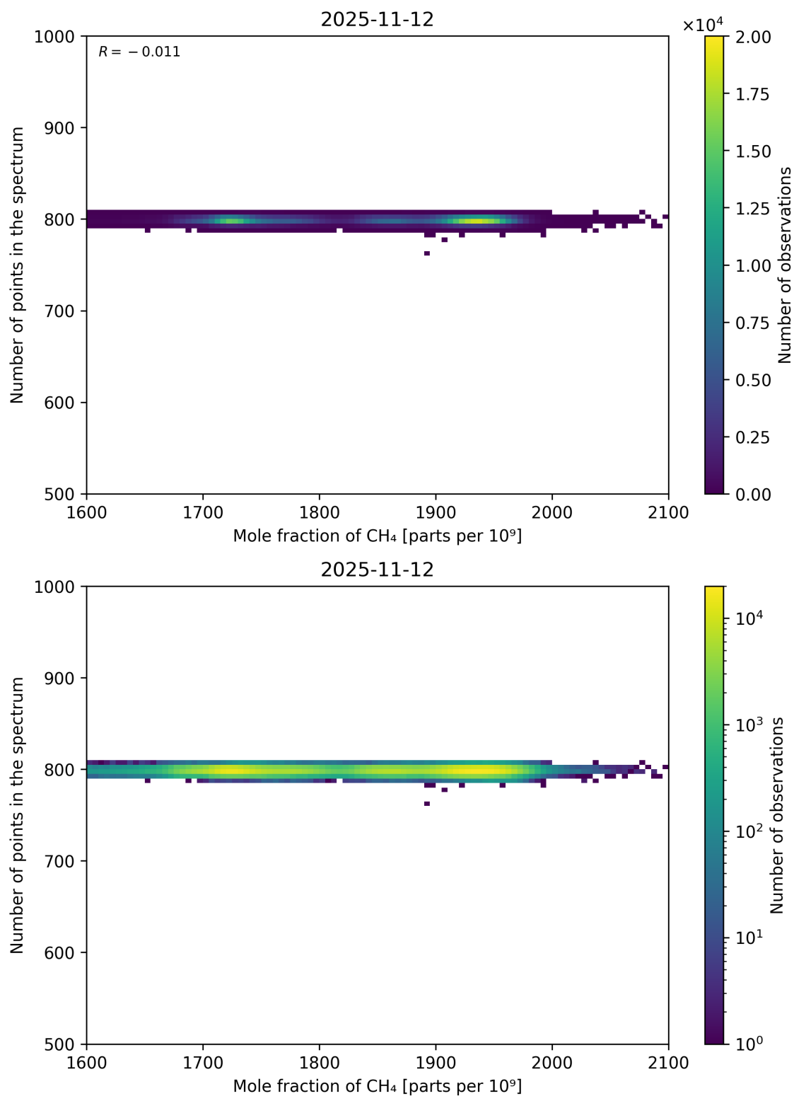
Figure 77: Scatter density plot of “Mole fraction of CH 4 ” against “Number of points in the spectrum” for 2025-11-12 to 2025-11-13.
