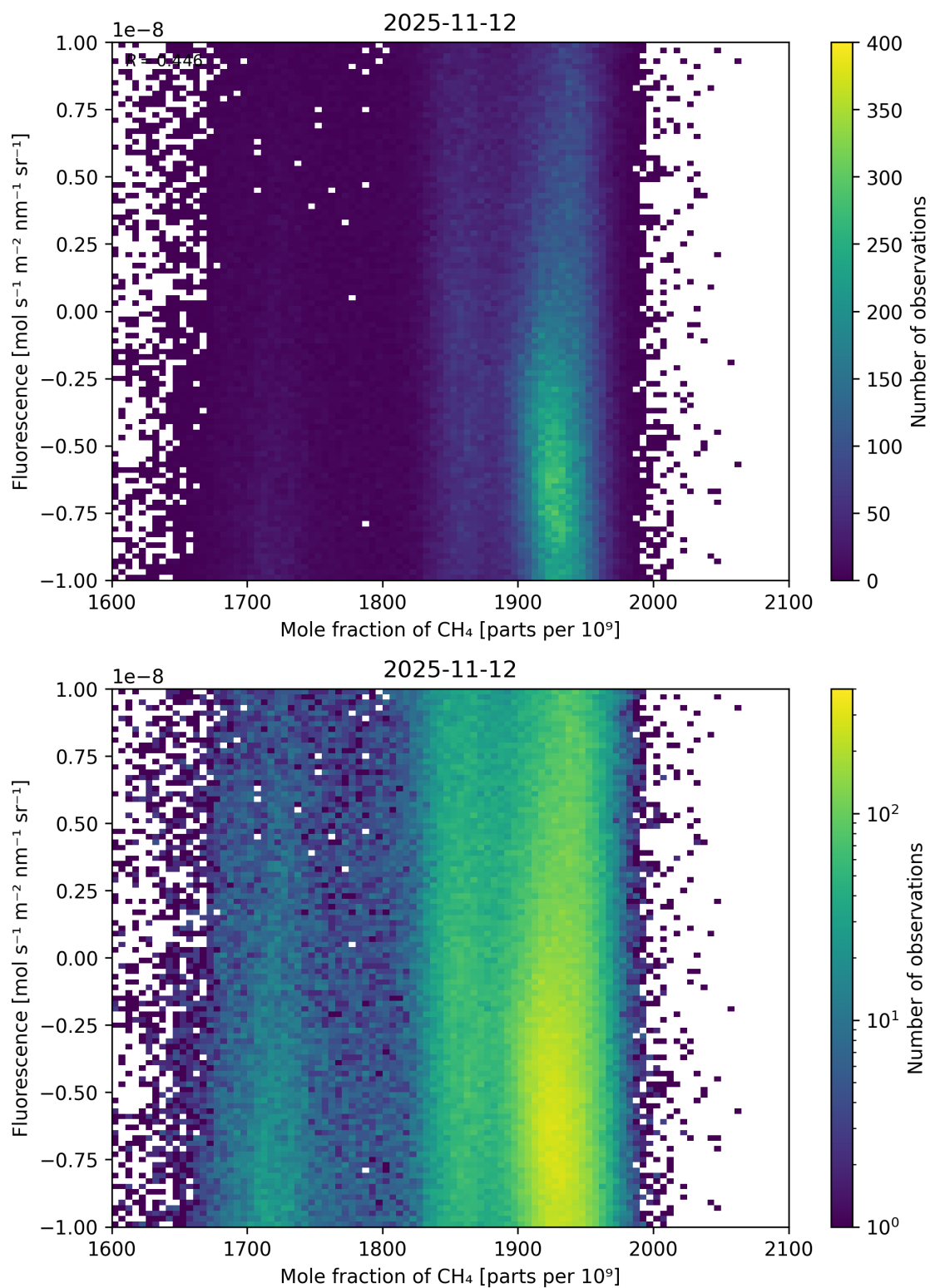
Figure 73: Scatter density plot of “Mole fraction of \text{CH}_4 ” against “Fluorescence” for 2025-11-12 to 2025-11-13.
