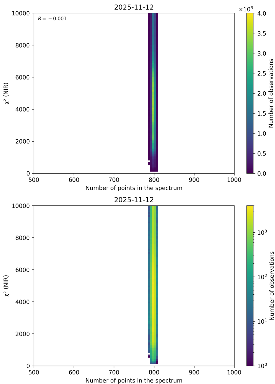
Figure 88: Scatter density plot of “Number of points in the spectrum” against “ \chi^2 (NIR)” for 2025-11-12 to 2025-11-13.
