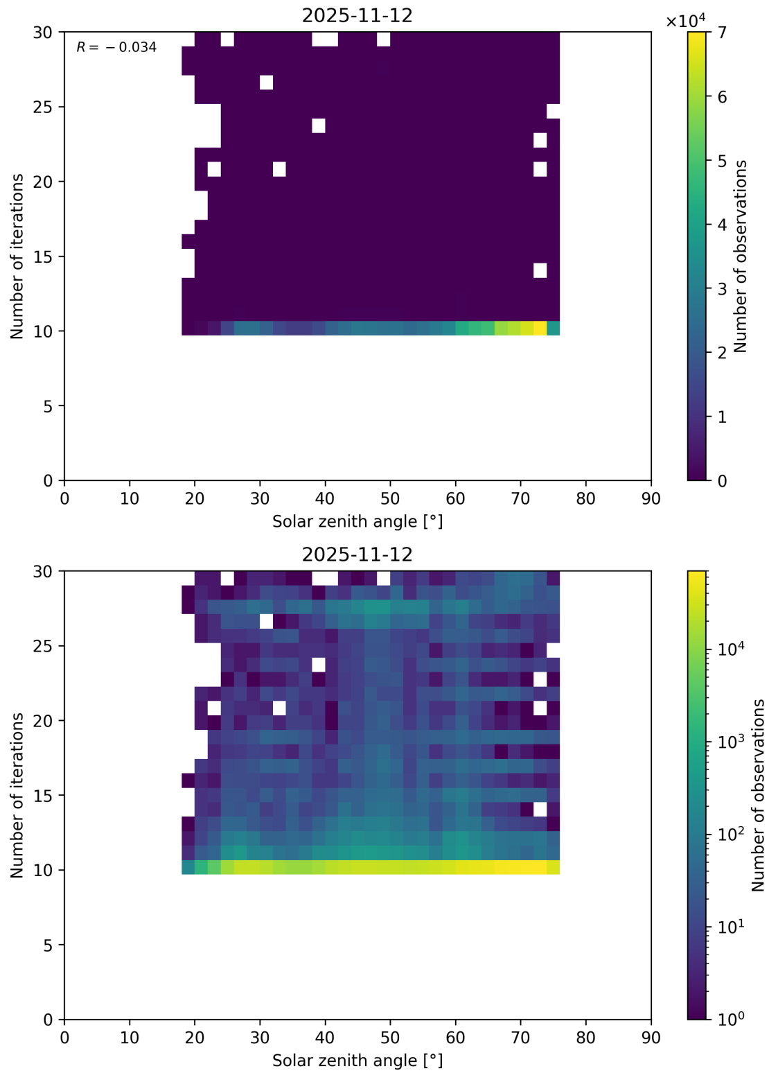
Figure 102: Scatter density plot of “Solar zenith angle” against “Number of iterations” for 2025-11-12 to 2025-11-13.
