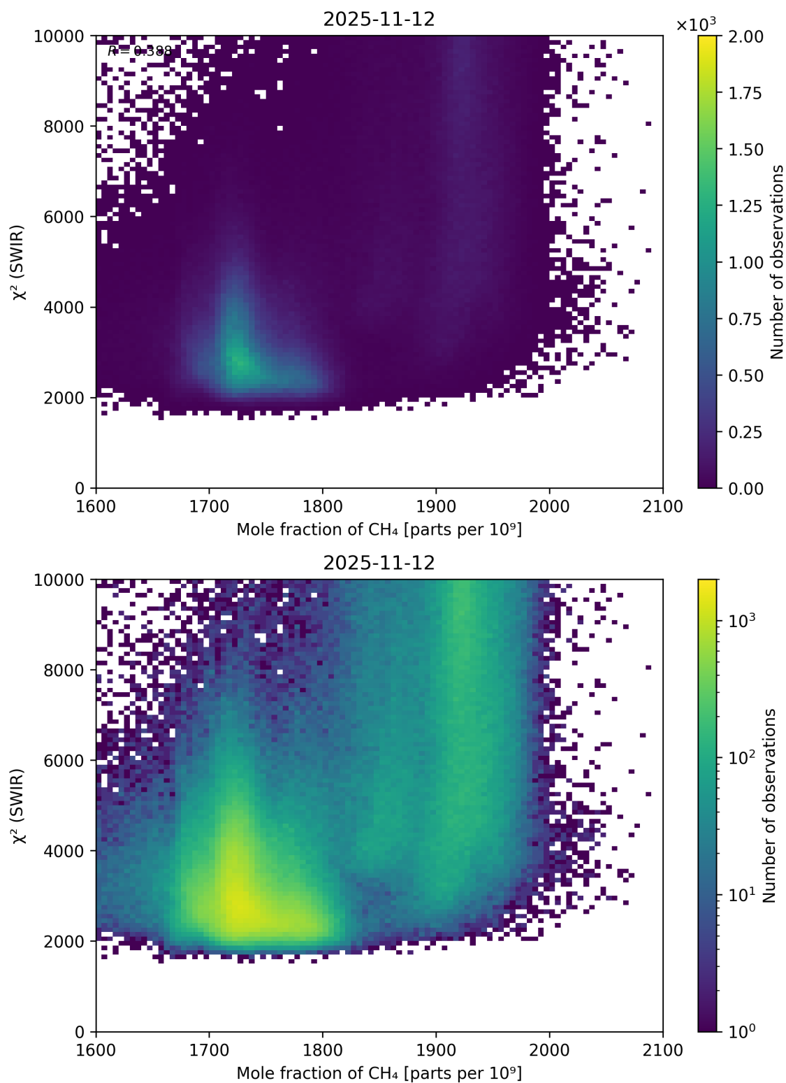
Figure 71: Scatter density plot of “Mole fraction of \text{CH}_4 ” against “ \chi^2 (SWIR)” for 2025-11-12 to 2025-11-13.
