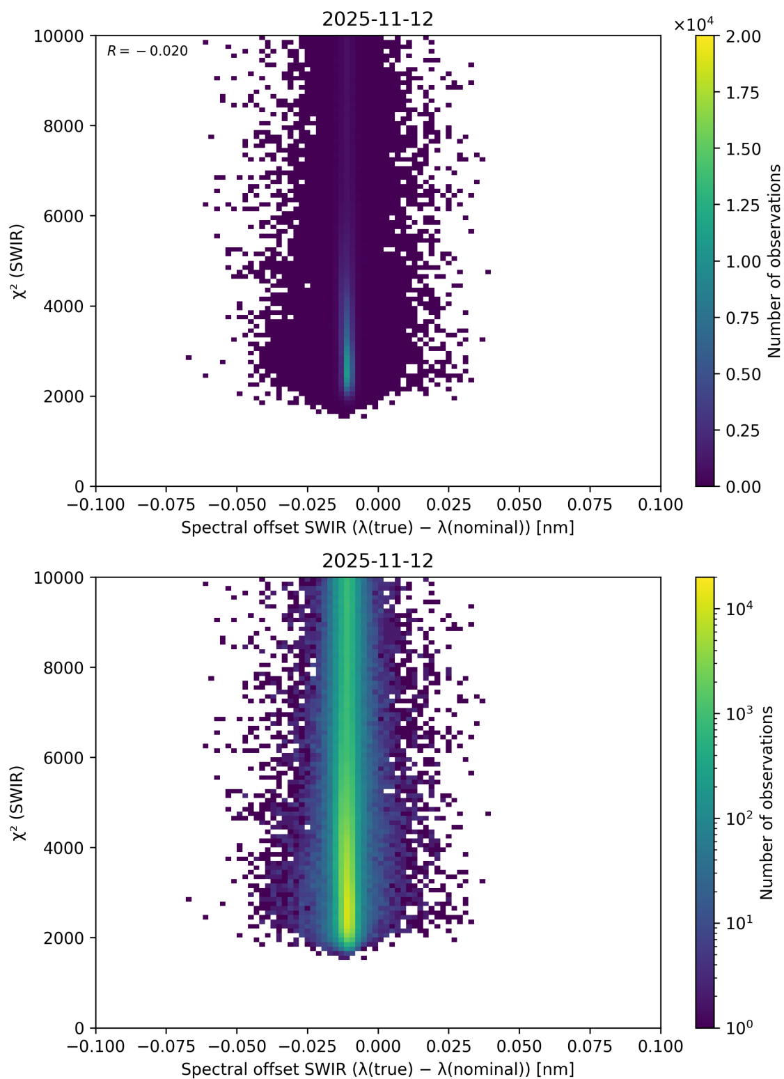
Figure 118: Scatter density plot of “Spectral offset SWIR ( \lambda_{\text{true}} - \lambda_{\text{nominal}} )” against “ \chi^2 (SWIR)” for 2025-11-12 to 2025-11-13.
