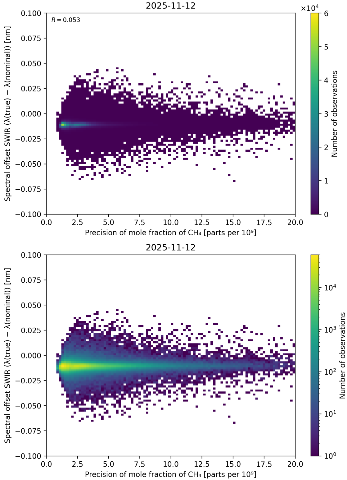
Figure 85: Scatter density plot of “Precision of mole fraction of \text{CH}_4 ” against “Spectral offset SWIR ( \lambda_{\text{true}} - \lambda_{\text{nominal}} )” for 2025-11-12 to 2025-11-13.
