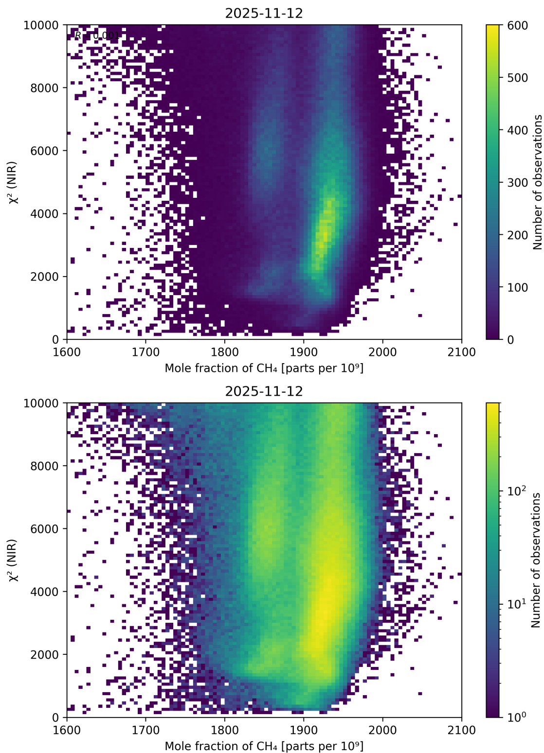
Figure 70: Scatter density plot of “Mole fraction of \text{CH}_4 ” against “ \chi^2 (NIR)” for 2025-11-12 to 2025-11-13.
