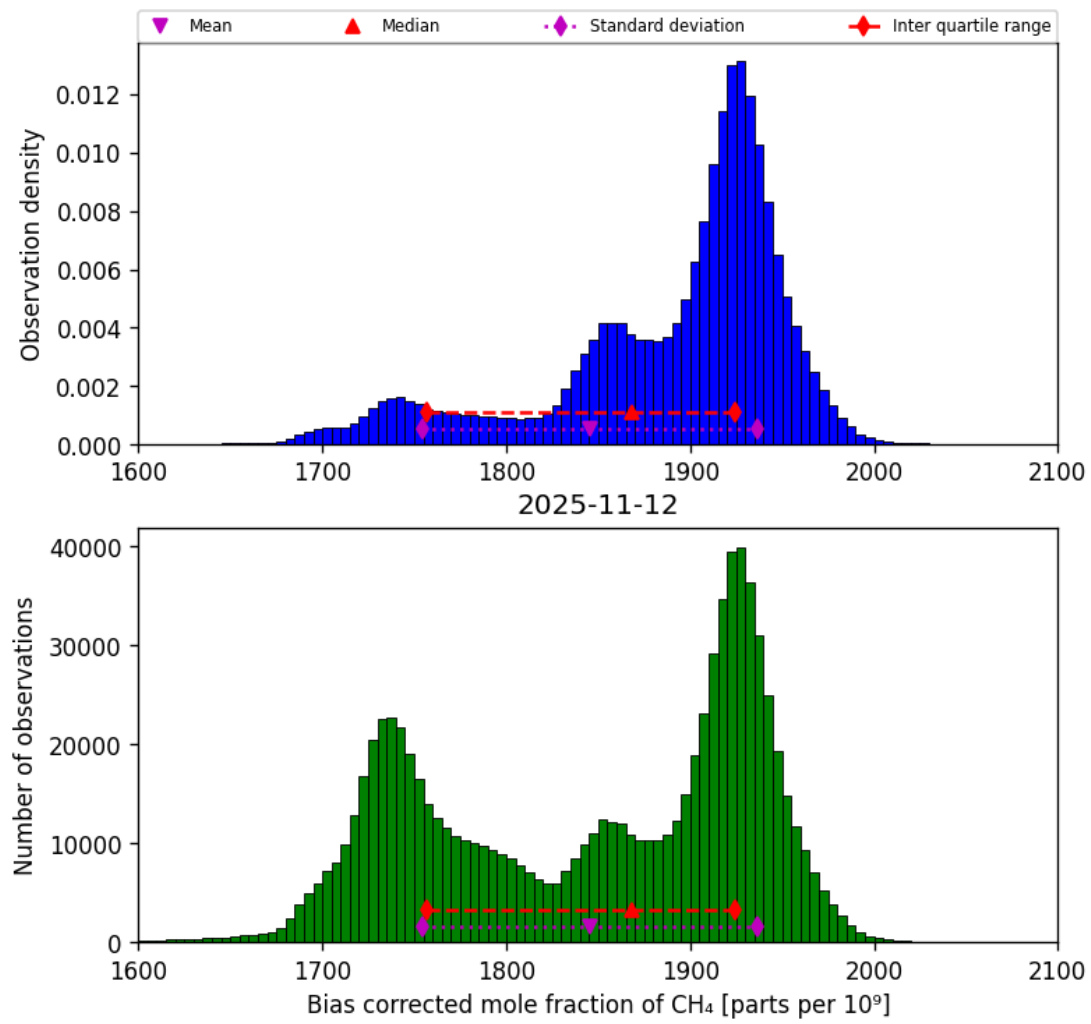
Figure 25: Histogram of “Bias corrected mole fraction of CH 4 ” for 2025-11-12 to 2025-11-13
