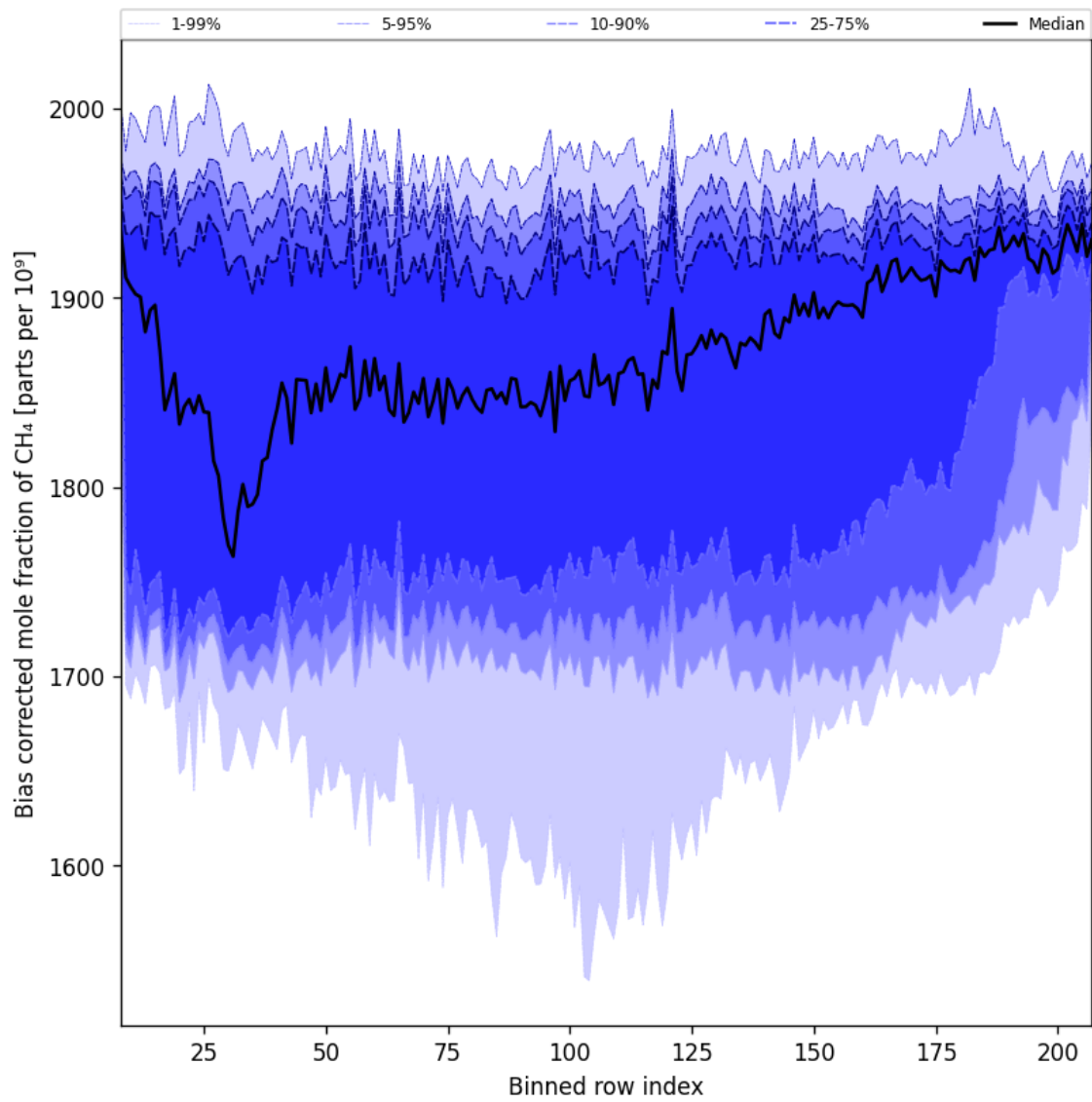
Figure 36: Along track statistics of “Bias corrected mole fraction of CH 4 ” for 2025-11-12 to 2025-11-13
