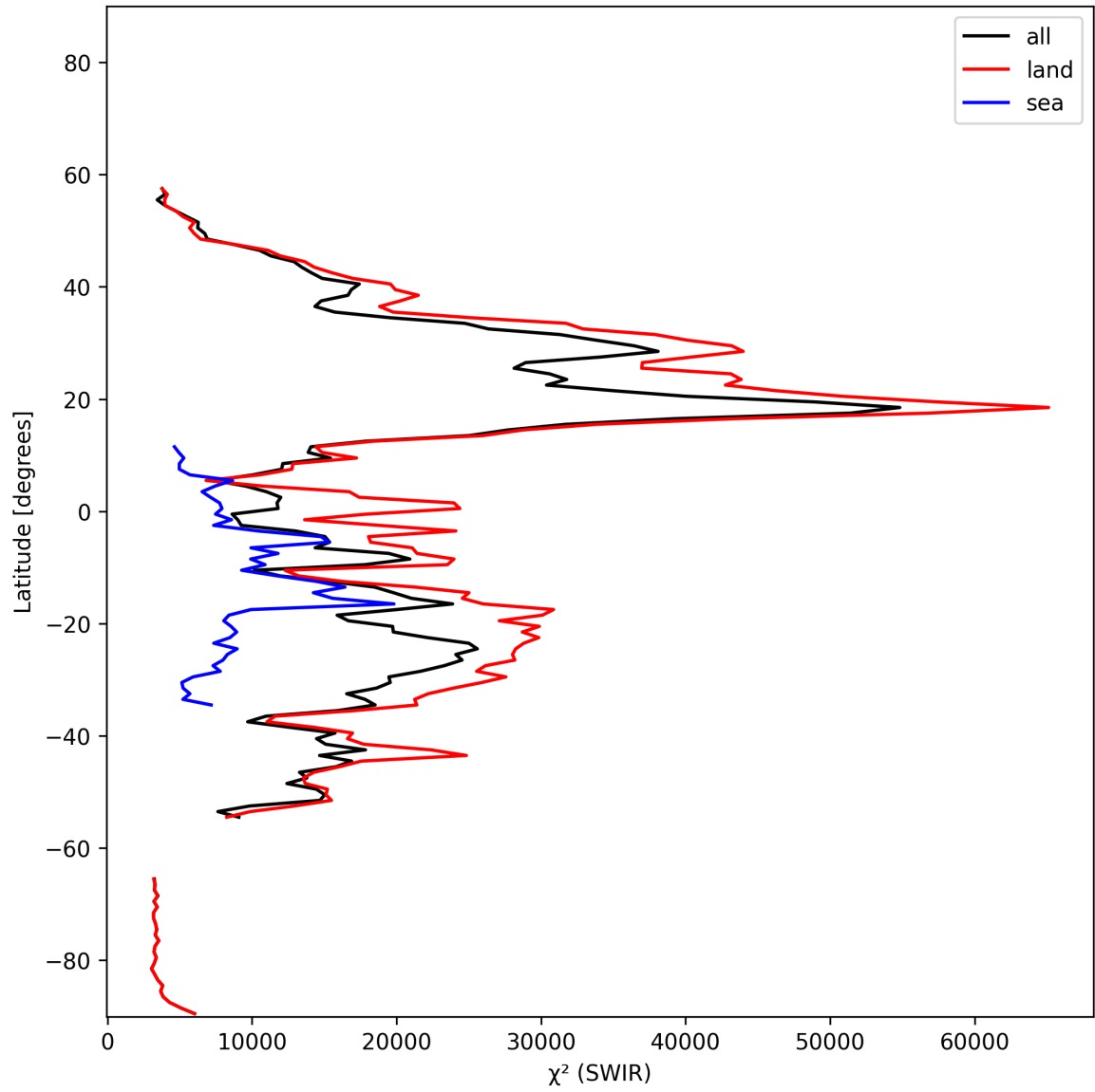
Figure 17: Zonal average of “ \chi^2 (SWIR)” for 2025-11-12 to 2025-11-13.
