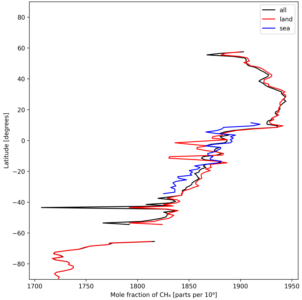
Figure 12: Zonal average of “Mole fraction of \text{CH}_4 ” for 2025-11-12 to 2025-11-13.
