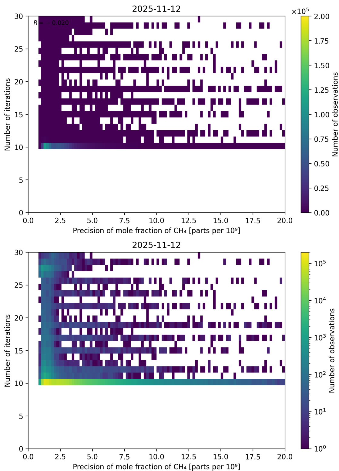
Figure 83: Scatter density plot of “Precision of mole fraction of CH 4 ” against “Number of iterations” for 2025-11-12 to 2025-11-13.
