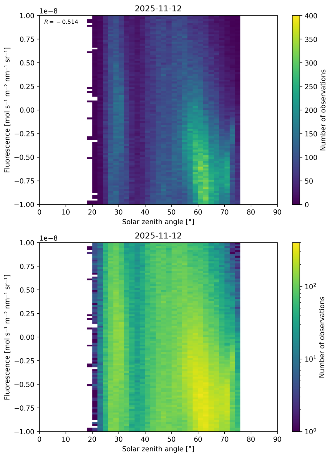
Figure 97: Scatter density plot of “Solar zenith angle” against “Fluorescence” for 2025-11-12 to 2025-11-13.
