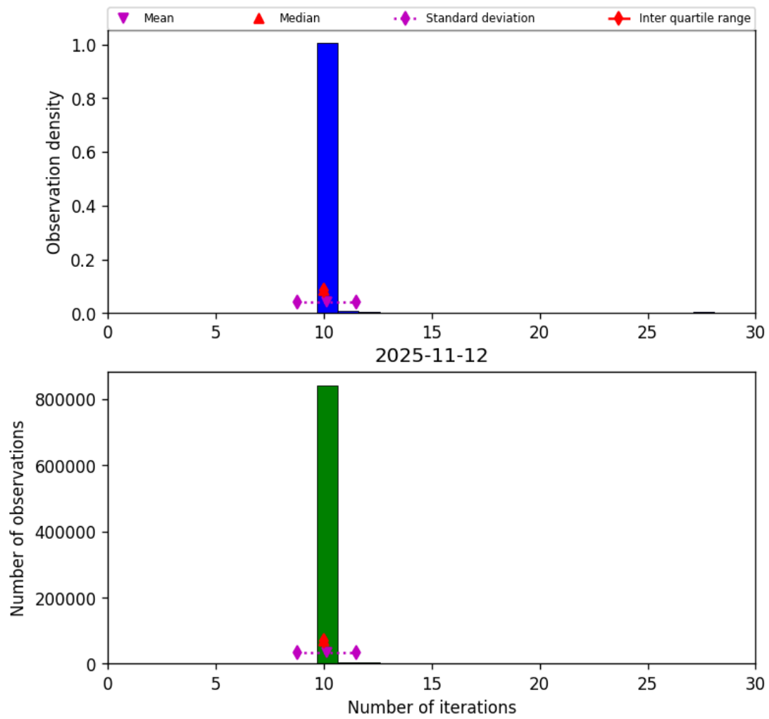
Figure 31: Histogram of “Number of iterations” for 2025-11-12 to 2025-11-13
