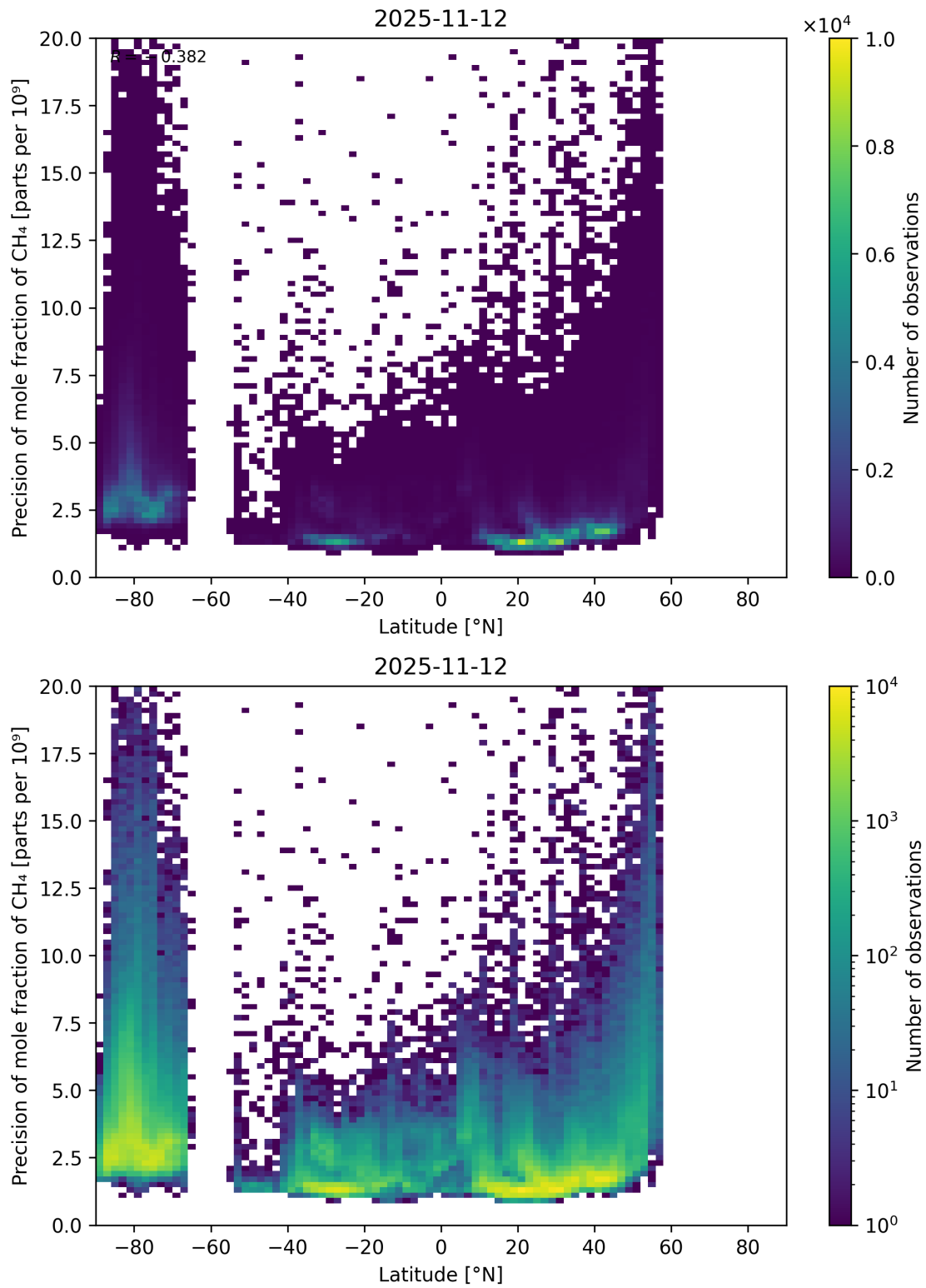
Figure 59: Scatter density plot of “Latitude” against “Precision of mole fraction of CH 4 ” for 2025-11-12 to 2025-11-13.
