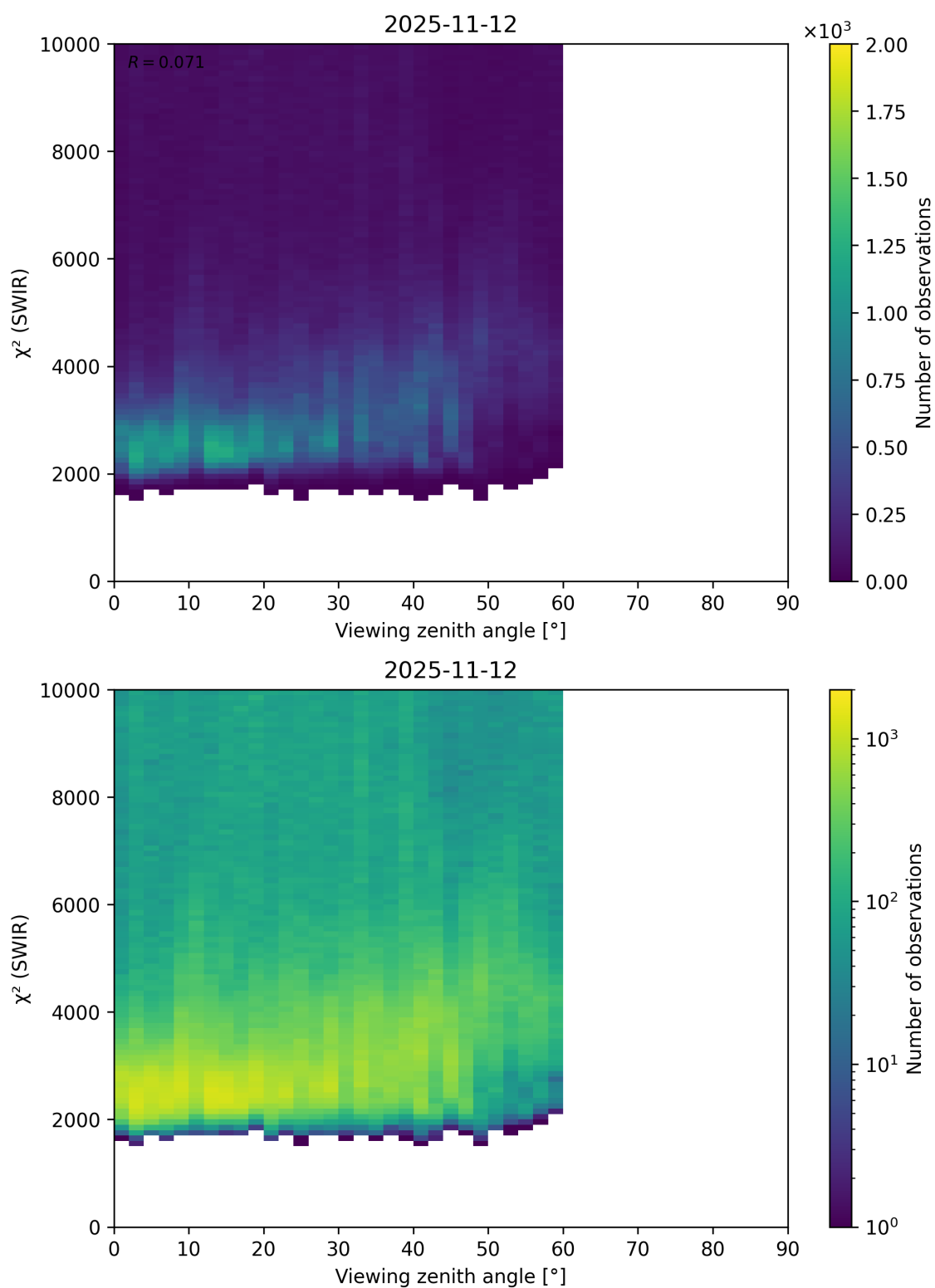
Figure 106: Scatter density plot of “Viewing zenith angle” against “ \chi^2 (SWIR)” for 2025-11-12 to 2025-11-13.
