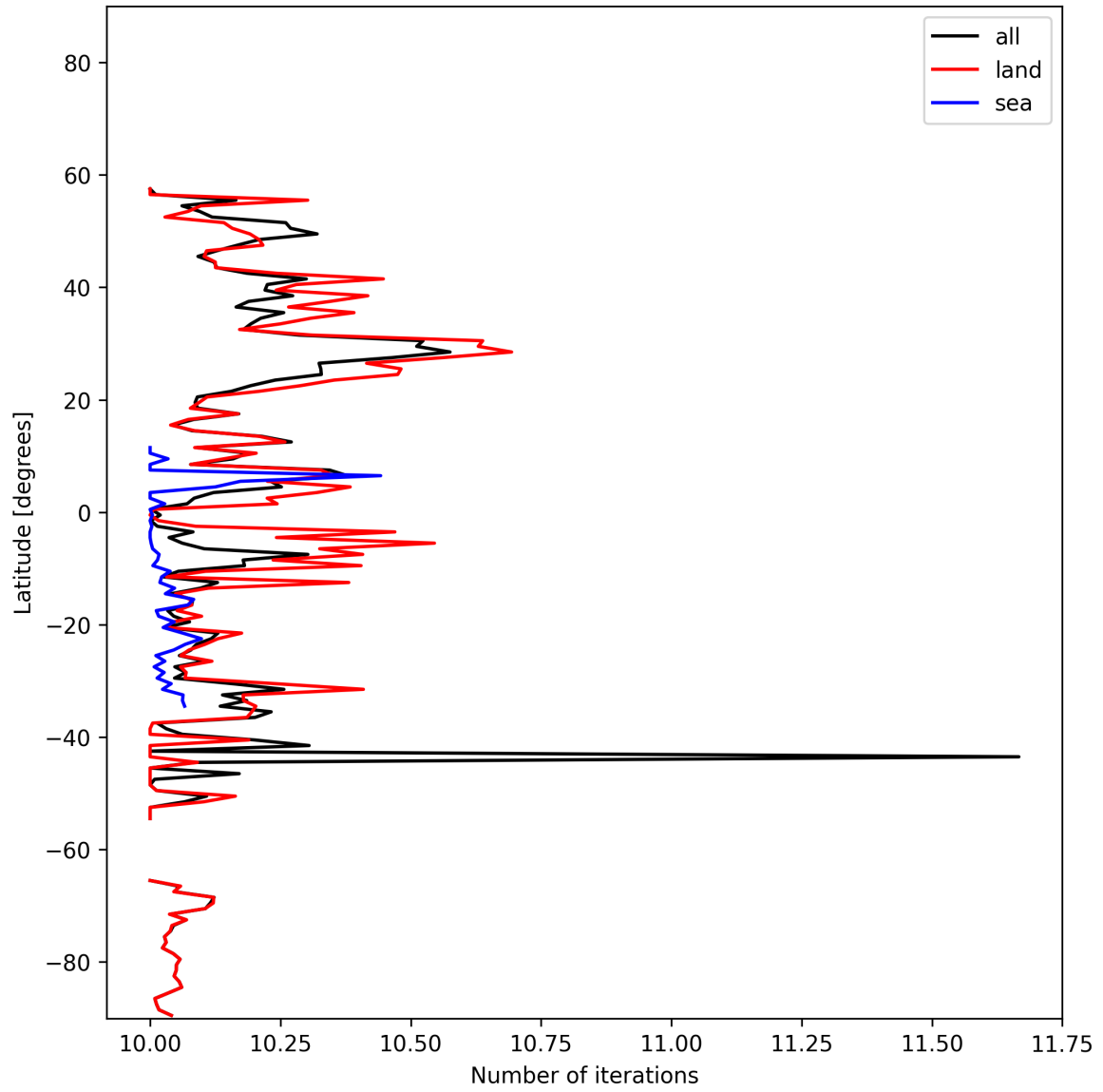
Figure 20: Zonal average of “Number of iterations” for 2025-11-12 to 2025-11-13.
