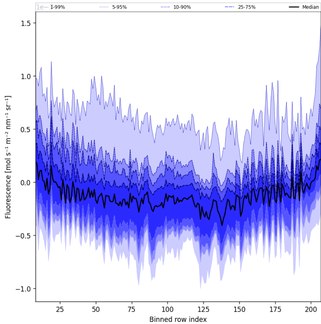
Figure 43: Along track statistics of “Fluorescence” for 2025-11-12 to 2025-11-13
