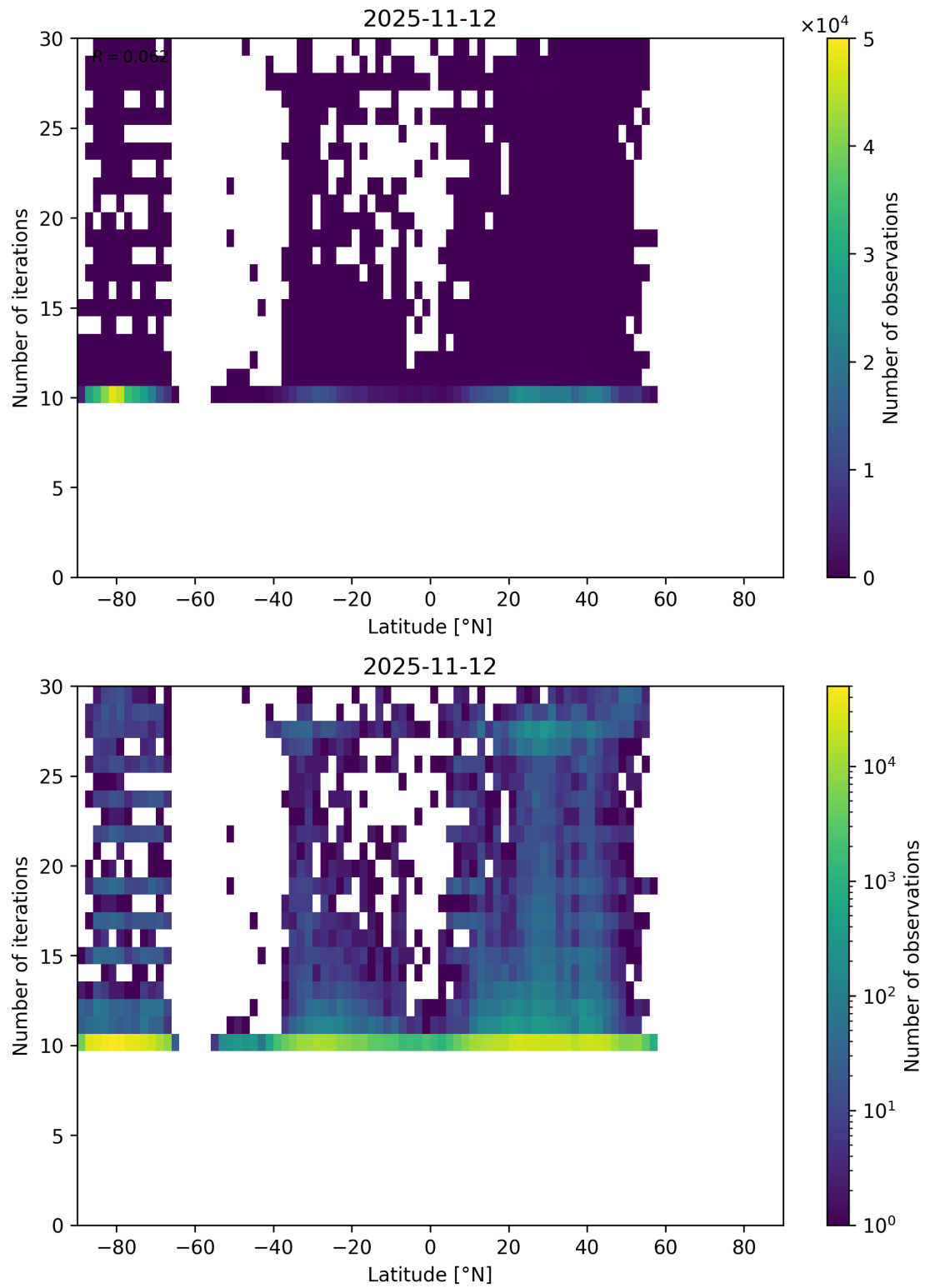
Figure 60: Scatter density plot of “Latitude” against “Number of iterations” for 2025-11-12 to 2025-11-13.
