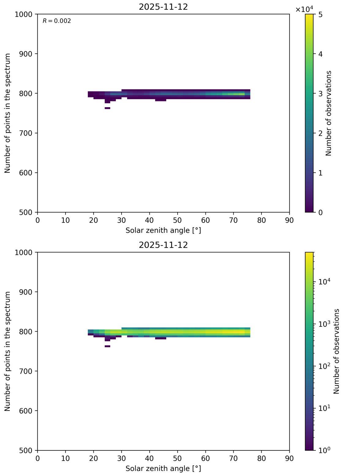
Figure 103: Scatter density plot of “Solar zenith angle” against “Number of points in the spectrum” for 2025-11-12 to 2025-11-13.
