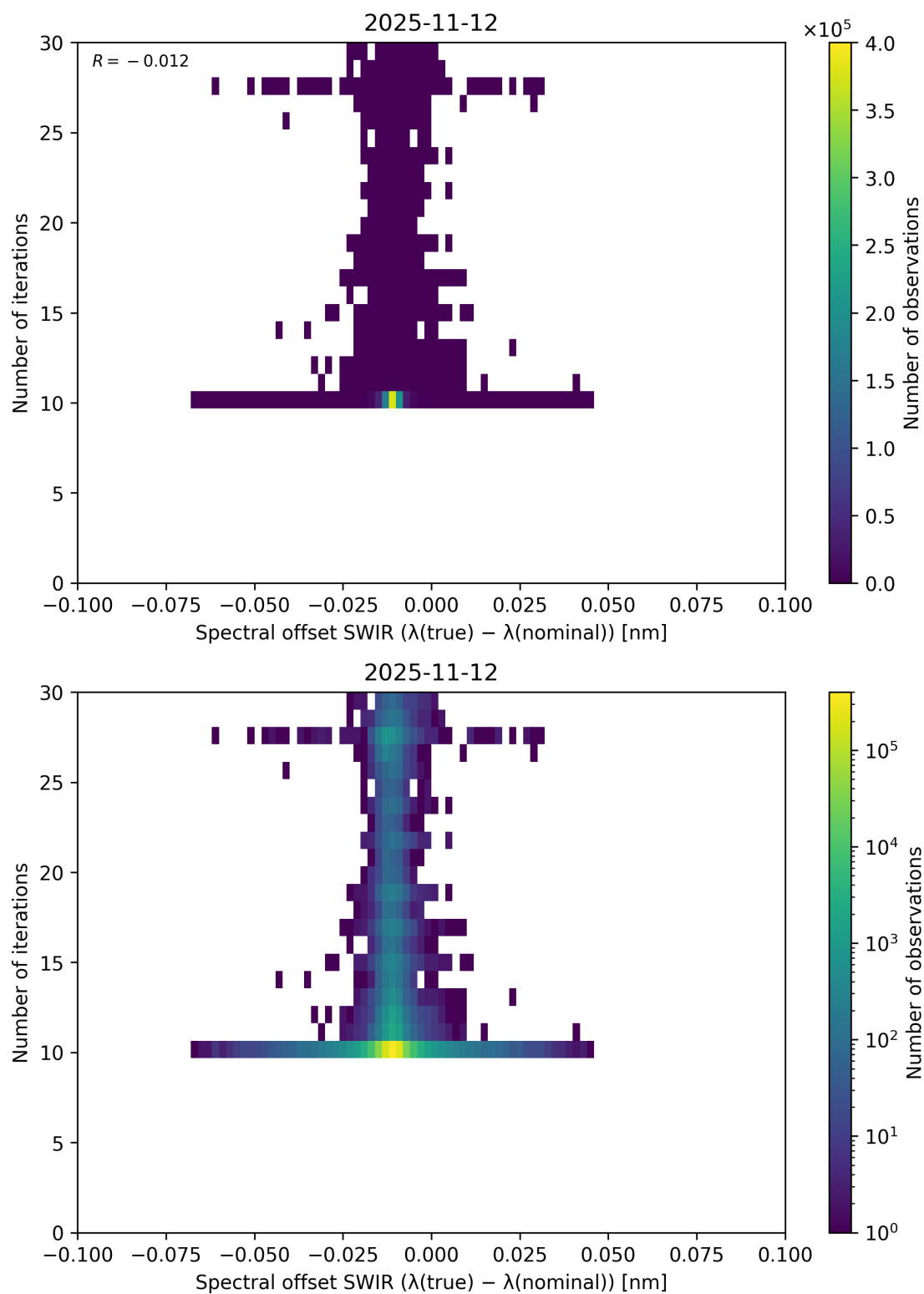
Figure 121: Scatter density plot of “Spectral offset SWIR ( \lambda_{\text{true}} - \lambda_{\text{nominal}} )” against “Number of iterations” for 2025-11-12 to 2025-11-13.
