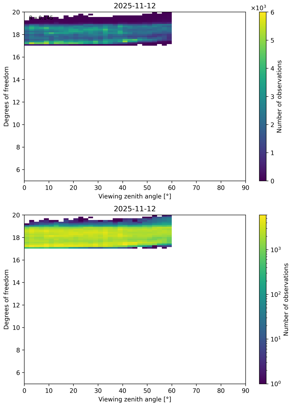
Figure 107: Scatter density plot of “Viewing zenith angle” against “Degrees of freedom” for 2025-11-12 to 2025-11-13.
