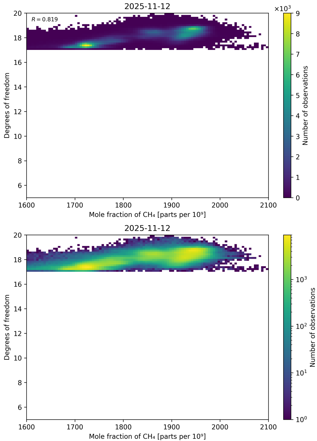
Figure 72: Scatter density plot of “Mole fraction of CH 4 ” against “Degrees of freedom” for 2025-11-12 to 2025-11-13.
