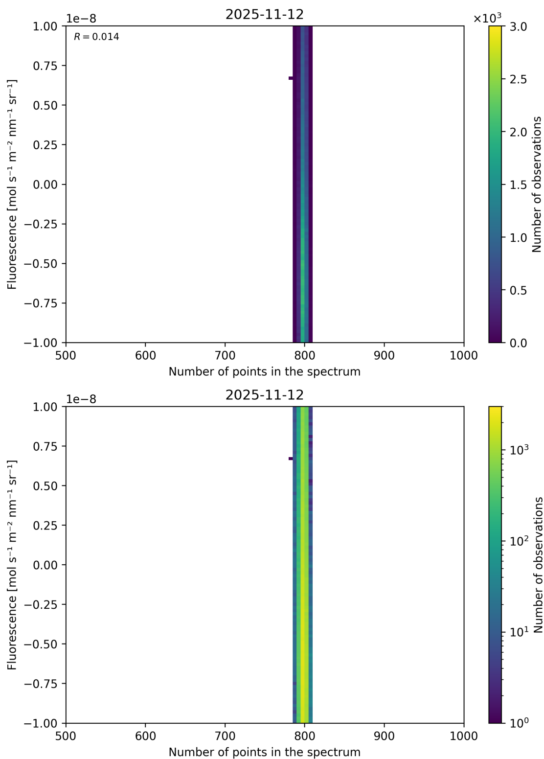
Figure 91: Scatter density plot of “Number of points in the spectrum” against “Fluorescence” for 2025-11-12 to 2025-11-13.
