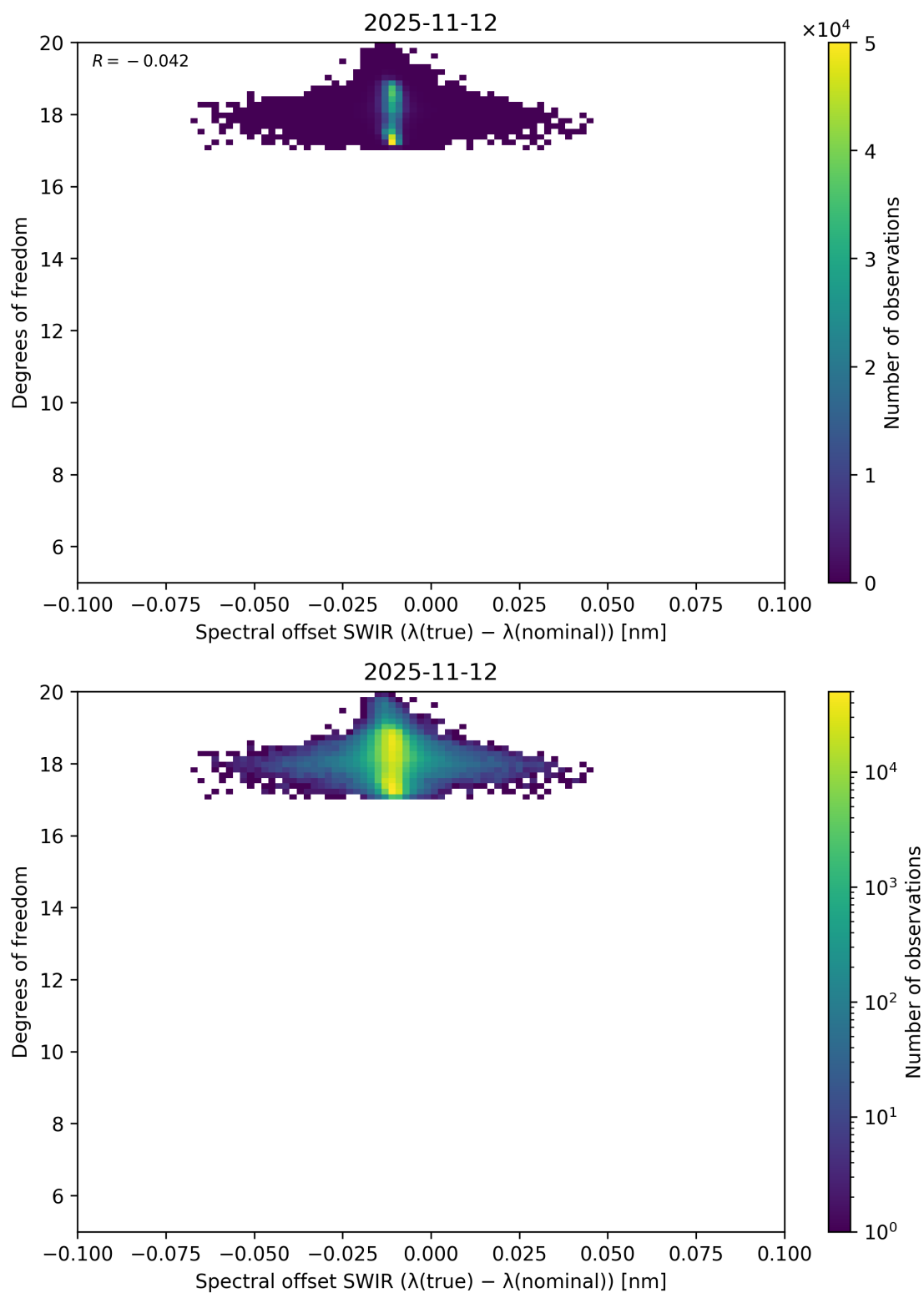
Figure 119: Scatter density plot of “Spectral offset SWIR ( \lambda_{\text{true}} - \lambda_{\text{nominal}} )” against “Degrees of freedom” for 2025-11-12 to 2025-11-13.
