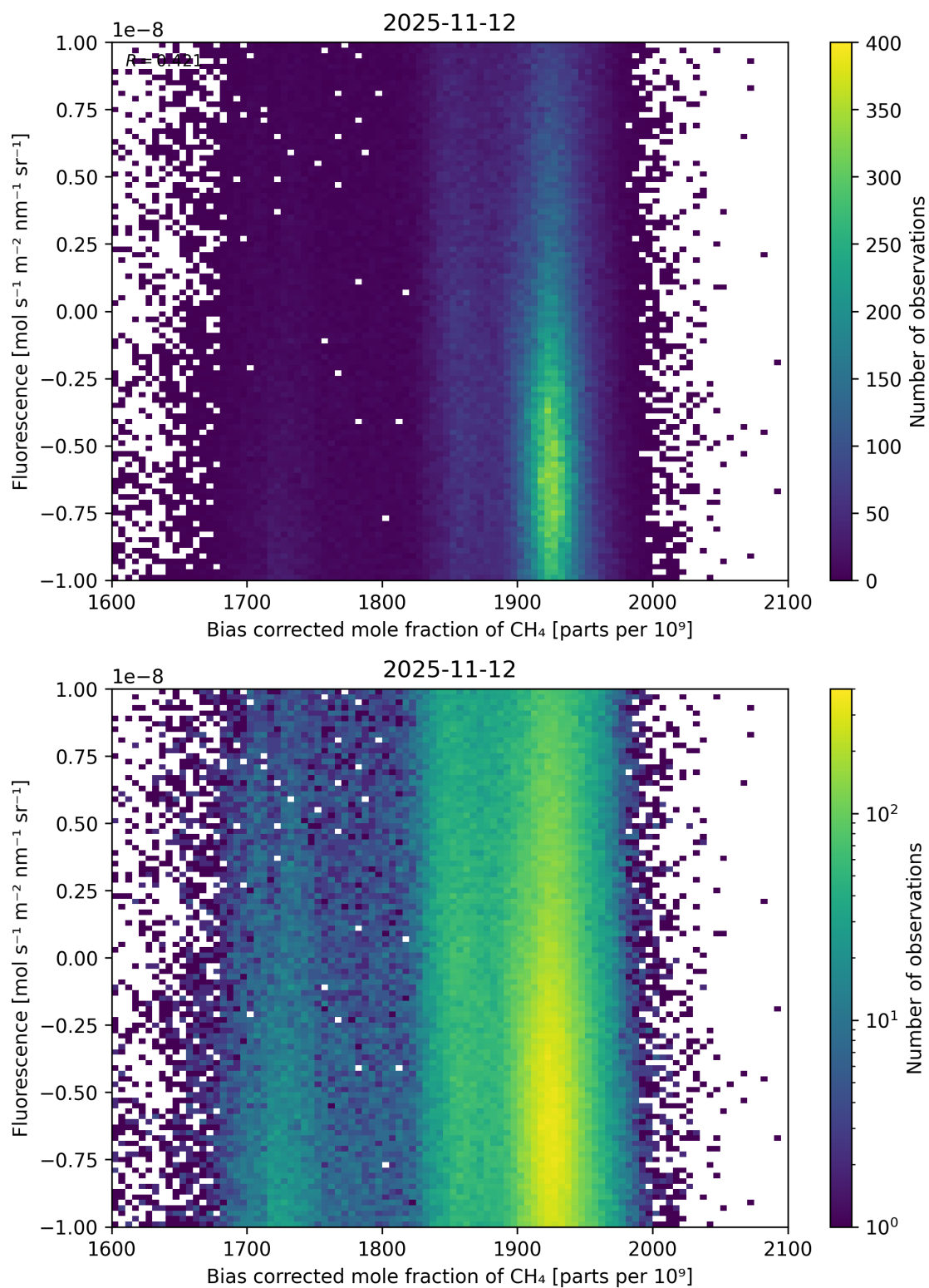
Figure 66: Scatter density plot of “Bias corrected mole fraction of \text{CH}_4 ” against “Fluorescence” for 2025-11-12 to 2025-11-13.
