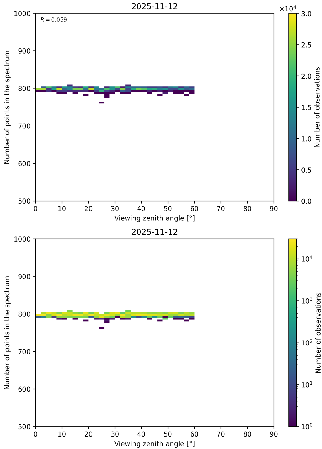
Figure 114: Scatter density plot of “Viewing zenith angle” against “Number of points in the spectrum” for 2025-11-12 to 2025-11-13.
