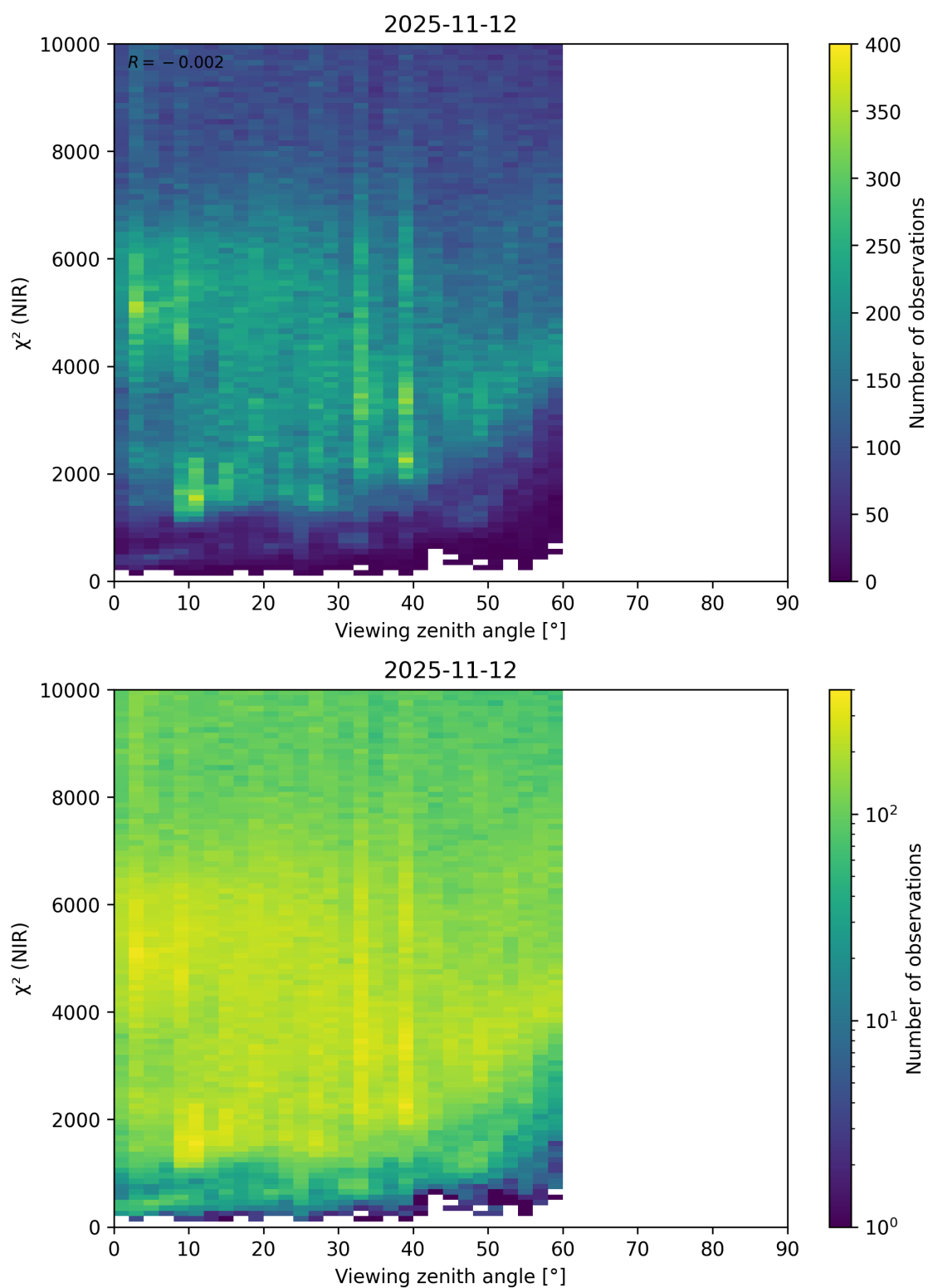
Figure 105: Scatter density plot of “Viewing zenith angle” against “ \chi^2 (NIR)” for 2025-11-12 to 2025-11-13.
