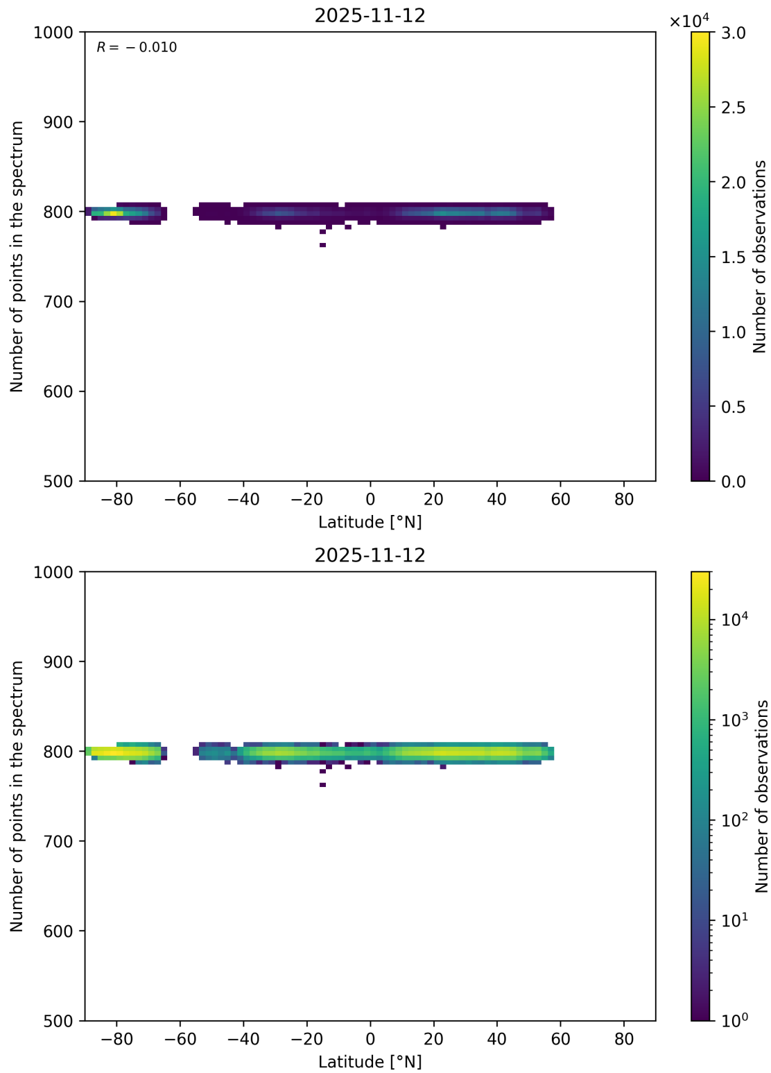
Figure 61: Scatter density plot of “Latitude” against “Number of points in the spectrum” for 2025-11-12 to 2025-11-13.
