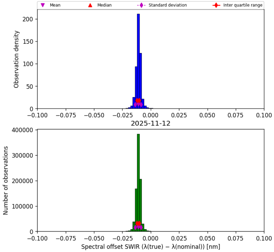
Figure 27: Histogram of “Spectral offset SWIR ( \lambda_{\text{true}} - \lambda_{\text{nominal}} )” for 2025-11-12 to 2025-11-13
