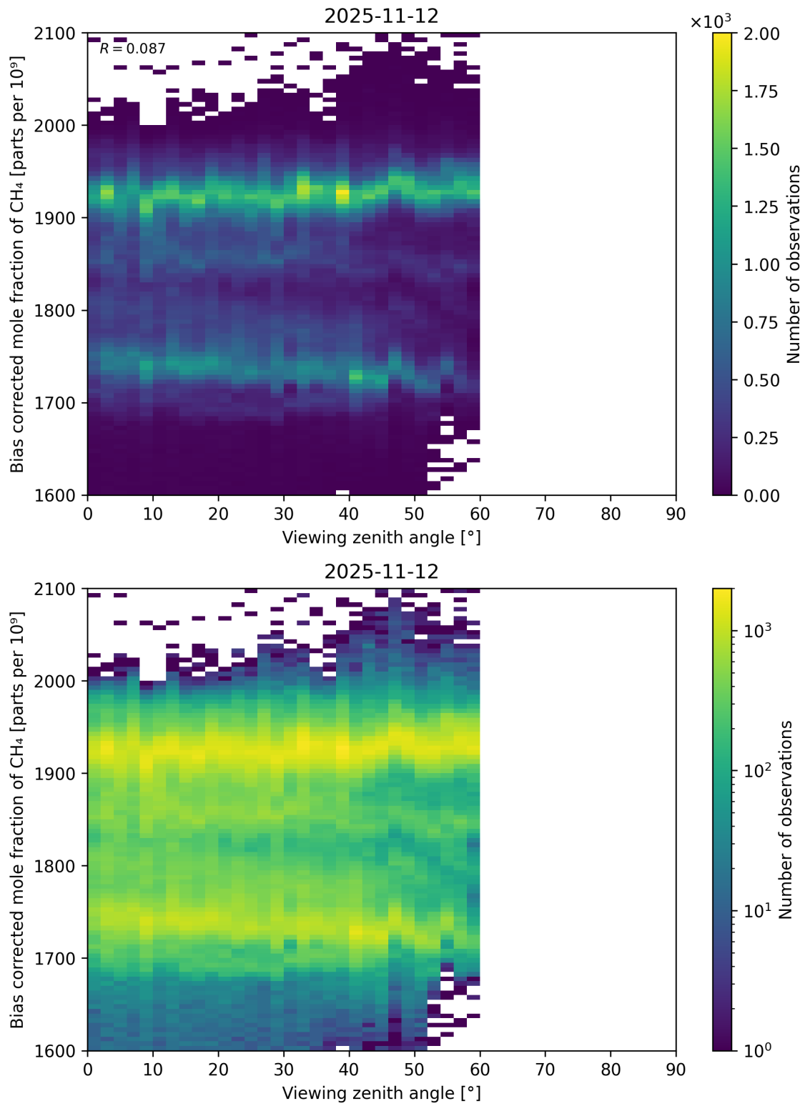
Figure 111: Scatter density plot of “Viewing zenith angle” against “Bias corrected mole fraction of CH 4 ” for 2025-11-12 to 2025-11-13.
