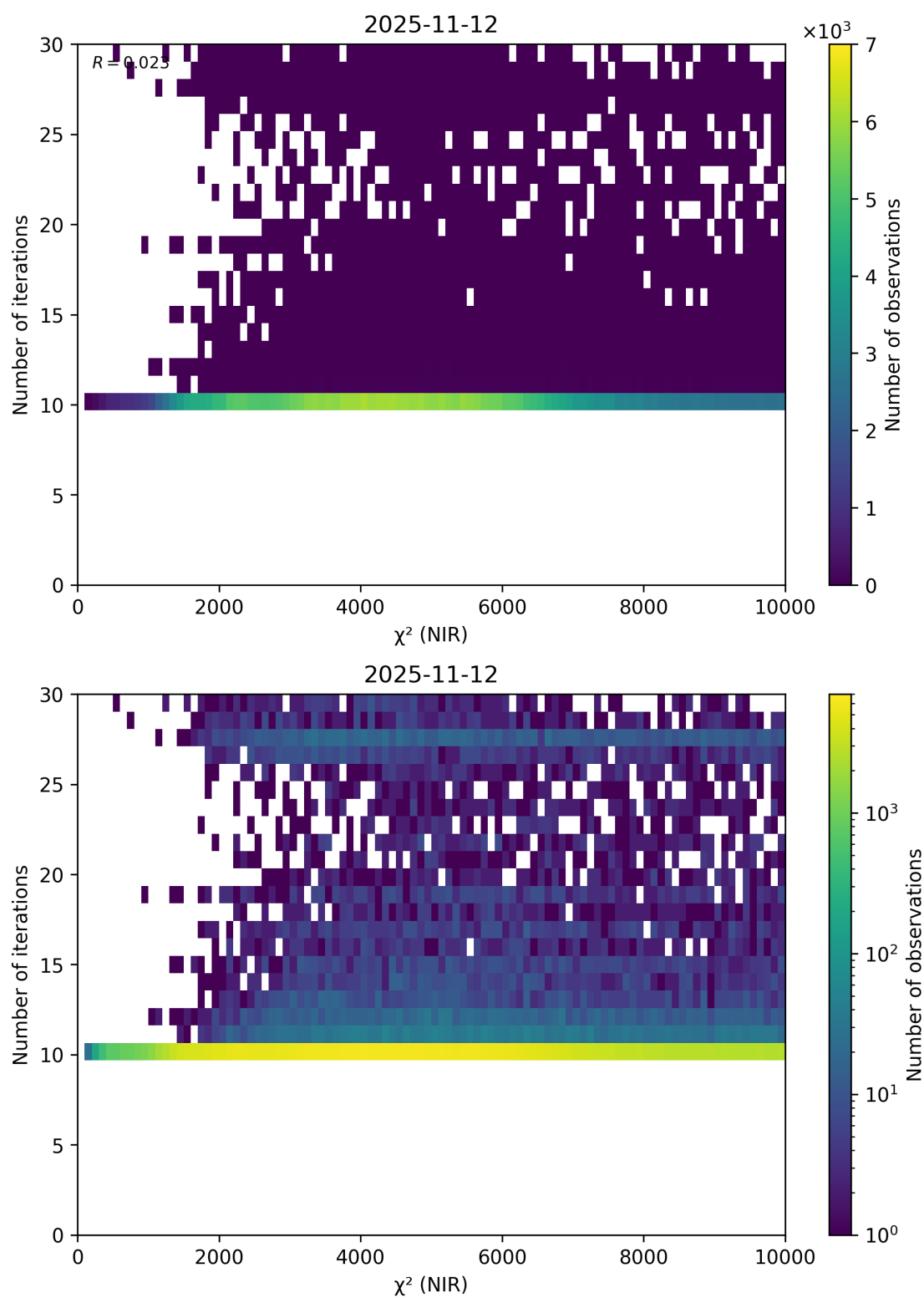
Figure 46: Scatter density plot of “ \chi^2 (NIR)” against “Number of iterations” for 2025-11-12 to 2025-11-13.
