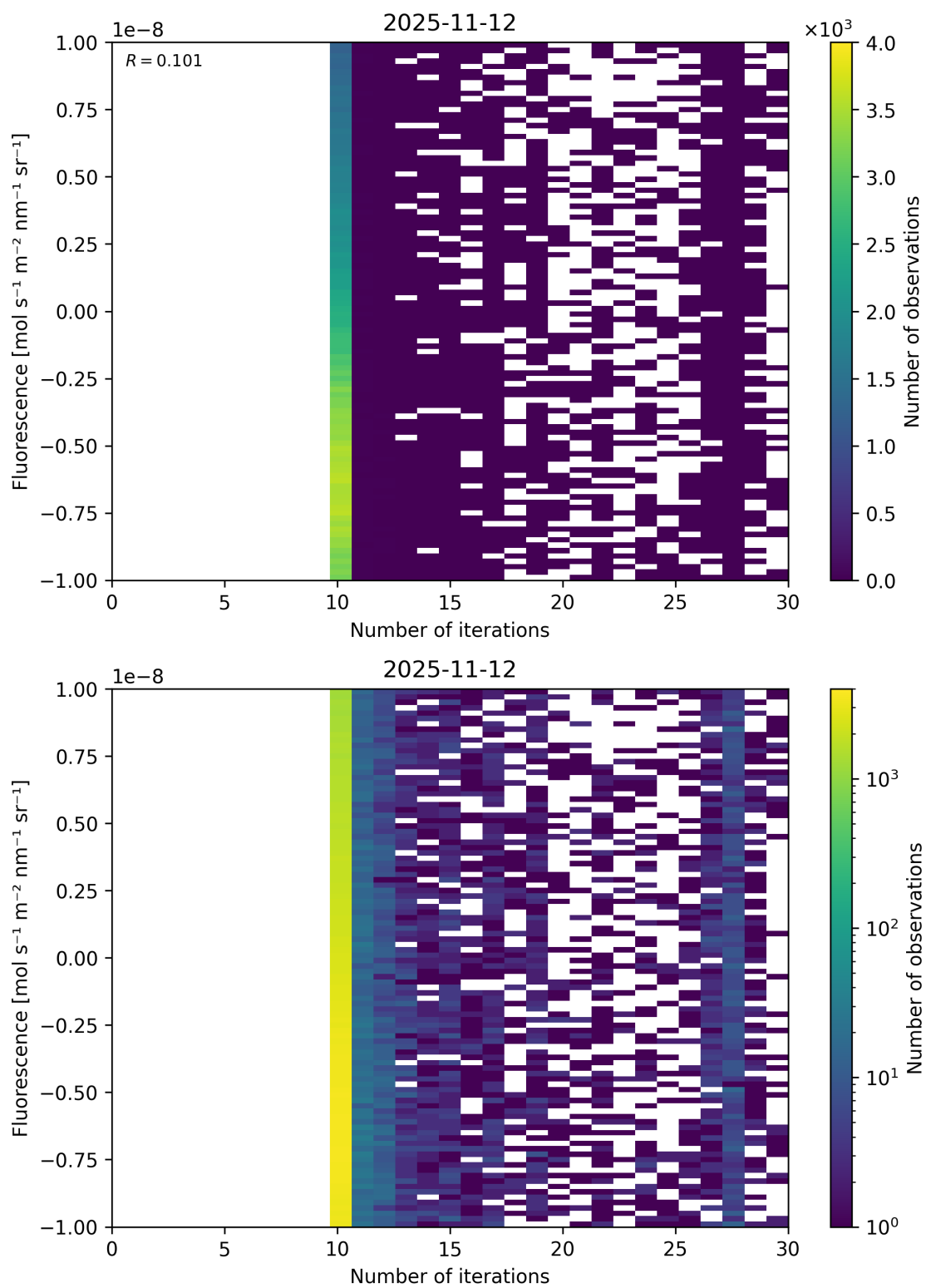
Figure 87: Scatter density plot of “Number of iterations” against “Fluorescence” for 2025-11-12 to 2025-11-13.
