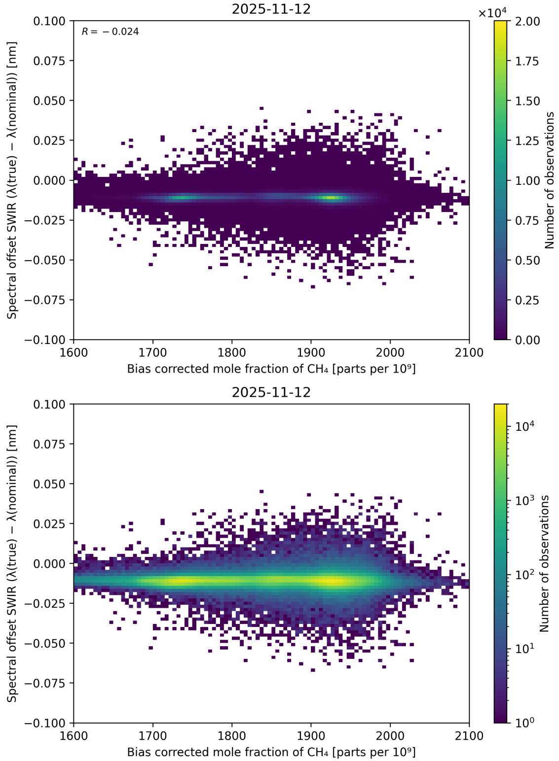
Figure 69: Scatter density plot of “Bias corrected mole fraction of \text{CH}_4 ” against “Spectral offset SWIR ( \lambda_{\text{true}} - \lambda_{\text{nominal}} )” for 2025-11-12 to 2025-11-13.
