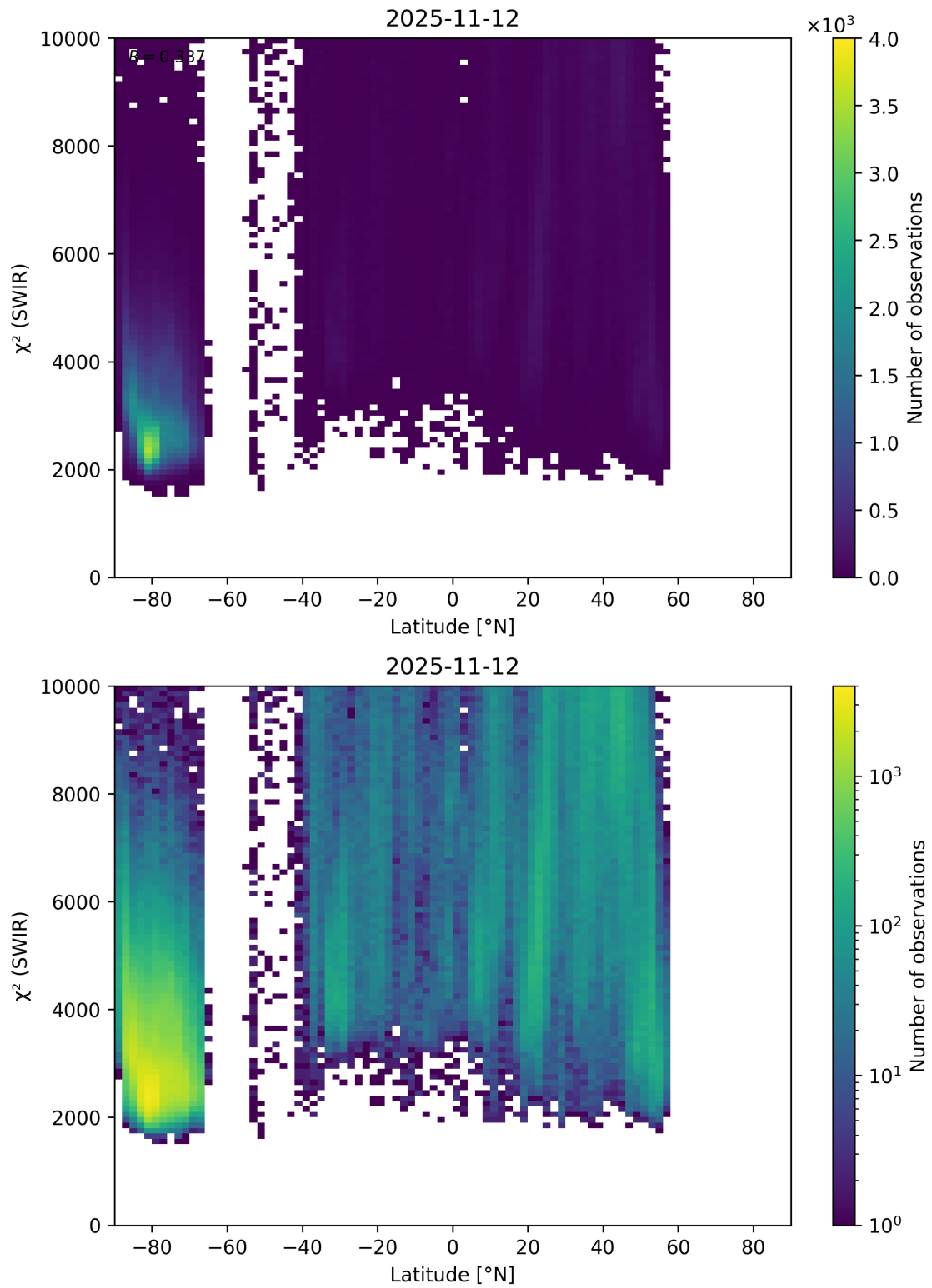
Figure 54: Scatter density plot of “Latitude” against “ \chi^2 (SWIR)” for 2025-11-12 to 2025-11-13.
