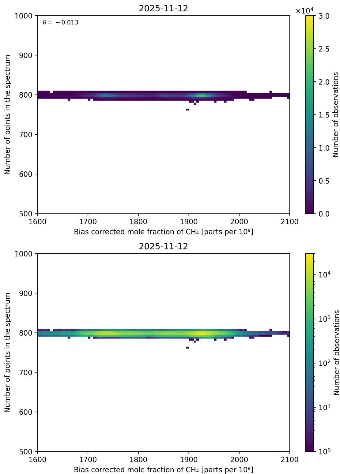
Figure 68: Scatter density plot of “Bias corrected mole fraction of CH 4 ” against “Number of points in the spectrum” for 2025-11-12 to 2025-11-13.
