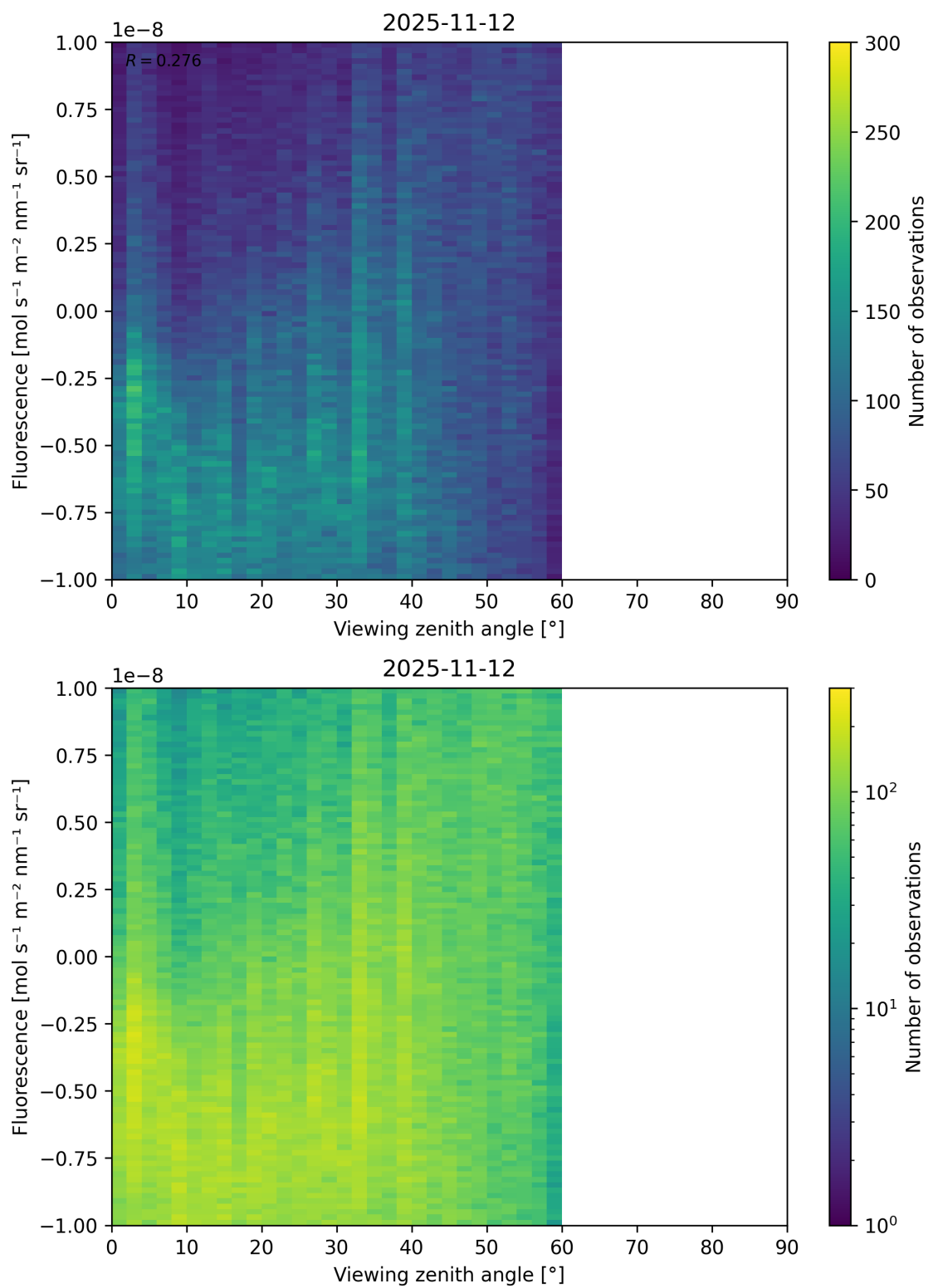
Figure 108: Scatter density plot of “Viewing zenith angle” against “Fluorescence” for 2025-11-12 to 2025-11-13.
