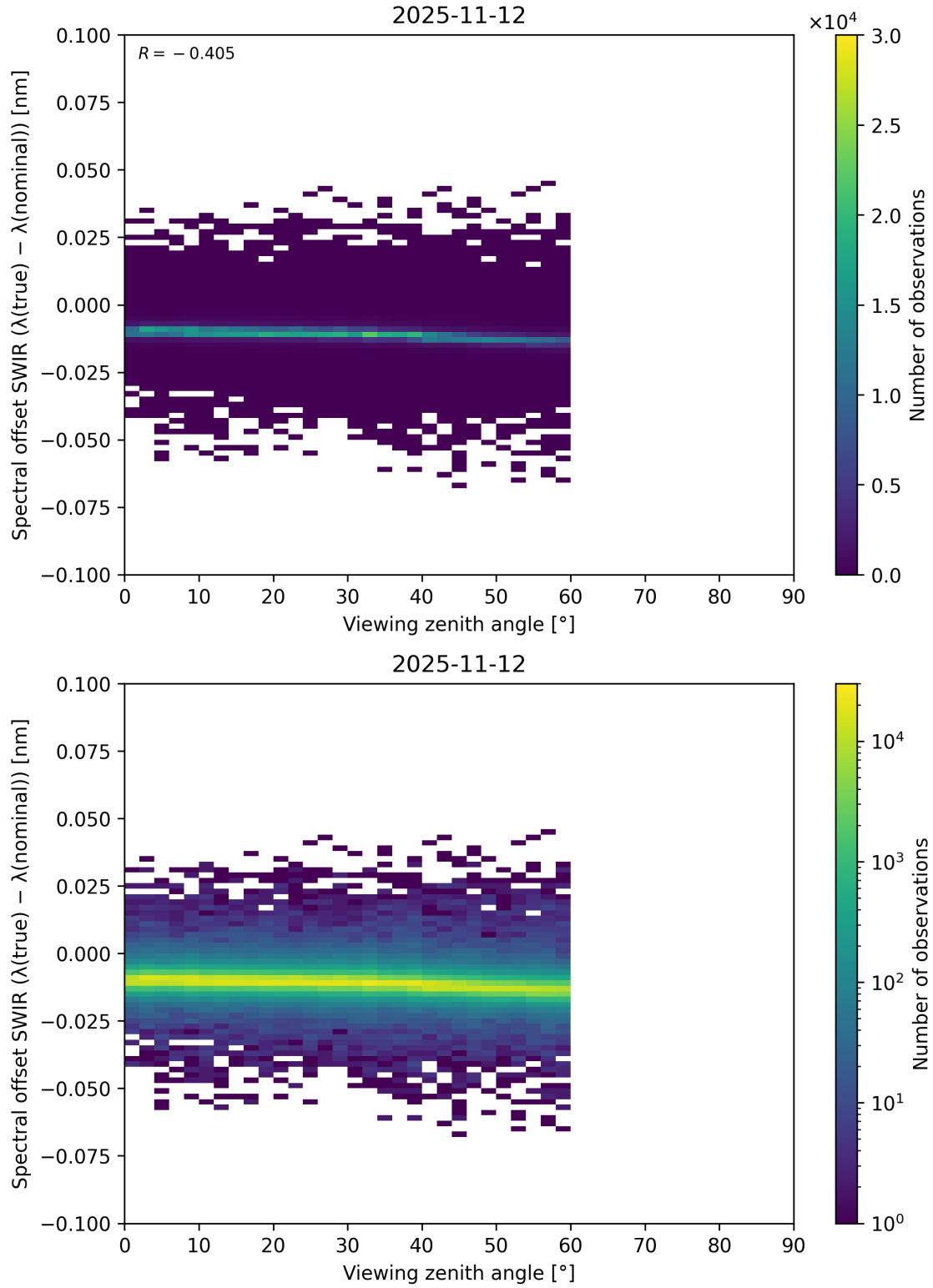
Figure 116: Scatter density plot of “Viewing zenith angle” against “Spectral offset SWIR ( \lambda_{\text{true}} - \lambda_{\text{nominal}} )” for 2025-11-12 to 2025-11-13.
