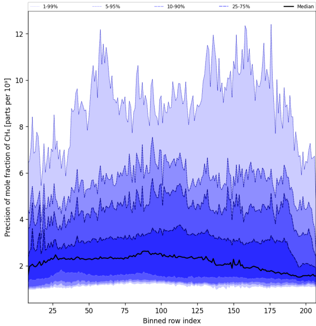
Figure 35: Along track statistics of “Precision of mole fraction of CH 4 ” for 2025-11-12 to 2025-11-13
