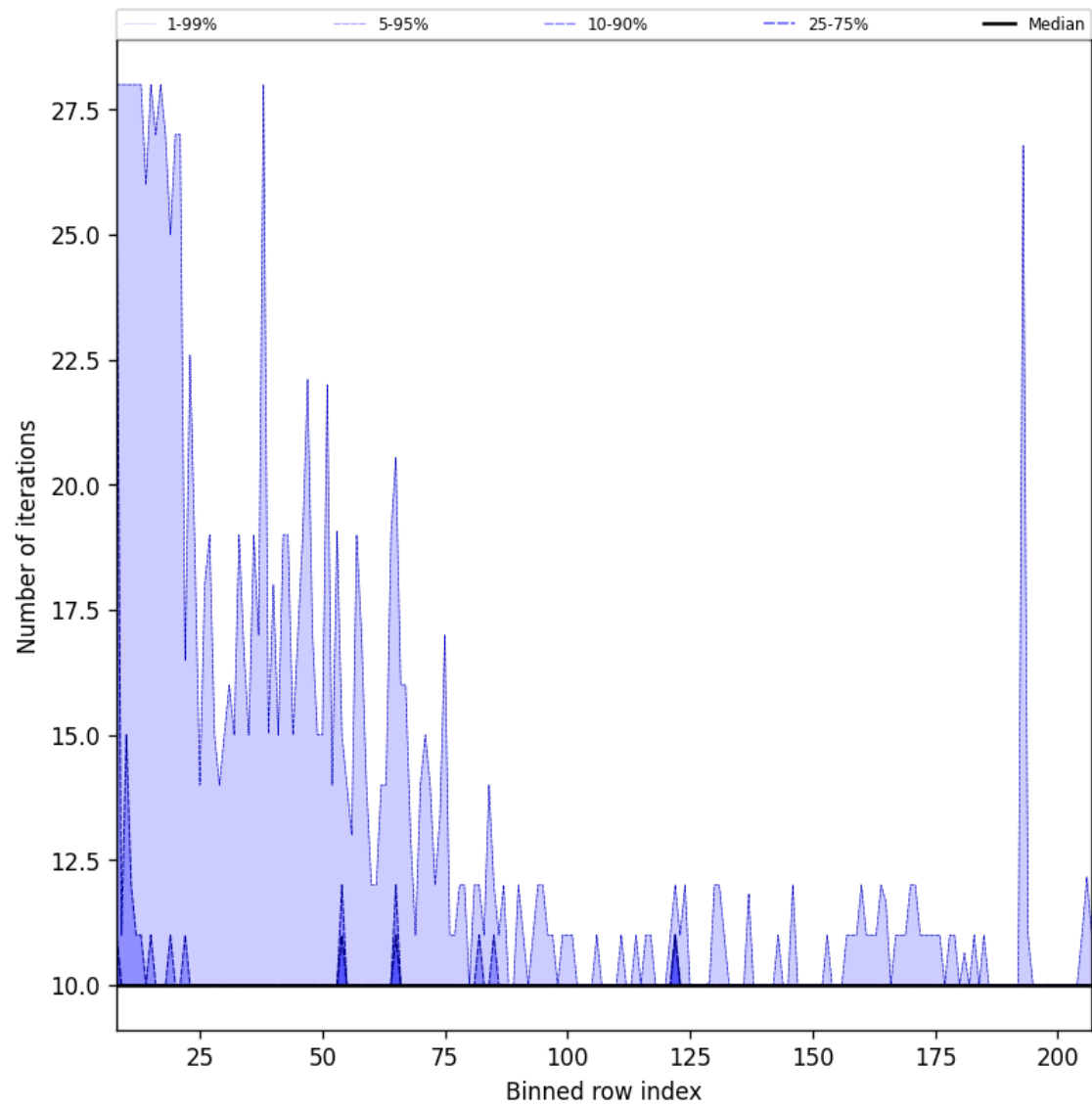
Figure 42: Along track statistics of “Number of iterations” for 2025-11-12 to 2025-11-13
