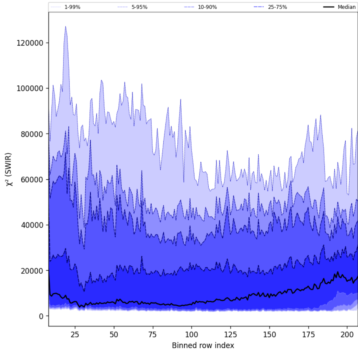
Figure 39: Along track statistics of “ \chi^2 (SWIR)” for 2025-11-12 to 2025-11-13
