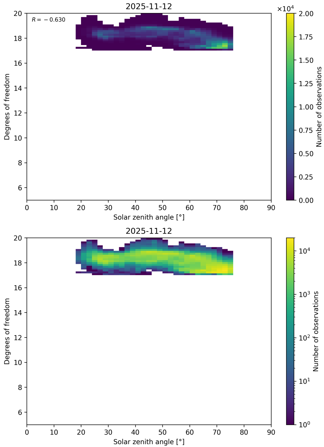
Figure 96: Scatter density plot of “Solar zenith angle” against “Degrees of freedom” for 2025-11-12 to 2025-11-13.
