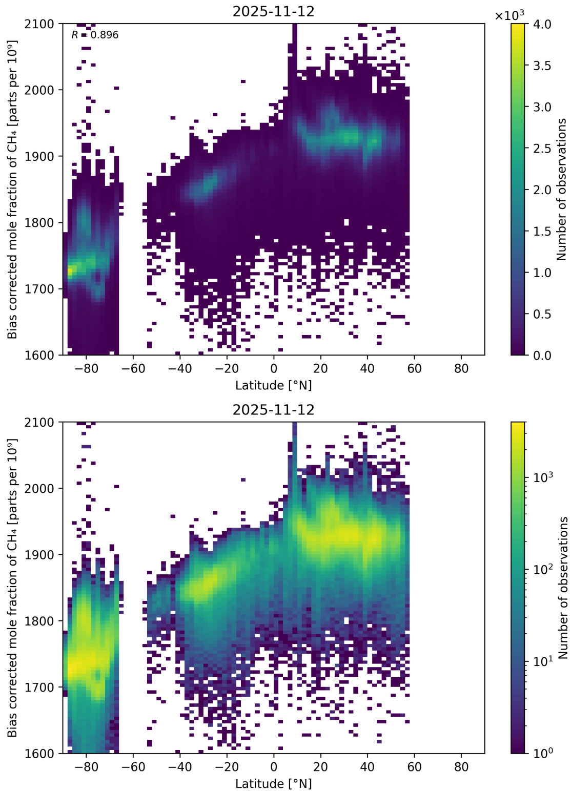
Figure 58: Scatter density plot of “Latitude” against “Bias corrected mole fraction of CH 4 ” for 2025-11-12 to 2025-11-13.
