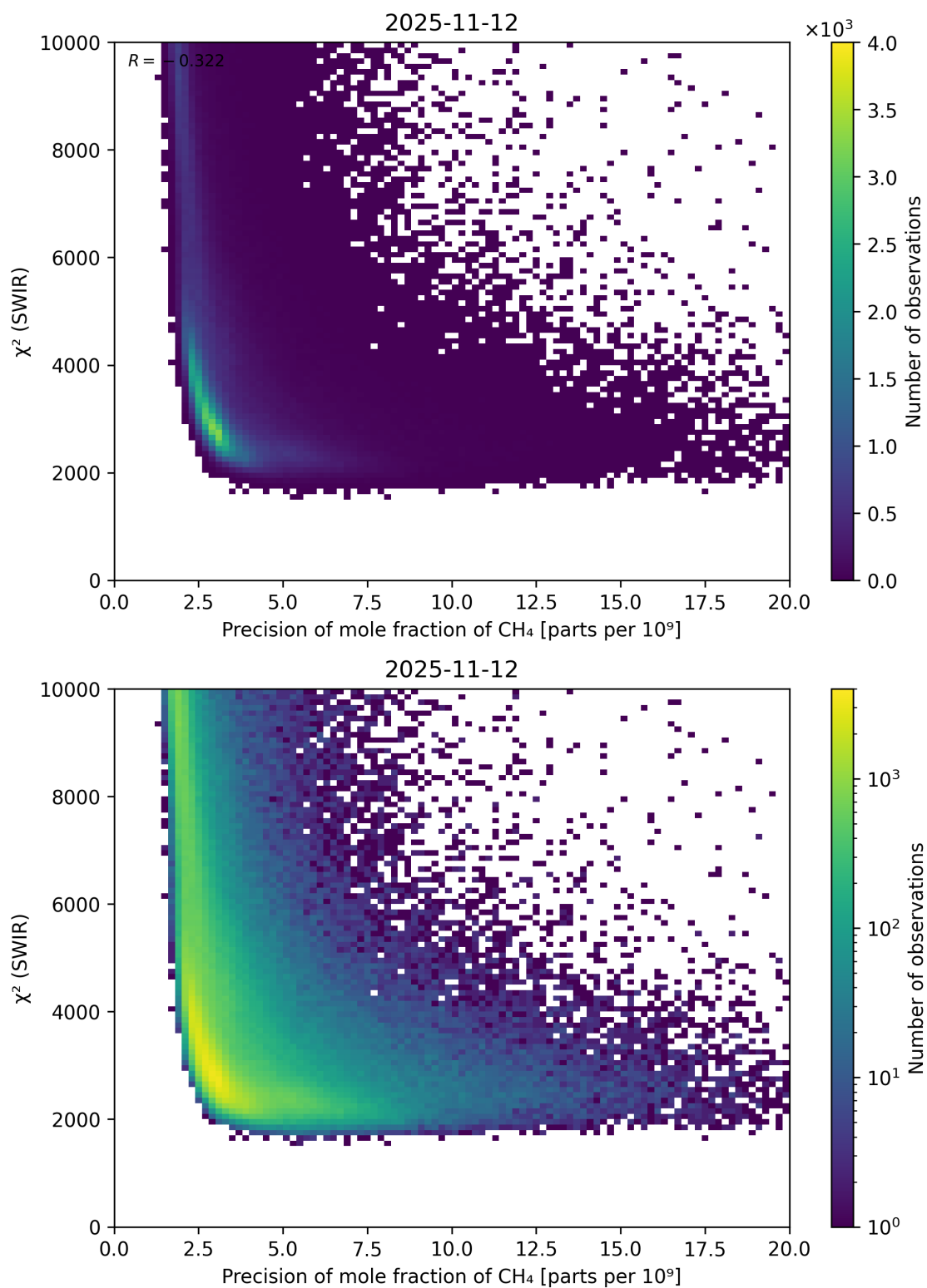
Figure 79: Scatter density plot of “Precision of mole fraction of \text{CH}_4 ” against “ \chi^2 (SWIR)” for 2025-11-12 to 2025-11-13.
