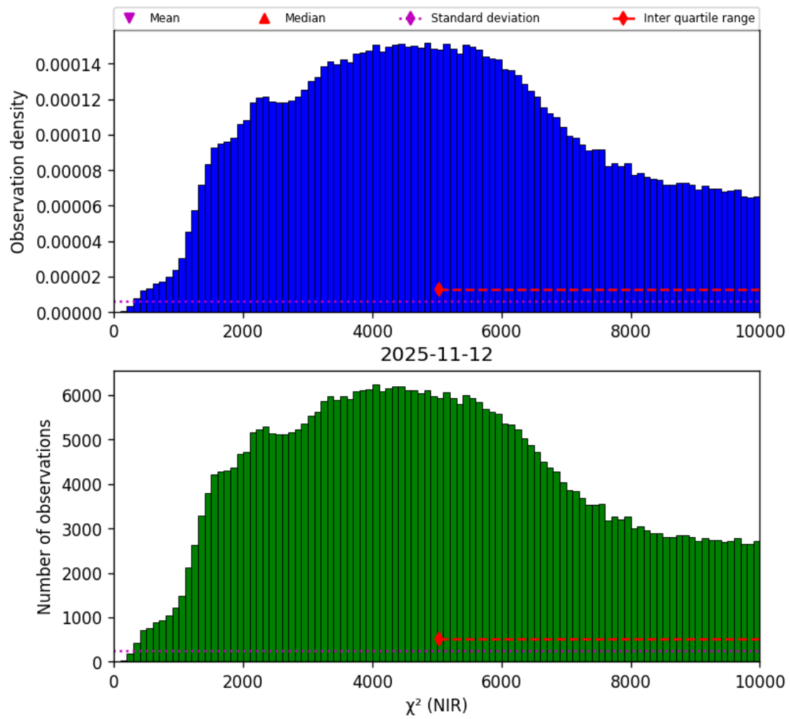
Figure 29: Histogram of “ \chi^2 (NIR)” for 2025-11-12 to 2025-11-13
