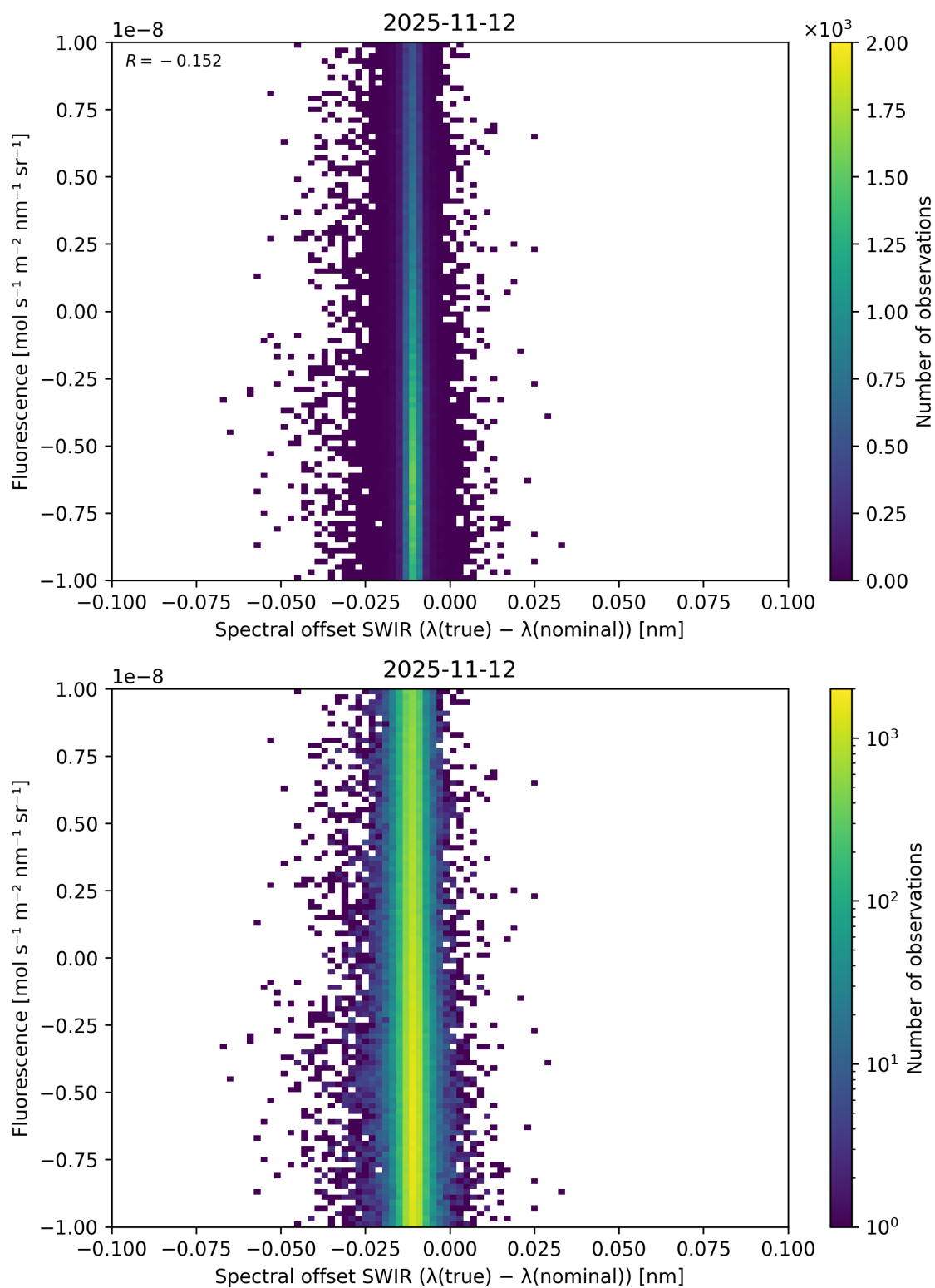
Figure 120: Scatter density plot of “Spectral offset SWIR ( \lambda_{\text{true}} - \lambda_{\text{nominal}} )” against “Fluorescence” for 2025-11-12 to 2025-11-13.
