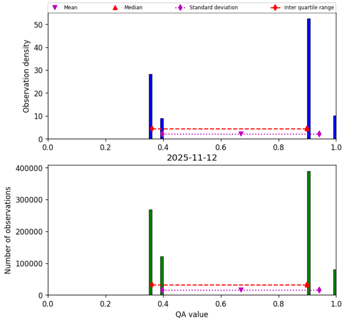
Figure 22: Histogram of “QA value” for 2025-11-12 to 2025-11-13
