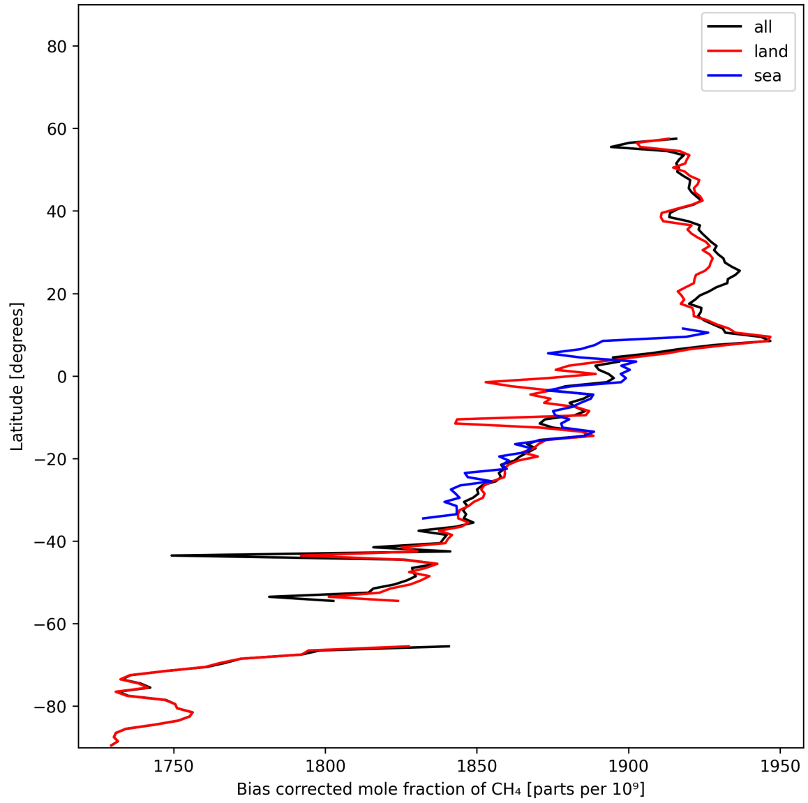
Figure 14: Zonal average of “Bias corrected mole fraction of \text{CH}_4 ” for 2025-11-12 to 2025-11-13.
