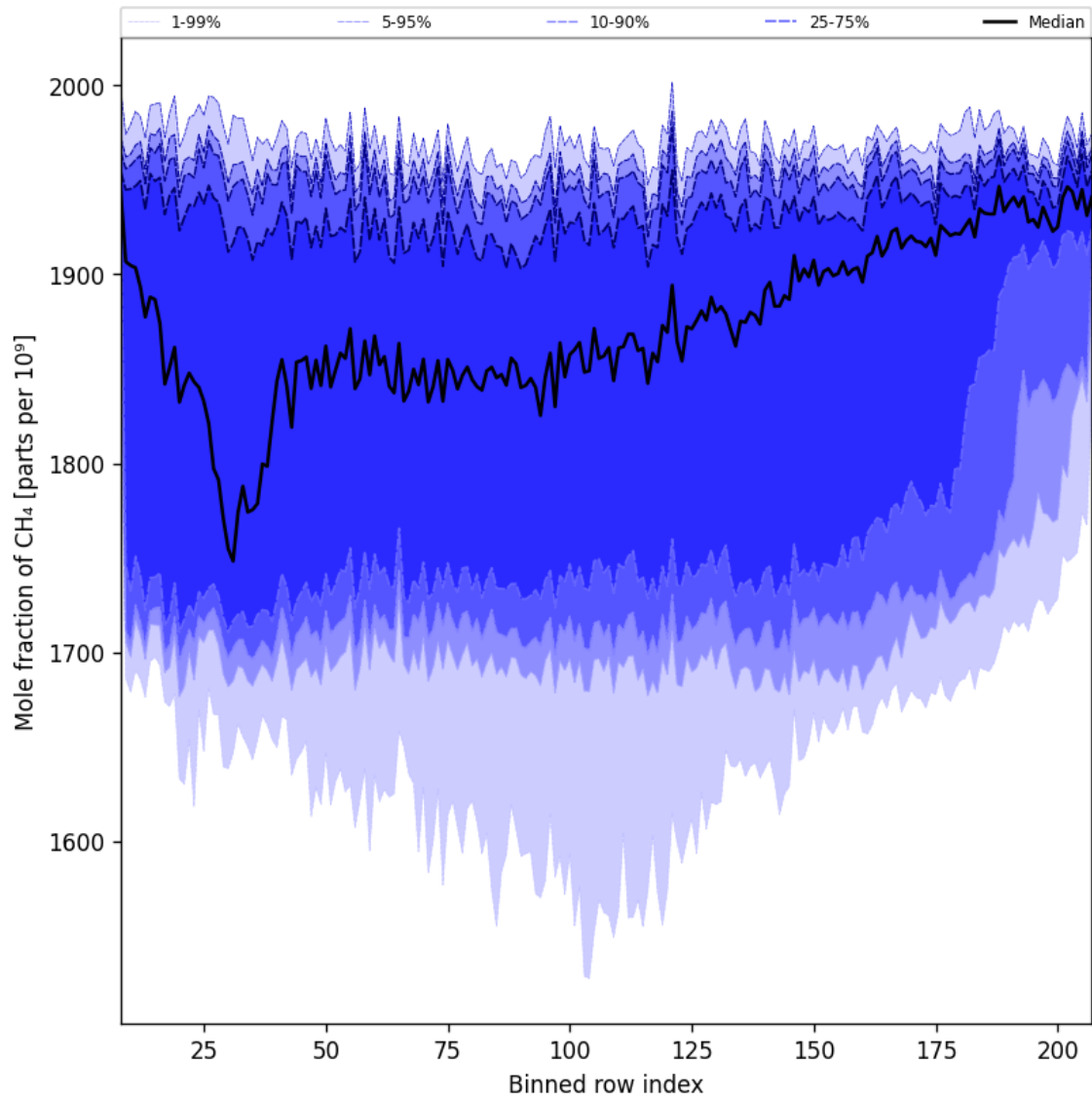
Figure 34: Along track statistics of “Mole fraction of CH 4 ” for 2025-11-12 to 2025-11-13
