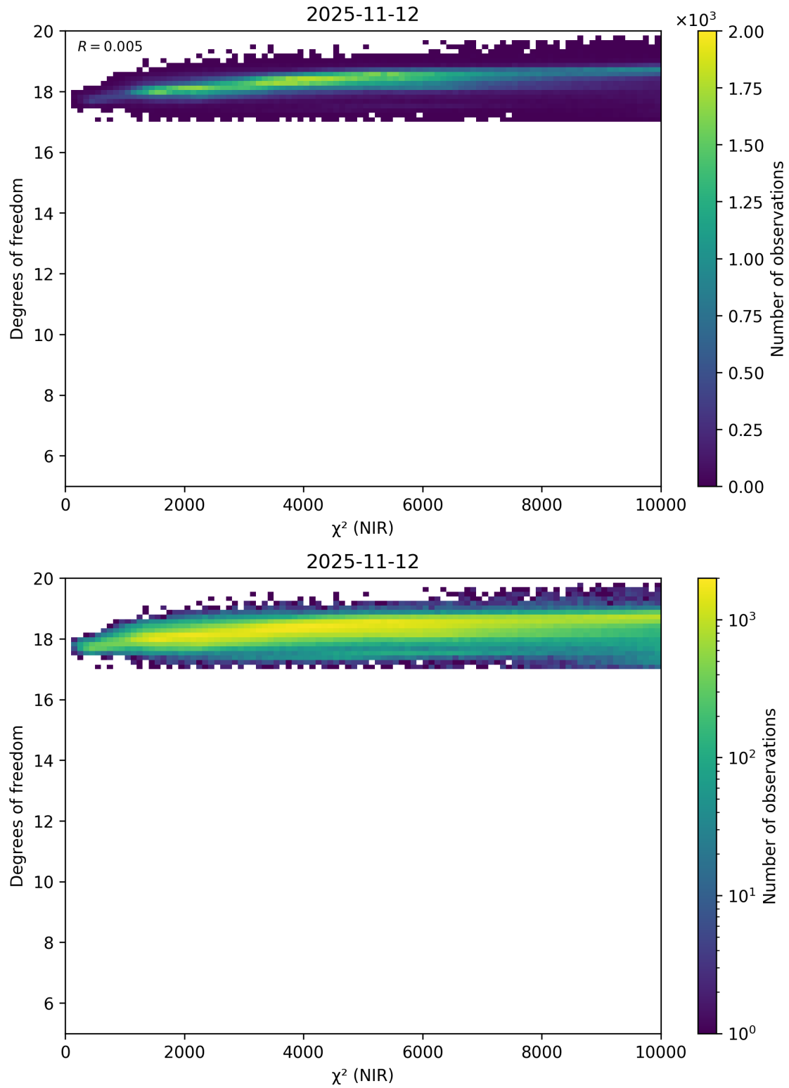
Figure 44: Scatter density plot of “ \chi^2 (NIR)” against “Degrees of freedom” for 2025-11-12 to 2025-11-13.
