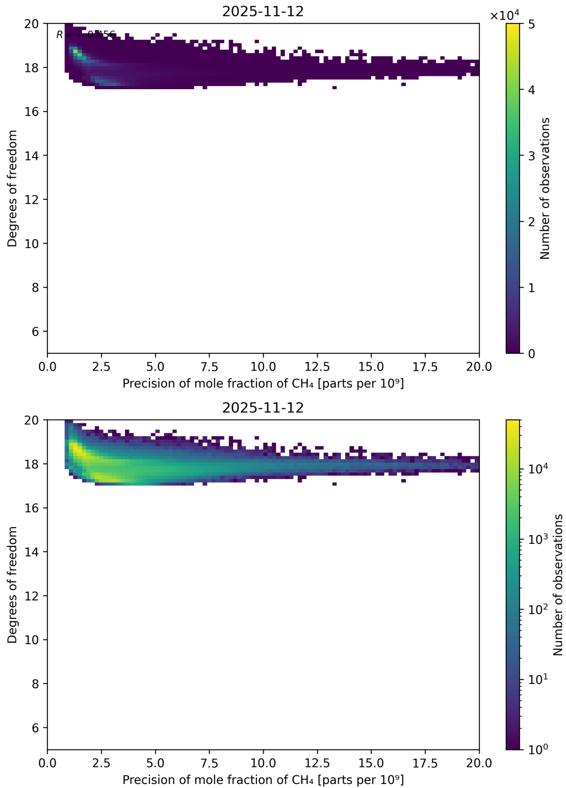
Figure 80: Scatter density plot of “Precision of mole fraction of CH 4 ” against “Degrees of freedom” for 2025-11-12 to 2025-11-13.
