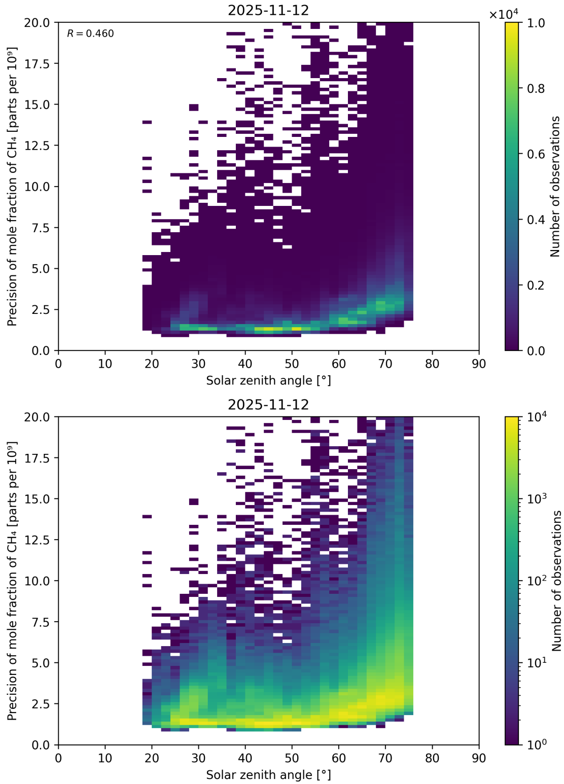
Figure 101: Scatter density plot of “Solar zenith angle” against “Precision of mole fraction of \text{CH}_4 ” for 2025-11-12 to 2025-11-13.
