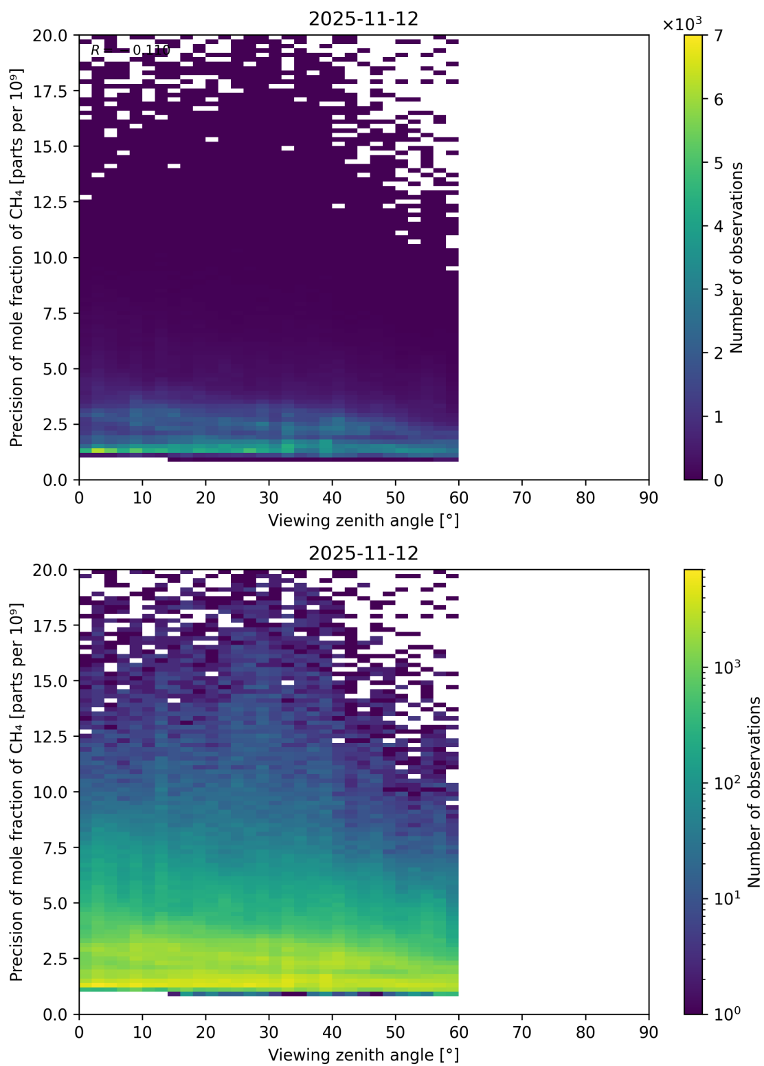
Figure 112: Scatter density plot of “Viewing zenith angle” against “Precision of mole fraction of CH 4 ” for 2025-11-12 to 2025-11-13.
