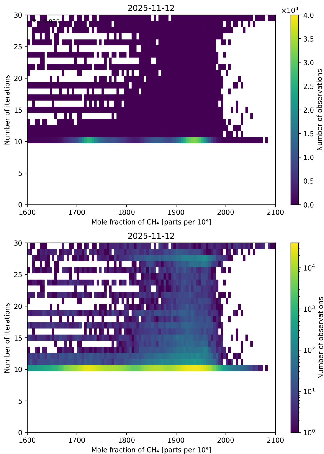
Figure 76: Scatter density plot of “Mole fraction of CH 4 ” against “Number of iterations” for 2025-11-12 to 2025-11-13.
