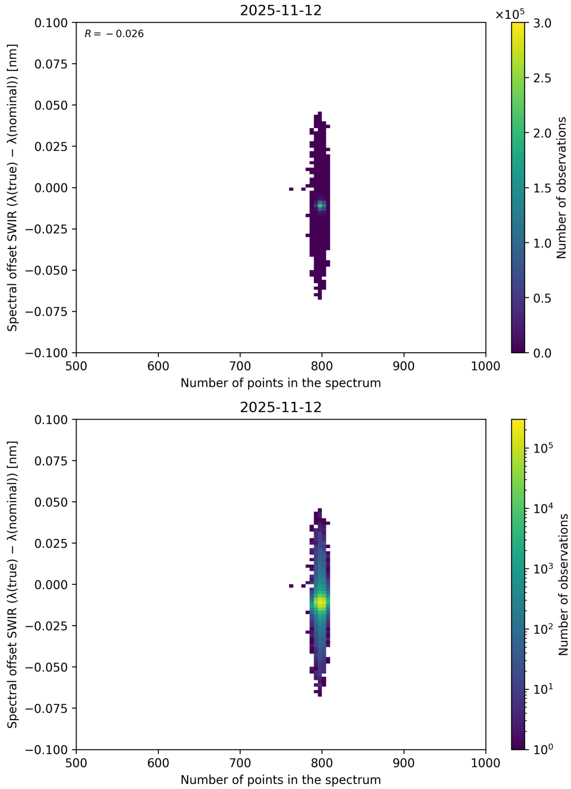
Figure 93: Scatter density plot of “Number of points in the spectrum” against “Spectral offset SWIR ( \lambda_{\text{true}} - \lambda_{\text{nominal}} )” for 2025-11-12 to 2025-11-13.
