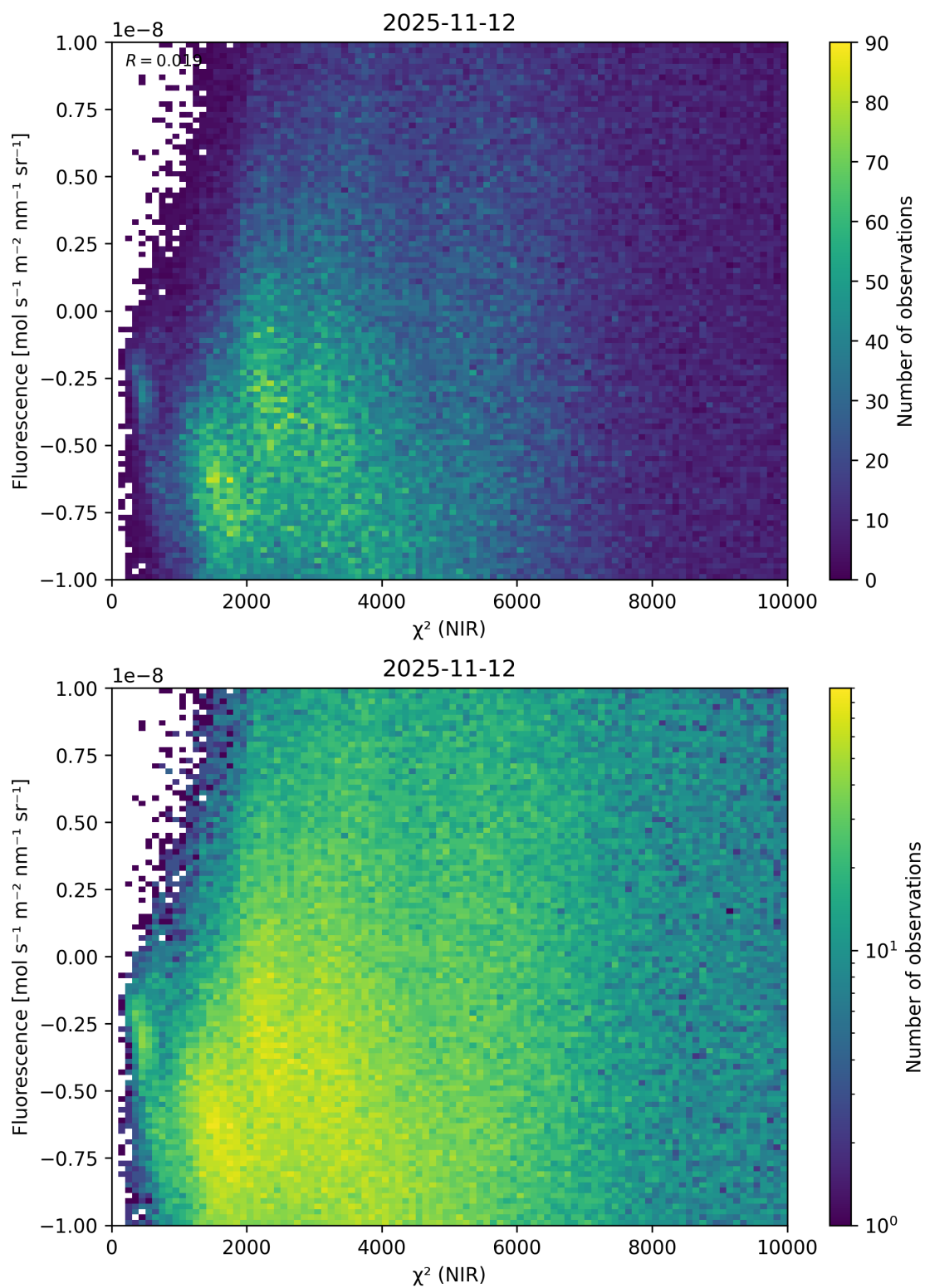
Figure 45: Scatter density plot of “ \chi^2 (NIR)” against “Fluorescence” for 2025-11-12 to 2025-11-13.
