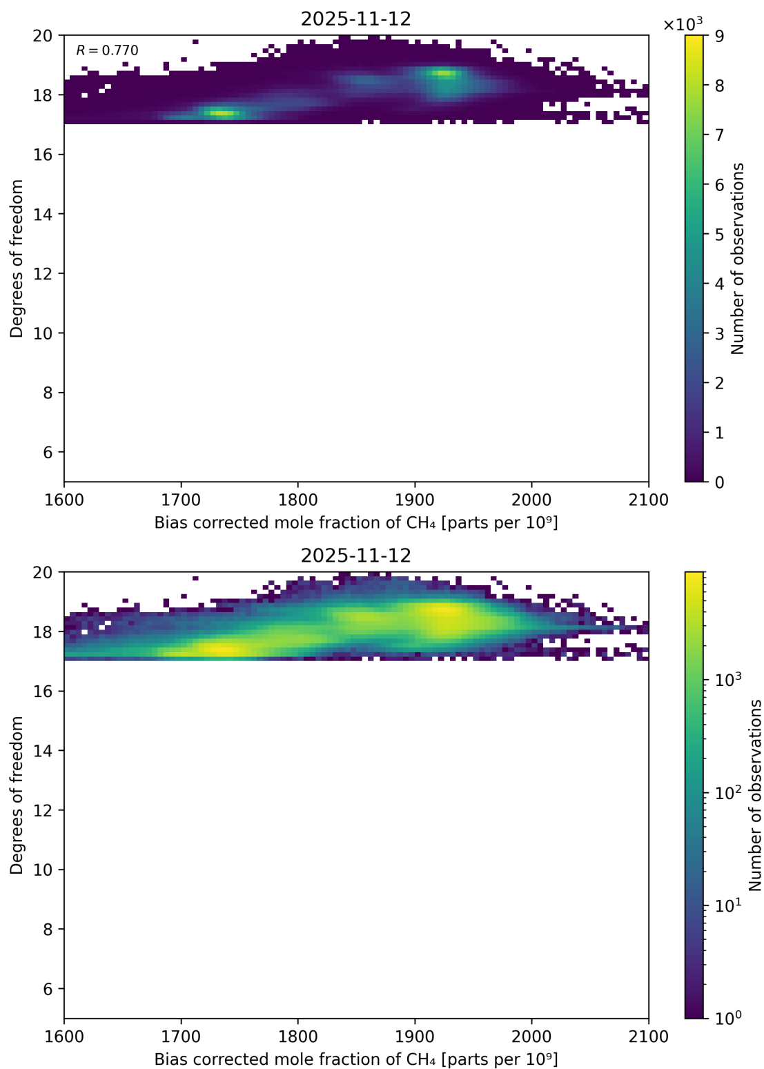
Figure 65: Scatter density plot of “Bias corrected mole fraction of CH 4 ” against “Degrees of freedom” for 2025-11-12 to 2025-11-13.
