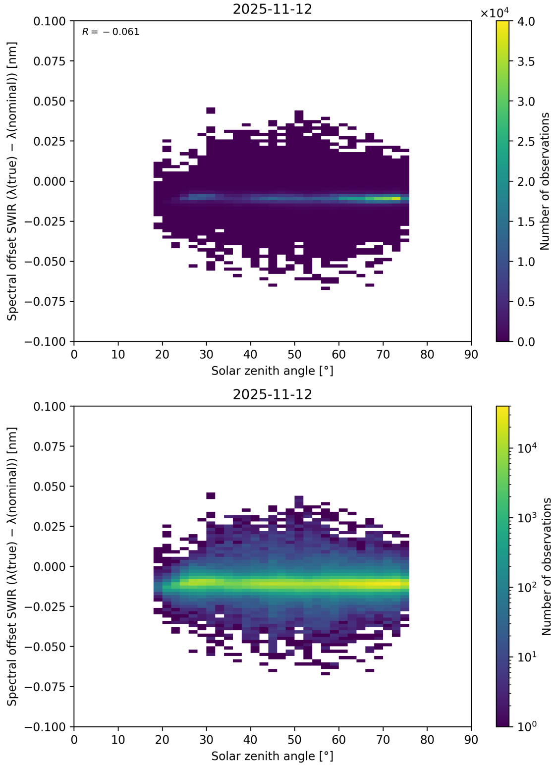
Figure 104: Scatter density plot of “Solar zenith angle” against “Spectral offset SWIR ( \lambda_{\text{true}} - \lambda_{\text{nominal}} )” for 2025-11-12 to 2025-11-13.
