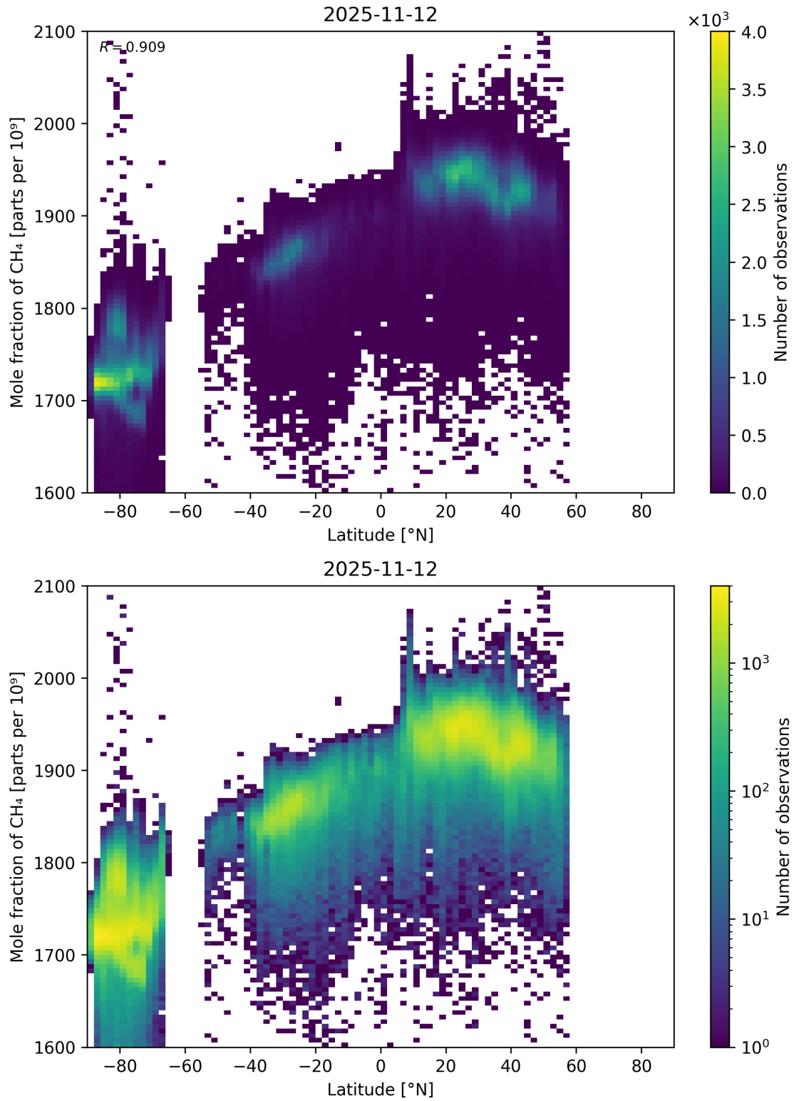
Figure 57: Scatter density plot of “Latitude” against “Mole fraction of CH 4 ” for 2025-11-12 to 2025-11-13.
