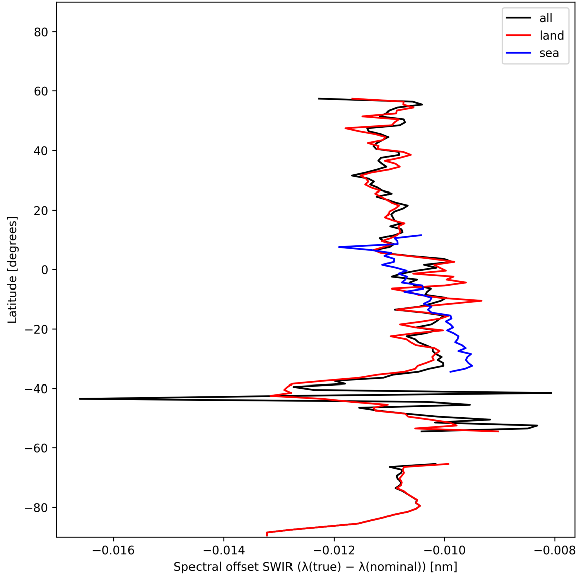
Figure 16: Zonal average of “Spectral offset SWIR ( \lambda_{\text{true}} - \lambda_{\text{nominal}} )” for 2025-11-12 to 2025-11-13.
