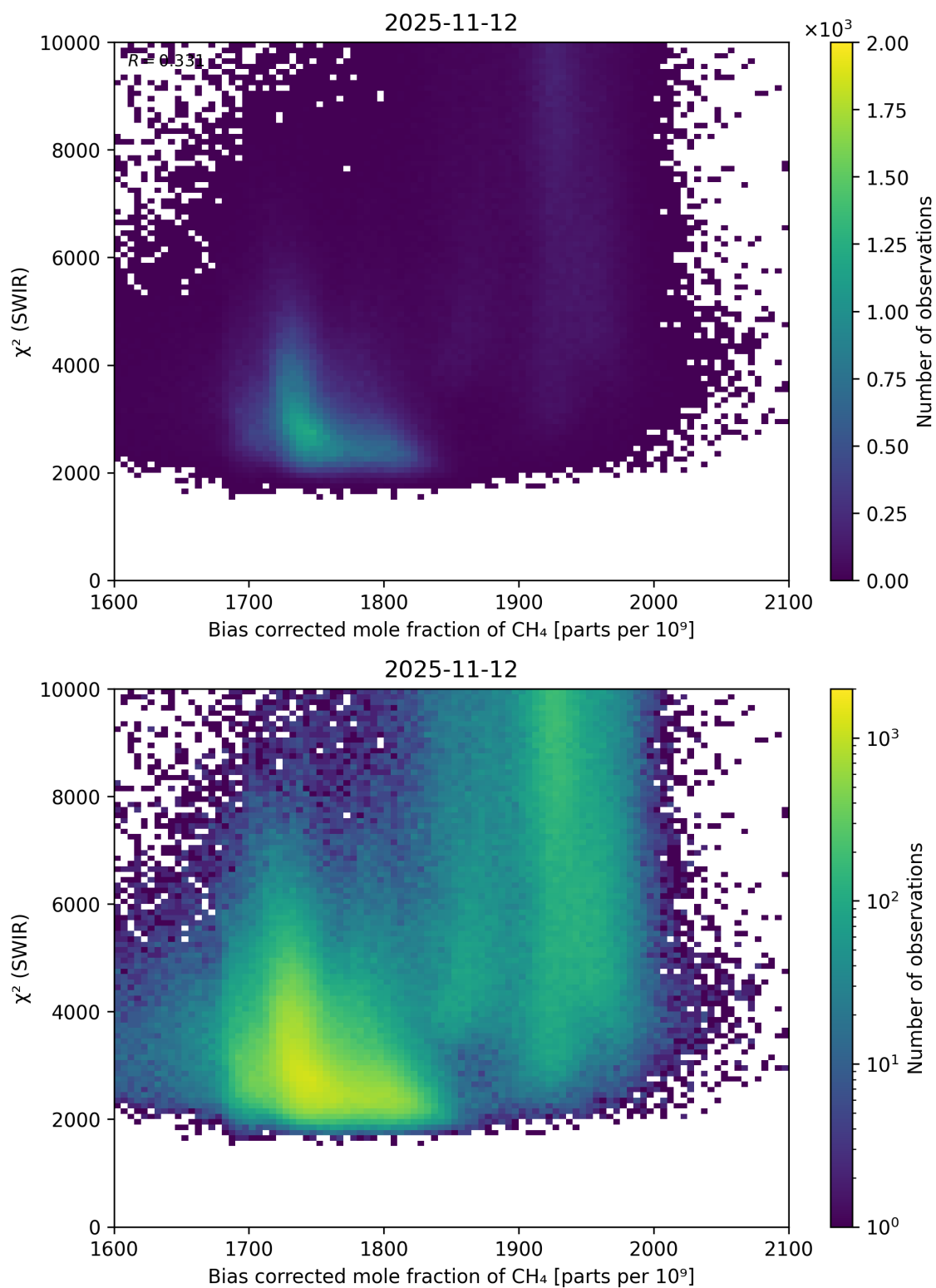
Figure 64: Scatter density plot of “Bias corrected mole fraction of CH 4 ” against “ \chi^2 (SWIR)” for 2025-11-12 to 2025-11-13.
