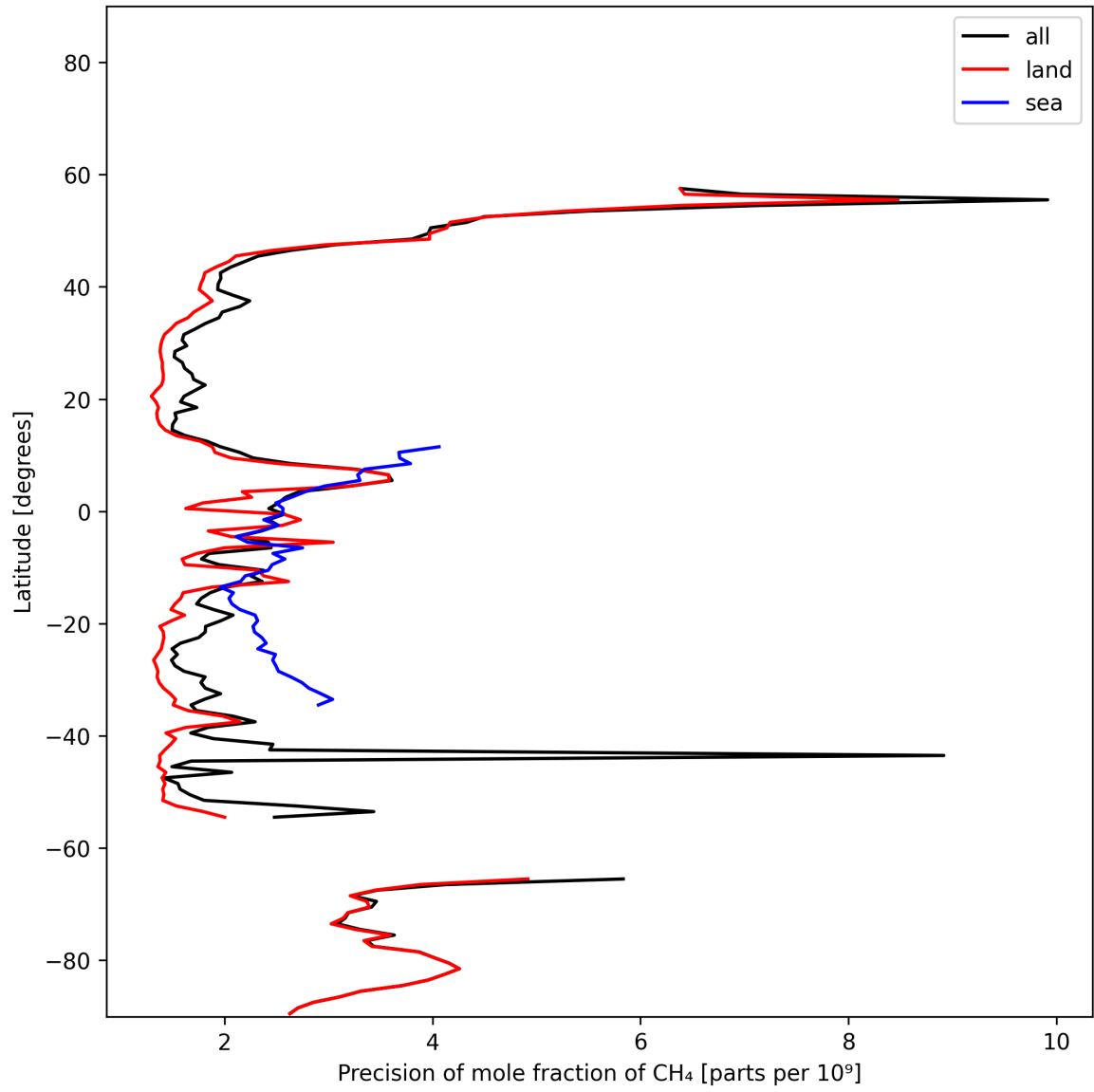
Figure 13: Zonal average of “Precision of mole fraction of CH 4 ” for 2025-11-12 to 2025-11-13.
