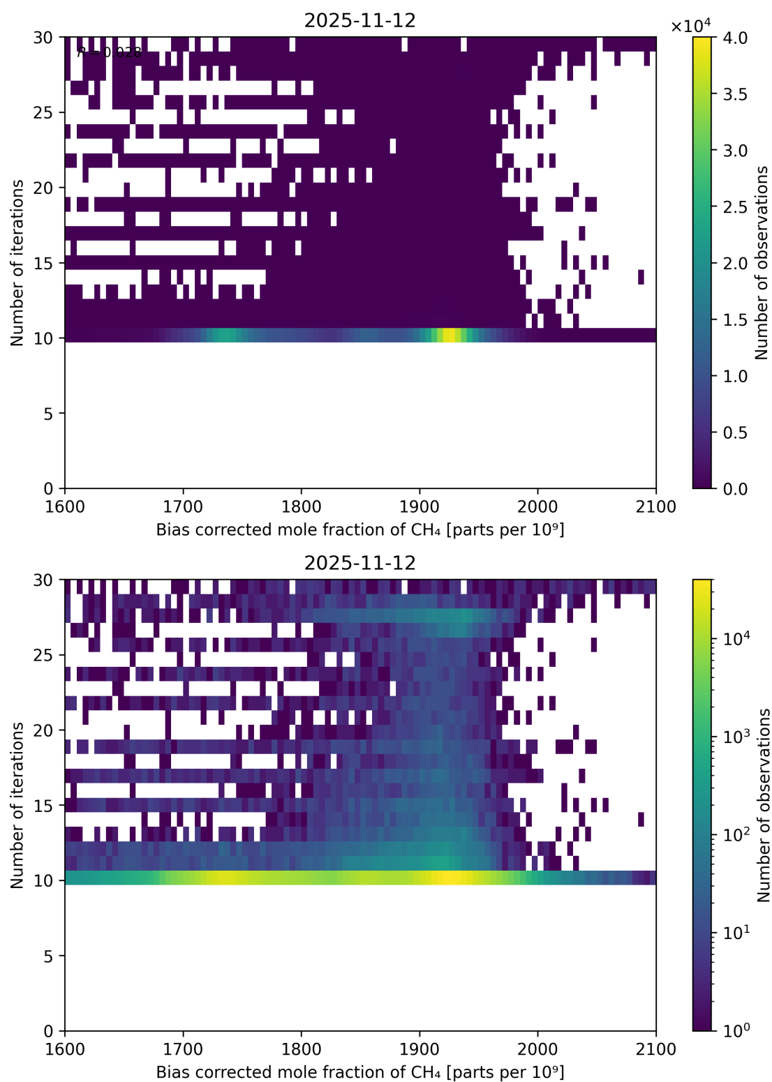
Figure 67: Scatter density plot of “Bias corrected mole fraction of \text{CH}_4 ” against “Number of iterations” for 2025-11-12 to 2025-11-13.
