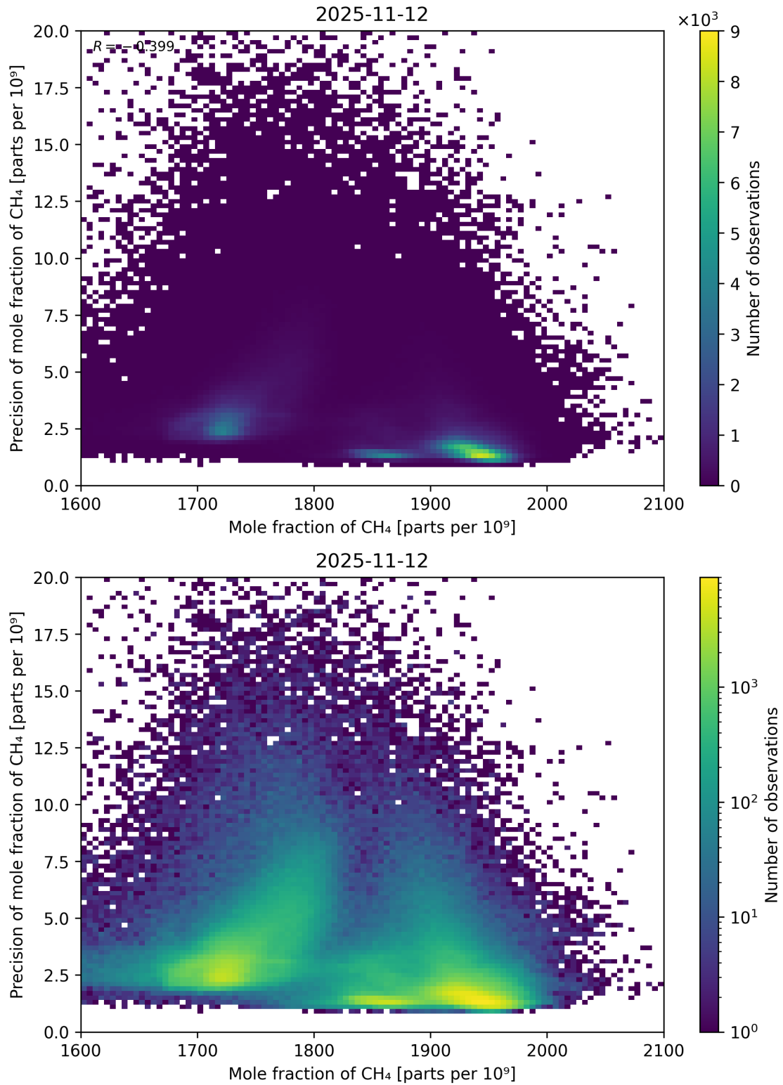
Figure 75: Scatter density plot of “Mole fraction of CH 4 ” against “Precision of mole fraction of CH 4 ” for 2025-11-12 to 2025-11-13.
