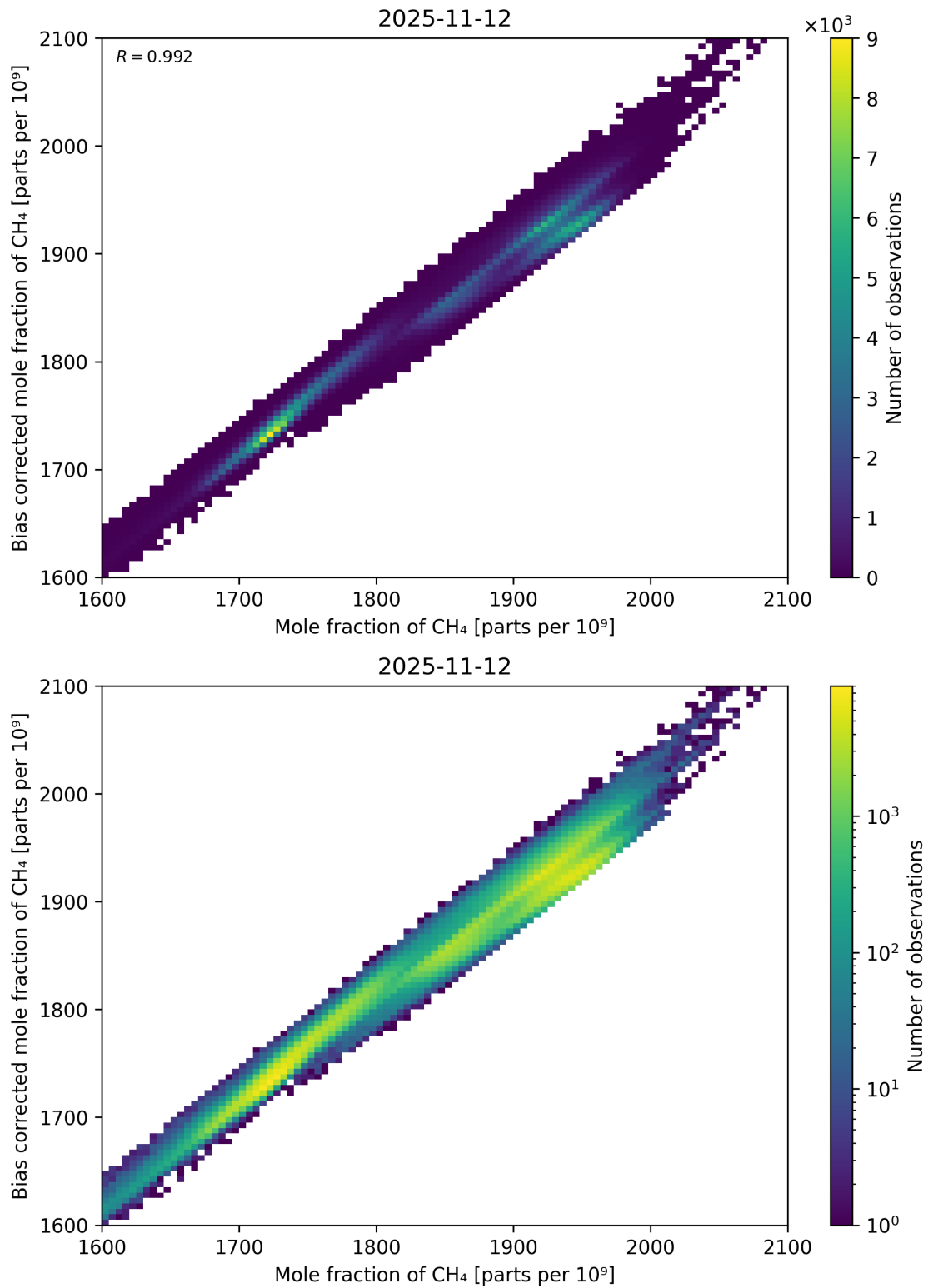
Figure 74: Scatter density plot of “Mole fraction of CH 4 ” against “Bias corrected mole fraction of CH 4 ” for 2025-11-12 to 2025-11-13.
