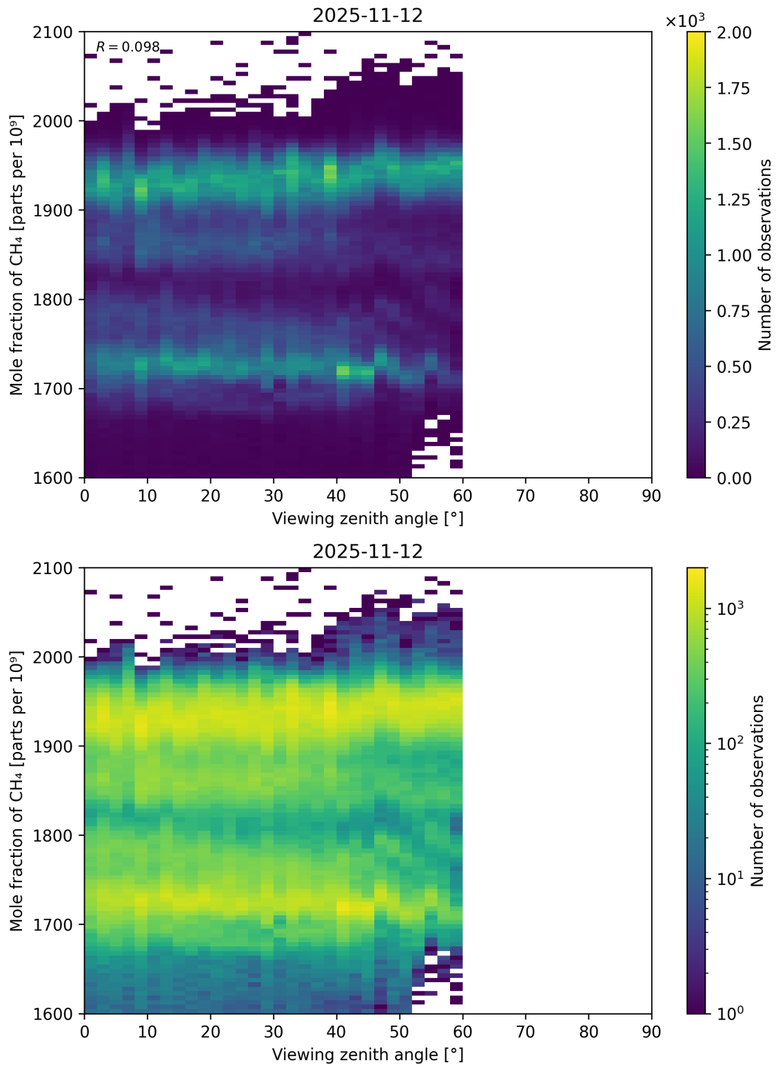
Figure 110: Scatter density plot of “Viewing zenith angle” against “Mole fraction of CH 4 ” for 2025-11-12 to 2025-11-13.
