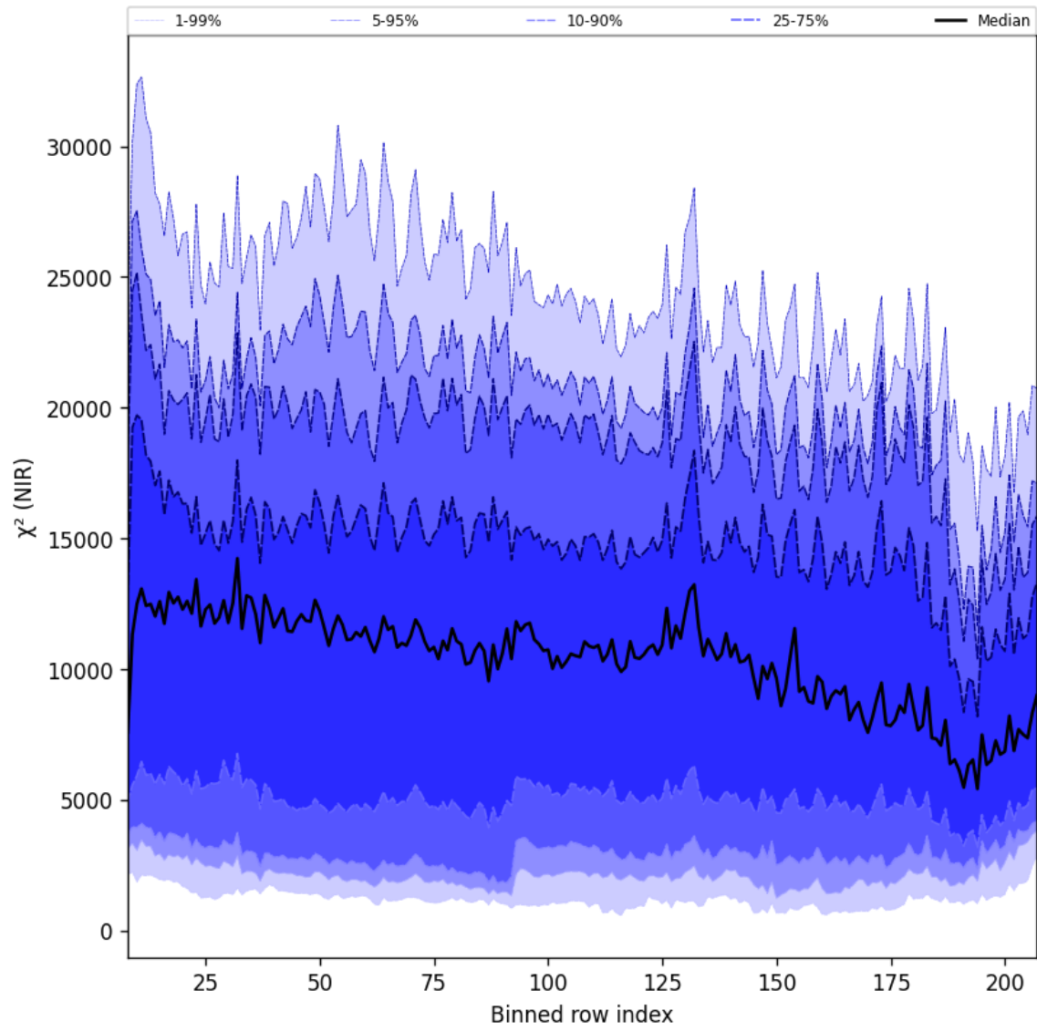
Figure 40: Along track statistics of “ \chi^2 (NIR)” for 2025-11-12 to 2025-11-13
