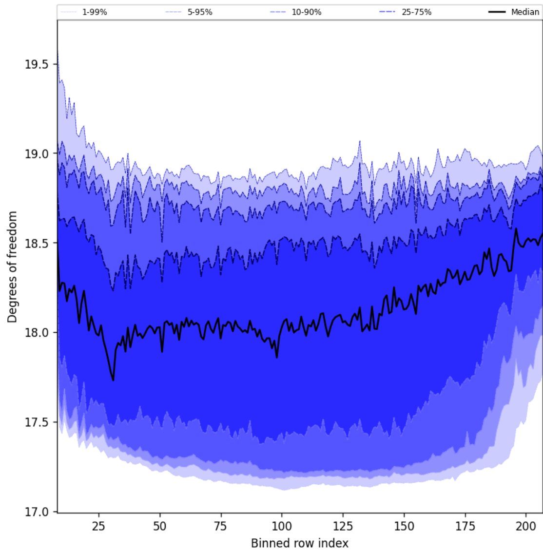
Figure 41: Along track statistics of “Degrees of freedom” for 2025-11-12 to 2025-11-13
