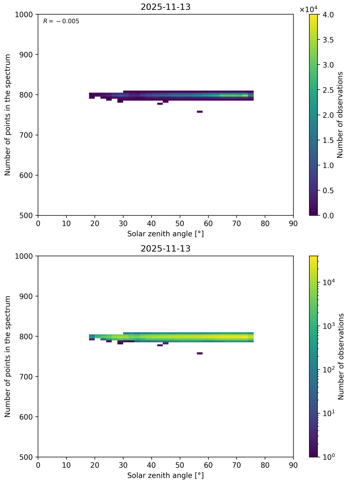
Figure 103: Scatter density plot of “Solar zenith angle” against “Number of points in the spectrum” for 2025-11-12 to 2025-11-14.
