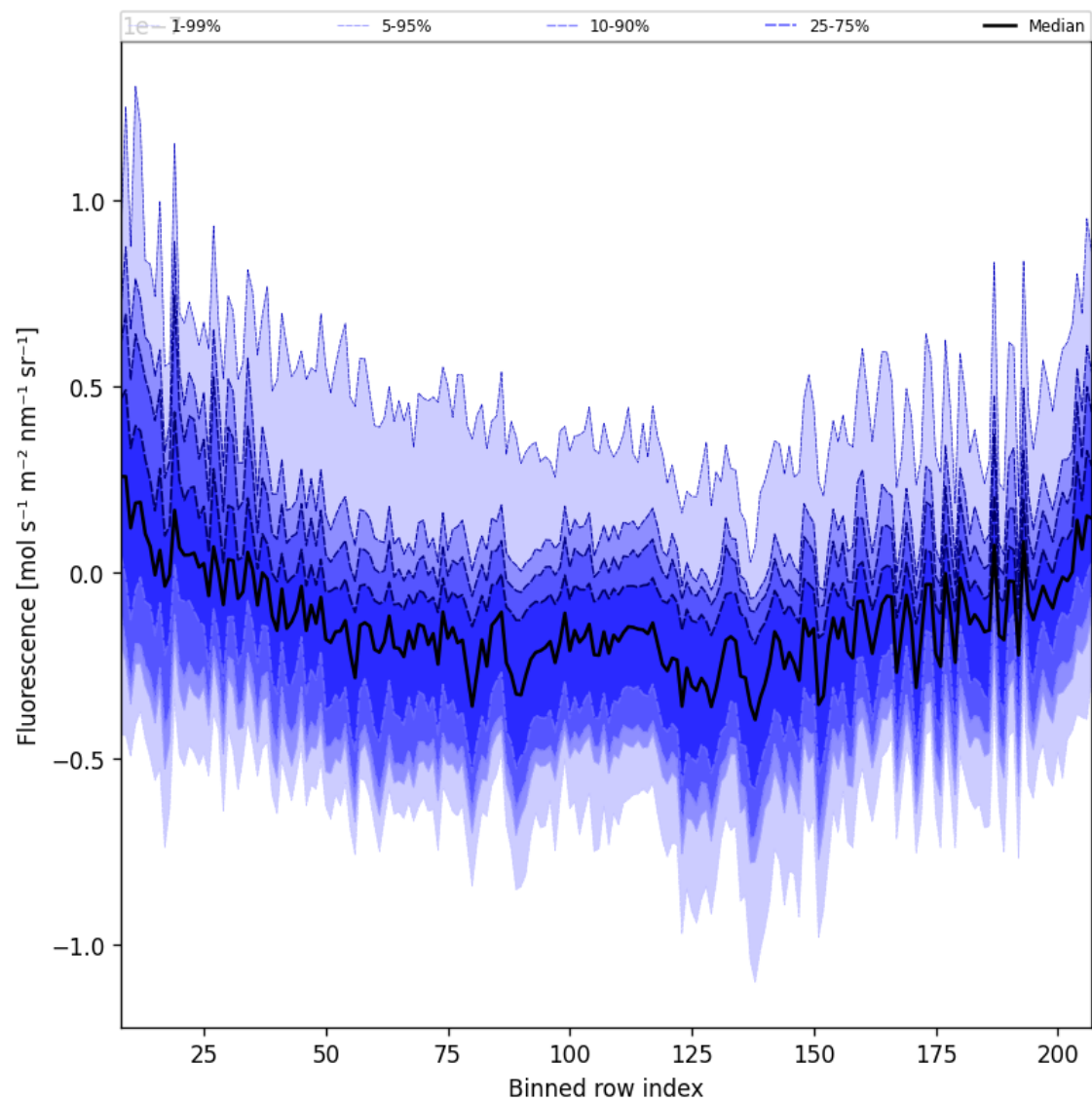
Figure 43: Along track statistics of “Fluorescence” for 2025-11-12 to 2025-11-14
