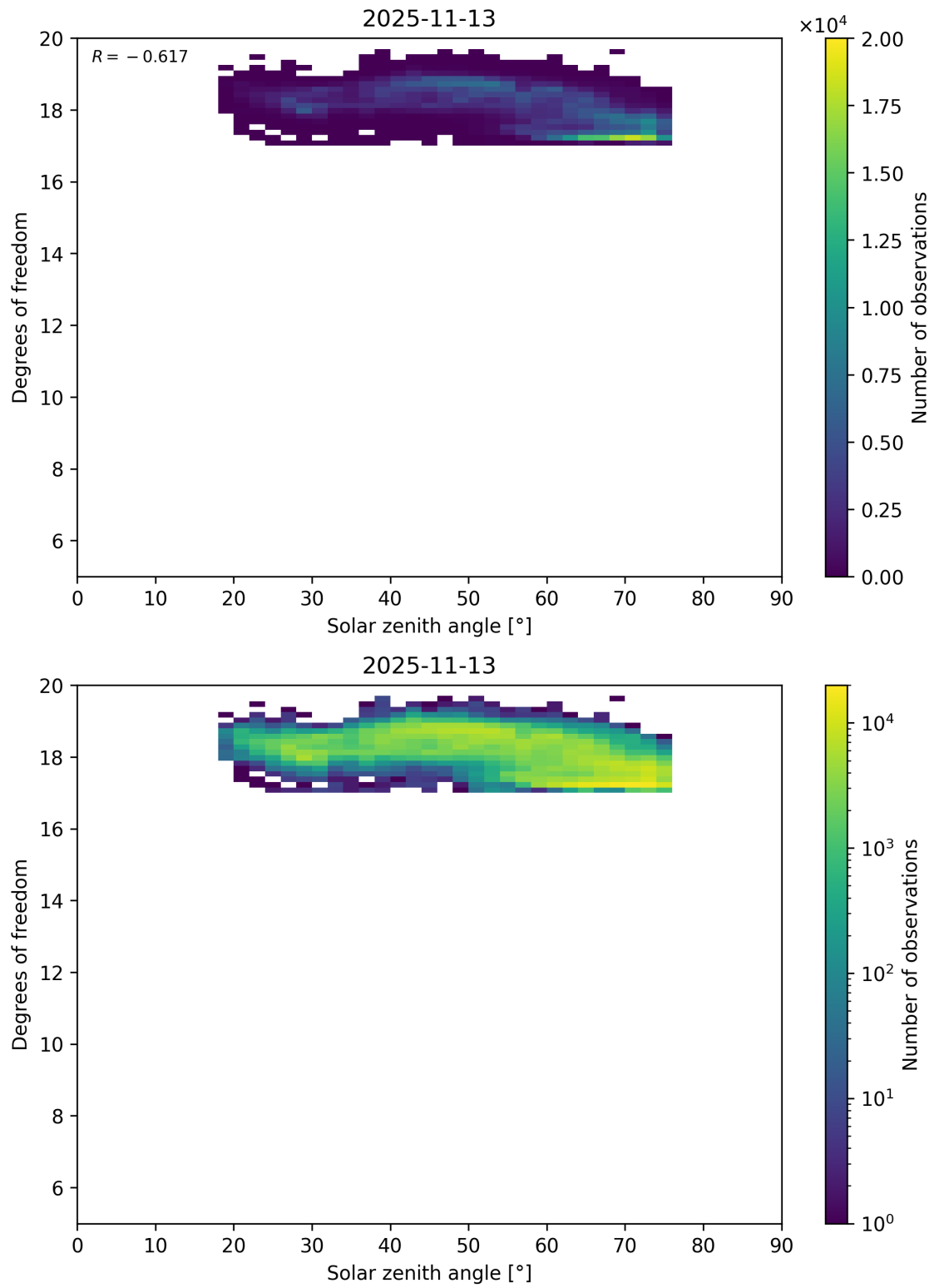
Figure 96: Scatter density plot of “Solar zenith angle” against “Degrees of freedom” for 2025-11-12 to 2025-11-14.
