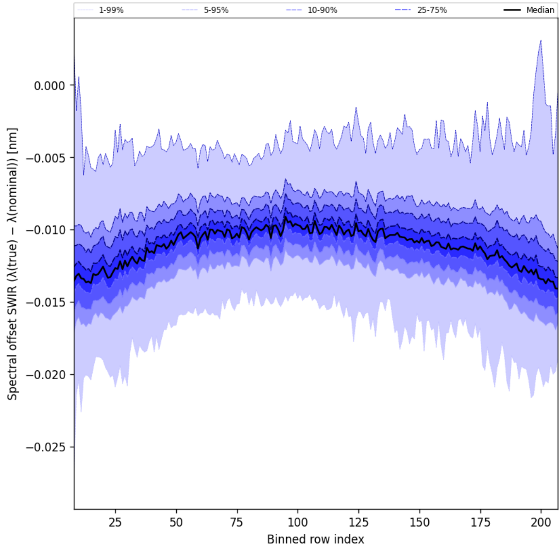
Figure 38: Along track statistics of “Spectral offset SWIR ( \lambda_{\text{true}} - \lambda_{\text{nominal}} )” for 2025-11-12 to 2025-11-14
