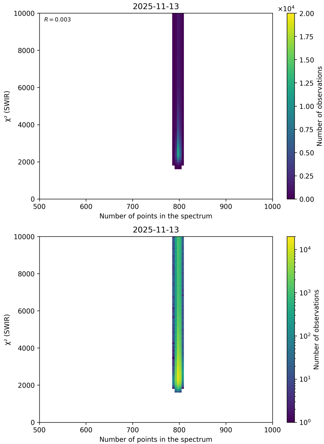
Figure 89: Scatter density plot of “Number of points in the spectrum” against “ \chi^2 (SWIR)” for 2025-11-12 to 2025-11-14.
