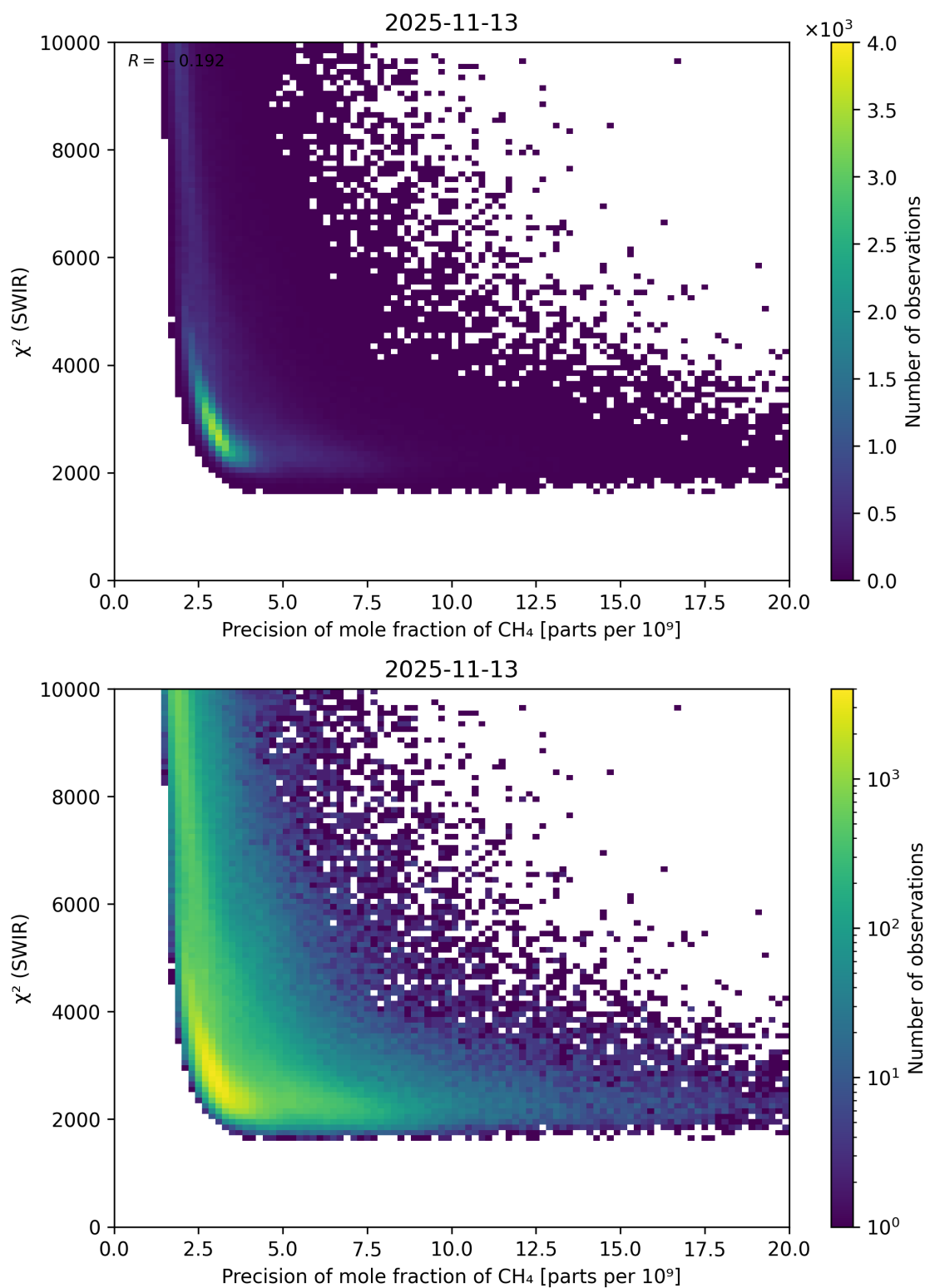
Figure 79: Scatter density plot of “Precision of mole fraction of \text{CH}_4 ” against “ \chi^2 (SWIR)” for 2025-11-12 to 2025-11-14.
