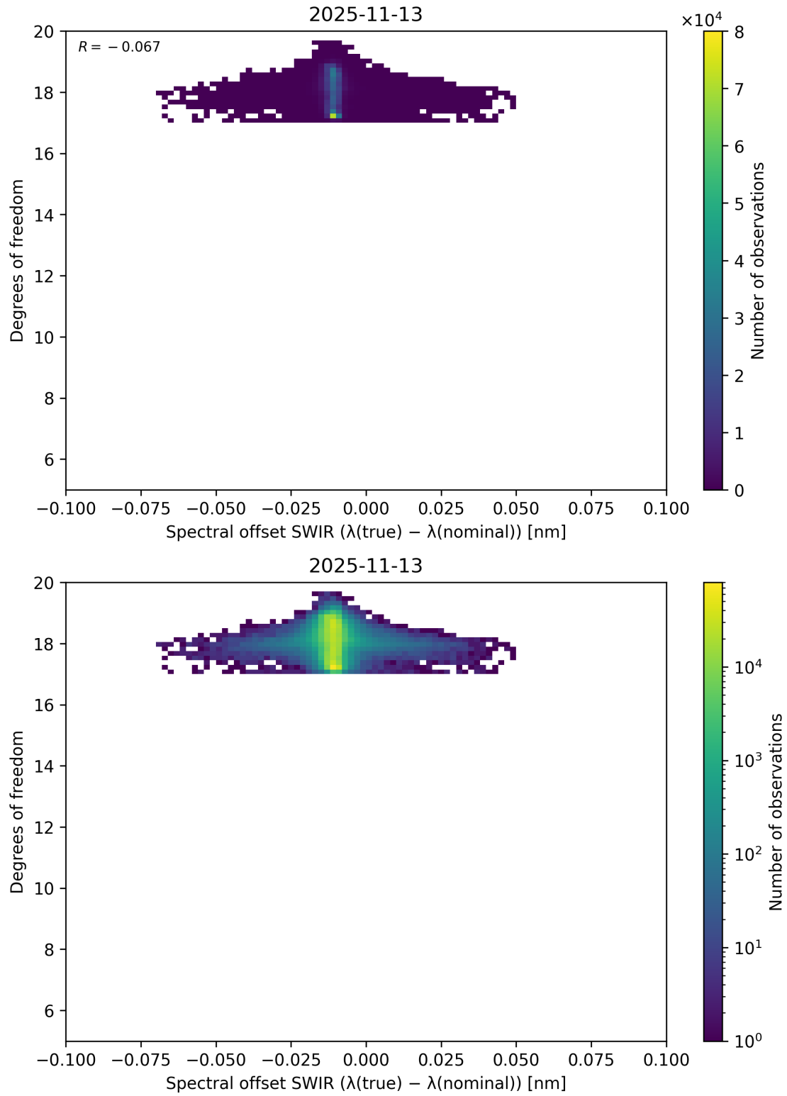
Figure 119: Scatter density plot of “Spectral offset SWIR ( \lambda_{\text{true}} - \lambda_{\text{nominal}} )” against “Degrees of freedom” for 2025-11-12 to 2025-11-14.
