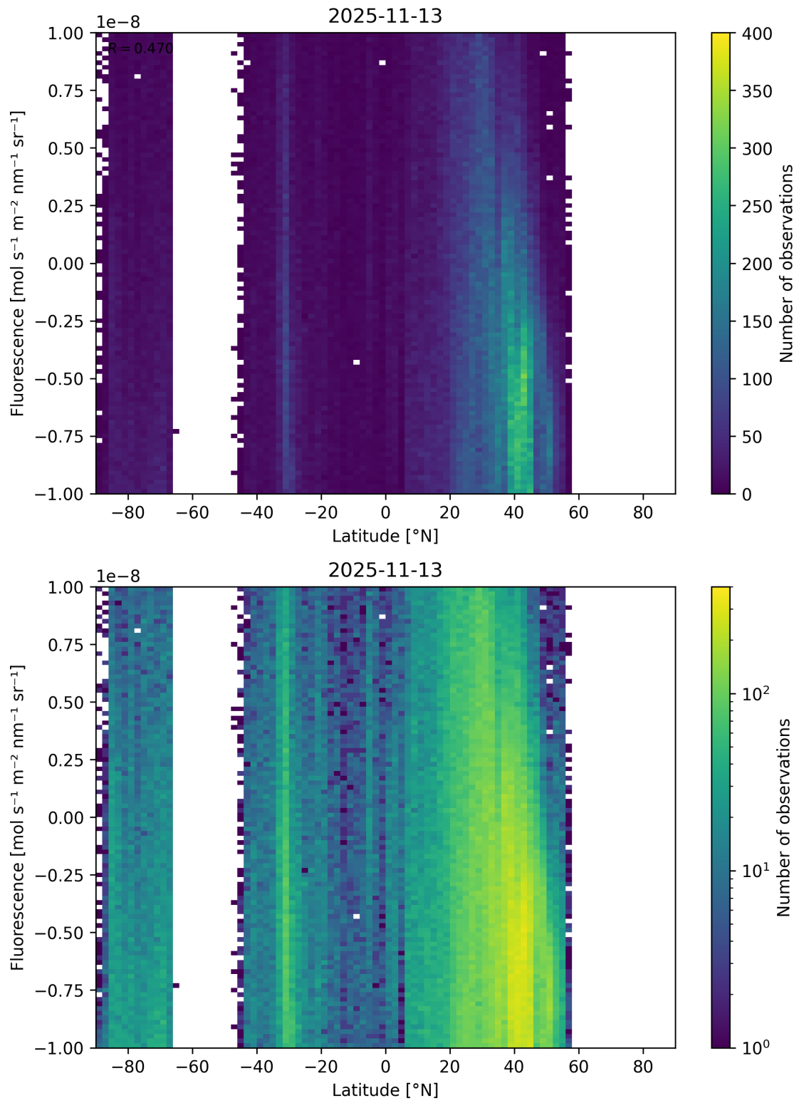
Figure 56: Scatter density plot of “Latitude” against “Fluorescence” for 2025-11-12 to 2025-11-14.
