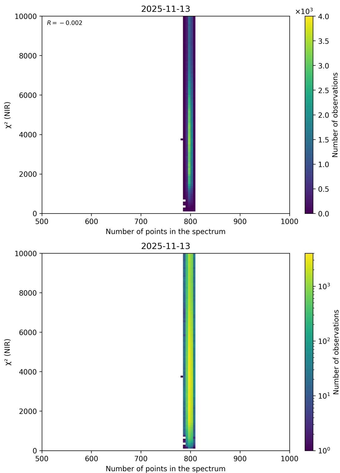
Figure 88: Scatter density plot of “Number of points in the spectrum” against “ \chi^2 (NIR)” for 2025-11-12 to 2025-11-14.
