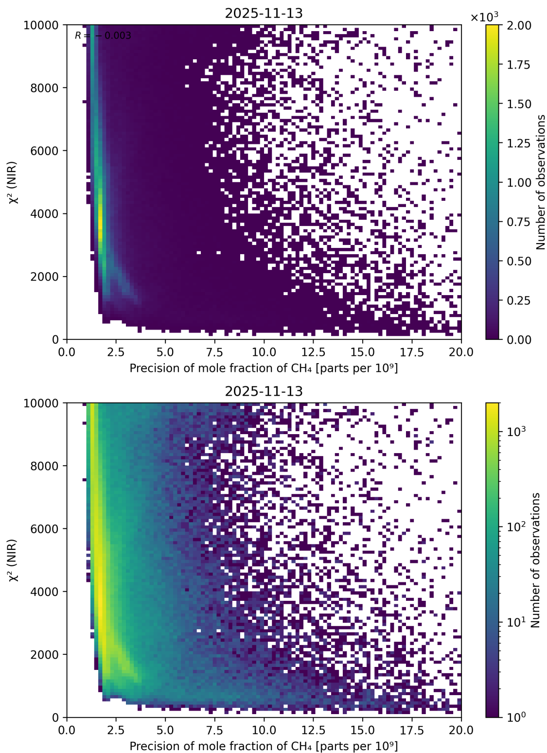
Figure 78: Scatter density plot of “Precision of mole fraction of \text{CH}_4 ” against “ \chi^2 (NIR)” for 2025-11-12 to 2025-11-14.
