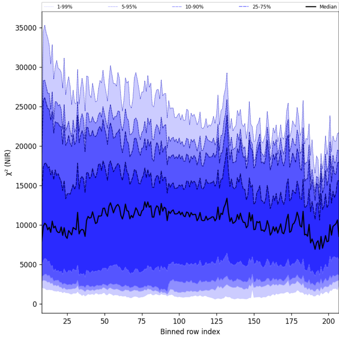
Figure 40: Along track statistics of “ \chi^2 (NIR)” for 2025-11-12 to 2025-11-14
