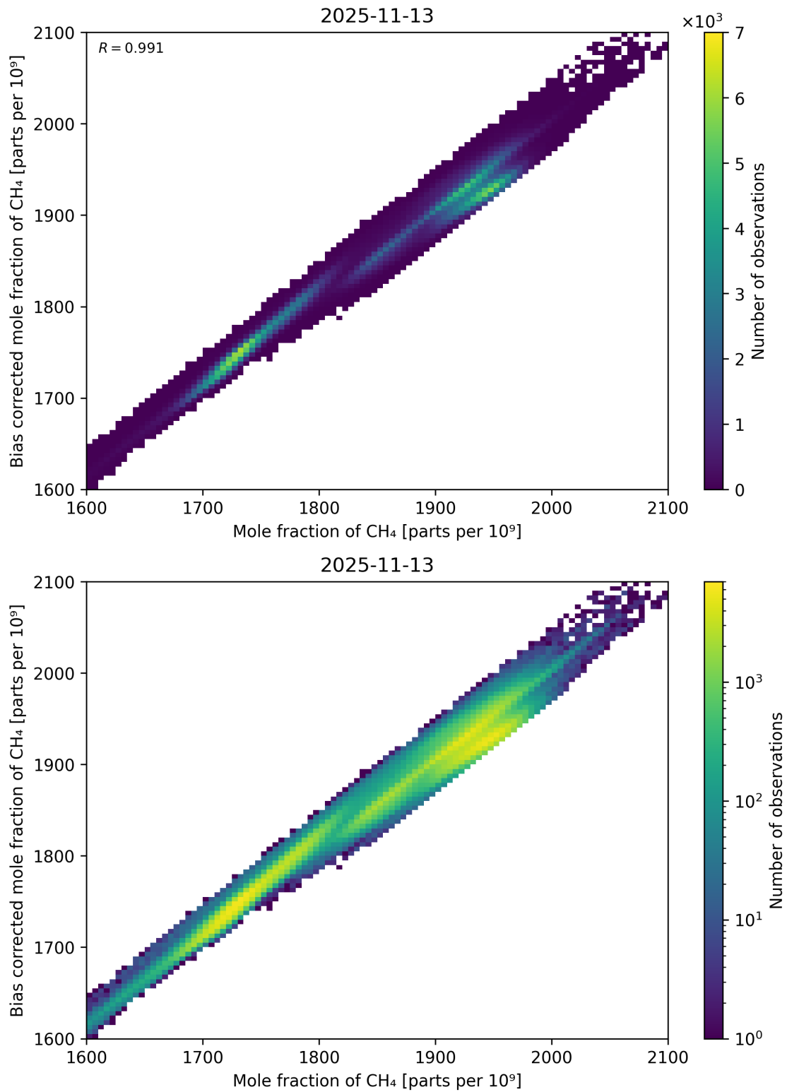
Figure 74: Scatter density plot of “Mole fraction of CH 4 ” against “Bias corrected mole fraction of CH 4 ” for 2025-11-12 to 2025-11-14.
