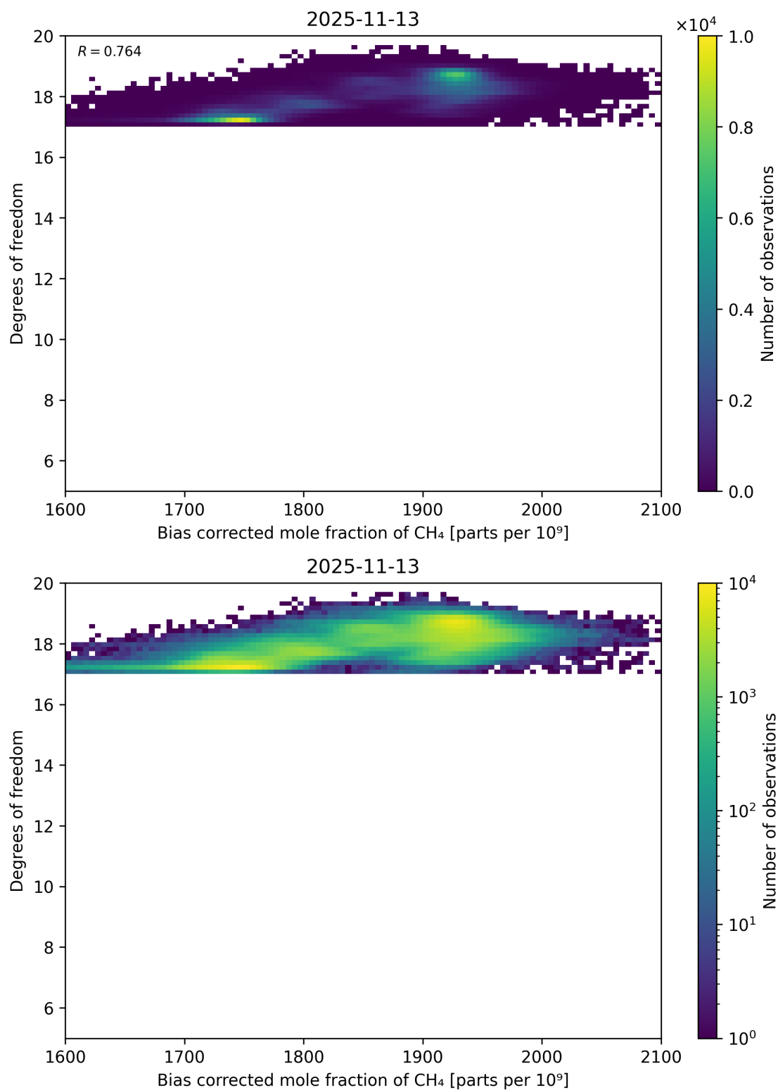
Figure 65: Scatter density plot of “Bias corrected mole fraction of \text{CH}_4 ” against “Degrees of freedom” for 2025-11-12 to 2025-11-14.
