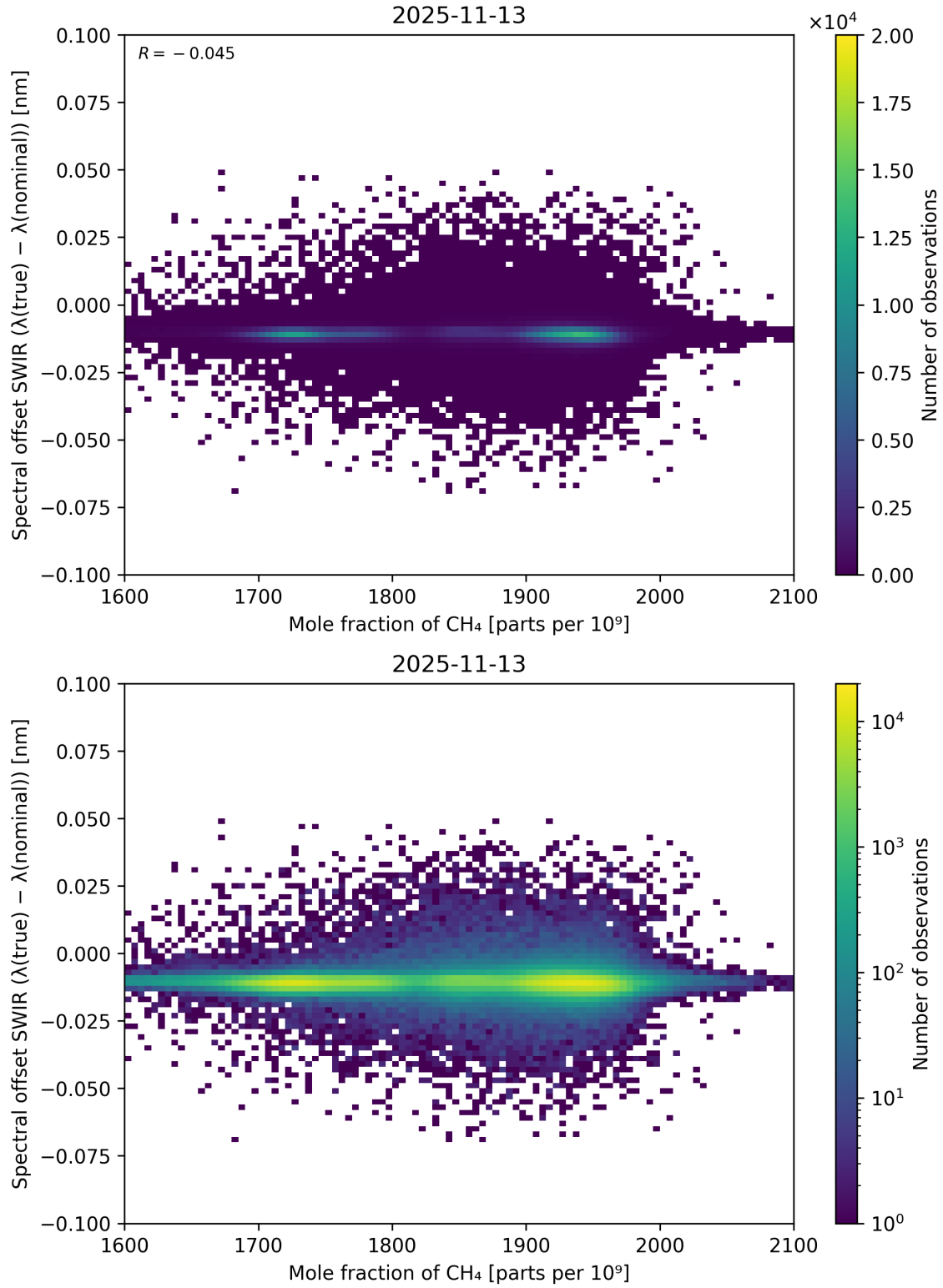
Figure 86: Scatter density plot of “Mole fraction of CH 4 ” against “Spectral offset SWIR ( \lambda_{\text{true}} - \lambda_{\text{nominal}} )” for 2025-11-12 to 2025-11-14.
