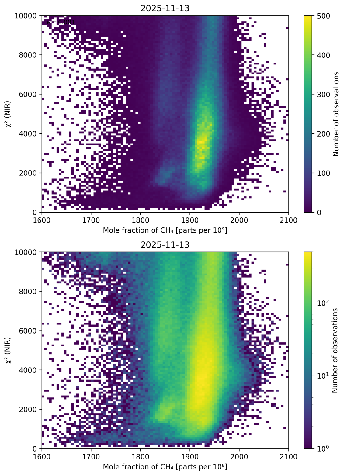
Figure 70: Scatter density plot of “Mole fraction of \text{CH}_4 ” against “ \chi^2 (NIR)” for 2025-11-12 to 2025-11-14.
