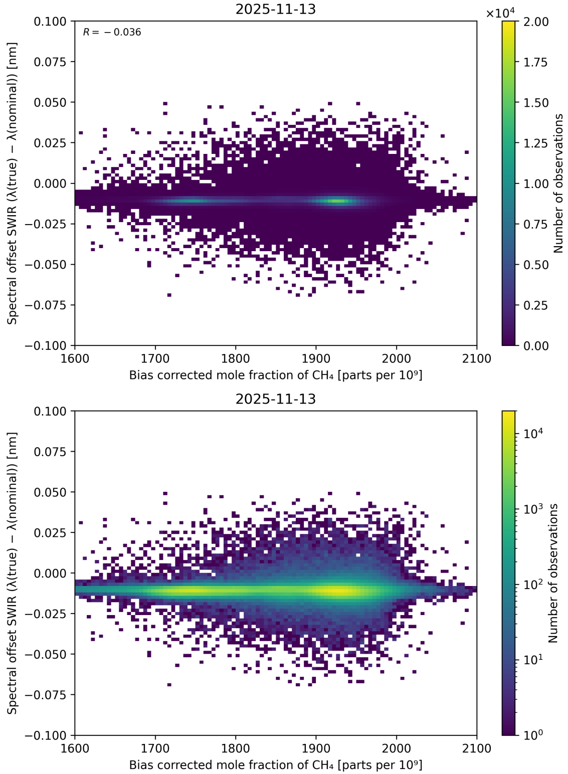
Figure 69: Scatter density plot of “Bias corrected mole fraction of \text{CH}_4 ” against “Spectral offset SWIR ( \lambda_{\text{true}} - \lambda_{\text{nominal}} )” for 2025-11-12 to 2025-11-14.
