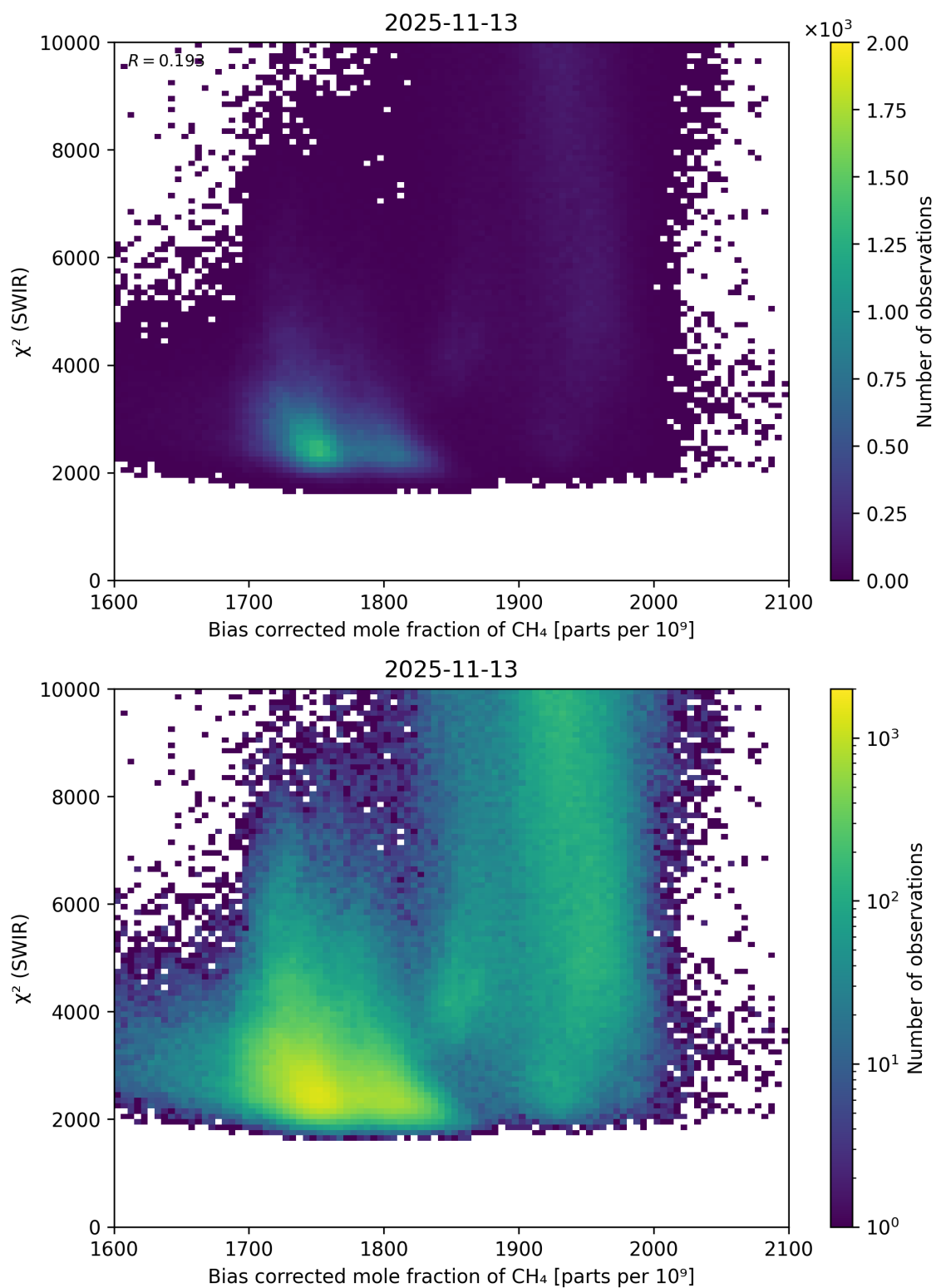
Figure 64: Scatter density plot of “Bias corrected mole fraction of \text{CH}_4 ” against “ \chi^2 (SWIR)” for 2025-11-12 to 2025-11-14.
