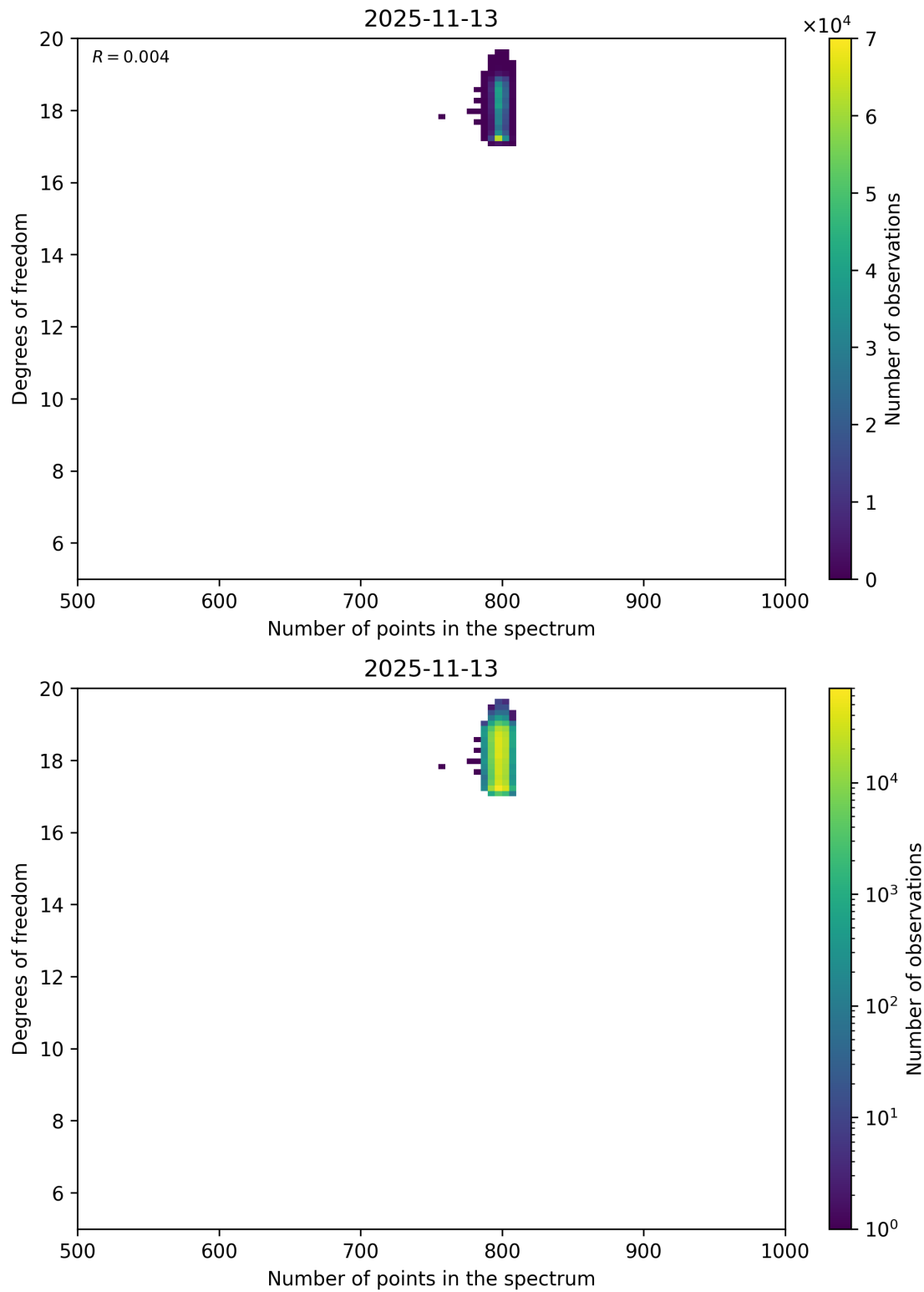
Figure 90: Scatter density plot of “Number of points in the spectrum” against “Degrees of freedom” for 2025-11-12 to 2025-11-14.
