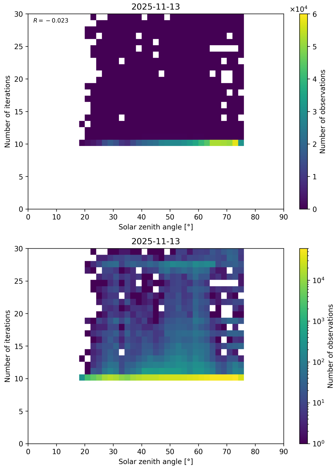
Figure 102: Scatter density plot of “Solar zenith angle” against “Number of iterations” for 2025-11-12 to 2025-11-14.
