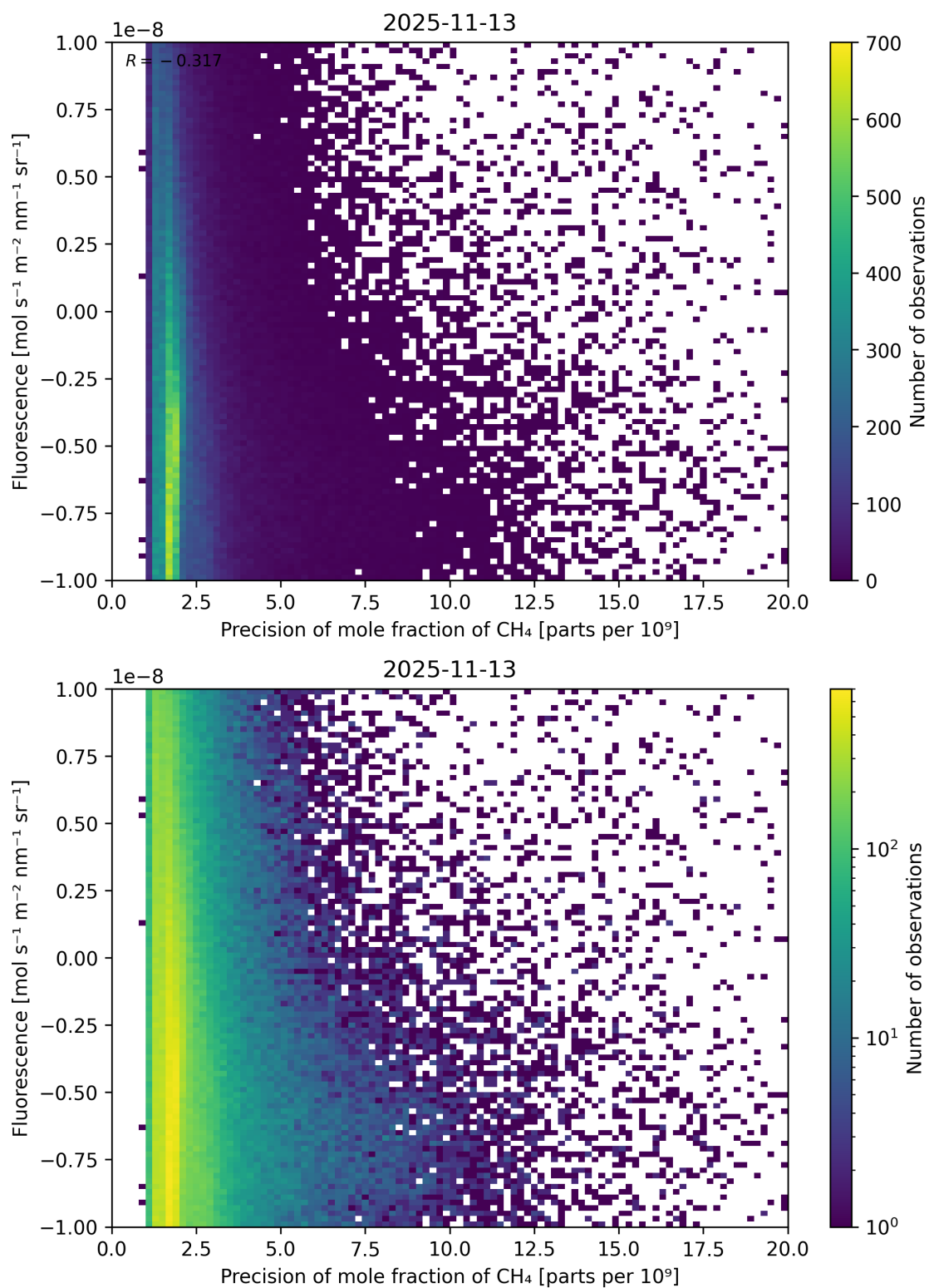
Figure 81: Scatter density plot of “Precision of mole fraction of \text{CH}_4 ” against “Fluorescence” for 2025-11-12 to 2025-11-14.
