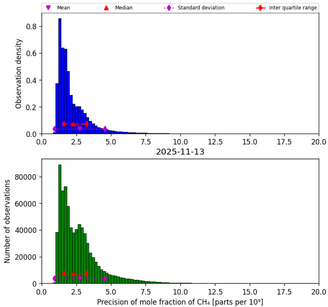
Figure 24: Histogram of “Precision of mole fraction of CH 4 ” for 2025-11-12 to 2025-11-14
