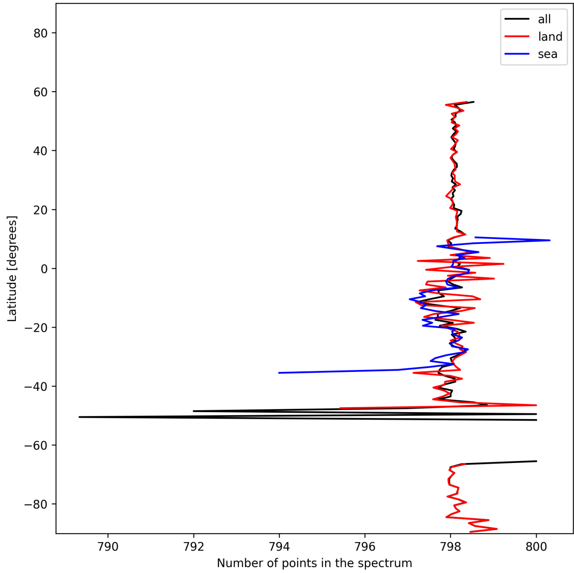
Figure 15: Zonal average of “Number of points in the spectrum” for 2025-11-12 to 2025-11-14.
