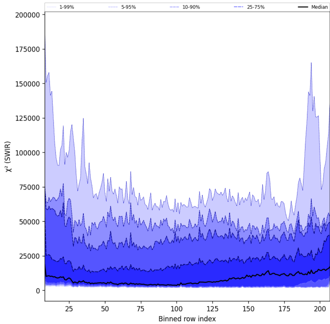
Figure 39: Along track statistics of “ \chi^2 (SWIR)” for 2025-11-12 to 2025-11-14
