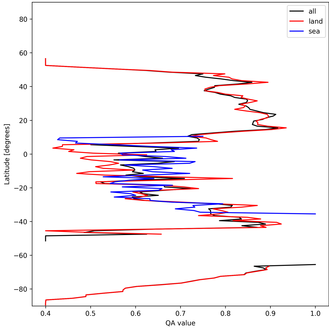
Figure 11: Zonal average of “QA value” for 2025-11-12 to 2025-11-14.
