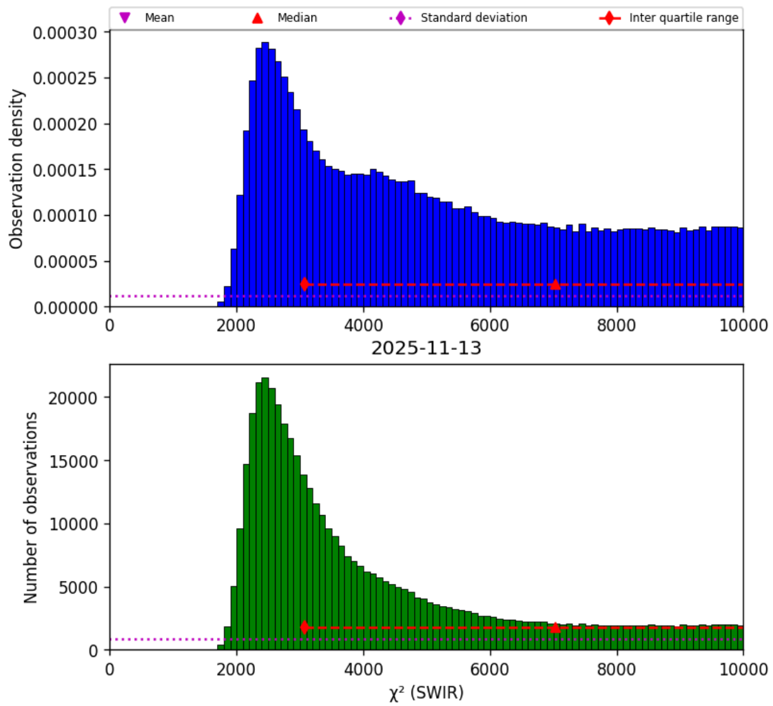
Figure 28: Histogram of “ \chi^2 (SWIR)” for 2025-11-12 to 2025-11-14
