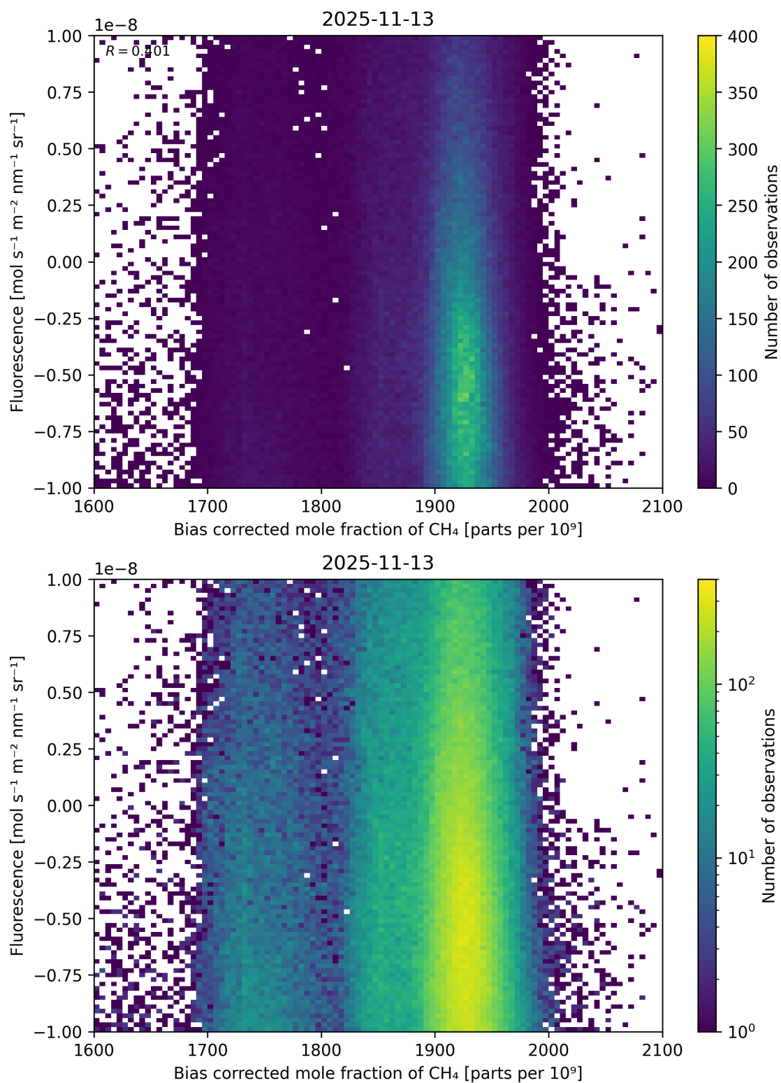
Figure 66: Scatter density plot of “Bias corrected mole fraction of CH 4 ” against “Fluorescence” for 2025-11-12 to 2025-11-14.
