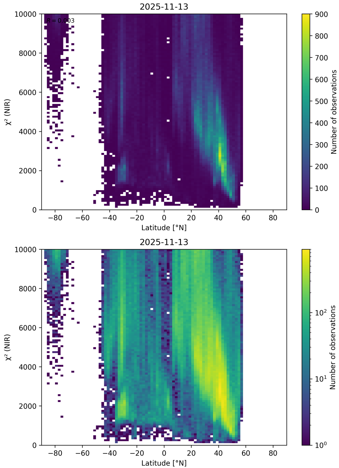
Figure 53: Scatter density plot of “Latitude” against “ \chi^2 (NIR)” for 2025-11-12 to 2025-11-14.
