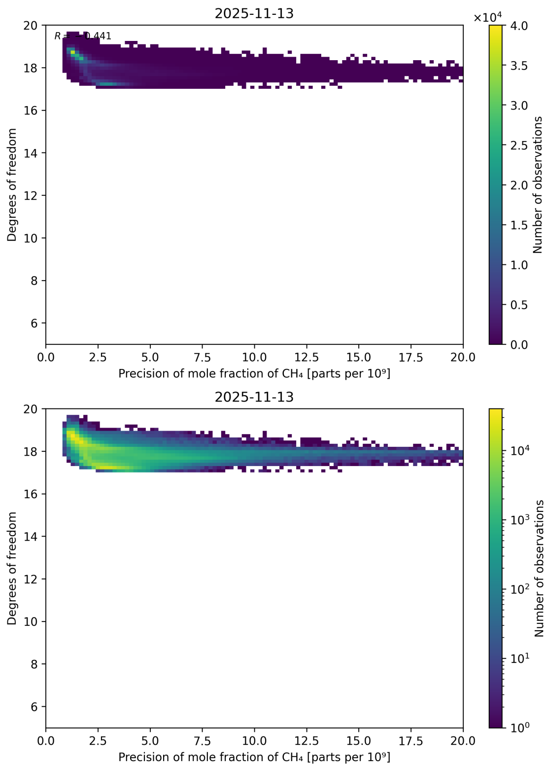
Figure 80: Scatter density plot of “Precision of mole fraction of CH 4 ” against “Degrees of freedom” for 2025-11-12 to 2025-11-14.
