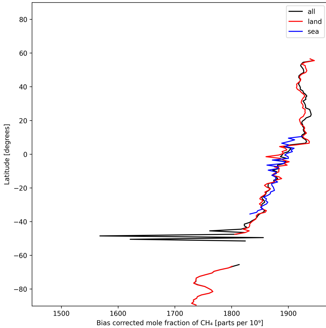
Figure 14: Zonal average of “Bias corrected mole fraction of CH 4 ” for 2025-11-12 to 2025-11-14.
