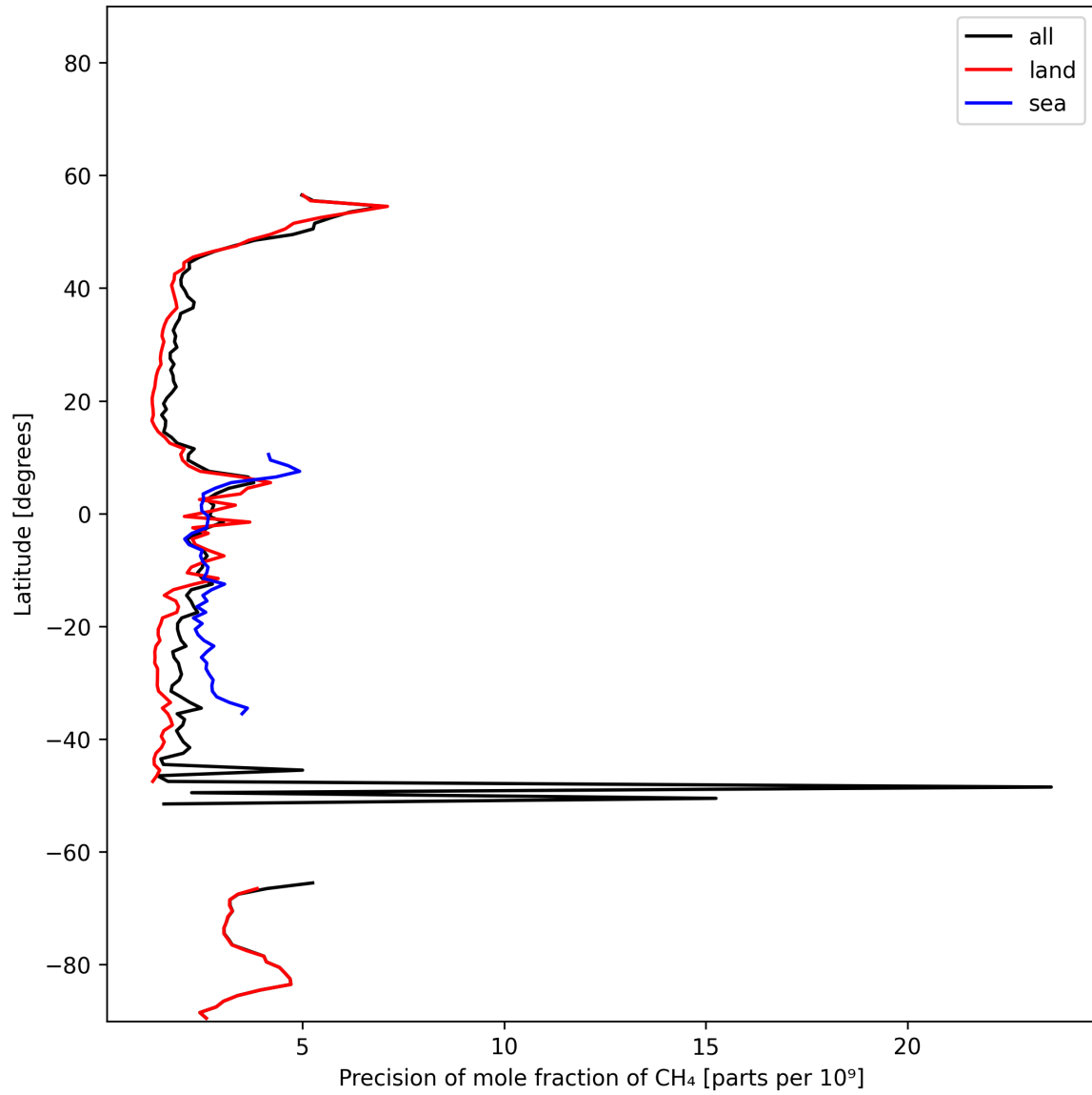
Figure 13: Zonal average of “Precision of mole fraction of CH 4 ” for 2025-11-12 to 2025-11-14.
