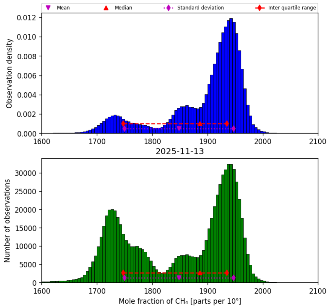
Figure 23: Histogram of “Mole fraction of CH 4 ” for 2025-11-12 to 2025-11-14
