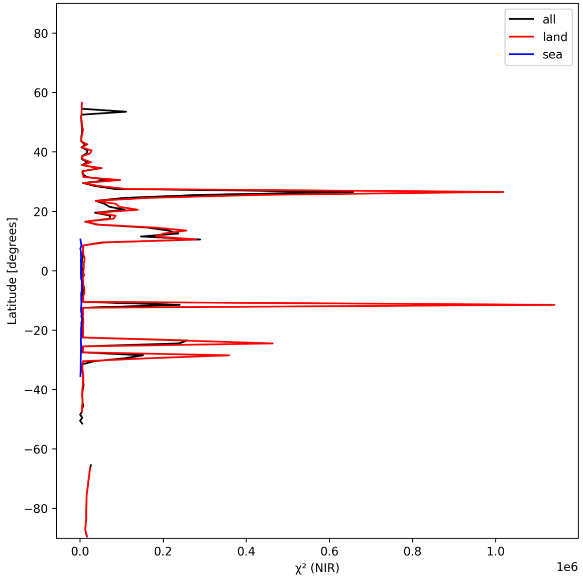
Figure 18: Zonal average of “ \chi^2 (NIR)” for 2025-11-12 to 2025-11-14.
