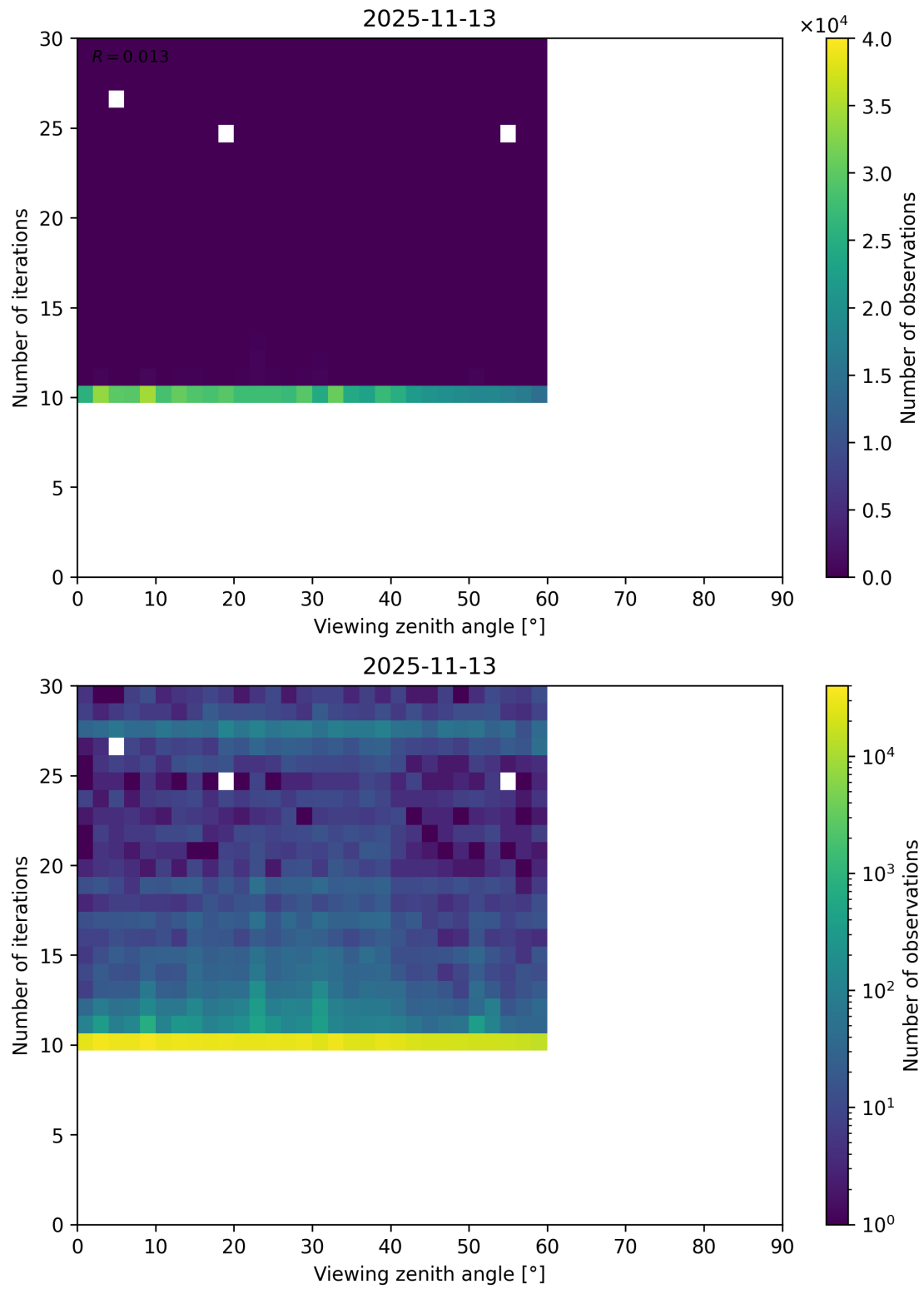
Figure 113: Scatter density plot of “Viewing zenith angle” against “Number of iterations” for 2025-11-12 to 2025-11-14.
