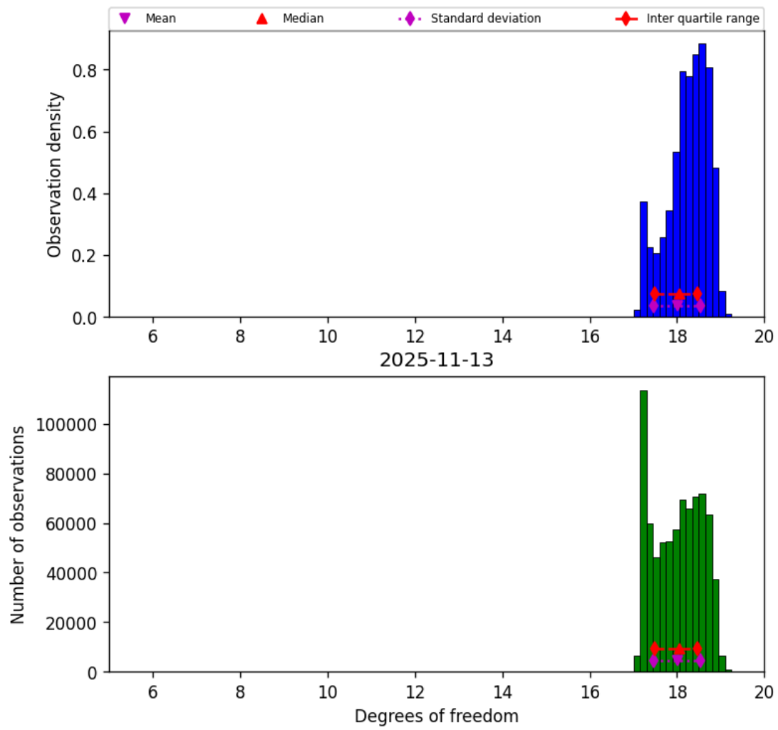
Figure 30: Histogram of “Degrees of freedom” for 2025-11-12 to 2025-11-14
