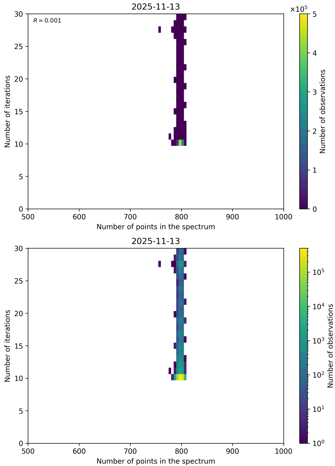
Figure 92: Scatter density plot of “Number of points in the spectrum” against “Number of iterations” for 2025-11-12 to 2025-11-14.
