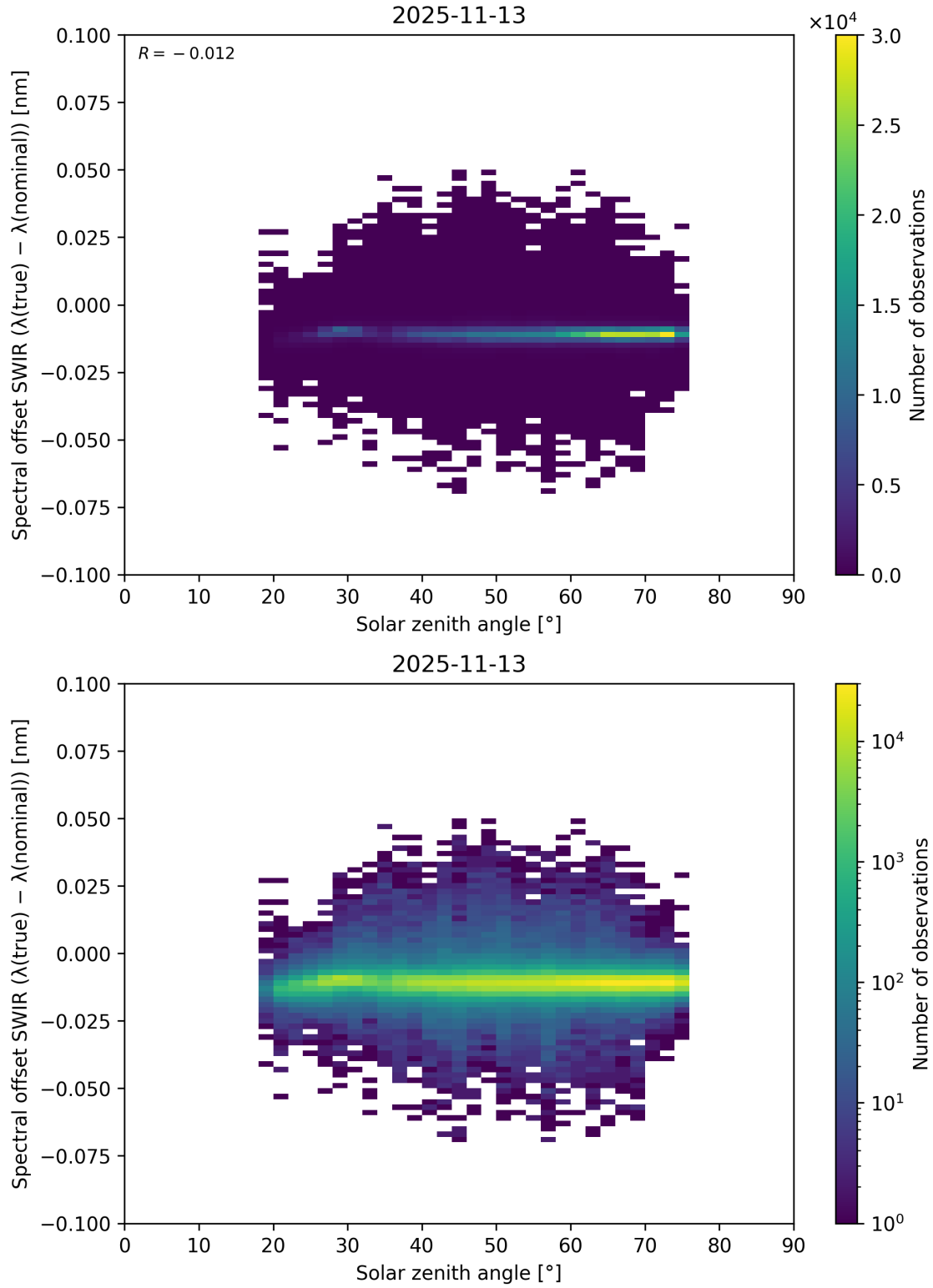
Figure 104: Scatter density plot of “Solar zenith angle” against “Spectral offset SWIR ( \lambda_{\text{true}} - \lambda_{\text{nominal}} )” for 2025-11-12 to 2025-11-14.
