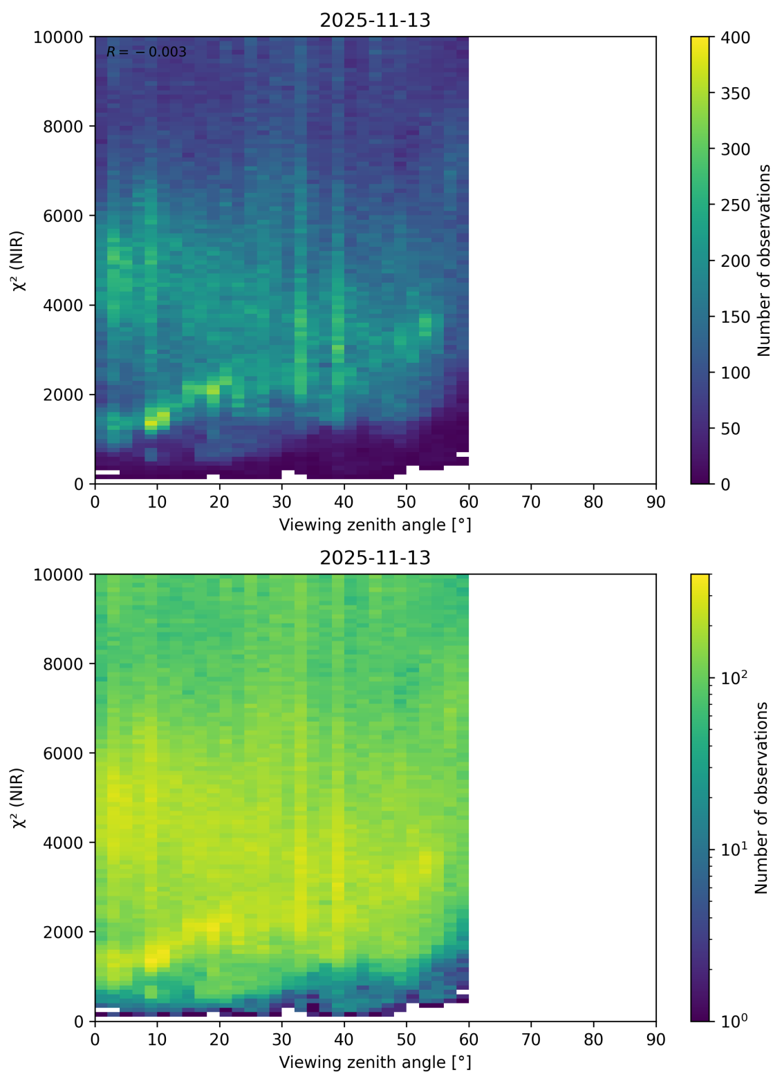
Figure 105: Scatter density plot of “Viewing zenith angle” against “ \chi^2 (NIR)” for 2025-11-12 to 2025-11-14.
