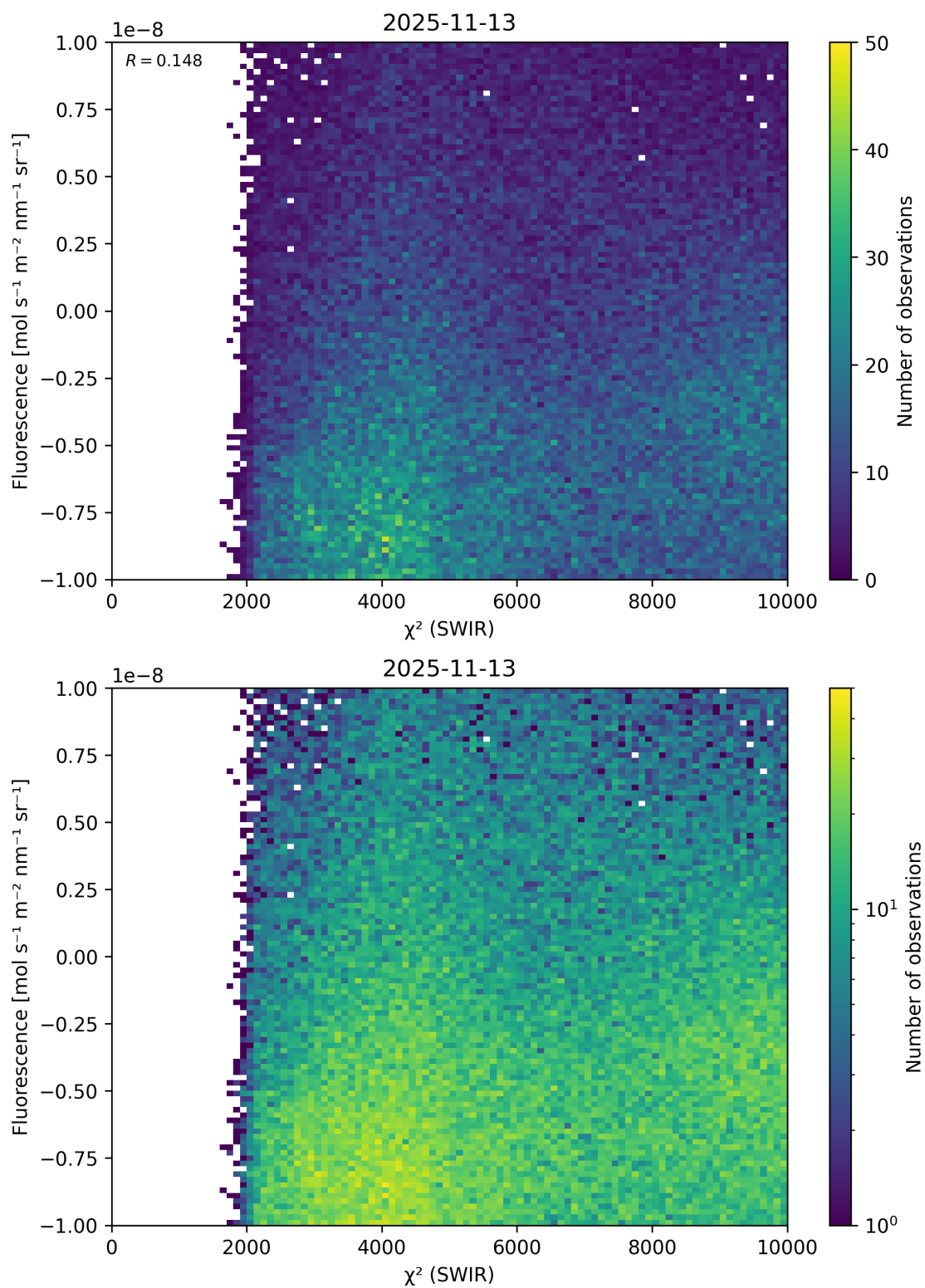
Figure 49: Scatter density plot of “ \chi^2 (SWIR)” against “Fluorescence” for 2025-11-12 to 2025-11-14.
