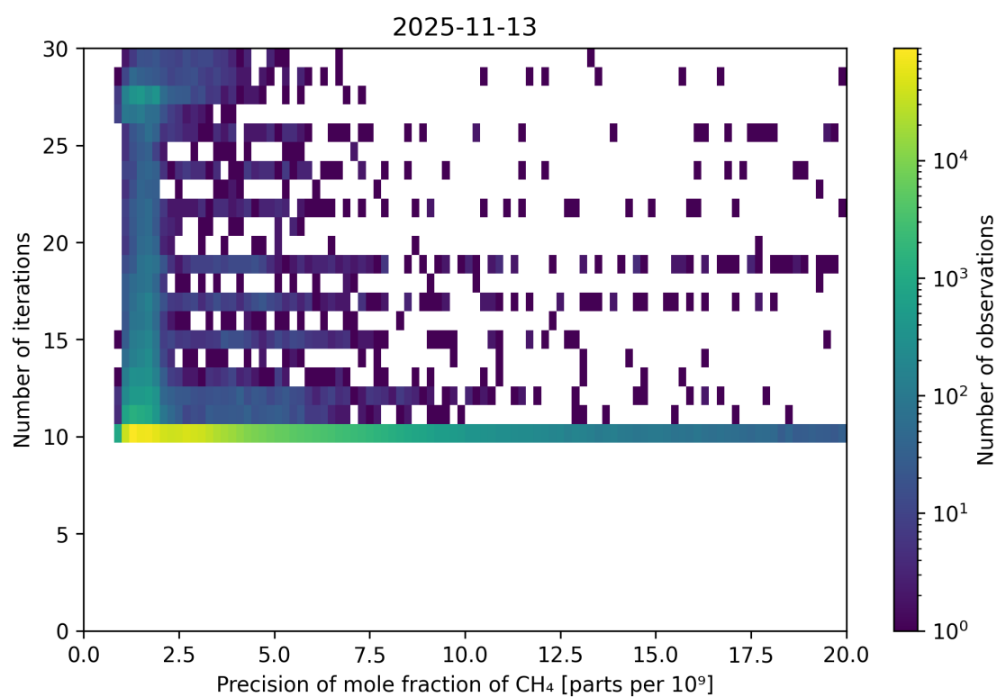
Figure 83: Scatter density plot of “Precision of mole fraction of \text{CH}_4 ” against “Number of iterations” for 2025-11-12 to 2025-11-14.
