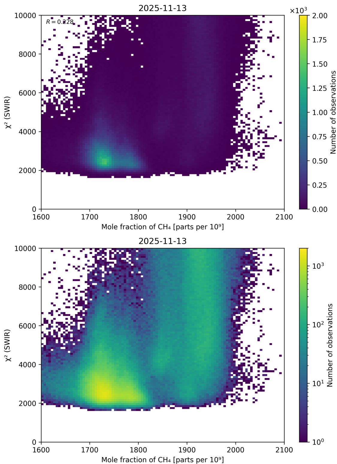
Figure 71: Scatter density plot of “Mole fraction of \text{CH}_4 ” against “ \chi^2 (SWIR)” for 2025-11-12 to 2025-11-14.
