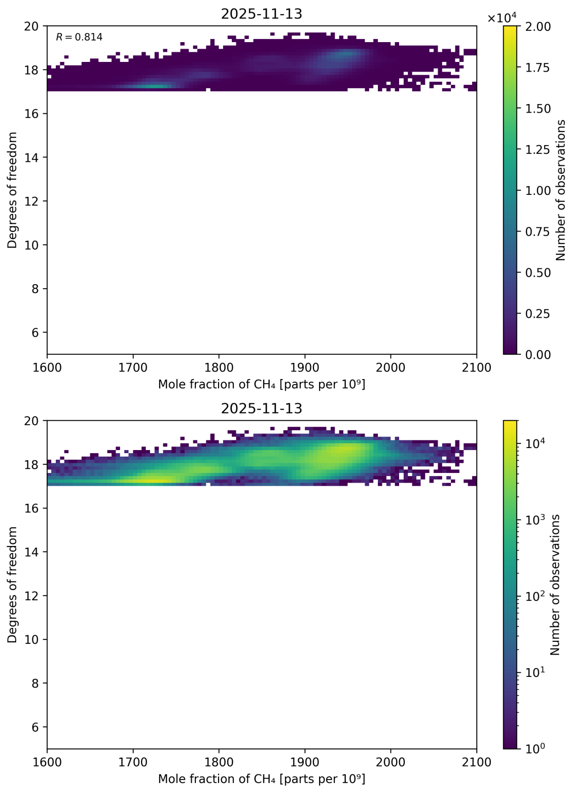
Figure 72: Scatter density plot of “Mole fraction of CH 4 ” against “Degrees of freedom” for 2025-11-12 to 2025-11-14.
