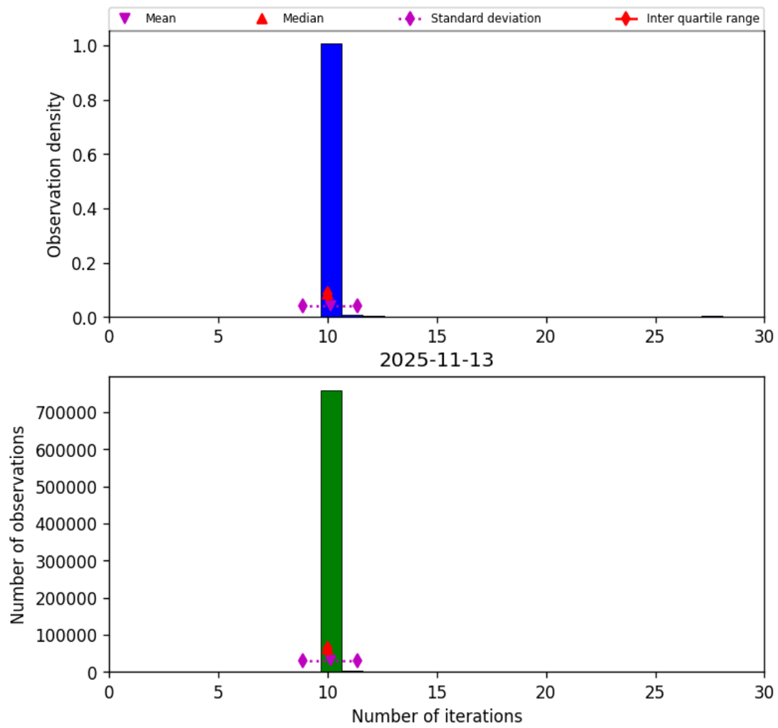
Figure 31: Histogram of “Number of iterations” for 2025-11-12 to 2025-11-14
