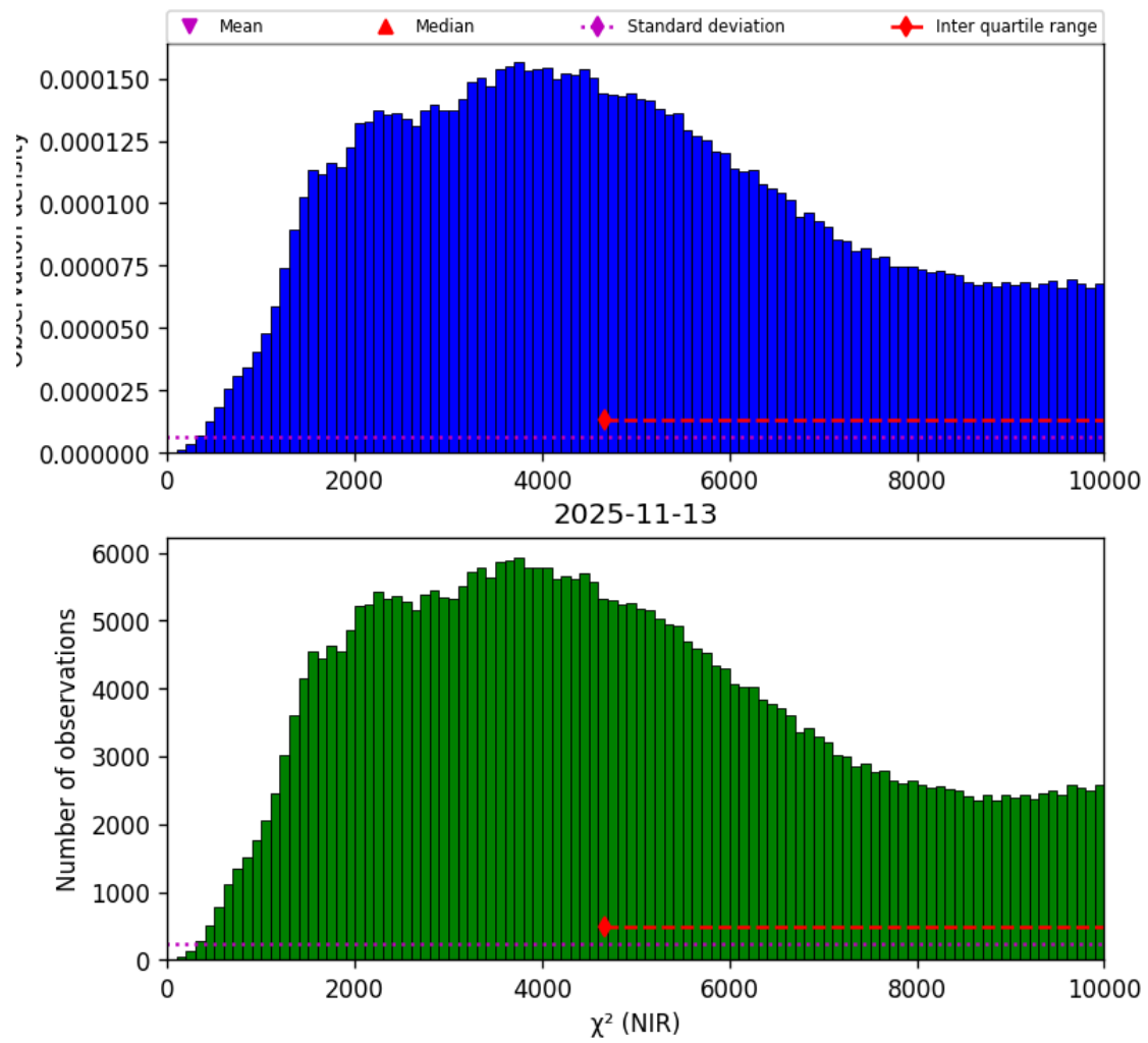
Figure 29: Histogram of “ \chi^2 (NIR)” for 2025-11-12 to 2025-11-14
