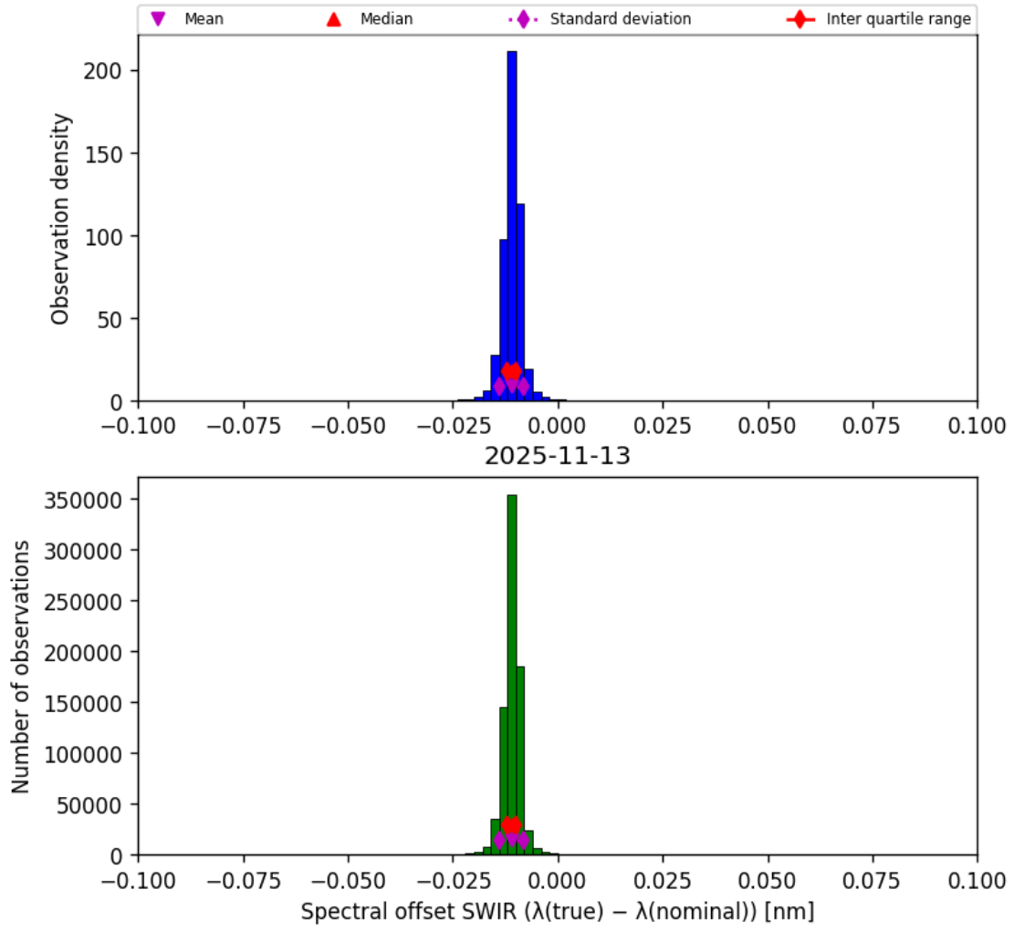
Figure 27: Histogram of “Spectral offset SWIR ( \lambda_{\text{true}} - \lambda_{\text{nominal}} )” for 2025-11-12 to 2025-11-14
