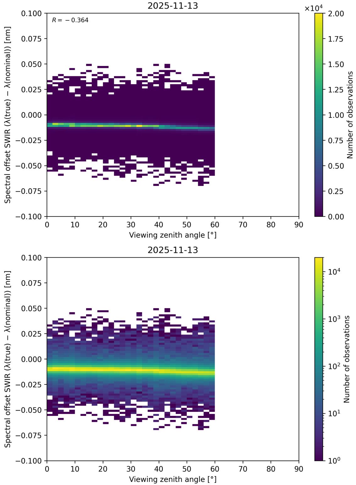
Figure 116: Scatter density plot of “Viewing zenith angle” against “Spectral offset SWIR ( \lambda_{\text{true}} - \lambda_{\text{nominal}} )” for 2025-11-12 to 2025-11-14.
