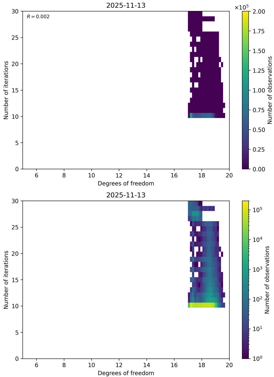
Figure 52: Scatter density plot of “Degrees of freedom” against “Number of iterations” for 2025-11-12 to 2025-11-14.
