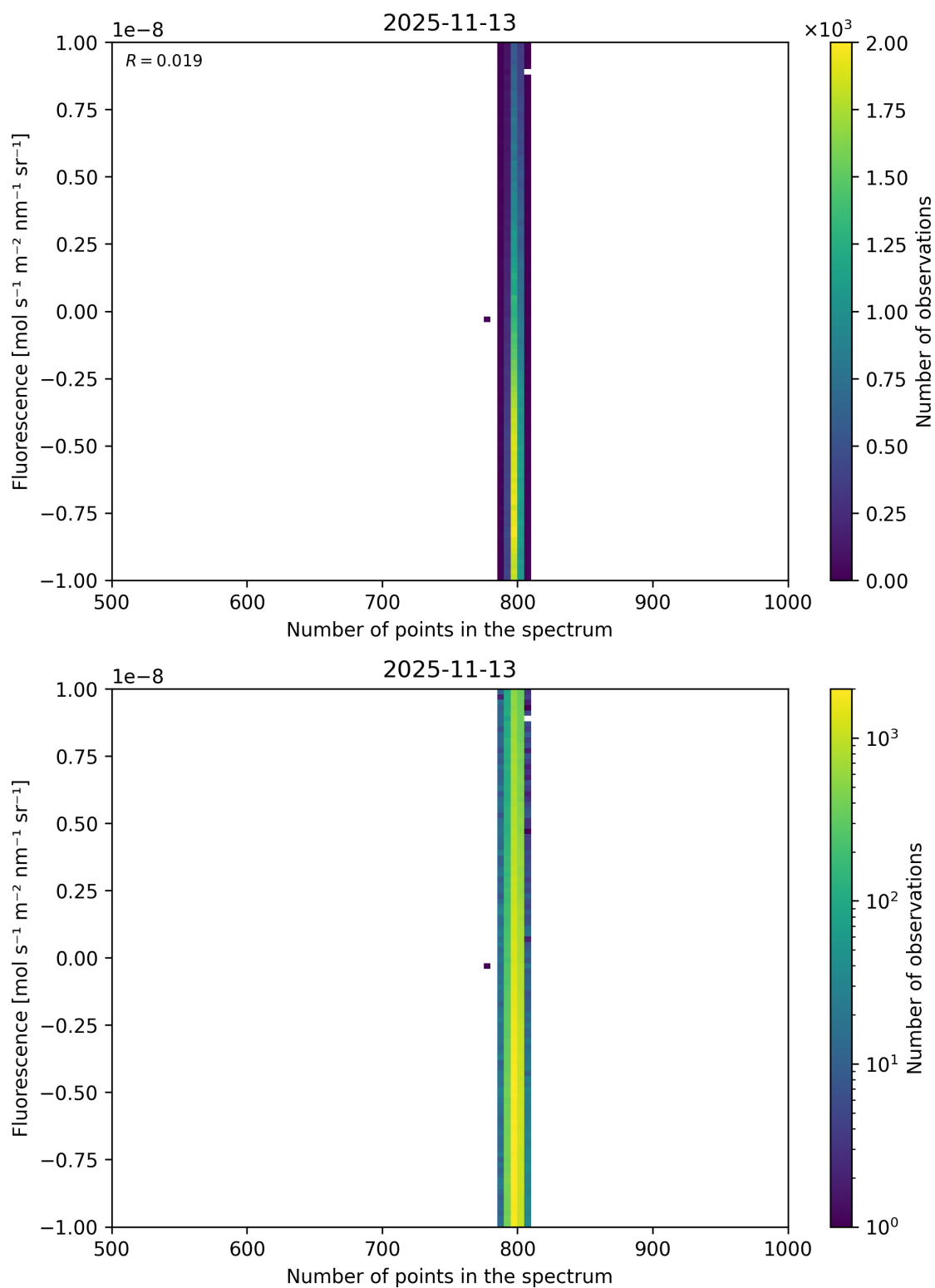
Figure 91: Scatter density plot of “Number of points in the spectrum” against “Fluorescence” for 2025-11-12 to 2025-11-14.
