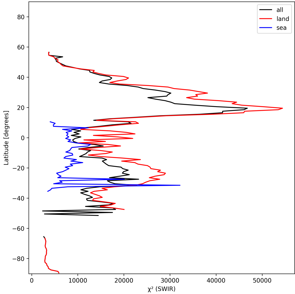
Figure 17: Zonal average of “ \chi^2 (SWIR)” for 2025-11-12 to 2025-11-14.
