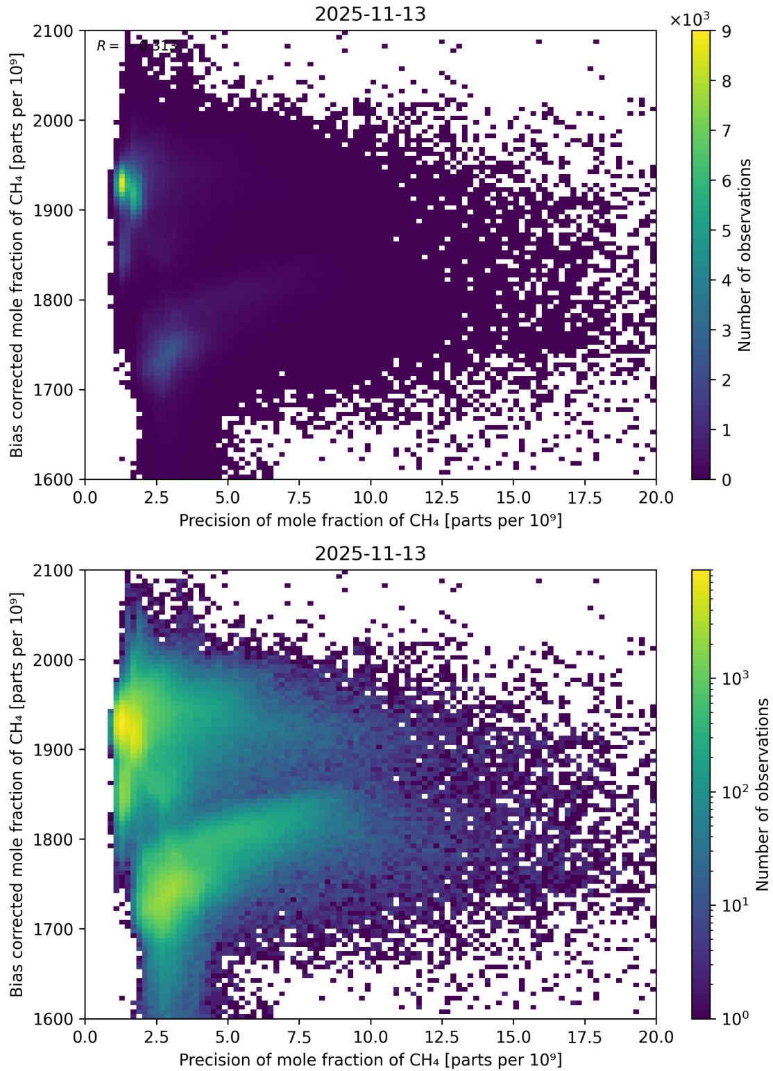
Figure 82: Scatter density plot of “Precision of mole fraction of CH 4 ” against “Bias corrected mole fraction of CH 4 ” for 2025-11-12 to 2025-11-14.
