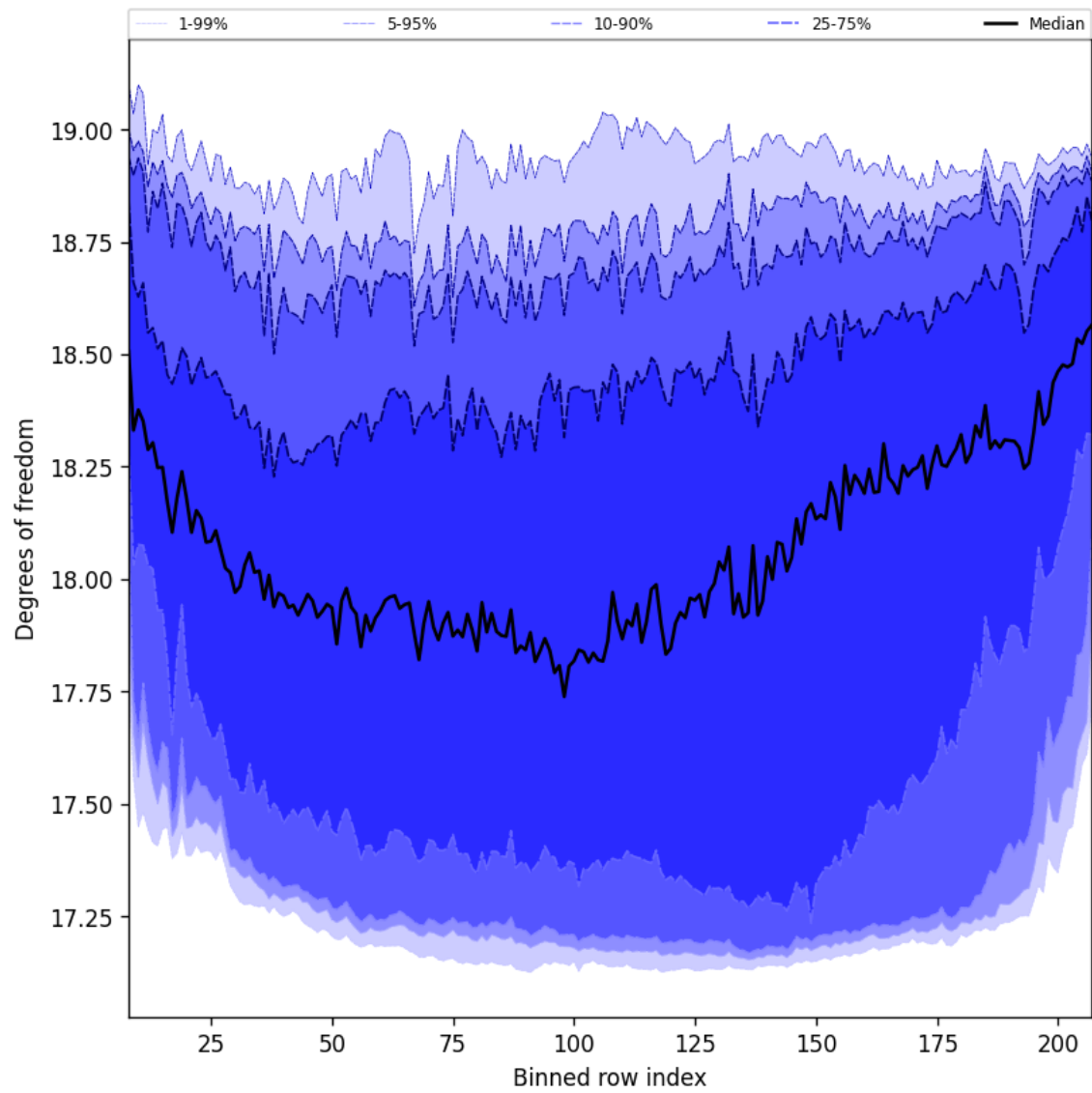
Figure 41: Along track statistics of “Degrees of freedom” for 2025-11-12 to 2025-11-14
