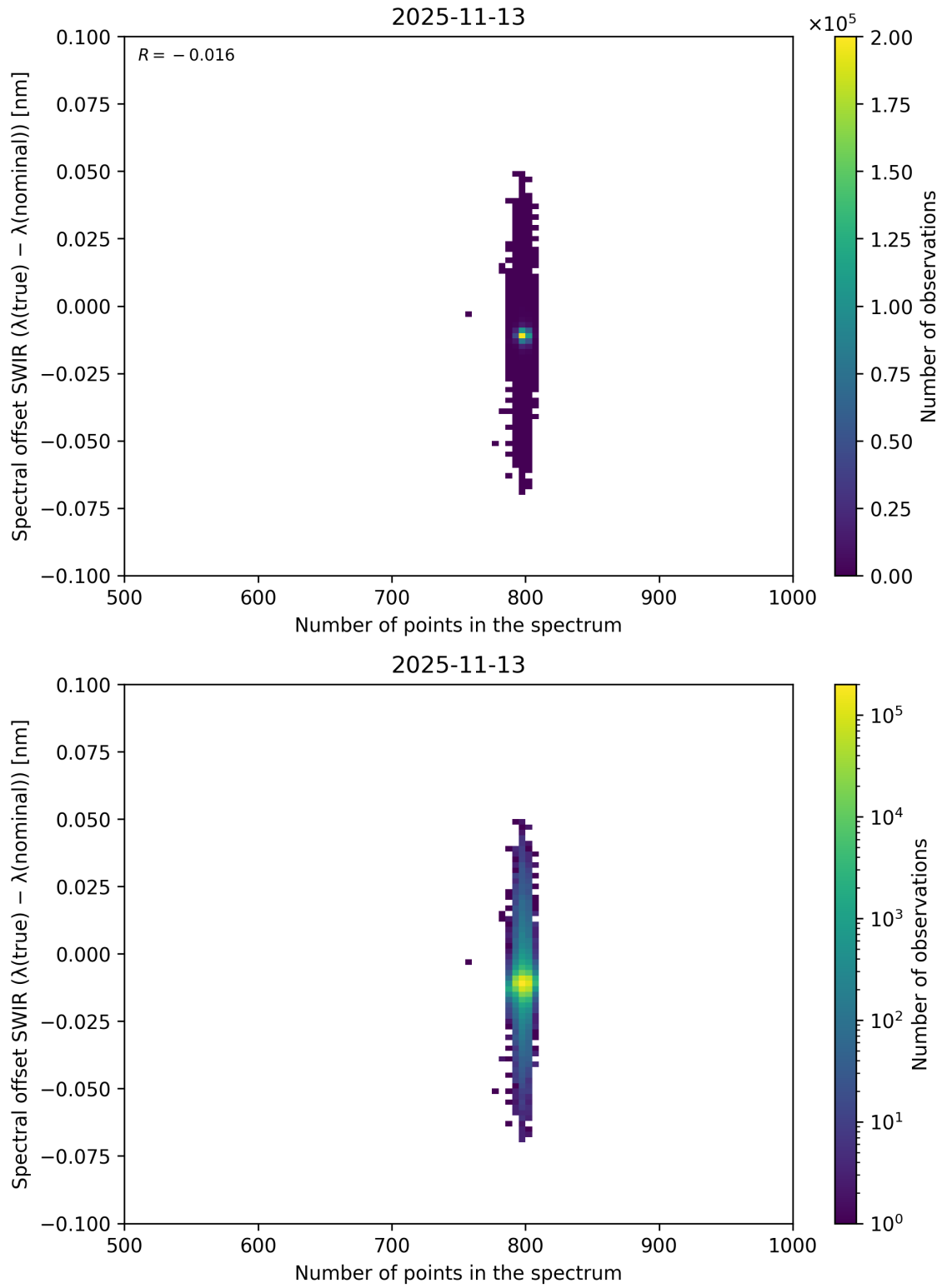
Figure 93: Scatter density plot of “Number of points in the spectrum” against “Spectral offset SWIR ( \lambda_{\text{true}} - \lambda_{\text{nominal}} )” for 2025-11-12 to 2025-11-14.
