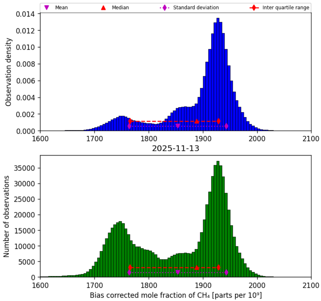
Figure 25: Histogram of “Bias corrected mole fraction of CH 4 ” for 2025-11-12 to 2025-11-14
