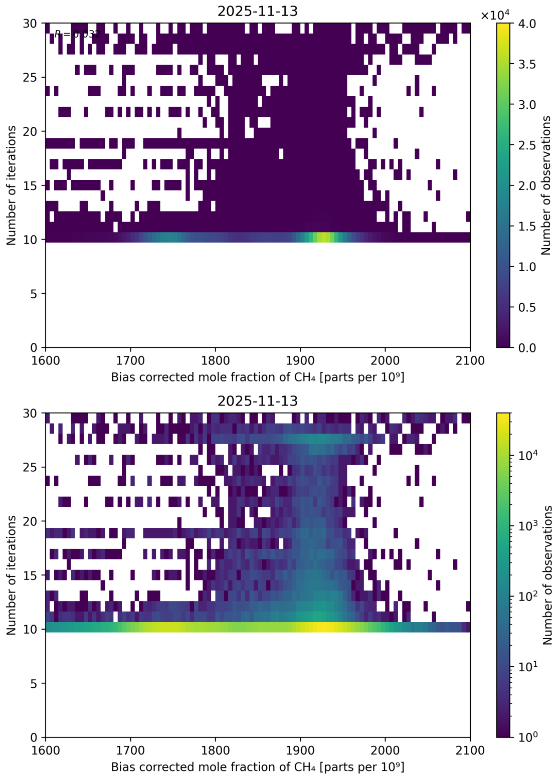
Figure 67: Scatter density plot of “Bias corrected mole fraction of \text{CH}_4 ” against “Number of iterations” for 2025-11-12 to 2025-11-14.
