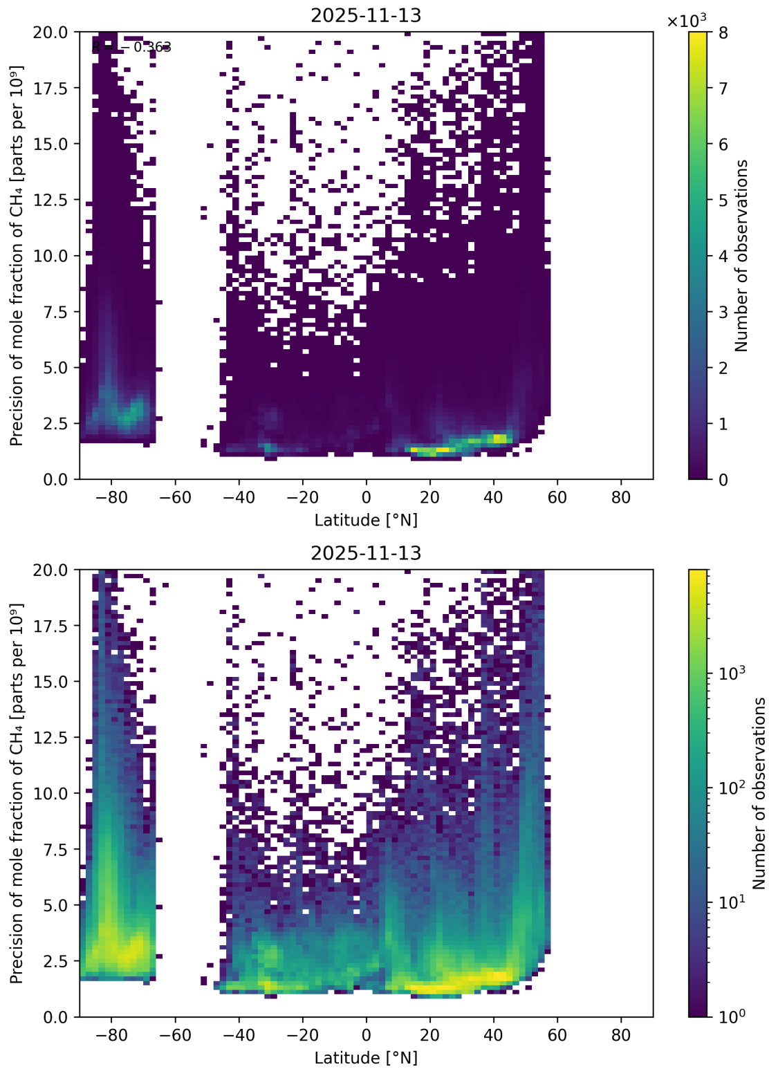
Figure 59: Scatter density plot of “Latitude” against “Precision of mole fraction of CH 4 ” for 2025-11-12 to 2025-11-14.
