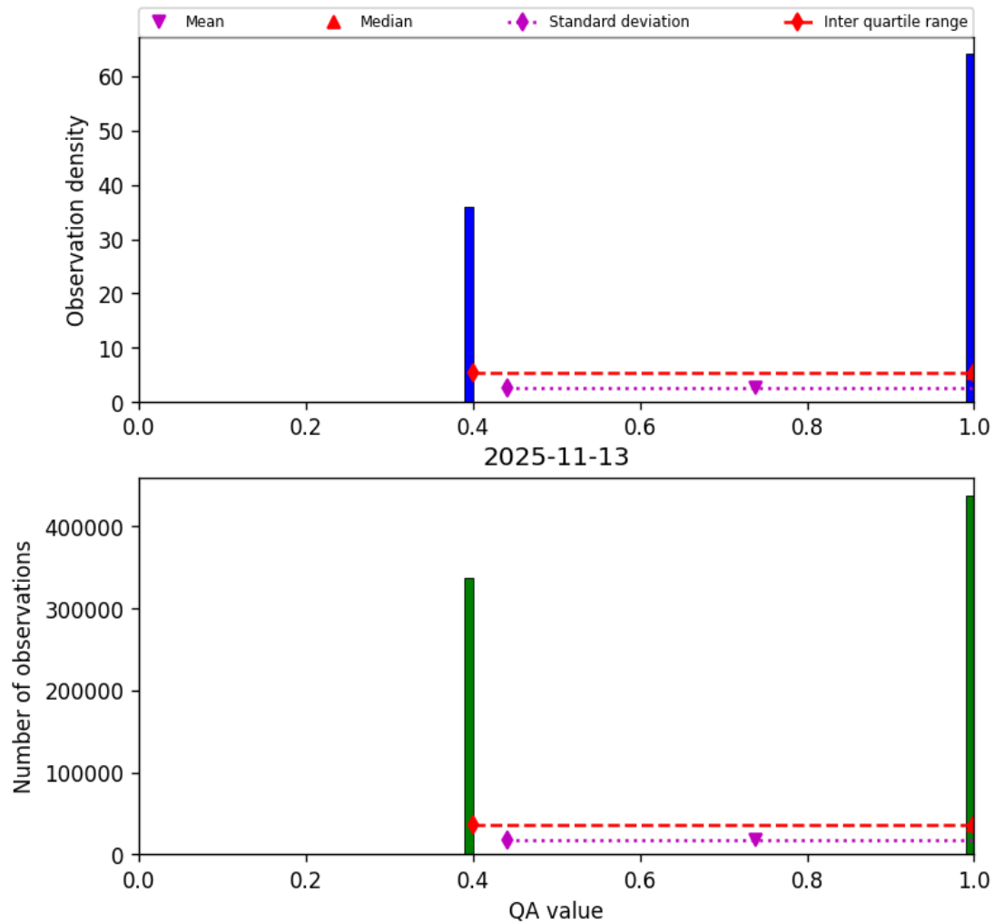
Figure 22: Histogram of “QA value” for 2025-11-12 to 2025-11-14
