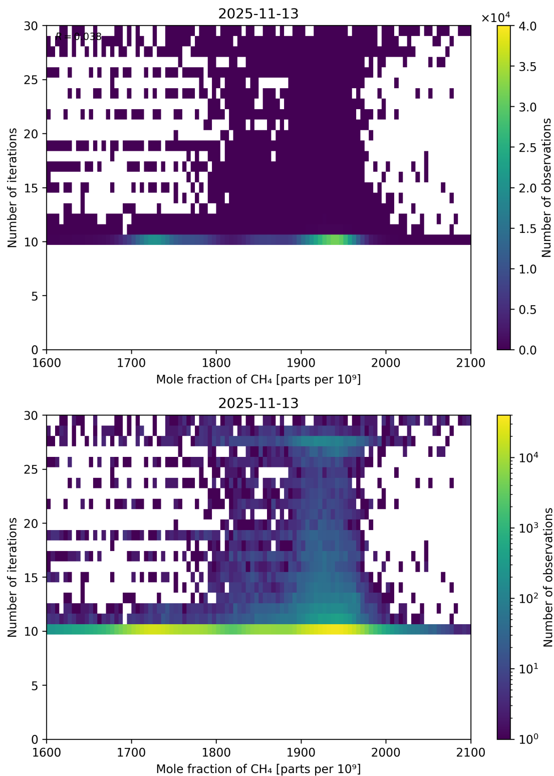
Figure 76: Scatter density plot of “Mole fraction of CH 4 ” against “Number of iterations” for 2025-11-12 to 2025-11-14.
