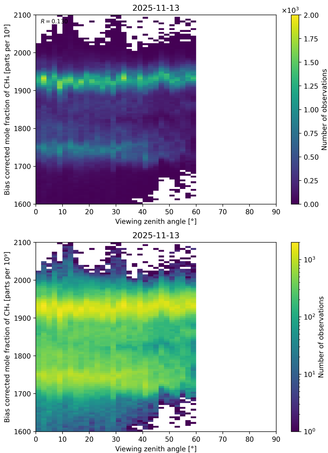
Figure 111: Scatter density plot of “Viewing zenith angle” against “Bias corrected mole fraction of CH 4 ” for 2025-11-12 to 2025-11-14.
