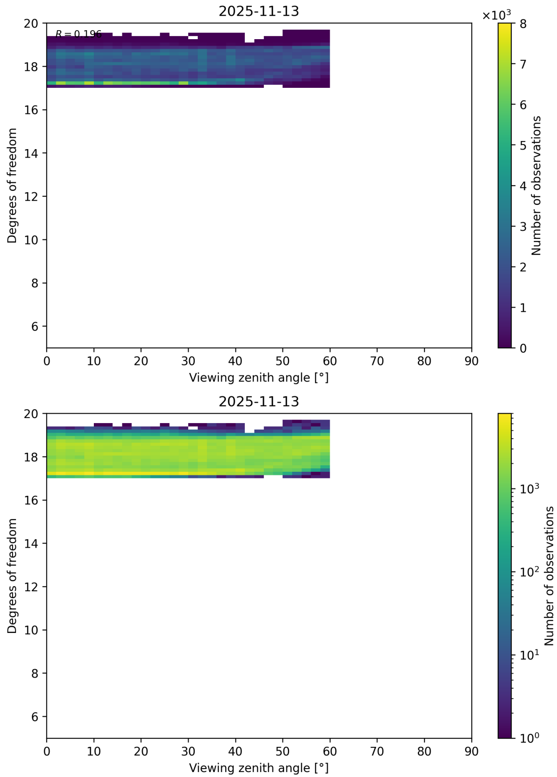
Figure 107: Scatter density plot of “Viewing zenith angle” against “Degrees of freedom” for 2025-11-12 to 2025-11-14.
