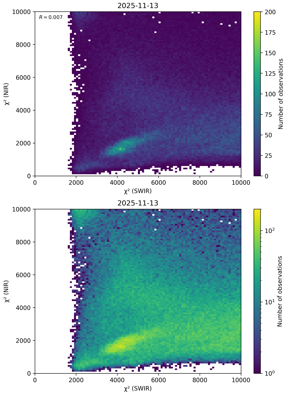
Figure 47: Scatter density plot of “ \chi^2 (SWIR)” against “ \chi^2 (NIR)” for 2025-11-12 to 2025-11-14.
