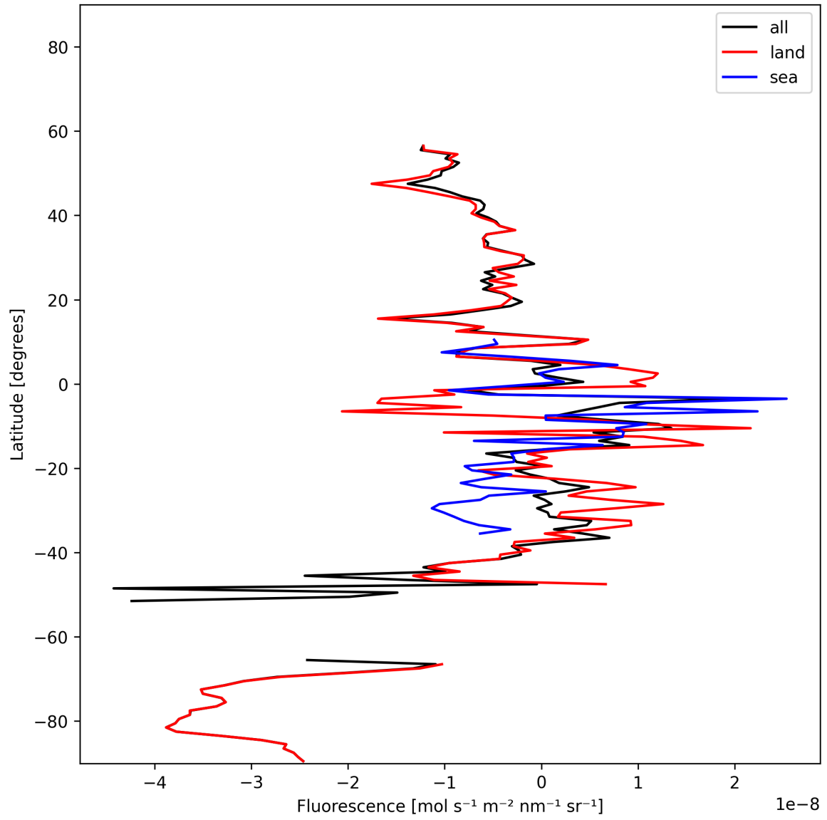
Figure 21: Zonal average of “Fluorescence” for 2025-11-12 to 2025-11-14.
