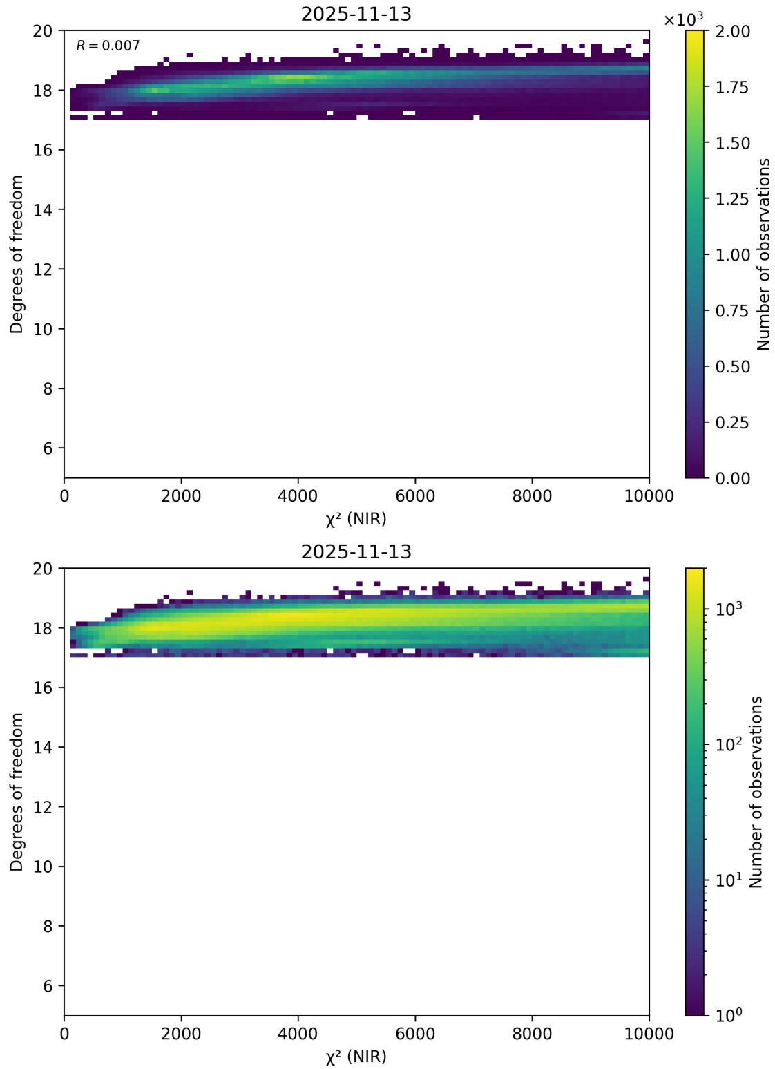
Figure 44: Scatter density plot of “ \chi^2 (NIR)” against “Degrees of freedom” for 2025-11-12 to 2025-11-14.
