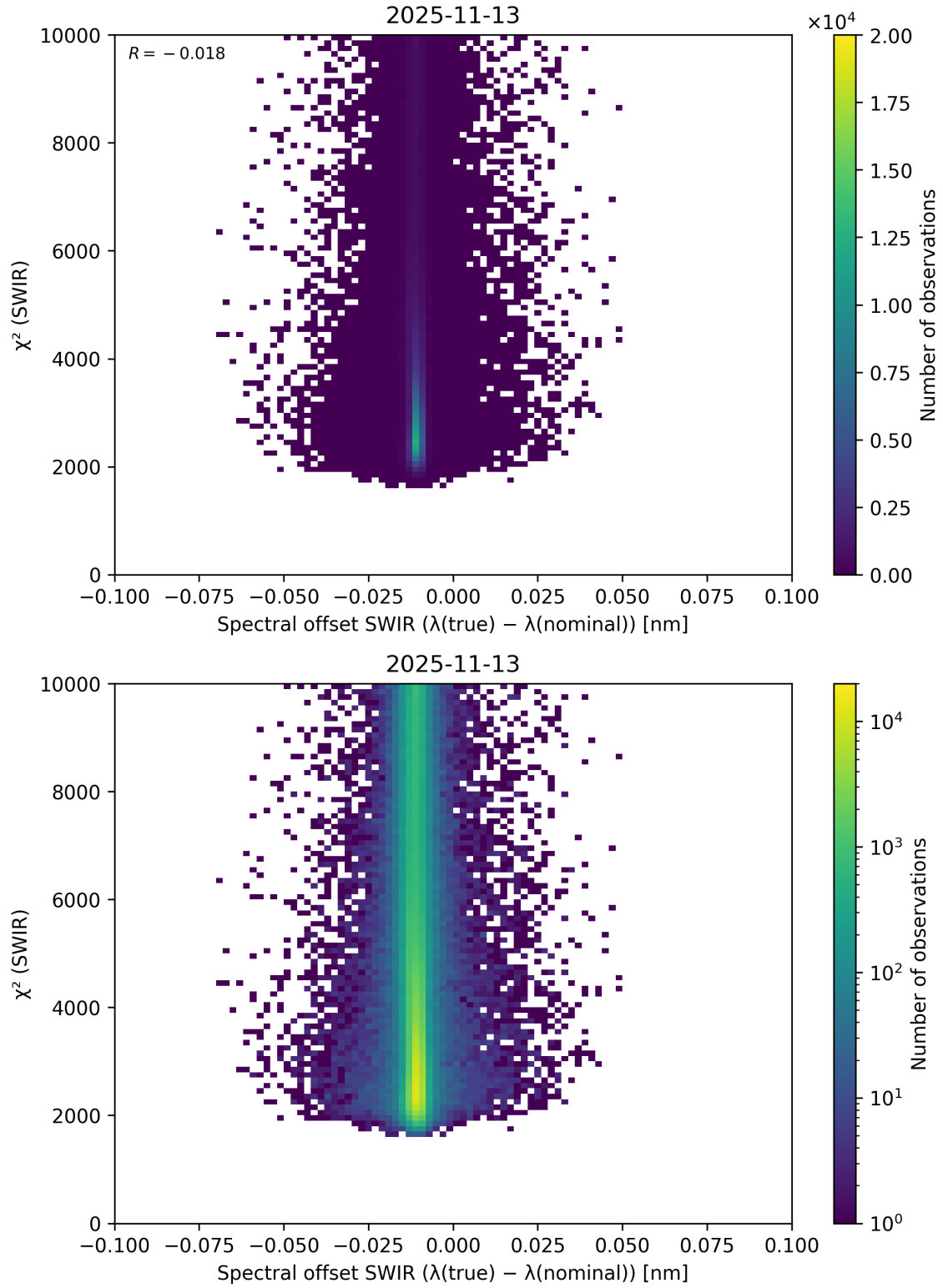
Figure 118: Scatter density plot of “Spectral offset SWIR ( \lambda_{\text{true}} - \lambda_{\text{nominal}} )” against “ \chi^2 (SWIR)” for 2025-11-12 to 2025-11-14.
