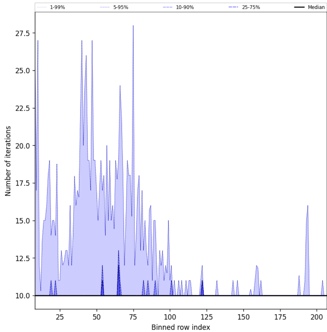
Figure 42: Along track statistics of “Number of iterations” for 2025-11-12 to 2025-11-14
