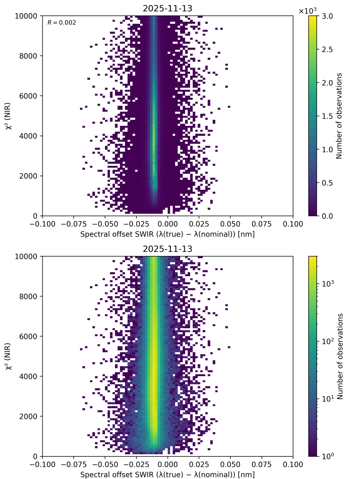
Figure 117: Scatter density plot of “Spectral offset SWIR ( \lambda_{\text{true}} - \lambda_{\text{nominal}} )” against “ \chi^2 (NIR)” for 2025-11-12 to 2025-11-14.
