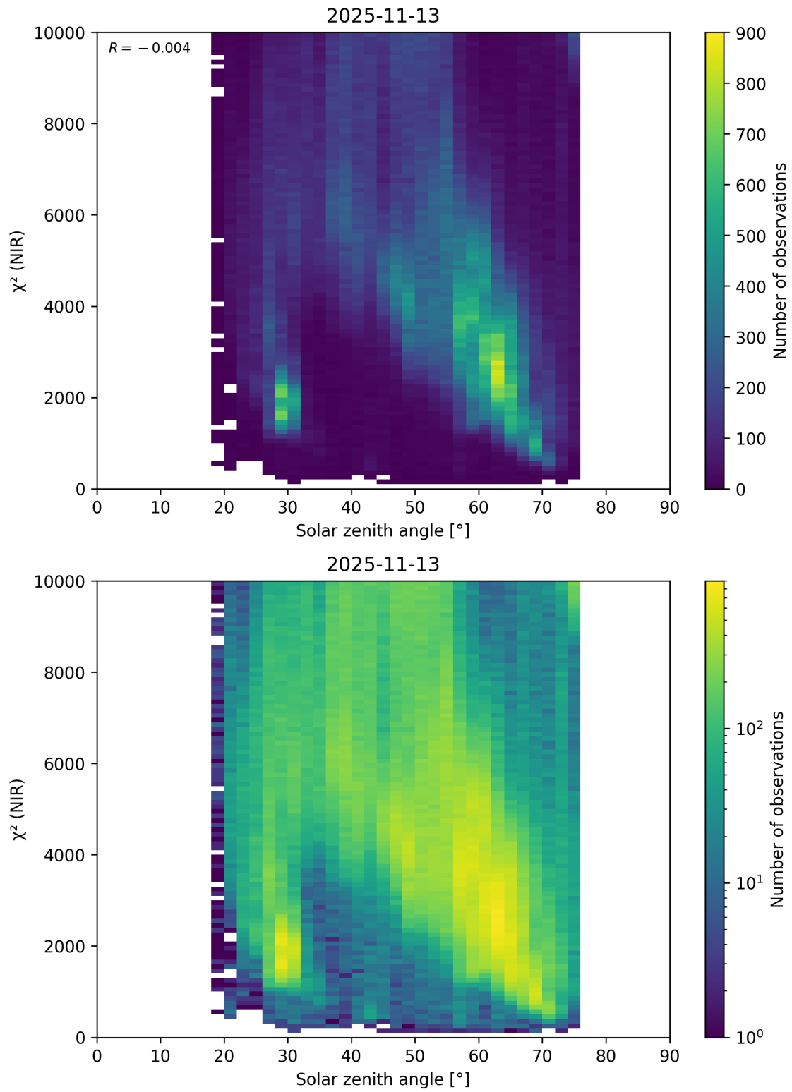
Figure 94: Scatter density plot of “Solar zenith angle” against “ \chi^2 (NIR)” for 2025-11-12 to 2025-11-14.
