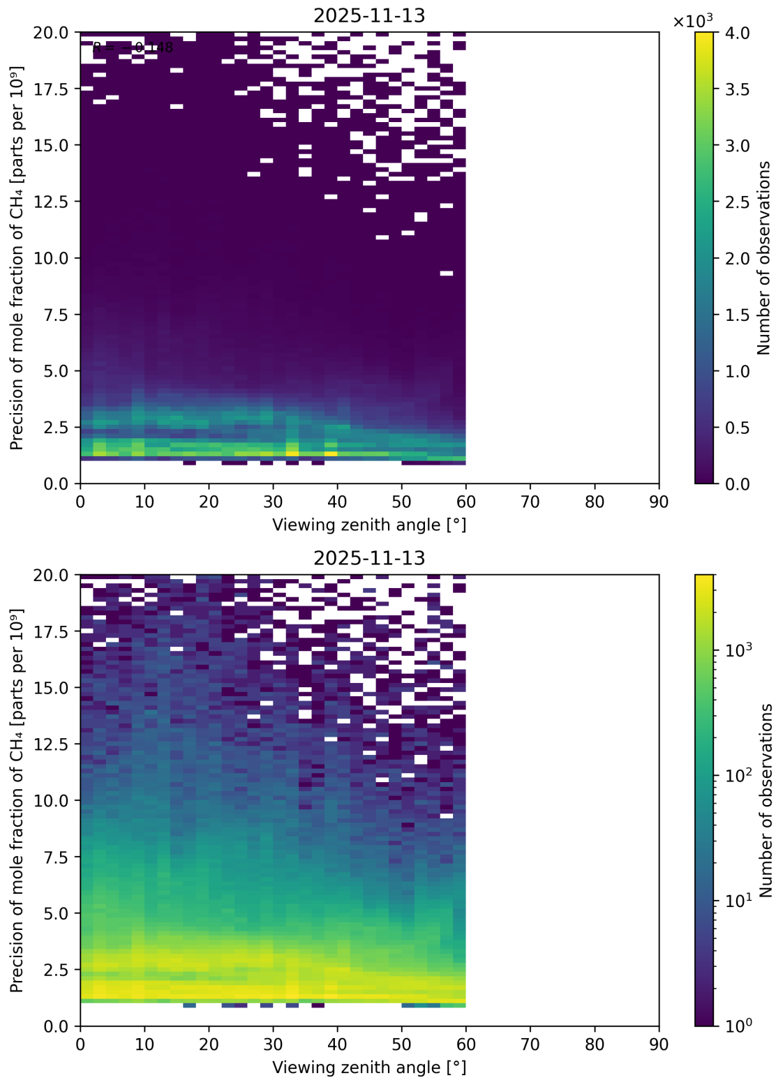
Figure 112: Scatter density plot of “Viewing zenith angle” against “Precision of mole fraction of CH 4 ” for 2025-11-12 to 2025-11-14.
