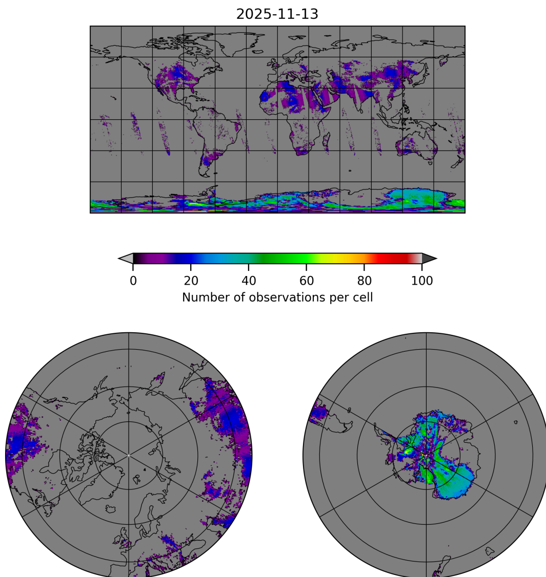
Figure 10: Map of the number of observations for 2025-11-12 to 2025-11-14
