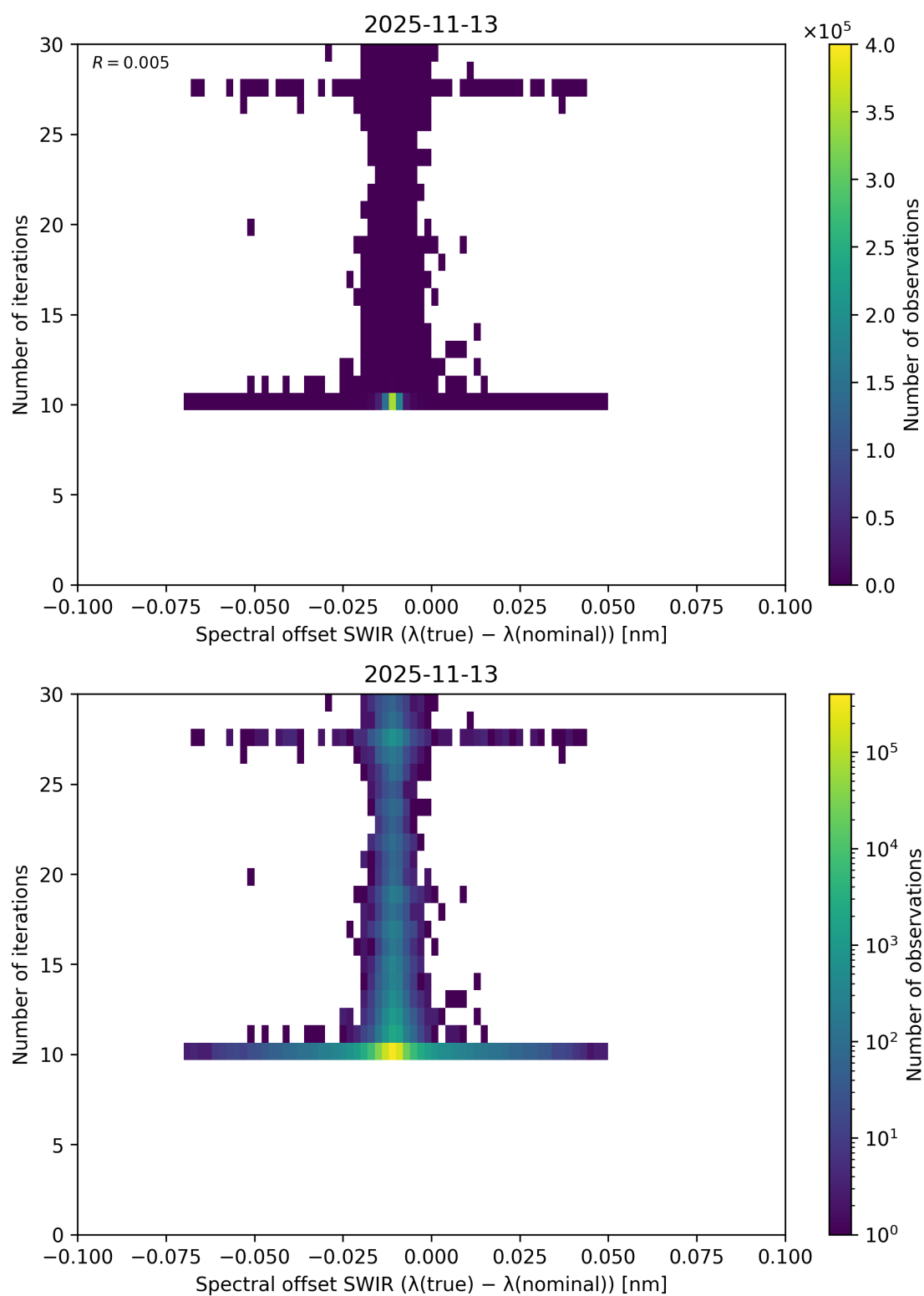
Figure 121: Scatter density plot of “Spectral offset SWIR ( \lambda_{\text{true}} - \lambda_{\text{nominal}} )” against “Number of iterations” for 2025-11-12 to 2025-11-14.
