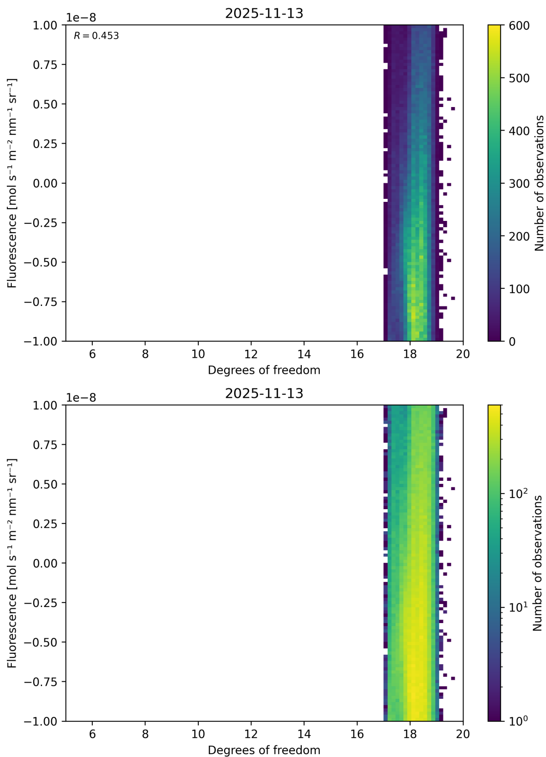
Figure 51: Scatter density plot of “Degrees of freedom” against “Fluorescence” for 2025-11-12 to 2025-11-14.
