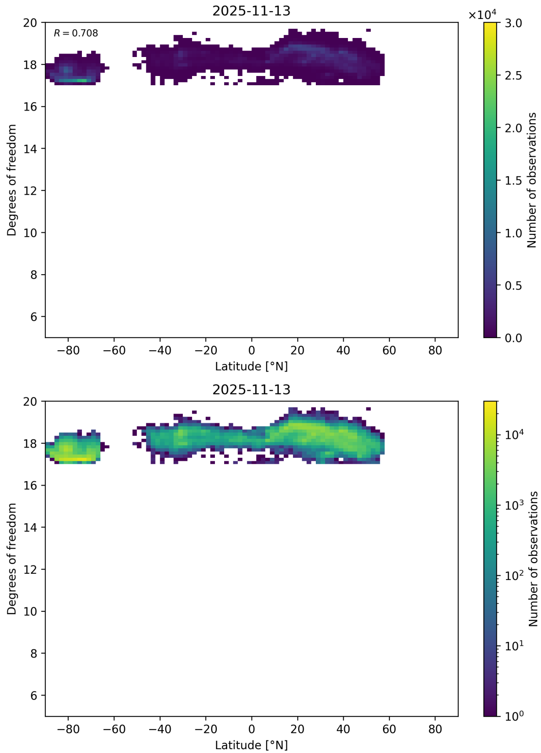
Figure 55: Scatter density plot of “Latitude” against “Degrees of freedom” for 2025-11-12 to 2025-11-14.
