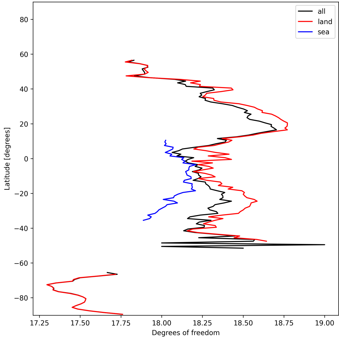
Figure 19: Zonal average of “Degrees of freedom” for 2025-11-12 to 2025-11-14.
