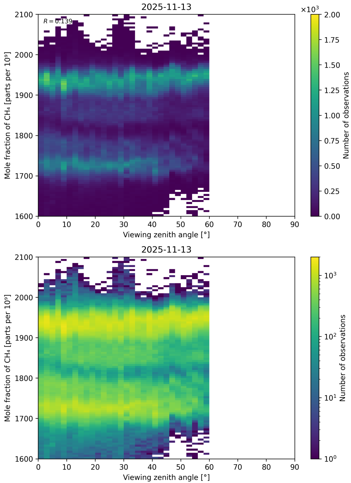
Figure 110: Scatter density plot of “Viewing zenith angle” against “Mole fraction of CH 4 ” for 2025-11-12 to 2025-11-14.
