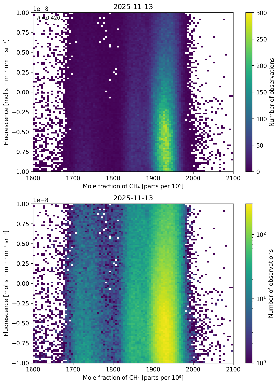
Figure 73: Scatter density plot of “Mole fraction of \text{CH}_4 ” against “Fluorescence” for 2025-11-12 to 2025-11-14.
