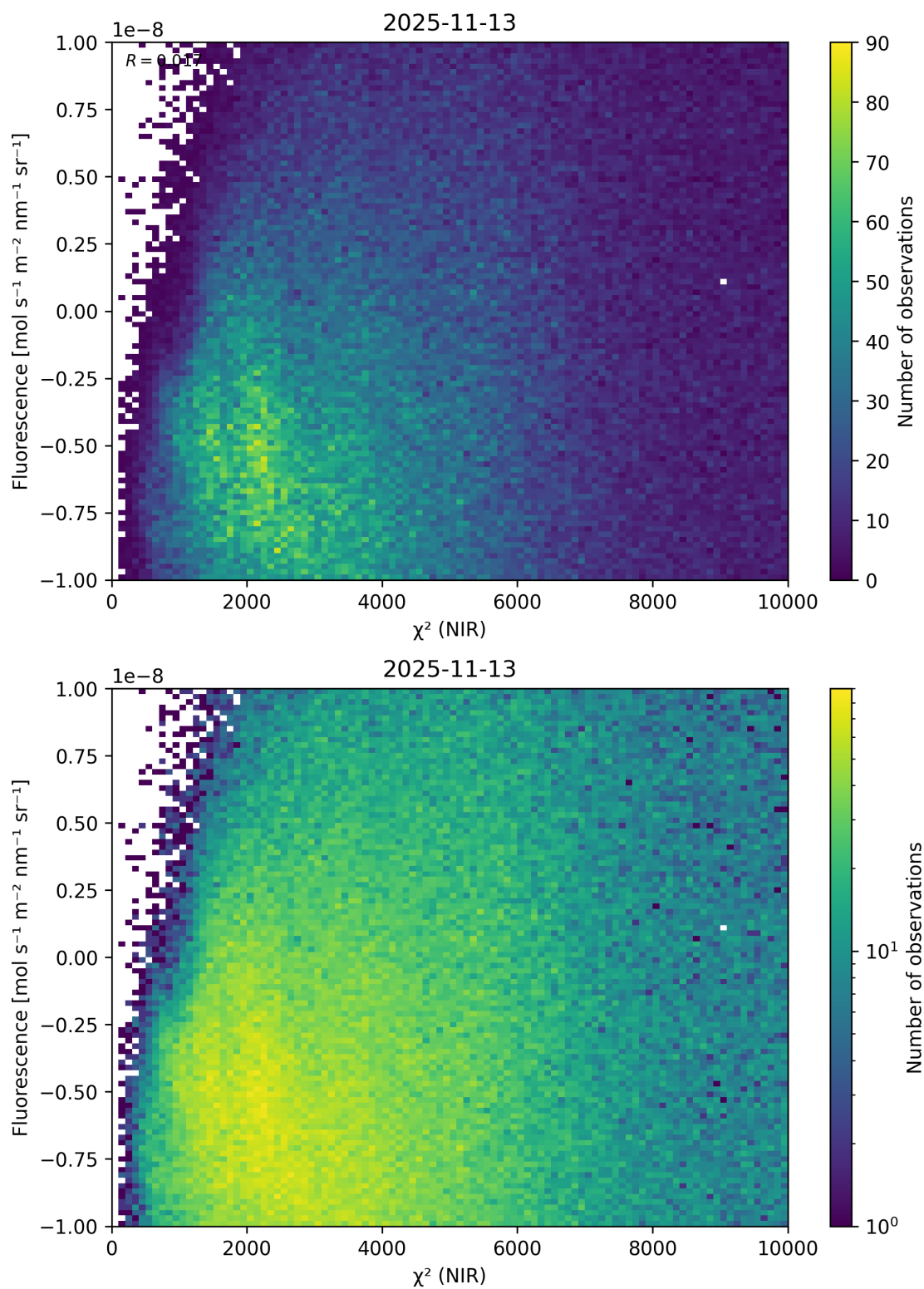
Figure 45: Scatter density plot of “ \chi^2 (NIR)” against “Fluorescence” for 2025-11-12 to 2025-11-14.
