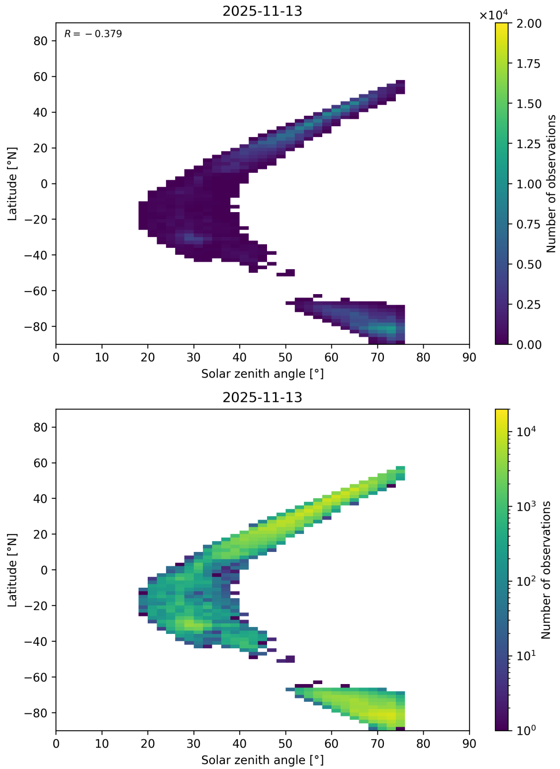
Figure 98: Scatter density plot of “Solar zenith angle” against “Latitude” for 2025-11-12 to 2025-11-14.
