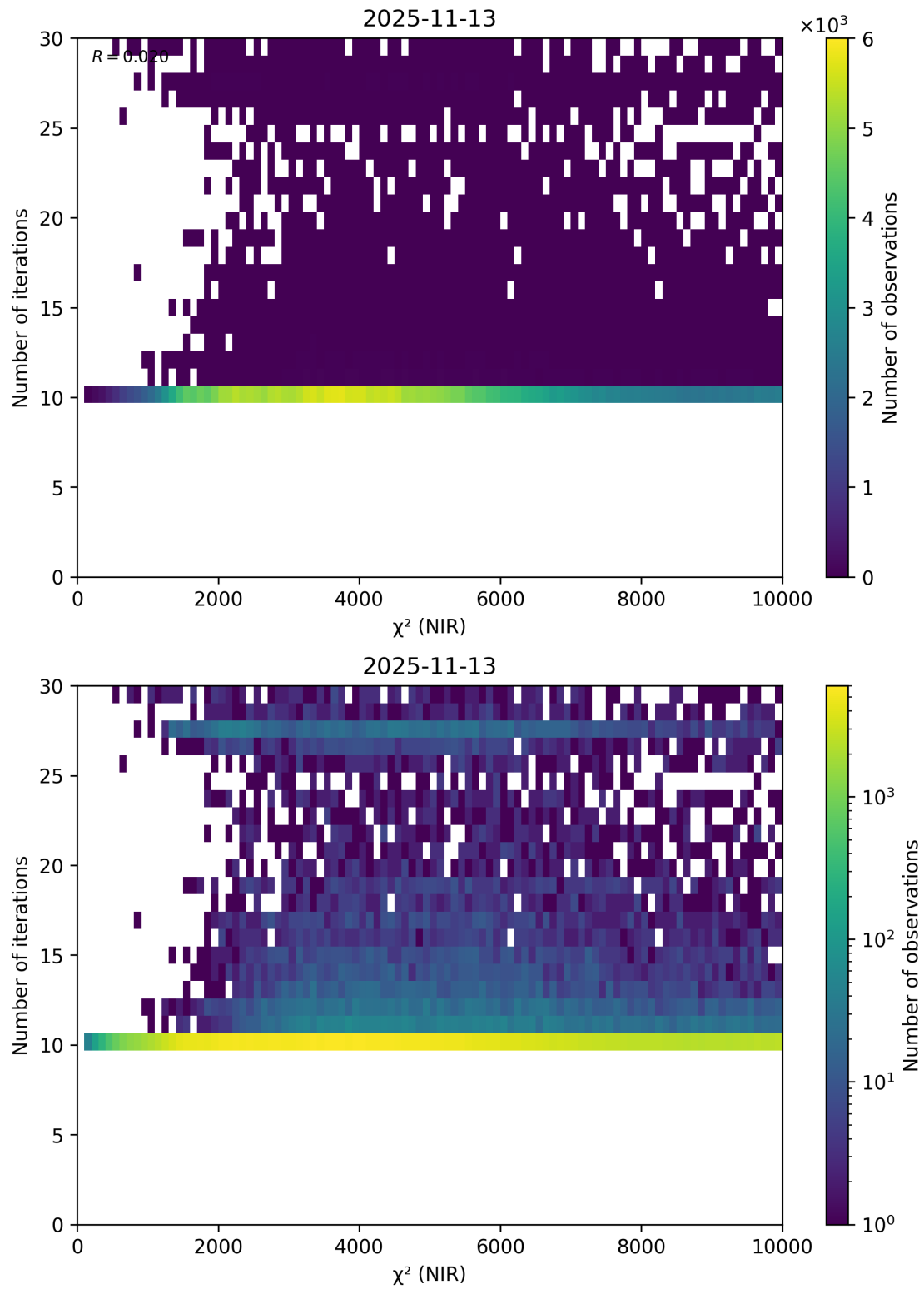
Figure 46: Scatter density plot of “ \chi^2 (NIR)” against “Number of iterations” for 2025-11-12 to 2025-11-14.
