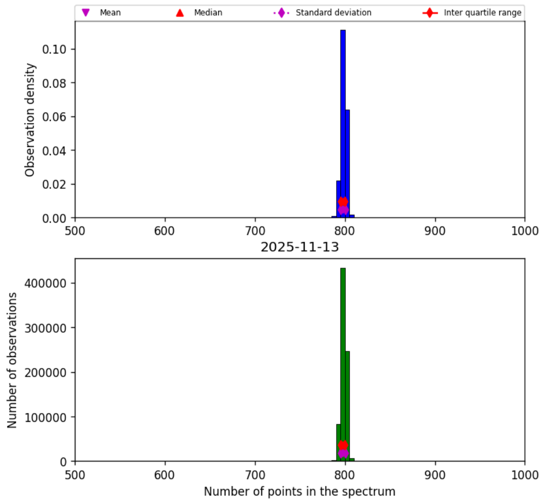
Figure 26: Histogram of “Number of points in the spectrum” for 2025-11-12 to 2025-11-14
