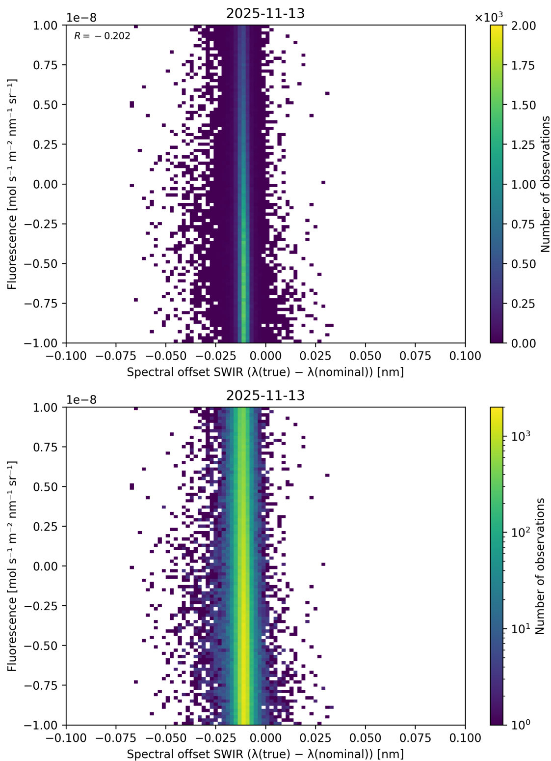
Figure 120: Scatter density plot of “Spectral offset SWIR ( \lambda_{\text{true}} - \lambda_{\text{nominal}} )” against “Fluorescence” for 2025-11-12 to 2025-11-14.
