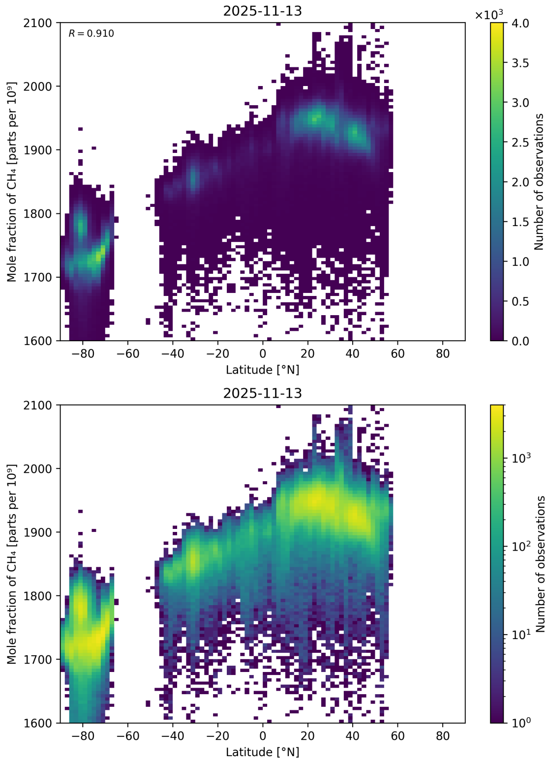
Figure 57: Scatter density plot of “Latitude” against “Mole fraction of CH 4 ” for 2025-11-12 to 2025-11-14.
