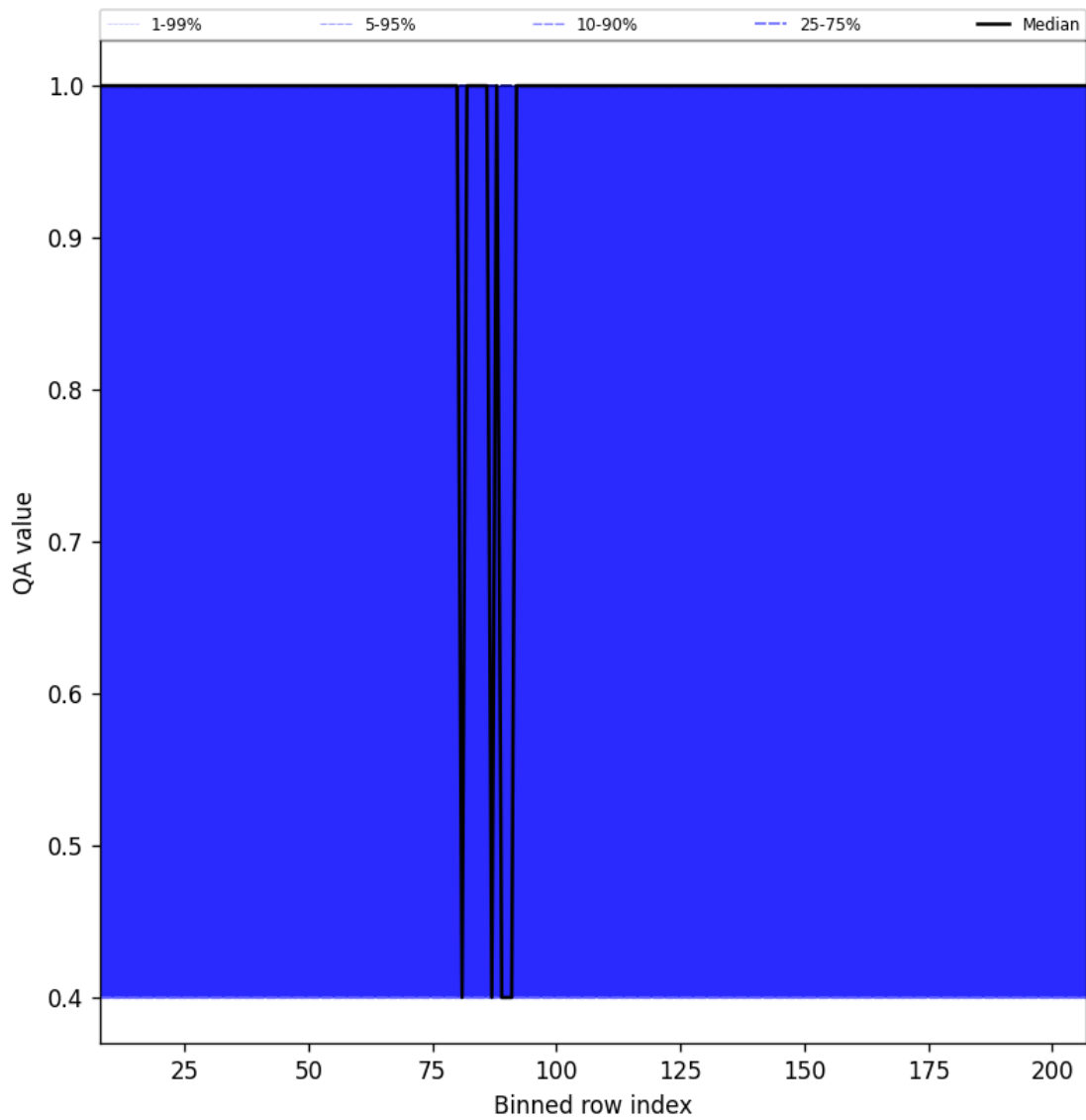
Figure 33: Along track statistics of “QA value” for 2025-11-12 to 2025-11-14
