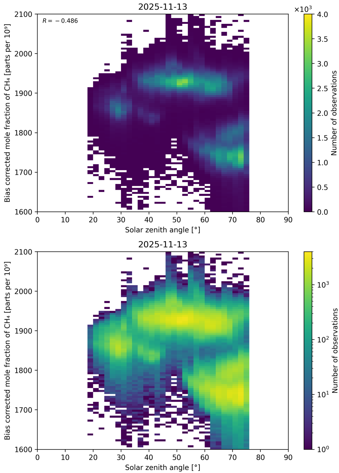
Figure 100: Scatter density plot of “Solar zenith angle” against “Bias corrected mole fraction of \text{CH}_4 ” for 2025-11-12 to 2025-11-14.
