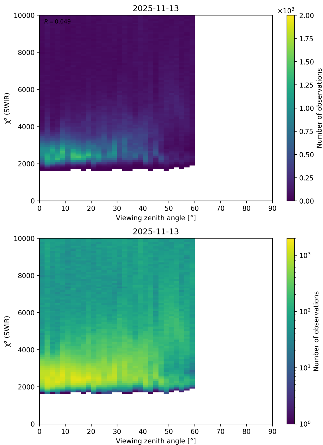
Figure 106: Scatter density plot of “Viewing zenith angle” against “ \chi^2 (SWIR)” for 2025-11-12 to 2025-11-14.
