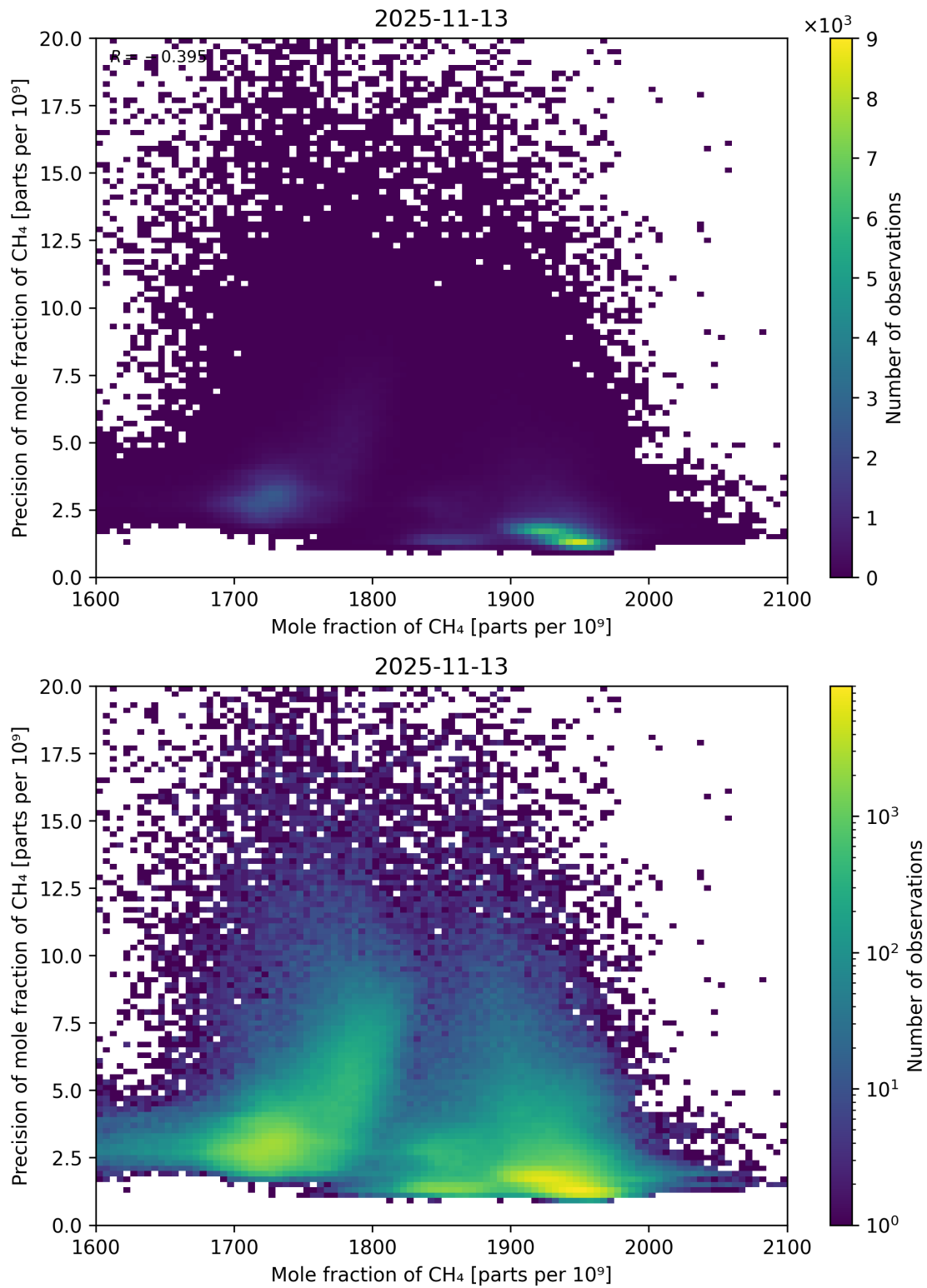
Figure 75: Scatter density plot of “Mole fraction of CH 4 ” against “Precision of mole fraction of CH 4 ” for 2025-11-12 to 2025-11-14.
