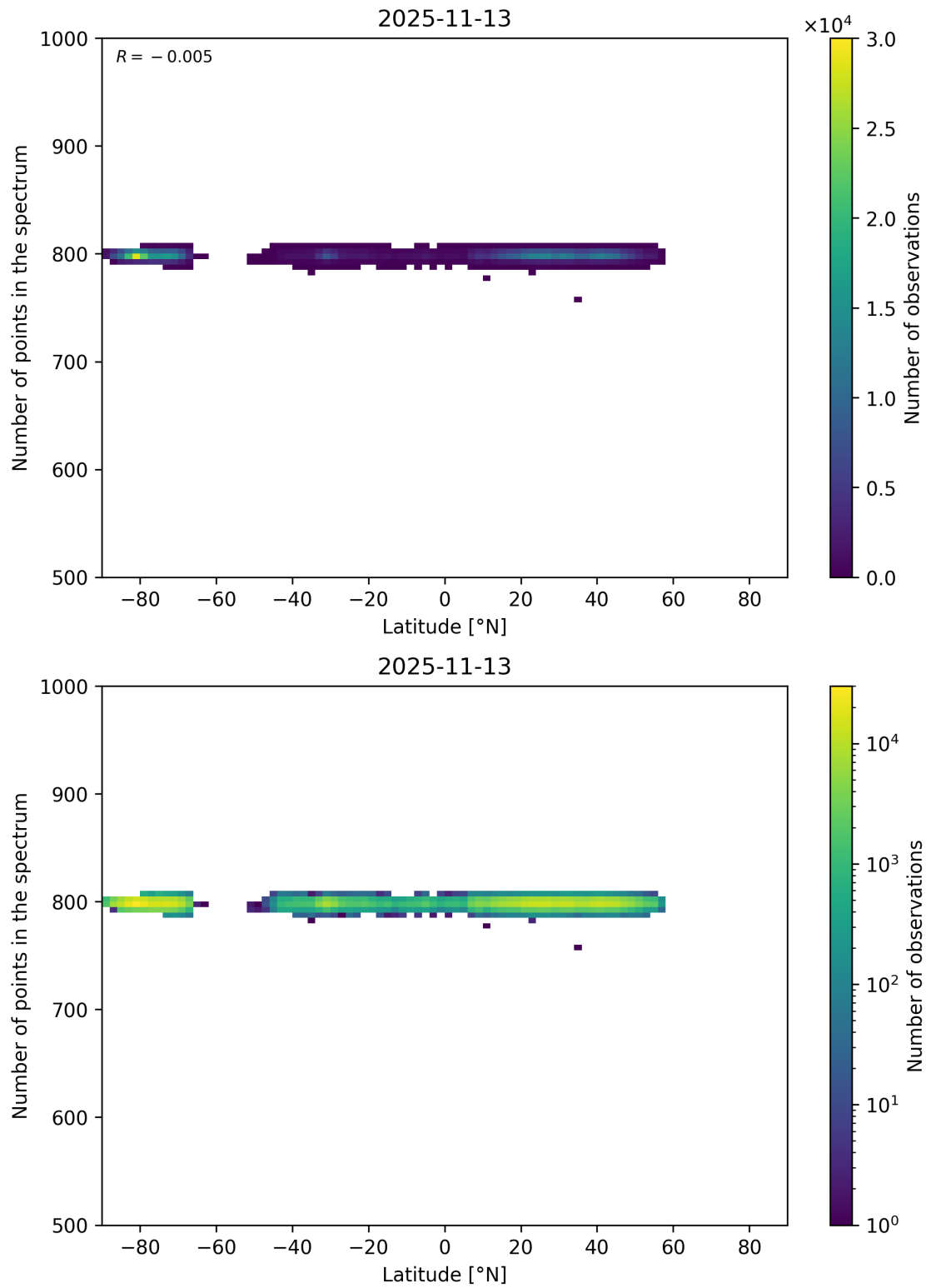
Figure 61: Scatter density plot of “Latitude” against “Number of points in the spectrum” for 2025-11-12 to 2025-11-14.
