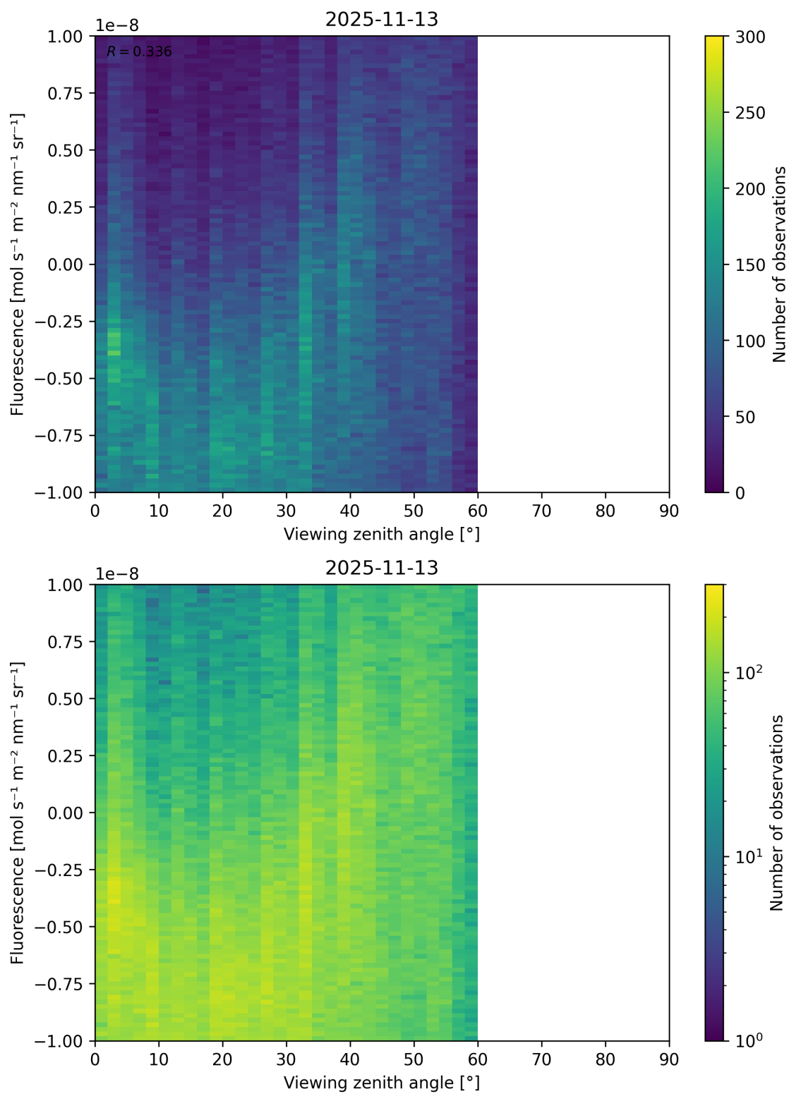
Figure 108: Scatter density plot of “Viewing zenith angle” against “Fluorescence” for 2025-11-12 to 2025-11-14.
