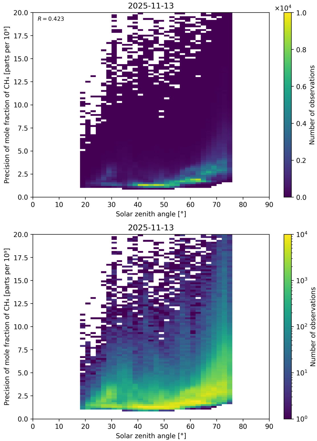
Figure 101: Scatter density plot of “Solar zenith angle” against “Precision of mole fraction of \text{CH}_4 ” for 2025-11-12 to 2025-11-14.
