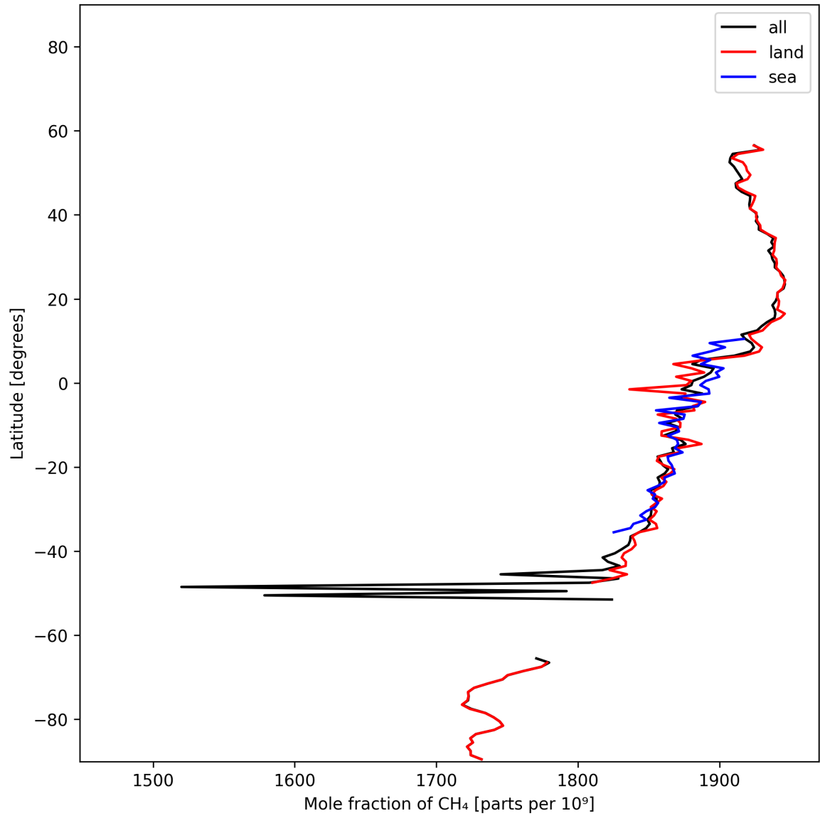
Figure 12: Zonal average of “Mole fraction of \text{CH}_4 ” for 2025-11-12 to 2025-11-14.
