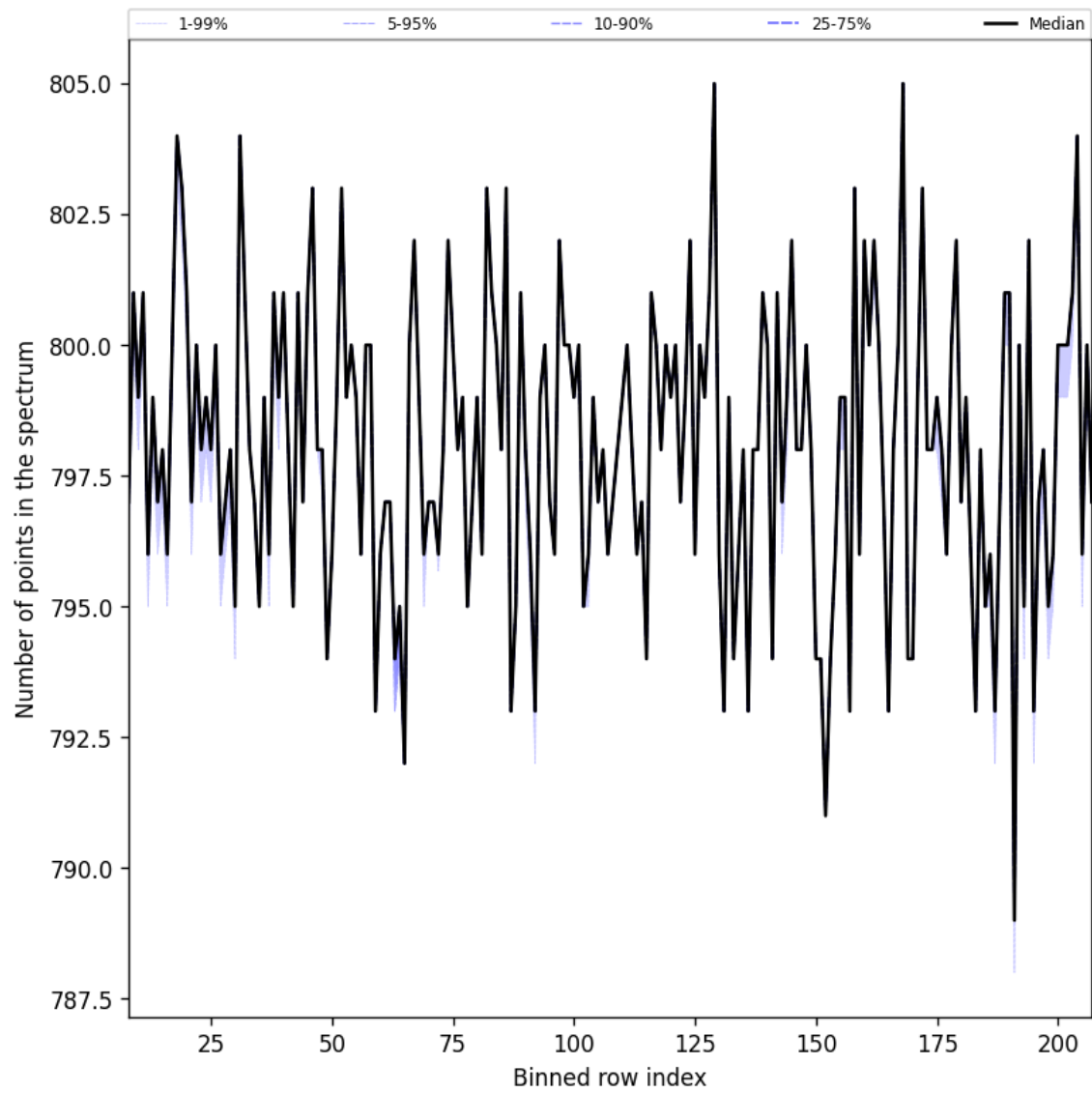
Figure 37: Along track statistics of “Number of points in the spectrum” for 2025-11-12 to 2025-11-14
