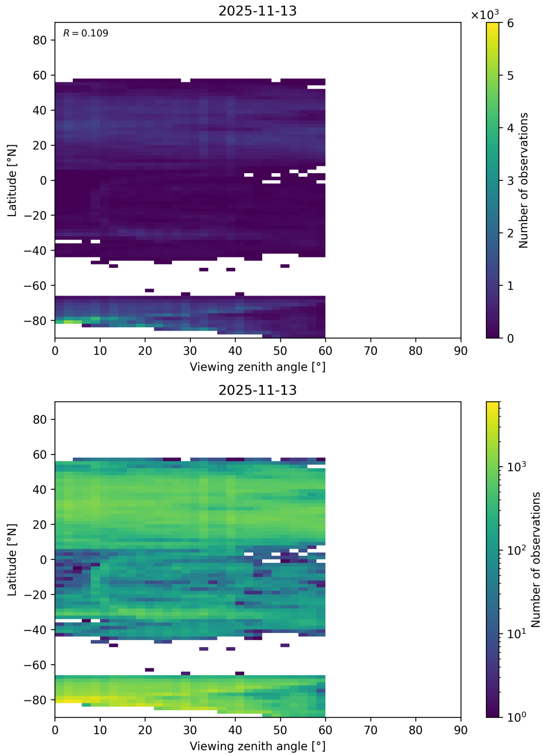
Figure 109: Scatter density plot of “Viewing zenith angle” against “Latitude” for 2025-11-12 to 2025-11-14.
