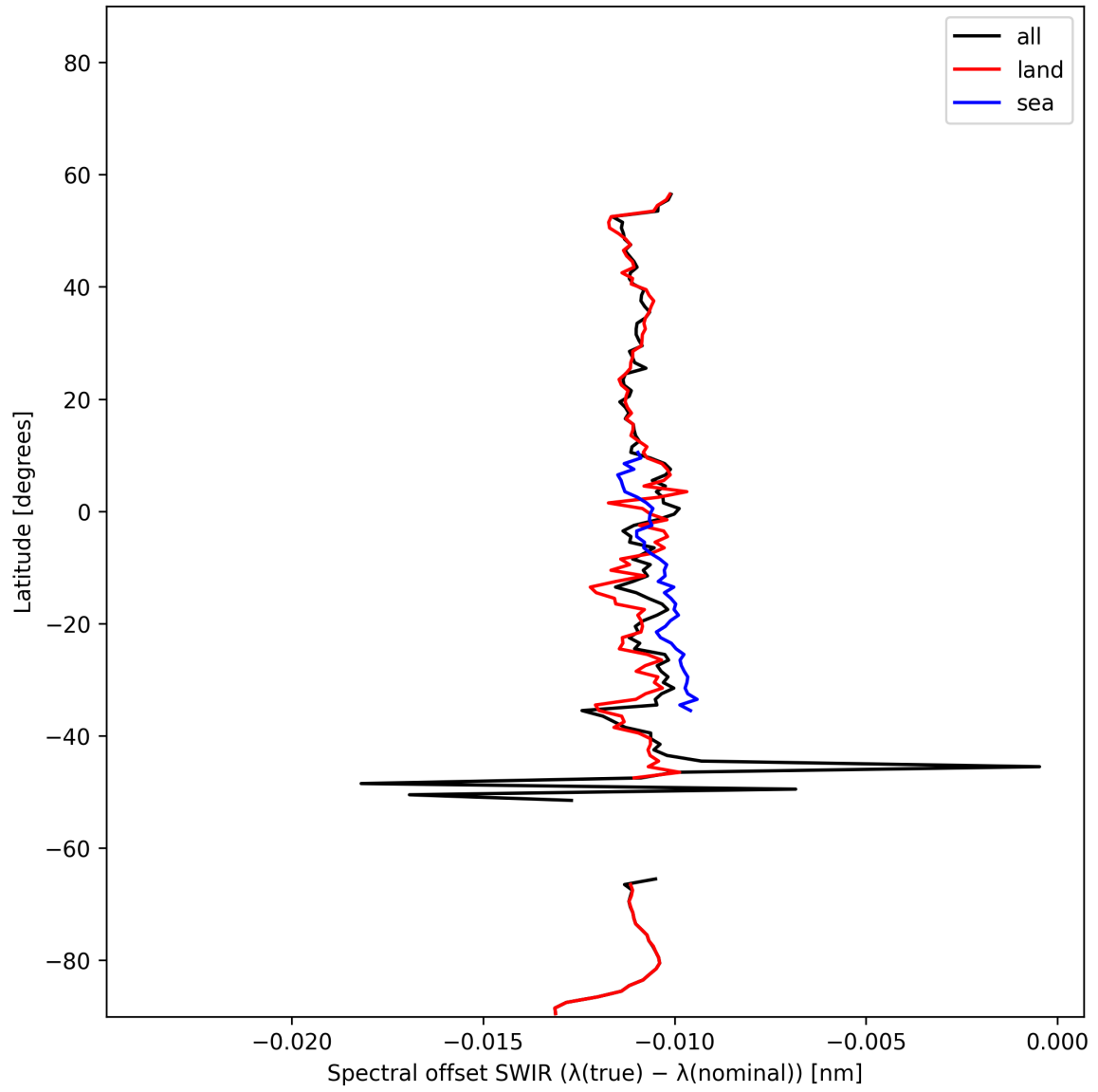
Figure 16: Zonal average of “Spectral offset SWIR ( \lambda_{\text{true}} - \lambda_{\text{nominal}} )” for 2025-11-12 to 2025-11-14.
