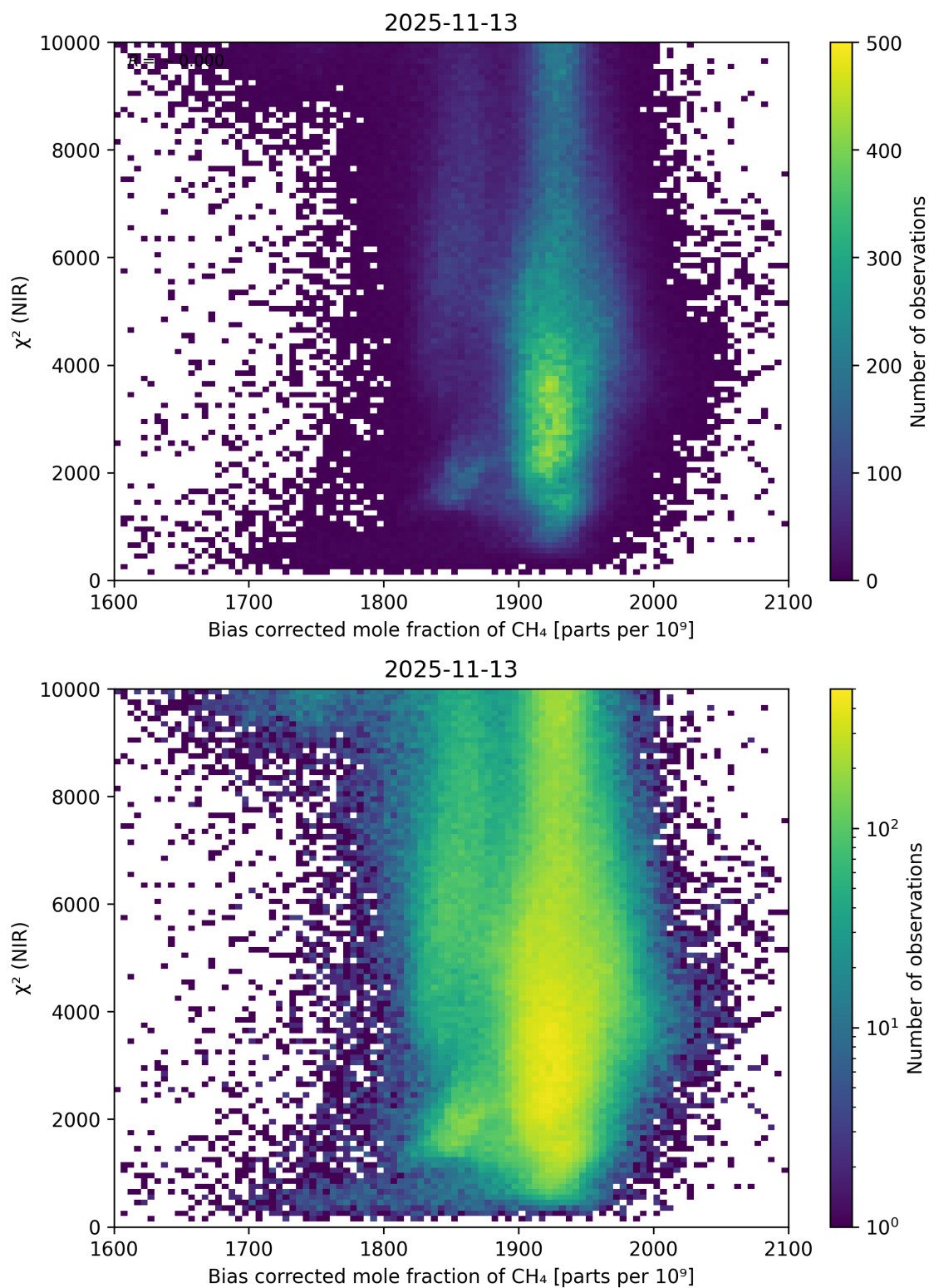
Figure 63: Scatter density plot of “Bias corrected mole fraction of \text{CH}_4 ” against “ \chi^2 (NIR)” for 2025-11-12 to 2025-11-14.
