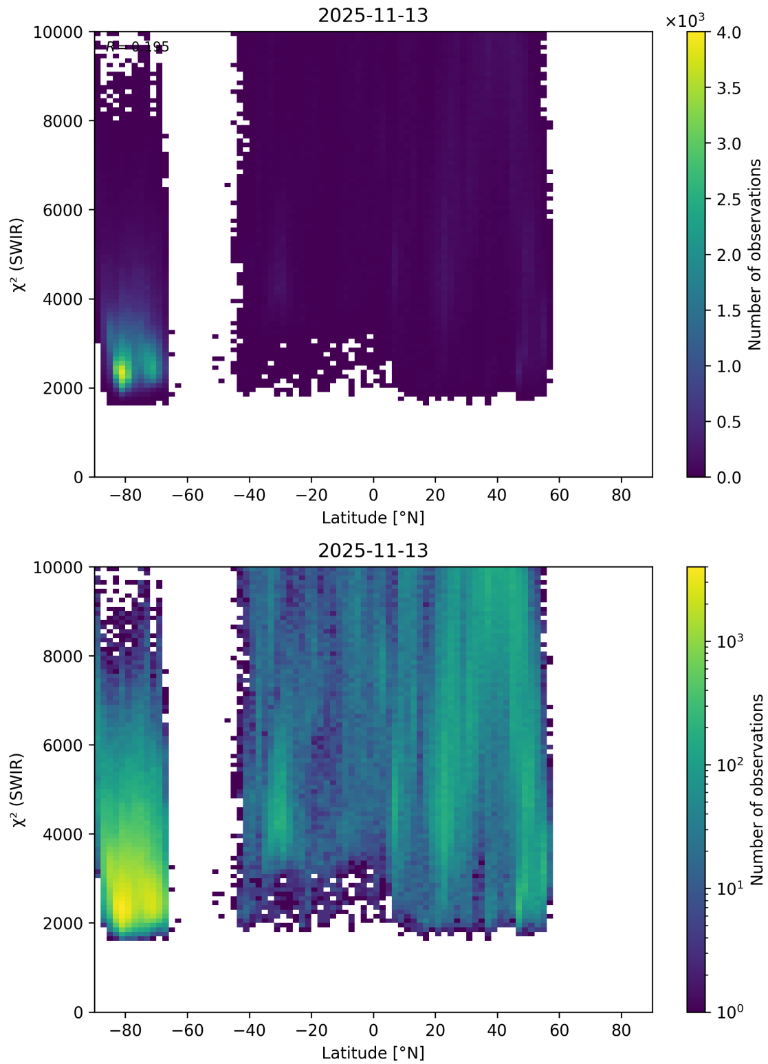
Figure 54: Scatter density plot of “Latitude” against “ \chi^2 (SWIR)” for 2025-11-12 to 2025-11-14.
