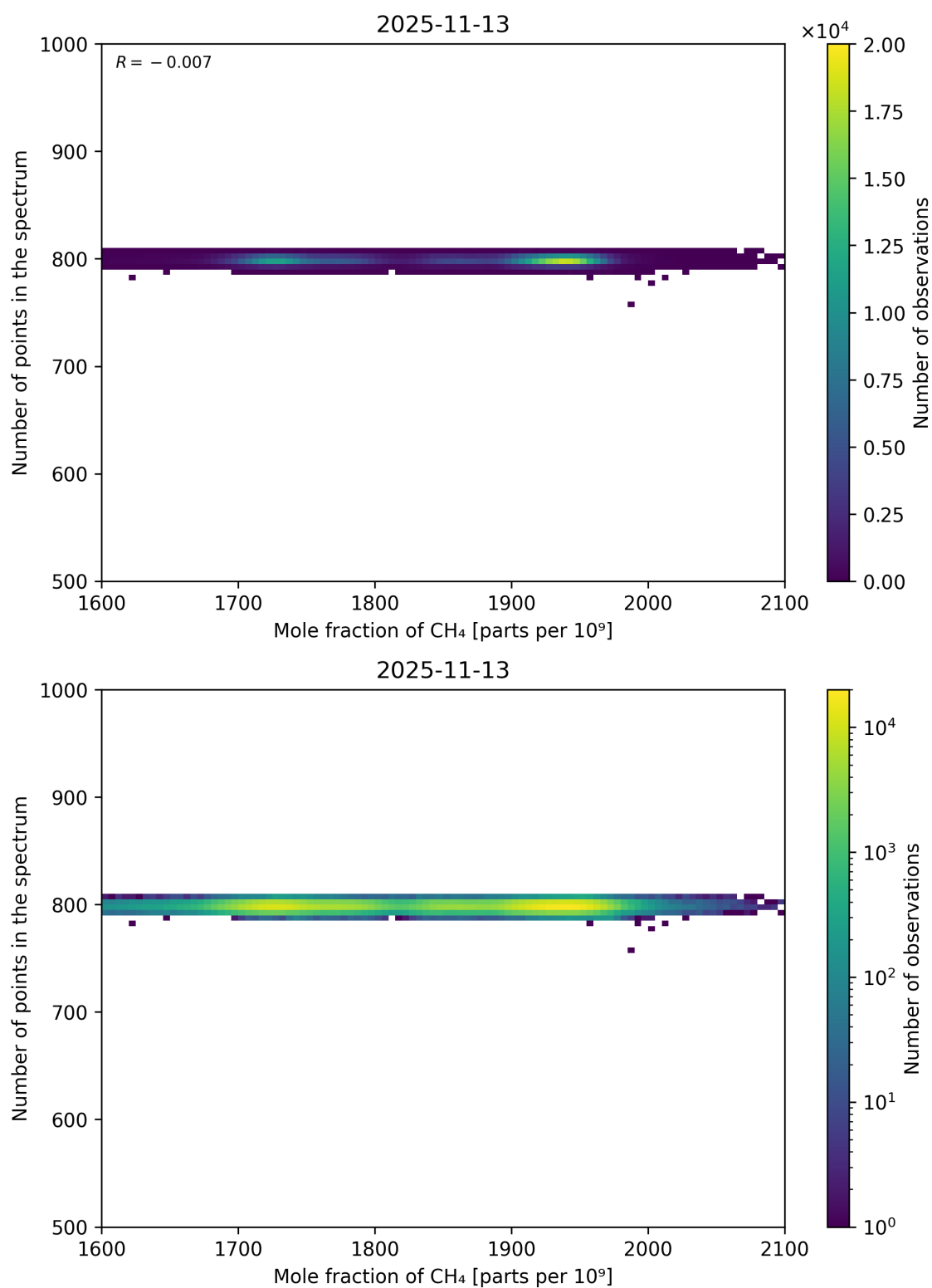
Figure 77: Scatter density plot of “Mole fraction of CH 4 ” against “Number of points in the spectrum” for 2025-11-12 to 2025-11-14.
