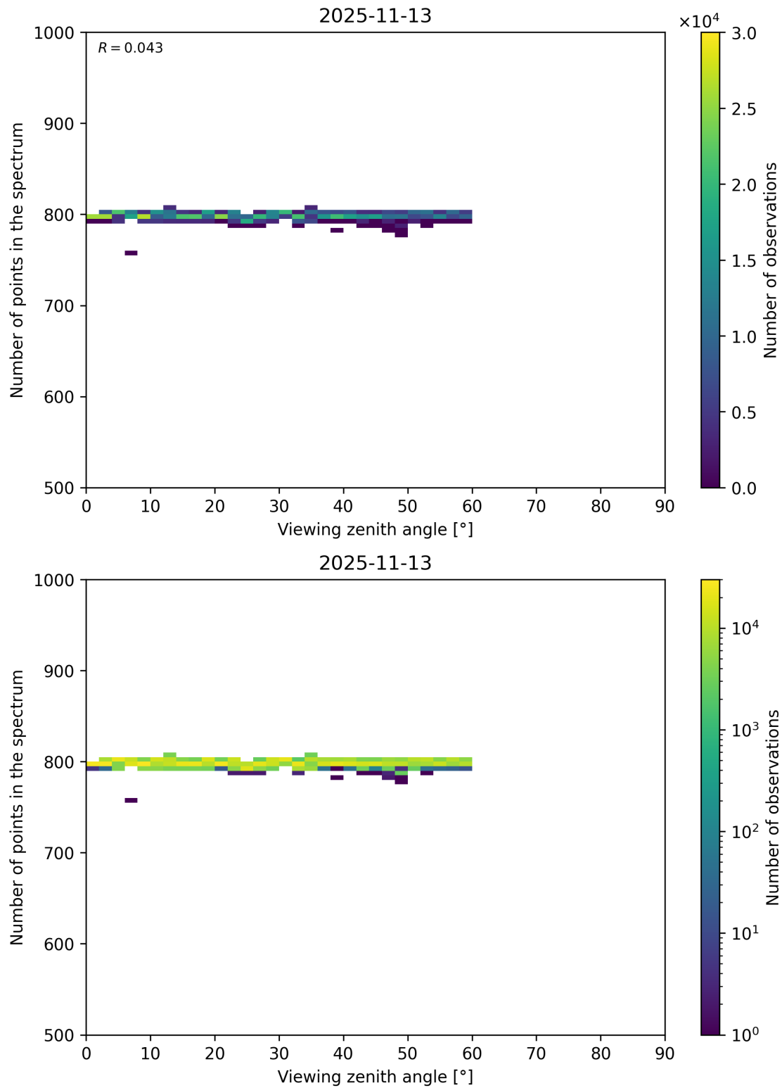
Figure 114: Scatter density plot of “Viewing zenith angle” against “Number of points in the spectrum” for 2025-11-12 to 2025-11-14.
