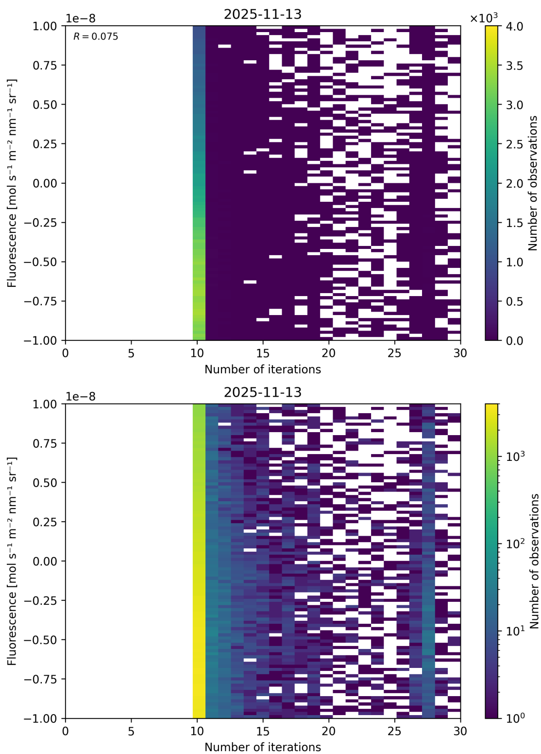
Figure 87: Scatter density plot of “Number of iterations” against “Fluorescence” for 2025-11-12 to 2025-11-14.
