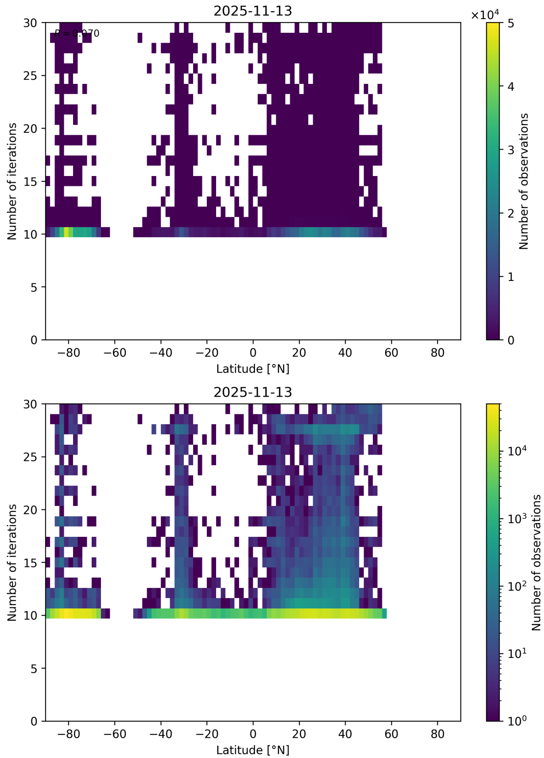
Figure 60: Scatter density plot of “Latitude” against “Number of iterations” for 2025-11-12 to 2025-11-14.
