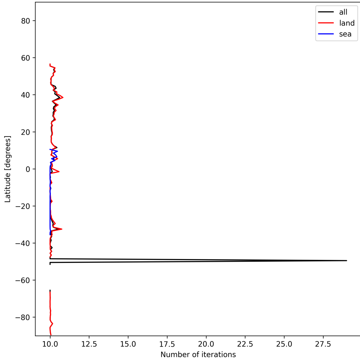
Figure 20: Zonal average of “Number of iterations” for 2025-11-12 to 2025-11-14.
