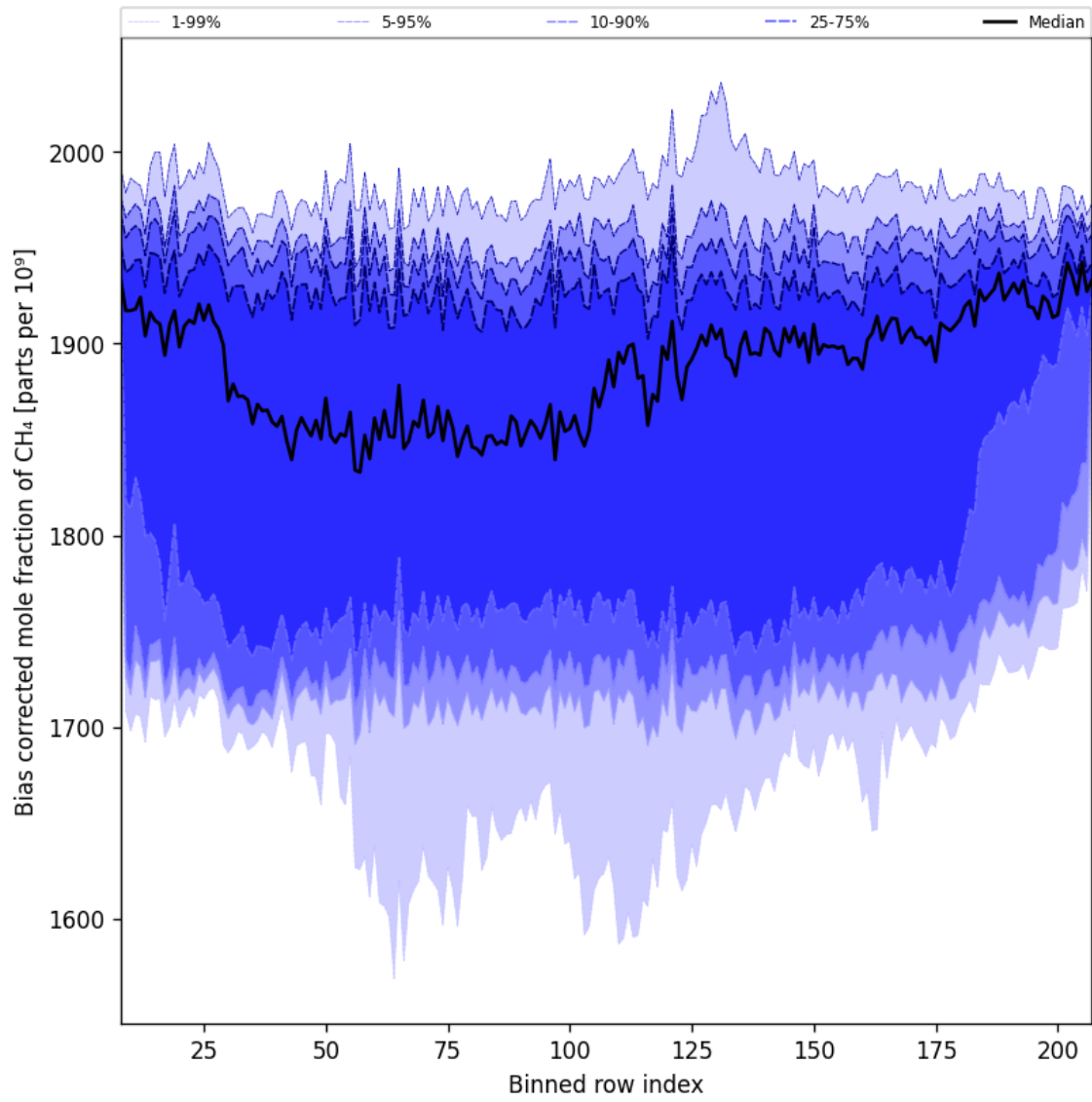
Figure 36: Along track statistics of “Bias corrected mole fraction of CH 4 ” for 2025-11-12 to 2025-11-14
