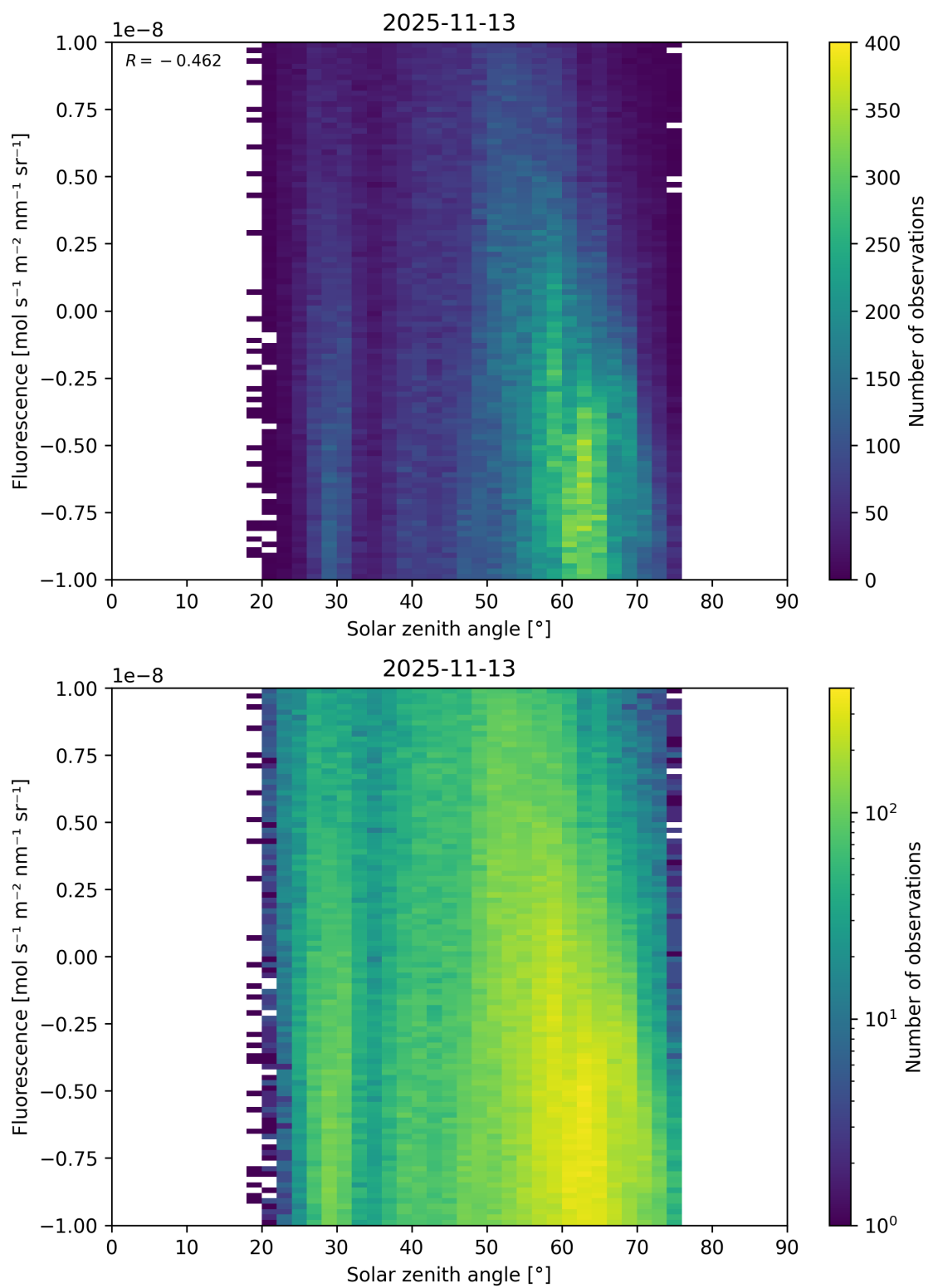
Figure 97: Scatter density plot of “Solar zenith angle” against “Fluorescence” for 2025-11-12 to 2025-11-14.
