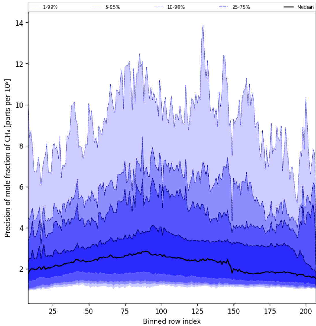
Figure 35: Along track statistics of “Precision of mole fraction of CH 4 ” for 2025-11-12 to 2025-11-14
