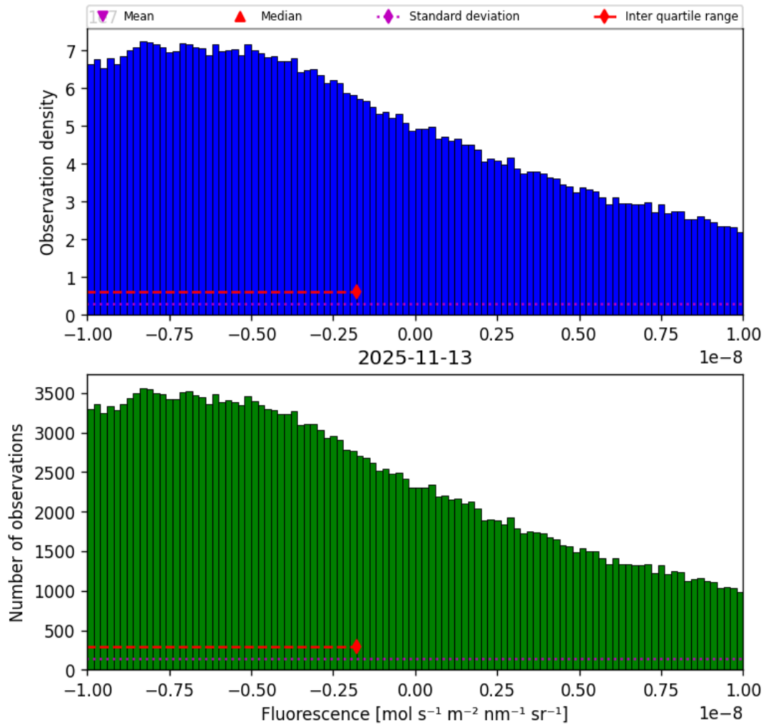
Figure 32: Histogram of “Fluorescence” for 2025-11-12 to 2025-11-14
