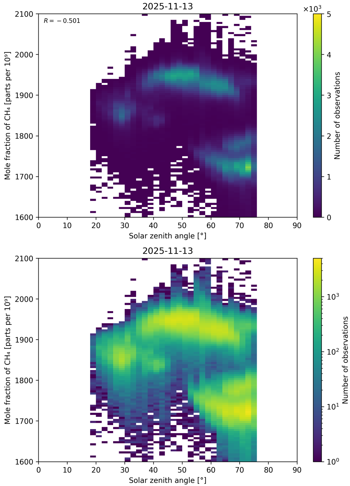
Figure 99: Scatter density plot of “Solar zenith angle” against “Mole fraction of CH 4 ” for 2025-11-12 to 2025-11-14.
