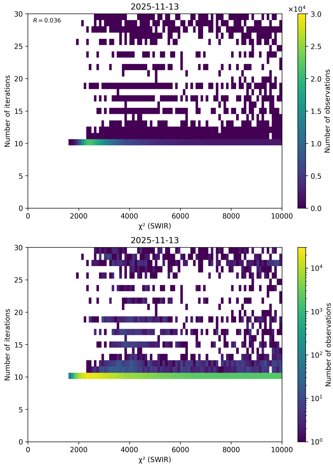
Figure 50: Scatter density plot of “ \chi^2 (SWIR)” against “Number of iterations” for 2025-11-12 to 2025-11-14.
