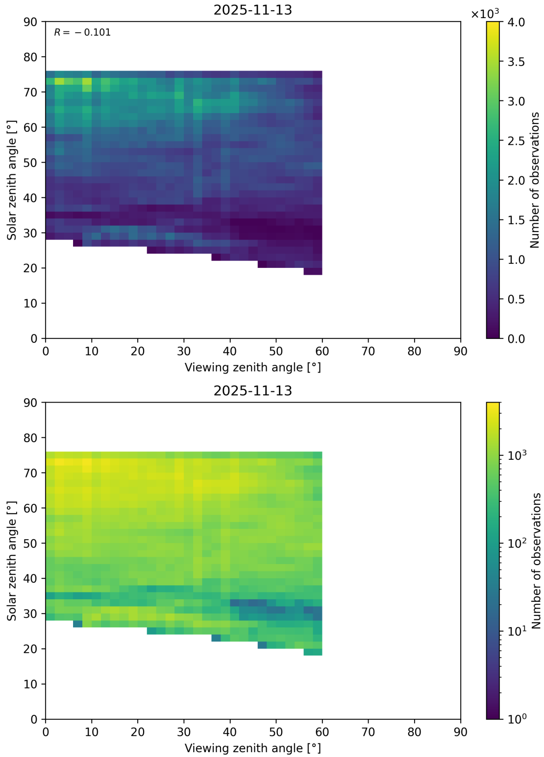
Figure 115: Scatter density plot of “Viewing zenith angle” against “Solar zenith angle” for 2025-11-12 to 2025-11-14.
