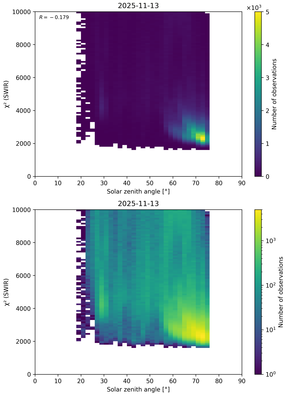
Figure 95: Scatter density plot of “Solar zenith angle” against “ \chi^2 (SWIR)” for 2025-11-12 to 2025-11-14.
