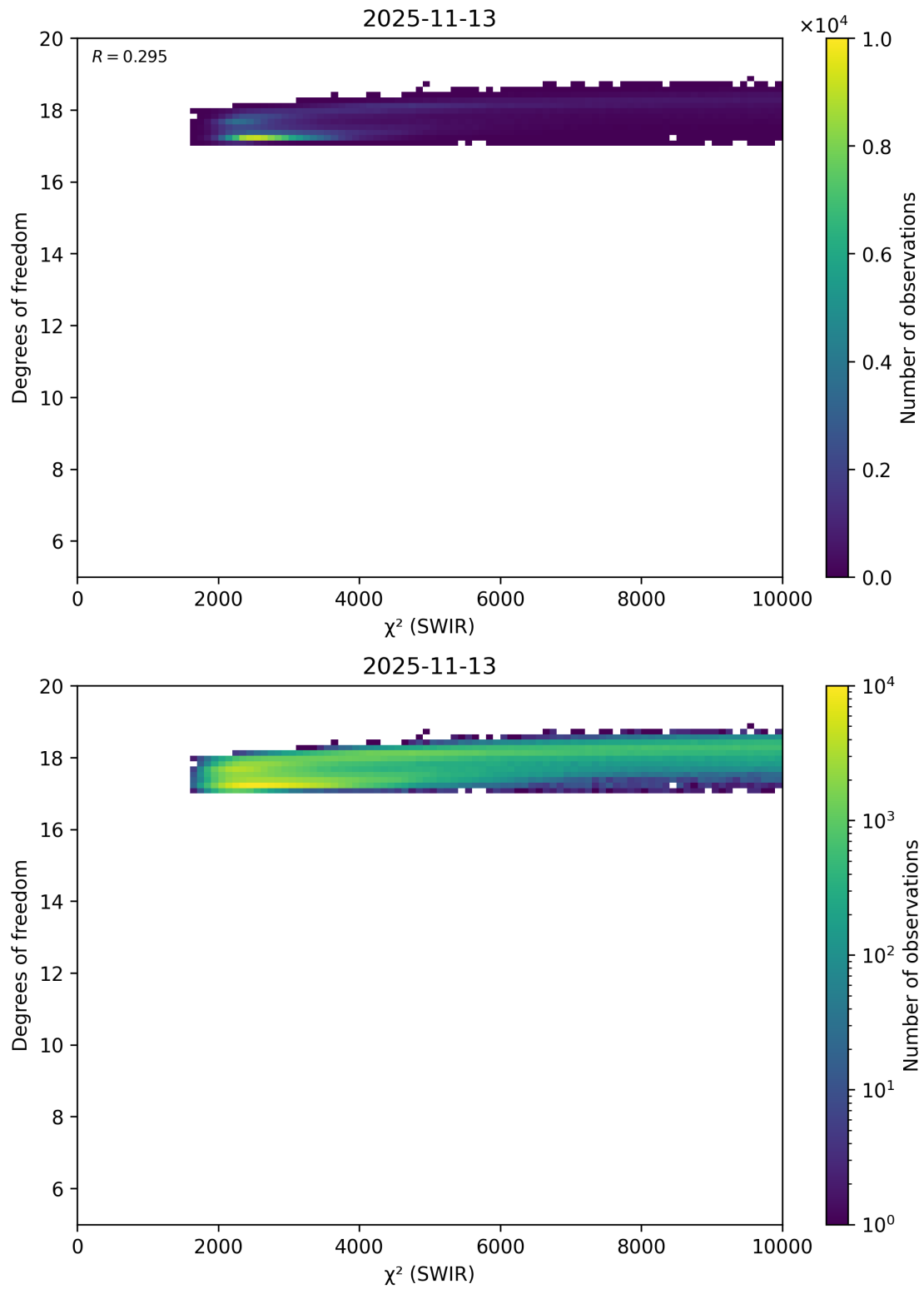
Figure 48: Scatter density plot of “ \chi^2 (SWIR)” against “Degrees of freedom” for 2025-11-12 to 2025-11-14.
