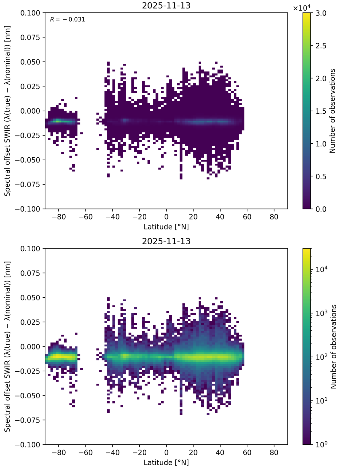
Figure 62: Scatter density plot of “Latitude” against “Spectral offset SWIR ( \lambda_{\text{true}} - \lambda_{\text{nominal}} )” for 2025-11-12 to 2025-11-14.
