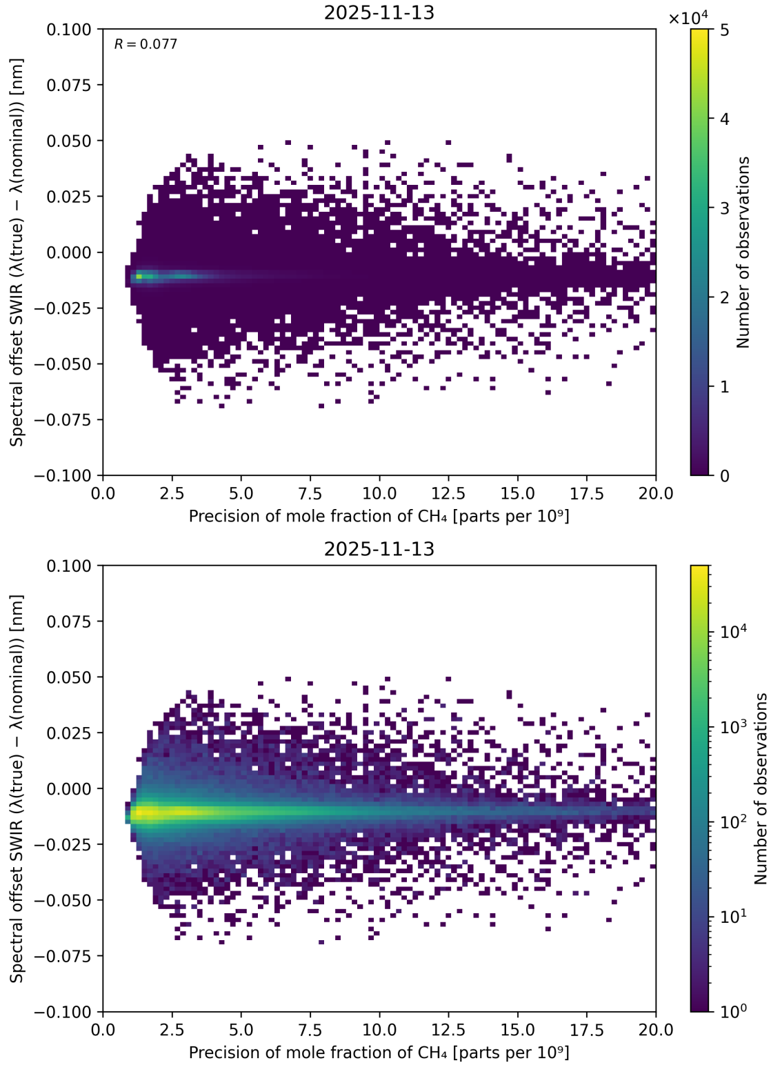
Figure 85: Scatter density plot of “Precision of mole fraction of CH 4 ” against “Spectral offset SWIR ( \lambda_{\text{true}} - \lambda_{\text{nominal}} )” for 2025-11-12 to 2025-11-14.
