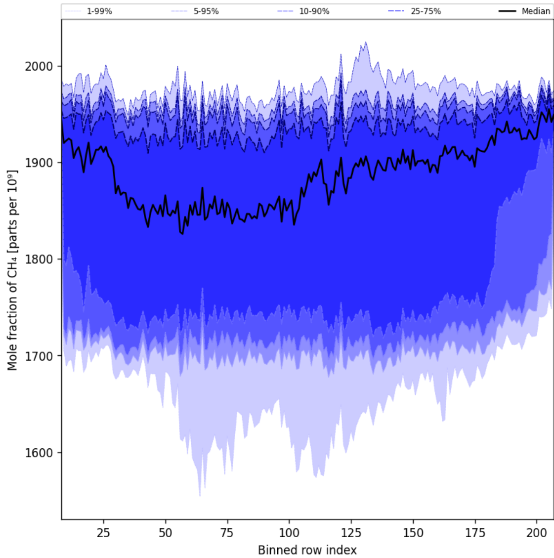
Figure 34: Along track statistics of “Mole fraction of CH 4 ” for 2025-11-12 to 2025-11-14
