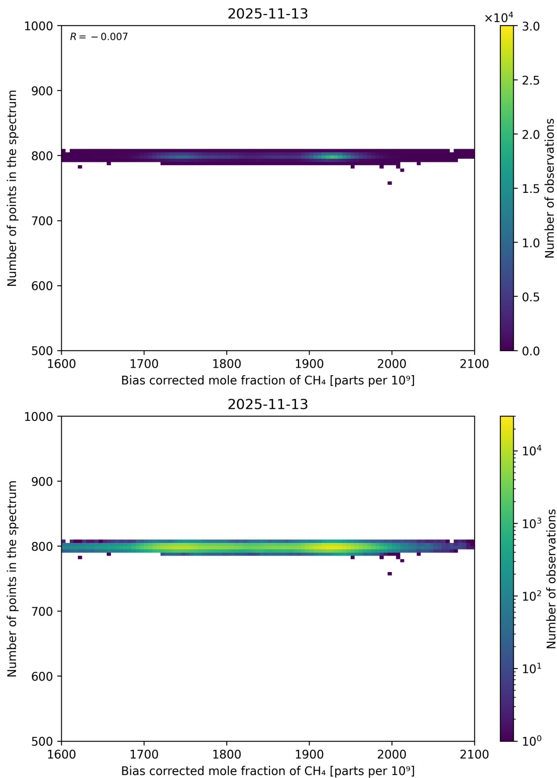
Figure 68: Scatter density plot of “Bias corrected mole fraction of CH 4 ” against “Number of points in the spectrum” for 2025-11-12 to 2025-11-14.
