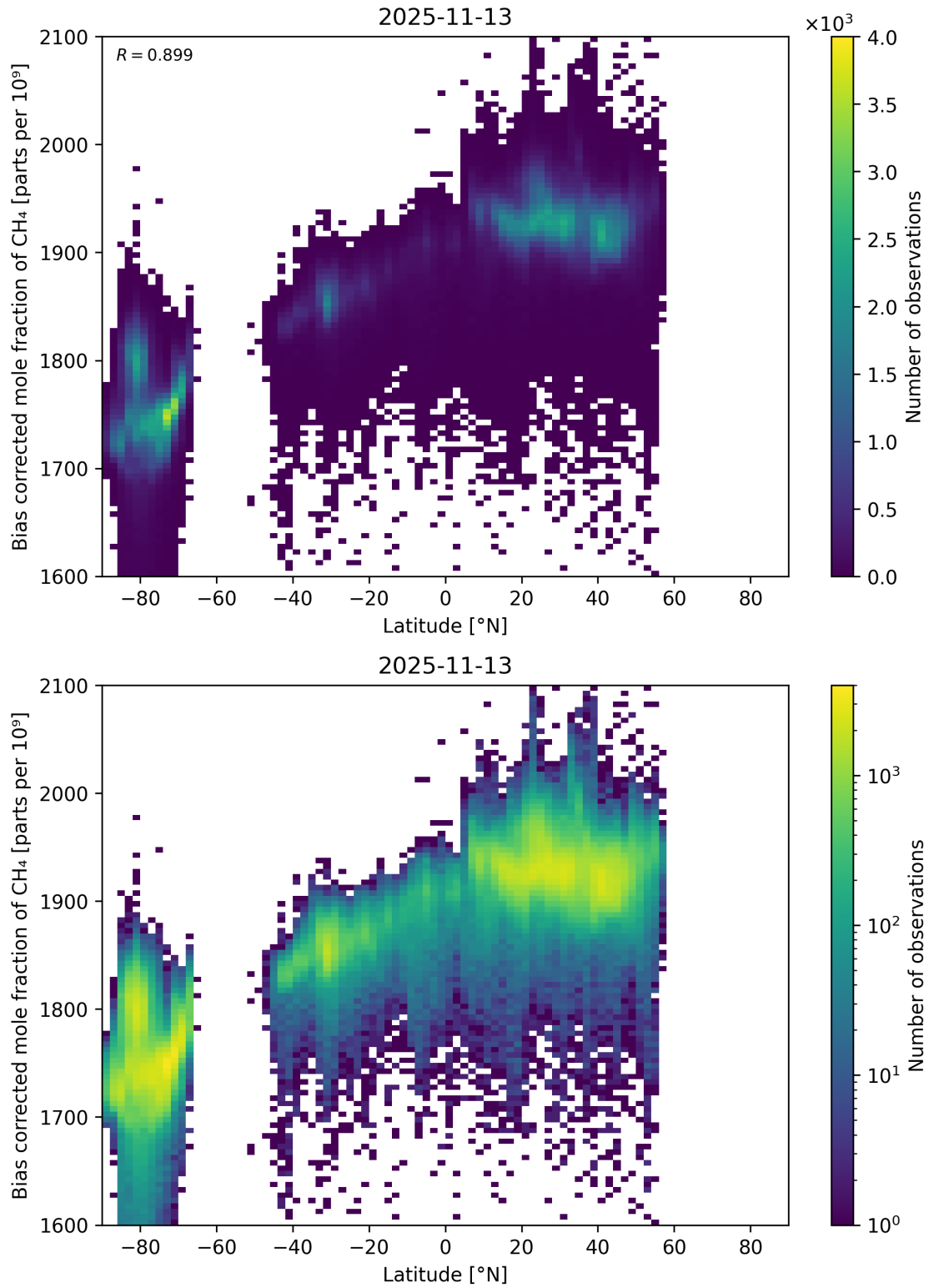
Figure 58: Scatter density plot of “Latitude” against “Bias corrected mole fraction of \text{CH}_4 ” for 2025-11-12 to 2025-11-14.
