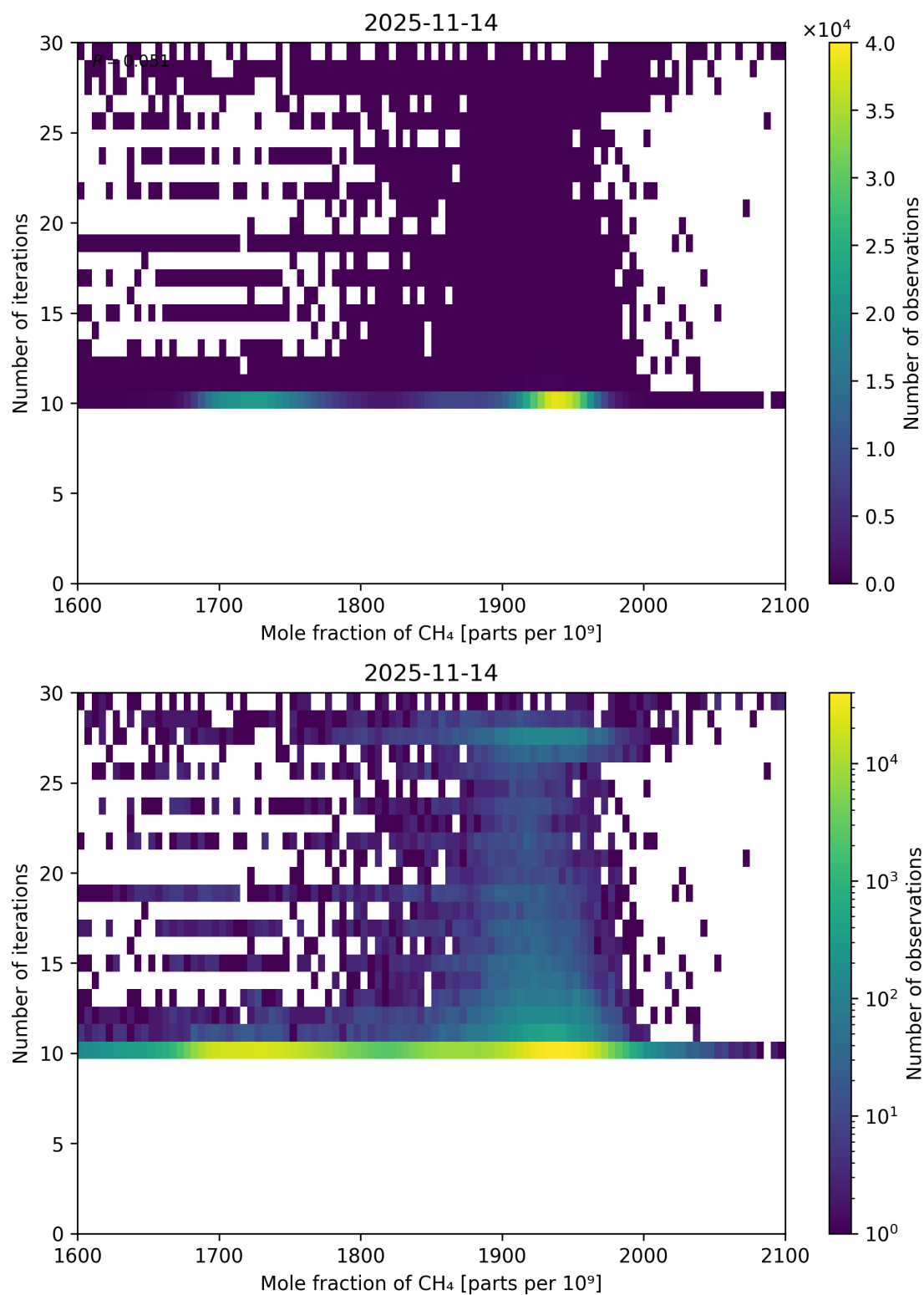
Figure 76: Scatter density plot of “Mole fraction of CH 4 ” against “Number of iterations” for 2025-11-13 to 2025-11-15.
