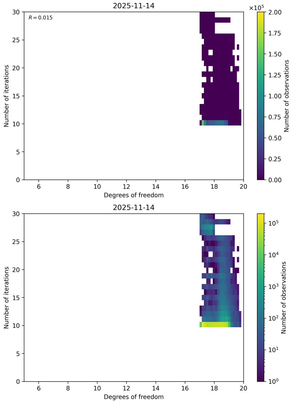
Figure 52: Scatter density plot of “Degrees of freedom” against “Number of iterations” for 2025-11-13 to 2025-11-15.
