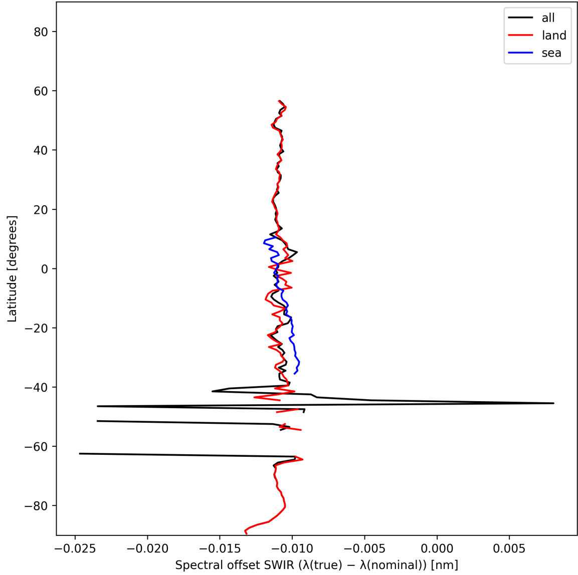
Figure 16: Zonal average of “Spectral offset SWIR ( \lambda_{\text{true}} - \lambda_{\text{nominal}} )” for 2025-11-13 to 2025-11-15.
