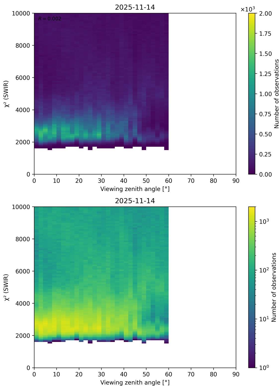
Figure 106: Scatter density plot of “Viewing zenith angle” against “ \chi^2 (SWIR)” for 2025-11-13 to 2025-11-15.
