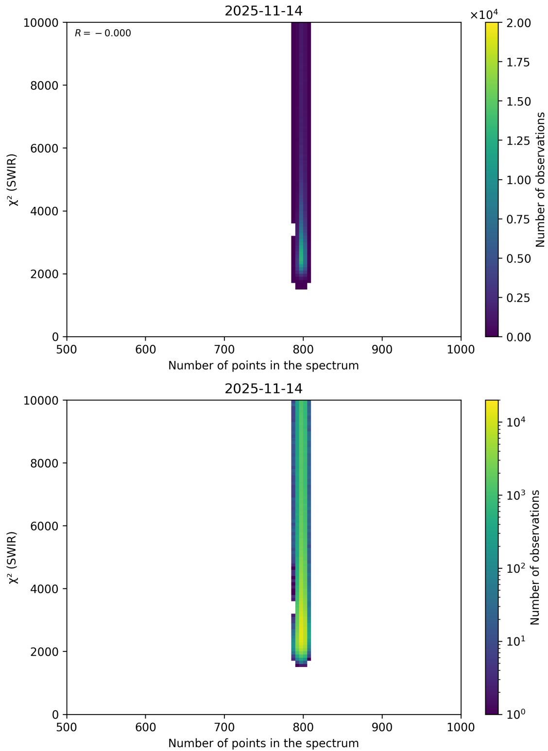
Figure 89: Scatter density plot of “Number of points in the spectrum” against “ \chi^2 (SWIR)” for 2025-11-13 to 2025-11-15.
