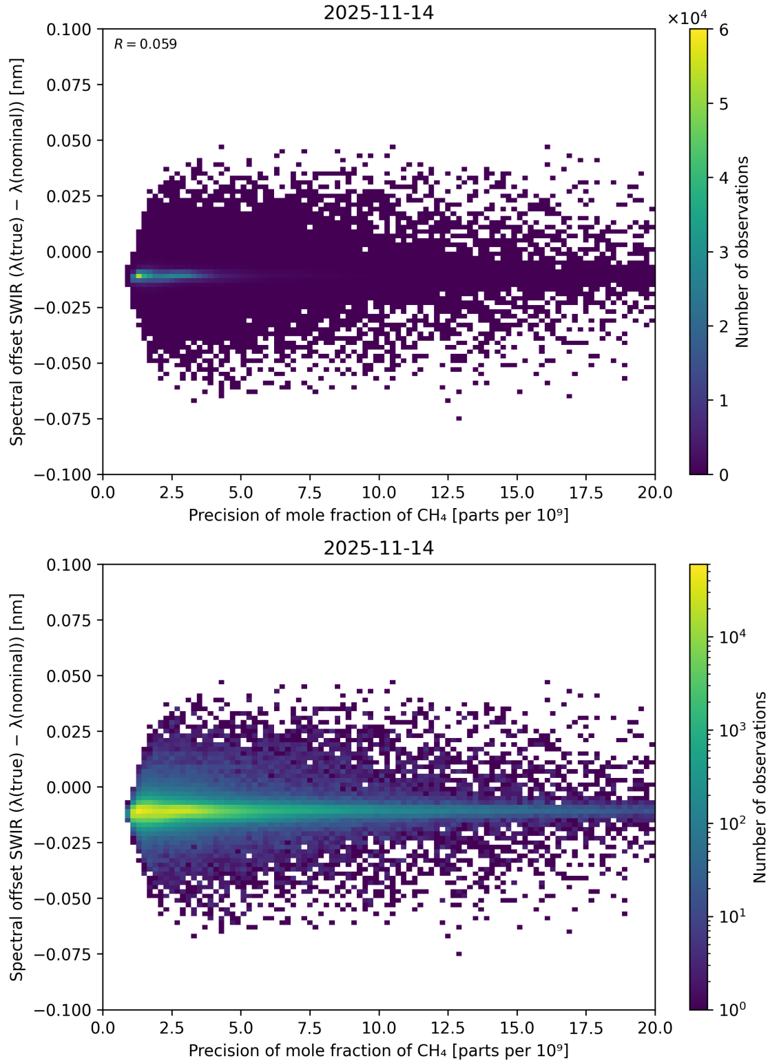
Figure 85: Scatter density plot of “Precision of mole fraction of CH 4 ” against “Spectral offset SWIR ( \lambda_{\text{true}} - \lambda_{\text{nominal}} )” for 2025-11-13 to 2025-11-15.
