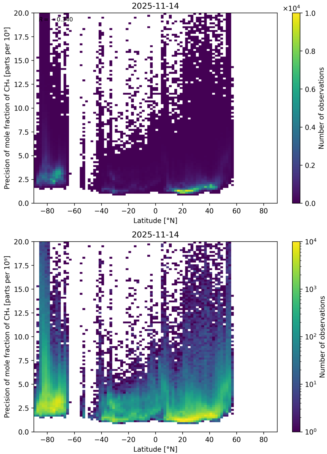
Figure 59: Scatter density plot of “Latitude” against “Precision of mole fraction of \text{CH}_4 ” for 2025-11-13 to 2025-11-15.
