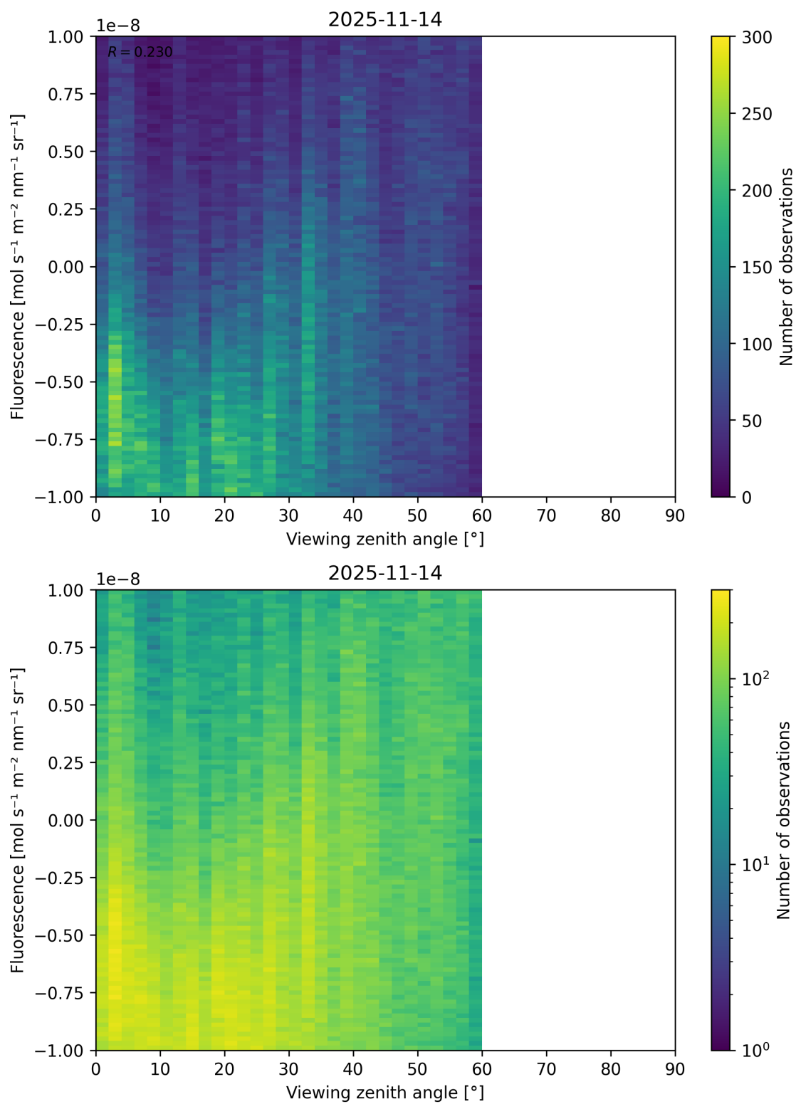
Figure 108: Scatter density plot of “Viewing zenith angle” against “Fluorescence” for 2025-11-13 to 2025-11-15.
