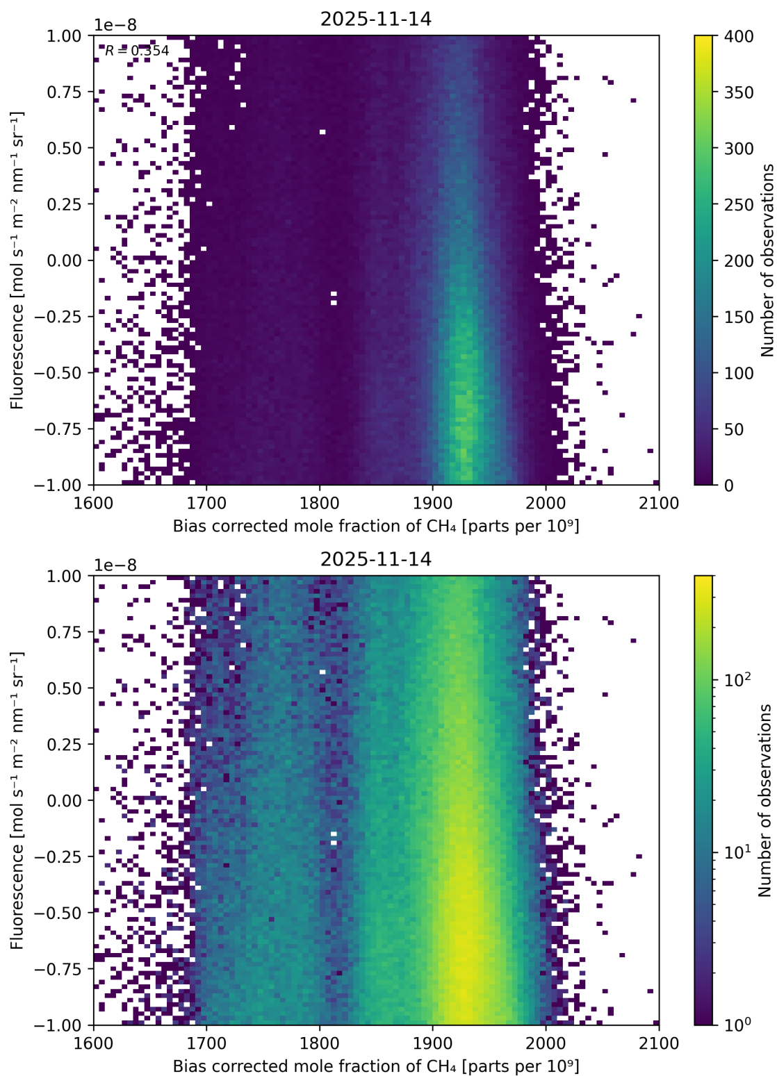
Figure 66: Scatter density plot of “Bias corrected mole fraction of \text{CH}_4 ” against “Fluorescence” for 2025-11-13 to 2025-11-15.
