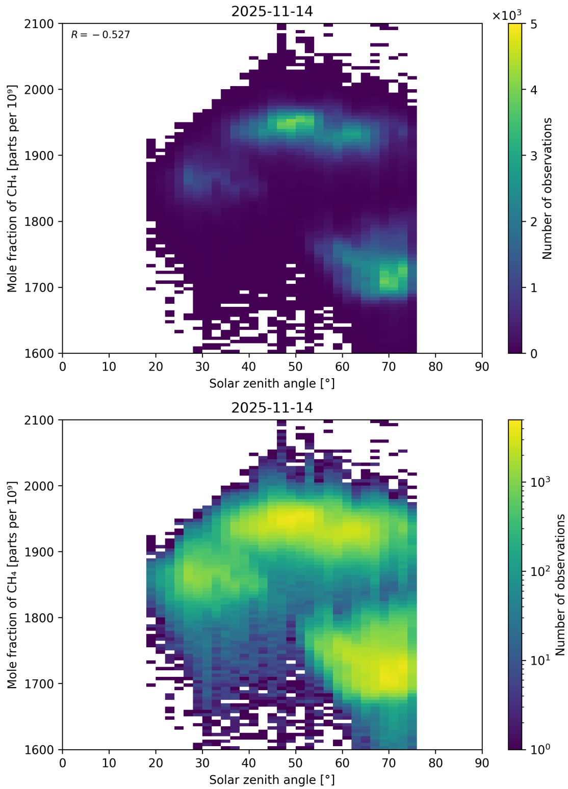
Figure 99: Scatter density plot of “Solar zenith angle” against “Mole fraction of CH 4 ” for 2025-11-13 to 2025-11-15.
