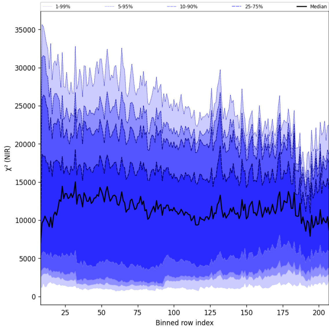
Figure 40: Along track statistics of " \chi^2 (NIR)" for 2025-11-13 to 2025-11-15
