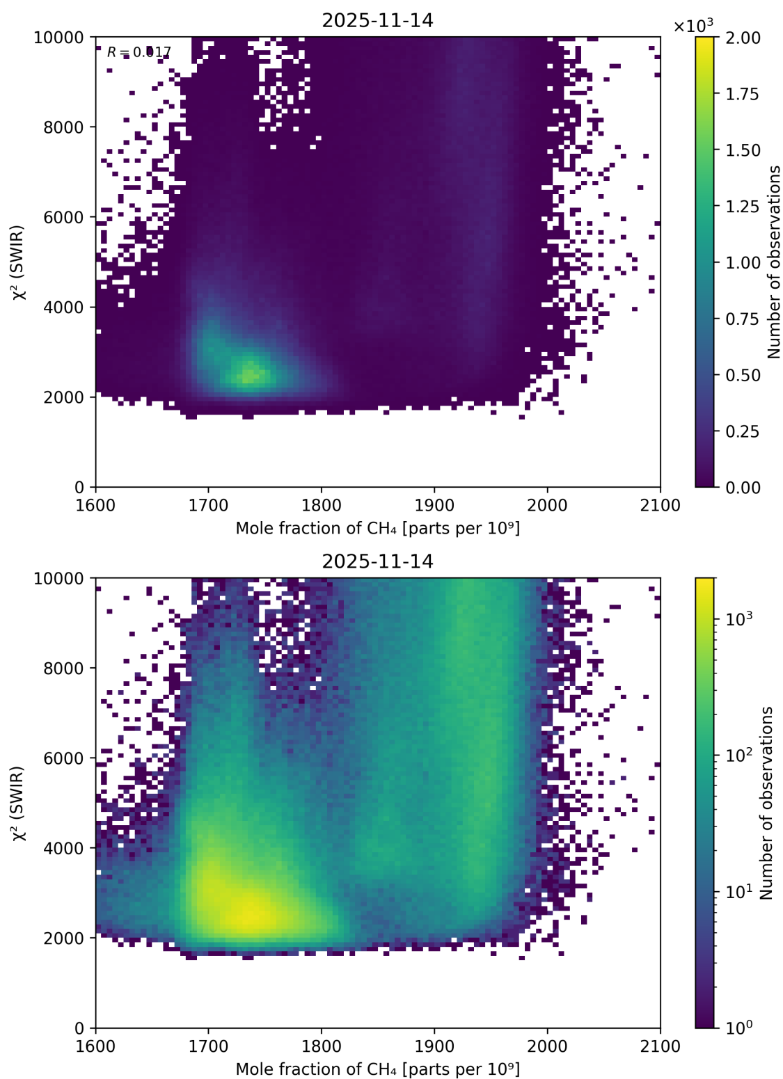
Figure 71: Scatter density plot of “Mole fraction of \text{CH}_4 ” against “ \chi^2 (SWIR)” for 2025-11-13 to 2025-11-15.
