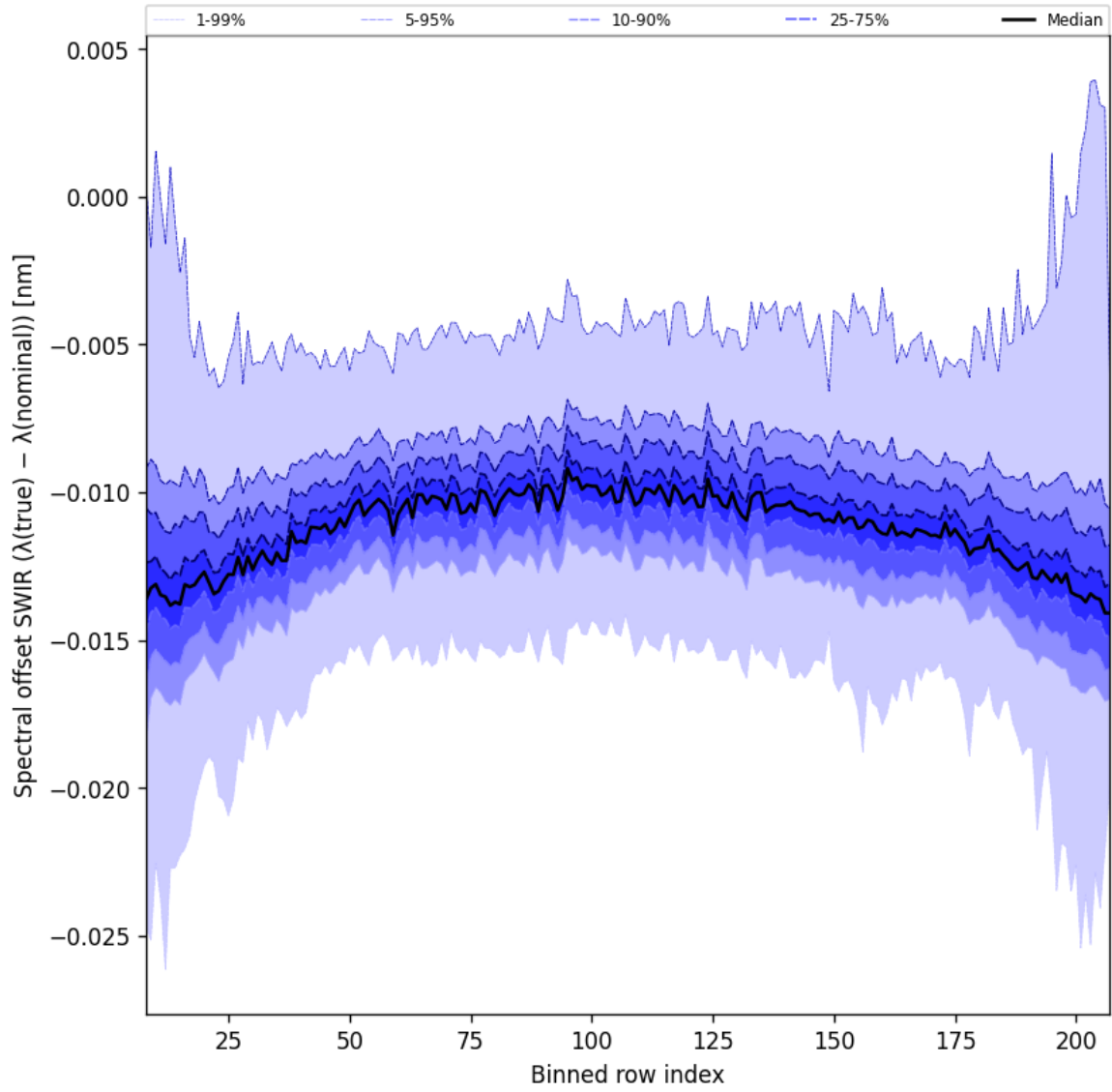
Figure 38: Along track statistics of “Spectral offset SWIR ( \lambda_{\text{true}} - \lambda_{\text{nominal}} )” for 2025-11-13 to 2025-11-15
