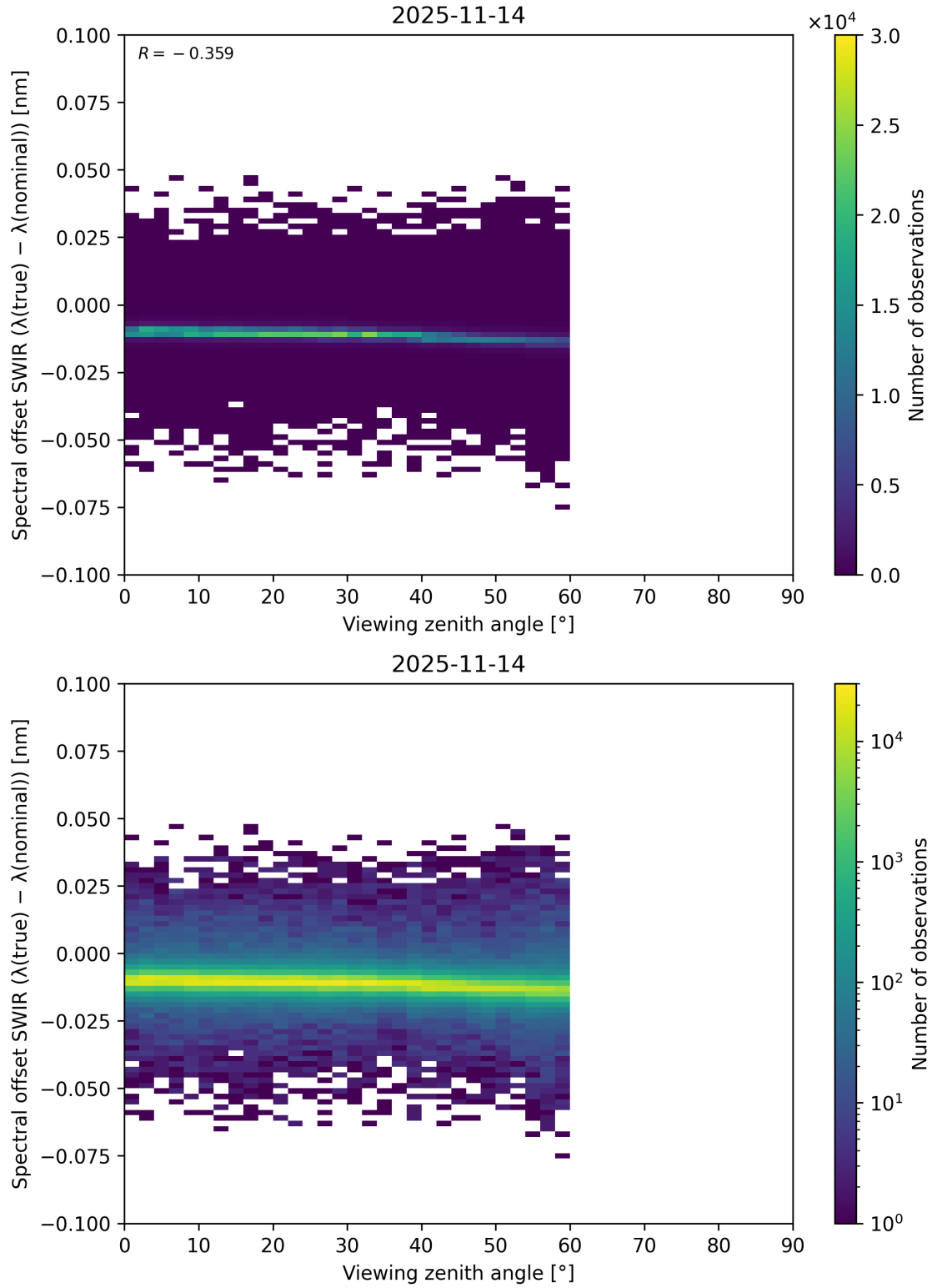
Figure 116: Scatter density plot of “Viewing zenith angle” against “Spectral offset SWIR ( \lambda_{\text{true}} - \lambda_{\text{nominal}} )” for 2025-11-13 to 2025-11-15.
