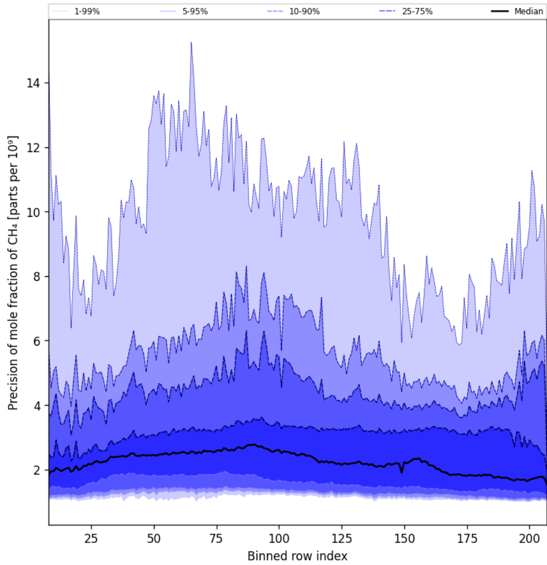
Figure 35: Along track statistics of “Precision of mole fraction of CH 4 ” for 2025-11-13 to 2025-11-15
