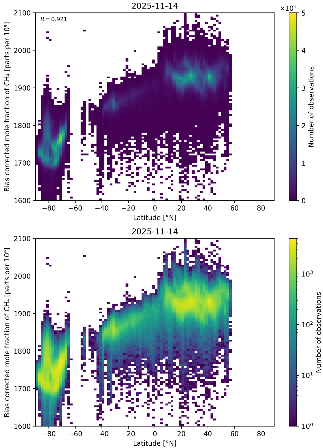
Figure 58: Scatter density plot of “Latitude” against “Bias corrected mole fraction of CH 4 ” for 2025-11-13 to 2025-11-15.
