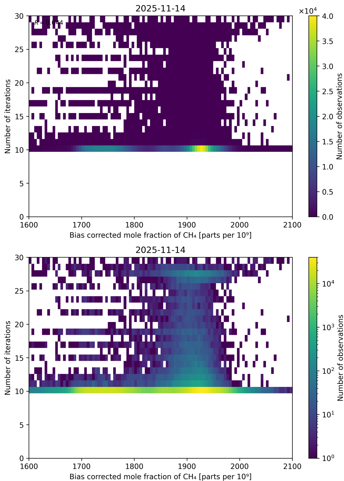
Figure 67: Scatter density plot of “Bias corrected mole fraction of \text{CH}_4 ” against “Number of iterations” for 2025-11-13 to 2025-11-15.
