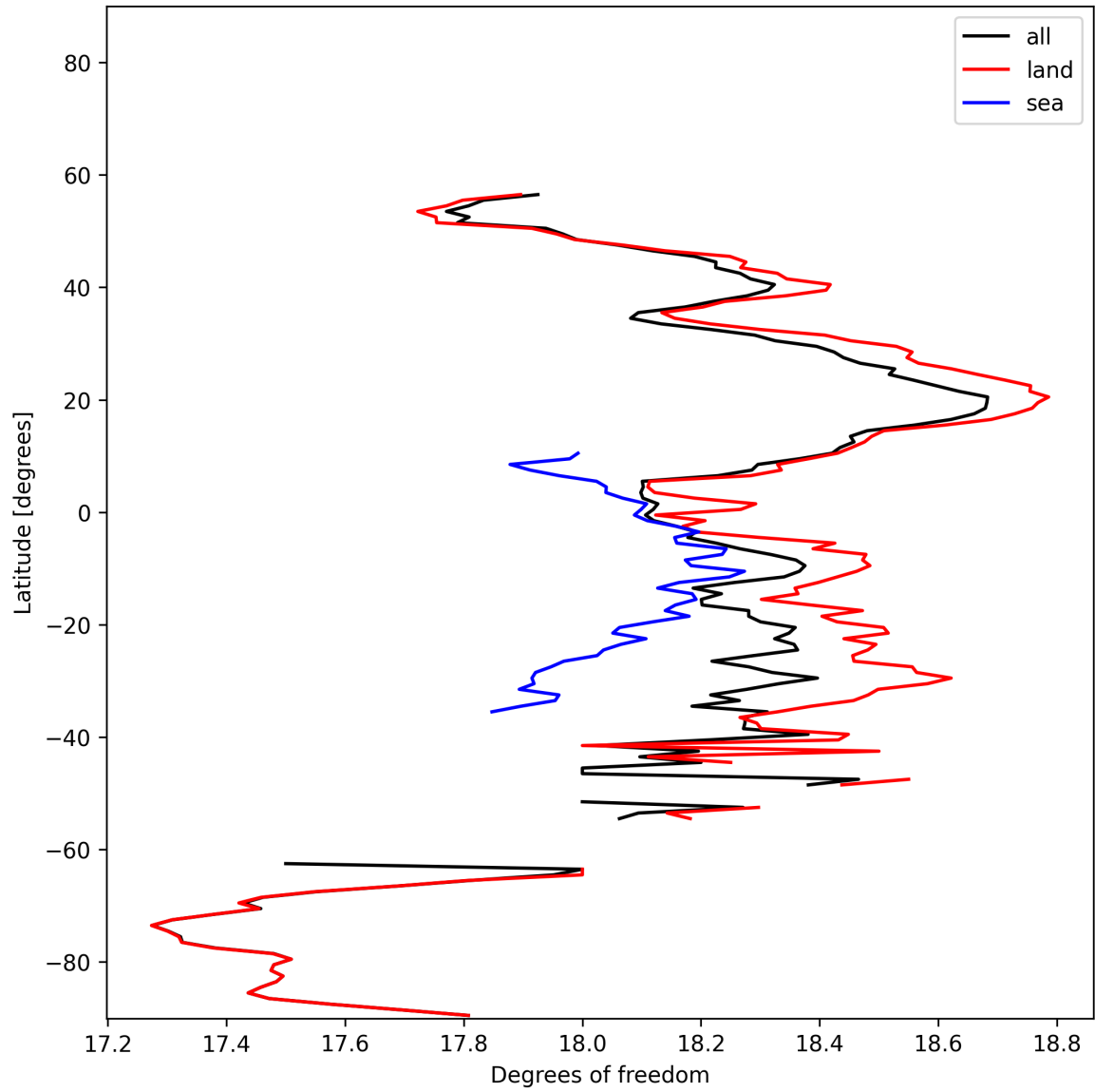
Figure 19: Zonal average of “Degrees of freedom” for 2025-11-13 to 2025-11-15.
