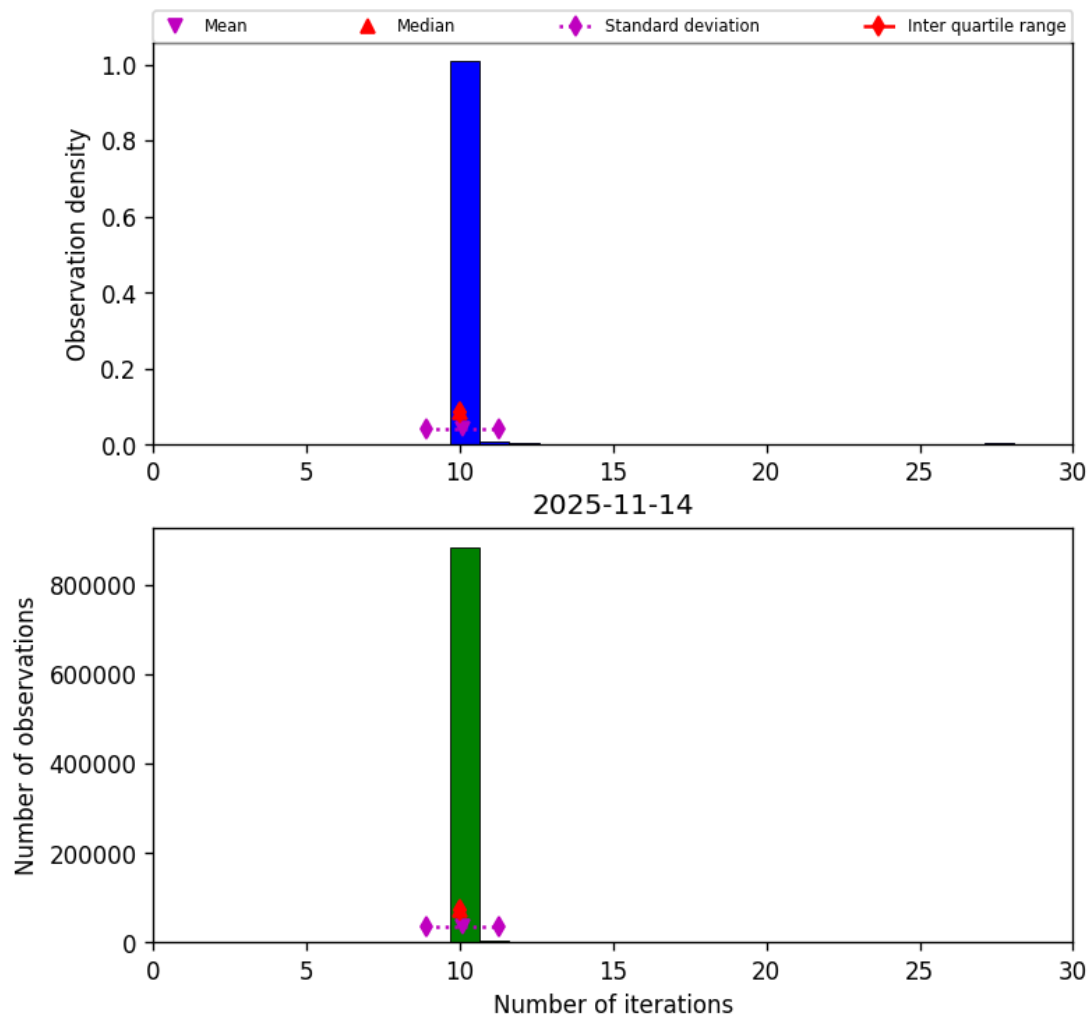
Figure 31: Histogram of “Number of iterations” for 2025-11-13 to 2025-11-15
