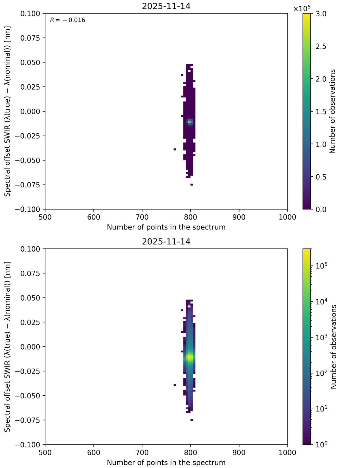
Figure 93: Scatter density plot of “Number of points in the spectrum” against “Spectral offset SWIR ( \lambda_{\text{true}} - \lambda_{\text{nominal}} )” for 2025-11-13 to 2025-11-15.
