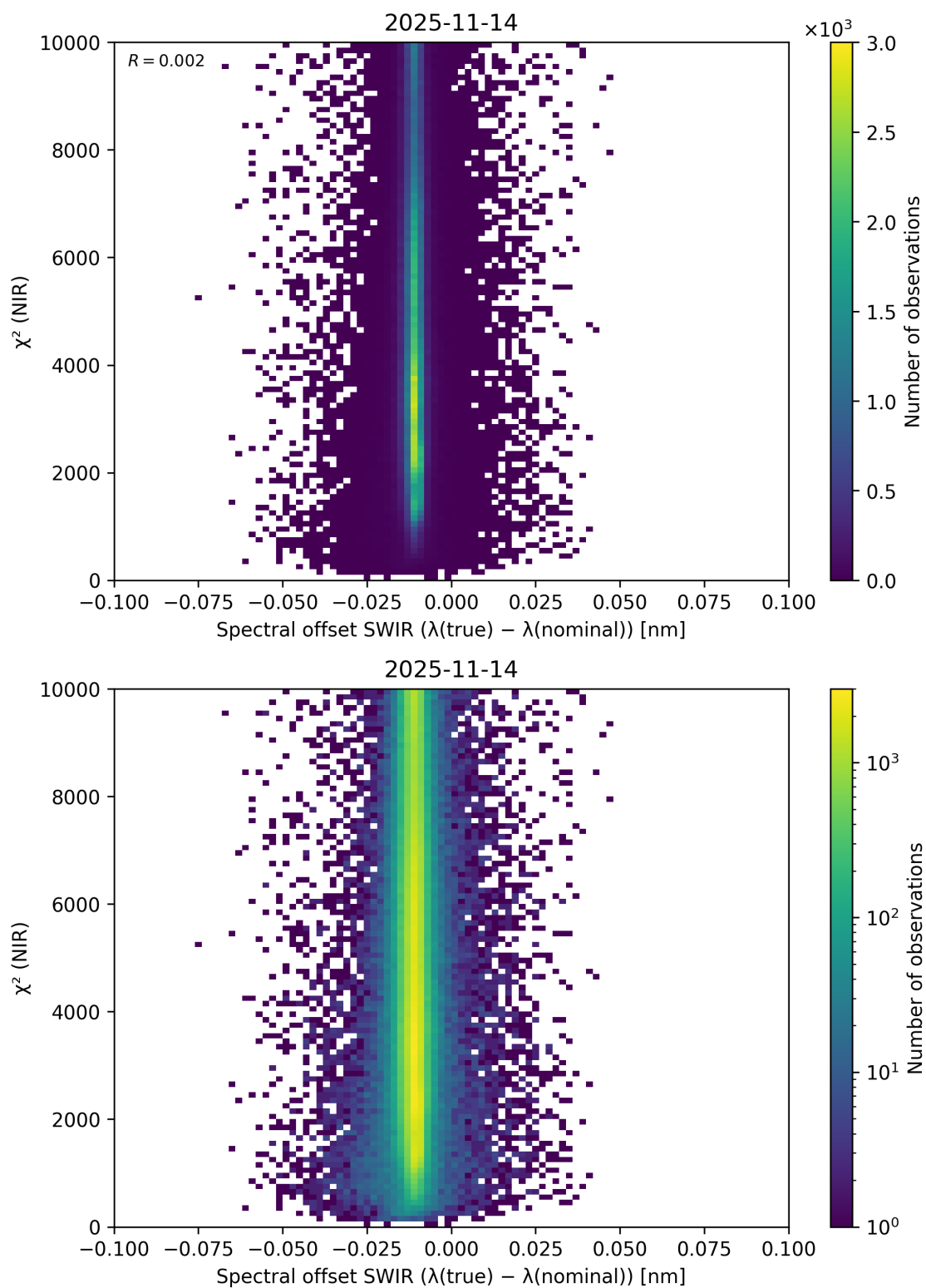
Figure 117: Scatter density plot of “Spectral offset SWIR ( \lambda_{\text{true}} - \lambda_{\text{nominal}} )” against “ \chi^2 (NIR)” for 2025-11-13 to 2025-11-15.
