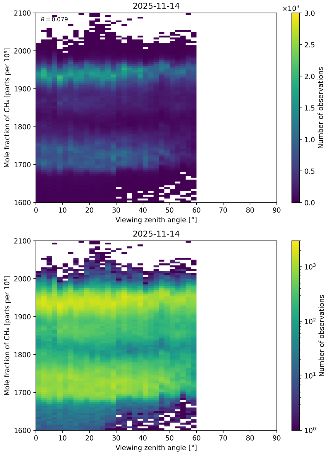
Figure 110: Scatter density plot of “Viewing zenith angle” against “Mole fraction of CH 4 ” for 2025-11-13 to 2025-11-15.
