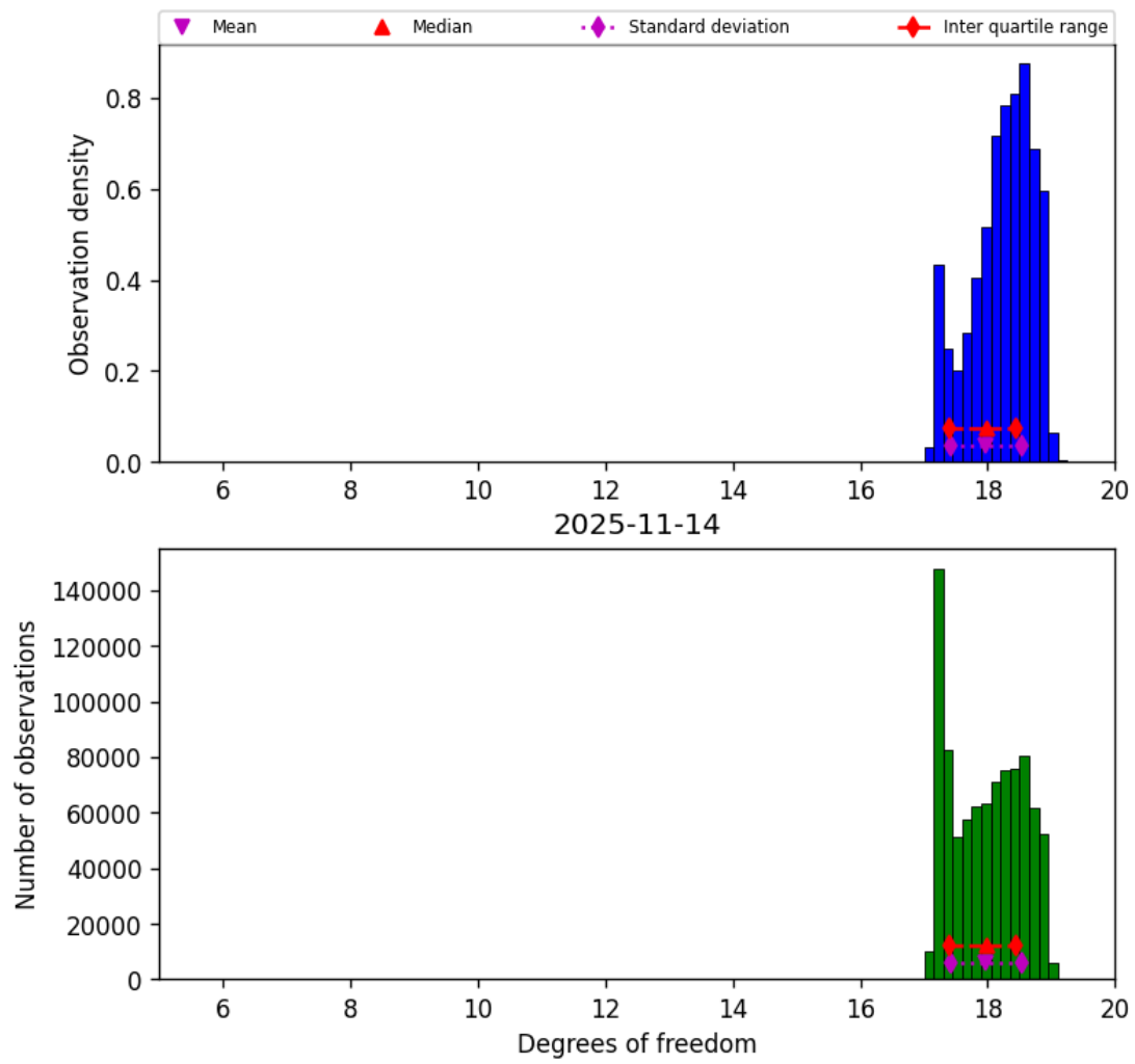
Figure 30: Histogram of “Degrees of freedom” for 2025-11-13 to 2025-11-15
