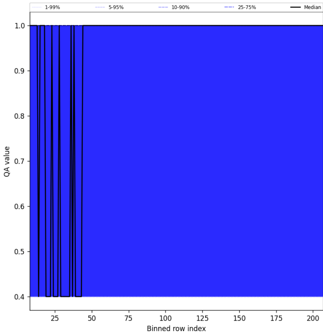
Figure 33: Along track statistics of “QA value” for 2025-11-13 to 2025-11-15
