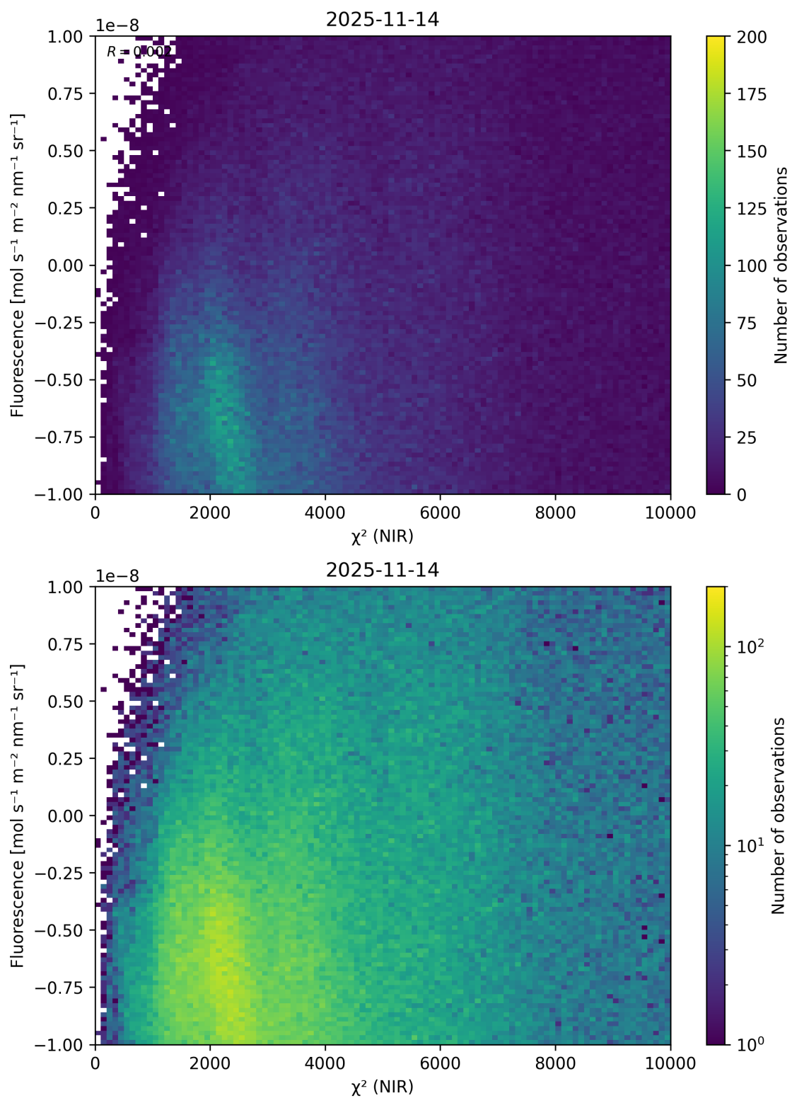
Figure 45: Scatter density plot of “ \chi^2 (NIR)” against “Fluorescence” for 2025-11-13 to 2025-11-15.
