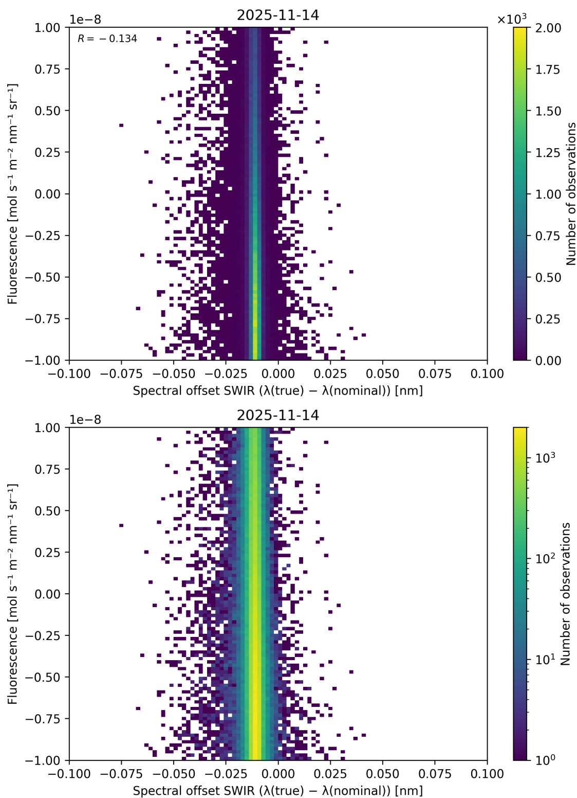
Figure 120: Scatter density plot of “Spectral offset SWIR ( \lambda_{\text{true}} - \lambda_{\text{nominal}} )” against “Fluorescence” for 2025-11-13 to 2025-11-15.
