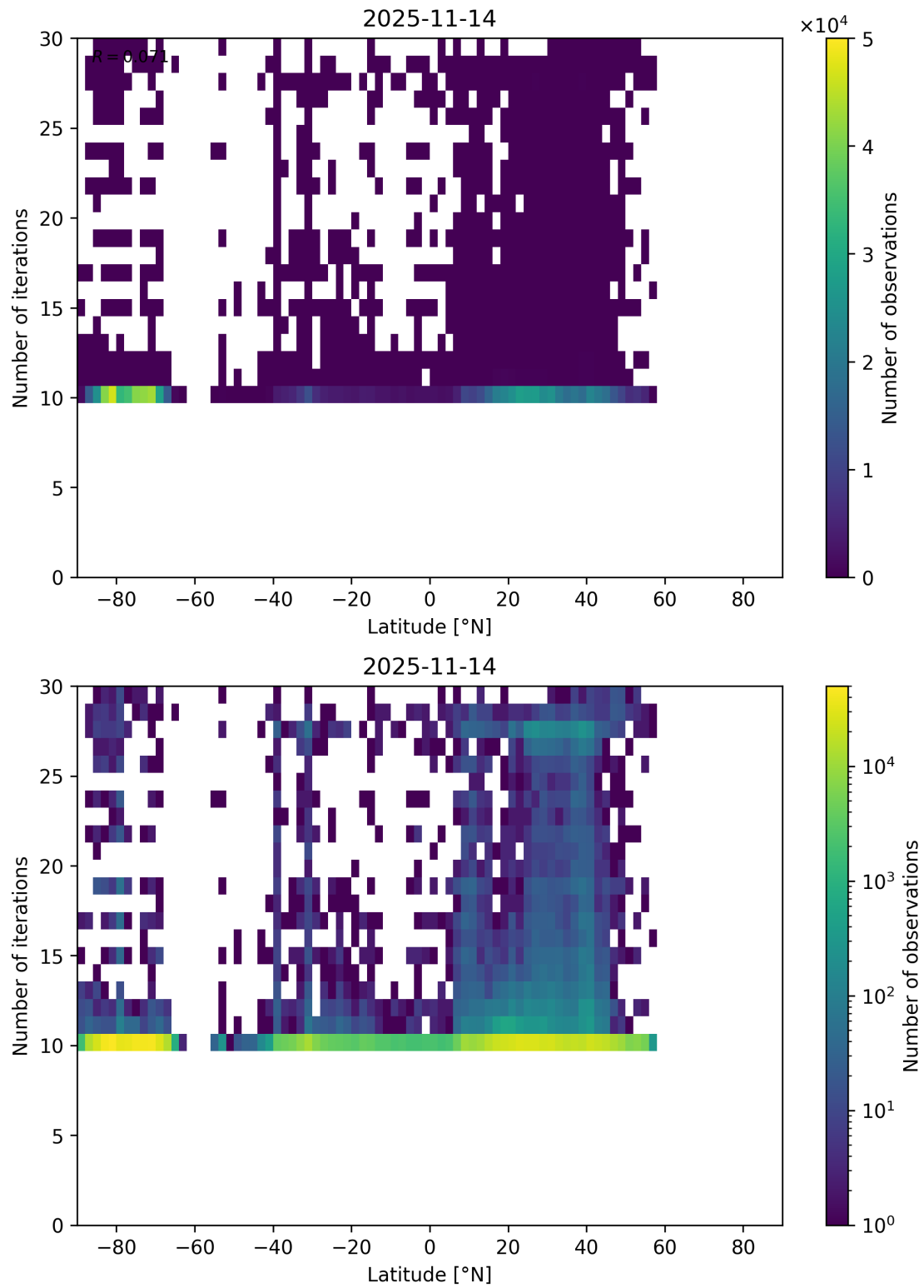
Figure 60: Scatter density plot of “Latitude” against “Number of iterations” for 2025-11-13 to 2025-11-15.
