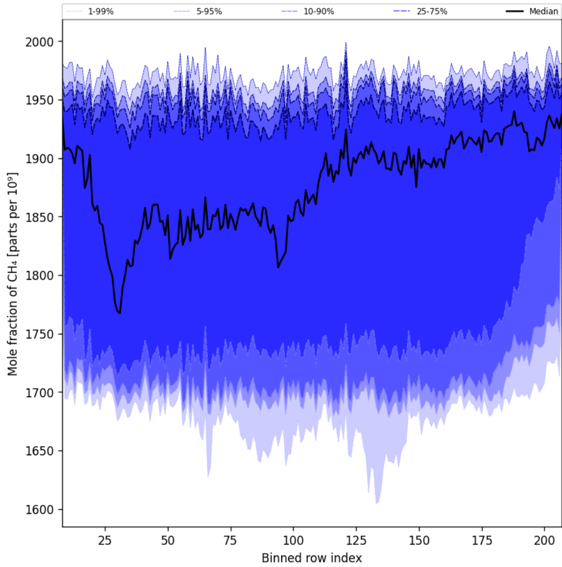
Figure 34: Along track statistics of “Mole fraction of CH 4 ” for 2025-11-13 to 2025-11-15
