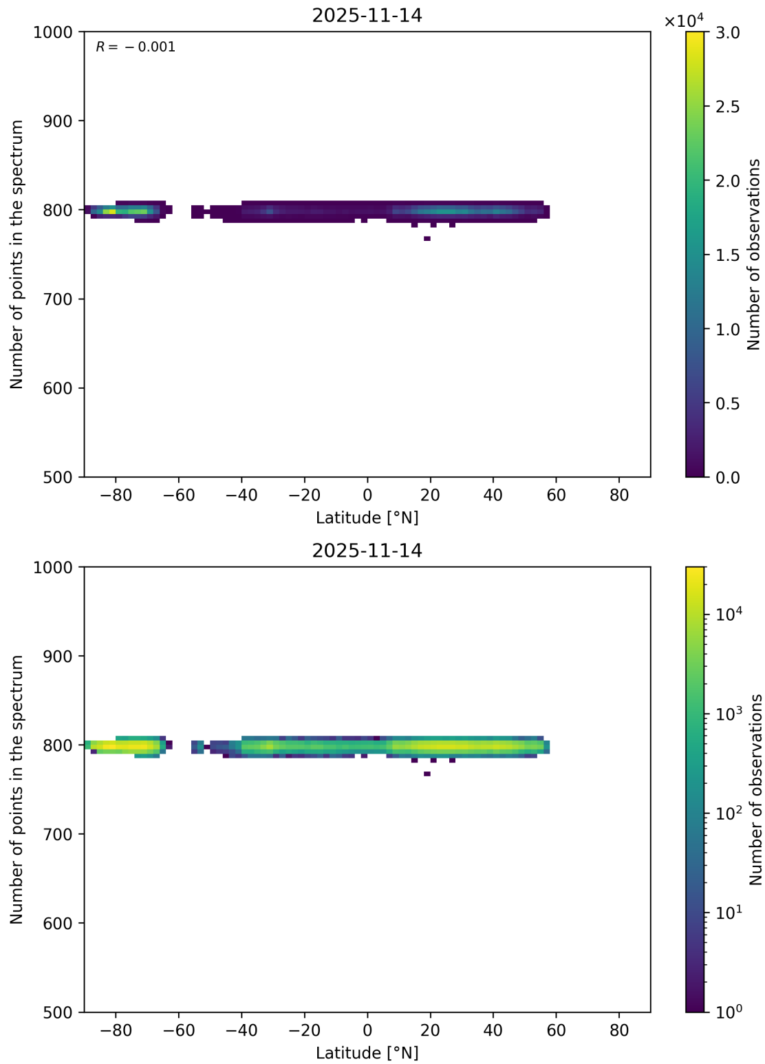
Figure 61: Scatter density plot of “Latitude” against “Number of points in the spectrum” for 2025-11-13 to 2025-11-15.
