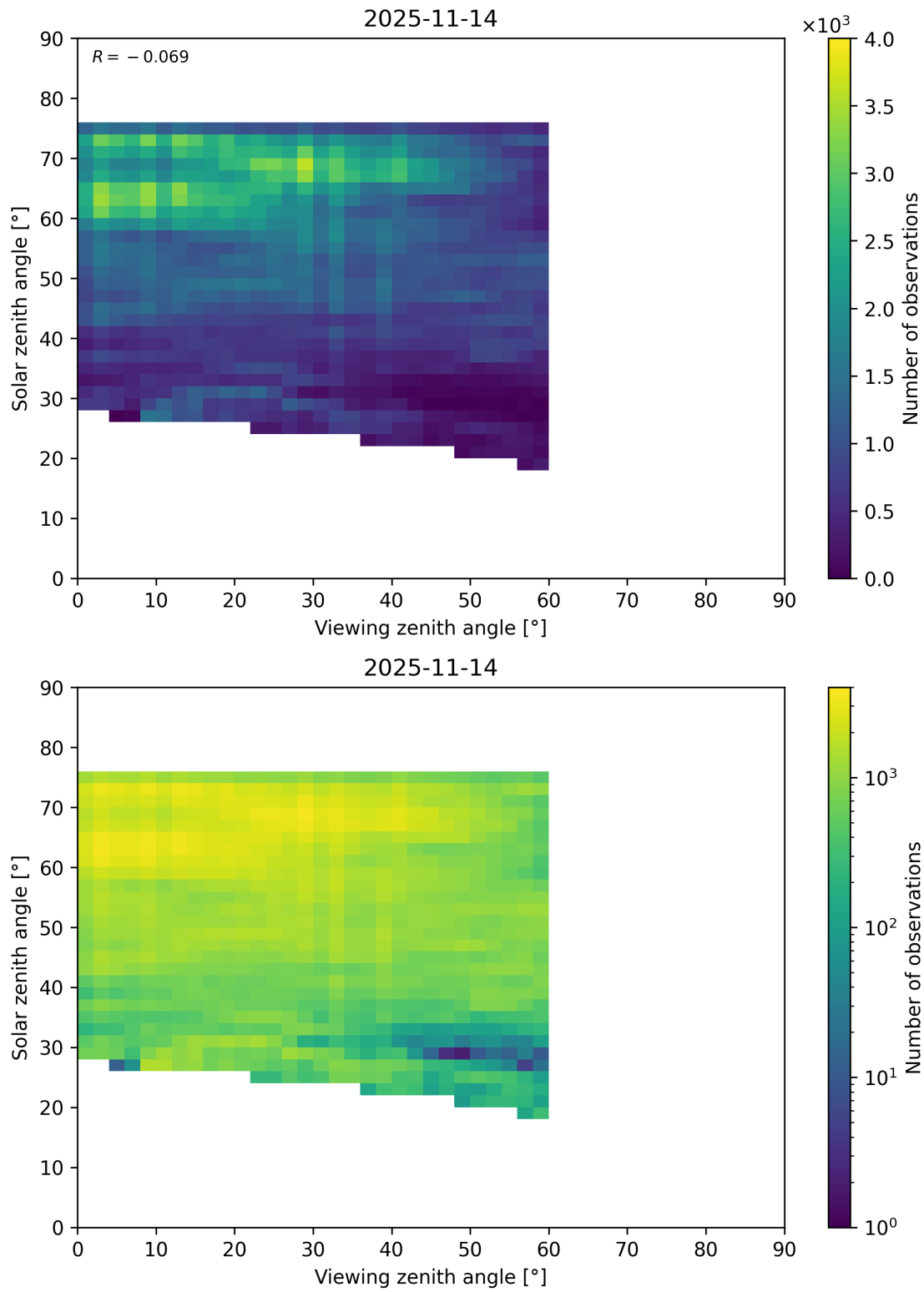
Figure 115: Scatter density plot of “Viewing zenith angle” against “Solar zenith angle” for 2025-11-13 to 2025-11-15.
