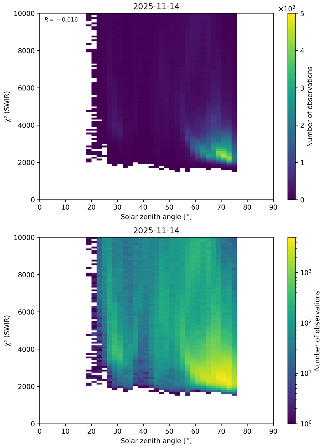
Figure 95: Scatter density plot of “Solar zenith angle” against “ \chi^2 (SWIR)” for 2025-11-13 to 2025-11-15.
