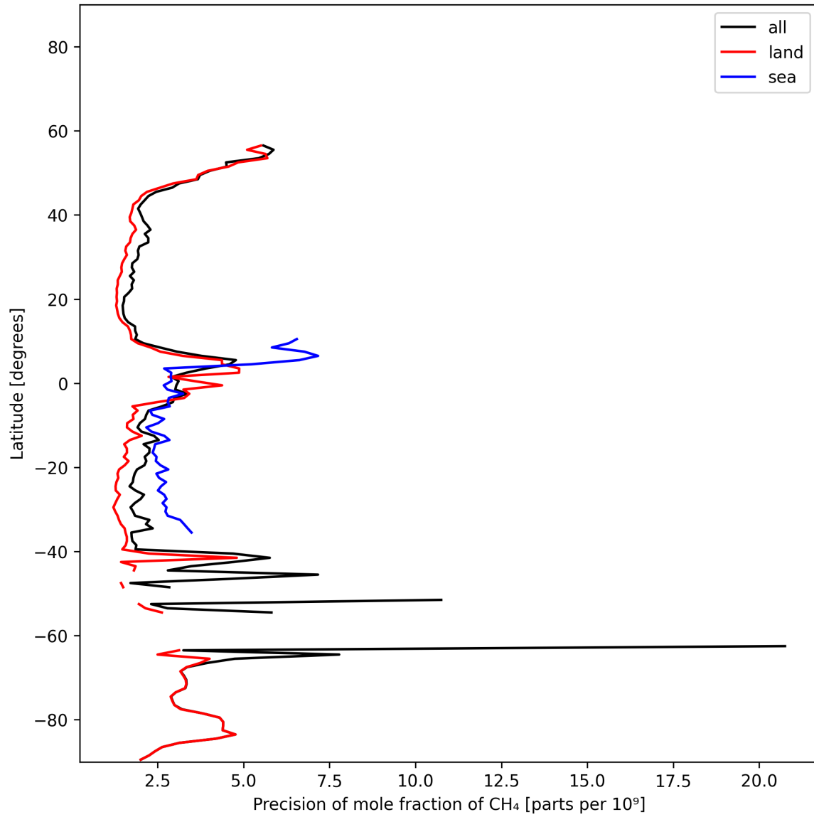
Figure 13: Zonal average of “Precision of mole fraction of CH 4 ” for 2025-11-13 to 2025-11-15.
