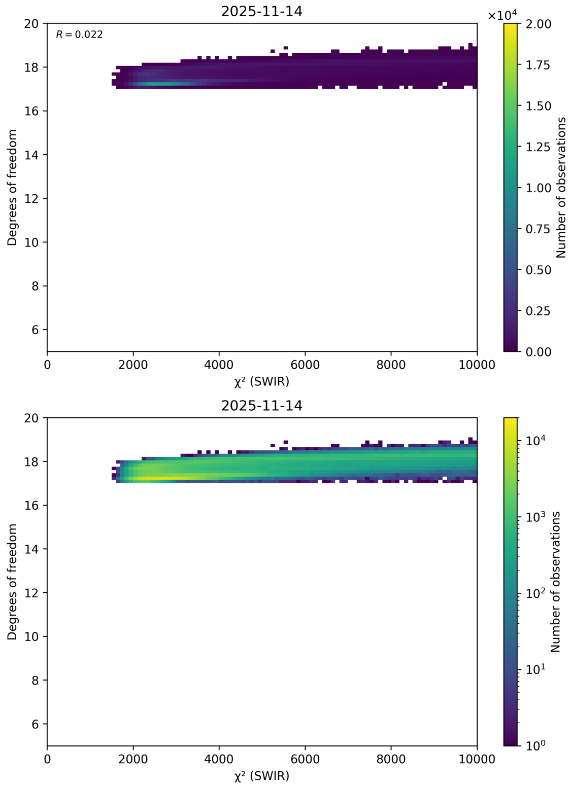
Figure 48: Scatter density plot of “ \chi^2 (SWIR)” against “Degrees of freedom” for 2025-11-13 to 2025-11-15.
