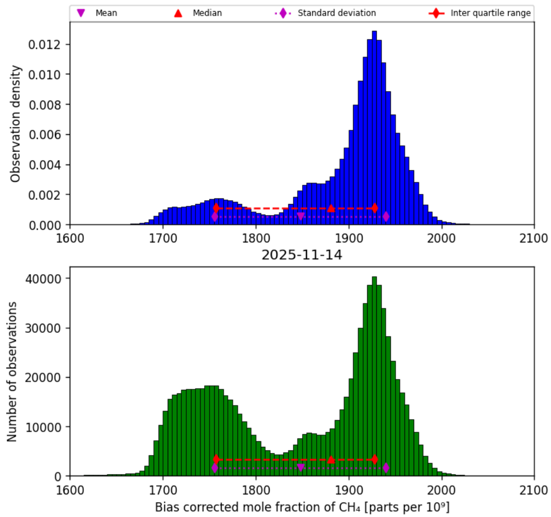
Figure 25: Histogram of “Bias corrected mole fraction of CH 4 ” for 2025-11-13 to 2025-11-15
