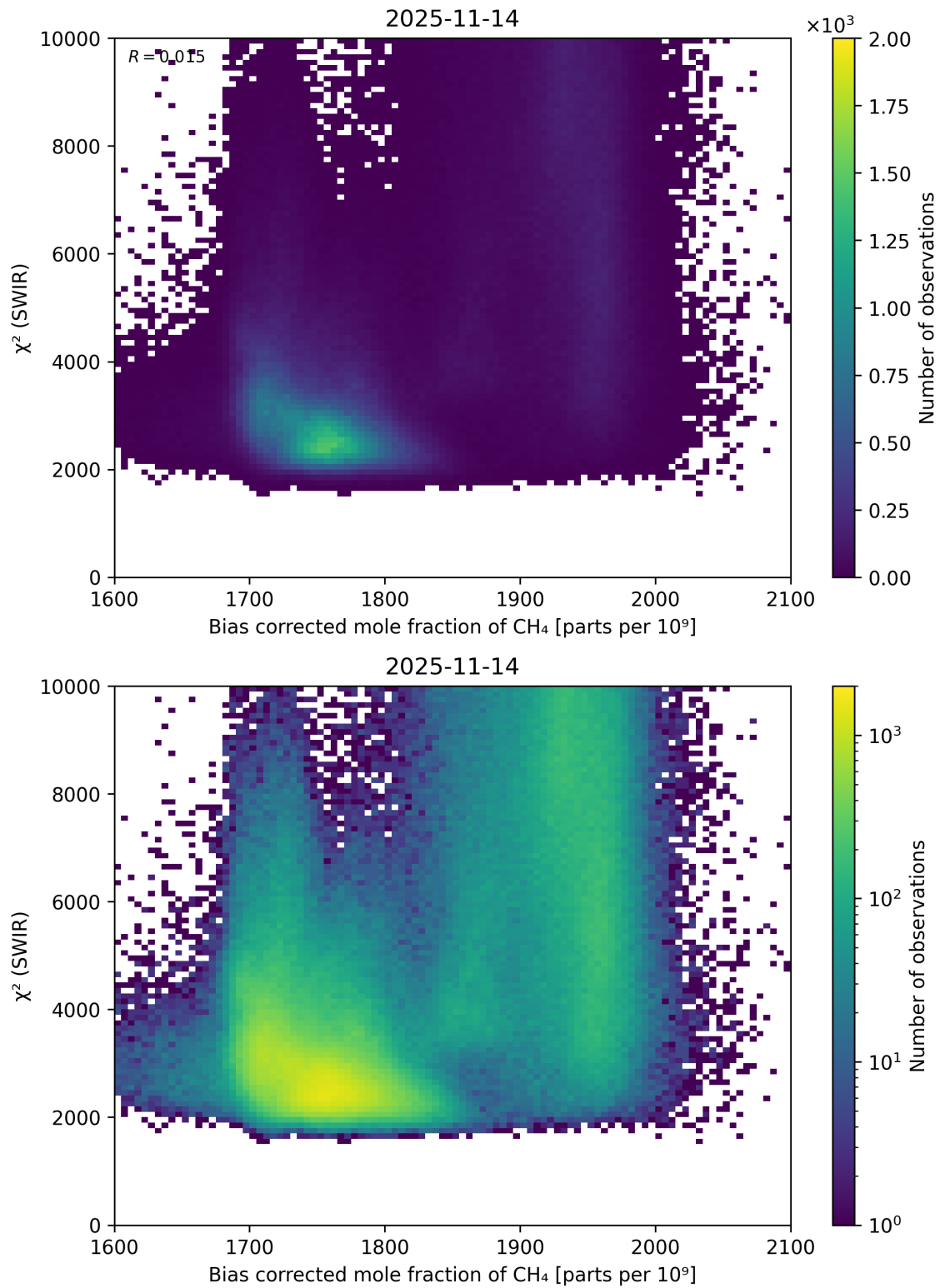
Figure 64: Scatter density plot of “Bias corrected mole fraction of \text{CH}_4 ” against “ \chi^2 (SWIR)” for 2025-11-13 to 2025-11-15.
