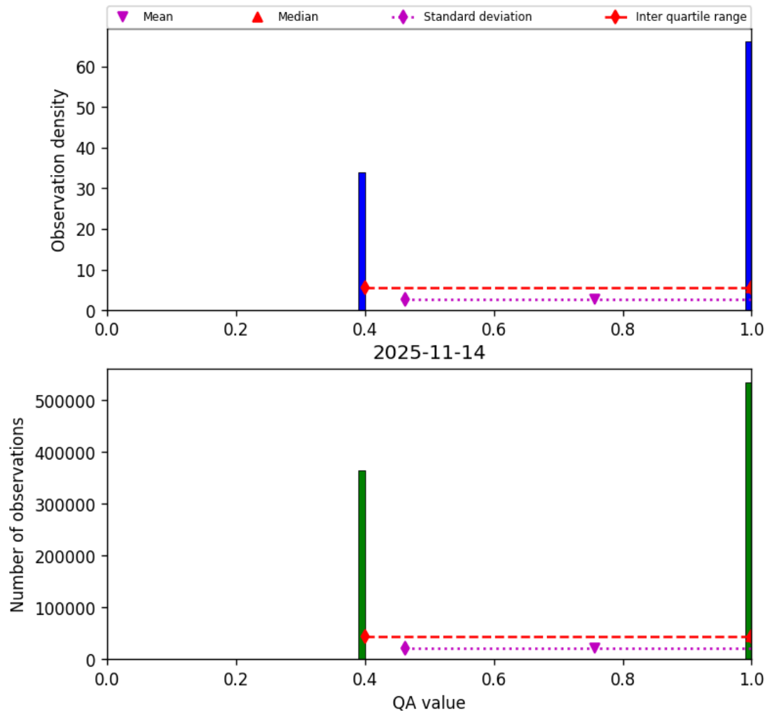
Figure 22: Histogram of “QA value” for 2025-11-13 to 2025-11-15
