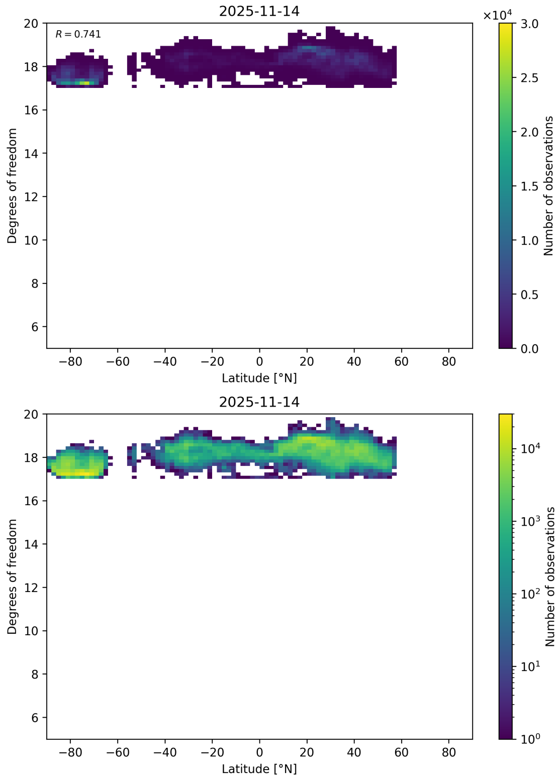
Figure 55: Scatter density plot of “Latitude” against “Degrees of freedom” for 2025-11-13 to 2025-11-15.
