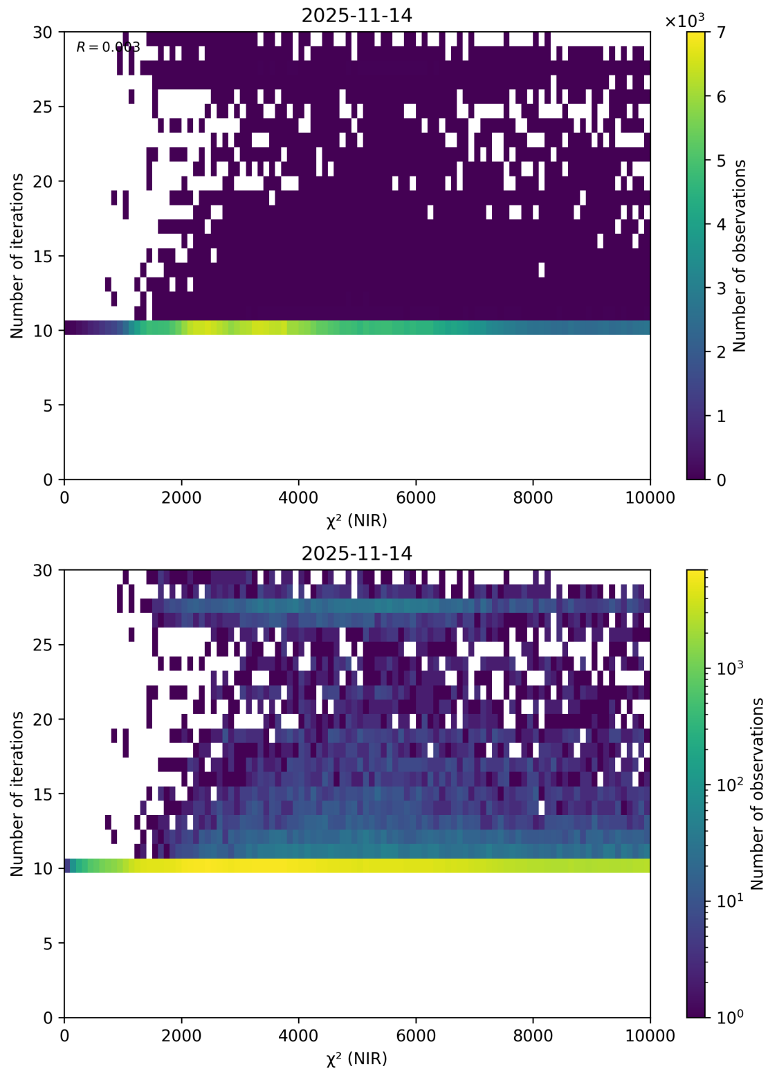
Figure 46: Scatter density plot of “ \chi^2 (NIR)” against “Number of iterations” for 2025-11-13 to 2025-11-15.
