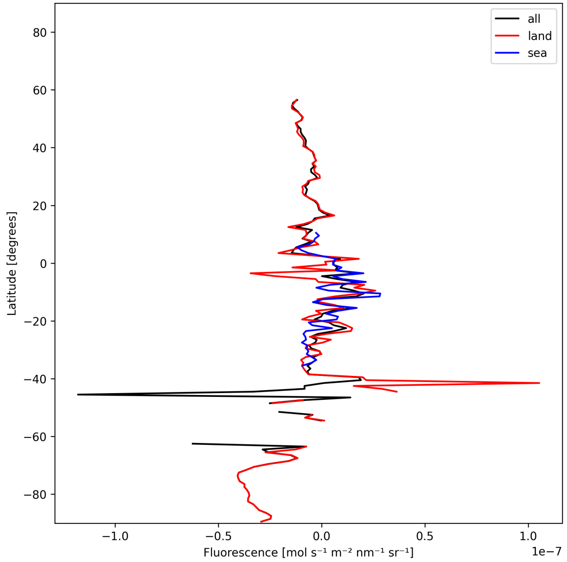
Figure 21: Zonal average of “Fluorescence” for 2025-11-13 to 2025-11-15.
