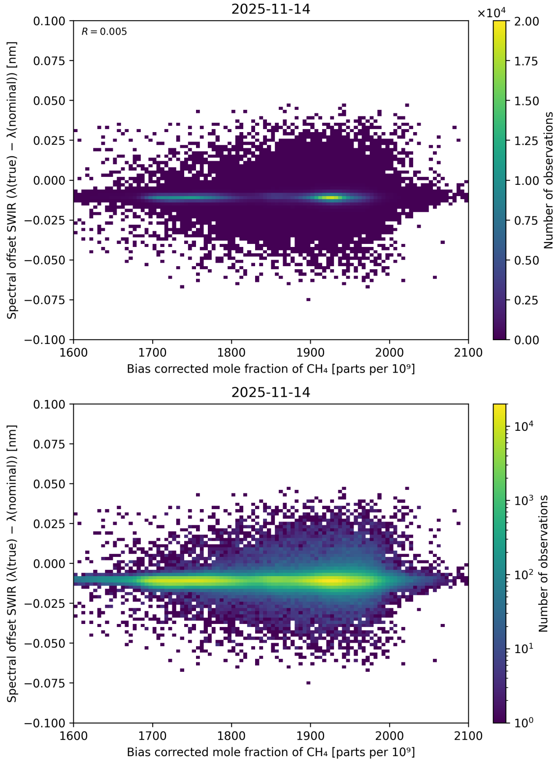
Figure 69: Scatter density plot of “Bias corrected mole fraction of \text{CH}_4 ” against “Spectral offset SWIR ( \lambda_{\text{true}} - \lambda_{\text{nominal}} )” for 2025-11-13 to 2025-11-15.
