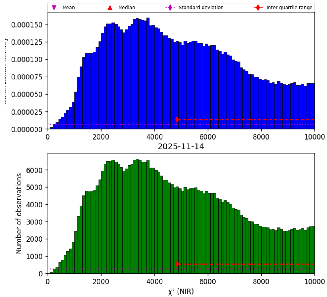
Figure 29: Histogram of “ \chi^2 (NIR)” for 2025-11-13 to 2025-11-15
