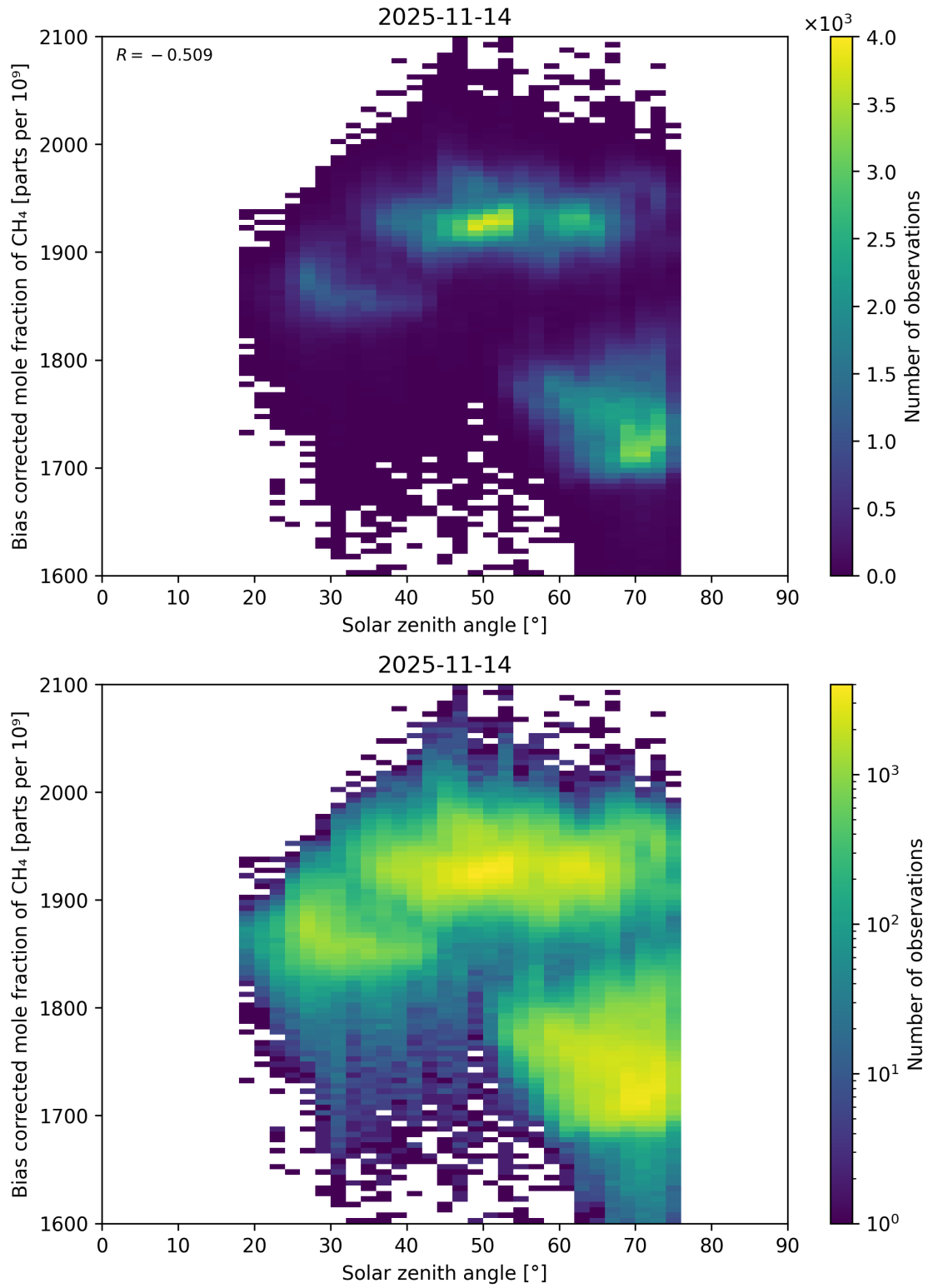
Figure 100: Scatter density plot of “Solar zenith angle” against “Bias corrected mole fraction of CH 4 ” for 2025-11-13 to 2025-11-15.
