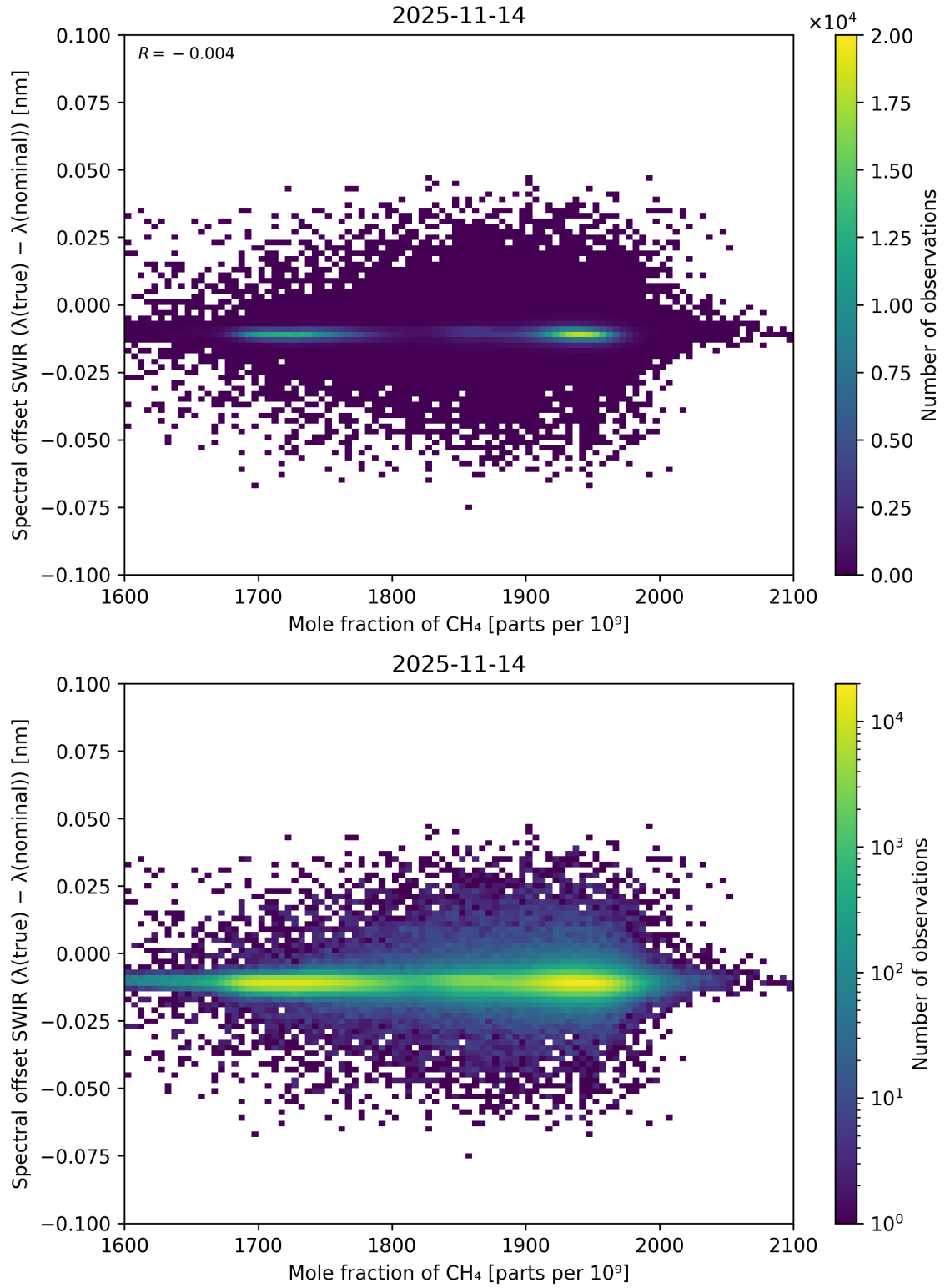
Figure 86: Scatter density plot of “Mole fraction of CH 4 ” against “Spectral offset SWIR ( \lambda_{\text{true}} - \lambda_{\text{nominal}} )” for 2025-11-13 to 2025-11-15.
