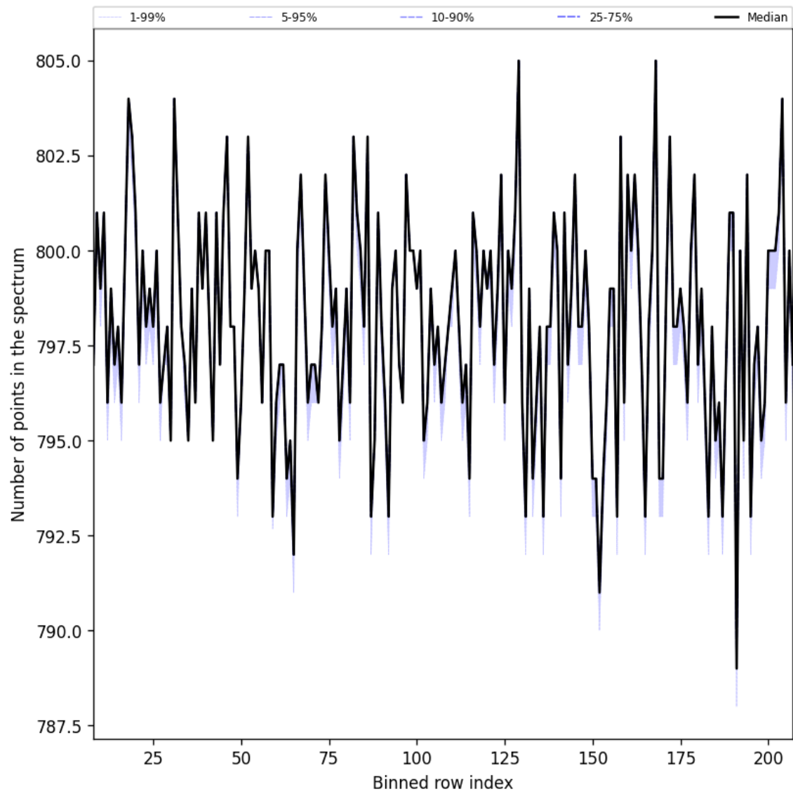
Figure 37: Along track statistics of “Number of points in the spectrum” for 2025-11-13 to 2025-11-15
