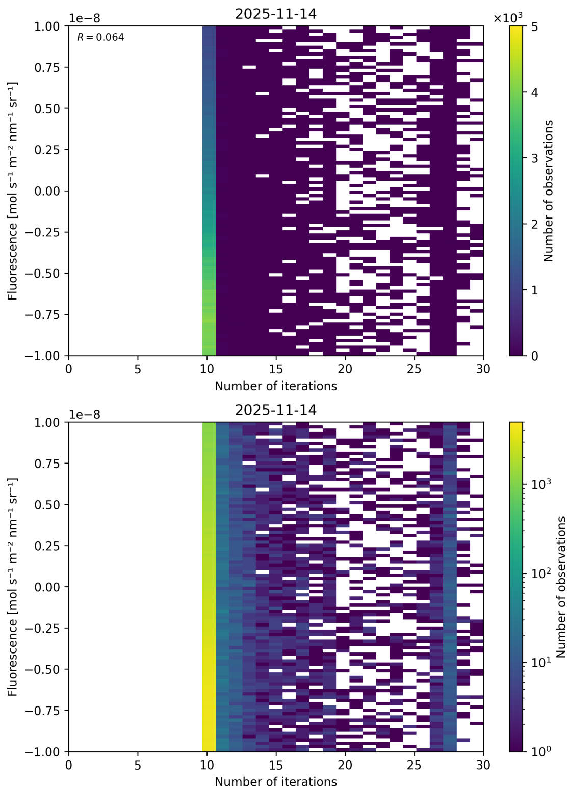
Figure 87: Scatter density plot of “Number of iterations” against “Fluorescence” for 2025-11-13 to 2025-11-15.
