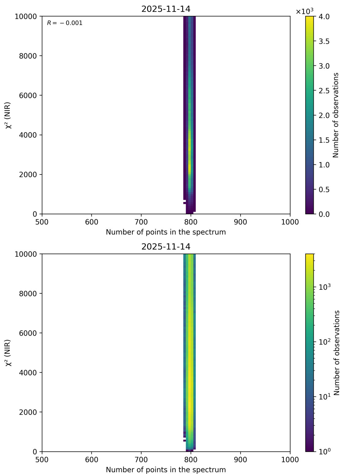
Figure 88: Scatter density plot of “Number of points in the spectrum” against “ \chi^2 (NIR)” for 2025-11-13 to 2025-11-15.
