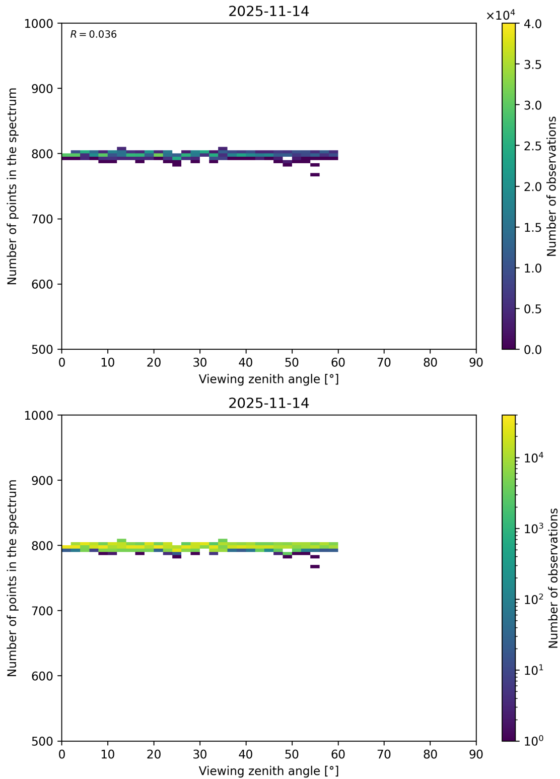
Figure 114: Scatter density plot of “Viewing zenith angle” against “Number of points in the spectrum” for 2025-11-13 to 2025-11-15.
