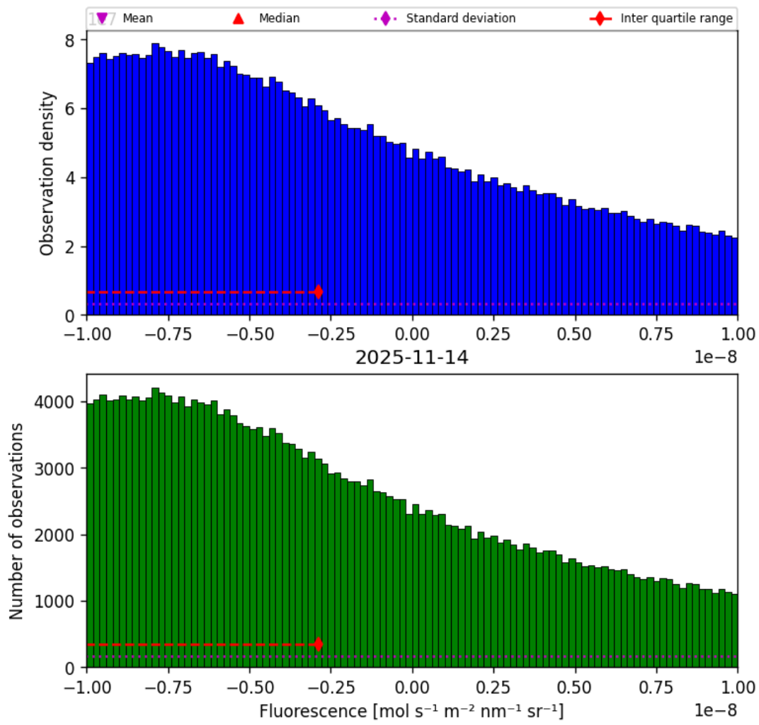
Figure 32: Histogram of “Fluorescence” for 2025-11-13 to 2025-11-15
