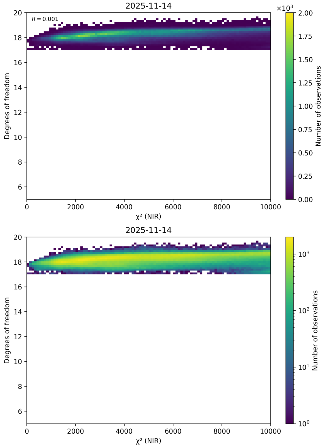
Figure 44: Scatter density plot of “ \chi^2 (NIR)” against “Degrees of freedom” for 2025-11-13 to 2025-11-15.
