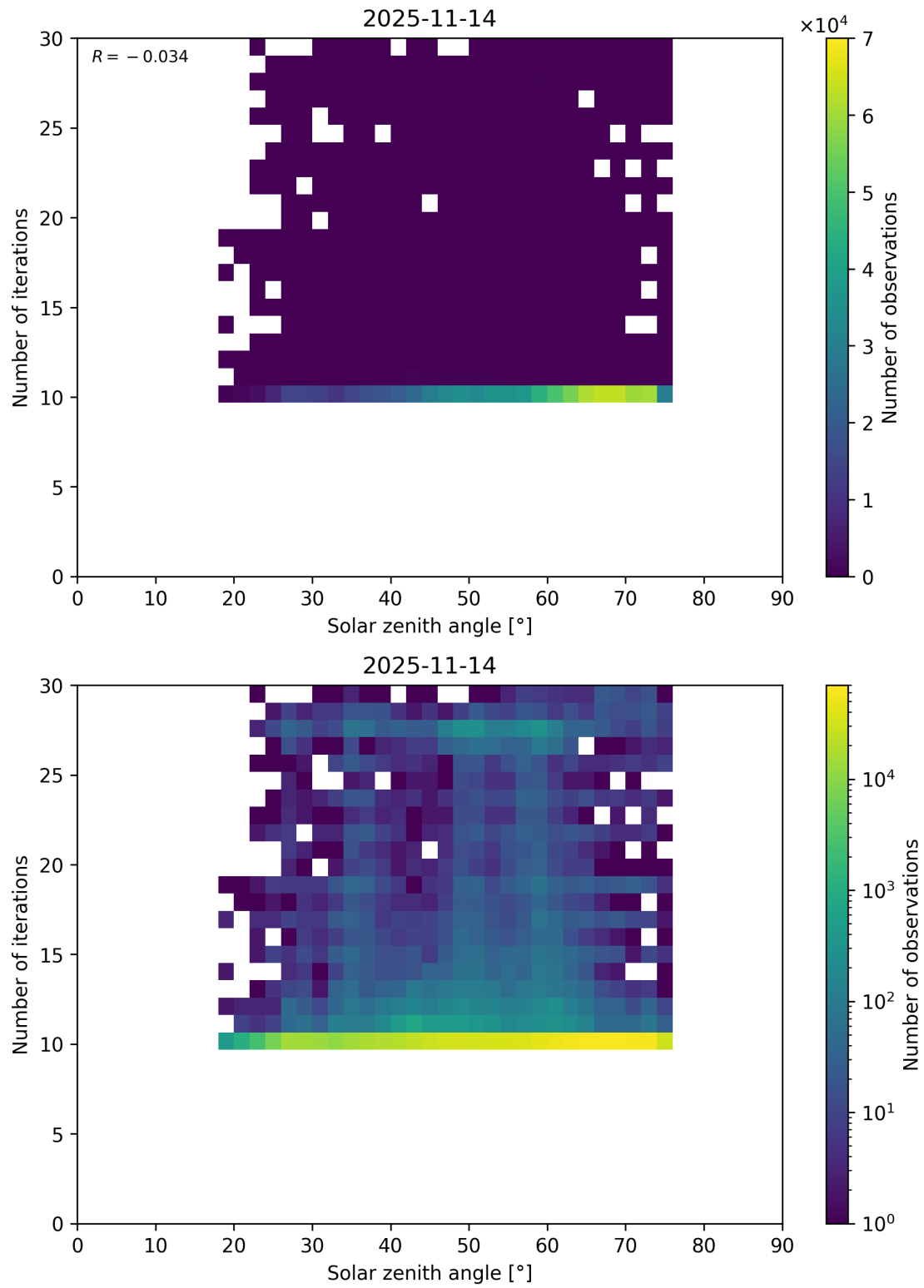
Figure 102: Scatter density plot of “Solar zenith angle” against “Number of iterations” for 2025-11-13 to 2025-11-15.
