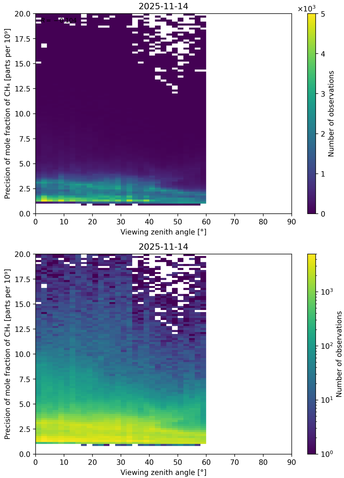
Figure 112: Scatter density plot of “Viewing zenith angle” against “Precision of mole fraction of CH 4 ” for 2025-11-13 to 2025-11-15.
