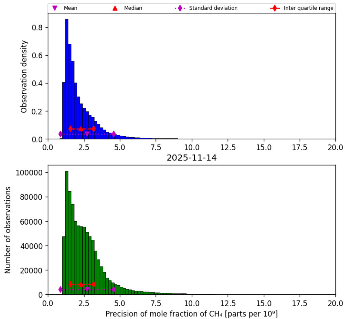
Figure 24: Histogram of “Precision of mole fraction of CH 4 ” for 2025-11-13 to 2025-11-15
