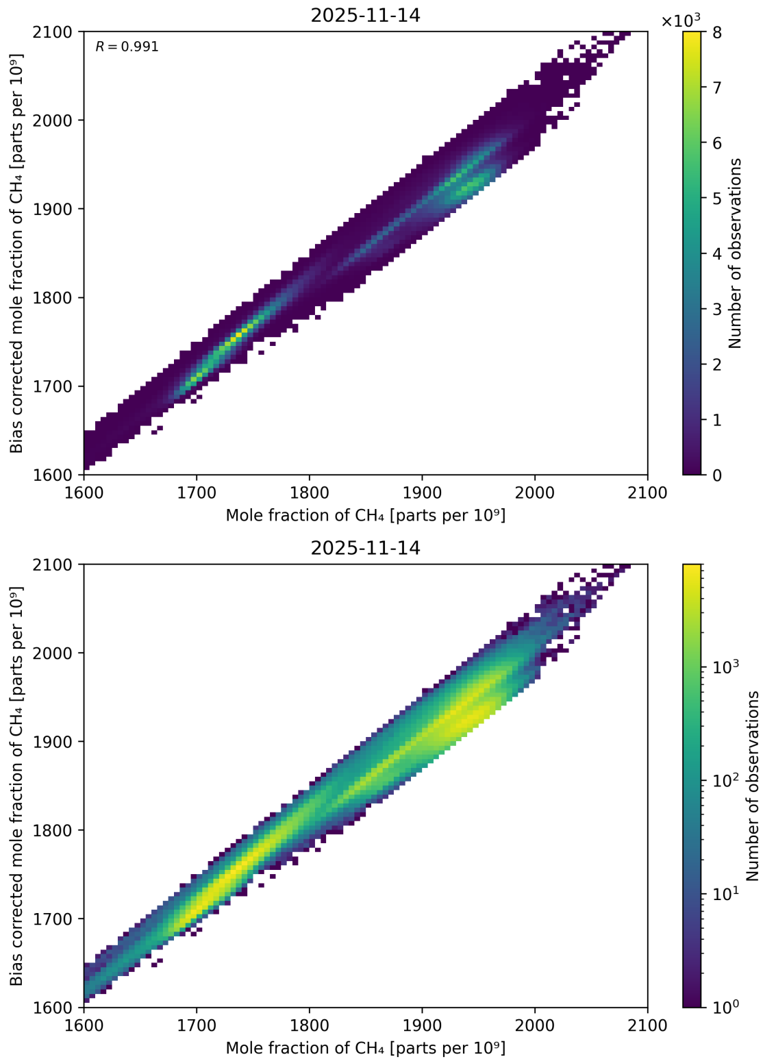
Figure 74: Scatter density plot of “Mole fraction of CH 4 ” against “Bias corrected mole fraction of CH 4 ” for 2025-11-13 to 2025-11-15.
