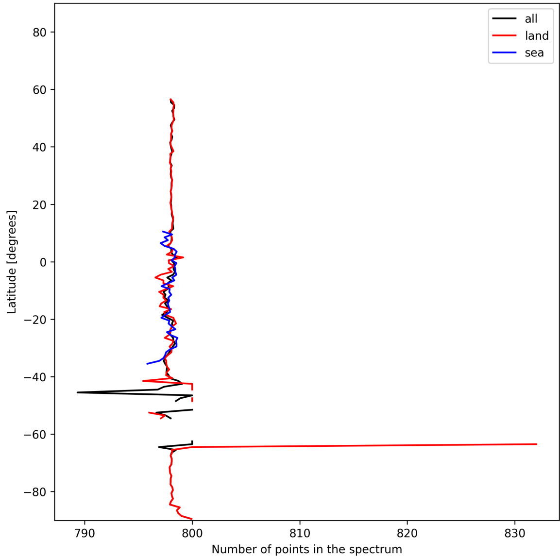
Figure 15: Zonal average of “Number of points in the spectrum” for 2025-11-13 to 2025-11-15.
