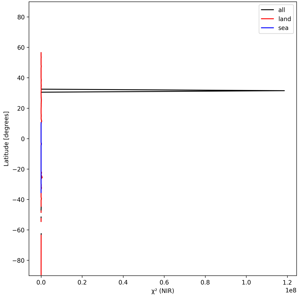
Figure 18: Zonal average of “ \chi^2 (NIR)” for 2025-11-13 to 2025-11-15.
