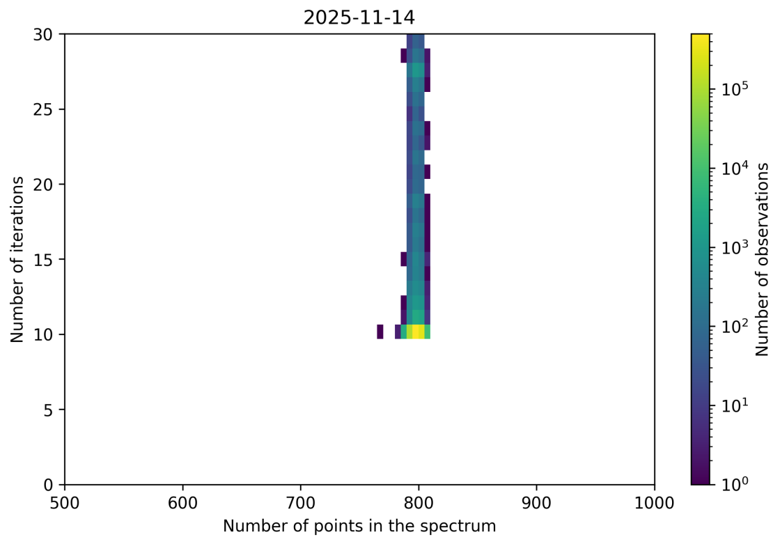
Figure 92: Scatter density plot of “Number of points in the spectrum” against “Number of iterations” for 2025-11-13 to 2025-11-15.
