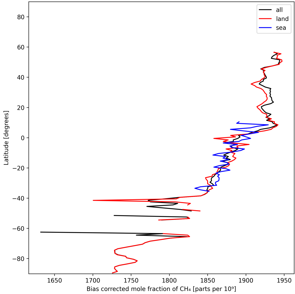
Figure 14: Zonal average of “Bias corrected mole fraction of CH 4 ” for 2025-11-13 to 2025-11-15.
