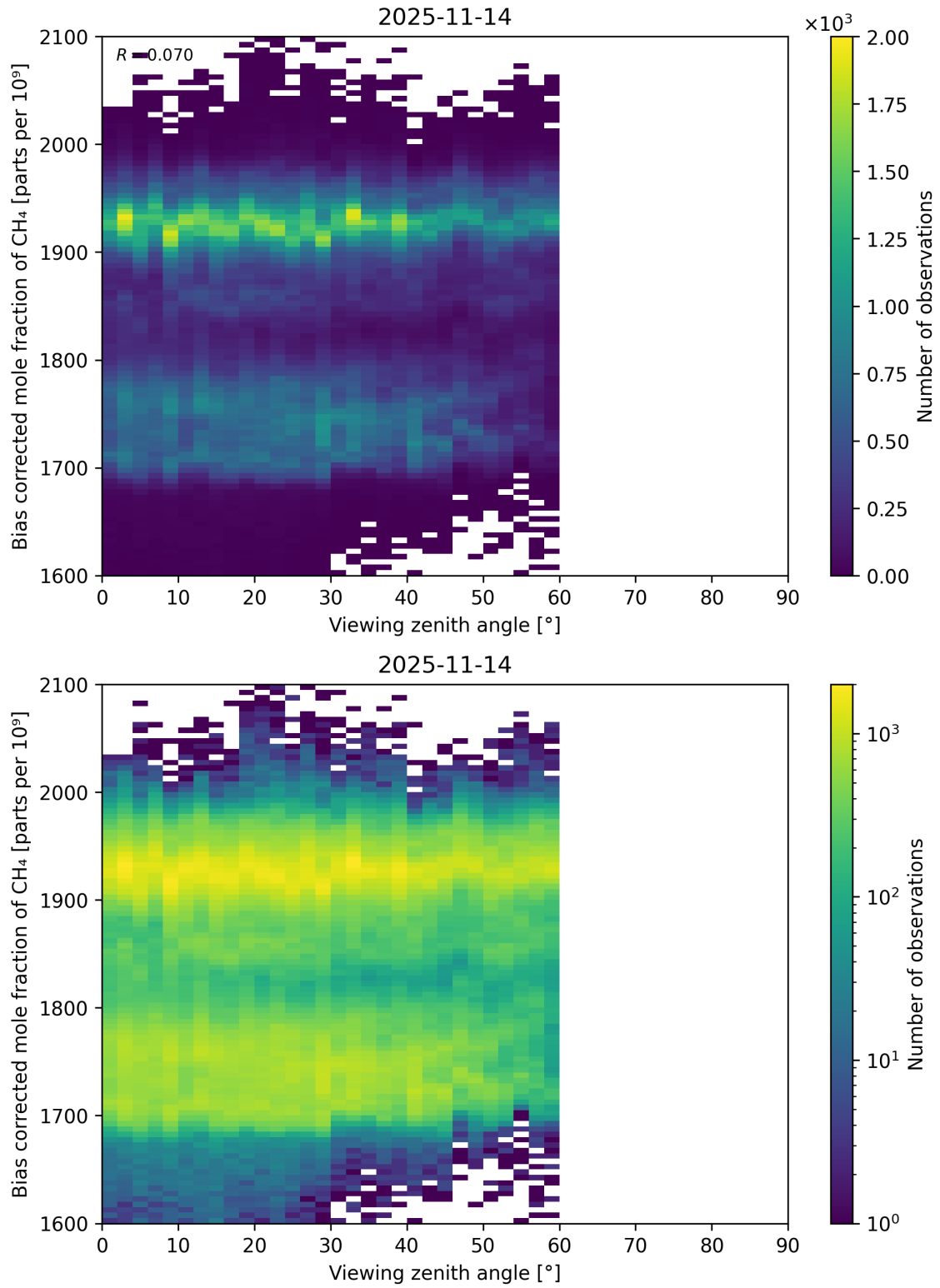
Figure 111: Scatter density plot of “Viewing zenith angle” against “Bias corrected mole fraction of CH 4 ” for 2025-11-13 to 2025-11-15.
