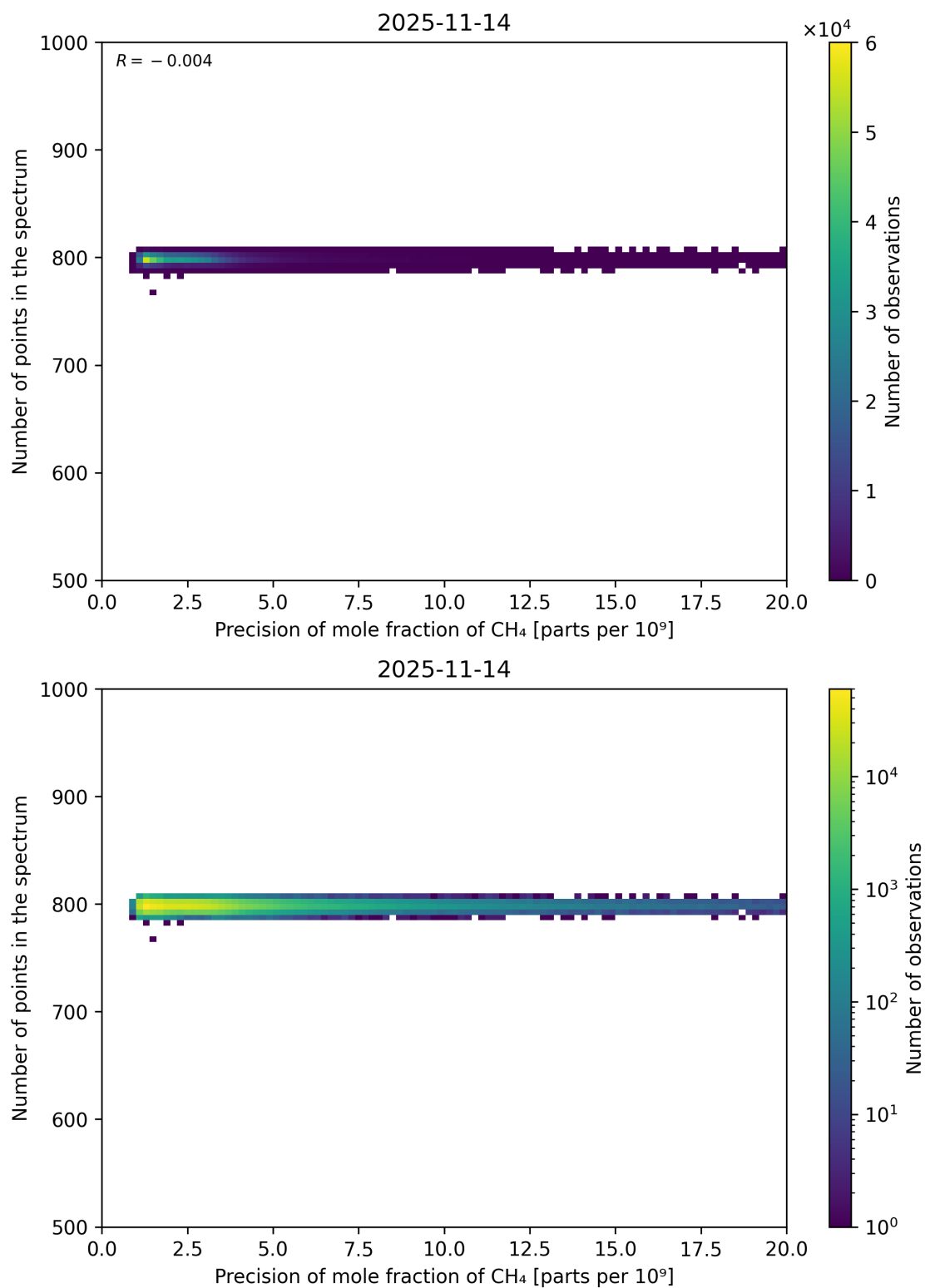
Figure 84: Scatter density plot of “Precision of mole fraction of CH 4 ” against “Number of points in the spectrum” for 2025-11-13 to 2025-11-15.
