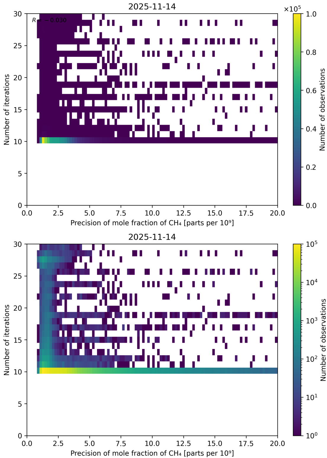
Figure 83: Scatter density plot of “Precision of mole fraction of CH 4 ” against “Number of iterations” for 2025-11-13 to 2025-11-15.
