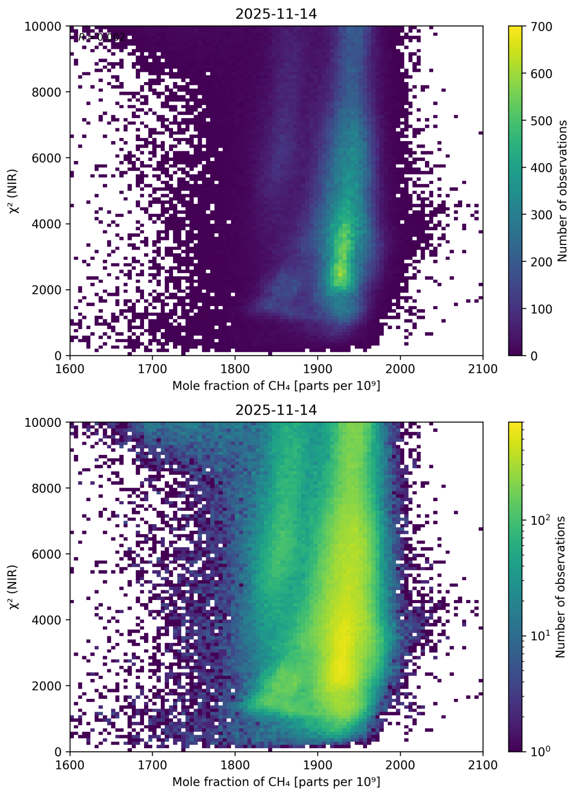
Figure 70: Scatter density plot of “Mole fraction of CH 4 ” against “ \chi^2 (NIR)” for 2025-11-13 to 2025-11-15.
