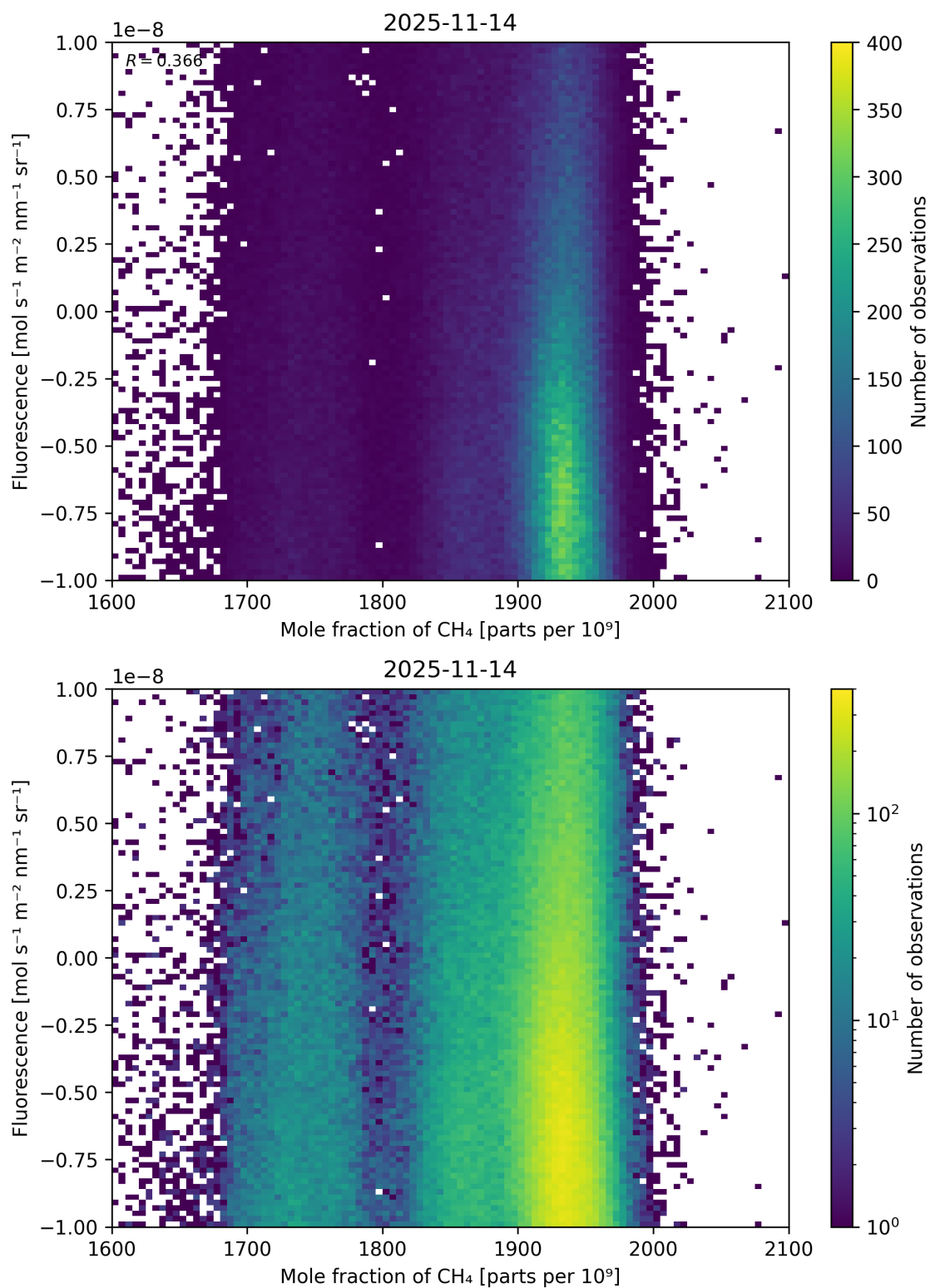
Figure 73: Scatter density plot of “Mole fraction of CH 4 ” against “Fluorescence” for 2025-11-13 to 2025-11-15.
