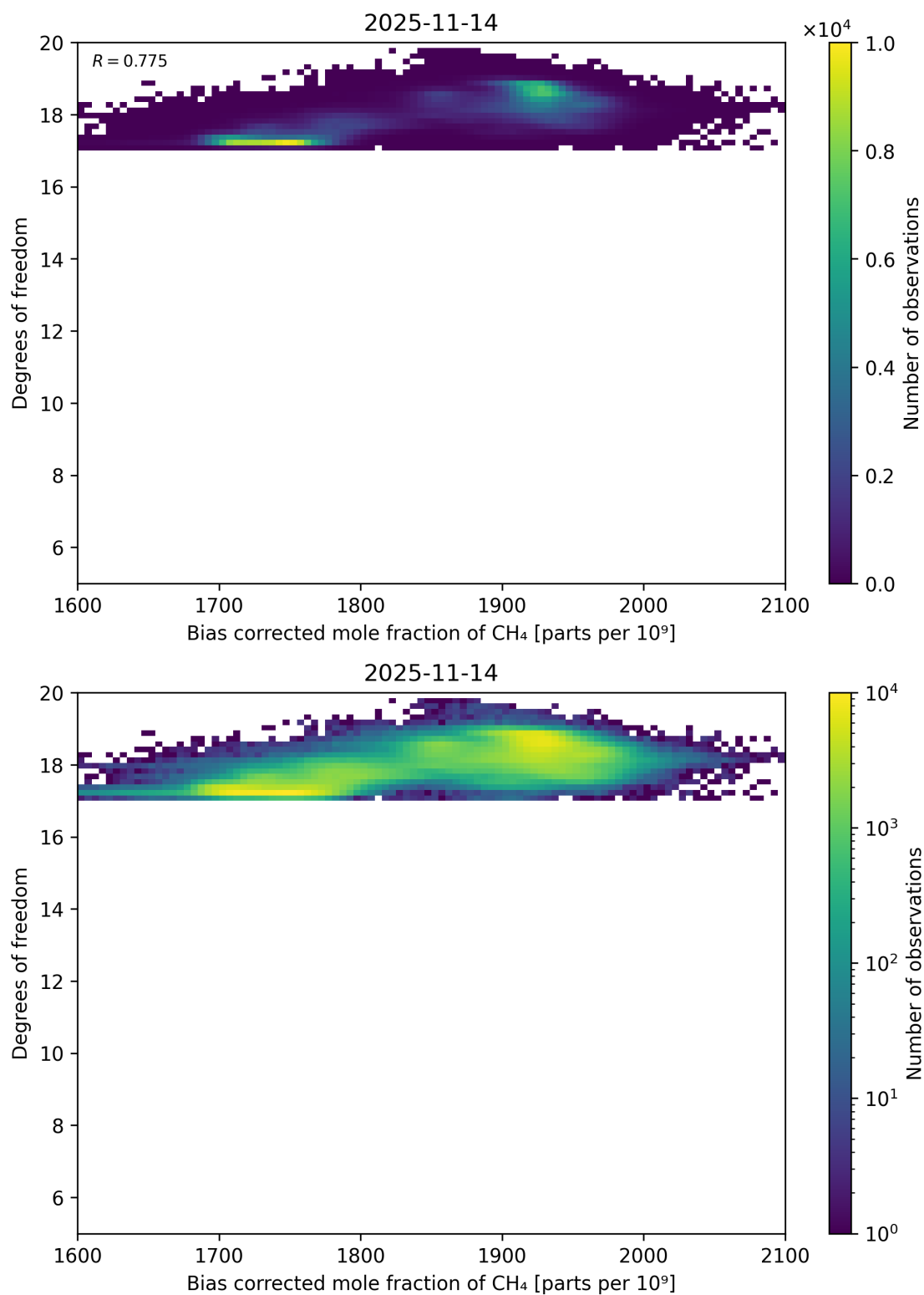
Figure 65: Scatter density plot of “Bias corrected mole fraction of CH 4 ” against “Degrees of freedom” for 2025-11-13 to 2025-11-15.
