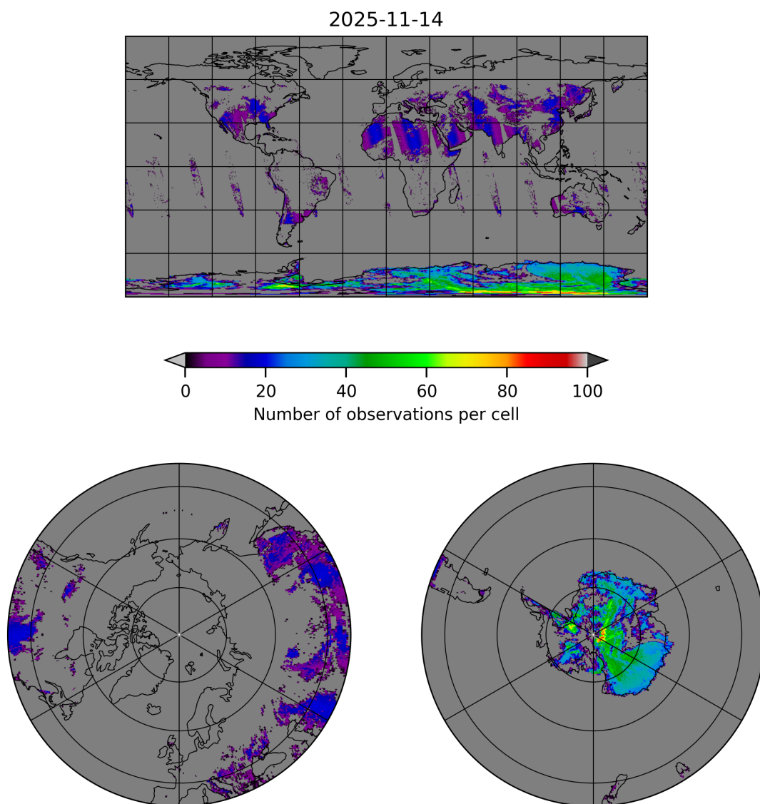
Figure 10: Map of the number of observations for 2025-11-13 to 2025-11-15
