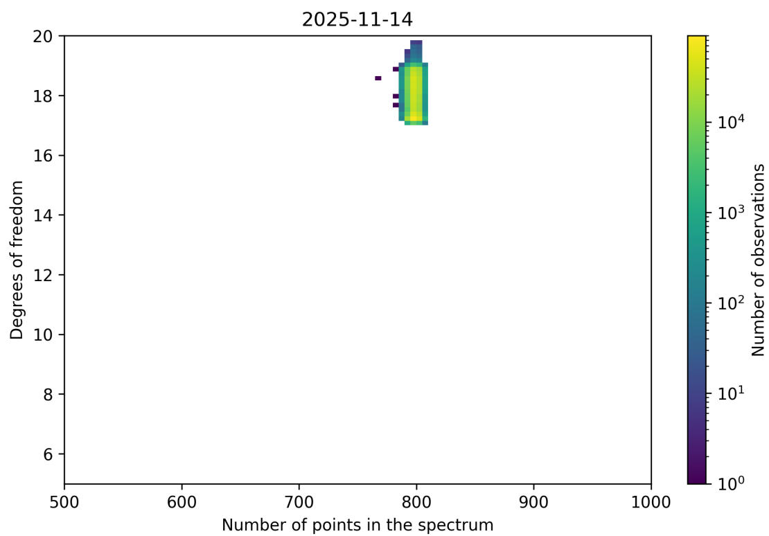
Figure 90: Scatter density plot of “Number of points in the spectrum” against “Degrees of freedom” for 2025-11-13 to 2025-11-15.
