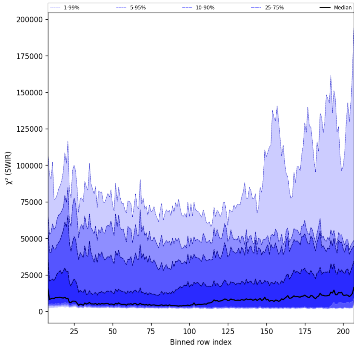
Figure 39: Along track statistics of “ \chi^2 (SWIR)” for 2025-11-13 to 2025-11-15
