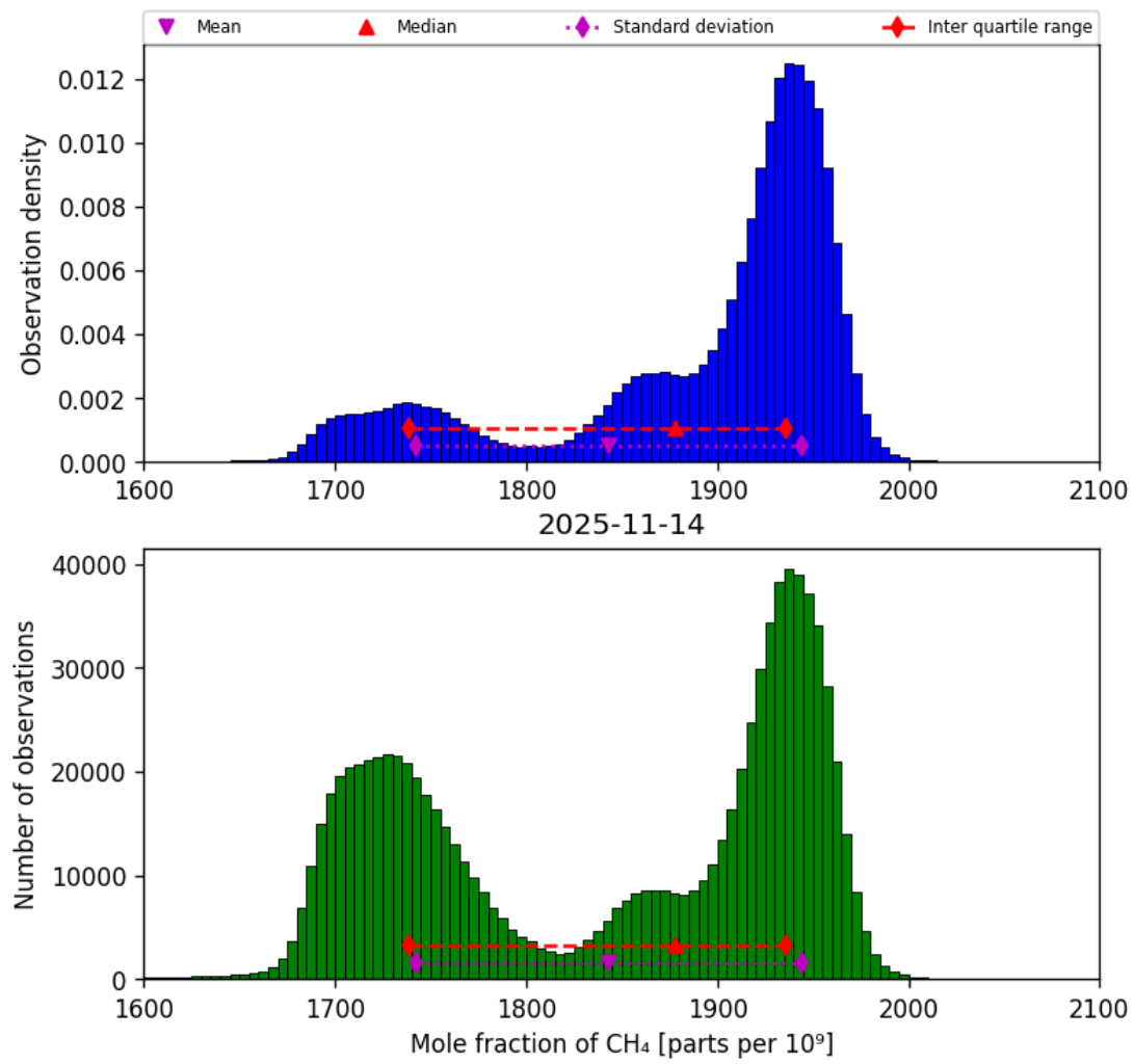
Figure 23: Histogram of “Mole fraction of CH 4 ” for 2025-11-13 to 2025-11-15
