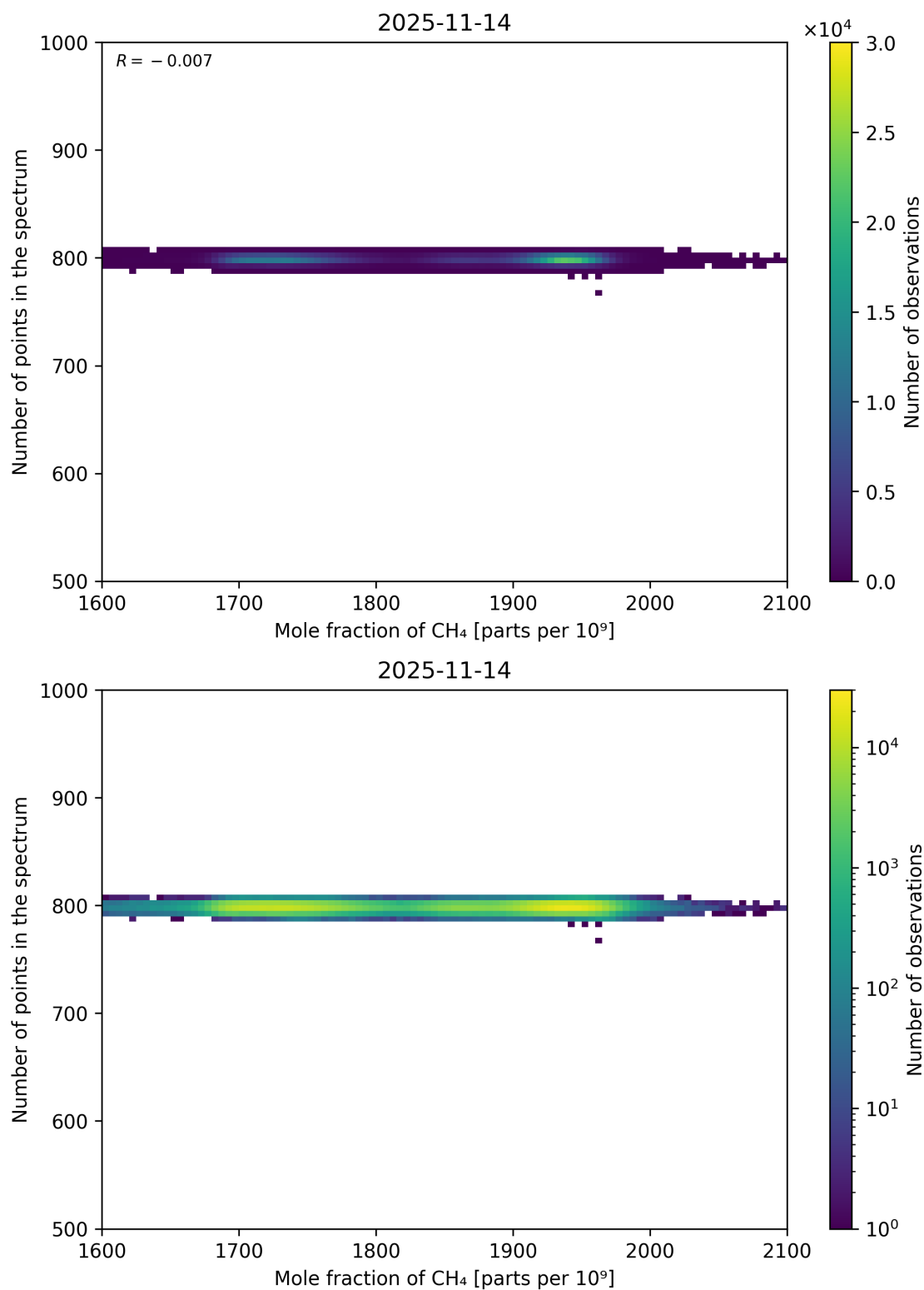
Figure 77: Scatter density plot of “Mole fraction of CH 4 ” against “Number of points in the spectrum” for 2025-11-13 to 2025-11-15.
