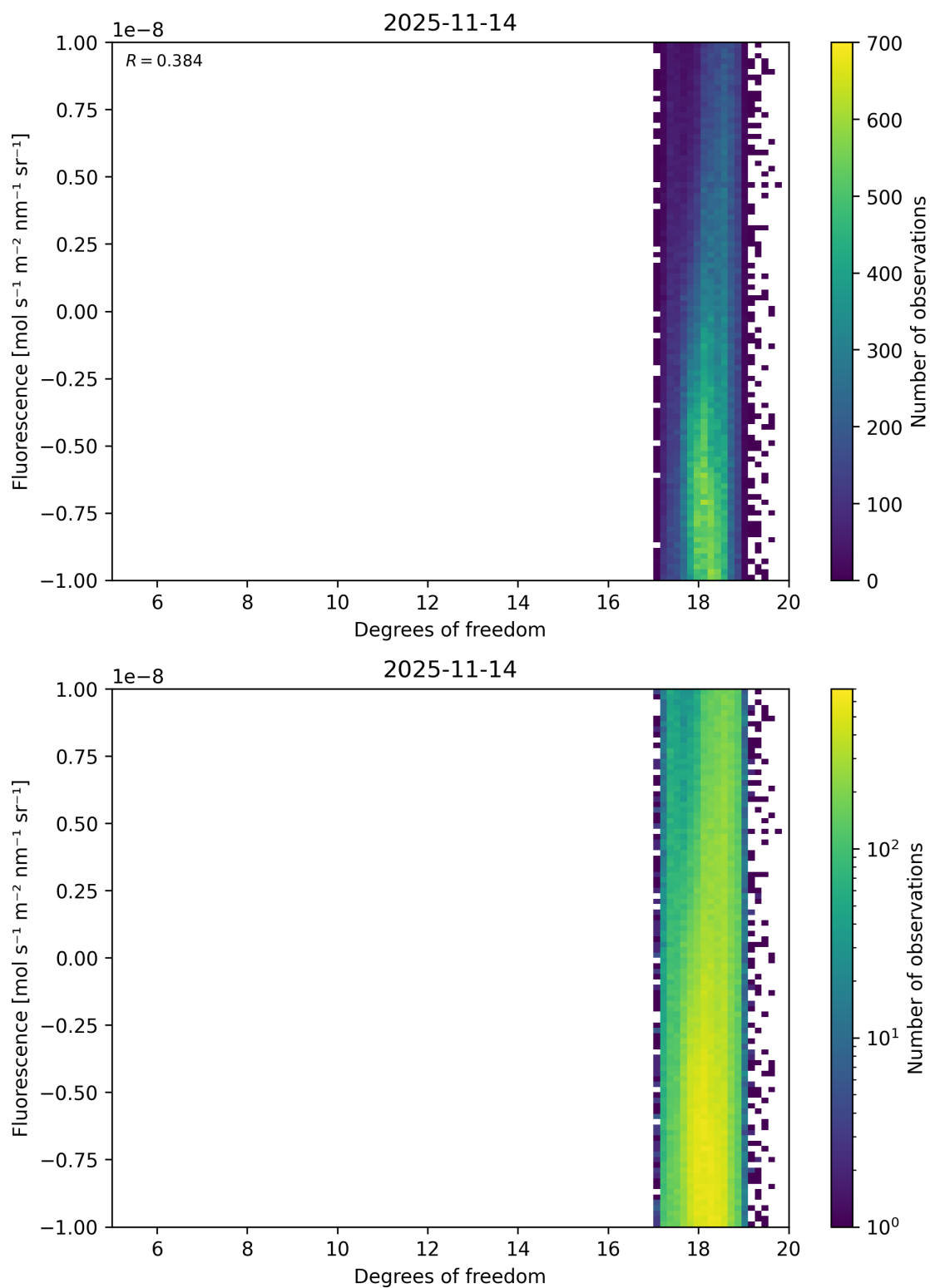
Figure 51: Scatter density plot of “Degrees of freedom” against “Fluorescence” for 2025-11-13 to 2025-11-15.
