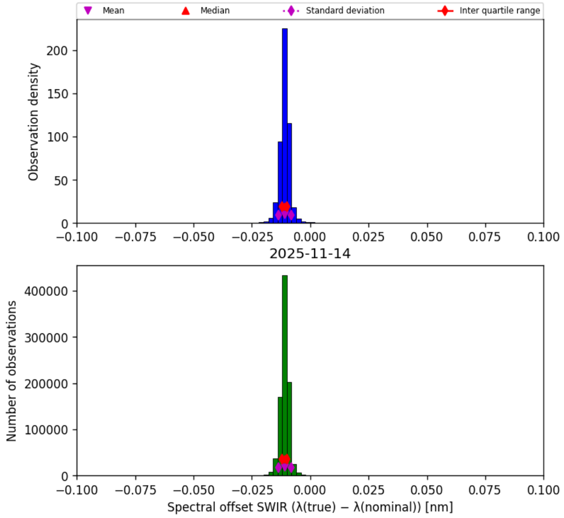
Figure 27: Histogram of “Spectral offset SWIR ( \lambda_{\text{true}} - \lambda_{\text{nominal}} )” for 2025-11-13 to 2025-11-15
