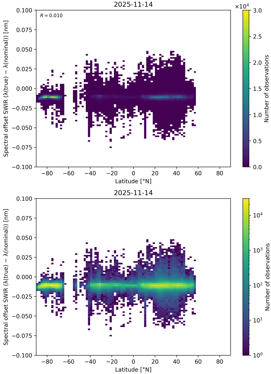
Figure 62: Scatter density plot of “Latitude” against “Spectral offset SWIR ( \lambda_{\text{true}} - \lambda_{\text{nominal}} )” for 2025-11-13 to 2025-11-15.
