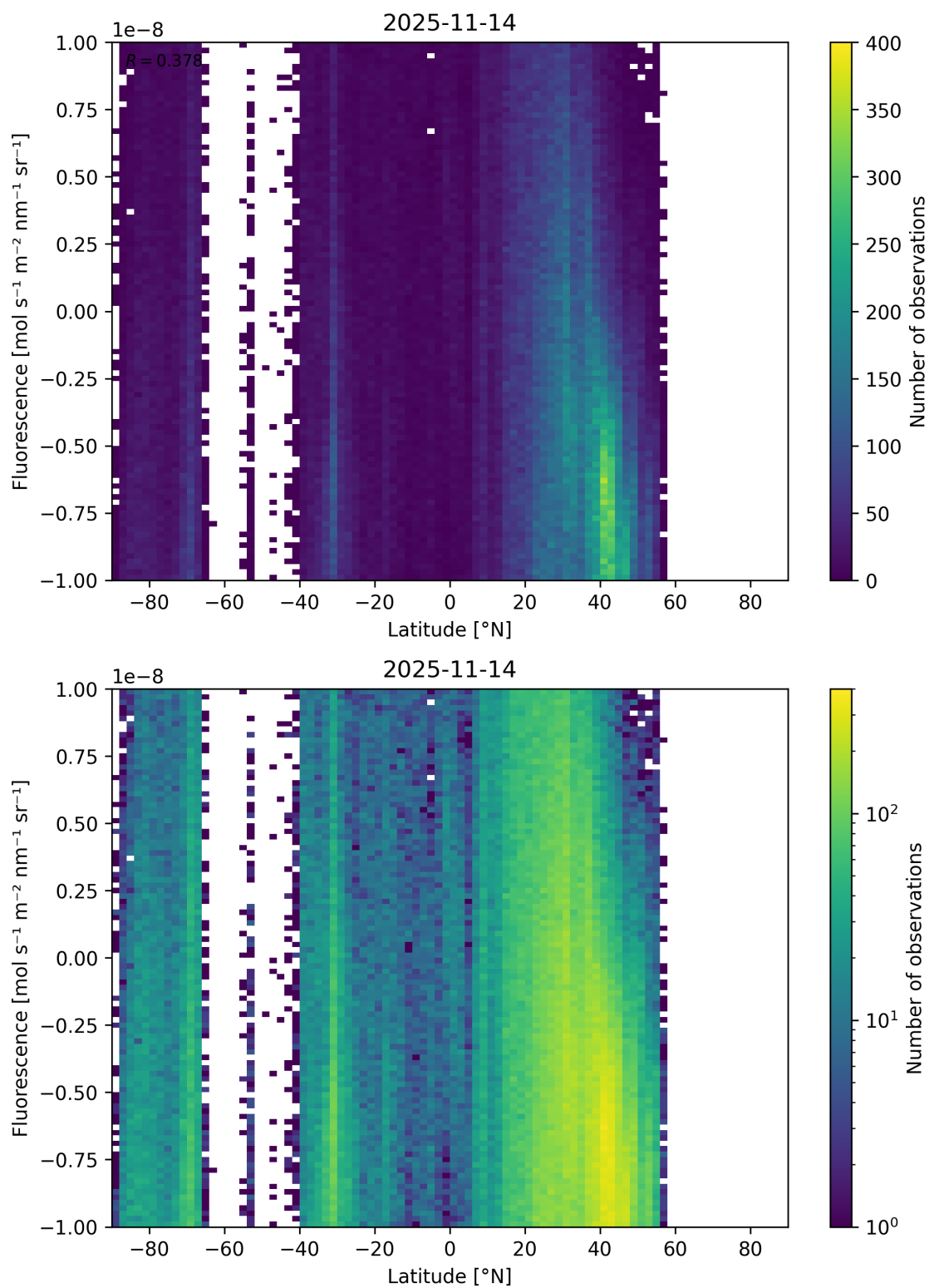
Figure 56: Scatter density plot of “Latitude” against “Fluorescence” for 2025-11-13 to 2025-11-15.
