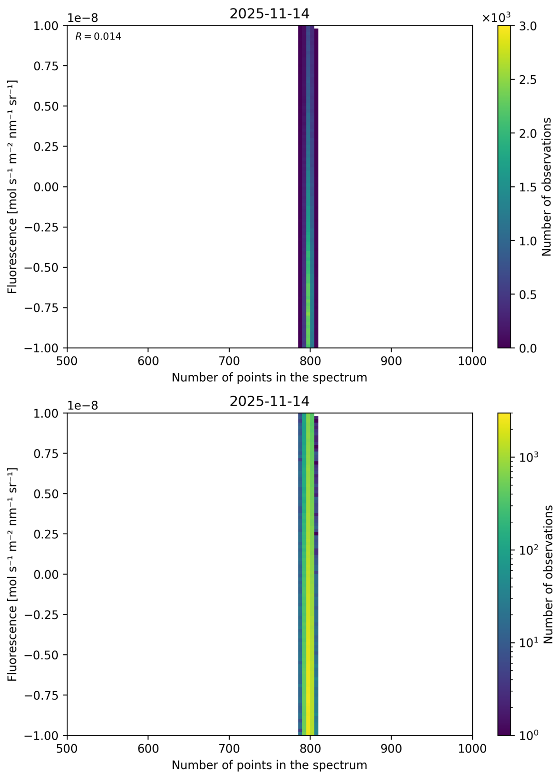
Figure 91: Scatter density plot of “Number of points in the spectrum” against “Fluorescence” for 2025-11-13 to 2025-11-15.
