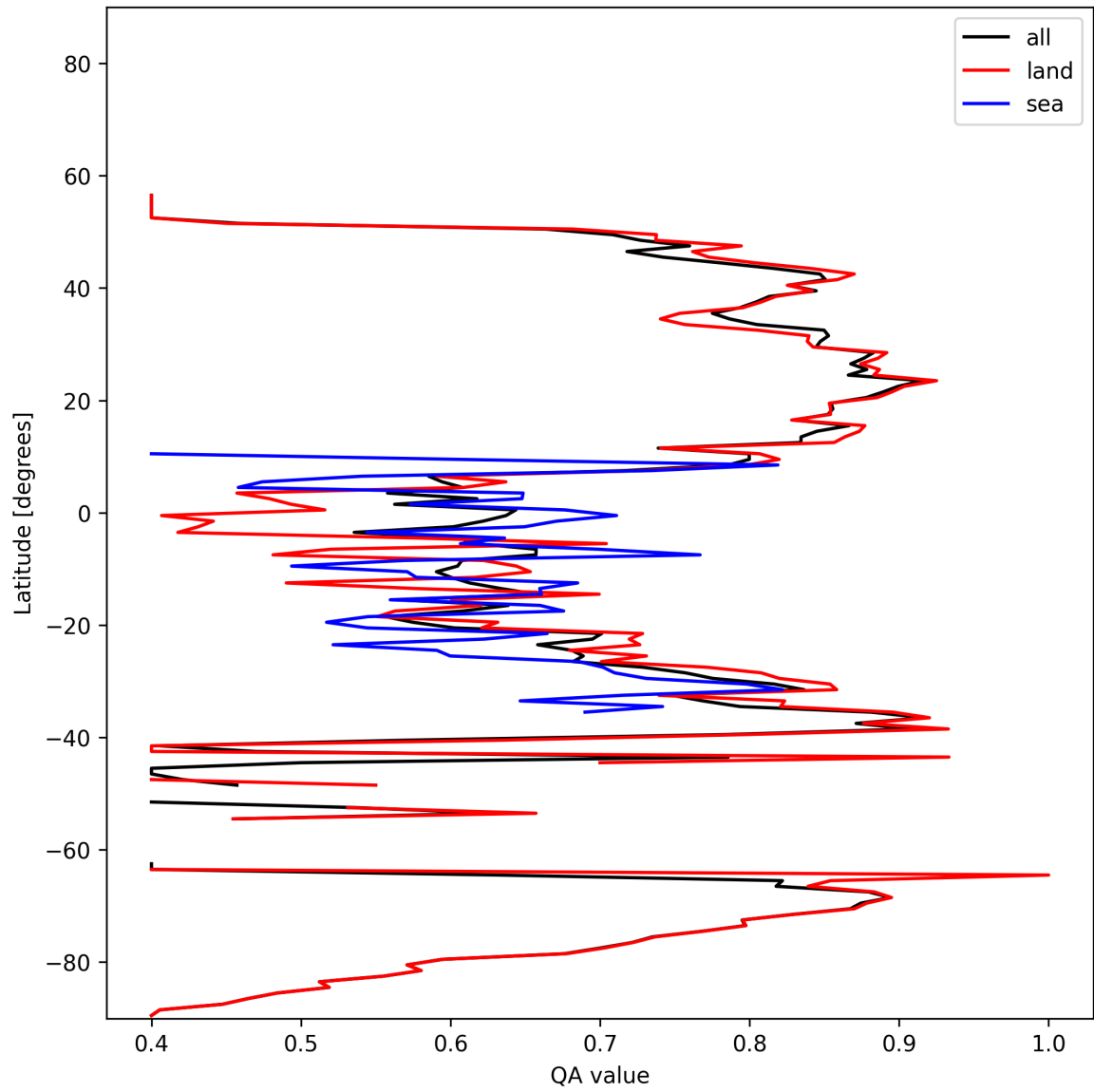
Figure 11: Zonal average of “QA value” for 2025-11-13 to 2025-11-15.
