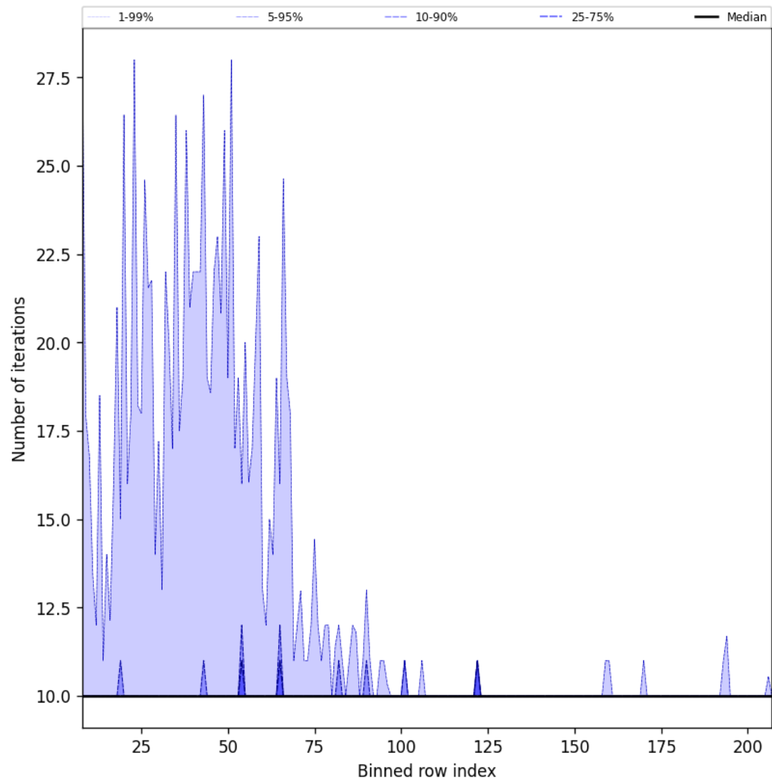
Figure 42: Along track statistics of “Number of iterations” for 2025-11-13 to 2025-11-15
