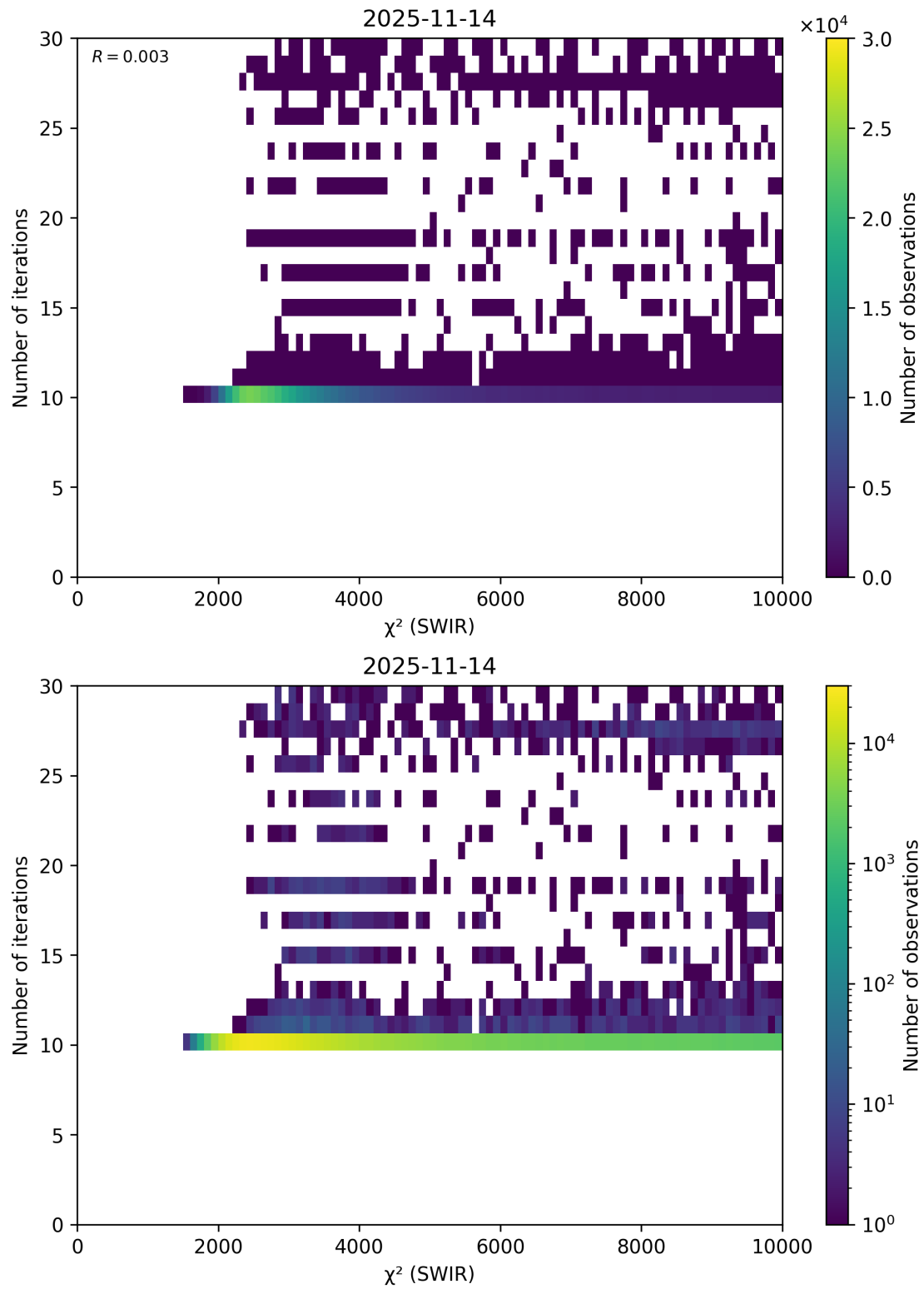
Figure 50: Scatter density plot of “ \chi^2 (SWIR)” against “Number of iterations” for 2025-11-13 to 2025-11-15.
