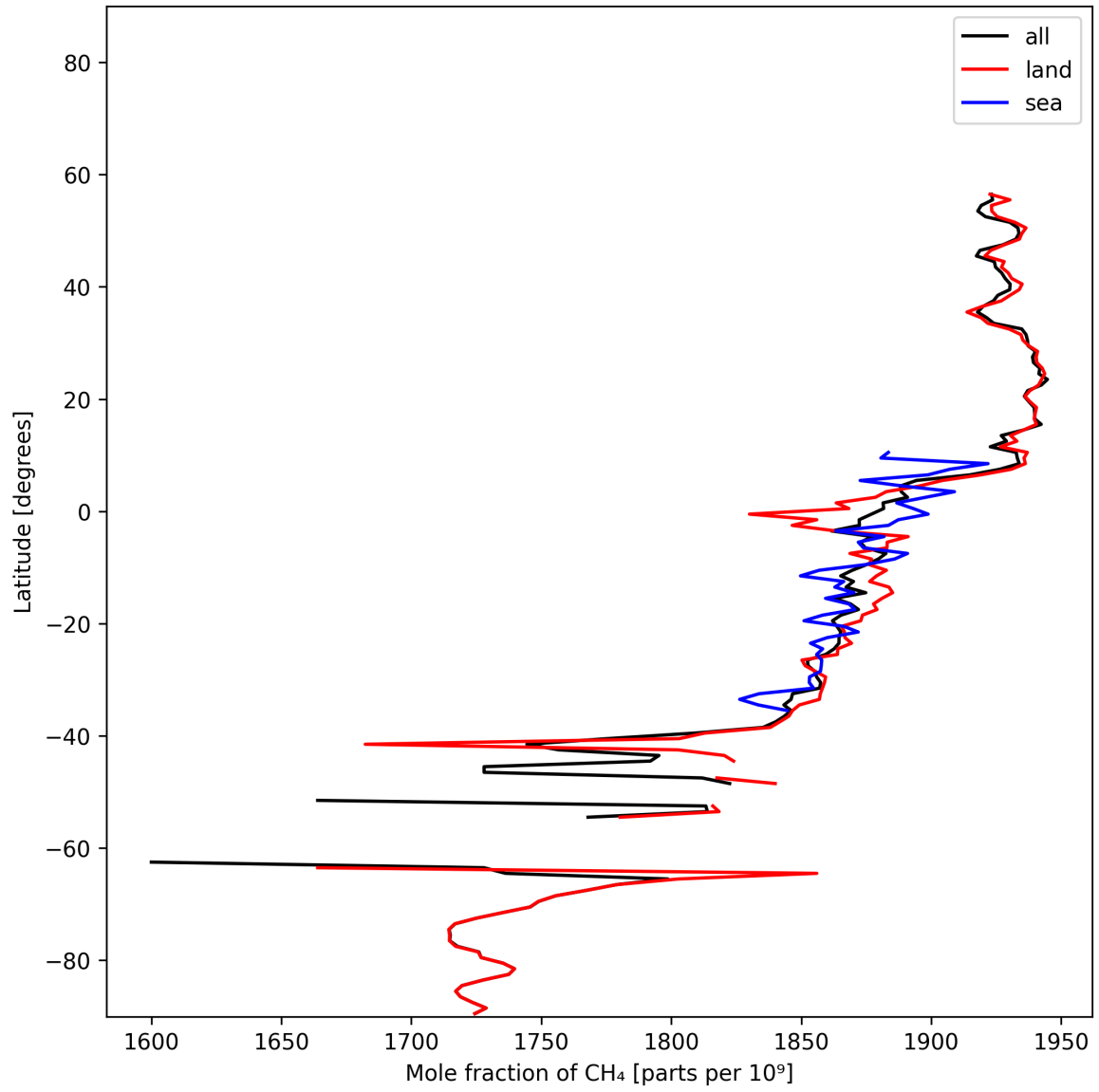
Figure 12: Zonal average of “Mole fraction of CH 4 ” for 2025-11-13 to 2025-11-15.
