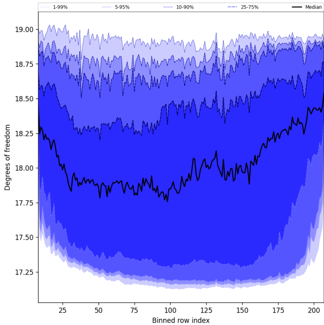
Figure 41: Along track statistics of “Degrees of freedom” for 2025-11-13 to 2025-11-15
