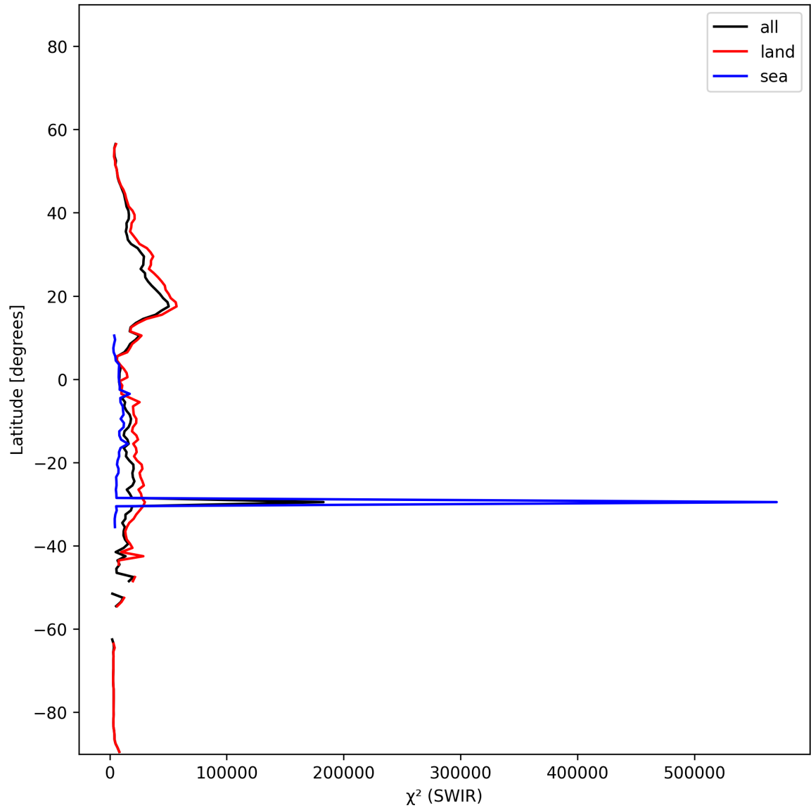
Figure 17: Zonal average of “ \chi^2 (SWIR)” for 2025-11-13 to 2025-11-15.
