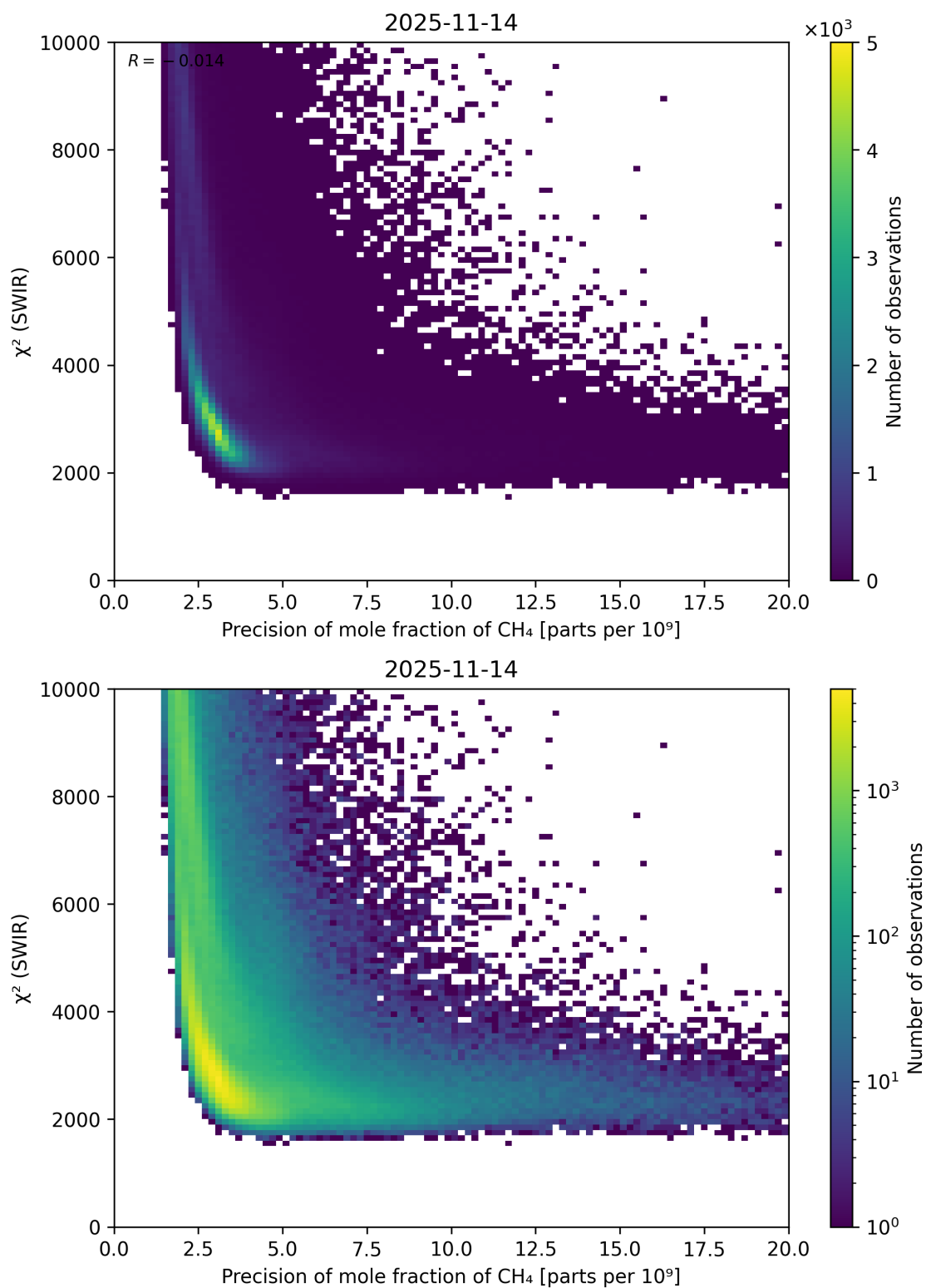
Figure 79: Scatter density plot of “Precision of mole fraction of \text{CH}_4 ” against “ \chi^2 (SWIR)” for 2025-11-13 to 2025-11-15.
