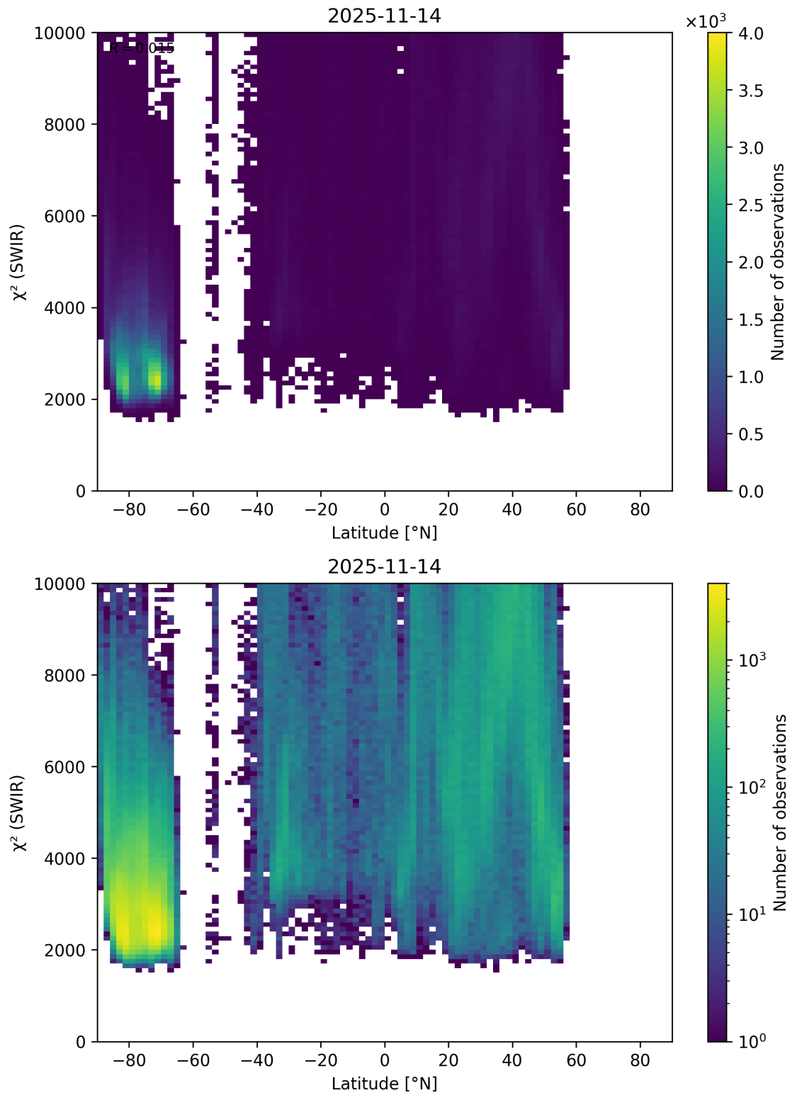
Figure 54: Scatter density plot of “Latitude” against “ \chi^2 (SWIR)” for 2025-11-13 to 2025-11-15.
