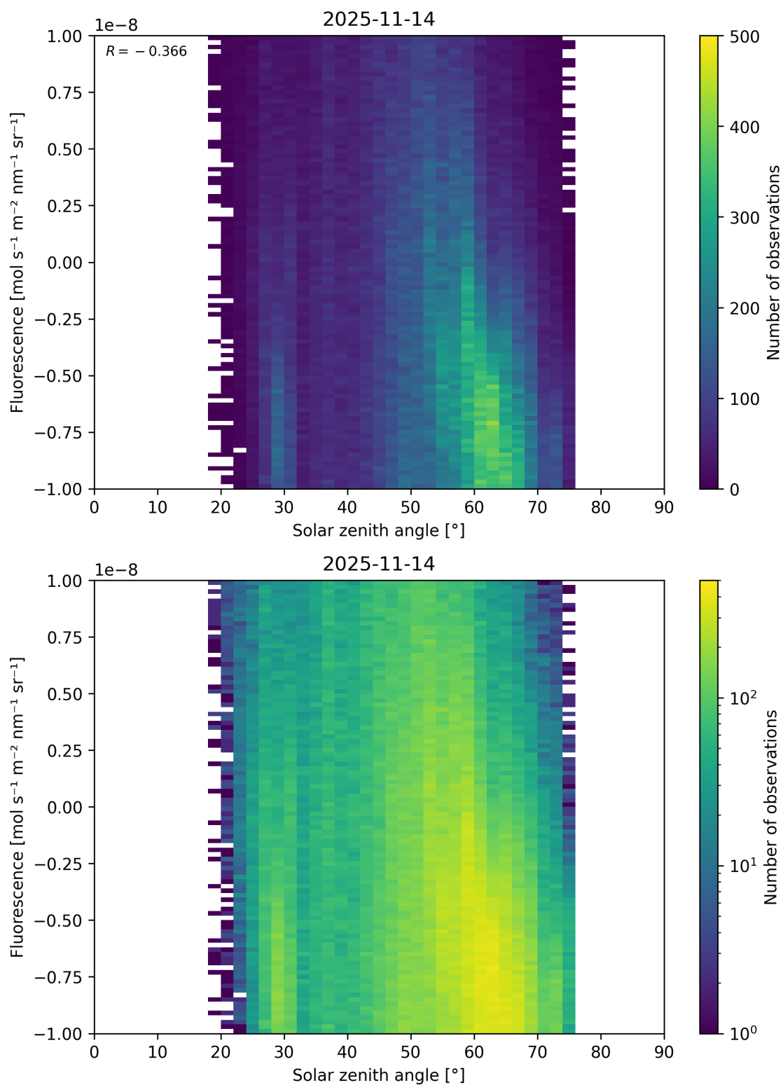
Figure 97: Scatter density plot of “Solar zenith angle” against “Fluorescence” for 2025-11-13 to 2025-11-15.
