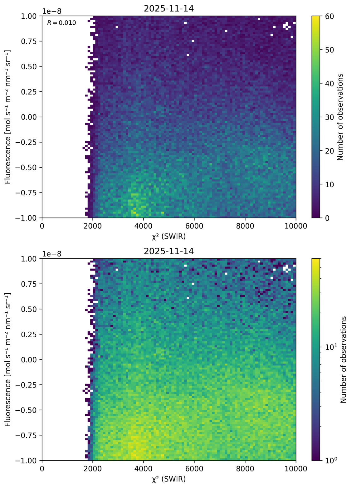
Figure 49: Scatter density plot of “ \chi^2 (SWIR)” against “Fluorescence” for 2025-11-13 to 2025-11-15.
