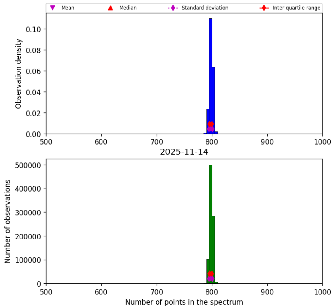
Figure 26: Histogram of “Number of points in the spectrum” for 2025-11-13 to 2025-11-15
