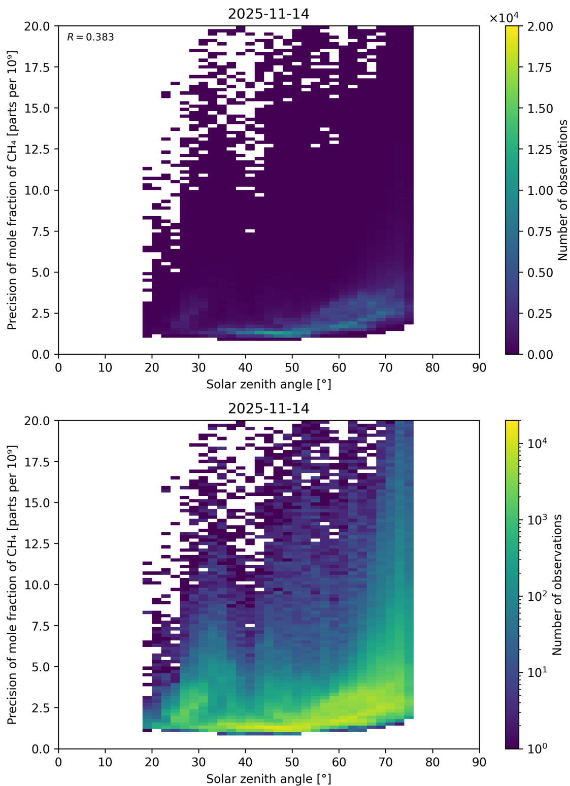
Figure 101: Scatter density plot of “Solar zenith angle” against “Precision of mole fraction of \text{CH}_4 ” for 2025-11-13 to 2025-11-15.
