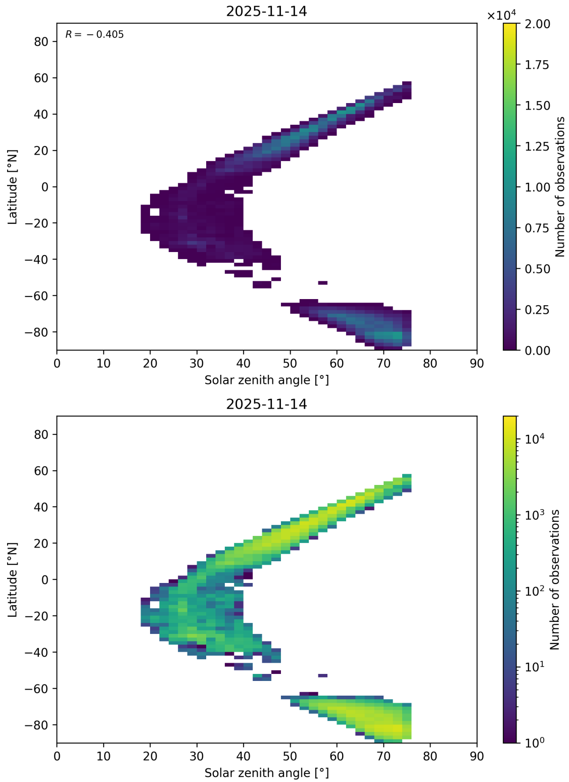
Figure 98: Scatter density plot of “Solar zenith angle” against “Latitude” for 2025-11-13 to 2025-11-15.
