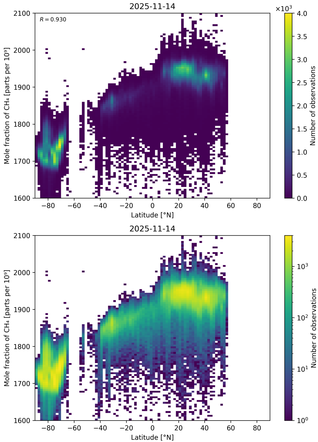
Figure 57: Scatter density plot of “Latitude” against “Mole fraction of CH 4 ” for 2025-11-13 to 2025-11-15.
