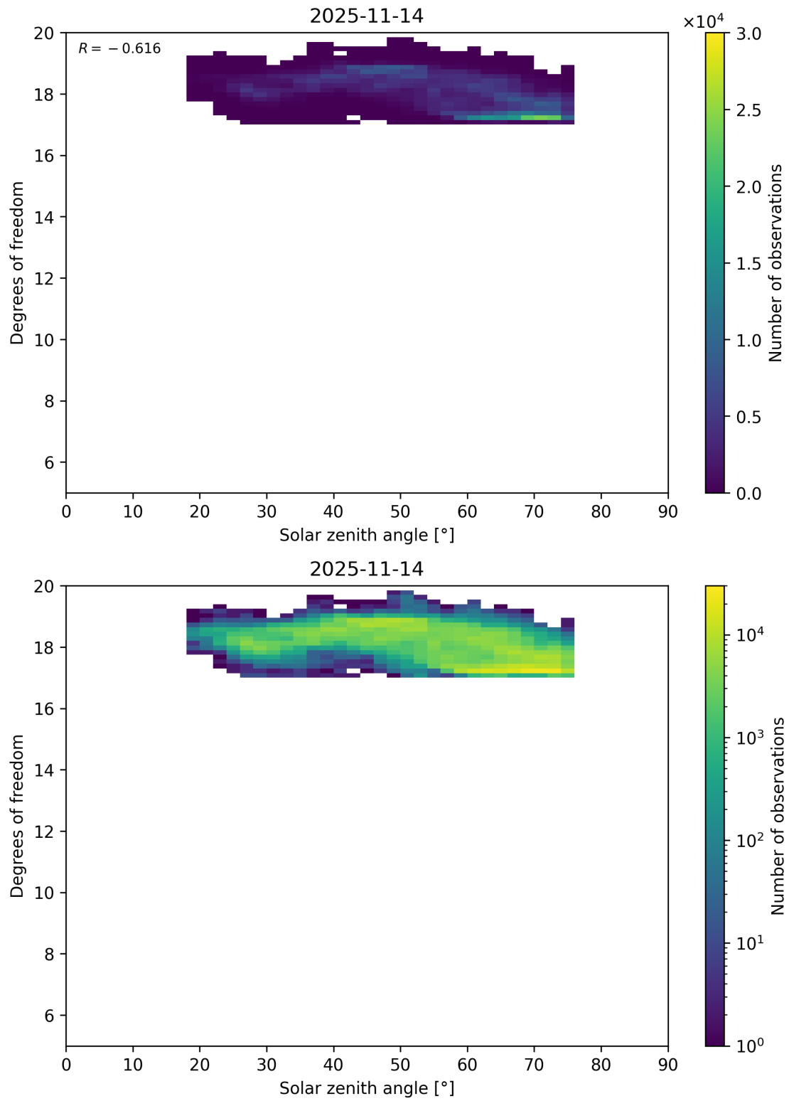
Figure 96: Scatter density plot of “Solar zenith angle” against “Degrees of freedom” for 2025-11-13 to 2025-11-15.
