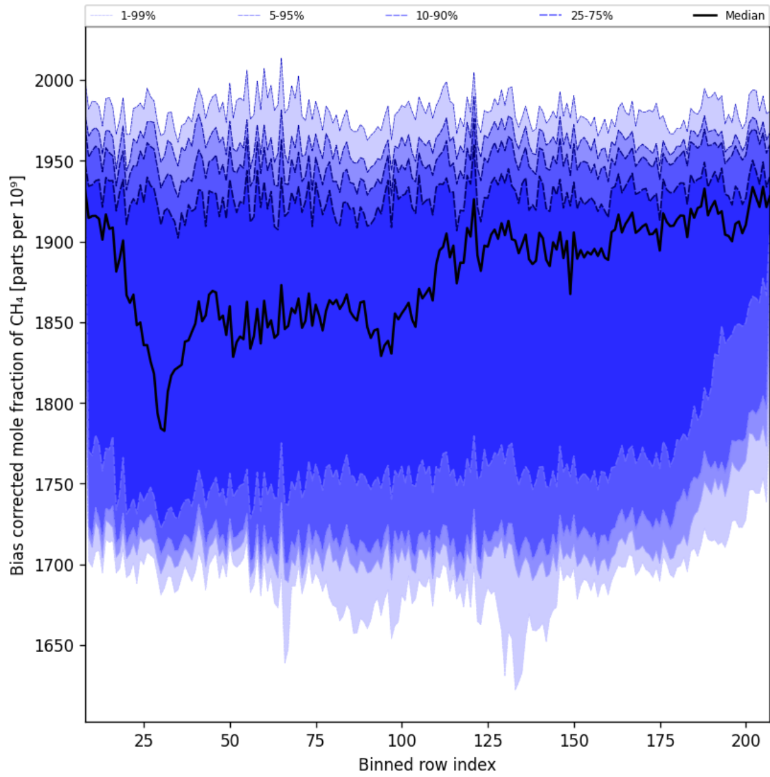
Figure 36: Along track statistics of “Bias corrected mole fraction of CH 4 ” for 2025-11-13 to 2025-11-15
