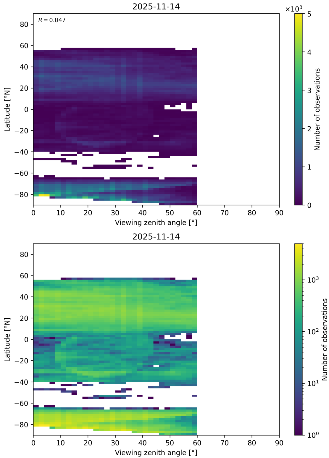
Figure 109: Scatter density plot of “Viewing zenith angle” against “Latitude” for 2025-11-13 to 2025-11-15.
