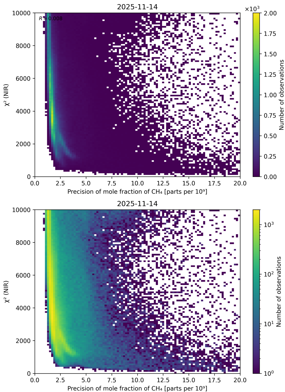
Figure 78: Scatter density plot of “Precision of mole fraction of \text{CH}_4 ” against “ \chi^2 (NIR)” for 2025-11-13 to 2025-11-15.
