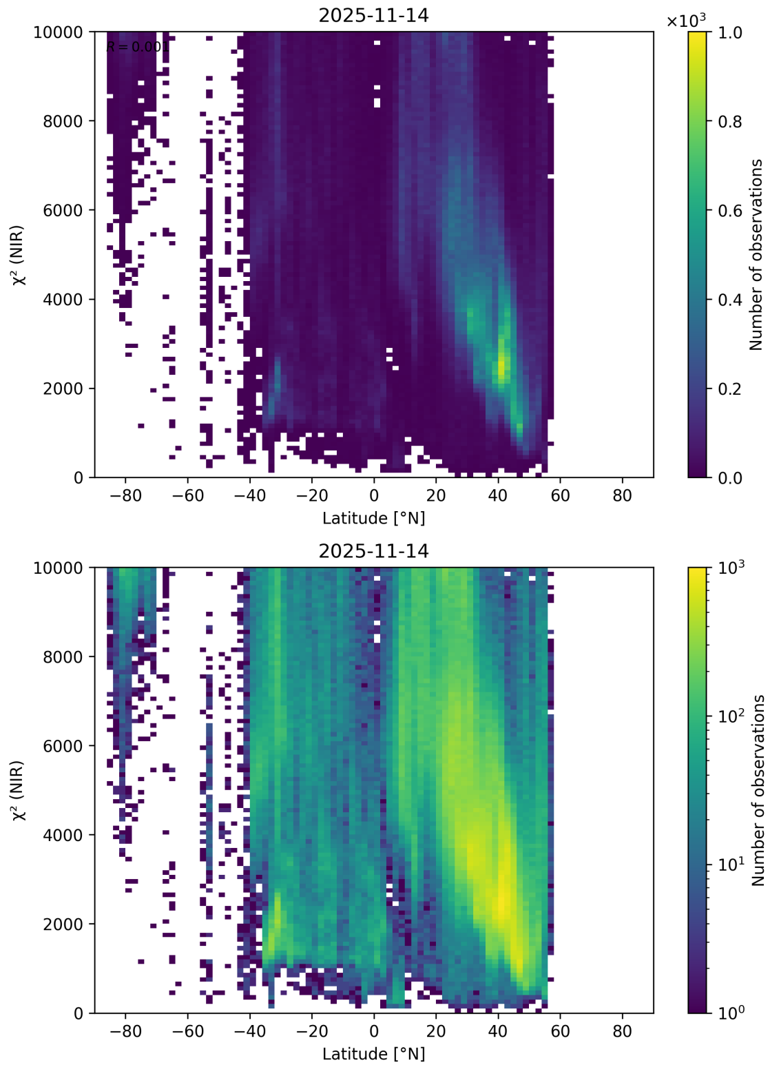
Figure 53: Scatter density plot of “Latitude” against “ \chi^2 (NIR)” for 2025-11-13 to 2025-11-15.
