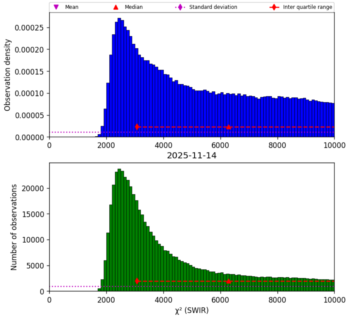
Figure 28: Histogram of " \chi^2 (SWIR)" for 2025-11-13 to 2025-11-15
