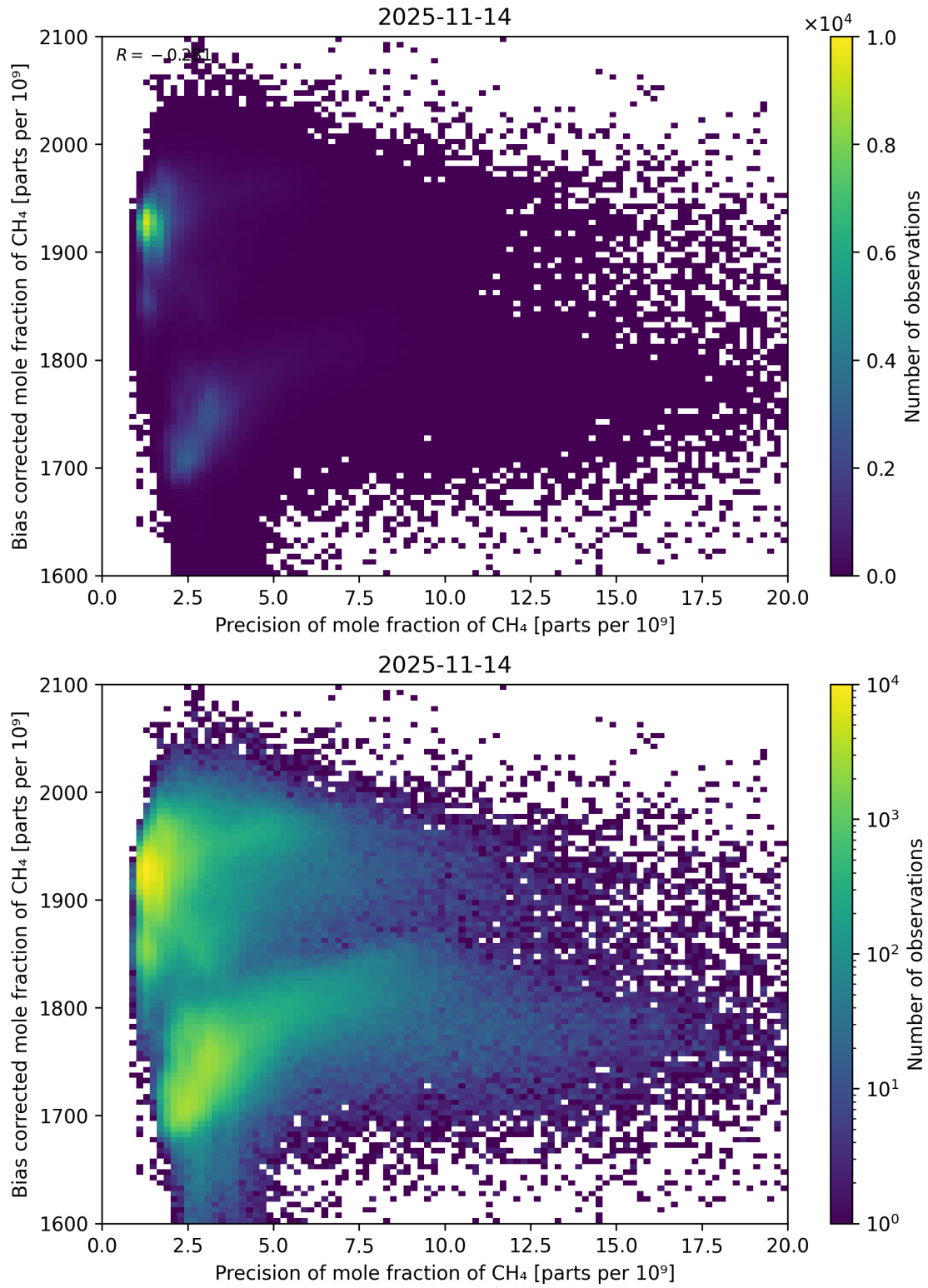
Figure 82: Scatter density plot of “Precision of mole fraction of CH 4 ” against “Bias corrected mole fraction of CH 4 ” for 2025-11-13 to 2025-11-15.
