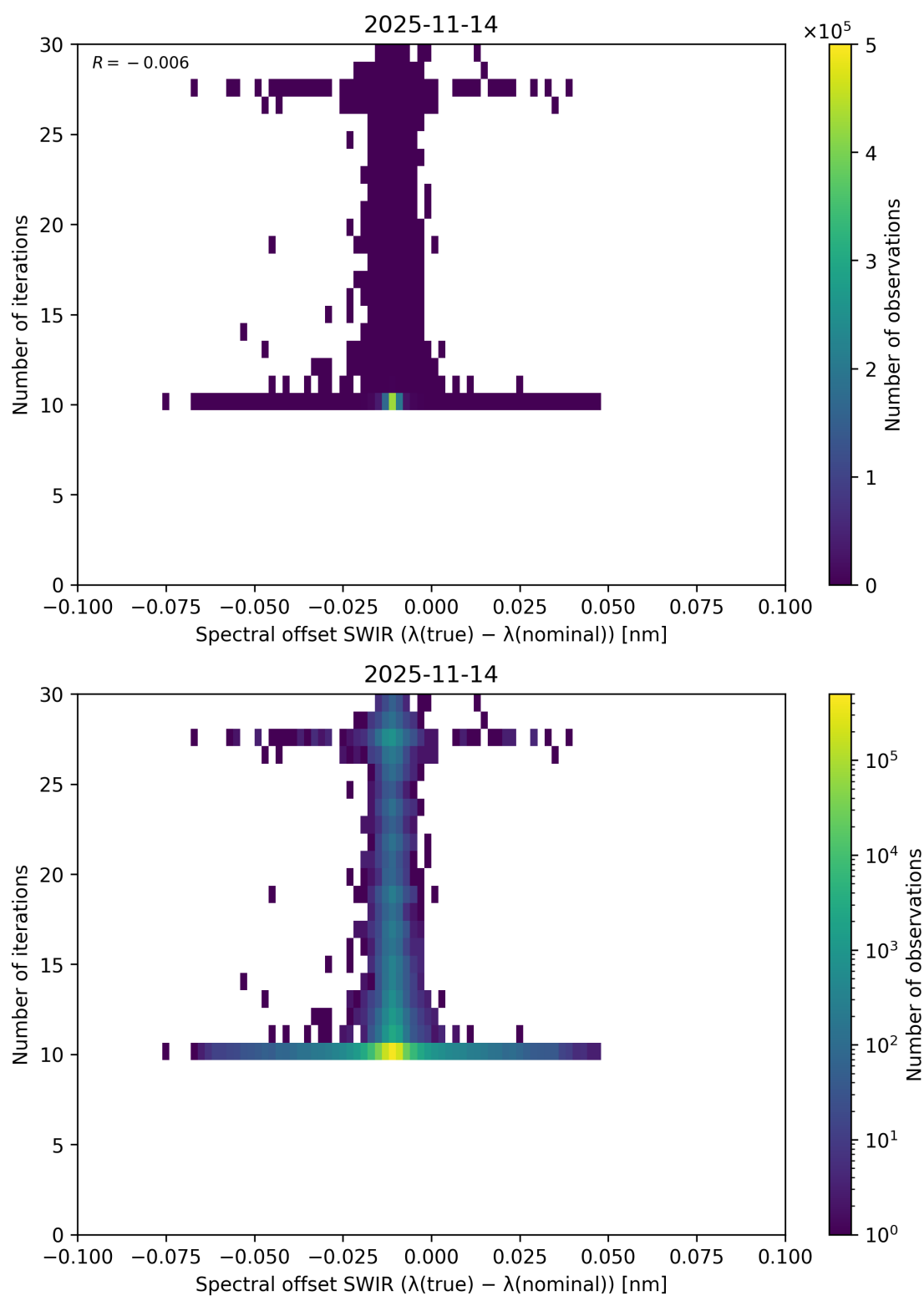
Figure 121: Scatter density plot of “Spectral offset SWIR ( \lambda_{\text{true}} - \lambda_{\text{nominal}} )” against “Number of iterations” for 2025-11-13 to 2025-11-15.
