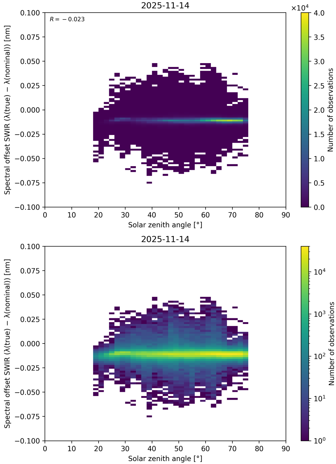
Figure 104: Scatter density plot of “Solar zenith angle” against “Spectral offset SWIR ( \lambda_{\text{true}} - \lambda_{\text{nominal}} )” for 2025-11-13 to 2025-11-15.
