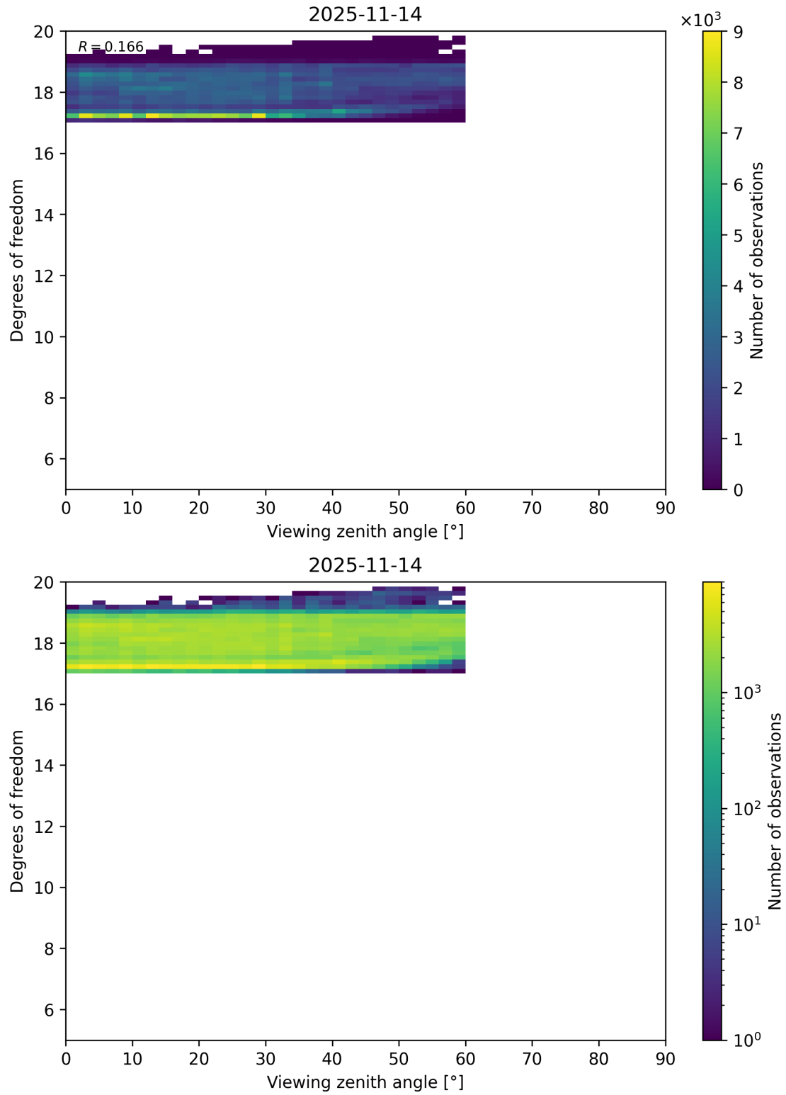
Figure 107: Scatter density plot of “Viewing zenith angle” against “Degrees of freedom” for 2025-11-13 to 2025-11-15.
