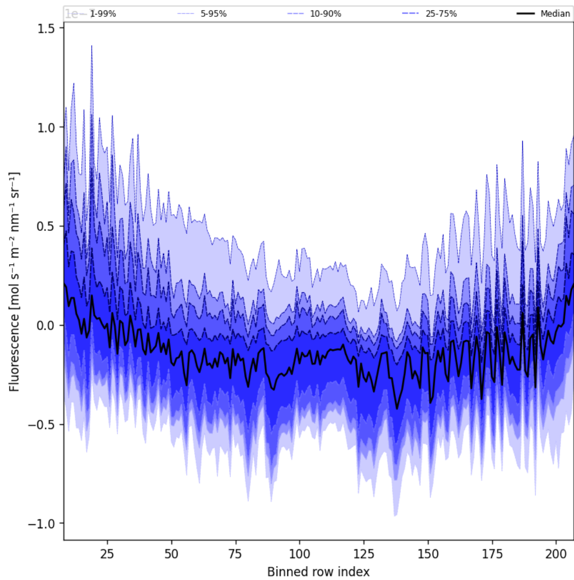
Figure 43: Along track statistics of "Fluorescence" for 2025-11-13 to 2025-11-15
