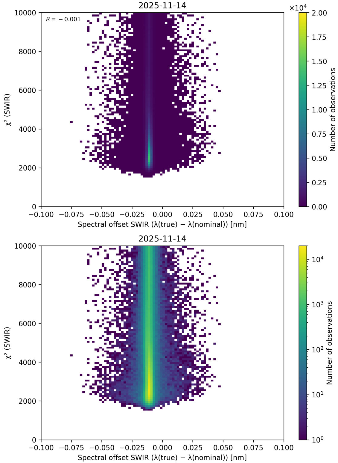
Figure 118: Scatter density plot of “Spectral offset SWIR ( \lambda_{\text{true}} - \lambda_{\text{nominal}} )” against “ \chi^2 (SWIR)” for 2025-11-13 to 2025-11-15.
