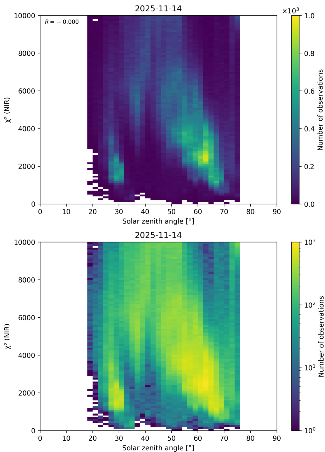
Figure 94: Scatter density plot of “Solar zenith angle” against “ \chi^2 (NIR)” for 2025-11-13 to 2025-11-15.
