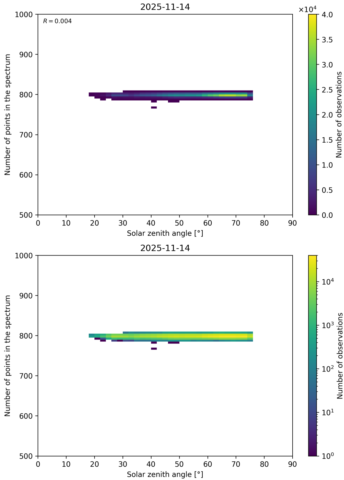
Figure 103: Scatter density plot of “Solar zenith angle” against “Number of points in the spectrum” for 2025-11-13 to 2025-11-15.
