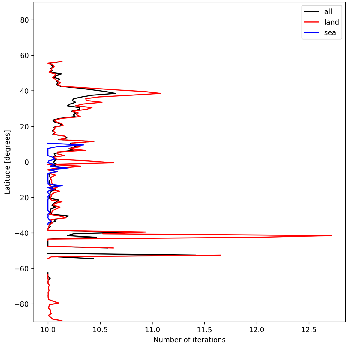
Figure 20: Zonal average of “Number of iterations” for 2025-11-13 to 2025-11-15.
