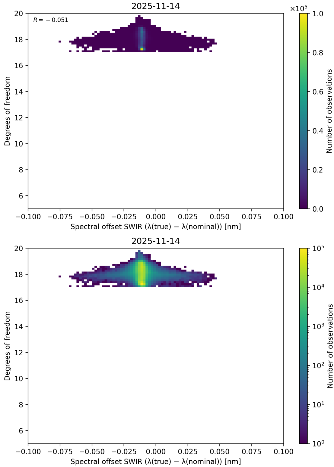
Figure 119: Scatter density plot of “Spectral offset SWIR ( \lambda_{\text{true}} - \lambda_{\text{nominal}} )” against “Degrees of freedom” for 2025-11-13 to 2025-11-15.
