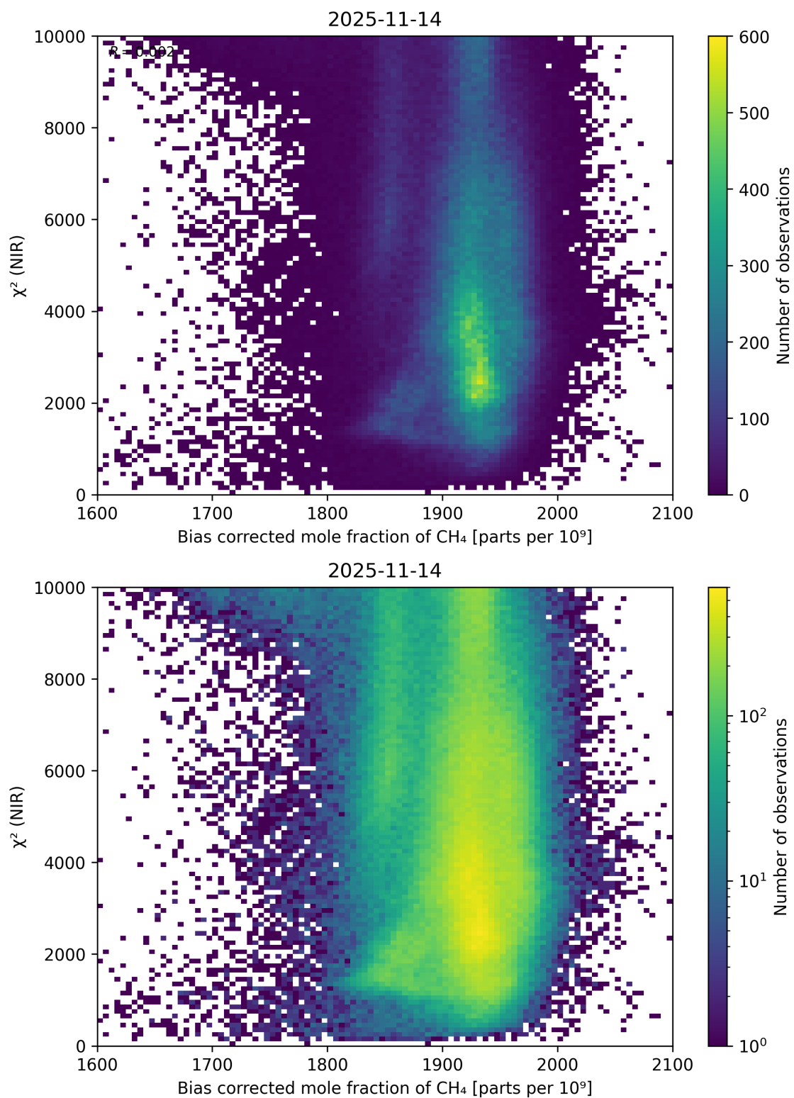
Figure 63: Scatter density plot of “Bias corrected mole fraction of \text{CH}_4 ” against “ \chi^2 (NIR)” for 2025-11-13 to 2025-11-15.
