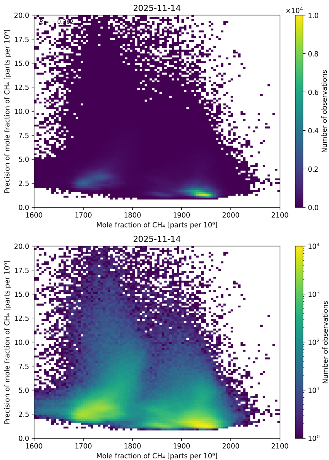
Figure 75: Scatter density plot of “Mole fraction of CH 4 ” against “Precision of mole fraction of CH 4 ” for 2025-11-13 to 2025-11-15.
