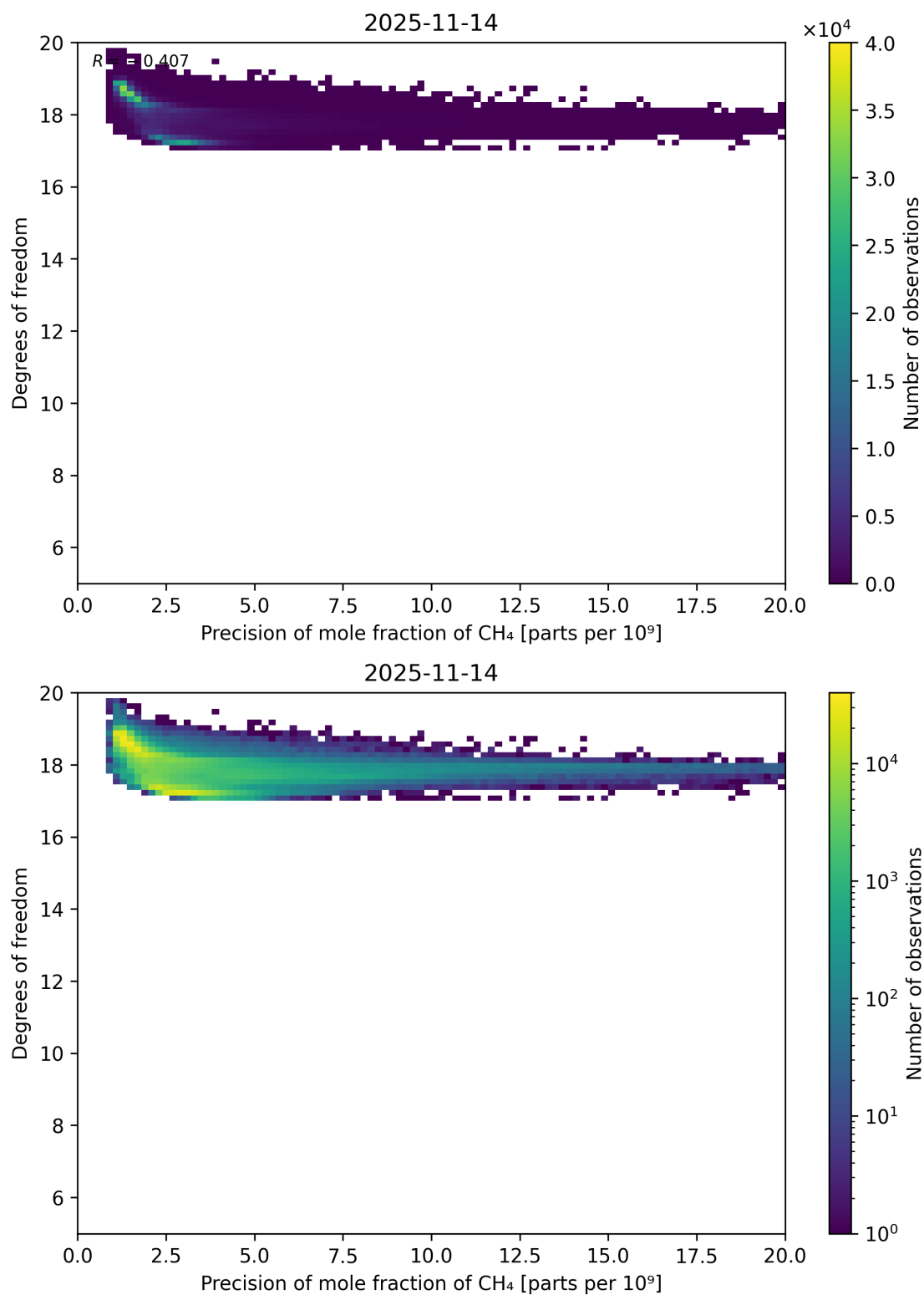
Figure 80: Scatter density plot of “Precision of mole fraction of \text{CH}_4 ” against “Degrees of freedom” for 2025-11-13 to 2025-11-15.
