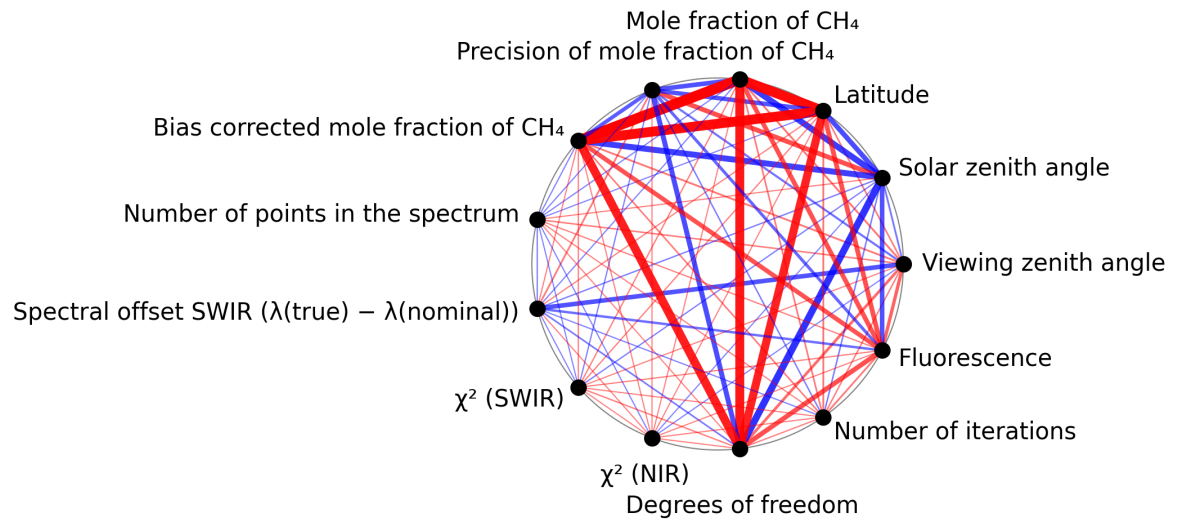
Figure 1: Map of correlation graph for 2025-11-13 to 2025-11-15.
