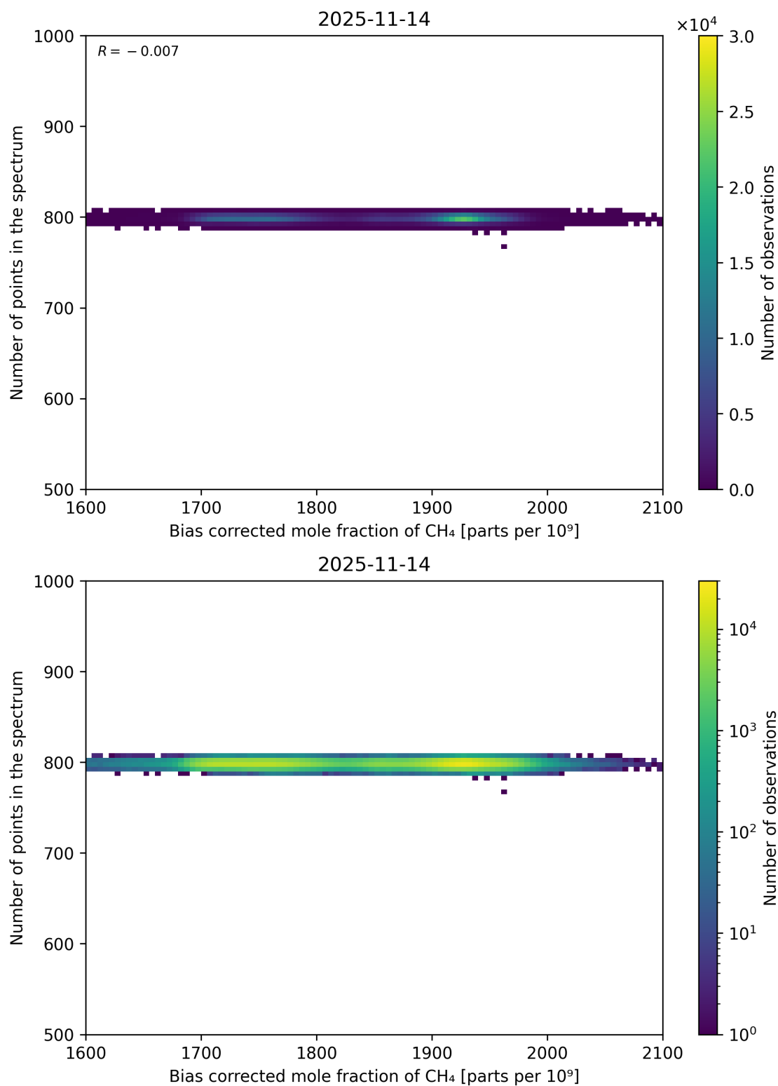
Figure 68: Scatter density plot of “Bias corrected mole fraction of CH 4 ” against “Number of points in the spectrum” for 2025-11-13 to 2025-11-15.
