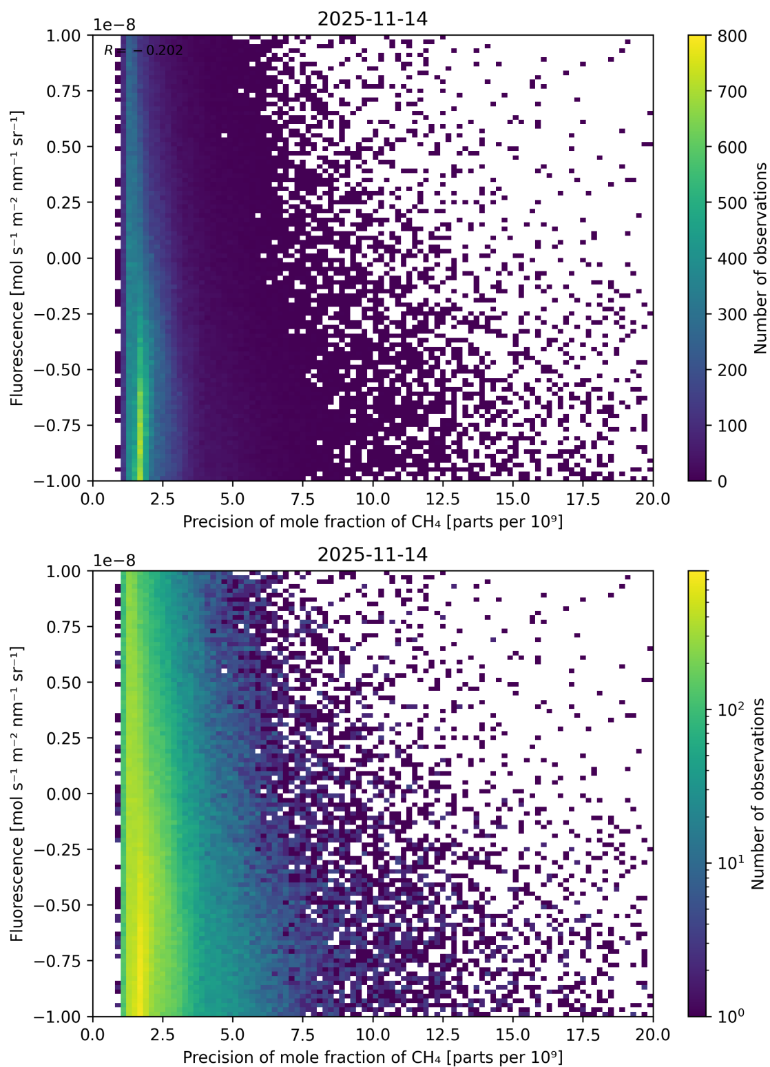
Figure 81: Scatter density plot of “Precision of mole fraction of CH 4 ” against “Fluorescence” for 2025-11-13 to 2025-11-15.
