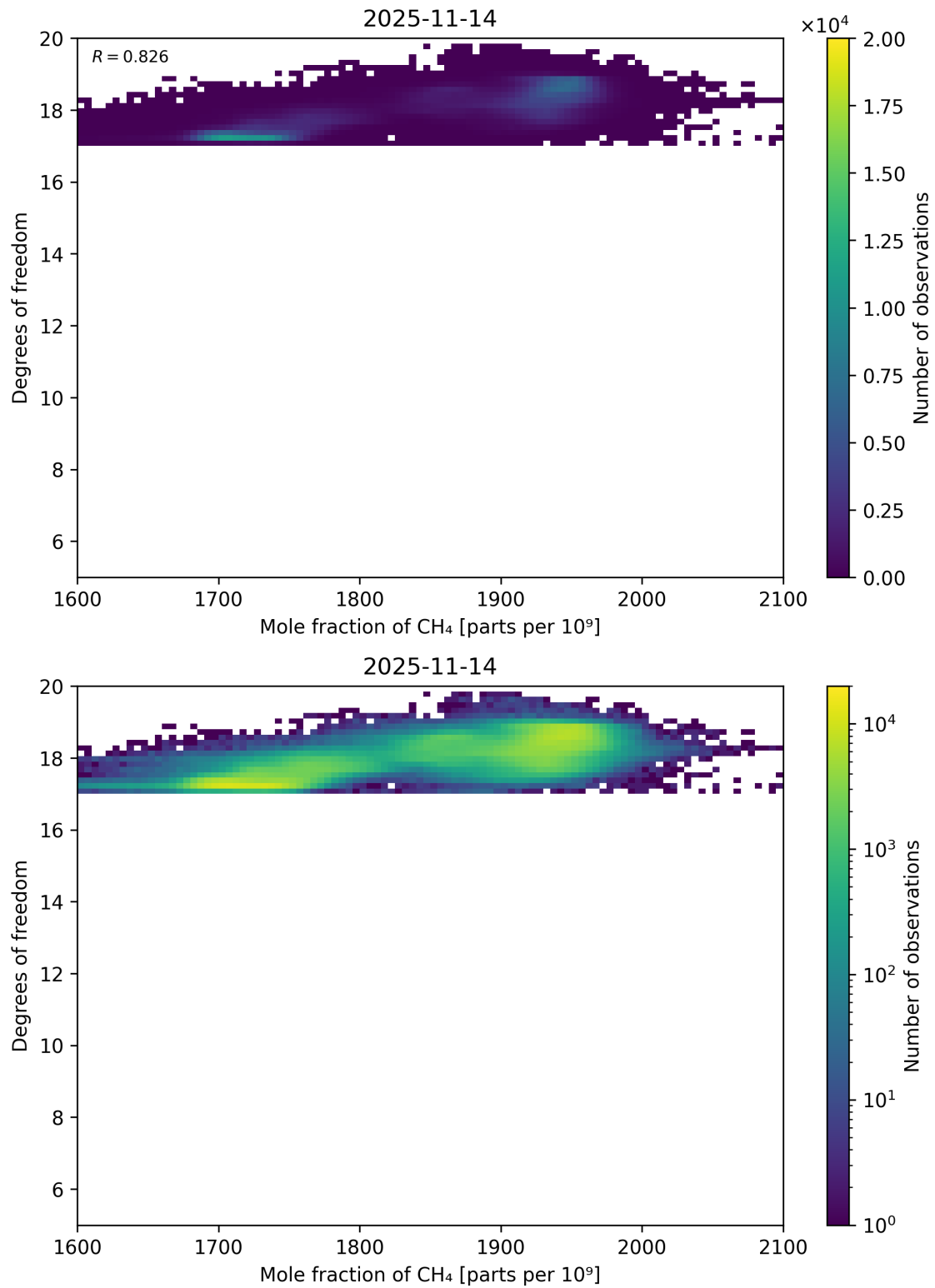
Figure 72: Scatter density plot of “Mole fraction of CH 4 ” against “Degrees of freedom” for 2025-11-13 to 2025-11-15.
