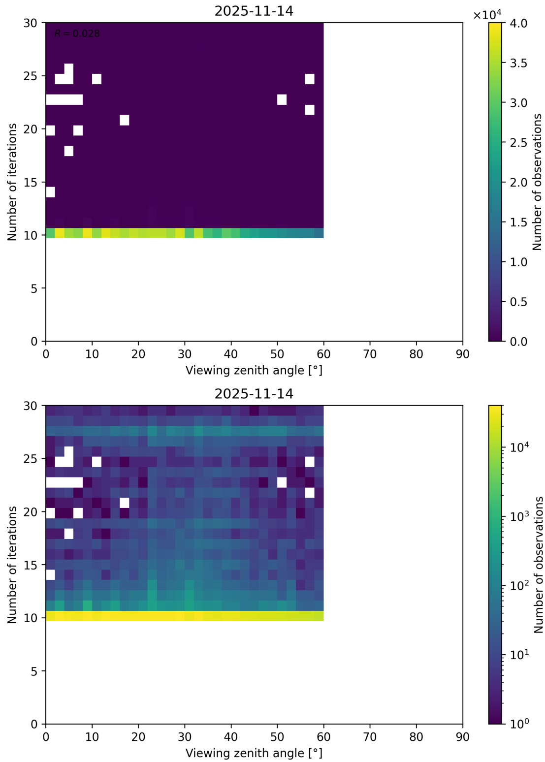
Figure 113: Scatter density plot of “Viewing zenith angle” against “Number of iterations” for 2025-11-13 to 2025-11-15.
