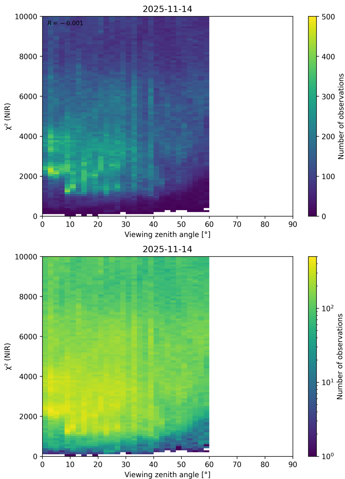
Figure 105: Scatter density plot of “Viewing zenith angle” against “ \chi^2 (NIR)” for 2025-11-13 to 2025-11-15.
