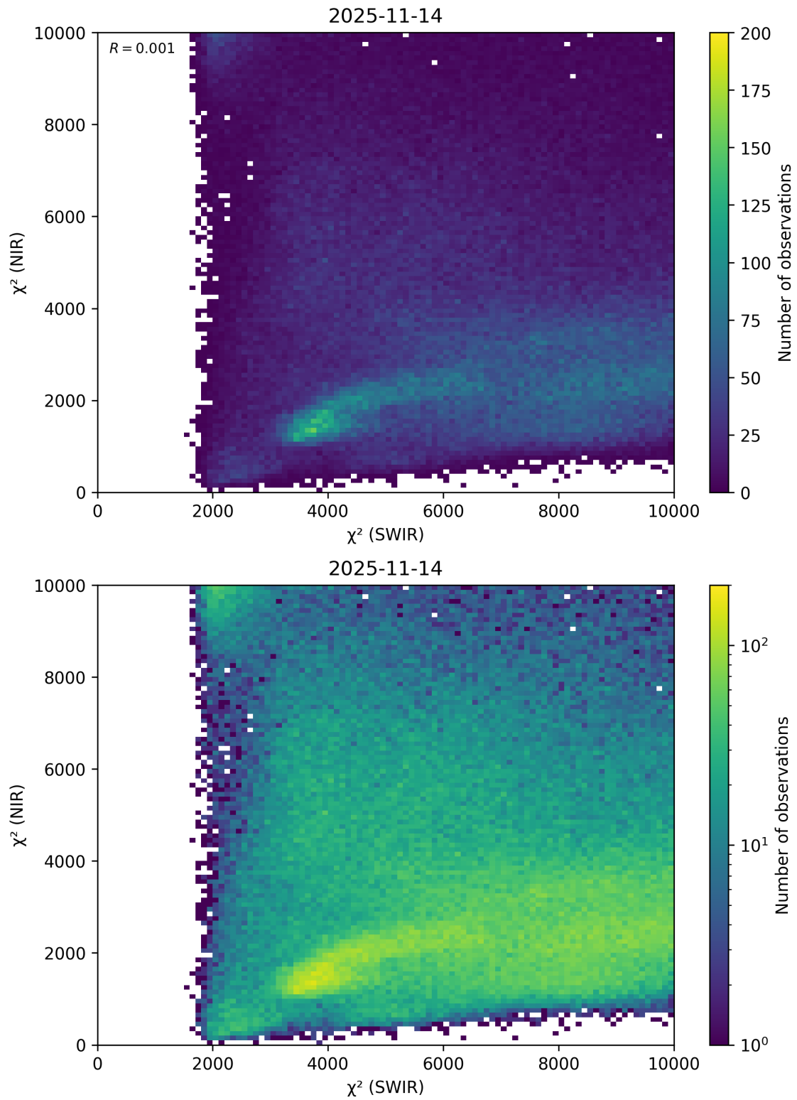
Figure 47: Scatter density plot of “ \chi^2 (SWIR)” against “ \chi^2 (NIR)” for 2025-11-13 to 2025-11-15.
