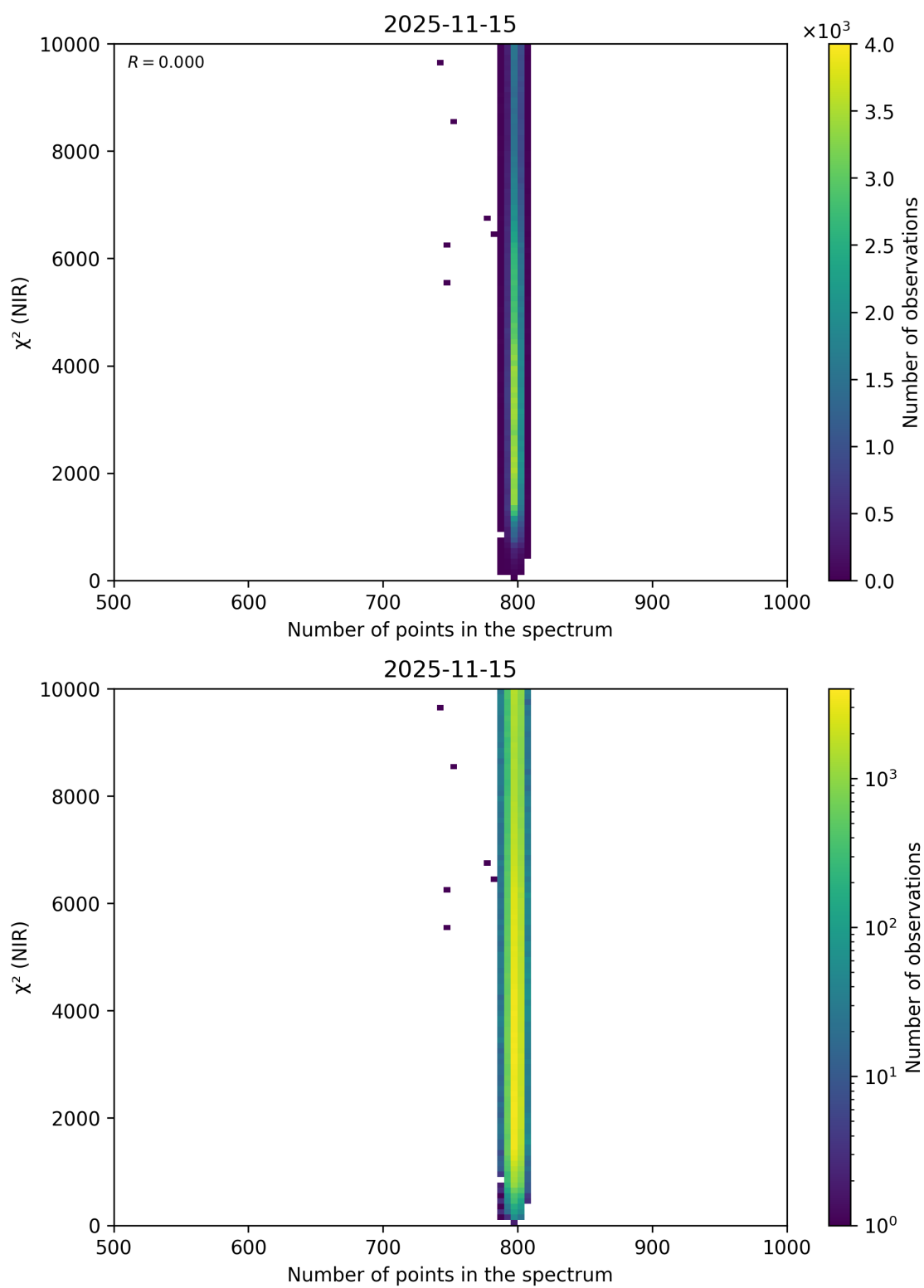
Figure 88: Scatter density plot of “Number of points in the spectrum” against “ \chi^2 (NIR)” for 2025-11-14 to 2025-11-16.
