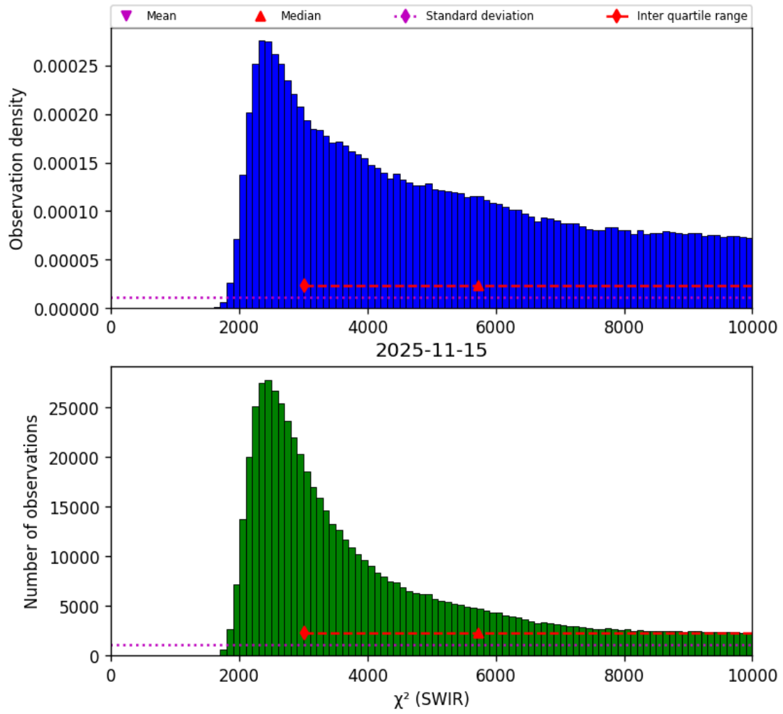
Figure 28: Histogram of “ \chi^2 (SWIR)” for 2025-11-14 to 2025-11-16
