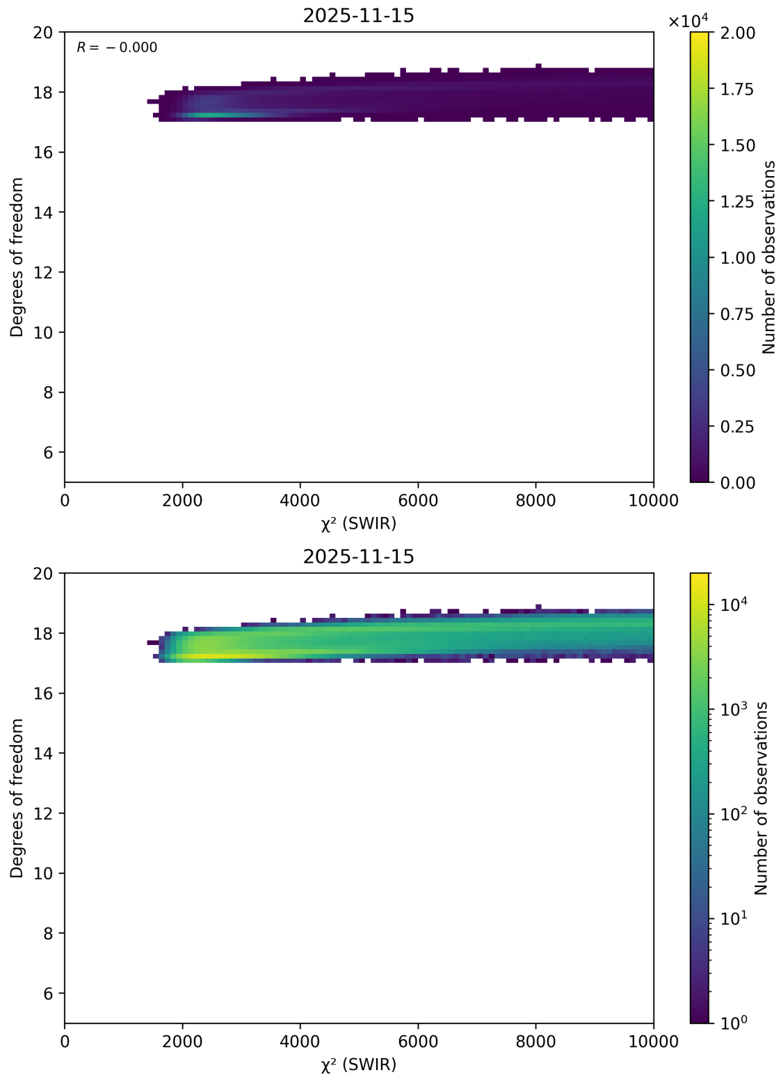
Figure 48: Scatter density plot of “ \chi^2 (SWIR)” against “Degrees of freedom” for 2025-11-14 to 2025-11-16.
