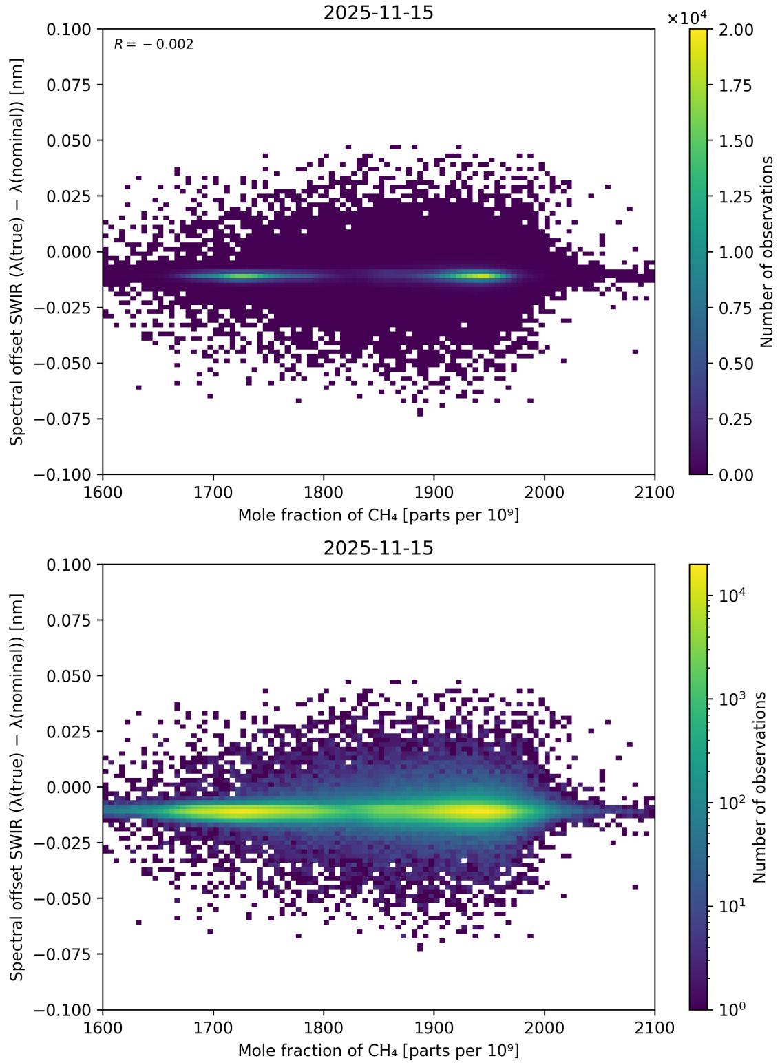
Figure 86: Scatter density plot of “Mole fraction of CH 4 ” against “Spectral offset SWIR ( \lambda_{\text{true}} - \lambda_{\text{nominal}} )” for 2025-11-14 to 2025-11-16.
