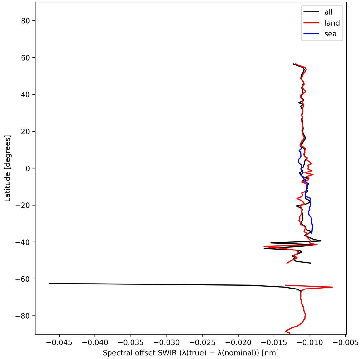
Figure 16: Zonal average of “Spectral offset SWIR ( \lambda_{\text{true}} - \lambda_{\text{nominal}} )” for 2025-11-14 to 2025-11-16.
