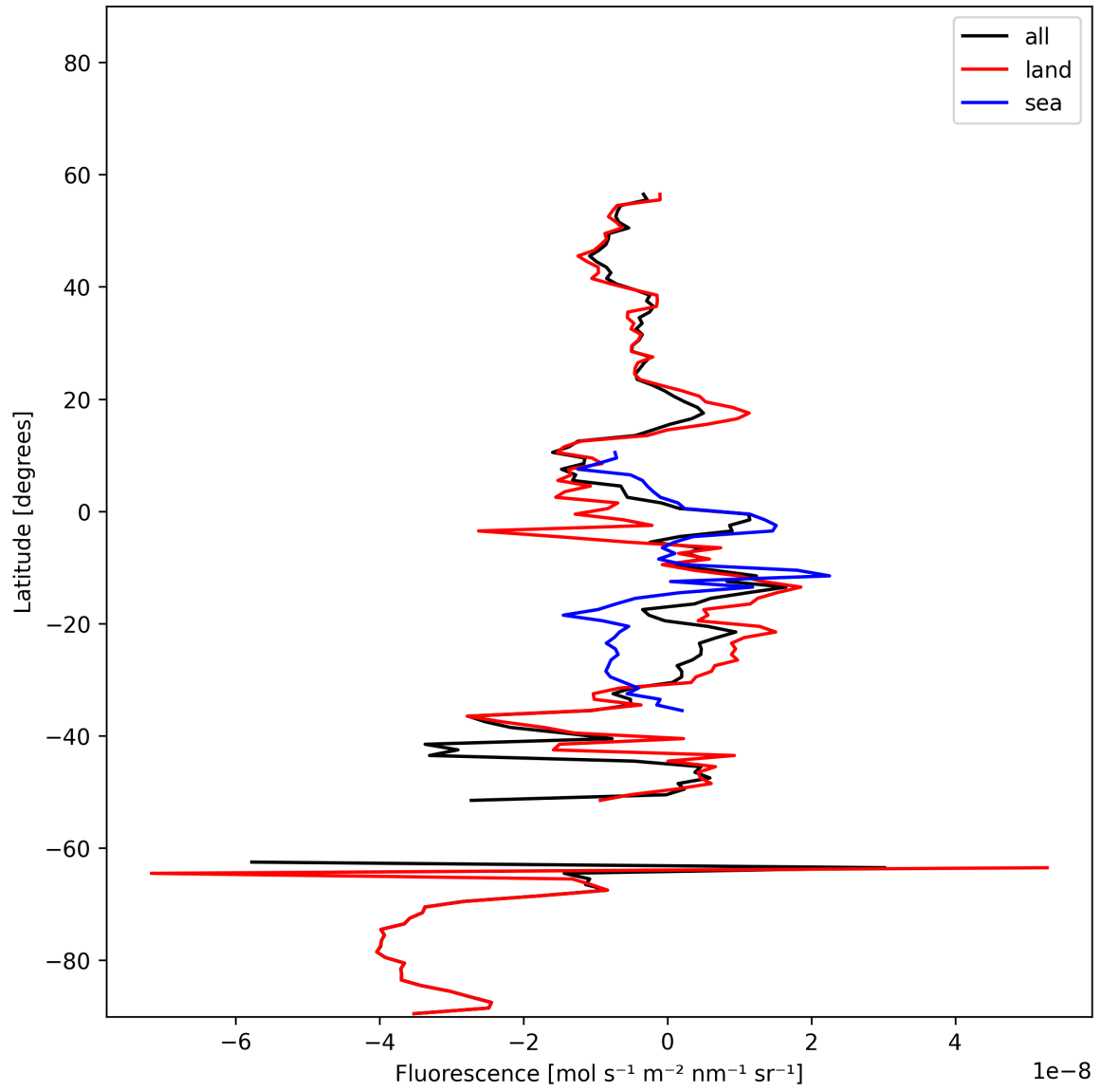
Figure 21: Zonal average of “Fluorescence” for 2025-11-14 to 2025-11-16.
