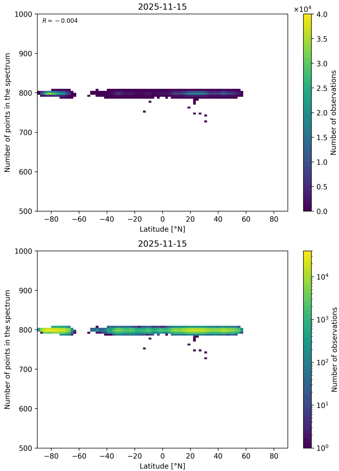
Figure 61: Scatter density plot of “Latitude” against “Number of points in the spectrum” for 2025-11-14 to 2025-11-16.
