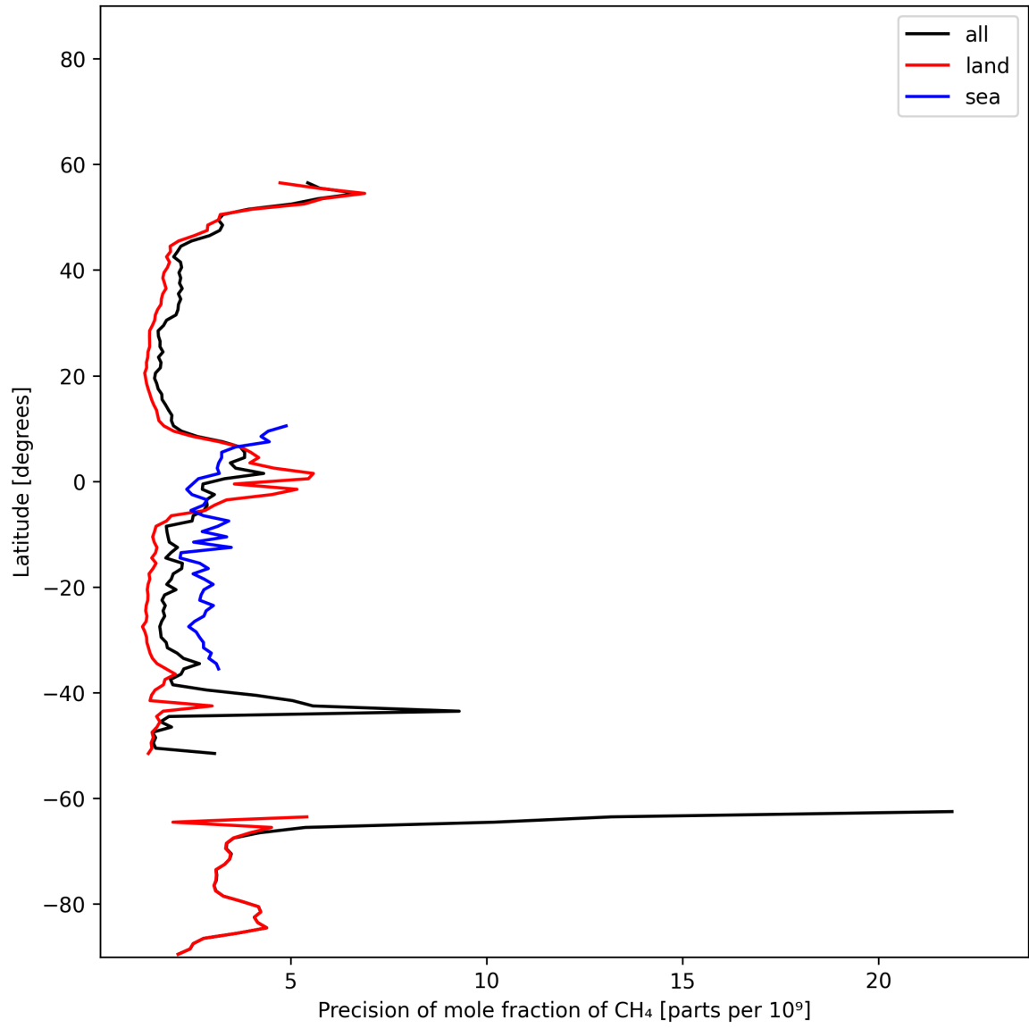
Figure 13: Zonal average of “Precision of mole fraction of CH 4 ” for 2025-11-14 to 2025-11-16.
