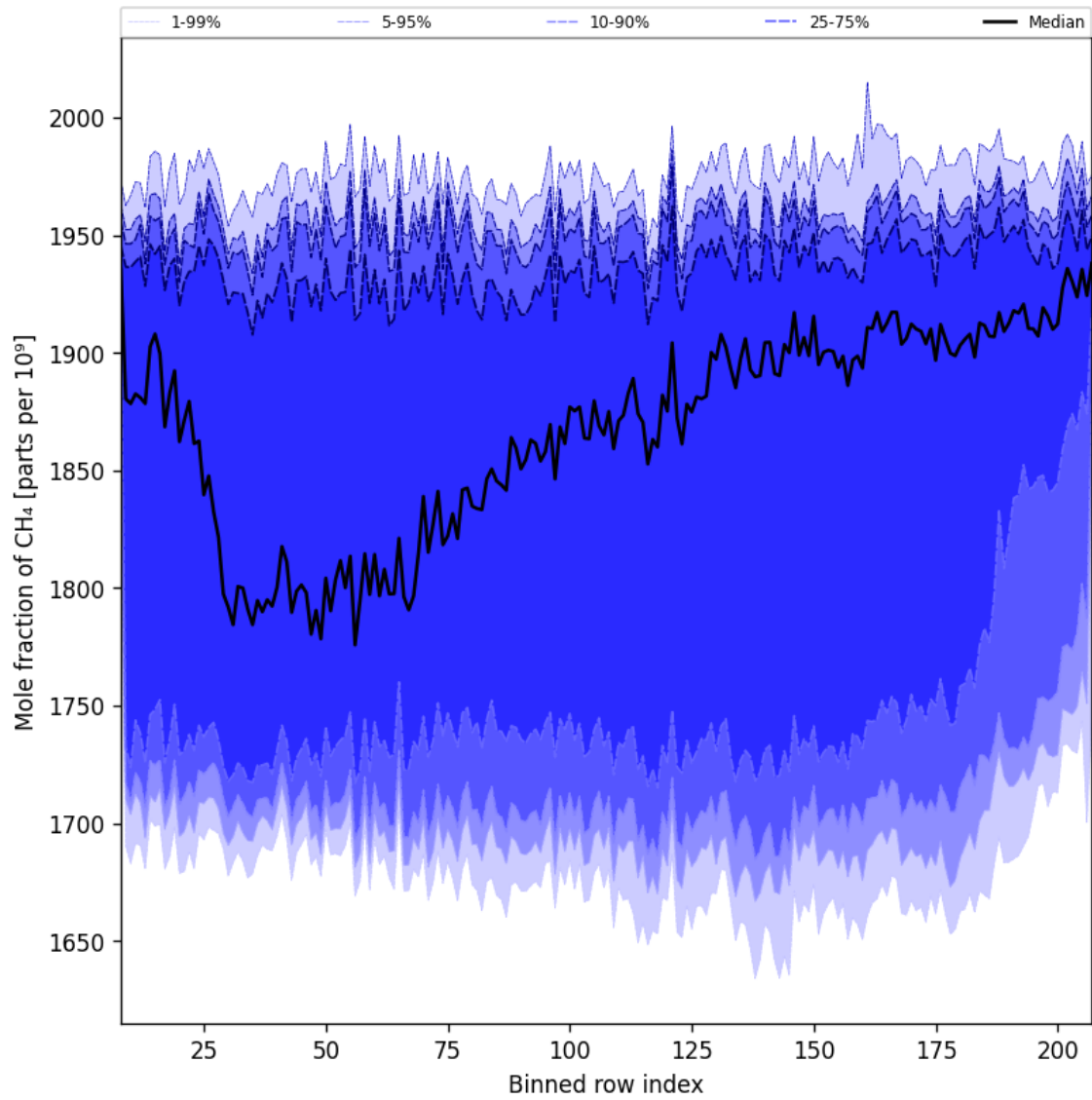
Figure 34: Along track statistics of “Mole fraction of CH 4 ” for 2025-11-14 to 2025-11-16
