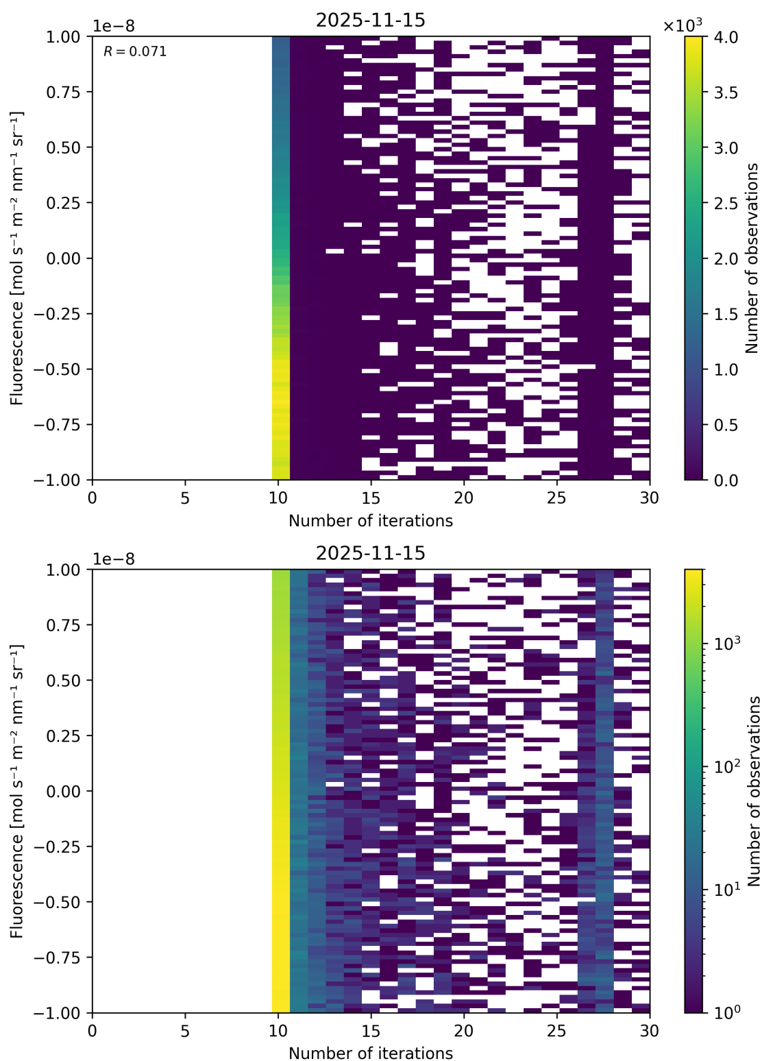
Figure 87: Scatter density plot of “Number of iterations” against “Fluorescence” for 2025-11-14 to 2025-11-16.
