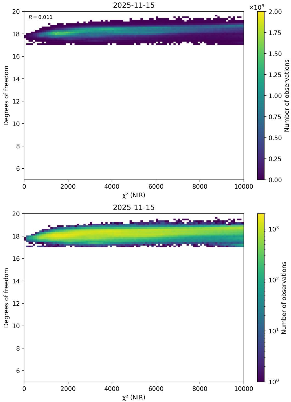
Figure 44: Scatter density plot of “ \chi^2 (NIR)” against “Degrees of freedom” for 2025-11-14 to 2025-11-16.
