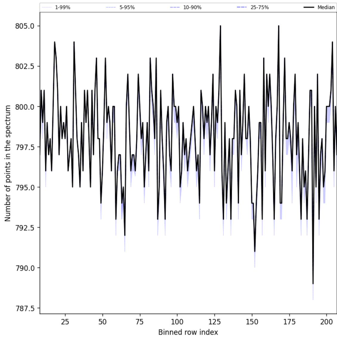
Figure 37: Along track statistics of “Number of points in the spectrum” for 2025-11-14 to 2025-11-16
