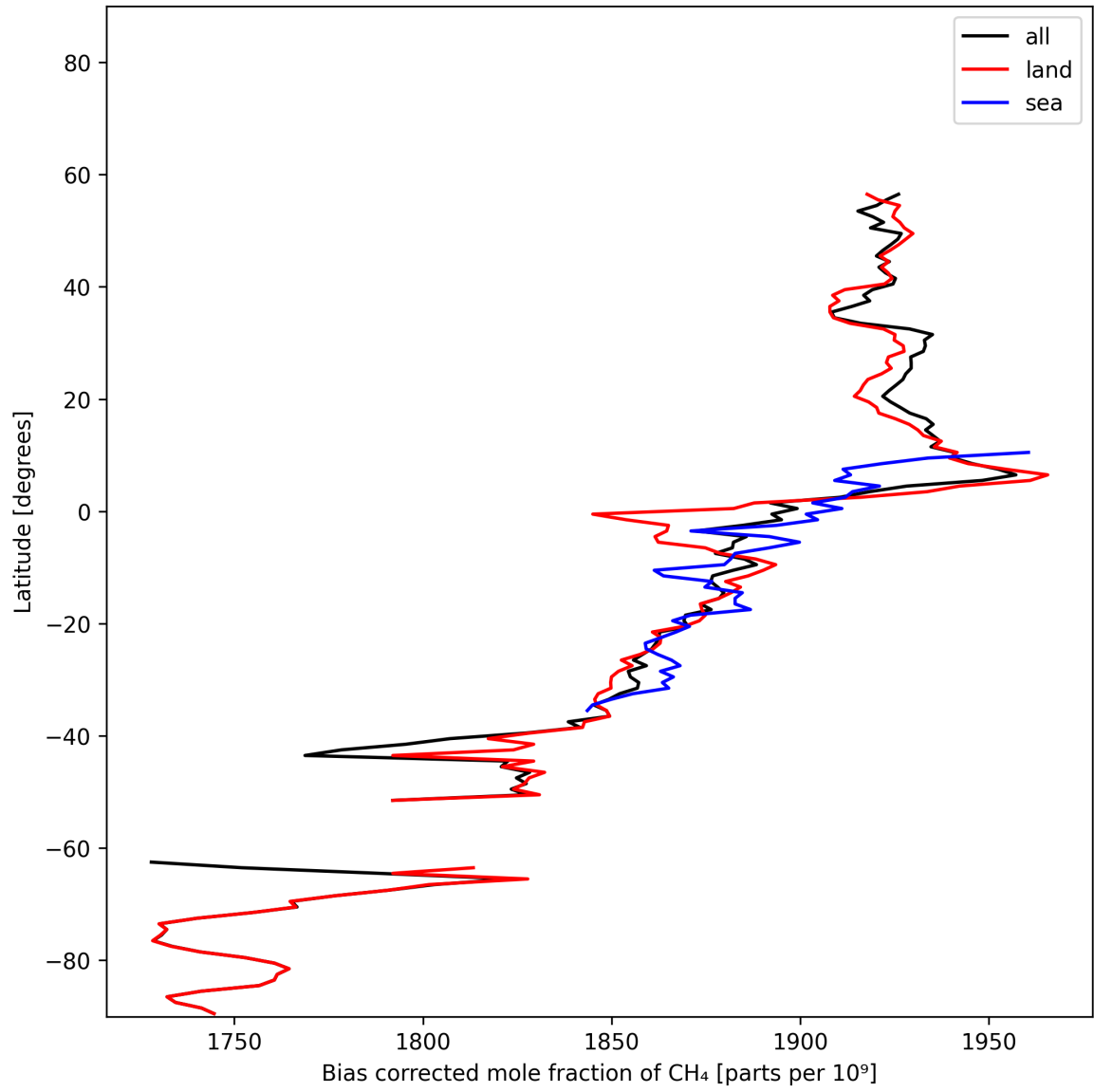
Figure 14: Zonal average of “Bias corrected mole fraction of CH 4 ” for 2025-11-14 to 2025-11-16.
