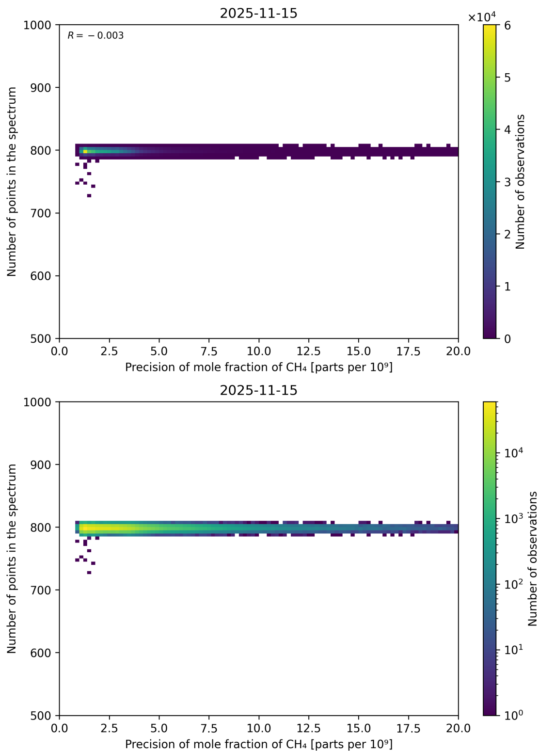
Figure 84: Scatter density plot of “Precision of mole fraction of CH 4 ” against “Number of points in the spectrum” for 2025-11-14 to 2025-11-16.
