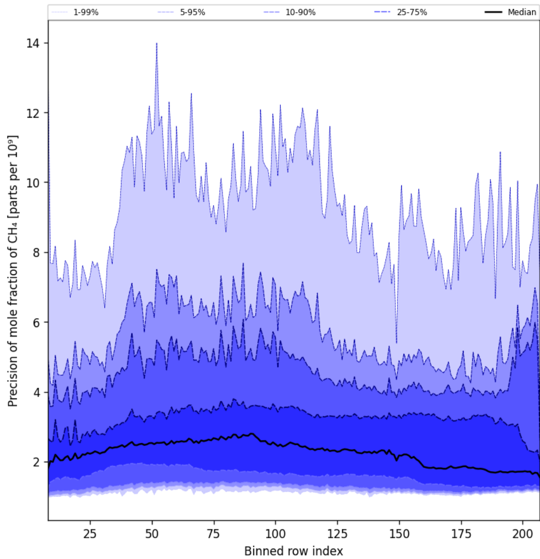
Figure 35: Along track statistics of “Precision of mole fraction of CH 4 ” for 2025-11-14 to 2025-11-16
