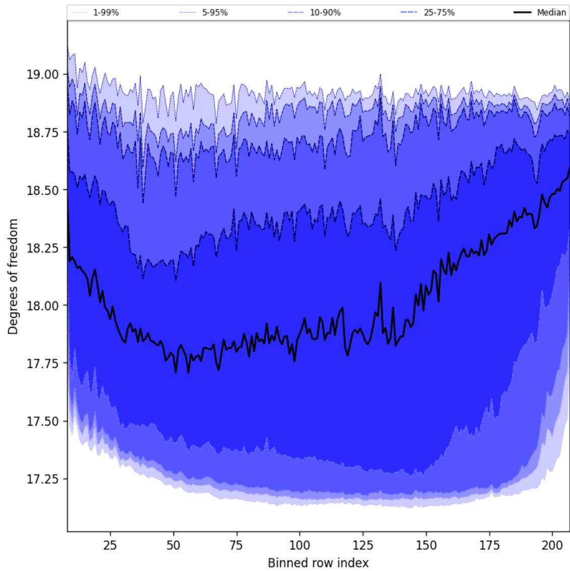
Figure 41: Along track statistics of “Degrees of freedom” for 2025-11-14 to 2025-11-16
