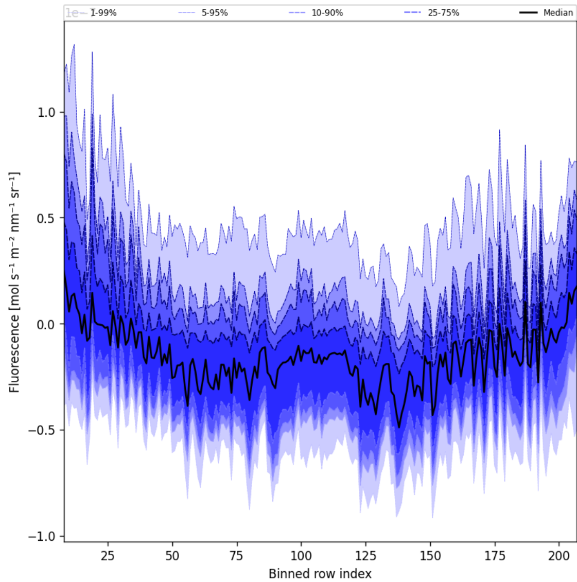
Figure 43: Along track statistics of “Fluorescence” for 2025-11-14 to 2025-11-16
