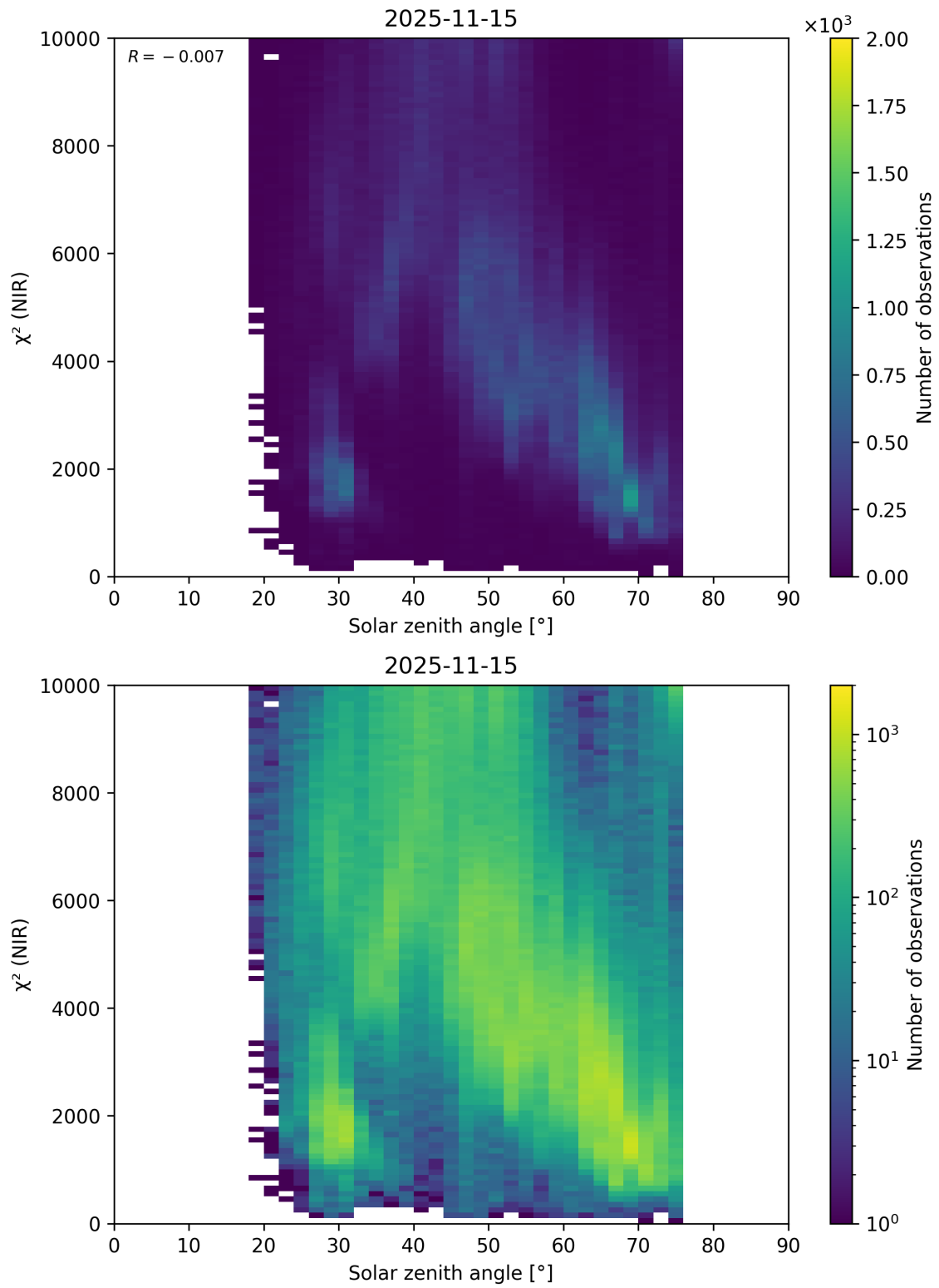
Figure 94: Scatter density plot of “Solar zenith angle” against “ \chi^2 (NIR)” for 2025-11-14 to 2025-11-16.
