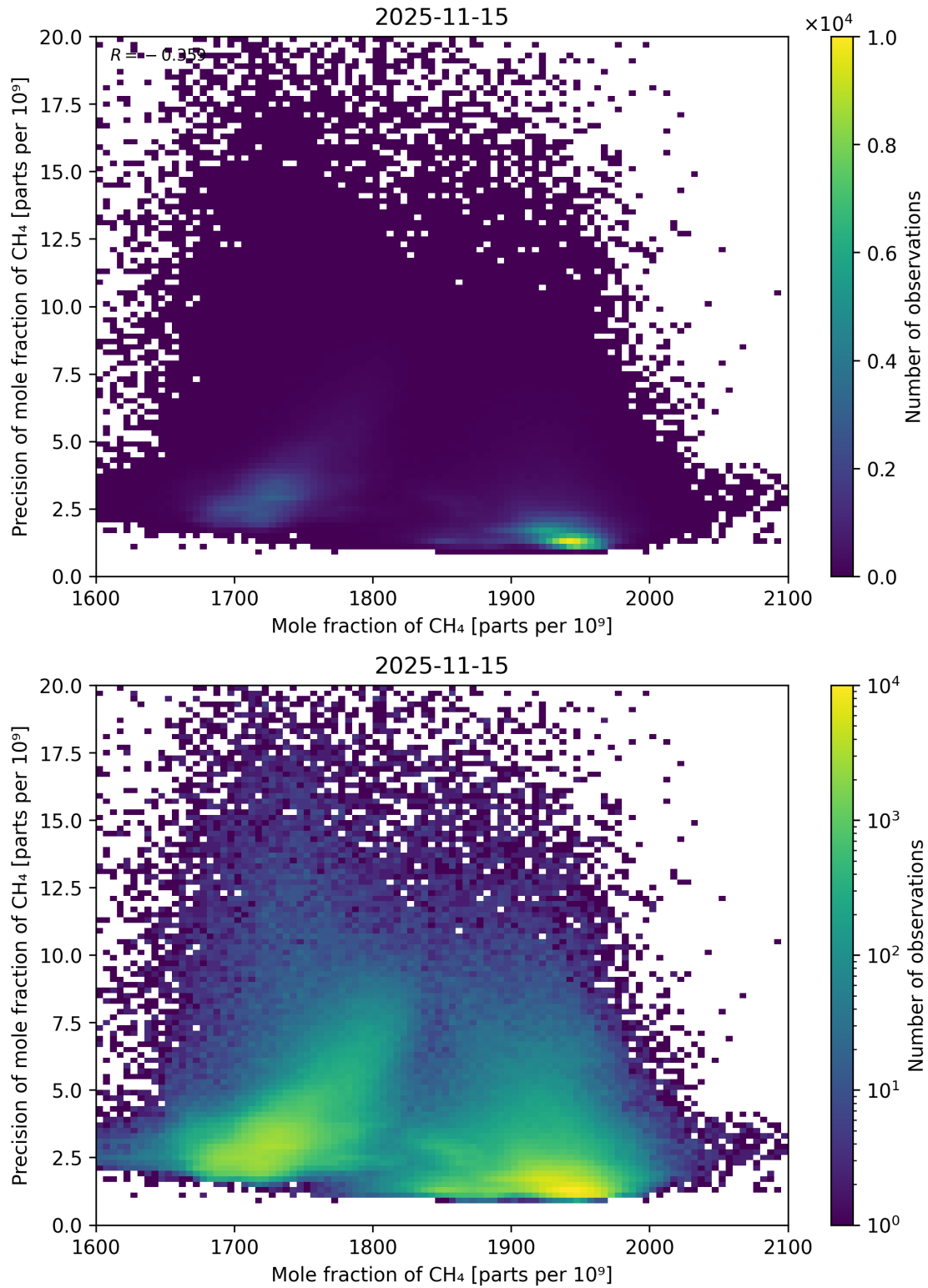
Figure 75: Scatter density plot of “Mole fraction of CH 4 ” against “Precision of mole fraction of CH 4 ” for 2025-11-14 to 2025-11-16.
