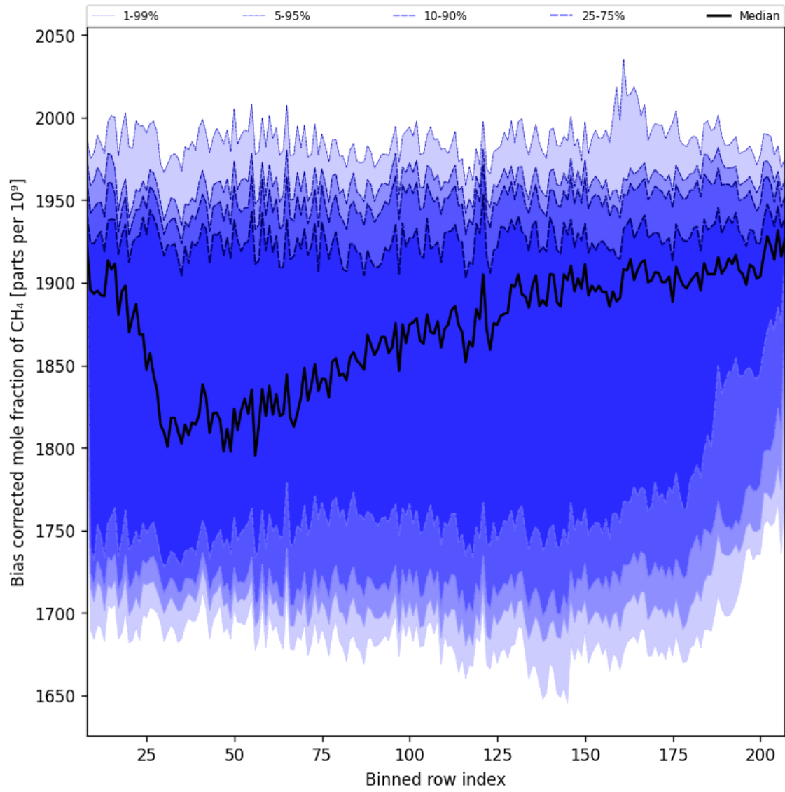
Figure 36: Along track statistics of “Bias corrected mole fraction of CH 4 ” for 2025-11-14 to 2025-11-16
