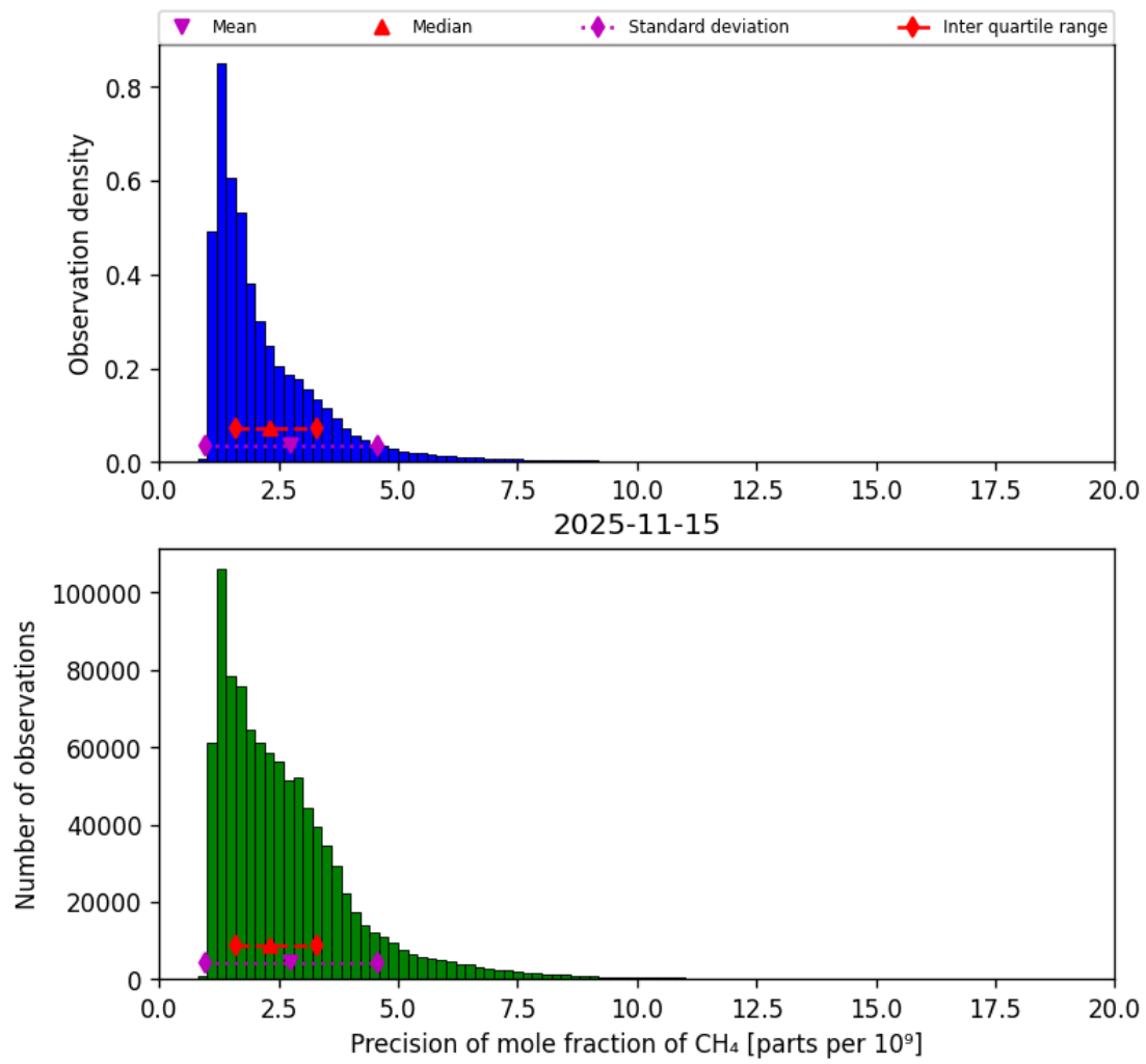
Figure 24: Histogram of “Precision of mole fraction of CH 4 ” for 2025-11-14 to 2025-11-16
