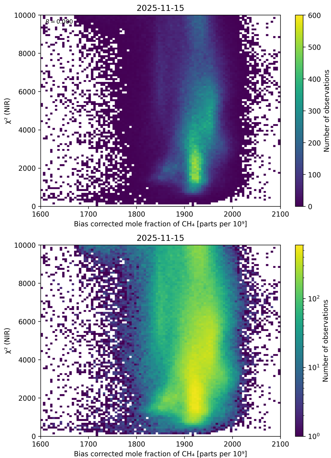
Figure 63: Scatter density plot of “Bias corrected mole fraction of \text{CH}_4 ” against “ \chi^2 (NIR)” for 2025-11-14 to 2025-11-16.
