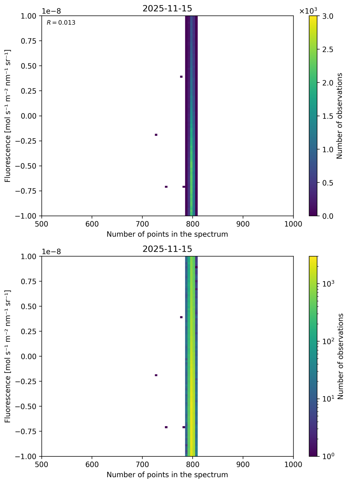
Figure 91: Scatter density plot of “Number of points in the spectrum” against “Fluorescence” for 2025-11-14 to 2025-11-16.
