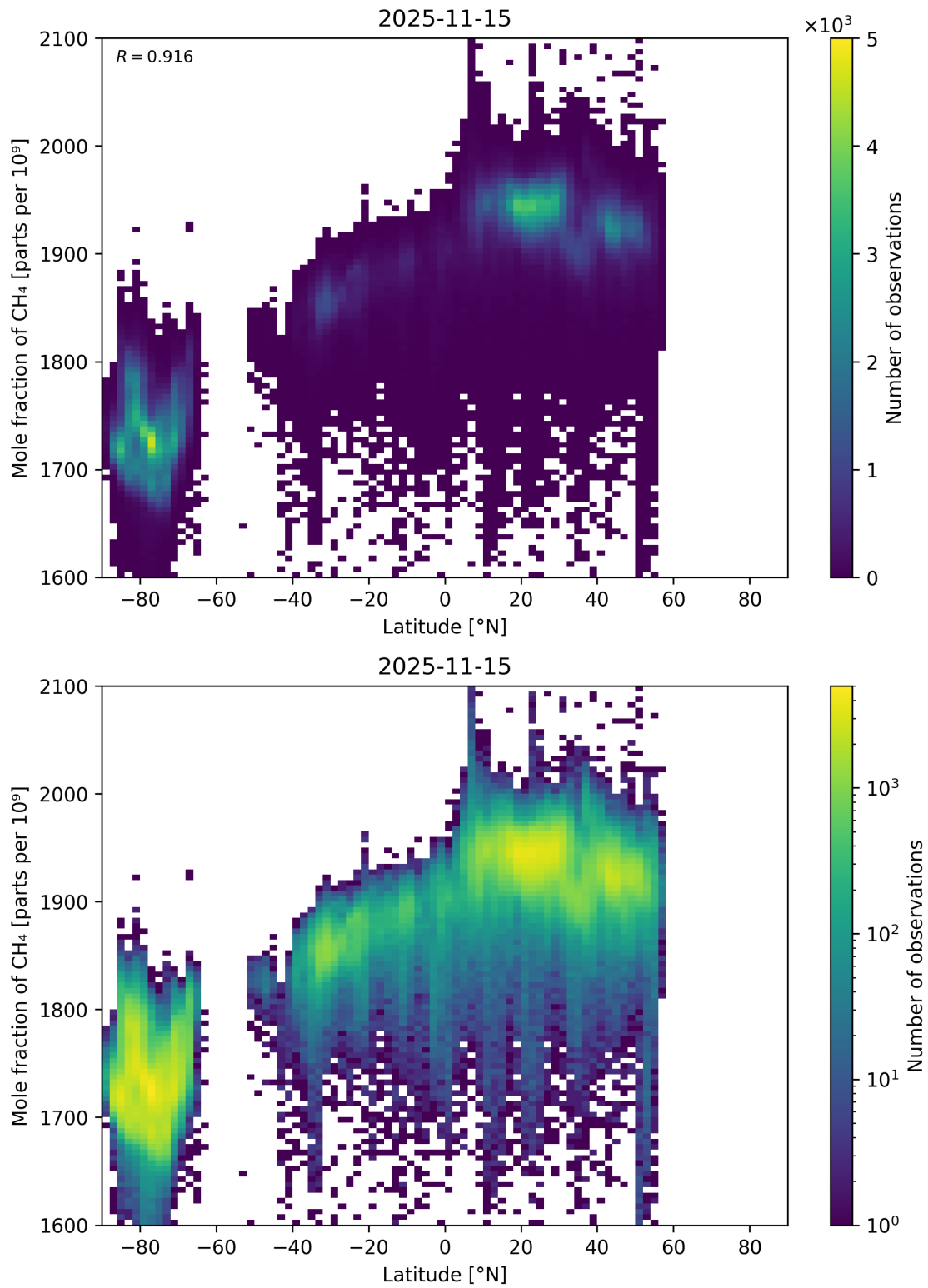
Figure 57: Scatter density plot of “Latitude” against “Mole fraction of \text{CH}_4 ” for 2025-11-14 to 2025-11-16.
