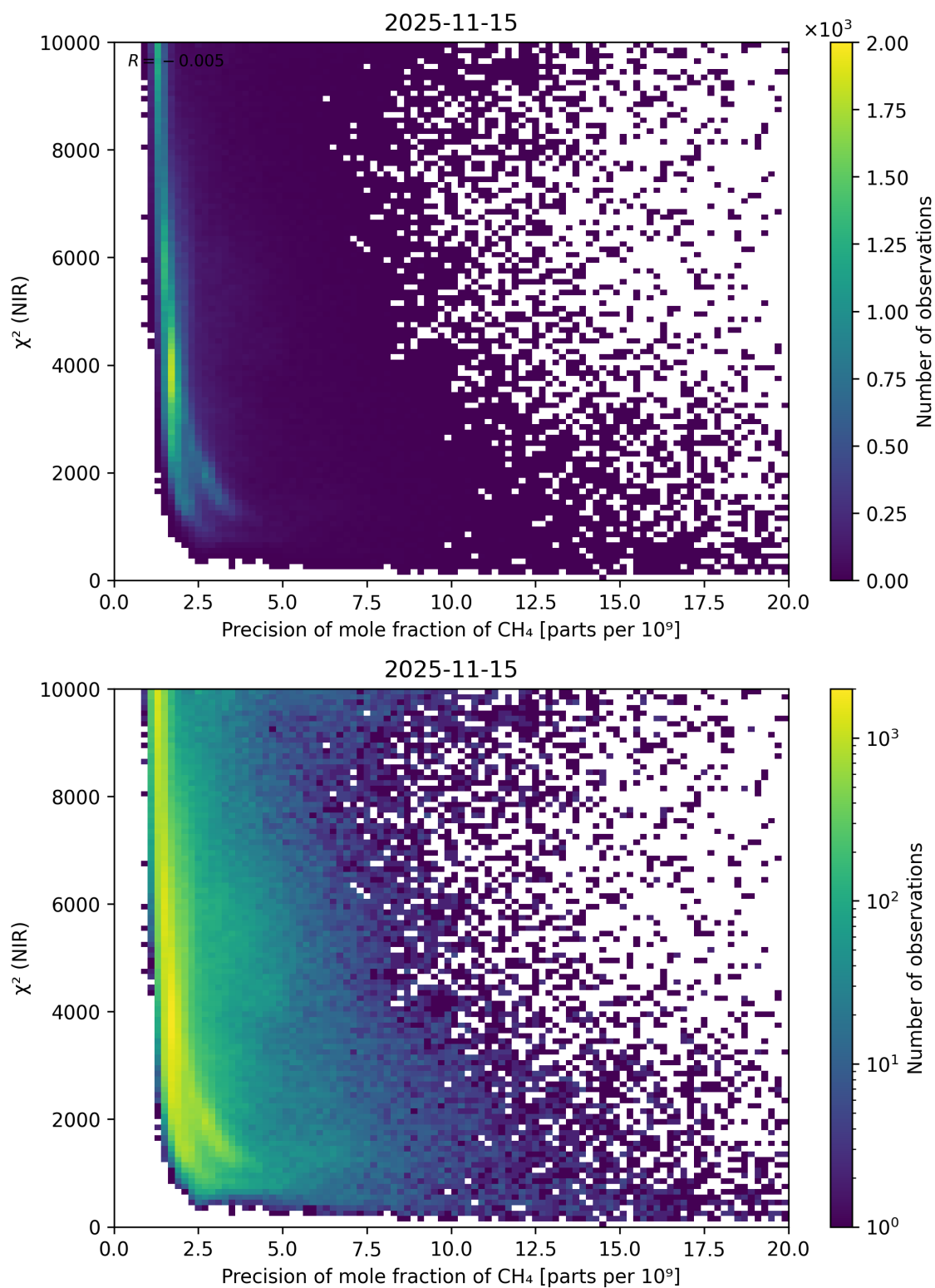
Figure 78: Scatter density plot of “Precision of mole fraction of CH 4 ” against “ \chi^2 (NIR)” for 2025-11-14 to 2025-11-16.
