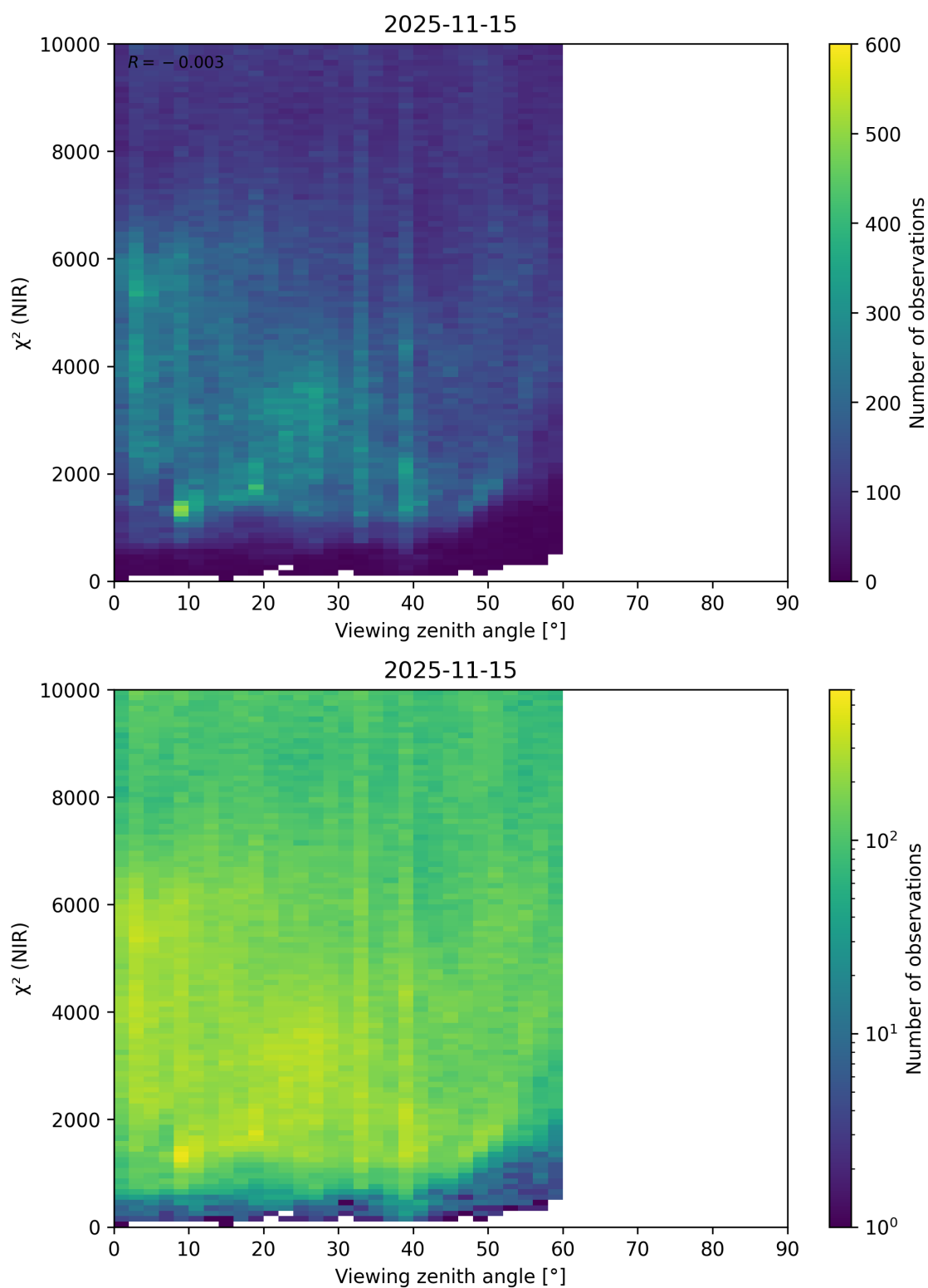
Figure 105: Scatter density plot of “Viewing zenith angle” against “ \chi^2 (NIR)” for 2025-11-14 to 2025-11-16.
