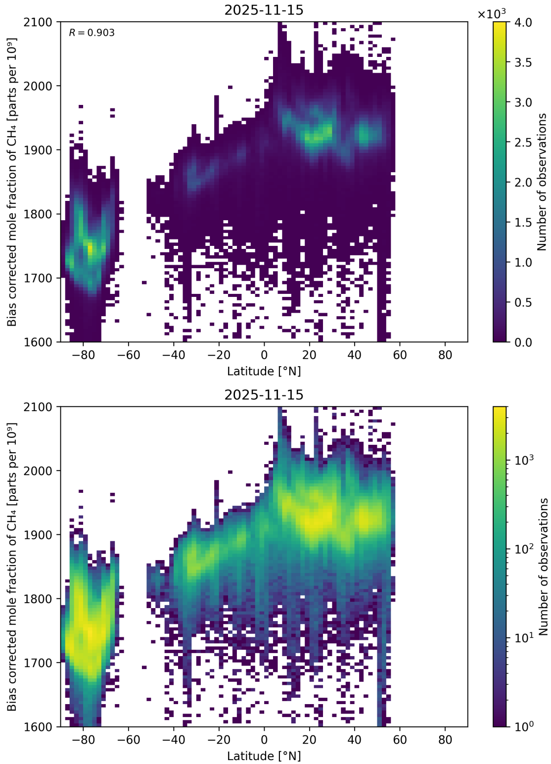
Figure 58: Scatter density plot of “Latitude” against “Bias corrected mole fraction of CH 4 ” for 2025-11-14 to 2025-11-16.
