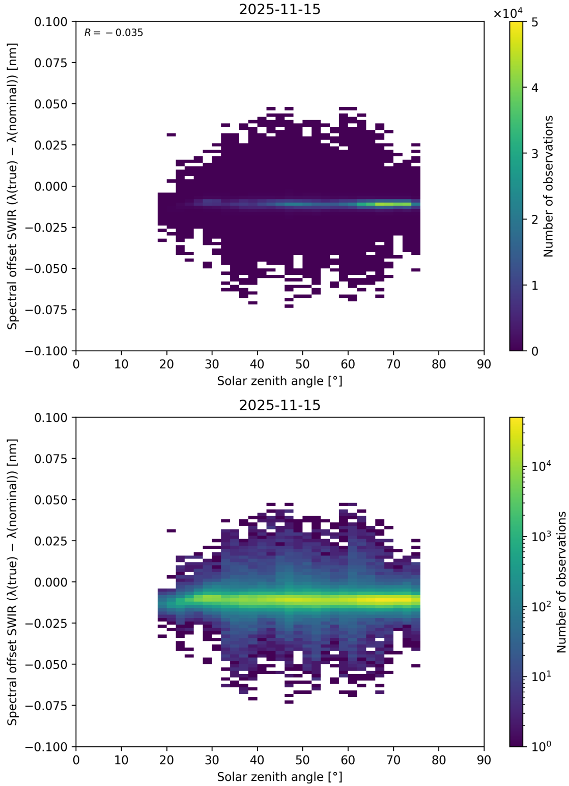
Figure 104: Scatter density plot of “Solar zenith angle” against “Spectral offset SWIR ( \lambda_{\text{true}} - \lambda_{\text{nominal}} )” for 2025-11-14 to 2025-11-16.
