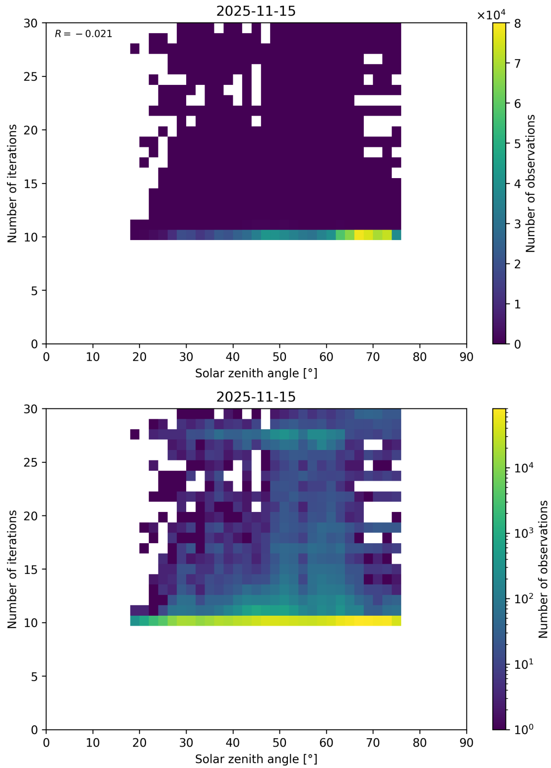
Figure 102: Scatter density plot of “Solar zenith angle” against “Number of iterations” for 2025-11-14 to 2025-11-16.
