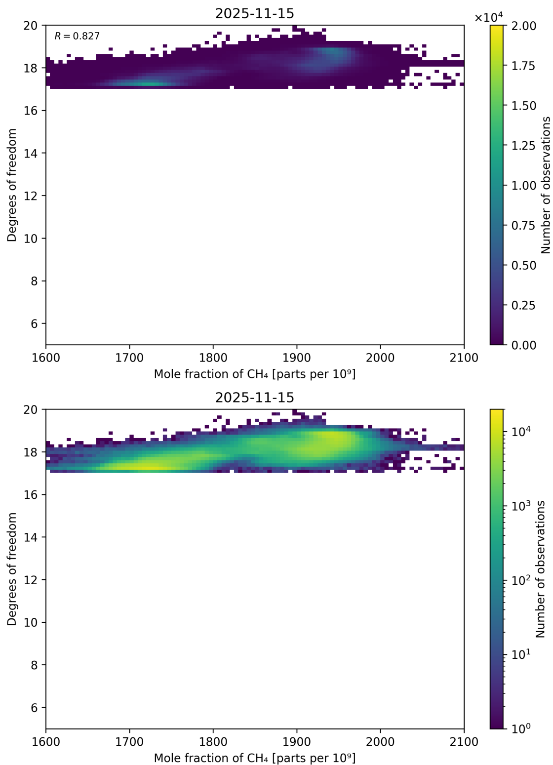
Figure 72: Scatter density plot of “Mole fraction of CH 4 ” against “Degrees of freedom” for 2025-11-14 to 2025-11-16.
