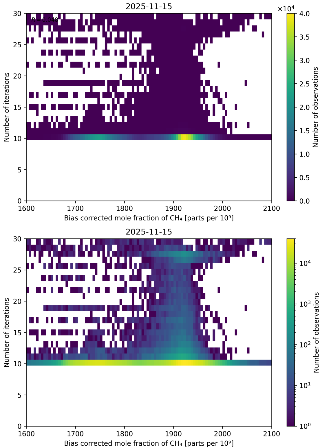
Figure 67: Scatter density plot of “Bias corrected mole fraction of \text{CH}_4 ” against “Number of iterations” for 2025-11-14 to 2025-11-16.
