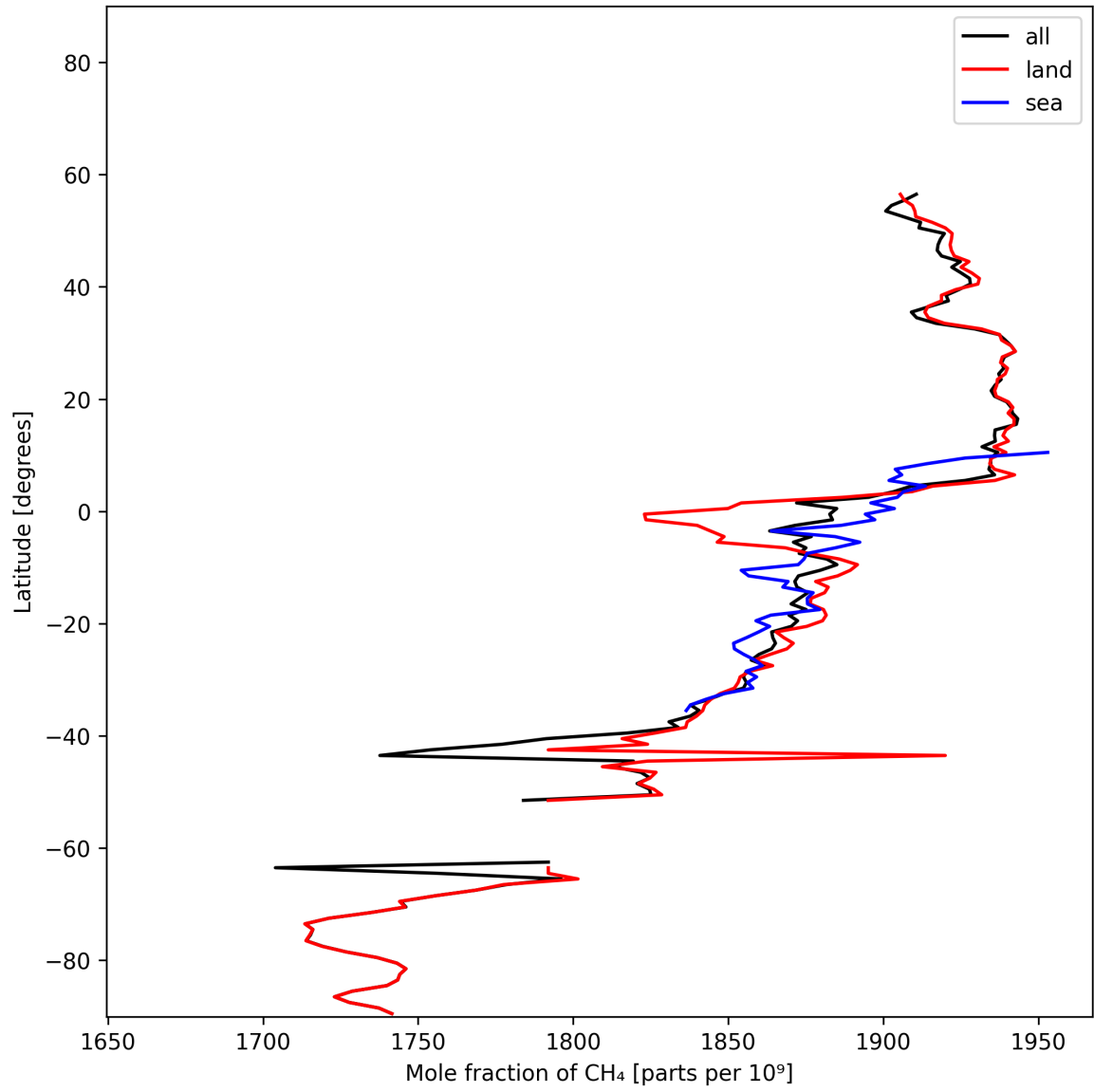
Figure 12: Zonal average of “Mole fraction of CH 4 ” for 2025-11-14 to 2025-11-16.
