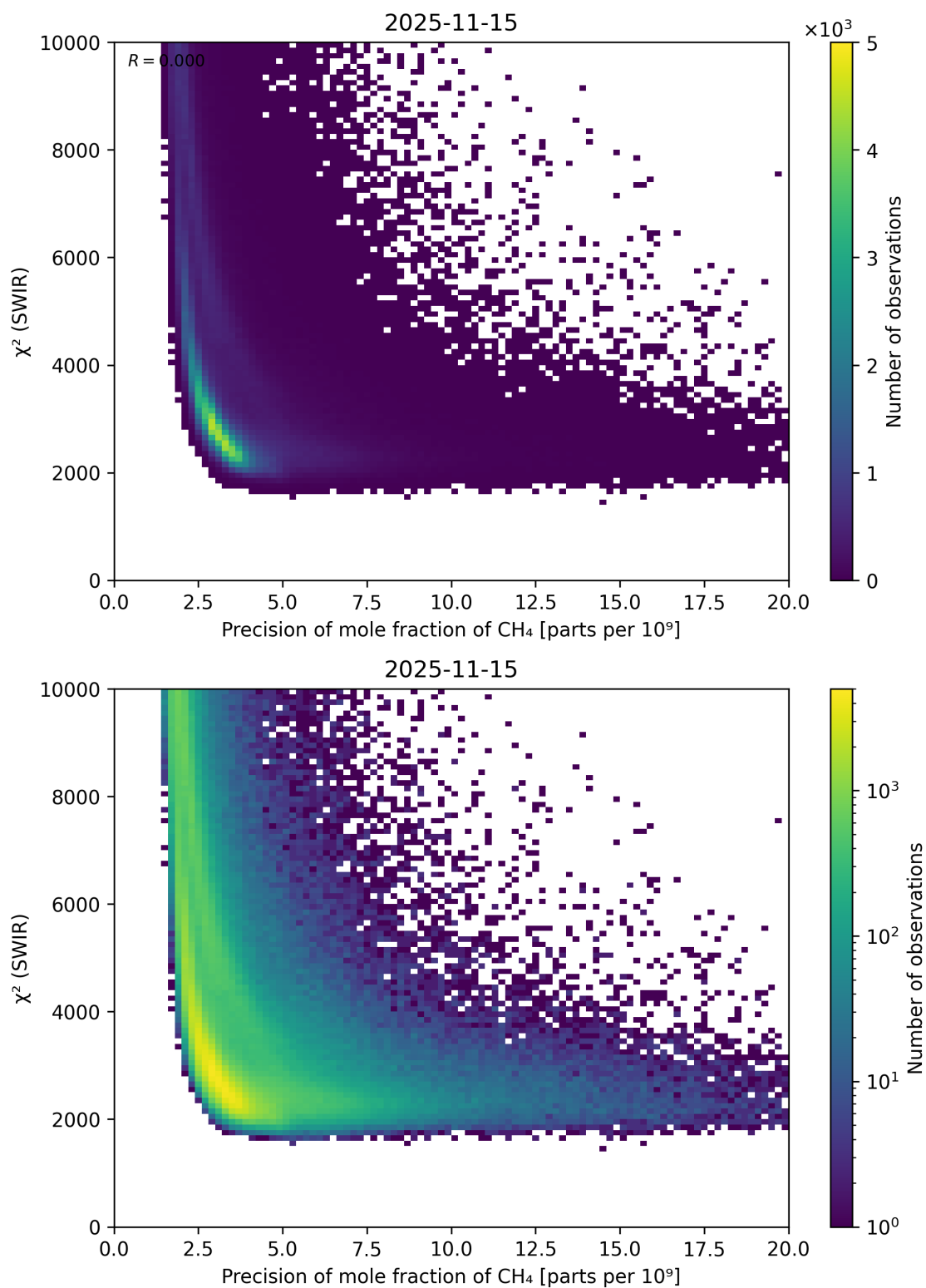
Figure 79: Scatter density plot of “Precision of mole fraction of CH 4 ” against “ \chi^2 (SWIR)” for 2025-11-14 to 2025-11-16.
