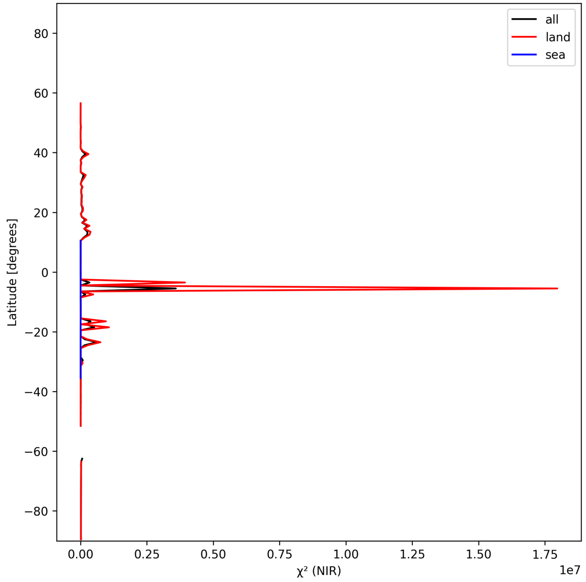
Figure 18: Zonal average of “ \chi^2 (NIR)” for 2025-11-14 to 2025-11-16.
