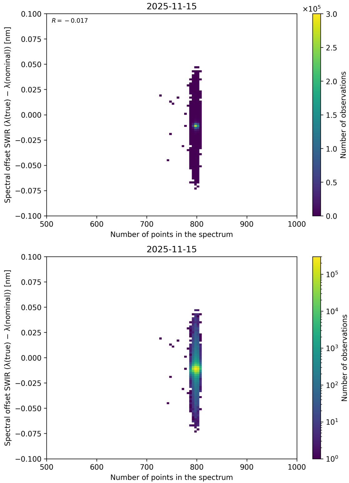
Figure 93: Scatter density plot of “Number of points in the spectrum” against “Spectral offset SWIR ( \lambda_{\text{true}} - \lambda_{\text{nominal}} )” for 2025-11-14 to 2025-11-16.
