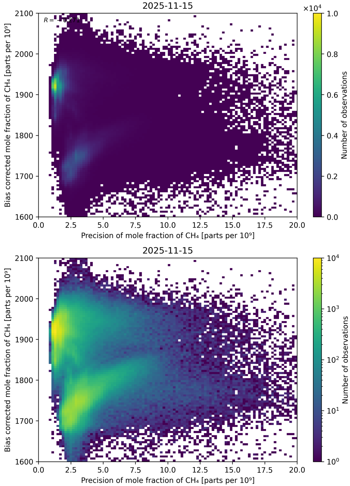
Figure 82: Scatter density plot of “Precision of mole fraction of \text{CH}_4 ” against “Bias corrected mole fraction of \text{CH}_4 ” for 2025-11-14 to 2025-11-16.
