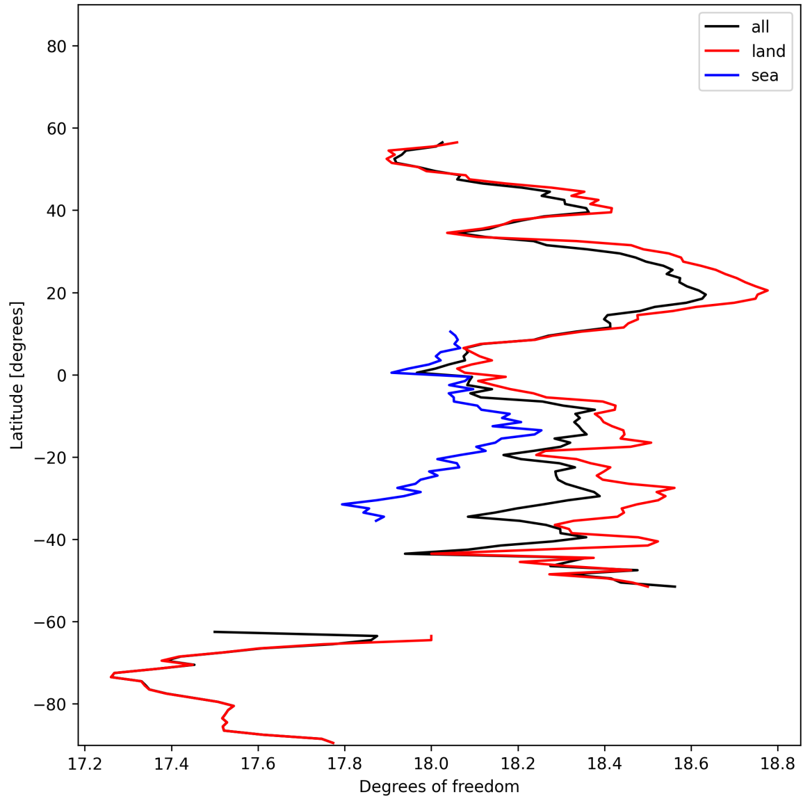
Figure 19: Zonal average of “Degrees of freedom” for 2025-11-14 to 2025-11-16.
