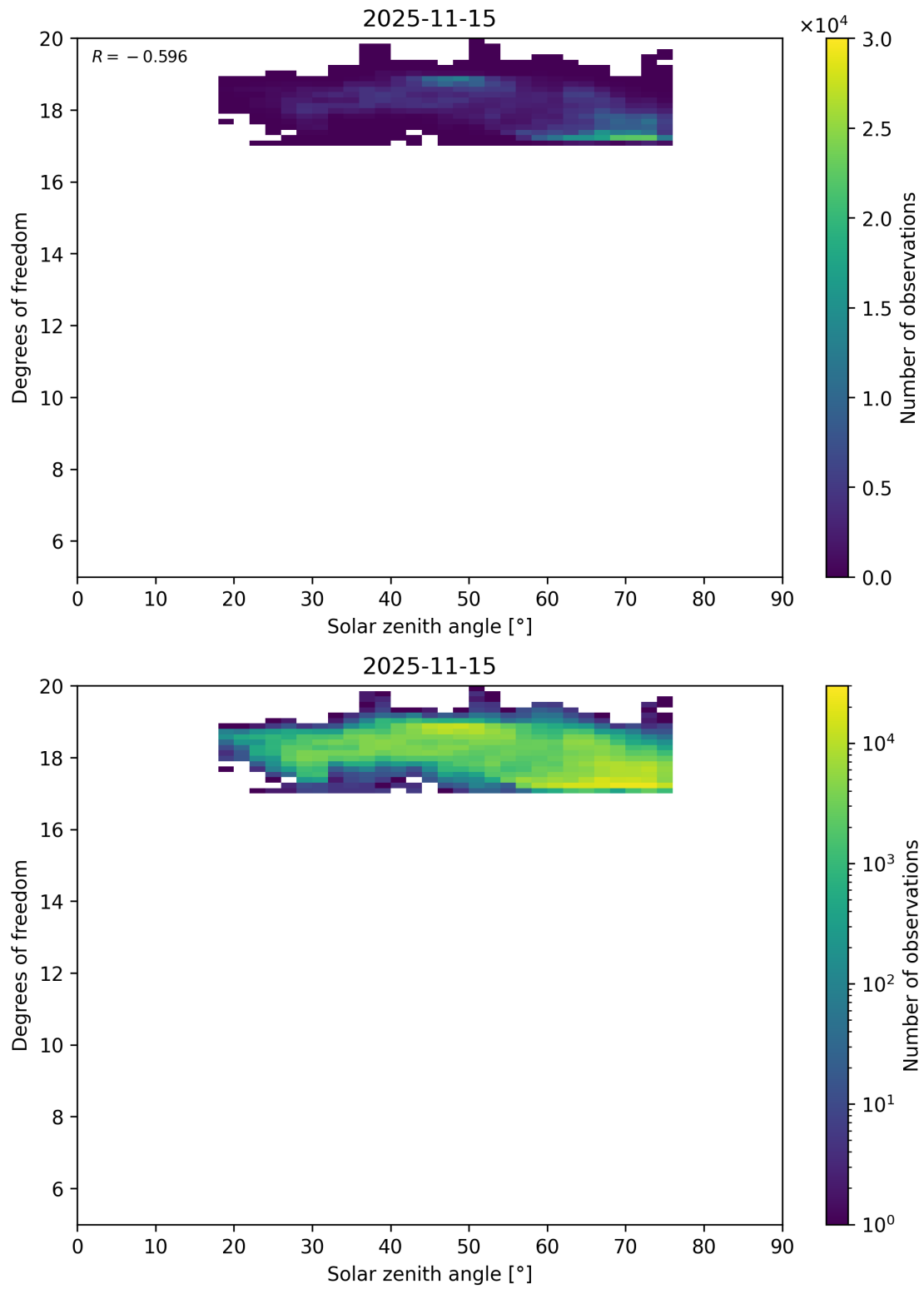
Figure 96: Scatter density plot of “Solar zenith angle” against “Degrees of freedom” for 2025-11-14 to 2025-11-16.
