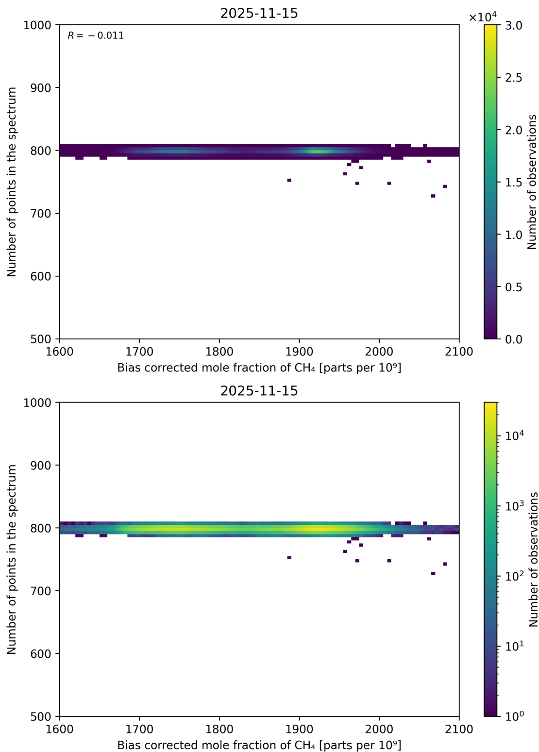
Figure 68: Scatter density plot of “Bias corrected mole fraction of CH 4 ” against “Number of points in the spectrum” for 2025-11-14 to 2025-11-16.
