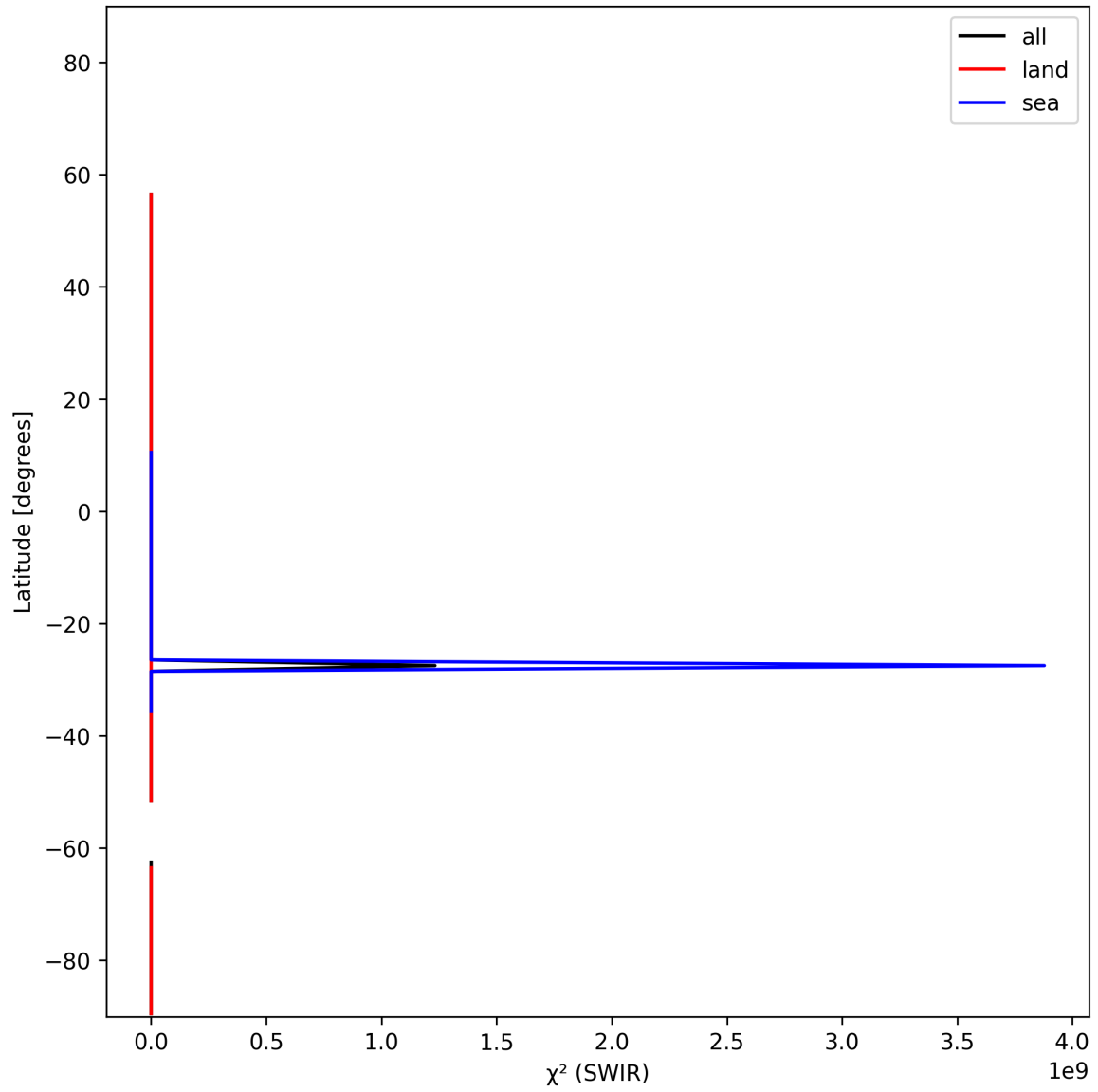
Figure 17: Zonal average of “ \chi^2 (SWIR)” for 2025-11-14 to 2025-11-16.
