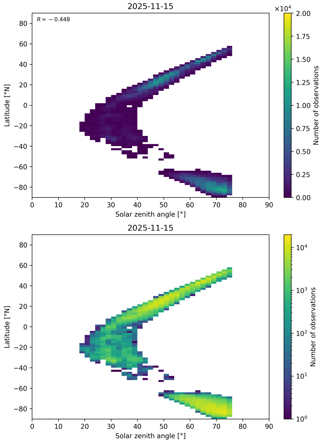
Figure 98: Scatter density plot of “Solar zenith angle” against “Latitude” for 2025-11-14 to 2025-11-16.
