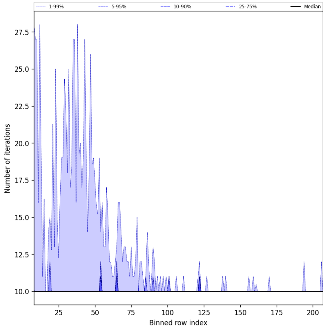
Figure 42: Along track statistics of “Number of iterations” for 2025-11-14 to 2025-11-16
