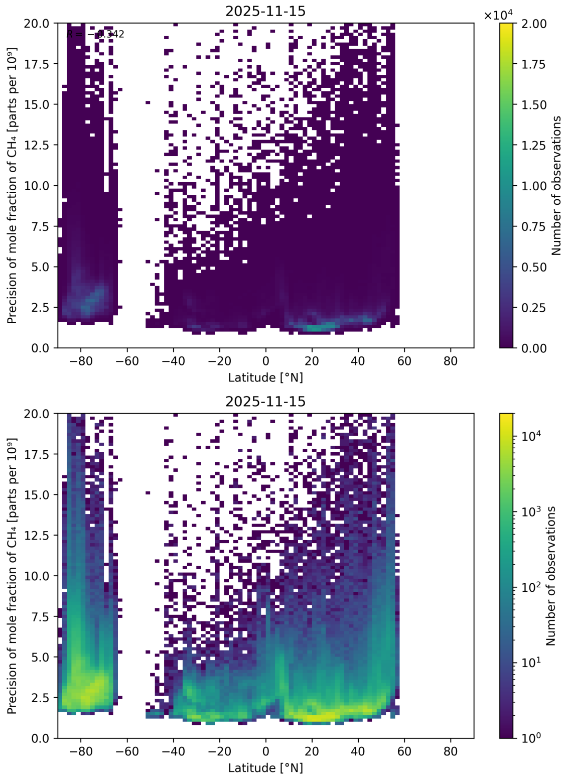
Figure 59: Scatter density plot of “Latitude” against “Precision of mole fraction of CH 4 ” for 2025-11-14 to 2025-11-16.
