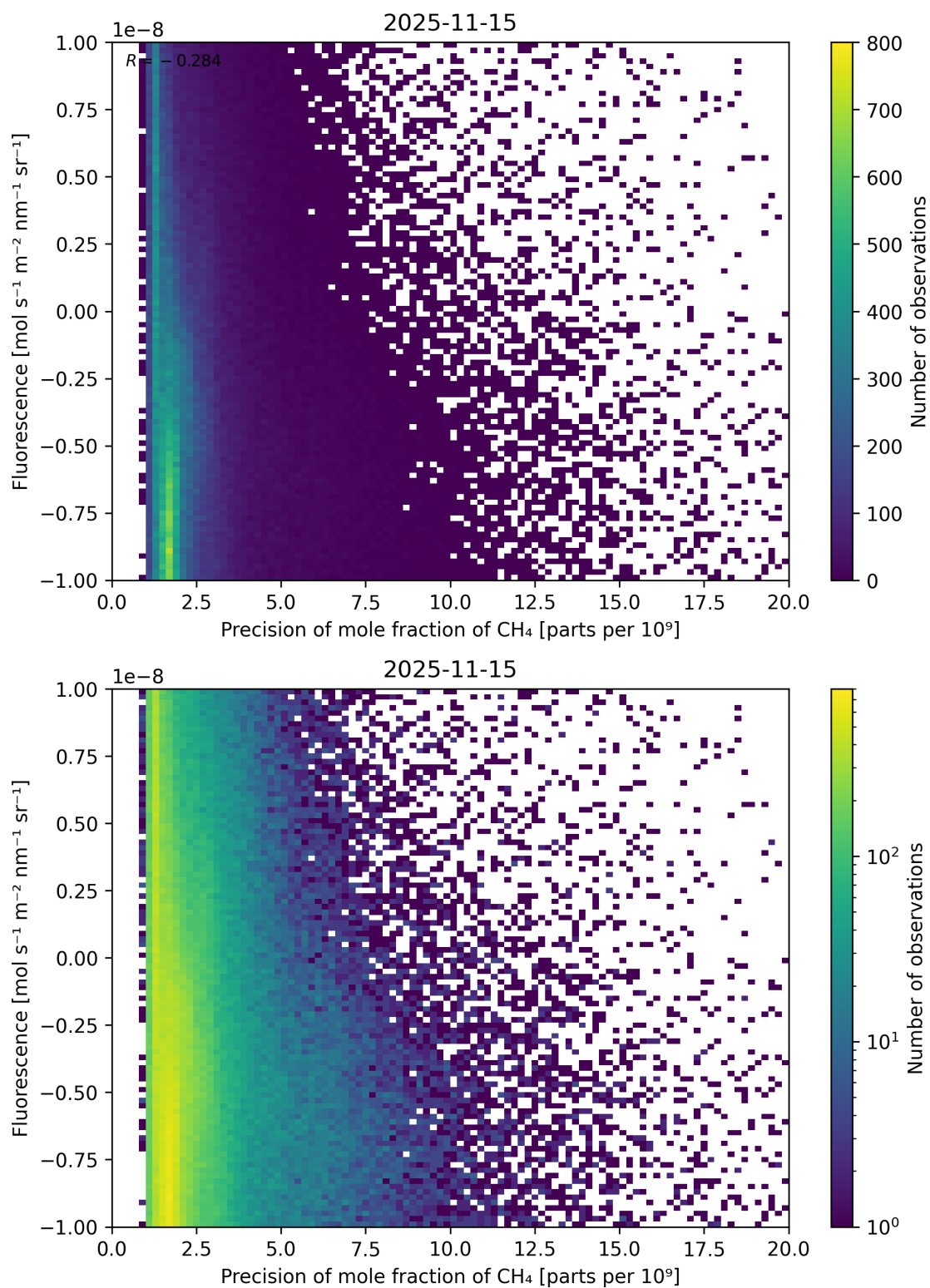
Figure 81: Scatter density plot of “Precision of mole fraction of \text{CH}_4 ” against “Fluorescence” for 2025-11-14 to 2025-11-16.
