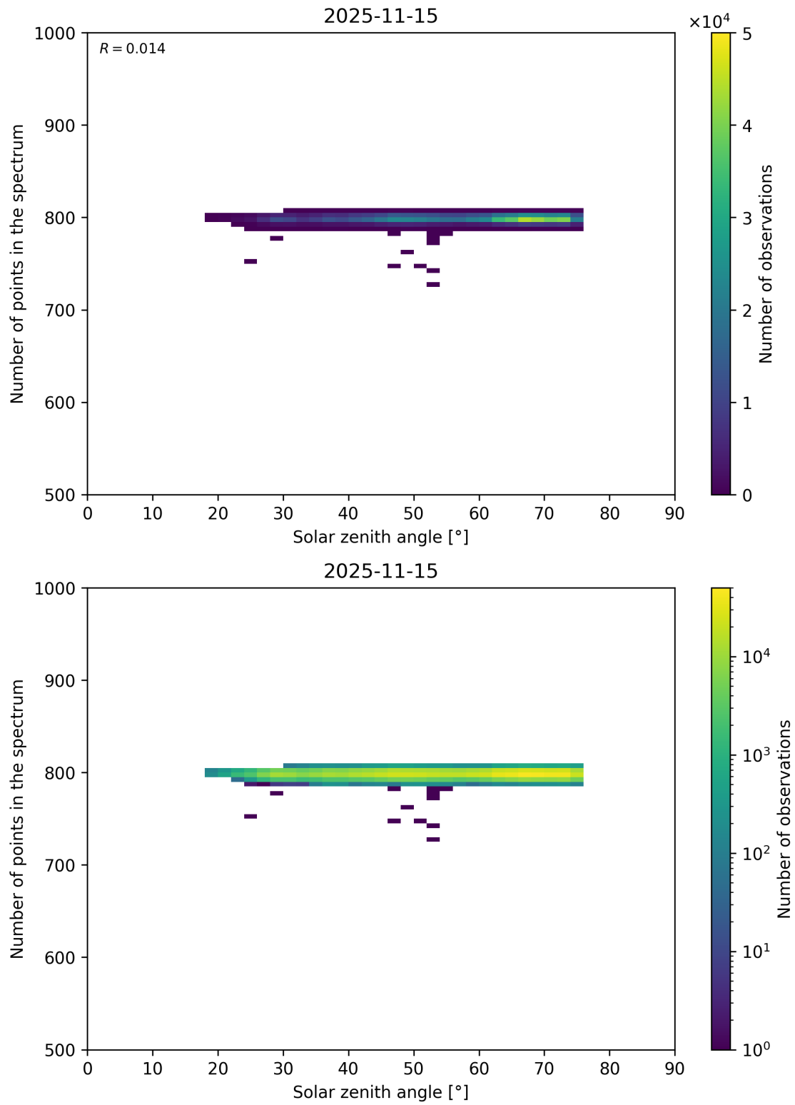
Figure 103: Scatter density plot of “Solar zenith angle” against “Number of points in the spectrum” for 2025-11-14 to 2025-11-16.
