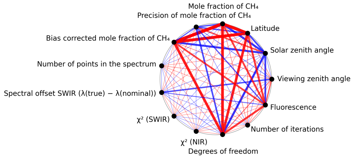
Figure 1: Map of correlation graph for 2025-11-14 to 2025-11-16.
