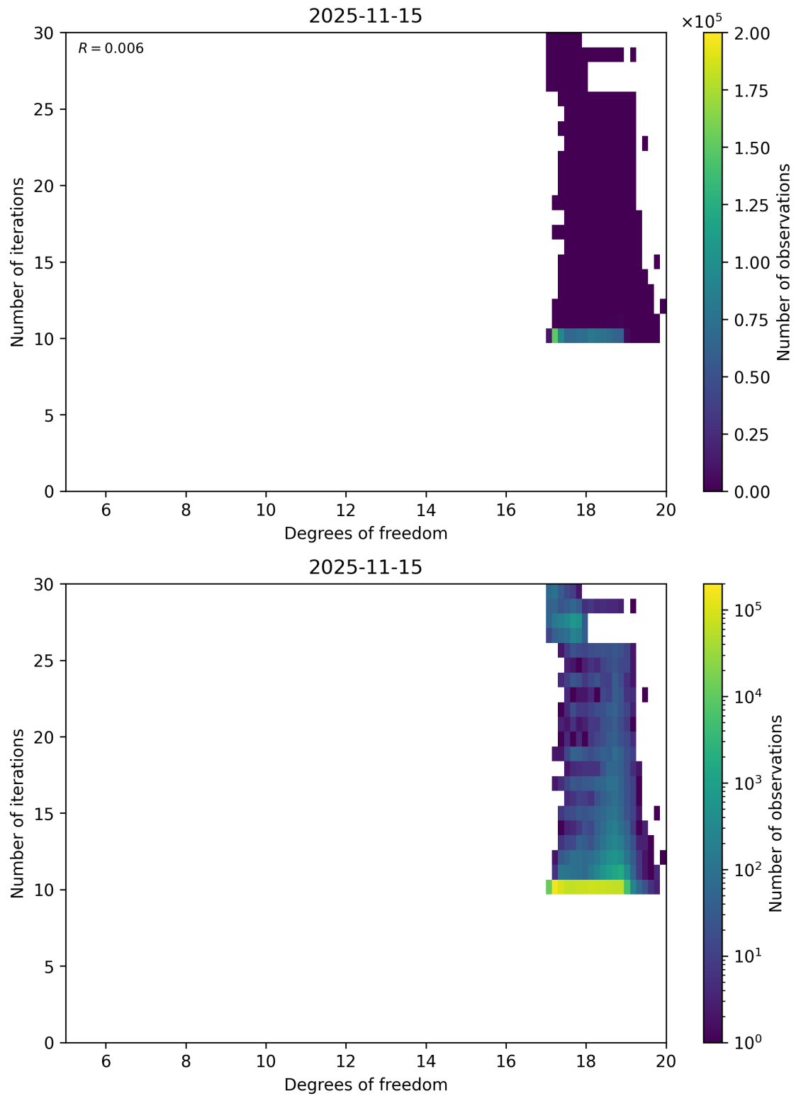
Figure 52: Scatter density plot of “Degrees of freedom” against “Number of iterations” for 2025-11-14 to 2025-11-16.
