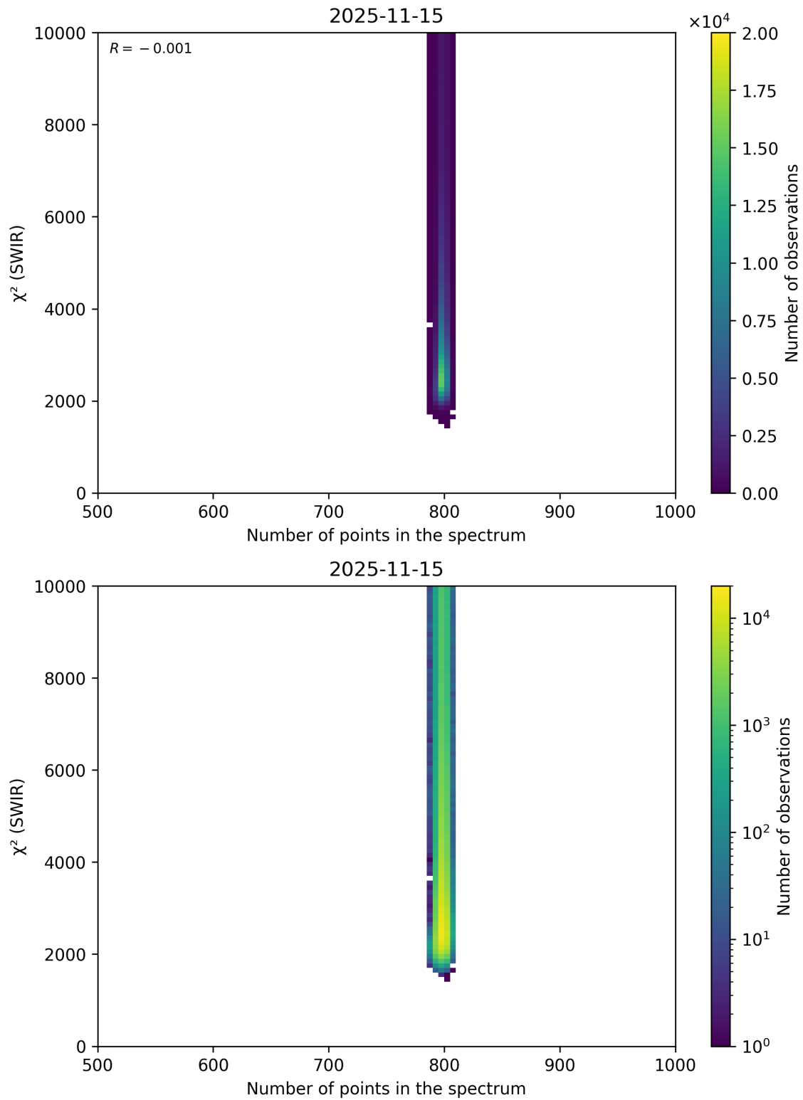
Figure 89: Scatter density plot of “Number of points in the spectrum” against “ \chi^2 (SWIR)” for 2025-11-14 to 2025-11-16.
