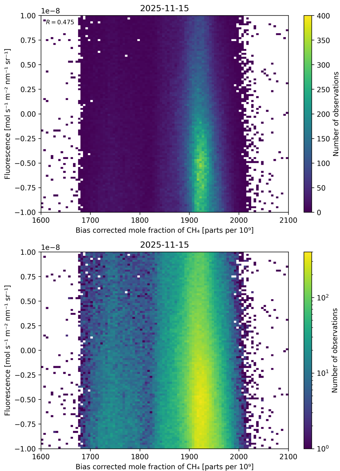
Figure 66: Scatter density plot of “Bias corrected mole fraction of \text{CH}_4 ” against “Fluorescence” for 2025-11-14 to 2025-11-16.
