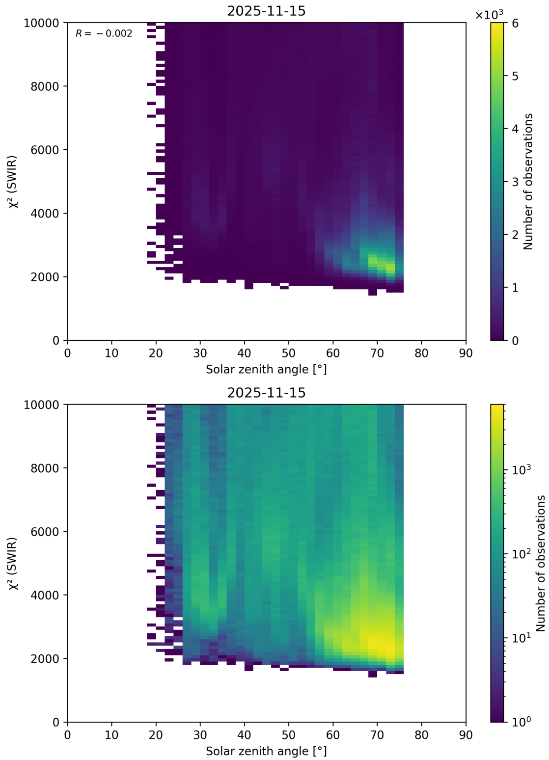
Figure 95: Scatter density plot of “Solar zenith angle” against “ \chi^2 (SWIR)” for 2025-11-14 to 2025-11-16.
