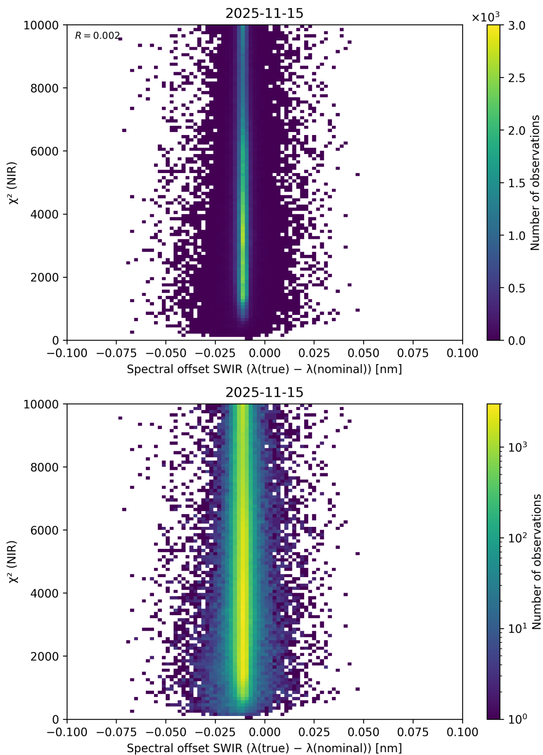
Figure 117: Scatter density plot of “Spectral offset SWIR ( \lambda_{\text{true}} - \lambda_{\text{nominal}} )” against “ \chi^2 (NIR)” for 2025-11-14 to 2025-11-16.
