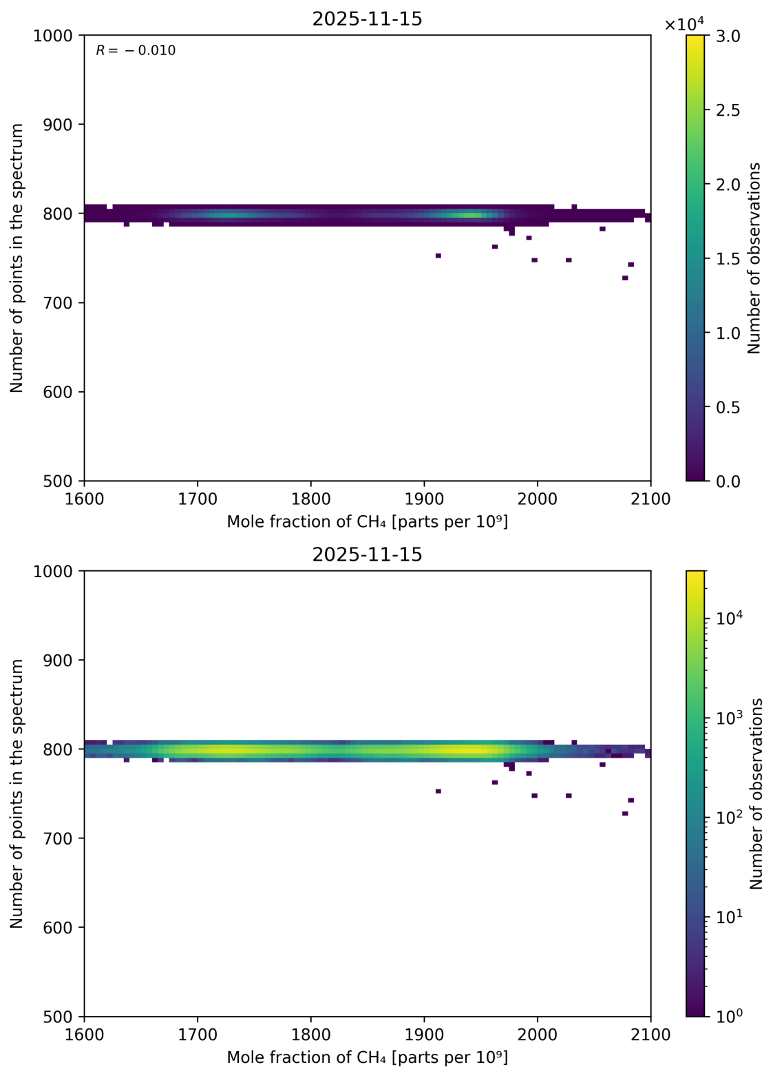
Figure 77: Scatter density plot of “Mole fraction of CH 4 ” against “Number of points in the spectrum” for 2025-11-14 to 2025-11-16.
