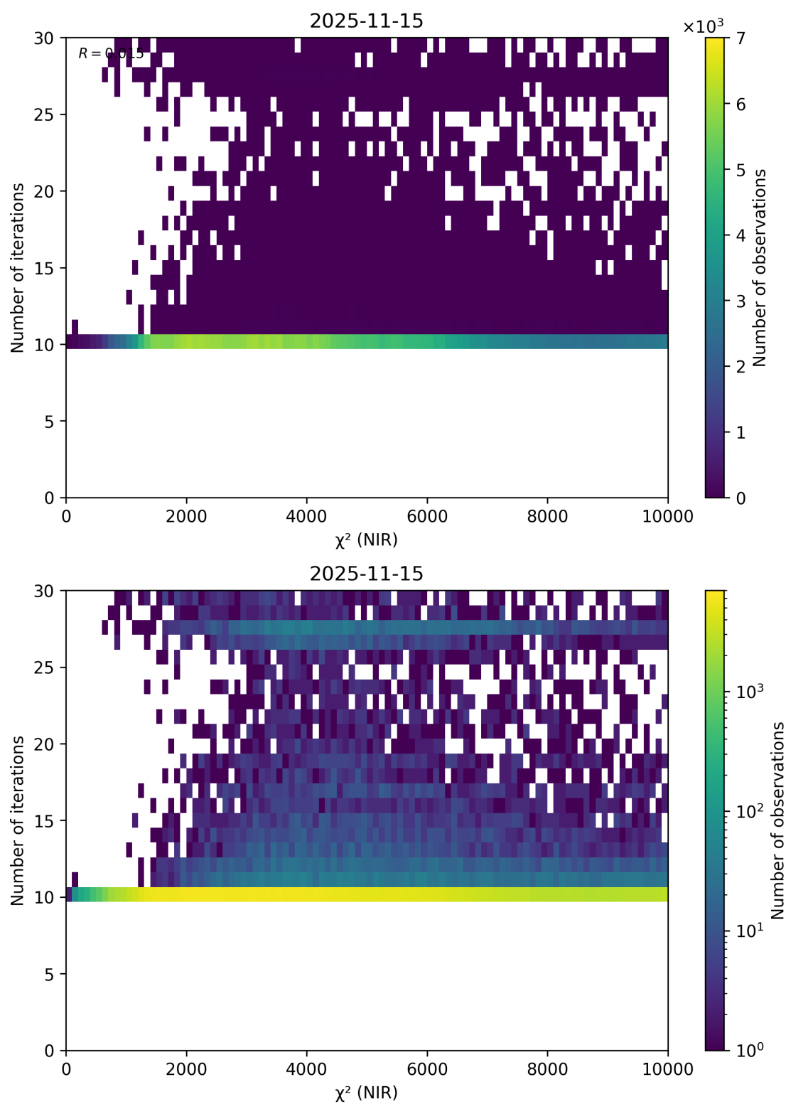
Figure 46: Scatter density plot of “ \chi^2 (NIR)” against “Number of iterations” for 2025-11-14 to 2025-11-16.
