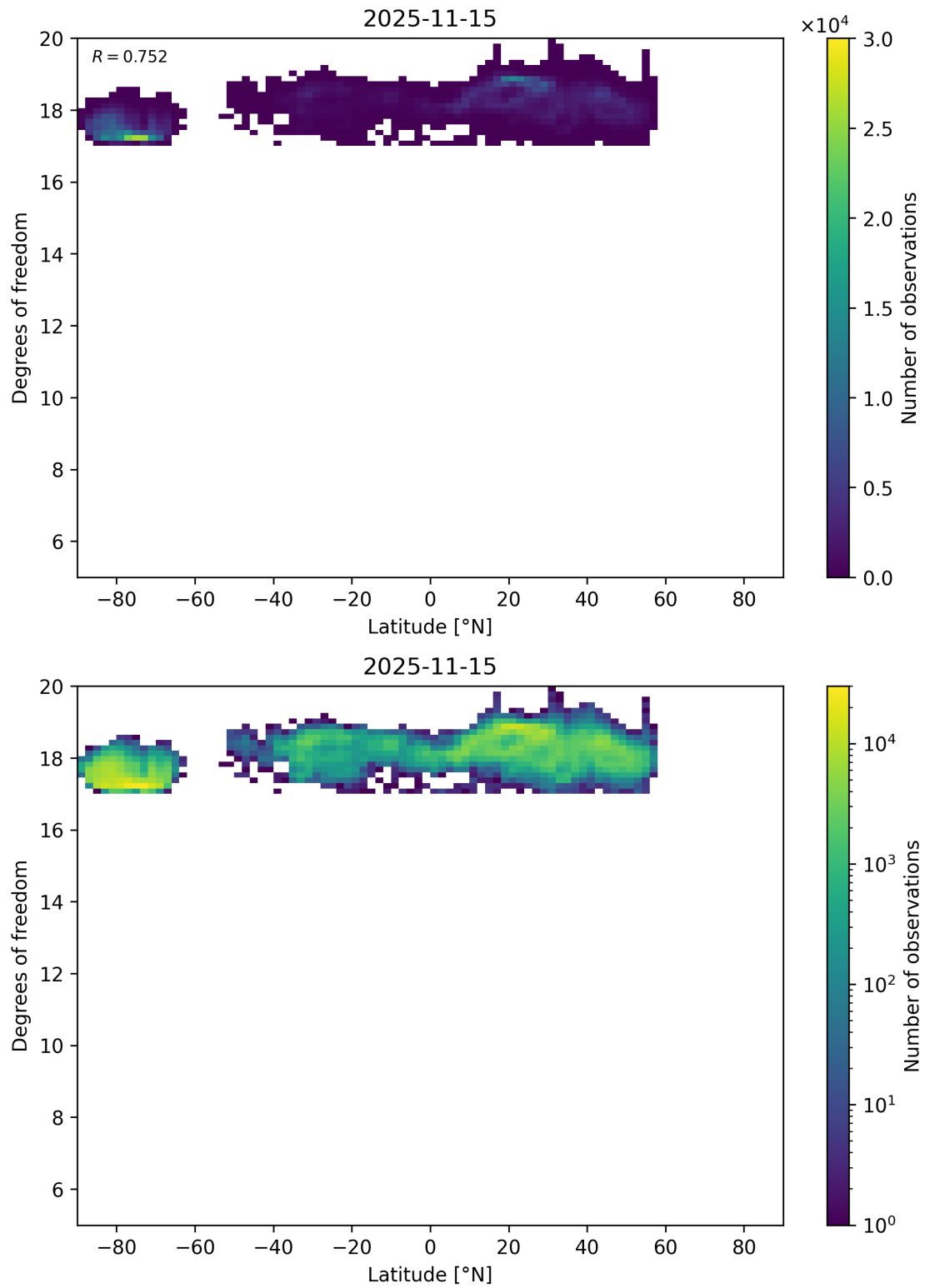
Figure 55: Scatter density plot of “Latitude” against “Degrees of freedom” for 2025-11-14 to 2025-11-16.
