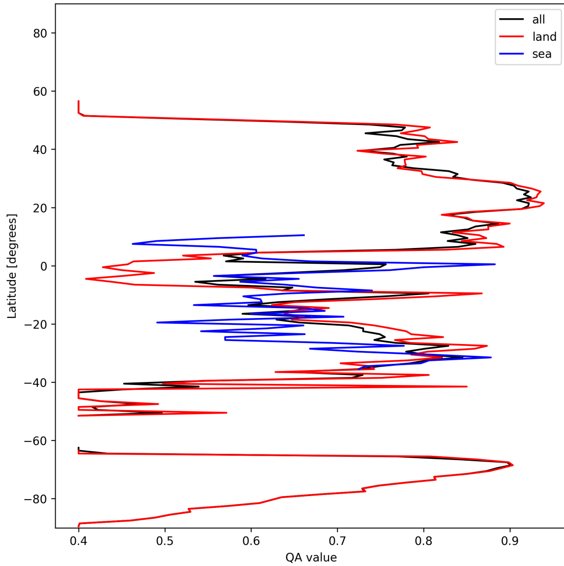
Figure 11: Zonal average of “QA value” for 2025-11-14 to 2025-11-16.
