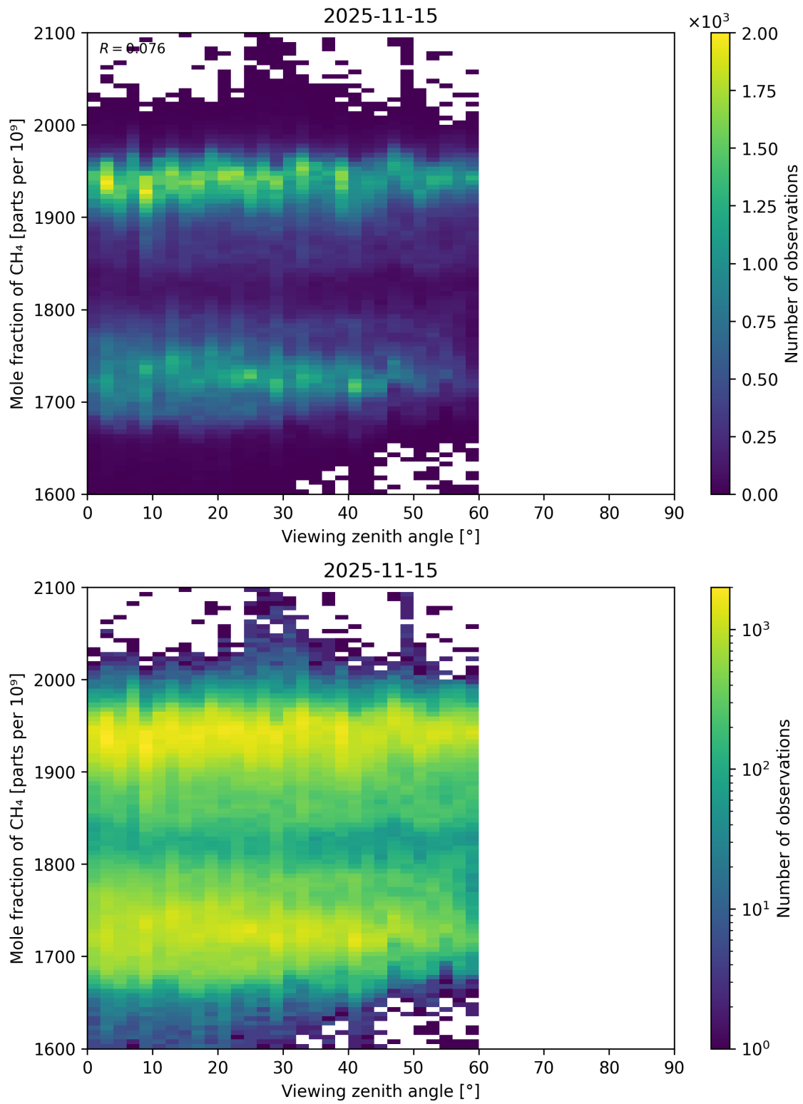
Figure 110: Scatter density plot of “Viewing zenith angle” against “Mole fraction of CH 4 ” for 2025-11-14 to 2025-11-16.
