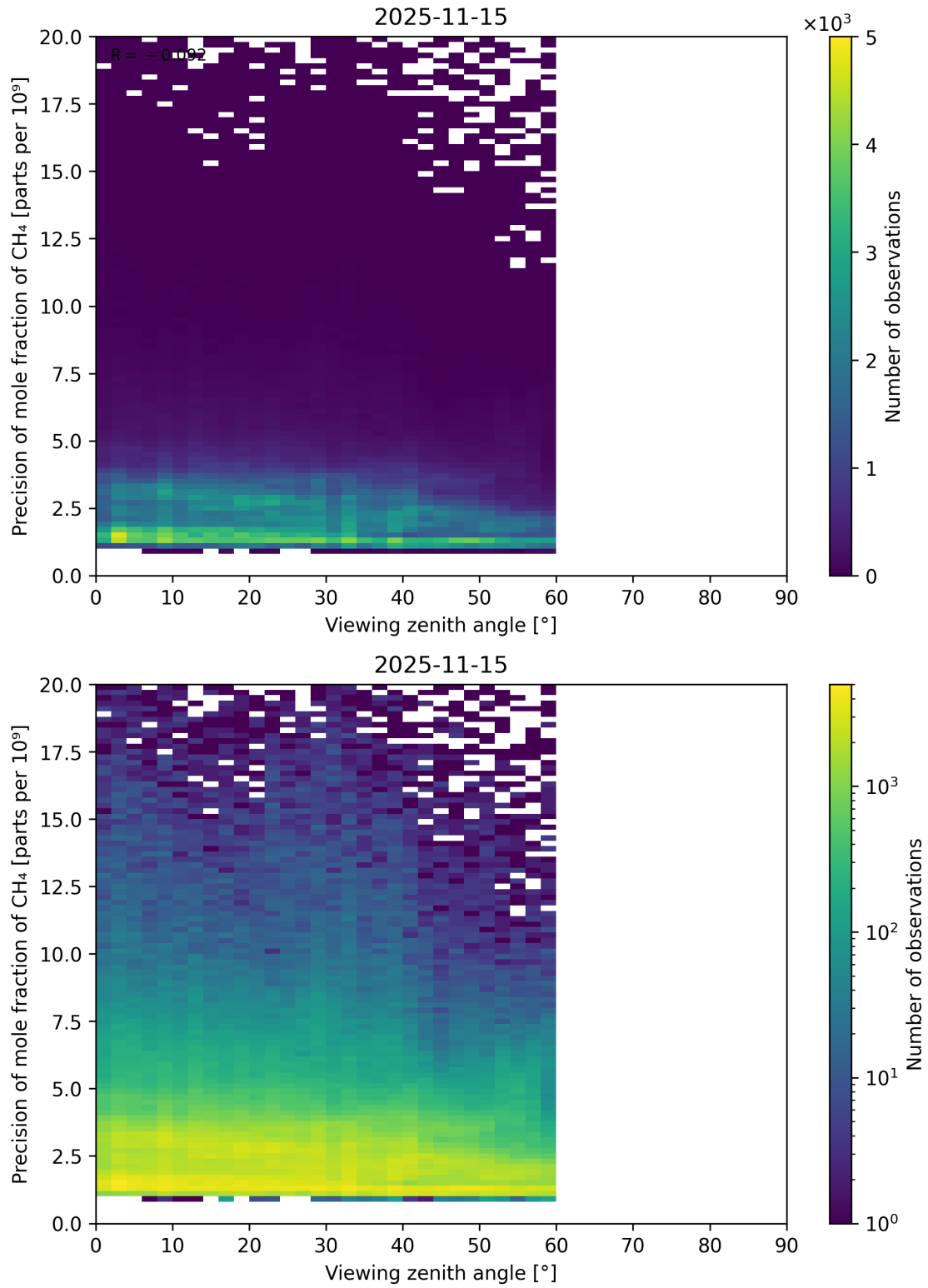
Figure 112: Scatter density plot of “Viewing zenith angle” against “Precision of mole fraction of CH 4 ” for 2025-11-14 to 2025-11-16.
