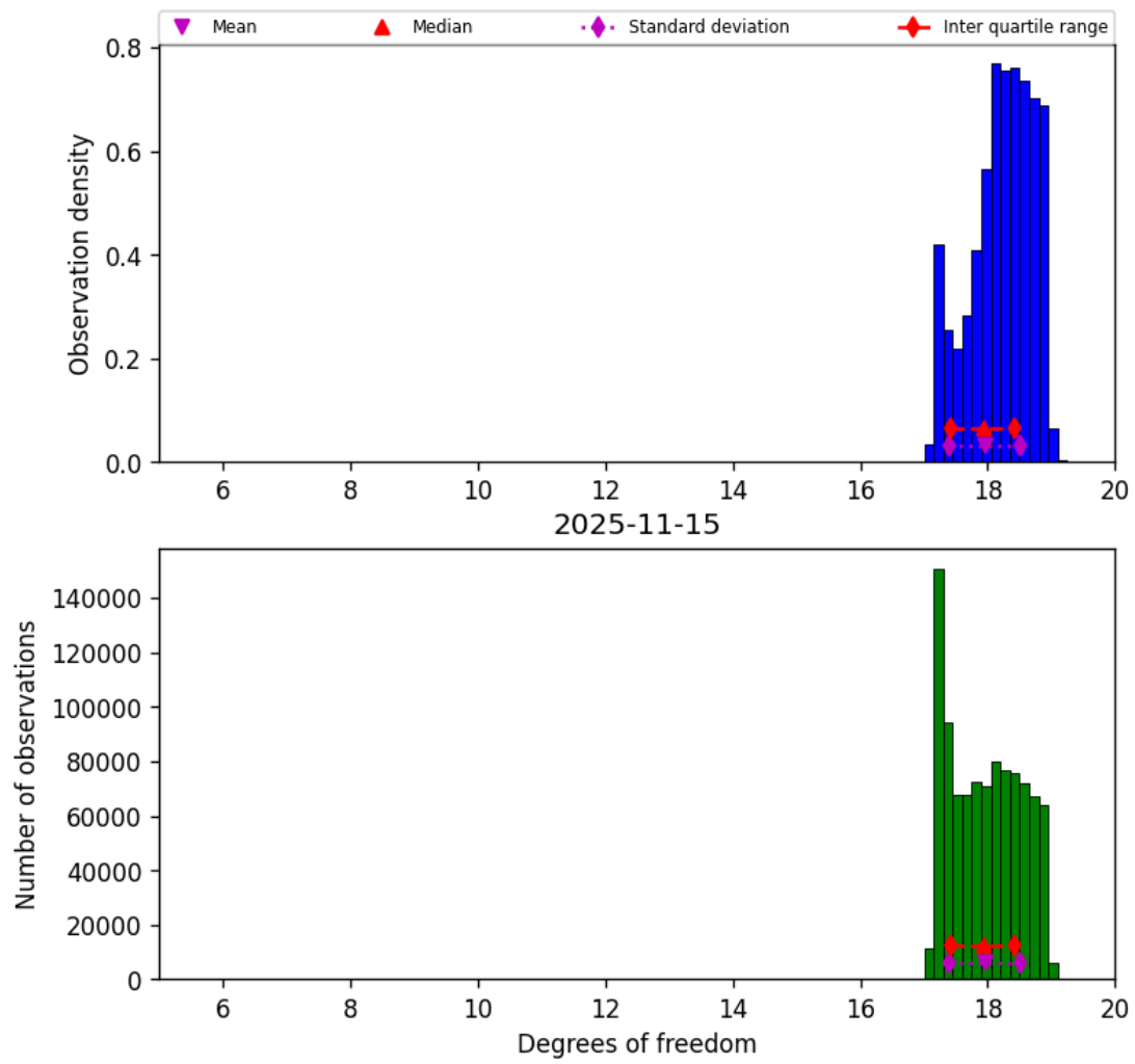
Figure 30: Histogram of “Degrees of freedom” for 2025-11-14 to 2025-11-16
