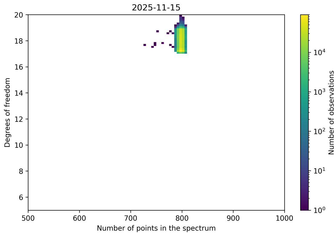
Figure 90: Scatter density plot of “Number of points in the spectrum” against “Degrees of freedom” for 2025-11-14 to 2025-11-16.
