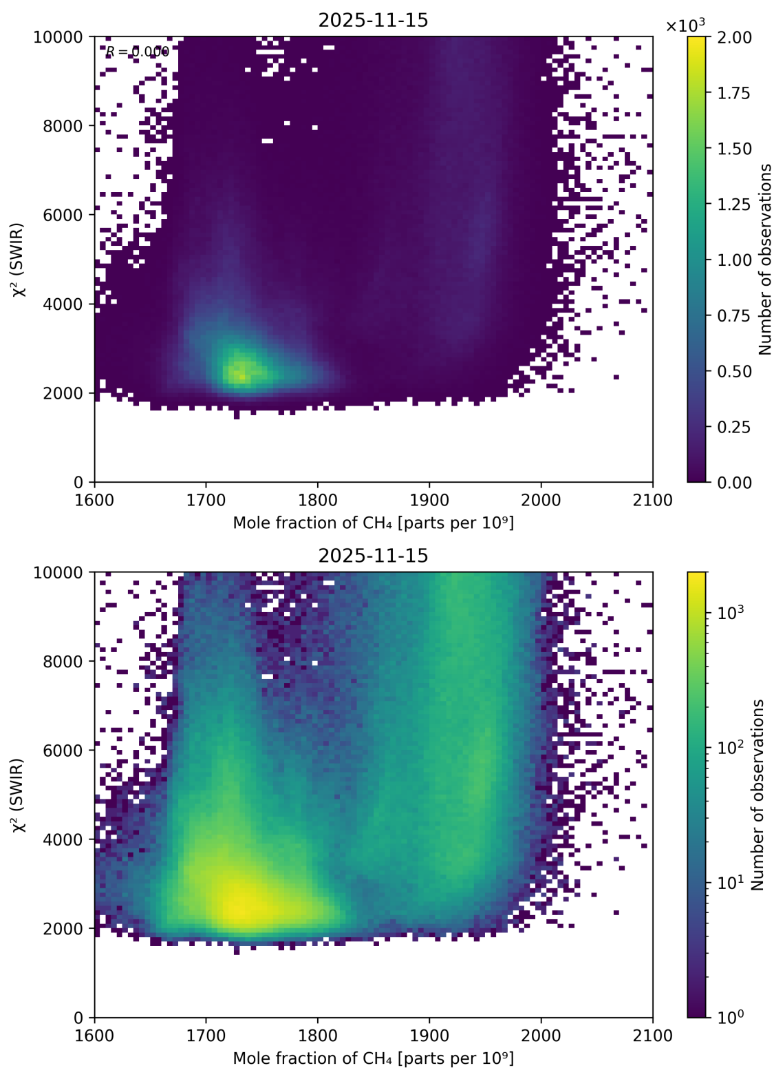
Figure 71: Scatter density plot of “Mole fraction of CH 4 ” against “ \chi^2 (SWIR)” for 2025-11-14 to 2025-11-16.
