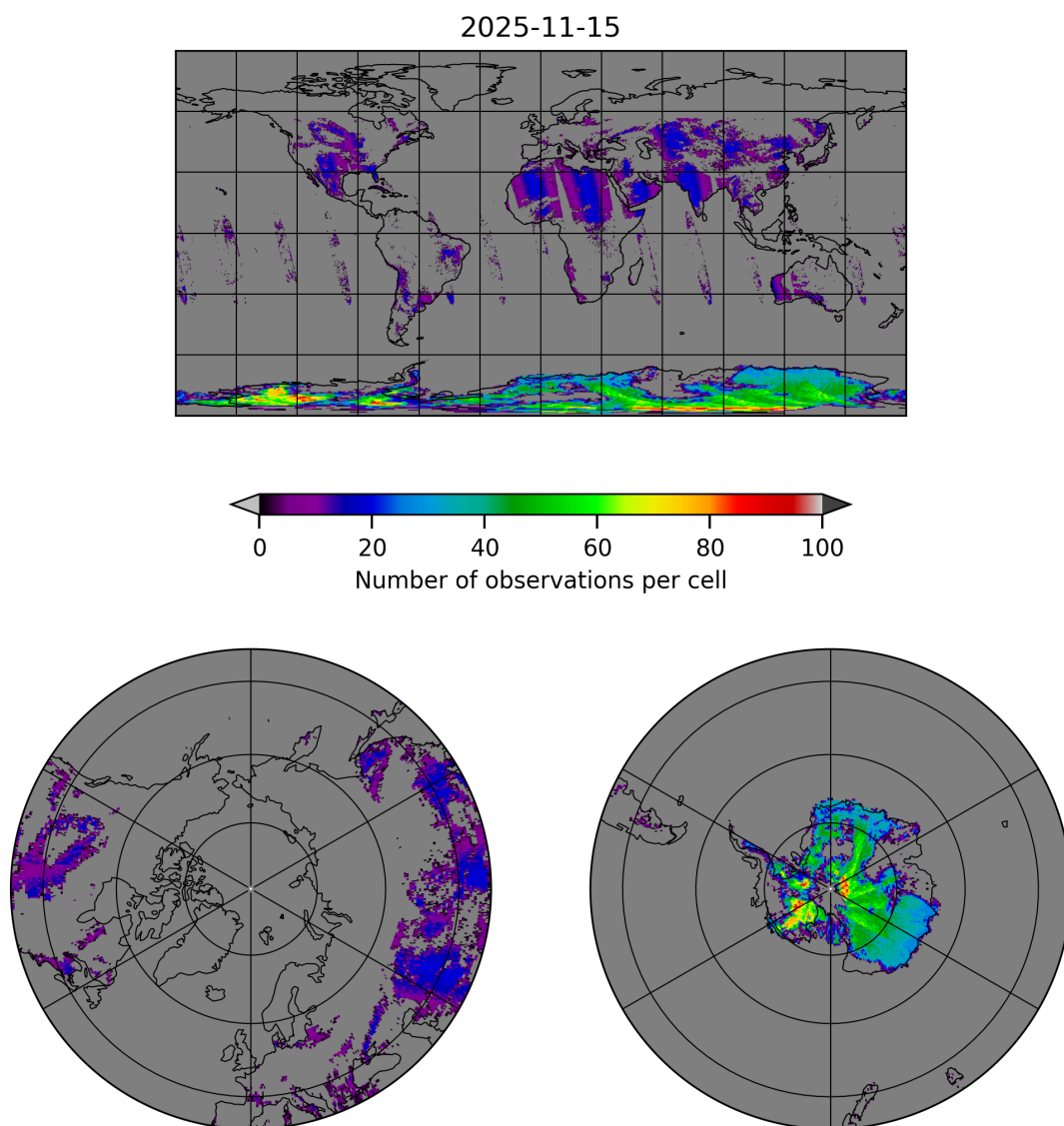
Figure 10: Map of the number of observations for 2025-11-14 to 2025-11-16
