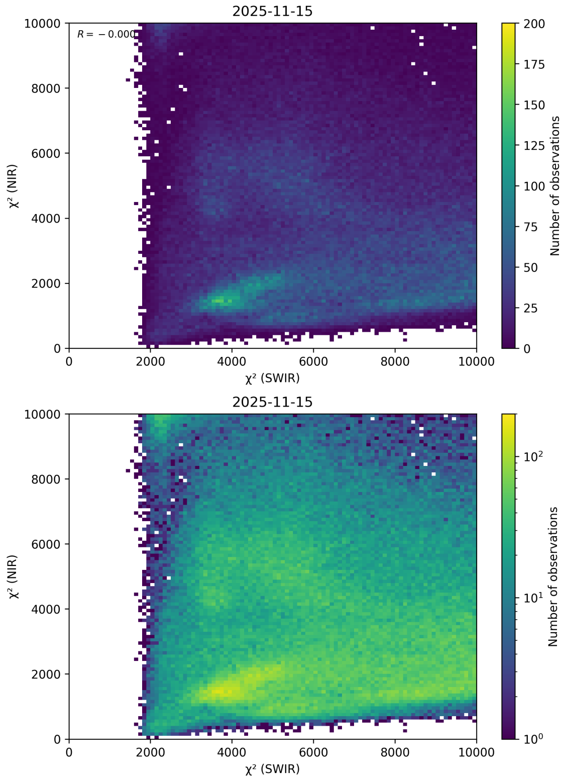
Figure 47: Scatter density plot of “ \chi^2 (SWIR)” against “ \chi^2 (NIR)” for 2025-11-14 to 2025-11-16.
