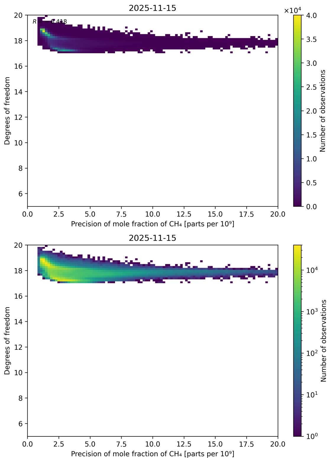
Figure 80: Scatter density plot of “Precision of mole fraction of CH 4 ” against “Degrees of freedom” for 2025-11-14 to 2025-11-16.
