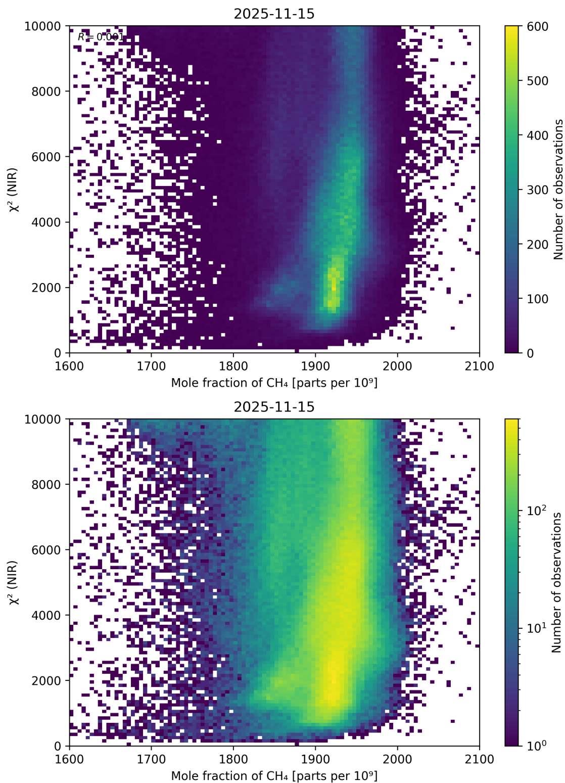
Figure 70: Scatter density plot of “Mole fraction of \text{CH}_4 ” against “ \chi^2 (NIR)” for 2025-11-14 to 2025-11-16.
