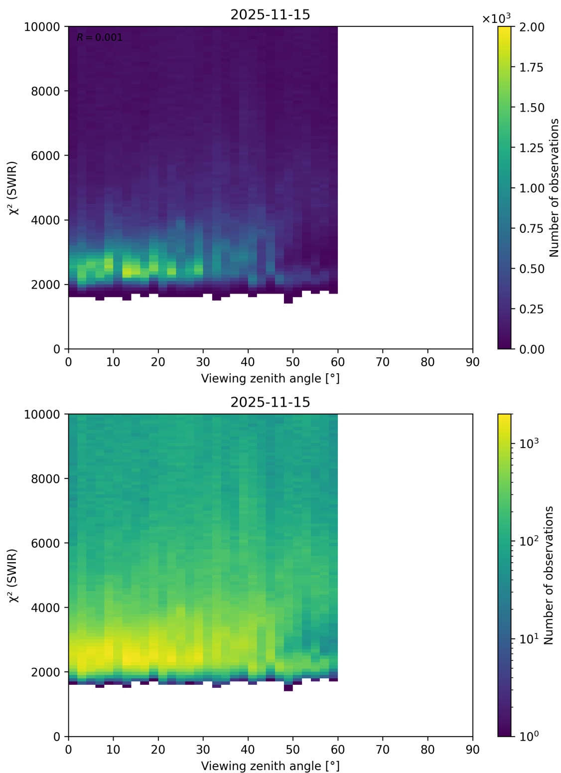
Figure 106: Scatter density plot of “Viewing zenith angle” against “ \chi^2 (SWIR)” for 2025-11-14 to 2025-11-16.
