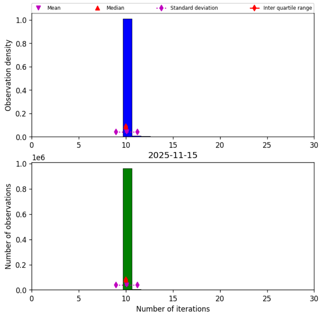
Figure 31: Histogram of “Number of iterations” for 2025-11-14 to 2025-11-16
