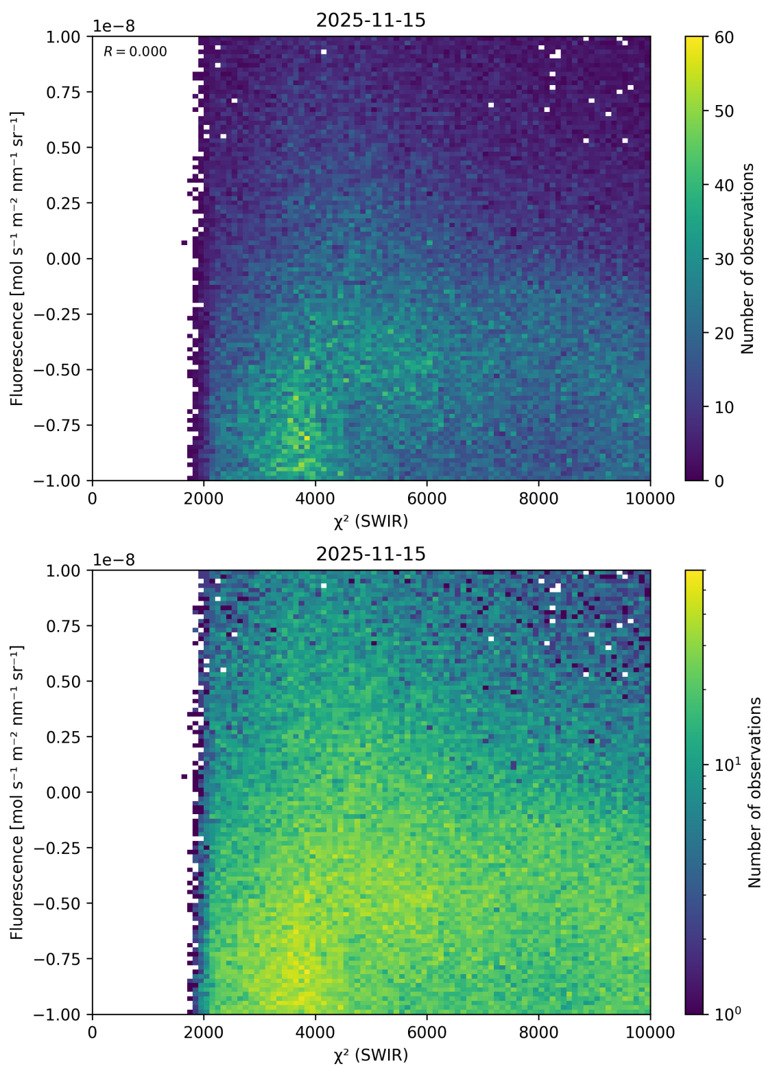
Figure 49: Scatter density plot of “ \chi^2 (SWIR)” against “Fluorescence” for 2025-11-14 to 2025-11-16.
