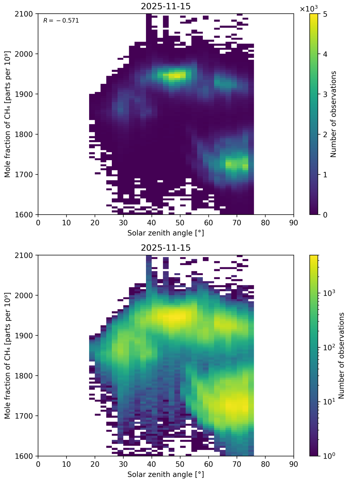
Figure 99: Scatter density plot of “Solar zenith angle” against “Mole fraction of CH 4 ” for 2025-11-14 to 2025-11-16.
