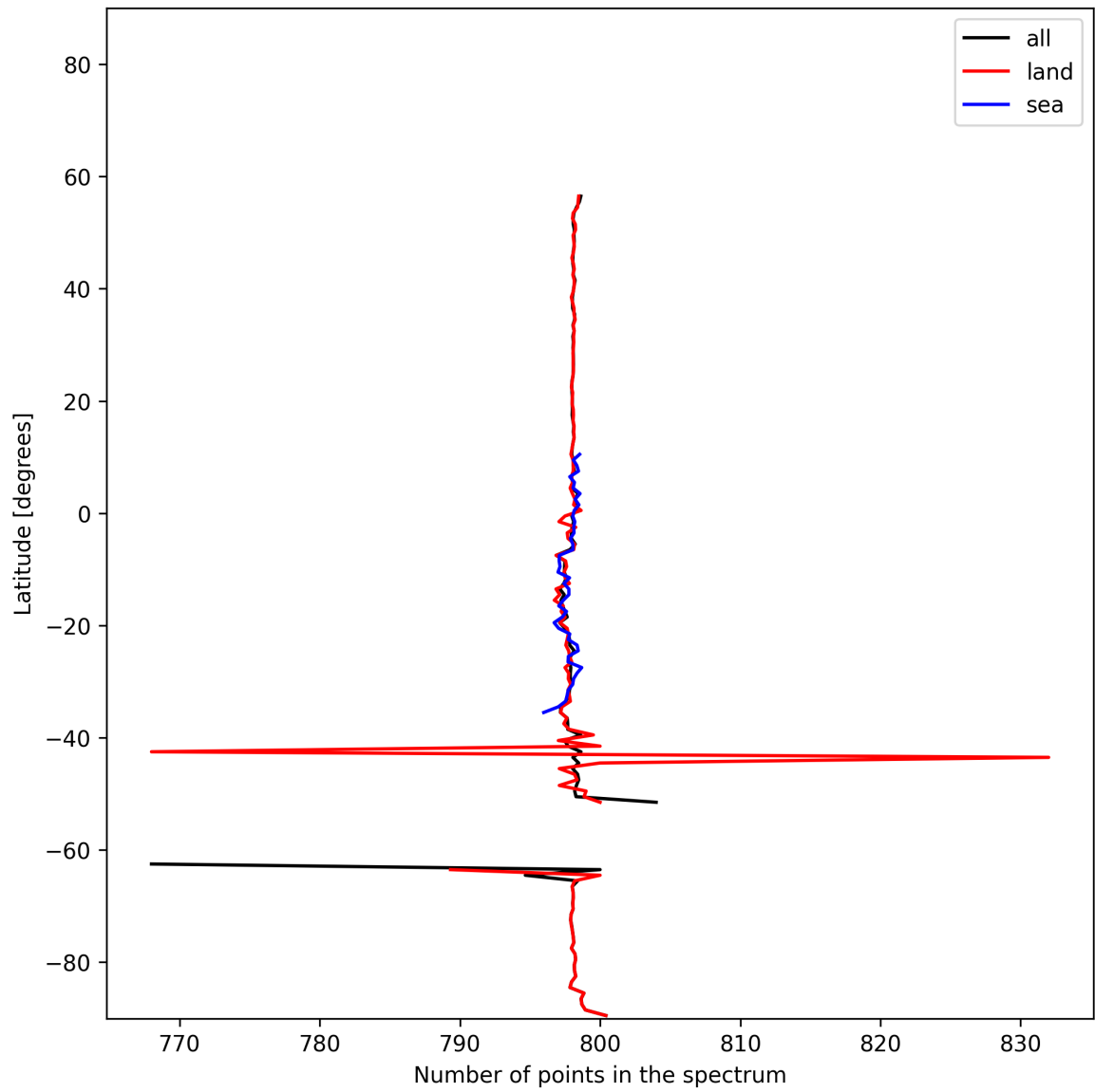
Figure 15: Zonal average of “Number of points in the spectrum” for 2025-11-14 to 2025-11-16.
