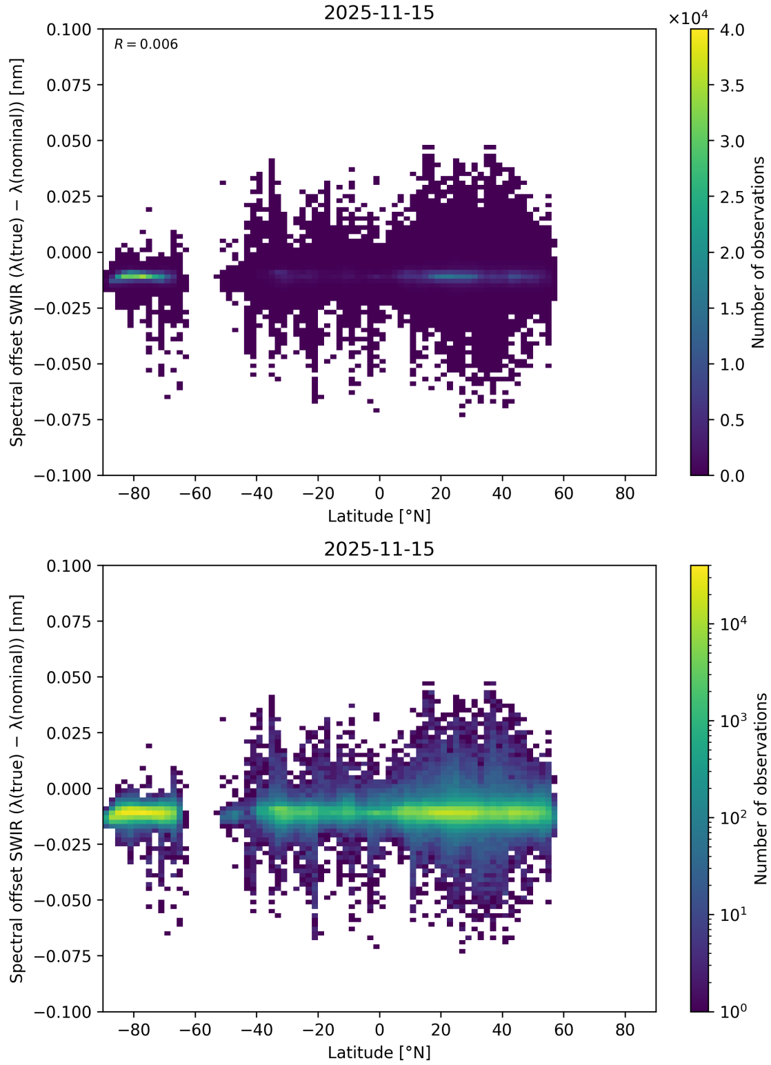
Figure 62: Scatter density plot of “Latitude” against “Spectral offset SWIR ( \lambda_{\text{true}} - \lambda_{\text{nominal}} )” for 2025-11-14 to 2025-11-16.
