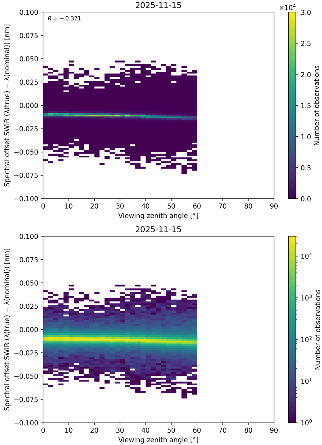
Figure 116: Scatter density plot of “Viewing zenith angle” against “Spectral offset SWIR ( \lambda_{\text{true}} - \lambda_{\text{nominal}} )” for 2025-11-14 to 2025-11-16.
