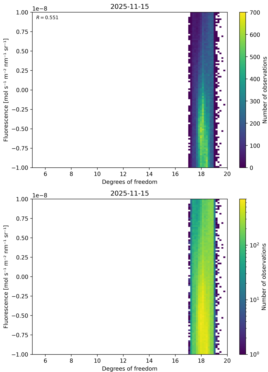
Figure 51: Scatter density plot of “Degrees of freedom” against “Fluorescence” for 2025-11-14 to 2025-11-16.
