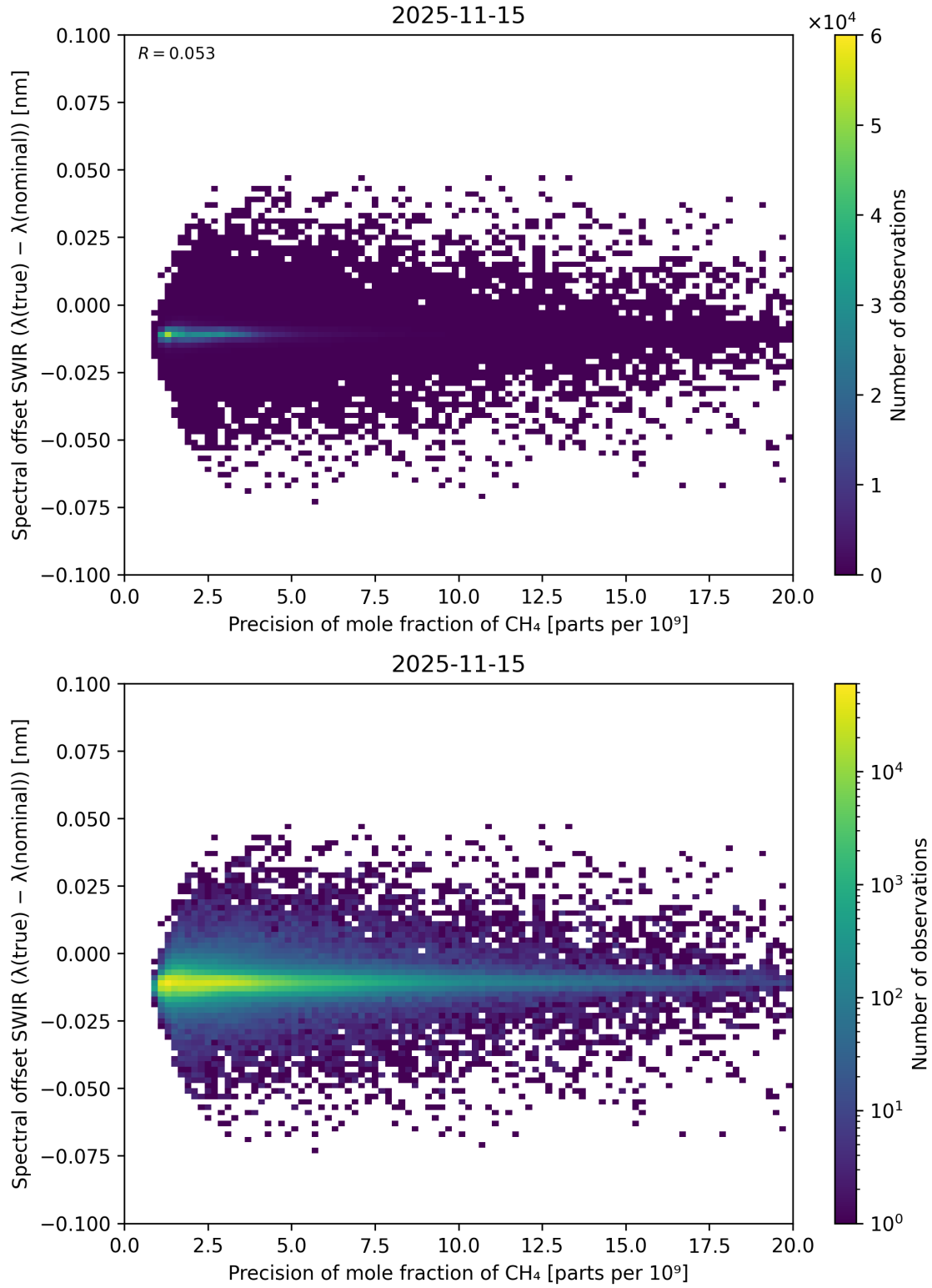
Figure 85: Scatter density plot of “Precision of mole fraction of CH 4 ” against “Spectral offset SWIR ( \lambda_{\text{true}} - \lambda_{\text{nominal}} )” for 2025-11-14 to 2025-11-16.
