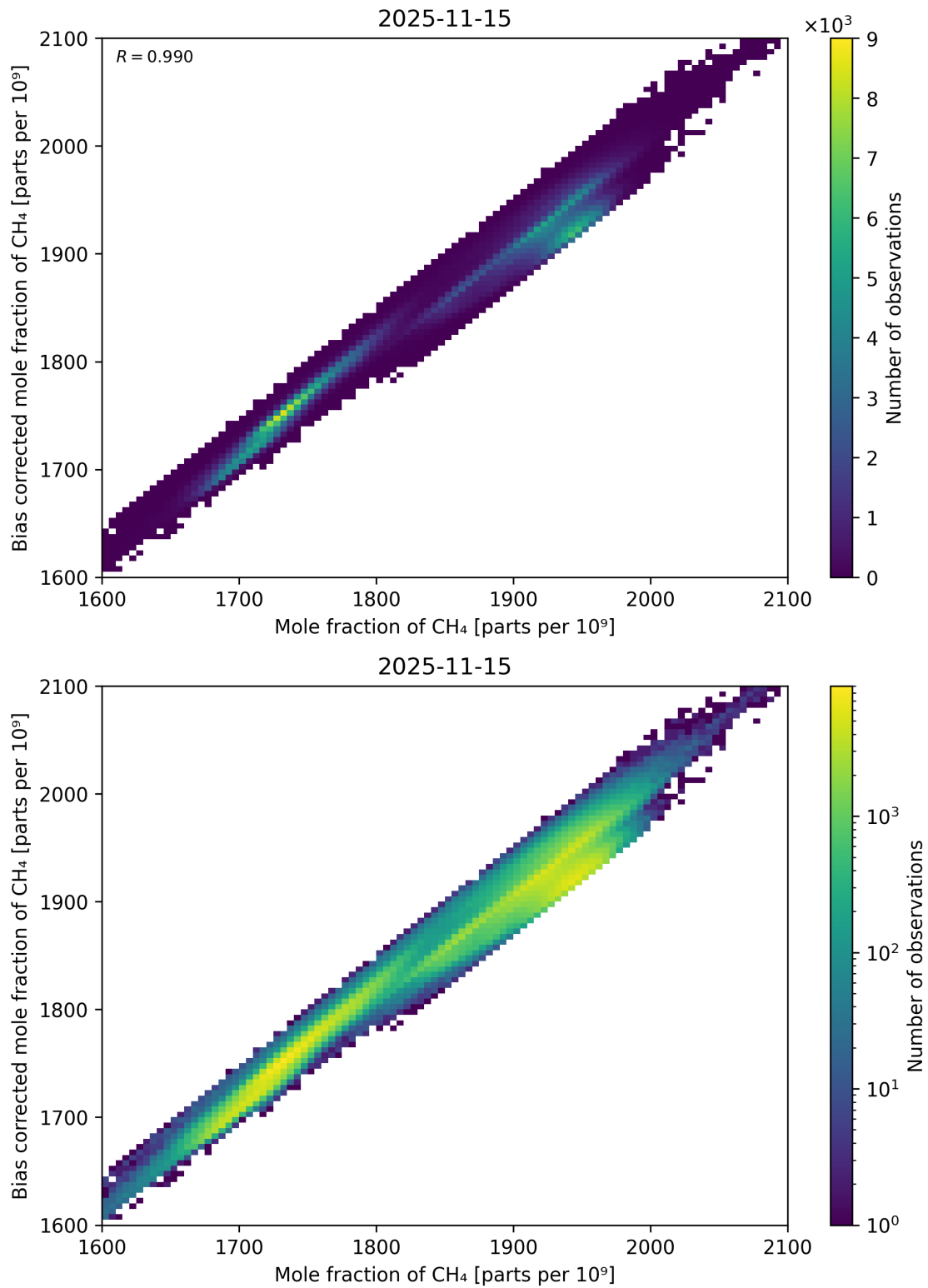
Figure 74: Scatter density plot of “Mole fraction of CH 4 ” against “Bias corrected mole fraction of CH 4 ” for 2025-11-14 to 2025-11-16.
