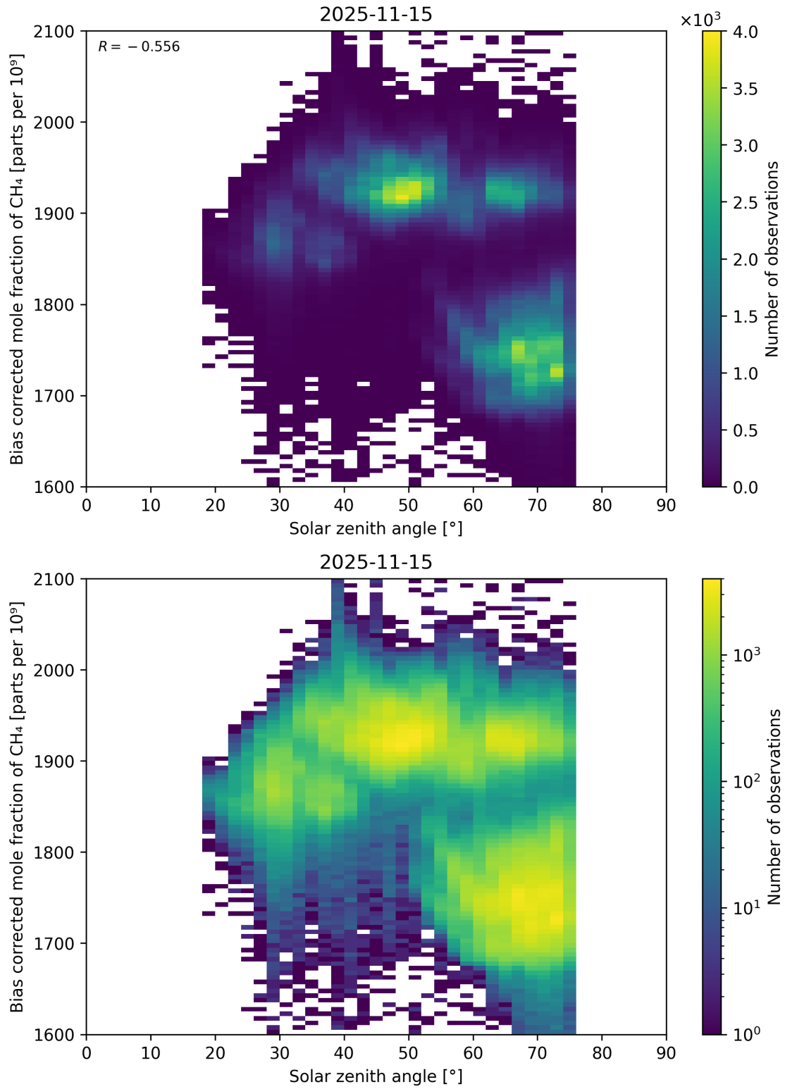
Figure 100: Scatter density plot of “Solar zenith angle” against “Bias corrected mole fraction of \text{CH}_4 ” for 2025-11-14 to 2025-11-16.
