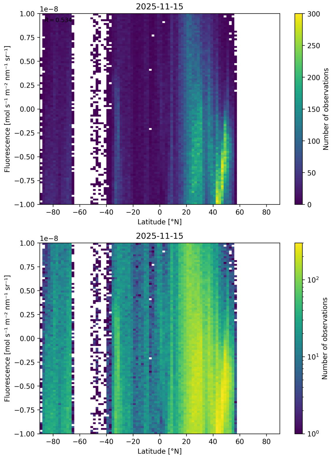
Figure 56: Scatter density plot of “Latitude” against “Fluorescence” for 2025-11-14 to 2025-11-16.
