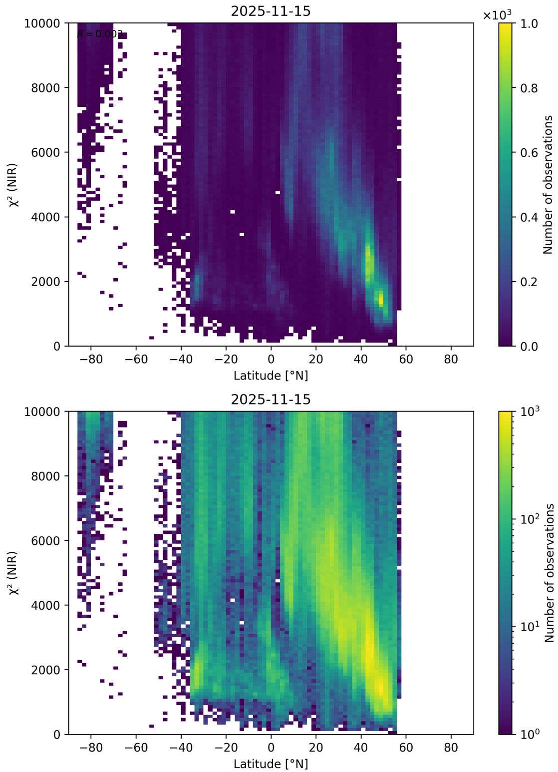
Figure 53: Scatter density plot of “Latitude” against “ \chi^2 (NIR)” for 2025-11-14 to 2025-11-16.
