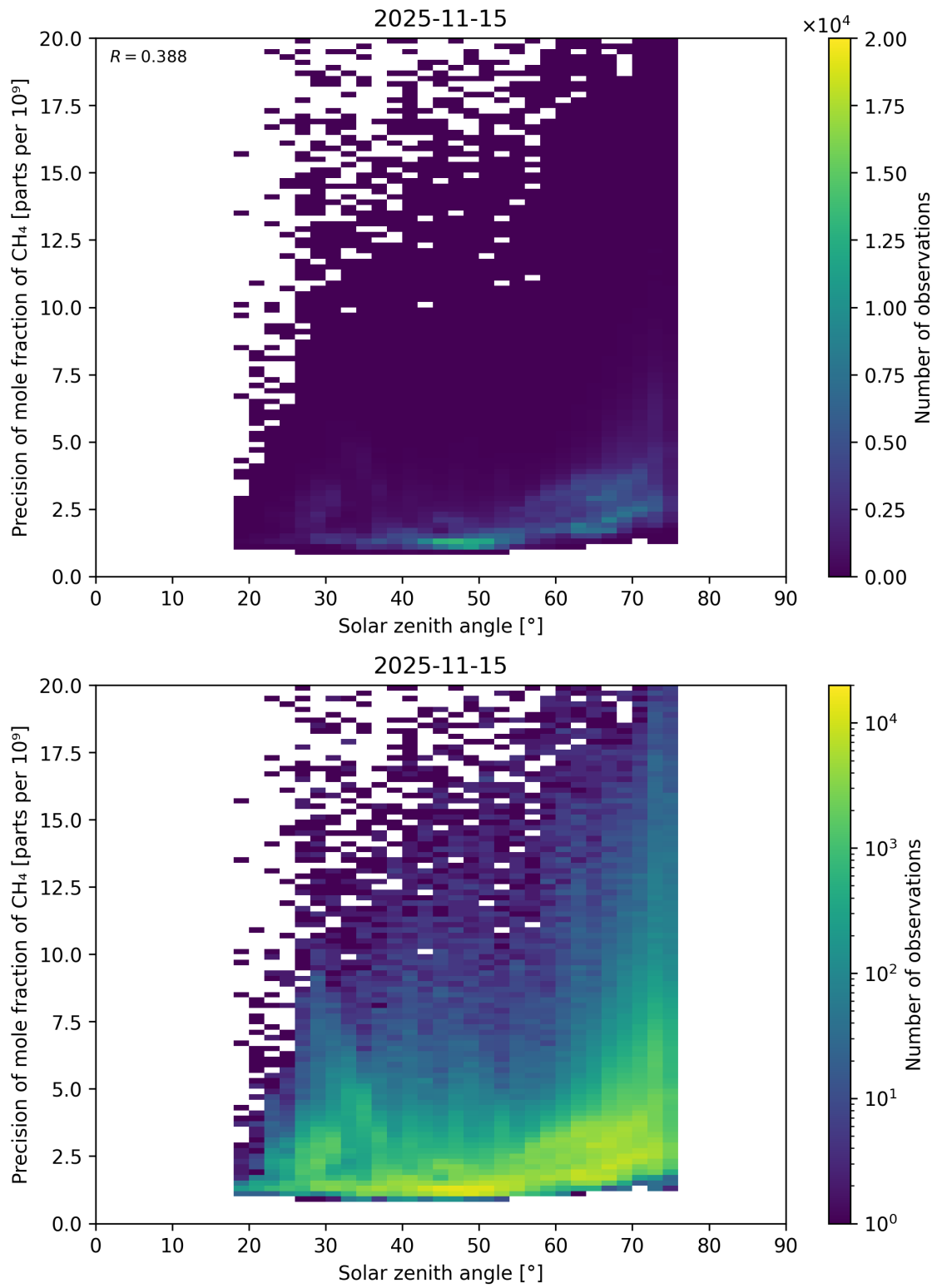
Figure 101: Scatter density plot of “Solar zenith angle” against “Precision of mole fraction of CH 4 ” for 2025-11-14 to 2025-11-16.
