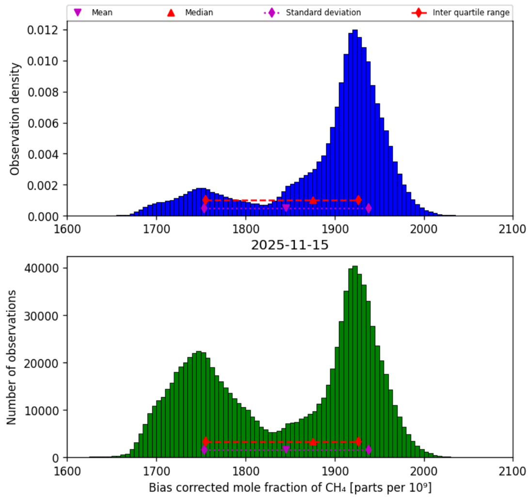
Figure 25: Histogram of “Bias corrected mole fraction of CH 4 ” for 2025-11-14 to 2025-11-16
