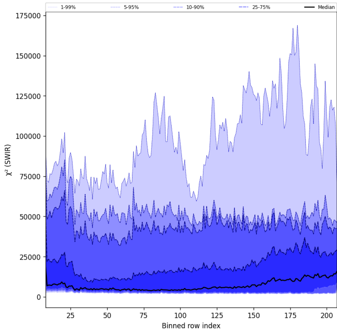
Figure 39: Along track statistics of “ \chi^2 (SWIR)” for 2025-11-14 to 2025-11-16
