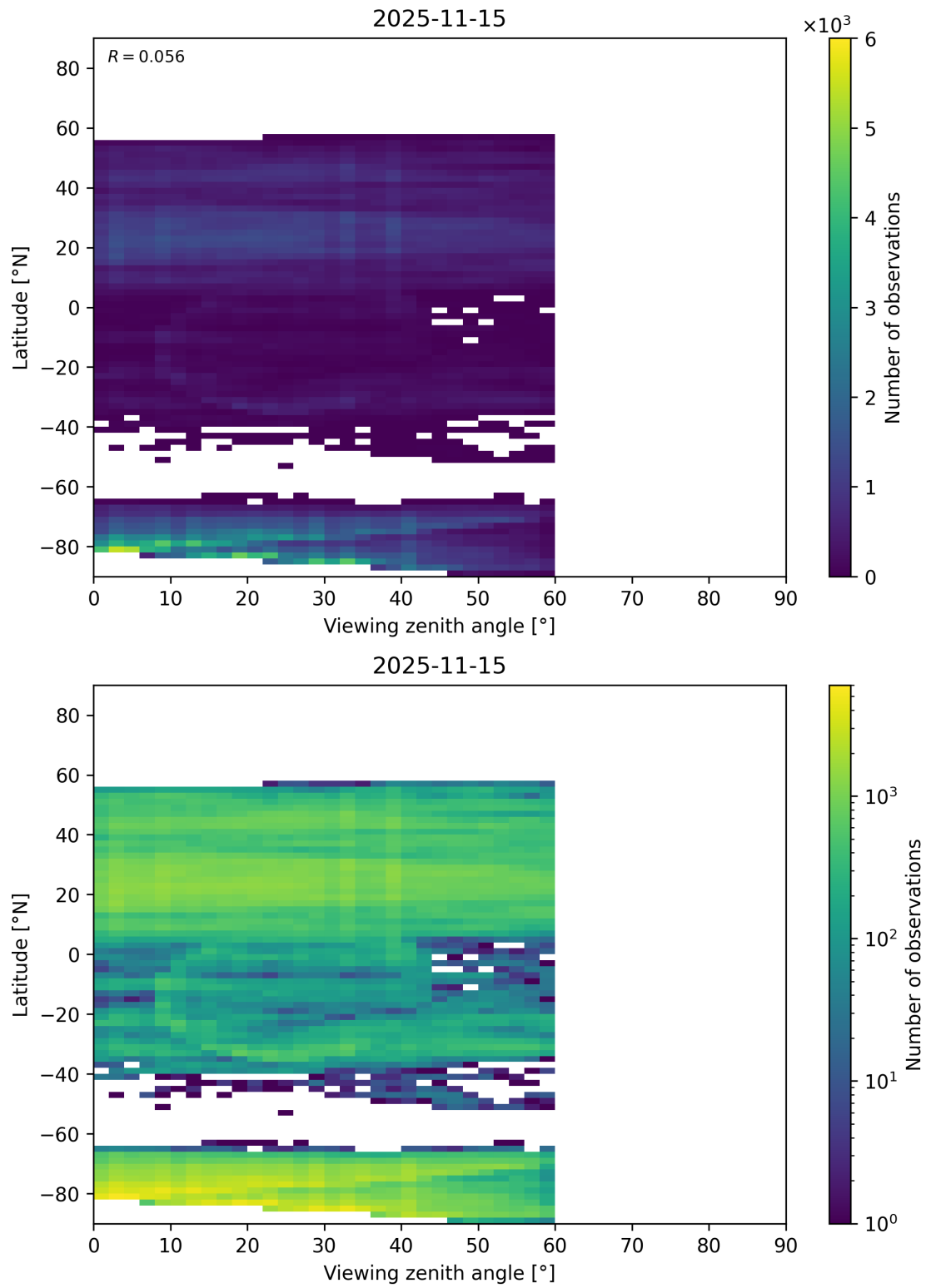
Figure 109: Scatter density plot of “Viewing zenith angle” against “Latitude” for 2025-11-14 to 2025-11-16.
