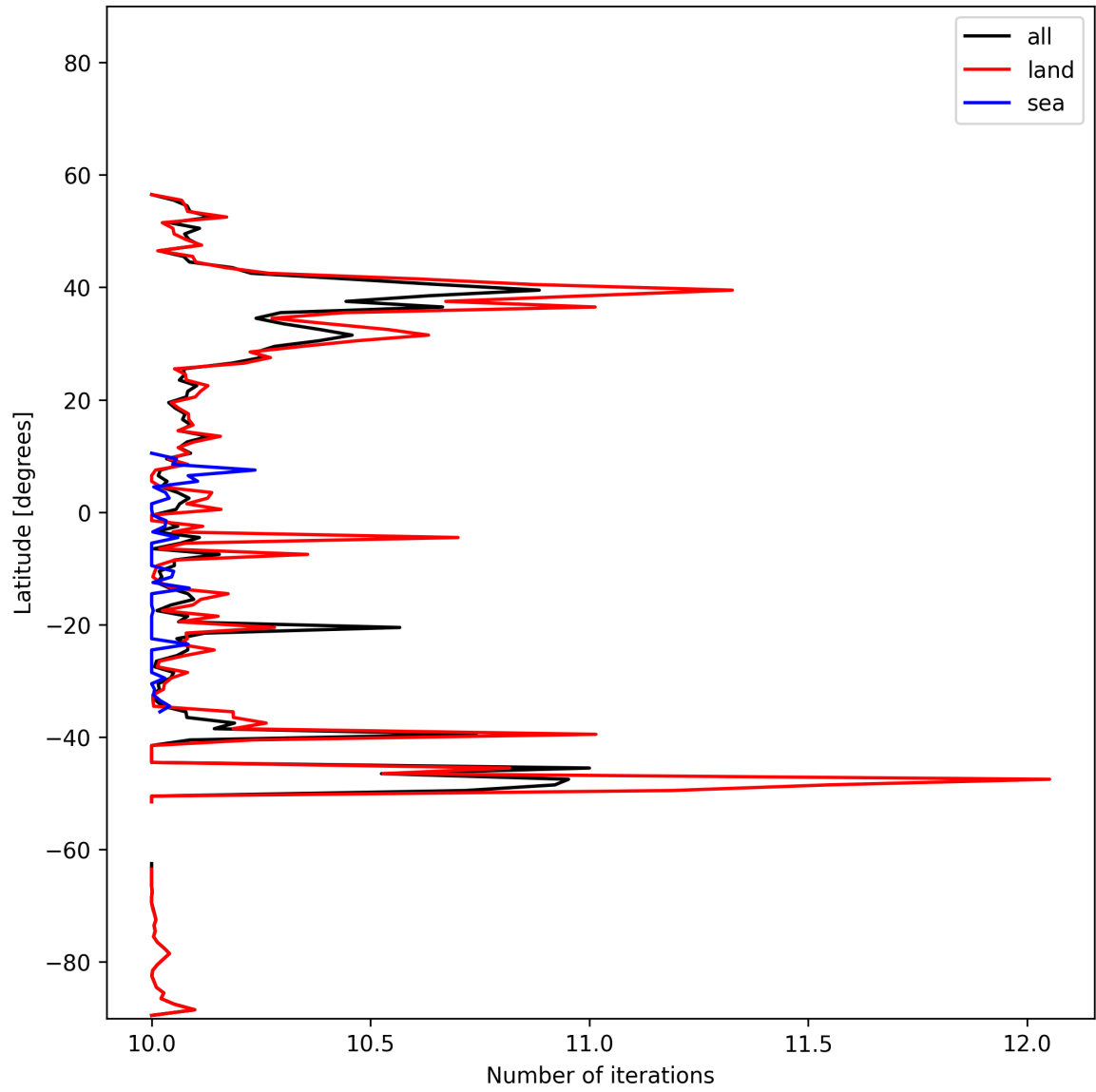
Figure 20: Zonal average of “Number of iterations” for 2025-11-14 to 2025-11-16.
