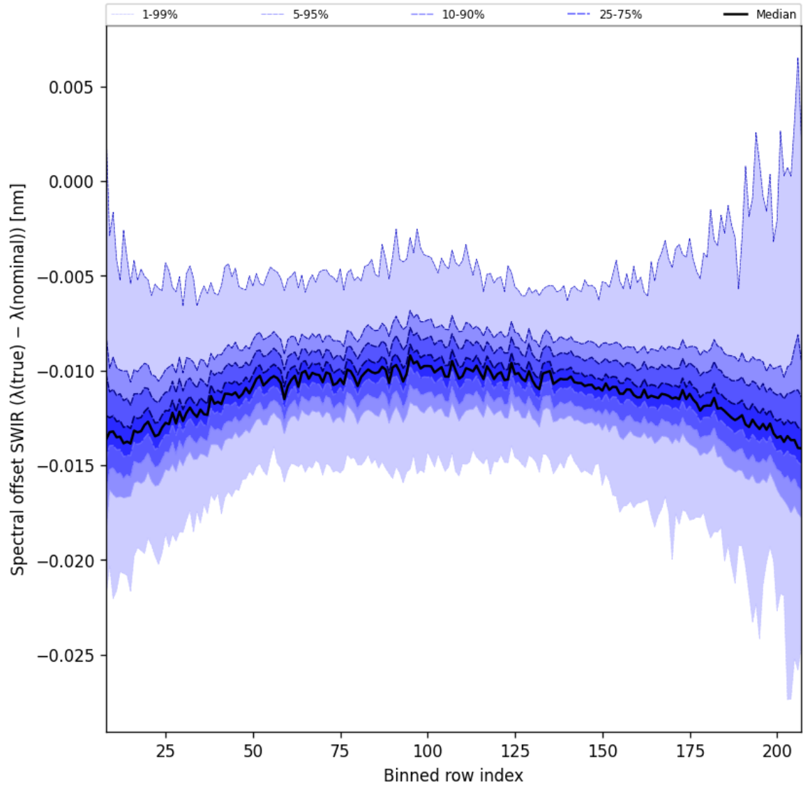
Figure 38: Along track statistics of “Spectral offset SWIR ( \lambda_{\text{true}} - \lambda_{\text{nominal}} )” for 2025-11-14 to 2025-11-16
