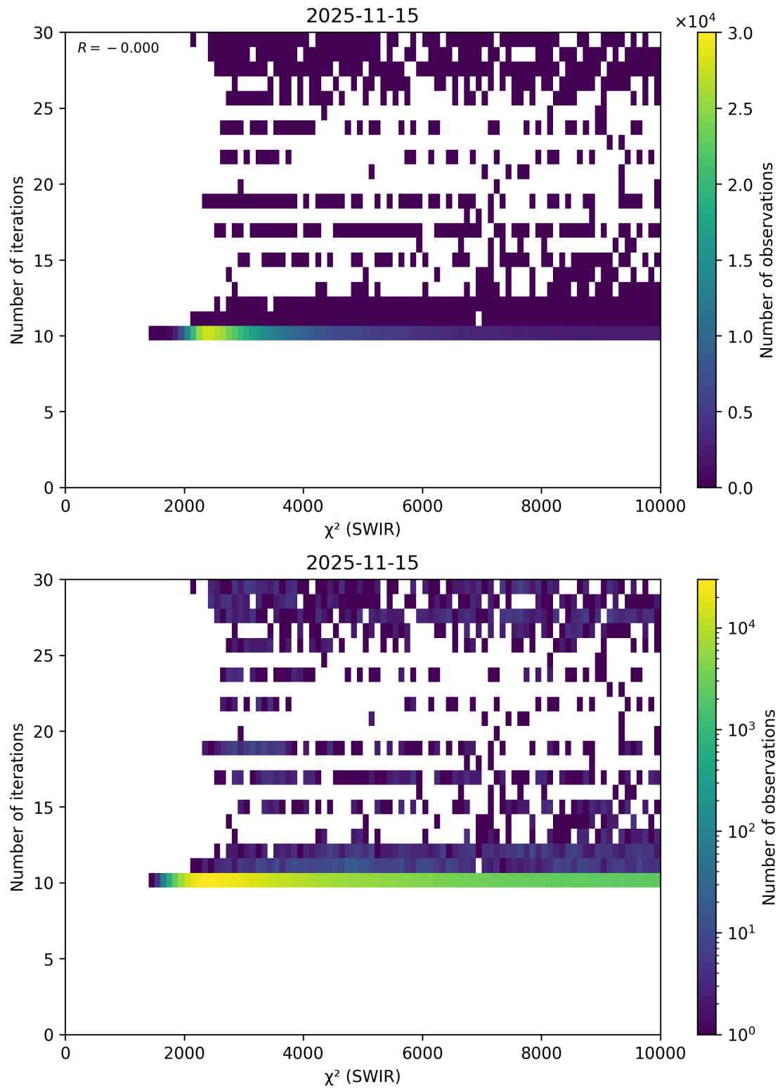
Figure 50: Scatter density plot of “ \chi^2 (SWIR)” against “Number of iterations” for 2025-11-14 to 2025-11-16.
