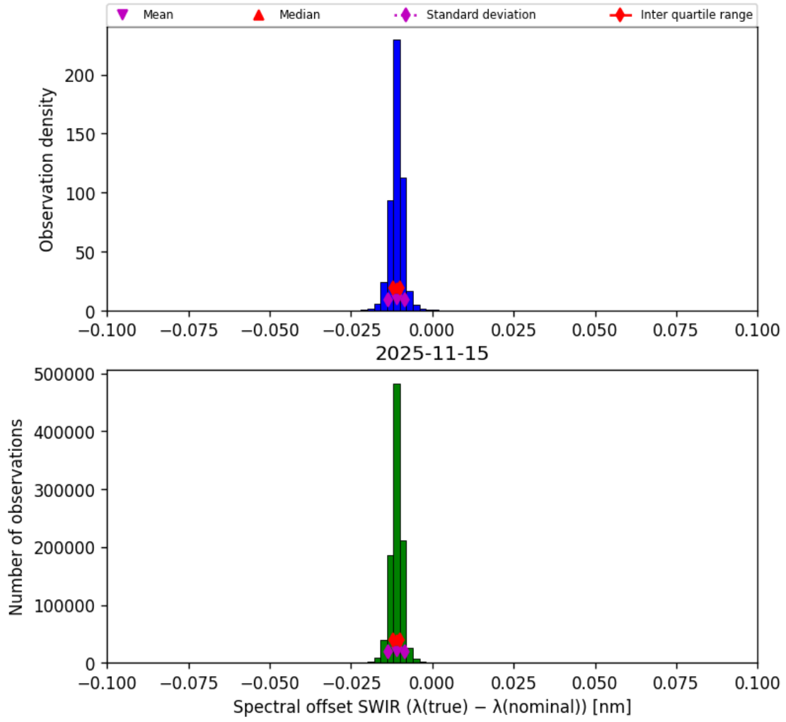
Figure 27: Histogram of “Spectral offset SWIR ( \lambda_{\text{true}} - \lambda_{\text{nominal}} )” for 2025-11-14 to 2025-11-16
