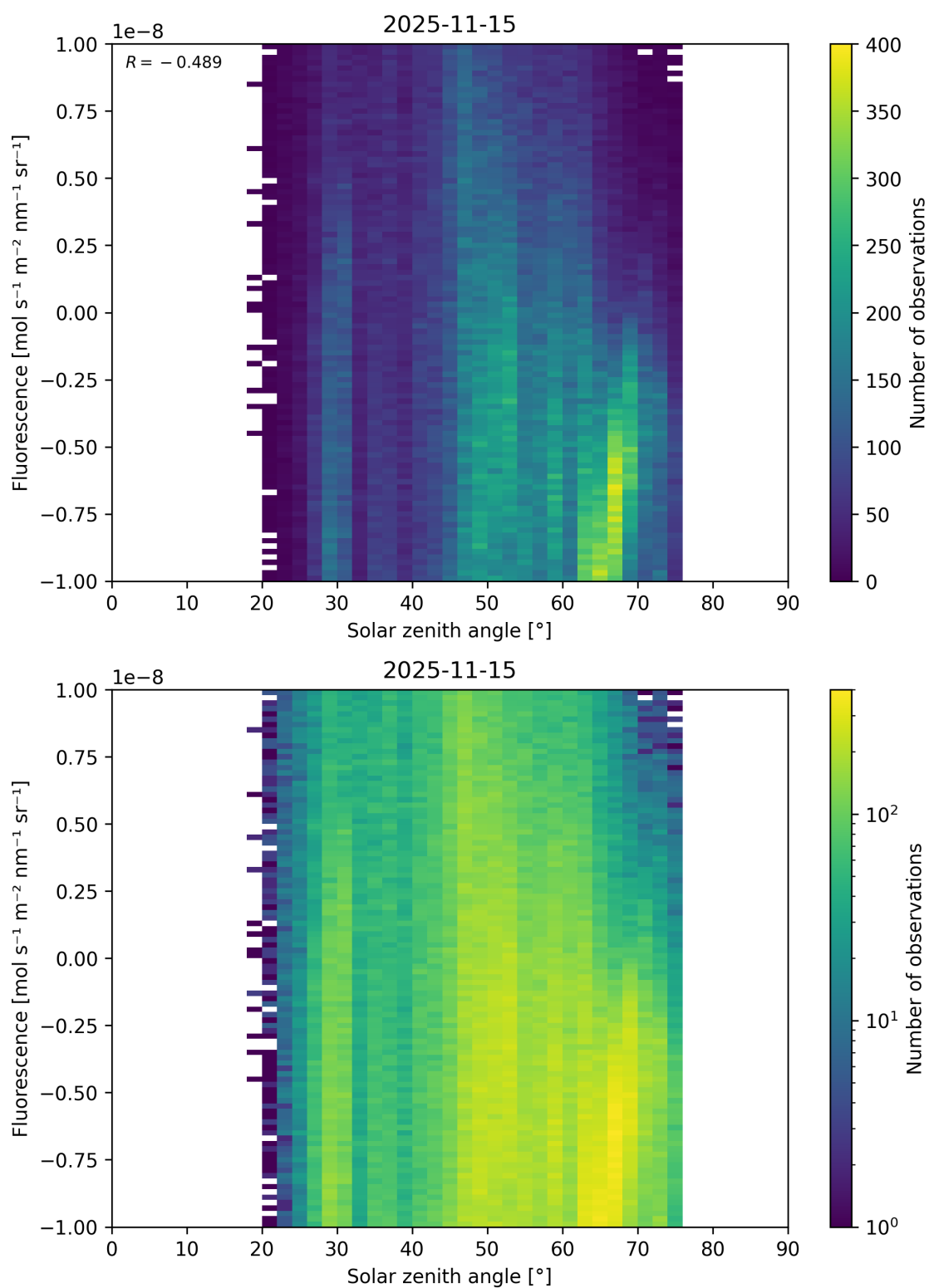
Figure 97: Scatter density plot of “Solar zenith angle” against “Fluorescence” for 2025-11-14 to 2025-11-16.
