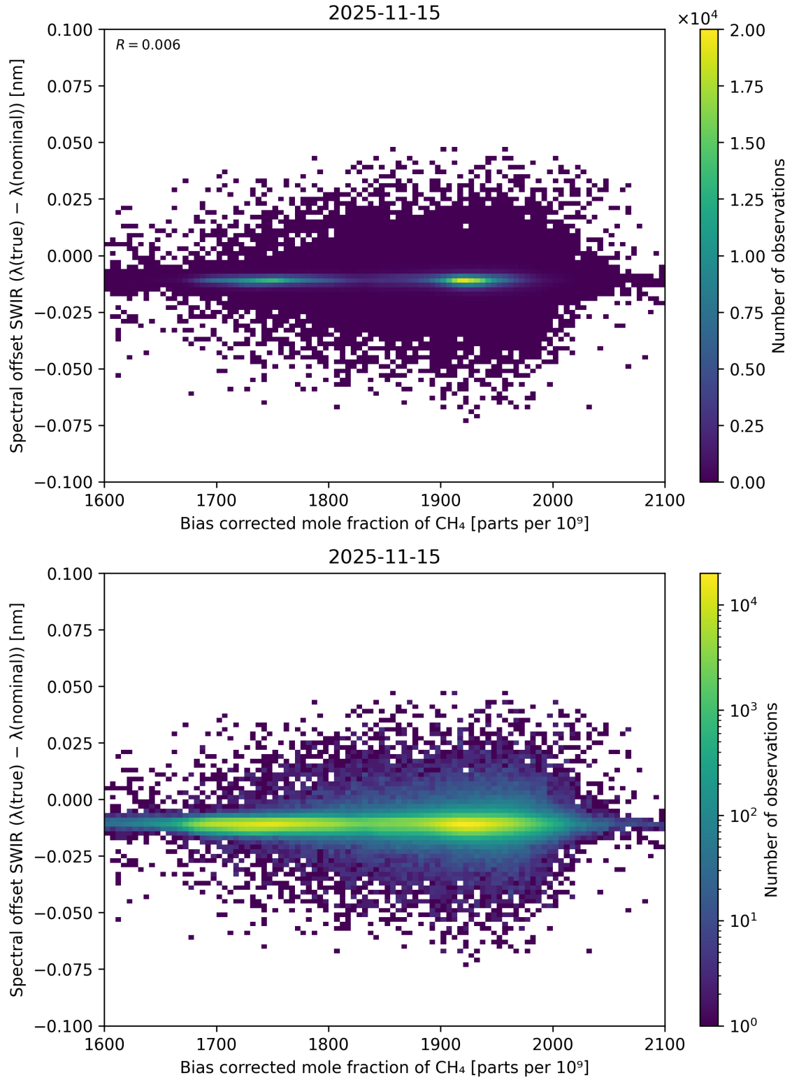
Figure 69: Scatter density plot of “Bias corrected mole fraction of \text{CH}_4 ” against “Spectral offset SWIR ( \lambda_{\text{true}} - \lambda_{\text{nominal}} )” for 2025-11-14 to 2025-11-16.
