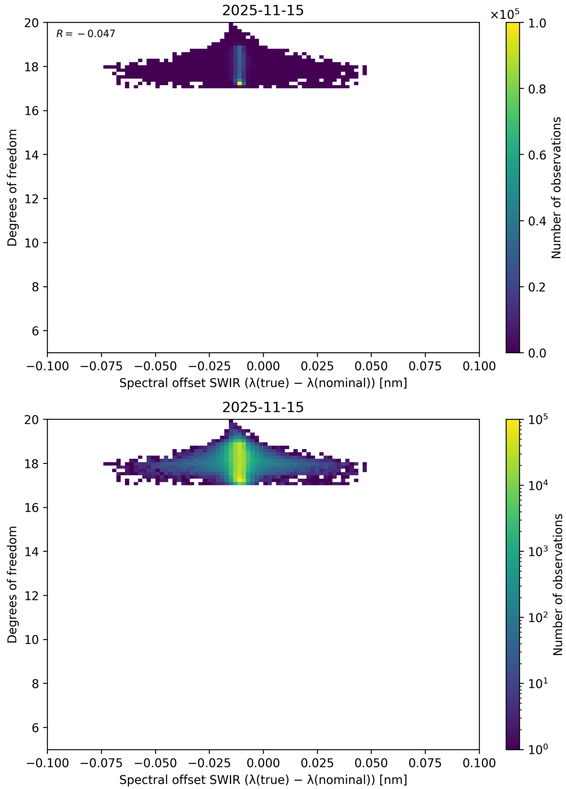
Figure 119: Scatter density plot of “Spectral offset SWIR ( \lambda_{\text{true}} - \lambda_{\text{nominal}} )” against “Degrees of freedom” for 2025-11-14 to 2025-11-16.
