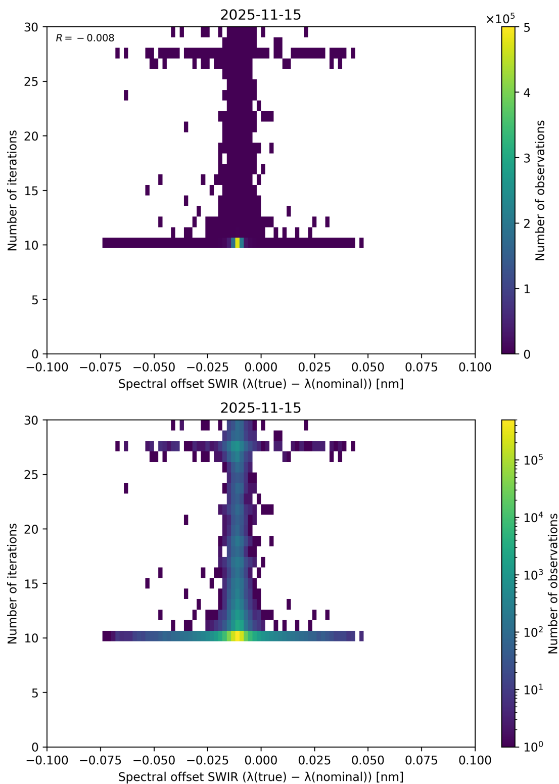
Figure 121: Scatter density plot of “Spectral offset SWIR ( \lambda_{\text{true}} - \lambda_{\text{nominal}} )” against “Number of iterations” for 2025-11-14 to 2025-11-16.
