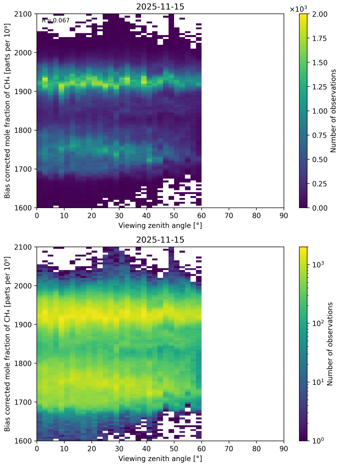
Figure 111: Scatter density plot of “Viewing zenith angle” against “Bias corrected mole fraction of CH 4 ” for 2025-11-14 to 2025-11-16.
