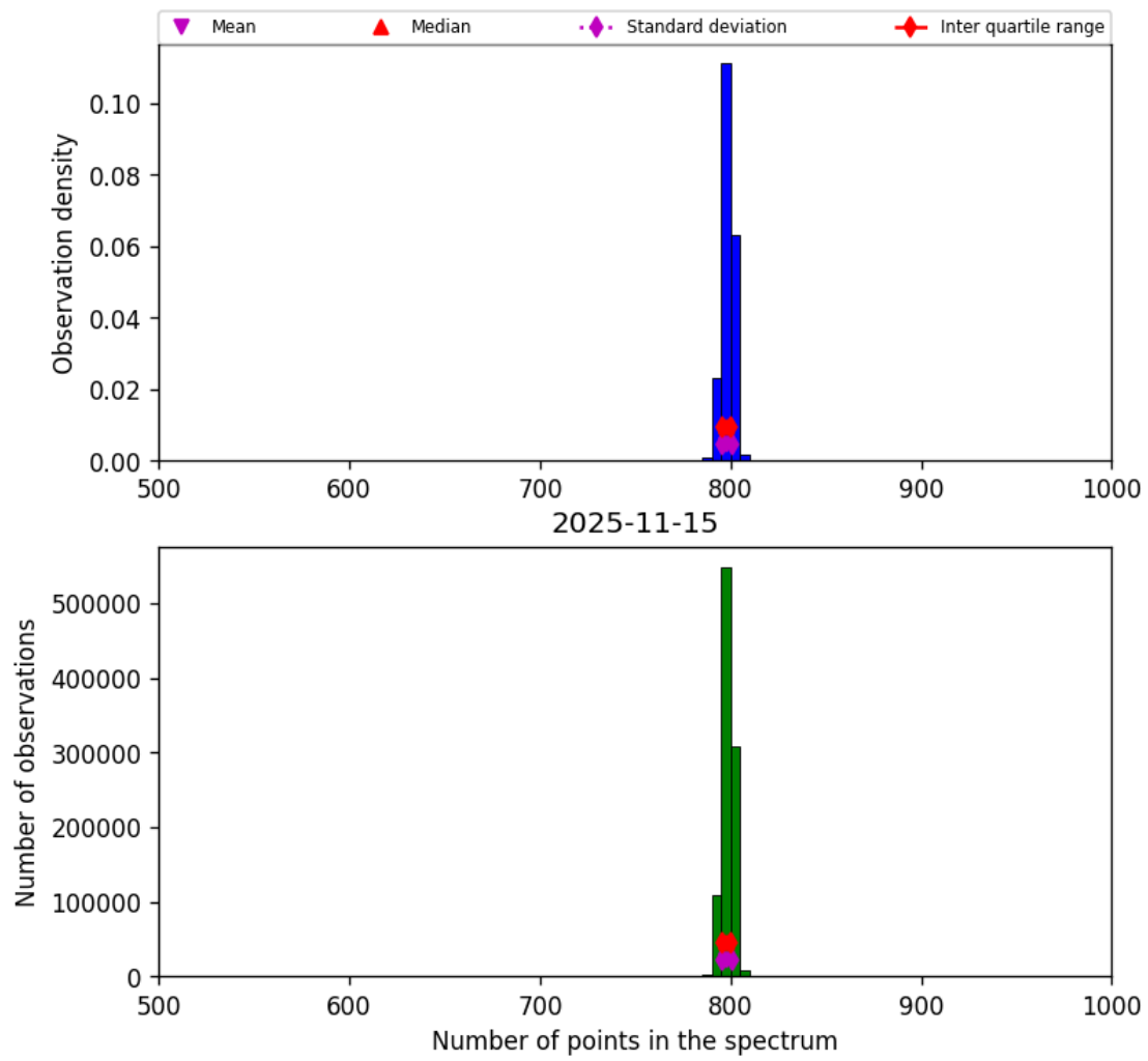
Figure 26: Histogram of “Number of points in the spectrum” for 2025-11-14 to 2025-11-16
