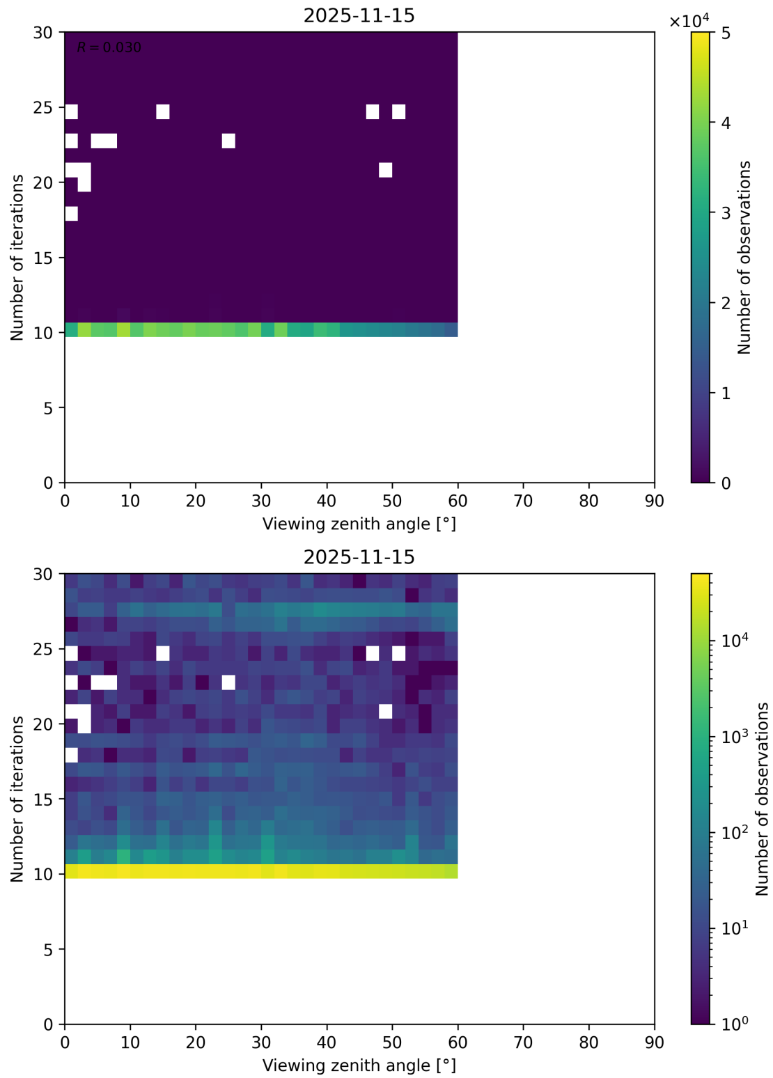
Figure 113: Scatter density plot of “Viewing zenith angle” against “Number of iterations” for 2025-11-14 to 2025-11-16.
