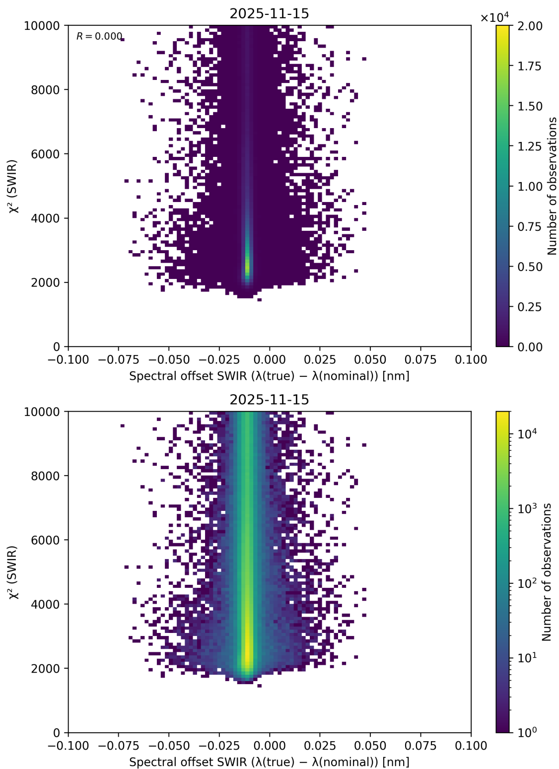
Figure 118: Scatter density plot of “Spectral offset SWIR ( \lambda_{\text{true}} - \lambda_{\text{nominal}} )” against “ \chi^2 (SWIR)” for 2025-11-14 to 2025-11-16.
