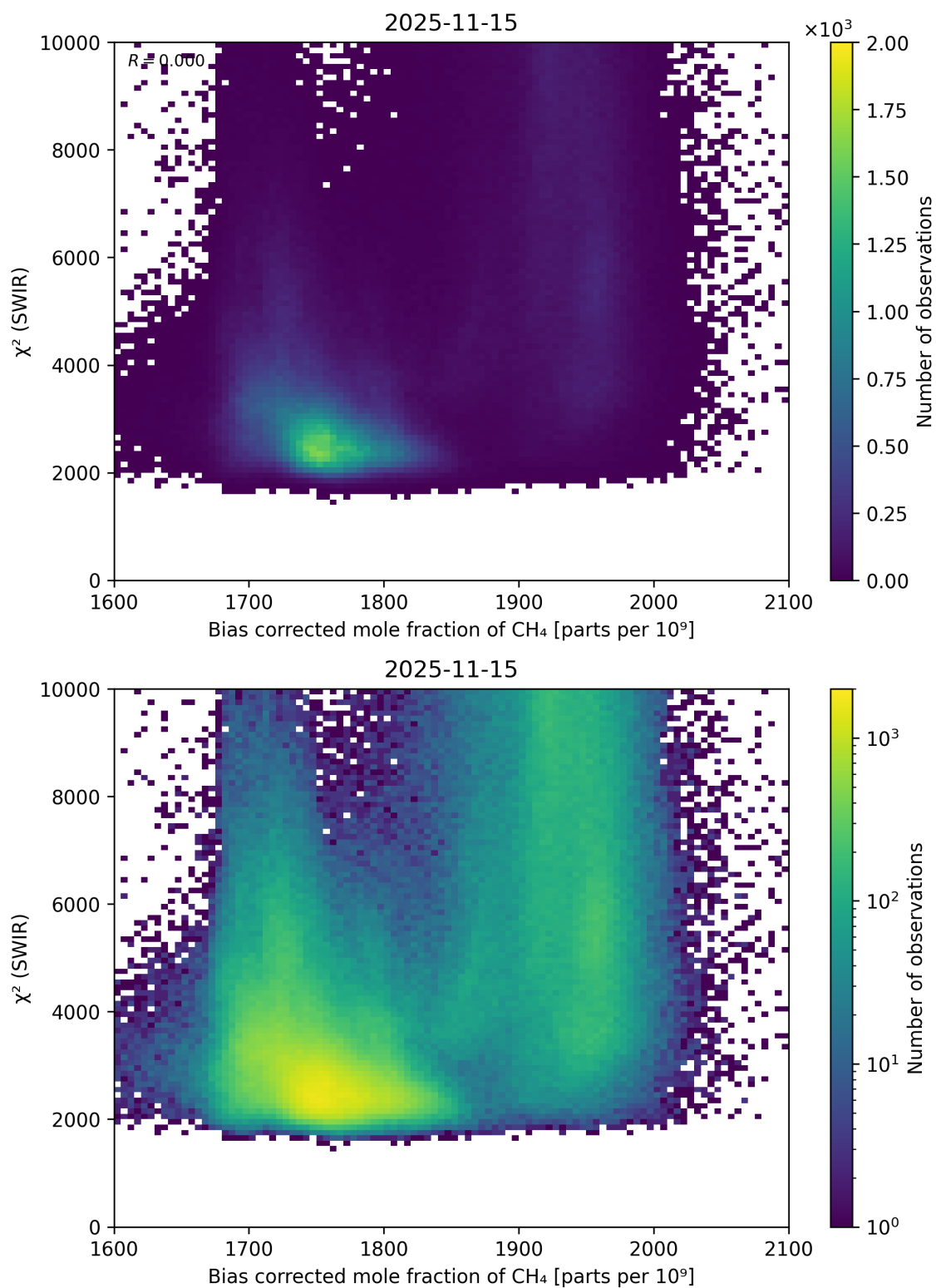
Figure 64: Scatter density plot of “Bias corrected mole fraction of CH 4 ” against “ \chi^2 (SWIR)” for 2025-11-14 to 2025-11-16.
