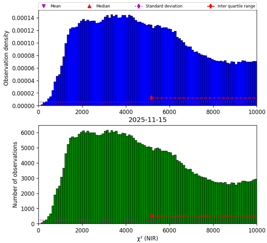
Figure 29: Histogram of " \chi^2 (NIR)" for 2025-11-14 to 2025-11-16
