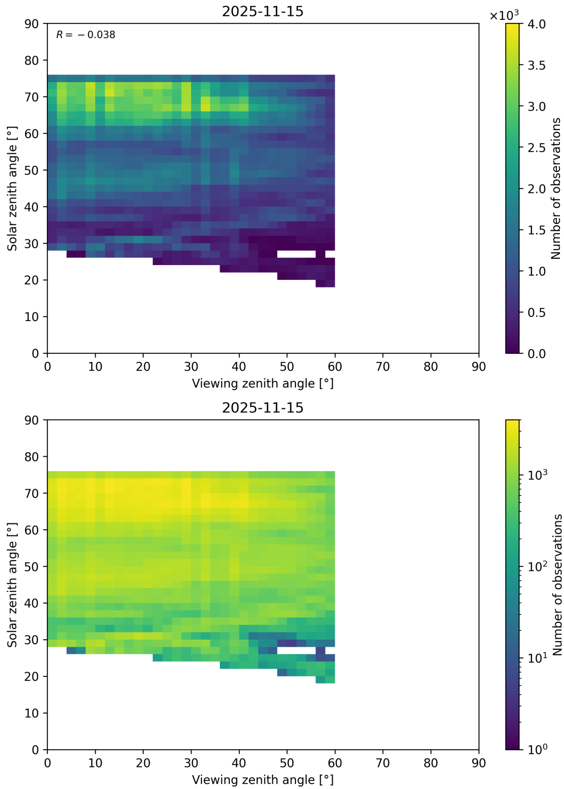
Figure 115: Scatter density plot of “Viewing zenith angle” against “Solar zenith angle” for 2025-11-14 to 2025-11-16.
