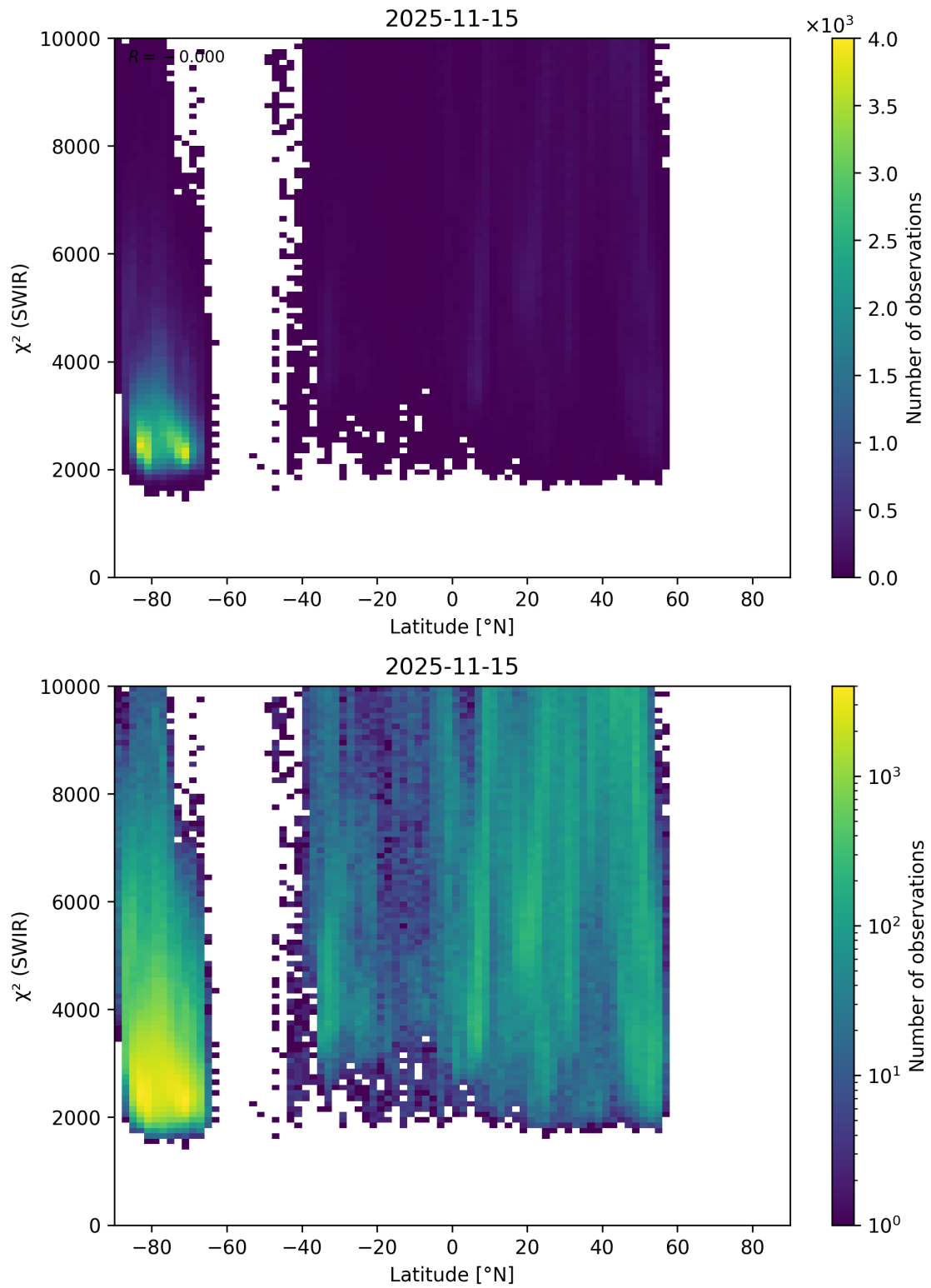
Figure 54: Scatter density plot of “Latitude” against “ \chi^2 (SWIR)” for 2025-11-14 to 2025-11-16.
