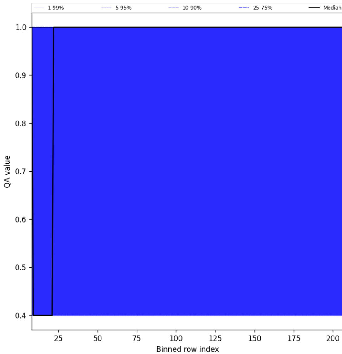
Figure 33: Along track statistics of “QA value” for 2025-11-14 to 2025-11-16
