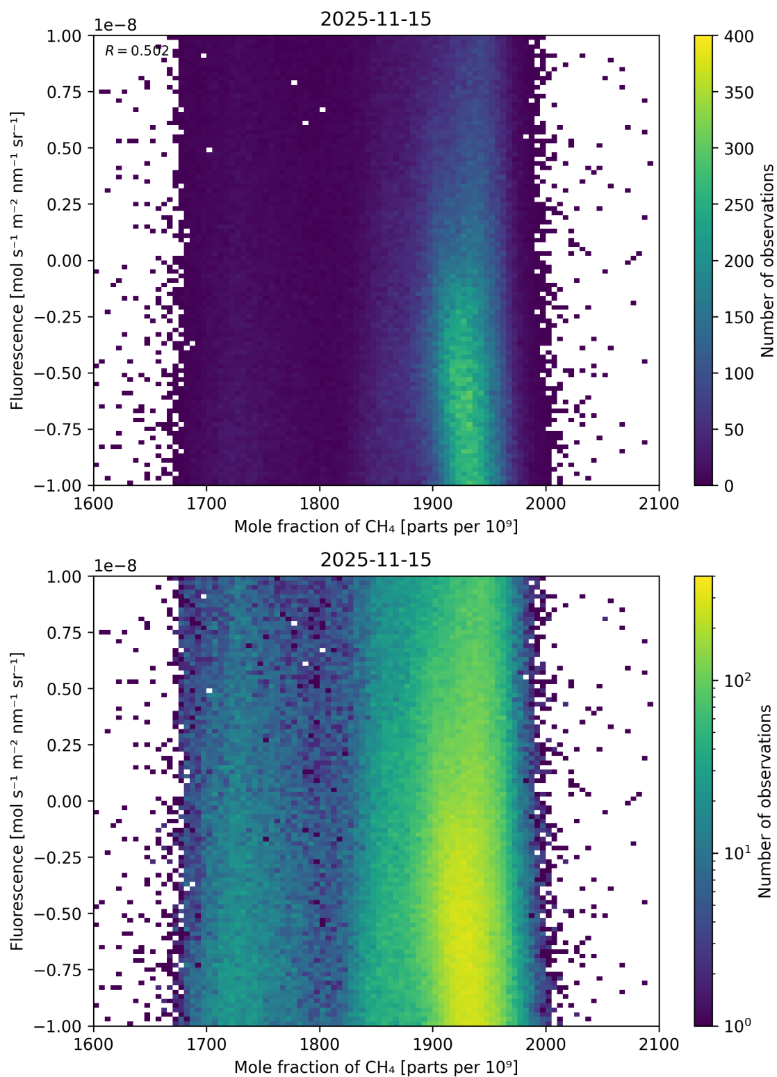
Figure 73: Scatter density plot of “Mole fraction of \text{CH}_4 ” against “Fluorescence” for 2025-11-14 to 2025-11-16.
