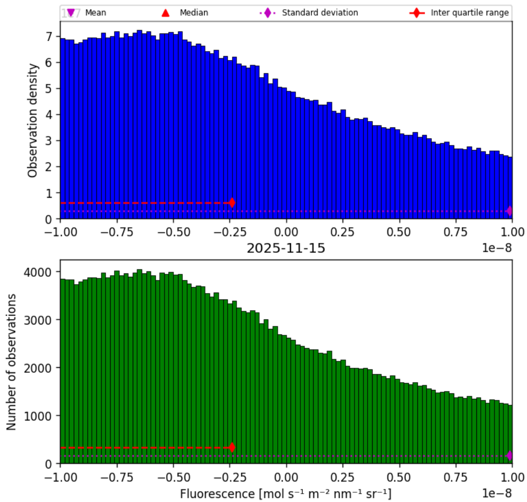
Figure 32: Histogram of “Fluorescence” for 2025-11-14 to 2025-11-16
