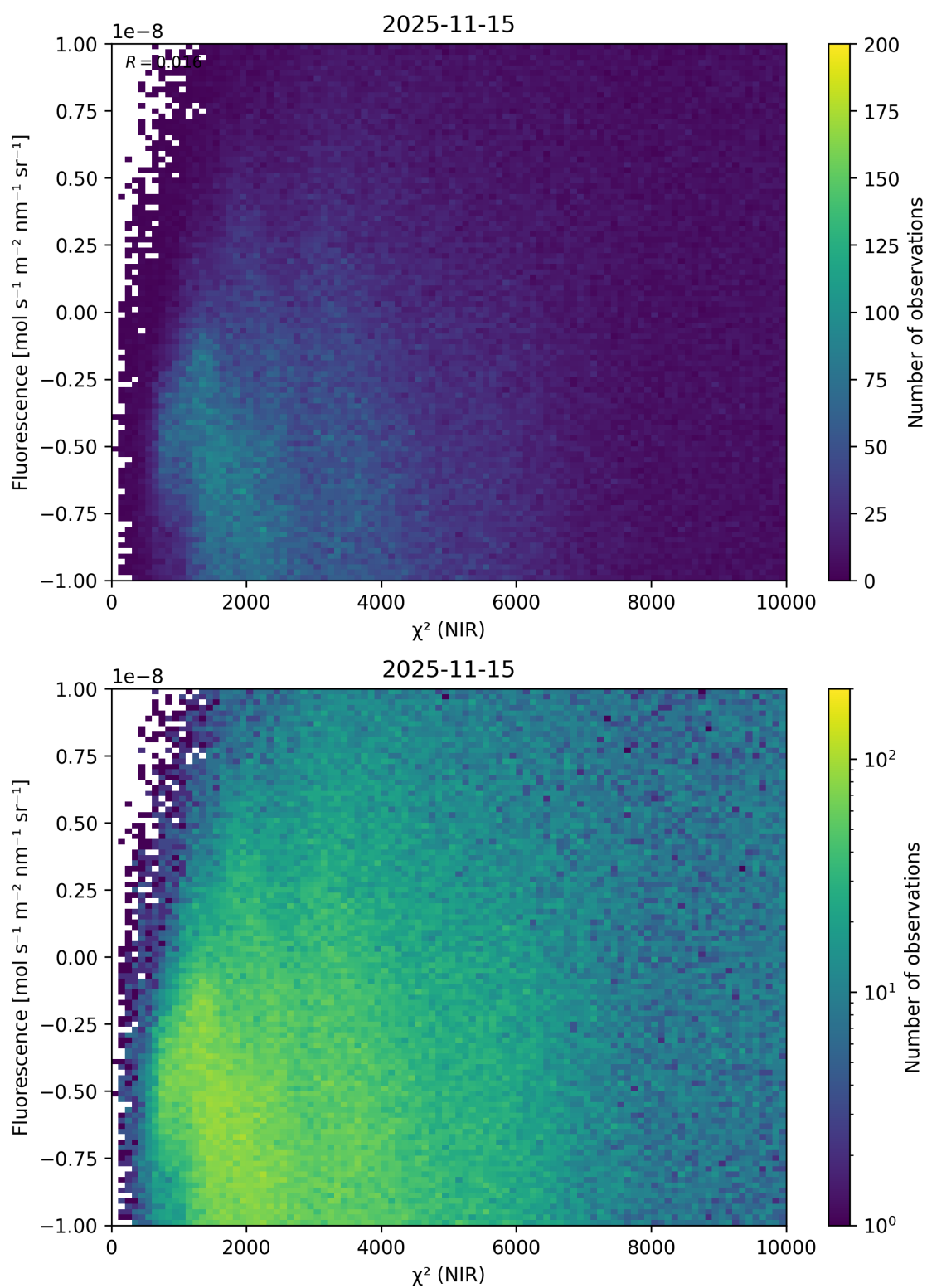
Figure 45: Scatter density plot of “ \chi^2 (NIR)” against “Fluorescence” for 2025-11-14 to 2025-11-16.
