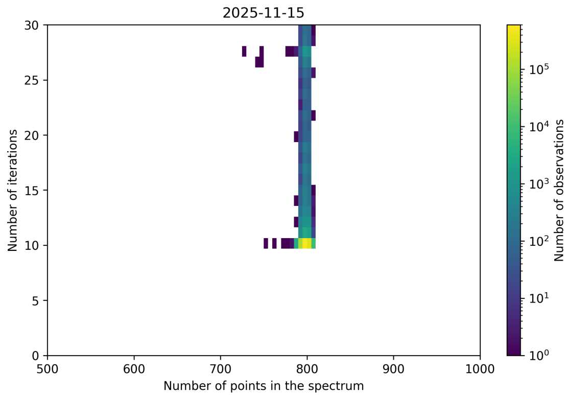
Figure 92: Scatter density plot of “Number of points in the spectrum” against “Number of iterations” for 2025-11-14 to 2025-11-16.
