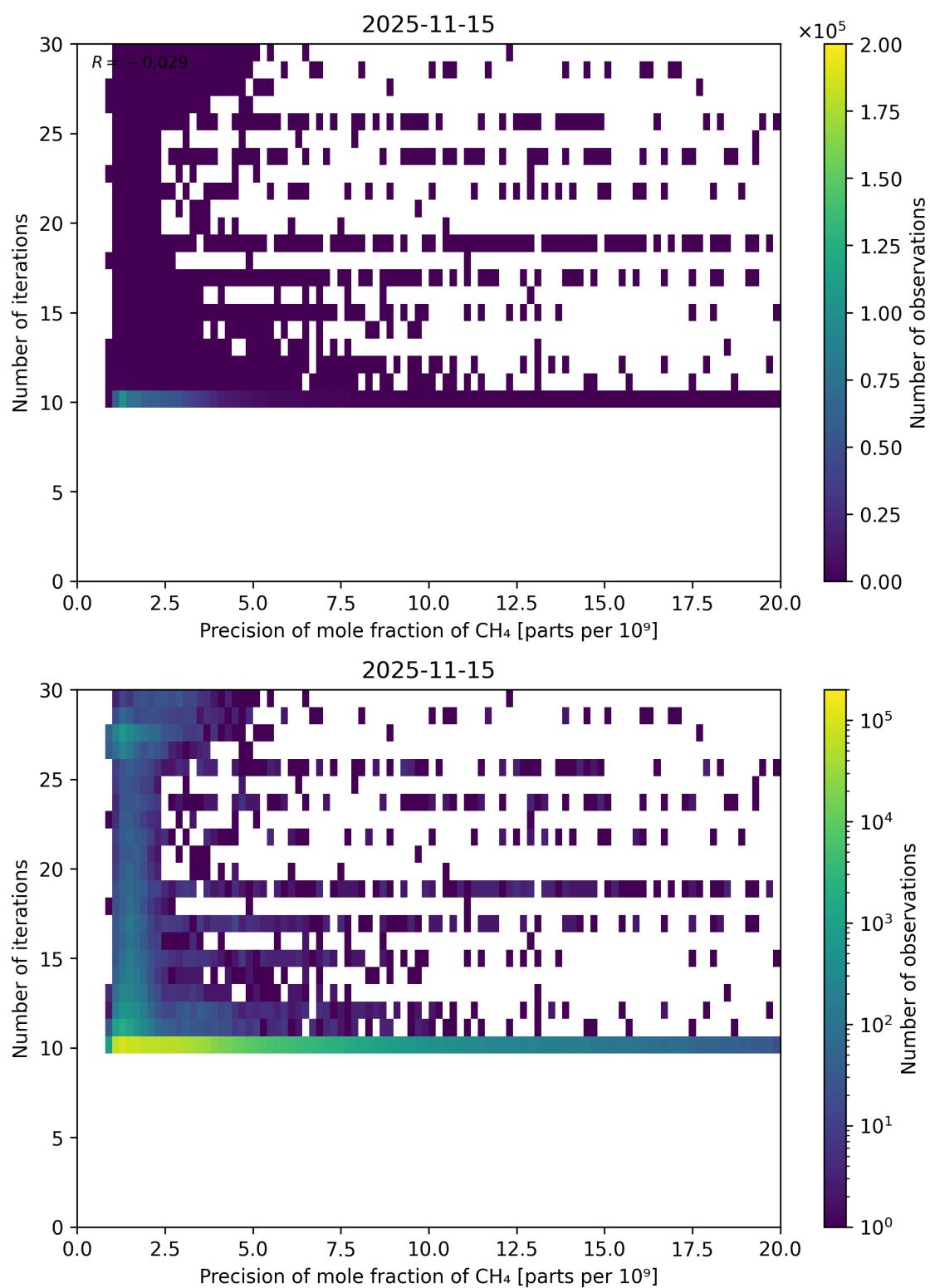
Figure 83: Scatter density plot of “Precision of mole fraction of CH 4 ” against “Number of iterations” for 2025-11-14 to 2025-11-16.
