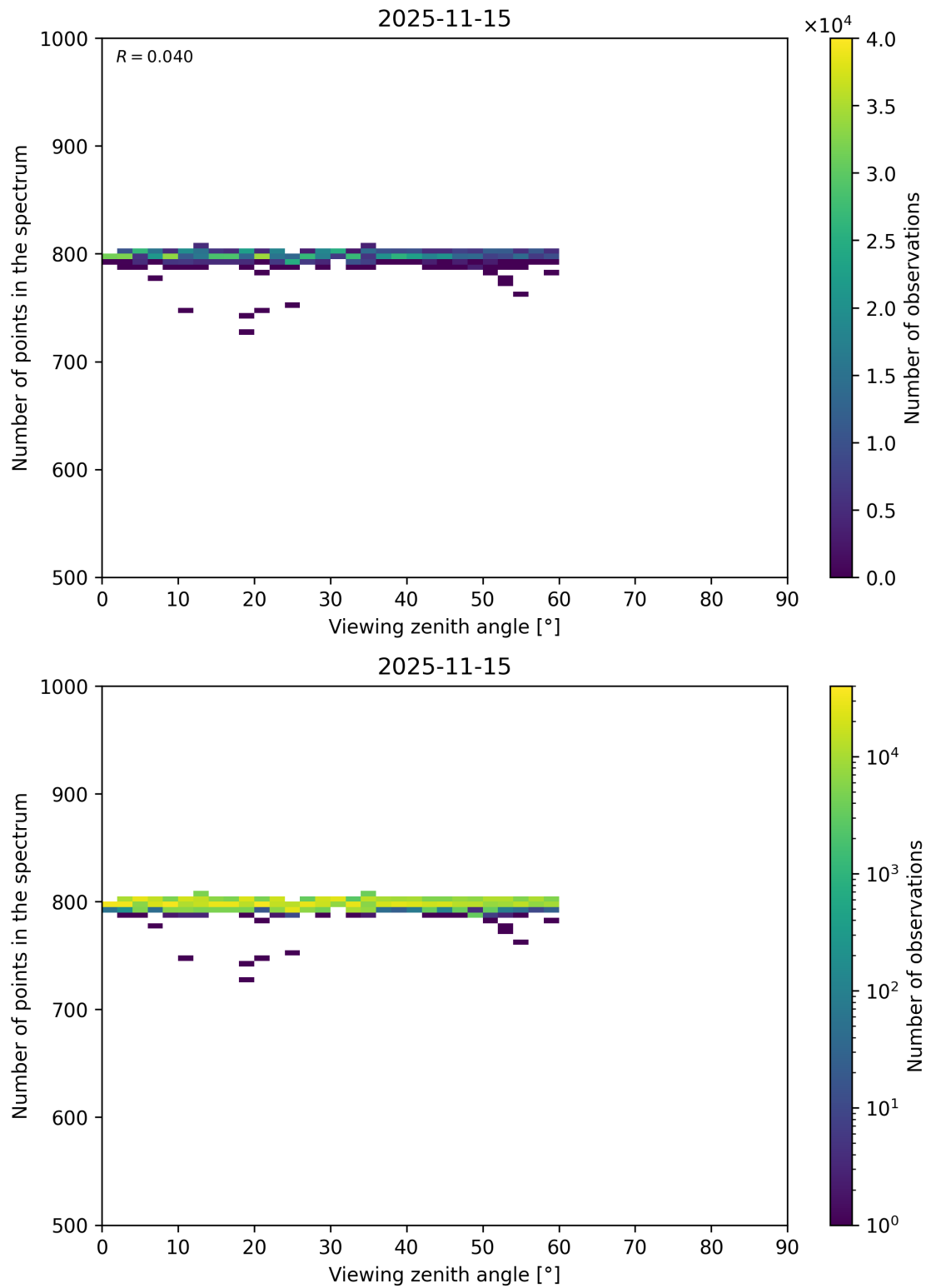
Figure 114: Scatter density plot of “Viewing zenith angle” against “Number of points in the spectrum” for 2025-11-14 to 2025-11-16.
