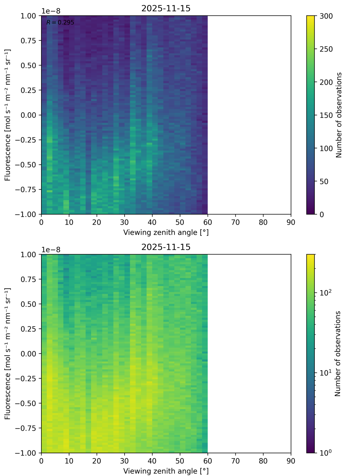
Figure 108: Scatter density plot of “Viewing zenith angle” against “Fluorescence” for 2025-11-14 to 2025-11-16.
