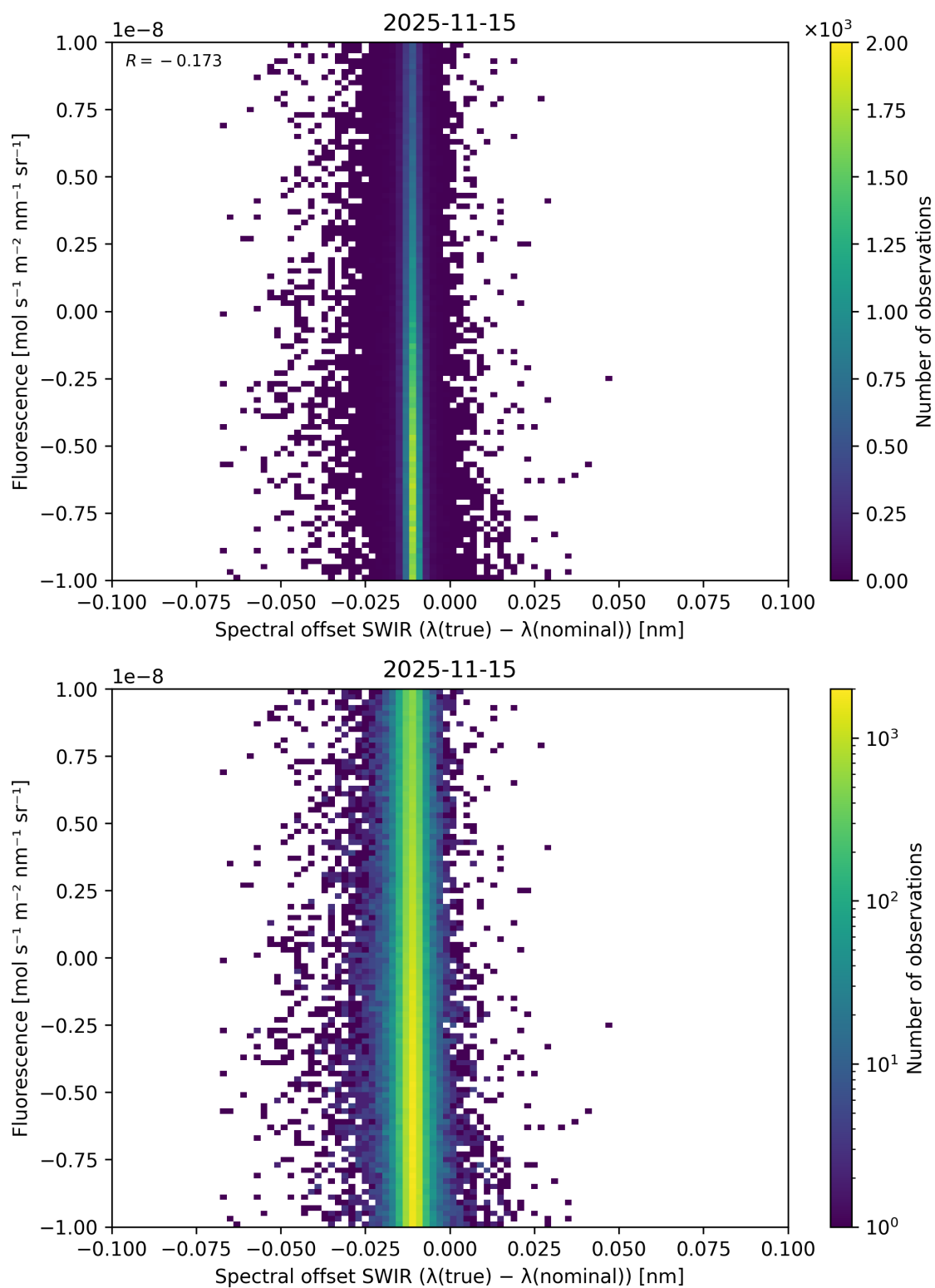
Figure 120: Scatter density plot of “Spectral offset SWIR ( \lambda_{\text{true}} - \lambda_{\text{nominal}} )” against “Fluorescence” for 2025-11-14 to 2025-11-16.
