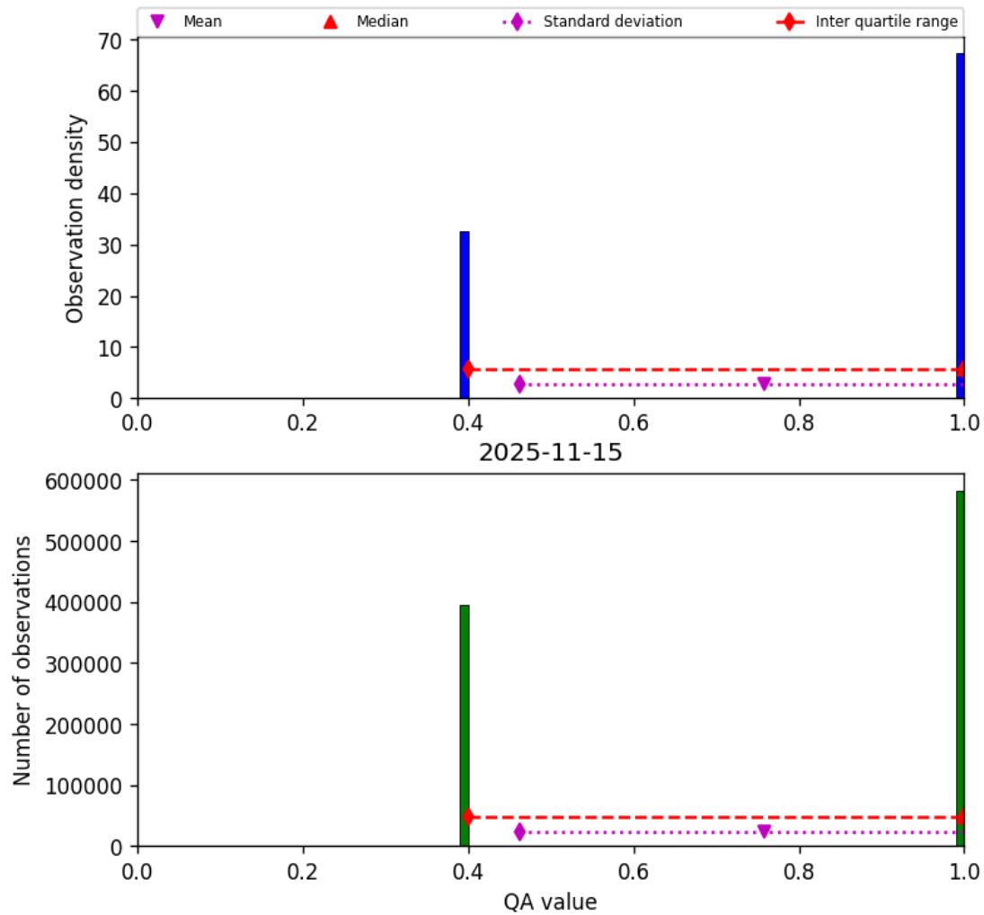
Figure 22: Histogram of “QA value” for 2025-11-14 to 2025-11-16
