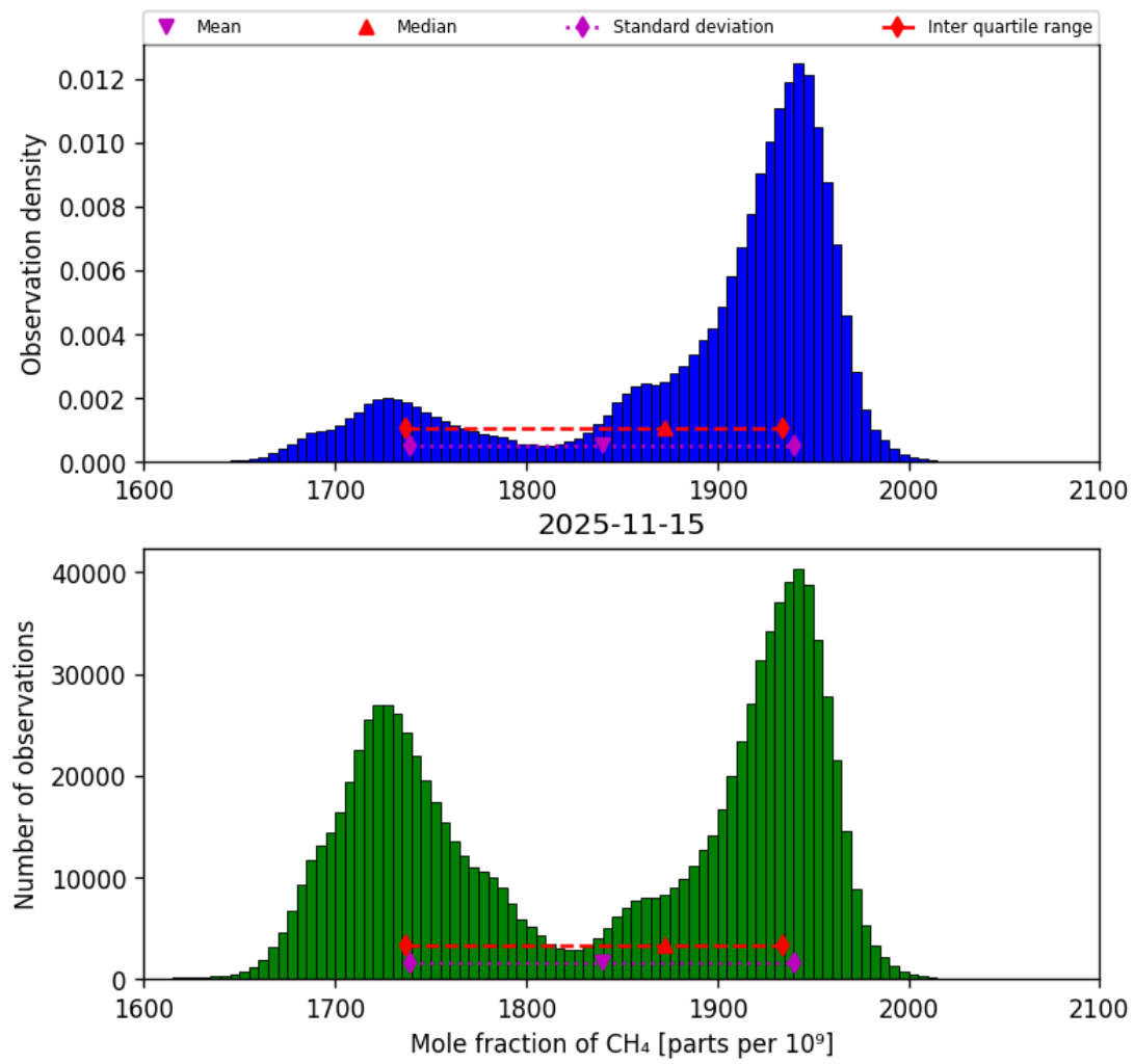
Figure 23: Histogram of “Mole fraction of CH 4 ” for 2025-11-14 to 2025-11-16
