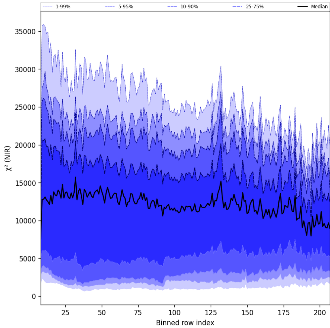
Figure 40: Along track statistics of “ \chi^2 (NIR)” for 2025-11-14 to 2025-11-16
