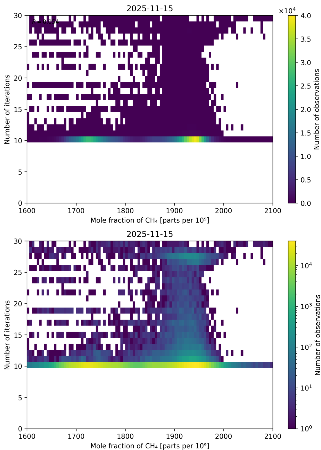
Figure 76: Scatter density plot of “Mole fraction of CH 4 ” against “Number of iterations” for 2025-11-14 to 2025-11-16.
