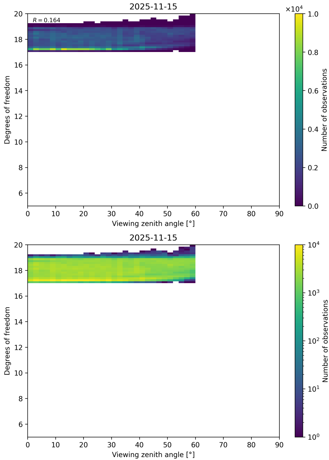
Figure 107: Scatter density plot of “Viewing zenith angle” against “Degrees of freedom” for 2025-11-14 to 2025-11-16.
