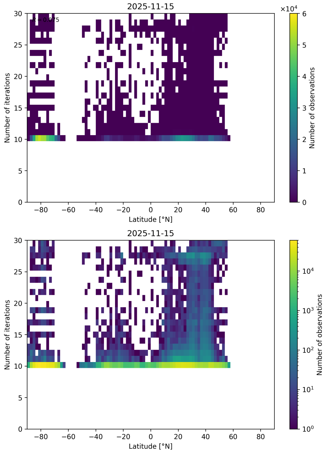
Figure 60: Scatter density plot of “Latitude” against “Number of iterations” for 2025-11-14 to 2025-11-16.
