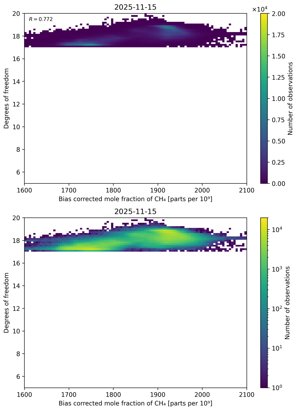
Figure 65: Scatter density plot of “Bias corrected mole fraction of CH 4 ” against “Degrees of freedom” for 2025-11-14 to 2025-11-16.
