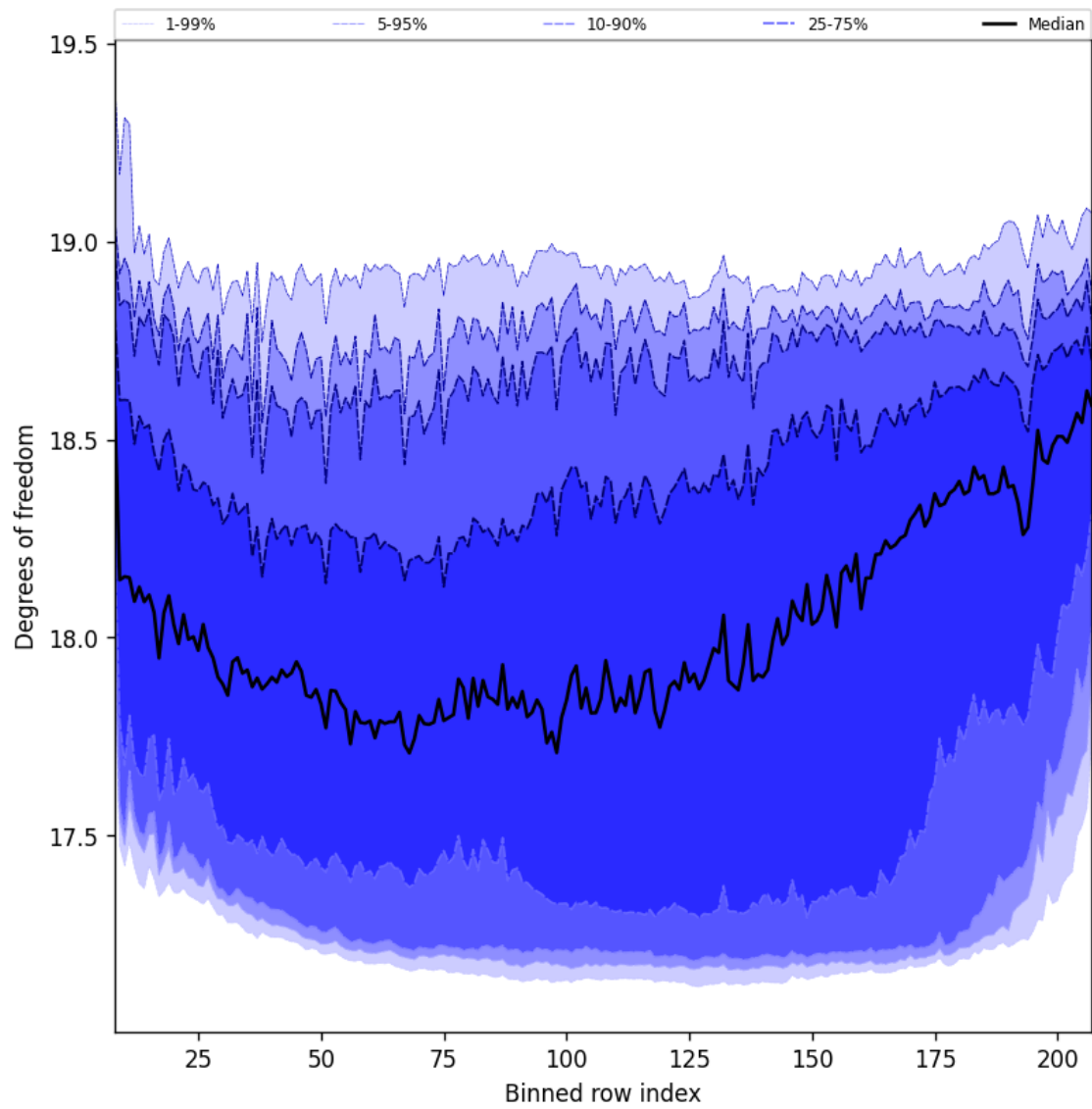
Figure 41: Along track statistics of “Degrees of freedom” for 2025-11-15 to 2025-11-17
