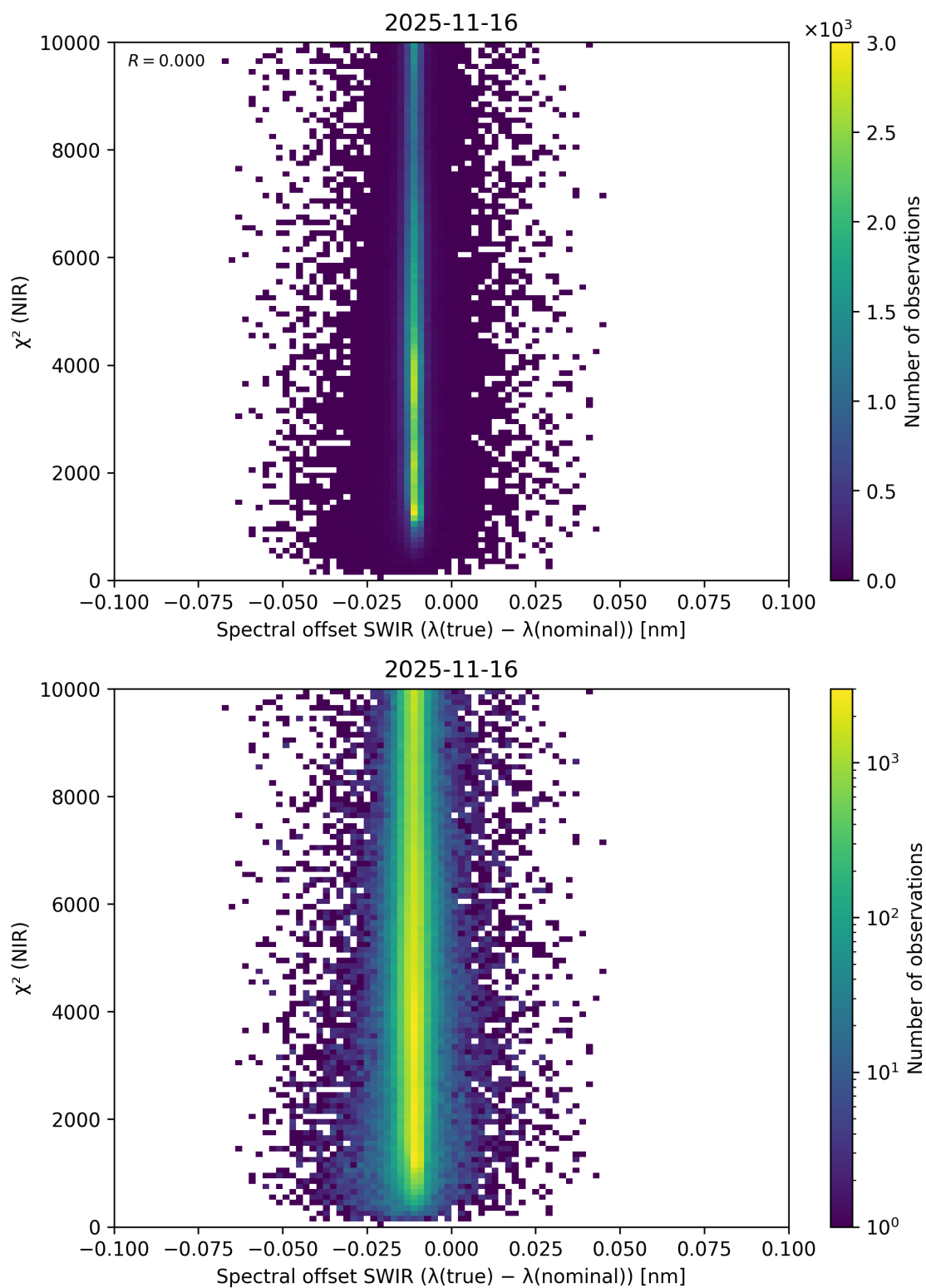
Figure 117: Scatter density plot of “Spectral offset SWIR ( \lambda_{\text{true}} - \lambda_{\text{nominal}} )” against “ \chi^2 (NIR)” for 2025-11-15 to 2025-11-17.
