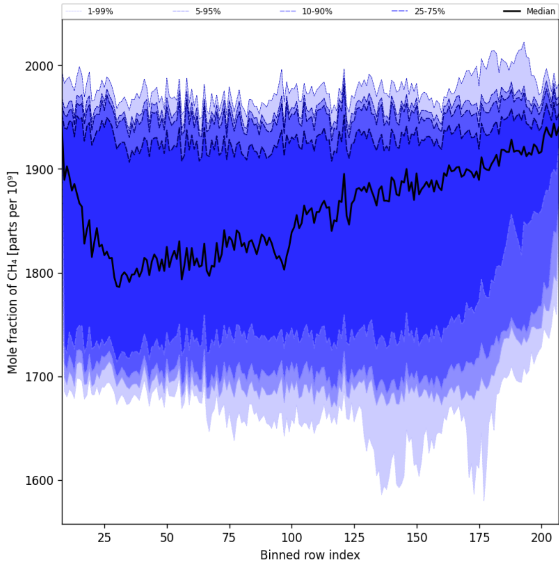
Figure 34: Along track statistics of “Mole fraction of CH 4 ” for 2025-11-15 to 2025-11-17
