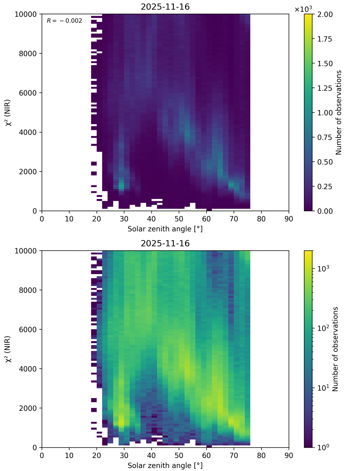
Figure 94: Scatter density plot of “Solar zenith angle” against “ \chi^2 (NIR)” for 2025-11-15 to 2025-11-17.
