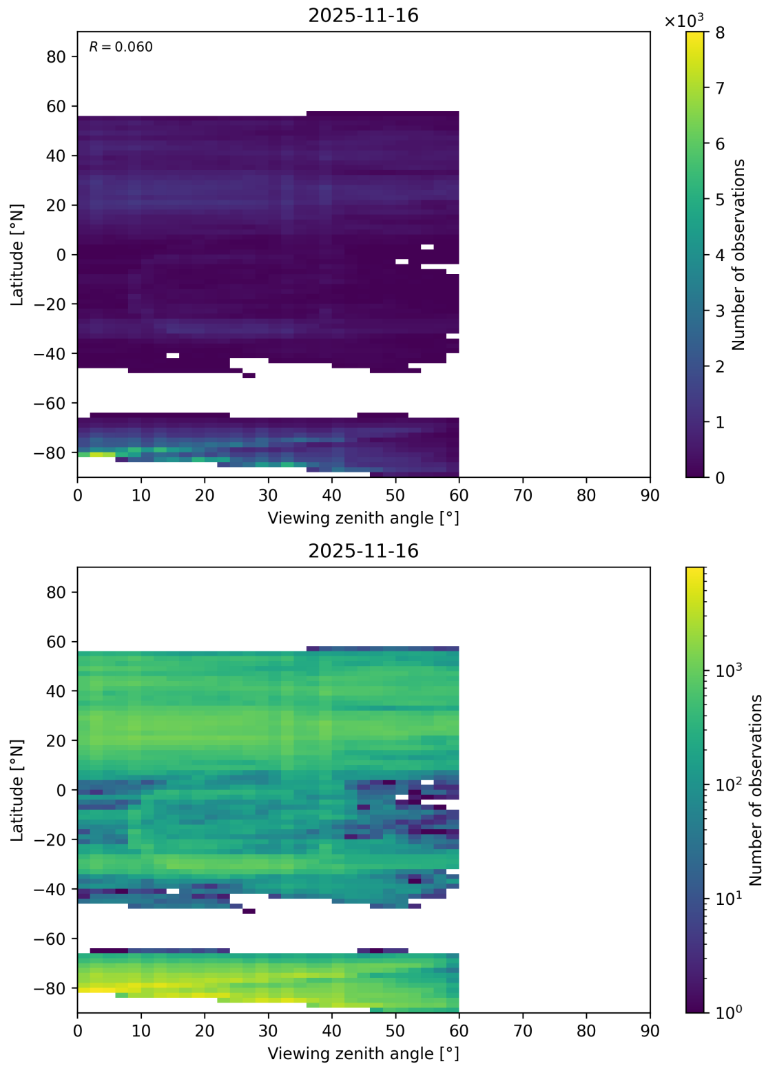
Figure 109: Scatter density plot of “Viewing zenith angle” against “Latitude” for 2025-11-15 to 2025-11-17.
