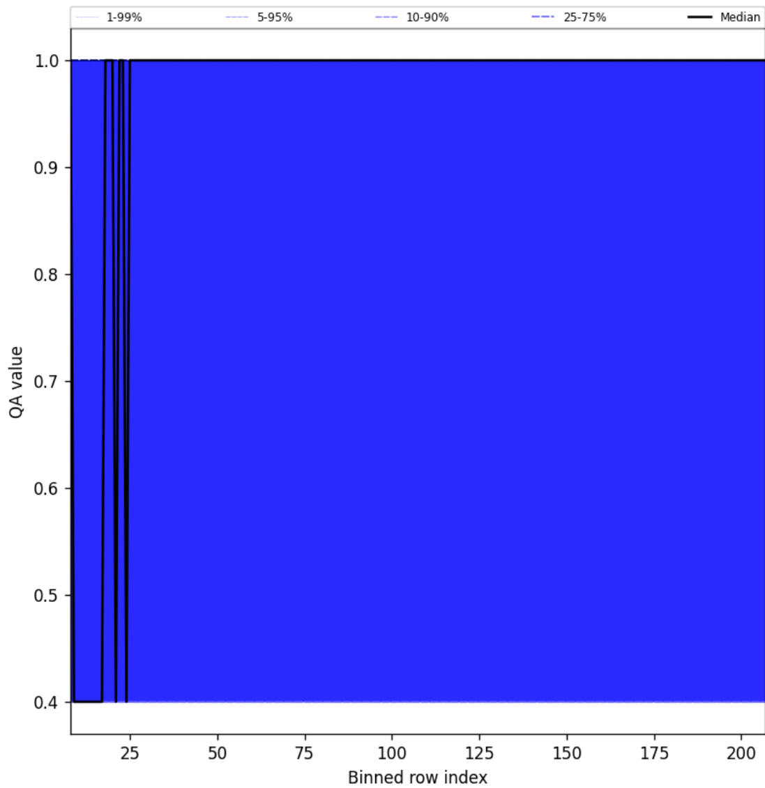
Figure 33: Along track statistics of “QA value” for 2025-11-15 to 2025-11-17
