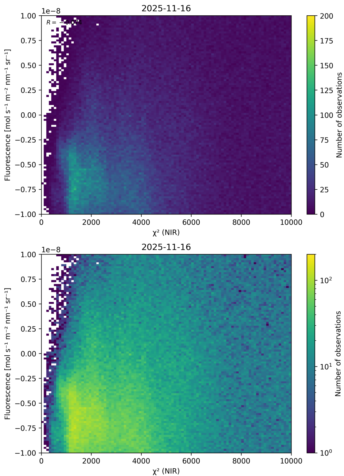
Figure 45: Scatter density plot of “ \chi^2 (NIR)” against “Fluorescence” for 2025-11-15 to 2025-11-17.
