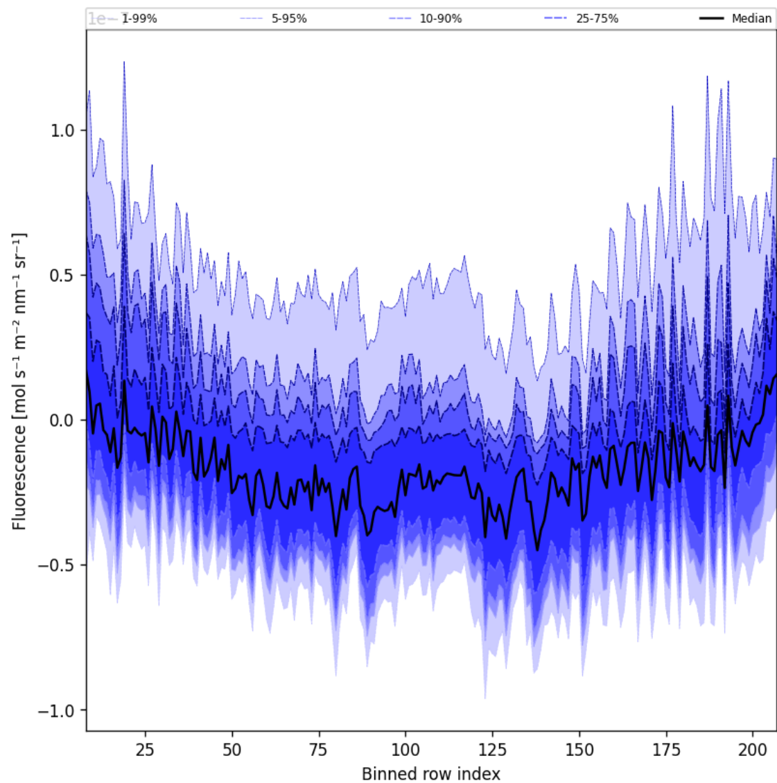
Figure 43: Along track statistics of “Fluorescence” for 2025-11-15 to 2025-11-17
