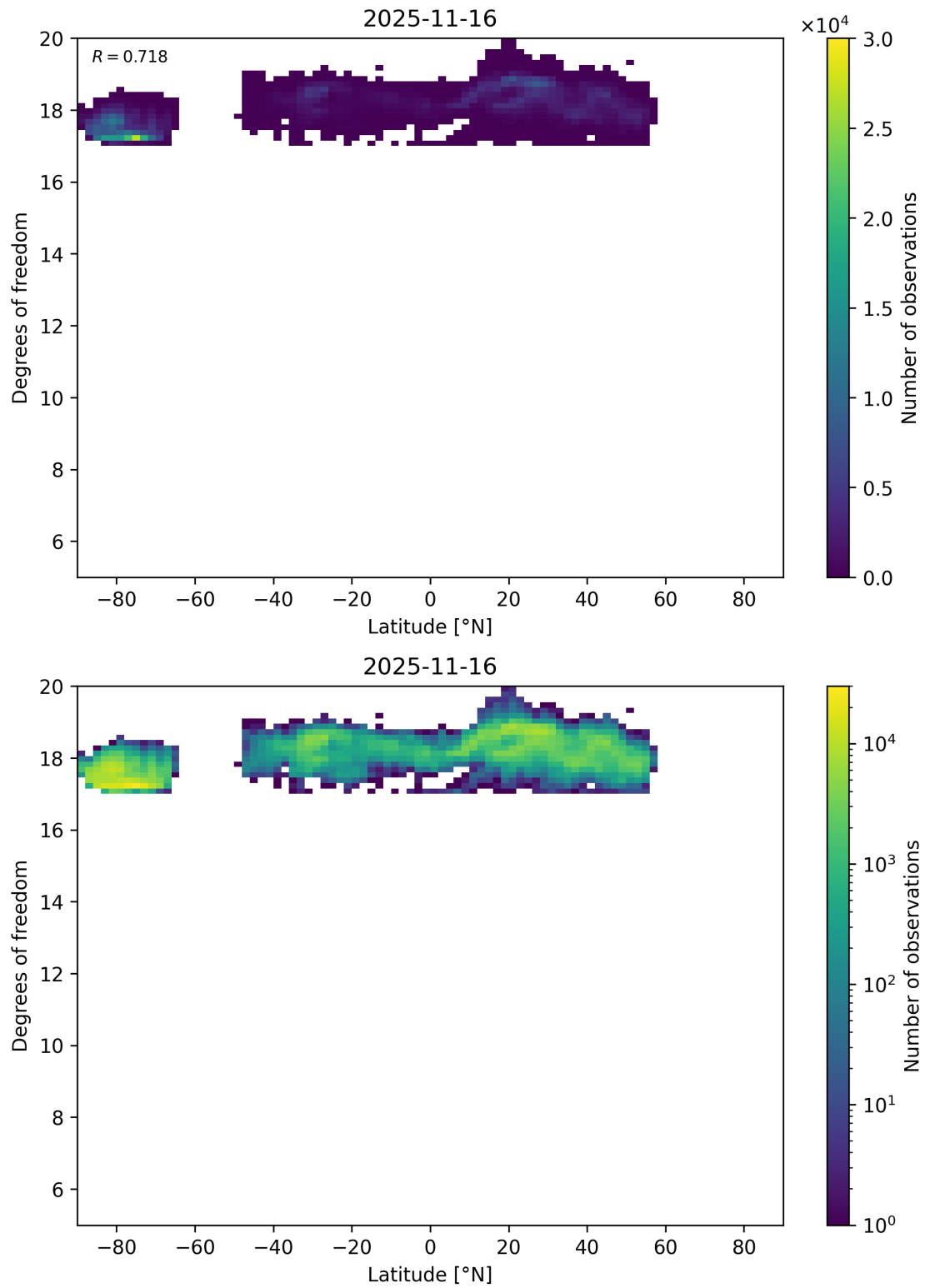
Figure 55: Scatter density plot of “Latitude” against “Degrees of freedom” for 2025-11-15 to 2025-11-17.
