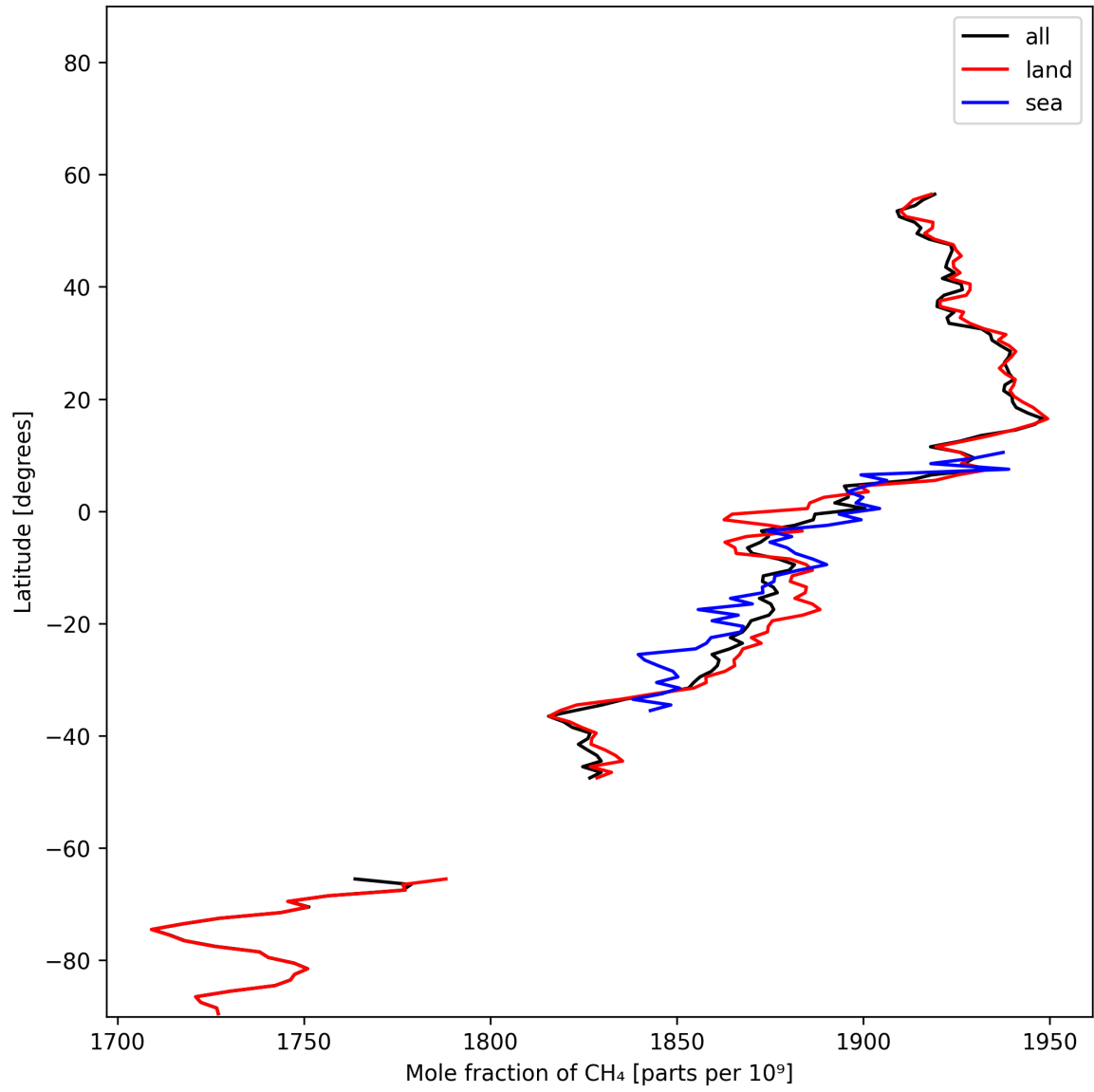
Figure 12: Zonal average of “Mole fraction of \text{CH}_4 ” for 2025-11-15 to 2025-11-17.
