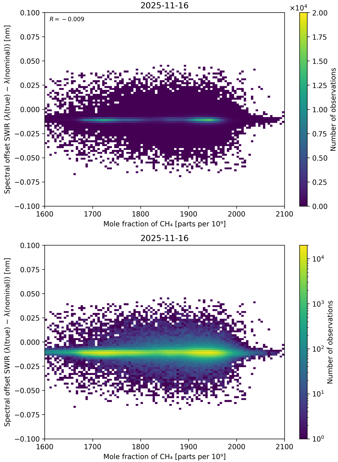
Figure 86: Scatter density plot of “Mole fraction of \text{CH}_4 ” against “Spectral offset SWIR ( \lambda_{\text{true}} - \lambda_{\text{nominal}} )” for 2025-11-15 to 2025-11-17.
