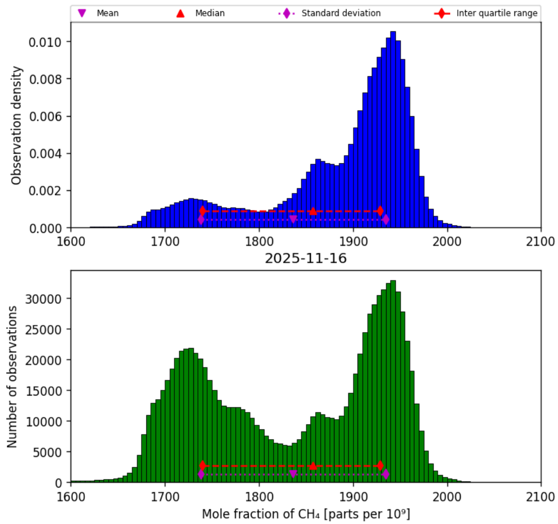
Figure 23: Histogram of “Mole fraction of CH 4 ” for 2025-11-15 to 2025-11-17
