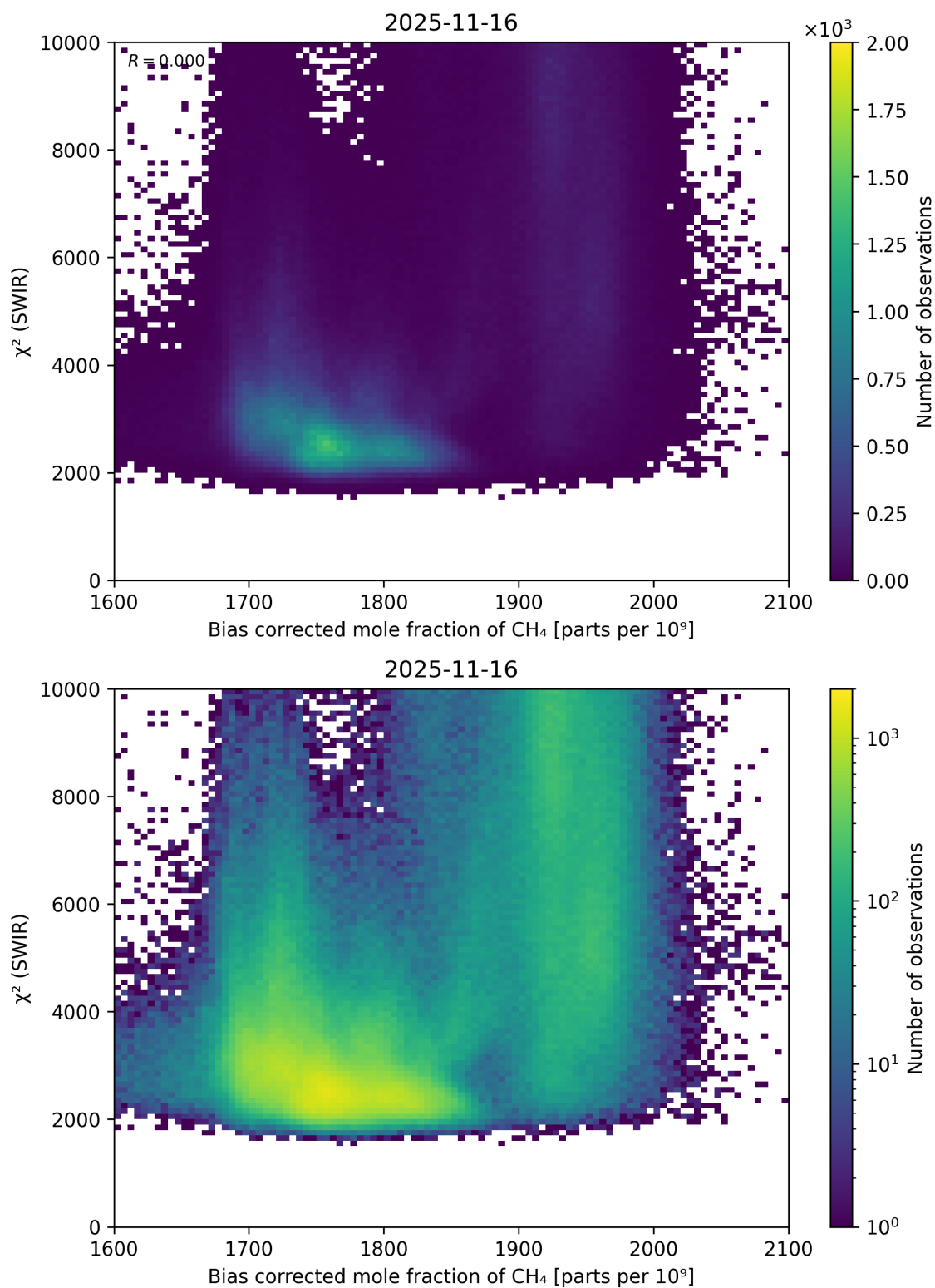
Figure 64: Scatter density plot of “Bias corrected mole fraction of CH 4 ” against “ \chi^2 (SWIR)” for 2025-11-15 to 2025-11-17.
