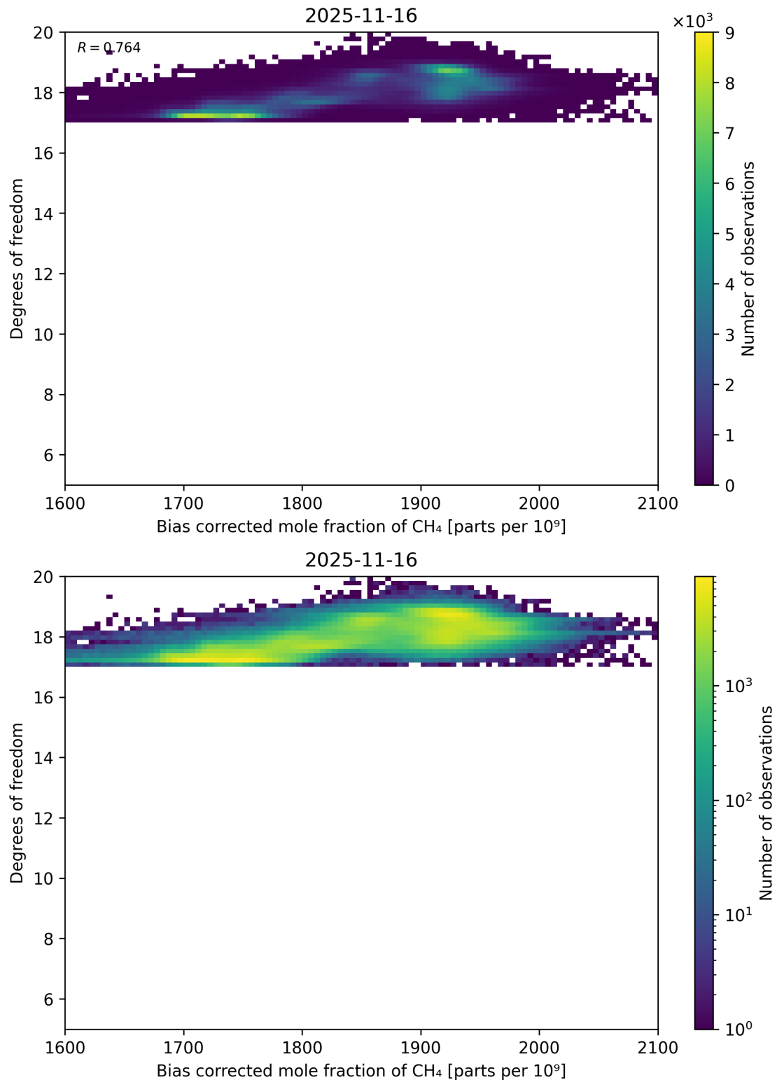
Figure 65: Scatter density plot of “Bias corrected mole fraction of CH 4 ” against “Degrees of freedom” for 2025-11-15 to 2025-11-17.
