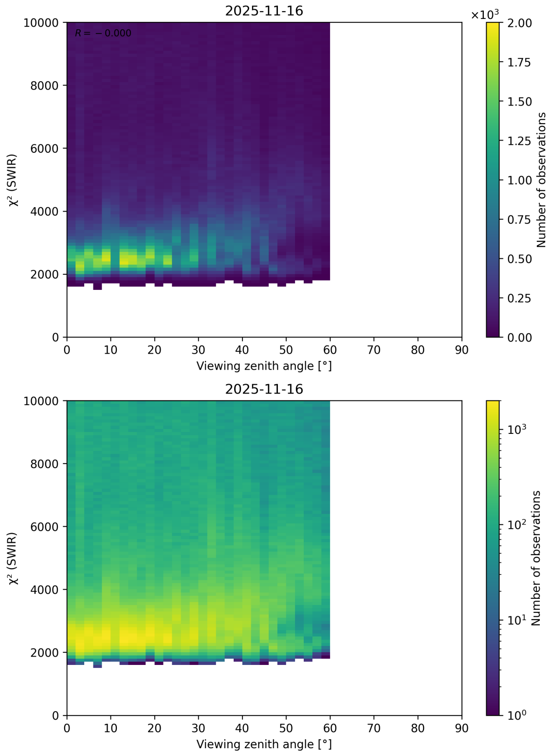
Figure 106: Scatter density plot of “Viewing zenith angle” against “ \chi^2 (SWIR)” for 2025-11-15 to 2025-11-17.
