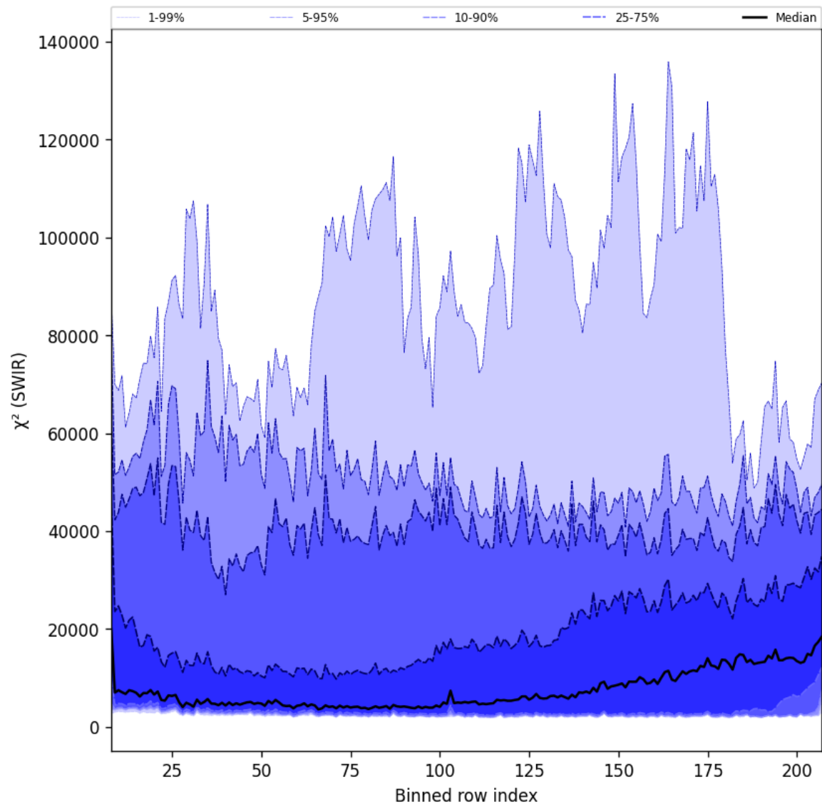
Figure 39: Along track statistics of “ \chi^2 (SWIR)” for 2025-11-15 to 2025-11-17
