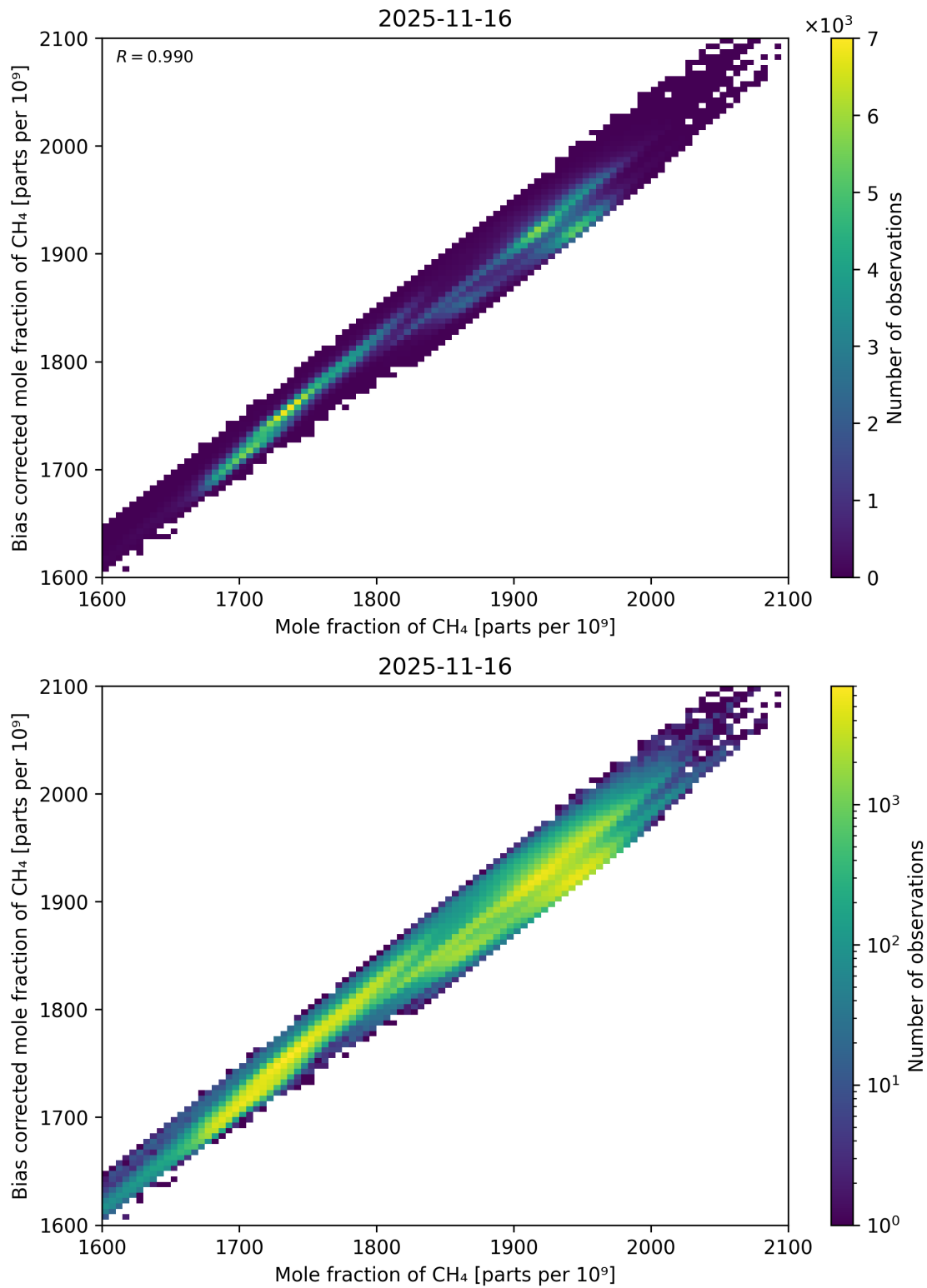
Figure 74: Scatter density plot of “Mole fraction of CH 4 ” against “Bias corrected mole fraction of CH 4 ” for 2025-11-15 to 2025-11-17.
