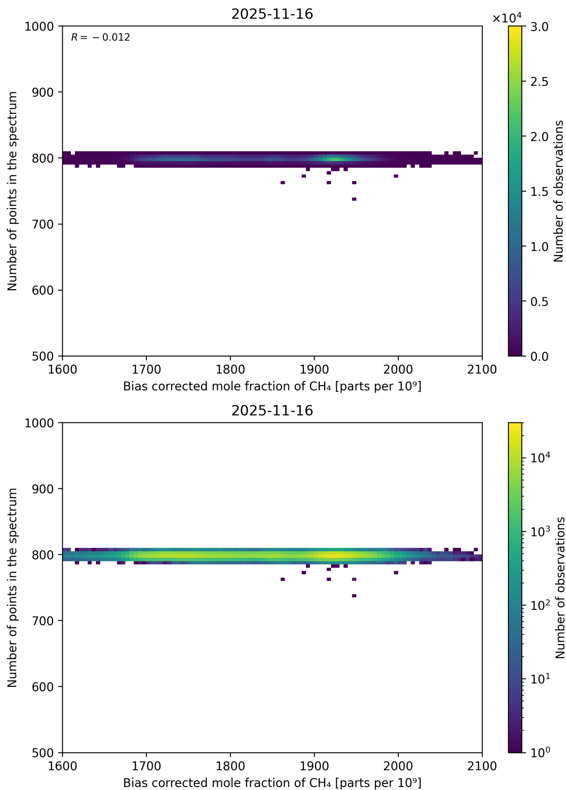
Figure 68: Scatter density plot of “Bias corrected mole fraction of CH 4 ” against “Number of points in the spectrum” for 2025-11-15 to 2025-11-17.
