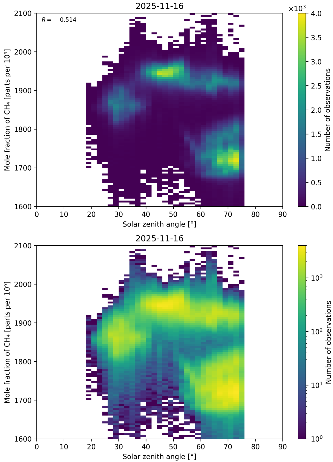
Figure 99: Scatter density plot of “Solar zenith angle” against “Mole fraction of CH 4 ” for 2025-11-15 to 2025-11-17.
