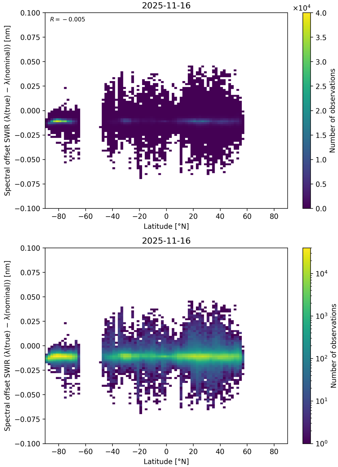
Figure 62: Scatter density plot of “Latitude” against “Spectral offset SWIR ( \lambda_{\text{true}} - \lambda_{\text{nominal}} )” for 2025-11-15 to 2025-11-17.
