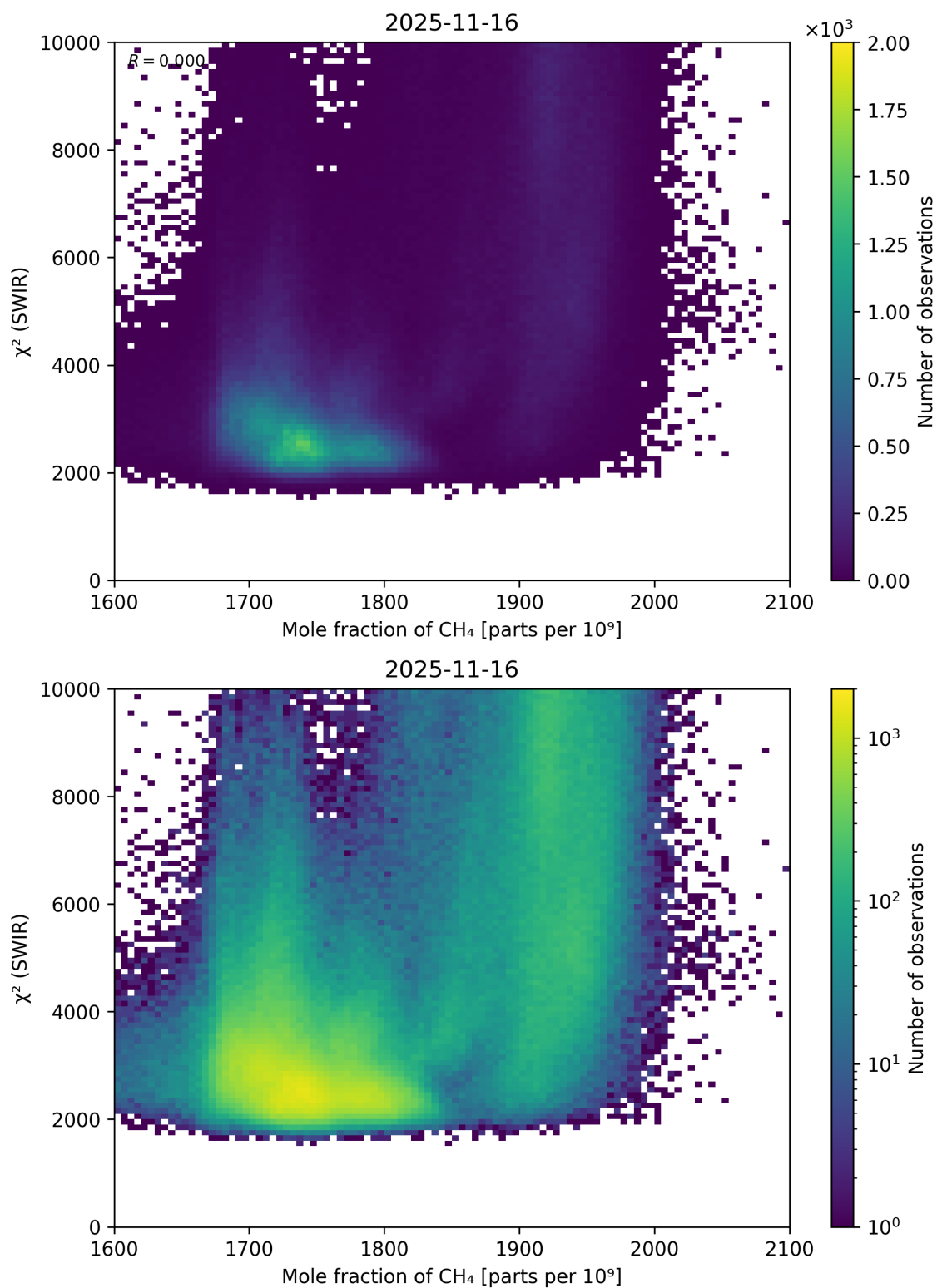
Figure 71: Scatter density plot of “Mole fraction of CH 4 ” against “ \chi^2 (SWIR)” for 2025-11-15 to 2025-11-17.
