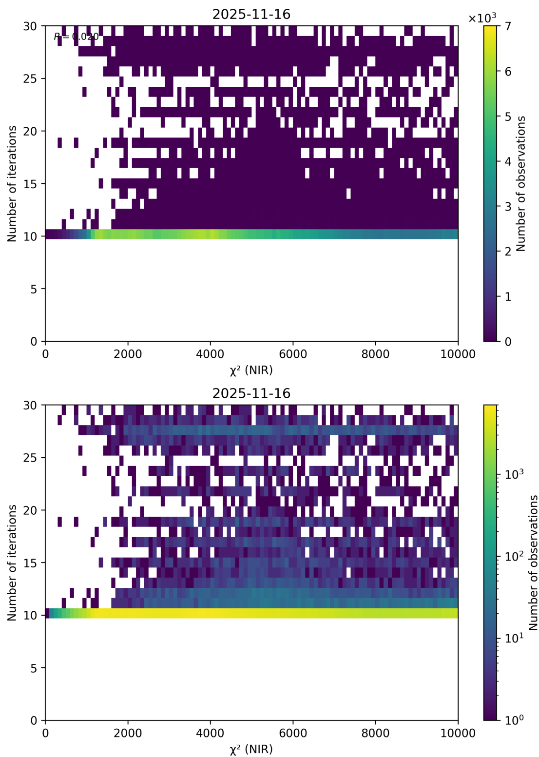
Figure 46: Scatter density plot of “ \chi^2 (NIR)” against “Number of iterations” for 2025-11-15 to 2025-11-17.
