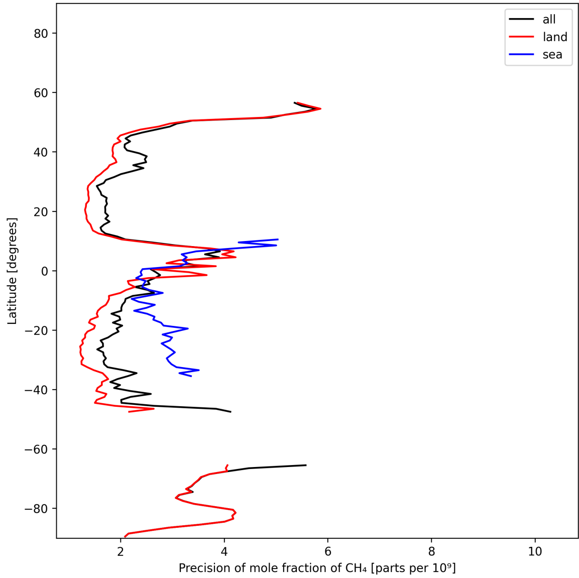
Figure 13: Zonal average of “Precision of mole fraction of CH 4 ” for 2025-11-15 to 2025-11-17.
