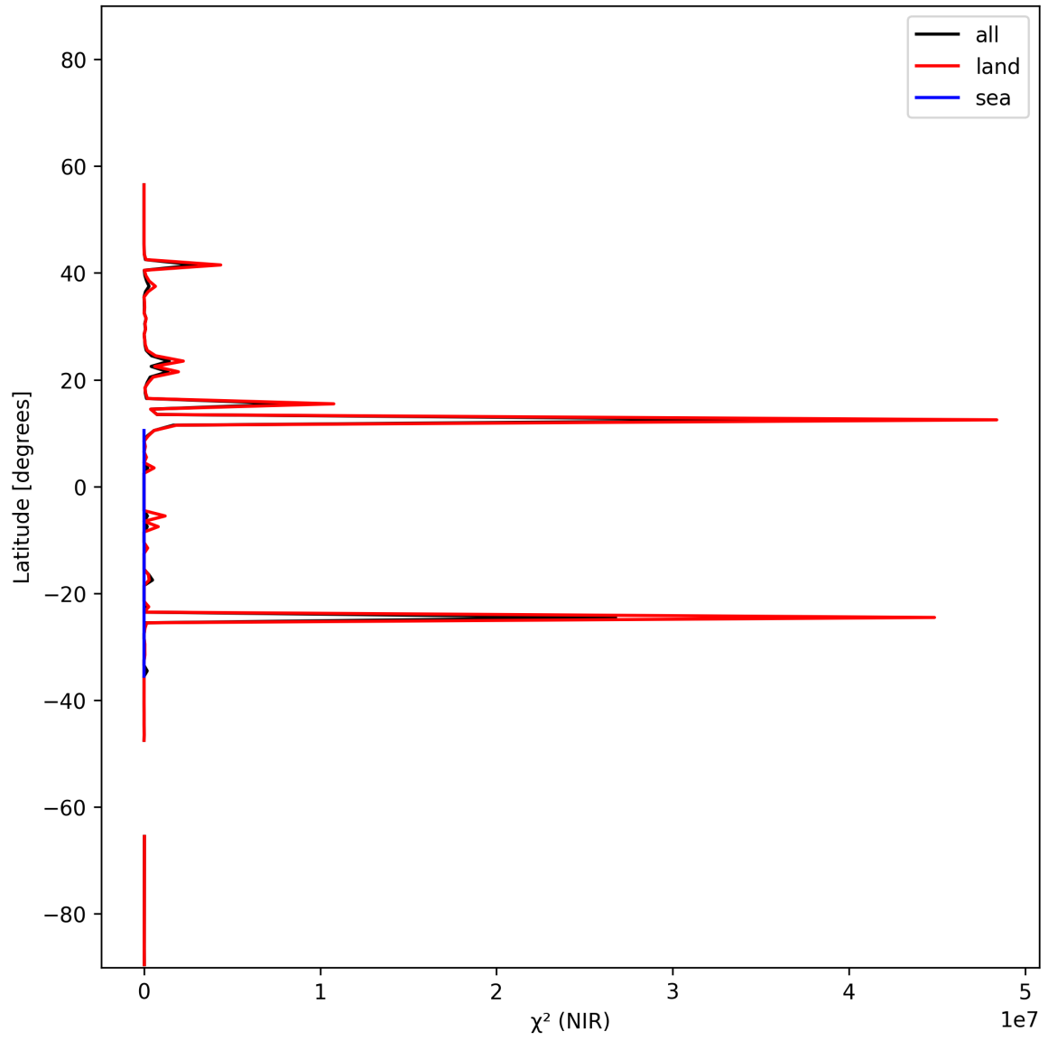
Figure 18: Zonal average of “ \chi^2 (NIR)” for 2025-11-15 to 2025-11-17.
