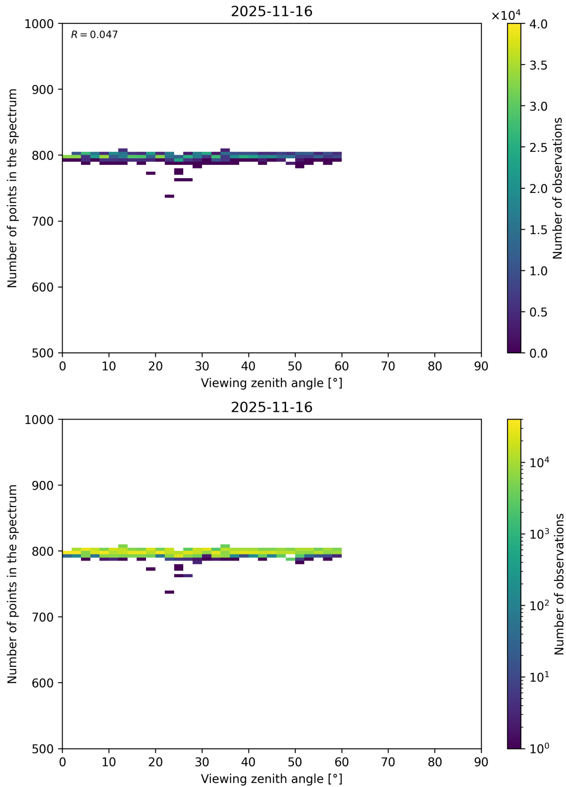
Figure 114: Scatter density plot of “Viewing zenith angle” against “Number of points in the spectrum” for 2025-11-15 to 2025-11-17.
