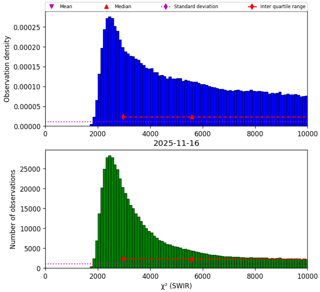
Figure 28: Histogram of “ \chi^2 (SWIR)” for 2025-11-15 to 2025-11-17
