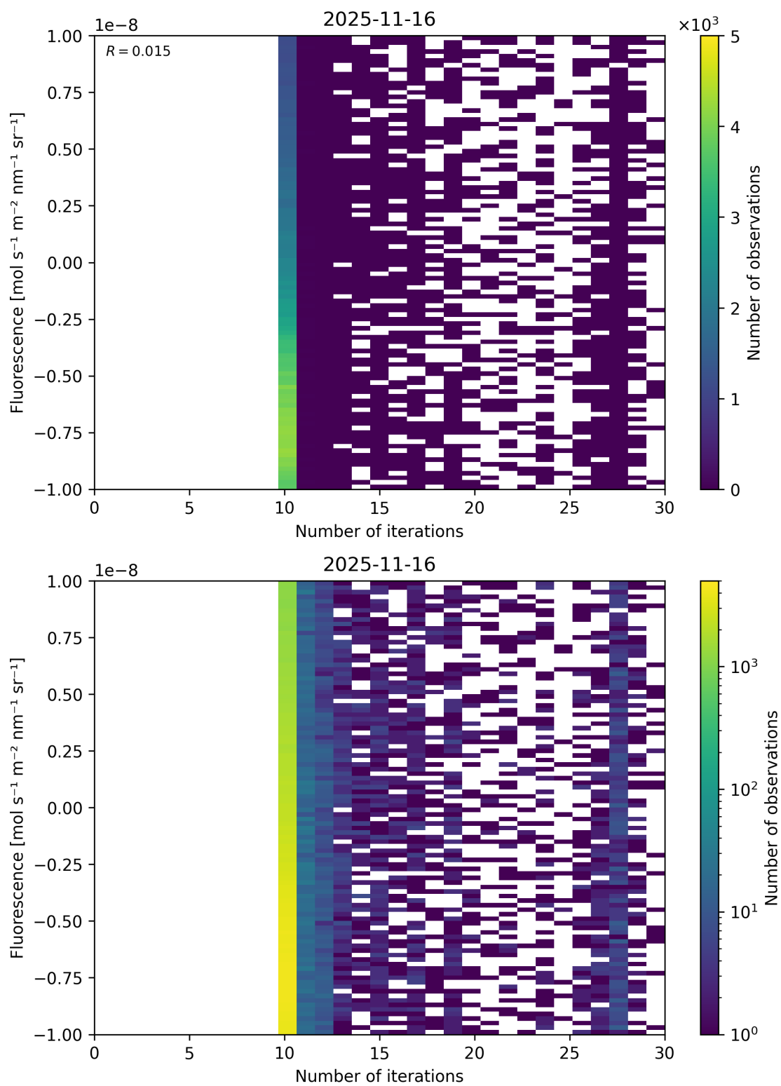
Figure 87: Scatter density plot of “Number of iterations” against “Fluorescence” for 2025-11-15 to 2025-11-17.
