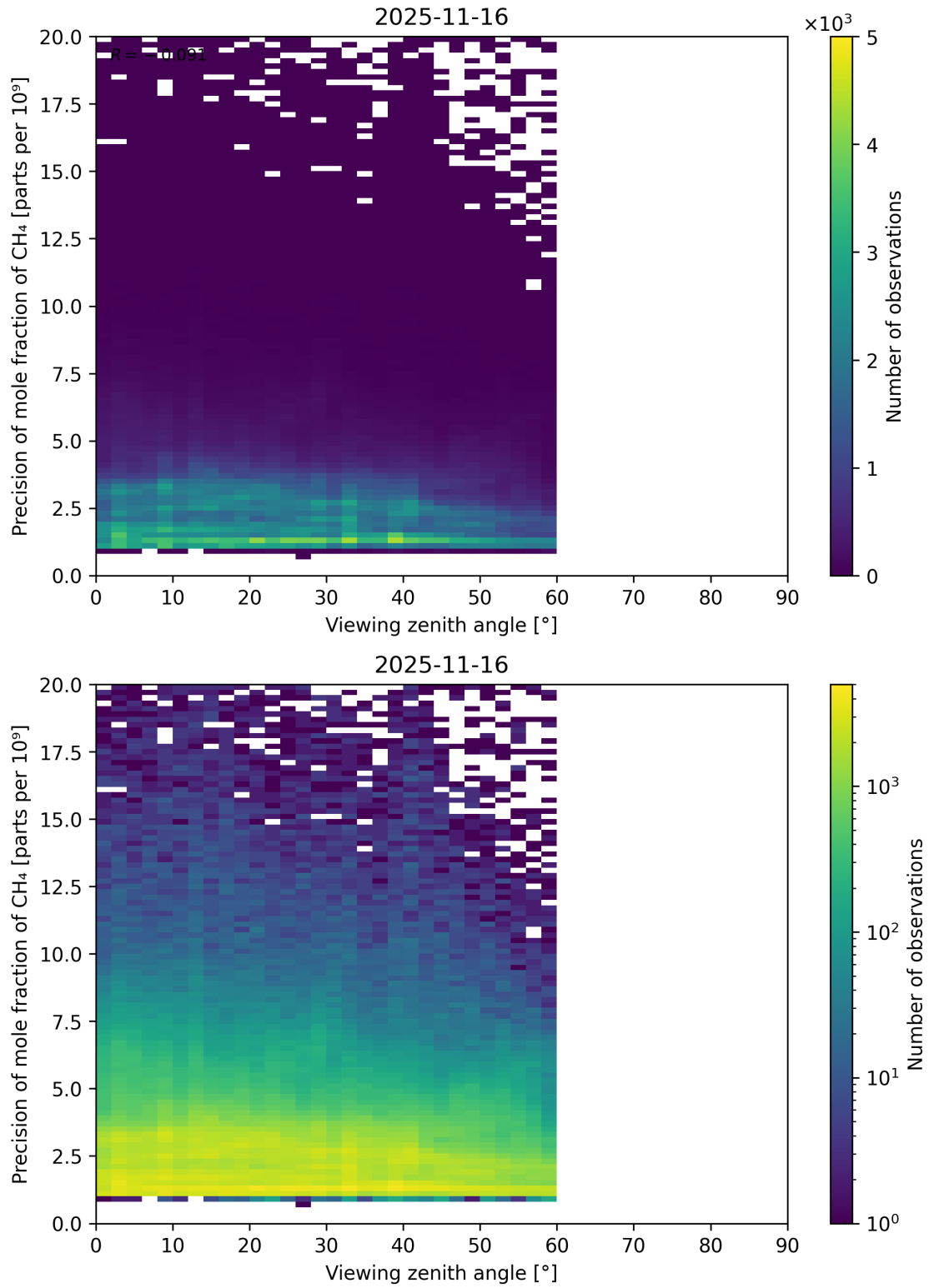
Figure 112: Scatter density plot of “Viewing zenith angle” against “Precision of mole fraction of CH 4 ” for 2025-11-15 to 2025-11-17.
