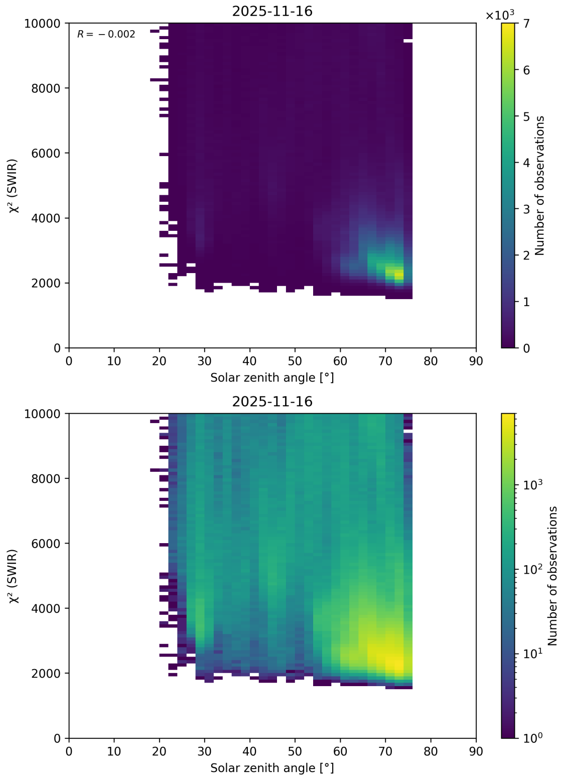
Figure 95: Scatter density plot of “Solar zenith angle” against “ \chi^2 (SWIR)” for 2025-11-15 to 2025-11-17.
