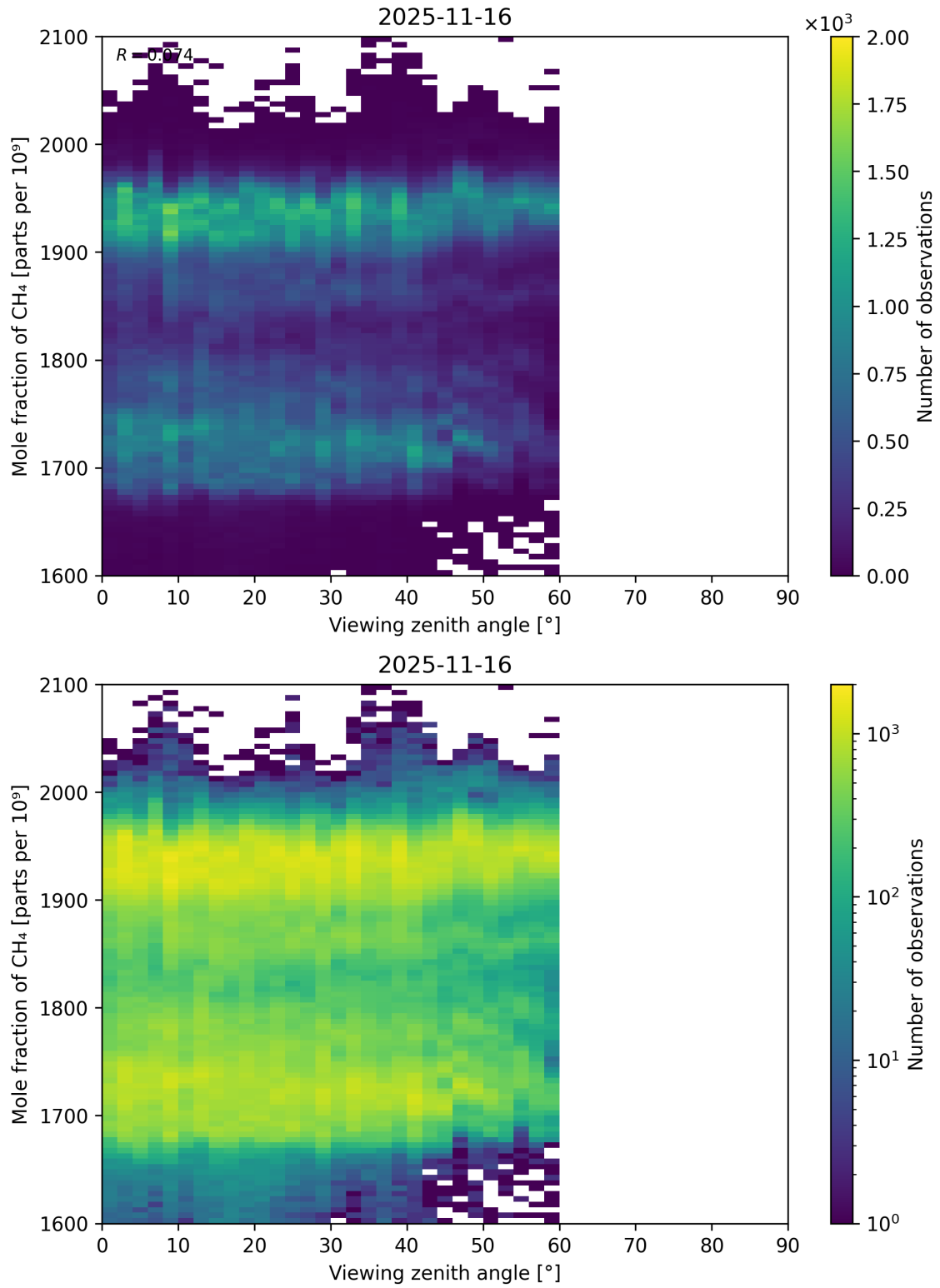
Figure 110: Scatter density plot of “Viewing zenith angle” against “Mole fraction of CH 4 ” for 2025-11-15 to 2025-11-17.
