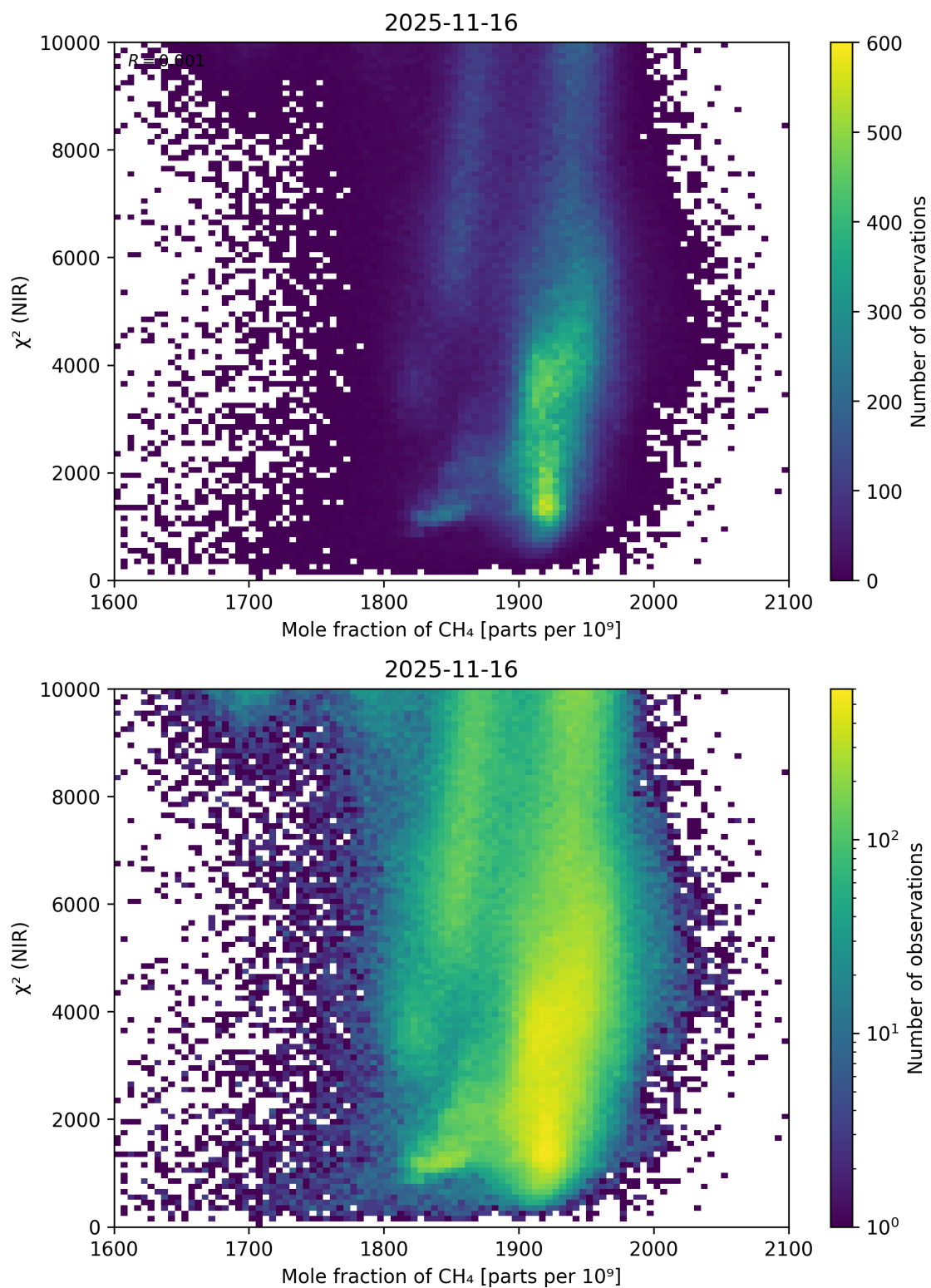
Figure 70: Scatter density plot of “Mole fraction of CH 4 ” against “ \chi^2 (NIR)” for 2025-11-15 to 2025-11-17.
