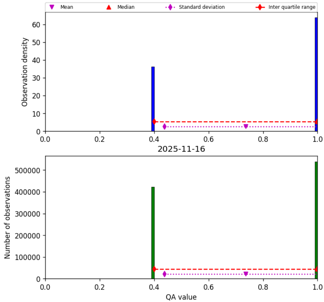
Figure 22: Histogram of “QA value” for 2025-11-15 to 2025-11-17
