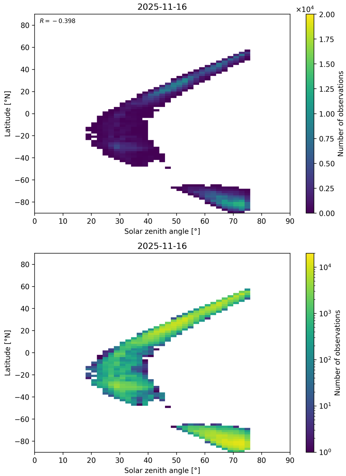
Figure 98: Scatter density plot of “Solar zenith angle” against “Latitude” for 2025-11-15 to 2025-11-17.
