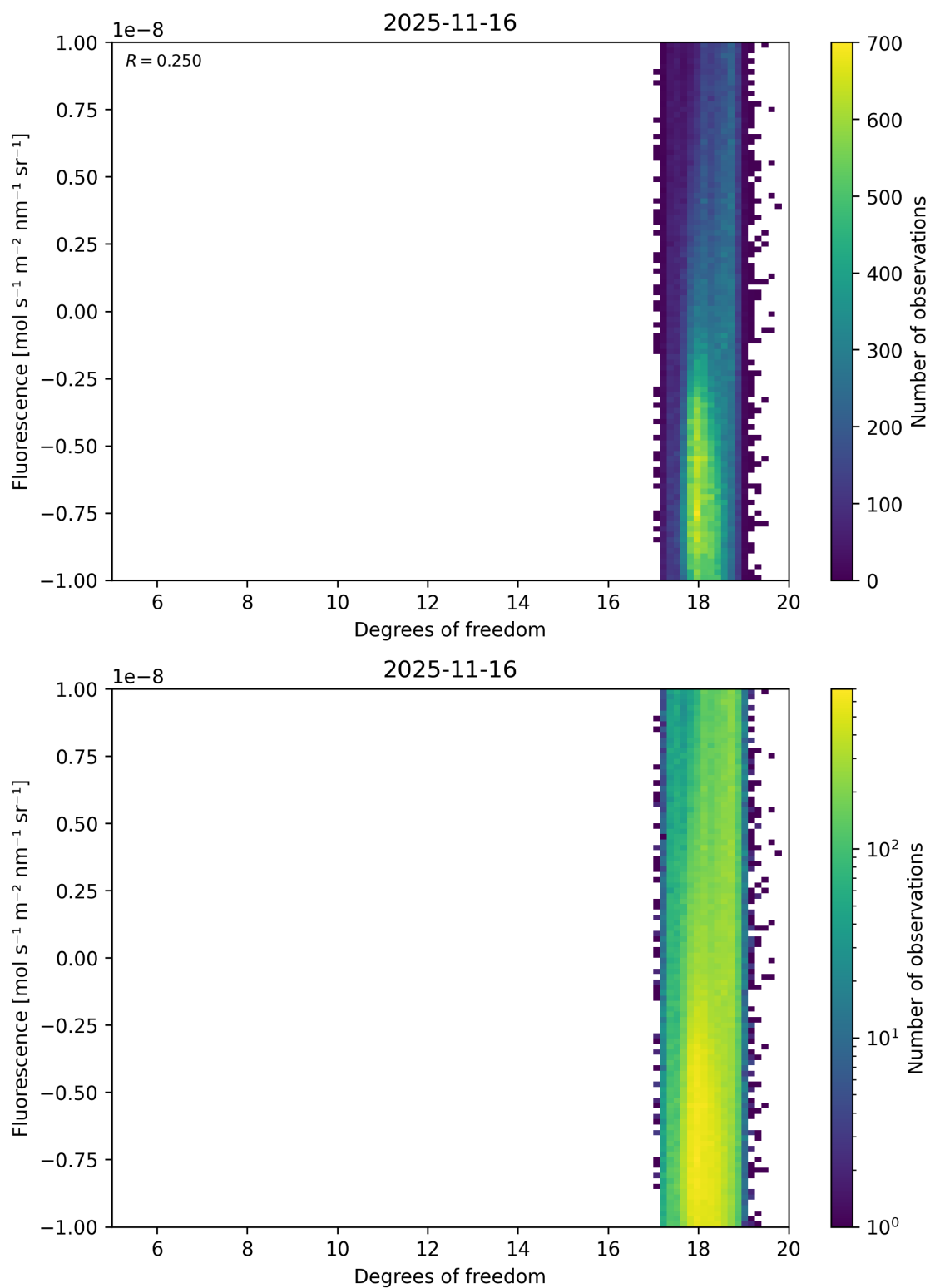
Figure 51: Scatter density plot of “Degrees of freedom” against “Fluorescence” for 2025-11-15 to 2025-11-17.
