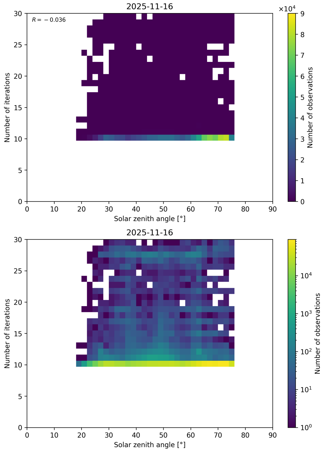
Figure 102: Scatter density plot of “Solar zenith angle” against “Number of iterations” for 2025-11-15 to 2025-11-17.
