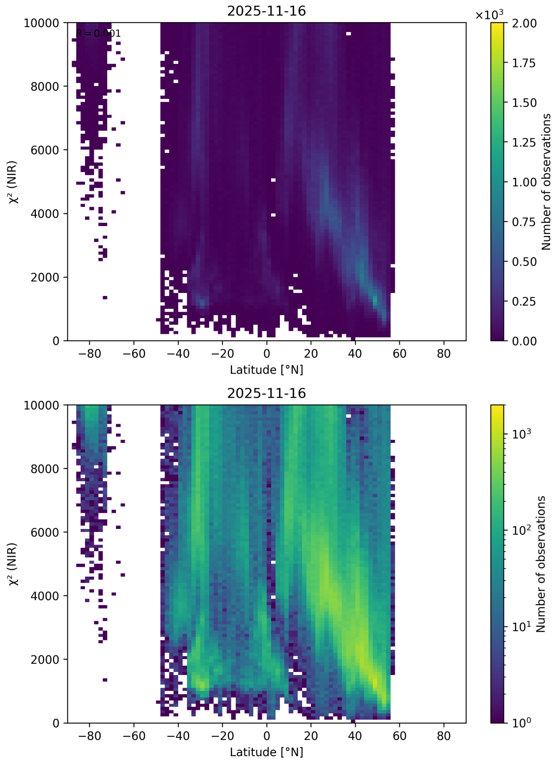
Figure 53: Scatter density plot of “Latitude” against “ \chi^2 (NIR)” for 2025-11-15 to 2025-11-17.
