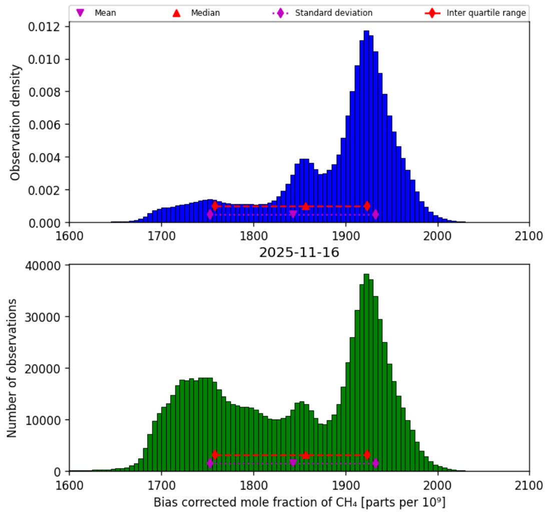
Figure 25: Histogram of “Bias corrected mole fraction of CH 4 ” for 2025-11-15 to 2025-11-17
