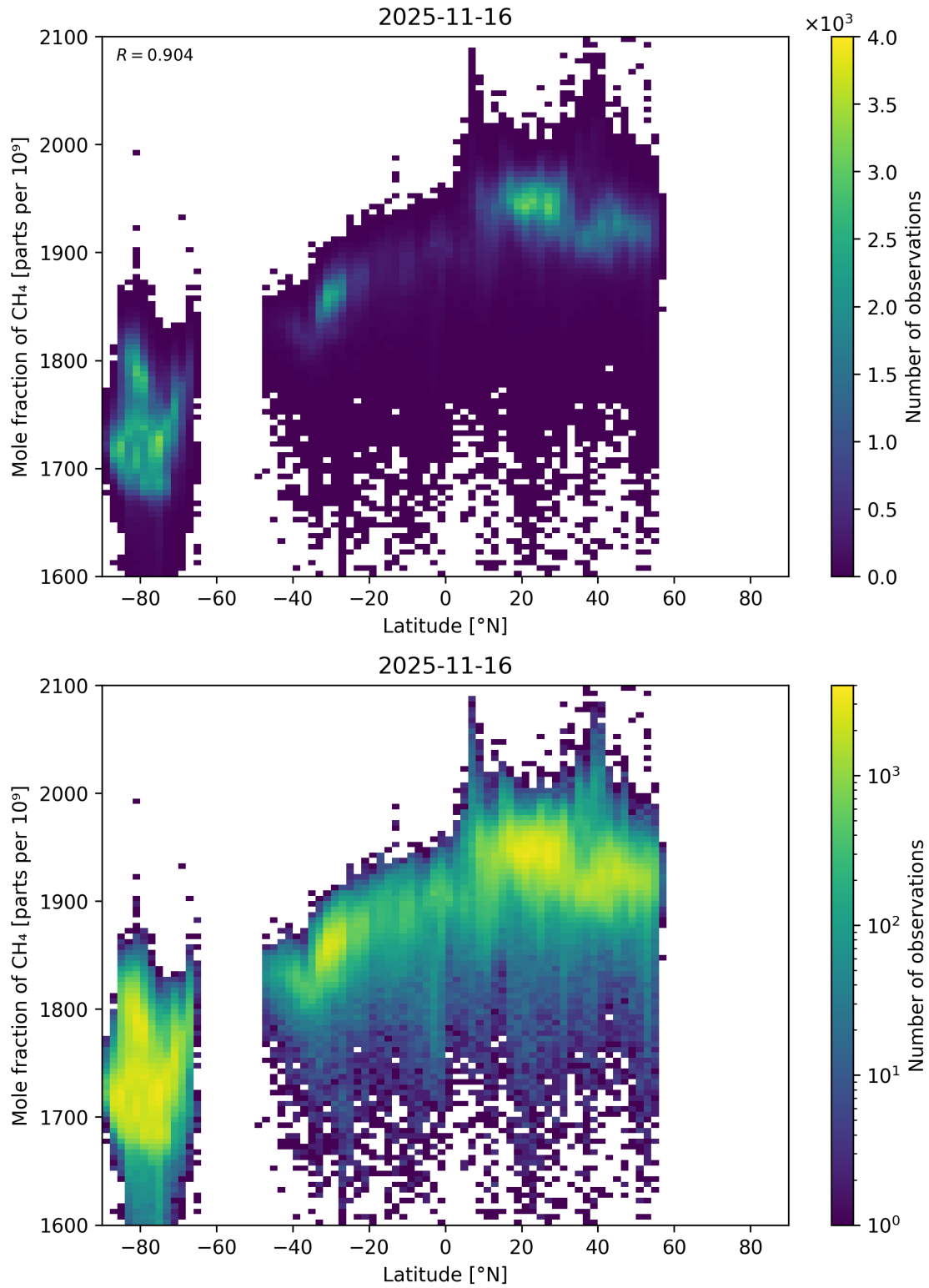
Figure 57: Scatter density plot of “Latitude” against “Mole fraction of CH 4 ” for 2025-11-15 to 2025-11-17.
