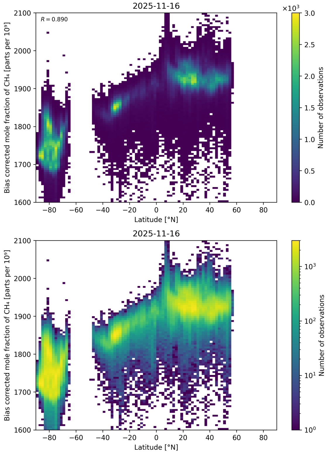
Figure 58: Scatter density plot of “Latitude” against “Bias corrected mole fraction of CH 4 ” for 2025-11-15 to 2025-11-17.
