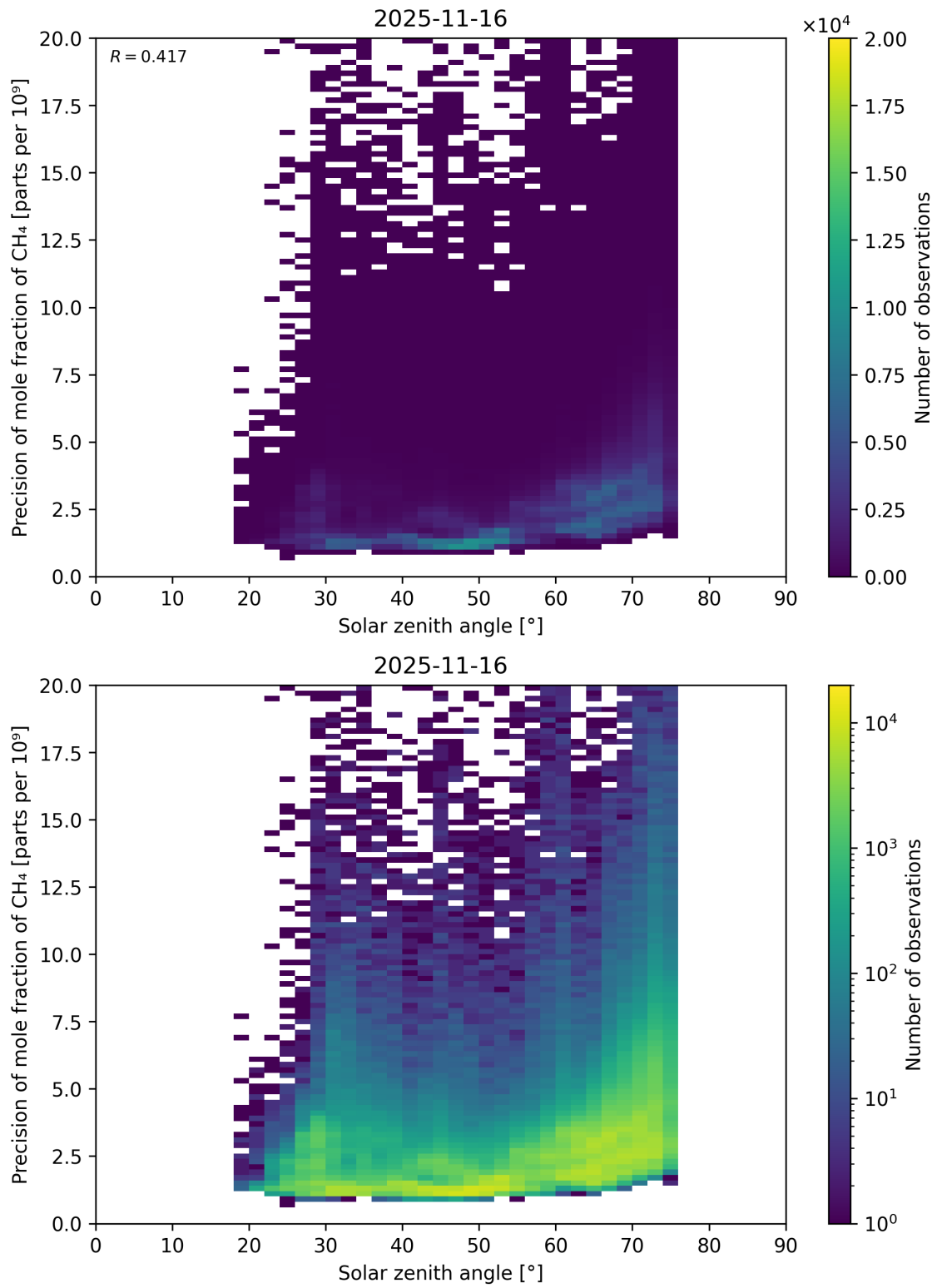
Figure 101: Scatter density plot of “Solar zenith angle” against “Precision of mole fraction of \text{CH}_4 ” for 2025-11-15 to 2025-11-17.
