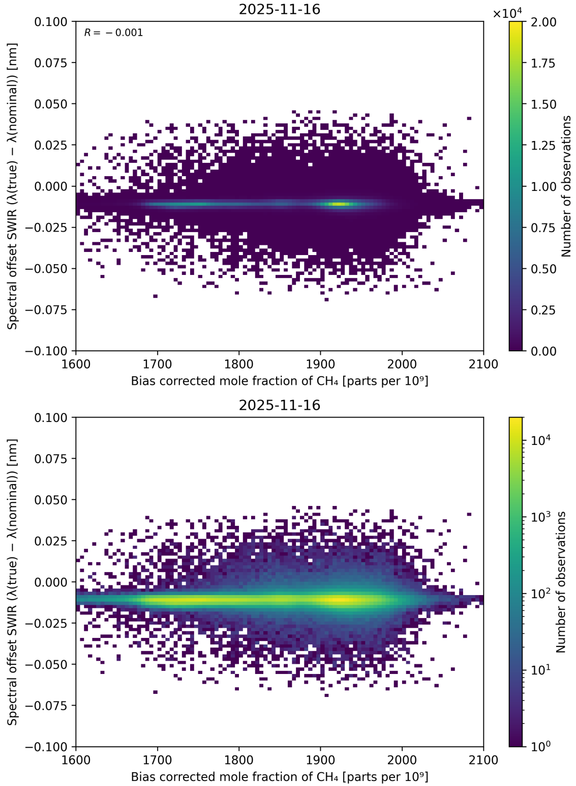
Figure 69: Scatter density plot of “Bias corrected mole fraction of \text{CH}_4 ” against “Spectral offset SWIR ( \lambda_{\text{true}} - \lambda_{\text{nominal}} )” for 2025-11-15 to 2025-11-17.
