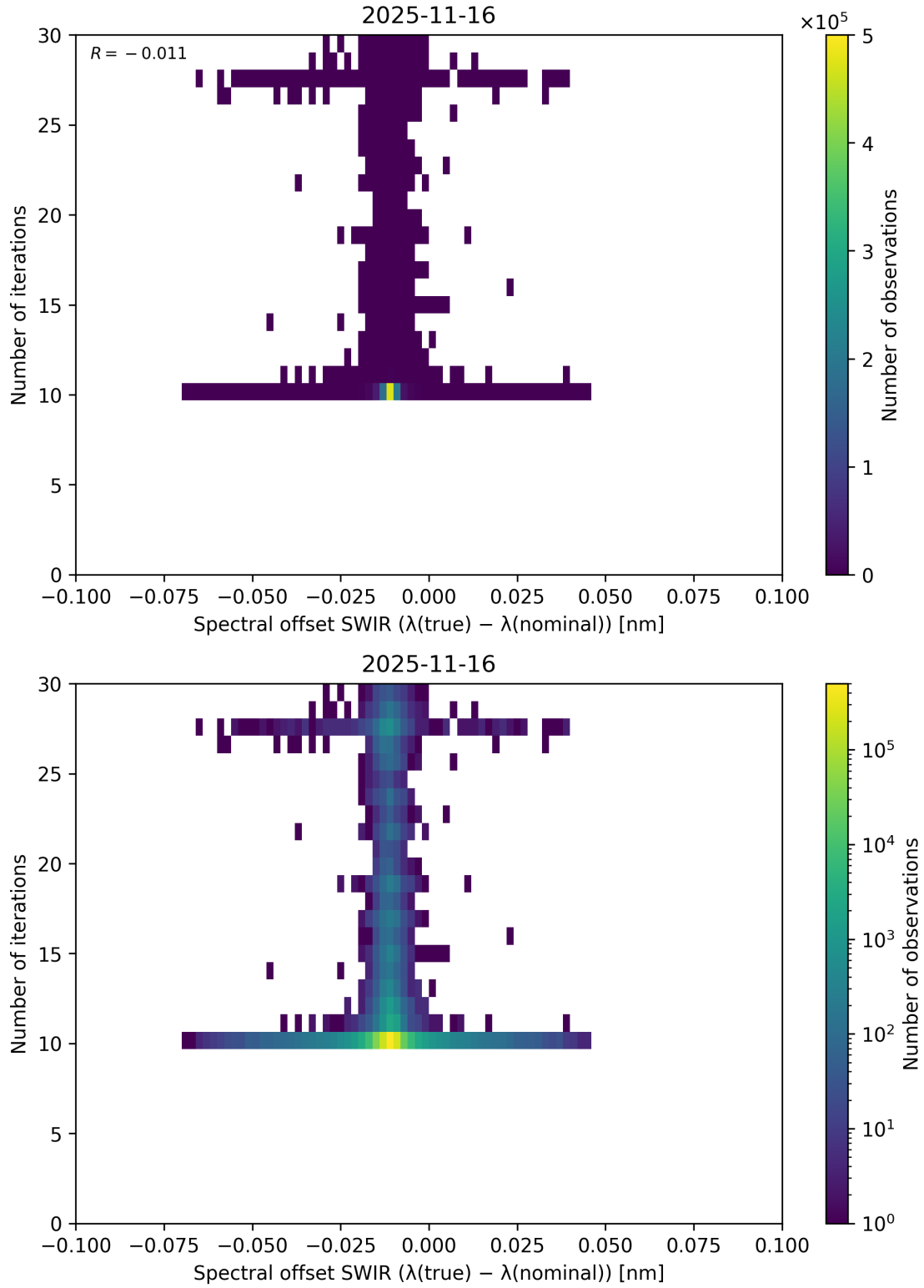
Figure 121: Scatter density plot of “Spectral offset SWIR ( \lambda_{\text{true}} - \lambda_{\text{nominal}} )” against “Number of iterations” for 2025-11-15 to 2025-11-17.
