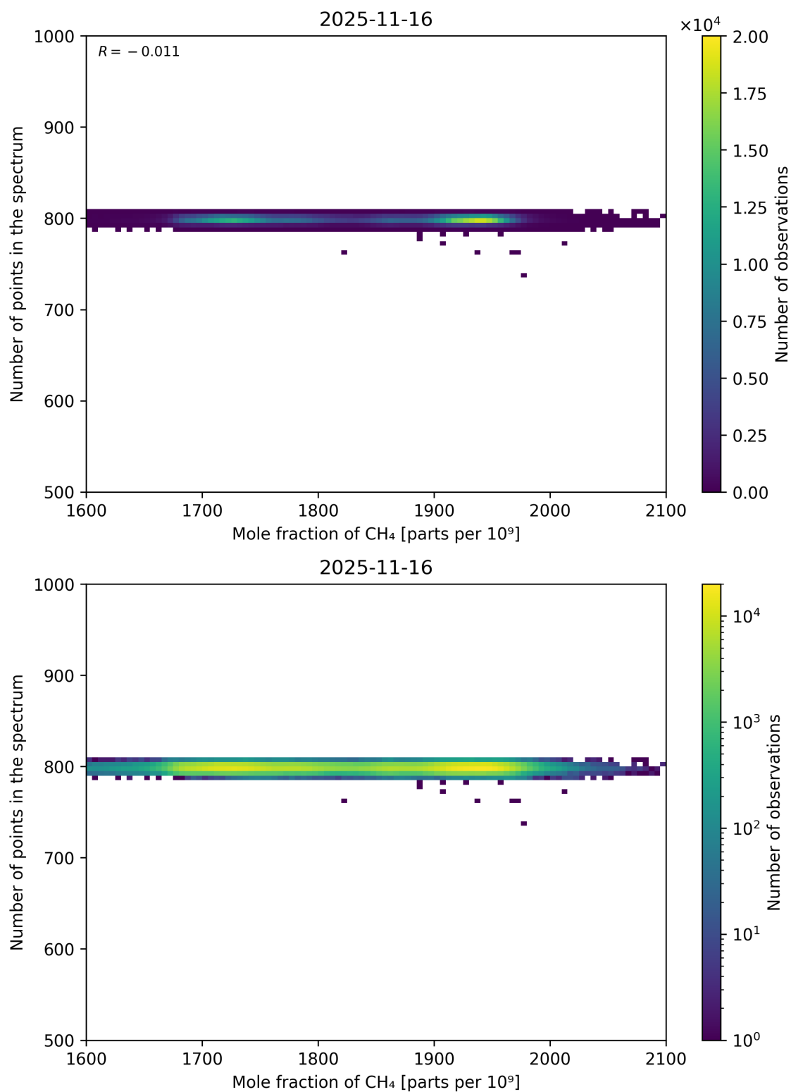
Figure 77: Scatter density plot of “Mole fraction of CH 4 ” against “Number of points in the spectrum” for 2025-11-15 to 2025-11-17.
