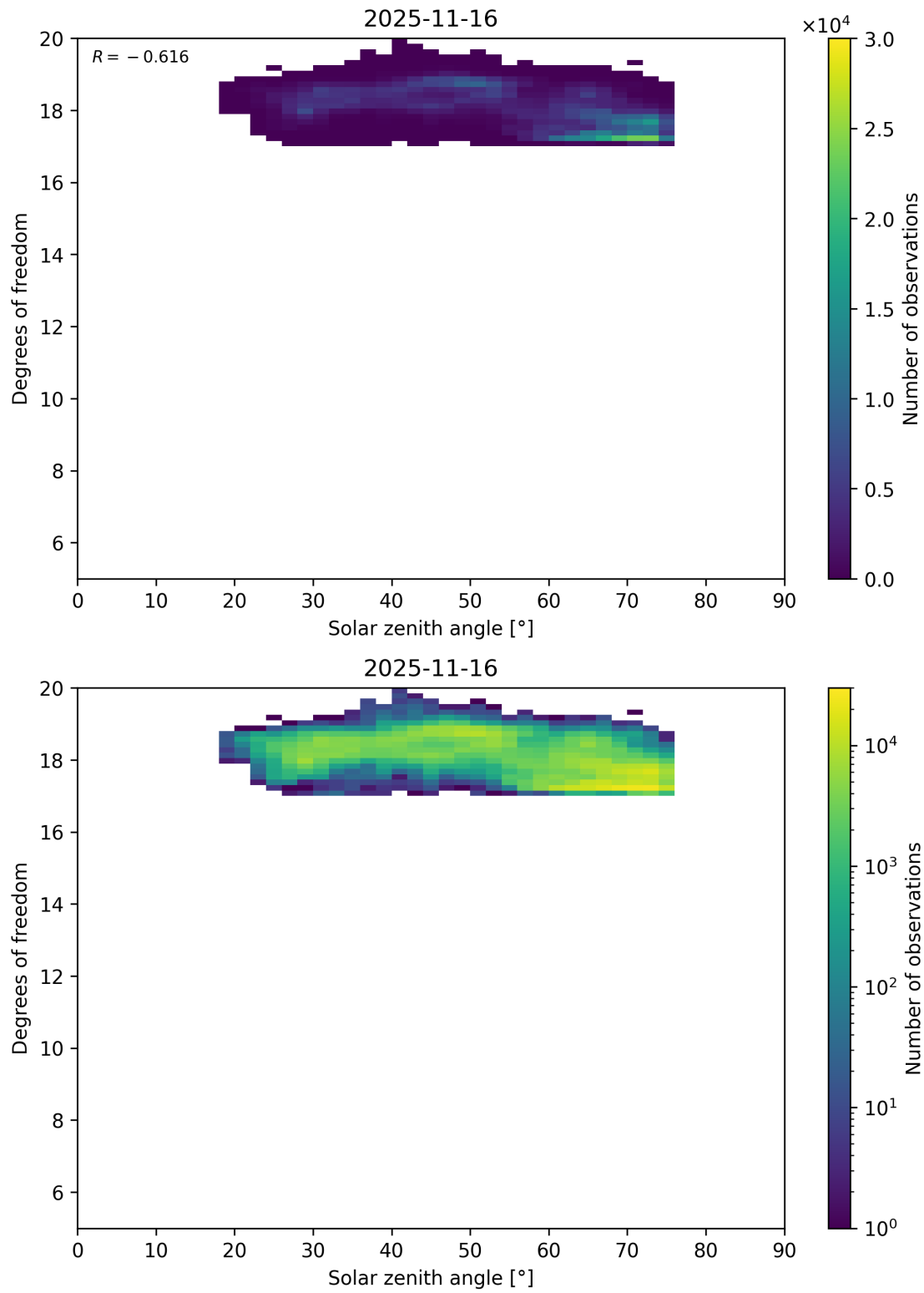
Figure 96: Scatter density plot of “Solar zenith angle” against “Degrees of freedom” for 2025-11-15 to 2025-11-17.
