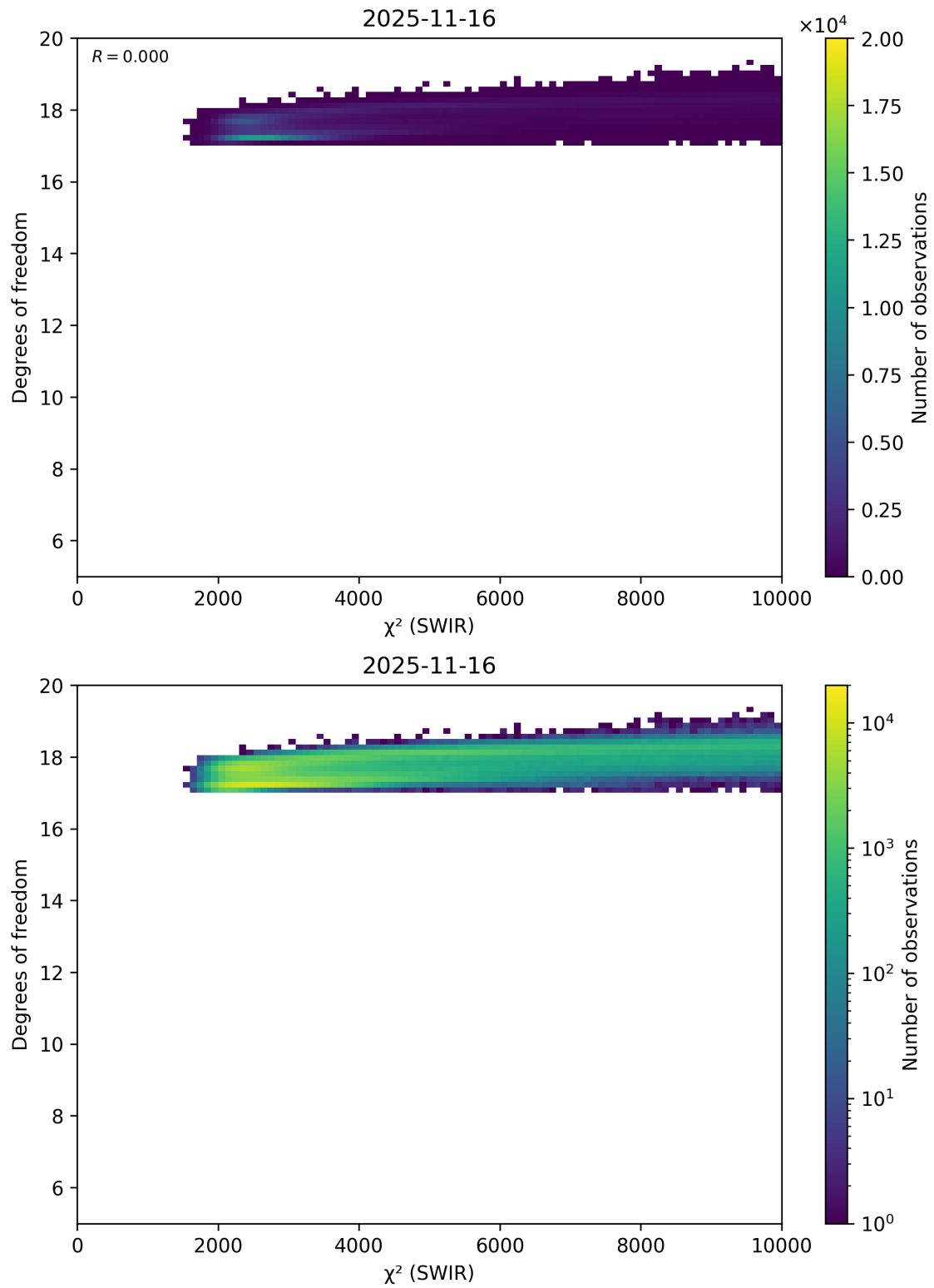
Figure 48: Scatter density plot of “ \chi^2 (SWIR)” against “Degrees of freedom” for 2025-11-15 to 2025-11-17.
