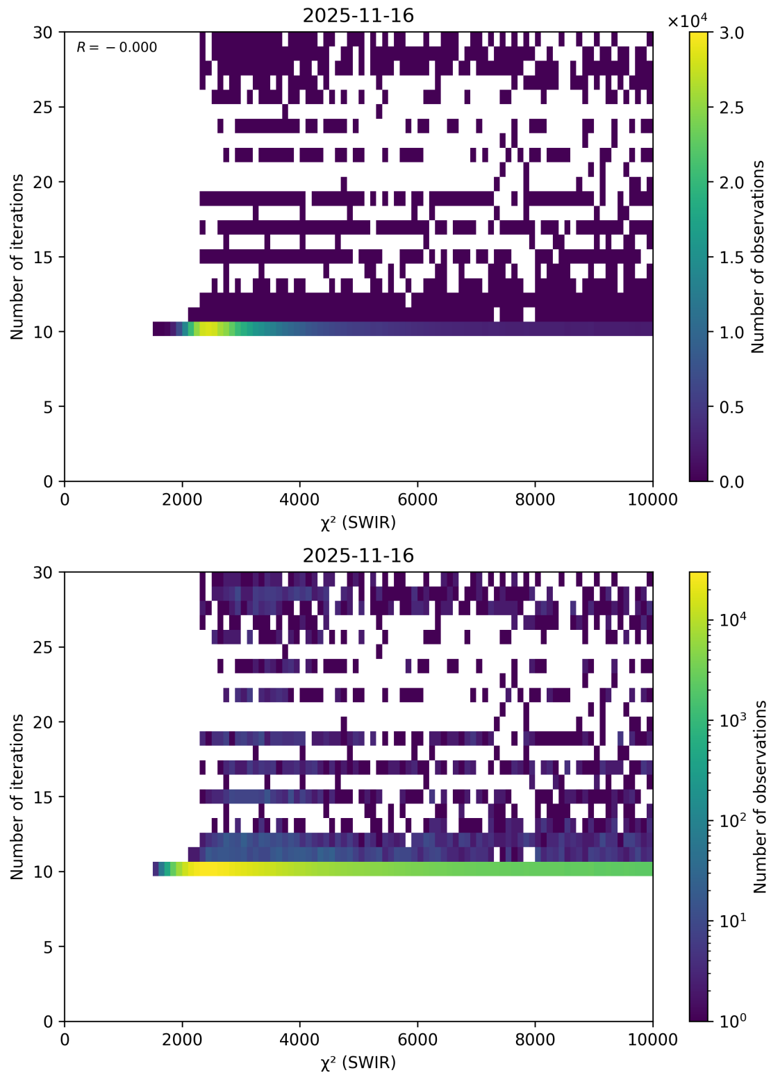
Figure 50: Scatter density plot of “ \chi^2 (SWIR)” against “Number of iterations” for 2025-11-15 to 2025-11-17.
