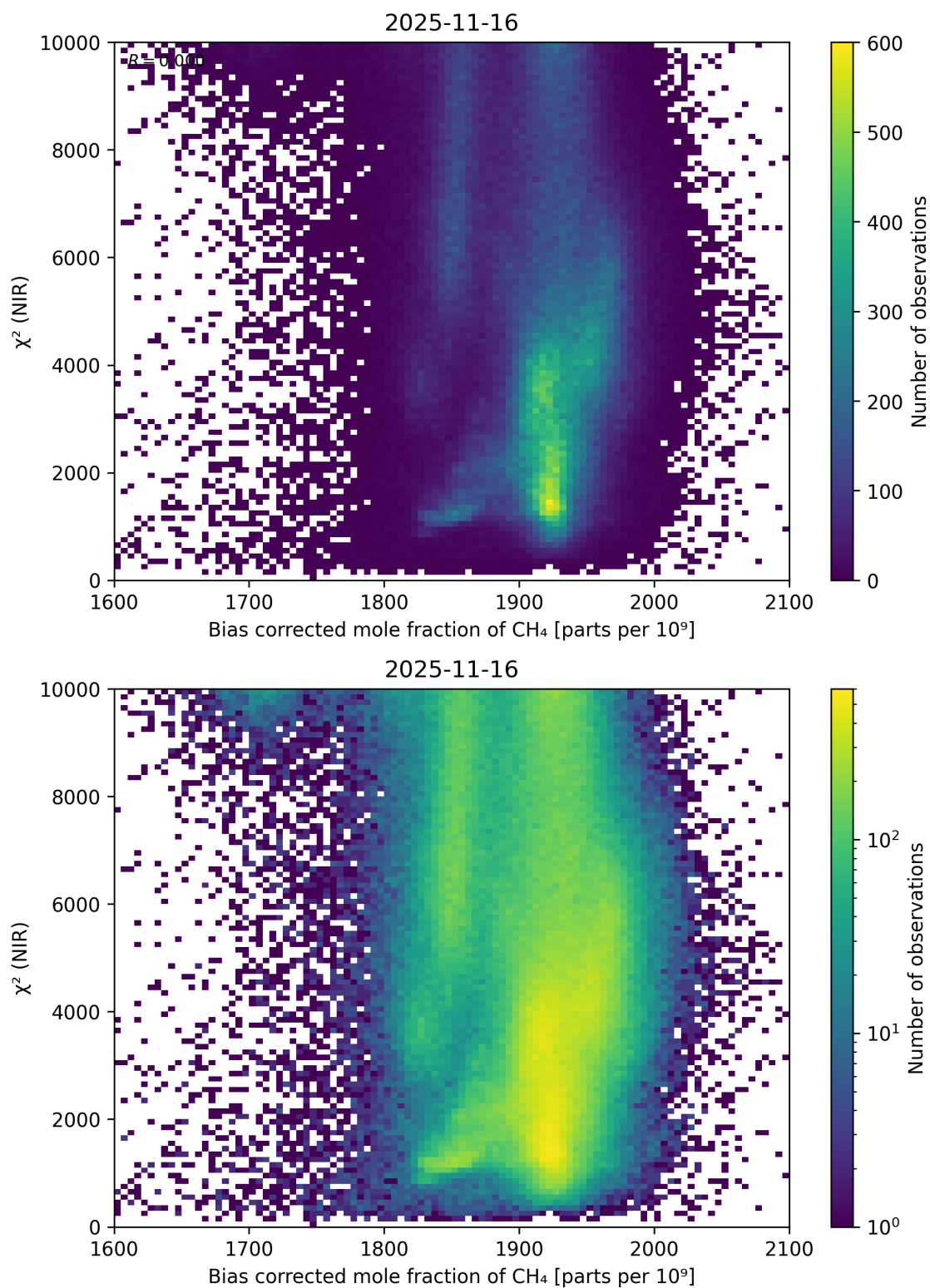
Figure 63: Scatter density plot of “Bias corrected mole fraction of \text{CH}_4 ” against “ \chi^2 (NIR)” for 2025-11-15 to 2025-11-17.
