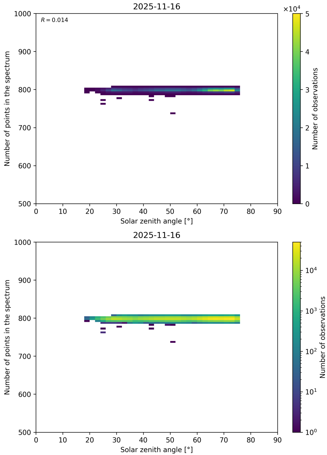
Figure 103: Scatter density plot of “Solar zenith angle” against “Number of points in the spectrum” for 2025-11-15 to 2025-11-17.
