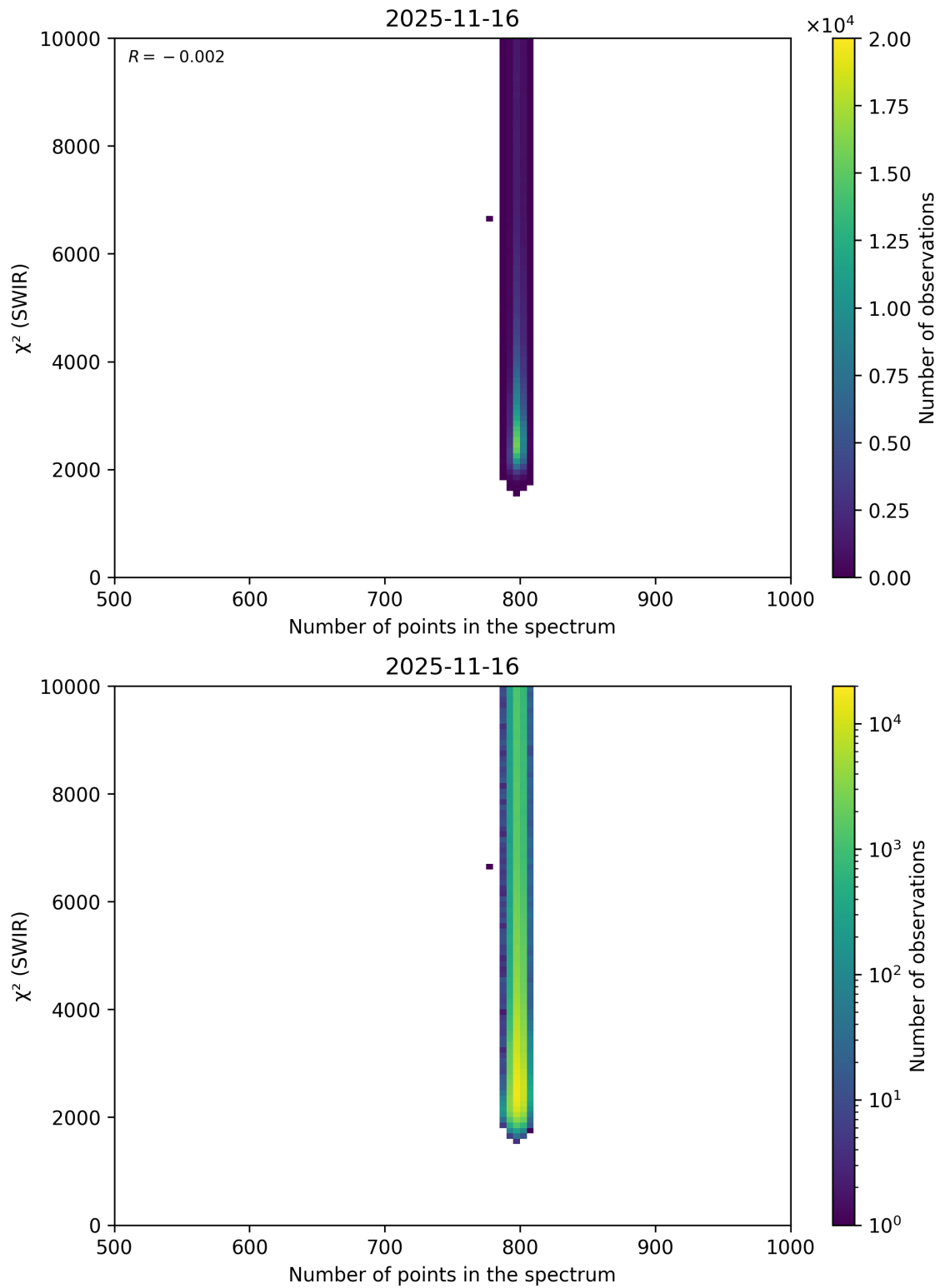
Figure 89: Scatter density plot of “Number of points in the spectrum” against “ \chi^2 (SWIR)” for 2025-11-15 to 2025-11-17.
