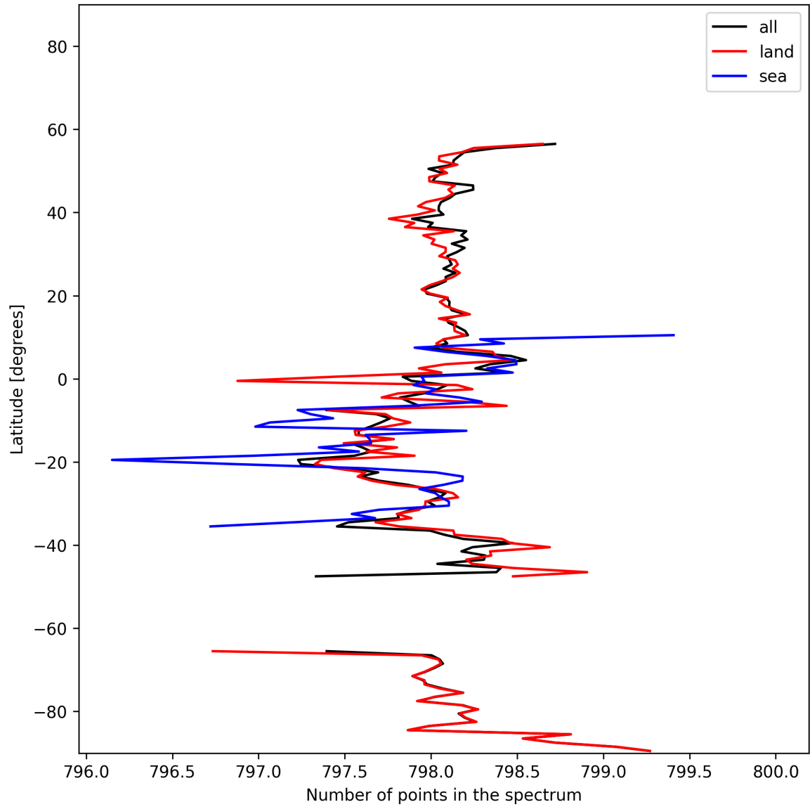
Figure 15: Zonal average of “Number of points in the spectrum” for 2025-11-15 to 2025-11-17.
