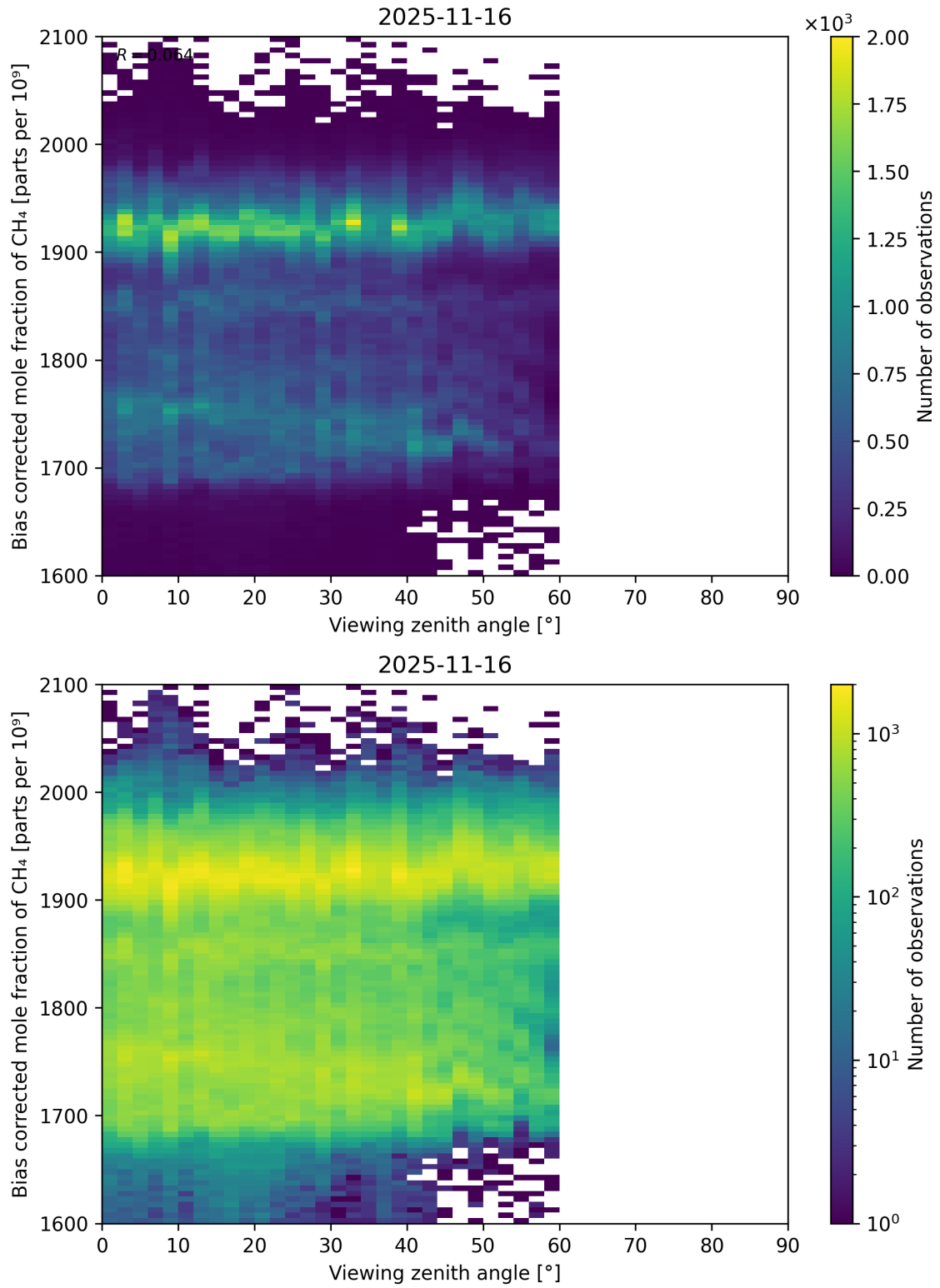
Figure 111: Scatter density plot of “Viewing zenith angle” against “Bias corrected mole fraction of CH 4 ” for 2025-11-15 to 2025-11-17.
