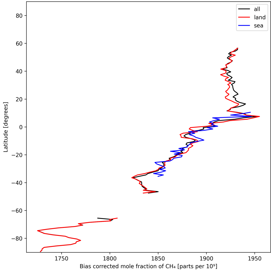
Figure 14: Zonal average of “Bias corrected mole fraction of CH 4 ” for 2025-11-15 to 2025-11-17.
