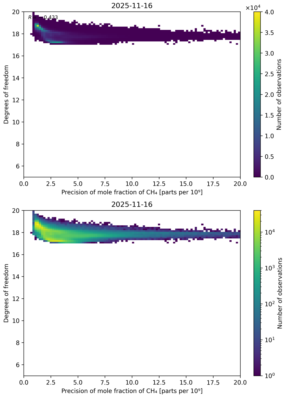
Figure 80: Scatter density plot of “Precision of mole fraction of CH 4 ” against “Degrees of freedom” for 2025-11-15 to 2025-11-17.
