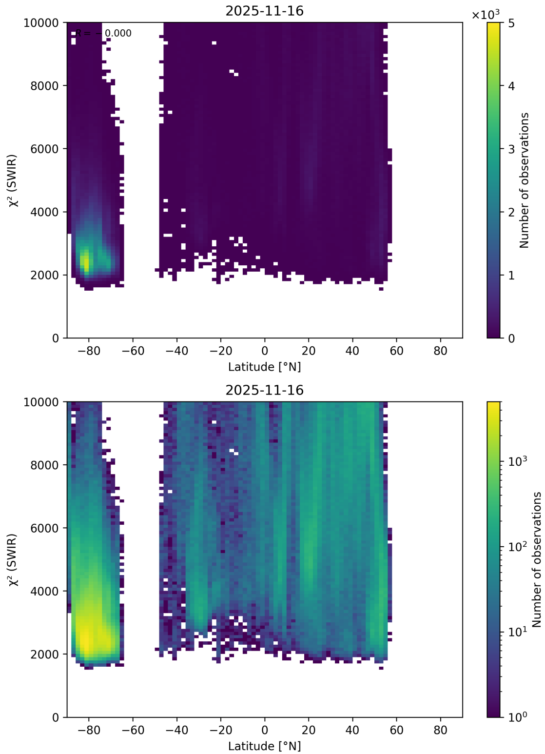
Figure 54: Scatter density plot of “Latitude” against “ \chi^2 (SWIR)” for 2025-11-15 to 2025-11-17.
