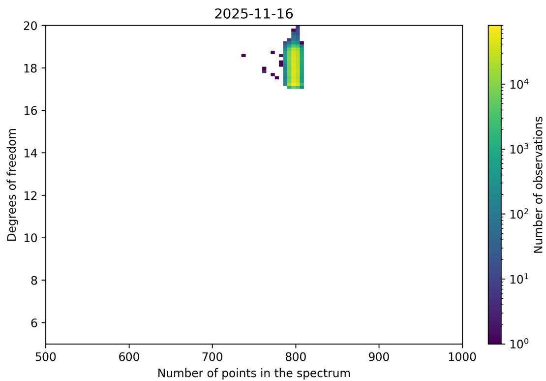
Figure 90: Scatter density plot of “Number of points in the spectrum” against “Degrees of freedom” for 2025-11-15 to 2025-11-17.
