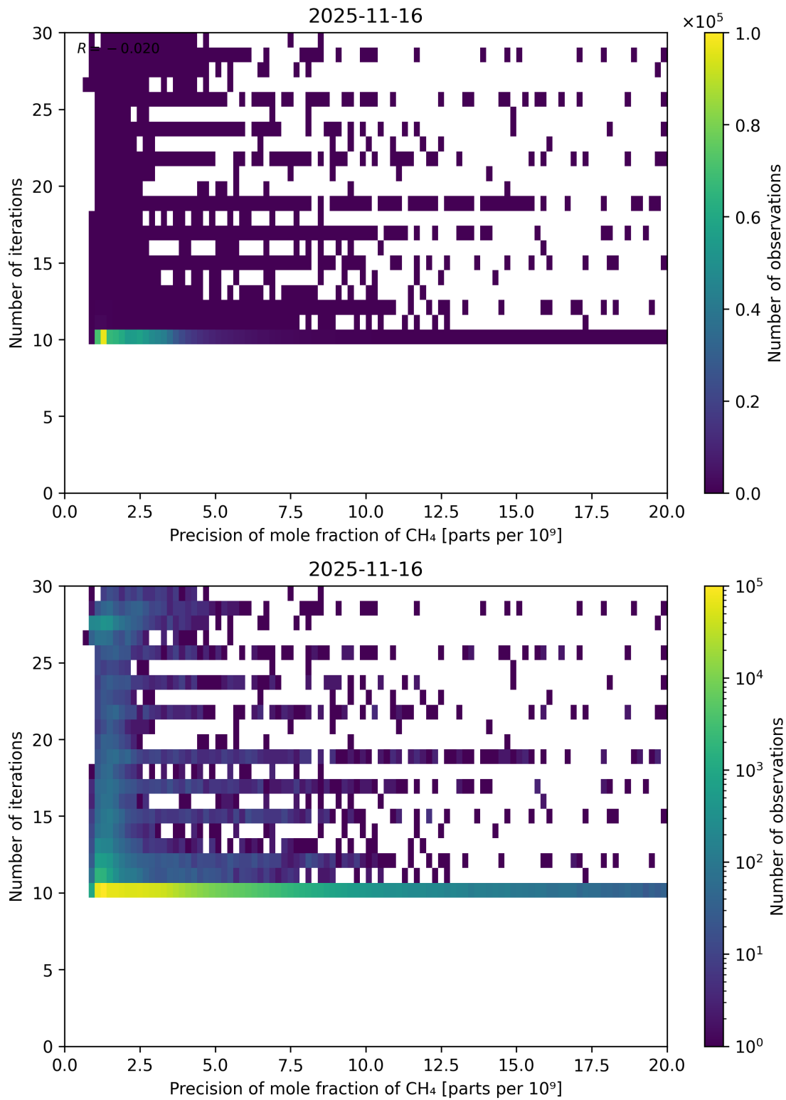
Figure 83: Scatter density plot of “Precision of mole fraction of CH 4 ” against “Number of iterations” for 2025-11-15 to 2025-11-17.
