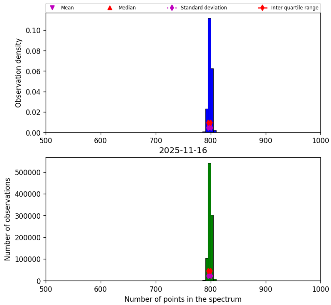
Figure 26: Histogram of “Number of points in the spectrum” for 2025-11-15 to 2025-11-17
