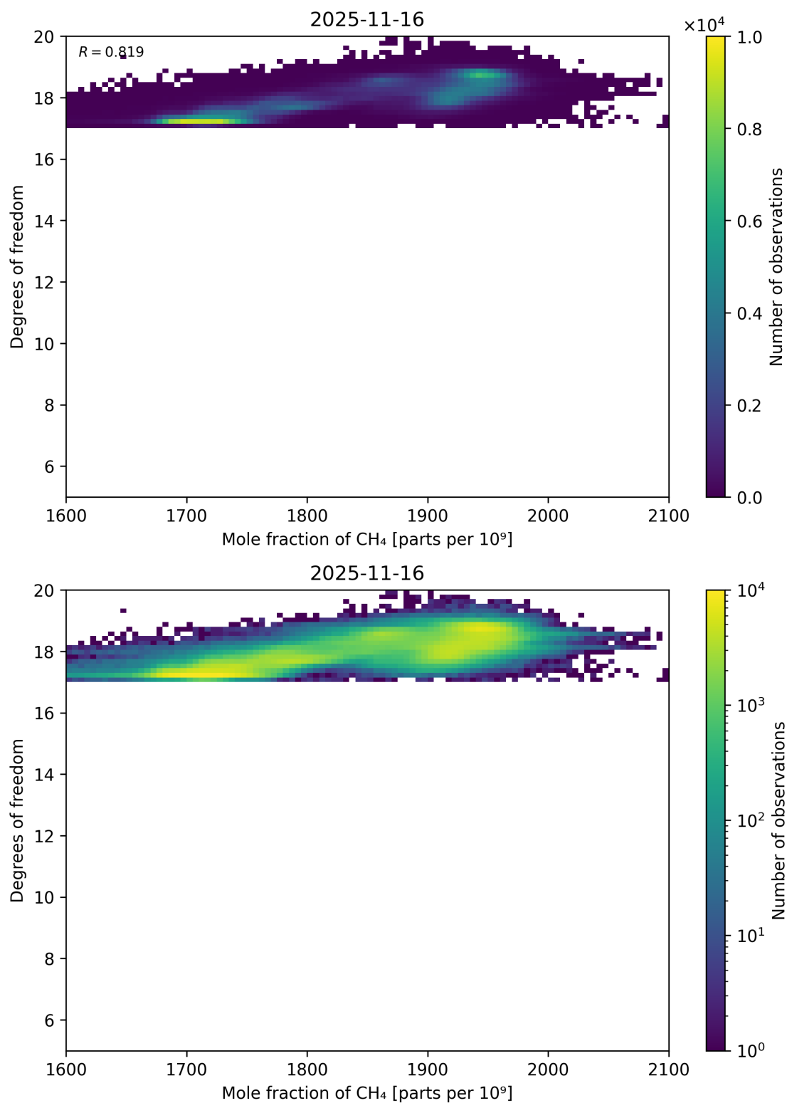
Figure 72: Scatter density plot of “Mole fraction of CH 4 ” against “Degrees of freedom” for 2025-11-15 to 2025-11-17.
