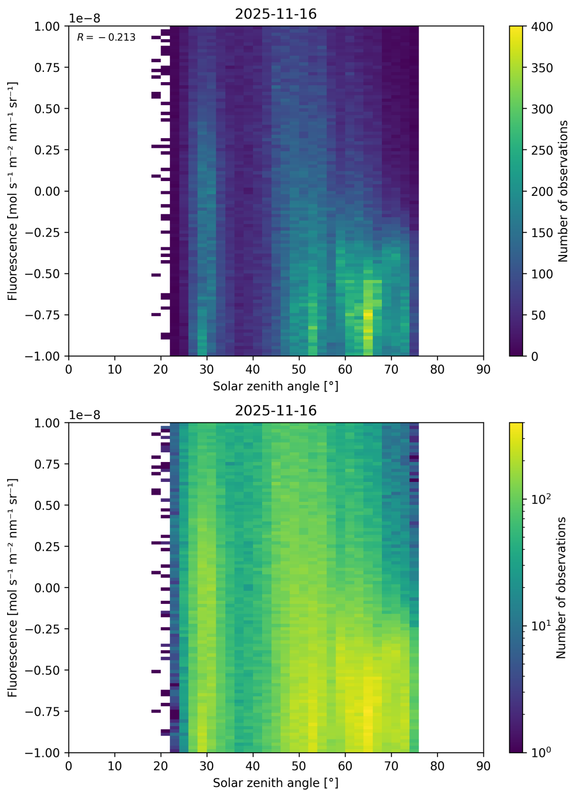
Figure 97: Scatter density plot of “Solar zenith angle” against “Fluorescence” for 2025-11-15 to 2025-11-17.
