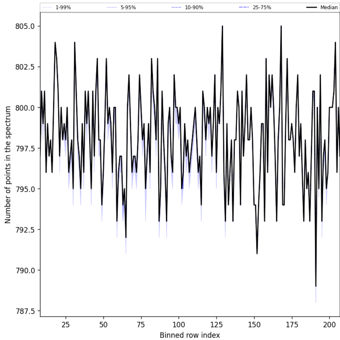
Figure 37: Along track statistics of “Number of points in the spectrum” for 2025-11-15 to 2025-11-17
