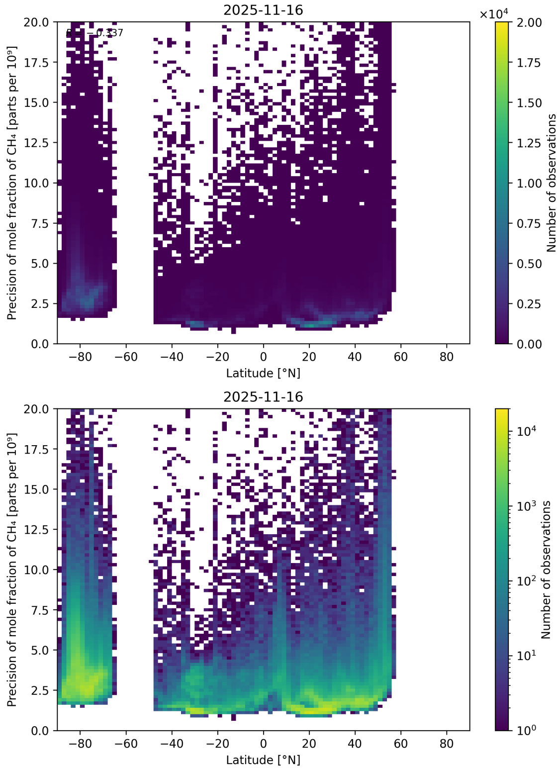
Figure 59: Scatter density plot of “Latitude” against “Precision of mole fraction of CH 4 ” for 2025-11-15 to 2025-11-17.
