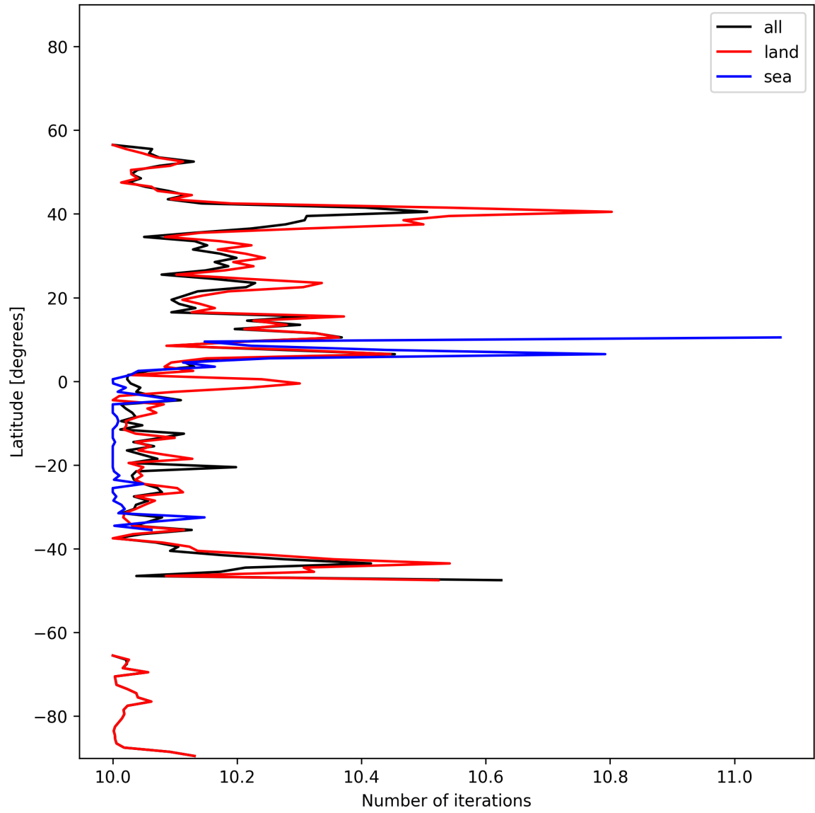
Figure 20: Zonal average of “Number of iterations” for 2025-11-15 to 2025-11-17.
