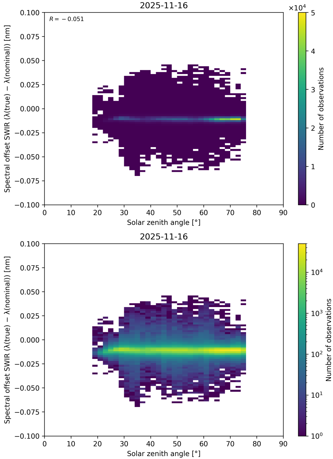
Figure 104: Scatter density plot of “Solar zenith angle” against “Spectral offset SWIR ( \lambda_{\text{true}} - \lambda_{\text{nominal}} )” for 2025-11-15 to 2025-11-17.
