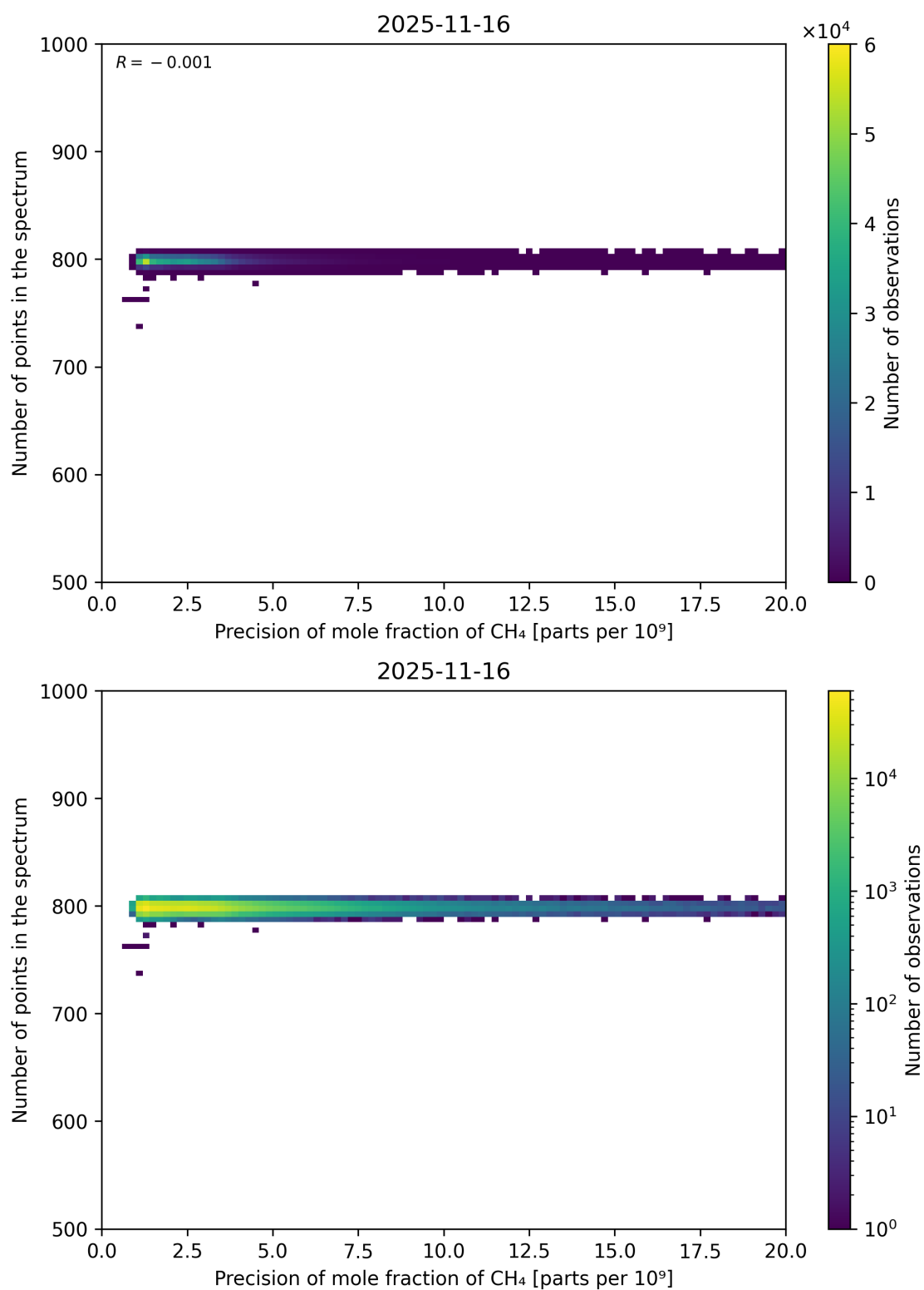
Figure 84: Scatter density plot of “Precision of mole fraction of CH 4 ” against “Number of points in the spectrum” for 2025-11-15 to 2025-11-17.
