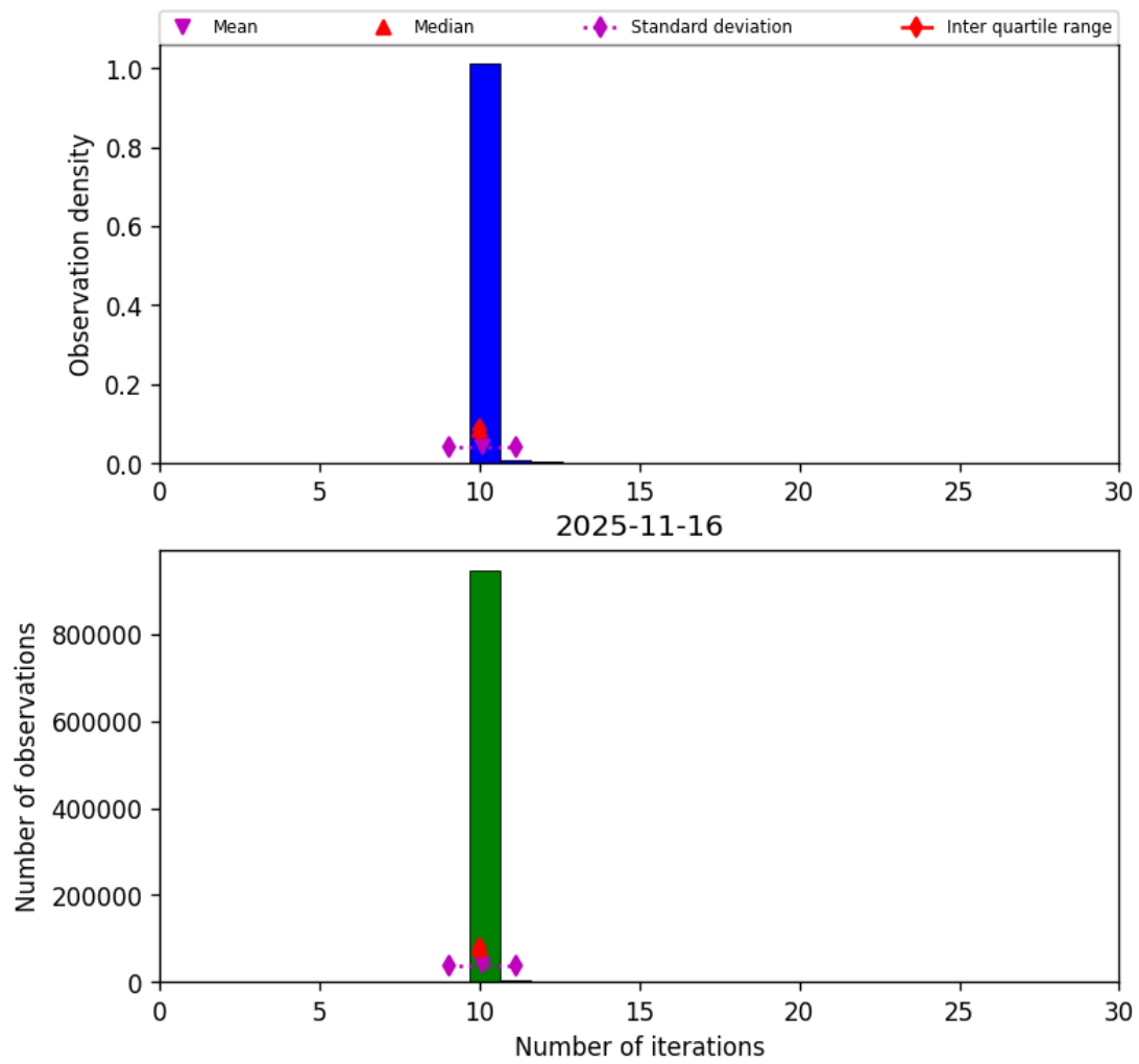
Figure 31: Histogram of “Number of iterations” for 2025-11-15 to 2025-11-17
