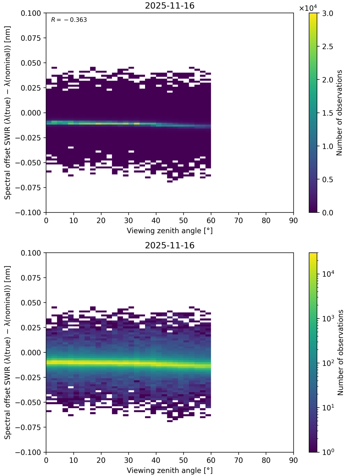
Figure 116: Scatter density plot of “Viewing zenith angle” against “Spectral offset SWIR ( \lambda_{\text{true}} - \lambda_{\text{nominal}} )” for 2025-11-15 to 2025-11-17.
