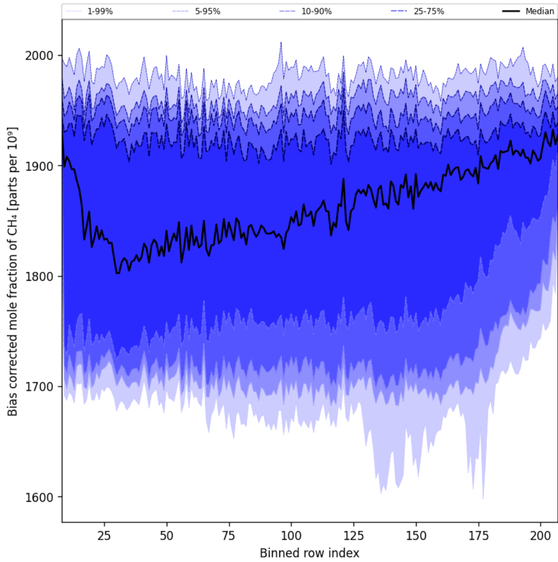
Figure 36: Along track statistics of “Bias corrected mole fraction of CH 4 ” for 2025-11-15 to 2025-11-17
