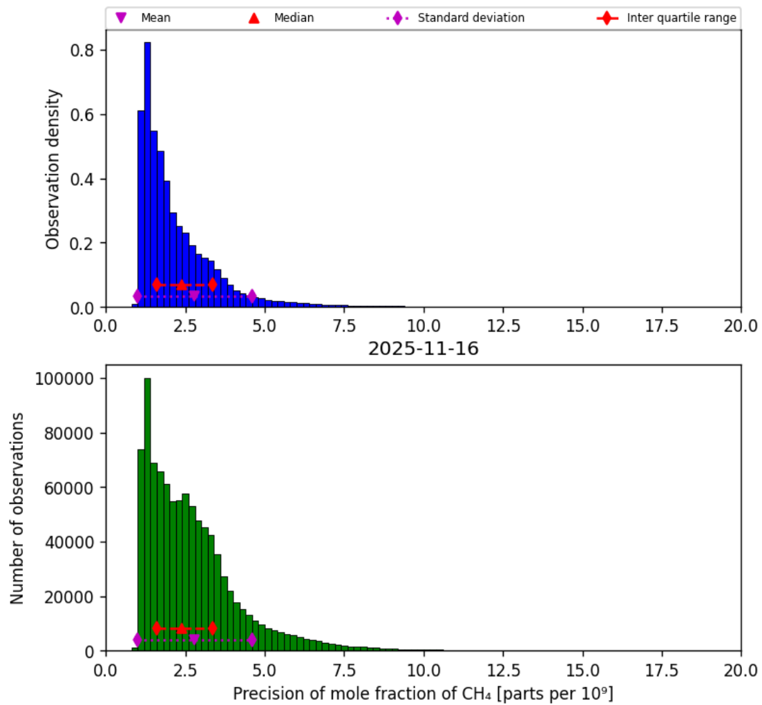
Figure 24: Histogram of “Precision of mole fraction of CH 4 ” for 2025-11-15 to 2025-11-17
