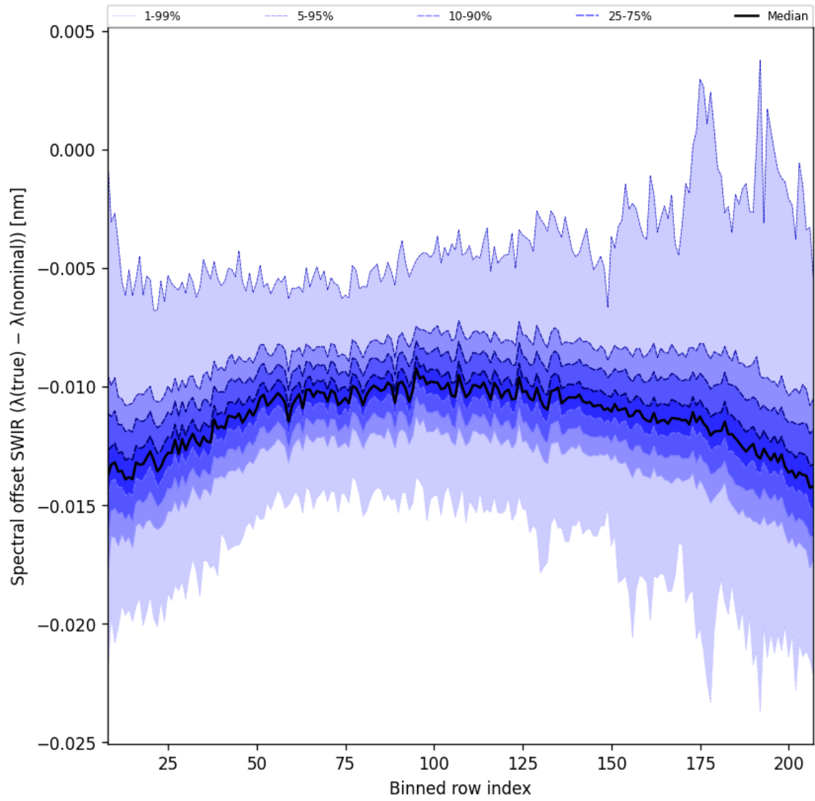
Figure 38: Along track statistics of “Spectral offset SWIR ( \lambda_{\text{true}} - \lambda_{\text{nominal}} )” for 2025-11-15 to 2025-11-17
