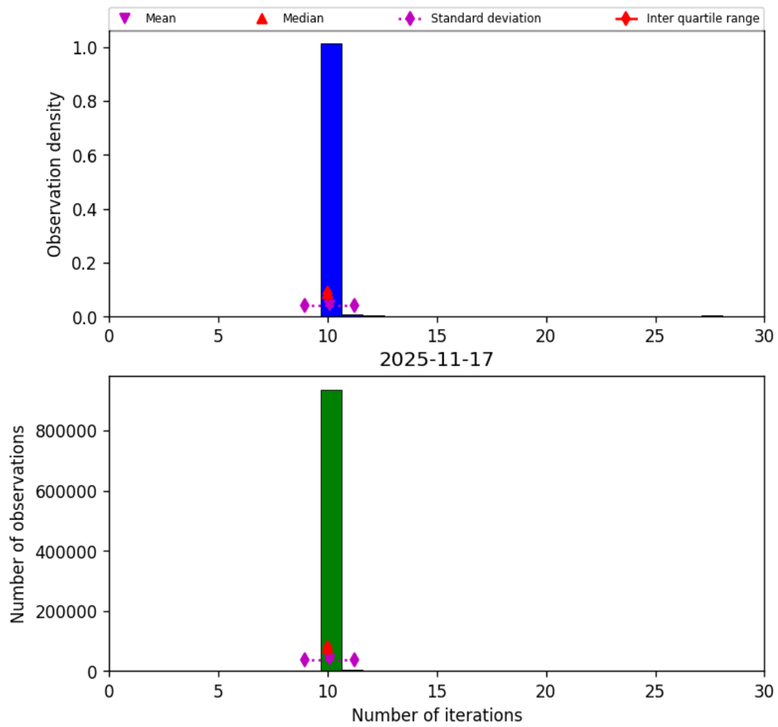
Figure 31: Histogram of “Number of iterations” for 2025-11-16 to 2025-11-18
