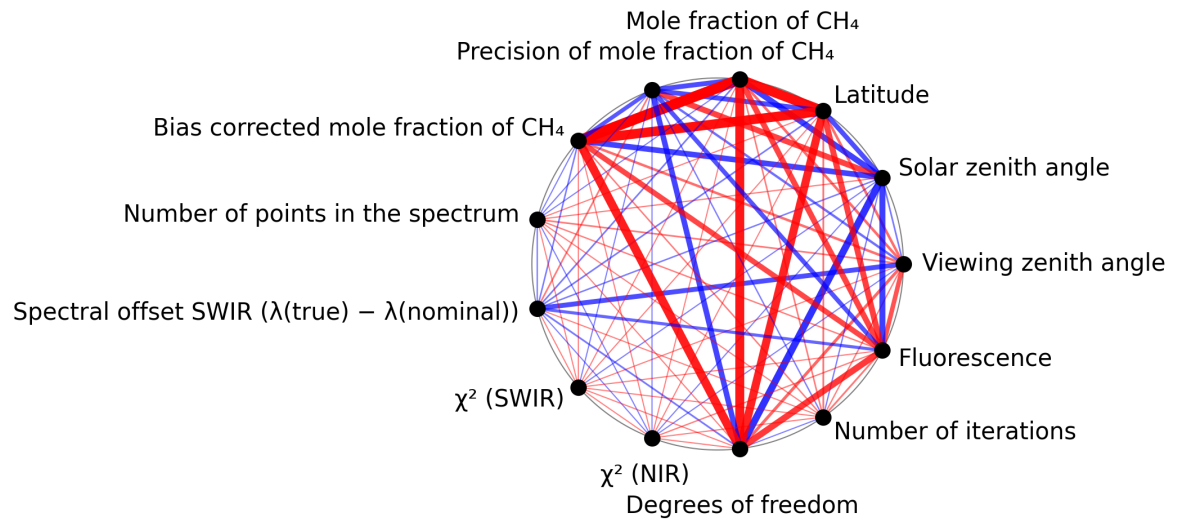
Figure 1: Map of correlation graph for 2025-11-16 to 2025-11-18.
