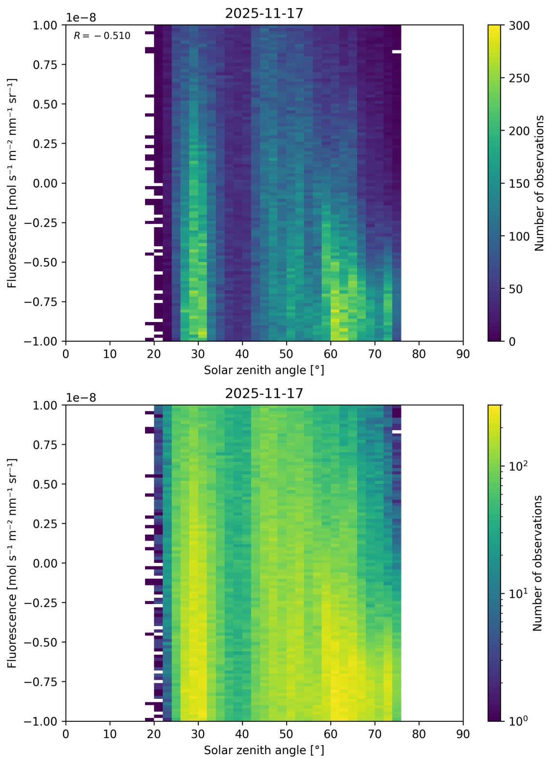
Figure 97: Scatter density plot of “Solar zenith angle” against “Fluorescence” for 2025-11-16 to 2025-11-18.
