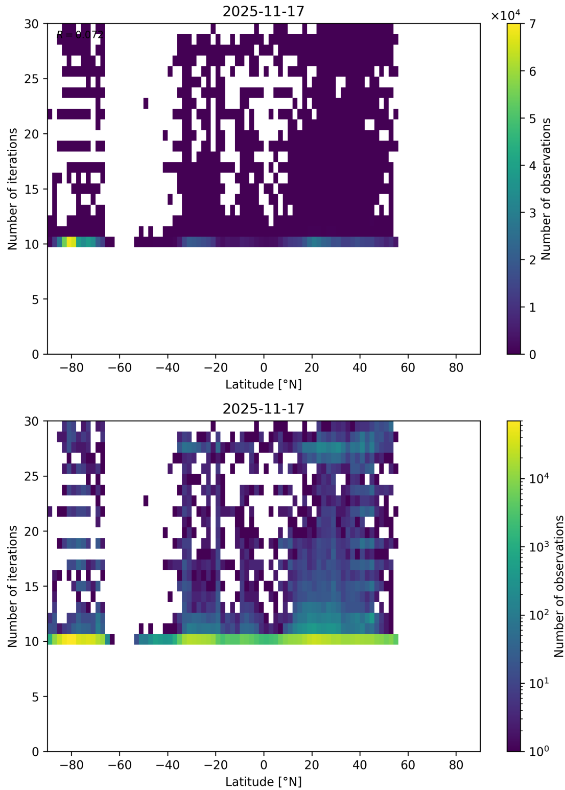
Figure 60: Scatter density plot of “Latitude” against “Number of iterations” for 2025-11-16 to 2025-11-18.
