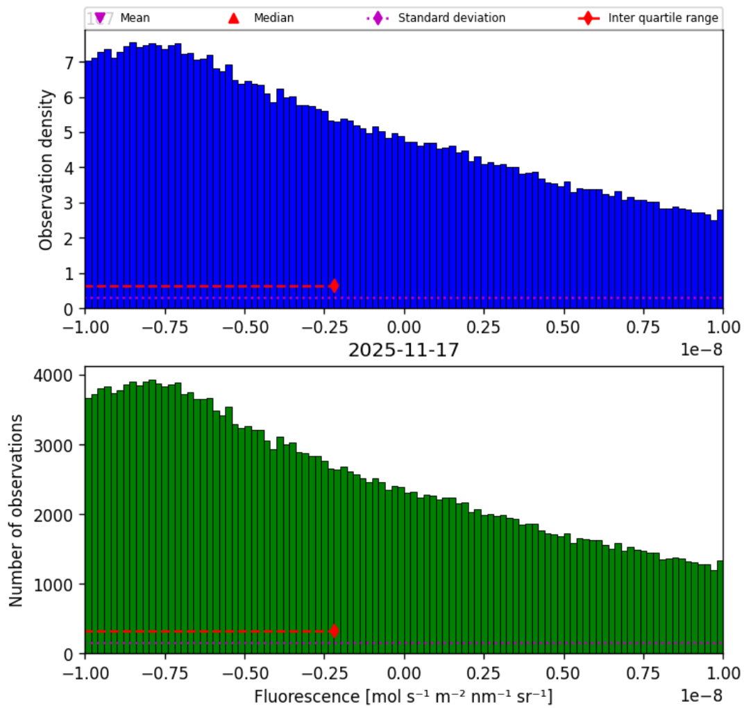
Figure 32: Histogram of “Fluorescence” for 2025-11-16 to 2025-11-18
