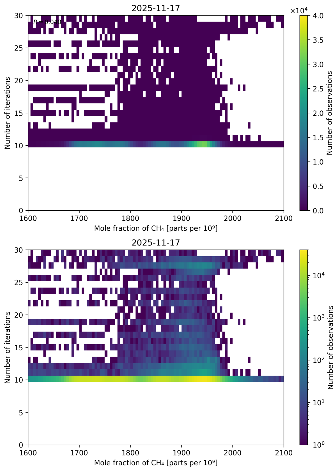
Figure 76: Scatter density plot of “Mole fraction of CH 4 ” against “Number of iterations” for 2025-11-16 to 2025-11-18.
