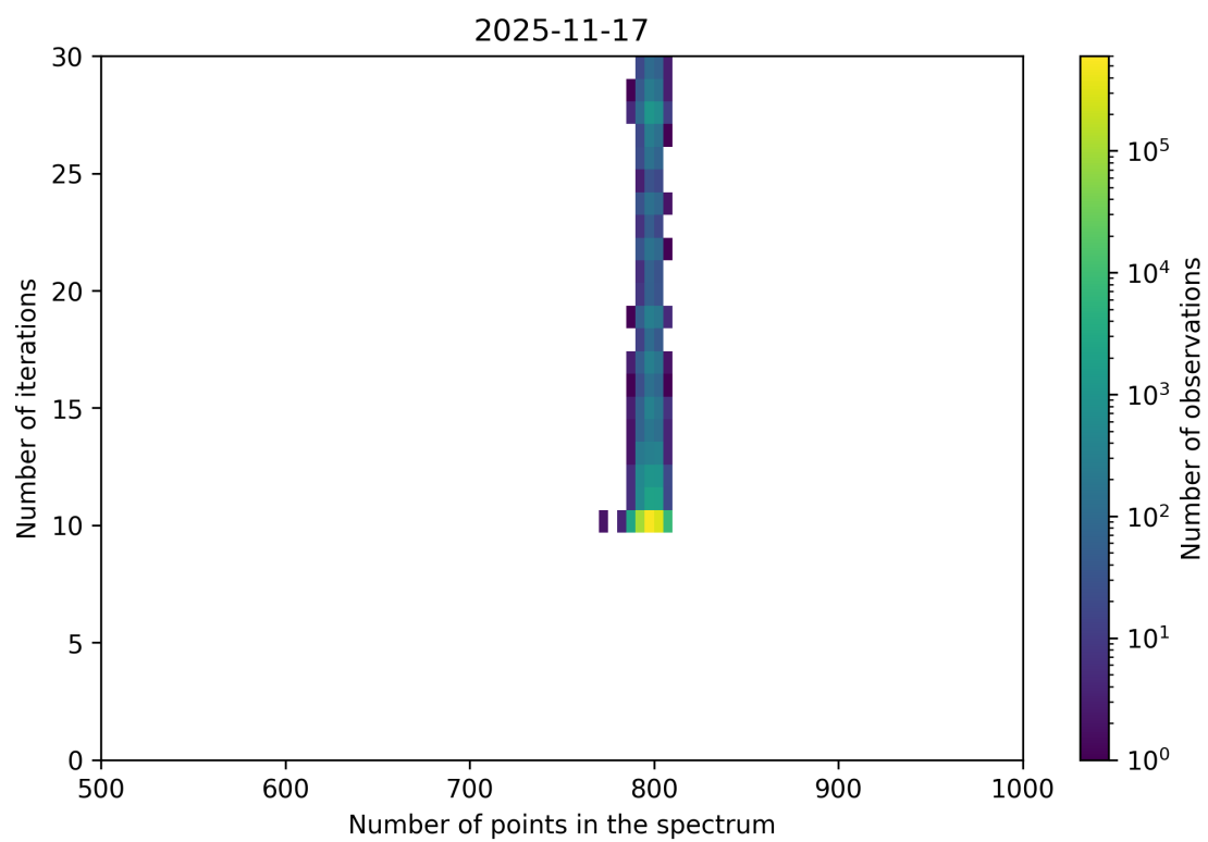
Figure 92: Scatter density plot of “Number of points in the spectrum” against “Number of iterations” for 2025-11-16 to 2025-11-18.
