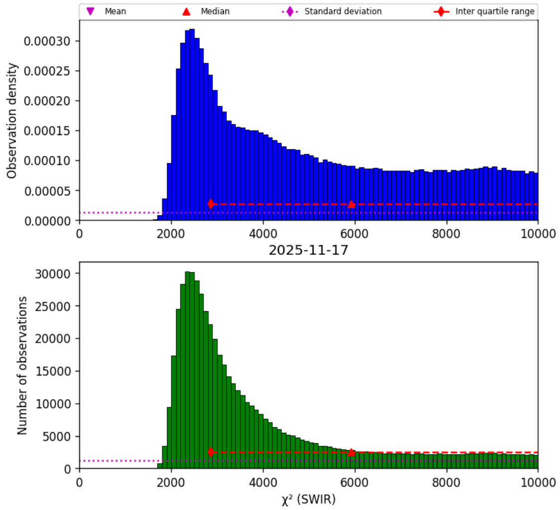
Figure 28: Histogram of “ \chi^2 (SWIR)” for 2025-11-16 to 2025-11-18
