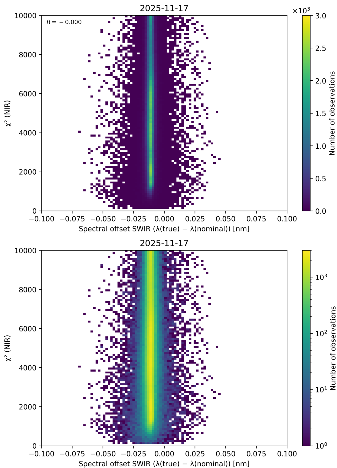
Figure 117: Scatter density plot of “Spectral offset SWIR ( \lambda_{\text{true}} - \lambda_{\text{nominal}} )” against “ \chi^2 (NIR)” for 2025-11-16 to 2025-11-18.
