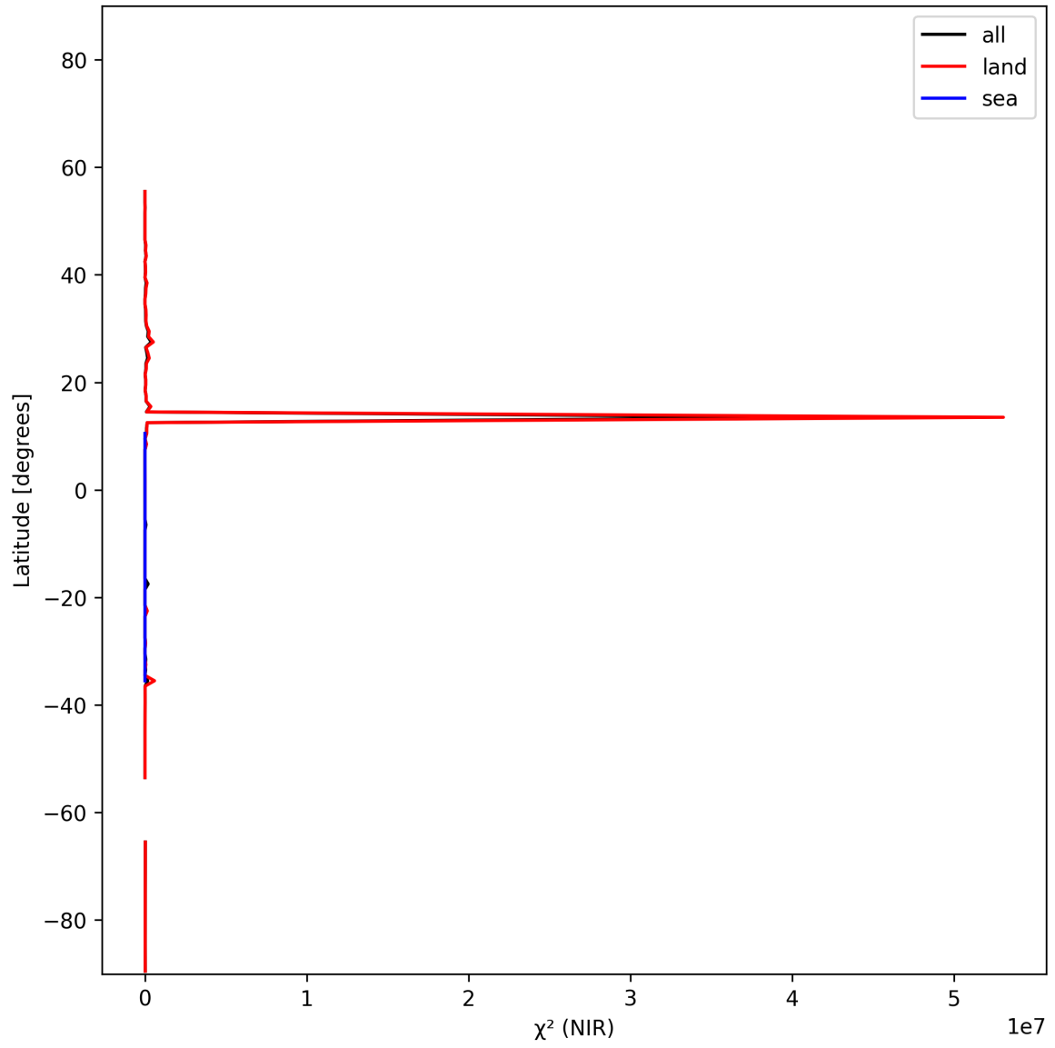
Figure 18: Zonal average of “ \chi^2 (NIR)” for 2025-11-16 to 2025-11-18.
