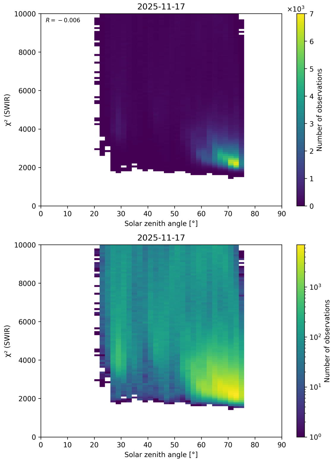
Figure 95: Scatter density plot of “Solar zenith angle” against “ \chi^2 (SWIR)” for 2025-11-16 to 2025-11-18.
