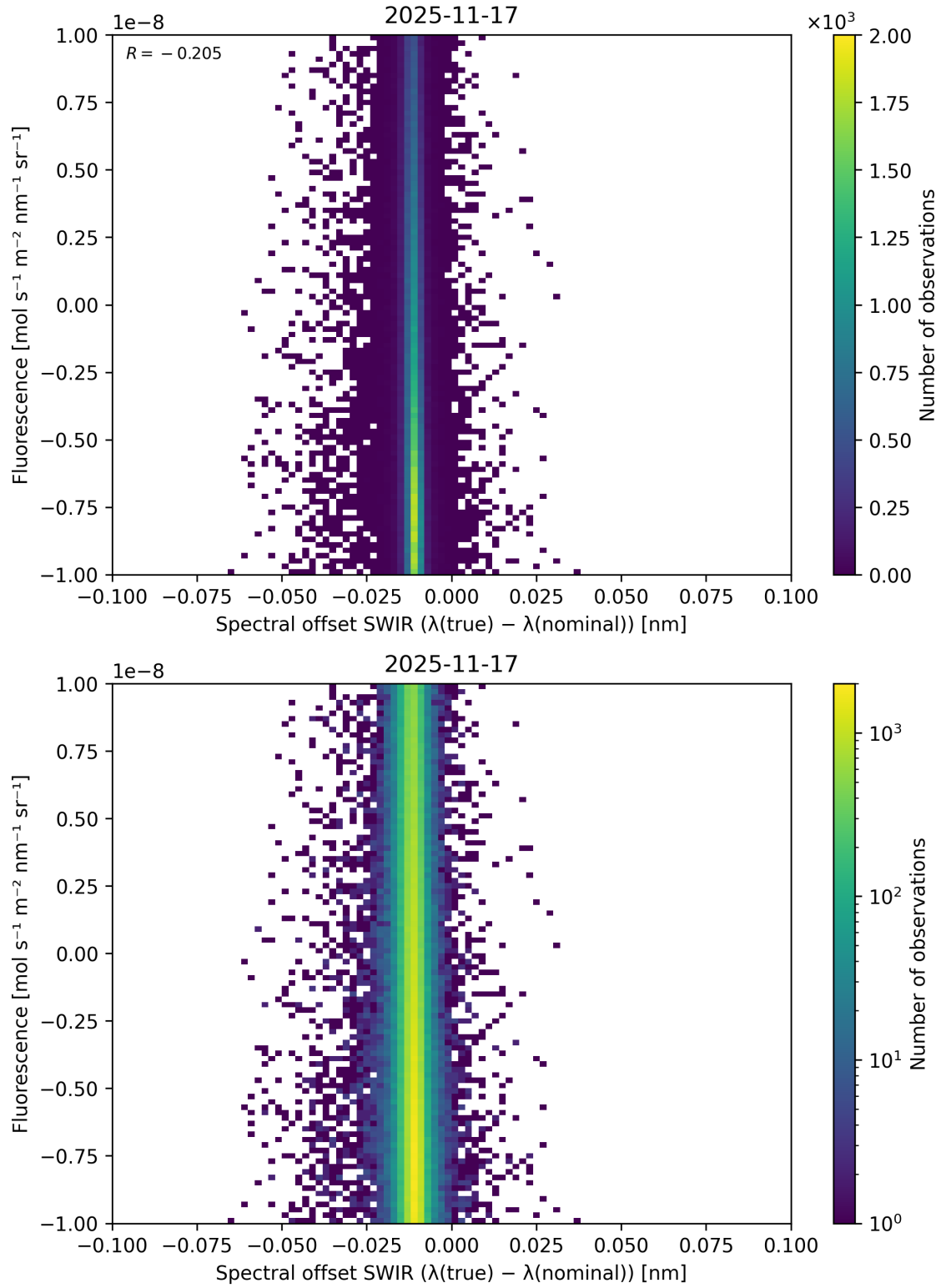
Figure 120: Scatter density plot of “Spectral offset SWIR ( \lambda_{\text{true}} - \lambda_{\text{nominal}} )” against “Fluorescence” for 2025-11-16 to 2025-11-18.
