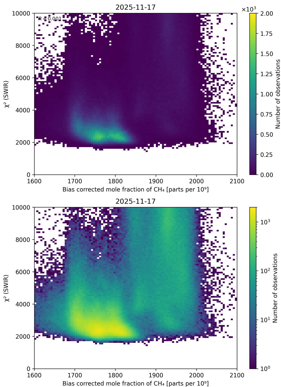
Figure 64: Scatter density plot of “Bias corrected mole fraction of CH 4 ” against “ \chi^2 (SWIR)” for 2025-11-16 to 2025-11-18.
