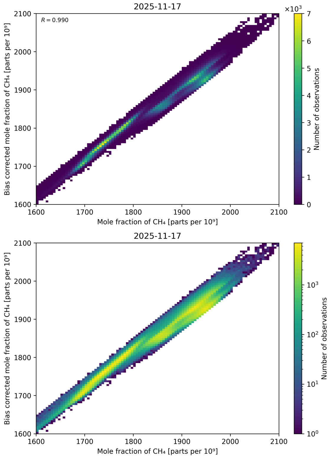
Figure 74: Scatter density plot of “Mole fraction of CH 4 ” against “Bias corrected mole fraction of CH 4 ” for 2025-11-16 to 2025-11-18.
