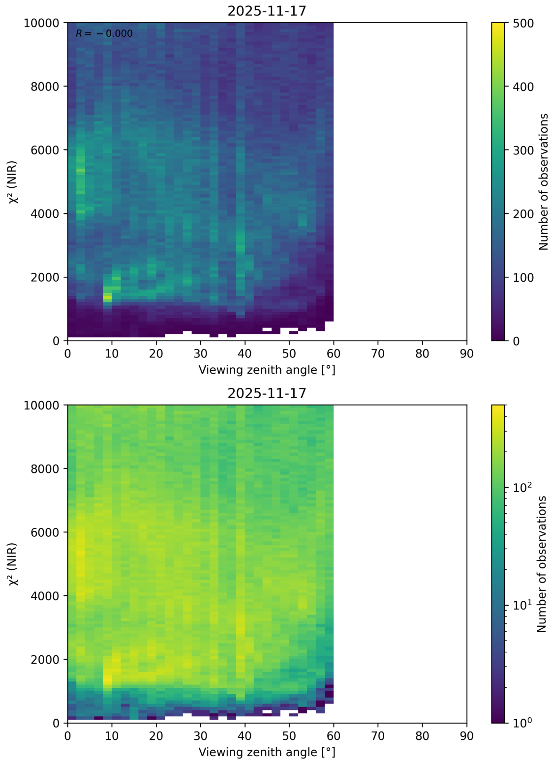
Figure 105: Scatter density plot of “Viewing zenith angle” against “ \chi^2 (NIR)” for 2025-11-16 to 2025-11-18.
