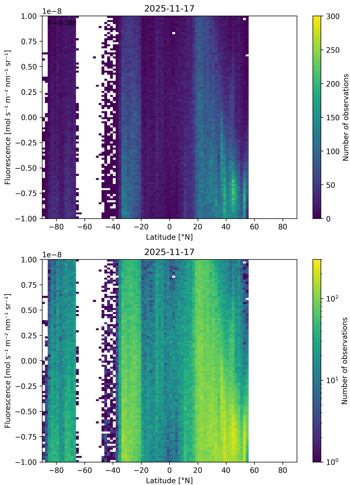
Figure 56: Scatter density plot of “Latitude” against “Fluorescence” for 2025-11-16 to 2025-11-18.
