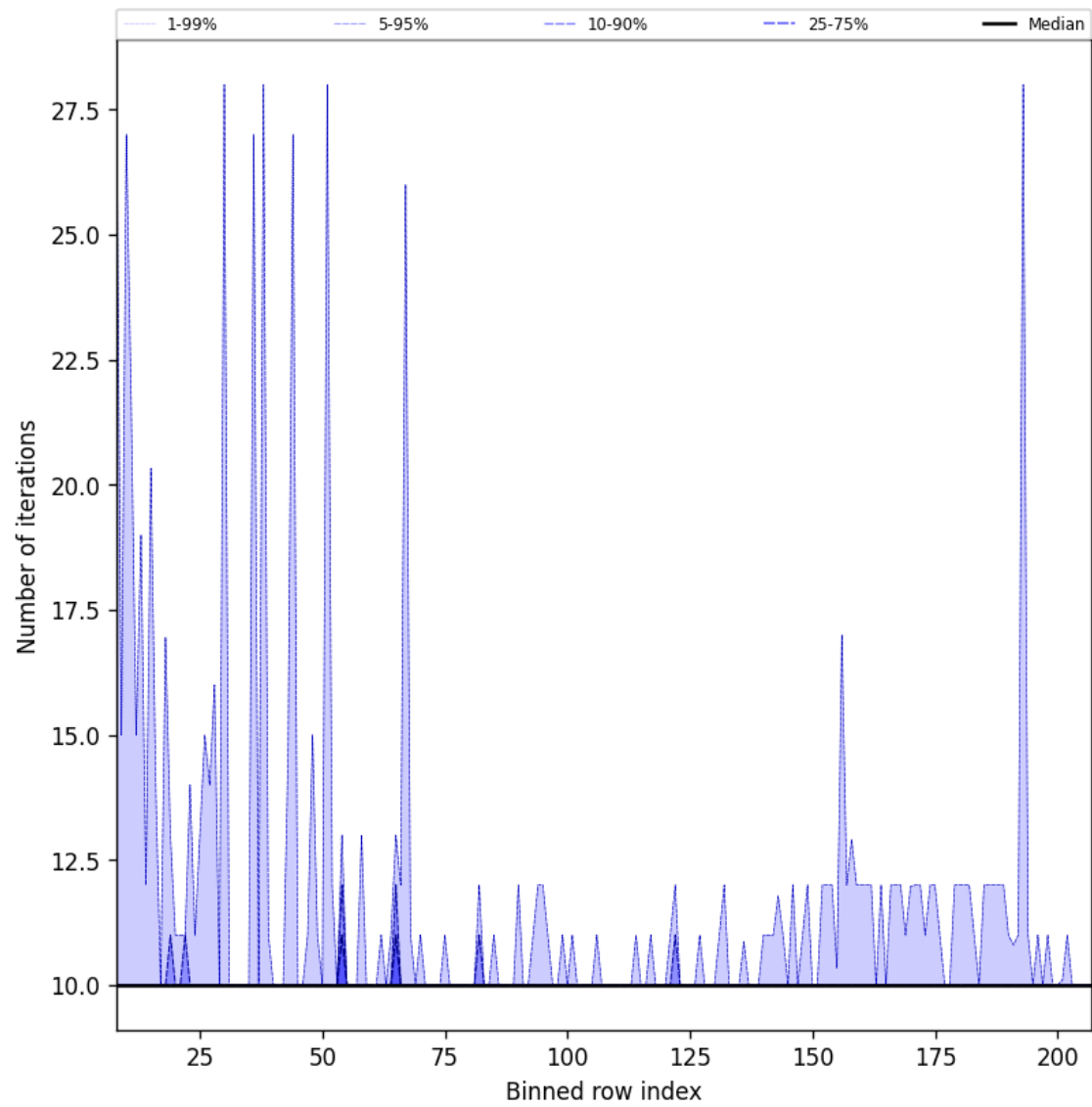
Figure 42: Along track statistics of “Number of iterations” for 2025-11-16 to 2025-11-18
