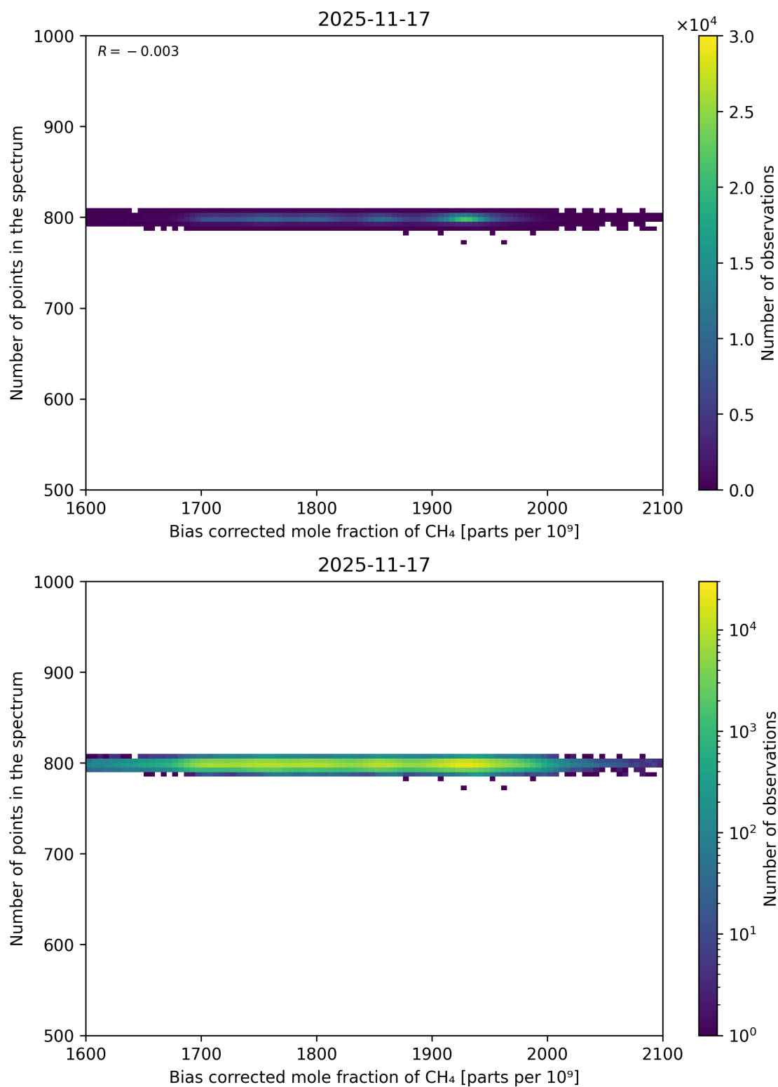
Figure 68: Scatter density plot of “Bias corrected mole fraction of CH 4 ” against “Number of points in the spectrum” for 2025-11-16 to 2025-11-18.
