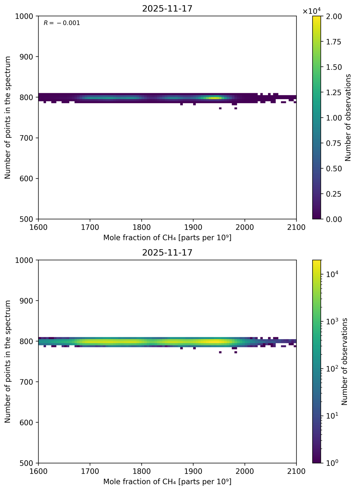
Figure 77: Scatter density plot of “Mole fraction of CH 4 ” against “Number of points in the spectrum” for 2025-11-16 to 2025-11-18.
