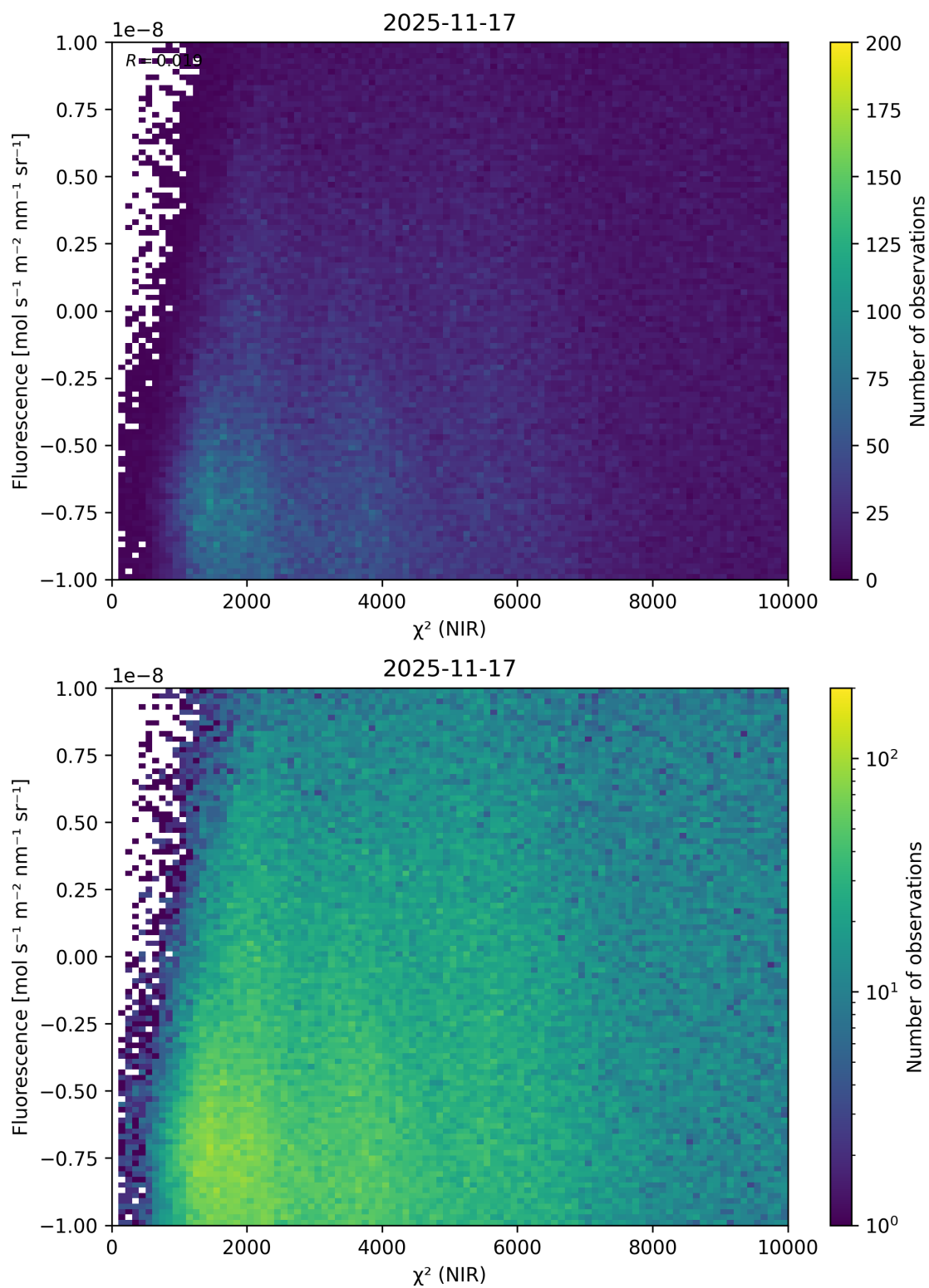
Figure 45: Scatter density plot of “ \chi^2 (NIR)” against “Fluorescence” for 2025-11-16 to 2025-11-18.
