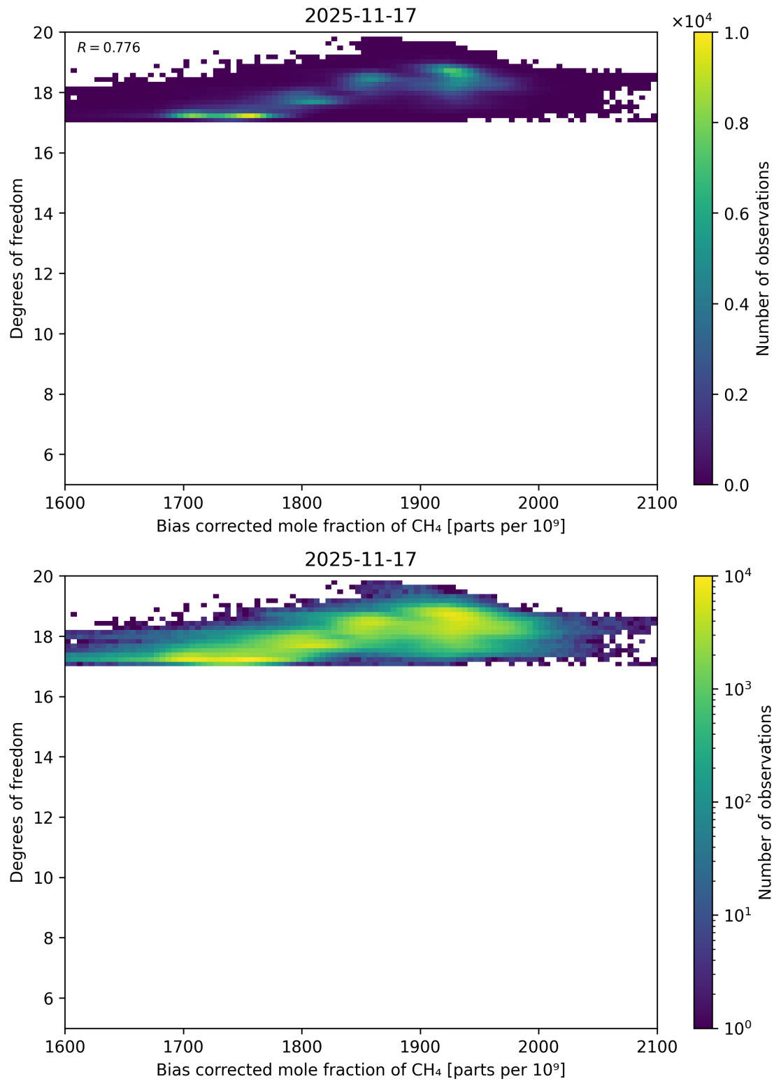
Figure 65: Scatter density plot of “Bias corrected mole fraction of CH 4 ” against “Degrees of freedom” for 2025-11-16 to 2025-11-18.
