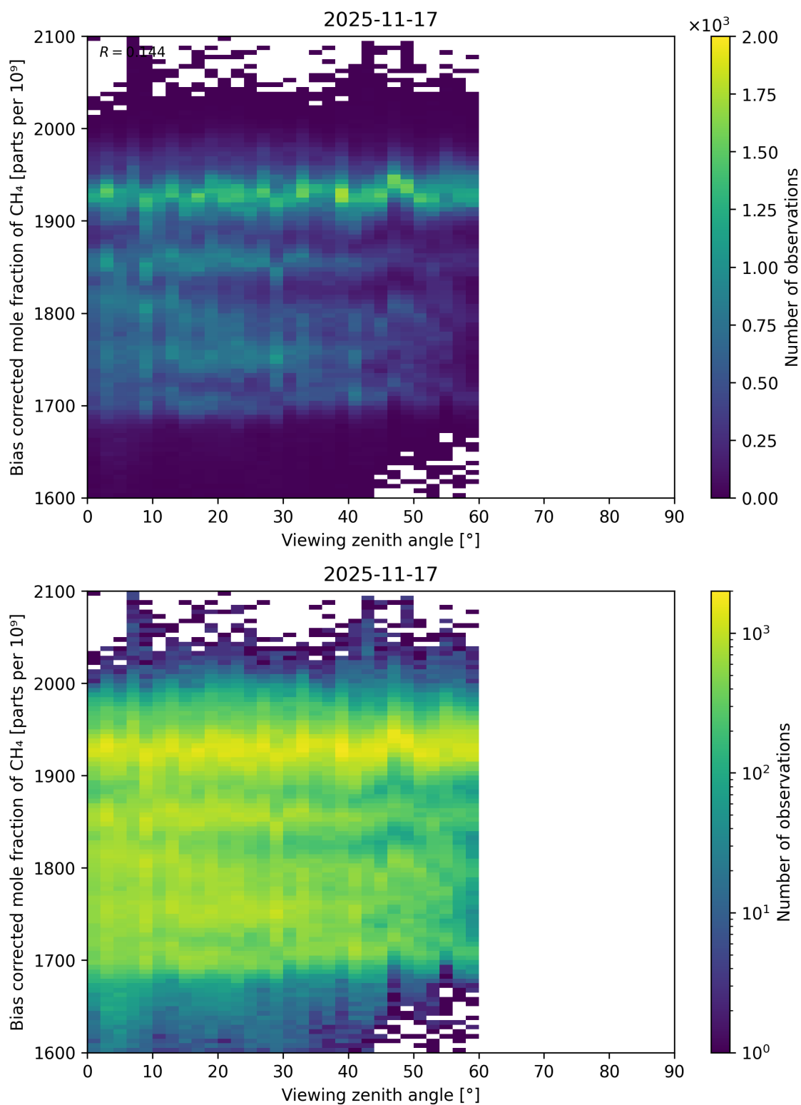
Figure 111: Scatter density plot of “Viewing zenith angle” against “Bias corrected mole fraction of CH 4 ” for 2025-11-16 to 2025-11-18.
