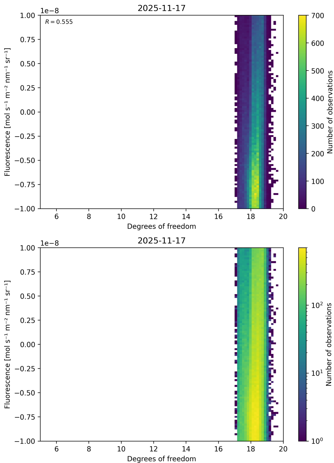
Figure 51: Scatter density plot of “Degrees of freedom” against “Fluorescence” for 2025-11-16 to 2025-11-18.
