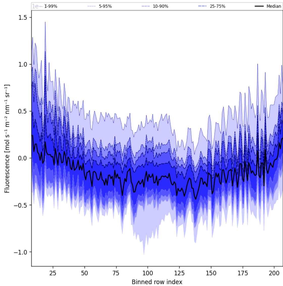
Figure 43: Along track statistics of “Fluorescence” for 2025-11-16 to 2025-11-18
