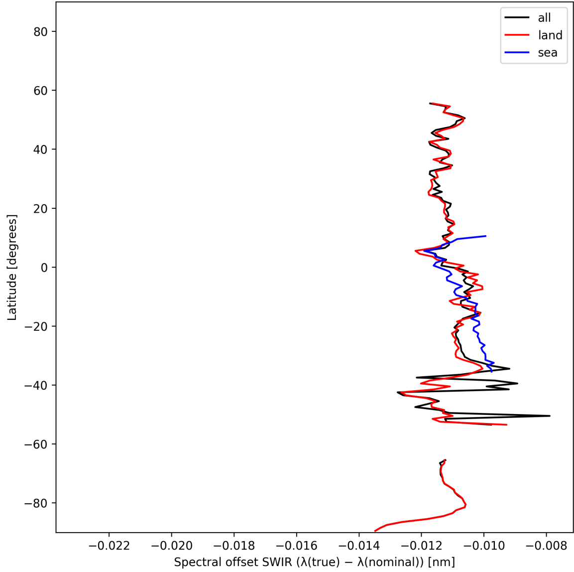
Figure 16: Zonal average of “Spectral offset SWIR ( \lambda_{\text{true}} - \lambda_{\text{nominal}} )” for 2025-11-16 to 2025-11-18.
