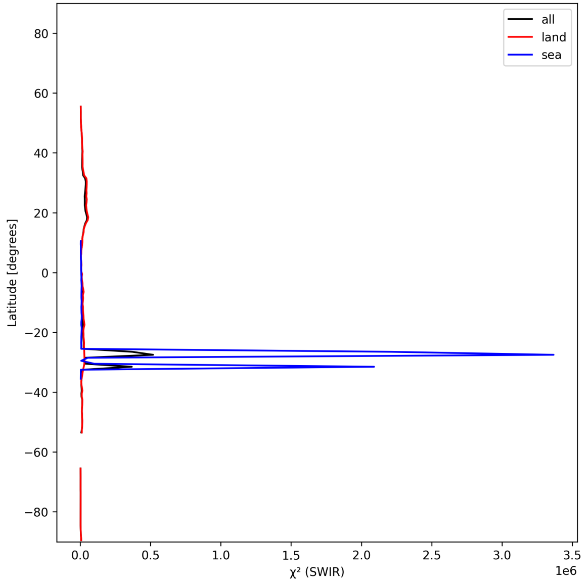
Figure 17: Zonal average of “ \chi^2 (SWIR)” for 2025-11-16 to 2025-11-18.
