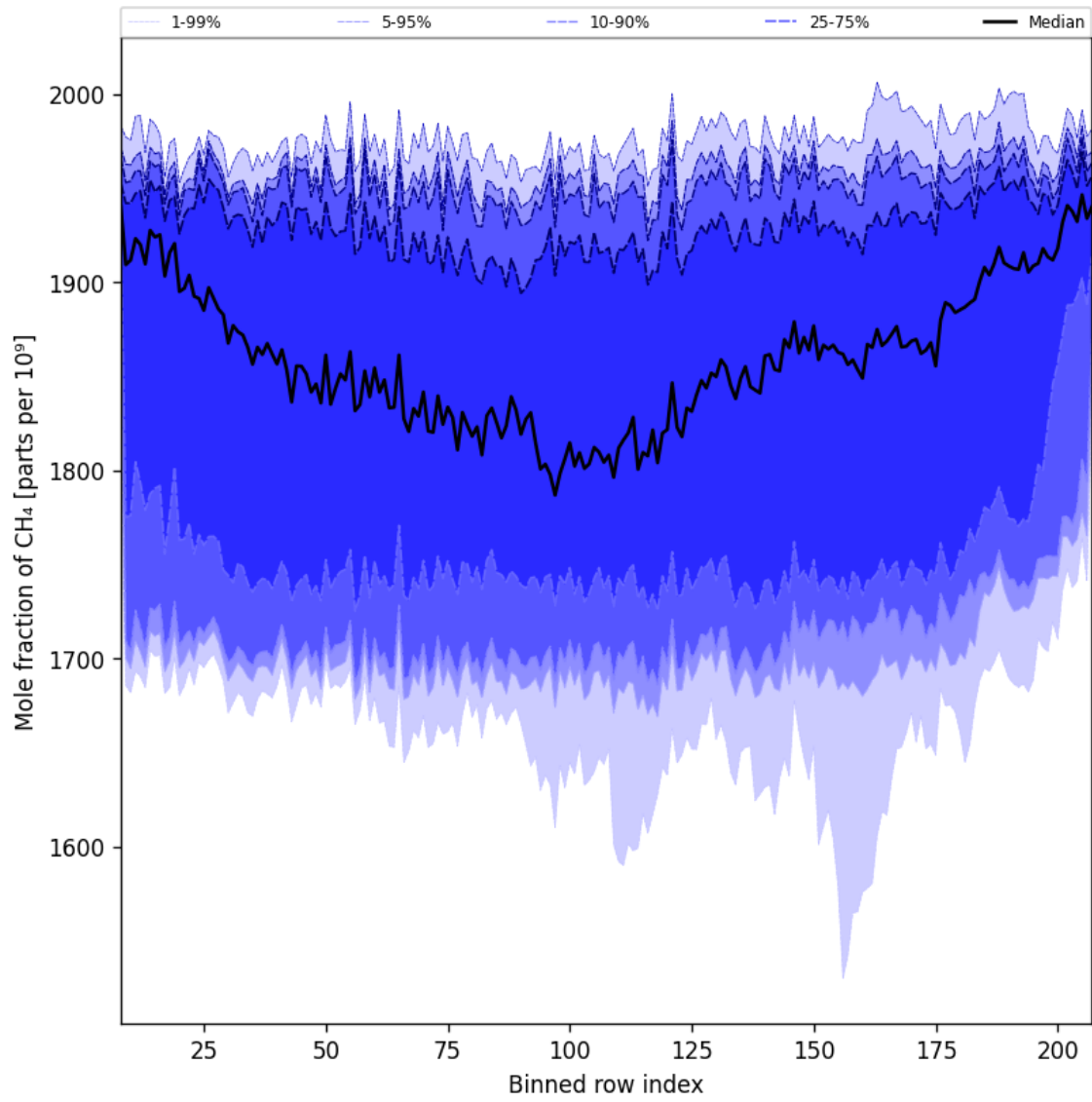
Figure 34: Along track statistics of “Mole fraction of CH 4 ” for 2025-11-16 to 2025-11-18
