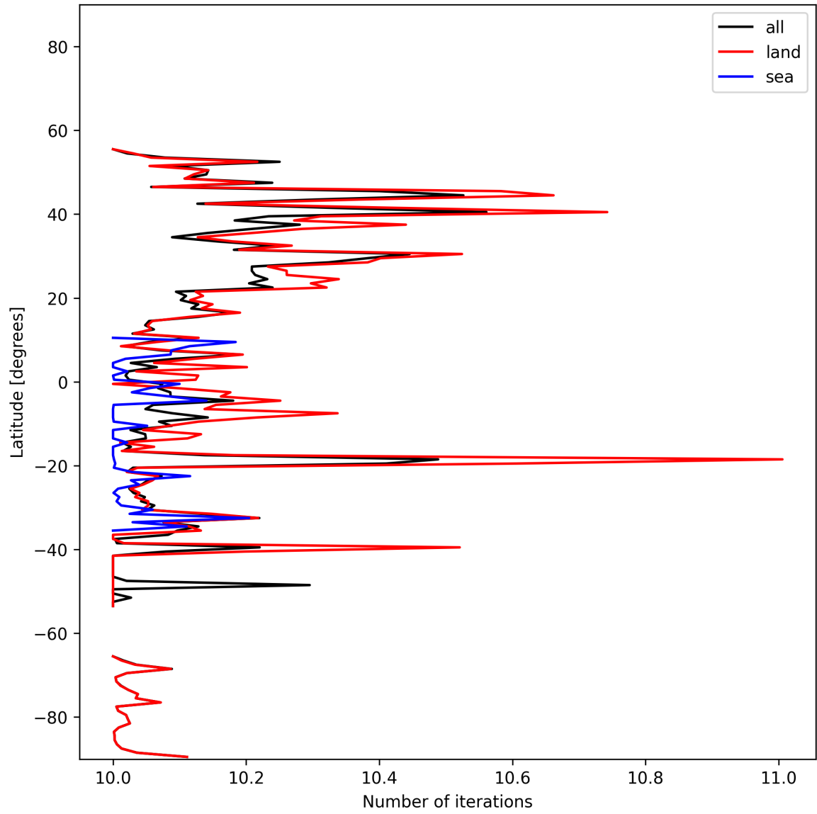
Figure 20: Zonal average of “Number of iterations” for 2025-11-16 to 2025-11-18.
