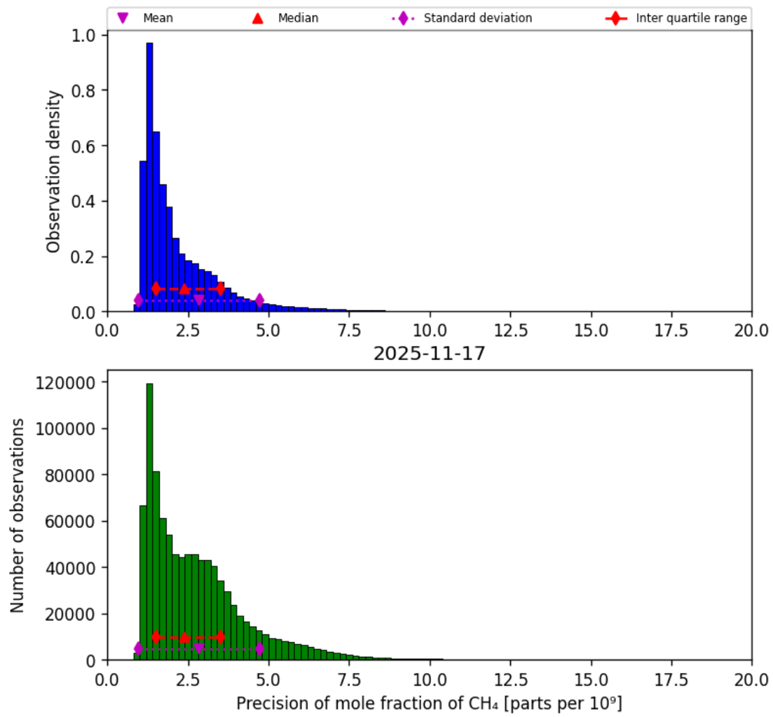
Figure 24: Histogram of “Precision of mole fraction of CH 4 ” for 2025-11-16 to 2025-11-18
