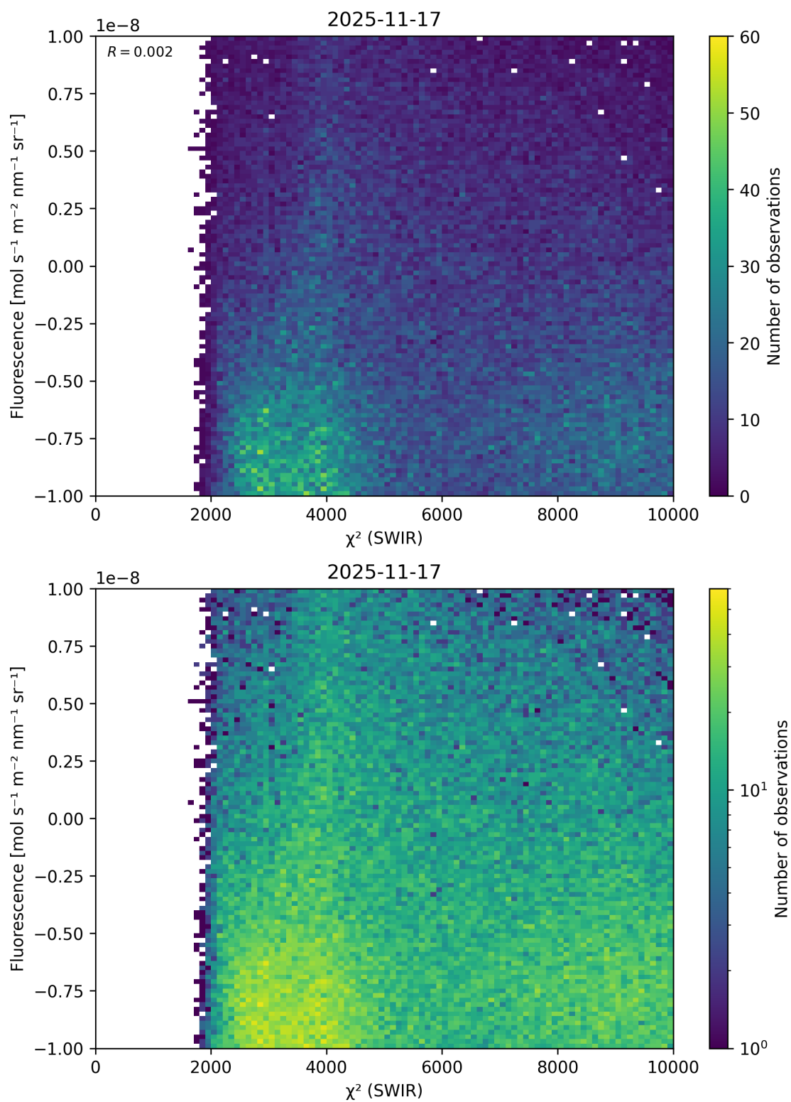
Figure 49: Scatter density plot of “ \chi^2 (SWIR)” against “Fluorescence” for 2025-11-16 to 2025-11-18.
