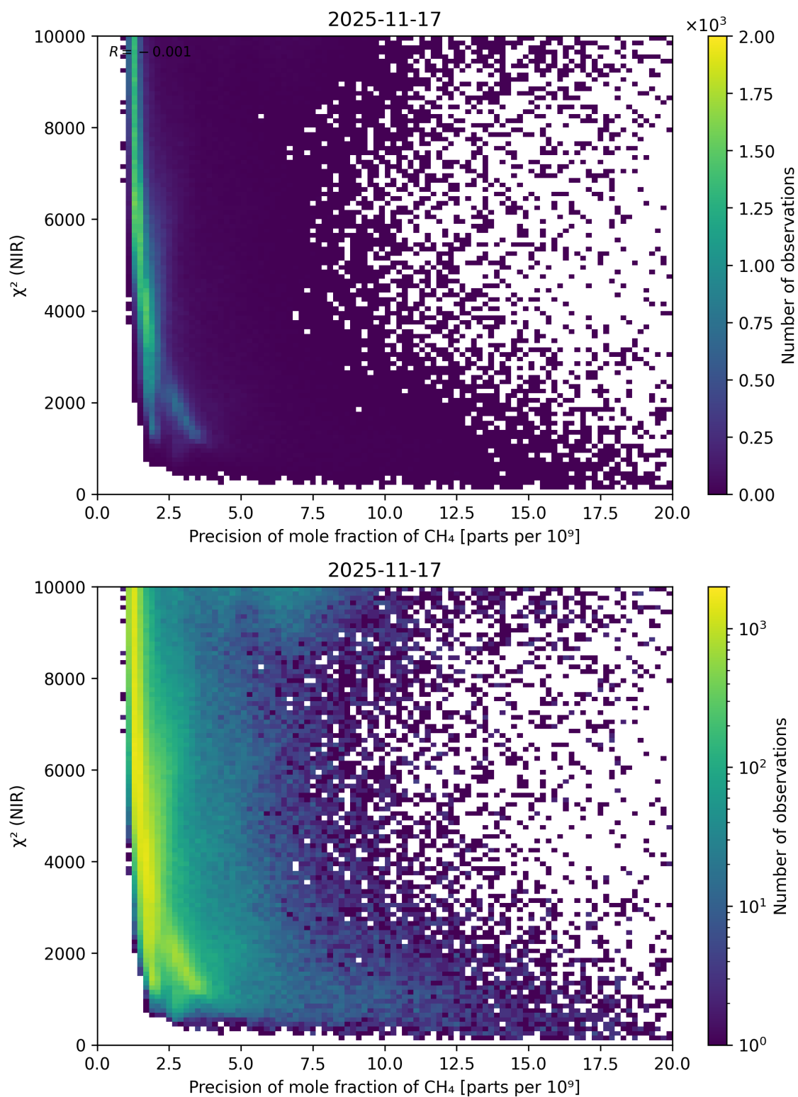
Figure 78: Scatter density plot of “Precision of mole fraction of CH 4 ” against “ \chi^2 (NIR)” for 2025-11-16 to 2025-11-18.
