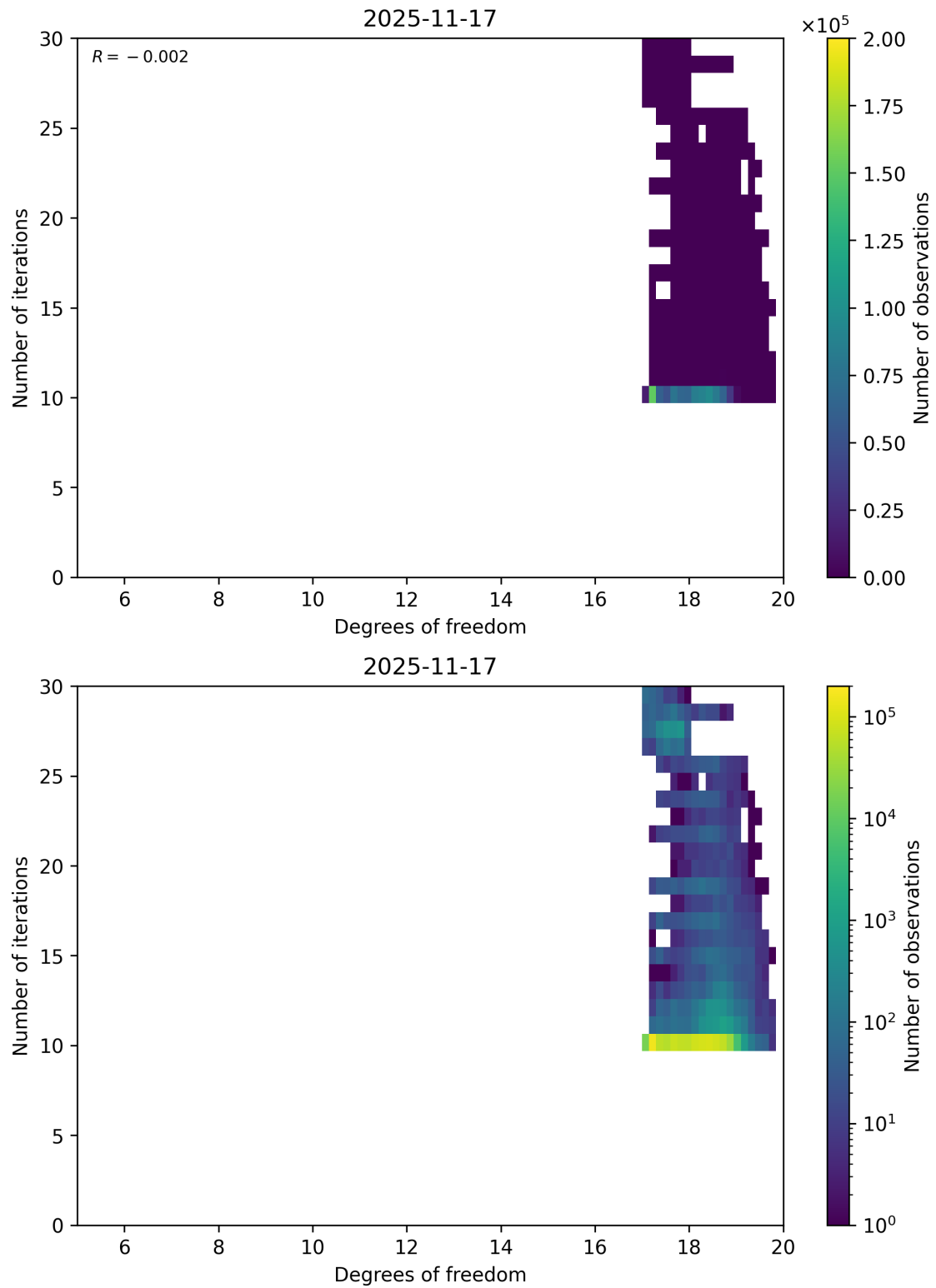
Figure 52: Scatter density plot of “Degrees of freedom” against “Number of iterations” for 2025-11-16 to 2025-11-18.
