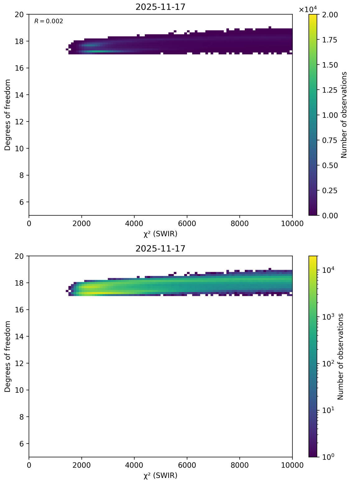
Figure 48: Scatter density plot of “ \chi^2 (SWIR)” against “Degrees of freedom” for 2025-11-16 to 2025-11-18.
