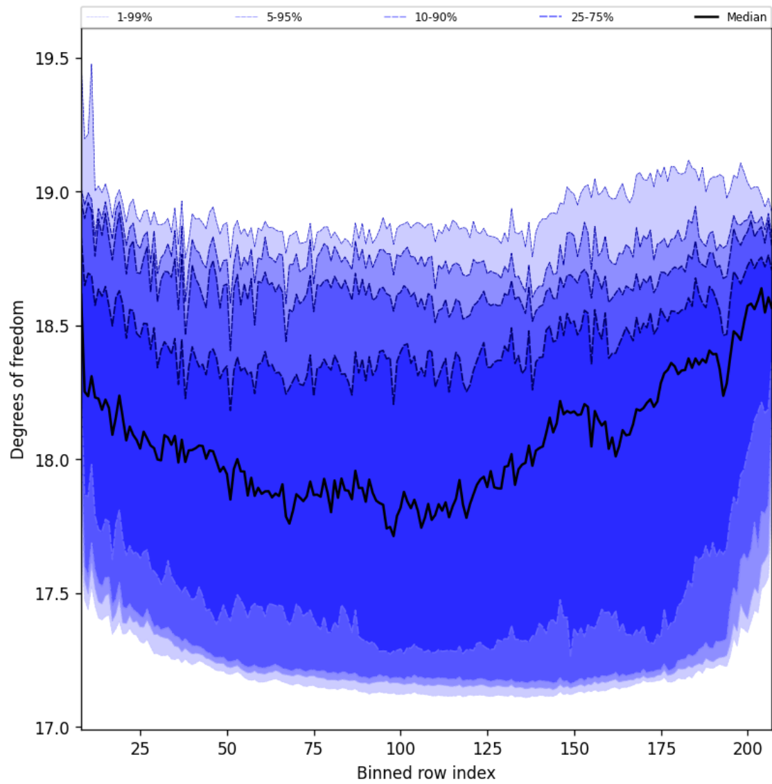
Figure 41: Along track statistics of “Degrees of freedom” for 2025-11-16 to 2025-11-18
