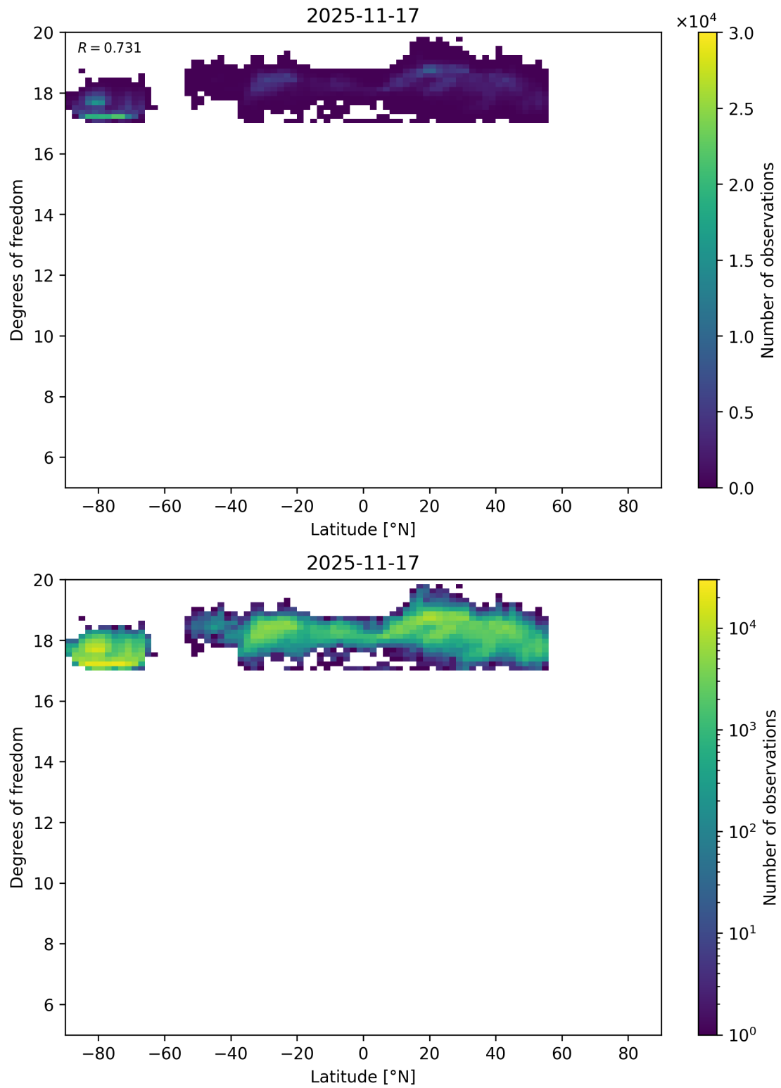
Figure 55: Scatter density plot of “Latitude” against “Degrees of freedom” for 2025-11-16 to 2025-11-18.
