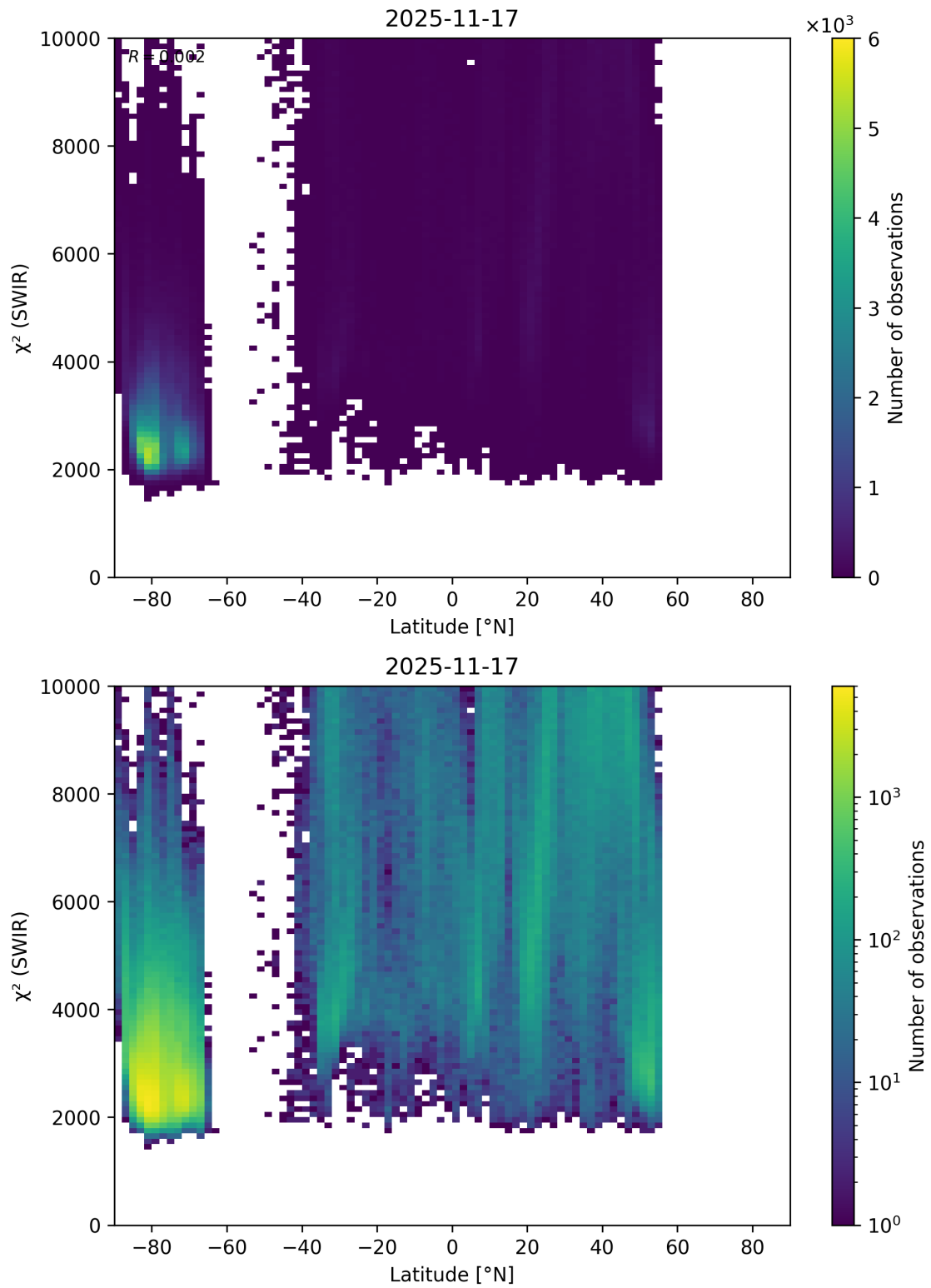
Figure 54: Scatter density plot of “Latitude” against “ \chi^2 (SWIR)” for 2025-11-16 to 2025-11-18.
