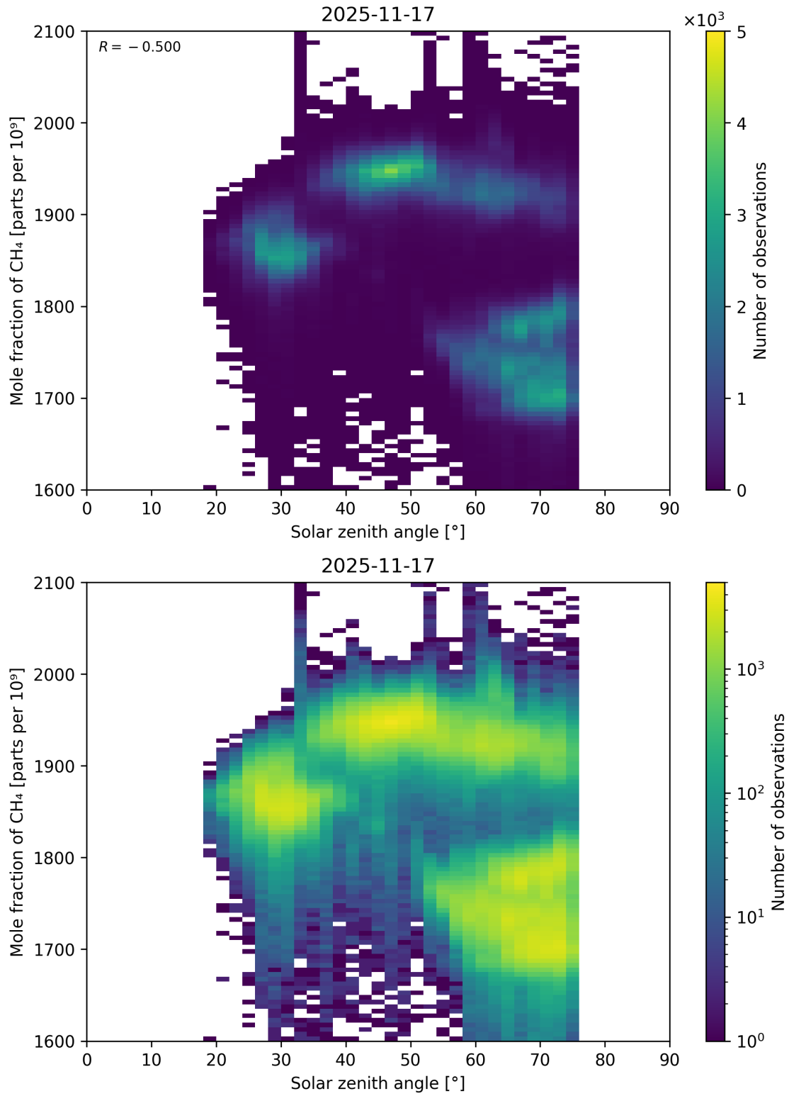
Figure 99: Scatter density plot of “Solar zenith angle” against “Mole fraction of \text{CH}_4 ” for 2025-11-16 to 2025-11-18.
