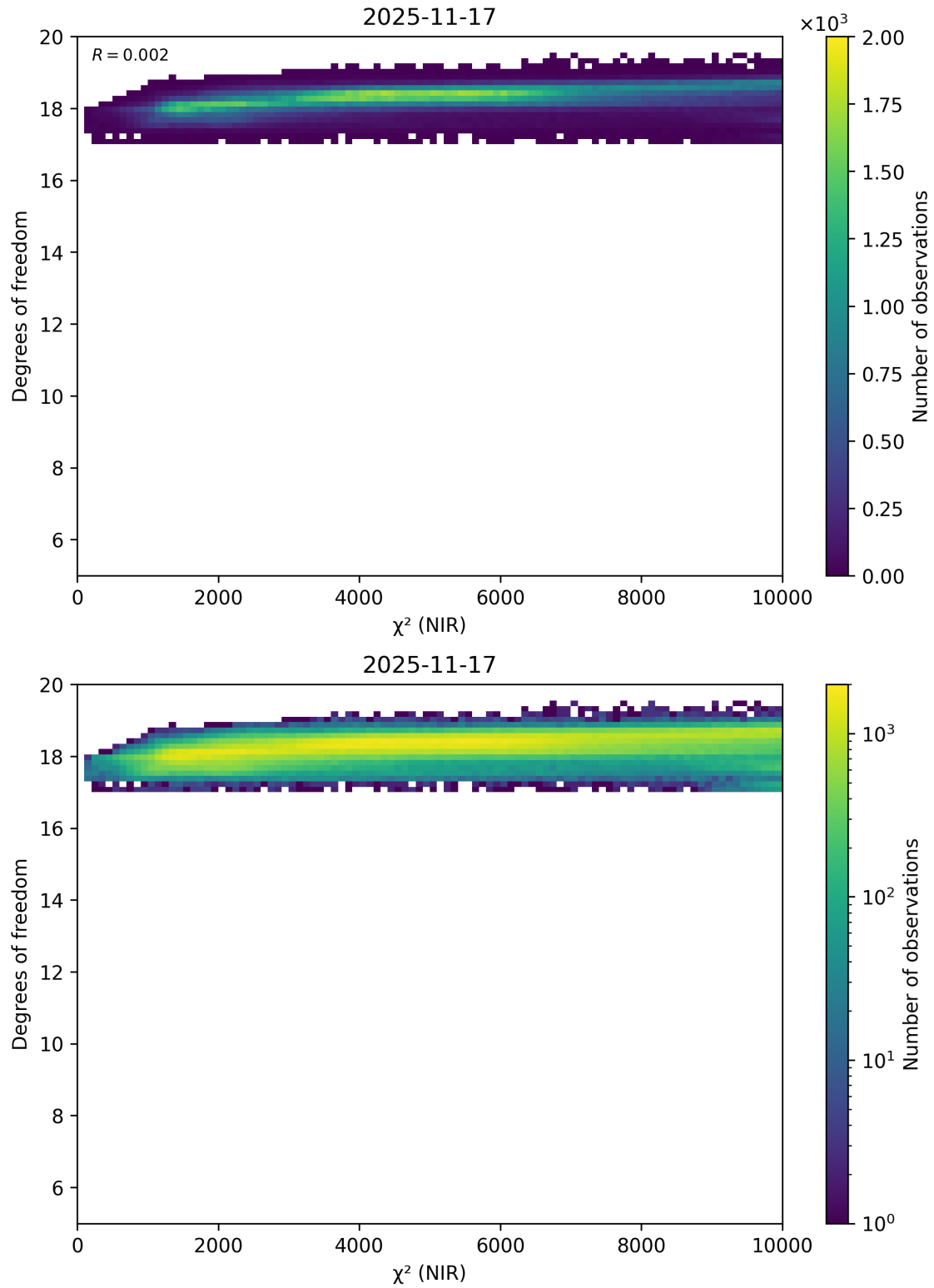
Figure 44: Scatter density plot of “ \chi^2 (NIR)” against “Degrees of freedom” for 2025-11-16 to 2025-11-18.
