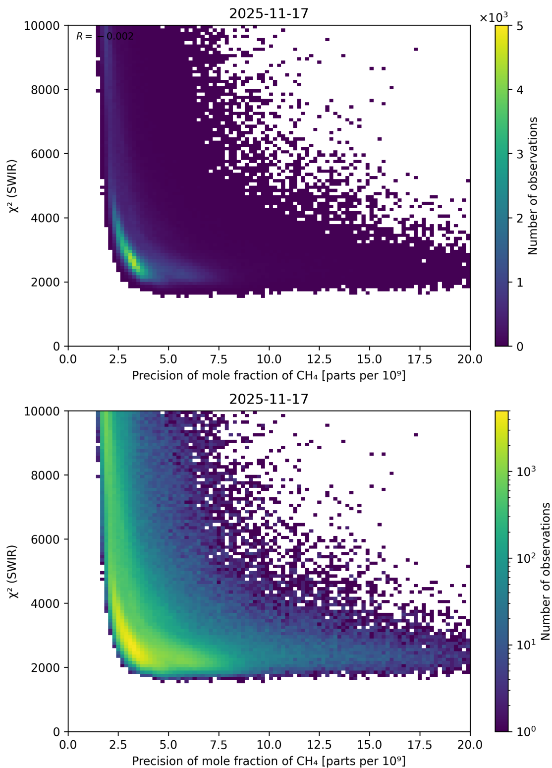
Figure 79: Scatter density plot of “Precision of mole fraction of \text{CH}_4 ” against “ \chi^2 (SWIR)” for 2025-11-16 to 2025-11-18.
