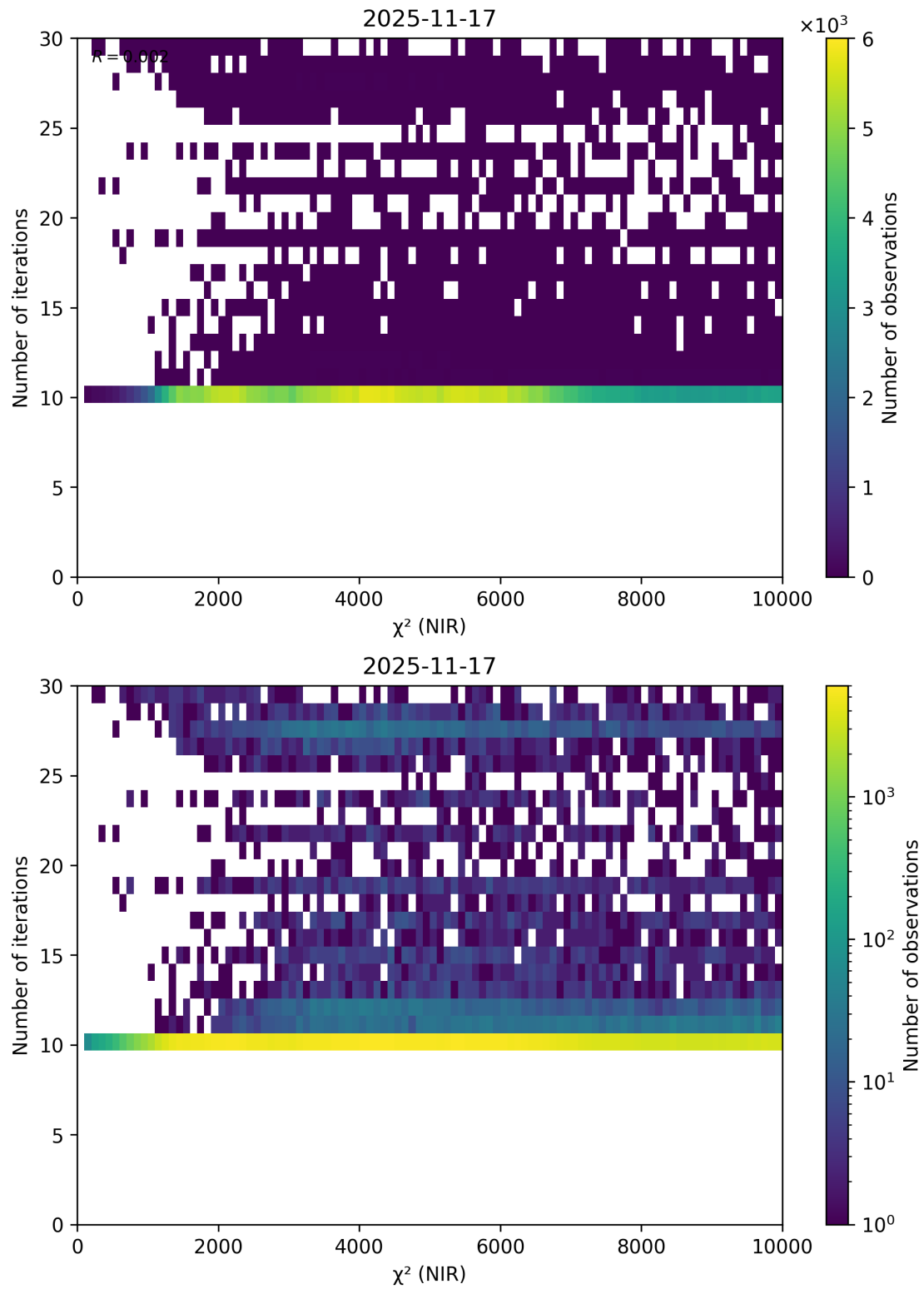
Figure 46: Scatter density plot of “ \chi^2 (NIR)” against “Number of iterations” for 2025-11-16 to 2025-11-18.
