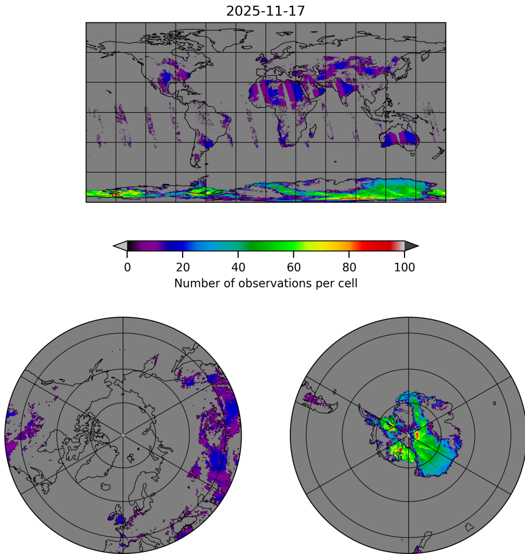
Figure 10: Map of the number of observations for 2025-11-16 to 2025-11-18
