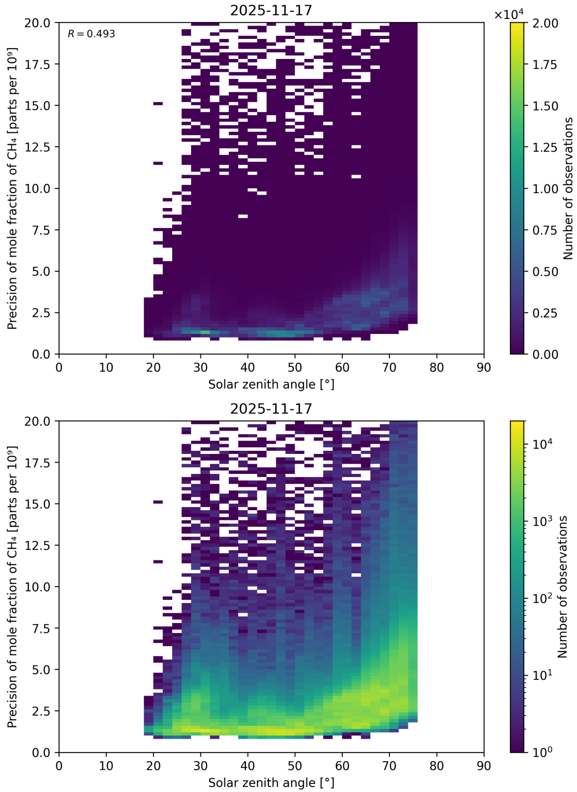
Figure 101: Scatter density plot of “Solar zenith angle” against “Precision of mole fraction of CH 4 ” for 2025-11-16 to 2025-11-18.
