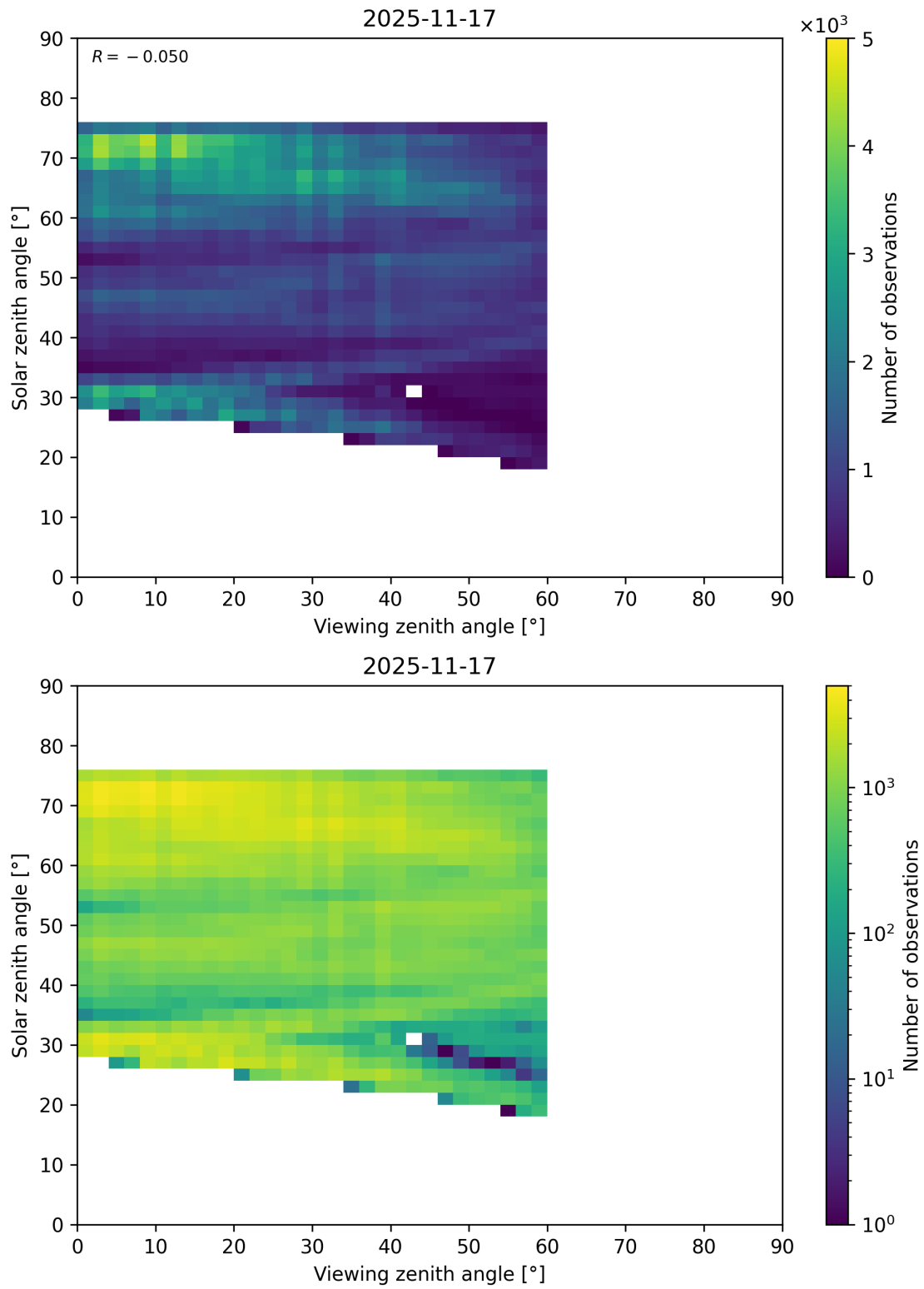
Figure 115: Scatter density plot of “Viewing zenith angle” against “Solar zenith angle” for 2025-11-16 to 2025-11-18.
