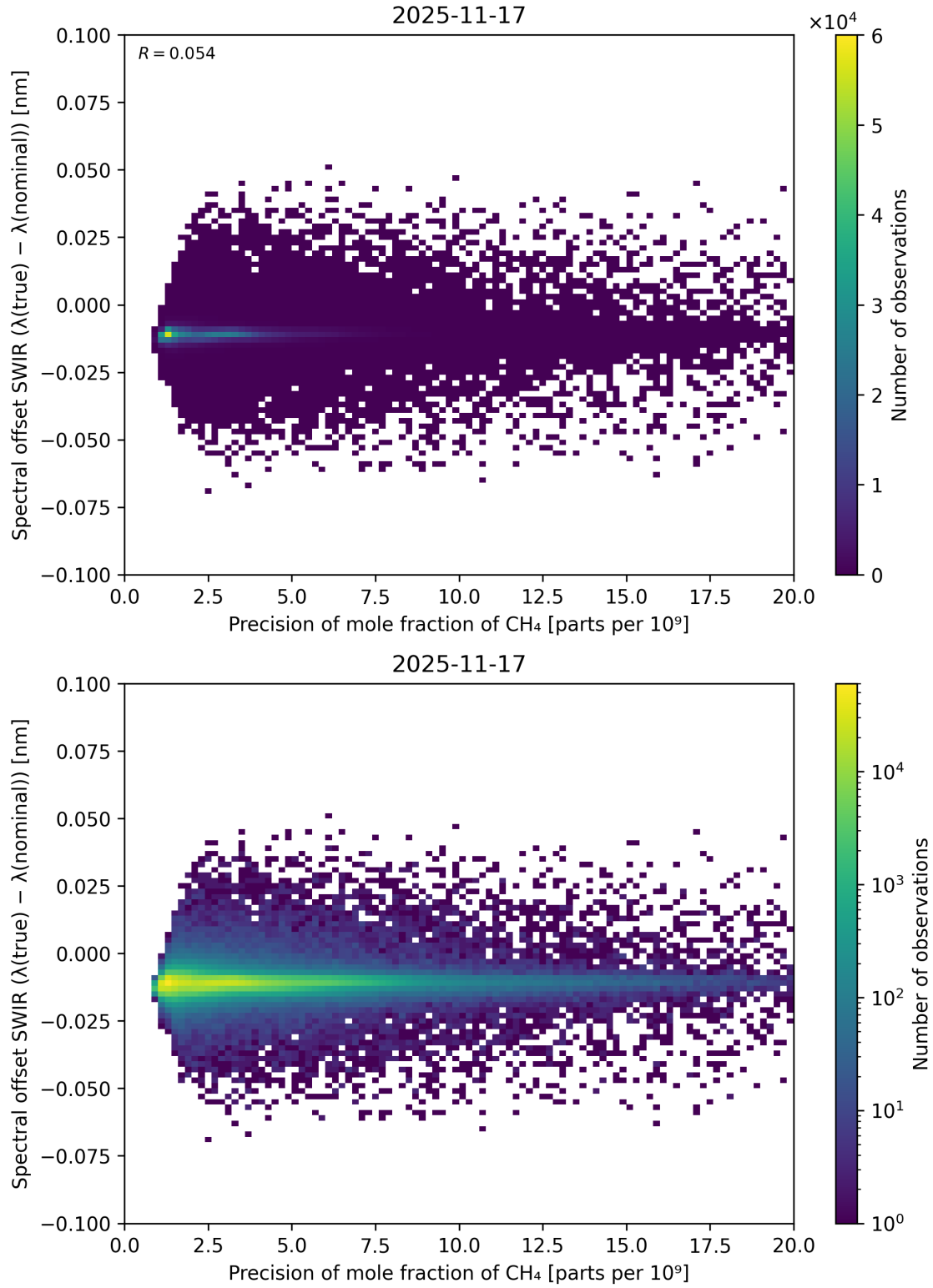
Figure 85: Scatter density plot of “Precision of mole fraction of CH 4 ” against “Spectral offset SWIR ( \lambda_{\text{true}} - \lambda_{\text{nominal}} )” for 2025-11-16 to 2025-11-18.
