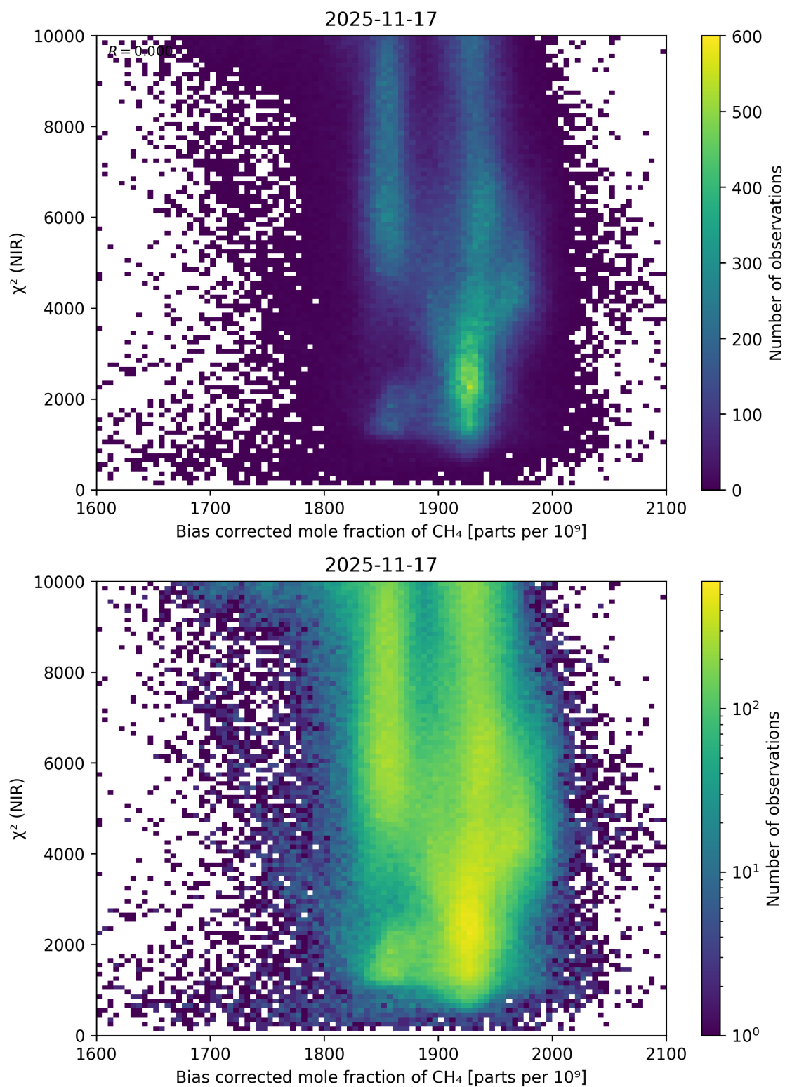
Figure 63: Scatter density plot of “Bias corrected mole fraction of \text{CH}_4 ” against “ \chi^2 (NIR)” for 2025-11-16 to 2025-11-18.
