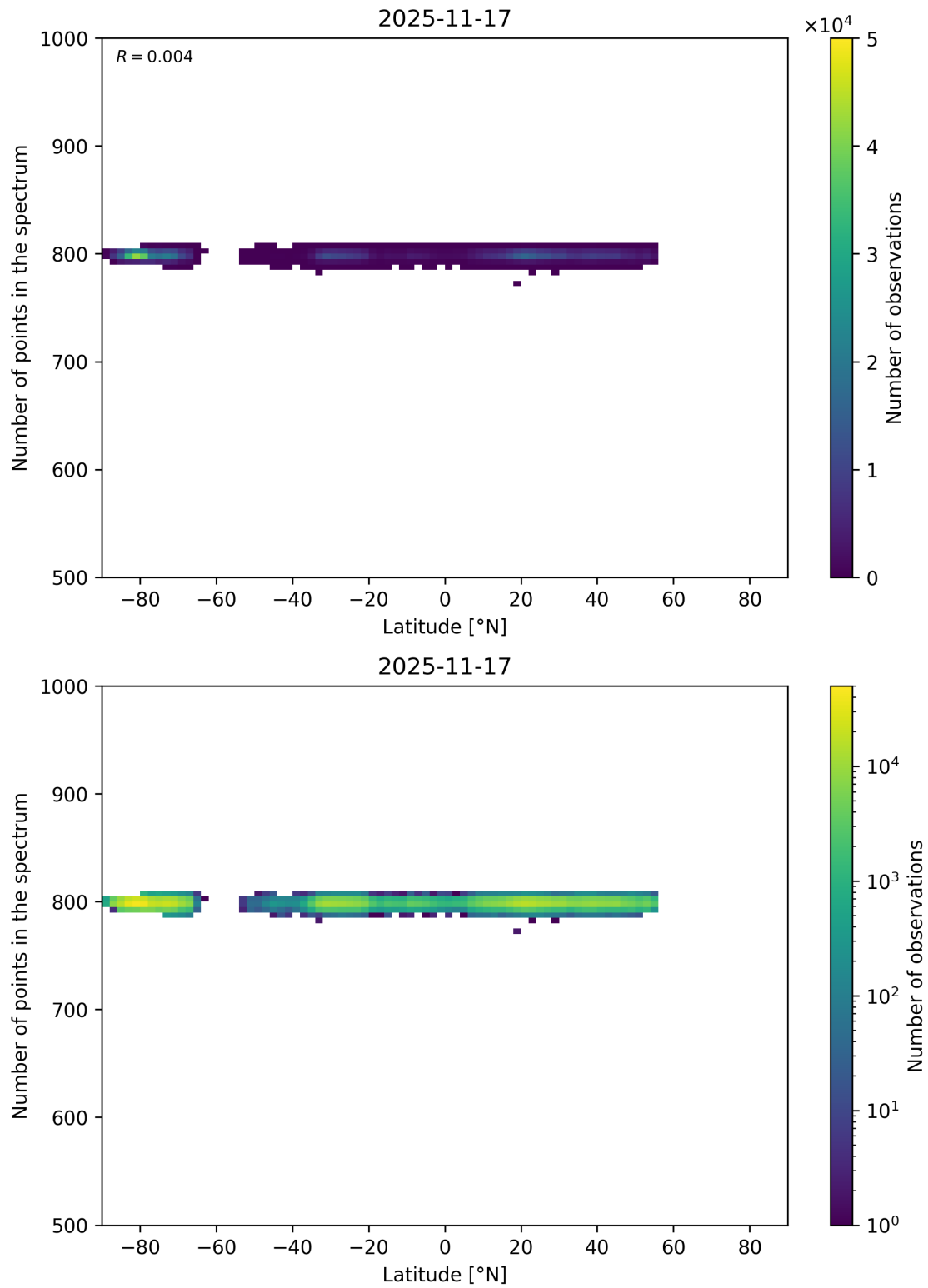
Figure 61: Scatter density plot of “Latitude” against “Number of points in the spectrum” for 2025-11-16 to 2025-11-18.
