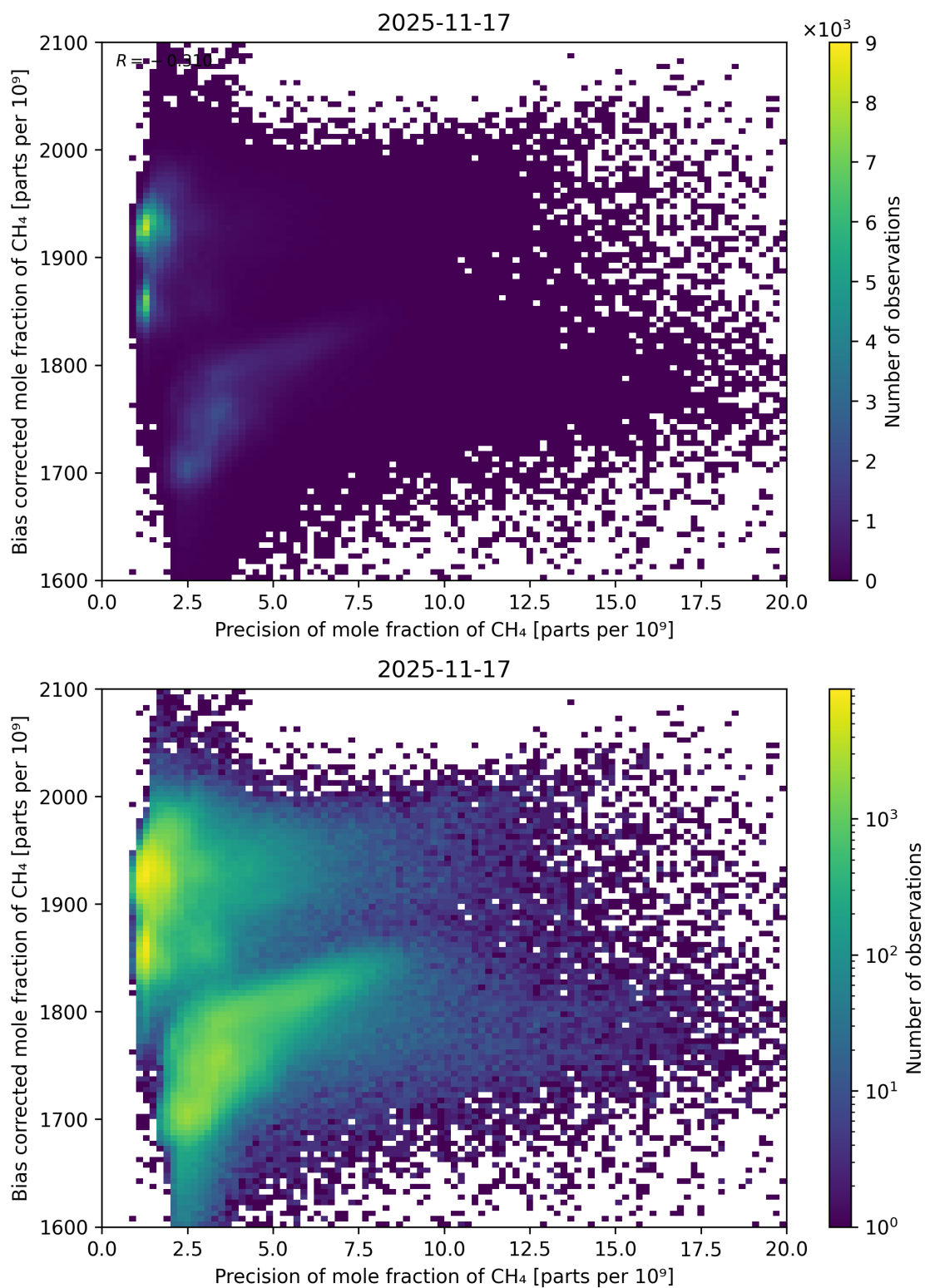
Figure 82: Scatter density plot of “Precision of mole fraction of CH 4 ” against “Bias corrected mole fraction of CH 4 ” for 2025-11-16 to 2025-11-18.
