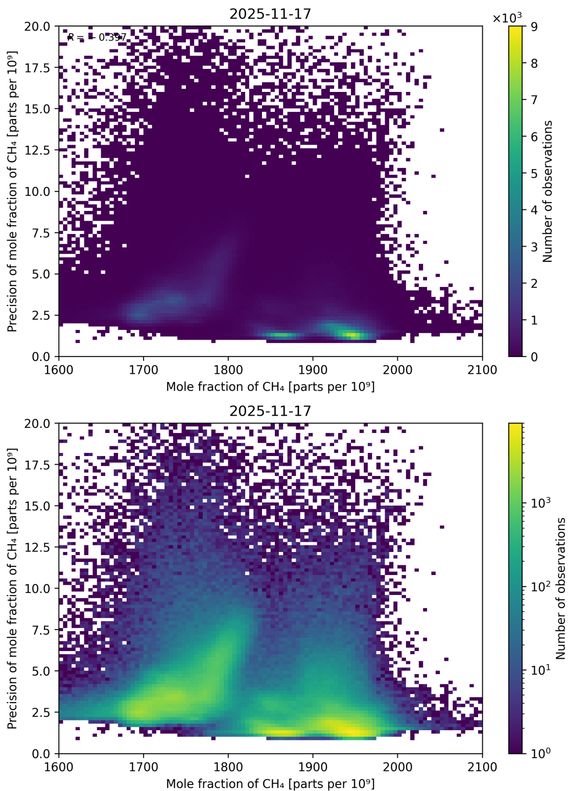
Figure 75: Scatter density plot of “Mole fraction of CH 4 ” against “Precision of mole fraction of CH 4 ” for 2025-11-16 to 2025-11-18.
