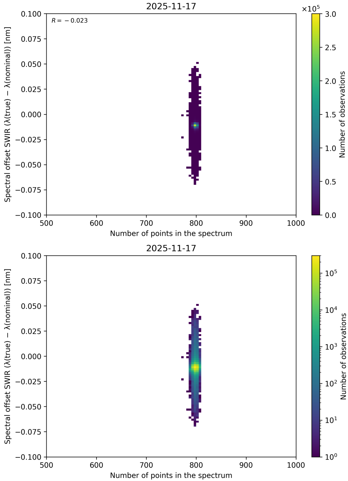
Figure 93: Scatter density plot of “Number of points in the spectrum” against “Spectral offset SWIR ( \lambda_{\text{true}} - \lambda_{\text{nominal}} )” for 2025-11-16 to 2025-11-18.
