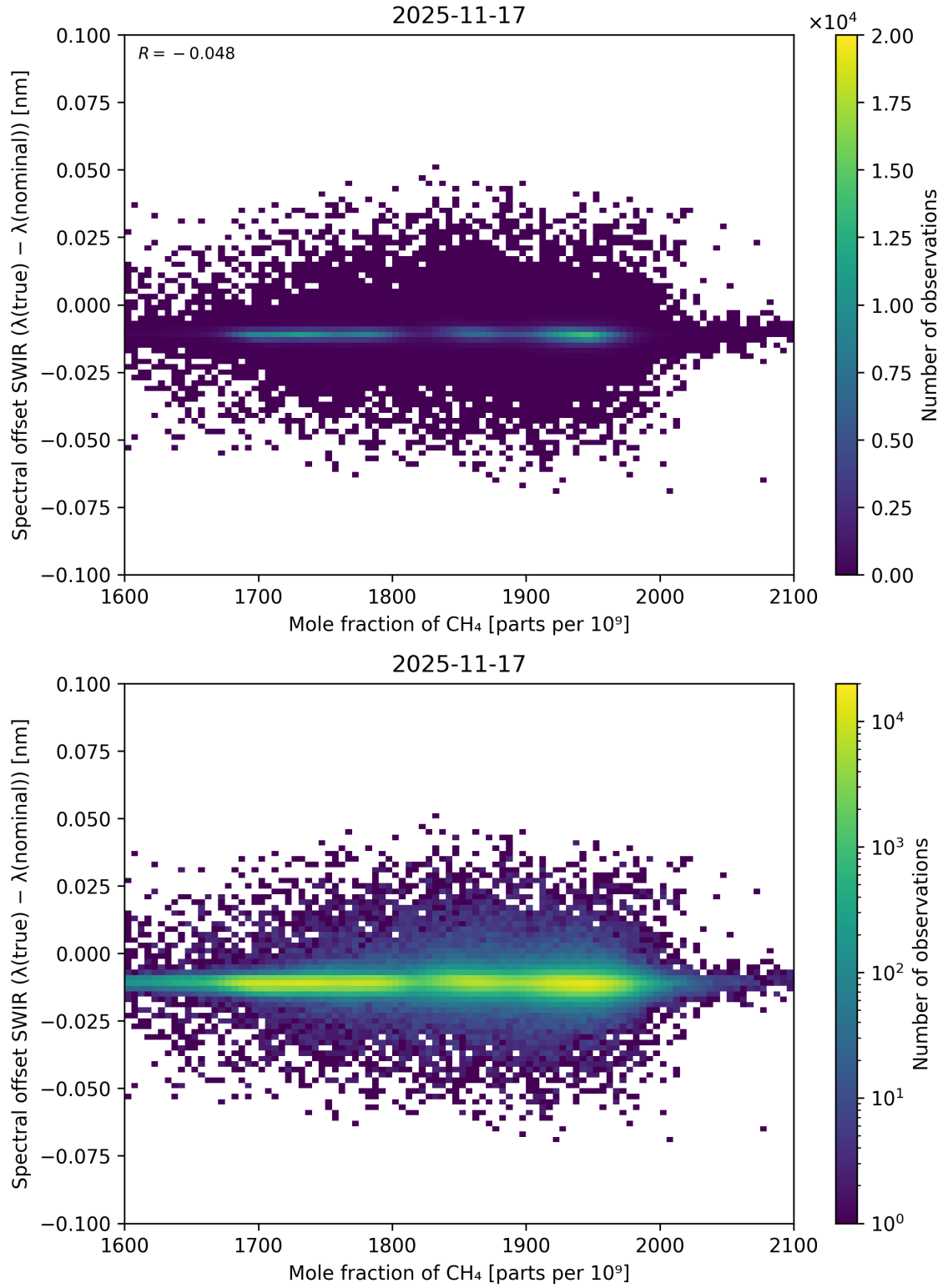
Figure 86: Scatter density plot of “Mole fraction of CH 4 ” against “Spectral offset SWIR ( \lambda_{\text{true}} - \lambda_{\text{nominal}} )” for 2025-11-16 to 2025-11-18.
