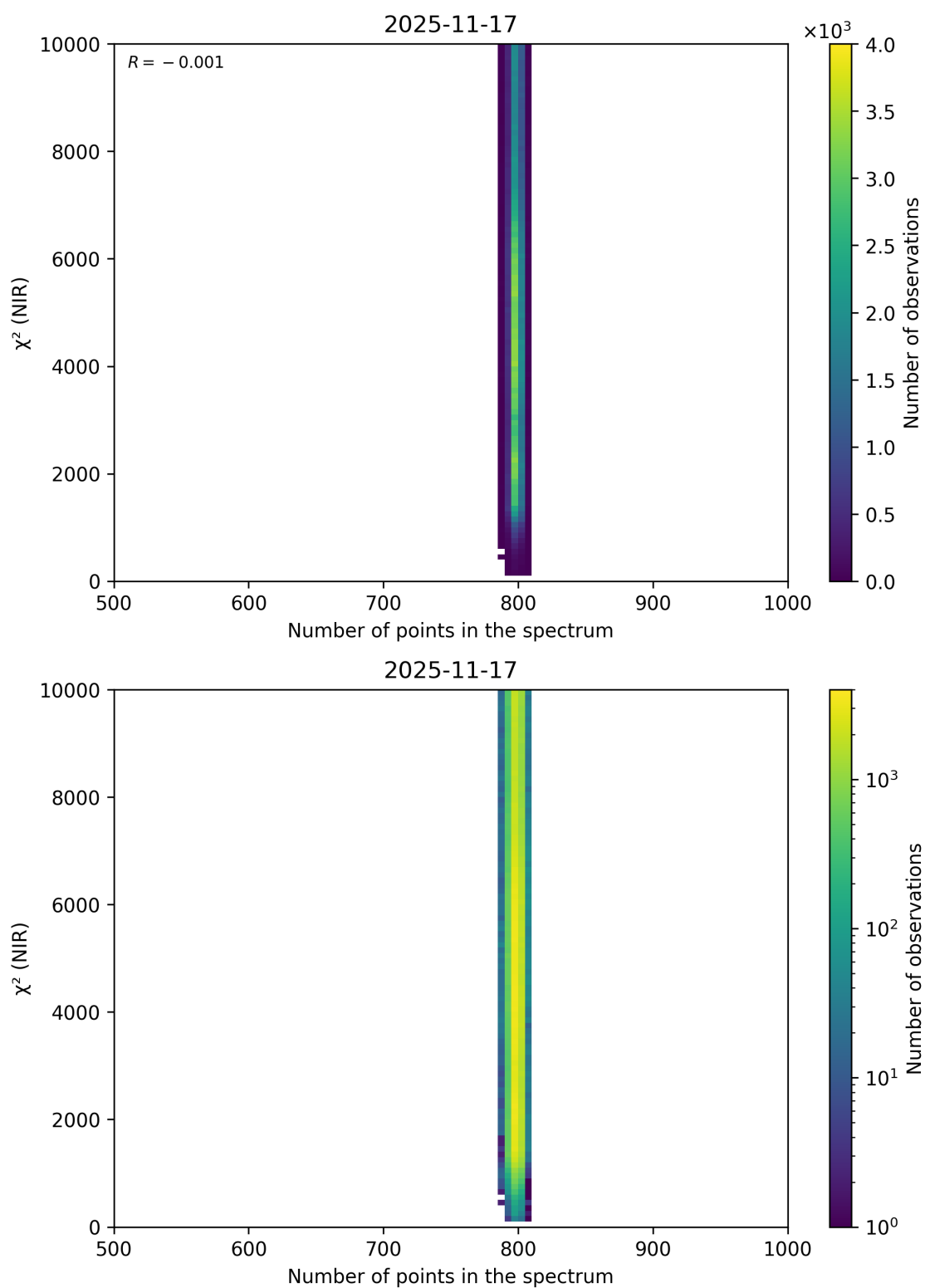
Figure 88: Scatter density plot of “Number of points in the spectrum” against “ \chi^2 (NIR)” for 2025-11-16 to 2025-11-18.
