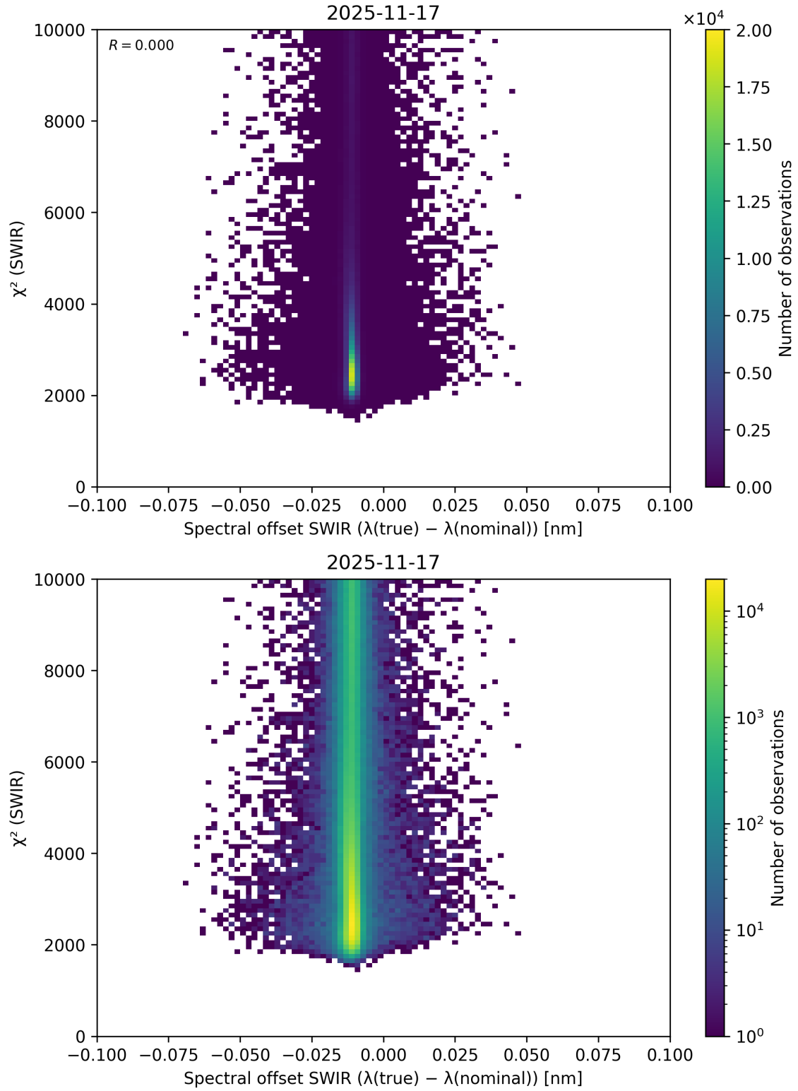
Figure 118: Scatter density plot of “Spectral offset SWIR ( \lambda_{\text{true}} - \lambda_{\text{nominal}} )” against “ \chi^2 (SWIR)” for 2025-11-16 to 2025-11-18.
