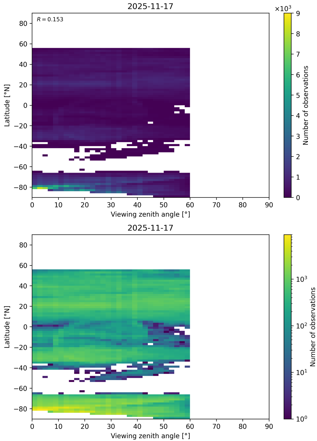
Figure 109: Scatter density plot of “Viewing zenith angle” against “Latitude” for 2025-11-16 to 2025-11-18.
