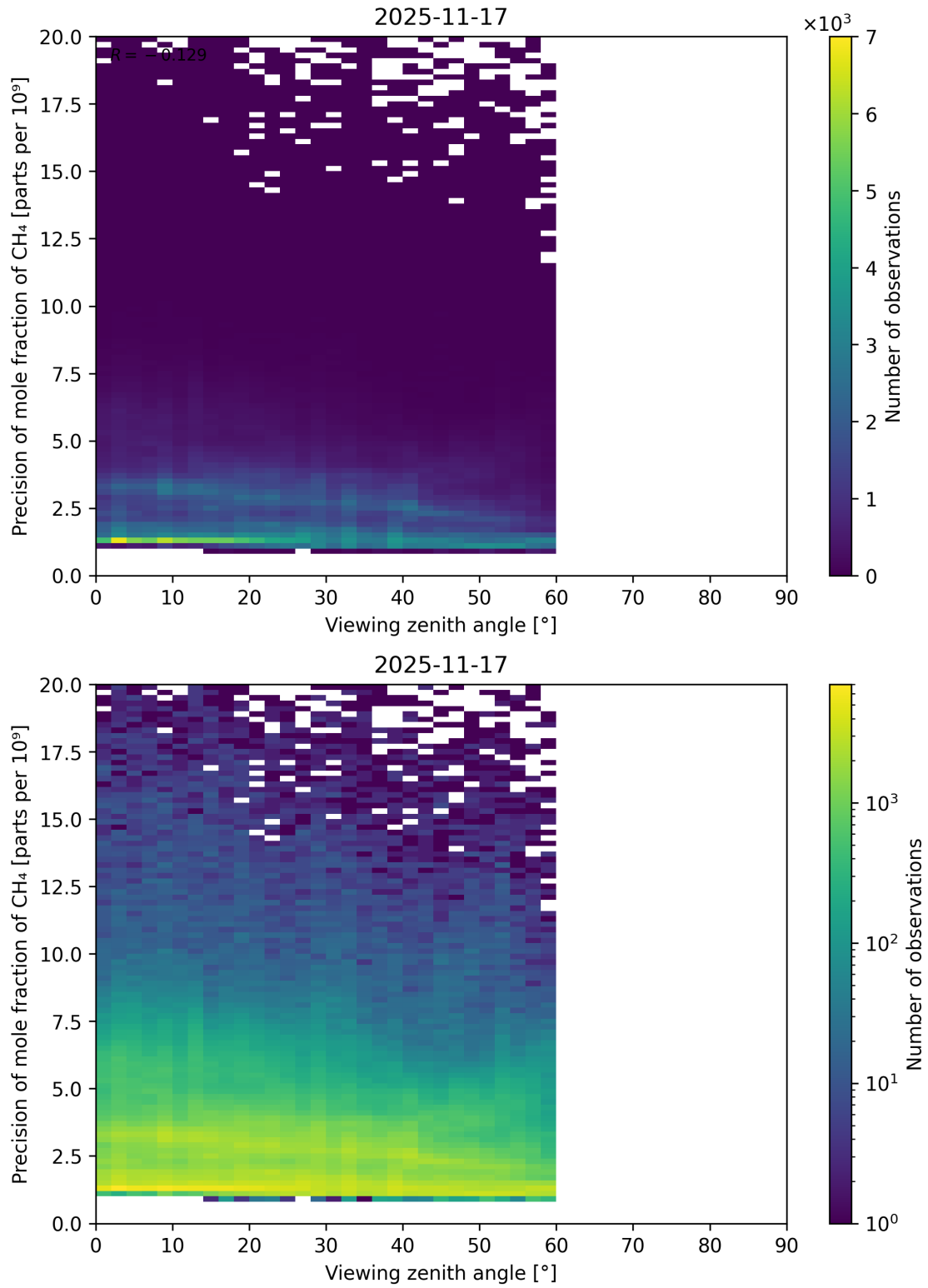
Figure 112: Scatter density plot of “Viewing zenith angle” against “Precision of mole fraction of CH 4 ” for 2025-11-16 to 2025-11-18.
