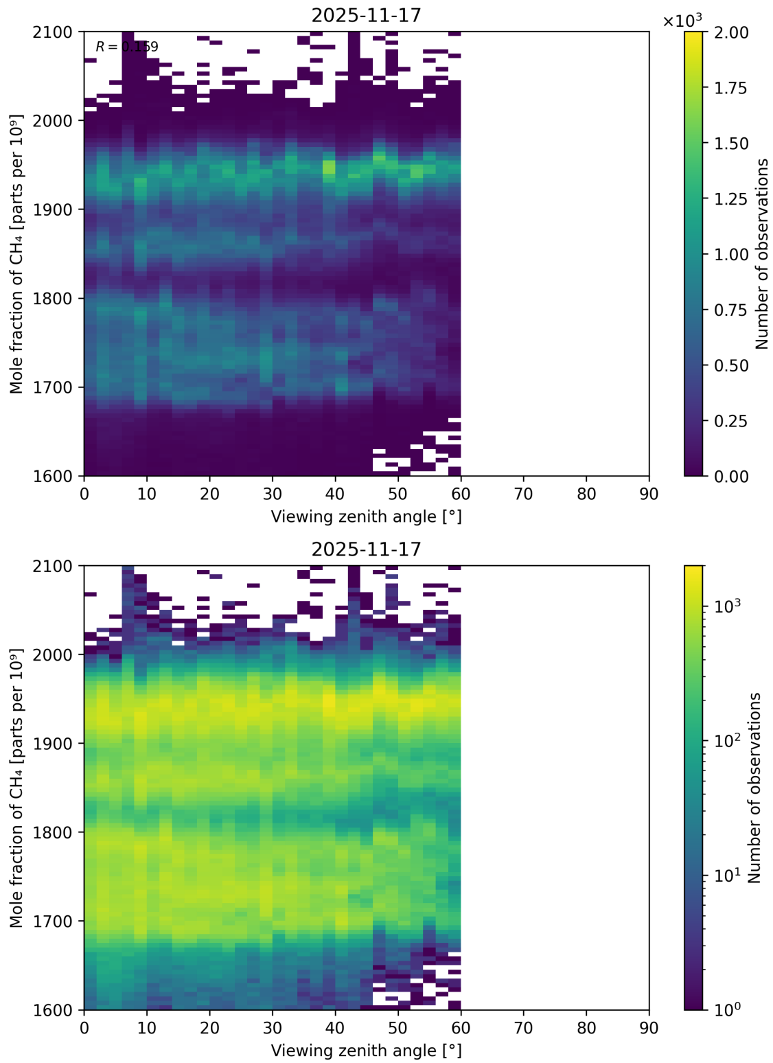
Figure 110: Scatter density plot of “Viewing zenith angle” against “Mole fraction of CH 4 ” for 2025-11-16 to 2025-11-18.
