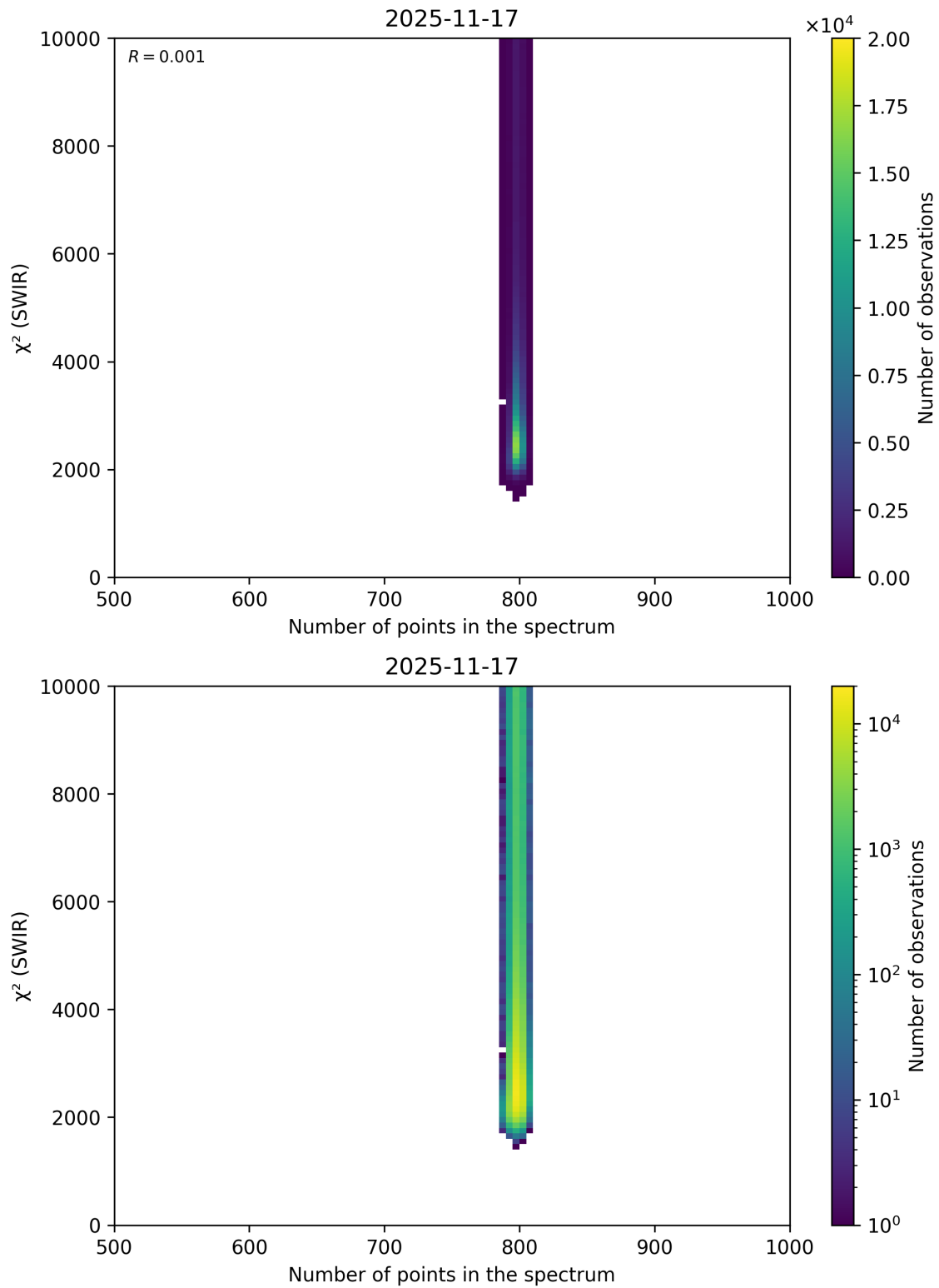
Figure 89: Scatter density plot of “Number of points in the spectrum” against “ \chi^2 (SWIR)” for 2025-11-16 to 2025-11-18.
