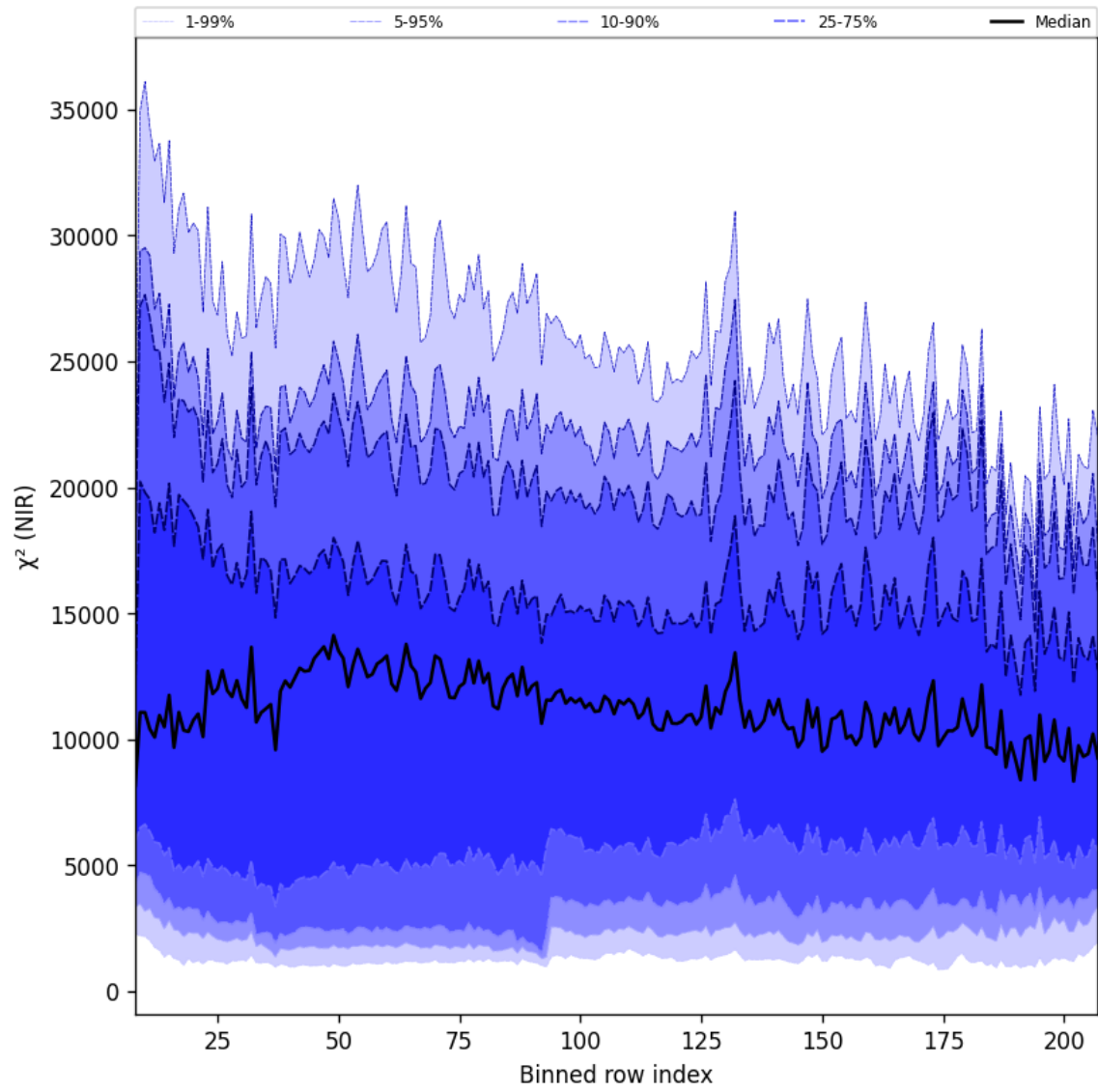
Figure 40: Along track statistics of “ \chi^2 (NIR)” for 2025-11-16 to 2025-11-18
