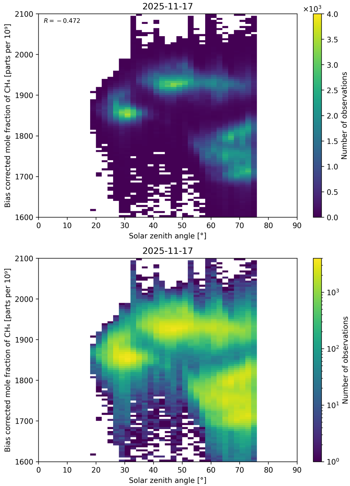
Figure 100: Scatter density plot of “Solar zenith angle” against “Bias corrected mole fraction of CH 4 ” for 2025-11-16 to 2025-11-18.
