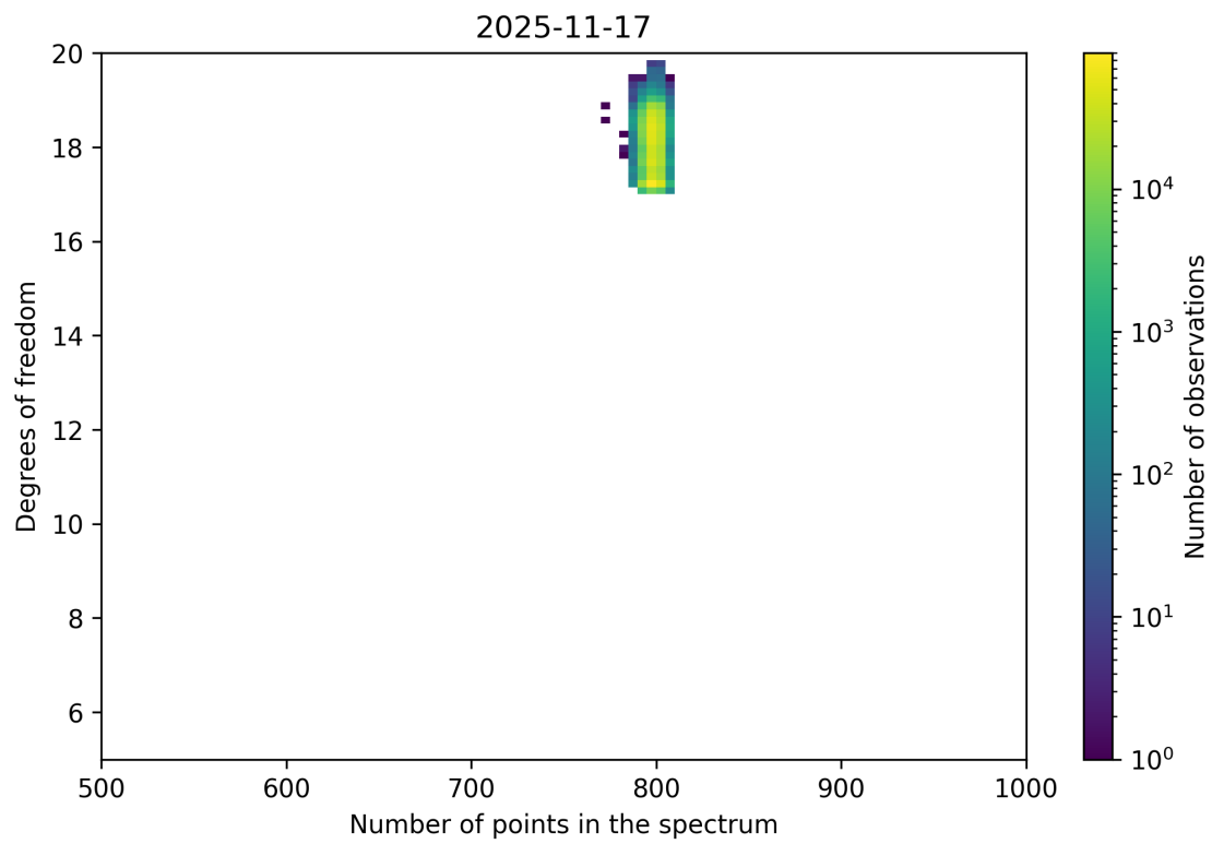
Figure 90: Scatter density plot of “Number of points in the spectrum” against “Degrees of freedom” for 2025-11-16 to 2025-11-18.
