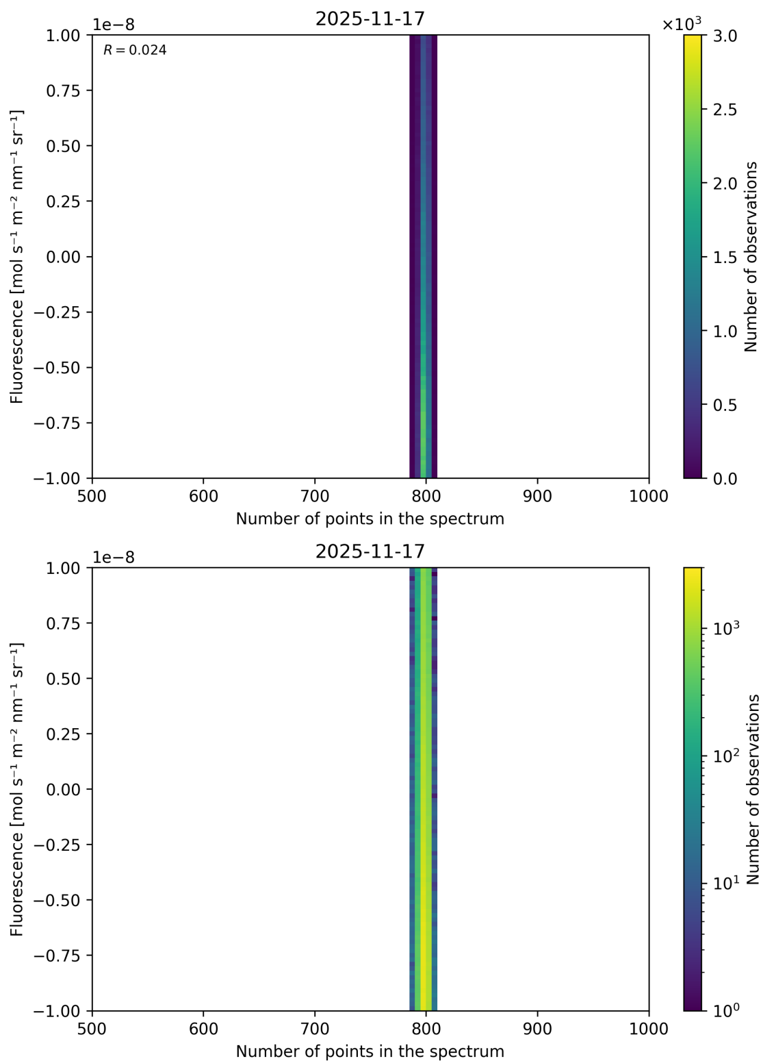
Figure 91: Scatter density plot of “Number of points in the spectrum” against “Fluorescence” for 2025-11-16 to 2025-11-18.
