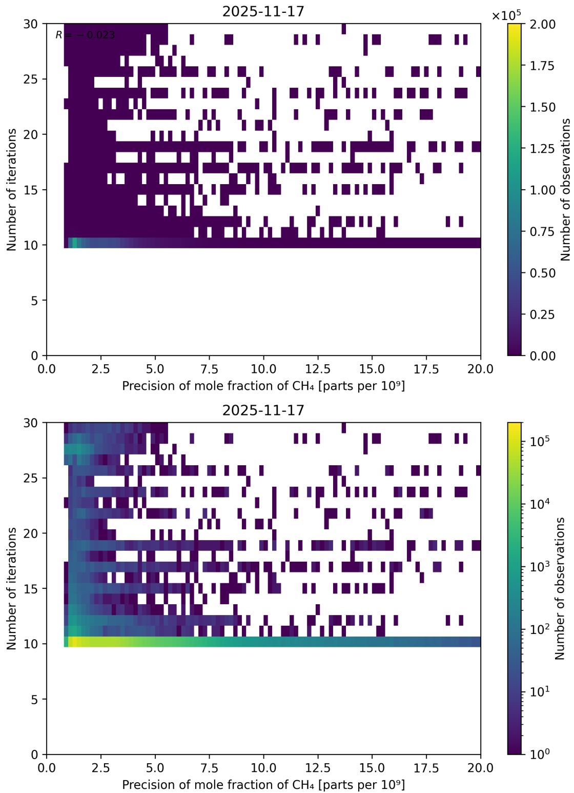
Figure 83: Scatter density plot of “Precision of mole fraction of CH 4 ” against “Number of iterations” for 2025-11-16 to 2025-11-18.
