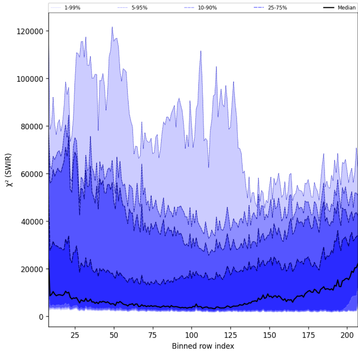
Figure 39: Along track statistics of “ \chi^2 (SWIR)” for 2025-11-16 to 2025-11-18
