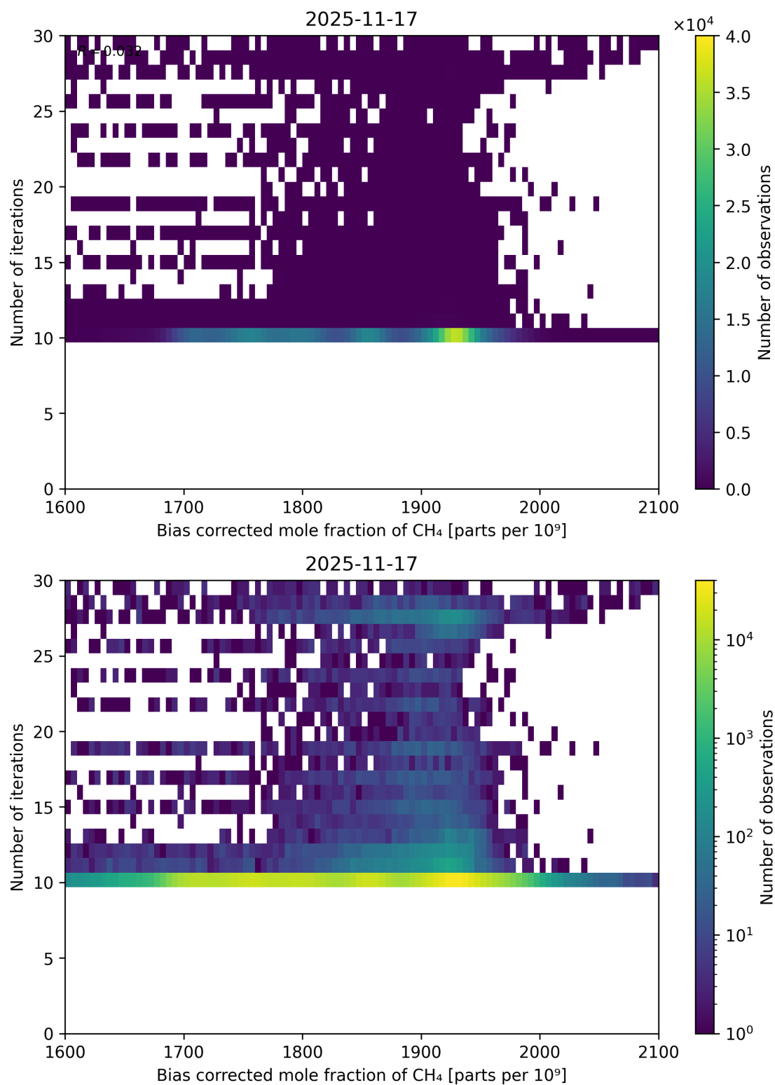
Figure 67: Scatter density plot of “Bias corrected mole fraction of \text{CH}_4 ” against “Number of iterations” for 2025-11-16 to 2025-11-18.
