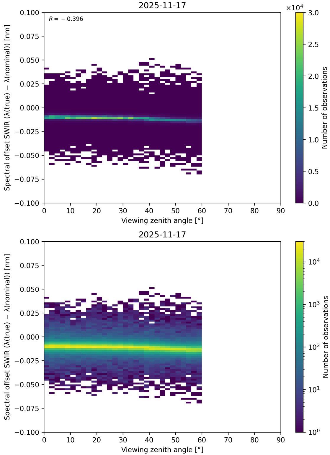
Figure 116: Scatter density plot of “Viewing zenith angle” against “Spectral offset SWIR ( \lambda_{\text{true}} - \lambda_{\text{nominal}} )” for 2025-11-16 to 2025-11-18.
