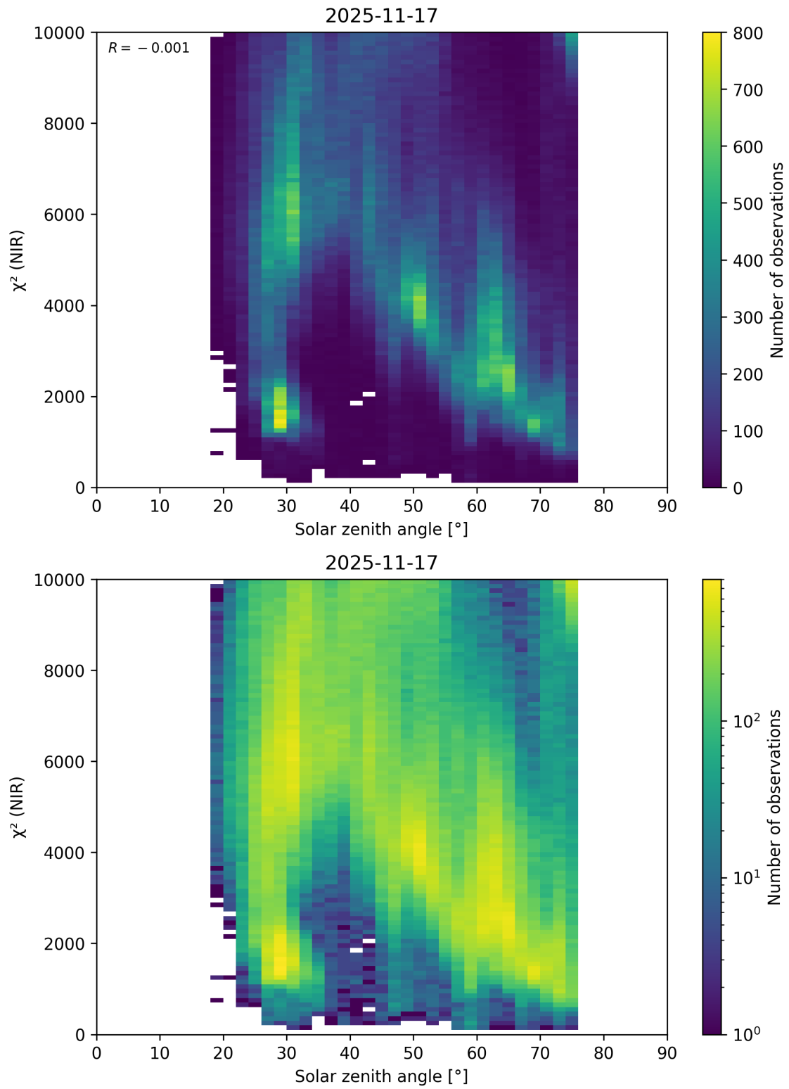
Figure 94: Scatter density plot of “Solar zenith angle” against “ \chi^2 (NIR)” for 2025-11-16 to 2025-11-18.
