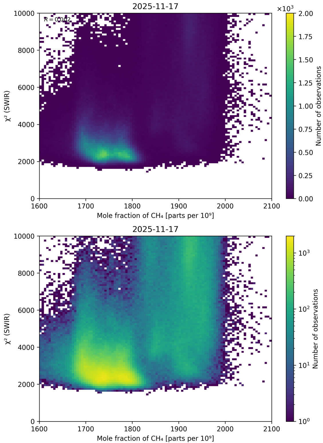
Figure 71: Scatter density plot of “Mole fraction of \text{CH}_4 ” against “ \chi^2 (SWIR)” for 2025-11-16 to 2025-11-18.
