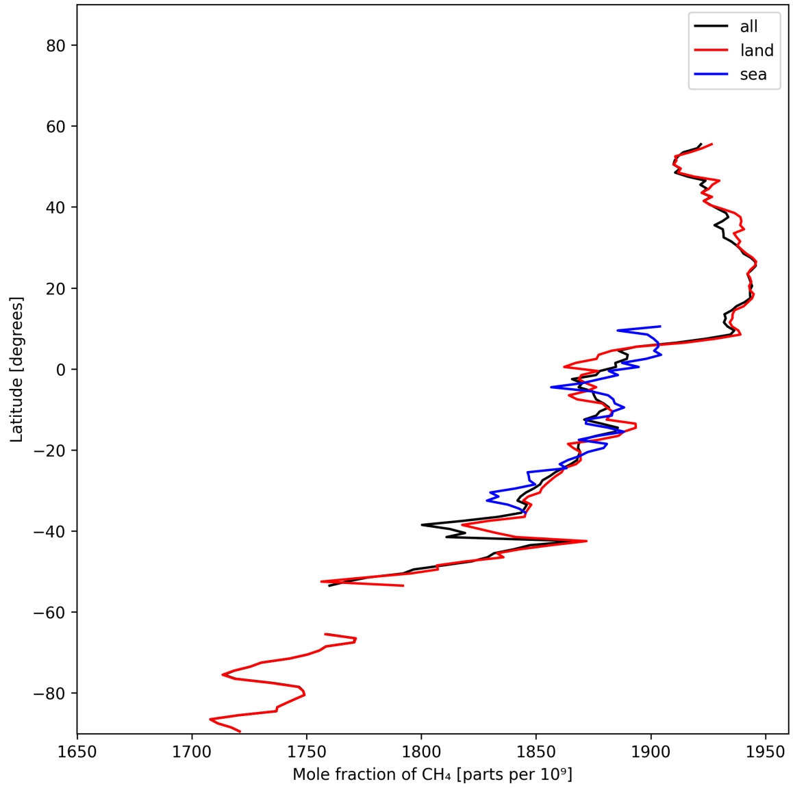
Figure 12: Zonal average of “Mole fraction of CH 4 ” for 2025-11-16 to 2025-11-18.
