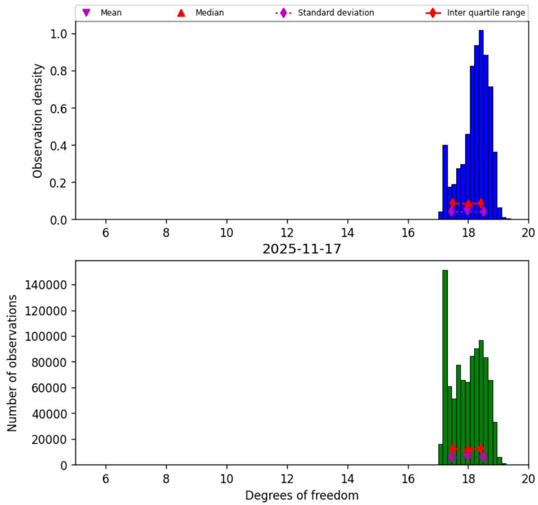
Figure 30: Histogram of “Degrees of freedom” for 2025-11-16 to 2025-11-18
