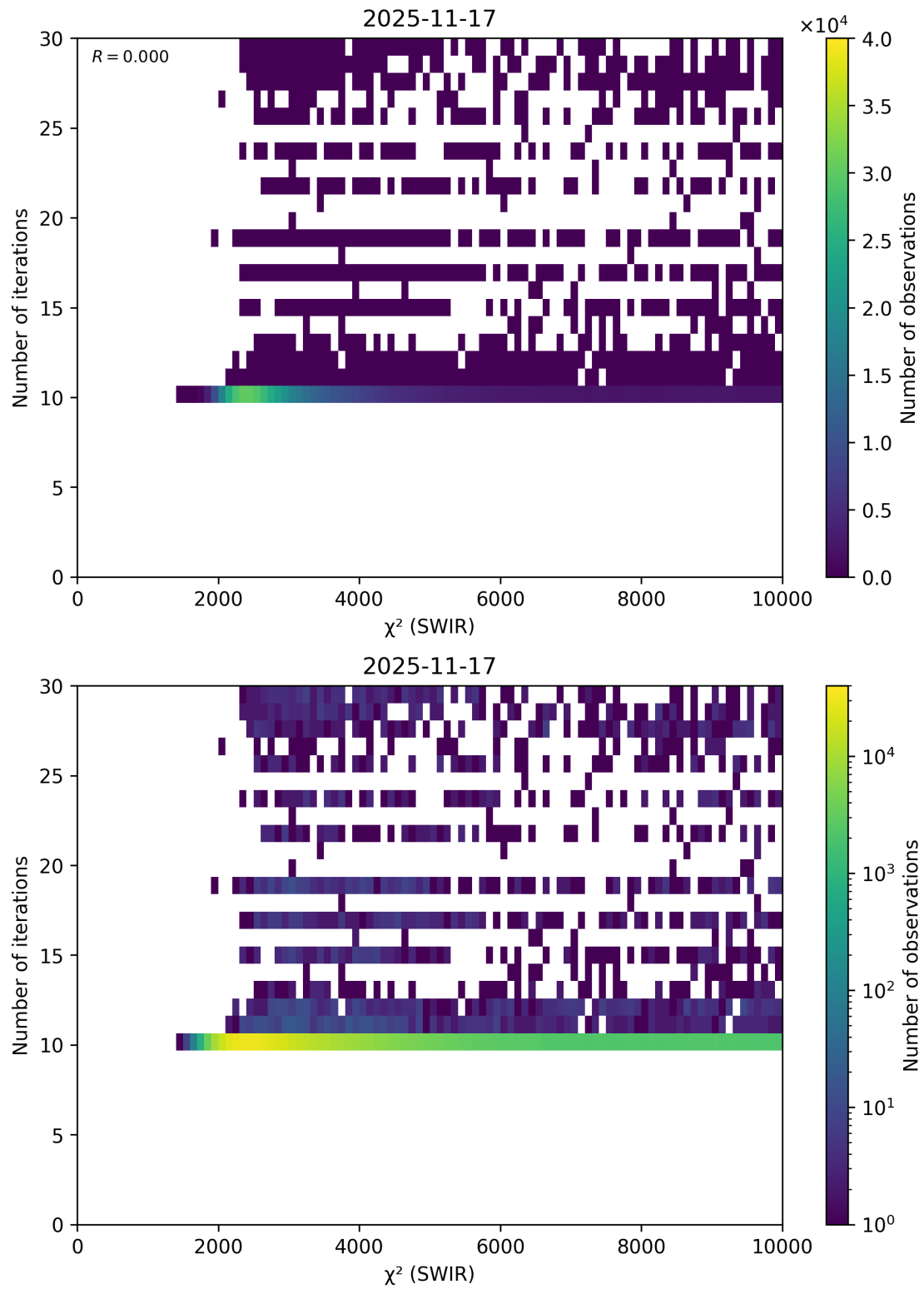
Figure 50: Scatter density plot of “ \chi^2 (SWIR)” against “Number of iterations” for 2025-11-16 to 2025-11-18.
