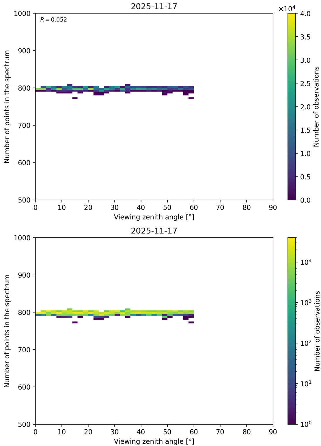
Figure 114: Scatter density plot of “Viewing zenith angle” against “Number of points in the spectrum” for 2025-11-16 to 2025-11-18.
