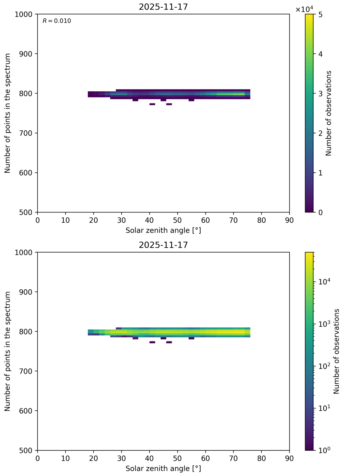
Figure 103: Scatter density plot of “Solar zenith angle” against “Number of points in the spectrum” for 2025-11-16 to 2025-11-18.
