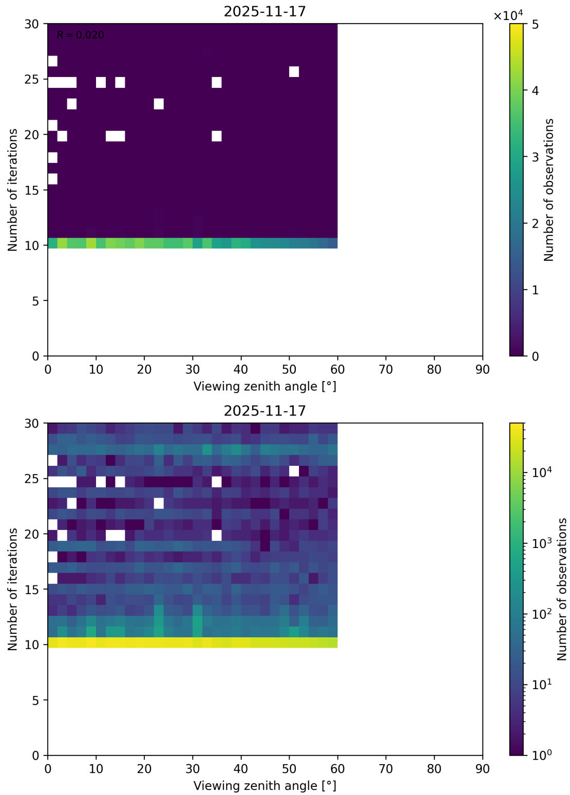
Figure 113: Scatter density plot of “Viewing zenith angle” against “Number of iterations” for 2025-11-16 to 2025-11-18.
