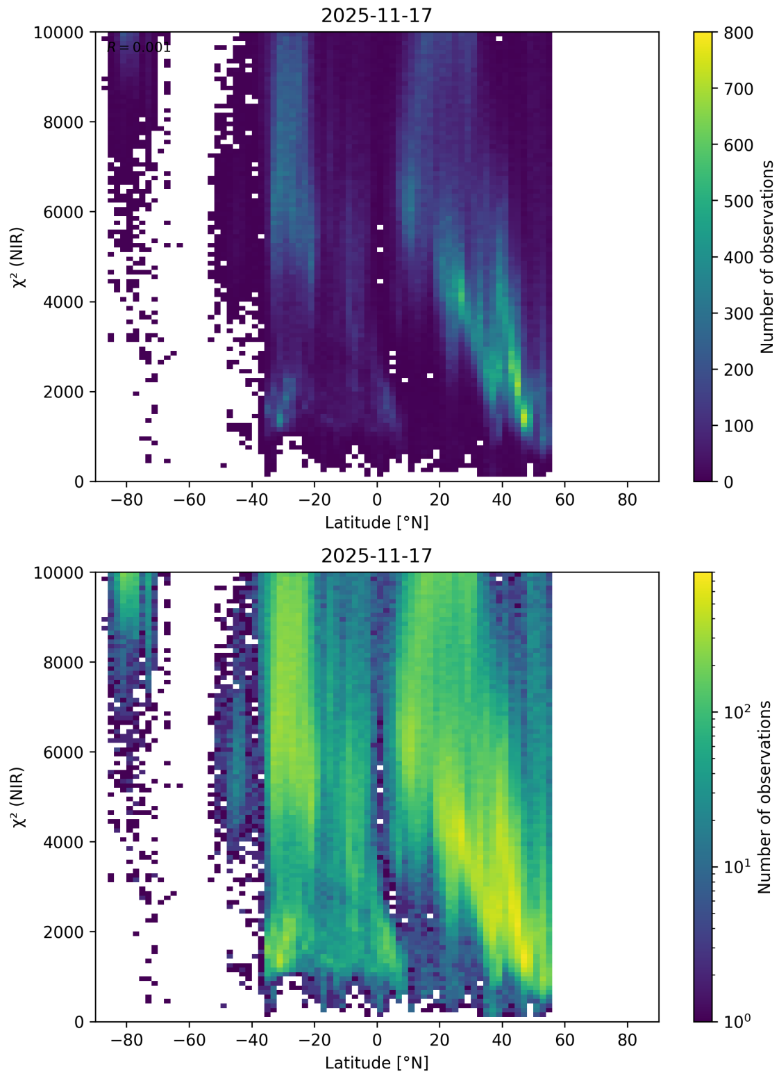
Figure 53: Scatter density plot of “Latitude” against “ \chi^2 (NIR)” for 2025-11-16 to 2025-11-18.
