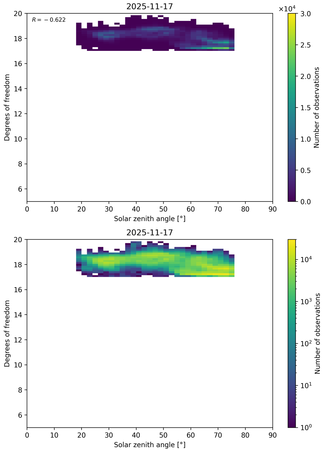
Figure 96: Scatter density plot of “Solar zenith angle” against “Degrees of freedom” for 2025-11-16 to 2025-11-18.
