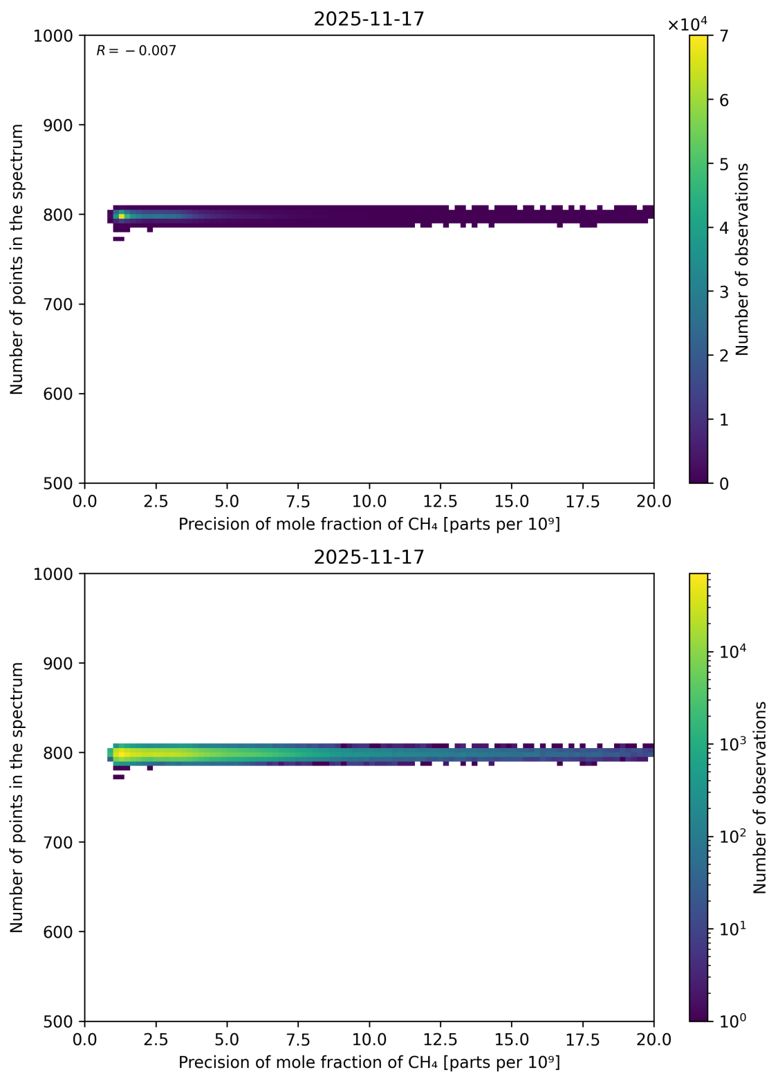
Figure 84: Scatter density plot of “Precision of mole fraction of CH 4 ” against “Number of points in the spectrum” for 2025-11-16 to 2025-11-18.
