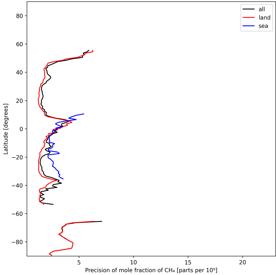
Figure 13: Zonal average of “Precision of mole fraction of CH 4 ” for 2025-11-16 to 2025-11-18.
