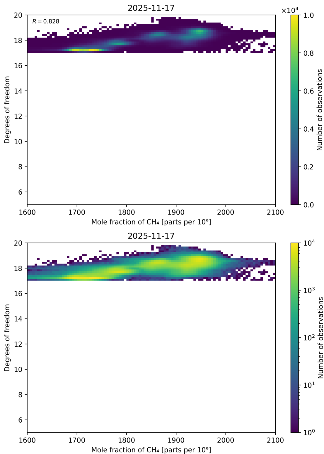
Figure 72: Scatter density plot of “Mole fraction of CH 4 ” against “Degrees of freedom” for 2025-11-16 to 2025-11-18.
