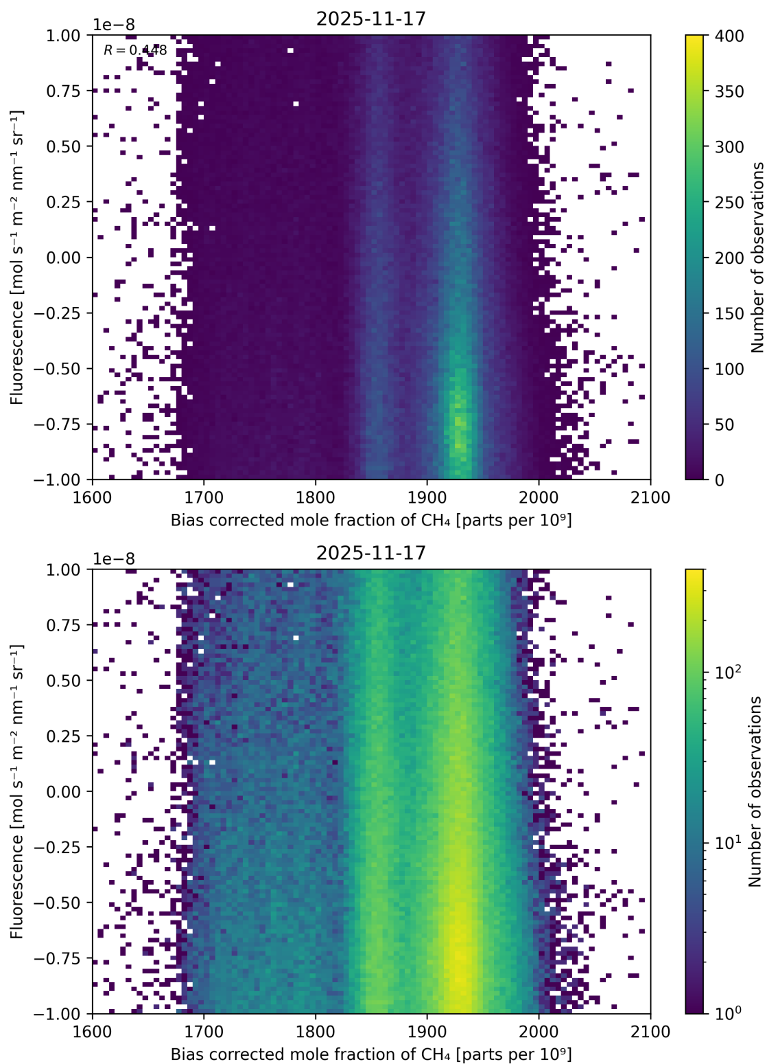
Figure 66: Scatter density plot of “Bias corrected mole fraction of \text{CH}_4 ” against “Fluorescence” for 2025-11-16 to 2025-11-18.
