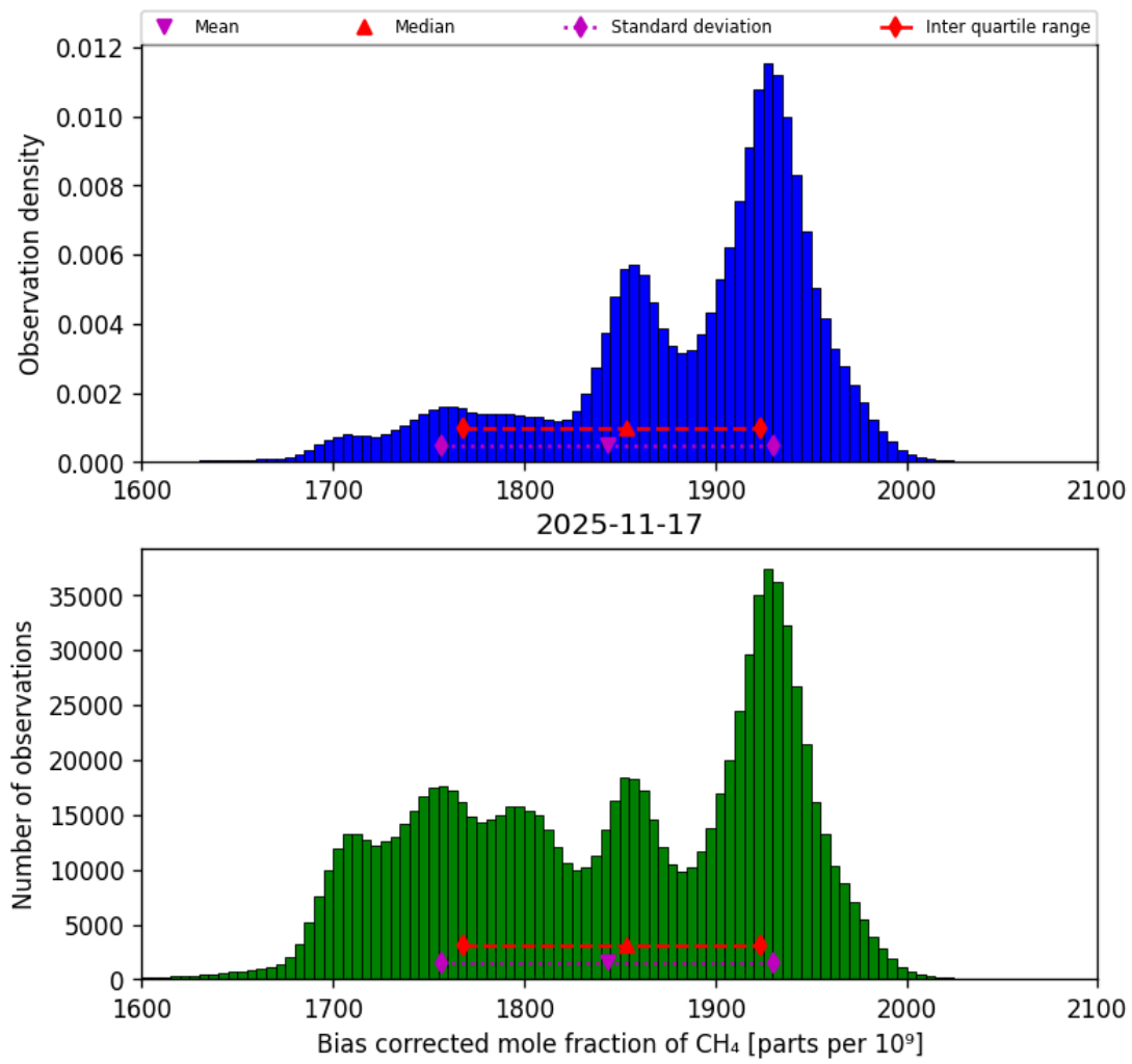
Figure 25: Histogram of “Bias corrected mole fraction of CH 4 ” for 2025-11-16 to 2025-11-18
