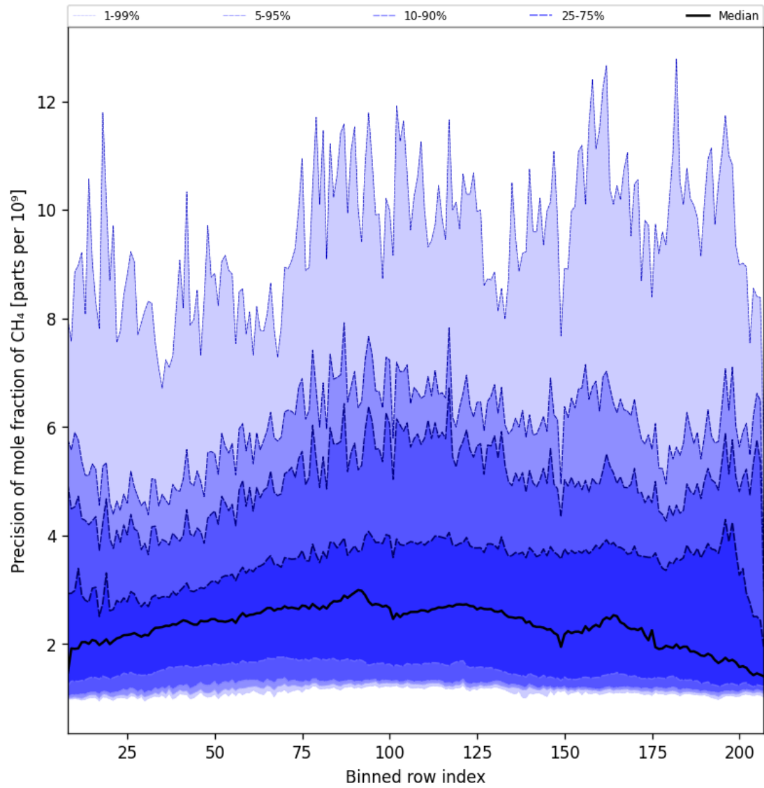
Figure 35: Along track statistics of “Precision of mole fraction of CH 4 ” for 2025-11-16 to 2025-11-18
