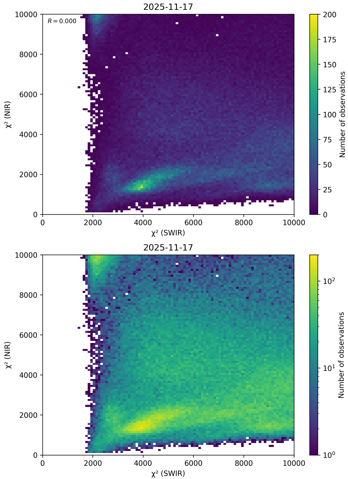
Figure 47: Scatter density plot of “ \chi^2 (SWIR)” against “ \chi^2 (NIR)” for 2025-11-16 to 2025-11-18.
