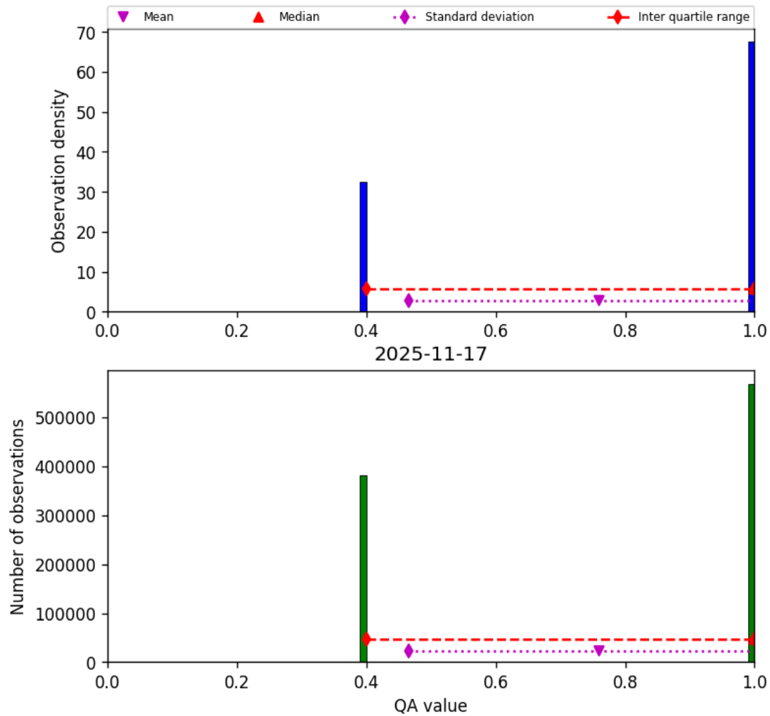
Figure 22: Histogram of “QA value” for 2025-11-16 to 2025-11-18
