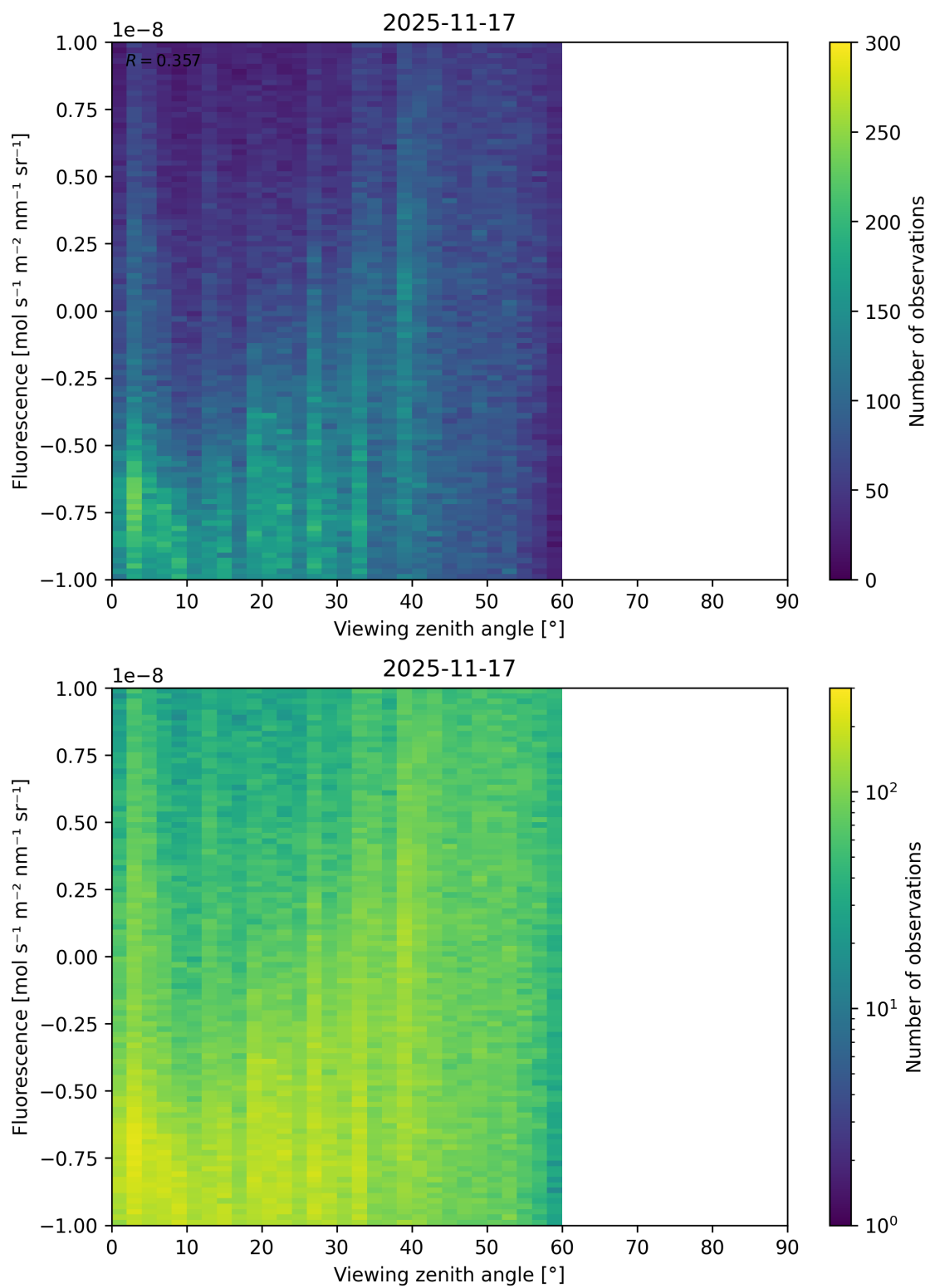
Figure 108: Scatter density plot of “Viewing zenith angle” against “Fluorescence” for 2025-11-16 to 2025-11-18.
