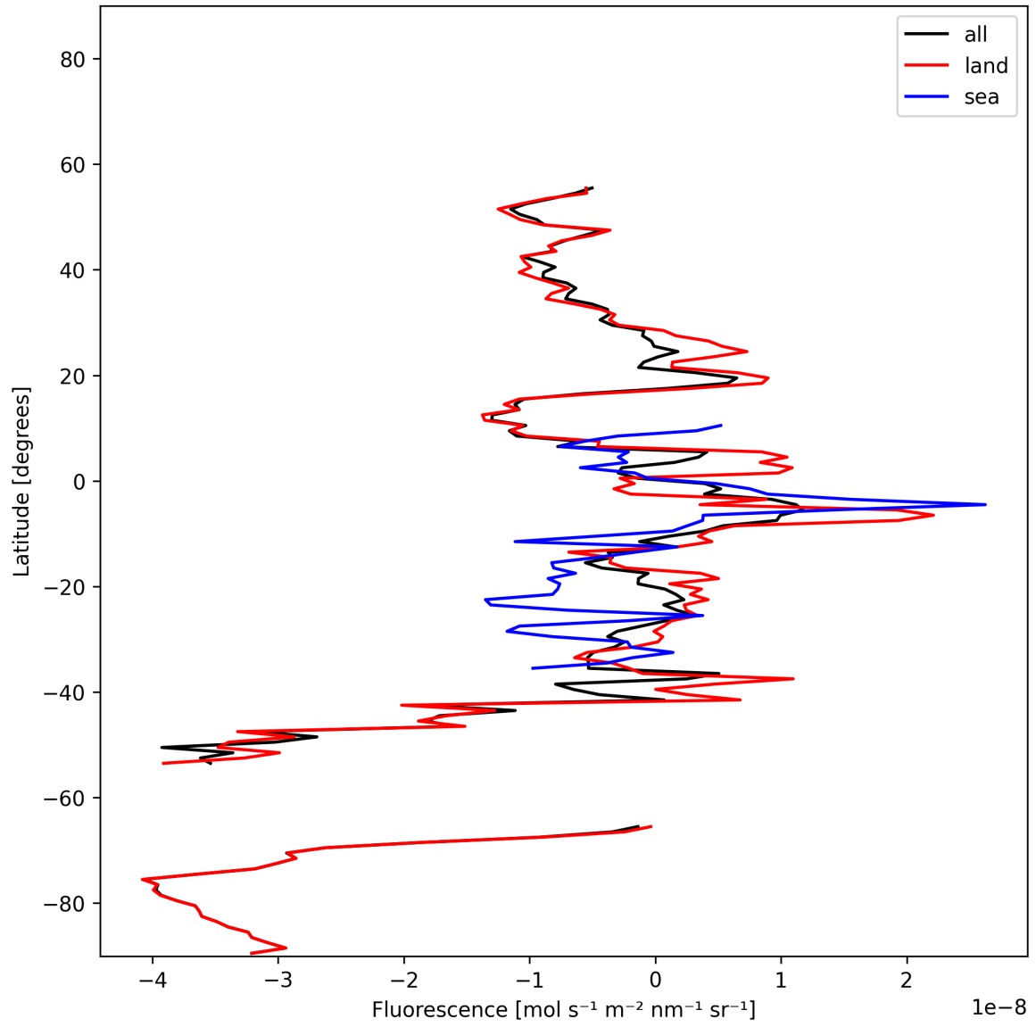
Figure 21: Zonal average of “Fluorescence” for 2025-11-16 to 2025-11-18.
