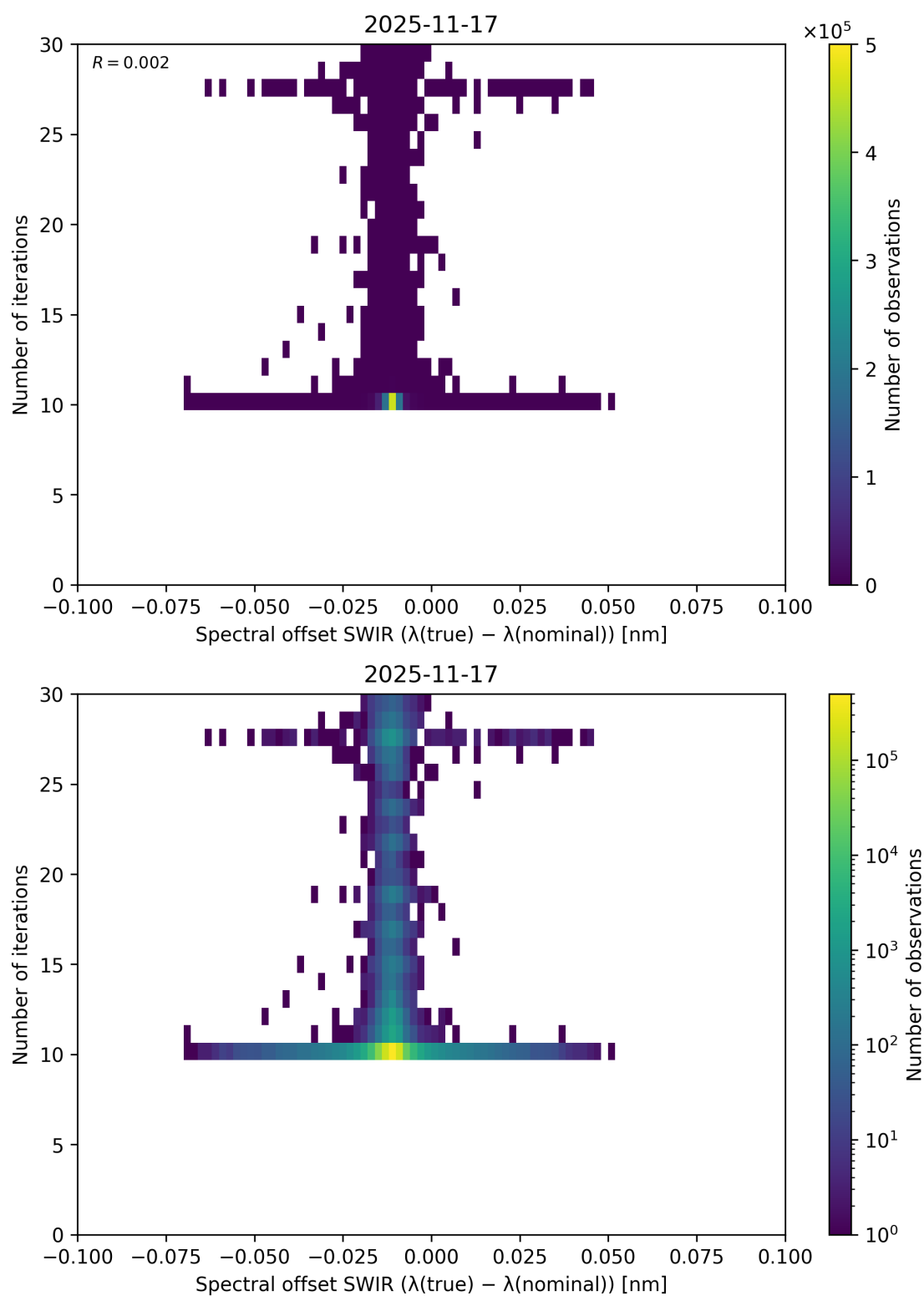
Figure 121: Scatter density plot of “Spectral offset SWIR ( \lambda_{\text{true}} - \lambda_{\text{nominal}} )” against “Number of iterations” for 2025-11-16 to 2025-11-18.
