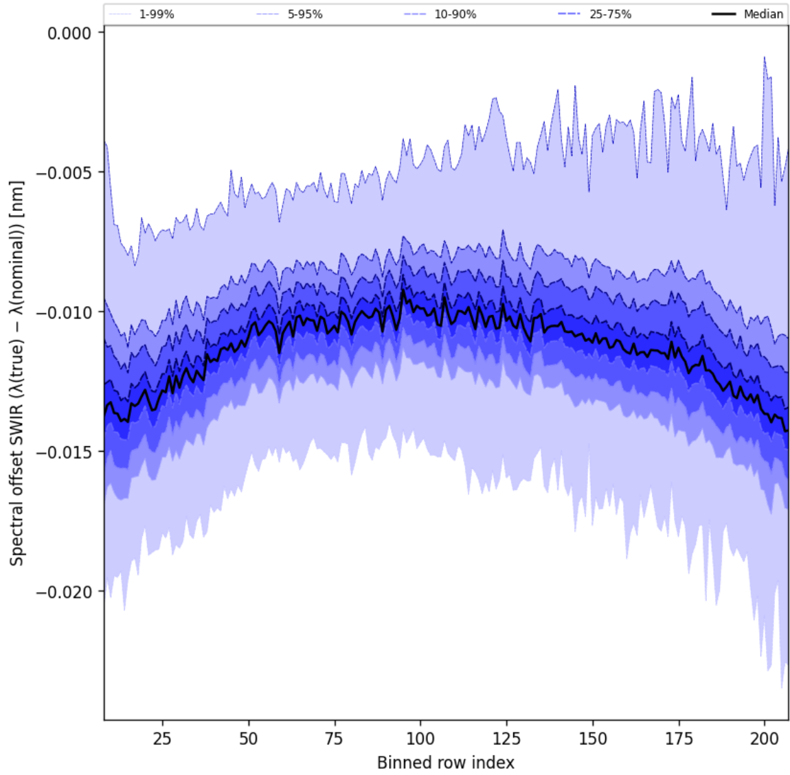
Figure 38: Along track statistics of “Spectral offset SWIR ( \lambda_{\text{true}} - \lambda_{\text{nominal}} )” for 2025-11-16 to 2025-11-18
