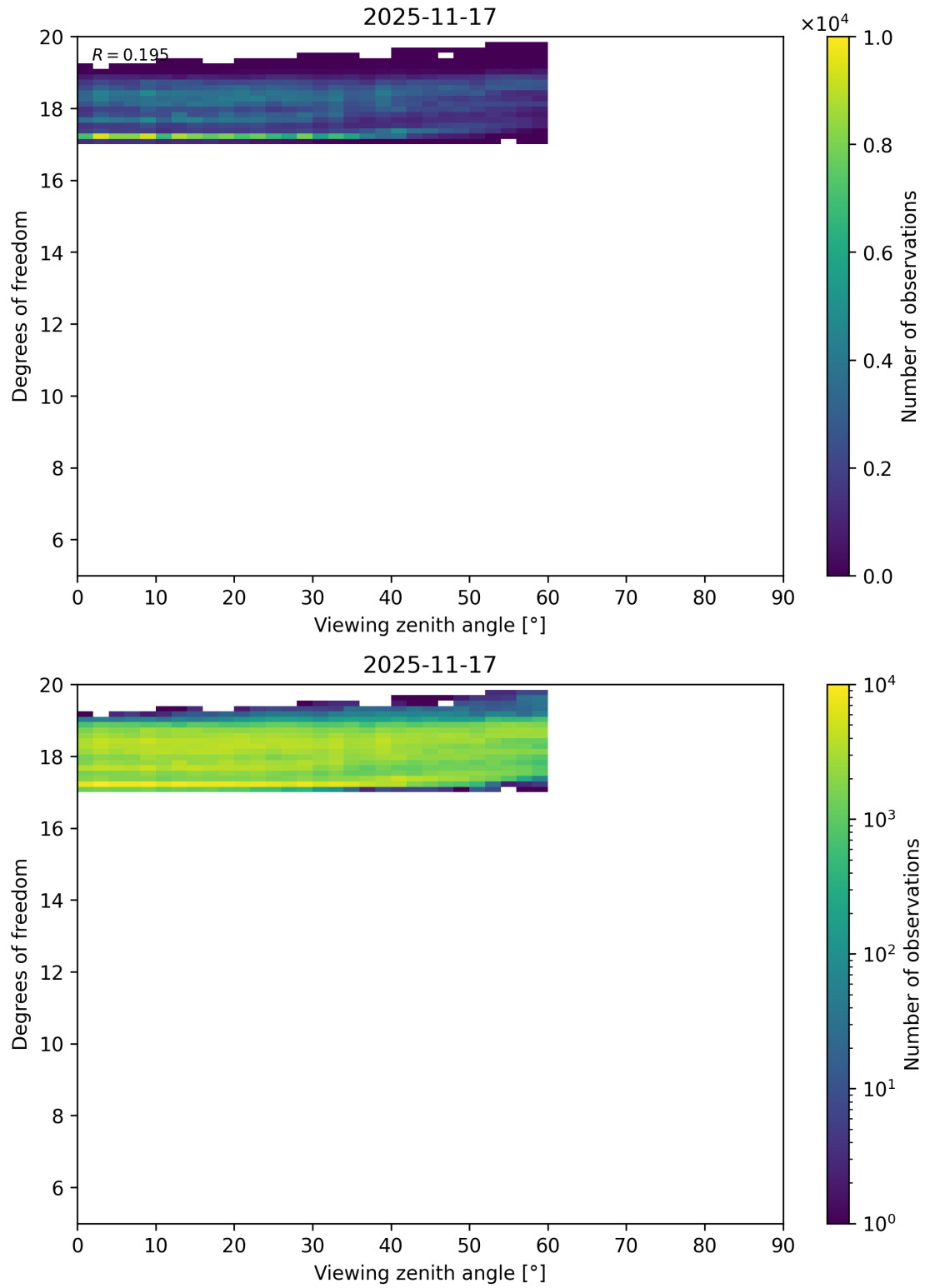
Figure 107: Scatter density plot of “Viewing zenith angle” against “Degrees of freedom” for 2025-11-16 to 2025-11-18.
