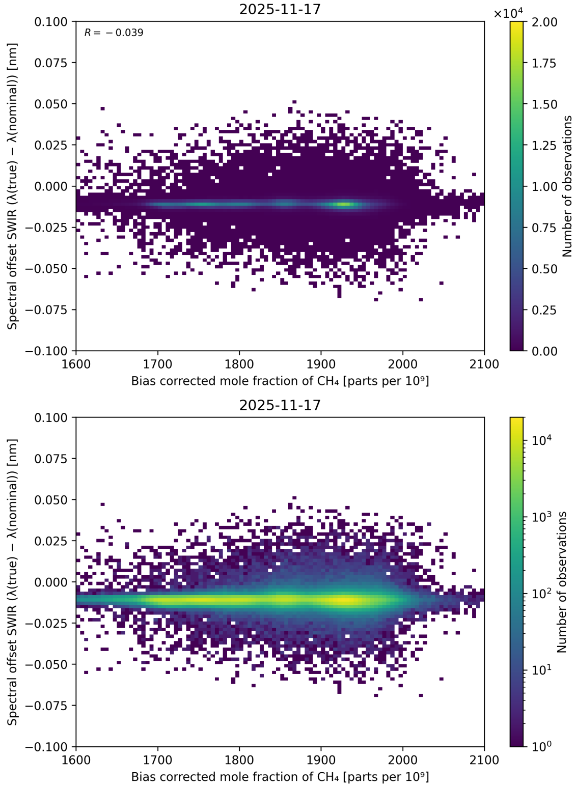
Figure 69: Scatter density plot of “Bias corrected mole fraction of \text{CH}_4 ” against “Spectral offset SWIR ( \lambda_{\text{true}} - \lambda_{\text{nominal}} )” for 2025-11-16 to 2025-11-18.
