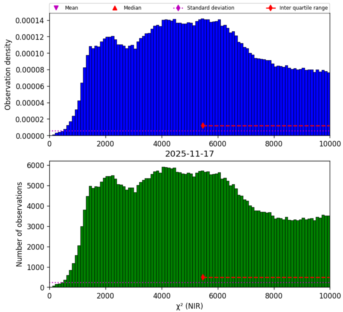
Figure 29: Histogram of “ \chi^2 (NIR)” for 2025-11-16 to 2025-11-18
