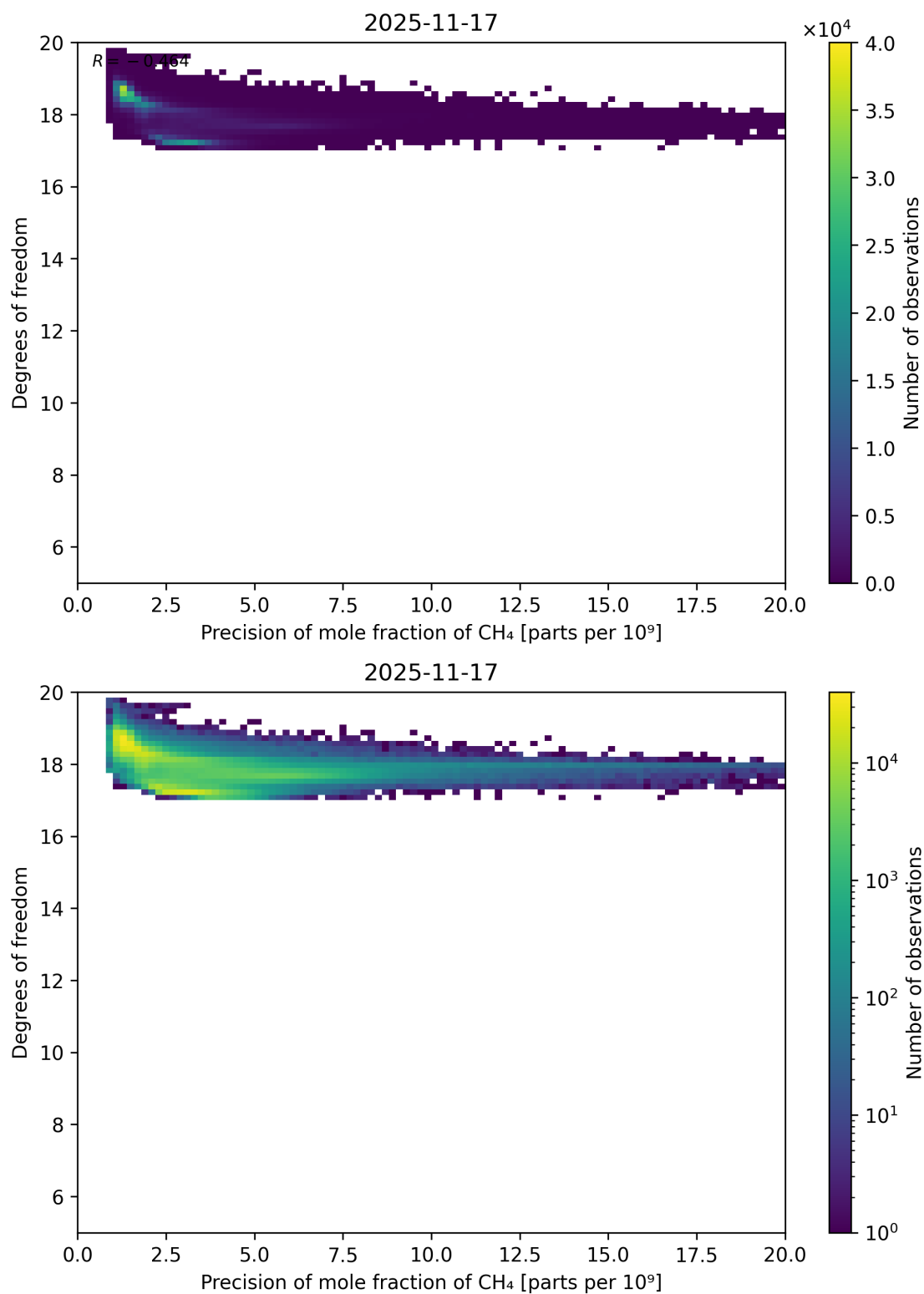
Figure 80: Scatter density plot of “Precision of mole fraction of CH 4 ” against “Degrees of freedom” for 2025-11-16 to 2025-11-18.
