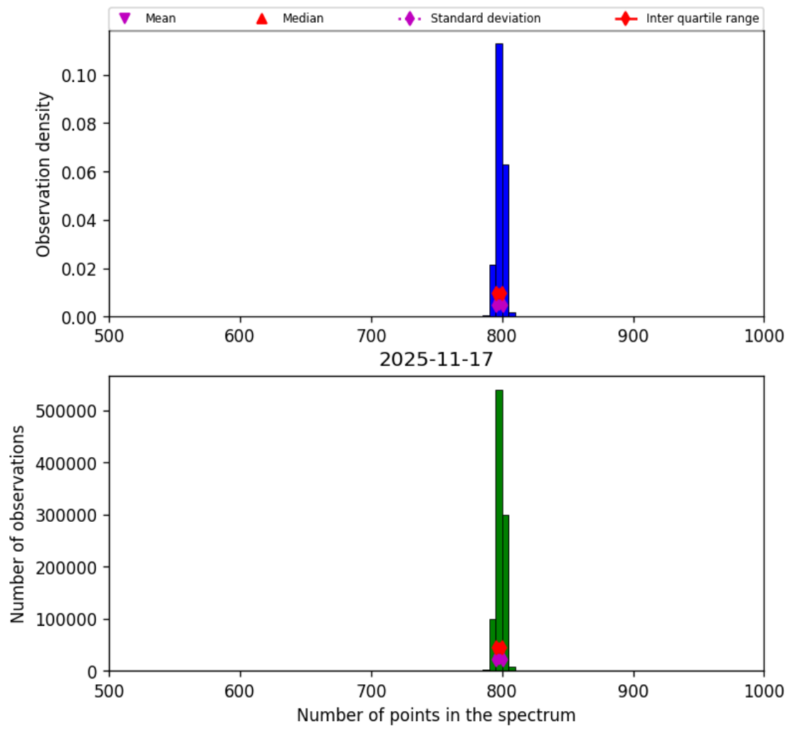
Figure 26: Histogram of “Number of points in the spectrum” for 2025-11-16 to 2025-11-18
