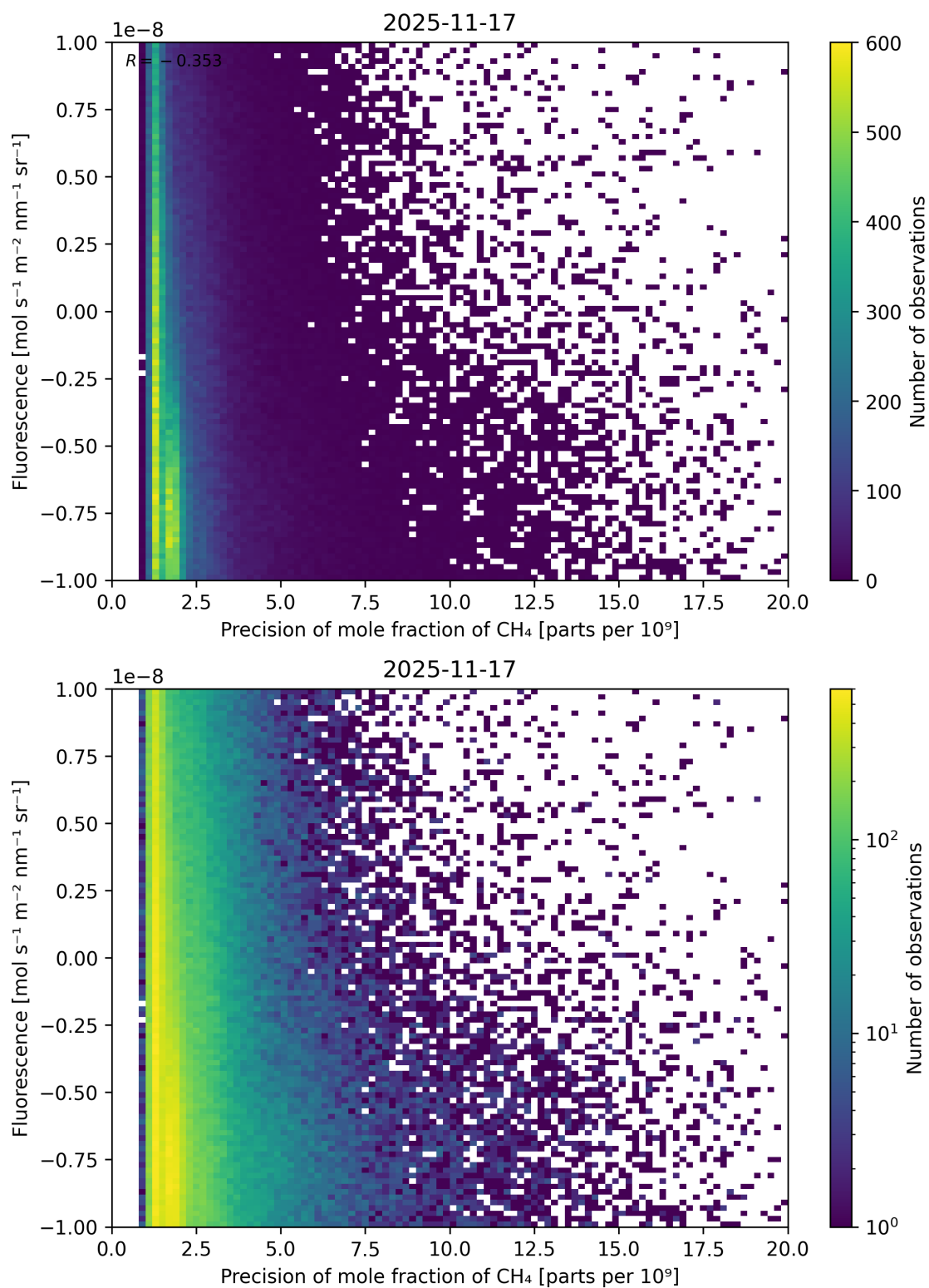
Figure 81: Scatter density plot of “Precision of mole fraction of \text{CH}_4 ” against “Fluorescence” for 2025-11-16 to 2025-11-18.
