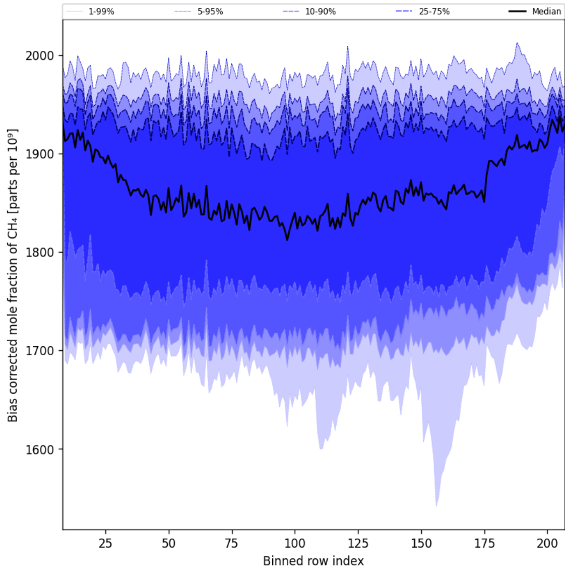
Figure 36: Along track statistics of “Bias corrected mole fraction of CH 4 ” for 2025-11-16 to 2025-11-18
