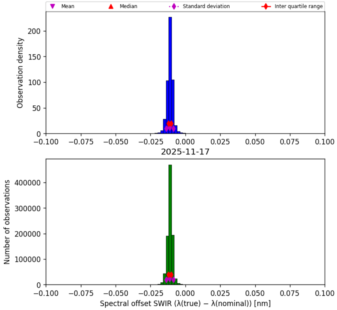
Figure 27: Histogram of “Spectral offset SWIR ( \lambda_{\text{true}} - \lambda_{\text{nominal}} )” for 2025-11-16 to 2025-11-18
