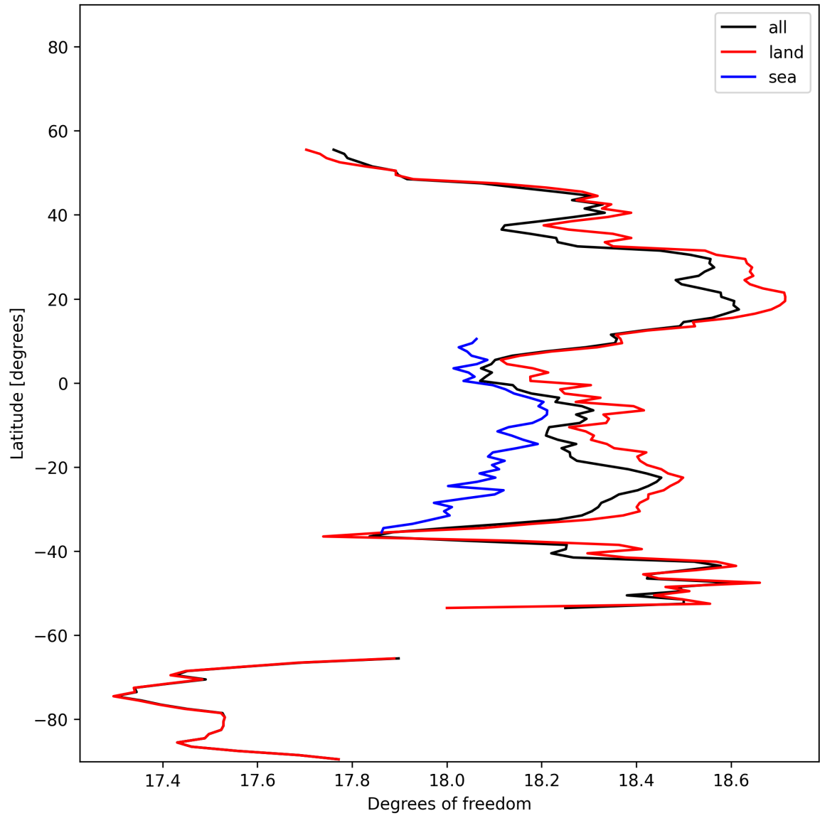
Figure 19: Zonal average of “Degrees of freedom” for 2025-11-16 to 2025-11-18.
