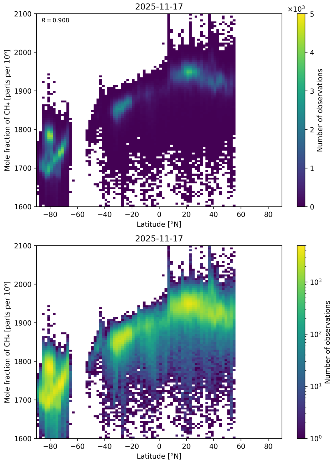
Figure 57: Scatter density plot of “Latitude” against “Mole fraction of CH 4 ” for 2025-11-16 to 2025-11-18.
