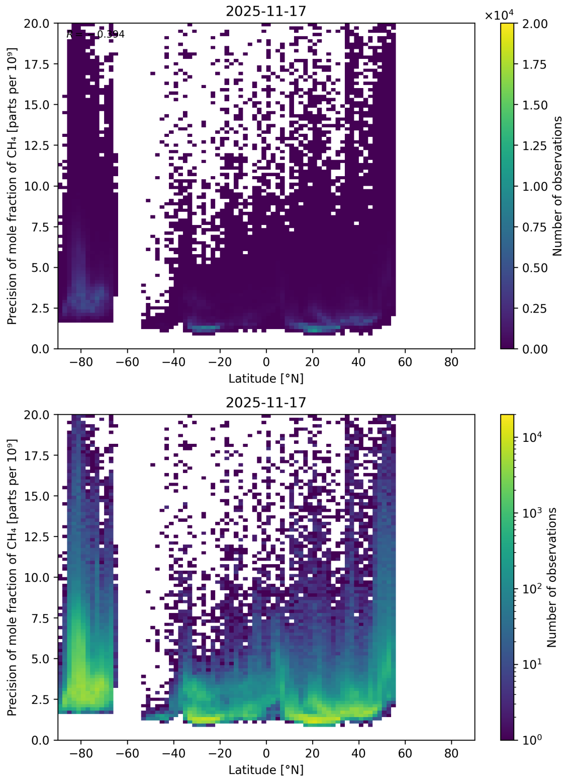
Figure 59: Scatter density plot of “Latitude” against “Precision of mole fraction of CH 4 ” for 2025-11-16 to 2025-11-18.
