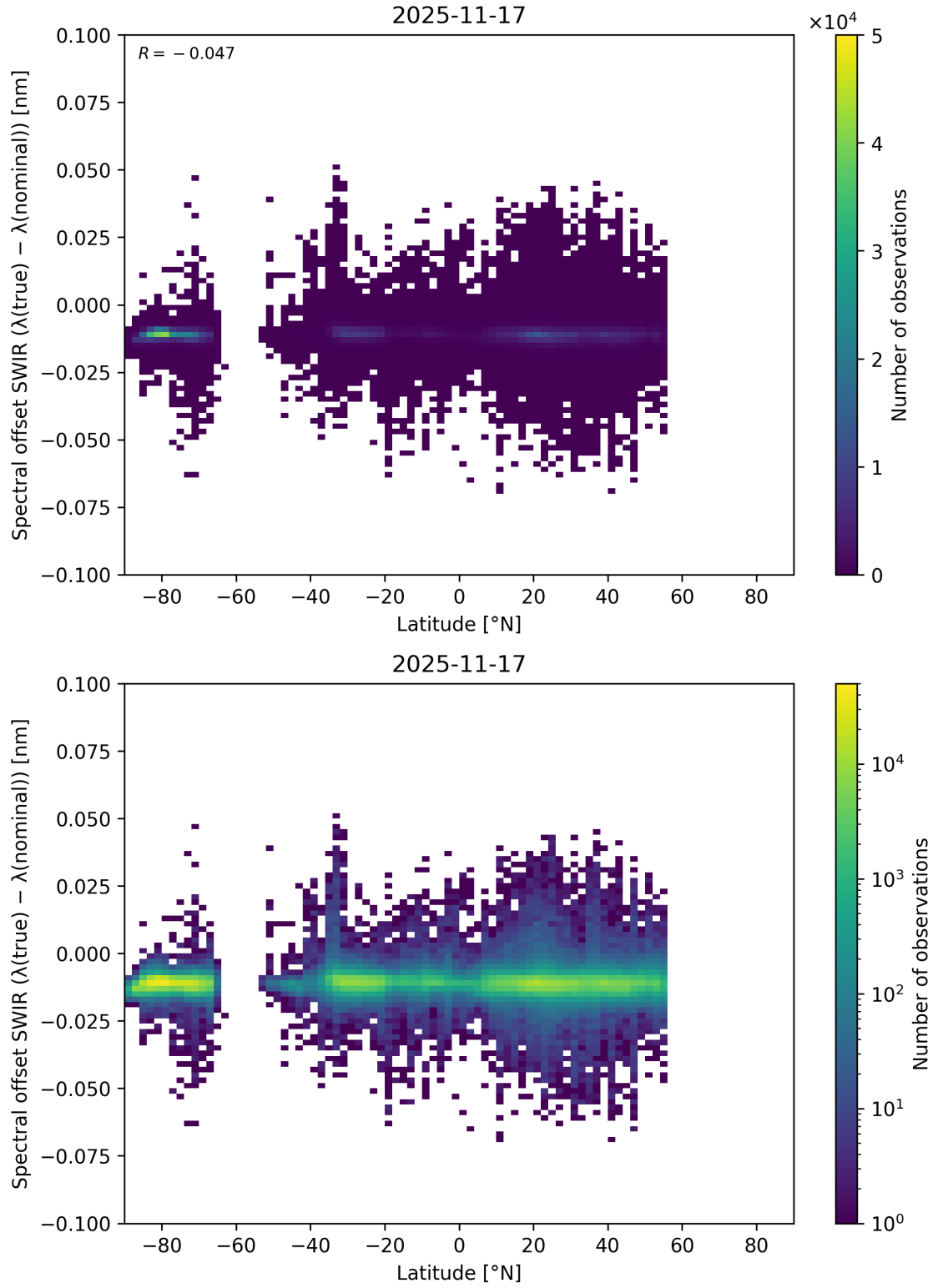
Figure 62: Scatter density plot of “Latitude” against “Spectral offset SWIR ( \lambda_{\text{true}} - \lambda_{\text{nominal}} )” for 2025-11-16 to 2025-11-18.
