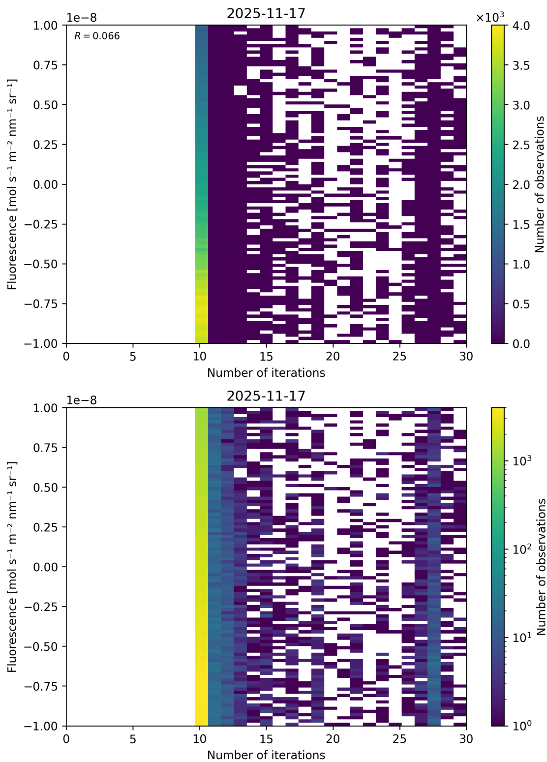
Figure 87: Scatter density plot of “Number of iterations” against “Fluorescence” for 2025-11-16 to 2025-11-18.
