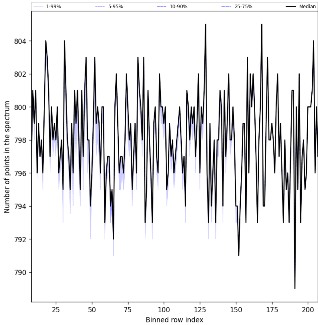
Figure 37: Along track statistics of “Number of points in the spectrum” for 2025-11-16 to 2025-11-18
