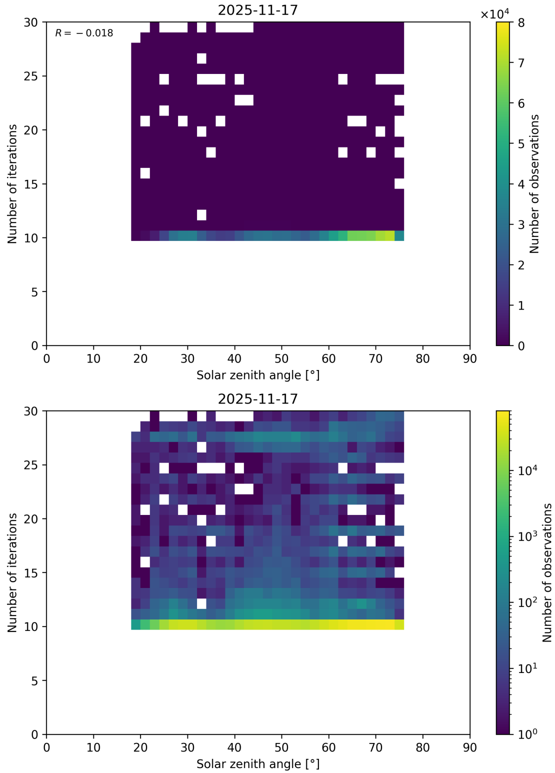
Figure 102: Scatter density plot of “Solar zenith angle” against “Number of iterations” for 2025-11-16 to 2025-11-18.
