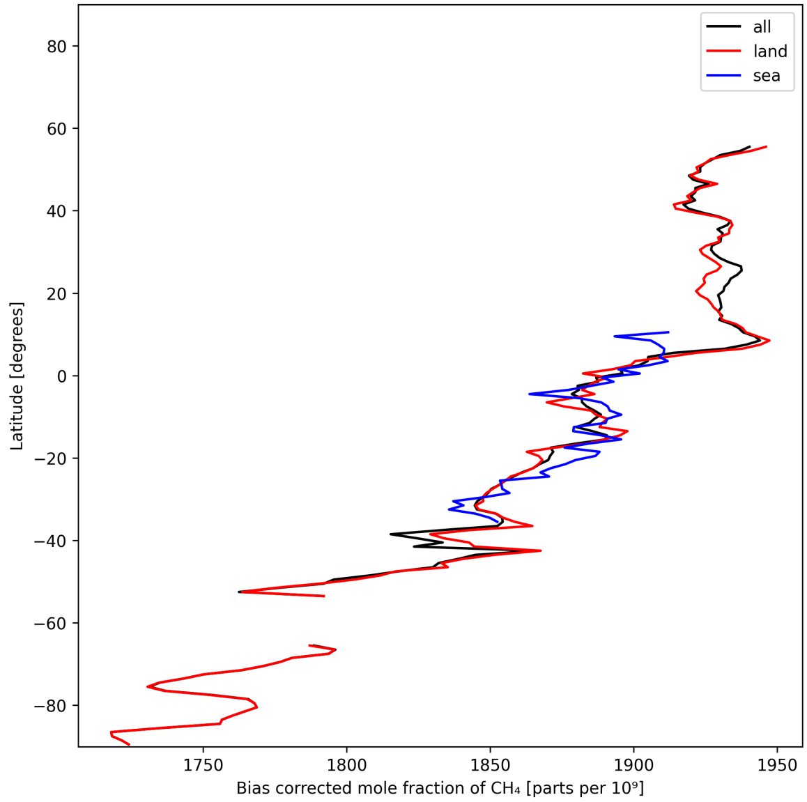
Figure 14: Zonal average of “Bias corrected mole fraction of CH 4 ” for 2025-11-16 to 2025-11-18.
