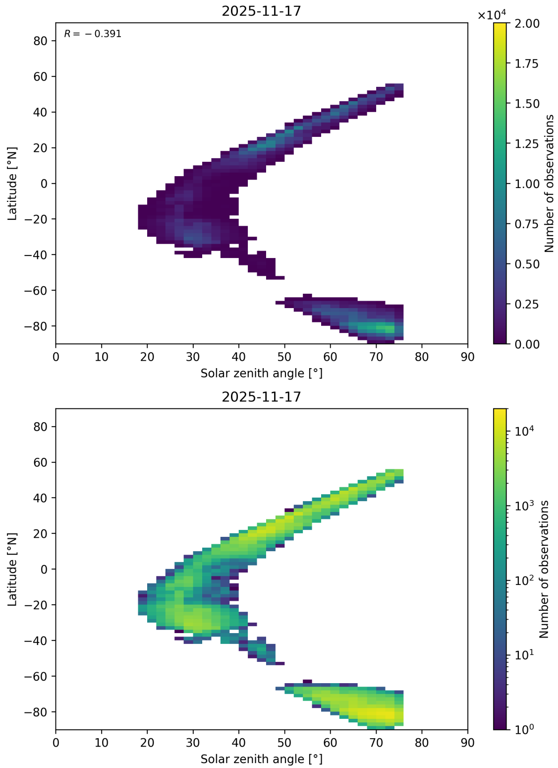
Figure 98: Scatter density plot of “Solar zenith angle” against “Latitude” for 2025-11-16 to 2025-11-18.
