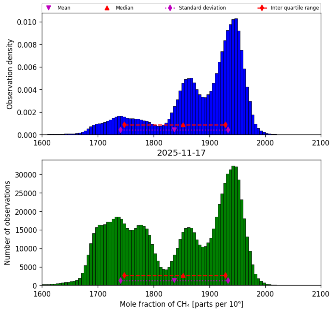
Figure 23: Histogram of “Mole fraction of CH 4 ” for 2025-11-16 to 2025-11-18
