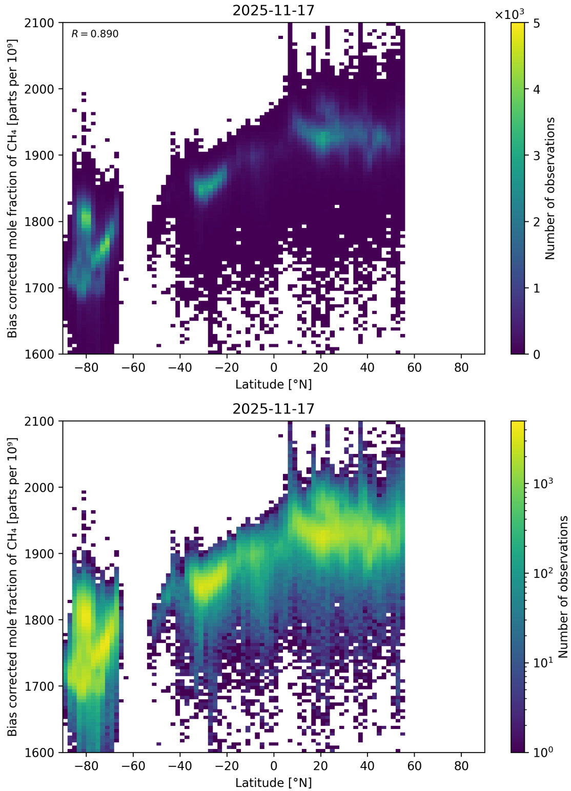
Figure 58: Scatter density plot of “Latitude” against “Bias corrected mole fraction of CH 4 ” for 2025-11-16 to 2025-11-18.
