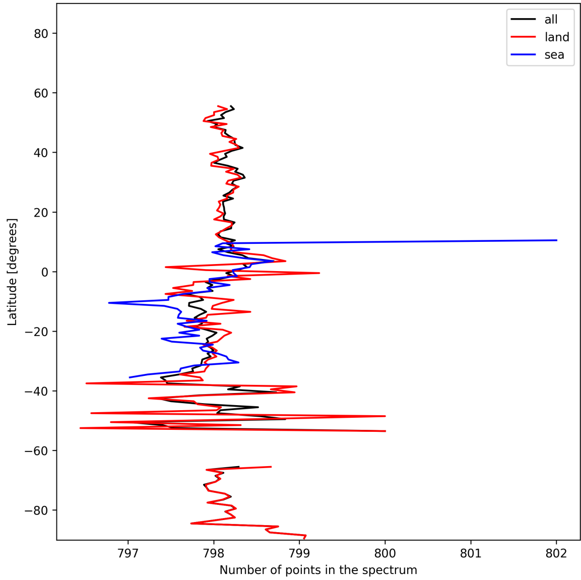
Figure 15: Zonal average of “Number of points in the spectrum” for 2025-11-16 to 2025-11-18.
