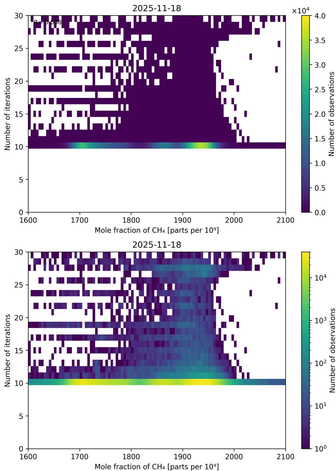
Figure 76: Scatter density plot of “Mole fraction of CH 4 ” against “Number of iterations” for 2025-11-18 to 2025-11-19.
