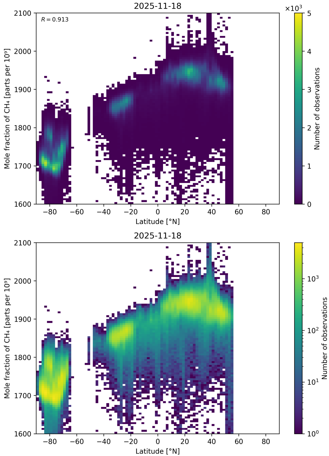
Figure 57: Scatter density plot of “Latitude” against “Mole fraction of CH 4 ” for 2025-11-18 to 2025-11-19.
