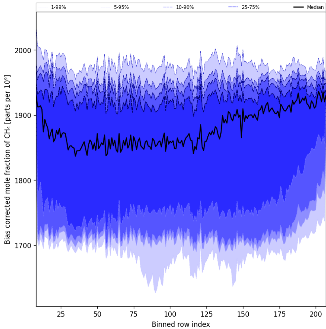
Figure 36: Along track statistics of “Bias corrected mole fraction of CH 4 ” for 2025-11-18 to 2025-11-19
