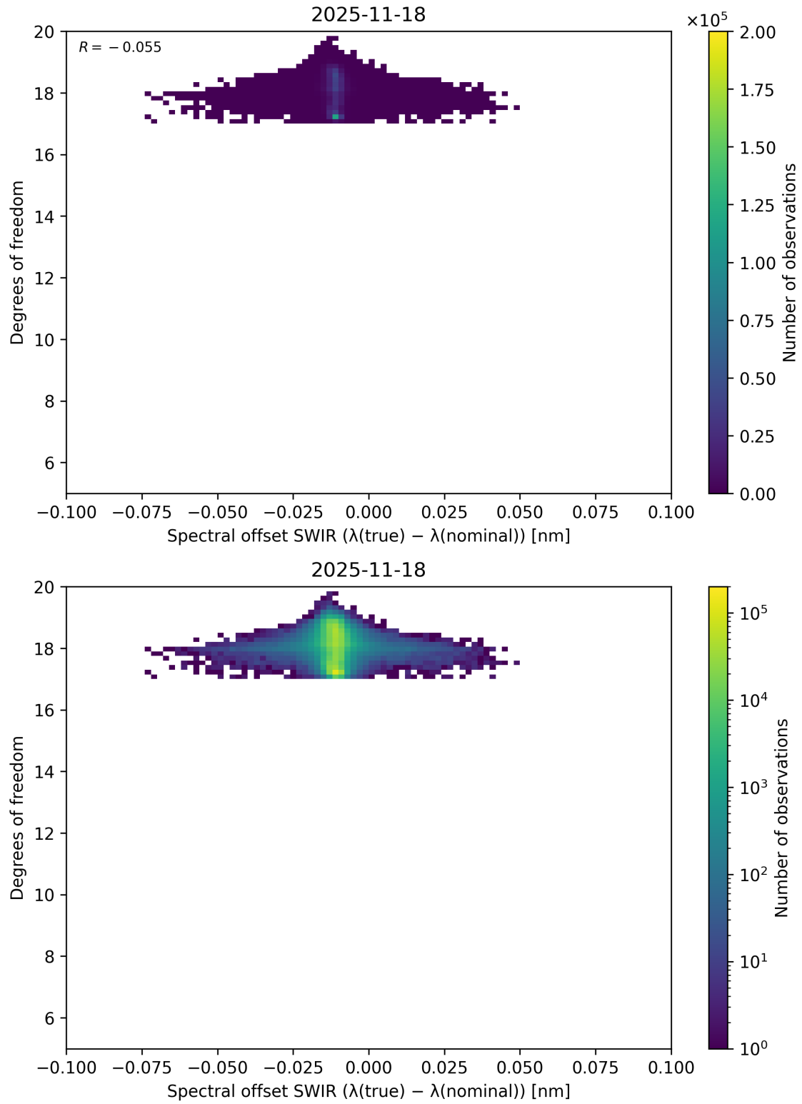
Figure 119: Scatter density plot of “Spectral offset SWIR ( \lambda_{\text{true}} - \lambda_{\text{nominal}} )” against “Degrees of freedom” for 2025-11-18 to 2025-11-19.
