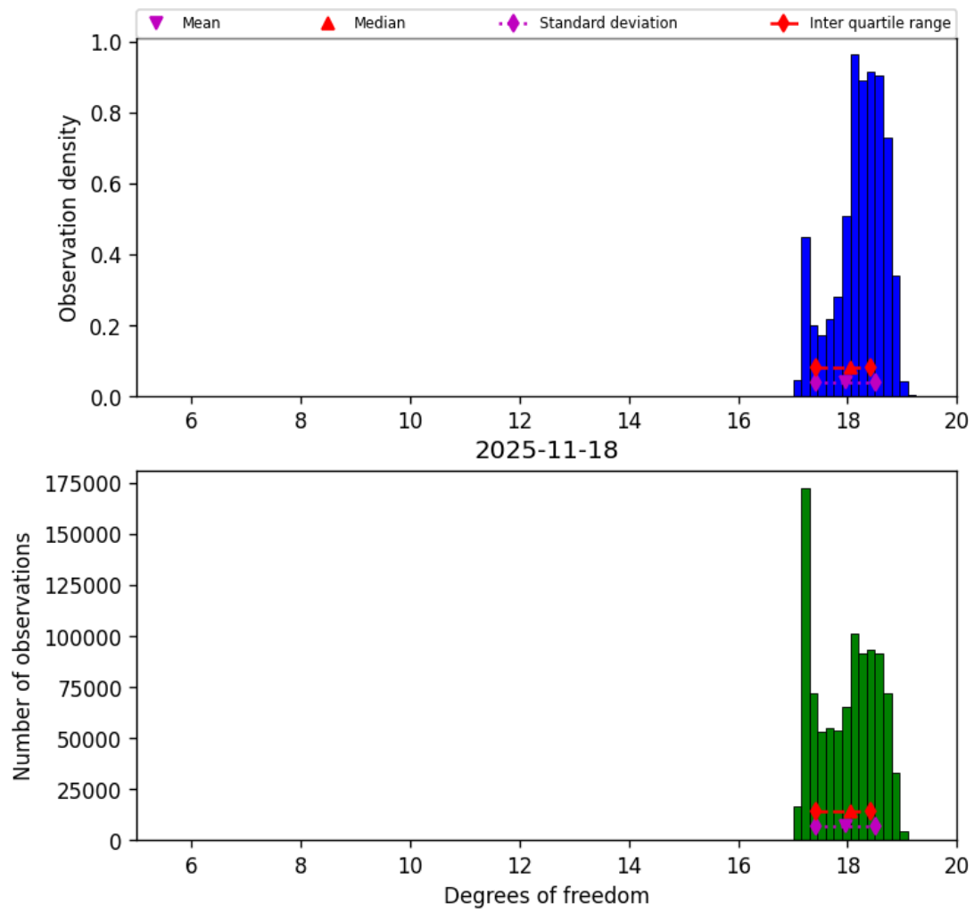
Figure 30: Histogram of “Degrees of freedom” for 2025-11-18 to 2025-11-19
