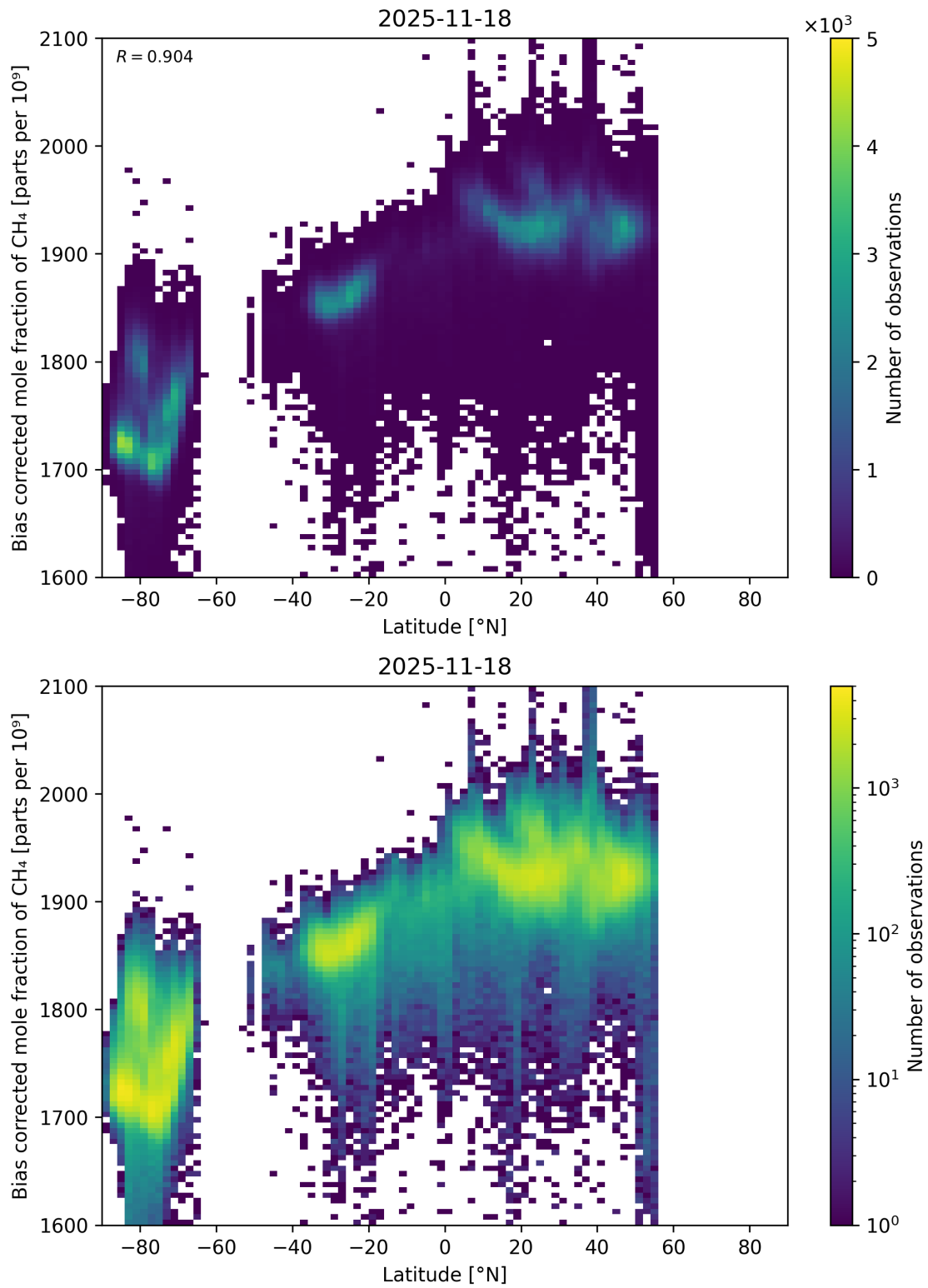
Figure 58: Scatter density plot of “Latitude” against “Bias corrected mole fraction of CH 4 ” for 2025-11-18 to 2025-11-19.
