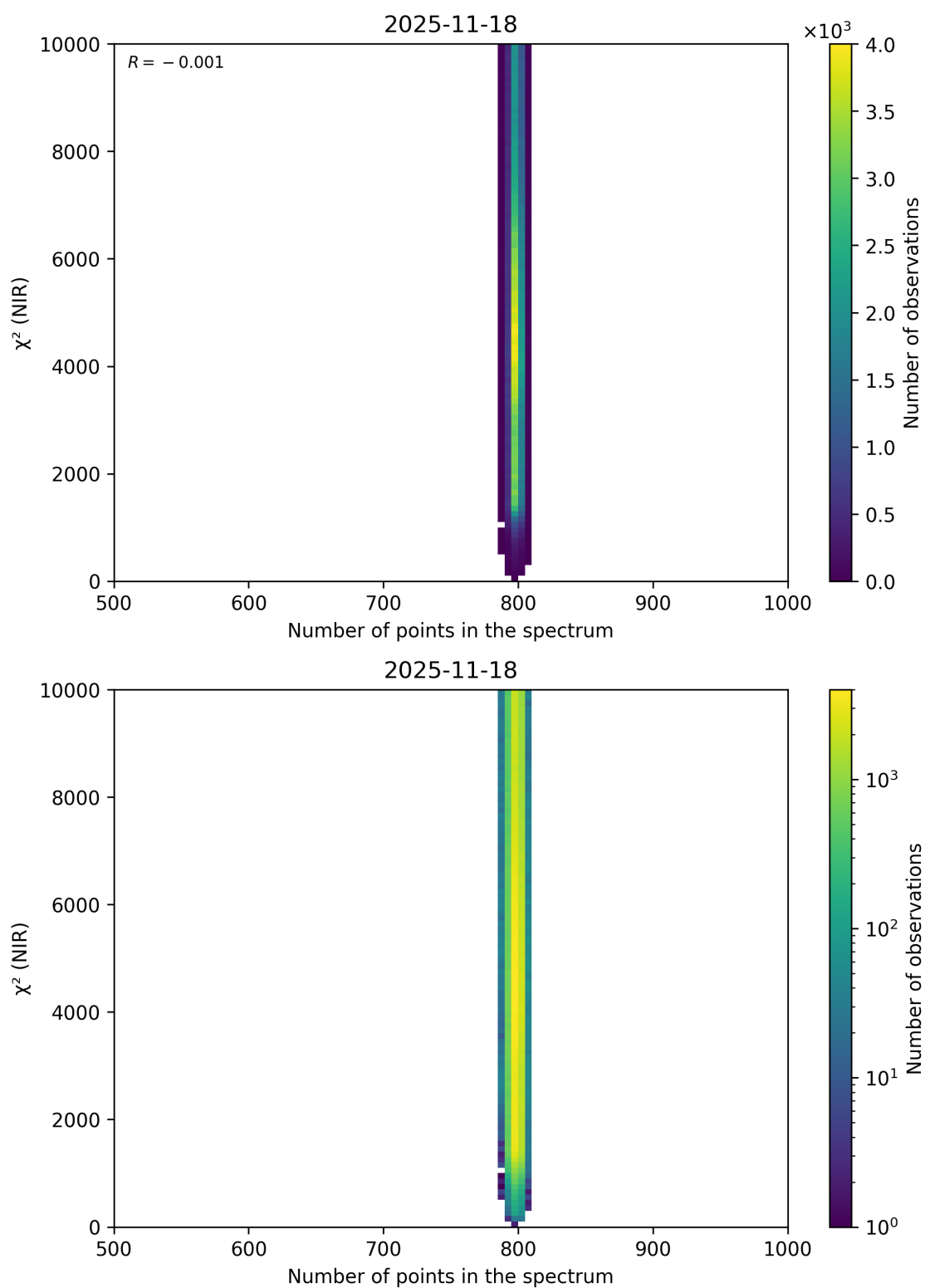
Figure 88: Scatter density plot of “Number of points in the spectrum” against “ \chi^2 (NIR)” for 2025-11-18 to 2025-11-19.
