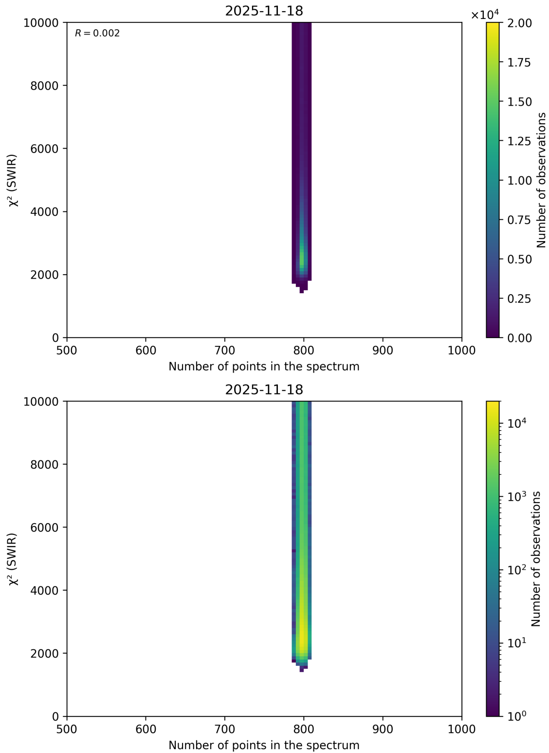
Figure 89: Scatter density plot of “Number of points in the spectrum” against “ \chi^2 (SWIR)” for 2025-11-18 to 2025-11-19.
