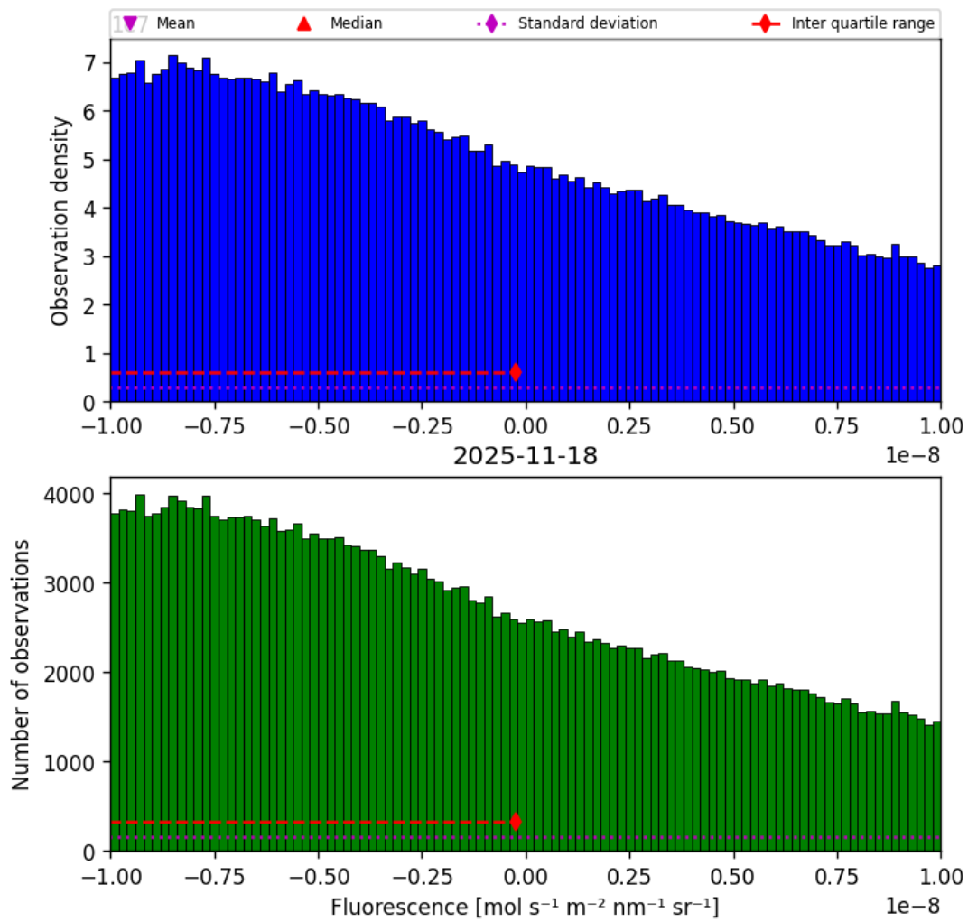
Figure 32: Histogram of “Fluorescence” for 2025-11-18 to 2025-11-19
