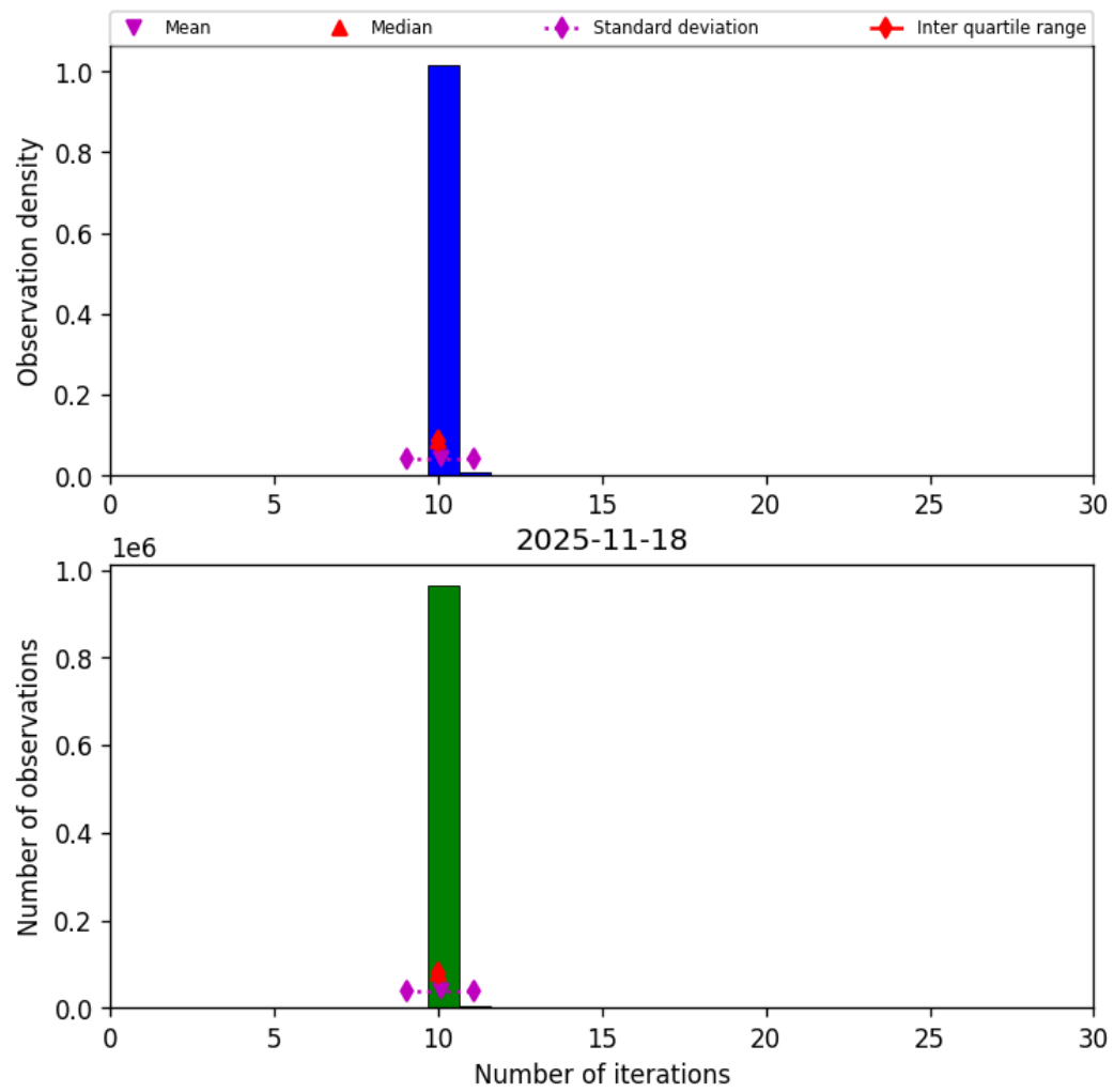
Figure 31: Histogram of “Number of iterations” for 2025-11-18 to 2025-11-19
