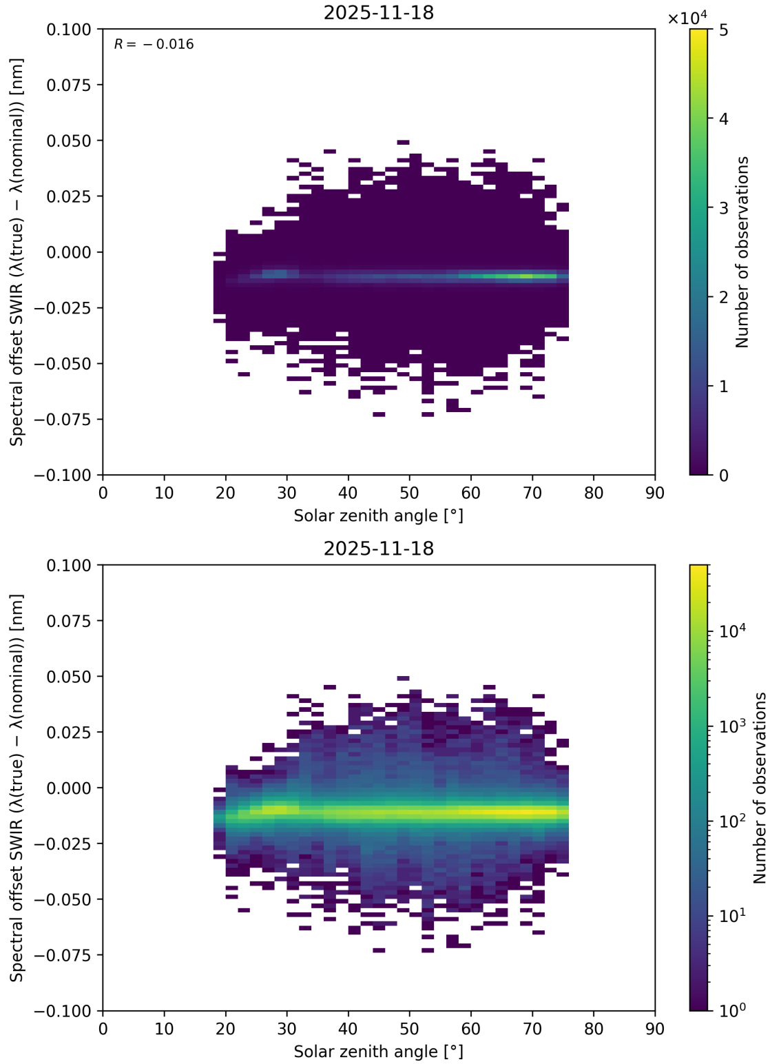
Figure 104: Scatter density plot of “Solar zenith angle” against “Spectral offset SWIR ( \lambda_{\text{true}} - \lambda_{\text{nominal}} )” for 2025-11-18 to 2025-11-19.
