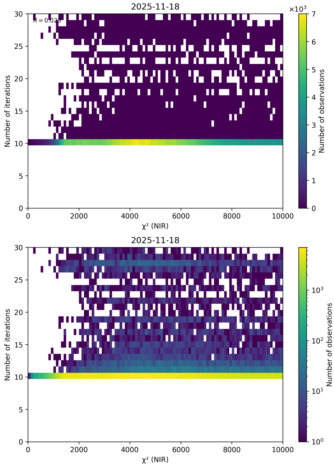
Figure 46: Scatter density plot of “ \chi^2 (NIR)” against “Number of iterations” for 2025-11-18 to 2025-11-19.
