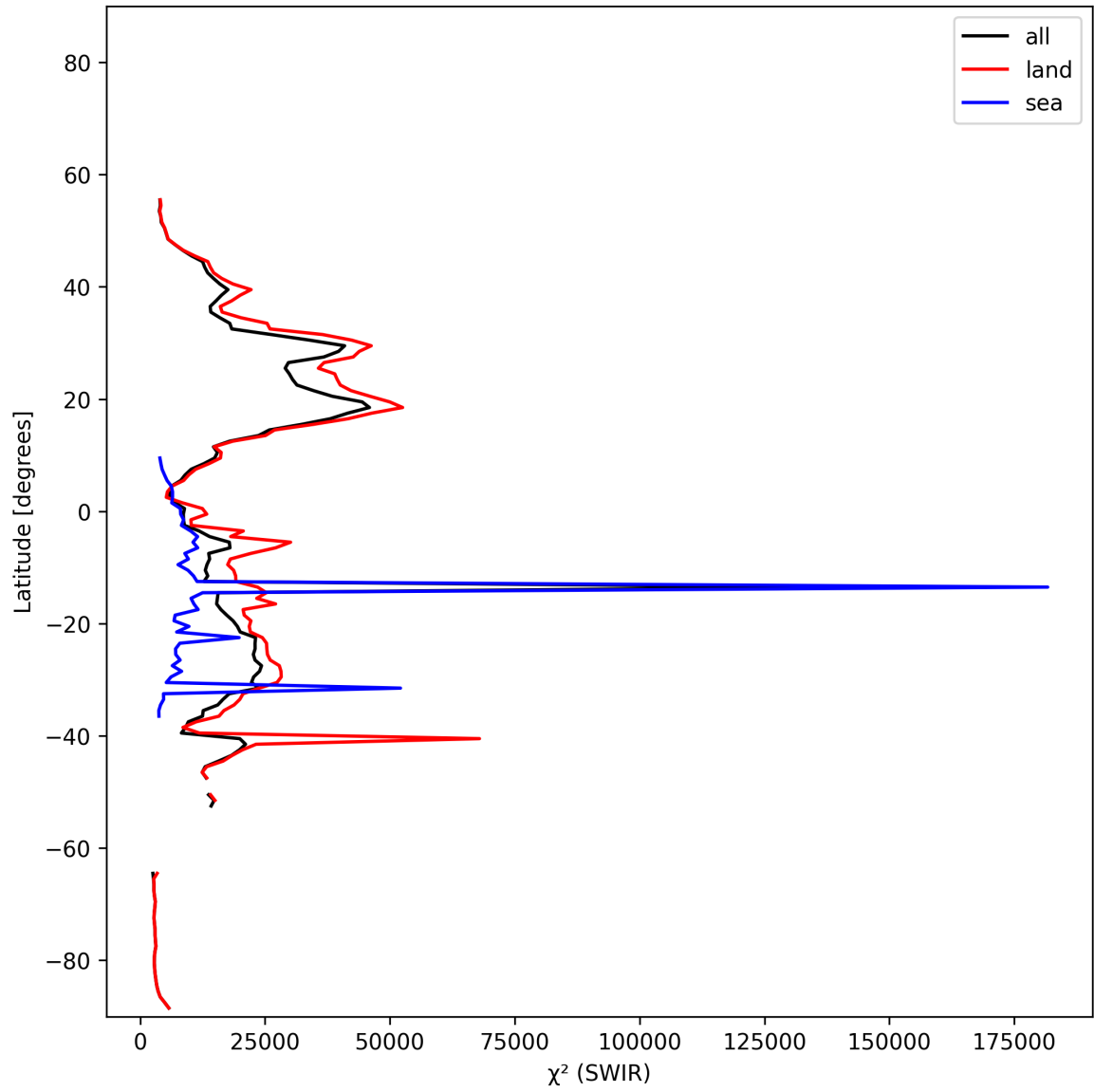
Figure 17: Zonal average of “ \chi^2 (SWIR)” for 2025-11-18 to 2025-11-19.
