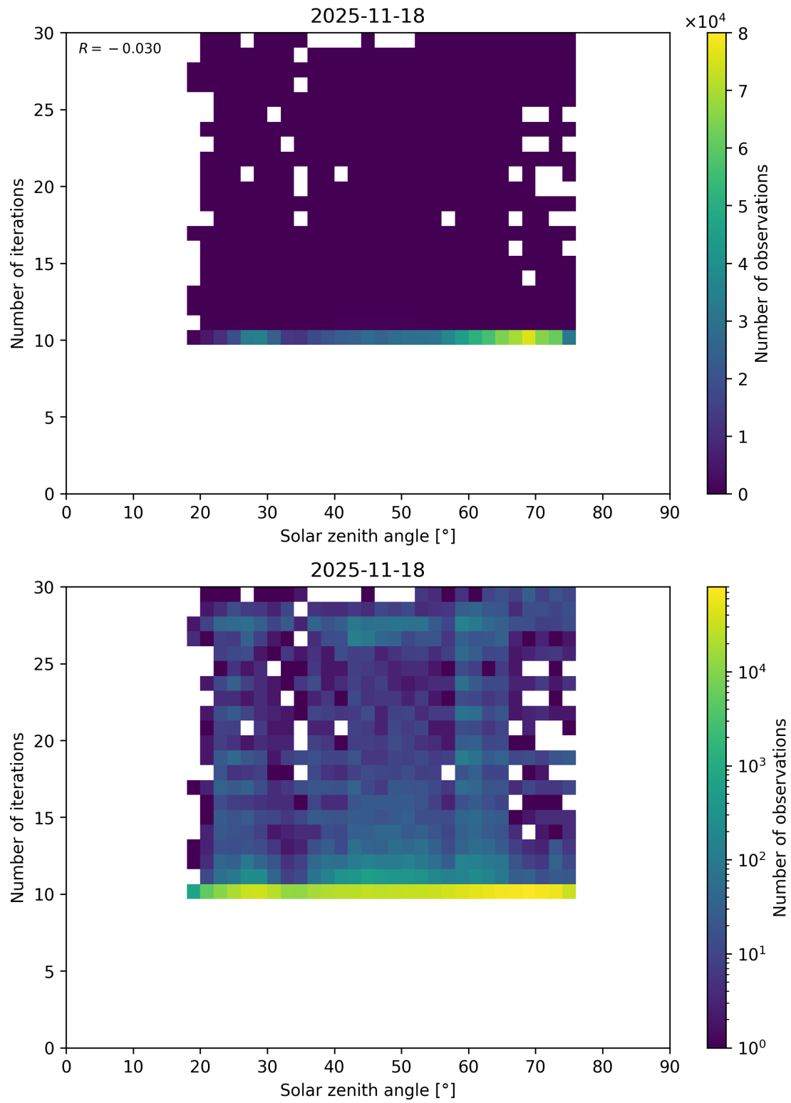
Figure 102: Scatter density plot of “Solar zenith angle” against “Number of iterations” for 2025-11-18 to 2025-11-19.
