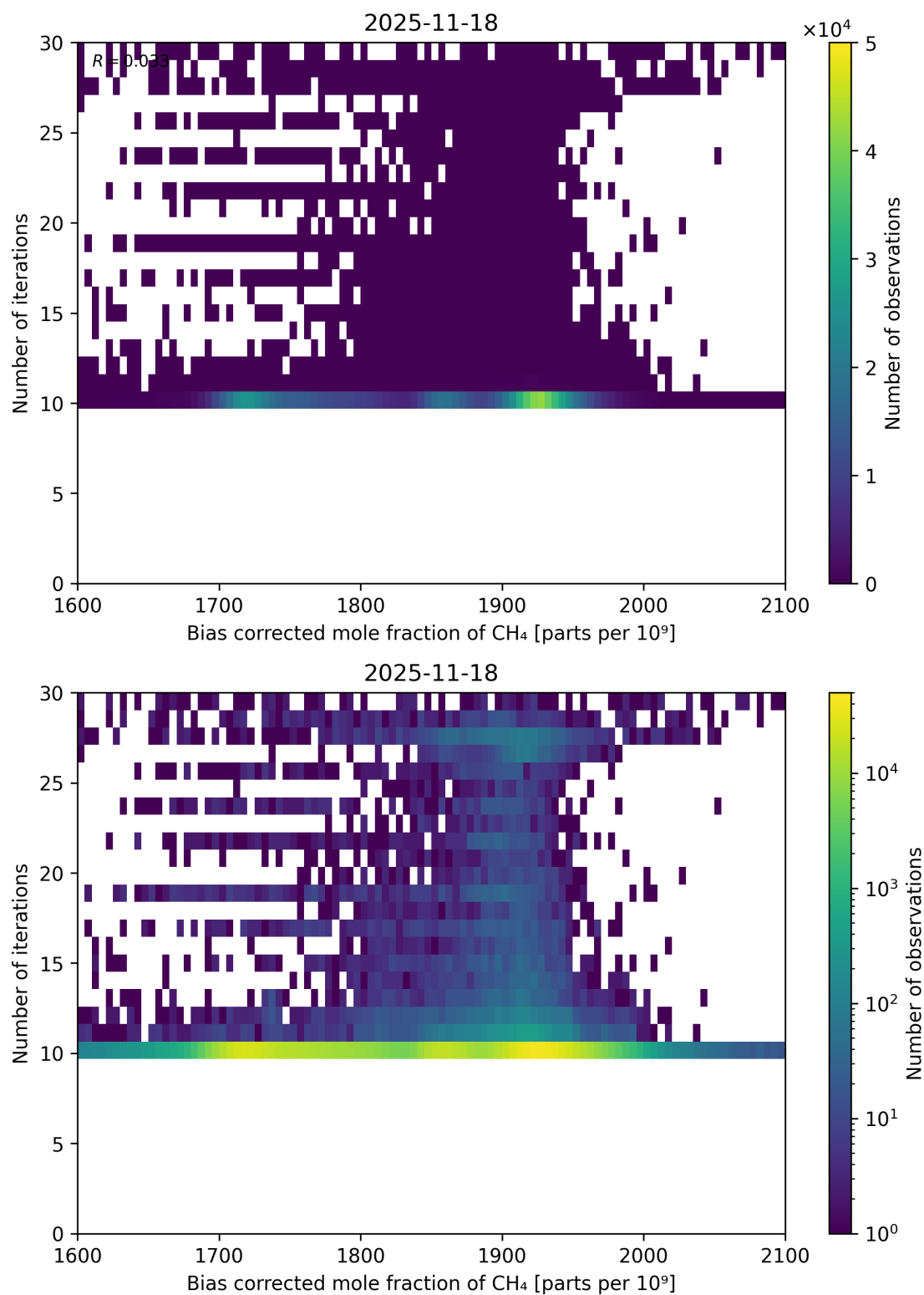
Figure 67: Scatter density plot of “Bias corrected mole fraction of CH 4 ” against “Number of iterations” for 2025-11-18 to 2025-11-19.
