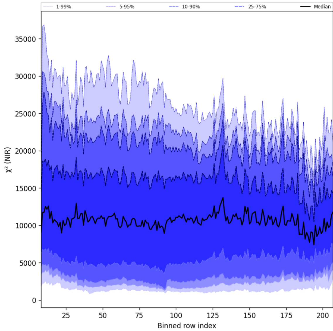
Figure 40: Along track statistics of “ \chi^2 (NIR)” for 2025-11-18 to 2025-11-19
