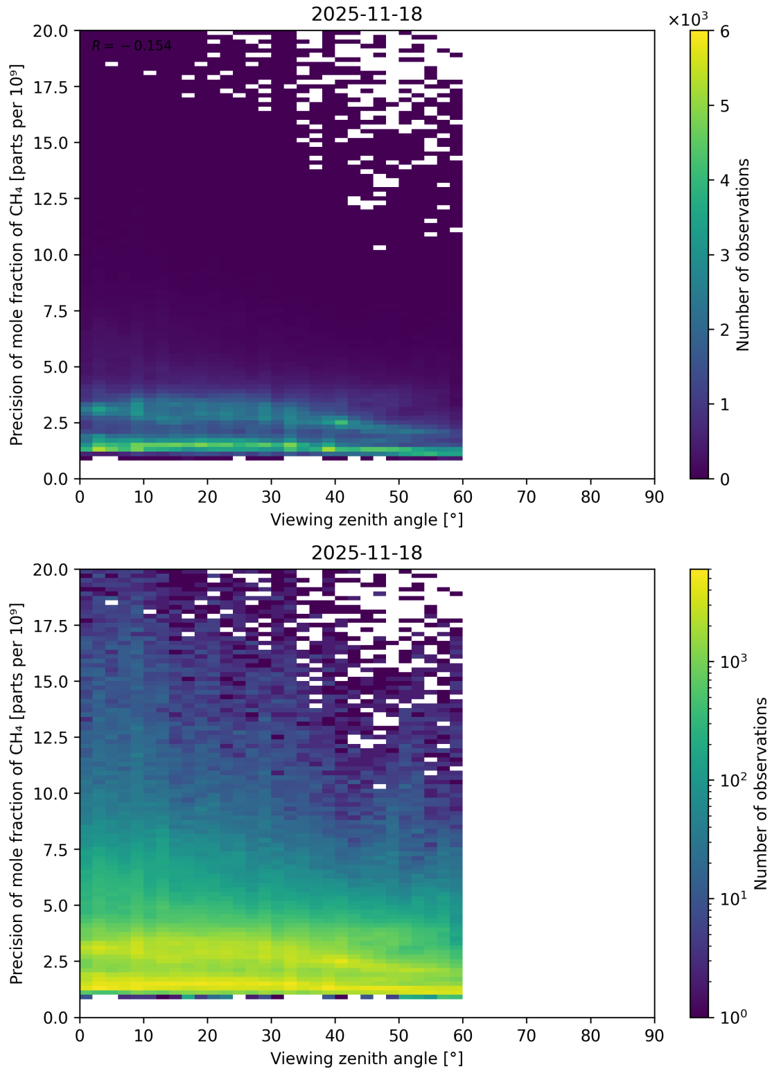
Figure 112: Scatter density plot of “Viewing zenith angle” against “Precision of mole fraction of \text{CH}_4 ” for 2025-11-18 to 2025-11-19.
