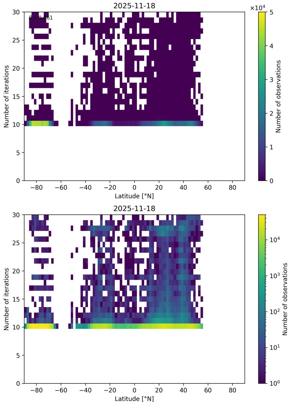
Figure 60: Scatter density plot of “Latitude” against “Number of iterations” for 2025-11-18 to 2025-11-19.
