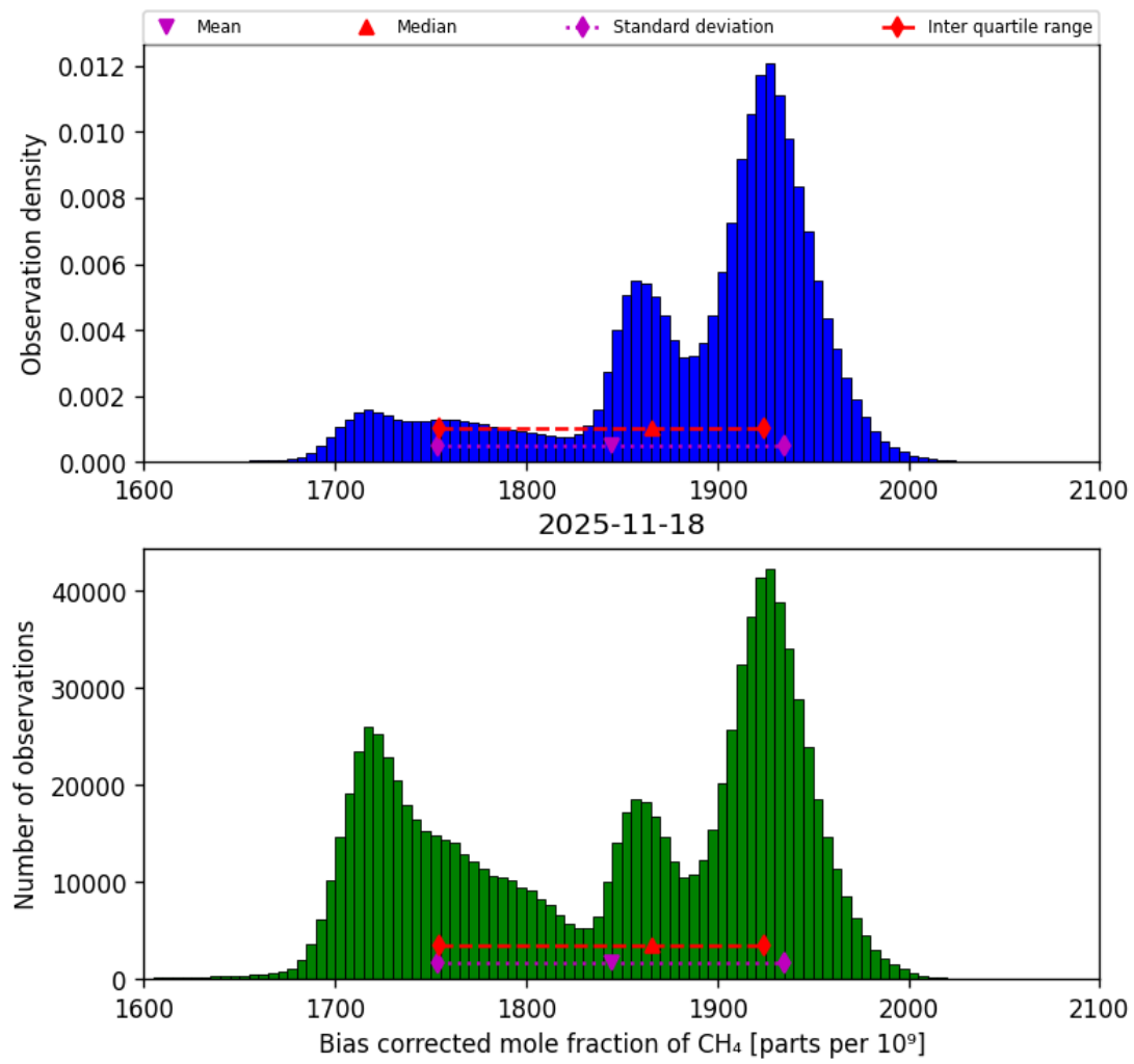
Figure 25: Histogram of “Bias corrected mole fraction of CH 4 ” for 2025-11-18 to 2025-11-19
