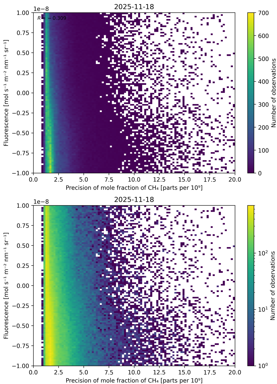
Figure 81: Scatter density plot of “Precision of mole fraction of CH 4 ” against “Fluorescence” for 2025-11-18 to 2025-11-19.
