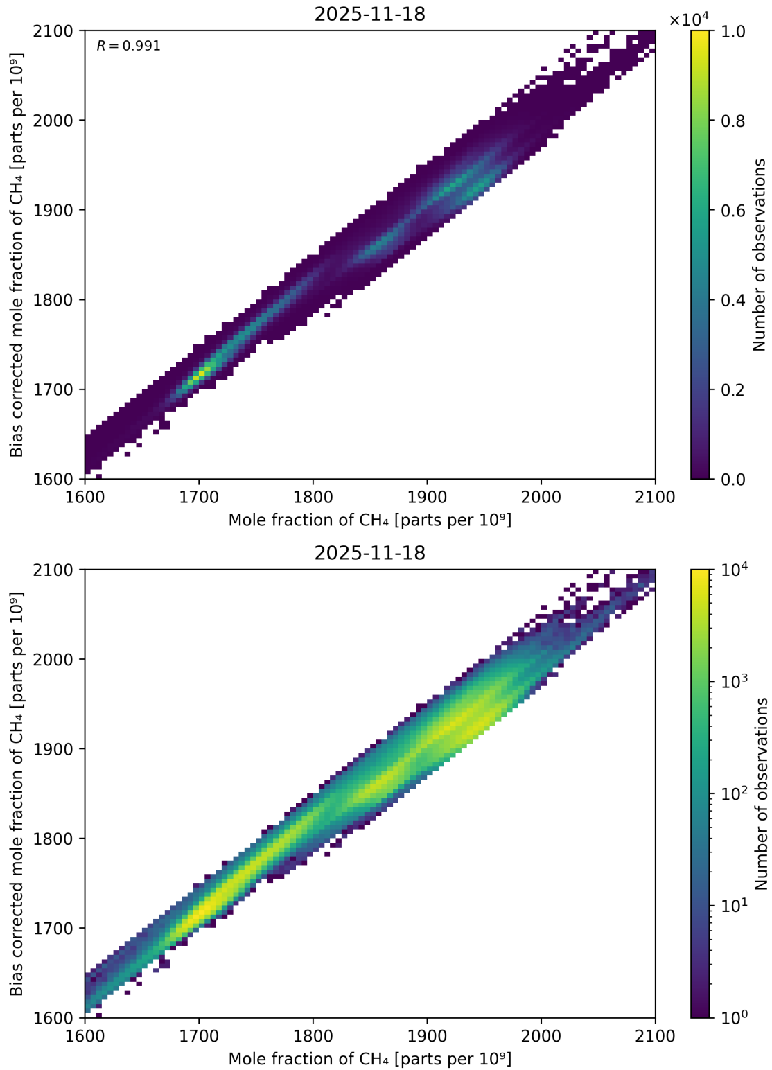
Figure 74: Scatter density plot of “Mole fraction of CH 4 ” against “Bias corrected mole fraction of CH 4 ” for 2025-11-18 to 2025-11-19.
