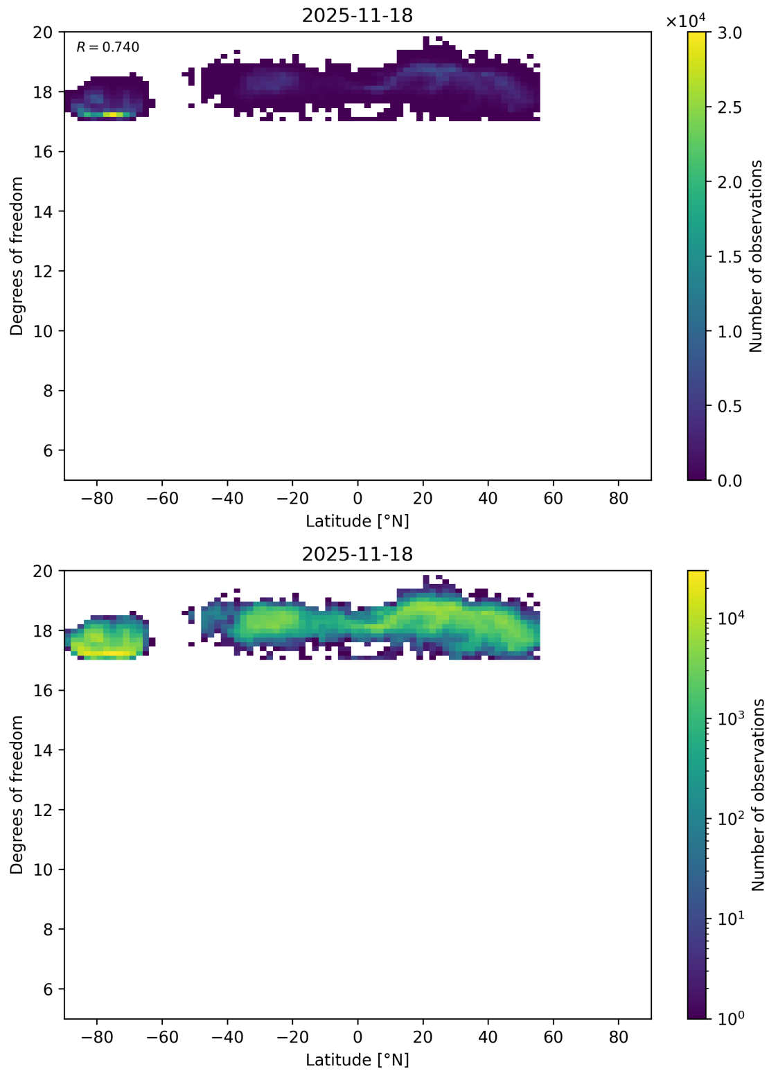
Figure 55: Scatter density plot of “Latitude” against “Degrees of freedom” for 2025-11-18 to 2025-11-19.
