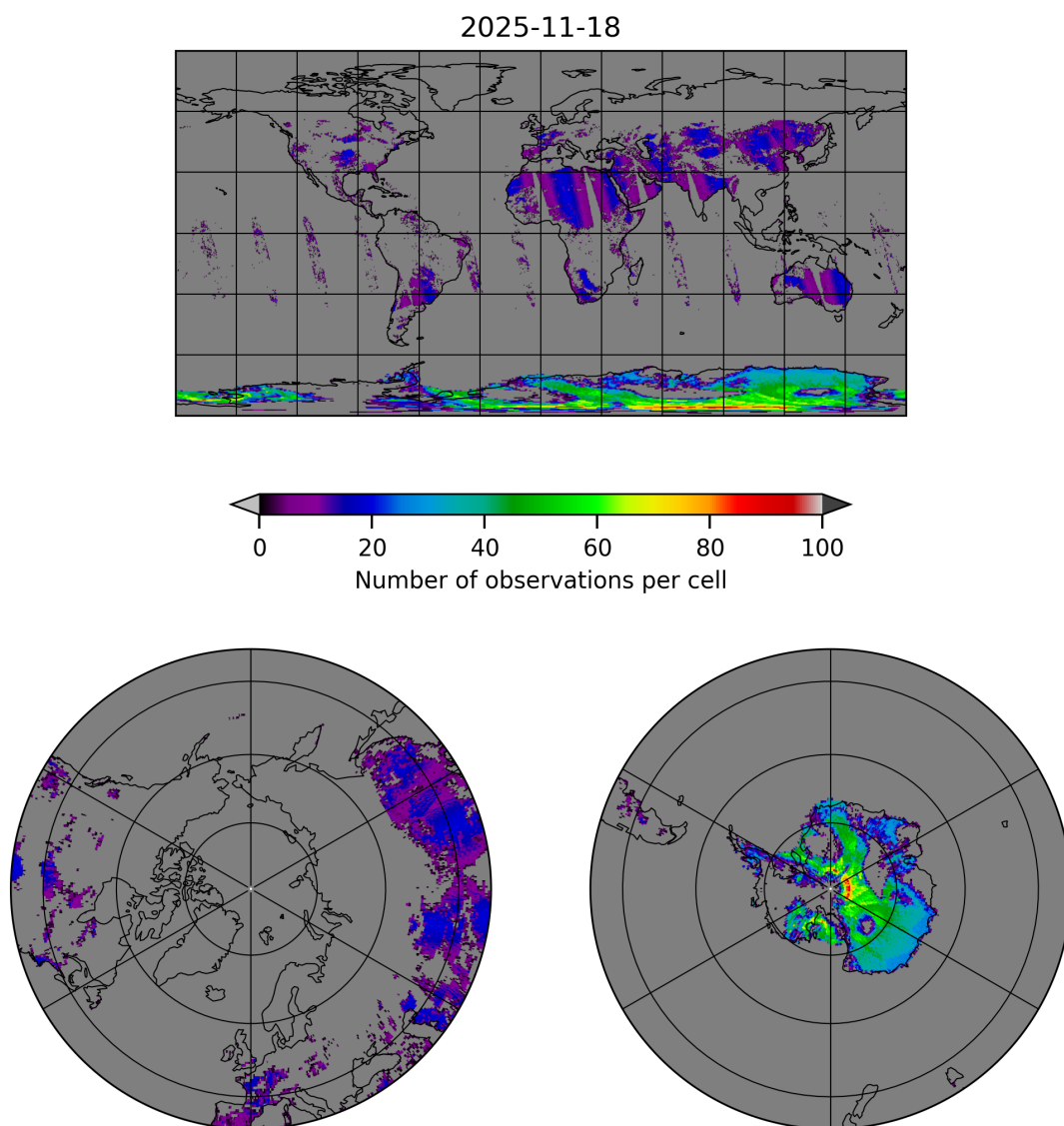
Figure 10: Map of the number of observations for 2025-11-18 to 2025-11-19
