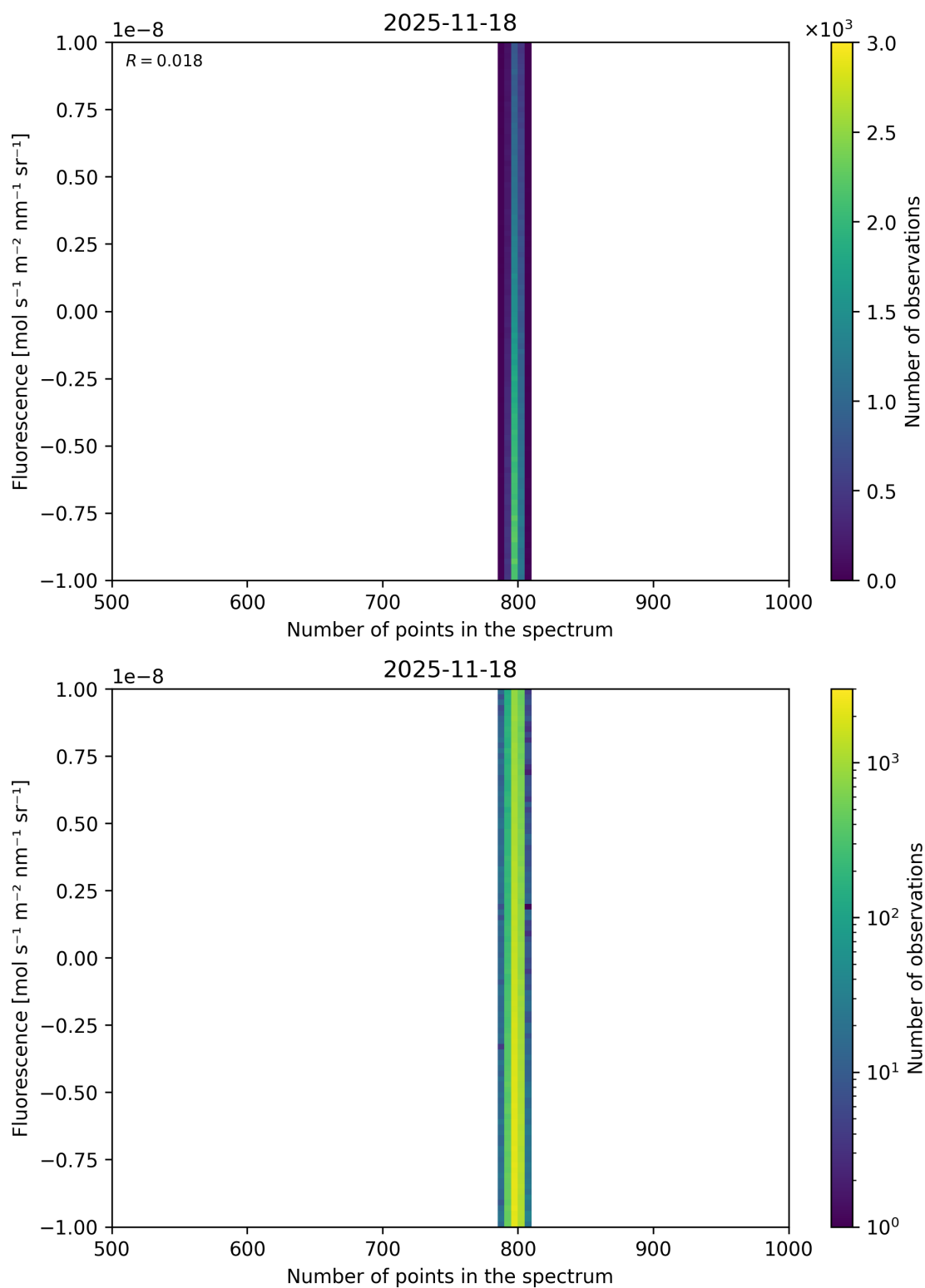
Figure 91: Scatter density plot of “Number of points in the spectrum” against “Fluorescence” for 2025-11-18 to 2025-11-19.
