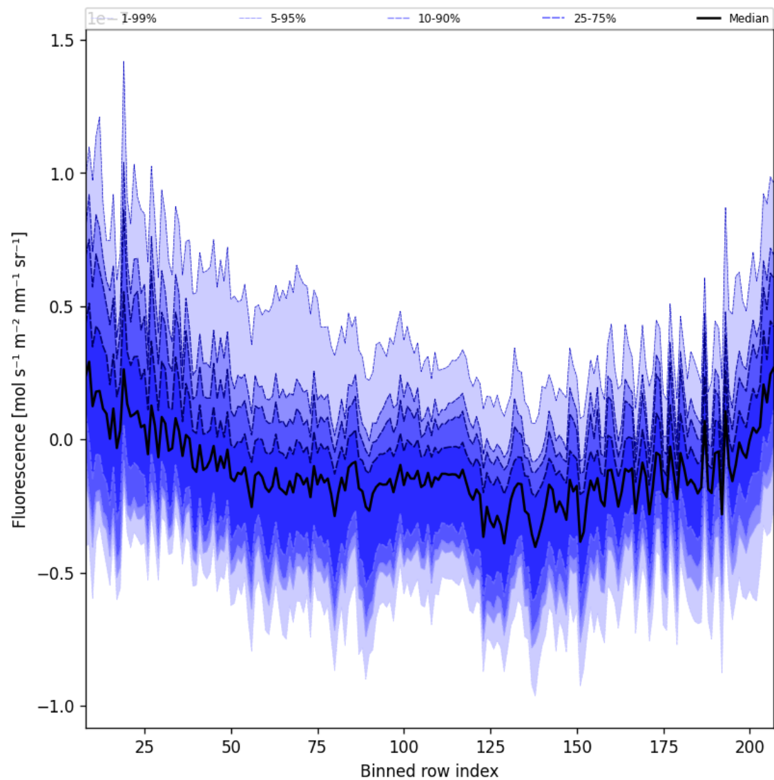
Figure 43: Along track statistics of "Fluorescence" for 2025-11-18 to 2025-11-19
