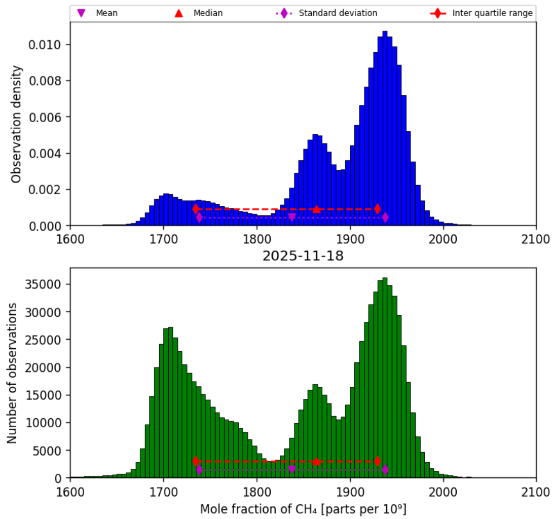
Figure 23: Histogram of “Mole fraction of CH 4 ” for 2025-11-18 to 2025-11-19
