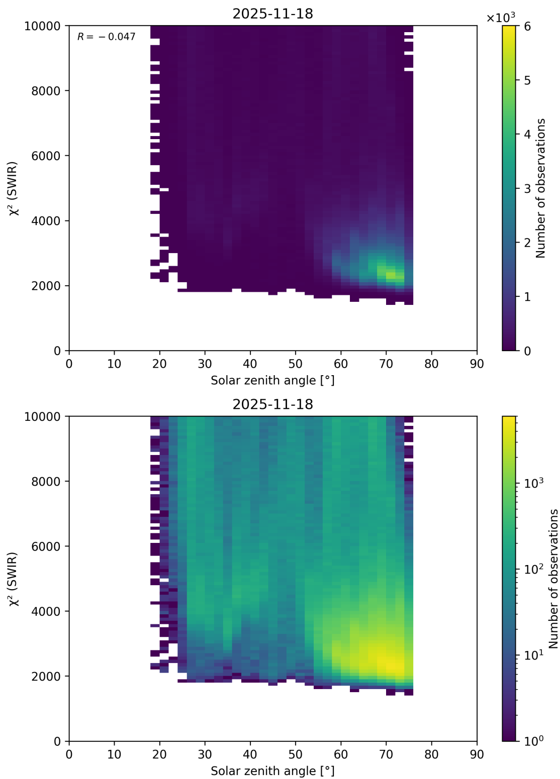
Figure 95: Scatter density plot of “Solar zenith angle” against “ \chi^2 (SWIR)” for 2025-11-18 to 2025-11-19.
