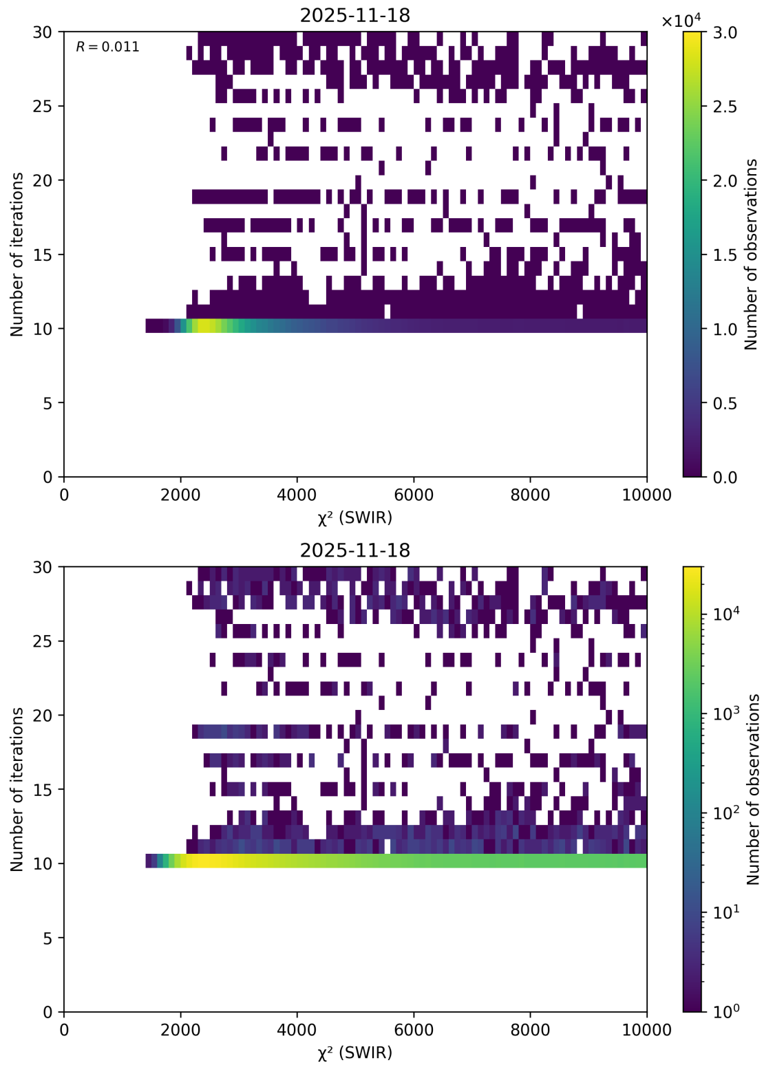
Figure 50: Scatter density plot of “ \chi^2 (SWIR)” against “Number of iterations” for 2025-11-18 to 2025-11-19.
