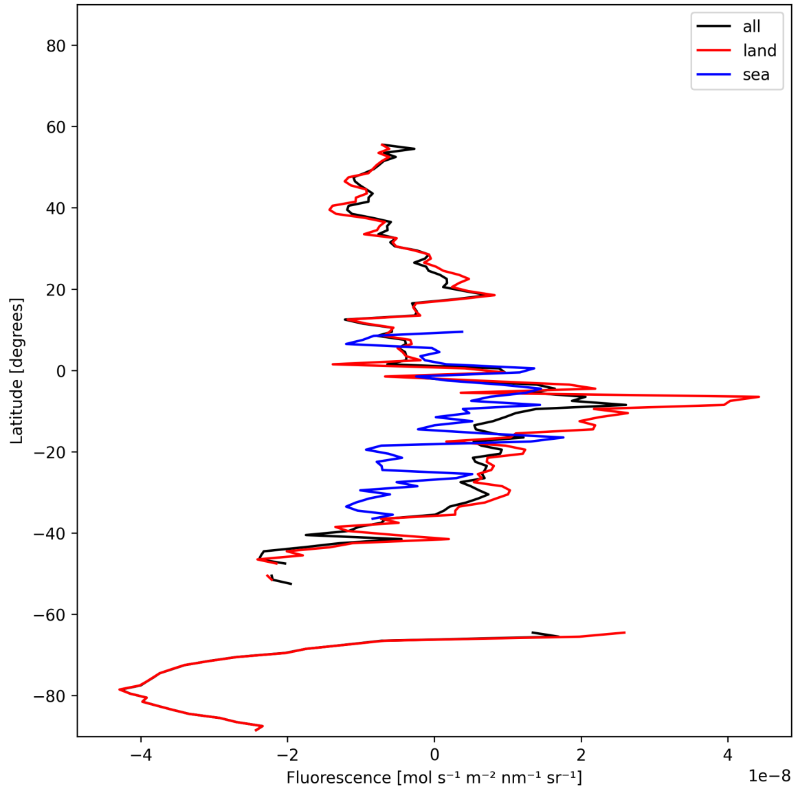
Figure 21: Zonal average of “Fluorescence” for 2025-11-18 to 2025-11-19.
