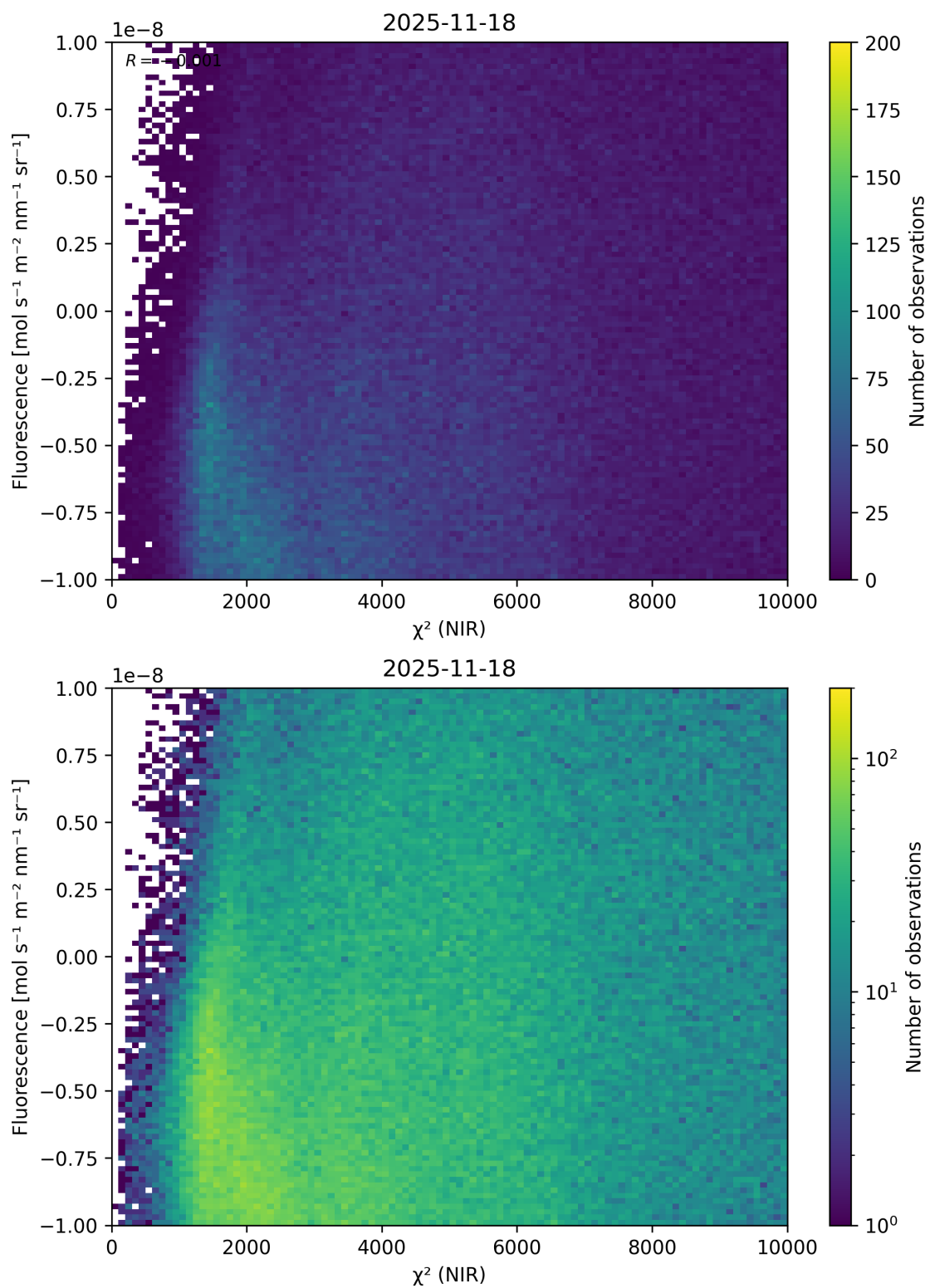
Figure 45: Scatter density plot of “ \chi^2 (NIR)” against “Fluorescence” for 2025-11-18 to 2025-11-19.
