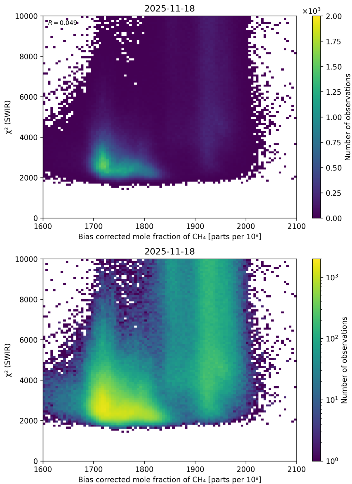
Figure 64: Scatter density plot of “Bias corrected mole fraction of CH 4 ” against “ \chi^2 (SWIR)” for 2025-11-18 to 2025-11-19.
