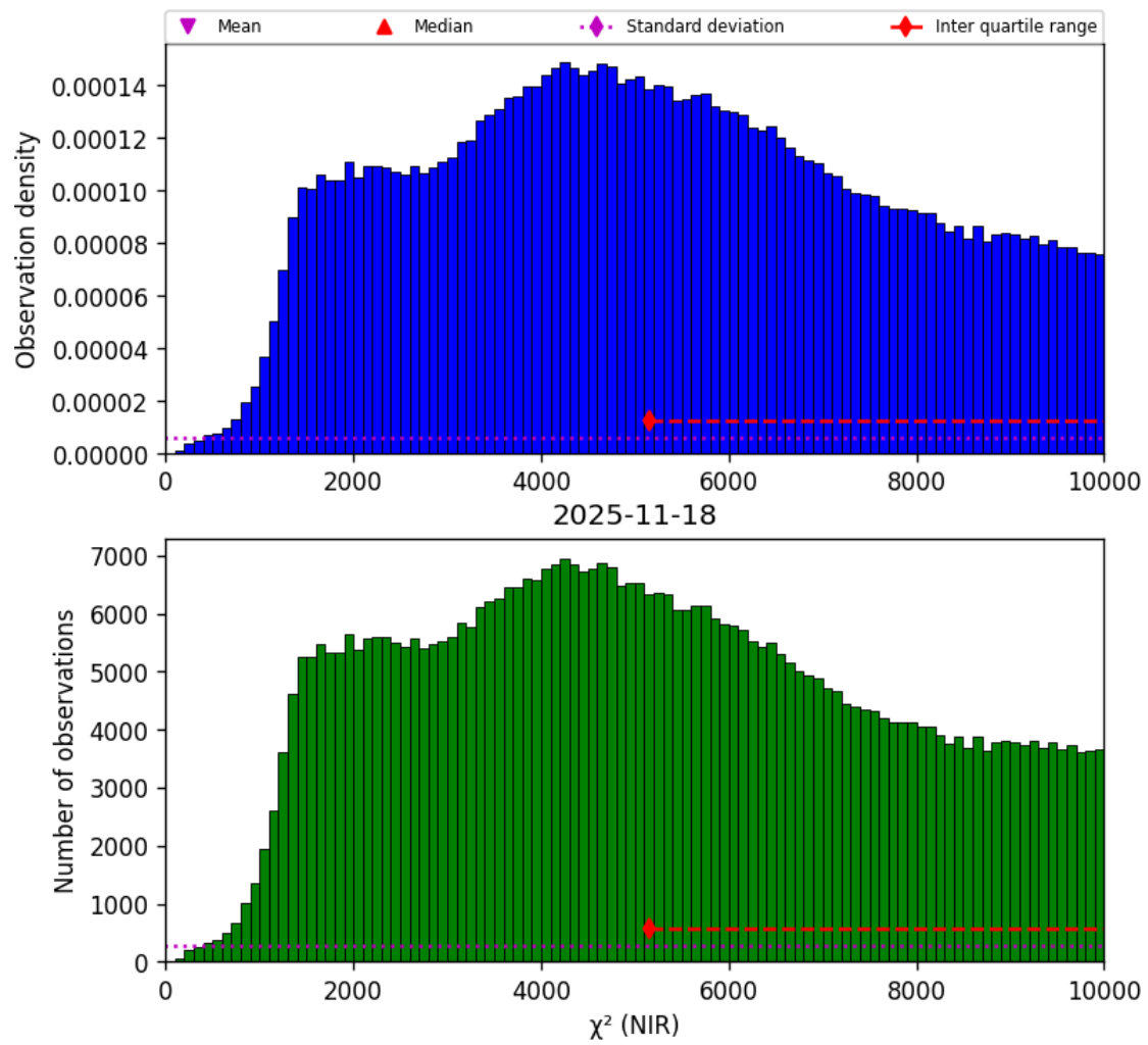
Figure 29: Histogram of “ \chi^2 (NIR)” for 2025-11-18 to 2025-11-19
