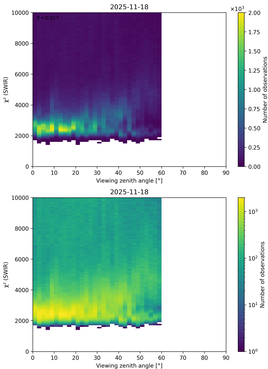
Figure 106: Scatter density plot of “Viewing zenith angle” against “ \chi^2 (SWIR)” for 2025-11-18 to 2025-11-19.
