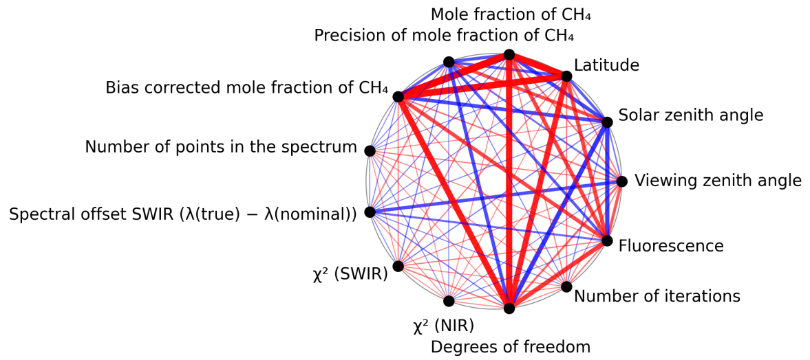
Figure 1: Map of correlation graph for 2025-11-18 to 2025-11-19.
