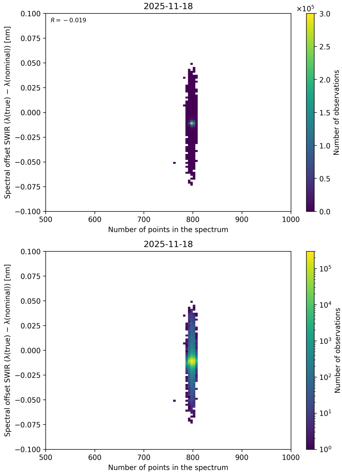
Figure 93: Scatter density plot of “Number of points in the spectrum” against “Spectral offset SWIR ( \lambda_{\text{true}} - \lambda_{\text{nominal}} )” for 2025-11-18 to 2025-11-19.
