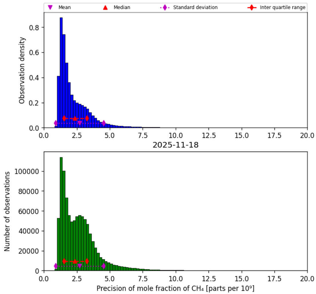
Figure 24: Histogram of “Precision of mole fraction of CH 4 ” for 2025-11-18 to 2025-11-19
