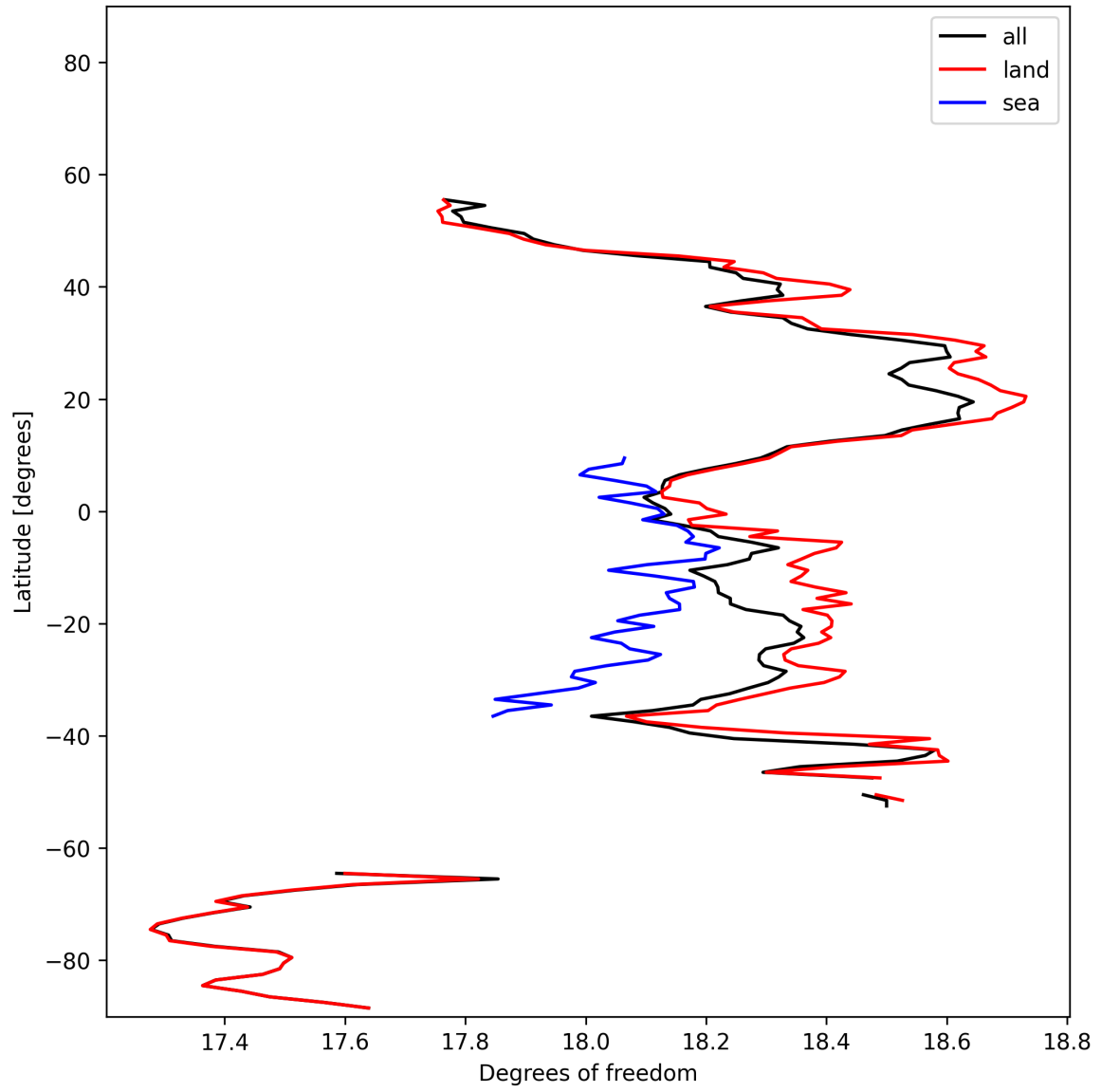
Figure 19: Zonal average of “Degrees of freedom” for 2025-11-18 to 2025-11-19.
