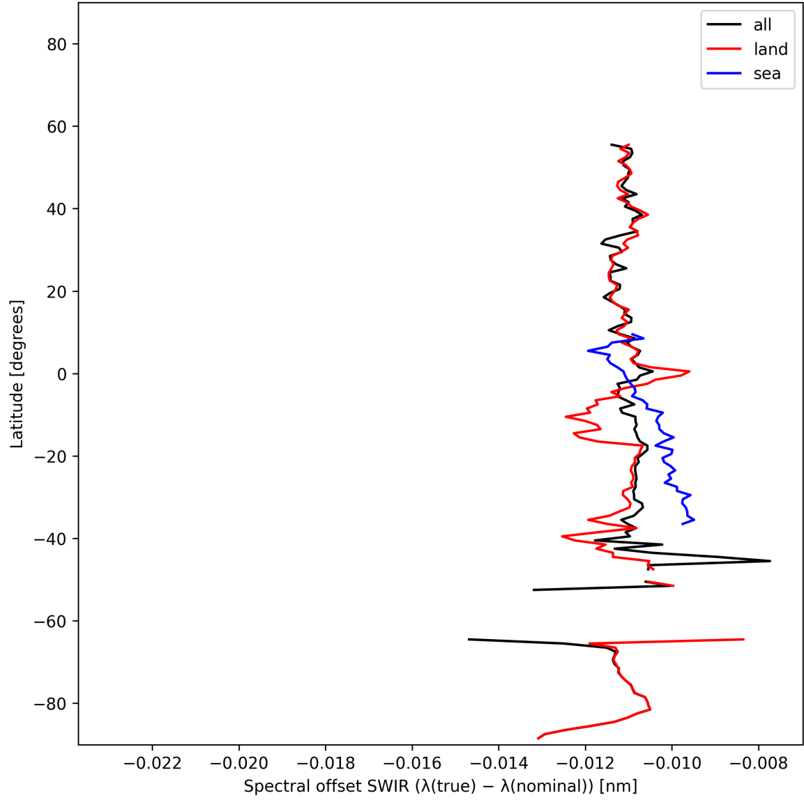
Figure 16: Zonal average of “Spectral offset SWIR ( \lambda_{\text{true}} - \lambda_{\text{nominal}} )” for 2025-11-18 to 2025-11-19.
