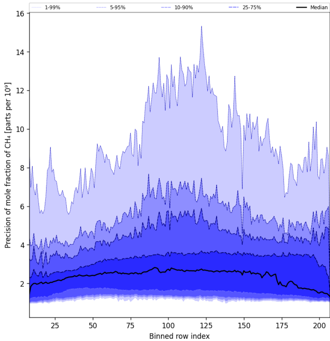
Figure 35: Along track statistics of “Precision of mole fraction of CH 4 ” for 2025-11-18 to 2025-11-19
