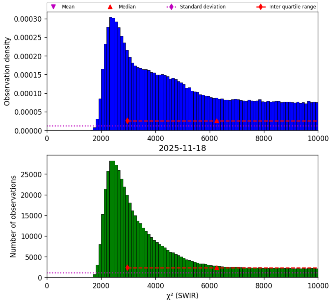
Figure 28: Histogram of “ \chi^2 (SWIR)” for 2025-11-18 to 2025-11-19
