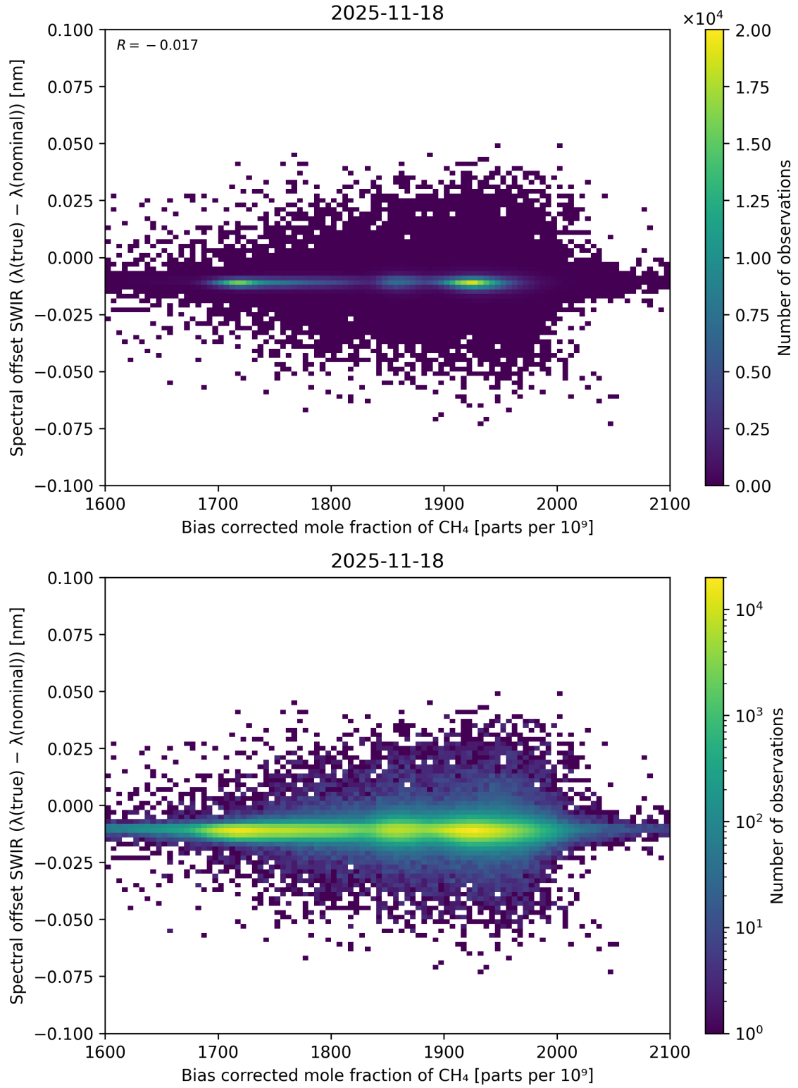
Figure 69: Scatter density plot of “Bias corrected mole fraction of \text{CH}_4 ” against “Spectral offset SWIR ( \lambda_{\text{true}} - \lambda_{\text{nominal}} )” for 2025-11-18 to 2025-11-19.
