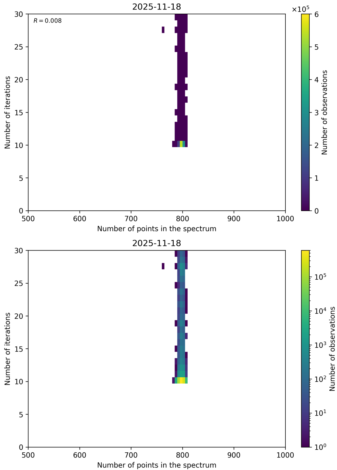
Figure 92: Scatter density plot of “Number of points in the spectrum” against “Number of iterations” for 2025-11-18 to 2025-11-19.
