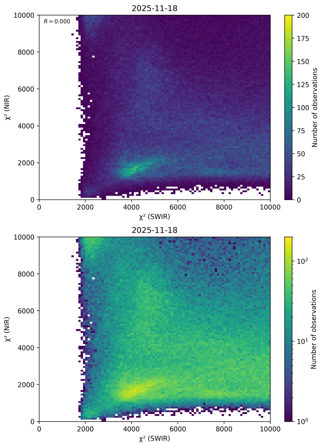
Figure 47: Scatter density plot of “ \chi^2 (SWIR)” against “ \chi^2 (NIR)” for 2025-11-18 to 2025-11-19.
