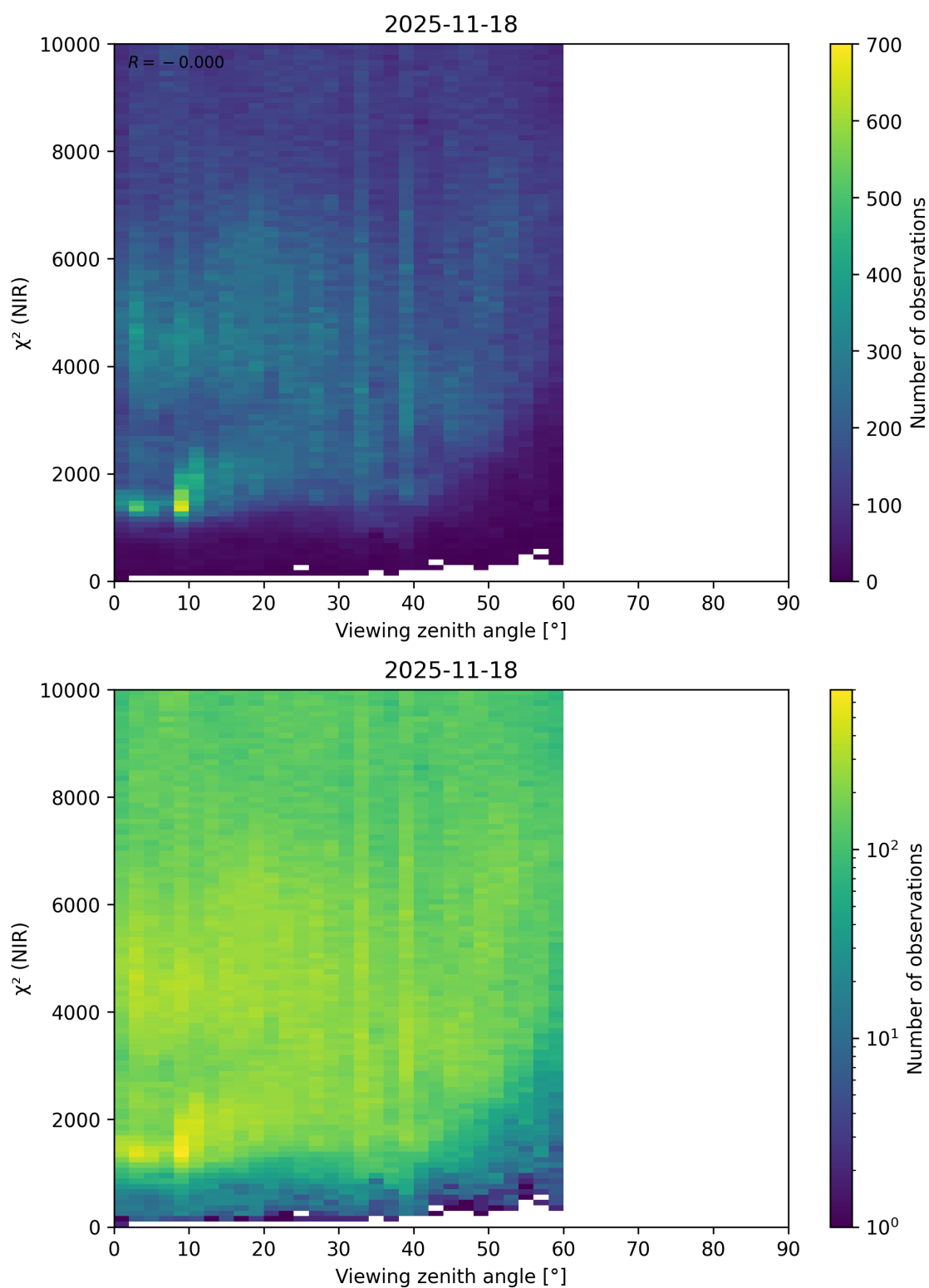
Figure 105: Scatter density plot of “Viewing zenith angle” against “ \chi^2 (NIR)” for 2025-11-18 to 2025-11-19.
