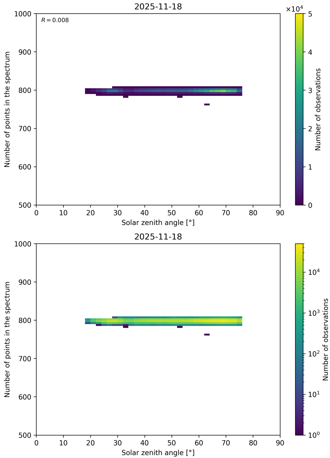
Figure 103: Scatter density plot of “Solar zenith angle” against “Number of points in the spectrum” for 2025-11-18 to 2025-11-19.
