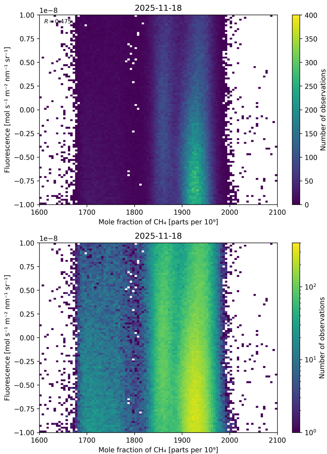
Figure 73: Scatter density plot of “Mole fraction of \text{CH}_4 ” against “Fluorescence” for 2025-11-18 to 2025-11-19.
