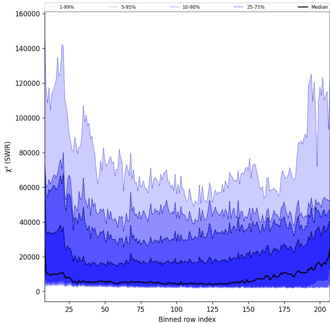
Figure 39: Along track statistics of “ \chi^2 (SWIR)” for 2025-11-18 to 2025-11-19
