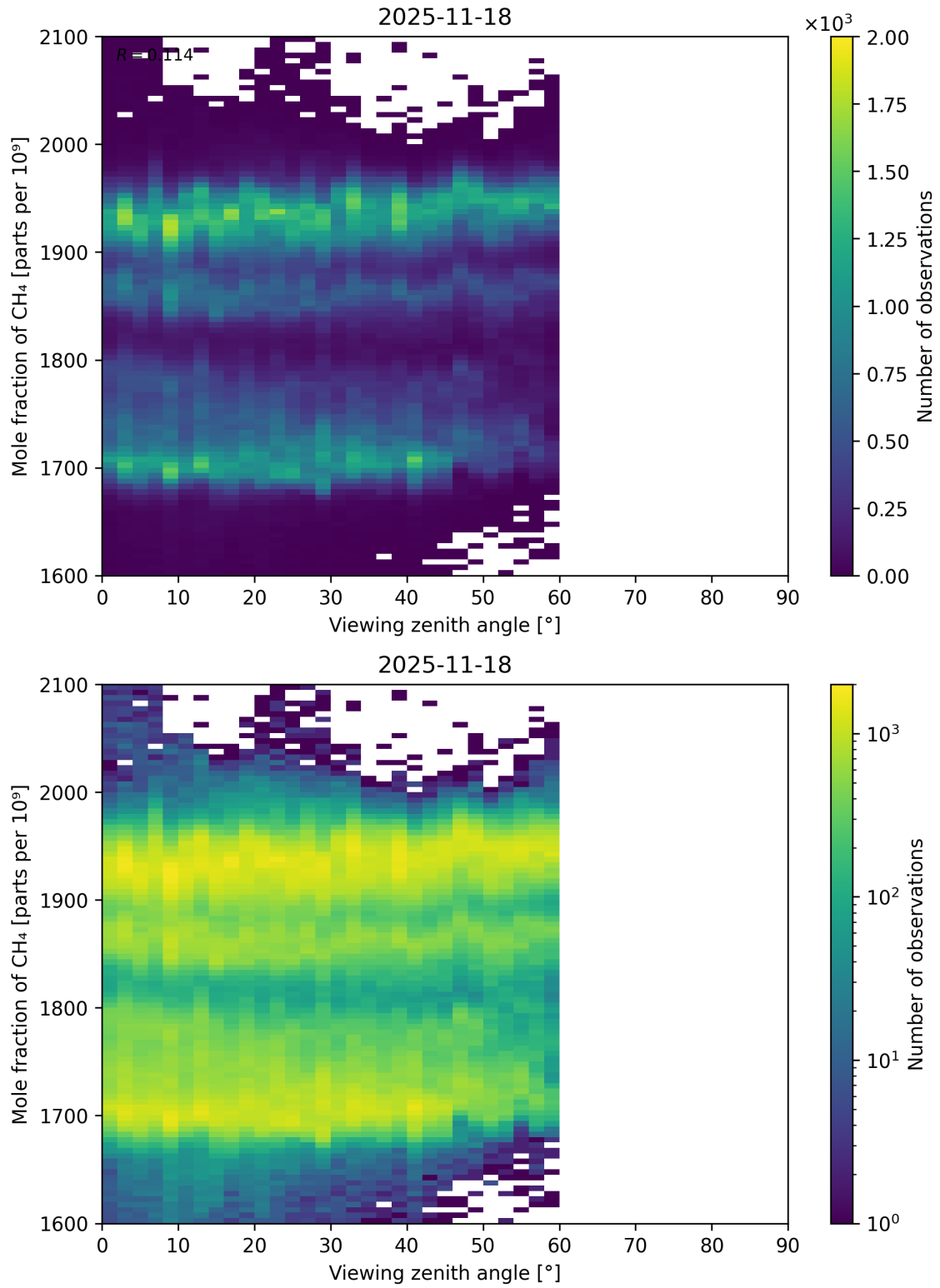
Figure 110: Scatter density plot of “Viewing zenith angle” against “Mole fraction of CH 4 ” for 2025-11-18 to 2025-11-19.
