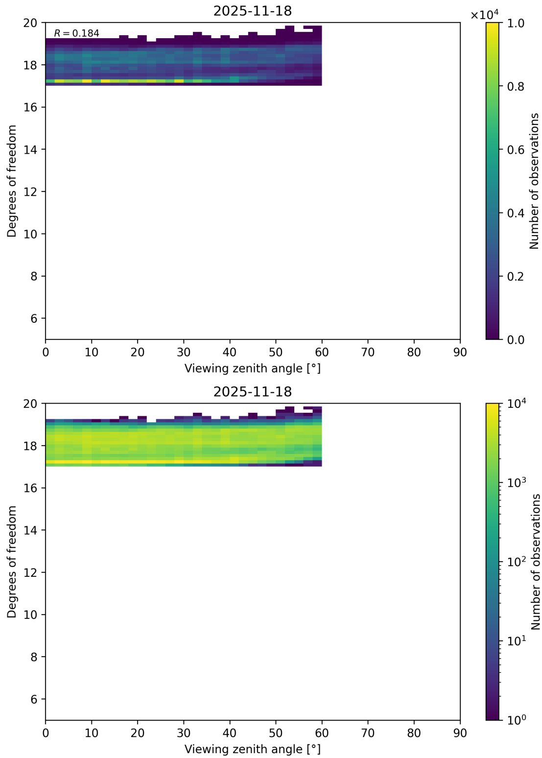
Figure 107: Scatter density plot of “Viewing zenith angle” against “Degrees of freedom” for 2025-11-18 to 2025-11-19.
