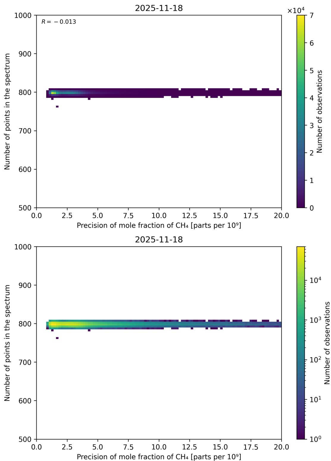
Figure 84: Scatter density plot of “Precision of mole fraction of CH 4 ” against “Number of points in the spectrum” for 2025-11-18 to 2025-11-19.
