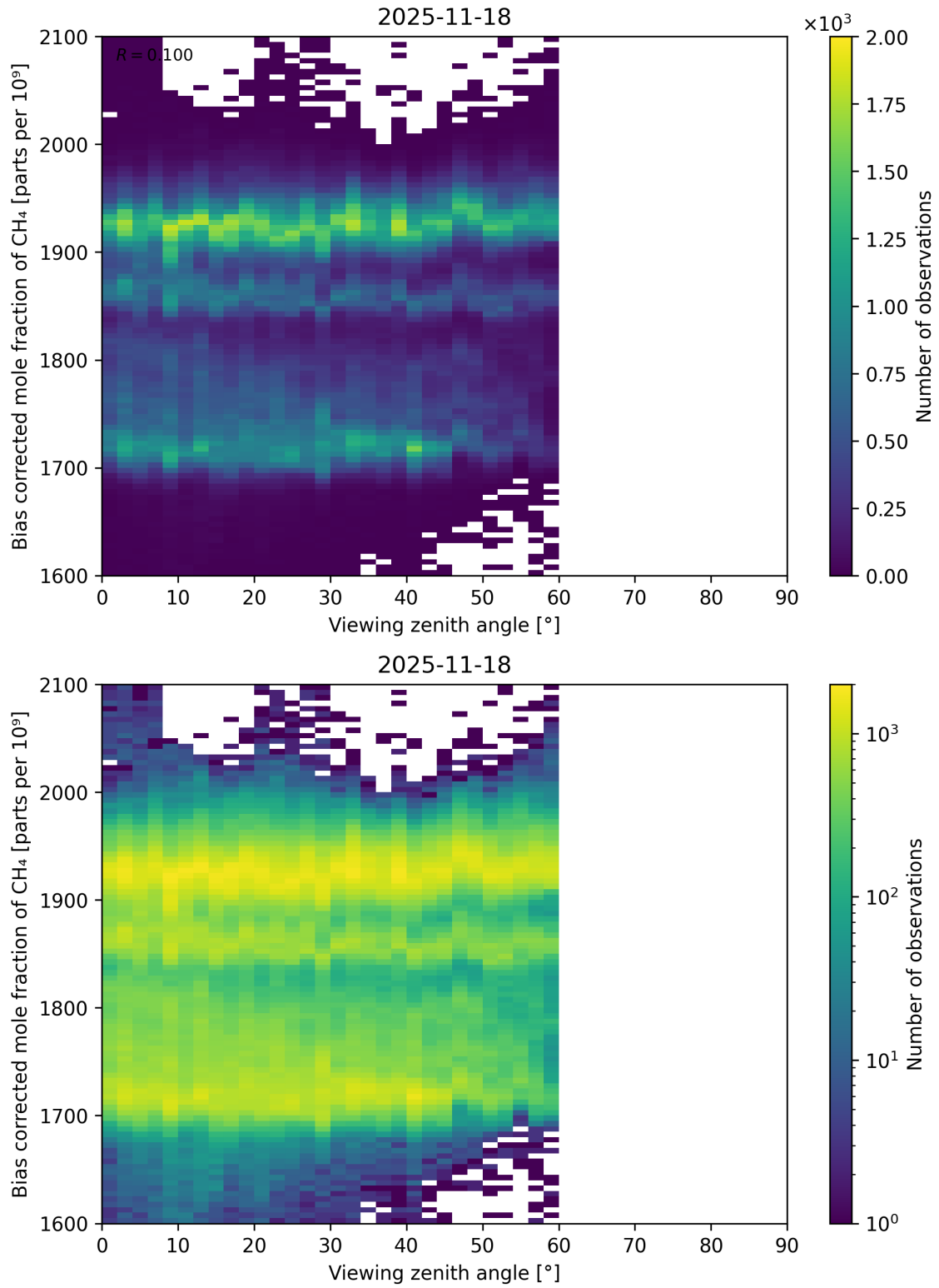
Figure 111: Scatter density plot of “Viewing zenith angle” against “Bias corrected mole fraction of CH 4 ” for 2025-11-18 to 2025-11-19.
