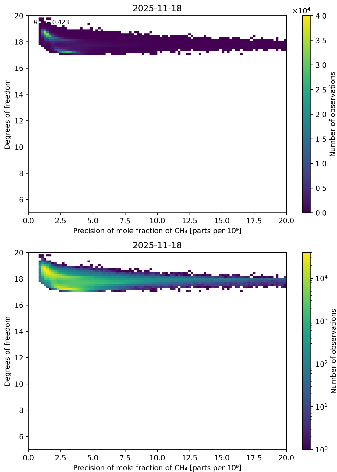
Figure 80: Scatter density plot of “Precision of mole fraction of CH 4 ” against “Degrees of freedom” for 2025-11-18 to 2025-11-19.
