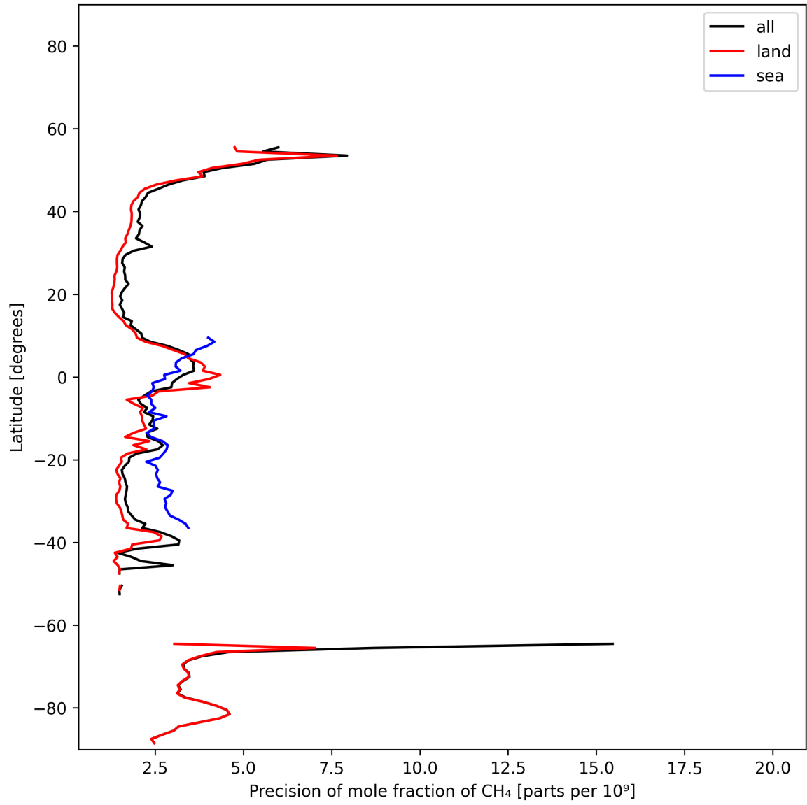
Figure 13: Zonal average of “Precision of mole fraction of CH 4 ” for 2025-11-18 to 2025-11-19.
