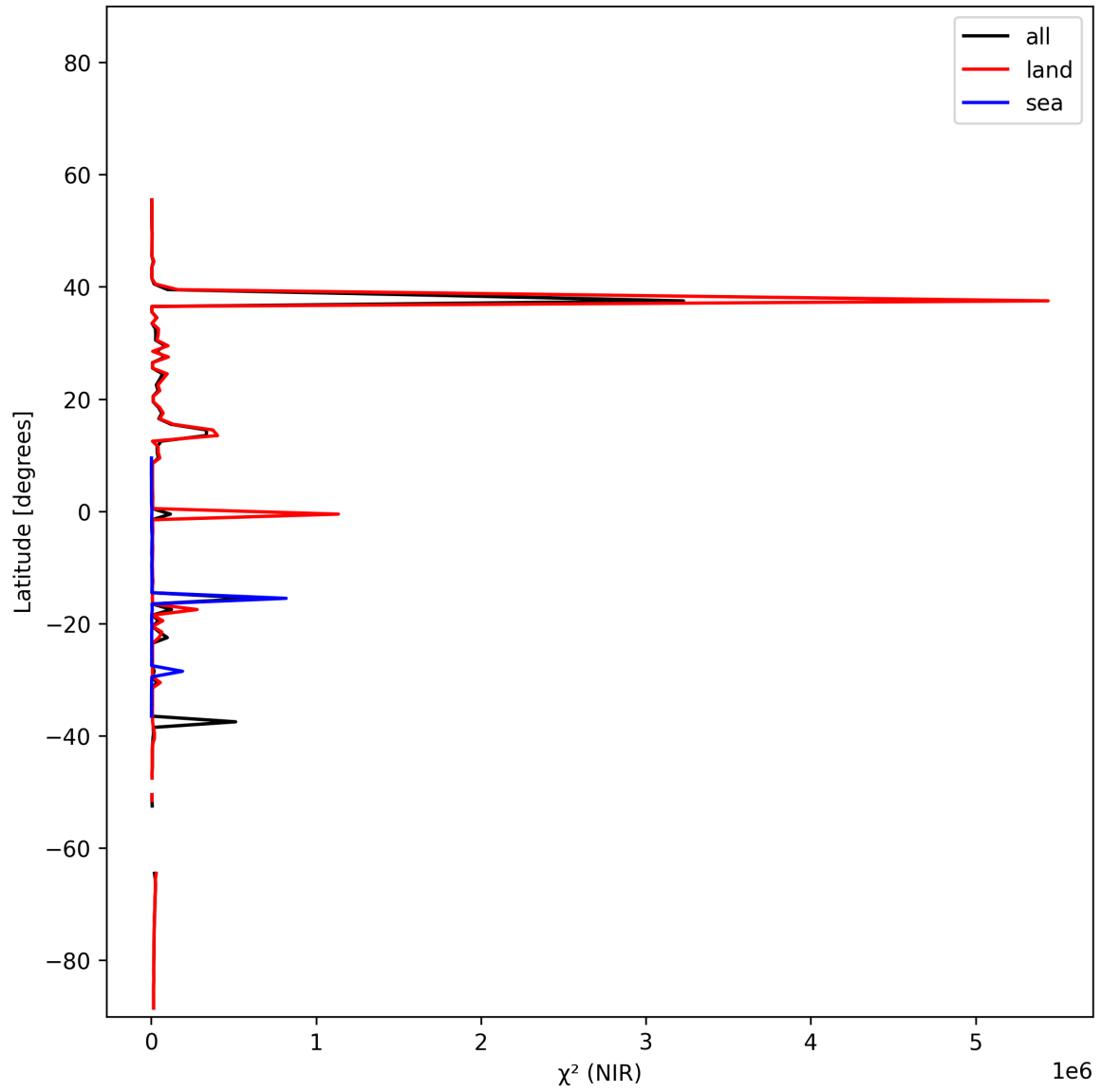
Figure 18: Zonal average of “ \chi^2 (NIR)” for 2025-11-18 to 2025-11-19.
