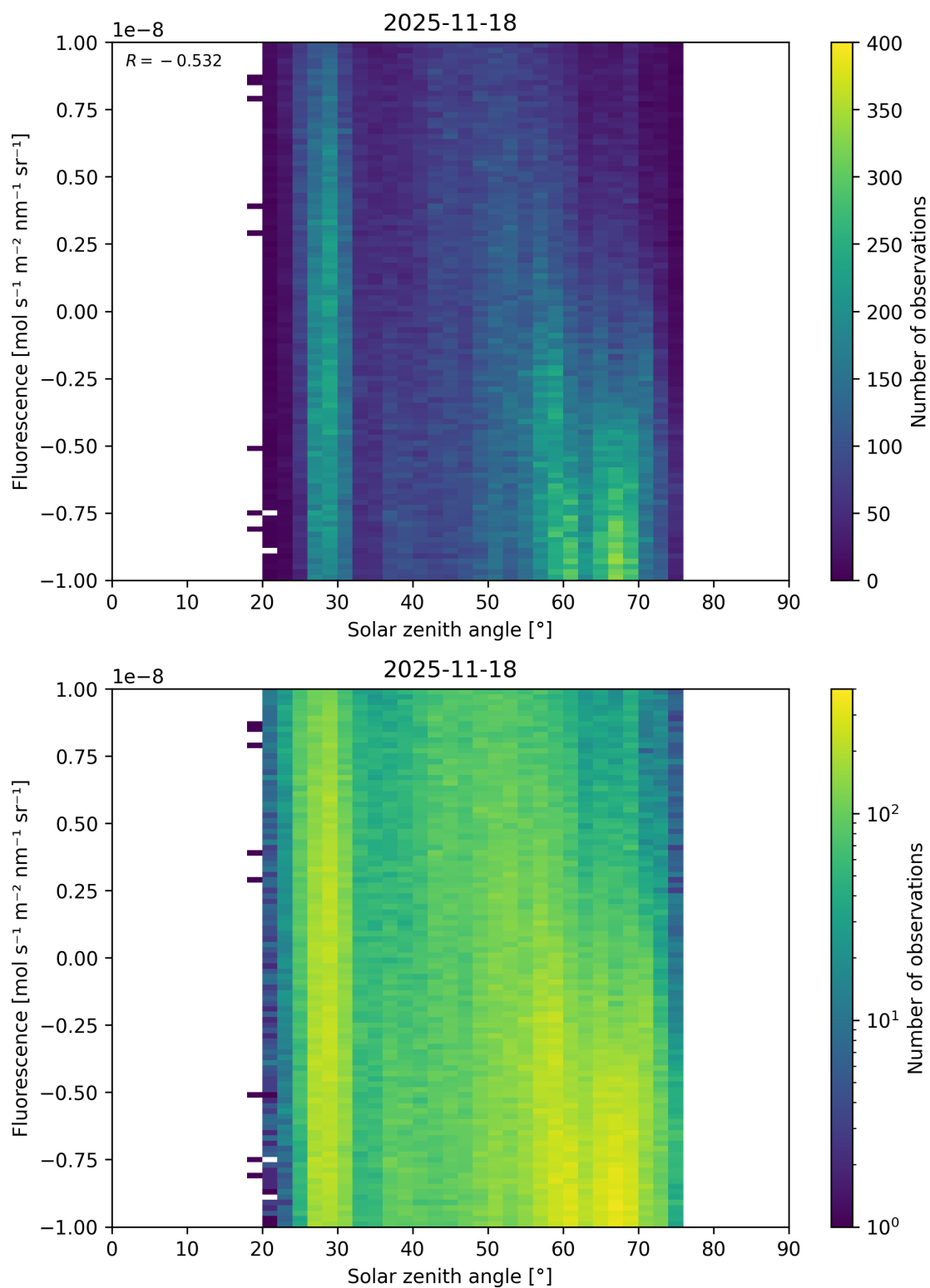
Figure 97: Scatter density plot of “Solar zenith angle” against “Fluorescence” for 2025-11-18 to 2025-11-19.
