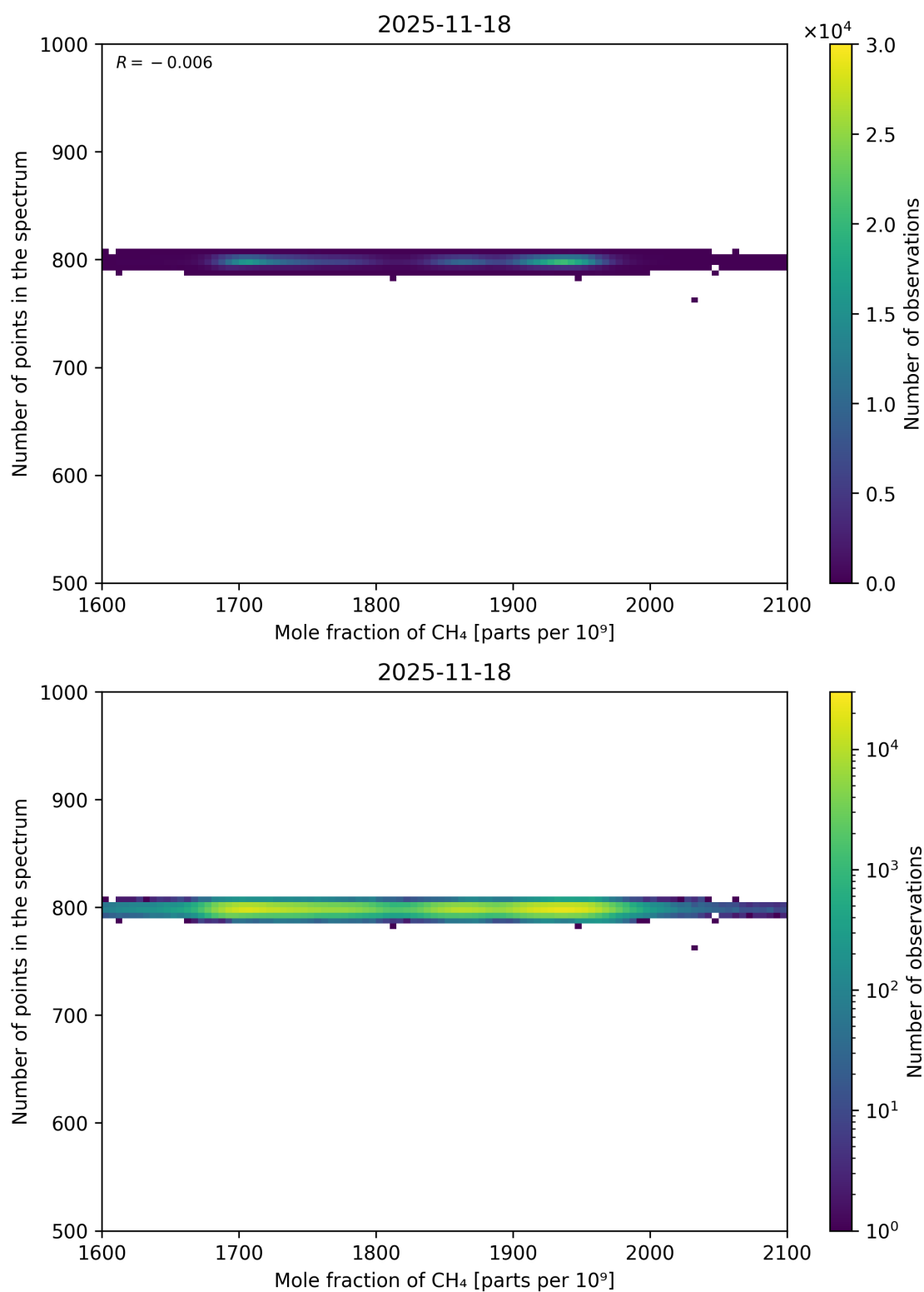
Figure 77: Scatter density plot of “Mole fraction of CH 4 ” against “Number of points in the spectrum” for 2025-11-18 to 2025-11-19.
