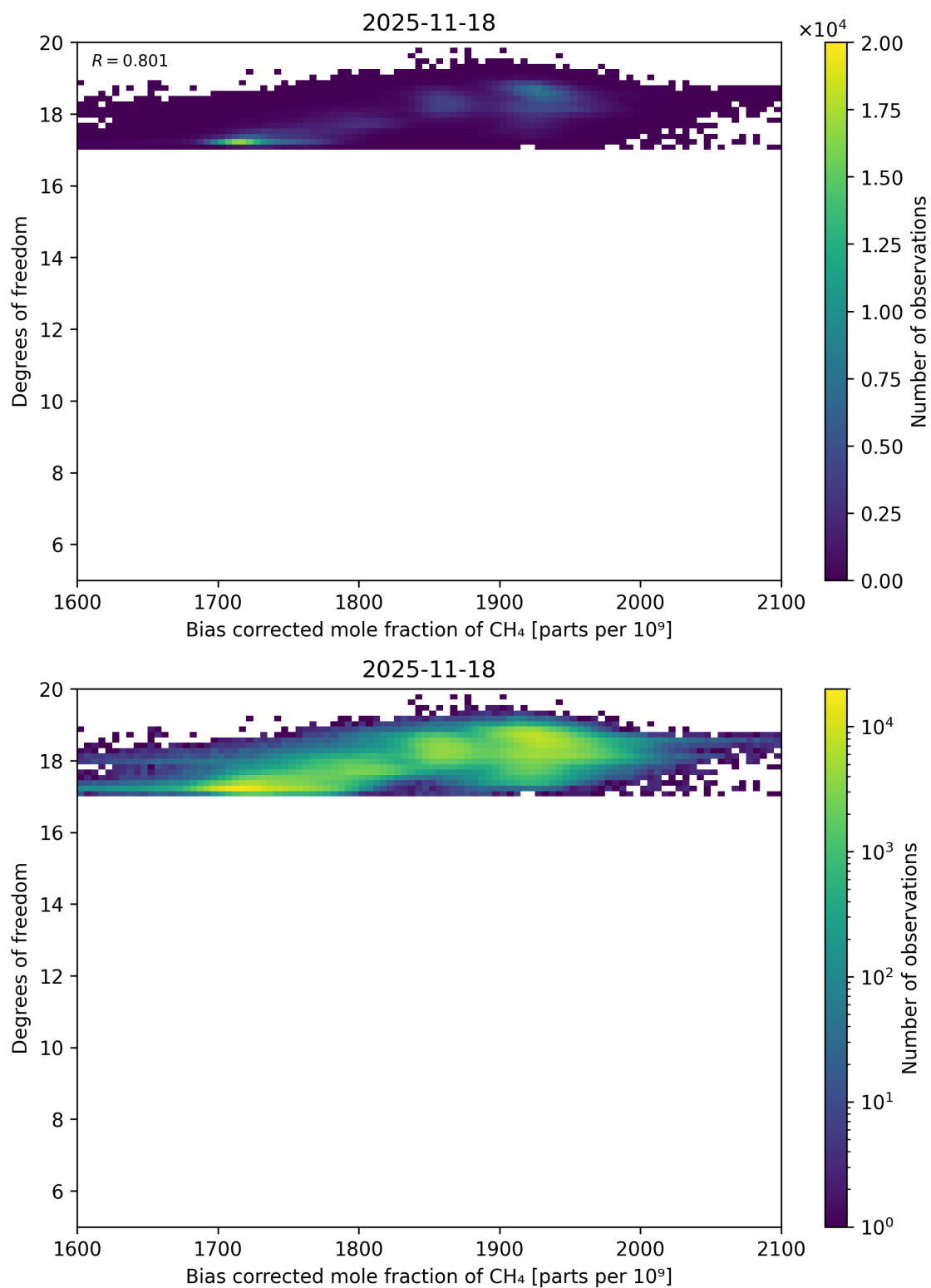
Figure 65: Scatter density plot of “Bias corrected mole fraction of \text{CH}_4 ” against “Degrees of freedom” for 2025-11-18 to 2025-11-19.
