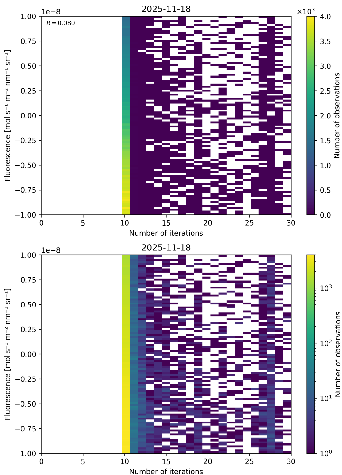
Figure 87: Scatter density plot of “Number of iterations” against “Fluorescence” for 2025-11-18 to 2025-11-19.
