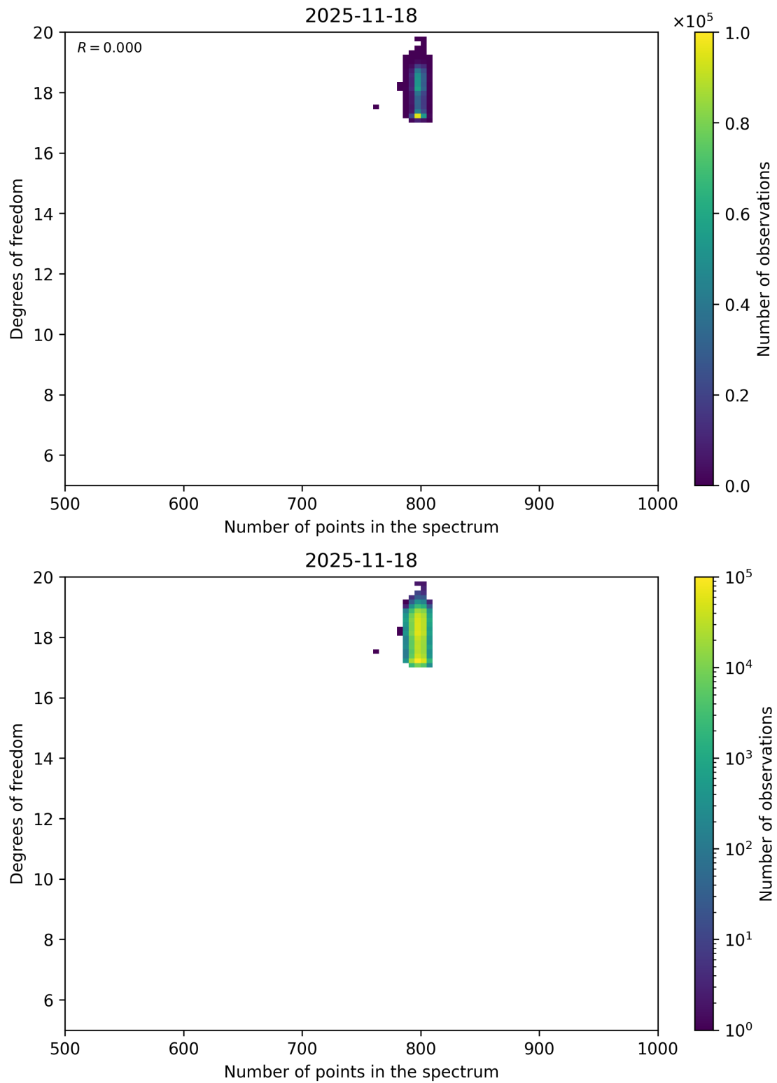
Figure 90: Scatter density plot of “Number of points in the spectrum” against “Degrees of freedom” for 2025-11-18 to 2025-11-19.
