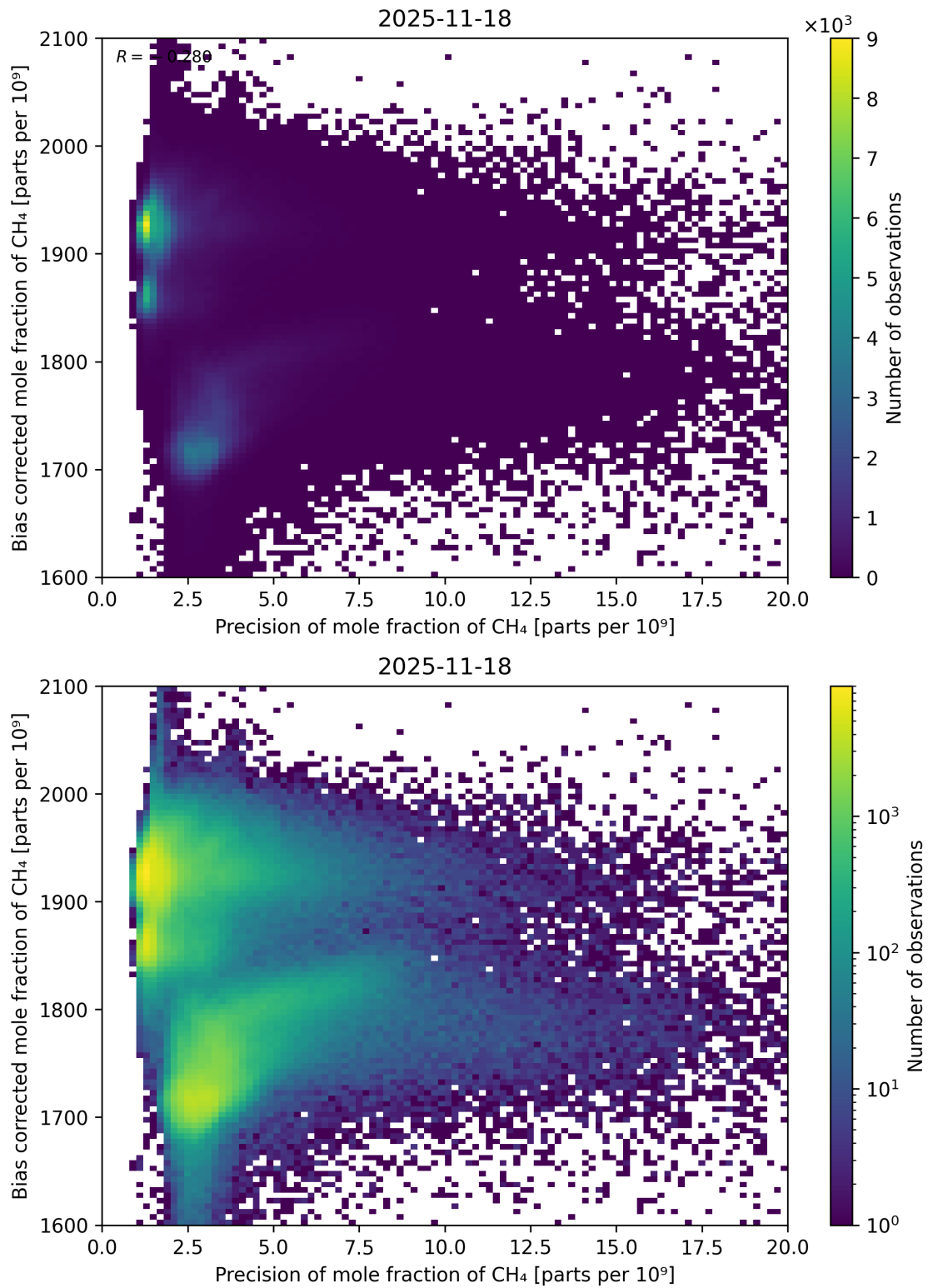
Figure 82: Scatter density plot of “Precision of mole fraction of CH 4 ” against “Bias corrected mole fraction of CH 4 ” for 2025-11-18 to 2025-11-19.
