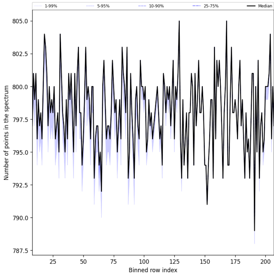
Figure 37: Along track statistics of “Number of points in the spectrum” for 2025-11-18 to 2025-11-19
