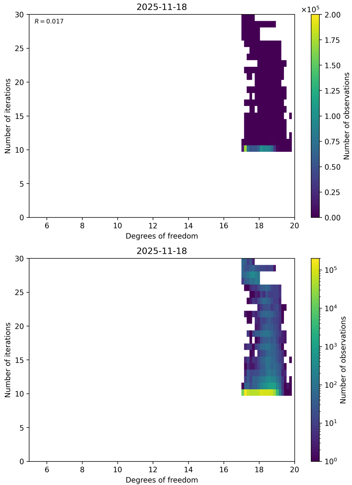
Figure 52: Scatter density plot of “Degrees of freedom” against “Number of iterations” for 2025-11-18 to 2025-11-19.
