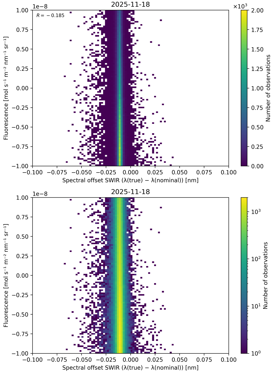
Figure 120: Scatter density plot of “Spectral offset SWIR ( \lambda_{\text{true}} - \lambda_{\text{nominal}} )” against “Fluorescence” for 2025-11-18 to 2025-11-19.
