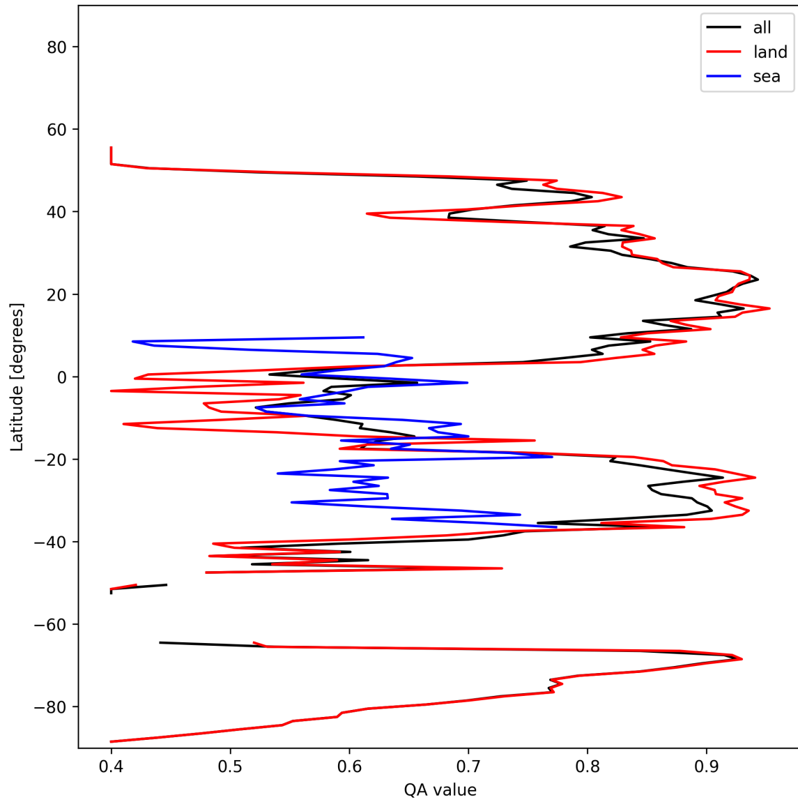
Figure 11: Zonal average of “QA value” for 2025-11-18 to 2025-11-19.
