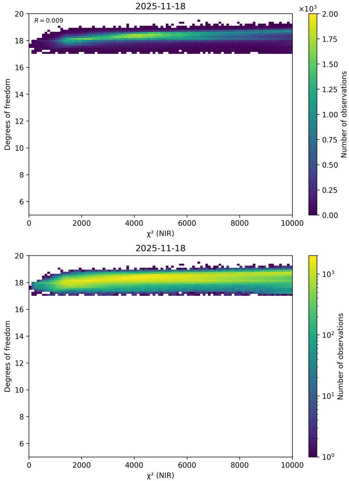
Figure 44: Scatter density plot of “ \chi^2 (NIR)” against “Degrees of freedom” for 2025-11-18 to 2025-11-19.
