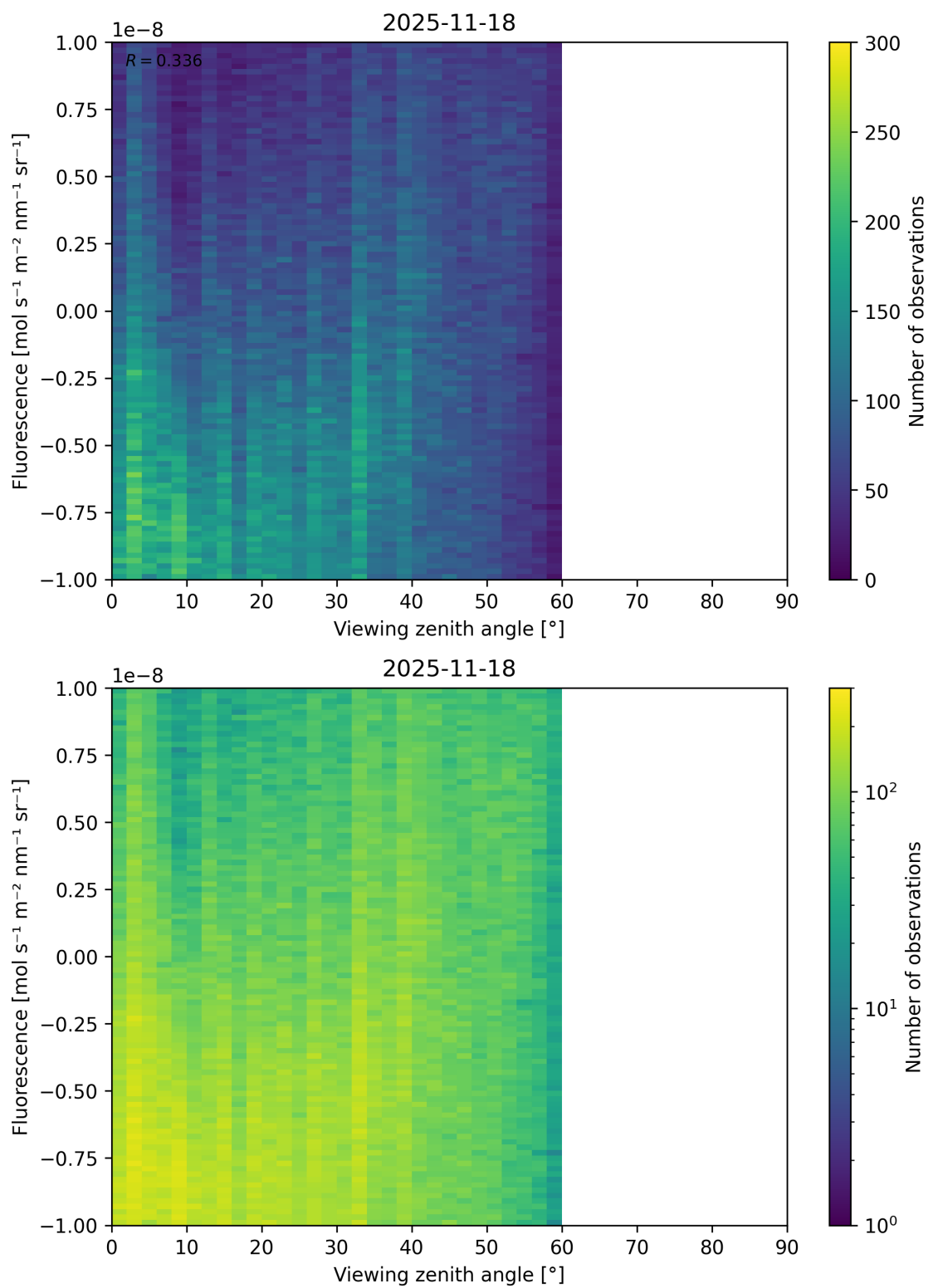
Figure 108: Scatter density plot of “Viewing zenith angle” against “Fluorescence” for 2025-11-18 to 2025-11-19.
