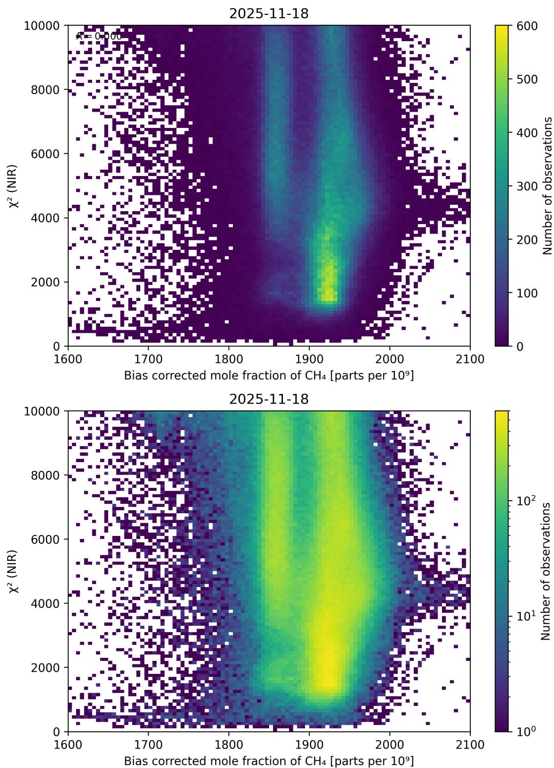
Figure 63: Scatter density plot of “Bias corrected mole fraction of \text{CH}_4 ” against “ \chi^2 (NIR)” for 2025-11-18 to 2025-11-19.
