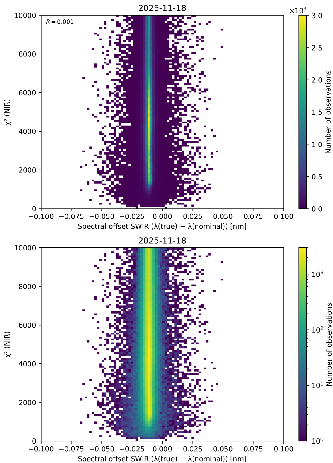
Figure 117: Scatter density plot of “Spectral offset SWIR ( \lambda_{\text{true}} - \lambda_{\text{nominal}} )” against “ \chi^2 (NIR)” for 2025-11-18 to 2025-11-19.
