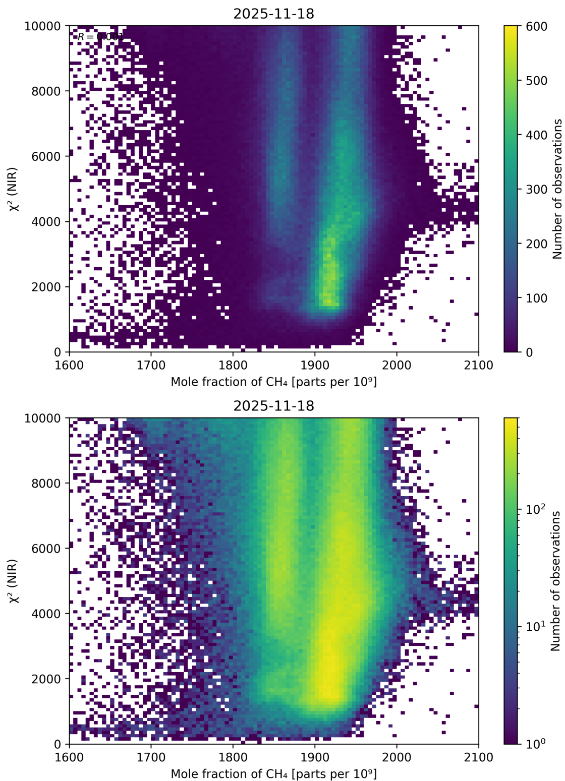
Figure 70: Scatter density plot of “Mole fraction of \text{CH}_4 ” against “ \chi^2 (NIR)” for 2025-11-18 to 2025-11-19.
