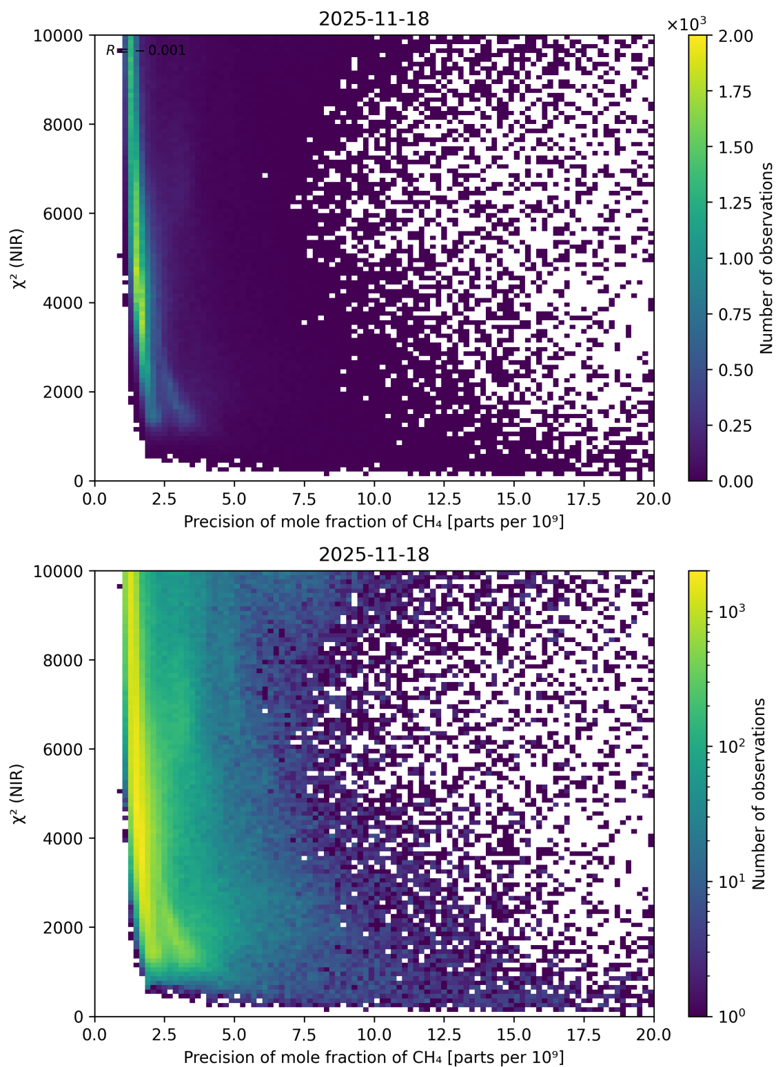
Figure 78: Scatter density plot of “Precision of mole fraction of CH 4 ” against “ \chi^2 (NIR)” for 2025-11-18 to 2025-11-19.
