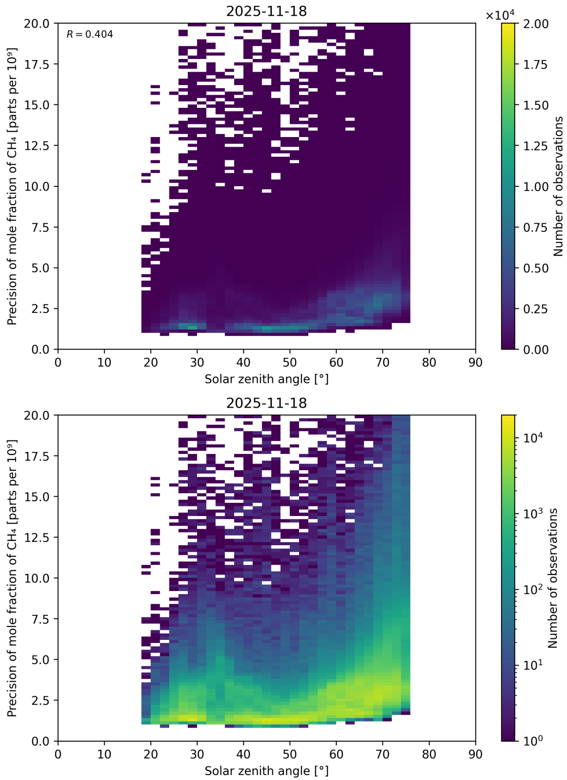
Figure 101: Scatter density plot of “Solar zenith angle” against “Precision of mole fraction of \text{CH}_4 ” for 2025-11-18 to 2025-11-19.
