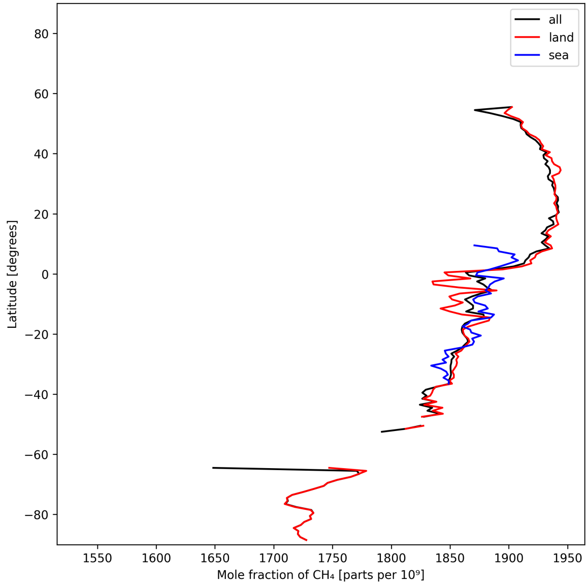
Figure 12: Zonal average of “Mole fraction of CH 4 ” for 2025-11-18 to 2025-11-19.
