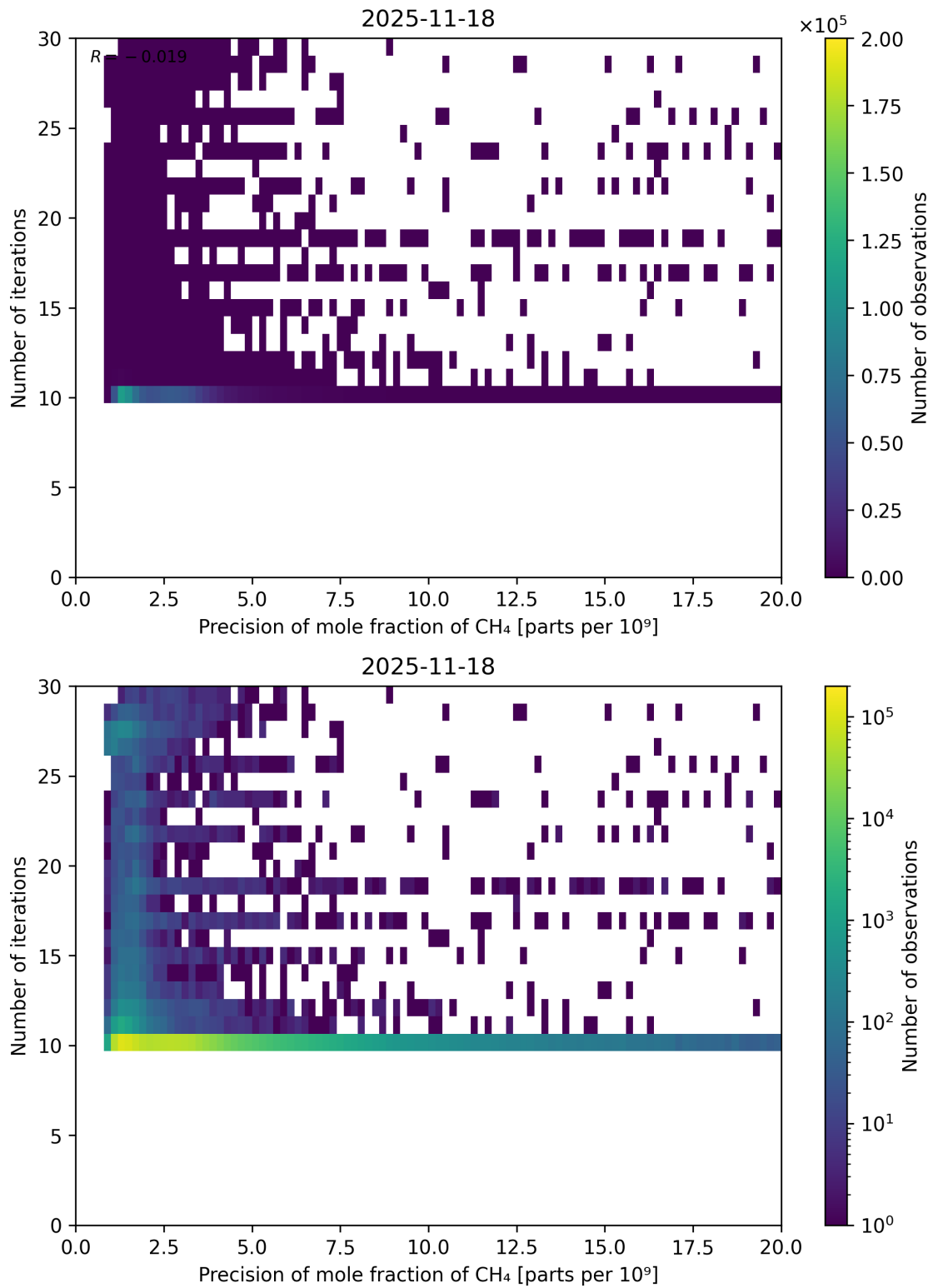
Figure 83: Scatter density plot of “Precision of mole fraction of CH 4 ” against “Number of iterations” for 2025-11-18 to 2025-11-19.
