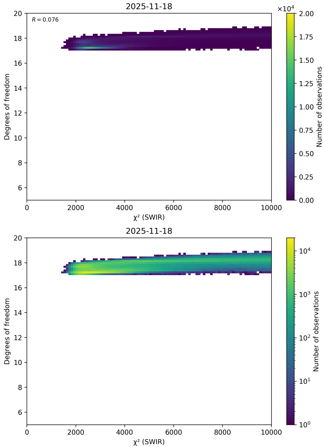
Figure 48: Scatter density plot of “ \chi^2 (SWIR)” against “Degrees of freedom” for 2025-11-18 to 2025-11-19.
