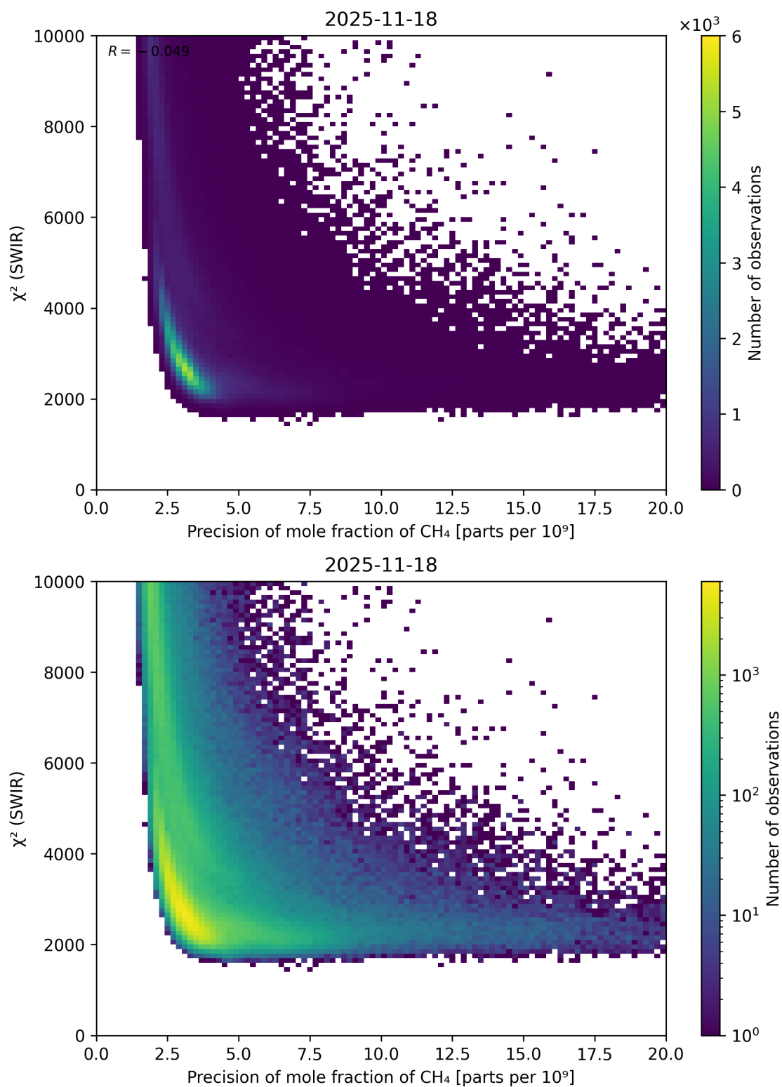
Figure 79: Scatter density plot of “Precision of mole fraction of \text{CH}_4 ” against “ \chi^2 (SWIR)” for 2025-11-18 to 2025-11-19.
