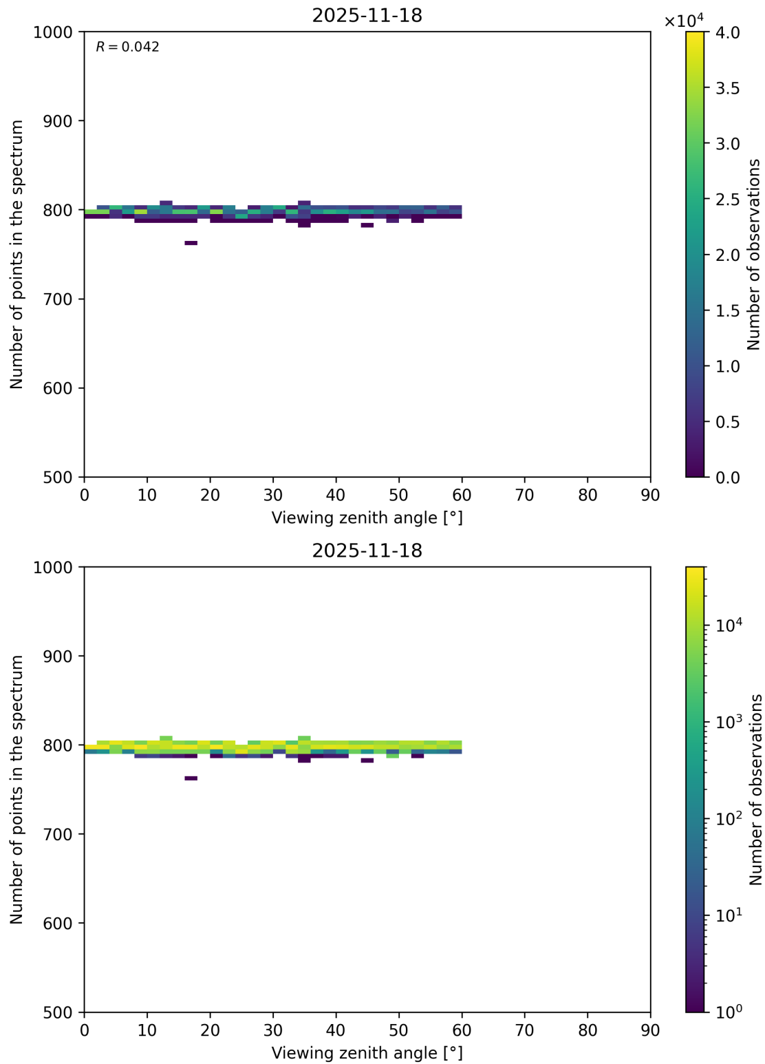
Figure 114: Scatter density plot of “Viewing zenith angle” against “Number of points in the spectrum” for 2025-11-18 to 2025-11-19.
