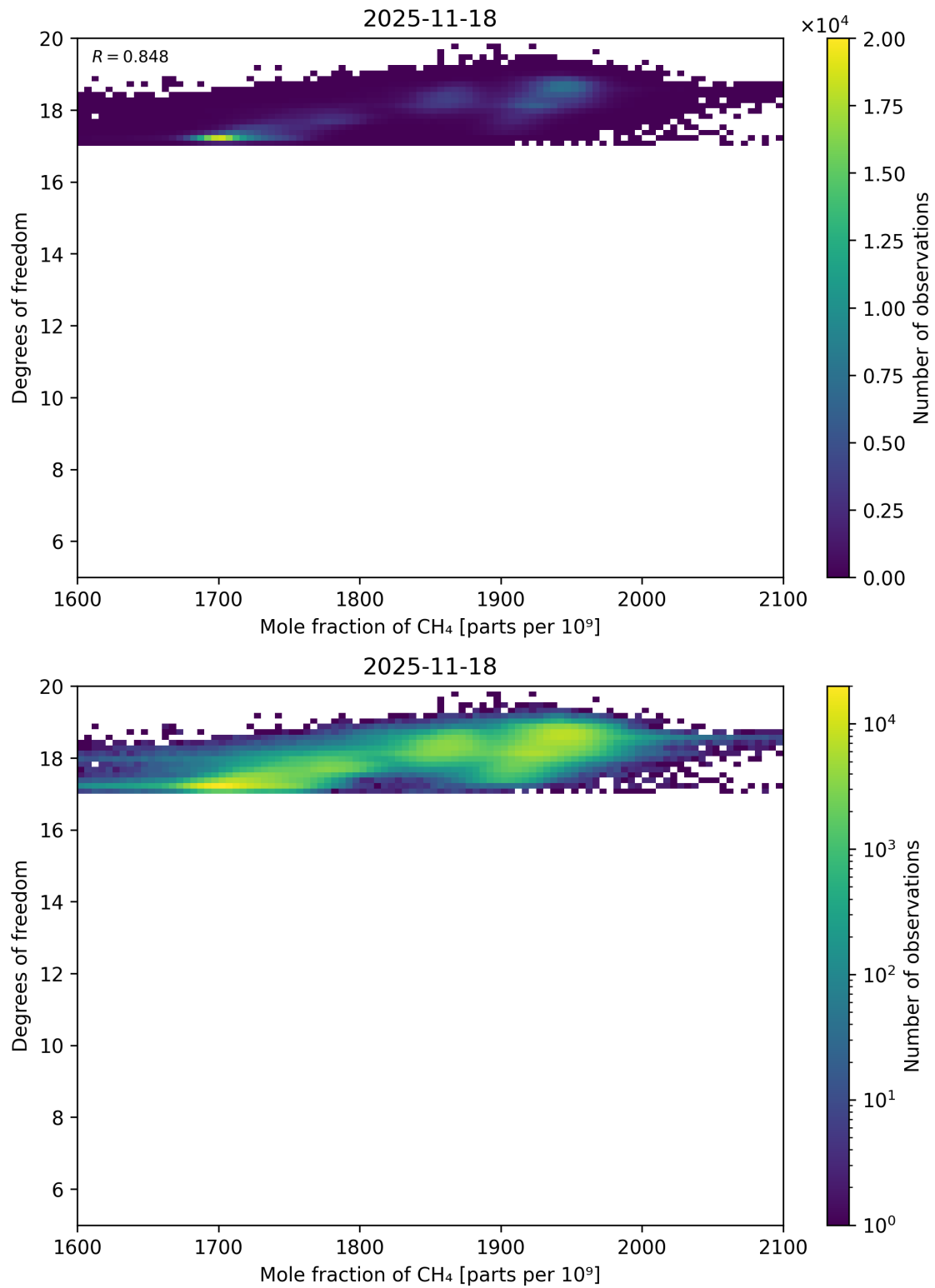
Figure 72: Scatter density plot of “Mole fraction of CH 4 ” against “Degrees of freedom” for 2025-11-18 to 2025-11-19.
