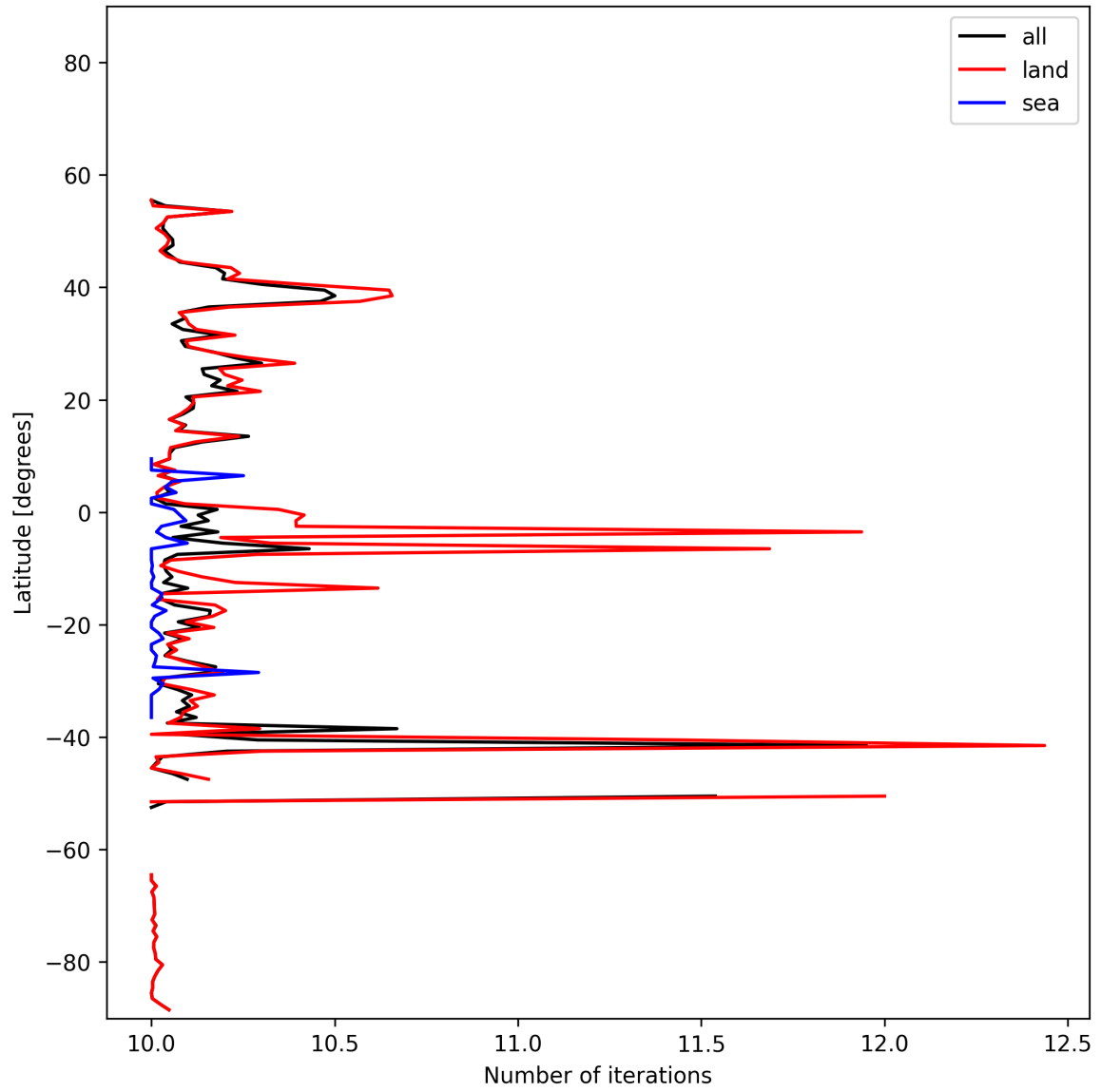
Figure 20: Zonal average of “Number of iterations” for 2025-11-18 to 2025-11-19.
