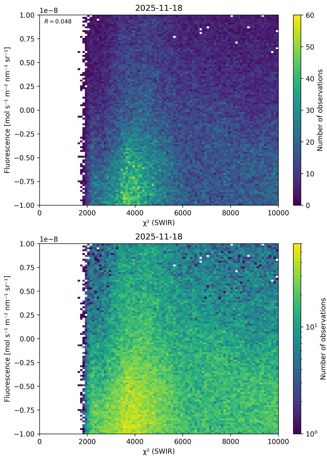
Figure 49: Scatter density plot of “ \chi^2 (SWIR)” against “Fluorescence” for 2025-11-18 to 2025-11-19.
