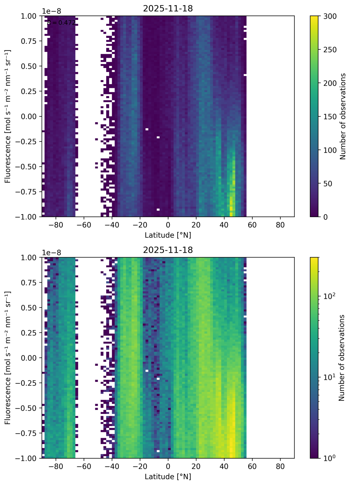
Figure 56: Scatter density plot of “Latitude” against “Fluorescence” for 2025-11-18 to 2025-11-19.
