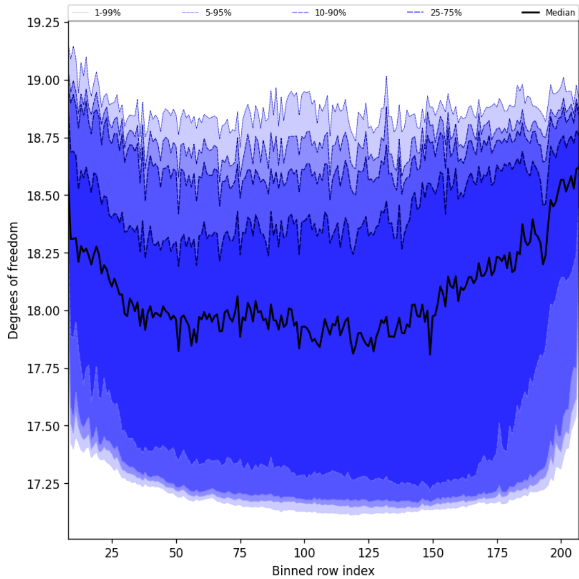
Figure 41: Along track statistics of “Degrees of freedom” for 2025-11-18 to 2025-11-19
