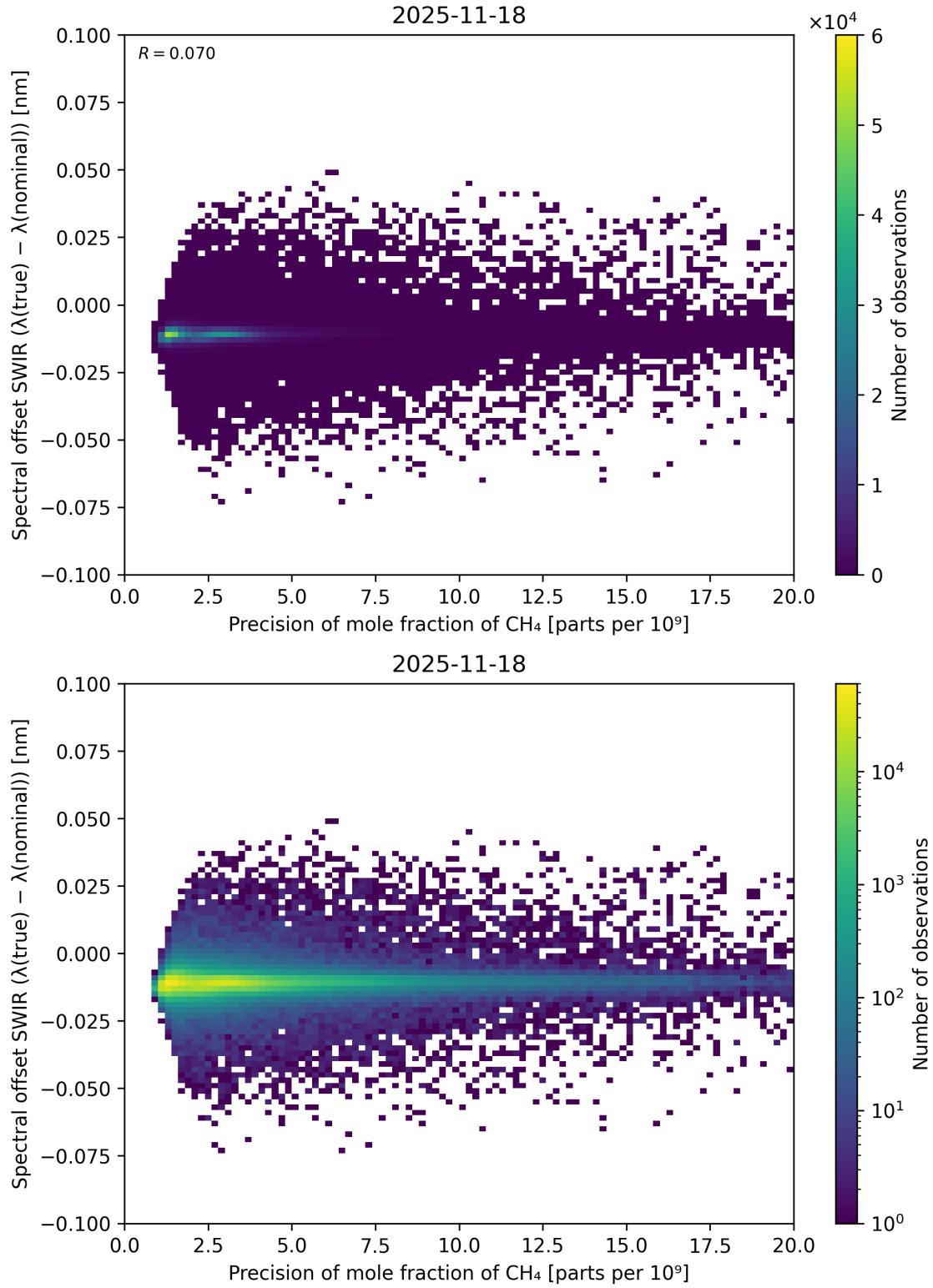
Figure 85: Scatter density plot of “Precision of mole fraction of \text{CH}_4 ” against “Spectral offset SWIR ( \lambda_{\text{true}} - \lambda_{\text{nominal}} )” for 2025-11-18 to 2025-11-19.
