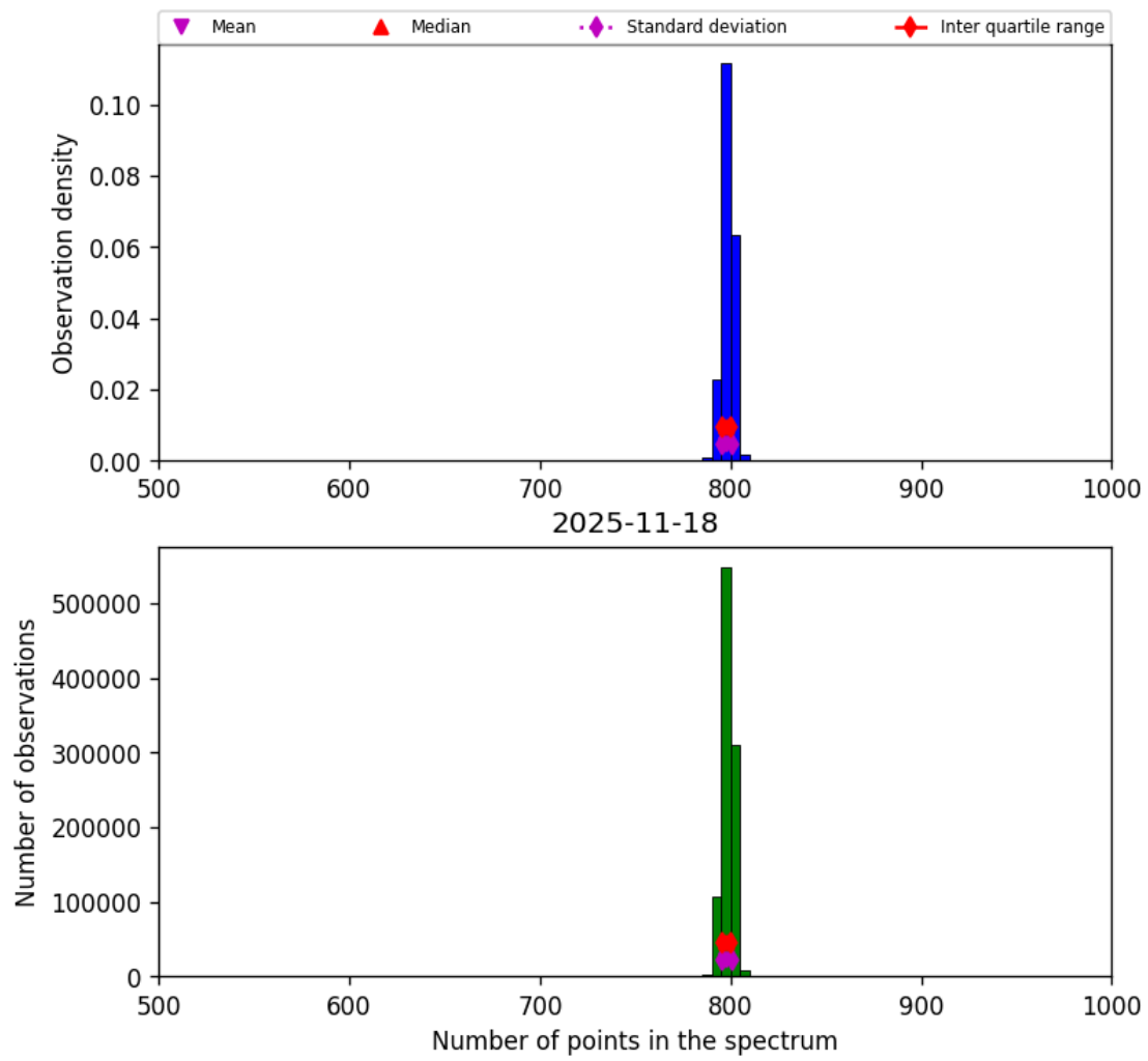
Figure 26: Histogram of “Number of points in the spectrum” for 2025-11-18 to 2025-11-19
