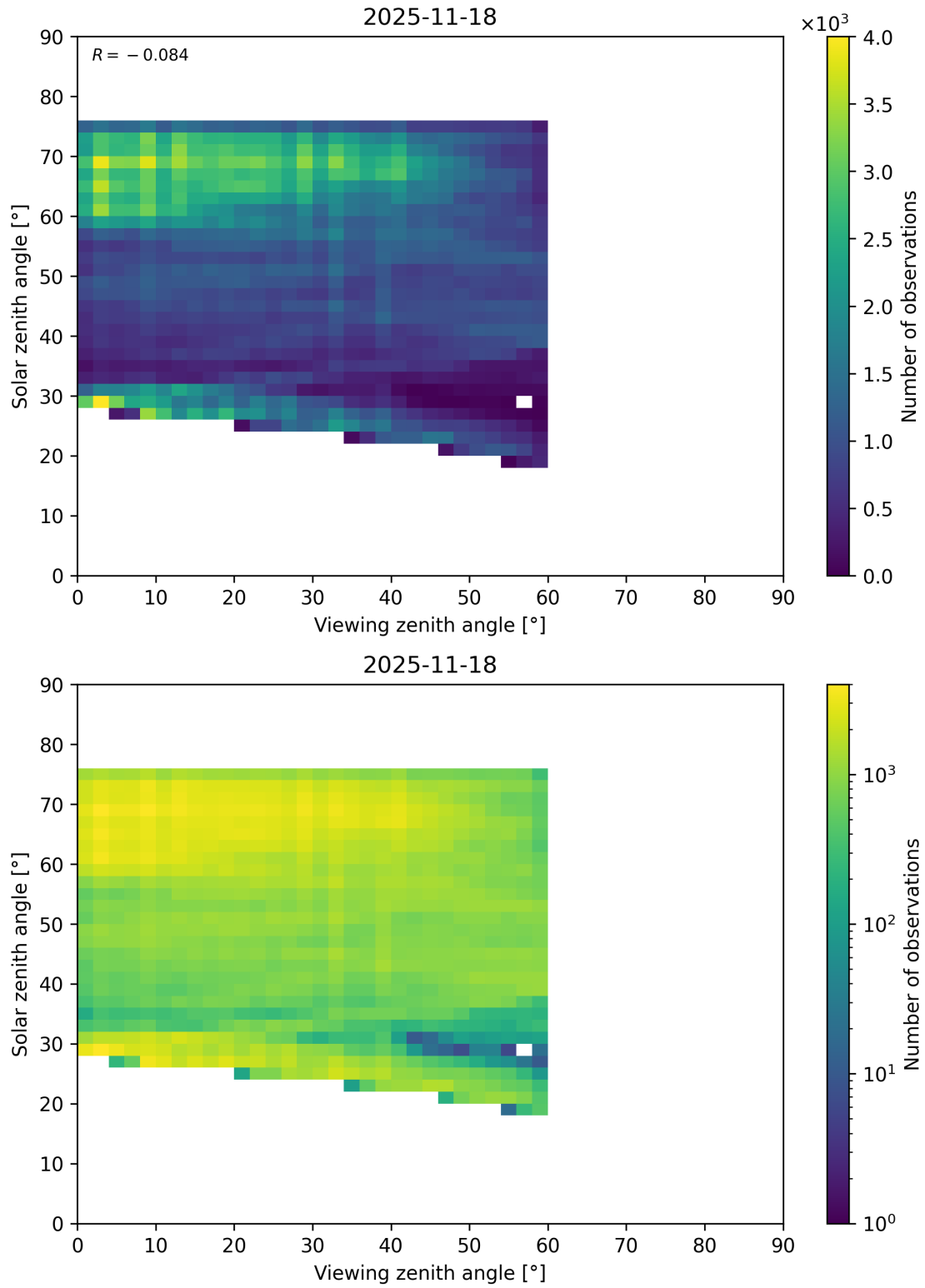
Figure 115: Scatter density plot of “Viewing zenith angle” against “Solar zenith angle” for 2025-11-18 to 2025-11-19.
