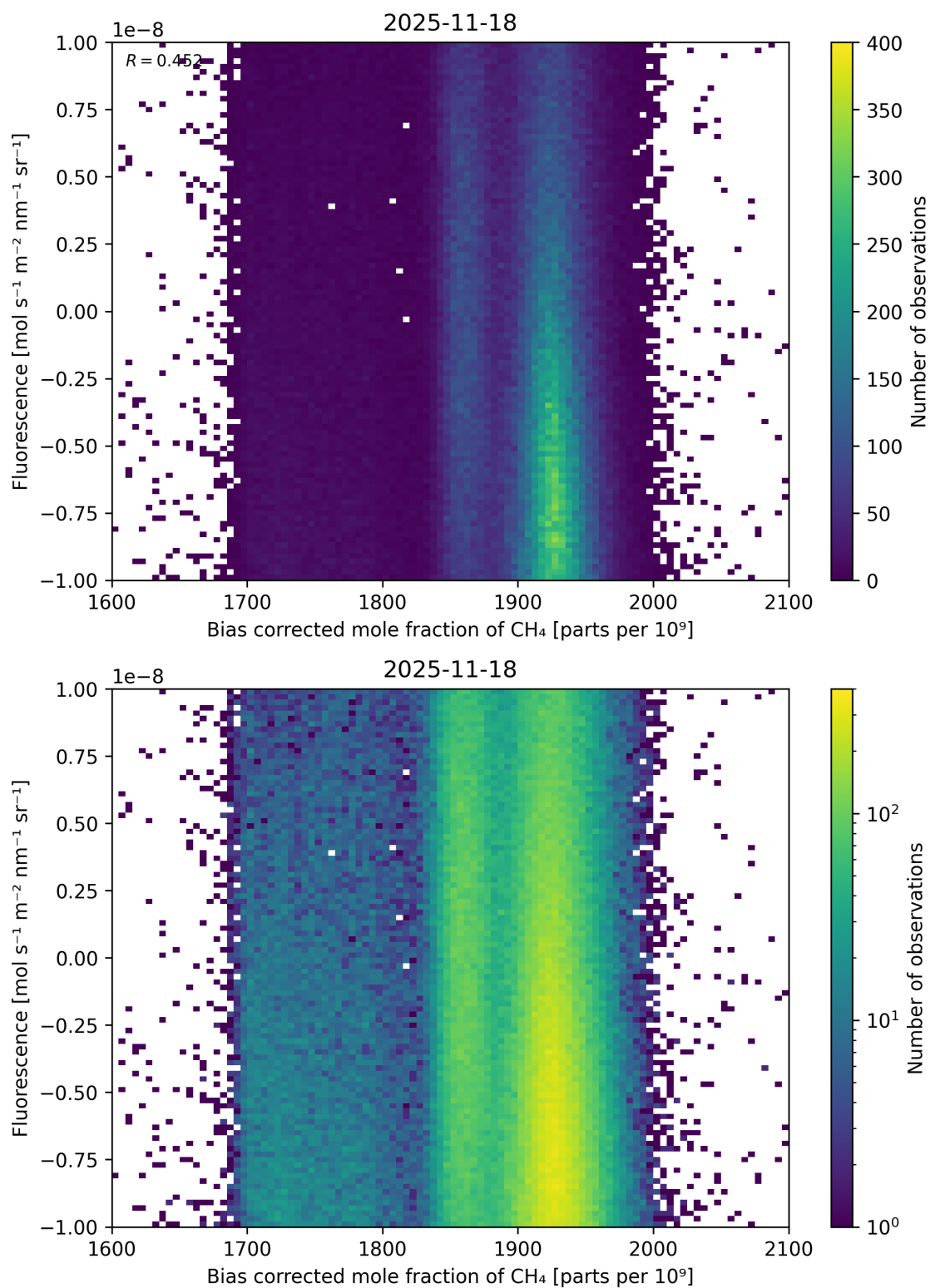
Figure 66: Scatter density plot of “Bias corrected mole fraction of \text{CH}_4 ” against “Fluorescence” for 2025-11-18 to 2025-11-19.
