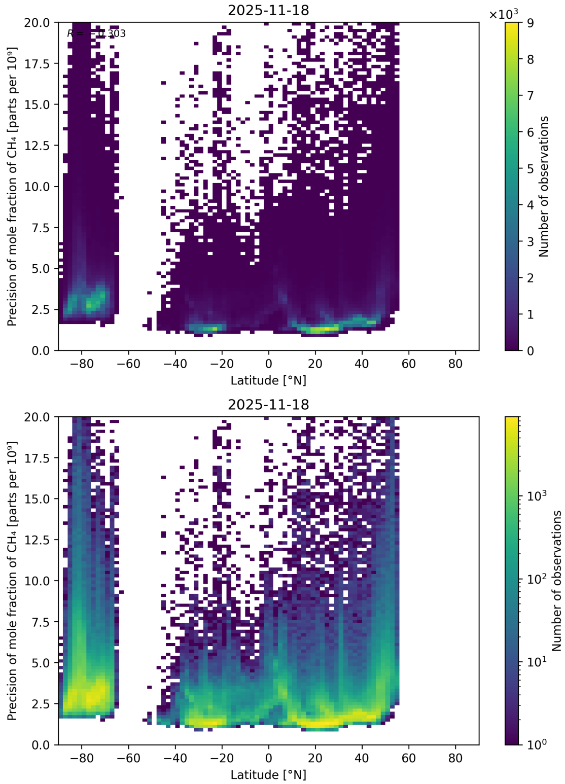
Figure 59: Scatter density plot of “Latitude” against “Precision of mole fraction of CH 4 ” for 2025-11-18 to 2025-11-19.
