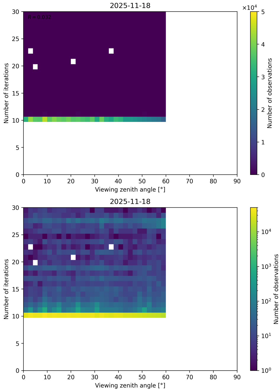
Figure 113: Scatter density plot of “Viewing zenith angle” against “Number of iterations” for 2025-11-18 to 2025-11-19.
