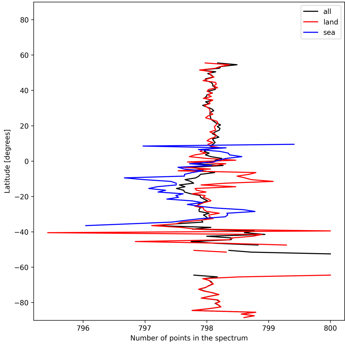
Figure 15: Zonal average of “Number of points in the spectrum” for 2025-11-18 to 2025-11-19.
