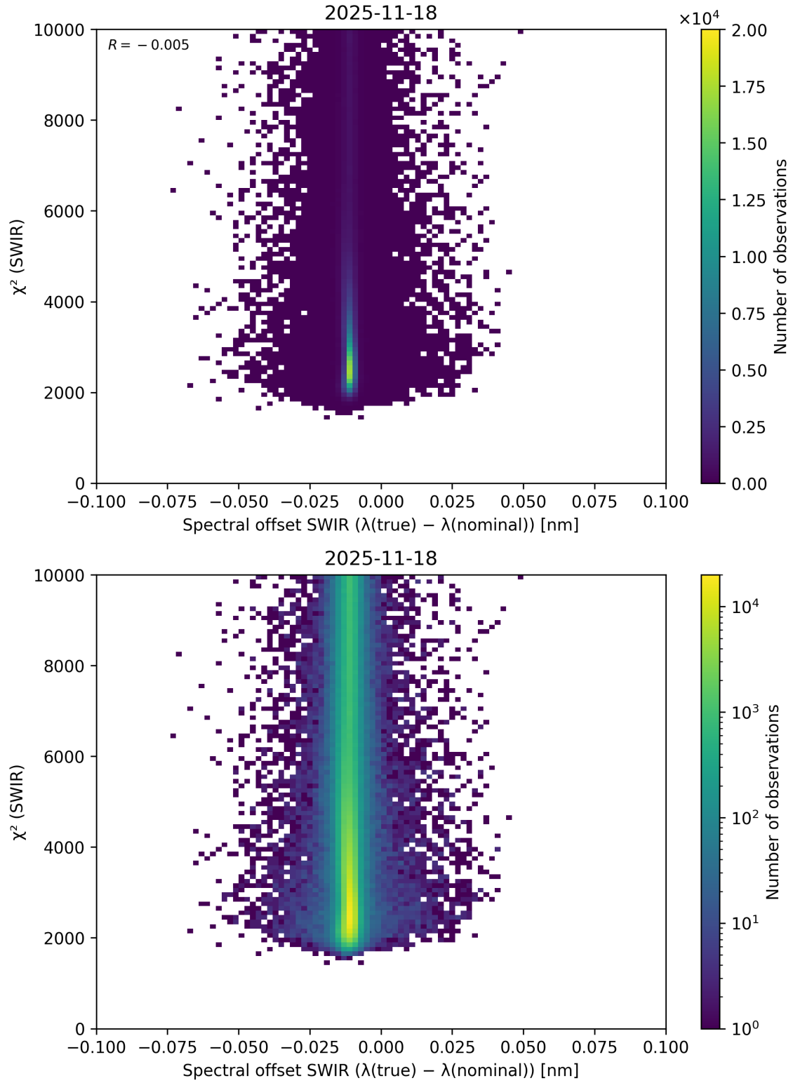
Figure 118: Scatter density plot of “Spectral offset SWIR ( \lambda_{\text{true}} - \lambda_{\text{nominal}} )” against “ \chi^2 (SWIR)” for 2025-11-18 to 2025-11-19.
