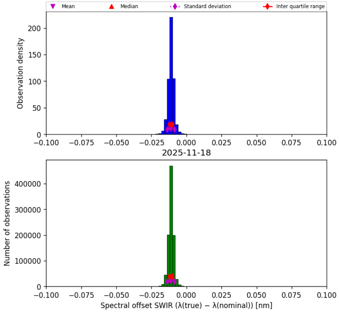
Figure 27: Histogram of “Spectral offset SWIR ( \lambda_{\text{true}} - \lambda_{\text{nominal}} )” for 2025-11-18 to 2025-11-19
