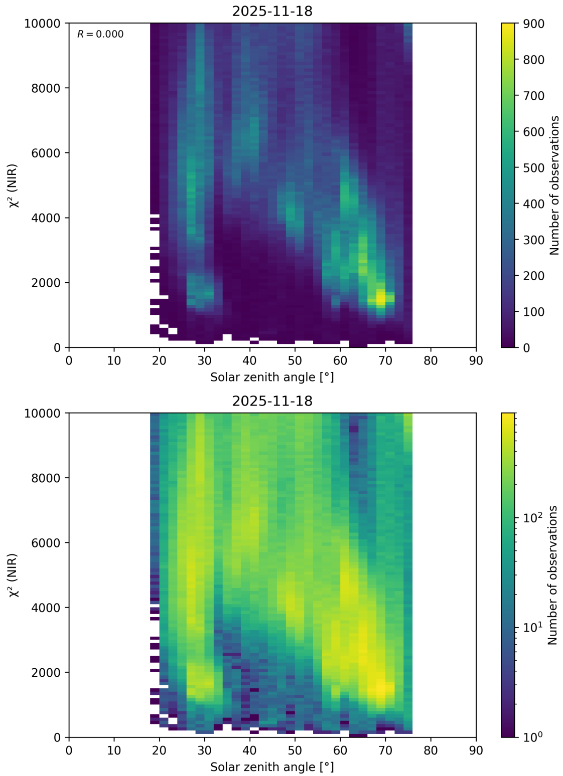
Figure 94: Scatter density plot of “Solar zenith angle” against “ \chi^2 (NIR)” for 2025-11-18 to 2025-11-19.
