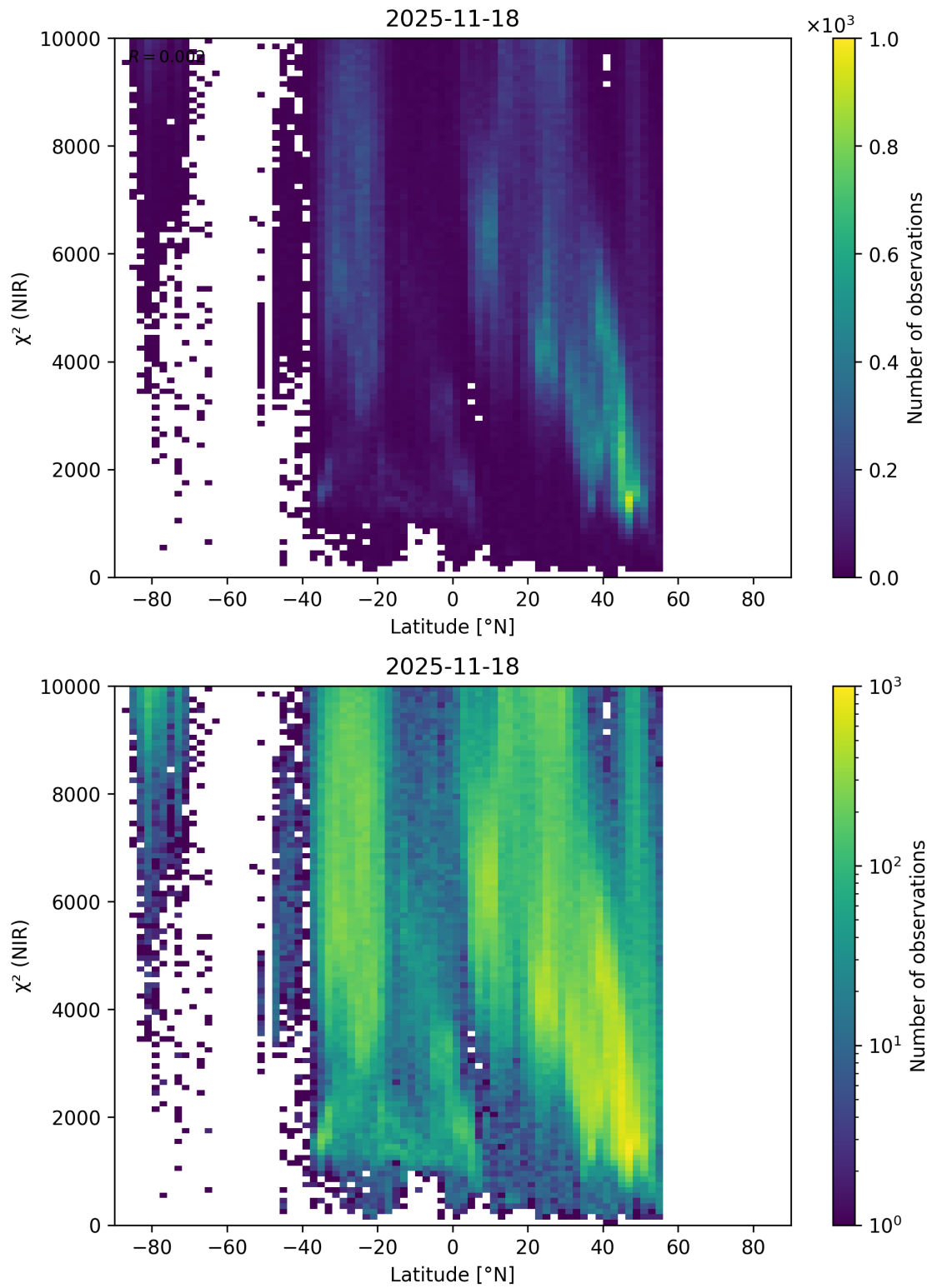
Figure 53: Scatter density plot of “Latitude” against “ \chi^2 (NIR)” for 2025-11-18 to 2025-11-19.
