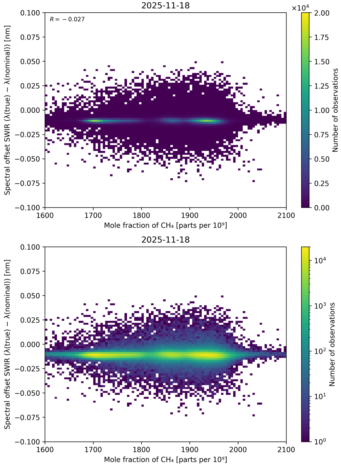
Figure 86: Scatter density plot of “Mole fraction of CH 4 ” against “Spectral offset SWIR ( \lambda_{\text{true}} - \lambda_{\text{nominal}} )” for 2025-11-18 to 2025-11-19.
