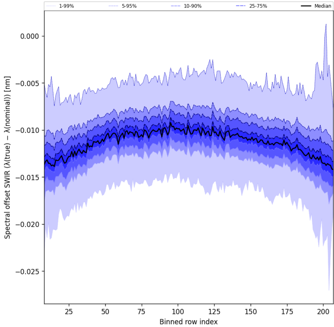
Figure 38: Along track statistics of “Spectral offset SWIR ( \lambda_{\text{true}} - \lambda_{\text{nominal}} )” for 2025-11-18 to 2025-11-19
