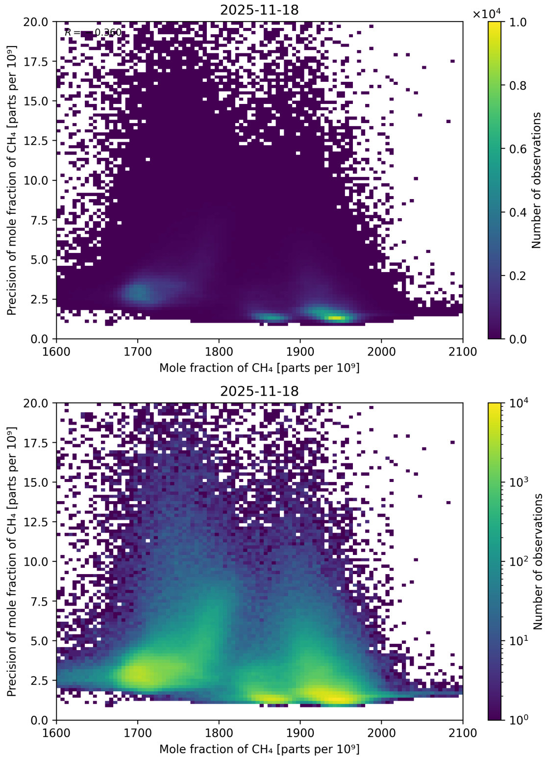
Figure 75: Scatter density plot of “Mole fraction of CH 4 ” against “Precision of mole fraction of CH 4 ” for 2025-11-18 to 2025-11-19.
