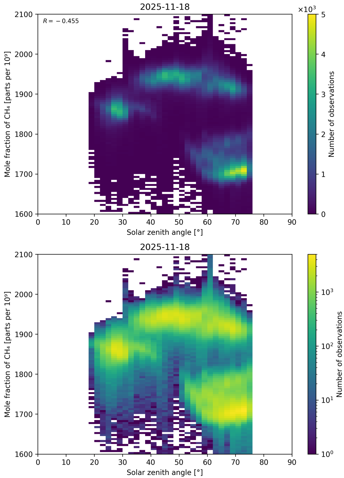
Figure 99: Scatter density plot of “Solar zenith angle” against “Mole fraction of CH 4 ” for 2025-11-18 to 2025-11-19.
