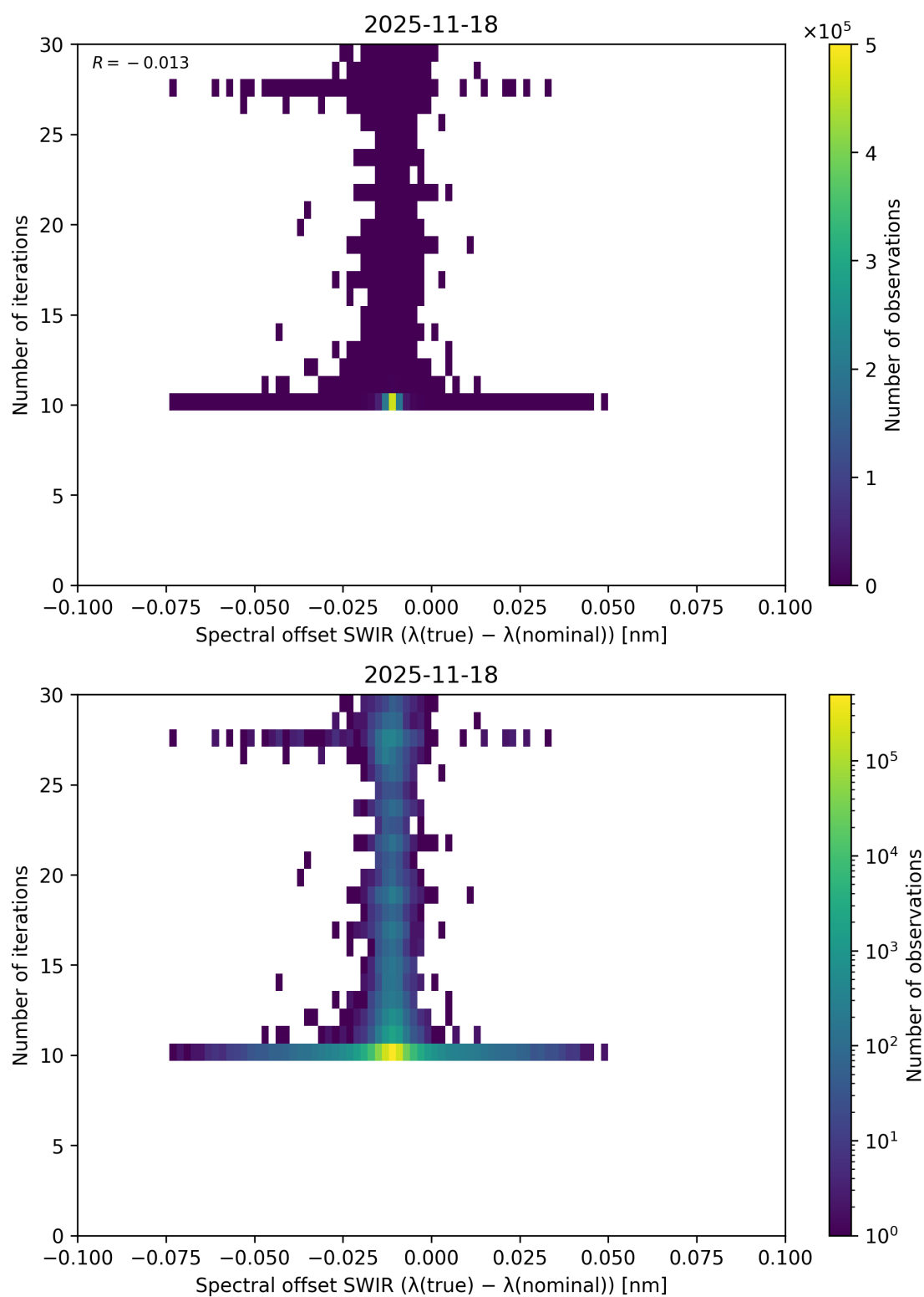
Figure 121: Scatter density plot of “Spectral offset SWIR ( \lambda_{\text{true}} - \lambda_{\text{nominal}} )” against “Number of iterations” for 2025-11-18 to 2025-11-19.
