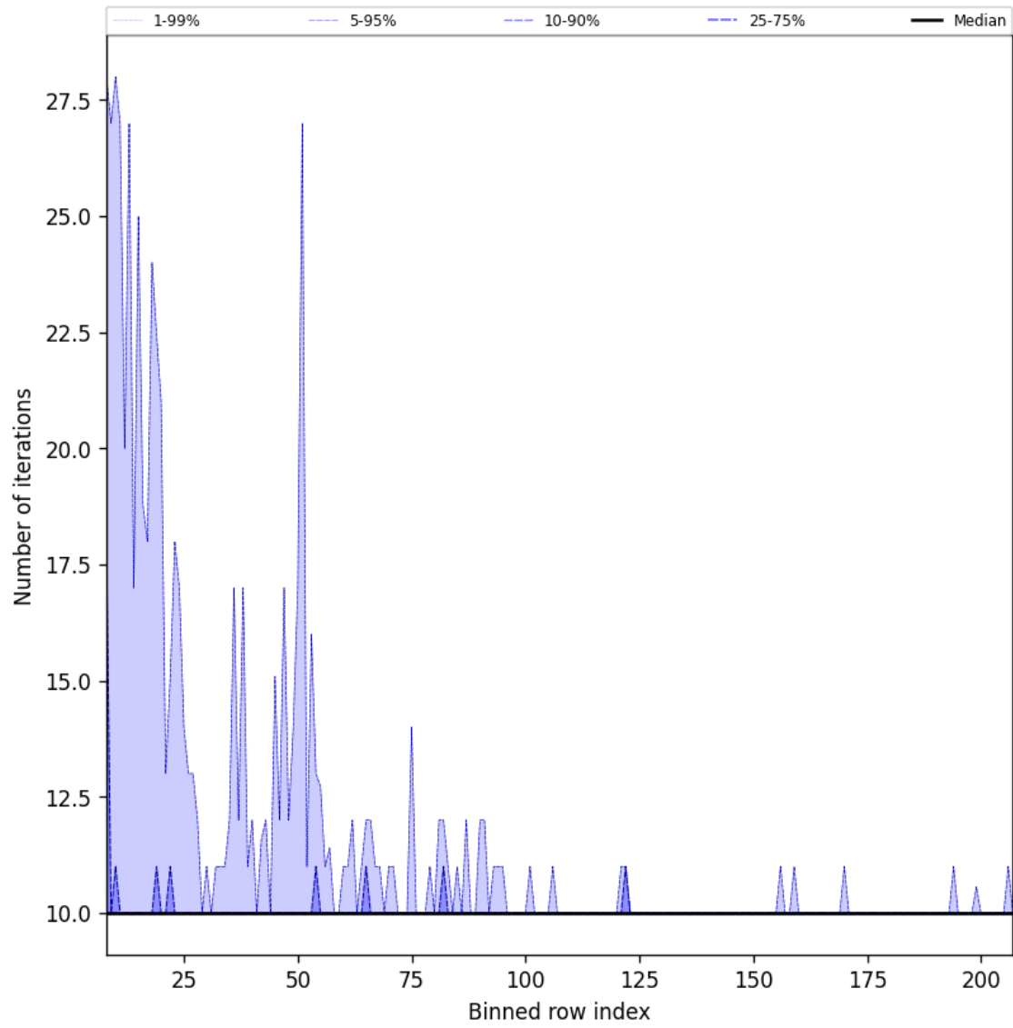
Figure 42: Along track statistics of “Number of iterations” for 2025-11-18 to 2025-11-19
