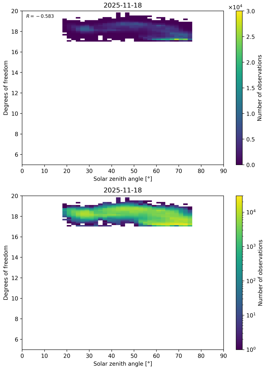
Figure 96: Scatter density plot of “Solar zenith angle” against “Degrees of freedom” for 2025-11-18 to 2025-11-19.
