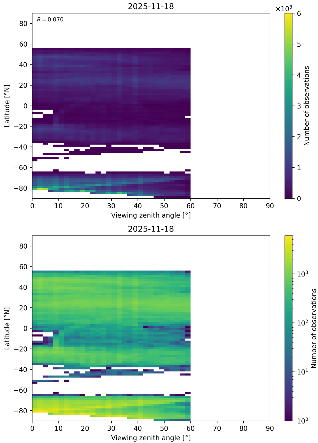
Figure 109: Scatter density plot of “Viewing zenith angle” against “Latitude” for 2025-11-18 to 2025-11-19.
