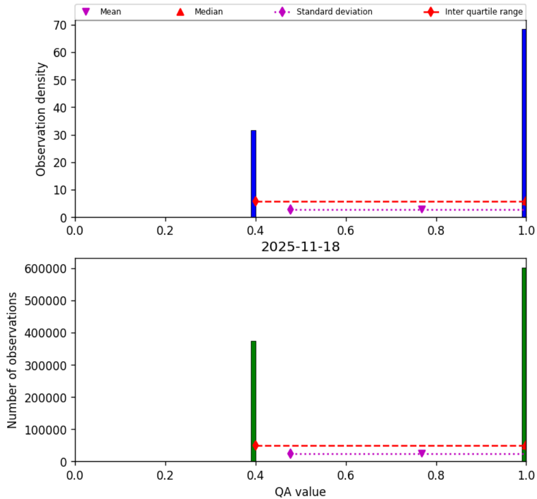
Figure 22: Histogram of “QA value” for 2025-11-18 to 2025-11-19
