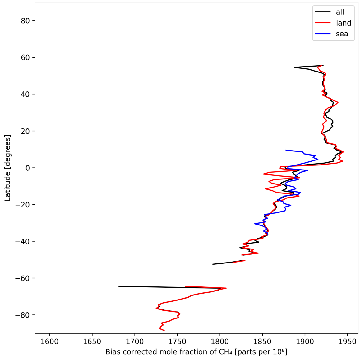
Figure 14: Zonal average of “Bias corrected mole fraction of CH 4 ” for 2025-11-18 to 2025-11-19.
