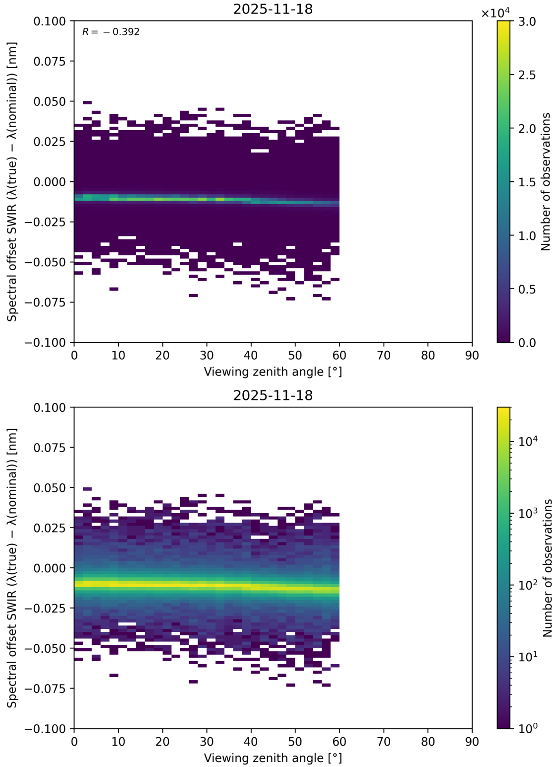
Figure 116: Scatter density plot of “Viewing zenith angle” against “Spectral offset SWIR ( \lambda_{\text{true}} - \lambda_{\text{nominal}} )” for 2025-11-18 to 2025-11-19.
