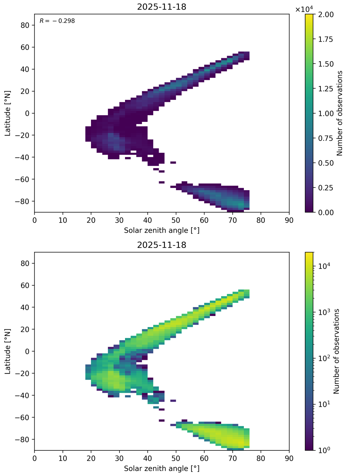
Figure 98: Scatter density plot of “Solar zenith angle” against “Latitude” for 2025-11-18 to 2025-11-19.
