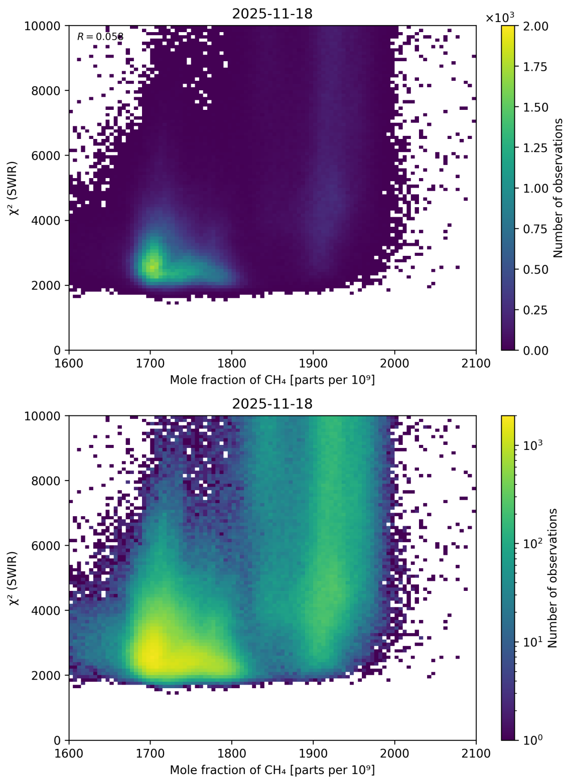
Figure 71: Scatter density plot of “Mole fraction of \text{CH}_4 ” against “ \chi^2 (SWIR)” for 2025-11-18 to 2025-11-19.
