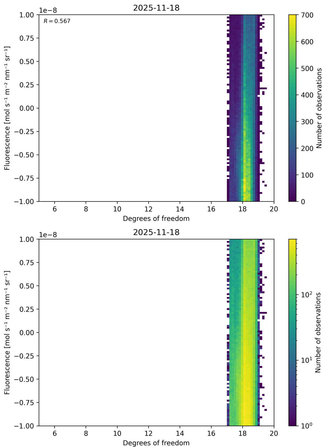
Figure 51: Scatter density plot of “Degrees of freedom” against “Fluorescence” for 2025-11-18 to 2025-11-19.
