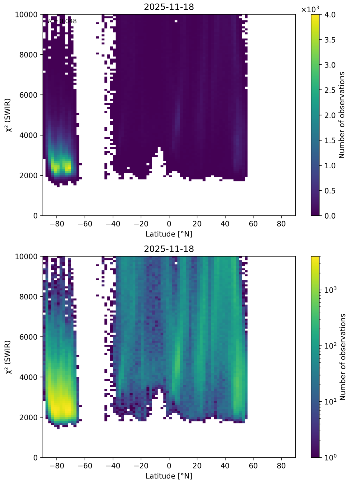
Figure 54: Scatter density plot of “Latitude” against “ \chi^2 (SWIR)” for 2025-11-18 to 2025-11-19.
