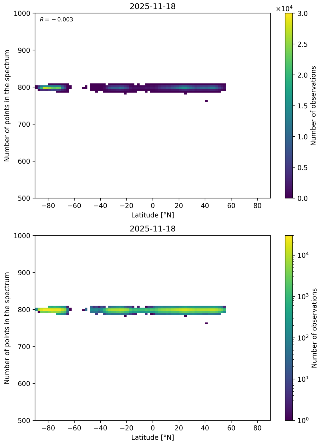
Figure 61: Scatter density plot of “Latitude” against “Number of points in the spectrum” for 2025-11-18 to 2025-11-19.
