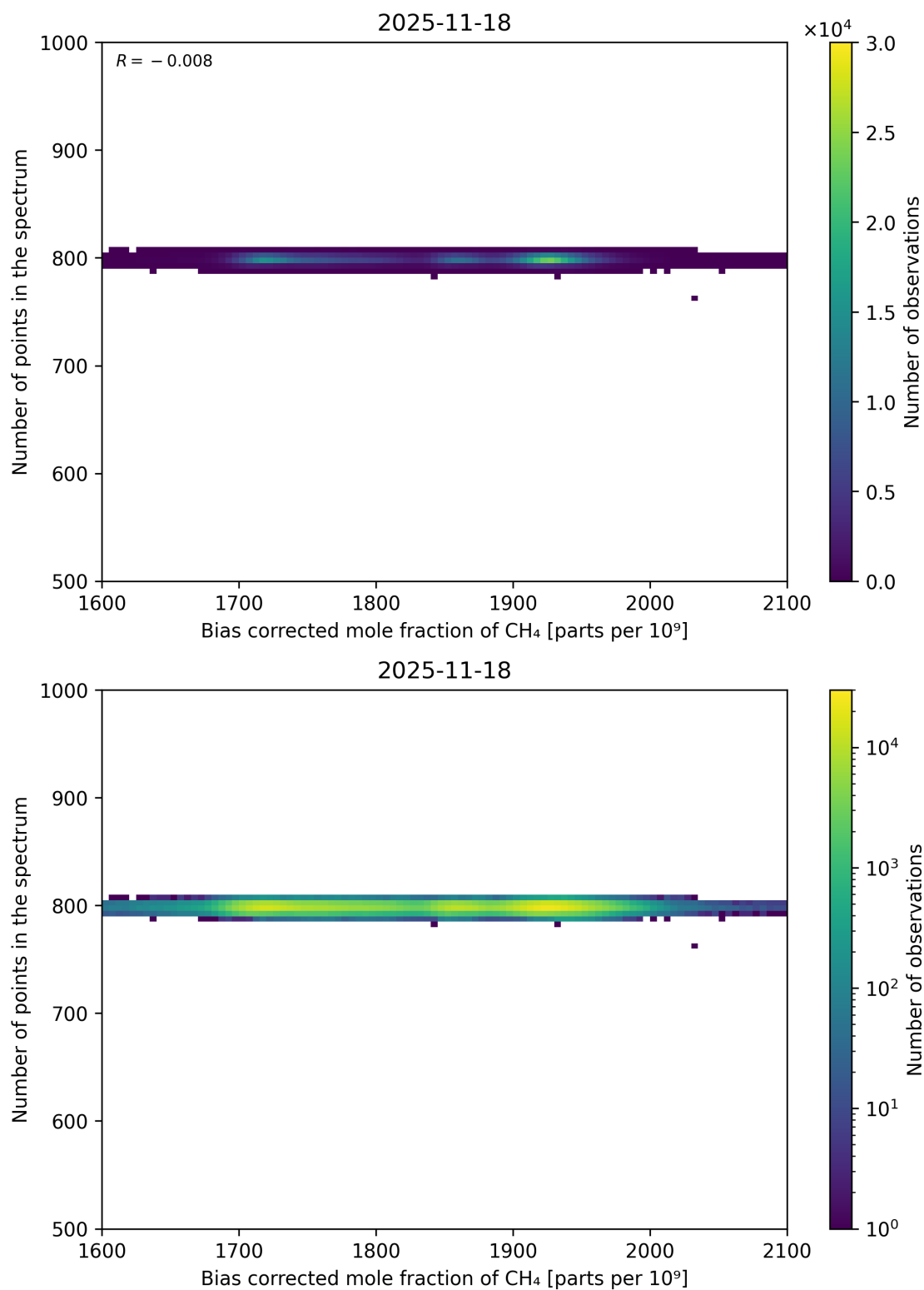
Figure 68: Scatter density plot of “Bias corrected mole fraction of CH 4 ” against “Number of points in the spectrum” for 2025-11-18 to 2025-11-19.
