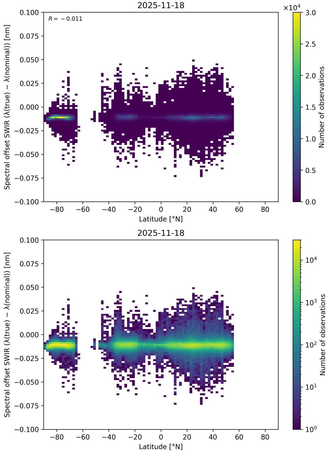
Figure 62: Scatter density plot of “Latitude” against “Spectral offset SWIR ( \lambda_{\text{true}} - \lambda_{\text{nominal}} )” for 2025-11-18 to 2025-11-19.
