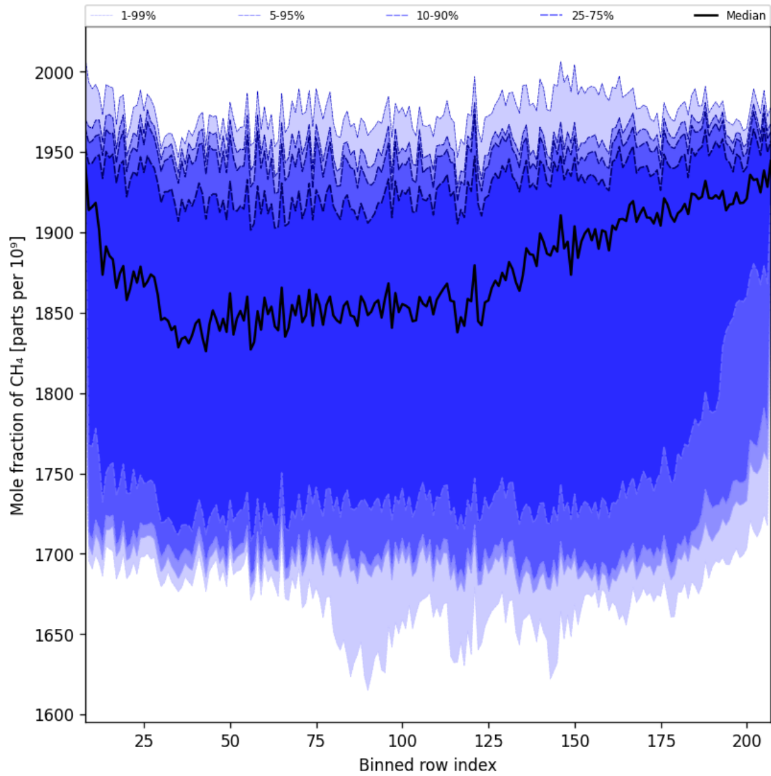
Figure 34: Along track statistics of “Mole fraction of CH 4 ” for 2025-11-18 to 2025-11-19
