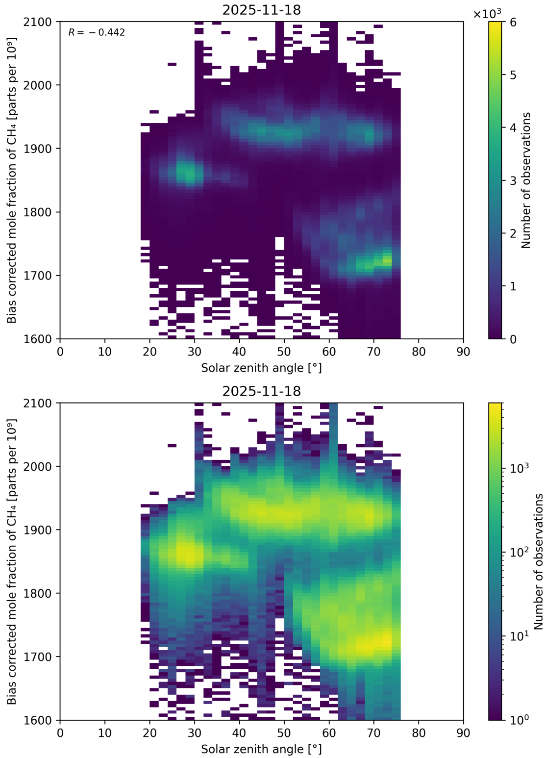
Figure 100: Scatter density plot of “Solar zenith angle” against “Bias corrected mole fraction of \text{CH}_4 ” for 2025-11-18 to 2025-11-19.
