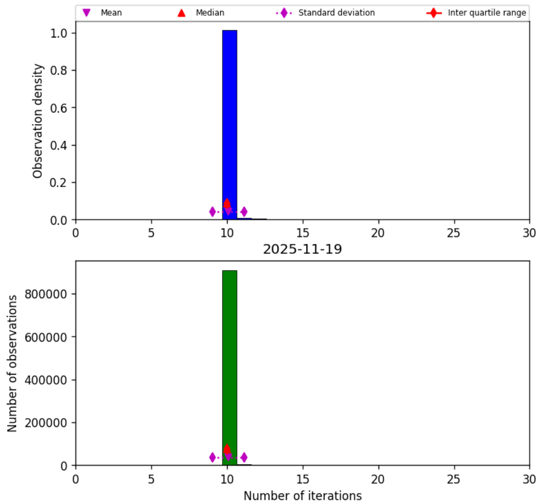
Figure 31: Histogram of “Number of iterations” for 2025-11-18 to 2025-11-20
