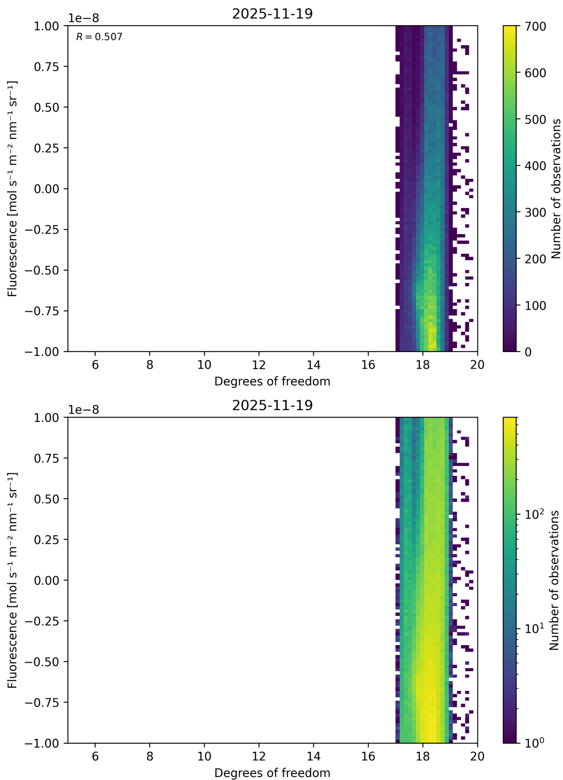
Figure 51: Scatter density plot of “Degrees of freedom” against “Fluorescence” for 2025-11-18 to 2025-11-20.
