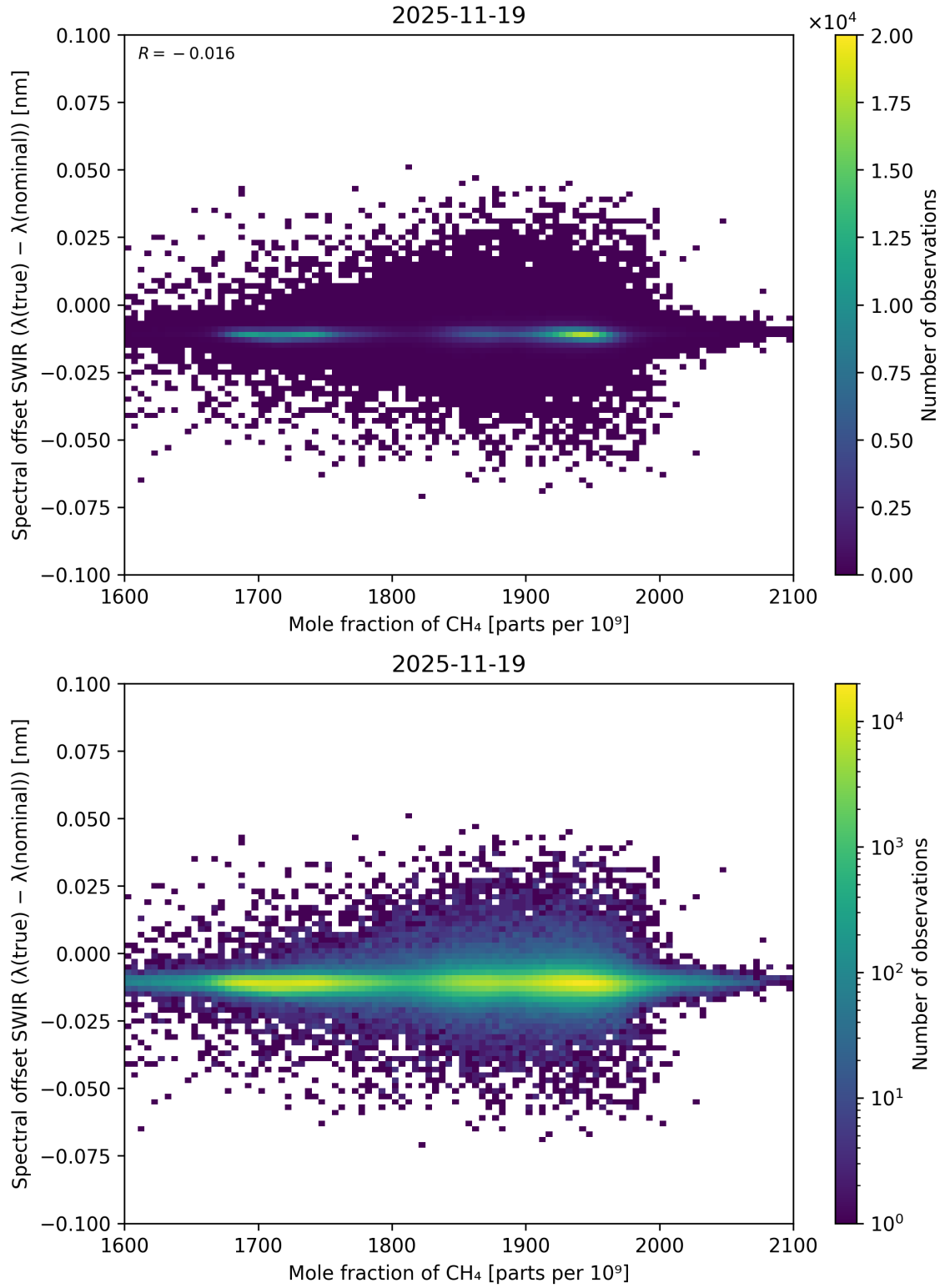
Figure 86: Scatter density plot of “Mole fraction of CH 4 ” against “Spectral offset SWIR ( \lambda_{\text{true}} - \lambda_{\text{nominal}} )” for 2025-11-18 to 2025-11-20.
