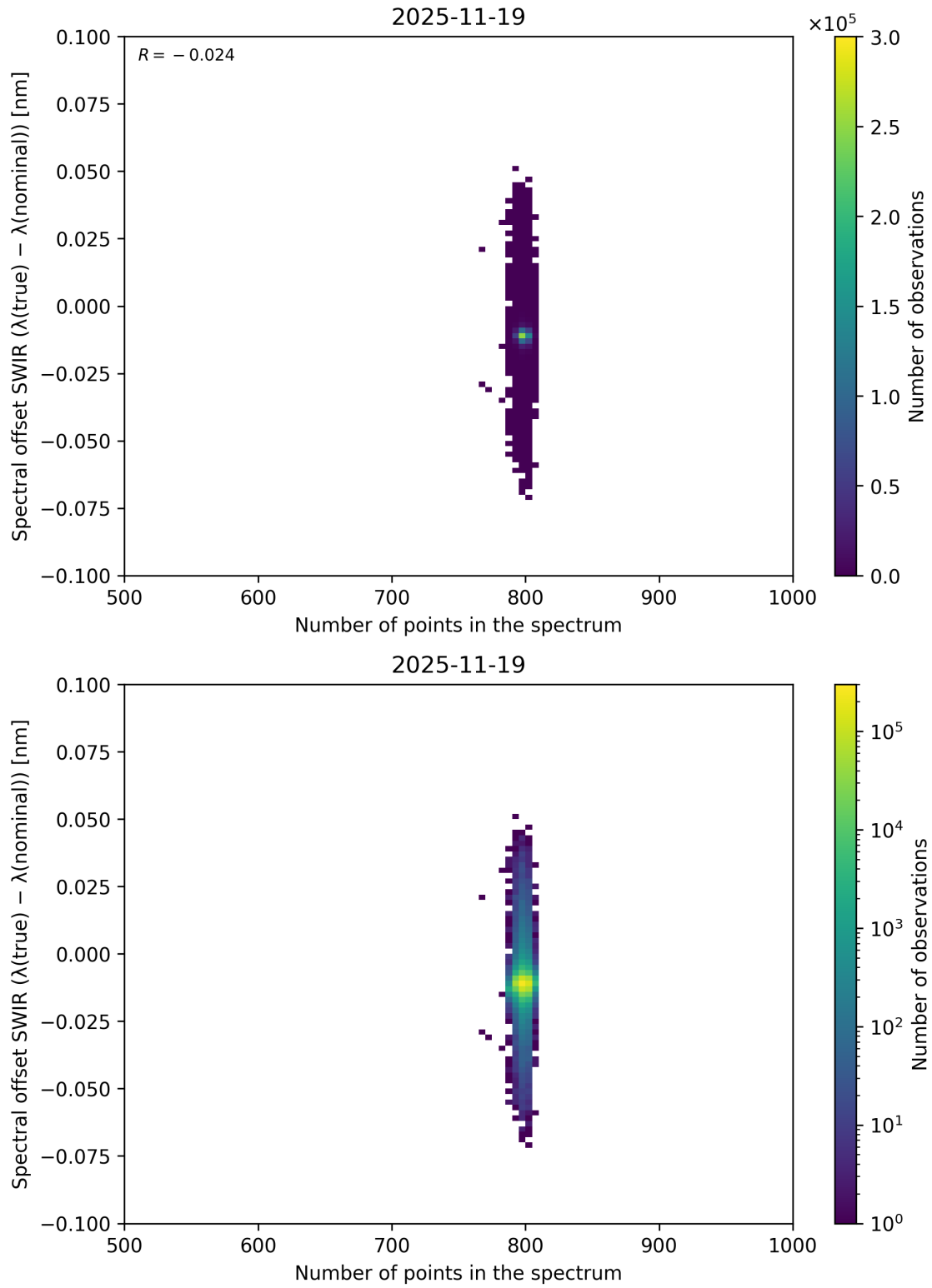
Figure 93: Scatter density plot of “Number of points in the spectrum” against “Spectral offset SWIR ( \lambda_{\text{true}} - \lambda_{\text{nominal}} )” for 2025-11-18 to 2025-11-20.
