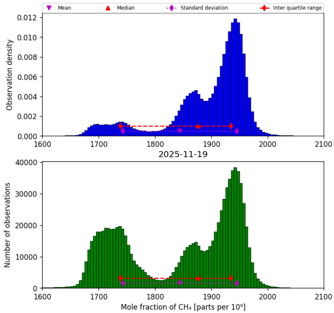
Figure 23: Histogram of “Mole fraction of CH 4 ” for 2025-11-18 to 2025-11-20
