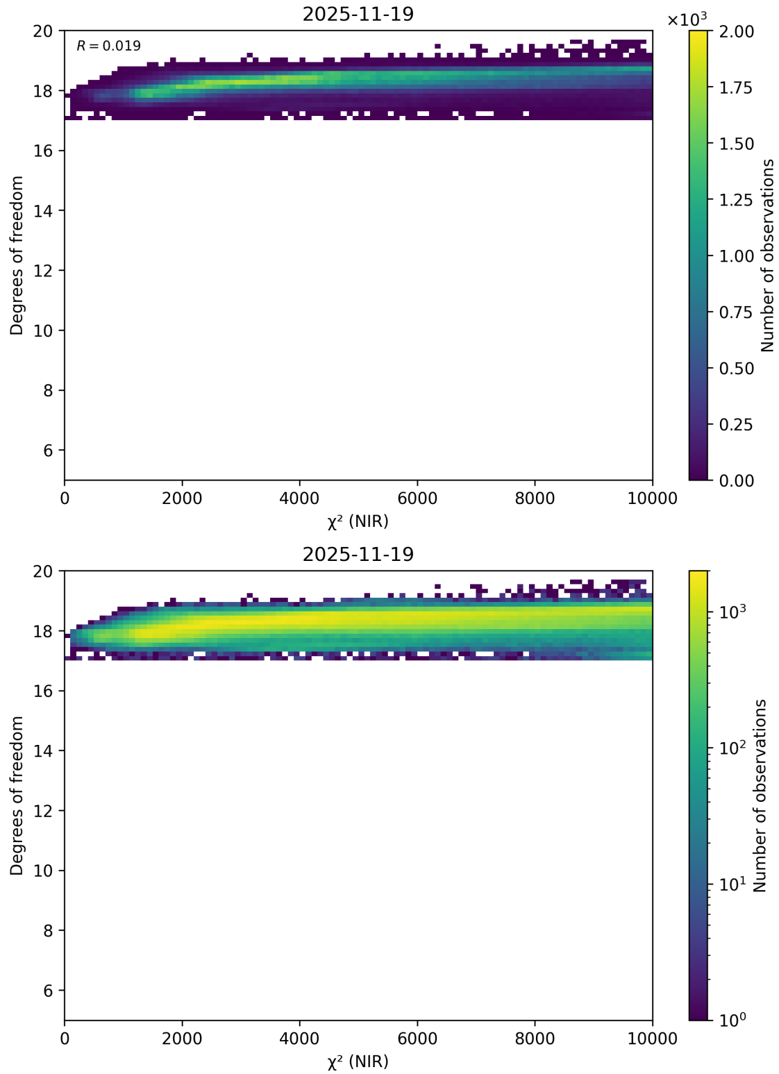
Figure 44: Scatter density plot of “ \chi^2 (NIR)” against “Degrees of freedom” for 2025-11-18 to 2025-11-20.
