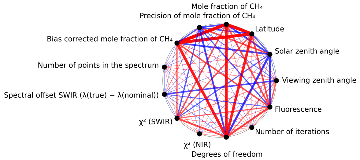
Figure 1: Map of correlation graph for 2025-11-18 to 2025-11-20.
