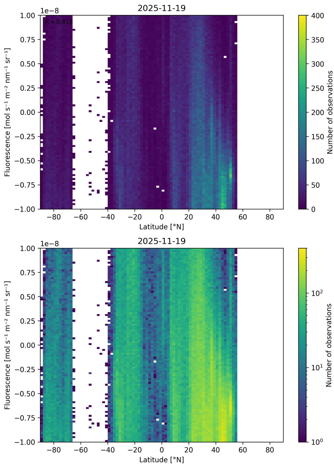
Figure 56: Scatter density plot of “Latitude” against “Fluorescence” for 2025-11-18 to 2025-11-20.
