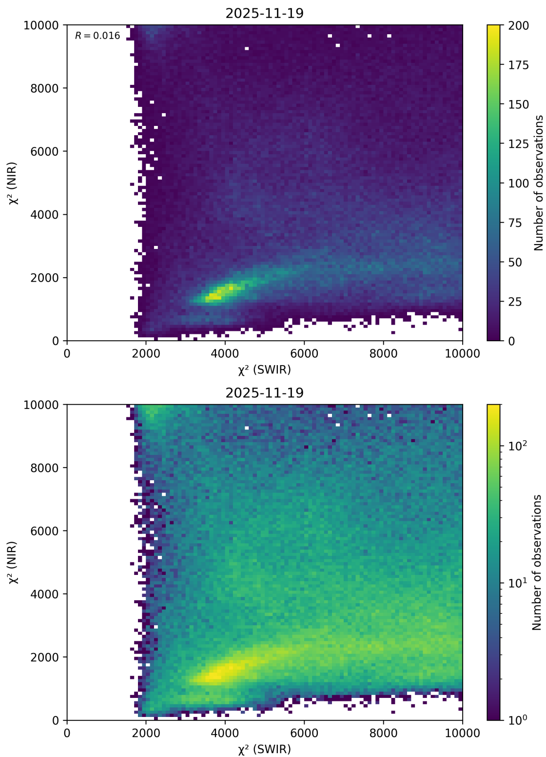
Figure 47: Scatter density plot of “ \chi^2 (SWIR)” against “ \chi^2 (NIR)” for 2025-11-18 to 2025-11-20.
