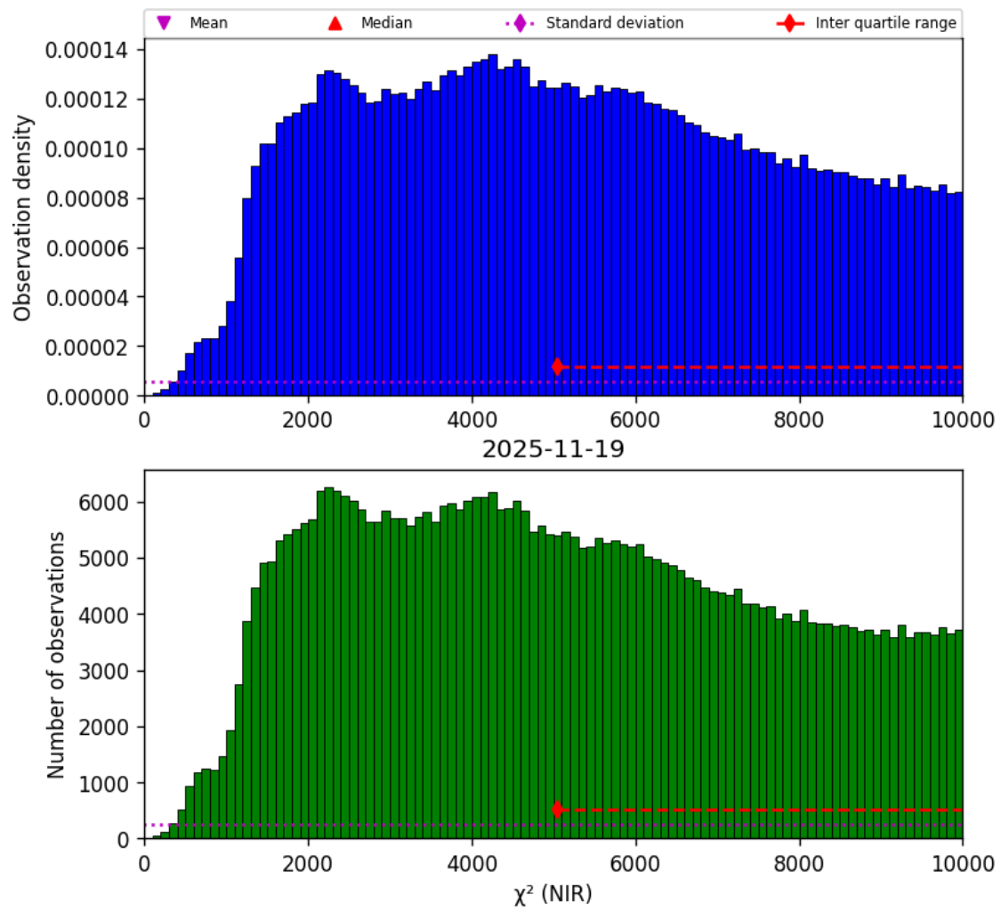
Figure 29: Histogram of “ \chi^2 (NIR)” for 2025-11-18 to 2025-11-20
