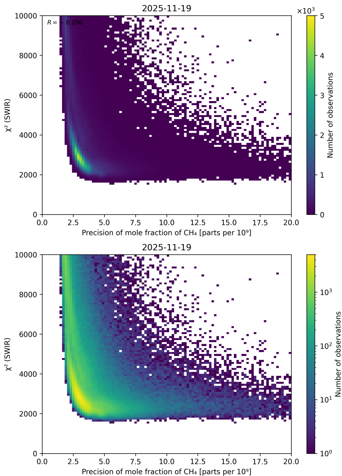
Figure 79: Scatter density plot of “Precision of mole fraction of \text{CH}_4 ” against “ \chi^2 (SWIR)” for 2025-11-18 to 2025-11-20.
