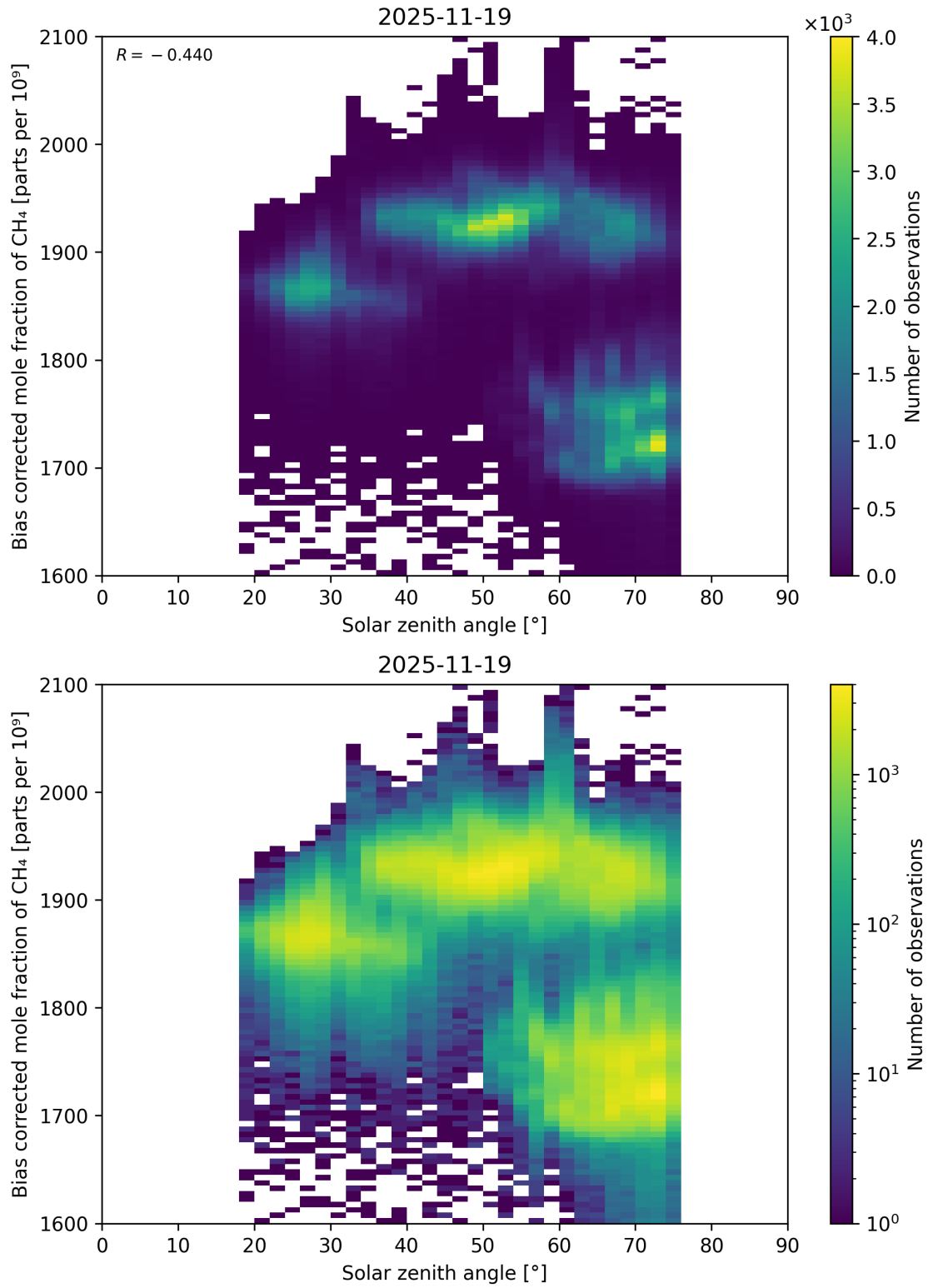
Figure 100: Scatter density plot of “Solar zenith angle” against “Bias corrected mole fraction of CH 4 ” for 2025-11-18 to 2025-11-20.
