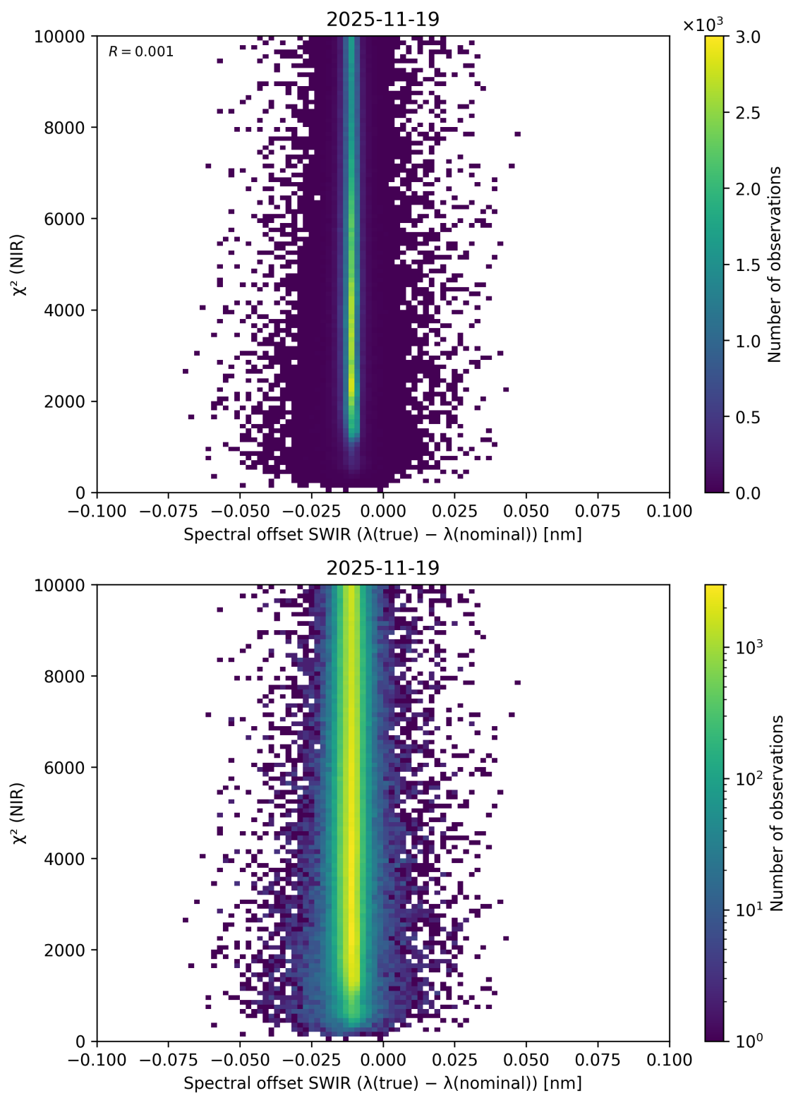
Figure 117: Scatter density plot of “Spectral offset SWIR ( \lambda_{\text{true}} - \lambda_{\text{nominal}} )” against “ \chi^2 (NIR)” for 2025-11-18 to 2025-11-20.
