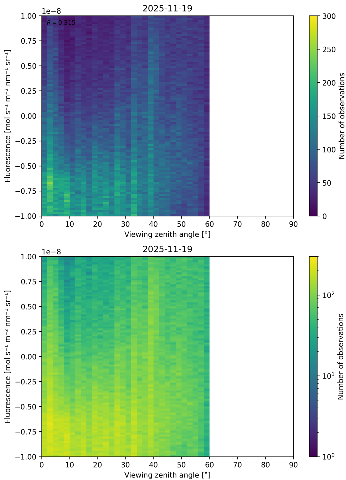
Figure 108: Scatter density plot of “Viewing zenith angle” against “Fluorescence” for 2025-11-18 to 2025-11-20.
