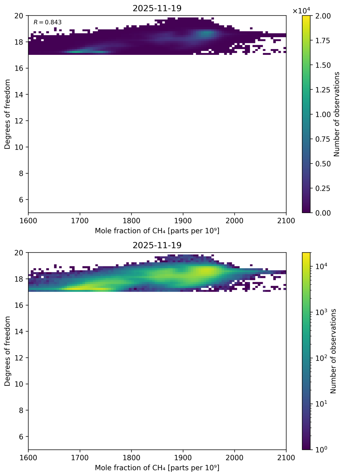
Figure 72: Scatter density plot of “Mole fraction of CH 4 ” against “Degrees of freedom” for 2025-11-18 to 2025-11-20.
