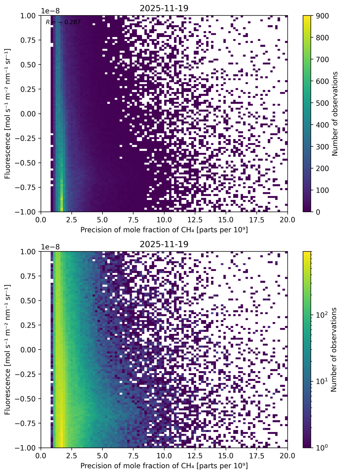
Figure 81: Scatter density plot of “Precision of mole fraction of CH 4 ” against “Fluorescence” for 2025-11-18 to 2025-11-20.
