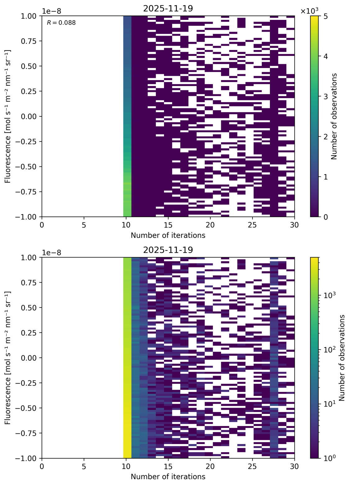
Figure 87: Scatter density plot of “Number of iterations” against “Fluorescence” for 2025-11-18 to 2025-11-20.
