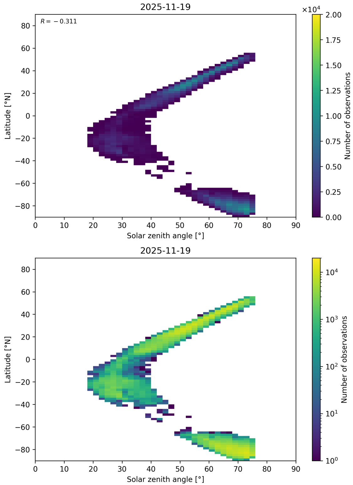
Figure 98: Scatter density plot of “Solar zenith angle” against “Latitude” for 2025-11-18 to 2025-11-20.
