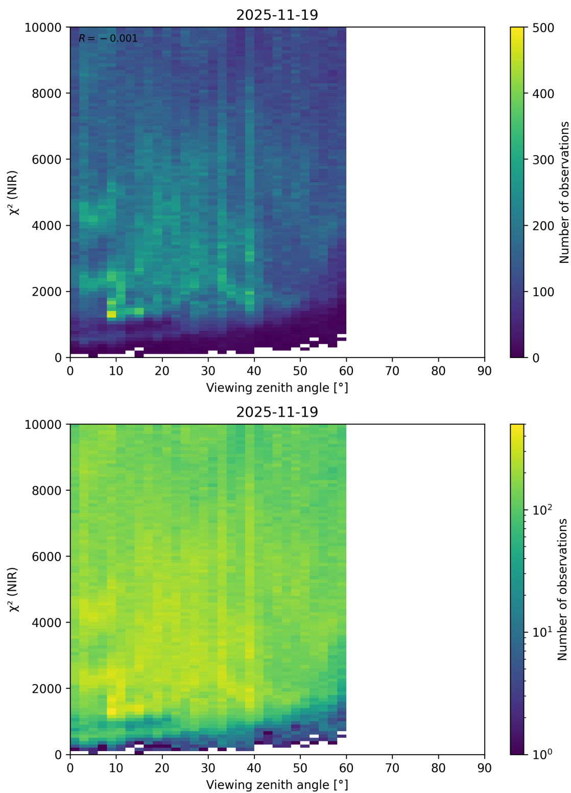
Figure 105: Scatter density plot of “Viewing zenith angle” against “ \chi^2 (NIR)” for 2025-11-18 to 2025-11-20.
