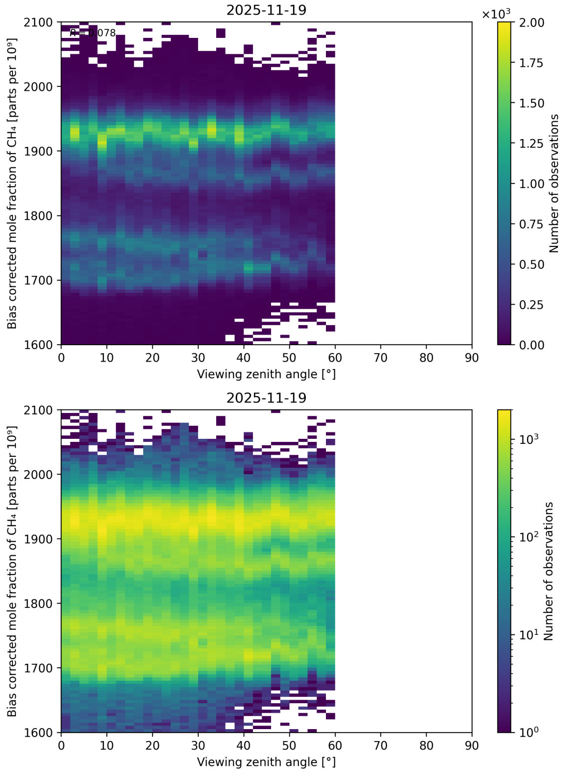
Figure 111: Scatter density plot of “Viewing zenith angle” against “Bias corrected mole fraction of CH 4 ” for 2025-11-18 to 2025-11-20.
