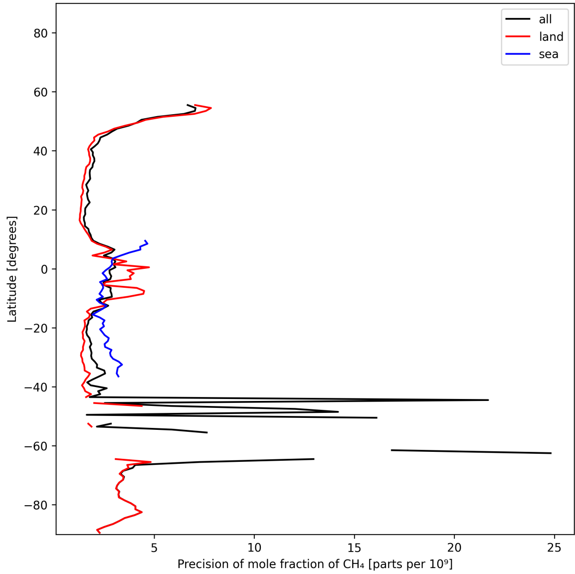
Figure 13: Zonal average of “Precision of mole fraction of CH 4 ” for 2025-11-18 to 2025-11-20.
