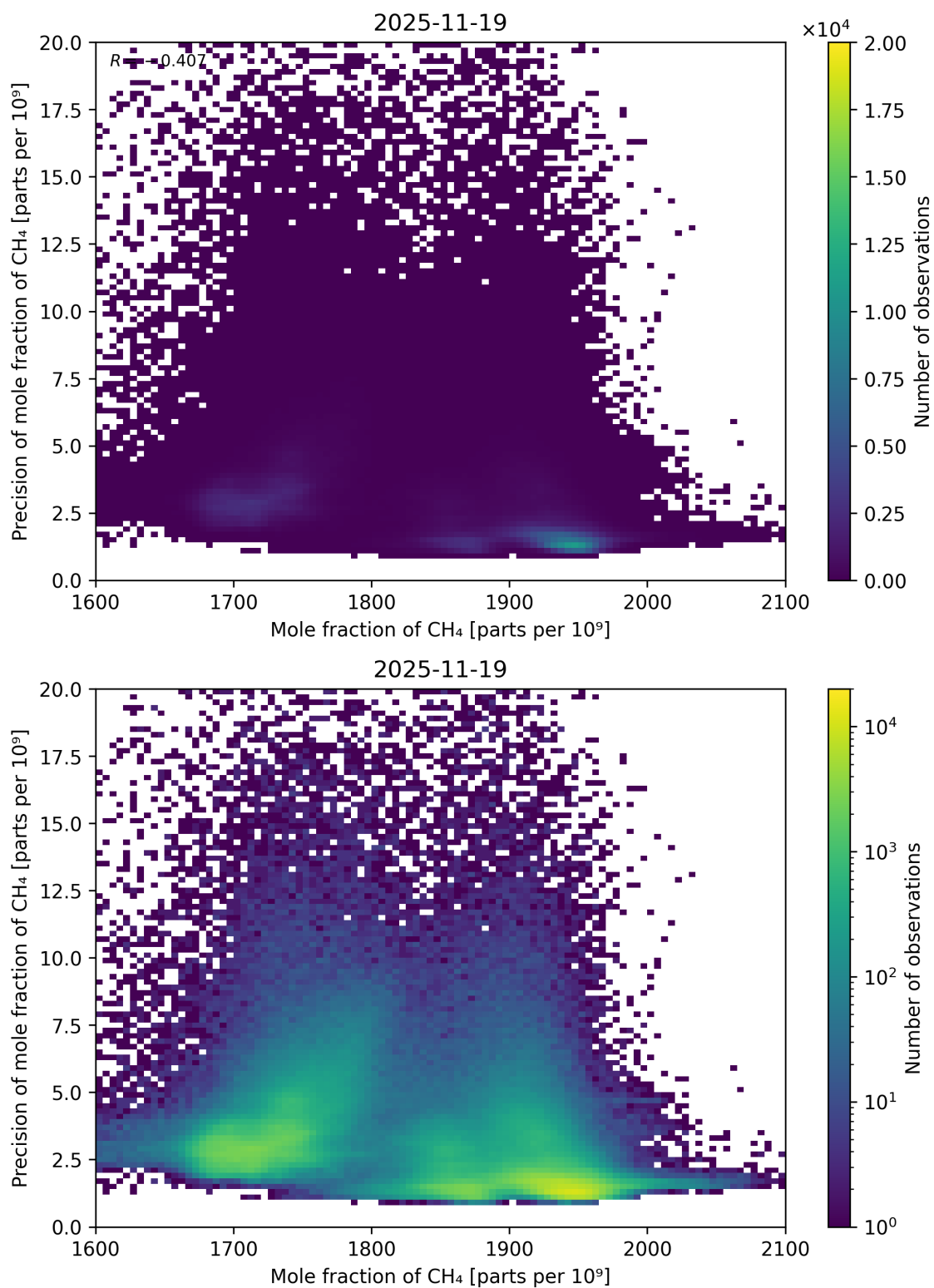
Figure 75: Scatter density plot of “Mole fraction of CH 4 ” against “Precision of mole fraction of CH 4 ” for 2025-11-18 to 2025-11-20.
