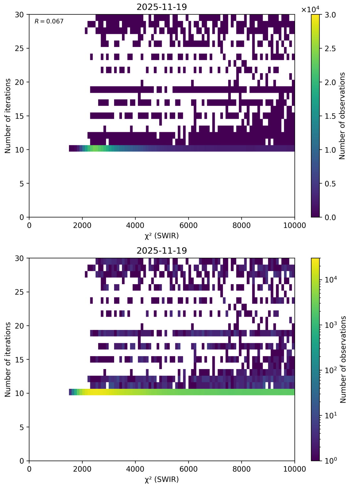
Figure 50: Scatter density plot of “ \chi^2 (SWIR)” against “Number of iterations” for 2025-11-18 to 2025-11-20.
