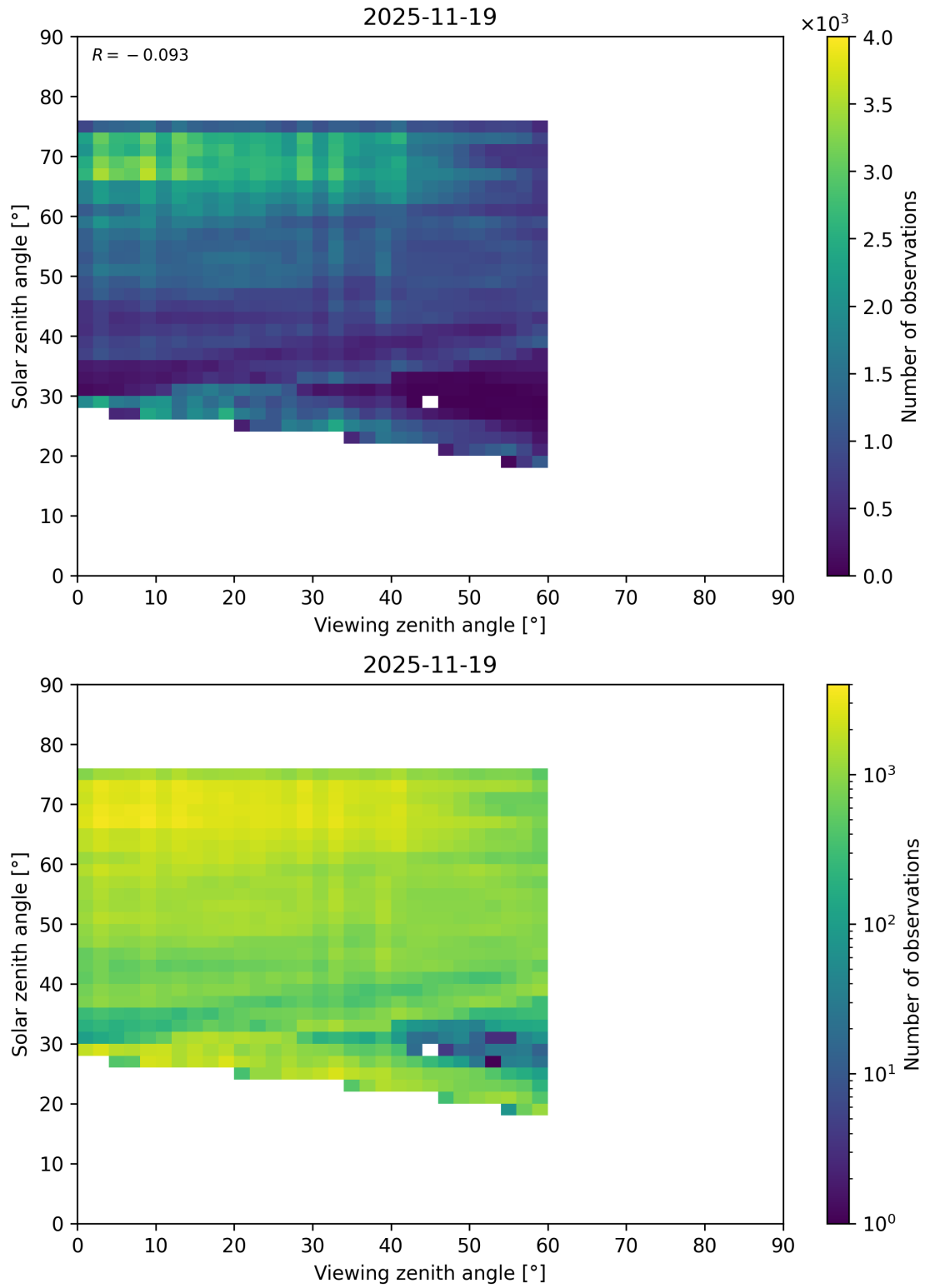
Figure 115: Scatter density plot of “Viewing zenith angle” against “Solar zenith angle” for 2025-11-18 to 2025-11-20.
