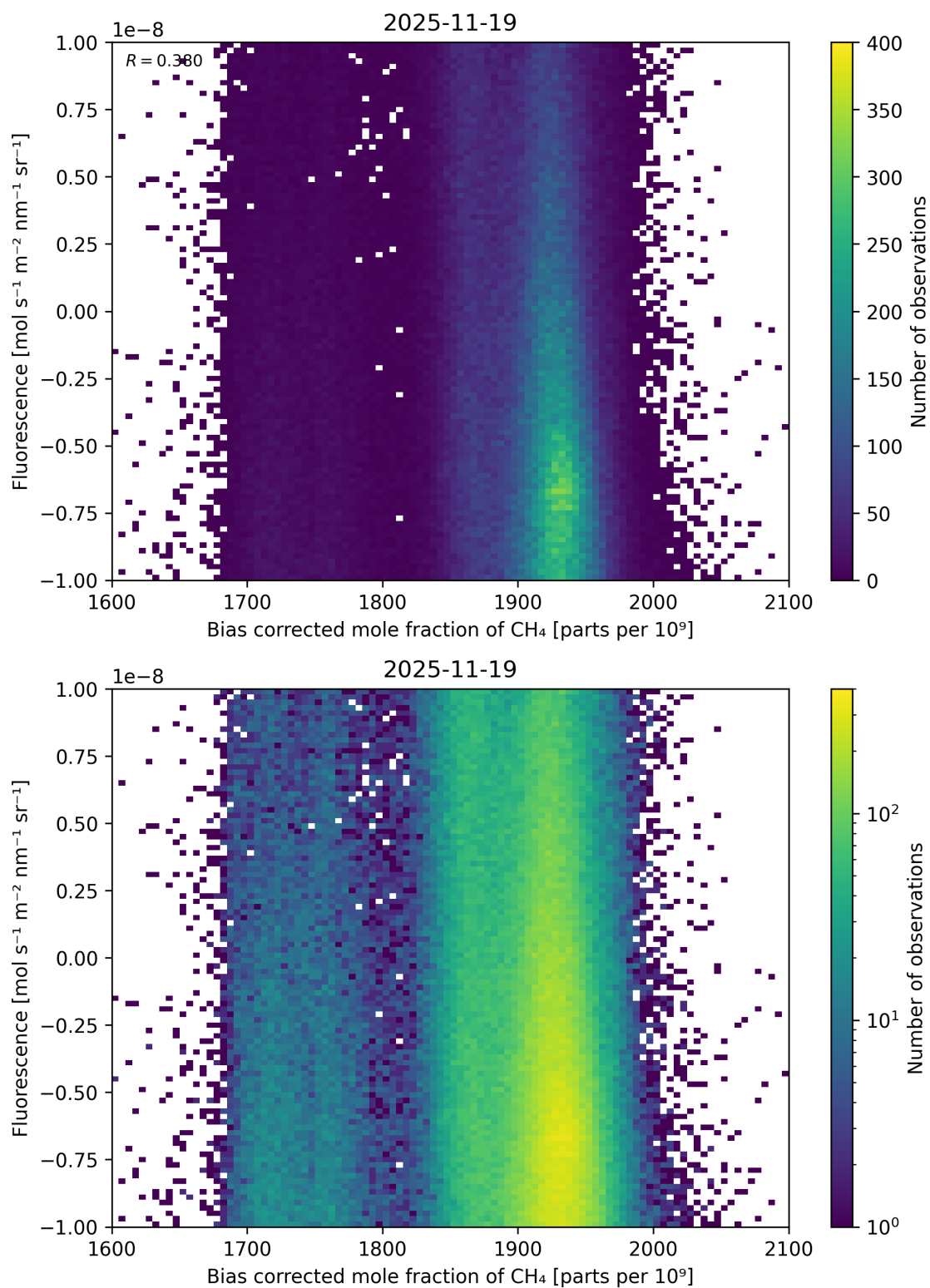
Figure 66: Scatter density plot of “Bias corrected mole fraction of \text{CH}_4 ” against “Fluorescence” for 2025-11-18 to 2025-11-20.
