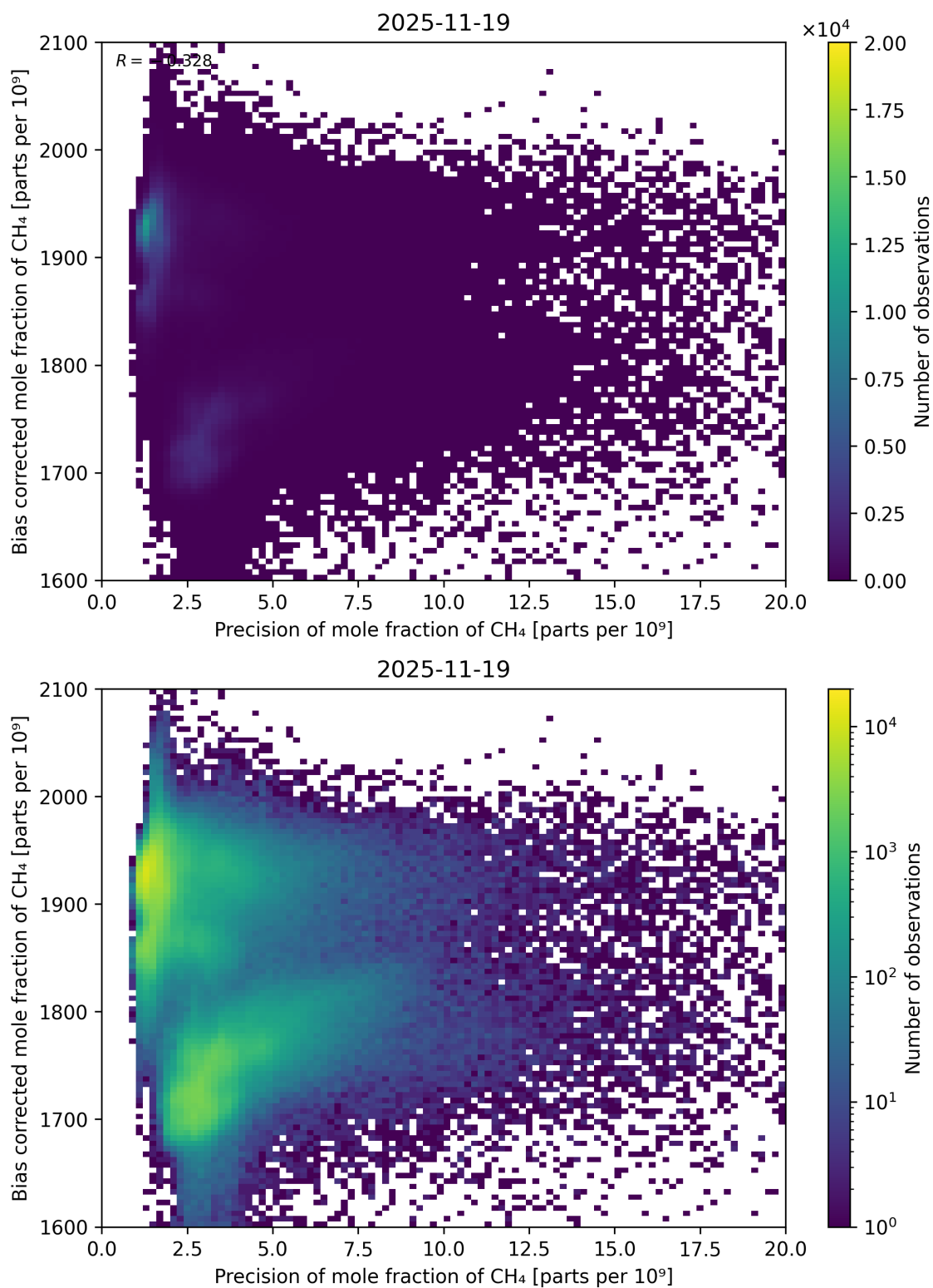
Figure 82: Scatter density plot of “Precision of mole fraction of CH 4 ” against “Bias corrected mole fraction of CH 4 ” for 2025-11-18 to 2025-11-20.
