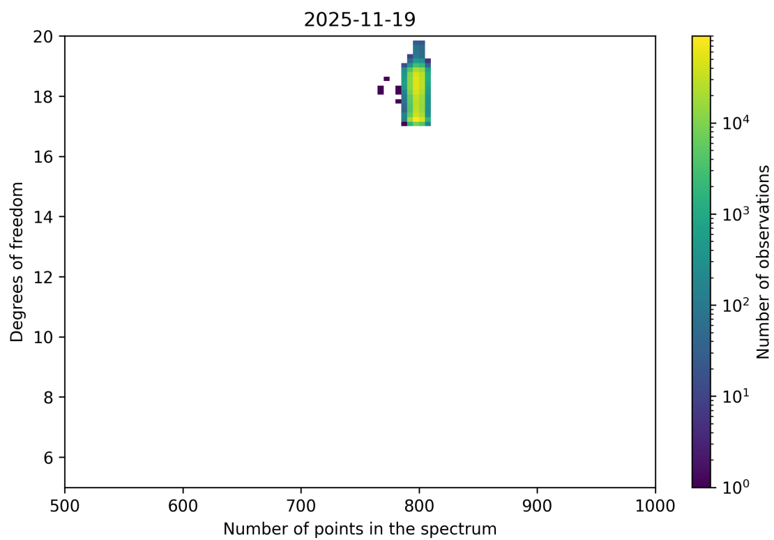
Figure 90: Scatter density plot of “Number of points in the spectrum” against “Degrees of freedom” for 2025-11-18 to 2025-11-20.
