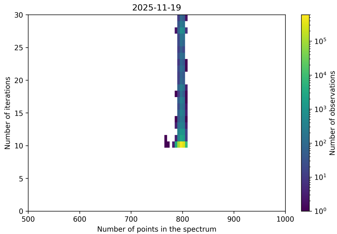
Figure 92: Scatter density plot of “Number of points in the spectrum” against “Number of iterations” for 2025-11-18 to 2025-11-20.
