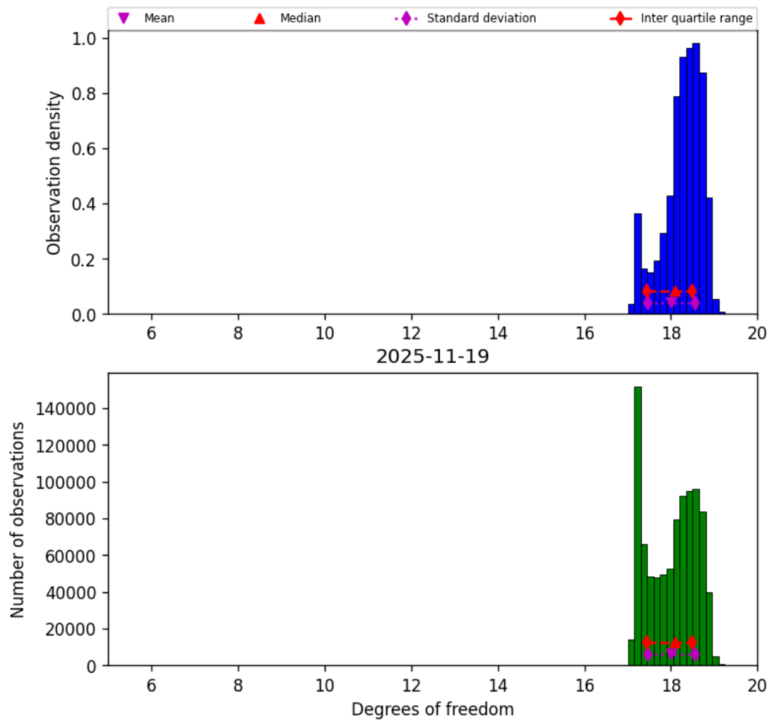
Figure 30: Histogram of “Degrees of freedom” for 2025-11-18 to 2025-11-20
