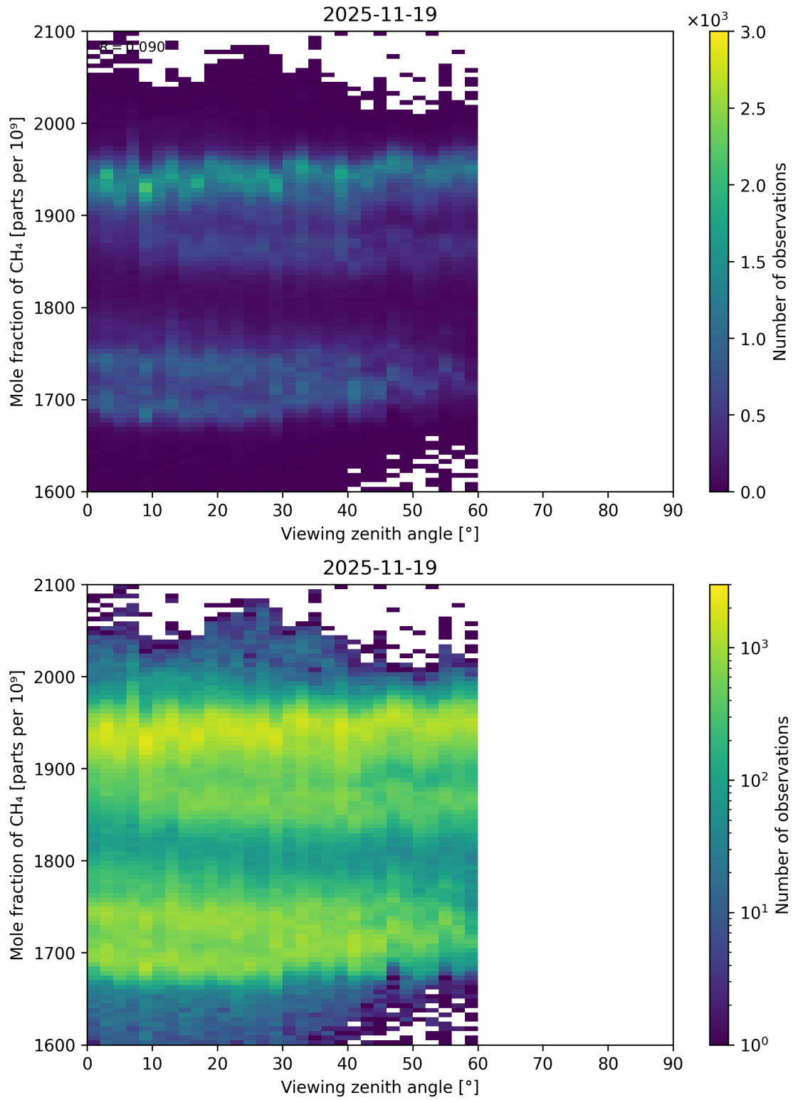
Figure 110: Scatter density plot of “Viewing zenith angle” against “Mole fraction of CH 4 ” for 2025-11-18 to 2025-11-20.
