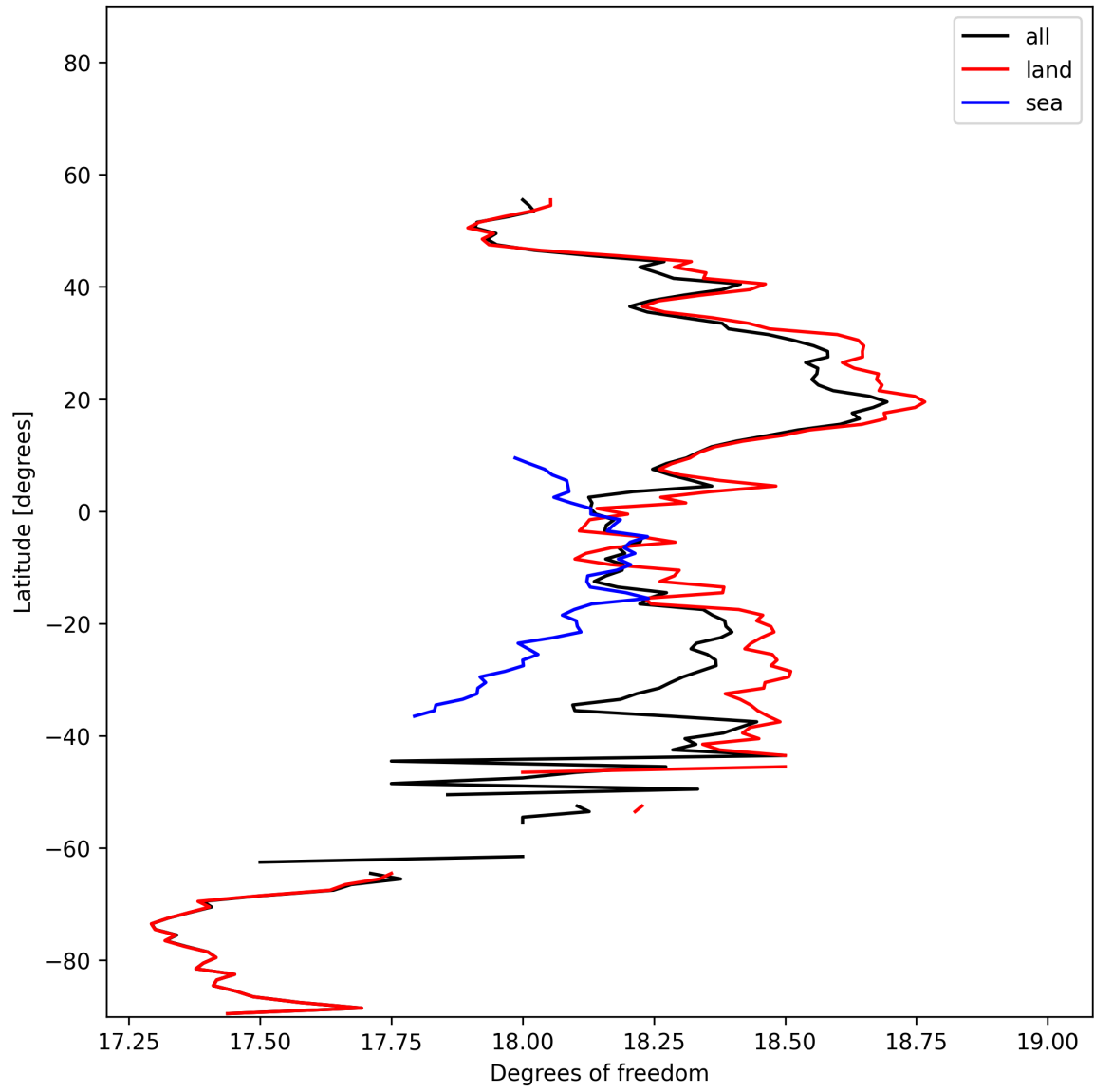
Figure 19: Zonal average of “Degrees of freedom” for 2025-11-18 to 2025-11-20.
