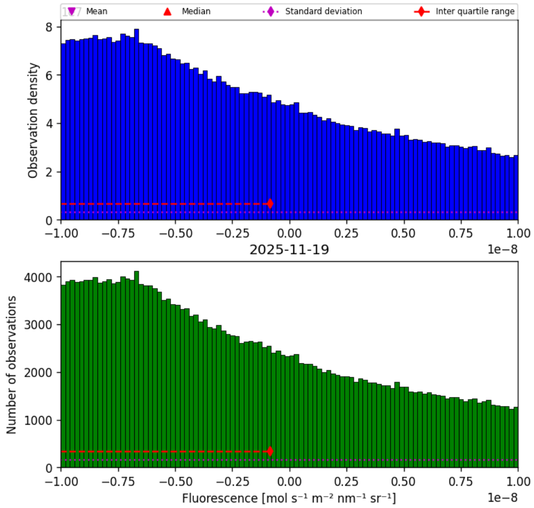
Figure 32: Histogram of “Fluorescence” for 2025-11-18 to 2025-11-20
