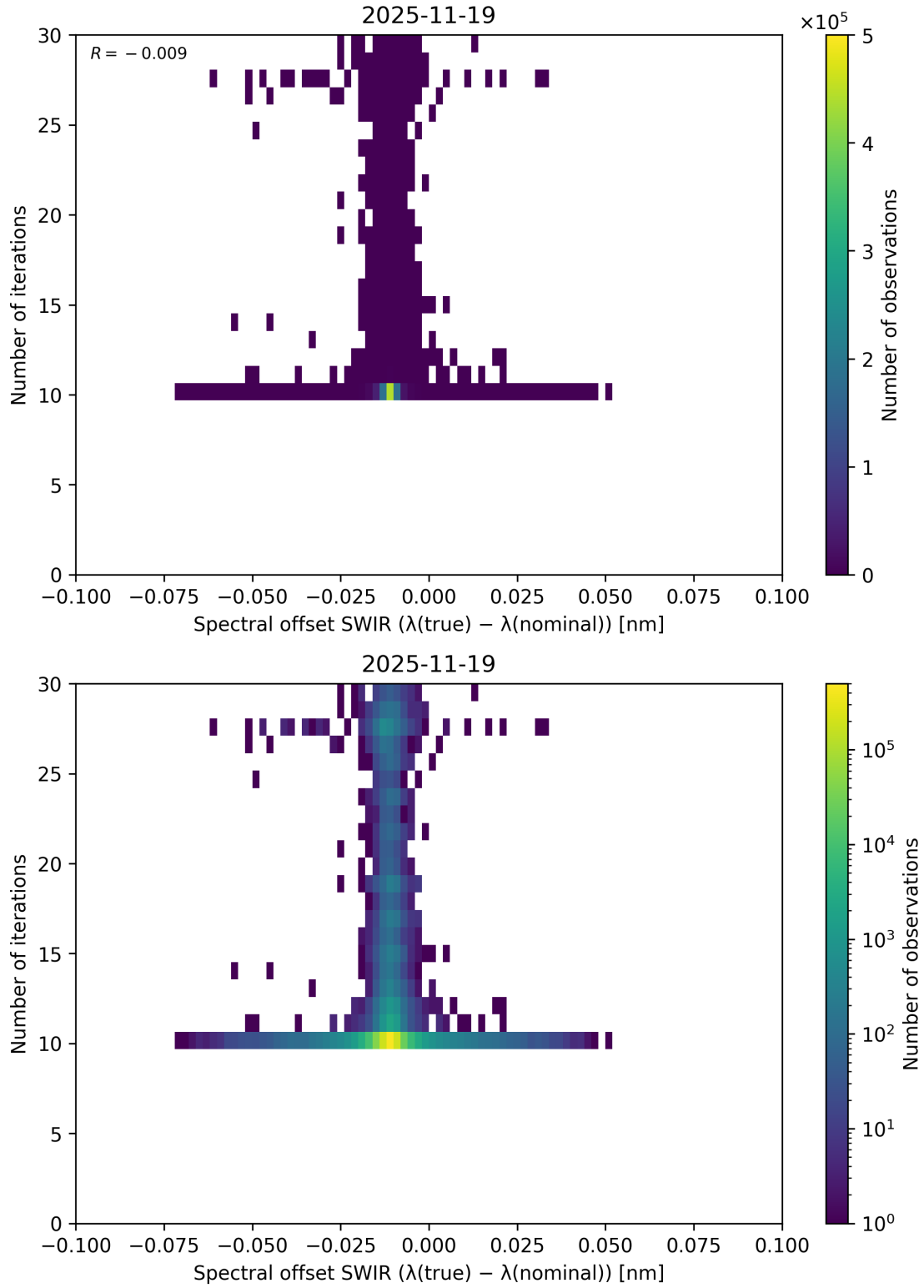
Figure 121: Scatter density plot of “Spectral offset SWIR ( \lambda_{\text{true}} - \lambda_{\text{nominal}} )” against “Number of iterations” for 2025-11-18 to 2025-11-20.
