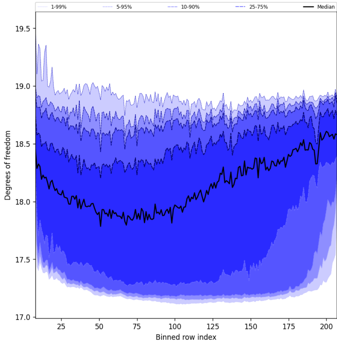
Figure 41: Along track statistics of “Degrees of freedom” for 2025-11-18 to 2025-11-20
