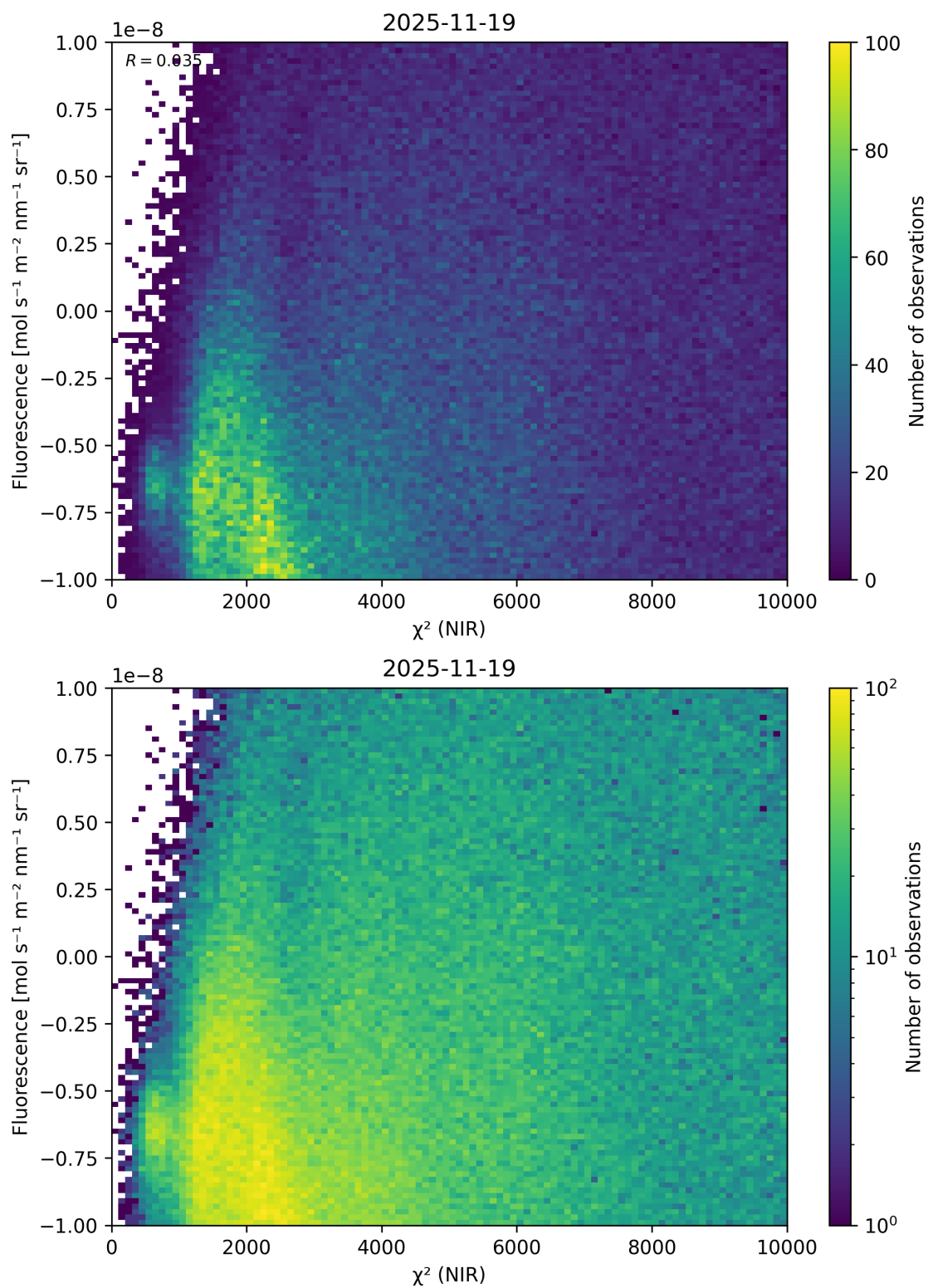
Figure 45: Scatter density plot of “ \chi^2 (NIR)” against “Fluorescence” for 2025-11-18 to 2025-11-20.
