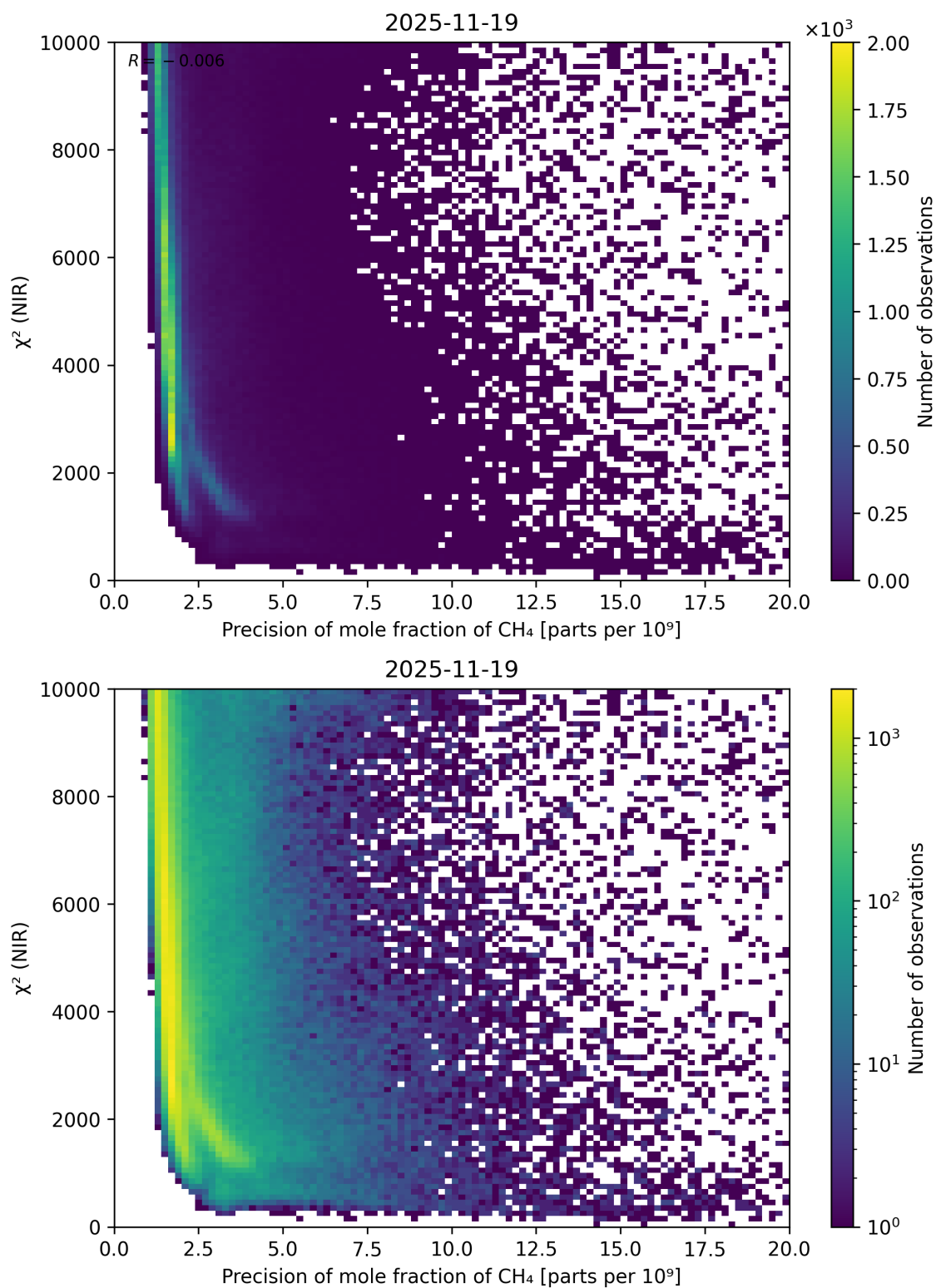
Figure 78: Scatter density plot of “Precision of mole fraction of CH 4 ” against “ \chi^2 (NIR)” for 2025-11-18 to 2025-11-20.
