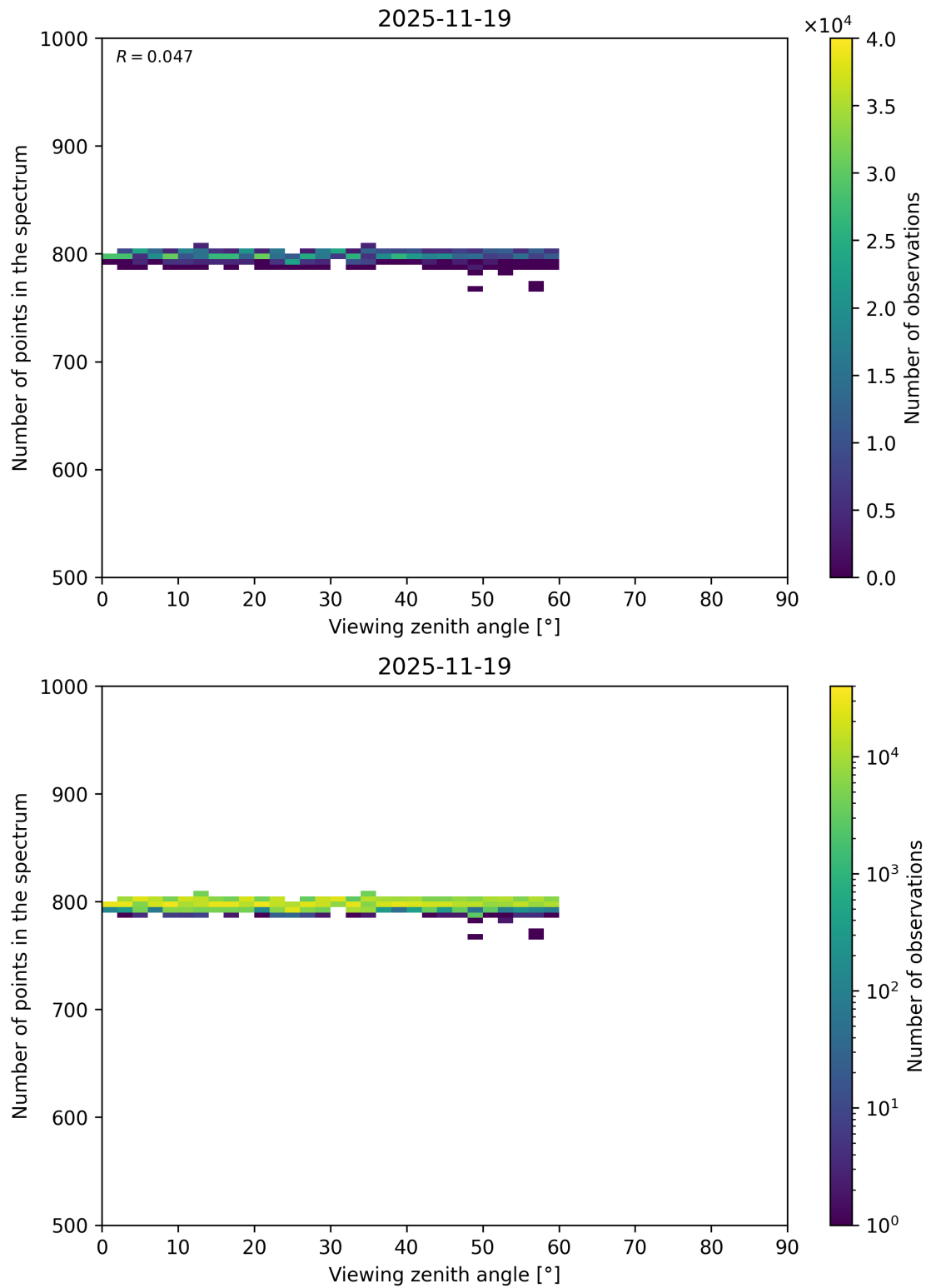
Figure 114: Scatter density plot of “Viewing zenith angle” against “Number of points in the spectrum” for 2025-11-18 to 2025-11-20.
