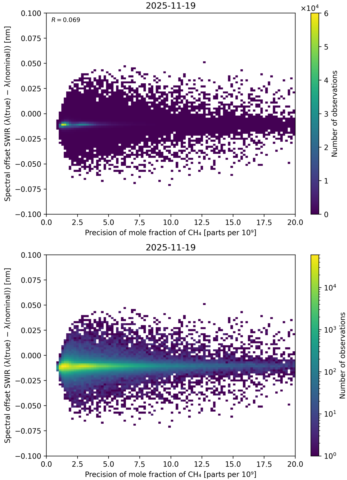
Figure 85: Scatter density plot of “Precision of mole fraction of CH 4 ” against “Spectral offset SWIR ( \lambda_{\text{true}} - \lambda_{\text{nominal}} )” for 2025-11-18 to 2025-11-20.
