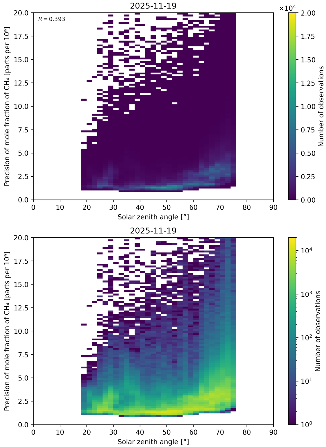
Figure 101: Scatter density plot of “Solar zenith angle” against “Precision of mole fraction of \text{CH}_4 ” for 2025-11-18 to 2025-11-20.
