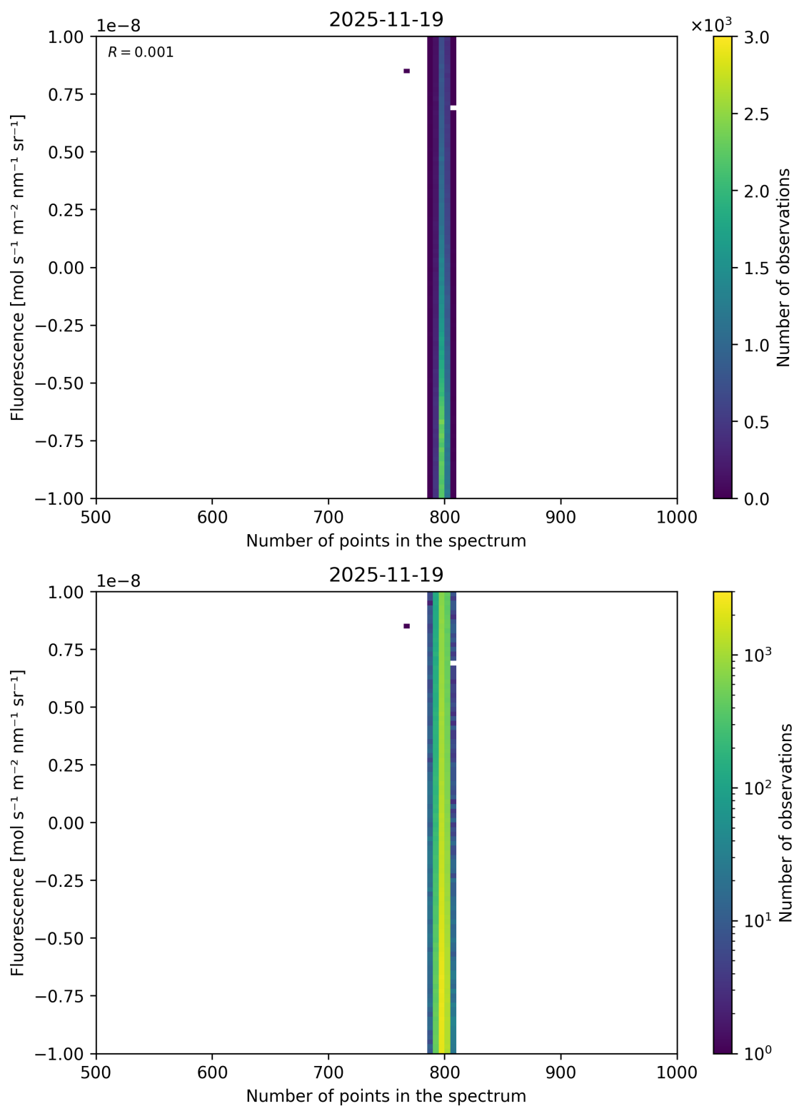
Figure 91: Scatter density plot of “Number of points in the spectrum” against “Fluorescence” for 2025-11-18 to 2025-11-20.
