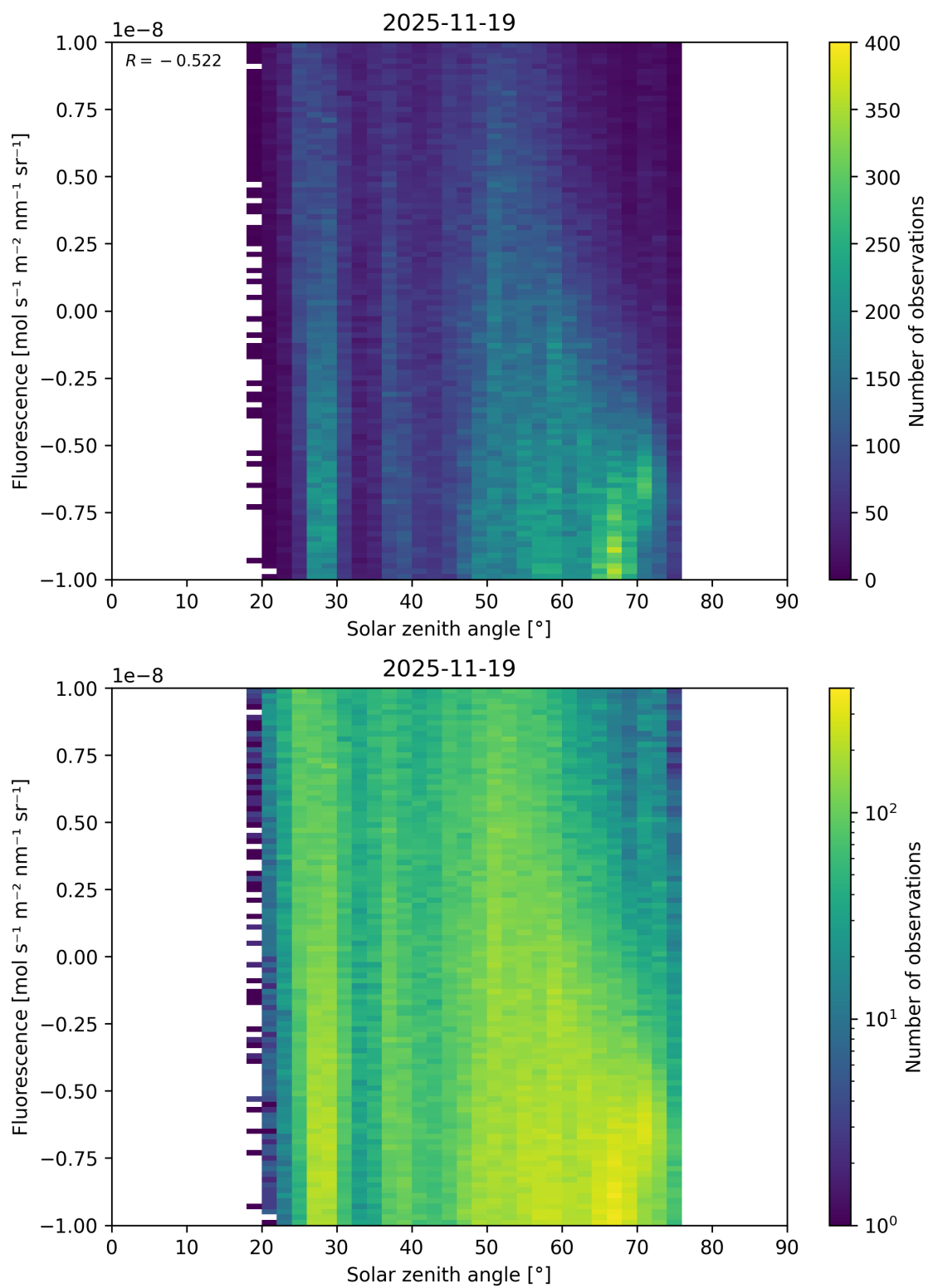
Figure 97: Scatter density plot of “Solar zenith angle” against “Fluorescence” for 2025-11-18 to 2025-11-20.
