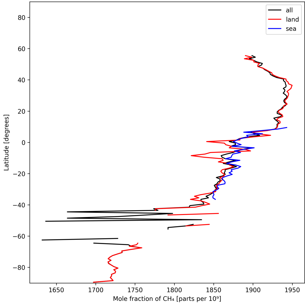
Figure 12: Zonal average of “Mole fraction of \text{CH}_4 ” for 2025-11-18 to 2025-11-20.
