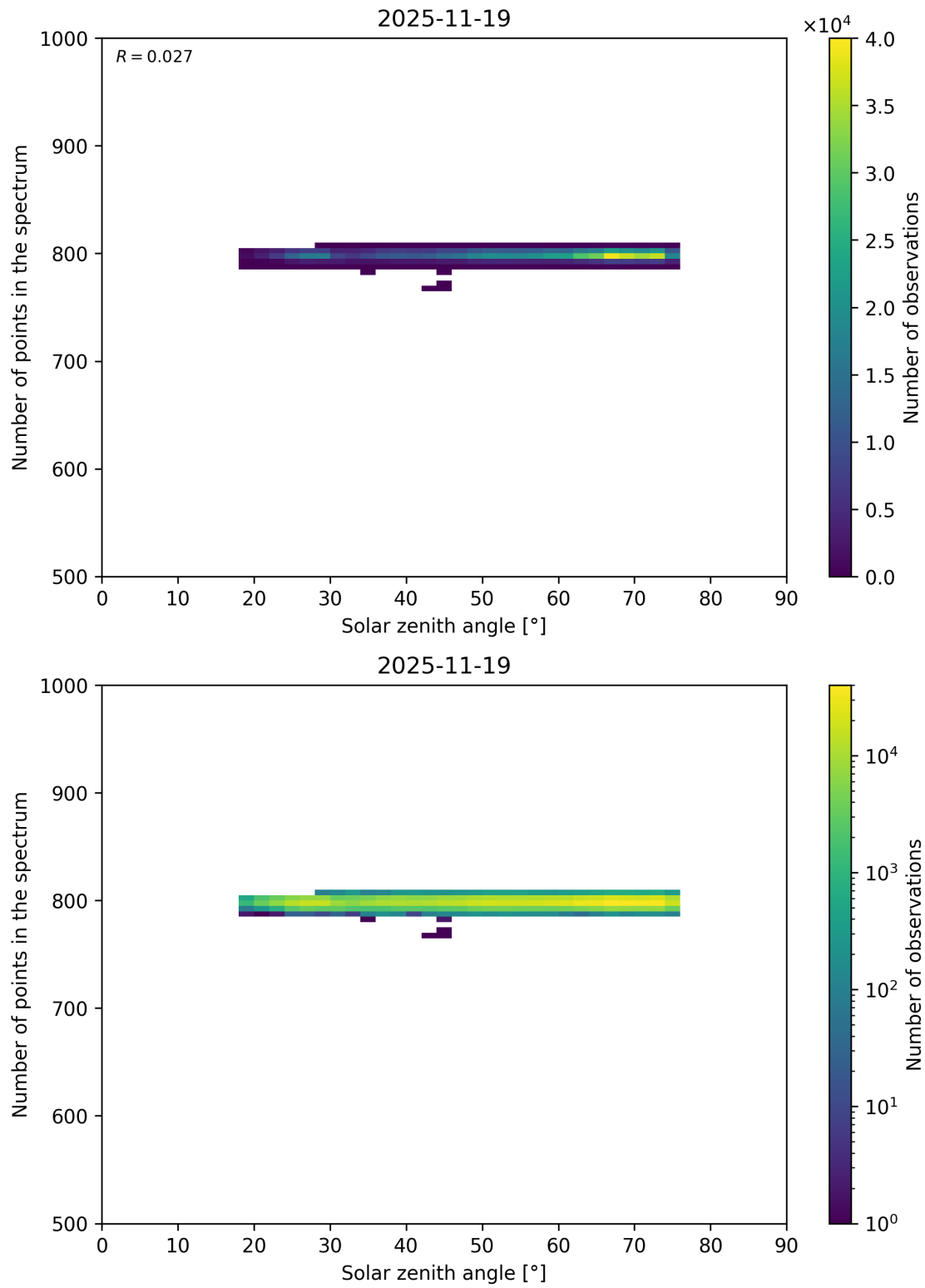
Figure 103: Scatter density plot of “Solar zenith angle” against “Number of points in the spectrum” for 2025-11-18 to 2025-11-20.
