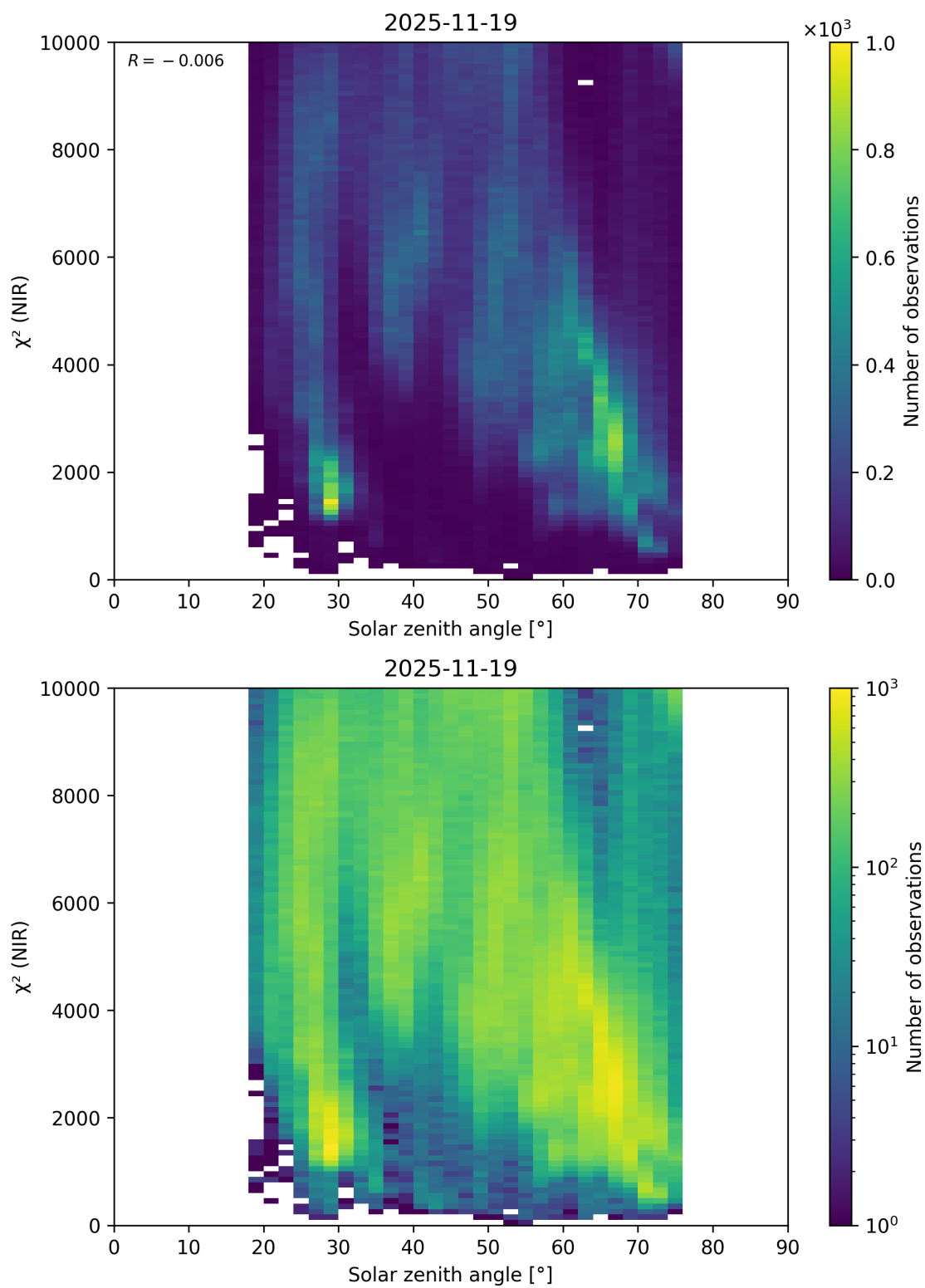
Figure 94: Scatter density plot of “Solar zenith angle” against “ \chi^2 (NIR)” for 2025-11-18 to 2025-11-20.
