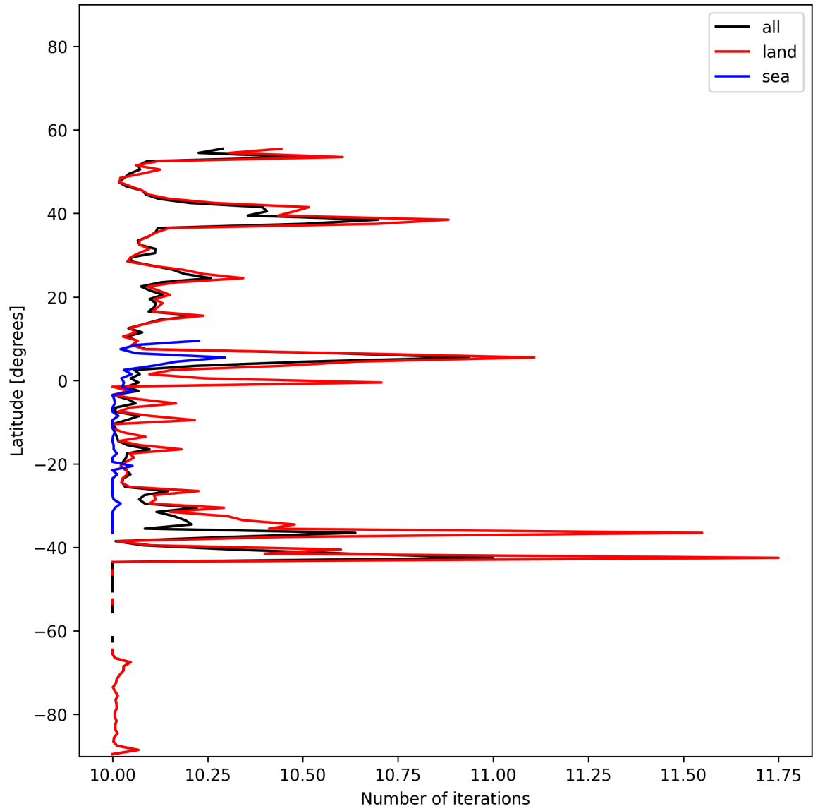
Figure 20: Zonal average of “Number of iterations” for 2025-11-18 to 2025-11-20.
