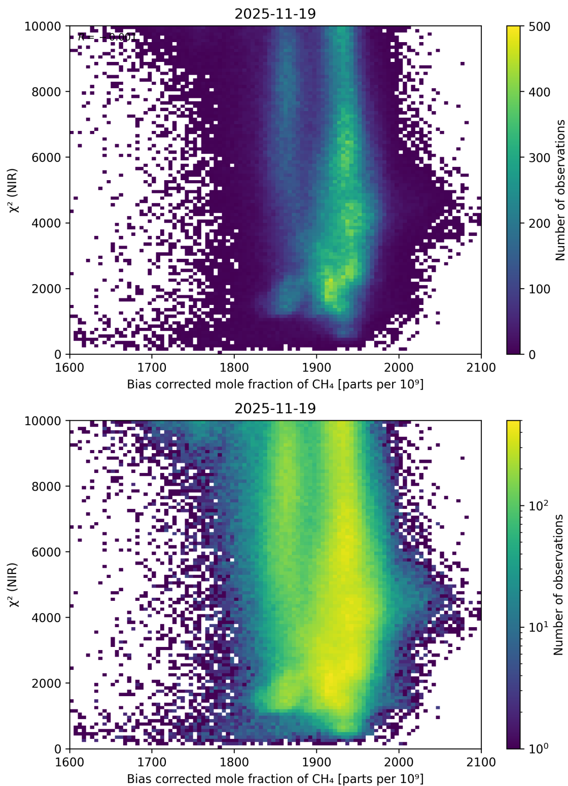
Figure 63: Scatter density plot of “Bias corrected mole fraction of CH 4 ” against “ \chi^2 (NIR)” for 2025-11-18 to 2025-11-20.
