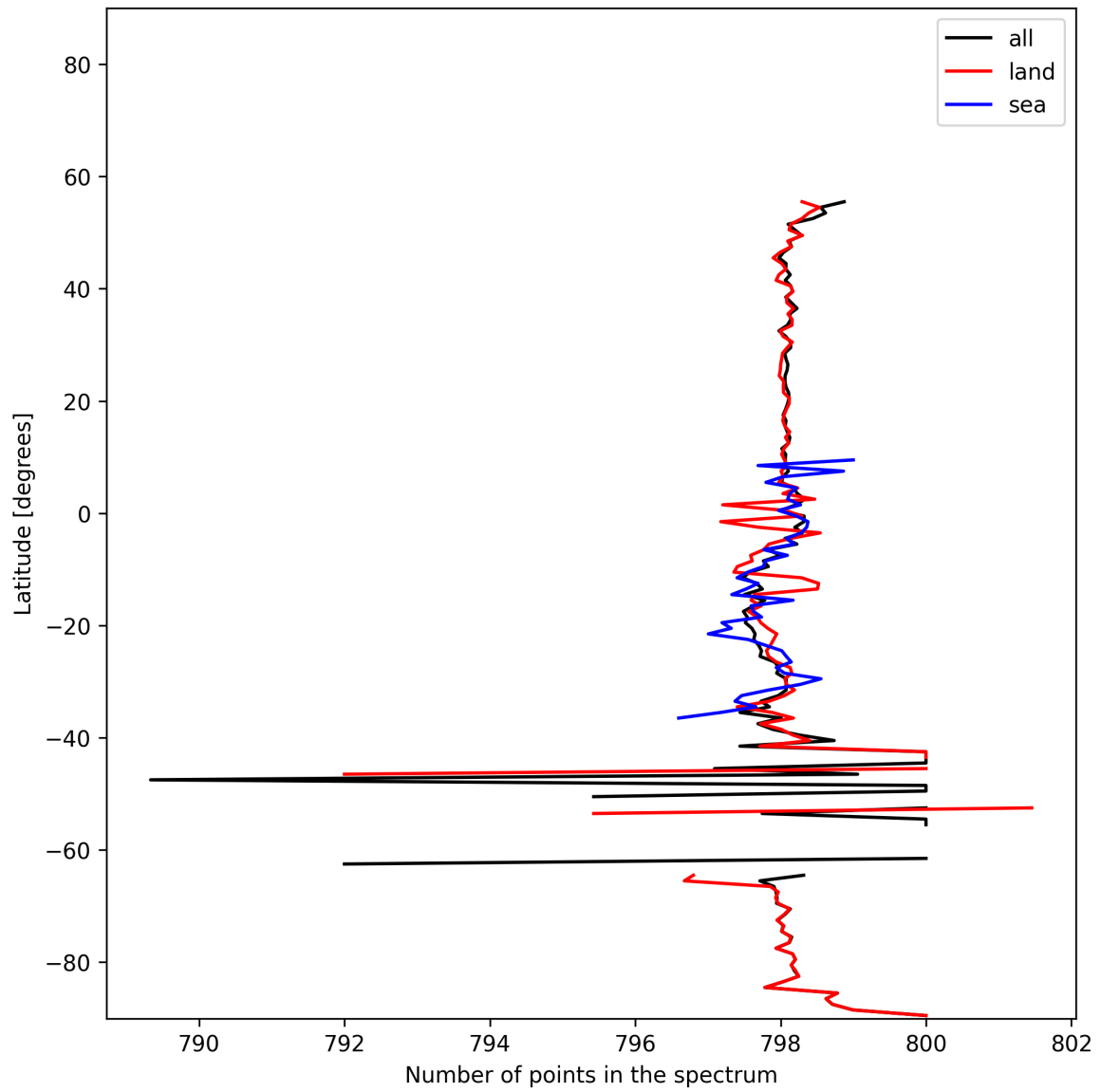
Figure 15: Zonal average of “Number of points in the spectrum” for 2025-11-18 to 2025-11-20.
