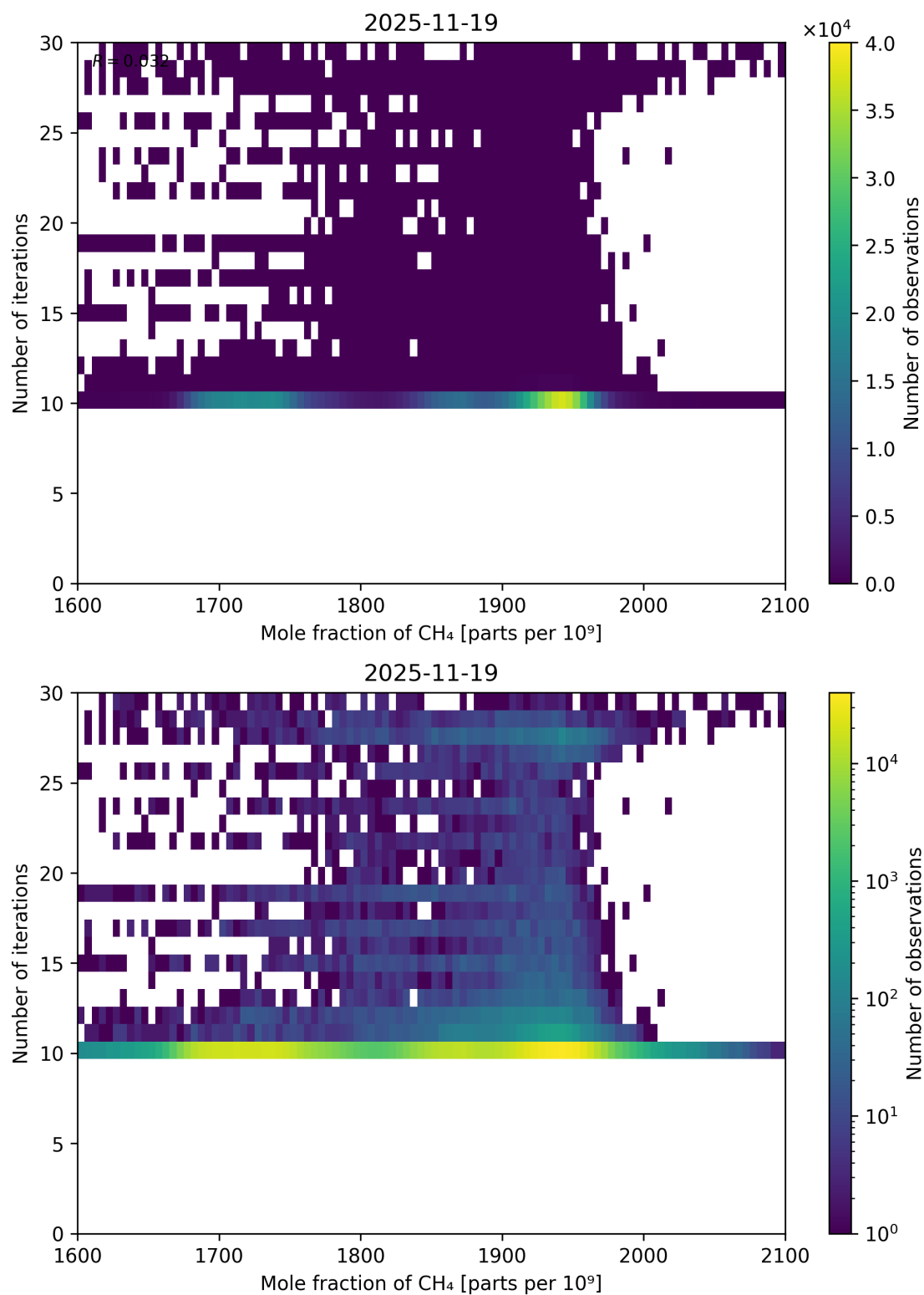
Figure 76: Scatter density plot of “Mole fraction of CH 4 ” against “Number of iterations” for 2025-11-18 to 2025-11-20.
