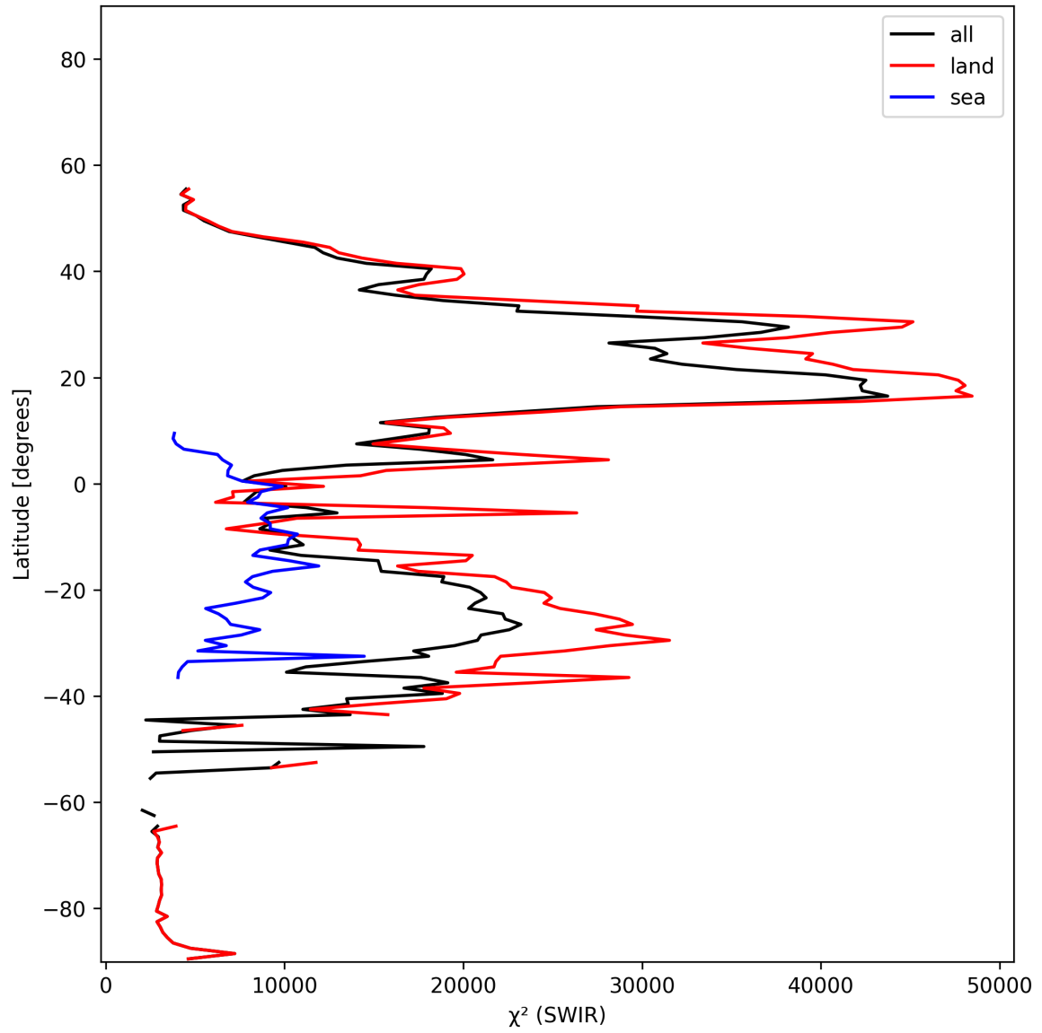
Figure 17: Zonal average of “ \chi^2 (SWIR)” for 2025-11-18 to 2025-11-20.
