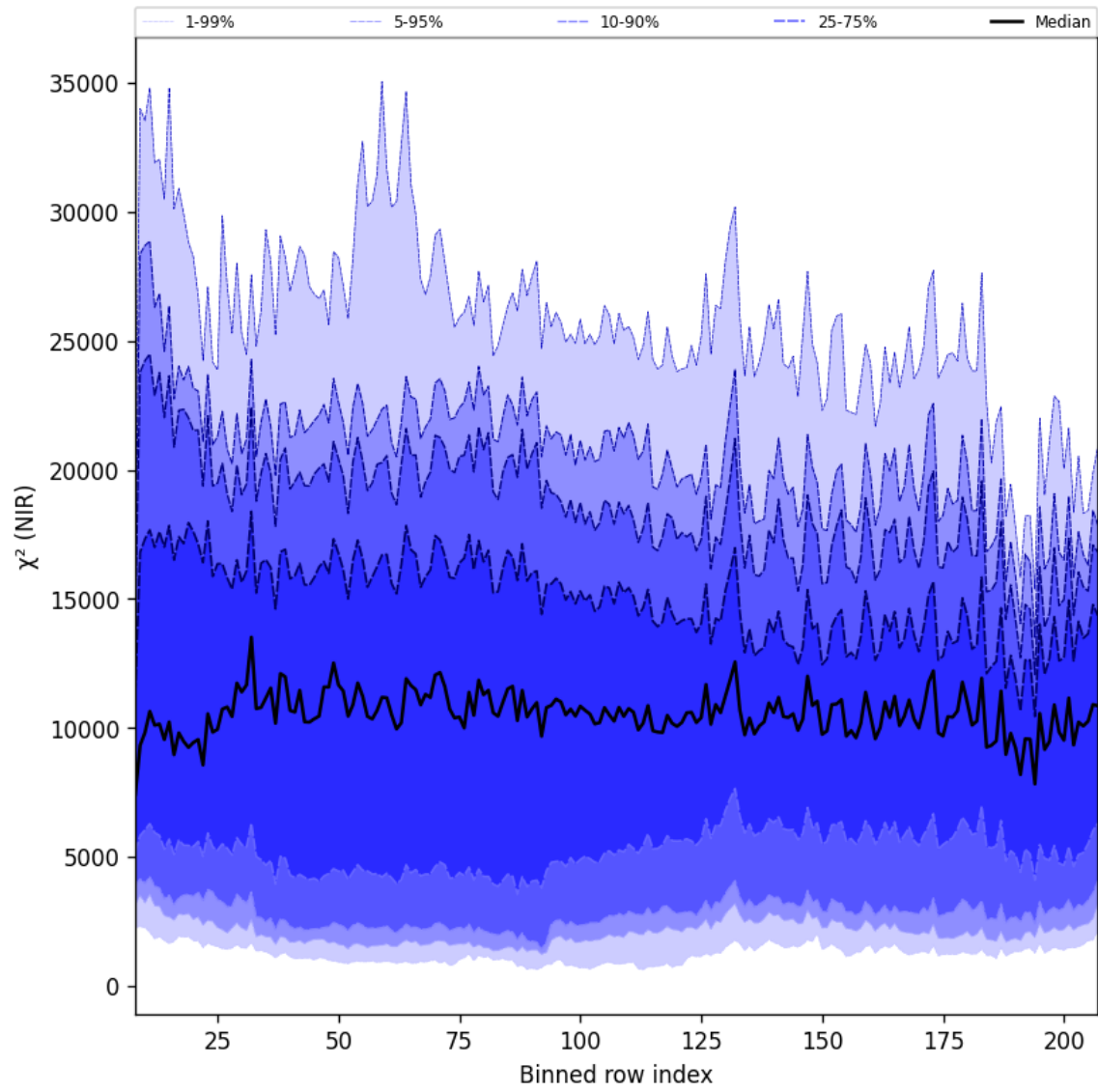
Figure 40: Along track statistics of “ \chi^2 (NIR)” for 2025-11-18 to 2025-11-20
