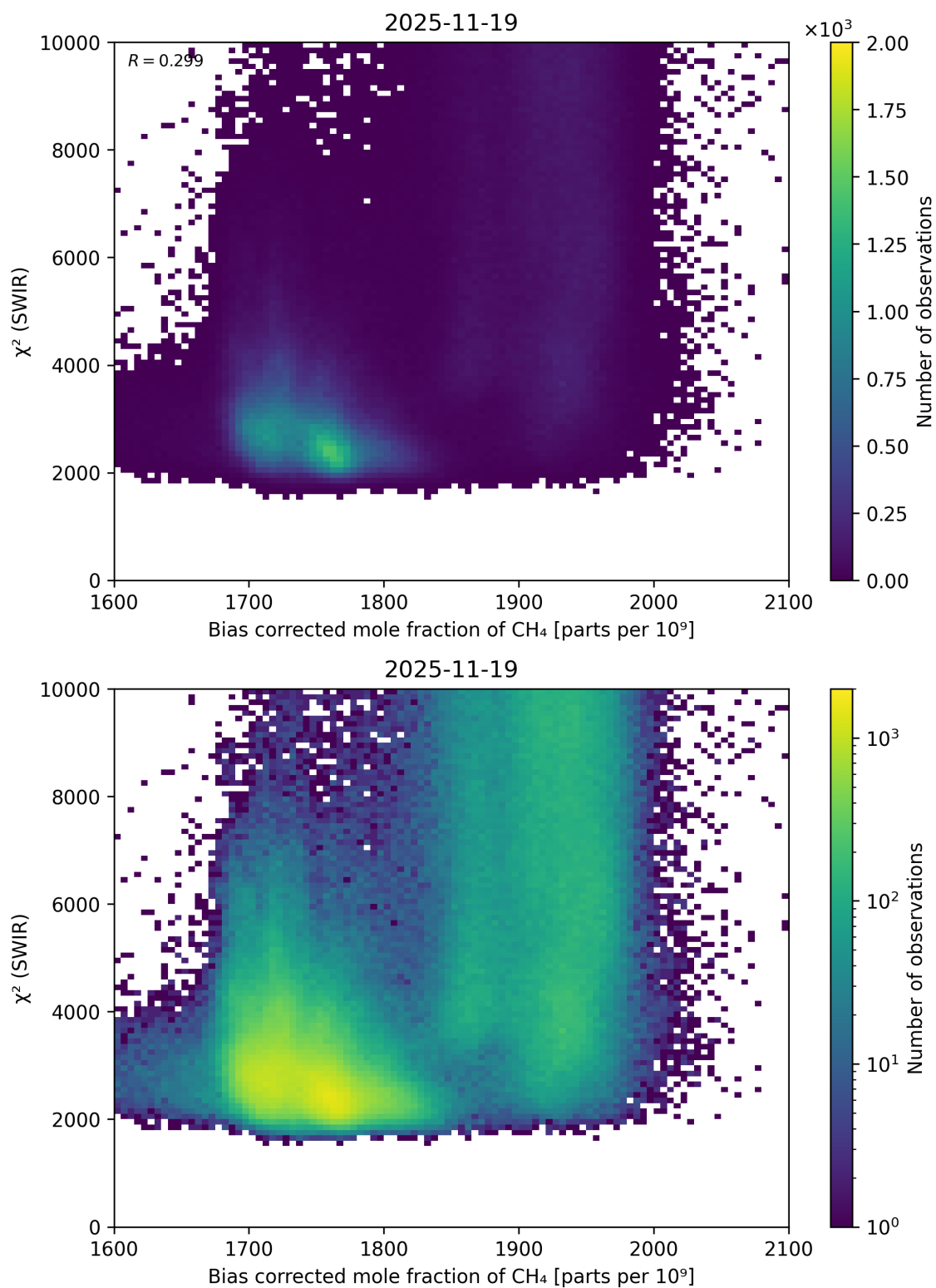
Figure 64: Scatter density plot of “Bias corrected mole fraction of \text{CH}_4 ” against “ \chi^2 (SWIR)” for 2025-11-18 to 2025-11-20.
