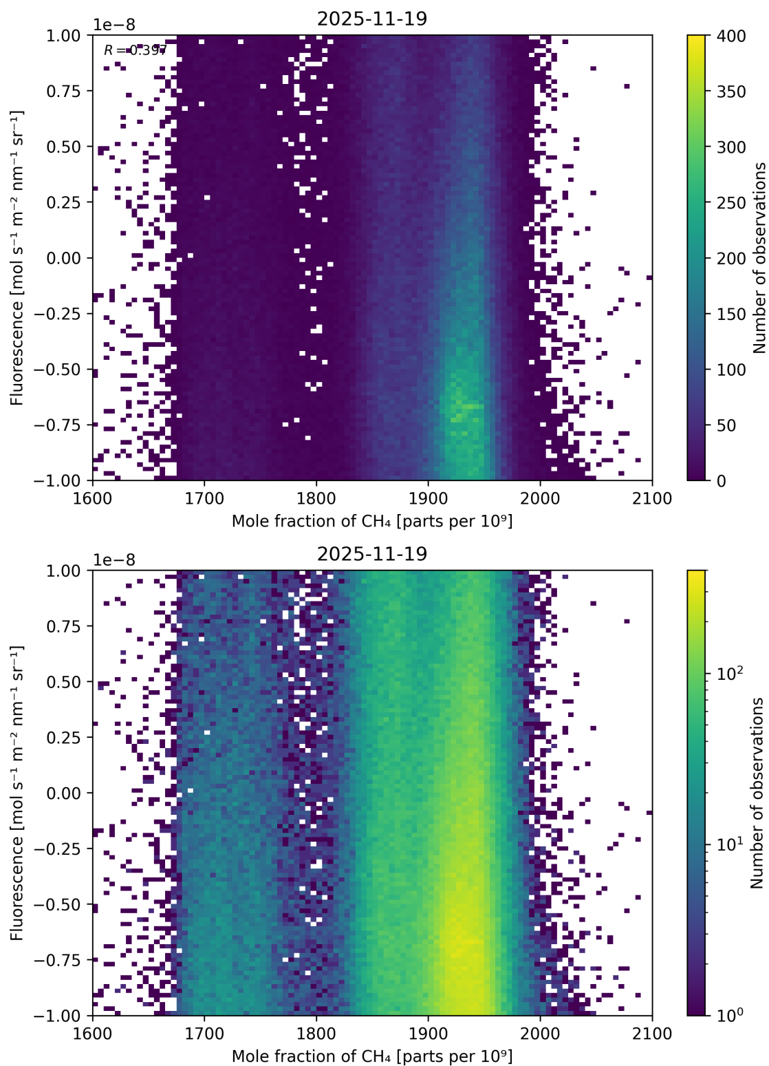
Figure 73: Scatter density plot of “Mole fraction of \text{CH}_4 ” against “Fluorescence” for 2025-11-18 to 2025-11-20.
