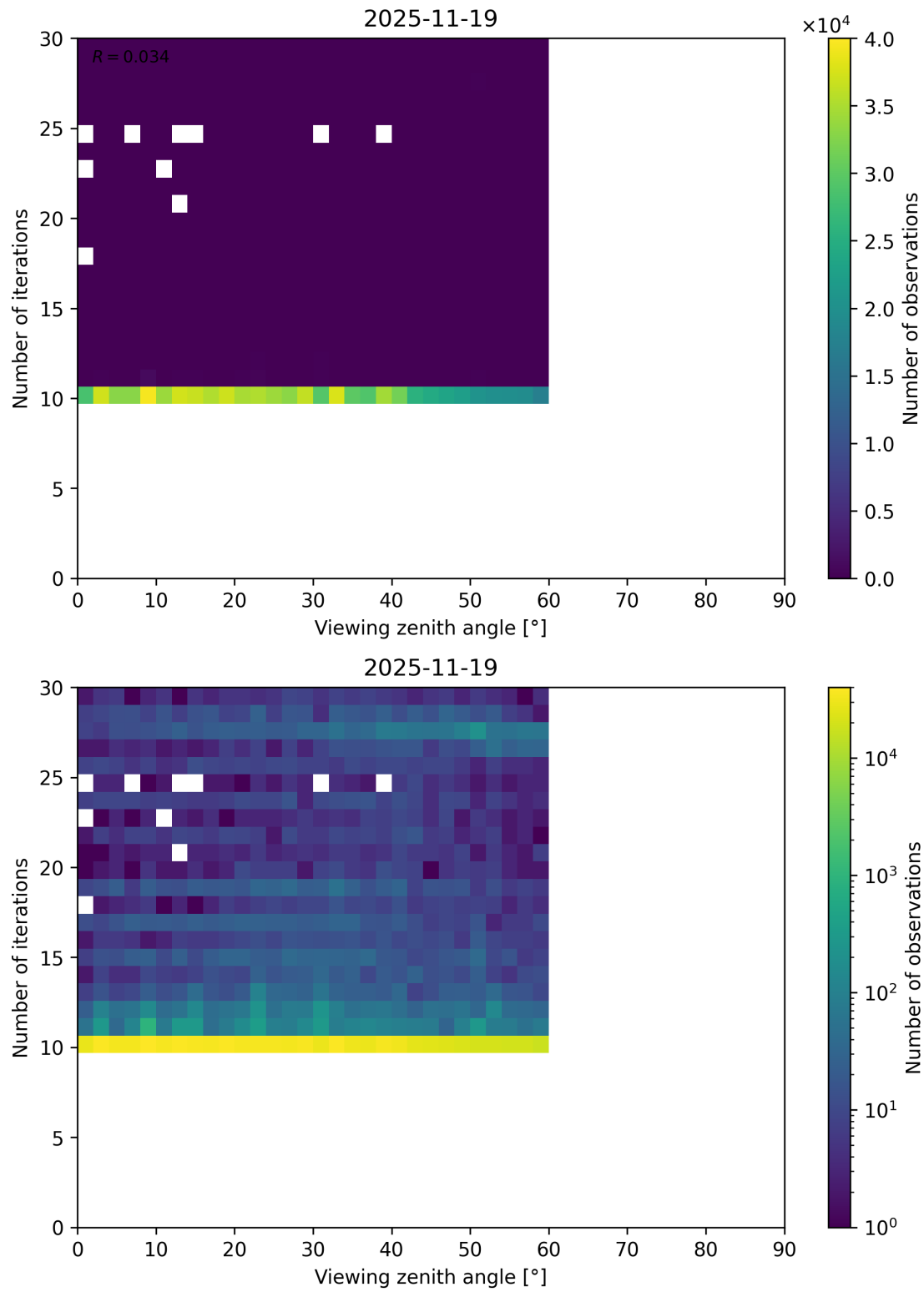
Figure 113: Scatter density plot of “Viewing zenith angle” against “Number of iterations” for 2025-11-18 to 2025-11-20.
