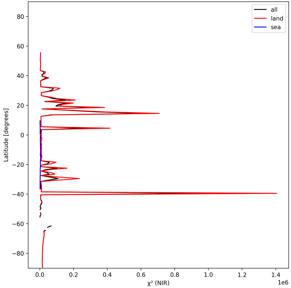
Figure 18: Zonal average of “ \chi^2 (NIR)” for 2025-11-18 to 2025-11-20.
