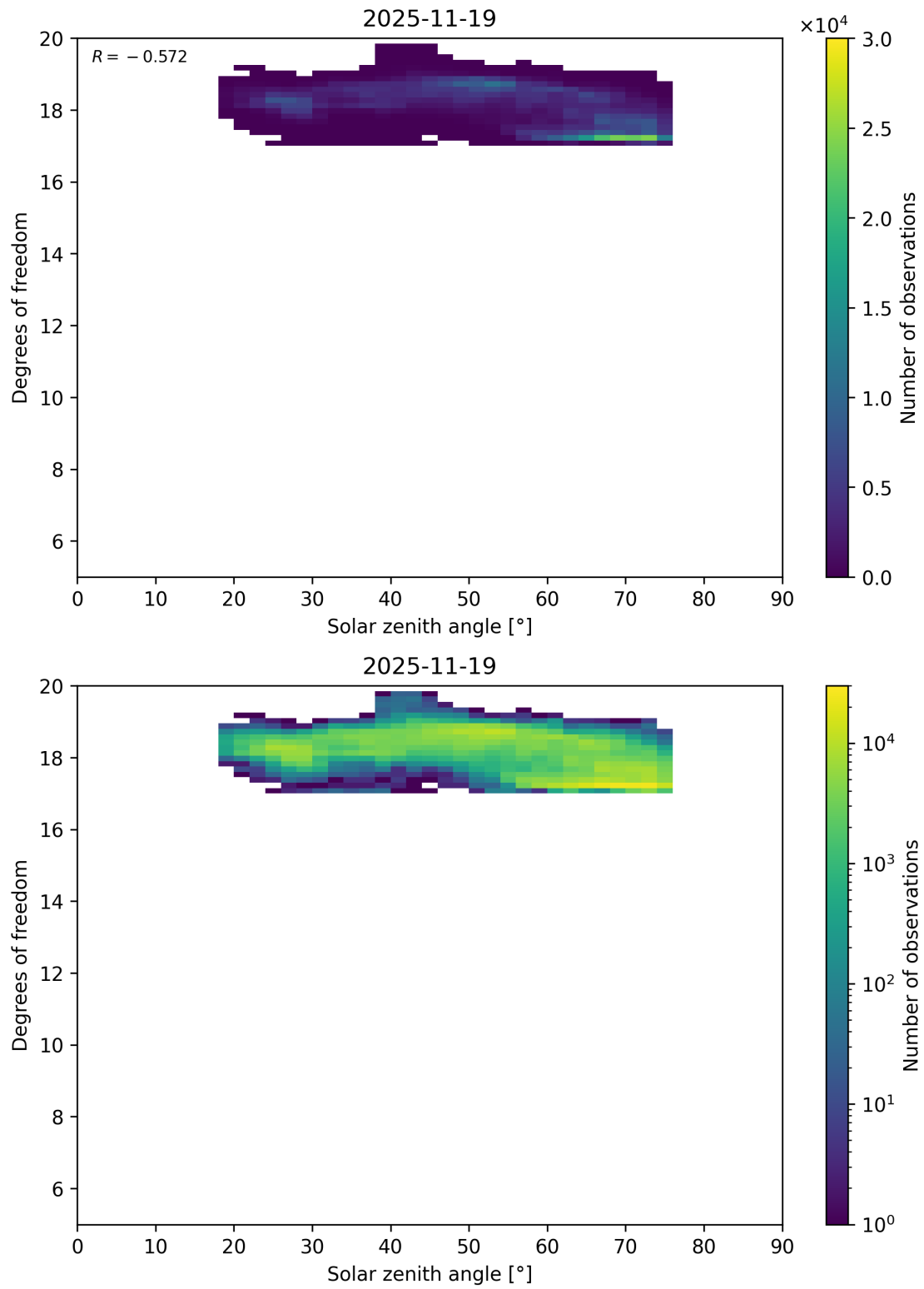
Figure 96: Scatter density plot of “Solar zenith angle” against “Degrees of freedom” for 2025-11-18 to 2025-11-20.
