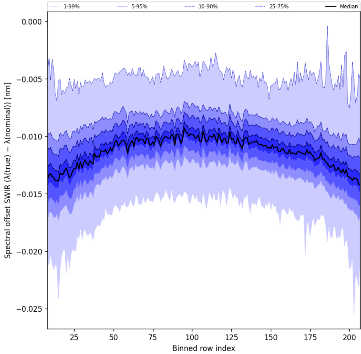
Figure 38: Along track statistics of “Spectral offset SWIR ( \lambda_{\text{true}} - \lambda_{\text{nominal}} )” for 2025-11-18 to 2025-11-20
