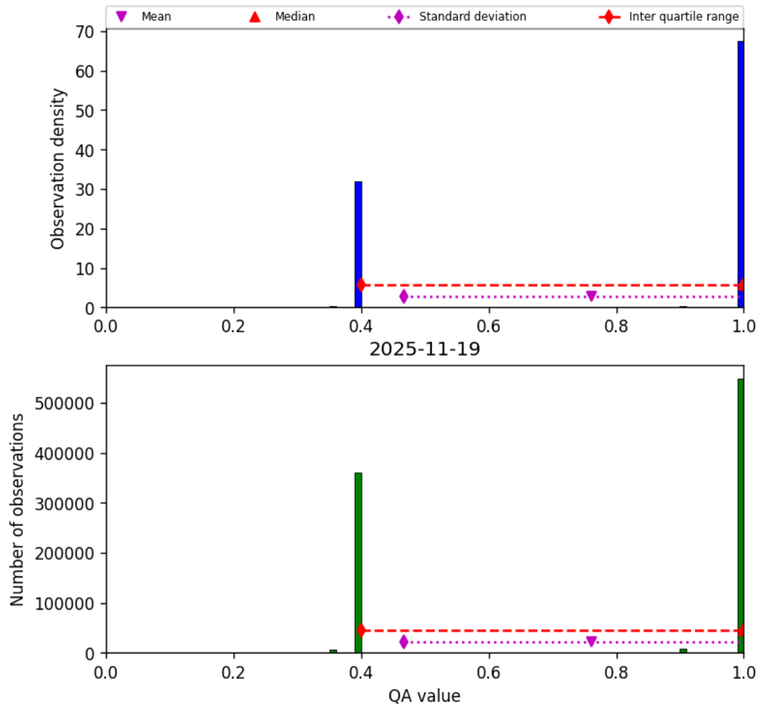
Figure 22: Histogram of “QA value” for 2025-11-18 to 2025-11-20
