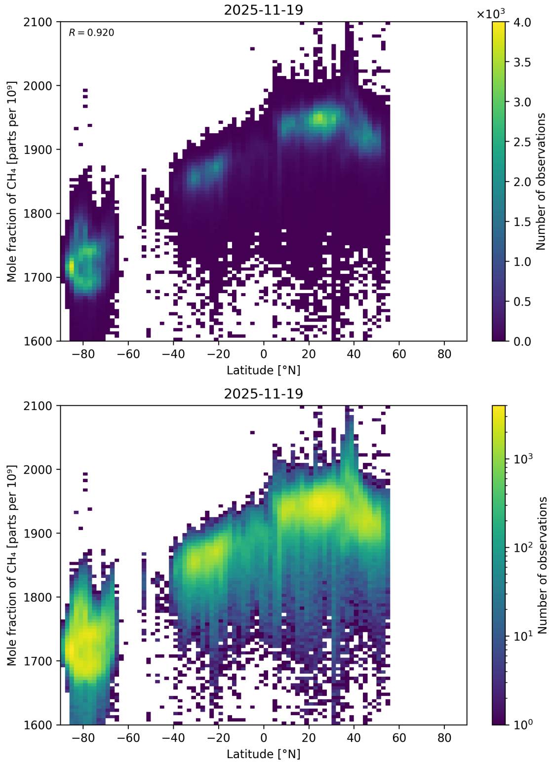
Figure 57: Scatter density plot of “Latitude” against “Mole fraction of CH 4 ” for 2025-11-18 to 2025-11-20.
