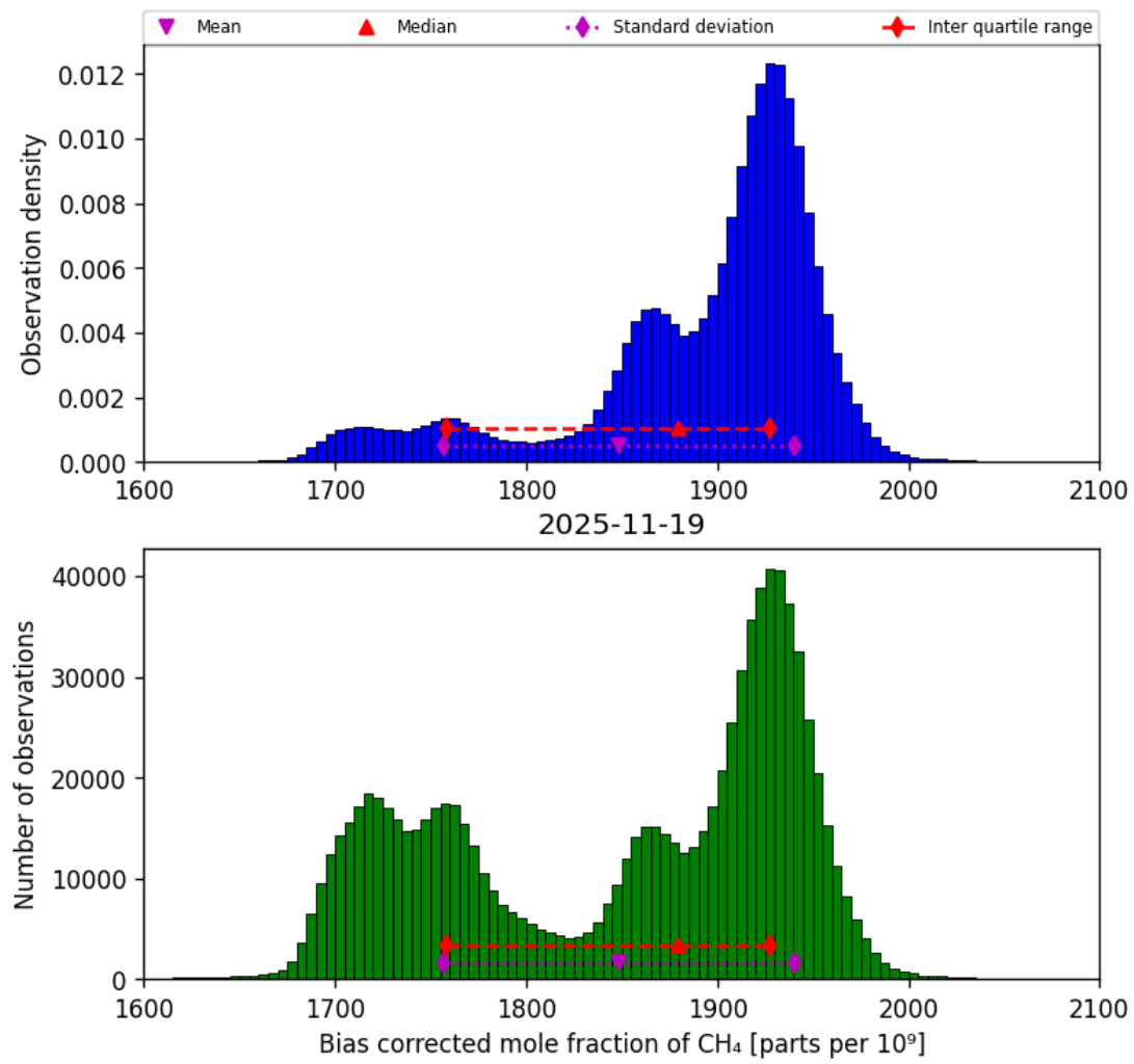
Figure 25: Histogram of “Bias corrected mole fraction of CH 4 ” for 2025-11-18 to 2025-11-20
