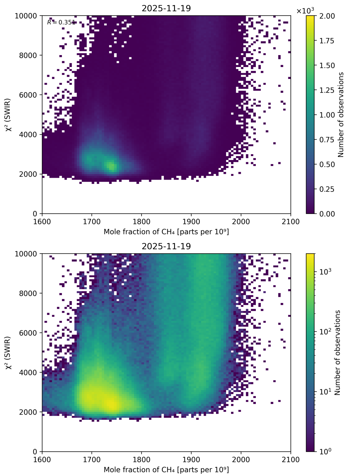
Figure 71: Scatter density plot of “Mole fraction of \text{CH}_4 ” against “ \chi^2 (SWIR)” for 2025-11-18 to 2025-11-20.
