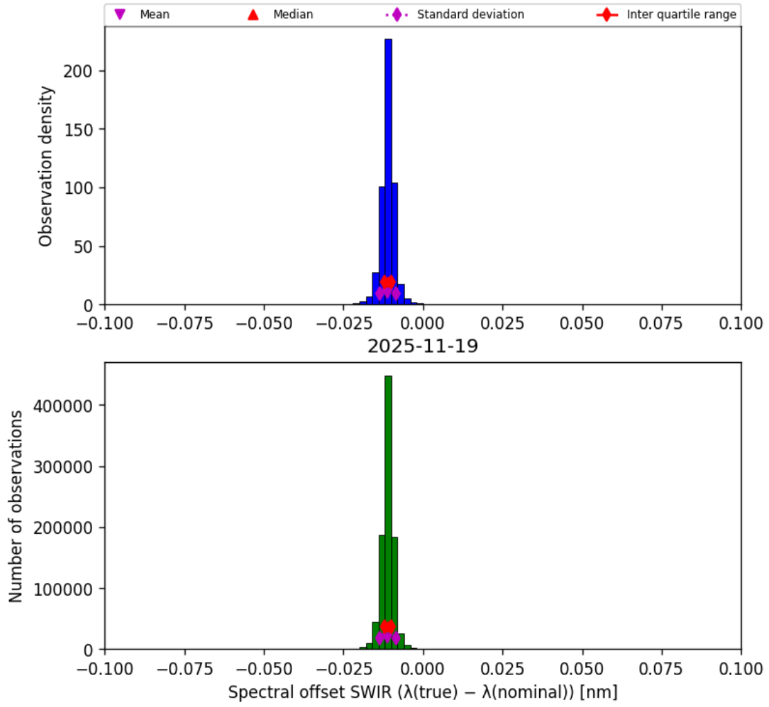
Figure 27: Histogram of “Spectral offset SWIR ( \lambda_{\text{true}} - \lambda_{\text{nominal}} )” for 2025-11-18 to 2025-11-20
