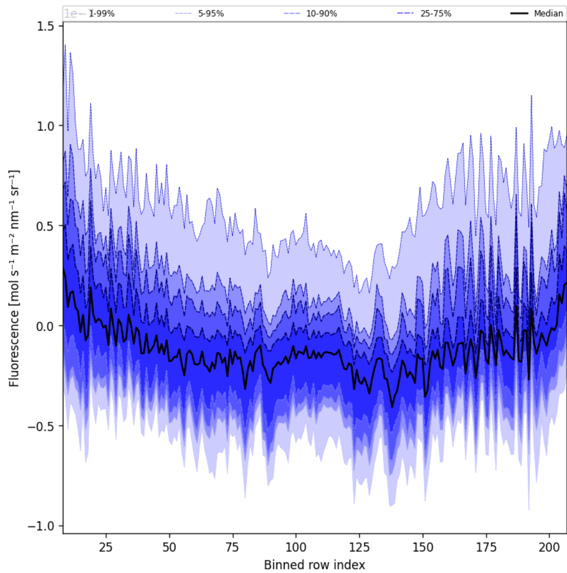
Figure 43: Along track statistics of “Fluorescence” for 2025-11-18 to 2025-11-20
