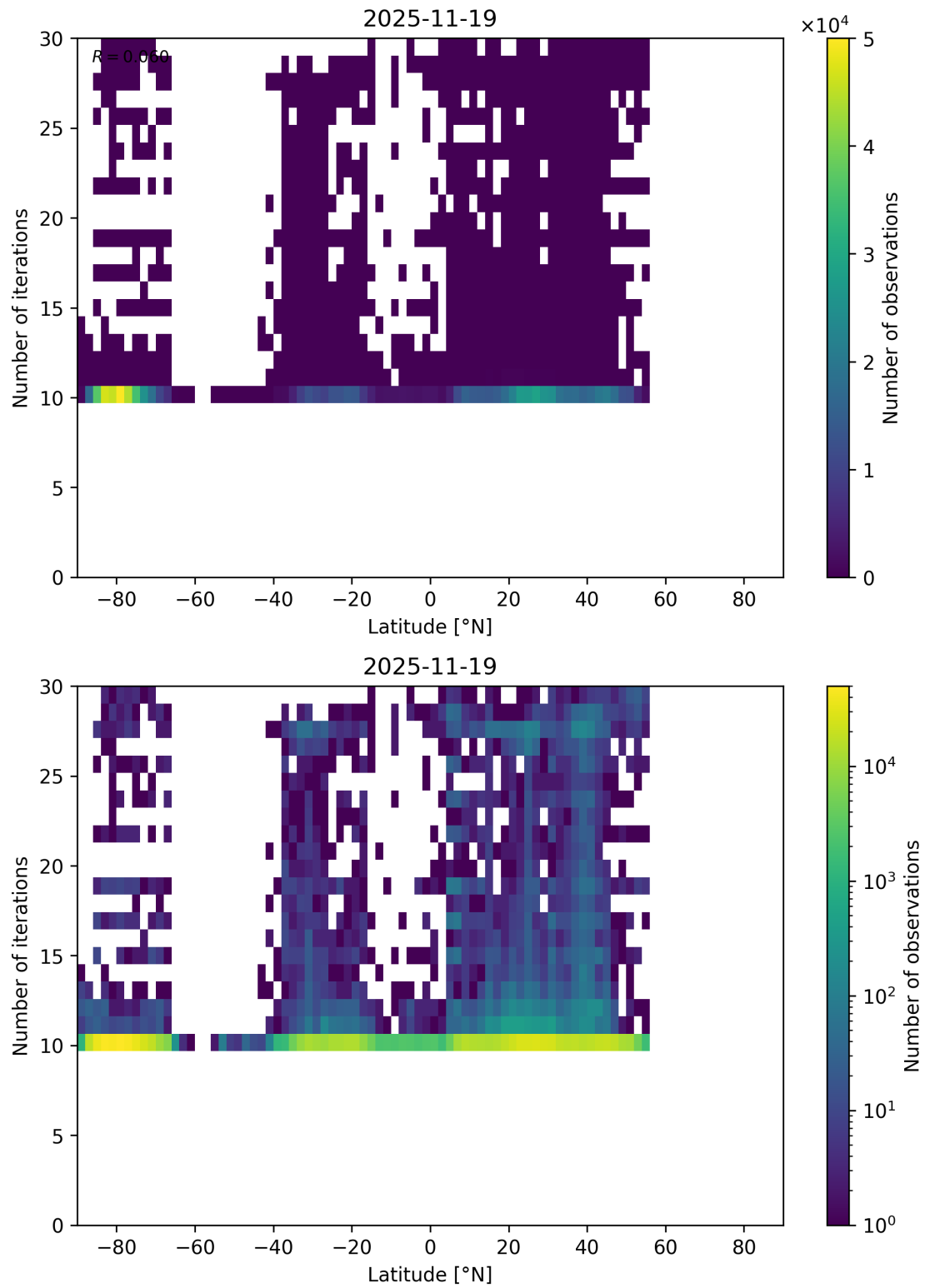
Figure 60: Scatter density plot of “Latitude” against “Number of iterations” for 2025-11-18 to 2025-11-20.
