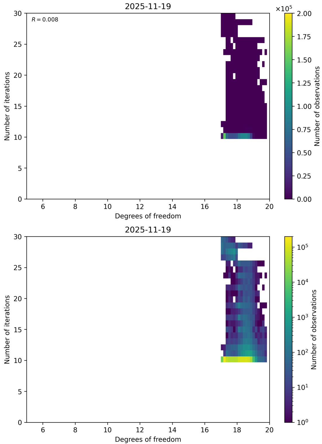
Figure 52: Scatter density plot of “Degrees of freedom” against “Number of iterations” for 2025-11-18 to 2025-11-20.
