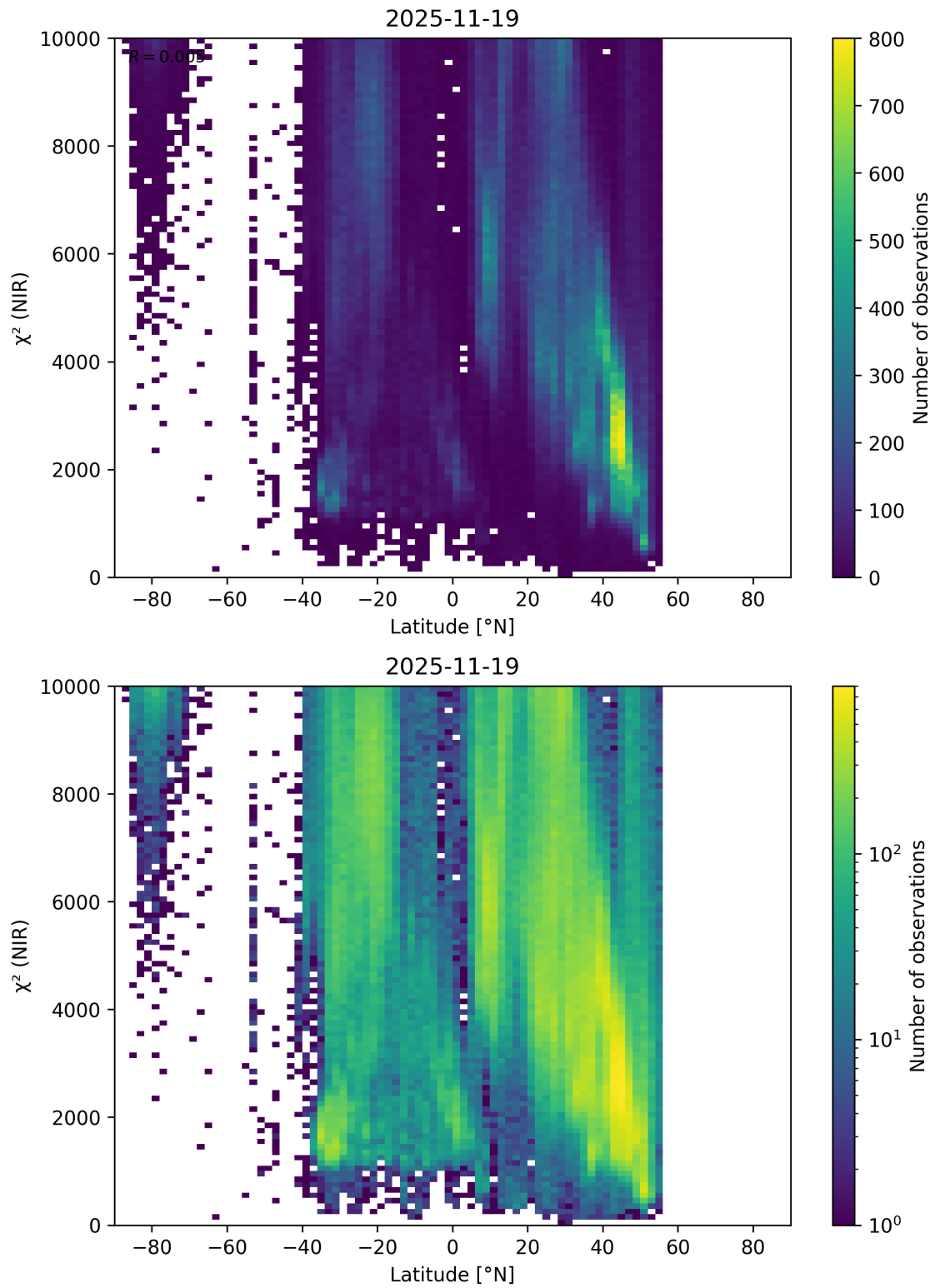
Figure 53: Scatter density plot of “Latitude” against “ \chi^2 (NIR)” for 2025-11-18 to 2025-11-20.
