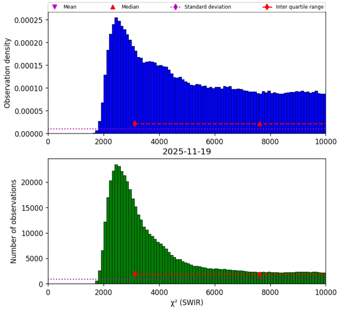
Figure 28: Histogram of “ \chi^2 (SWIR)” for 2025-11-18 to 2025-11-20
