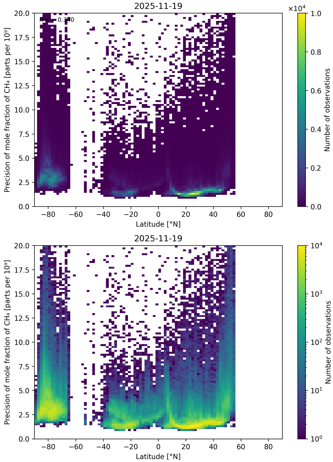
Figure 59: Scatter density plot of “Latitude” against “Precision of mole fraction of CH 4 ” for 2025-11-18 to 2025-11-20.
