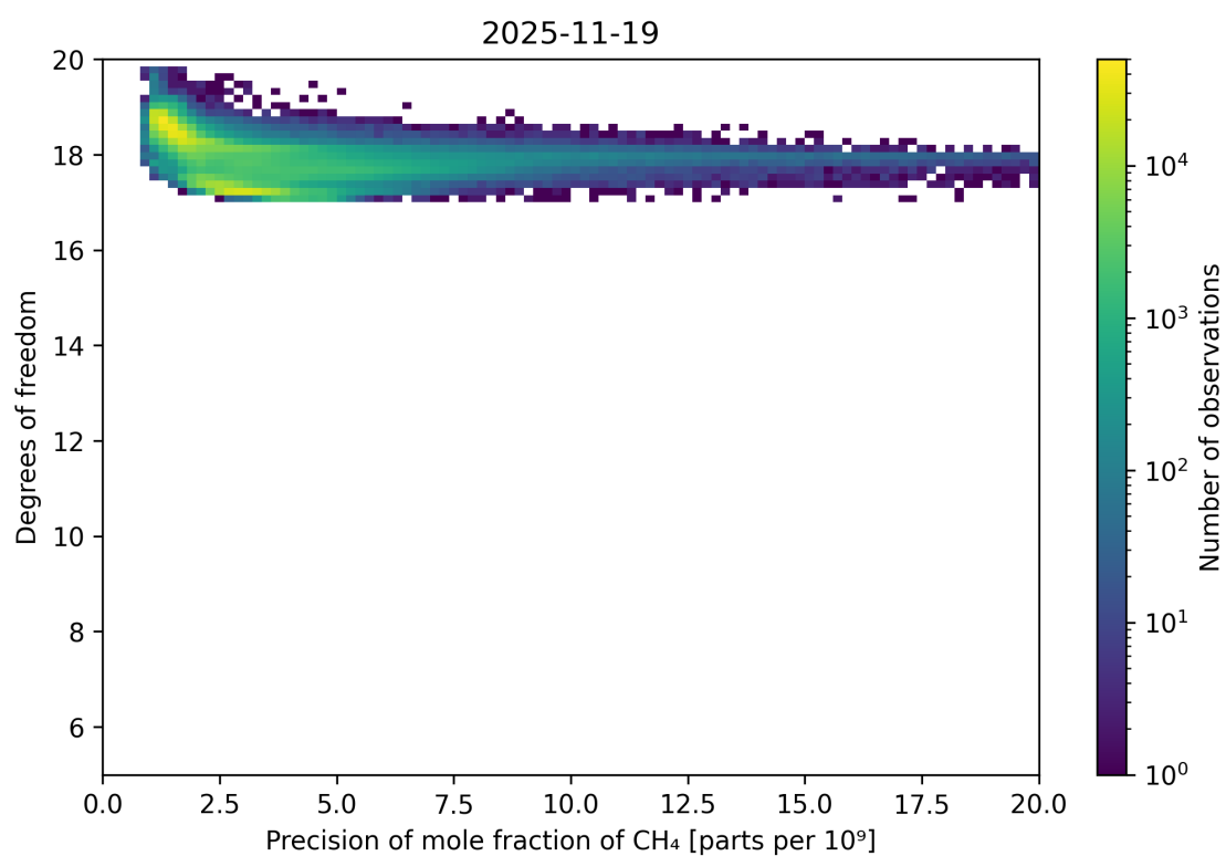
Figure 80: Scatter density plot of “Precision of mole fraction of CH 4 ” against “Degrees of freedom” for 2025-11-18 to 2025-11-20.
