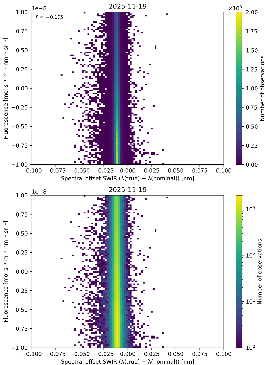
Figure 120: Scatter density plot of “Spectral offset SWIR ( \lambda_{\text{true}} - \lambda_{\text{nominal}} )” against “Fluorescence” for 2025-11-18 to 2025-11-20.
