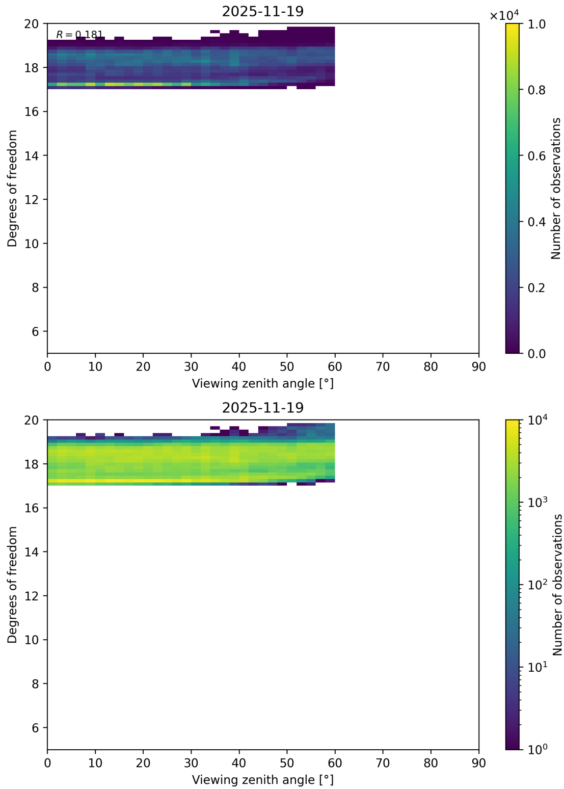
Figure 107: Scatter density plot of “Viewing zenith angle” against “Degrees of freedom” for 2025-11-18 to 2025-11-20.
