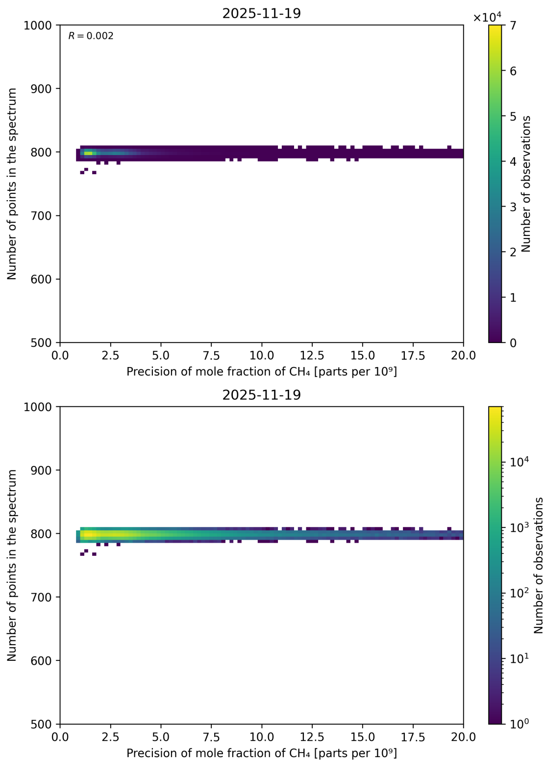
Figure 84: Scatter density plot of “Precision of mole fraction of CH 4 ” against “Number of points in the spectrum” for 2025-11-18 to 2025-11-20.
