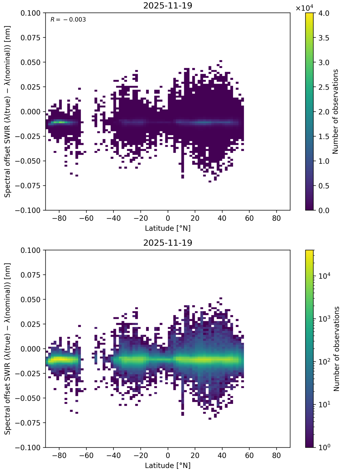
Figure 62: Scatter density plot of “Latitude” against “Spectral offset SWIR ( \lambda_{\text{true}} - \lambda_{\text{nominal}} )” for 2025-11-18 to 2025-11-20.
