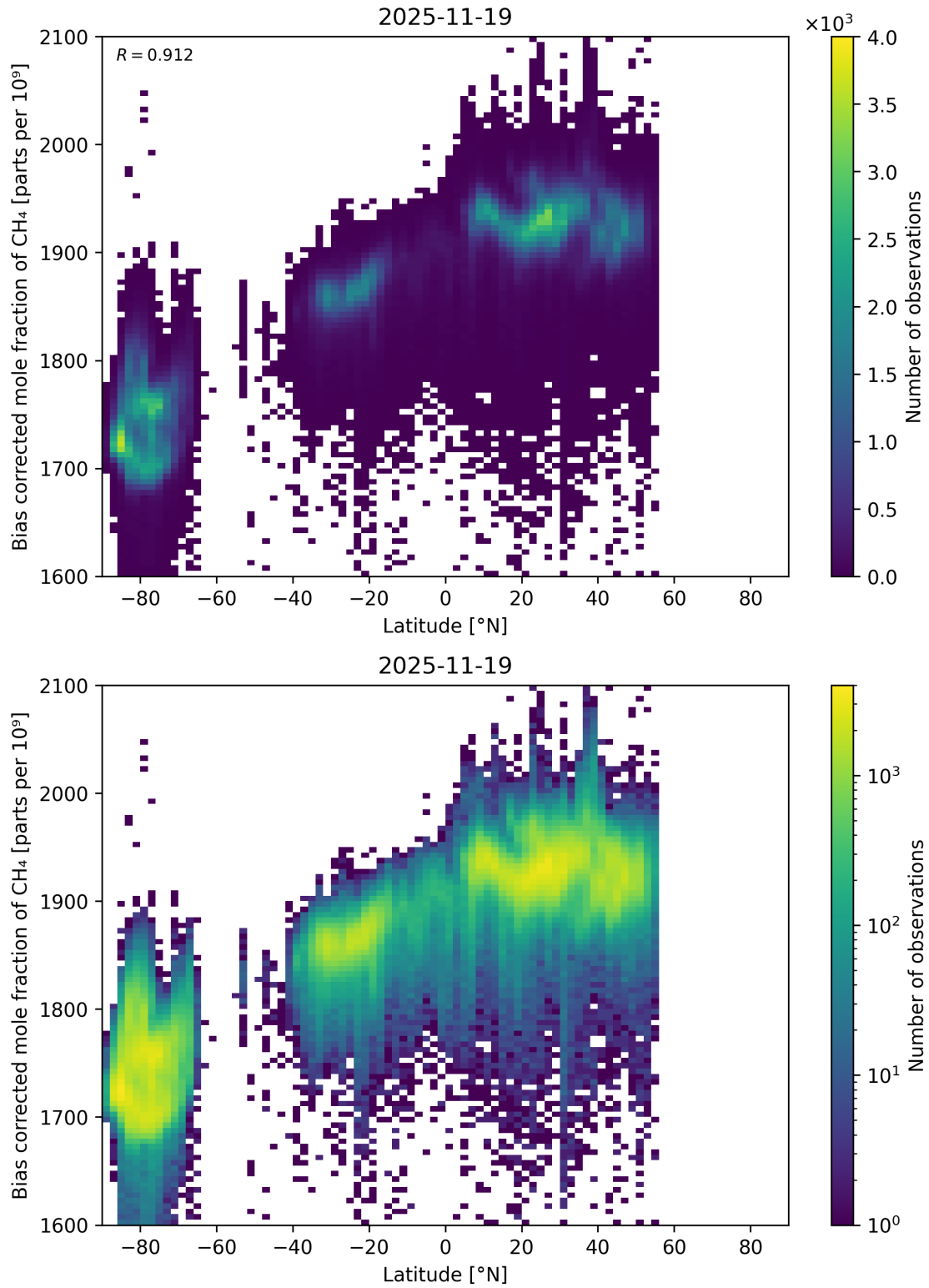
Figure 58: Scatter density plot of “Latitude” against “Bias corrected mole fraction of \text{CH}_4 ” for 2025-11-18 to 2025-11-20.
