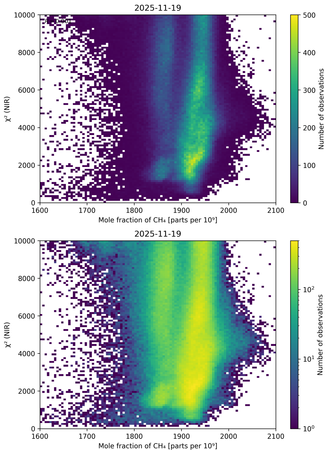
Figure 70: Scatter density plot of “Mole fraction of \text{CH}_4 ” against “ \chi^2 (NIR)” for 2025-11-18 to 2025-11-20.
