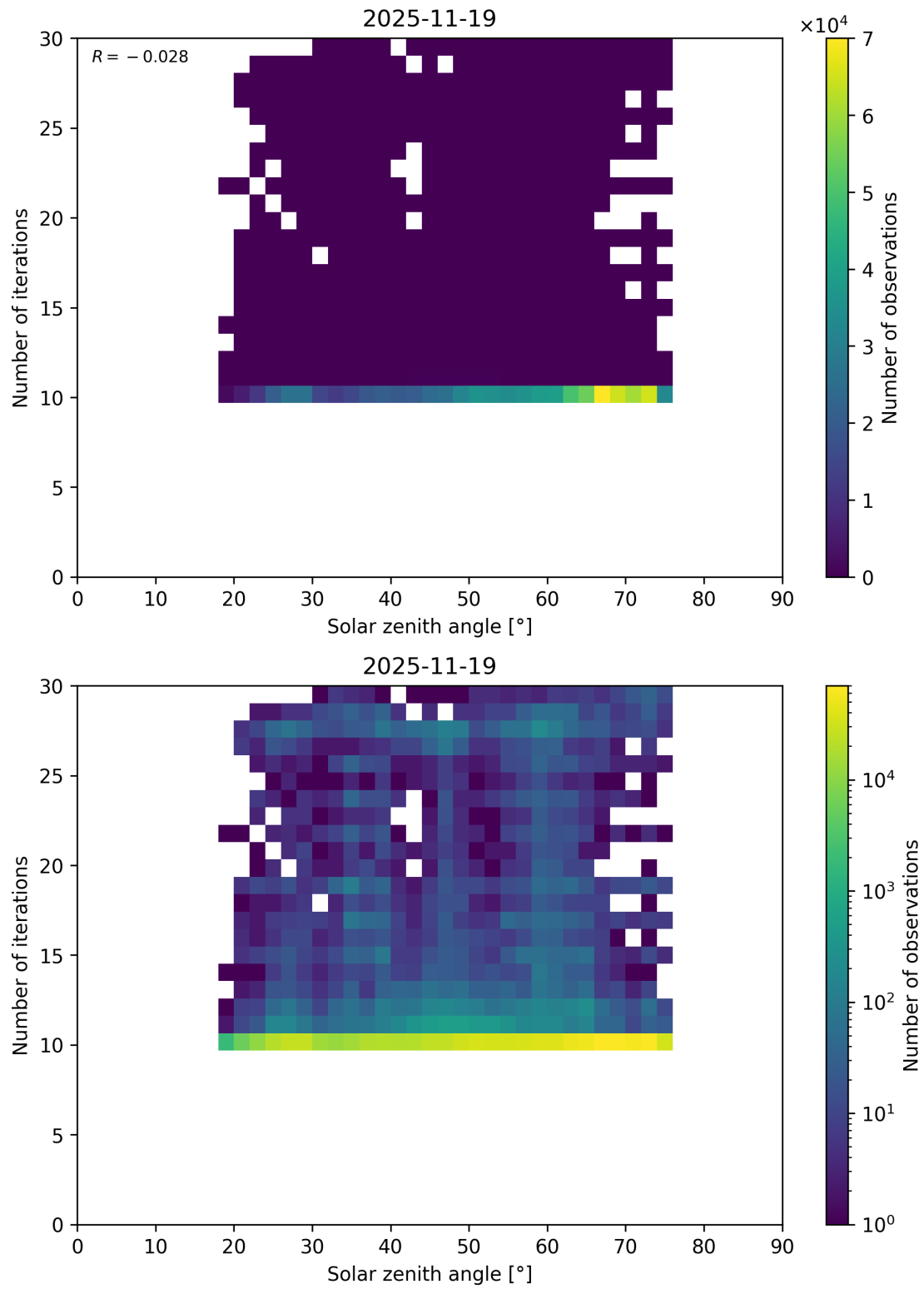
Figure 102: Scatter density plot of “Solar zenith angle” against “Number of iterations” for 2025-11-18 to 2025-11-20.
