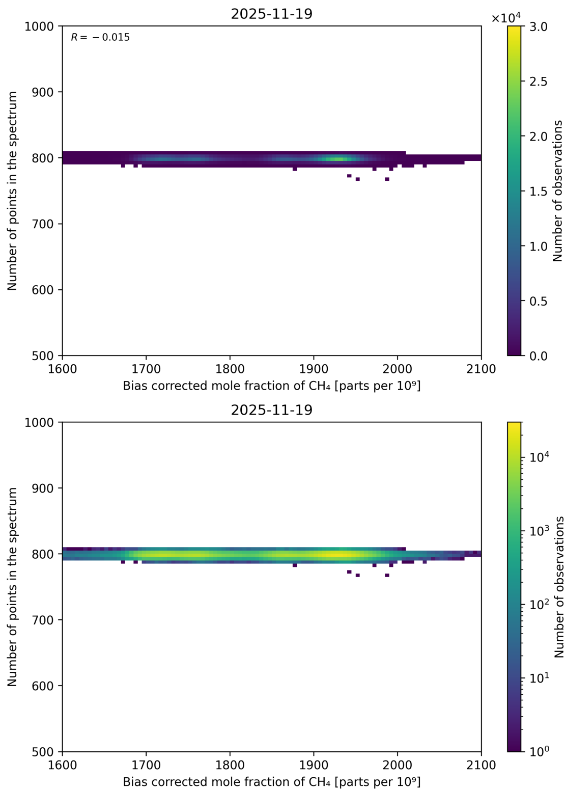
Figure 68: Scatter density plot of “Bias corrected mole fraction of CH 4 ” against “Number of points in the spectrum” for 2025-11-18 to 2025-11-20.
