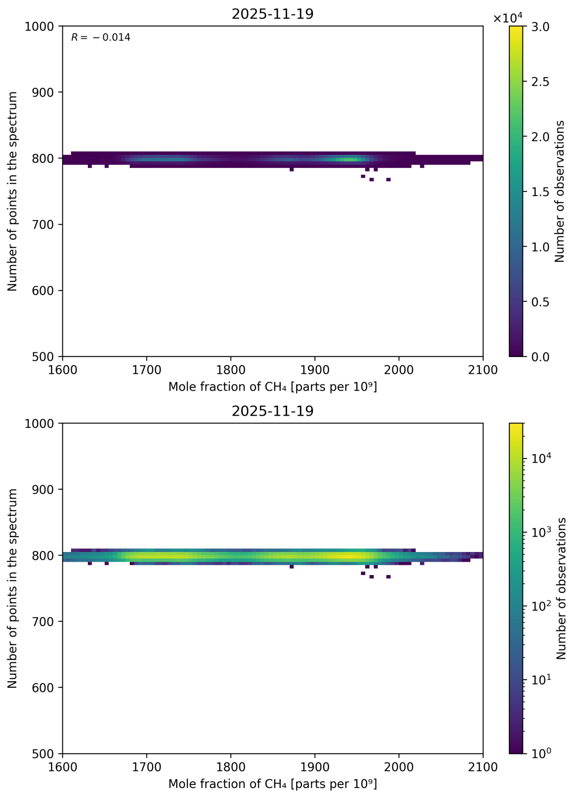
Figure 77: Scatter density plot of “Mole fraction of CH 4 ” against “Number of points in the spectrum” for 2025-11-18 to 2025-11-20.
