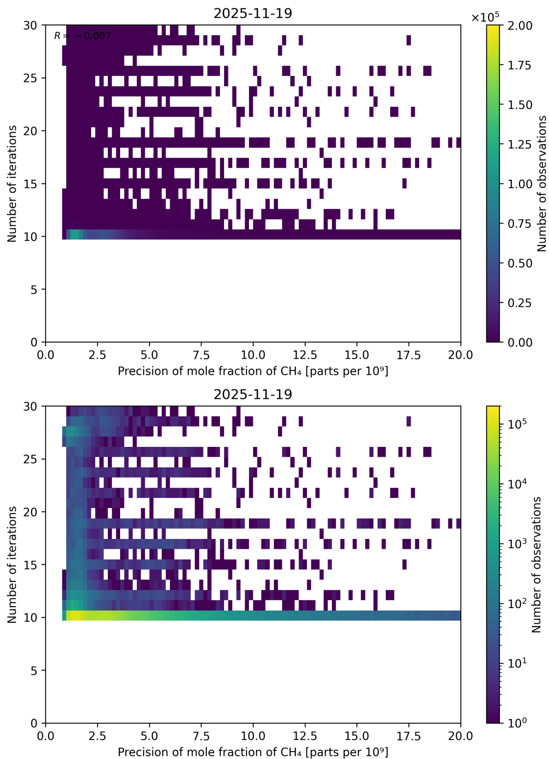
Figure 83: Scatter density plot of “Precision of mole fraction of \text{CH}_4 ” against “Number of iterations” for 2025-11-18 to 2025-11-20.
