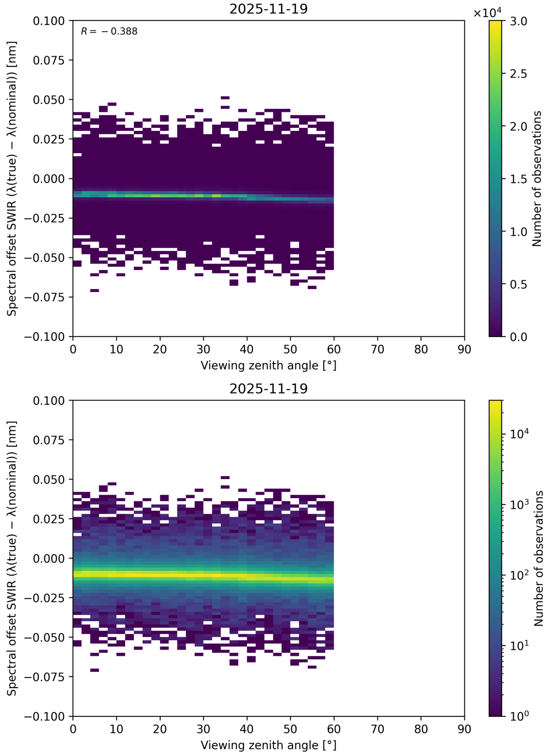
Figure 116: Scatter density plot of “Viewing zenith angle” against “Spectral offset SWIR ( \lambda_{\text{true}} - \lambda_{\text{nominal}} )” for 2025-11-18 to 2025-11-20.
