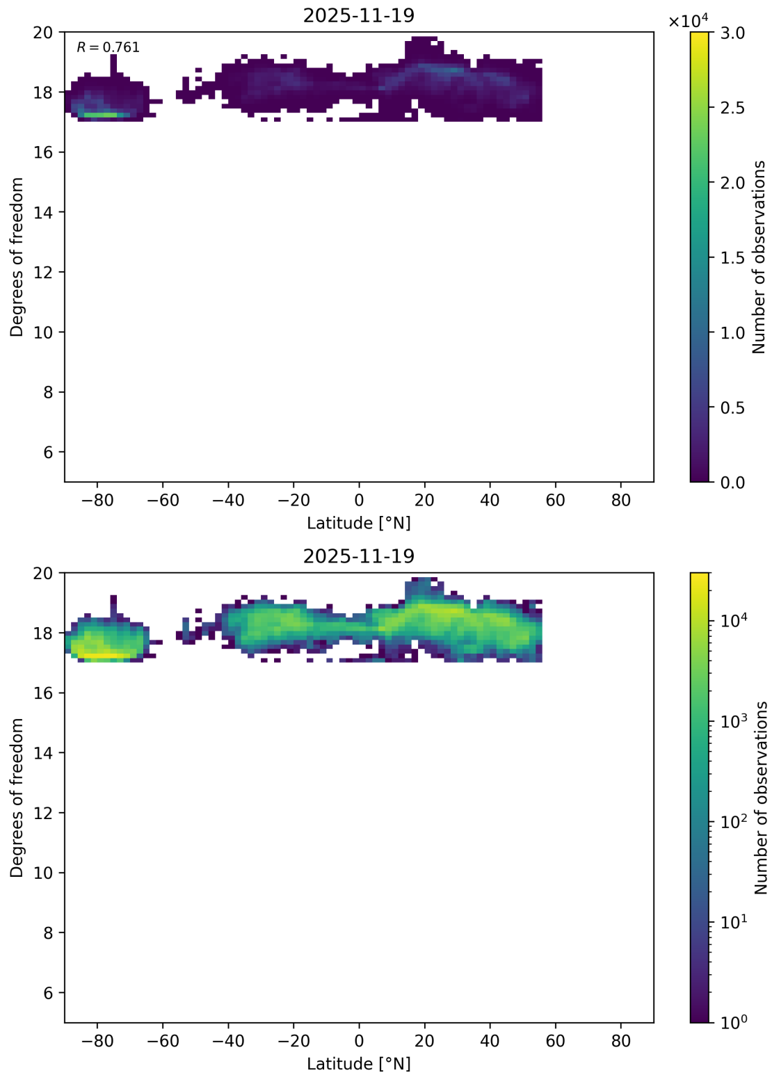
Figure 55: Scatter density plot of “Latitude” against “Degrees of freedom” for 2025-11-18 to 2025-11-20.
