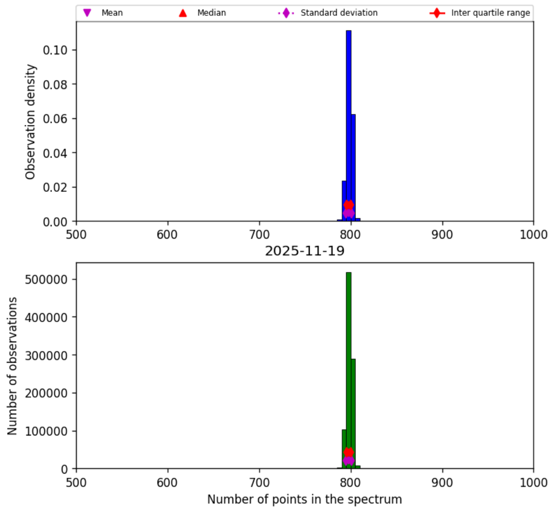
Figure 26: Histogram of “Number of points in the spectrum” for 2025-11-18 to 2025-11-20
