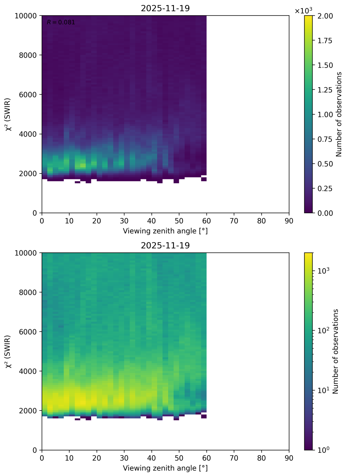
Figure 106: Scatter density plot of “Viewing zenith angle” against “ \chi^2 (SWIR)” for 2025-11-18 to 2025-11-20.
