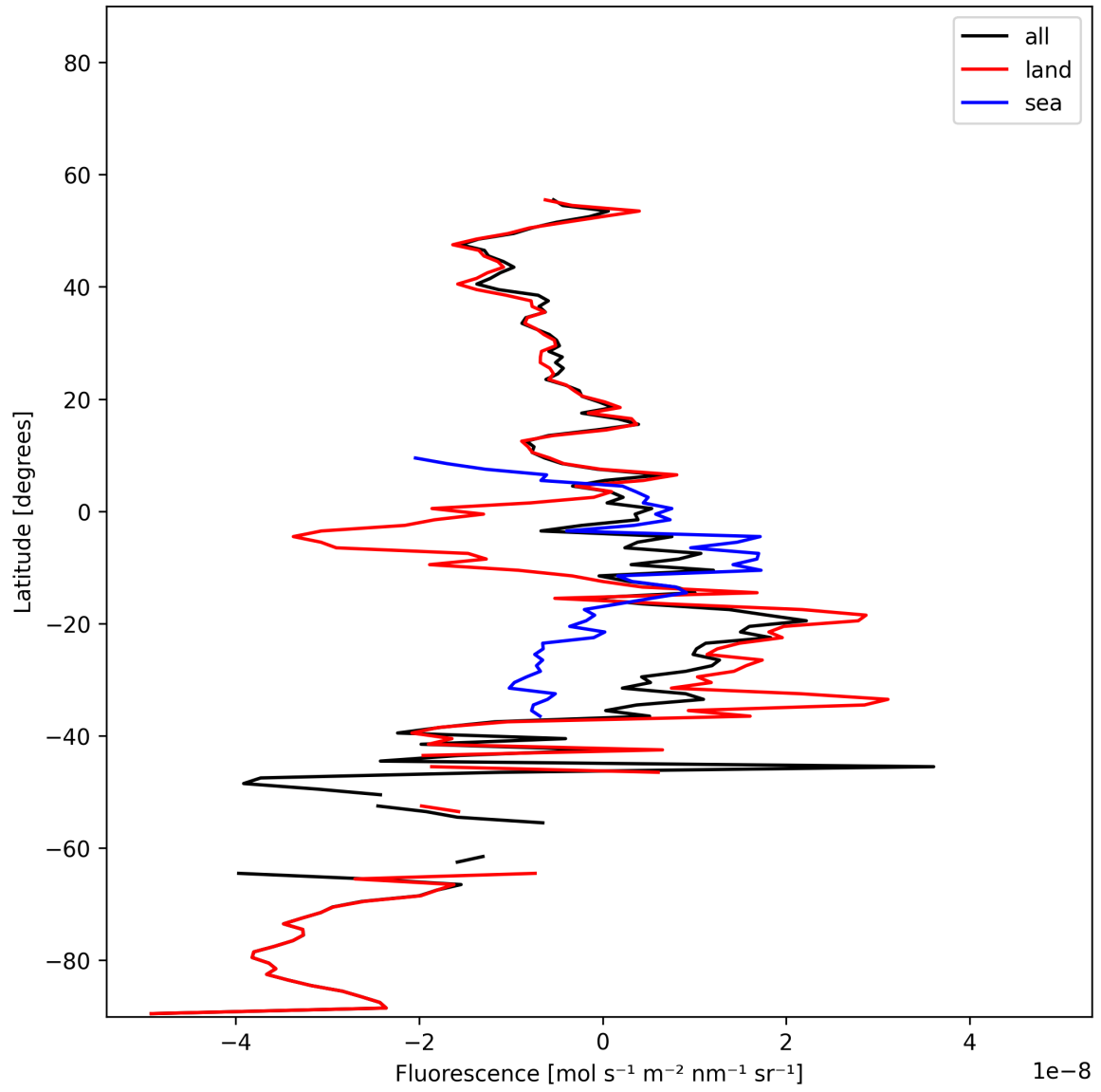
Figure 21: Zonal average of “Fluorescence” for 2025-11-18 to 2025-11-20.
