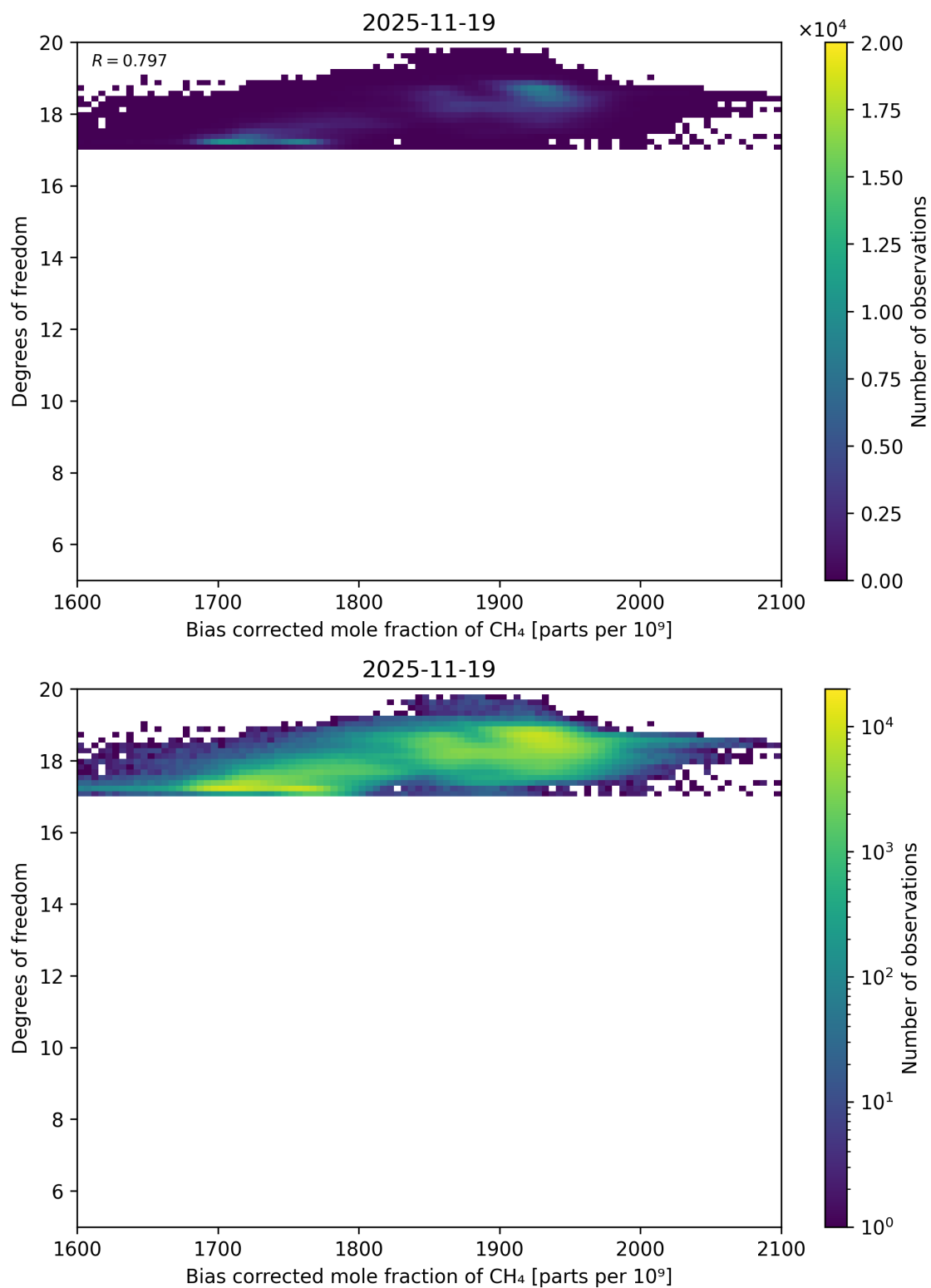
Figure 65: Scatter density plot of “Bias corrected mole fraction of CH 4 ” against “Degrees of freedom” for 2025-11-18 to 2025-11-20.
