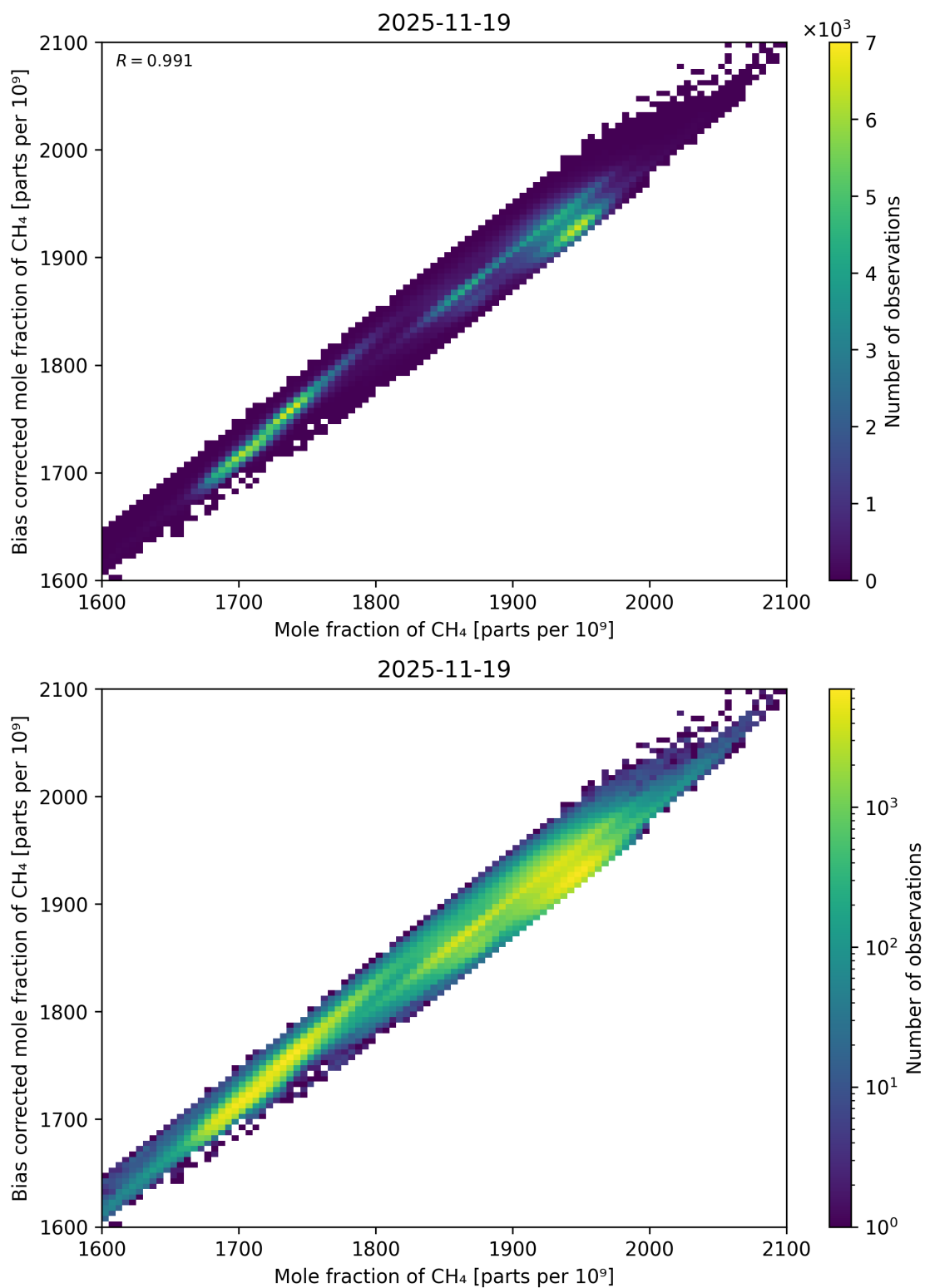
Figure 74: Scatter density plot of “Mole fraction of CH 4 ” against “Bias corrected mole fraction of CH 4 ” for 2025-11-18 to 2025-11-20.
