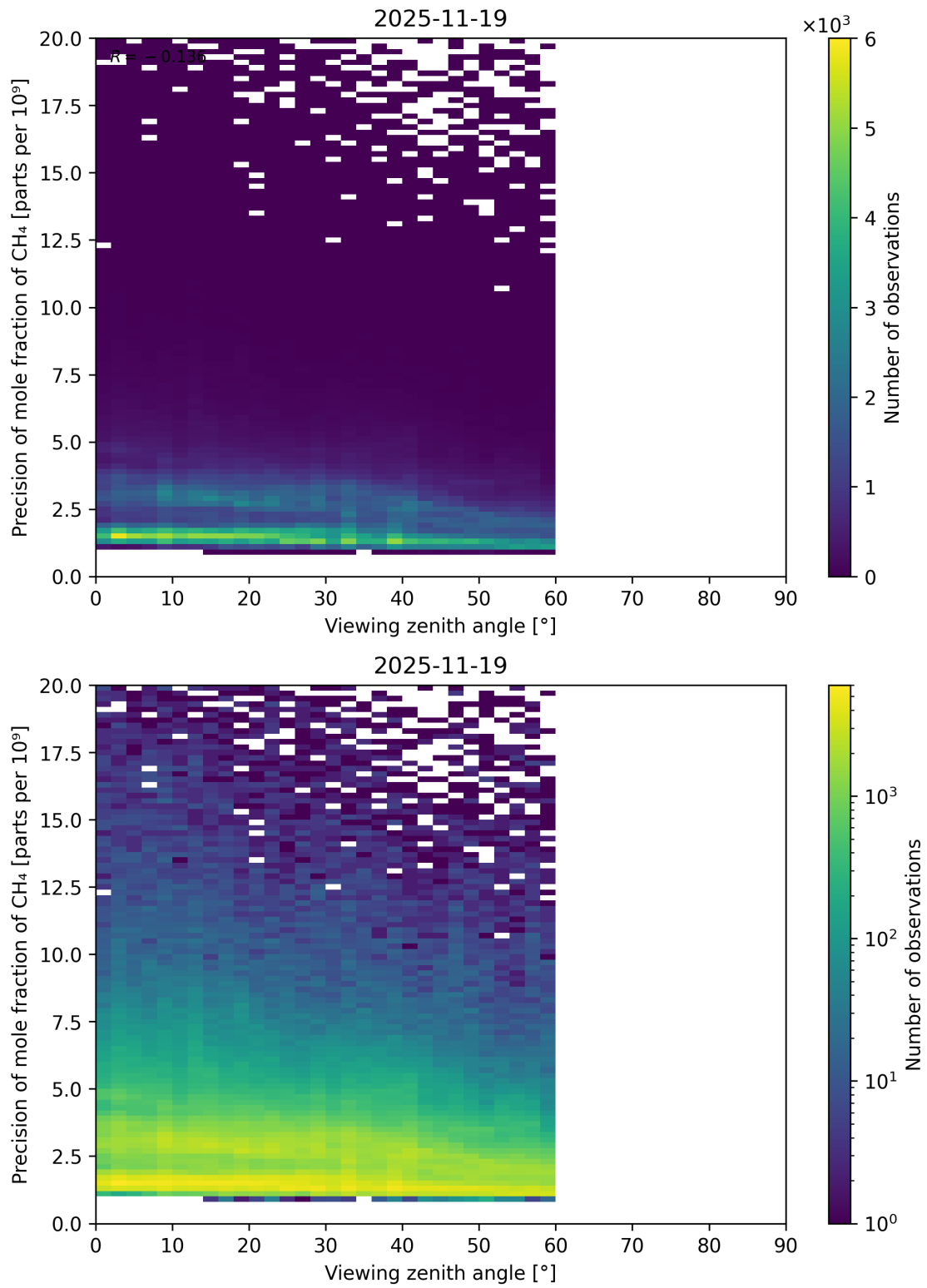
Figure 112: Scatter density plot of “Viewing zenith angle” against “Precision of mole fraction of CH 4 ” for 2025-11-18 to 2025-11-20.
