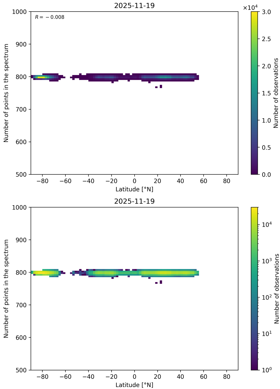
Figure 61: Scatter density plot of “Latitude” against “Number of points in the spectrum” for 2025-11-18 to 2025-11-20.
