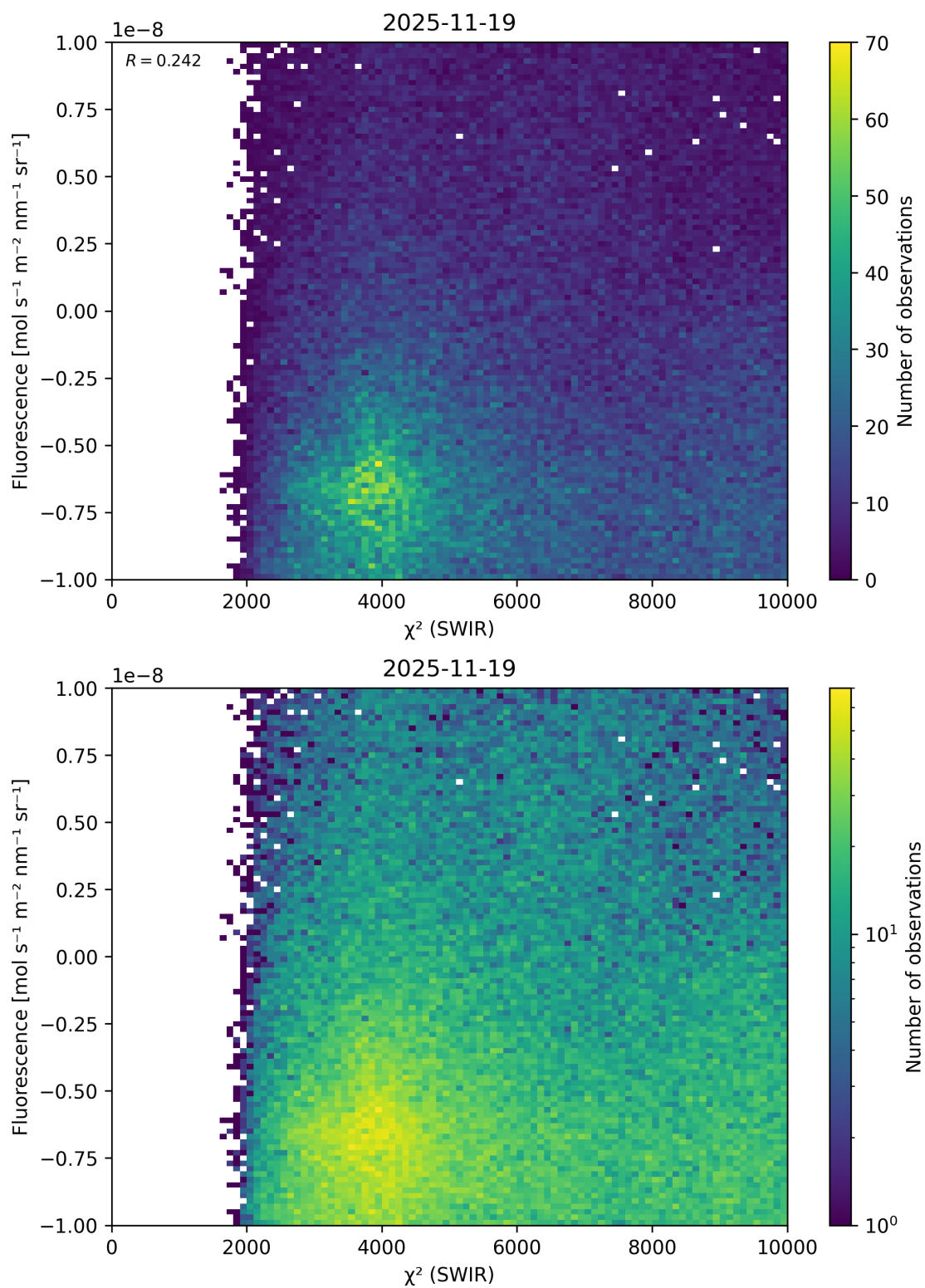
Figure 49: Scatter density plot of “ \chi^2 (SWIR)” against “Fluorescence” for 2025-11-18 to 2025-11-20.
