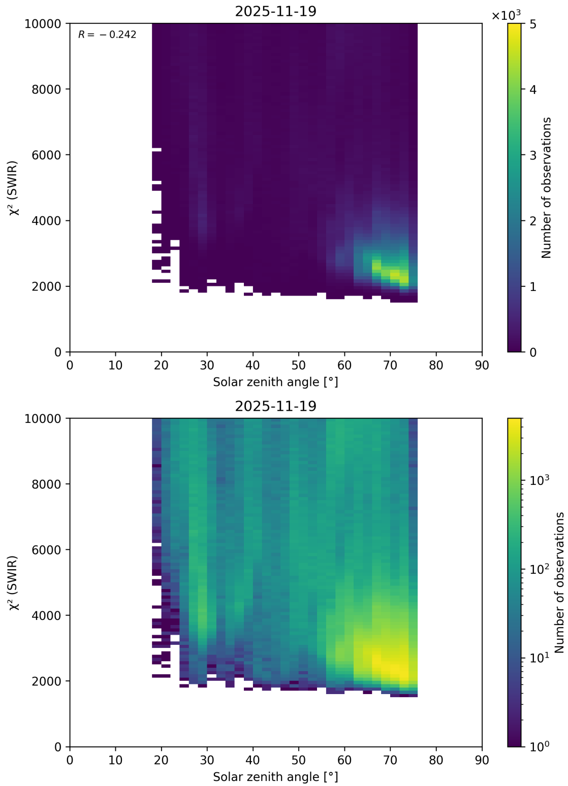
Figure 95: Scatter density plot of “Solar zenith angle” against “ \chi^2 (SWIR)” for 2025-11-18 to 2025-11-20.
