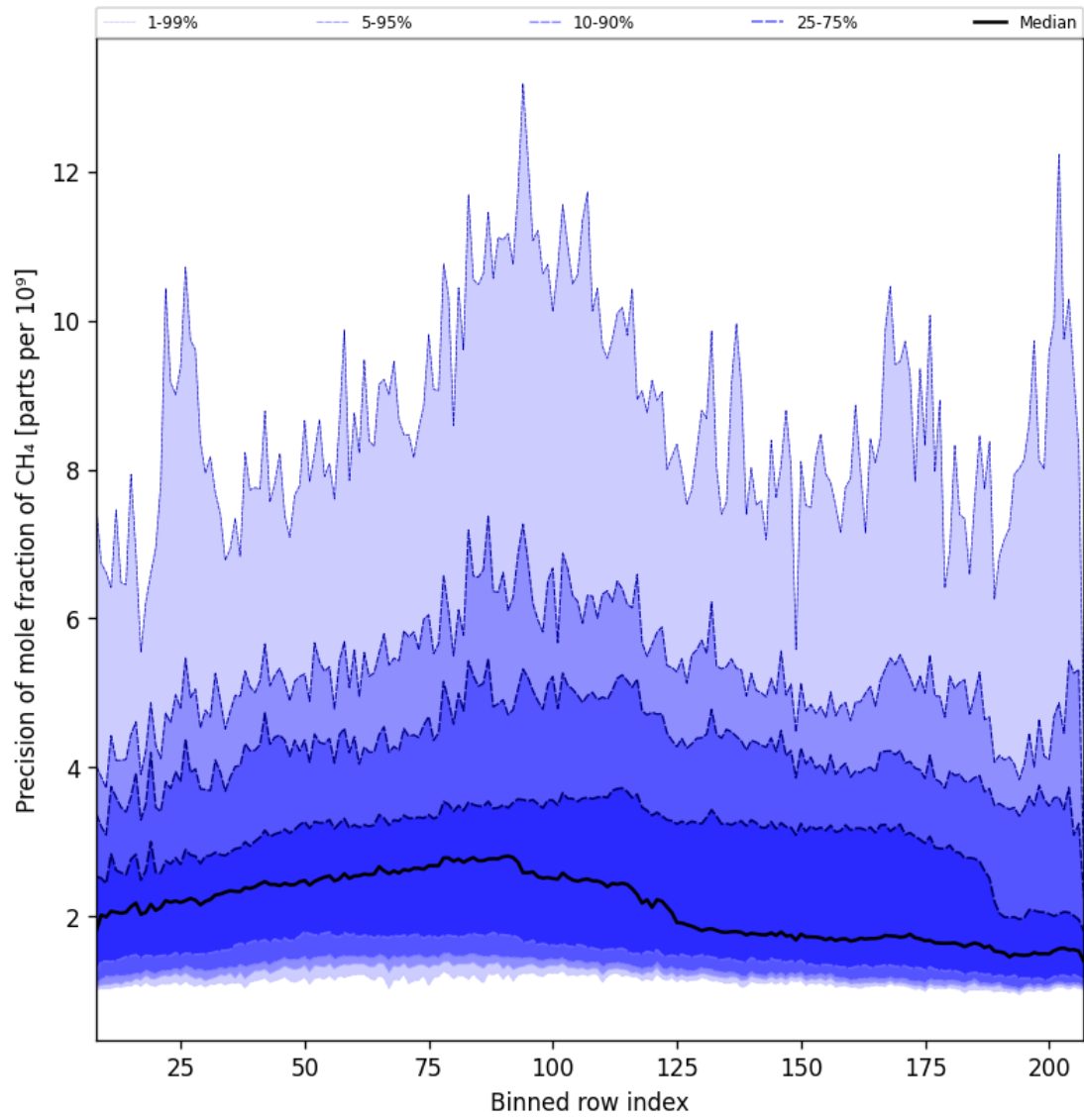
Figure 35: Along track statistics of “Precision of mole fraction of CH 4 ” for 2025-11-18 to 2025-11-20
