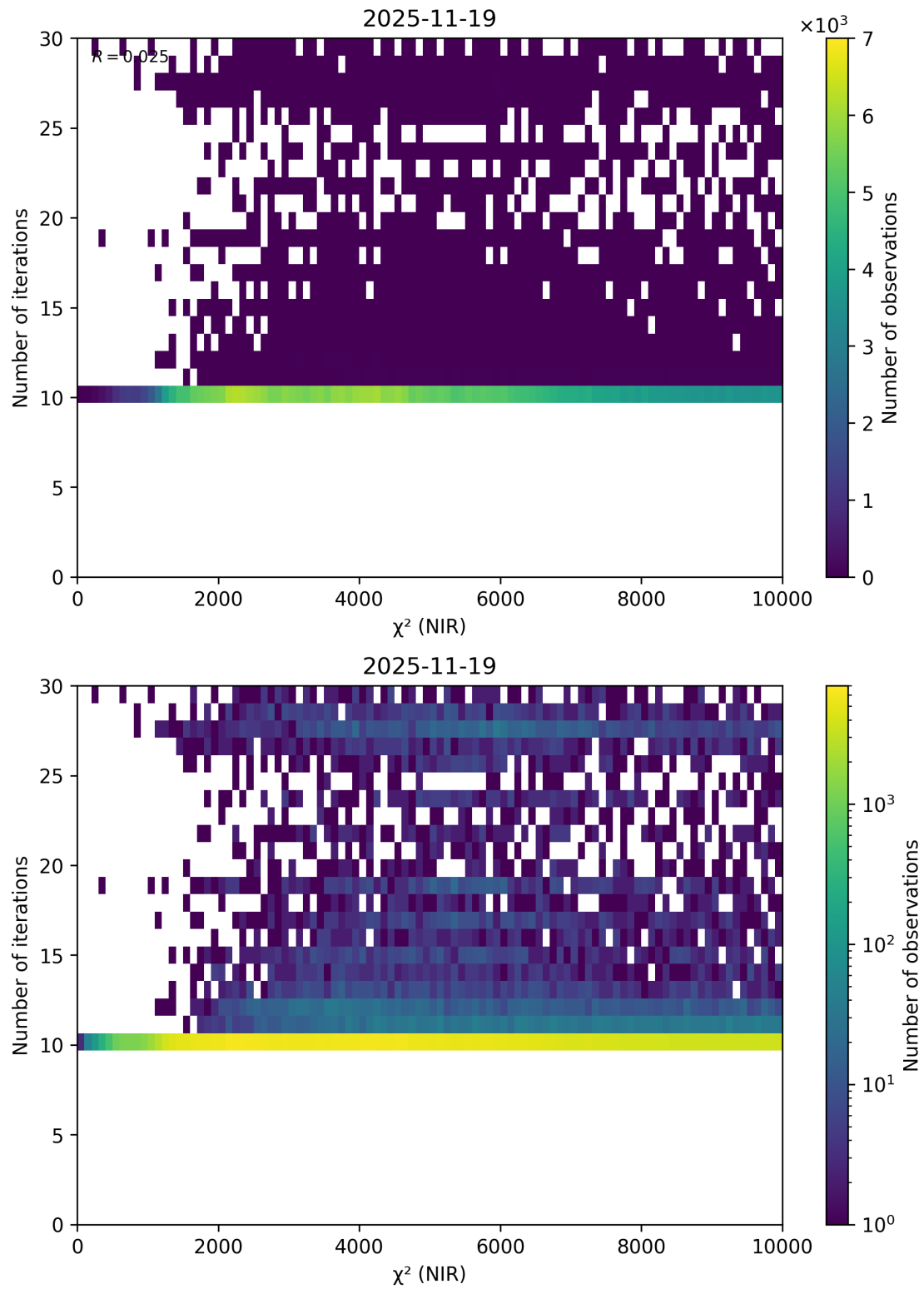
Figure 46: Scatter density plot of “ \chi^2 (NIR)” against “Number of iterations” for 2025-11-18 to 2025-11-20.
