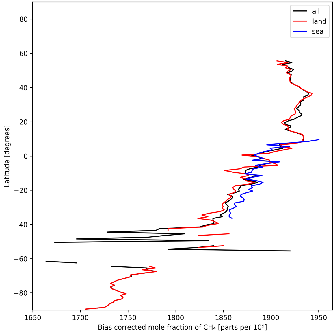
Figure 14: Zonal average of “Bias corrected mole fraction of CH 4 ” for 2025-11-18 to 2025-11-20.
