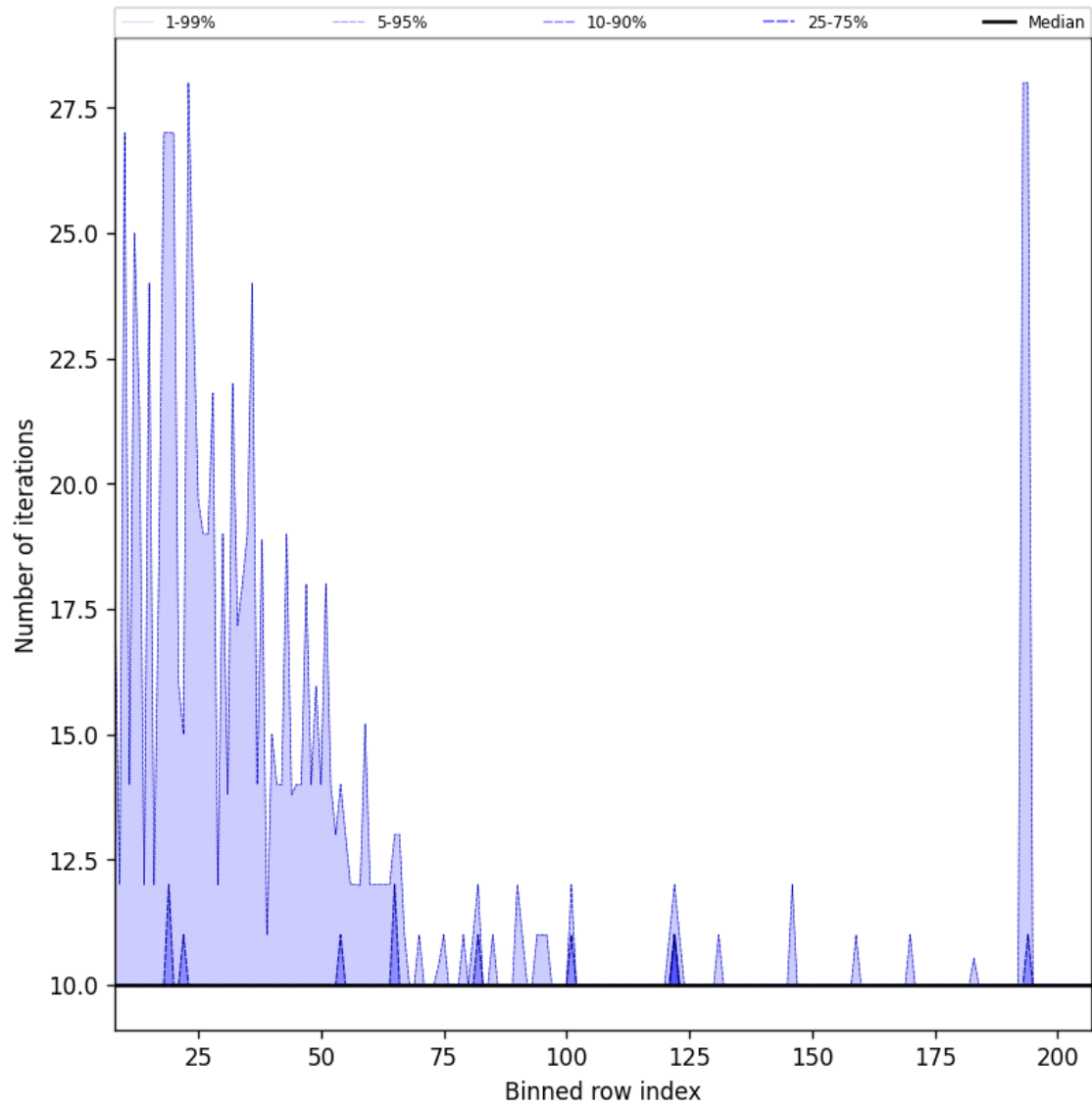
Figure 42: Along track statistics of “Number of iterations” for 2025-11-18 to 2025-11-20
