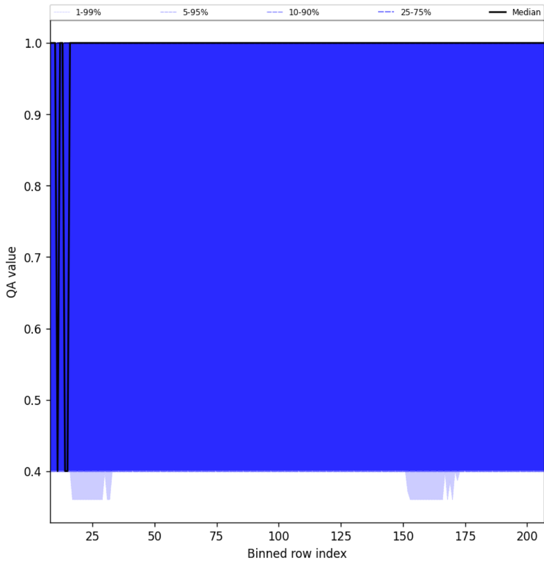
Figure 33: Along track statistics of “QA value” for 2025-11-18 to 2025-11-20
