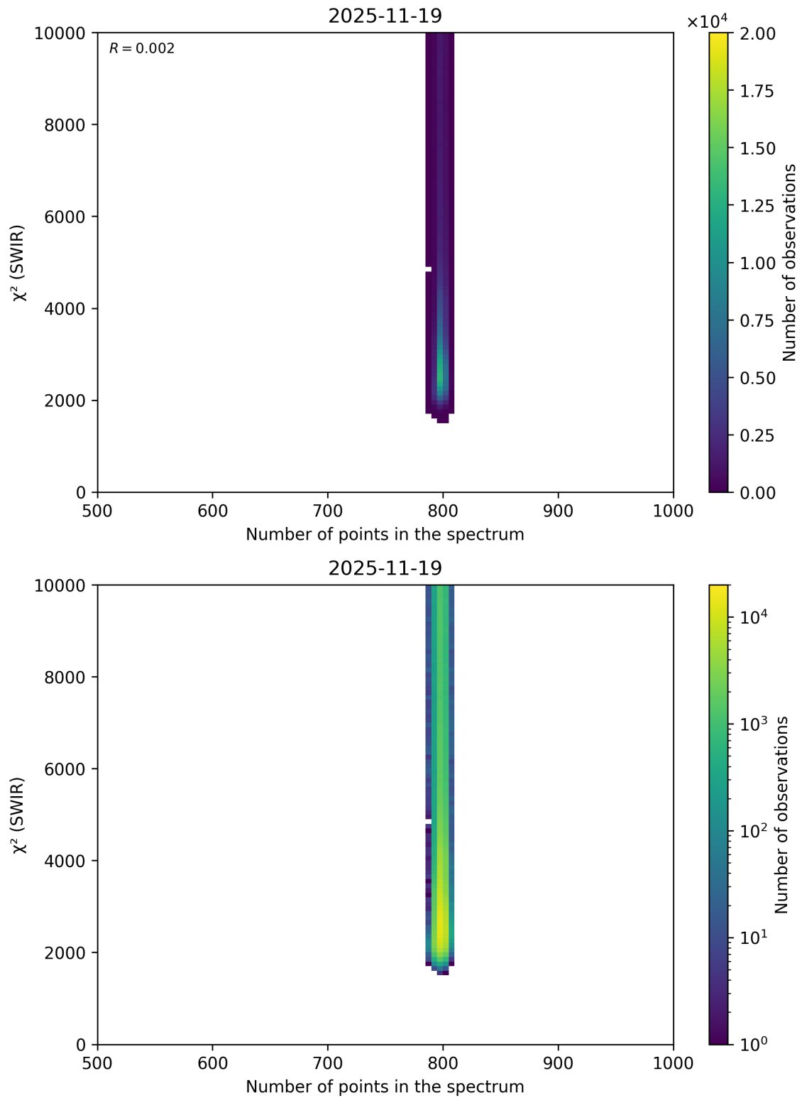
Figure 89: Scatter density plot of “Number of points in the spectrum” against “ \chi^2 (SWIR)” for 2025-11-18 to 2025-11-20.
