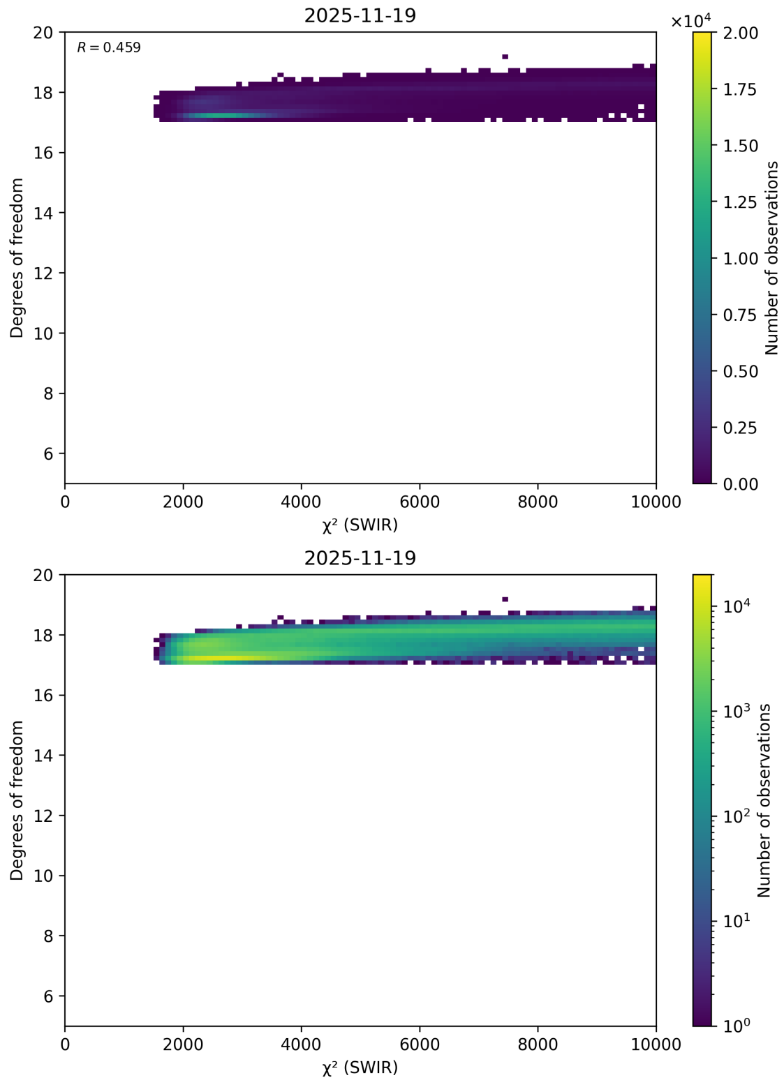
Figure 48: Scatter density plot of “ \chi^2 (SWIR)” against “Degrees of freedom” for 2025-11-18 to 2025-11-20.
