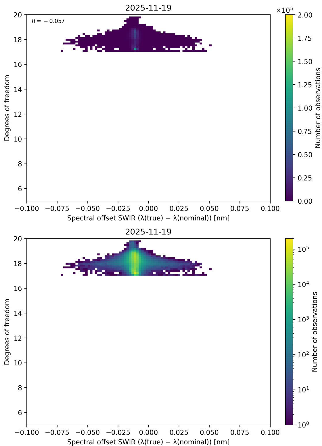
Figure 119: Scatter density plot of “Spectral offset SWIR ( \lambda_{\text{true}} - \lambda_{\text{nominal}} )” against “Degrees of freedom” for 2025-11-18 to 2025-11-20.
