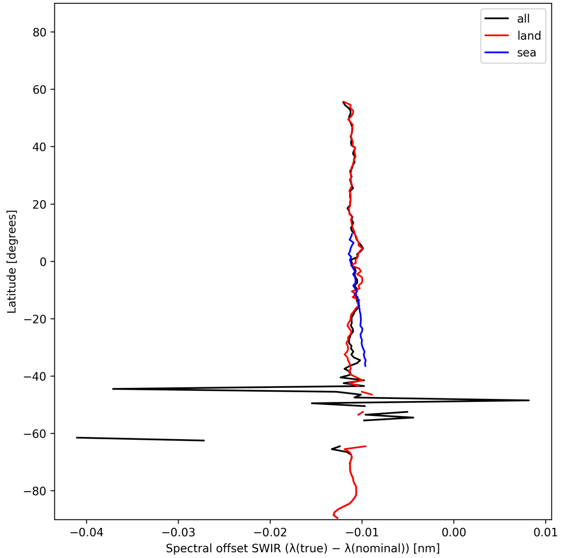
Figure 16: Zonal average of “Spectral offset SWIR ( \lambda_{\text{true}} - \lambda_{\text{nominal}} )” for 2025-11-18 to 2025-11-20.
