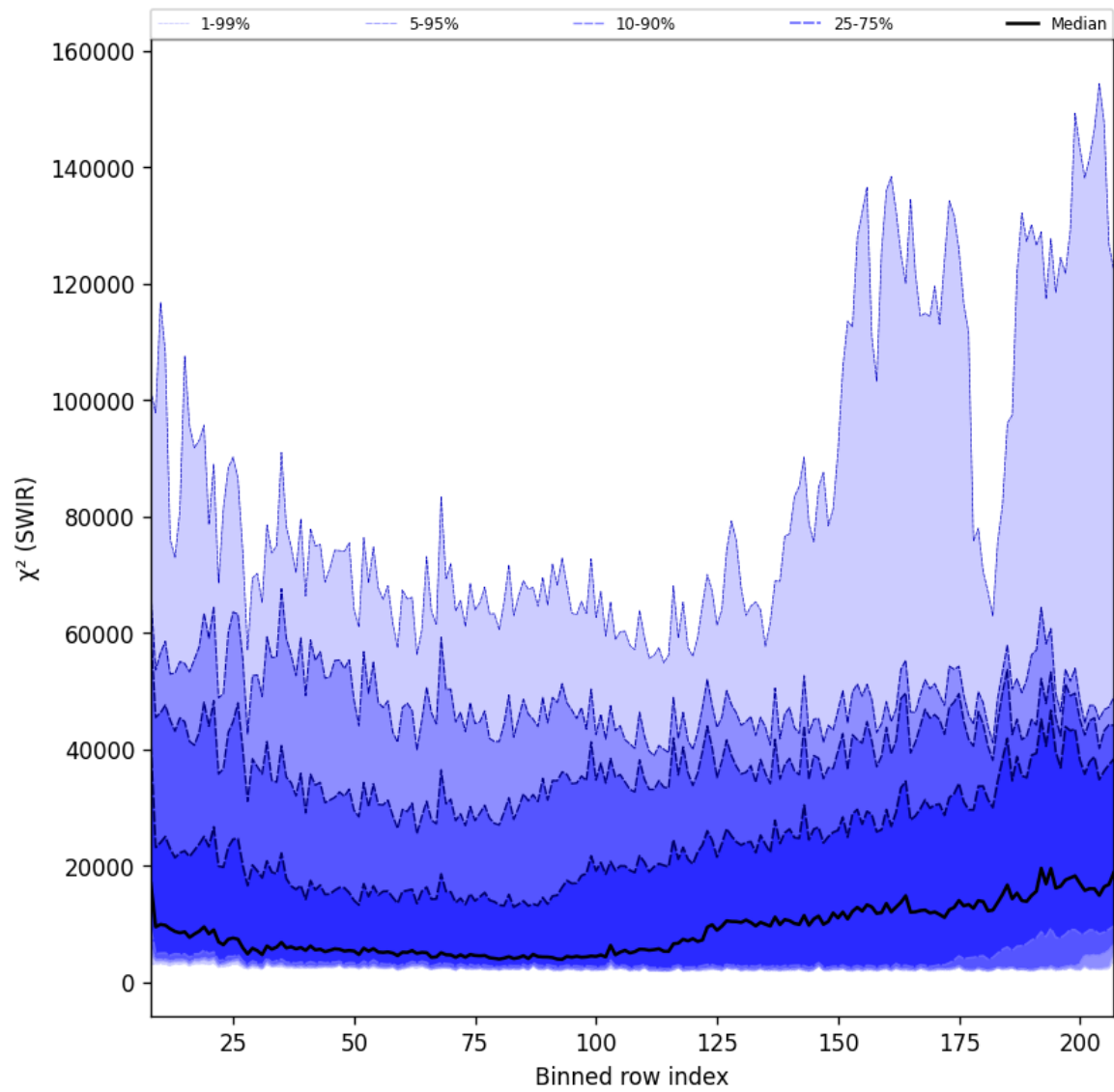
Figure 39: Along track statistics of “ \chi^2 (SWIR)” for 2025-11-18 to 2025-11-20
