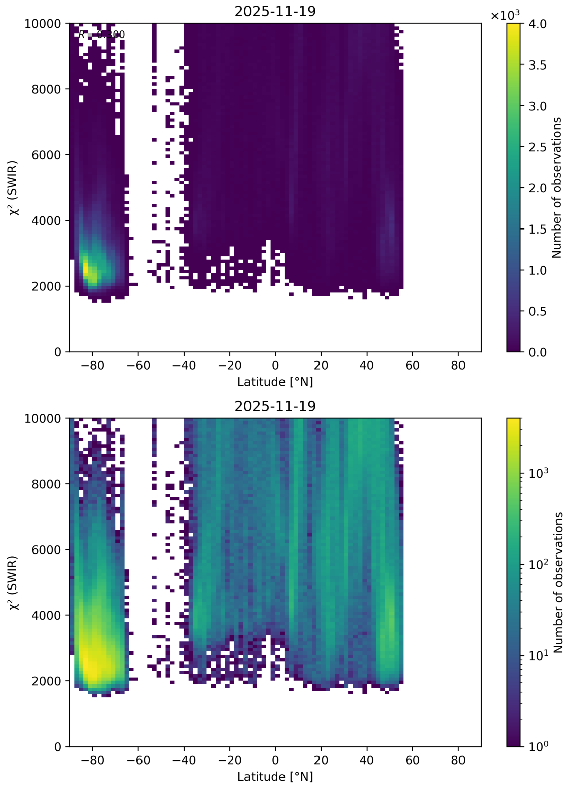
Figure 54: Scatter density plot of “Latitude” against “ \chi^2 (SWIR)” for 2025-11-18 to 2025-11-20.
