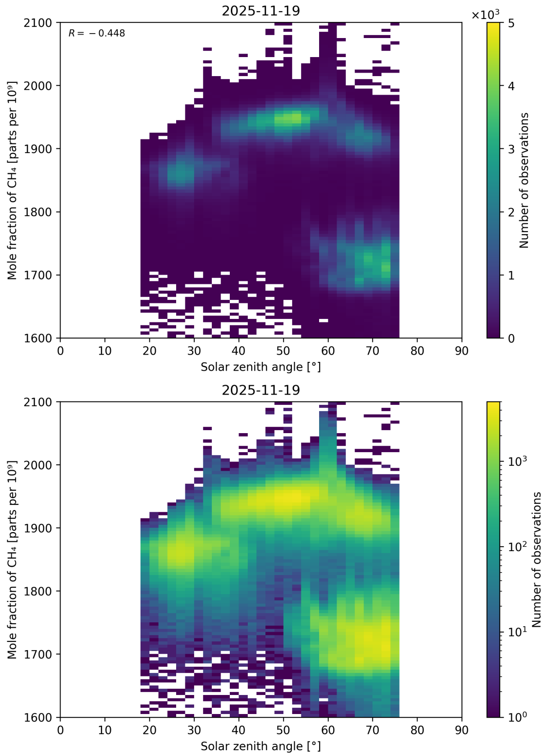
Figure 99: Scatter density plot of “Solar zenith angle” against “Mole fraction of CH 4 ” for 2025-11-18 to 2025-11-20.
