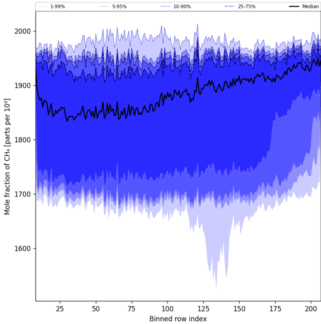
Figure 34: Along track statistics of “Mole fraction of CH 4 ” for 2025-11-18 to 2025-11-20
