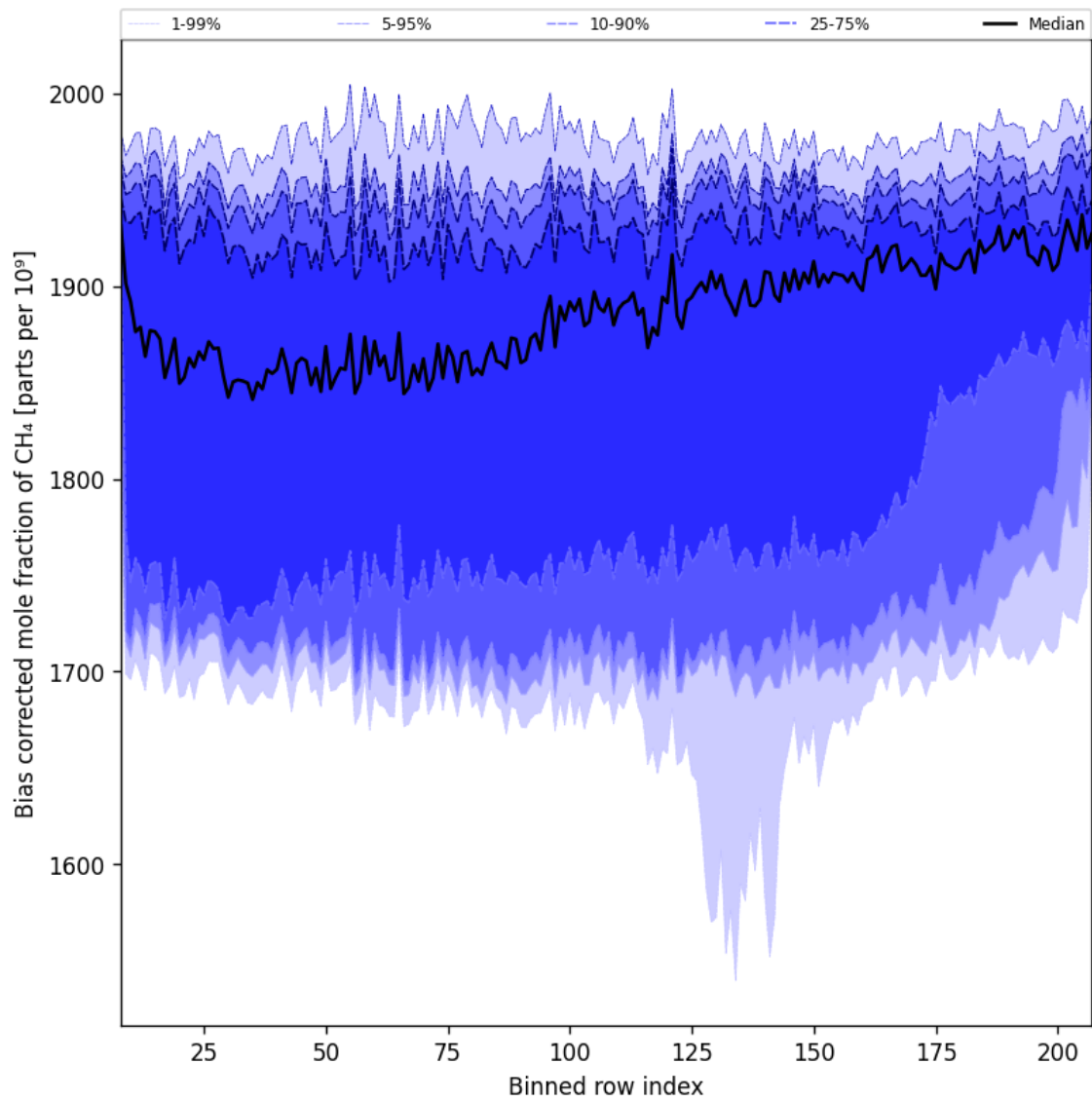
Figure 36: Along track statistics of “Bias corrected mole fraction of CH 4 ” for 2025-11-18 to 2025-11-20
