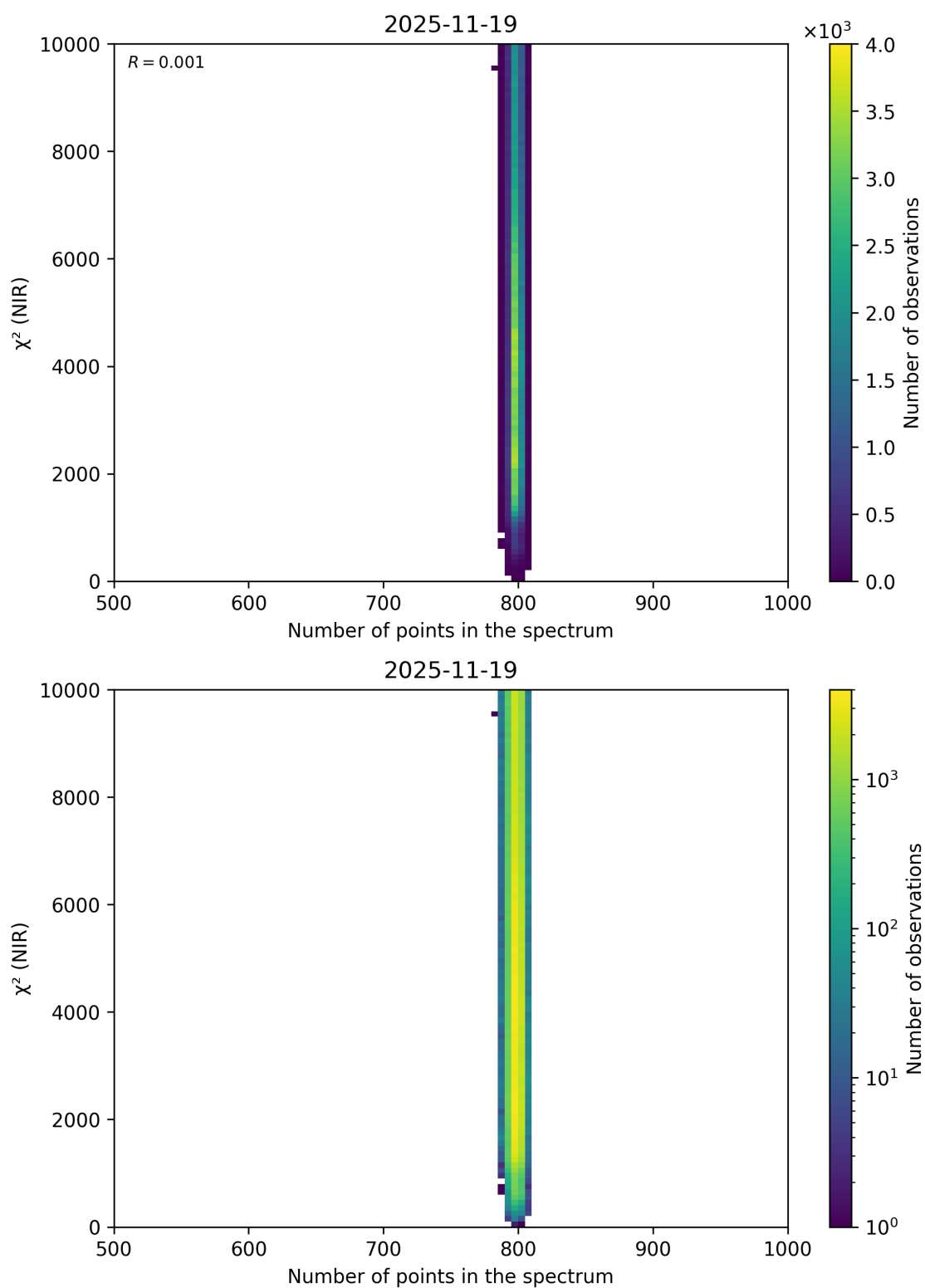
Figure 88: Scatter density plot of “Number of points in the spectrum” against “ \chi^2 (NIR)” for 2025-11-18 to 2025-11-20.
