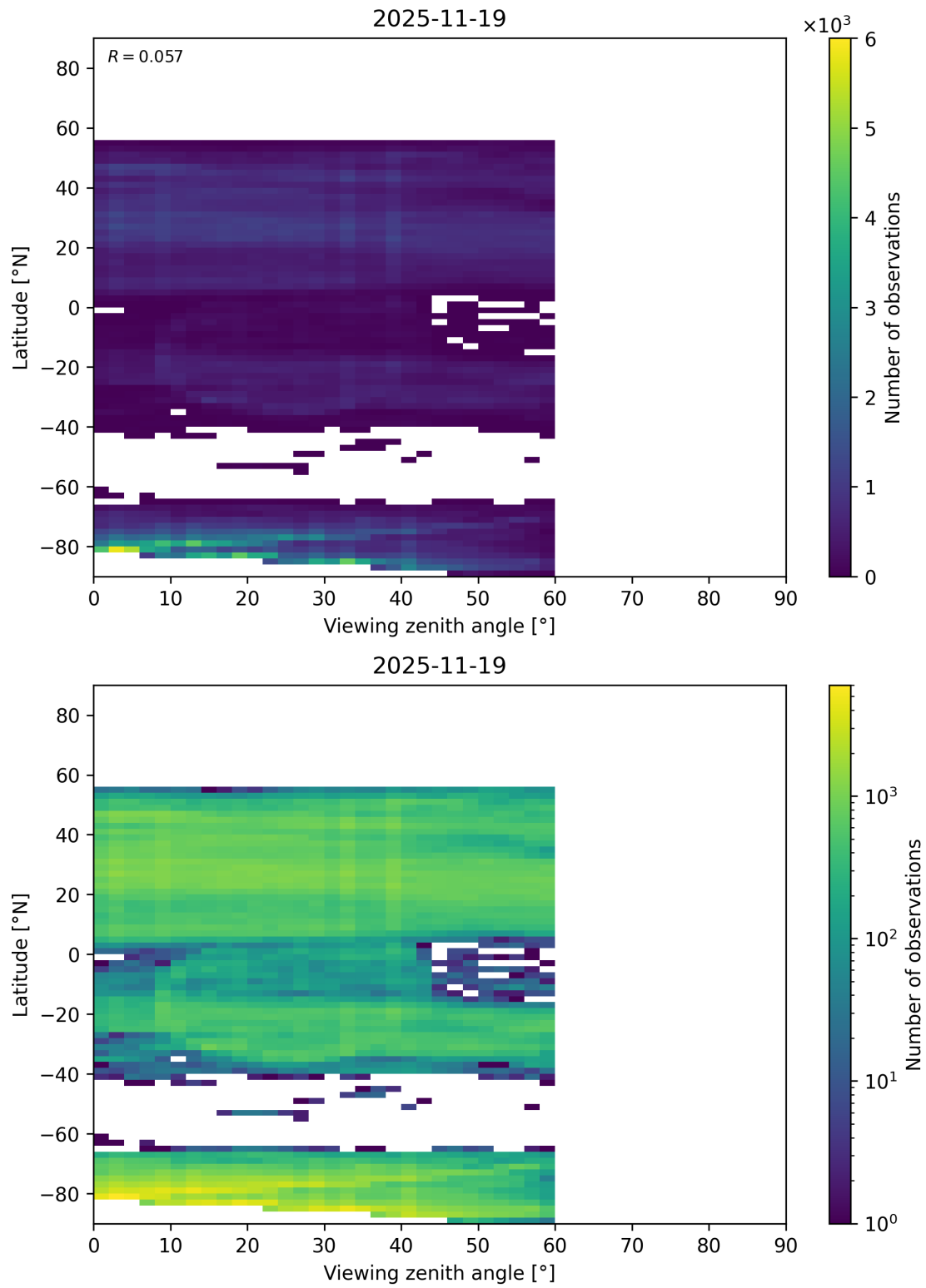
Figure 109: Scatter density plot of “Viewing zenith angle” against “Latitude” for 2025-11-18 to 2025-11-20.
