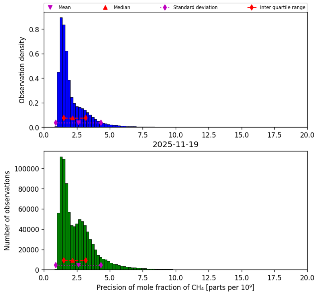
Figure 24: Histogram of “Precision of mole fraction of CH 4 ” for 2025-11-18 to 2025-11-20
