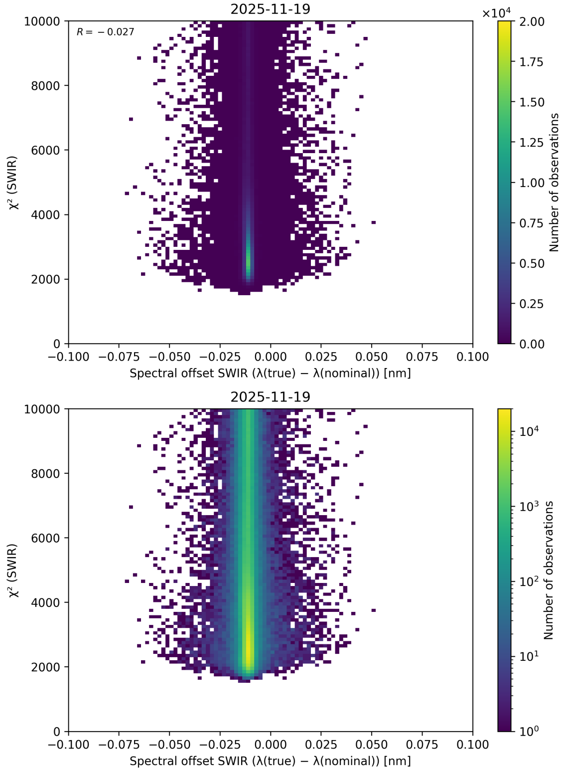
Figure 118: Scatter density plot of “Spectral offset SWIR ( \lambda_{\text{true}} - \lambda_{\text{nominal}} )” against “ \chi^2 (SWIR)” for 2025-11-18 to 2025-11-20.
