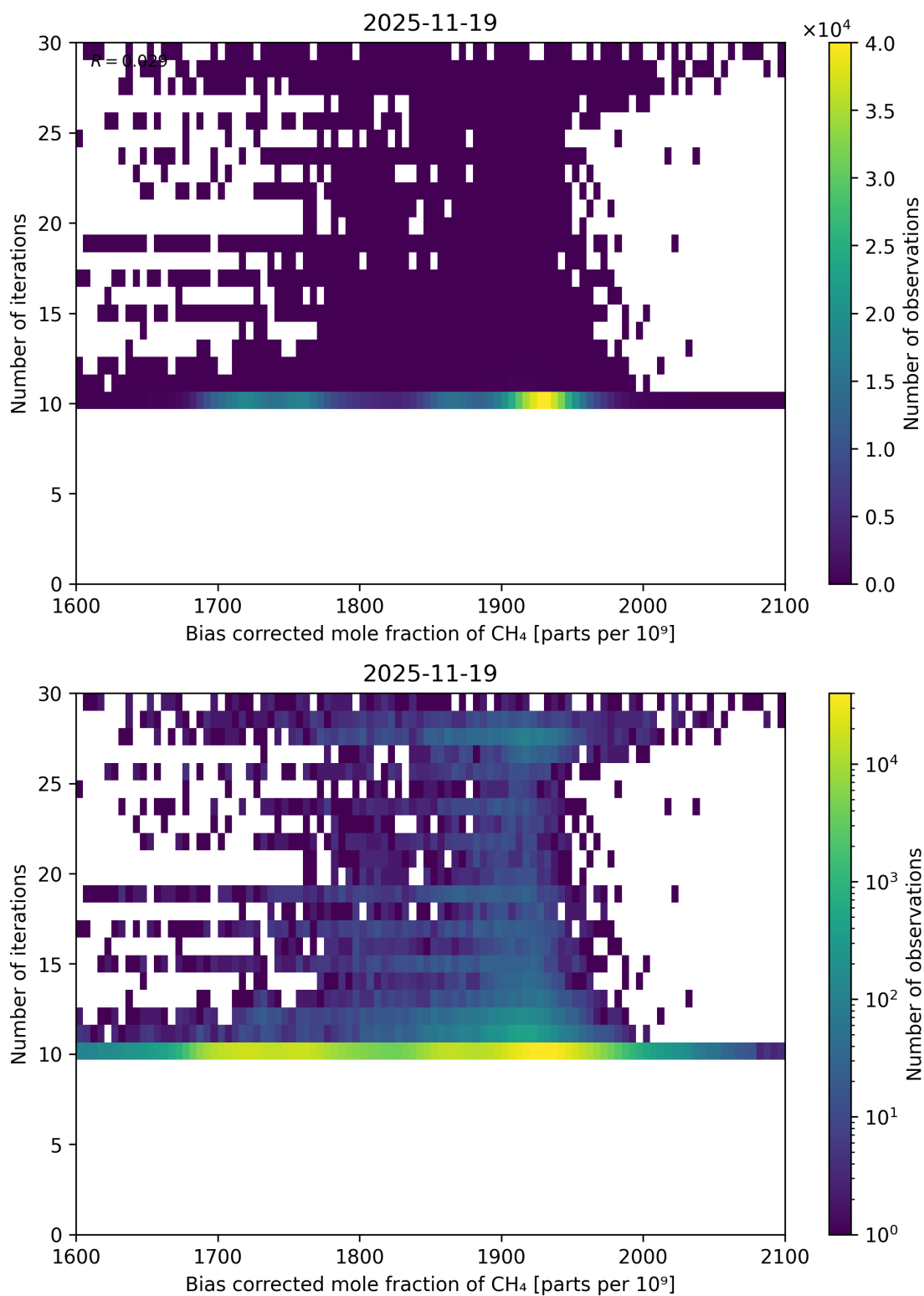
Figure 67: Scatter density plot of “Bias corrected mole fraction of \text{CH}_4 ” against “Number of iterations” for 2025-11-18 to 2025-11-20.
