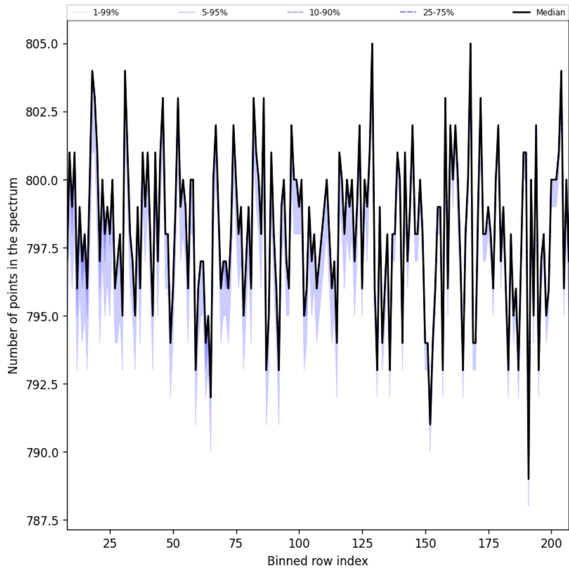
Figure 37: Along track statistics of “Number of points in the spectrum” for 2025-11-18 to 2025-11-20
