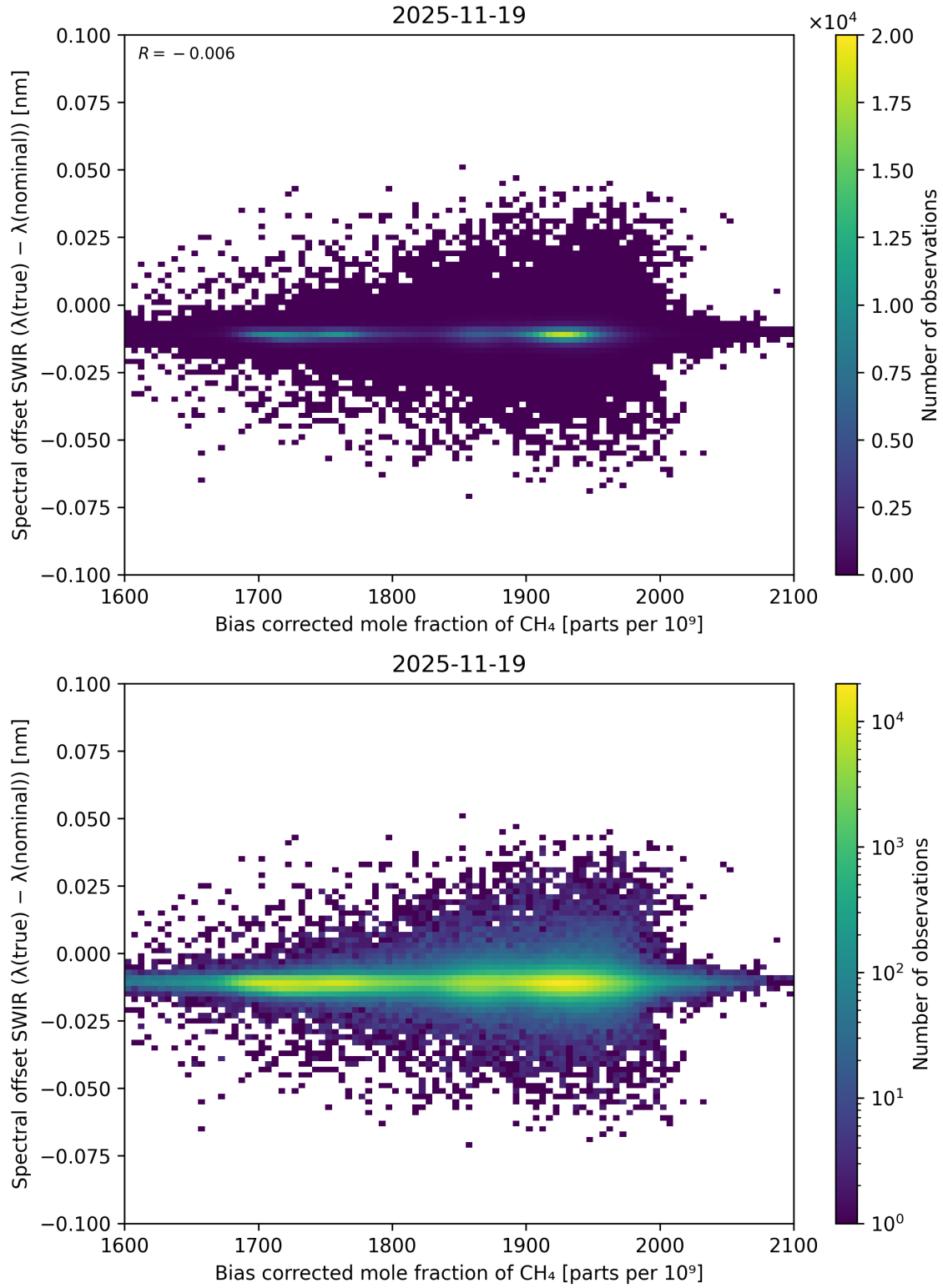
Figure 69: Scatter density plot of “Bias corrected mole fraction of \text{CH}_4 ” against “Spectral offset SWIR ( \lambda_{\text{true}} - \lambda_{\text{nominal}} )” for 2025-11-18 to 2025-11-20.
