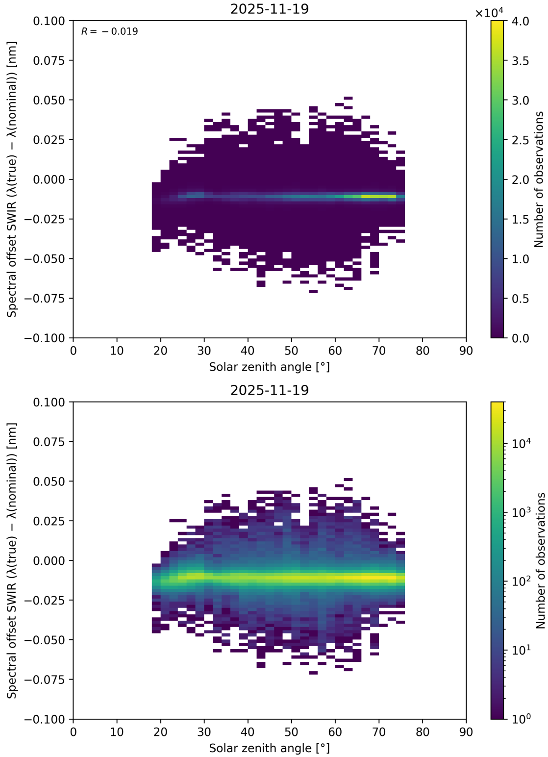
Figure 104: Scatter density plot of “Solar zenith angle” against “Spectral offset SWIR ( \lambda_{\text{true}} - \lambda_{\text{nominal}} )” for 2025-11-18 to 2025-11-20.
