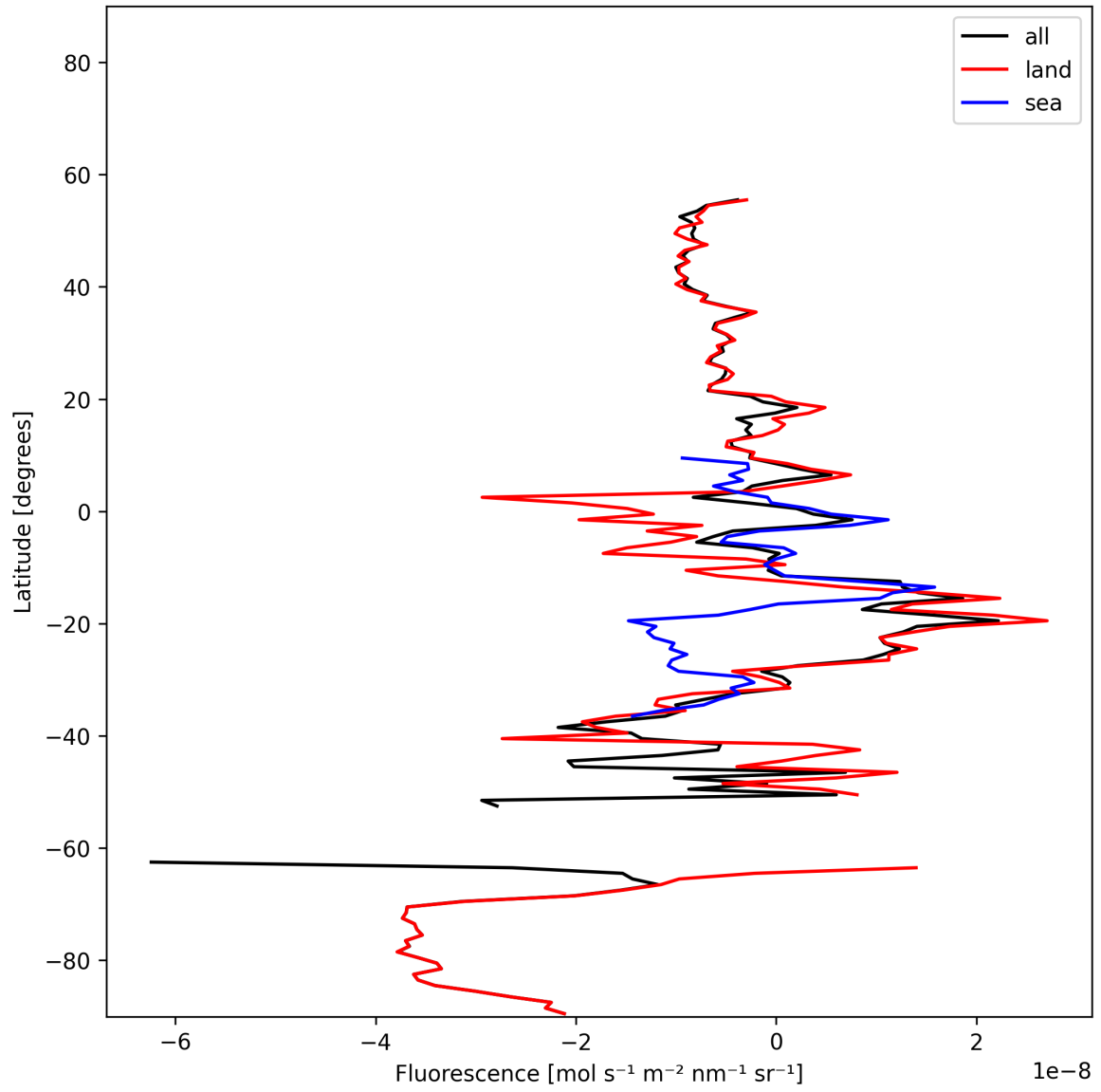
Figure 21: Zonal average of “Fluorescence” for 2025-11-19 to 2025-11-21.
