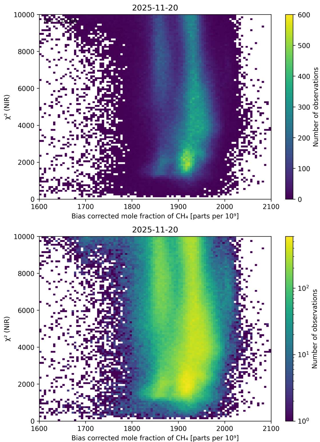
Figure 63: Scatter density plot of “Bias corrected mole fraction of \text{CH}_4 ” against “ \chi^2 (NIR)” for 2025-11-19 to 2025-11-21.
