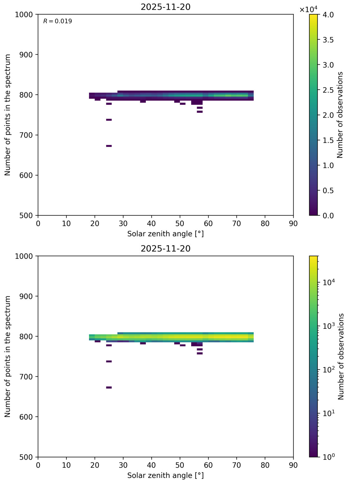
Figure 103: Scatter density plot of “Solar zenith angle” against “Number of points in the spectrum” for 2025-11-19 to 2025-11-21.
