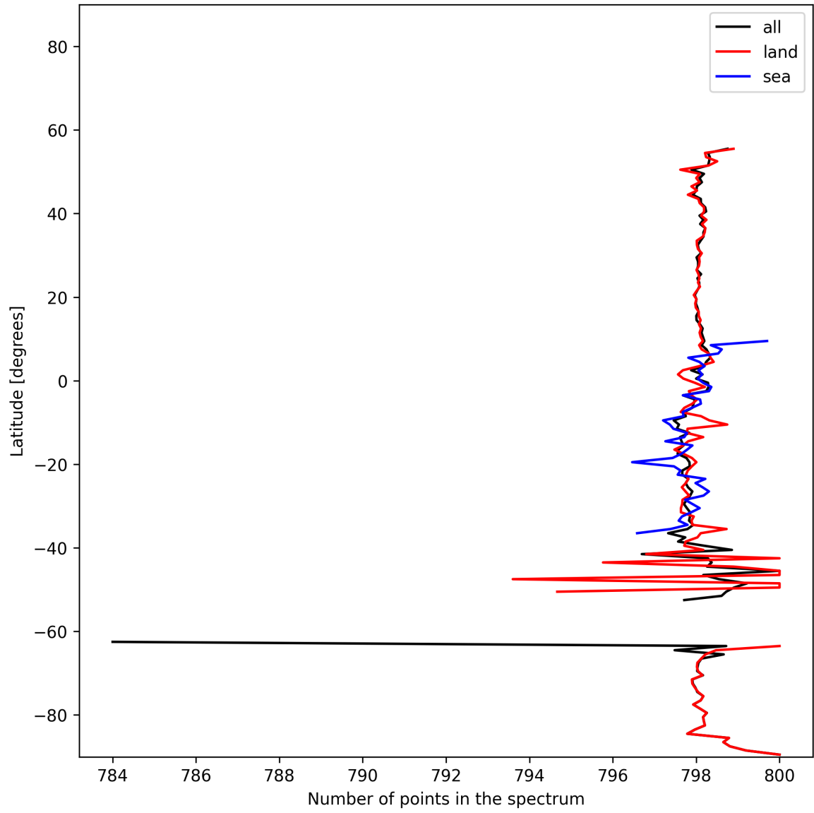
Figure 15: Zonal average of “Number of points in the spectrum” for 2025-11-19 to 2025-11-21.
