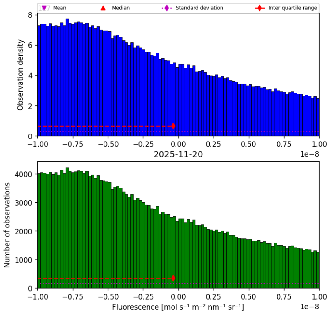
Figure 32: Histogram of “Fluorescence” for 2025-11-19 to 2025-11-21
