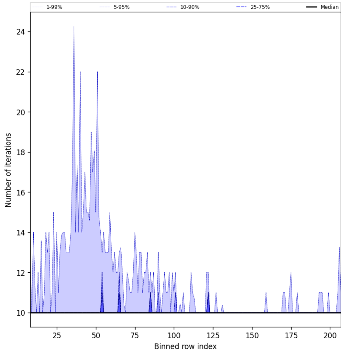
Figure 42: Along track statistics of “Number of iterations” for 2025-11-19 to 2025-11-21
