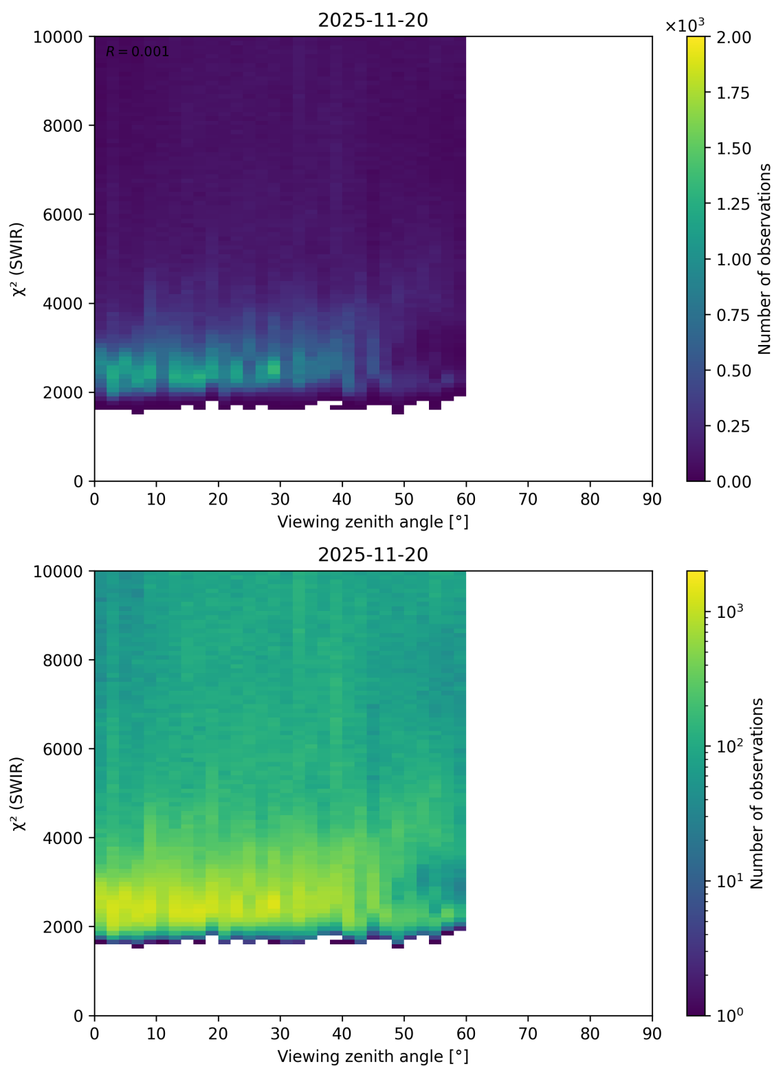
Figure 106: Scatter density plot of “Viewing zenith angle” against “ \chi^2 (SWIR)” for 2025-11-19 to 2025-11-21.
