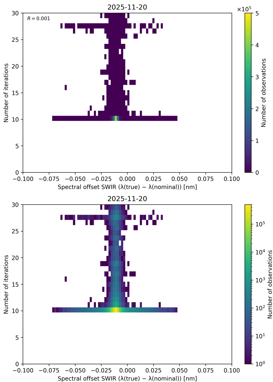
Figure 121: Scatter density plot of “Spectral offset SWIR ( \lambda_{\text{true}} - \lambda_{\text{nominal}} )” against “Number of iterations” for 2025-11-19 to 2025-11-21.
