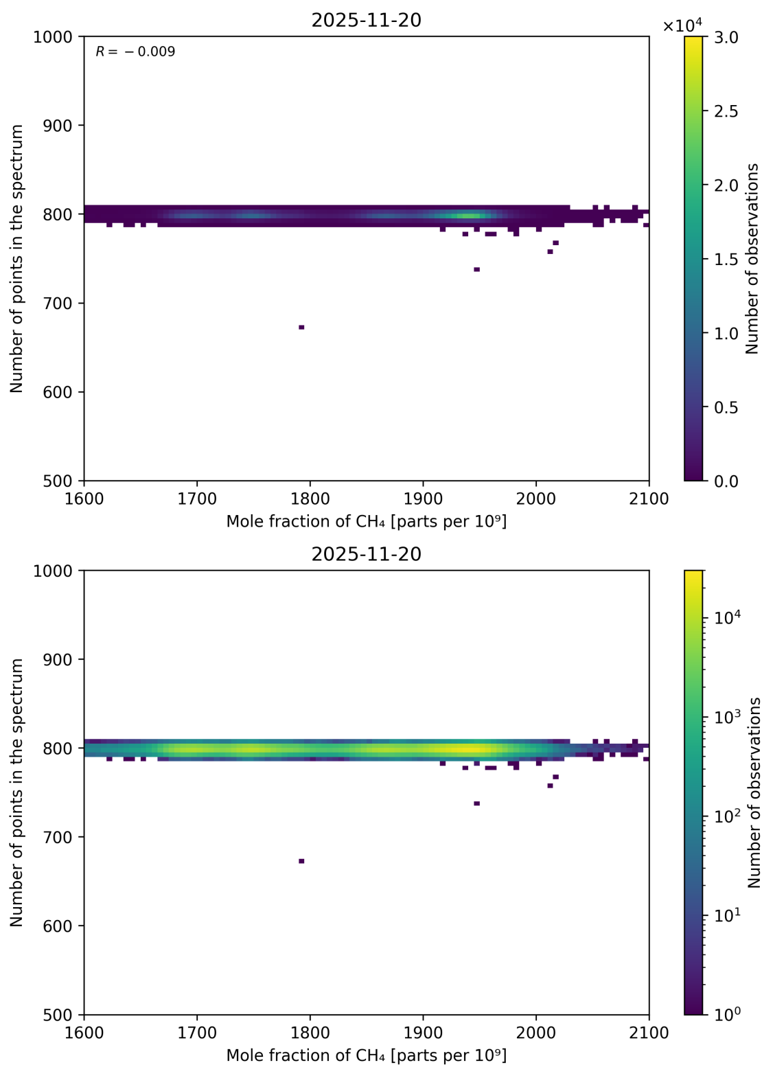
Figure 77: Scatter density plot of “Mole fraction of CH 4 ” against “Number of points in the spectrum” for 2025-11-19 to 2025-11-21.
