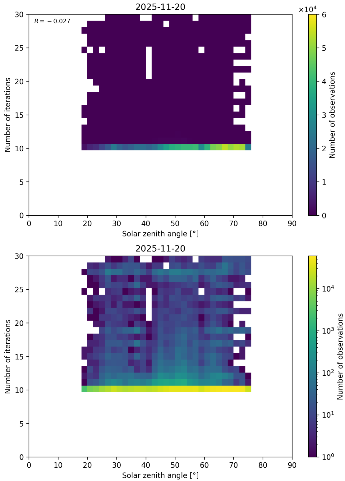
Figure 102: Scatter density plot of “Solar zenith angle” against “Number of iterations” for 2025-11-19 to 2025-11-21.
