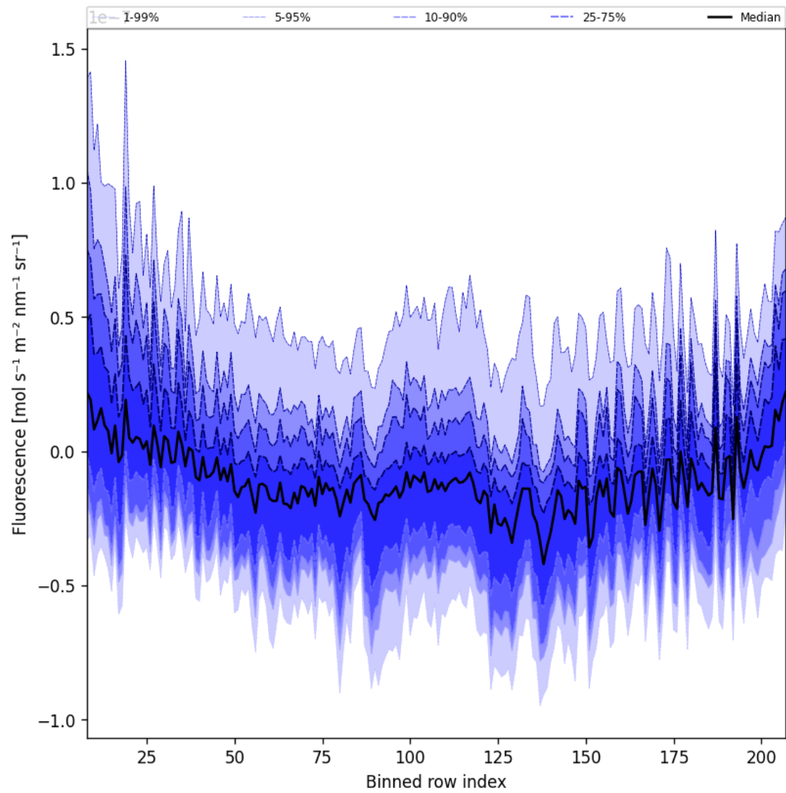
Figure 43: Along track statistics of “Fluorescence” for 2025-11-19 to 2025-11-21
