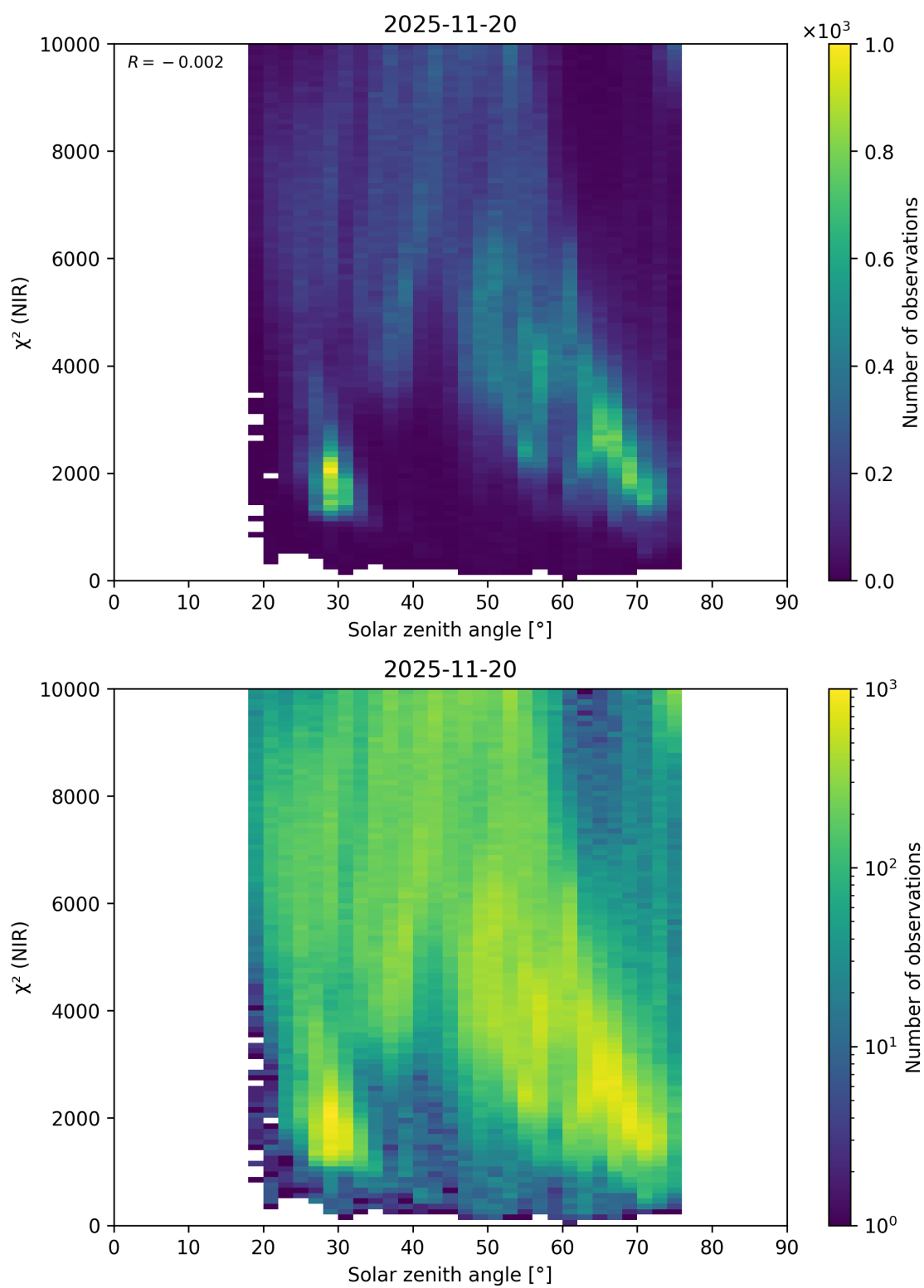
Figure 94: Scatter density plot of “Solar zenith angle” against “ \chi^2 (NIR)” for 2025-11-19 to 2025-11-21.
