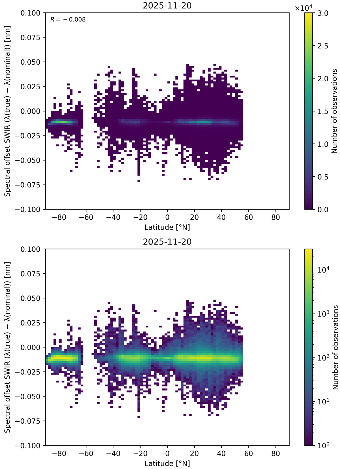
Figure 62: Scatter density plot of “Latitude” against “Spectral offset SWIR ( \lambda_{\text{true}} - \lambda_{\text{nominal}} )” for 2025-11-19 to 2025-11-21.
