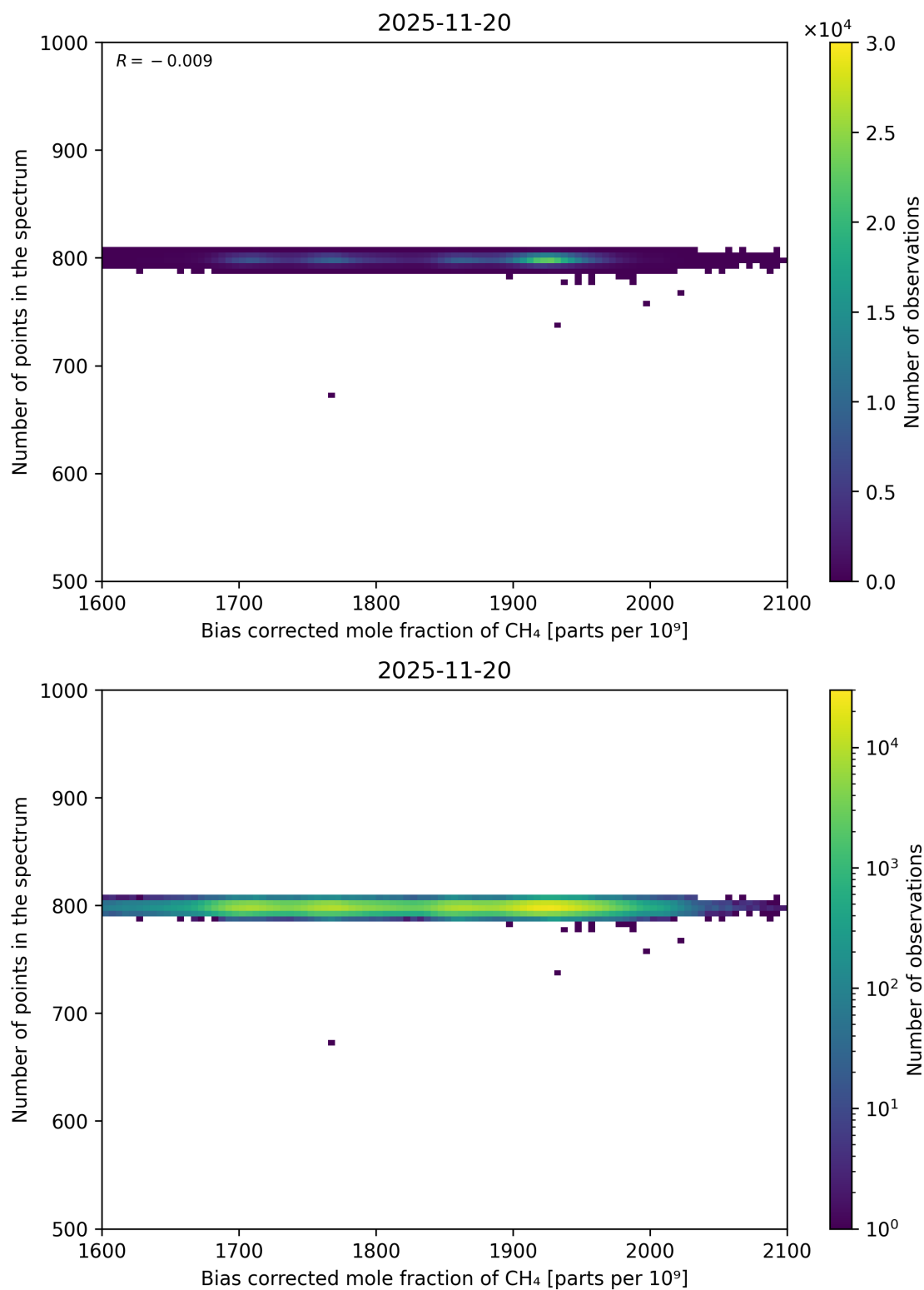
Figure 68: Scatter density plot of “Bias corrected mole fraction of CH 4 ” against “Number of points in the spectrum” for 2025-11-19 to 2025-11-21.
