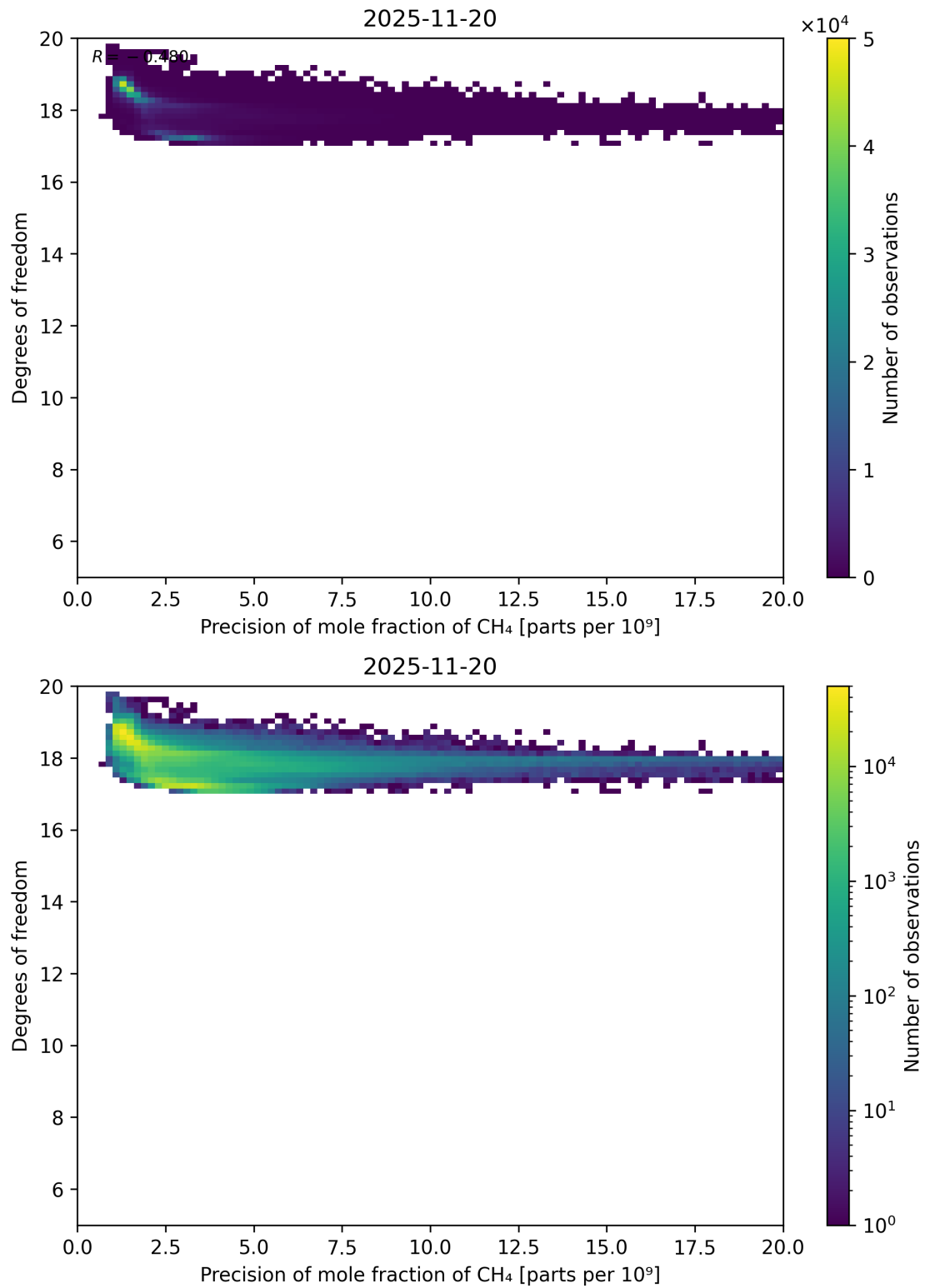
Figure 80: Scatter density plot of “Precision of mole fraction of CH 4 ” against “Degrees of freedom” for 2025-11-19 to 2025-11-21.
