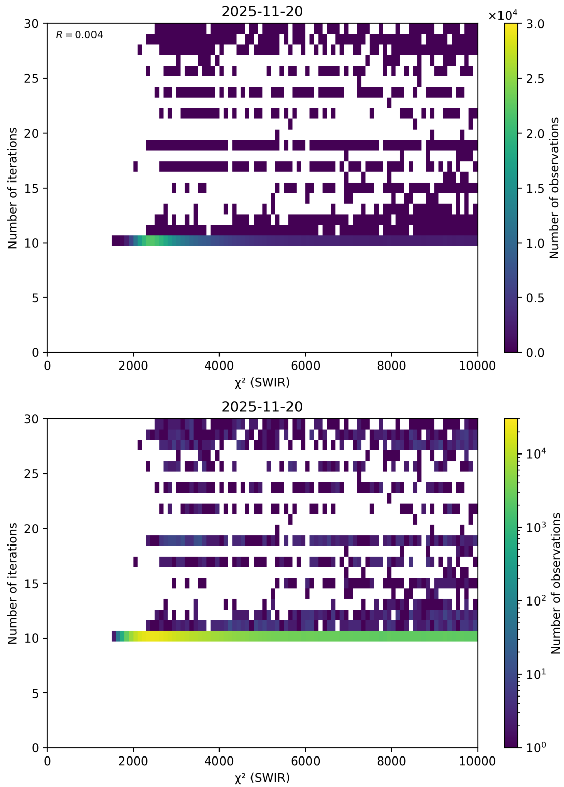
Figure 50: Scatter density plot of “ \chi^2 (SWIR)” against “Number of iterations” for 2025-11-19 to 2025-11-21.
