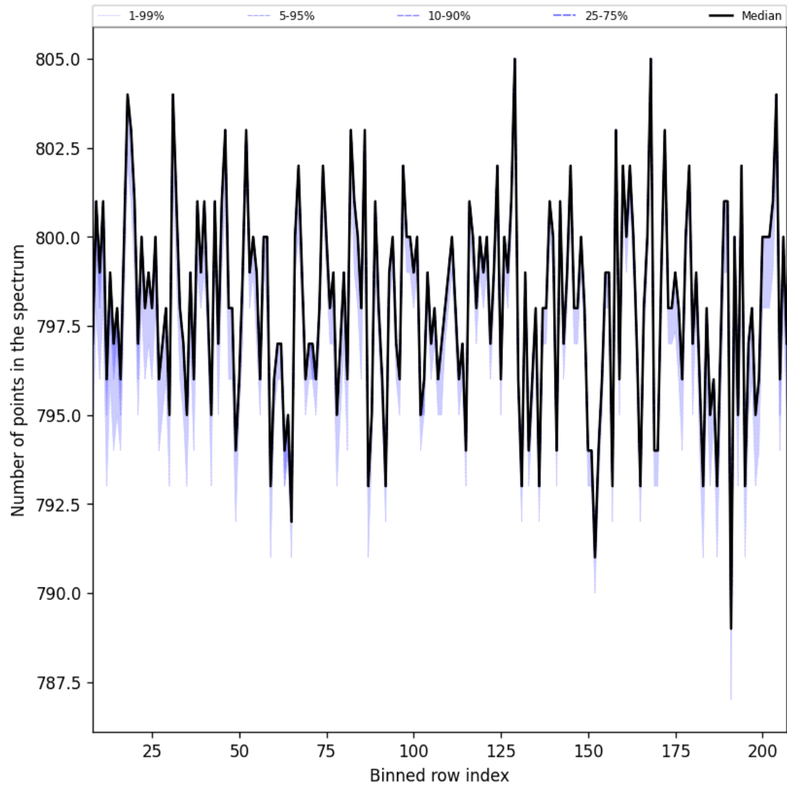
Figure 37: Along track statistics of “Number of points in the spectrum” for 2025-11-19 to 2025-11-21
