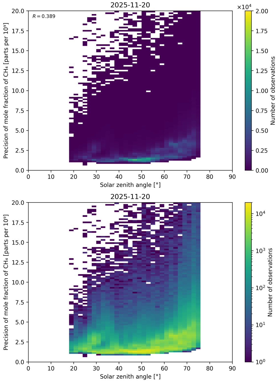
Figure 101: Scatter density plot of “Solar zenith angle” against “Precision of mole fraction of \text{CH}_4 ” for 2025-11-19 to 2025-11-21.
