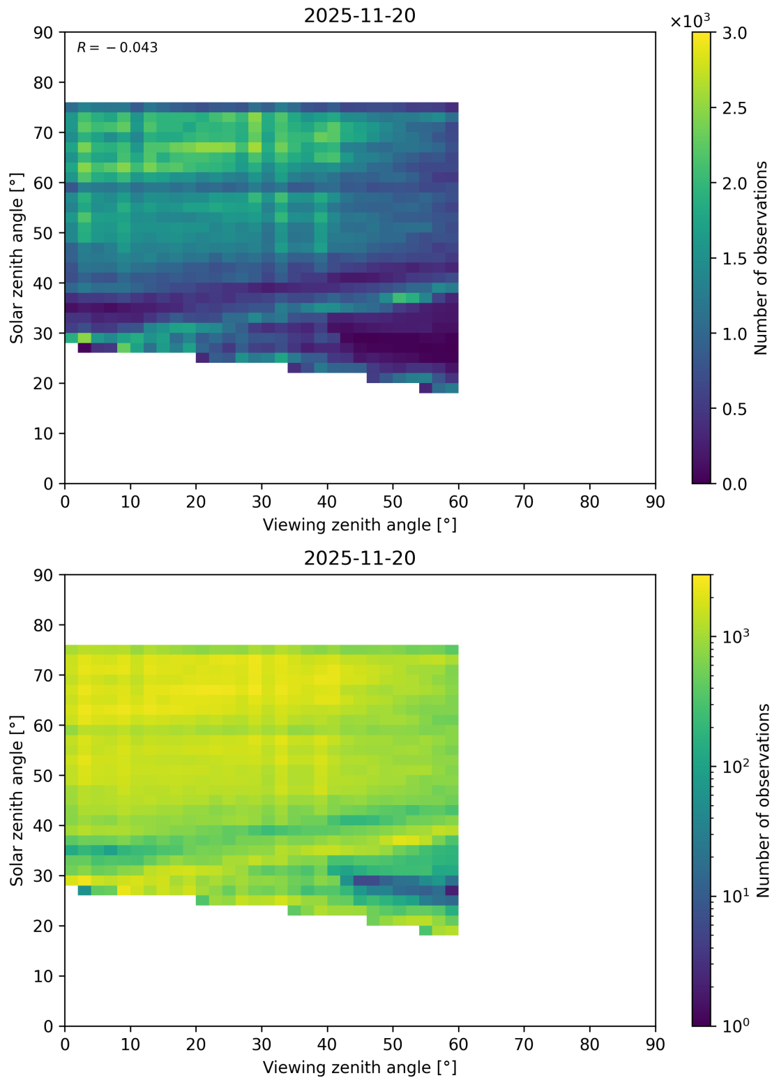
Figure 115: Scatter density plot of “Viewing zenith angle” against “Solar zenith angle” for 2025-11-19 to 2025-11-21.
