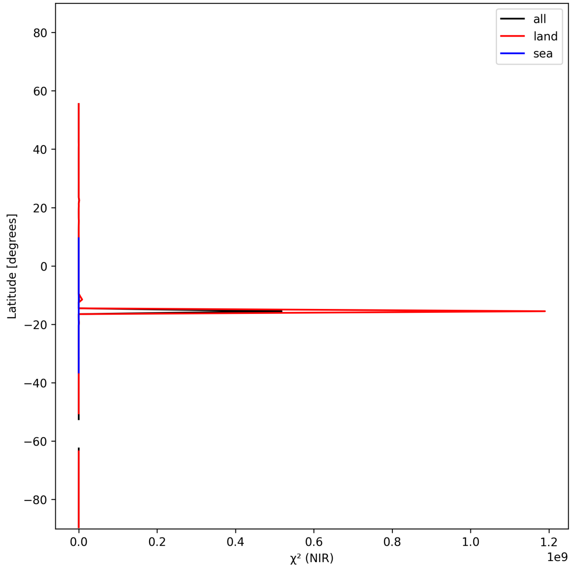
Figure 18: Zonal average of “ \chi^2 (NIR)” for 2025-11-19 to 2025-11-21.
