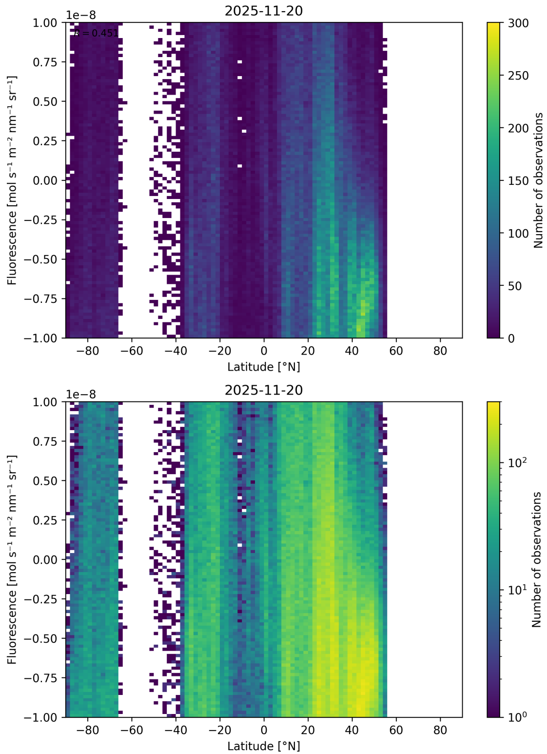
Figure 56: Scatter density plot of “Latitude” against “Fluorescence” for 2025-11-19 to 2025-11-21.
