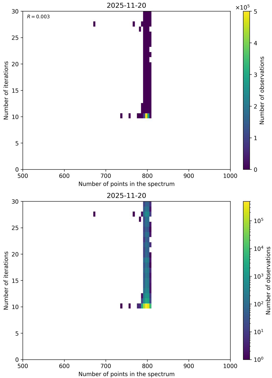
Figure 92: Scatter density plot of “Number of points in the spectrum” against “Number of iterations” for 2025-11-19 to 2025-11-21.
