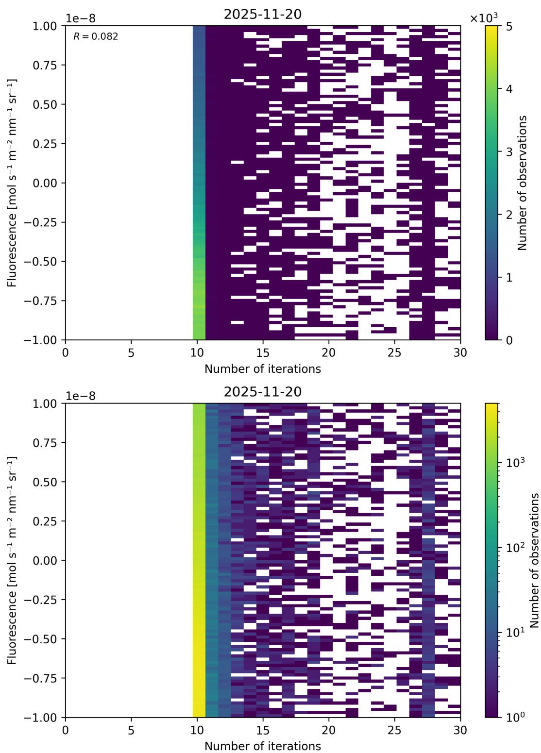
Figure 87: Scatter density plot of “Number of iterations” against “Fluorescence” for 2025-11-19 to 2025-11-21.
