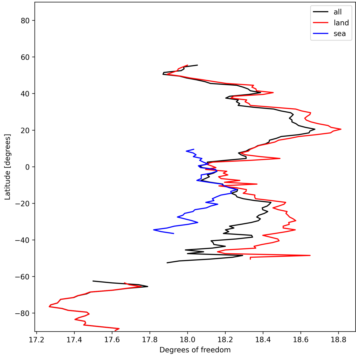
Figure 19: Zonal average of “Degrees of freedom” for 2025-11-19 to 2025-11-21.
