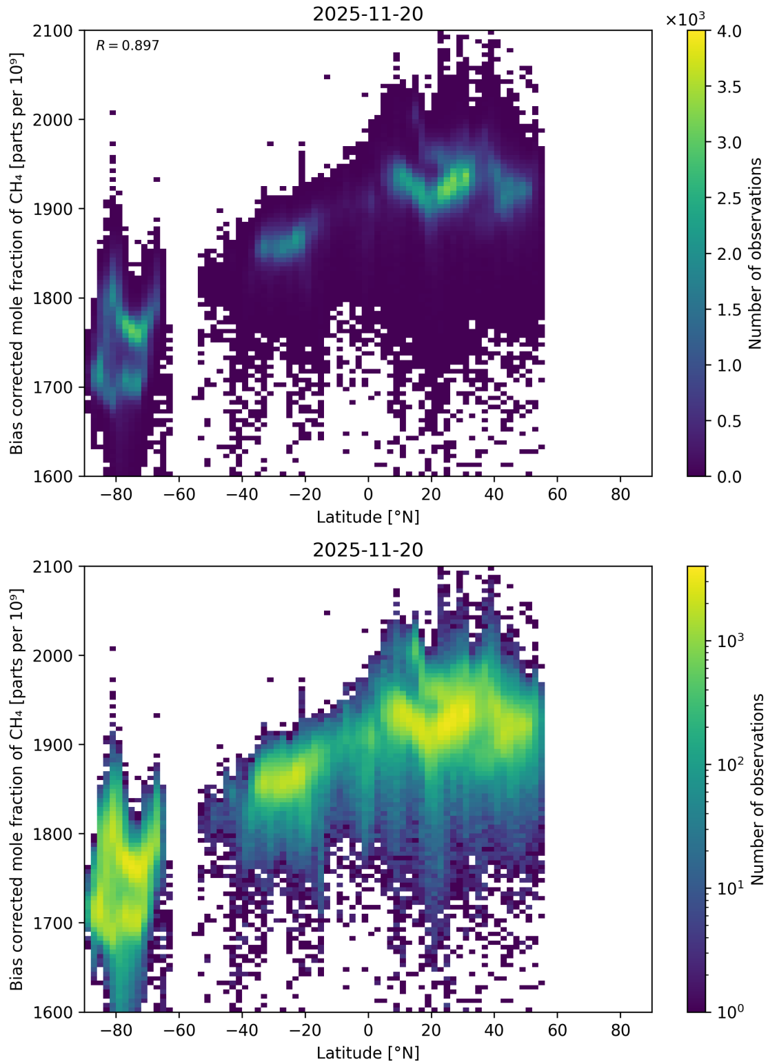
Figure 58: Scatter density plot of “Latitude” against “Bias corrected mole fraction of \text{CH}_4 ” for 2025-11-19 to 2025-11-21.
