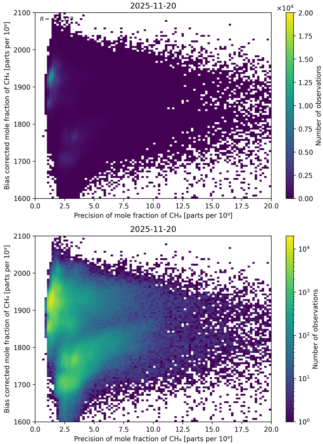
Figure 82: Scatter density plot of “Precision of mole fraction of CH 4 ” against “Bias corrected mole fraction of CH 4 ” for 2025-11-19 to 2025-11-21.
