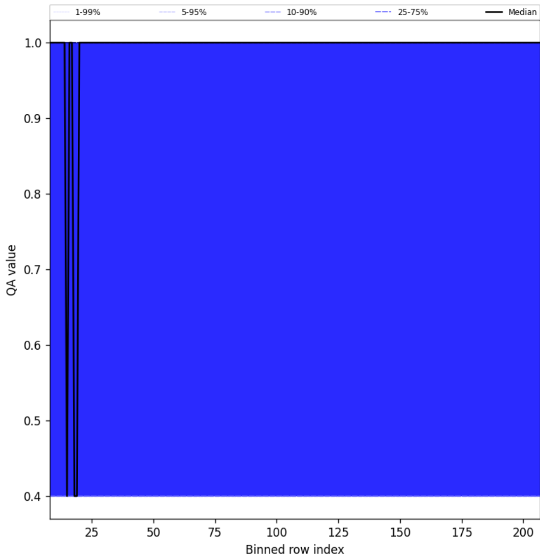
Figure 33: Along track statistics of “QA value” for 2025-11-19 to 2025-11-21
