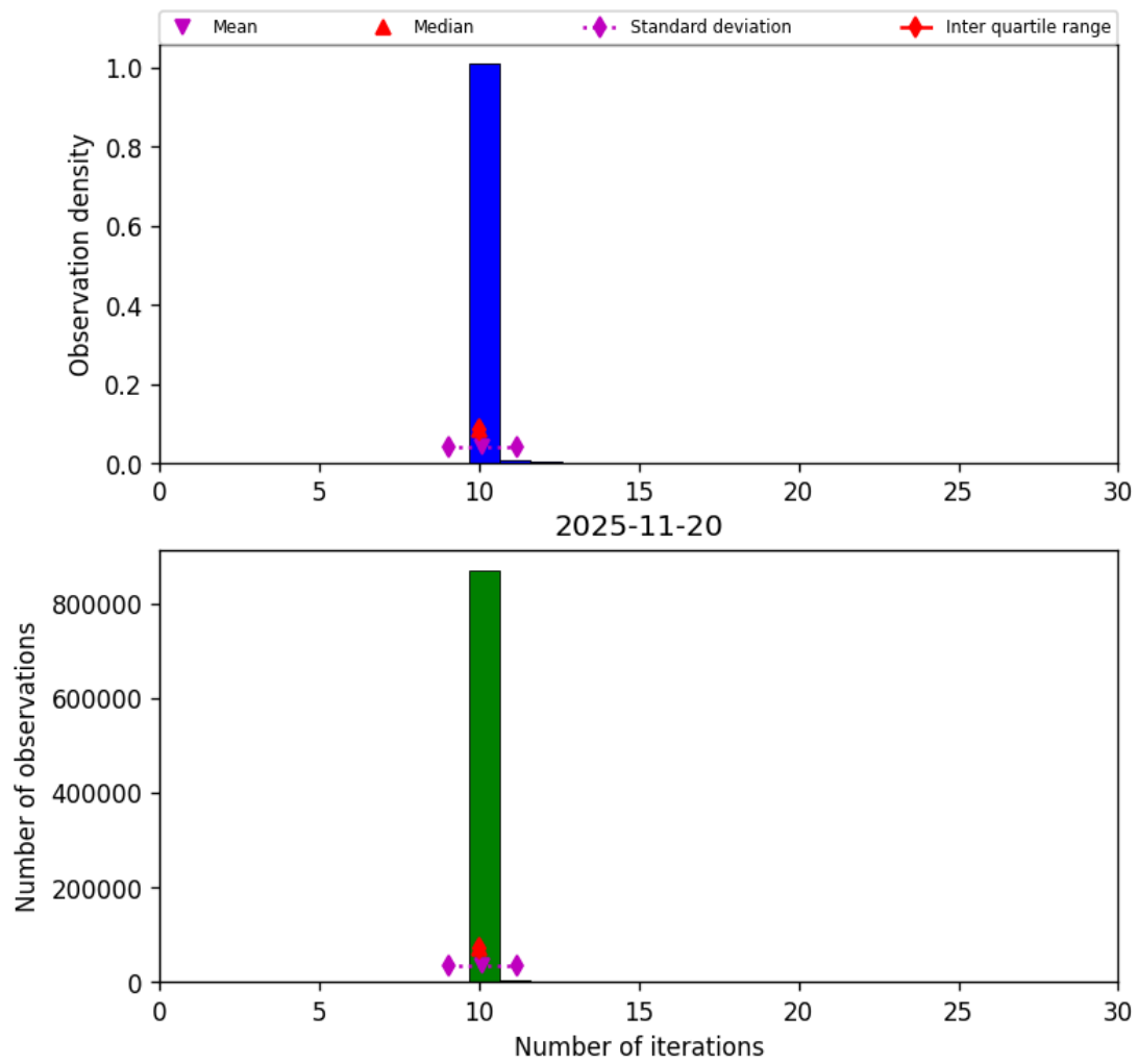
Figure 31: Histogram of “Number of iterations” for 2025-11-19 to 2025-11-21
