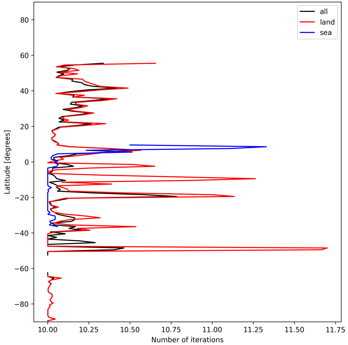
Figure 20: Zonal average of “Number of iterations” for 2025-11-19 to 2025-11-21.
