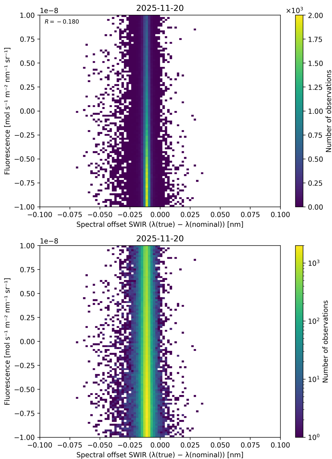
Figure 120: Scatter density plot of “Spectral offset SWIR ( \lambda_{\text{true}} - \lambda_{\text{nominal}} )” against “Fluorescence” for 2025-11-19 to 2025-11-21.
