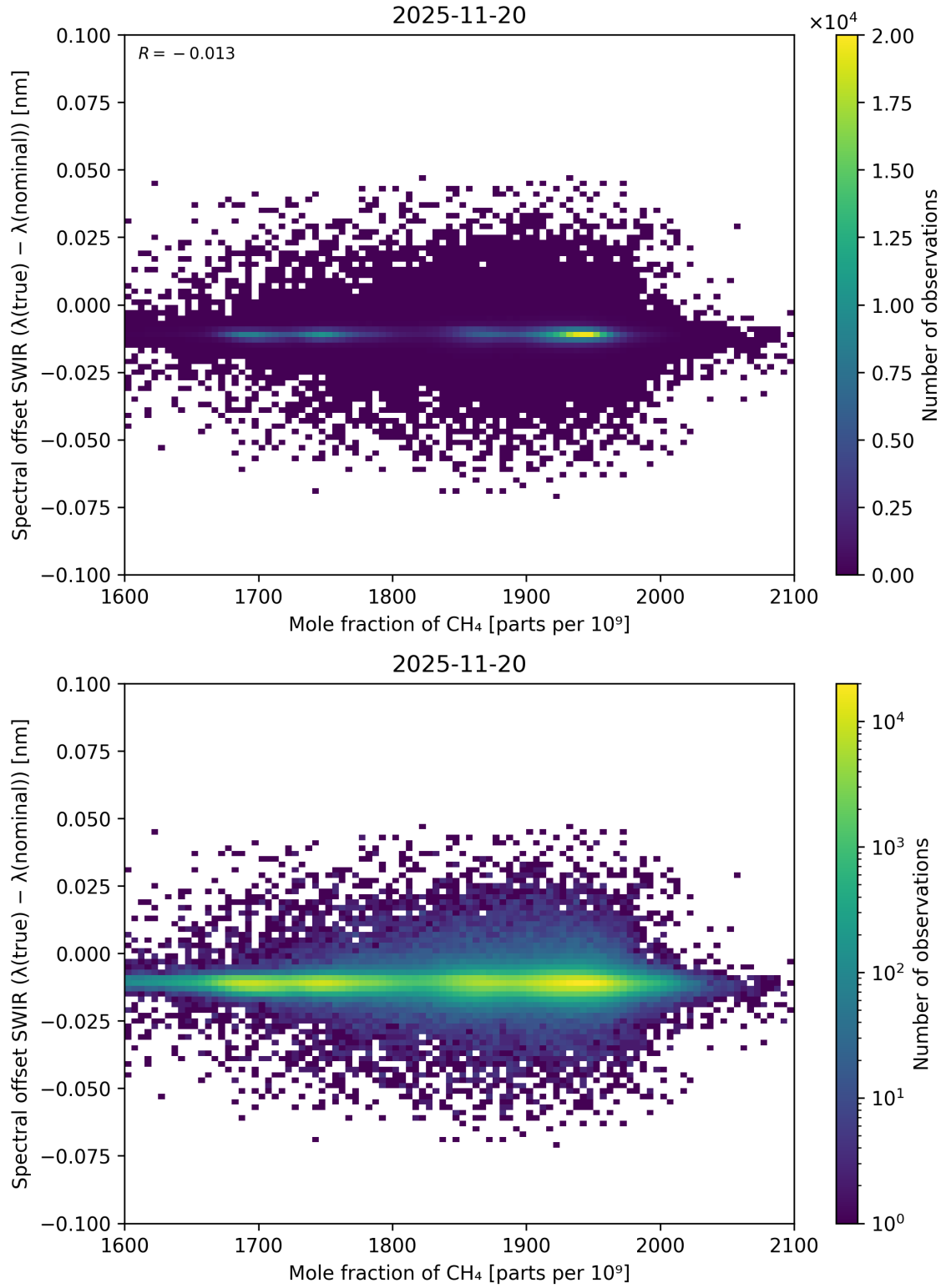
Figure 86: Scatter density plot of “Mole fraction of CH 4 ” against “Spectral offset SWIR ( \lambda_{\text{true}} - \lambda_{\text{nominal}} )” for 2025-11-19 to 2025-11-21.
