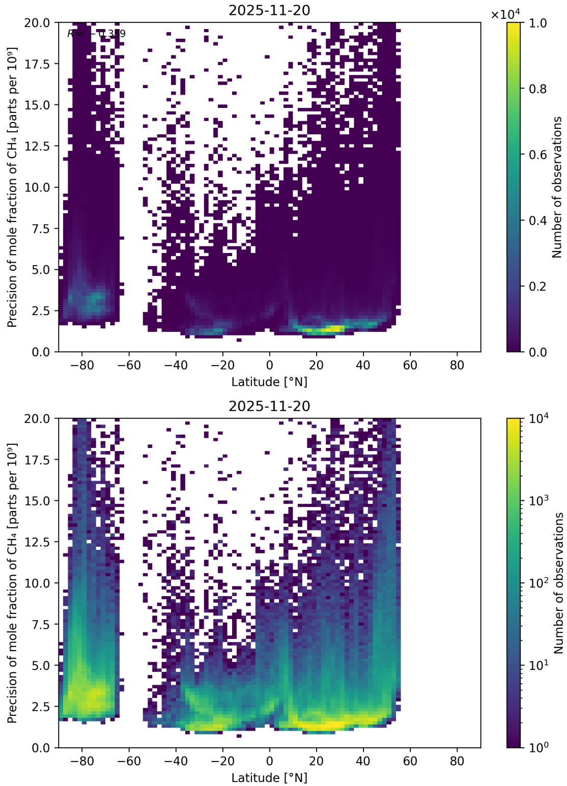
Figure 59: Scatter density plot of “Latitude” against “Precision of mole fraction of CH 4 ” for 2025-11-19 to 2025-11-21.
