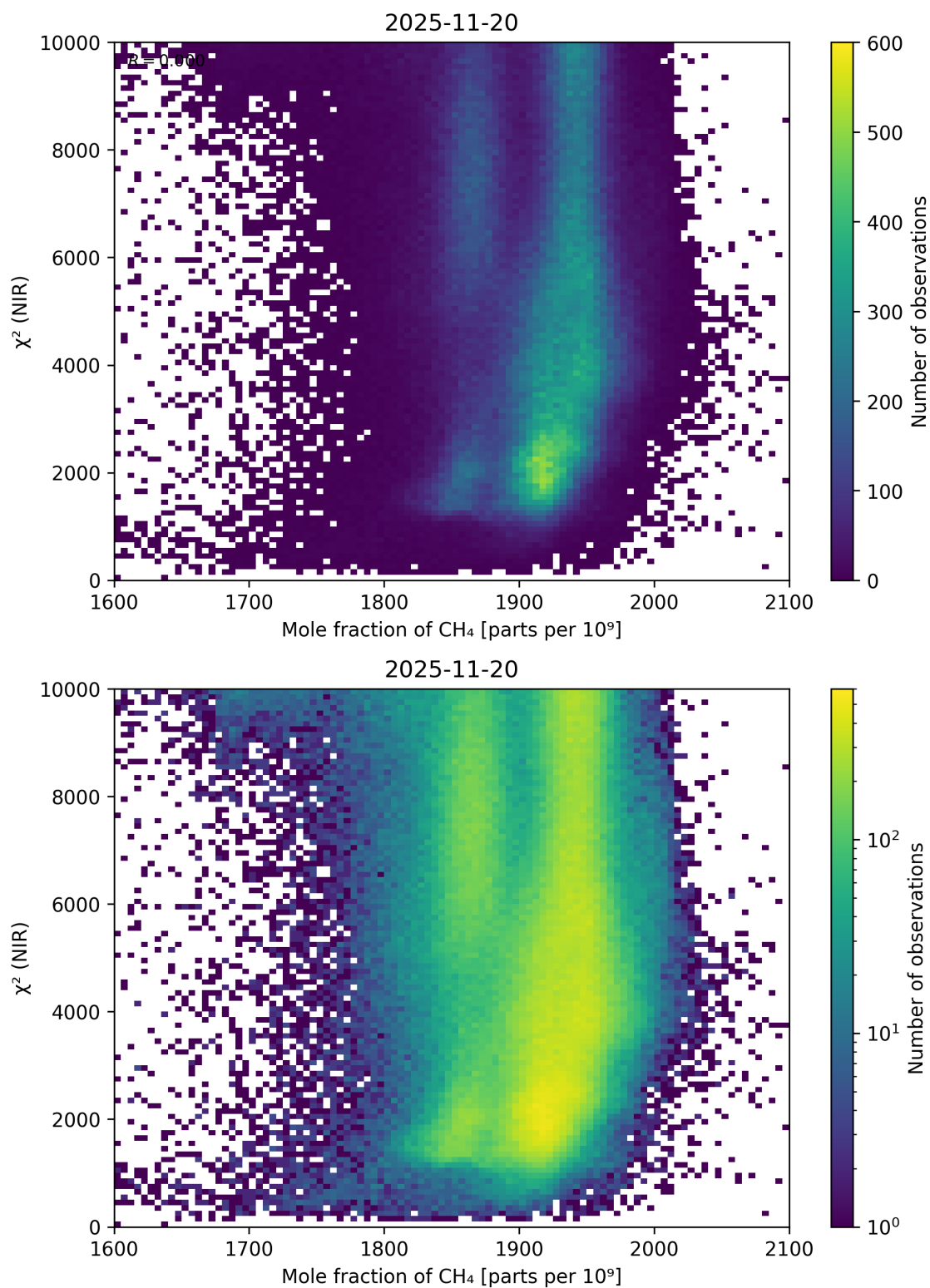
Figure 70: Scatter density plot of “Mole fraction of CH 4 ” against “ \chi^2 (NIR)” for 2025-11-19 to 2025-11-21.
