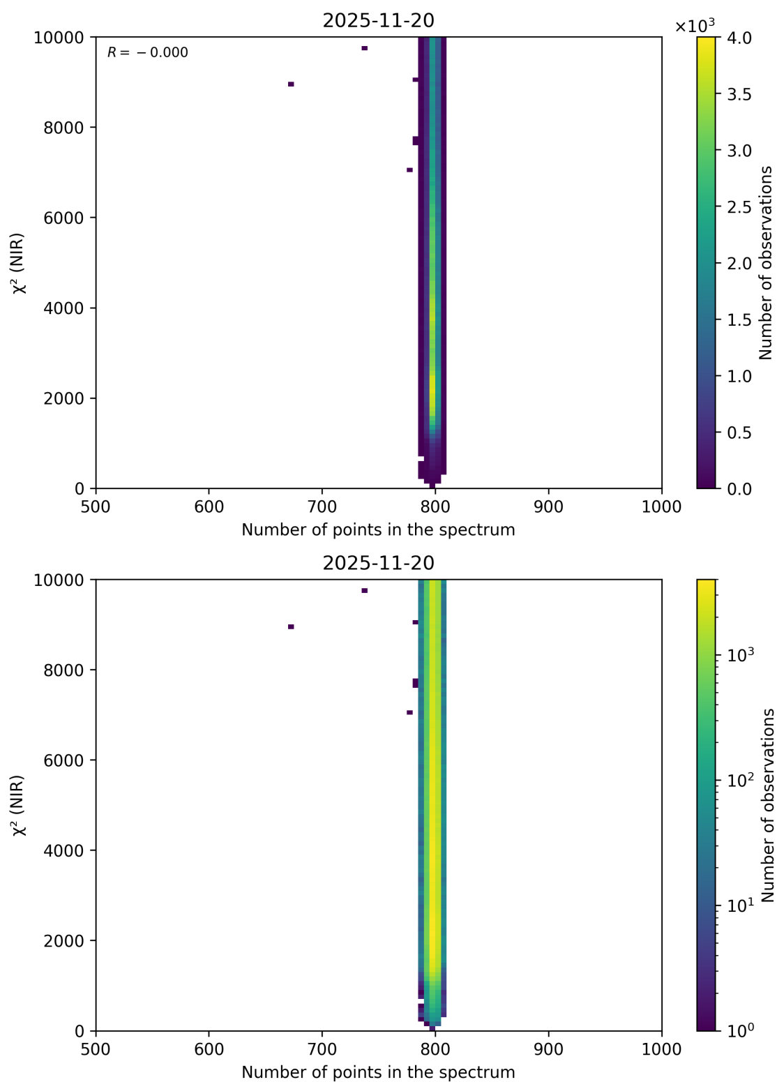
Figure 88: Scatter density plot of “Number of points in the spectrum” against “ \chi^2 (NIR)” for 2025-11-19 to 2025-11-21.
