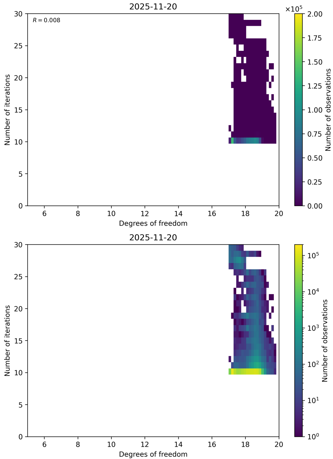
Figure 52: Scatter density plot of “Degrees of freedom” against “Number of iterations” for 2025-11-19 to 2025-11-21.
