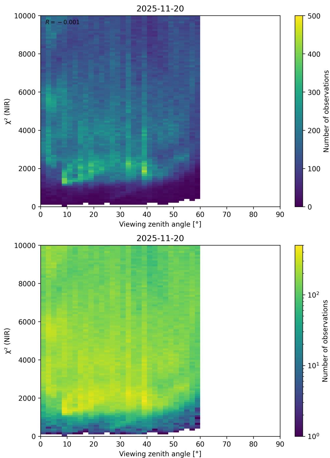
Figure 105: Scatter density plot of “Viewing zenith angle” against “ \chi^2 (NIR)” for 2025-11-19 to 2025-11-21.
