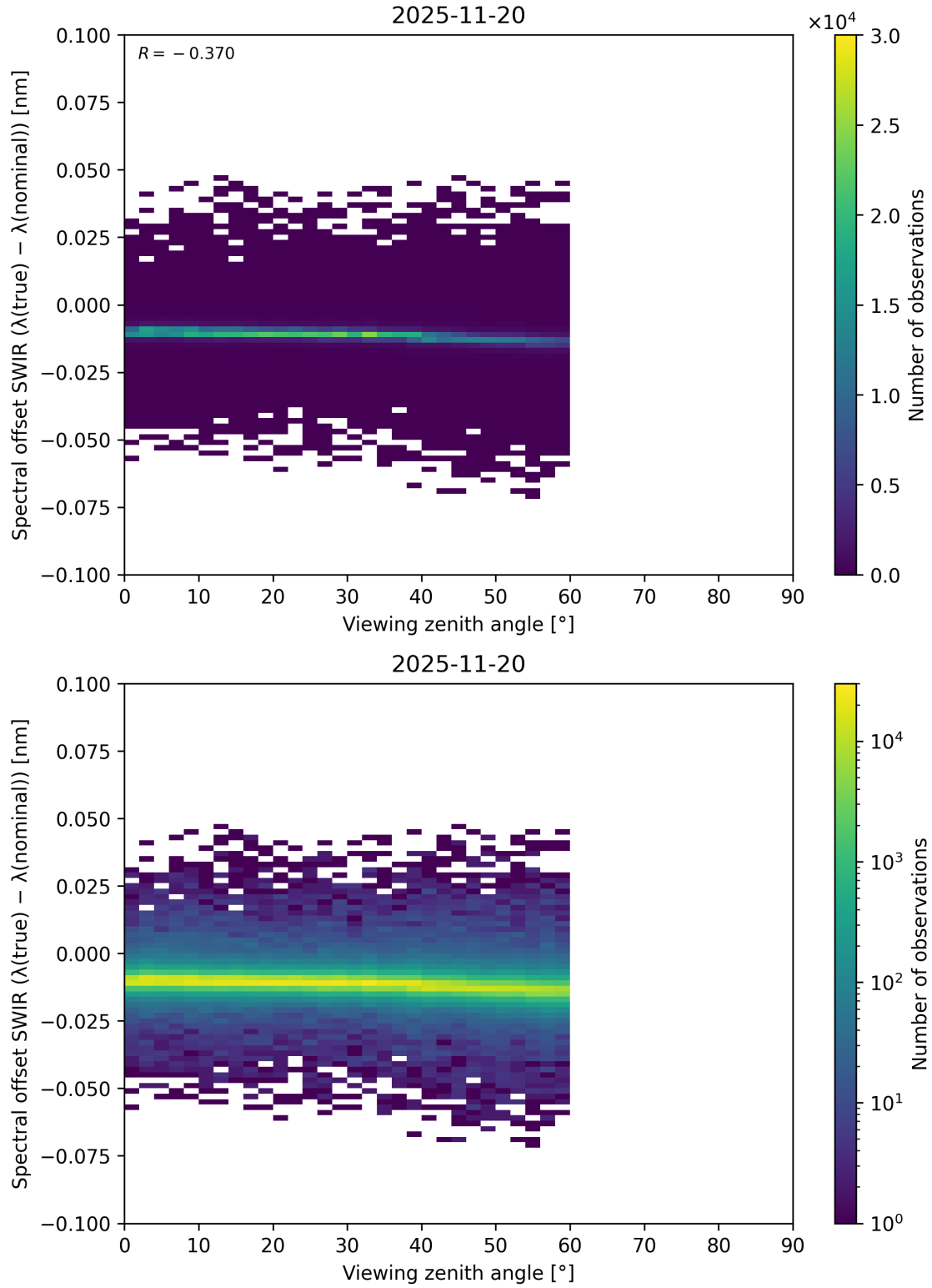
Figure 116: Scatter density plot of “Viewing zenith angle” against “Spectral offset SWIR ( \lambda_{\text{true}} - \lambda_{\text{nominal}} )” for 2025-11-19 to 2025-11-21.
