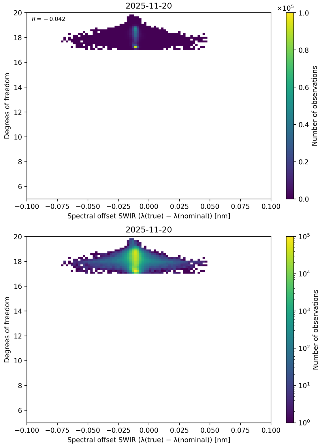
Figure 119: Scatter density plot of “Spectral offset SWIR ( \lambda_{\text{true}} - \lambda_{\text{nominal}} )” against “Degrees of freedom” for 2025-11-19 to 2025-11-21.
