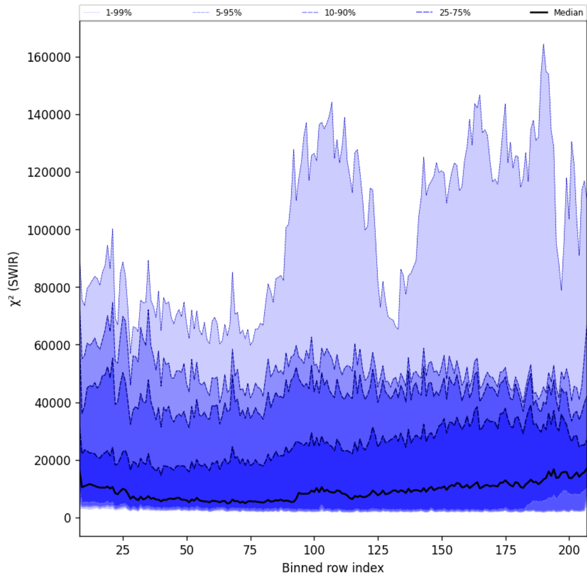
Figure 39: Along track statistics of " \chi^2 (SWIR)" for 2025-11-19 to 2025-11-21
