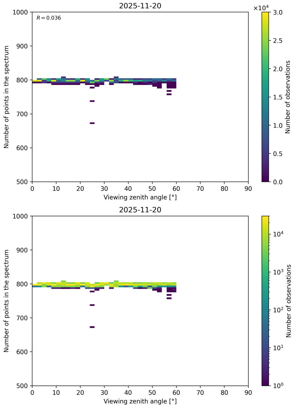
Figure 114: Scatter density plot of “Viewing zenith angle” against “Number of points in the spectrum” for 2025-11-19 to 2025-11-21.
