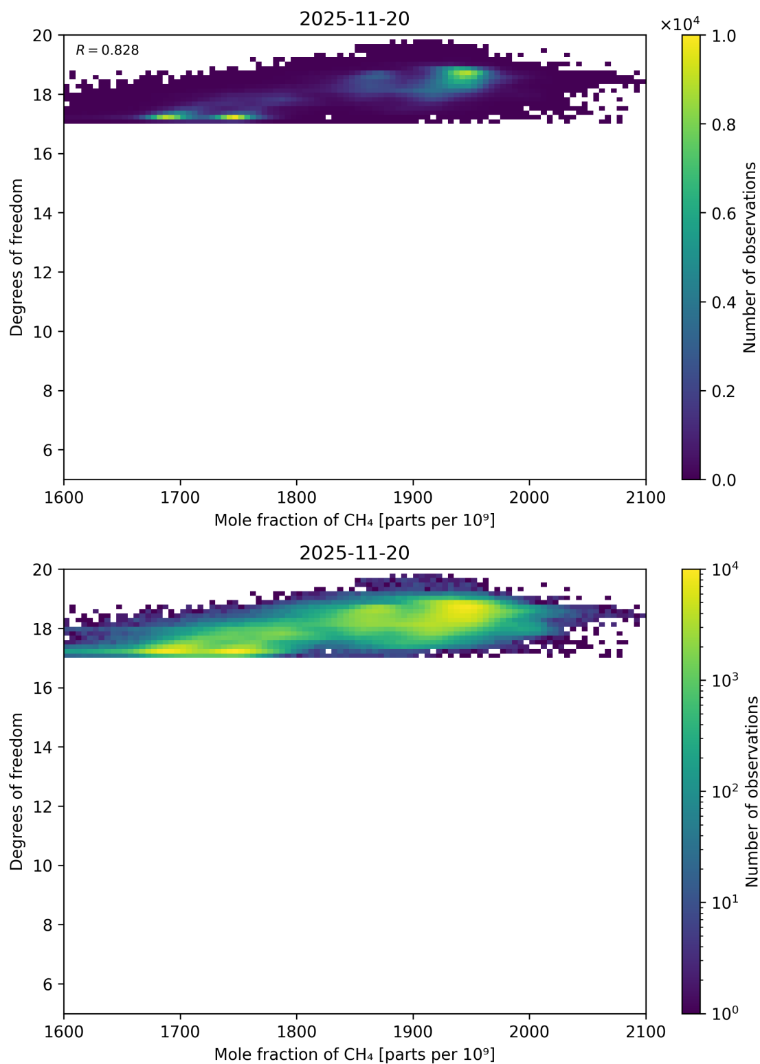
Figure 72: Scatter density plot of “Mole fraction of CH 4 ” against “Degrees of freedom” for 2025-11-19 to 2025-11-21.
