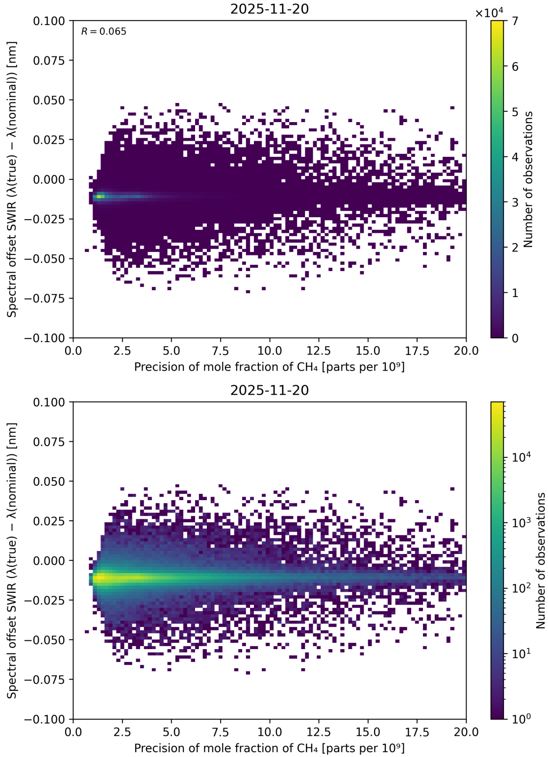
Figure 85: Scatter density plot of “Precision of mole fraction of \text{CH}_4 ” against “Spectral offset SWIR ( \lambda_{\text{true}} - \lambda_{\text{nominal}} )” for 2025-11-19 to 2025-11-21.
