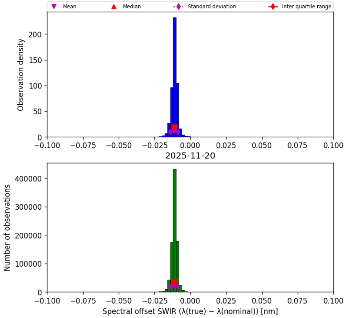
Figure 27: Histogram of “Spectral offset SWIR ( \lambda_{\text{true}} - \lambda_{\text{nominal}} )” for 2025-11-19 to 2025-11-21
