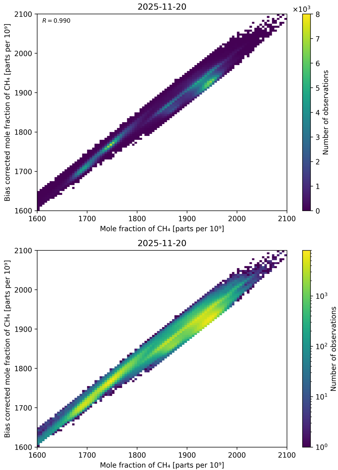
Figure 74: Scatter density plot of “Mole fraction of CH 4 ” against “Bias corrected mole fraction of CH 4 ” for 2025-11-19 to 2025-11-21.
