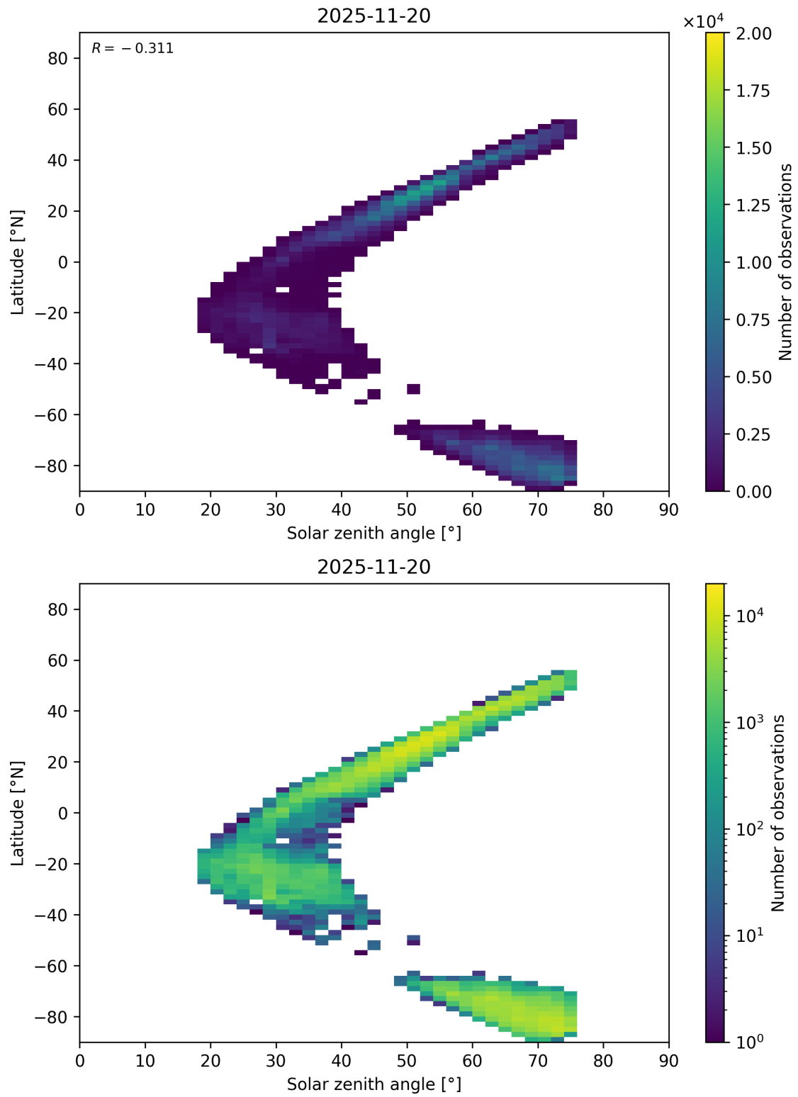
Figure 98: Scatter density plot of “Solar zenith angle” against “Latitude” for 2025-11-19 to 2025-11-21.
