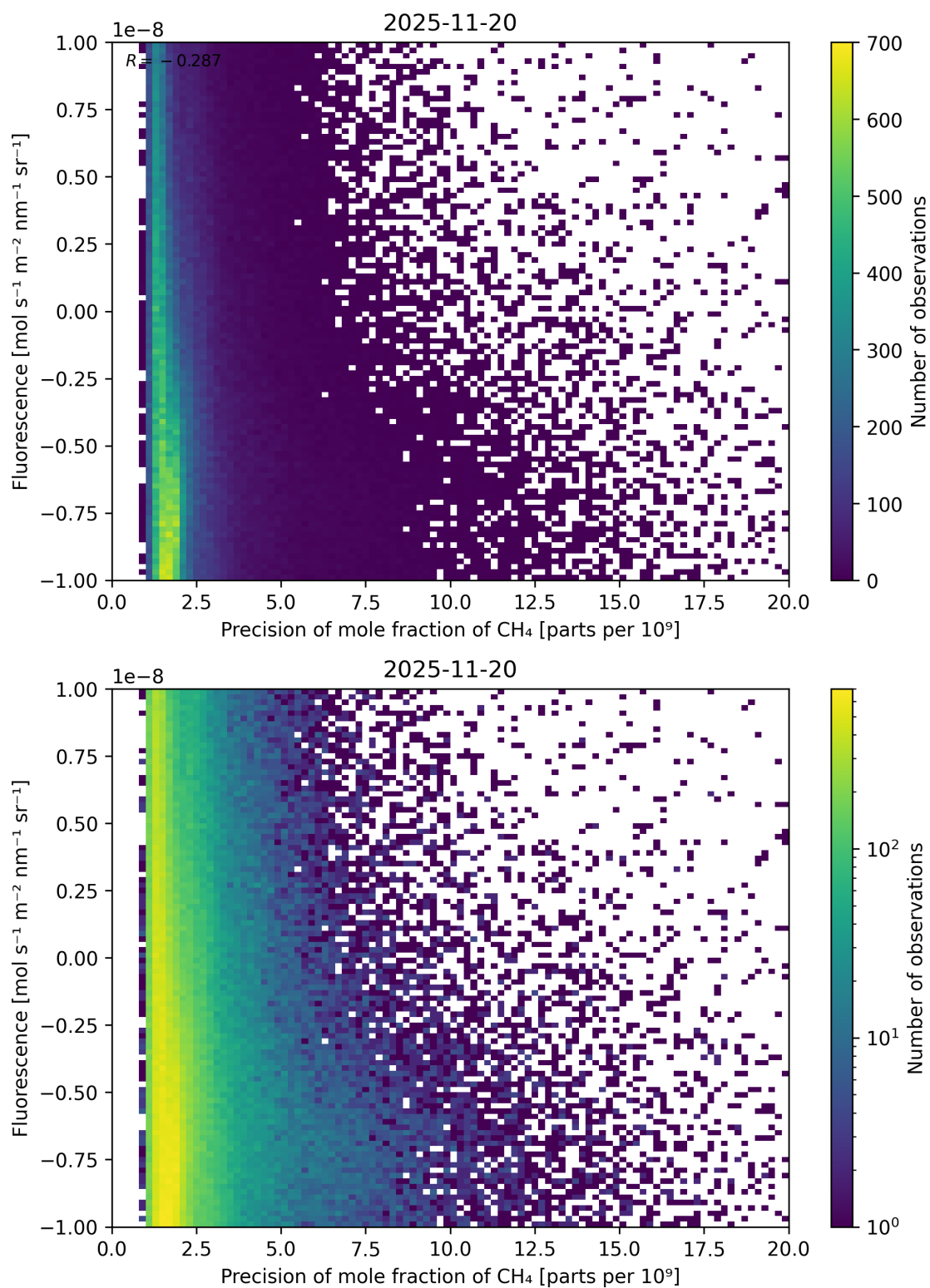
Figure 81: Scatter density plot of “Precision of mole fraction of \text{CH}_4 ” against “Fluorescence” for 2025-11-19 to 2025-11-21.
