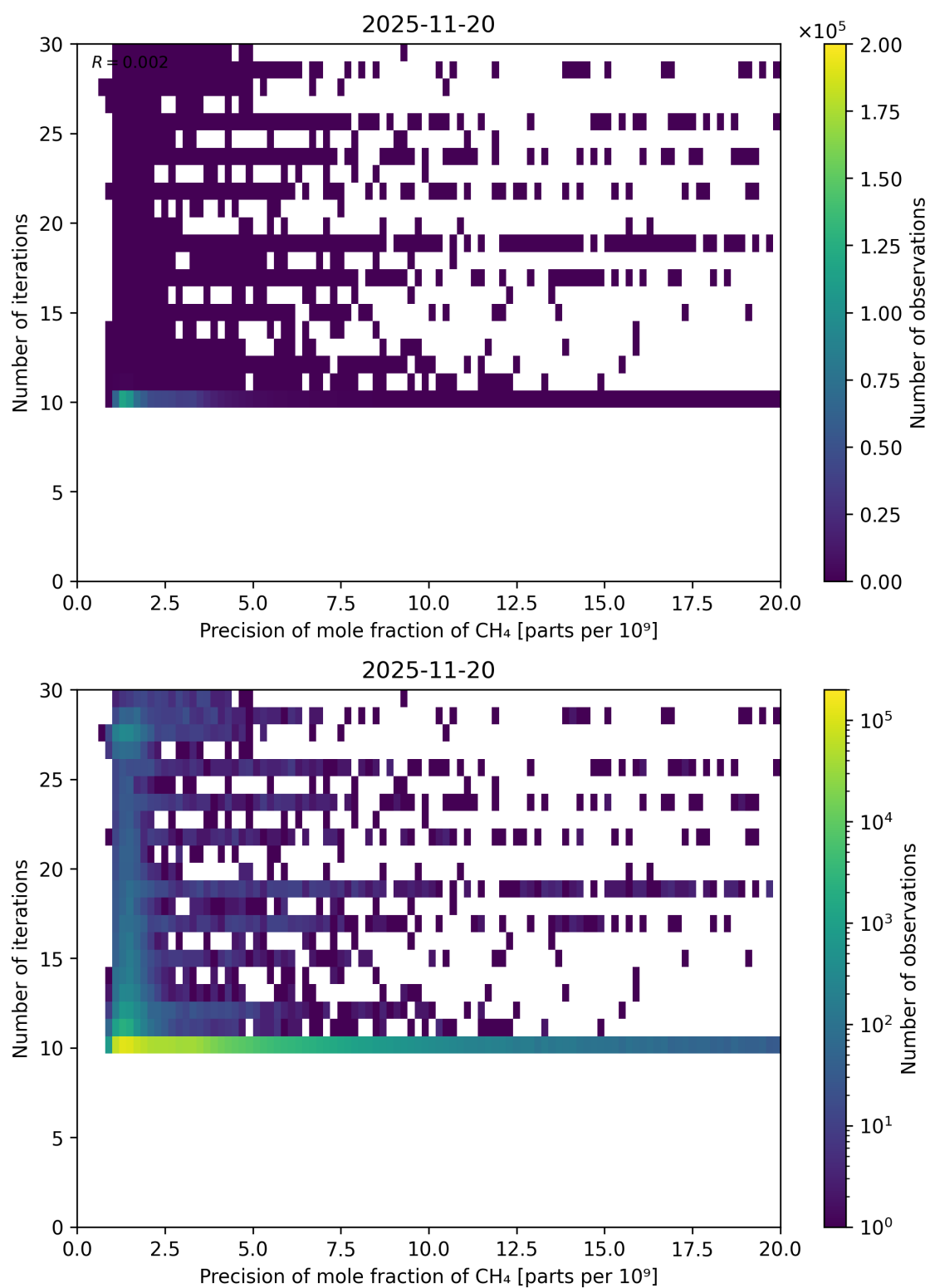
Figure 83: Scatter density plot of “Precision of mole fraction of CH 4 ” against “Number of iterations” for 2025-11-19 to 2025-11-21.
