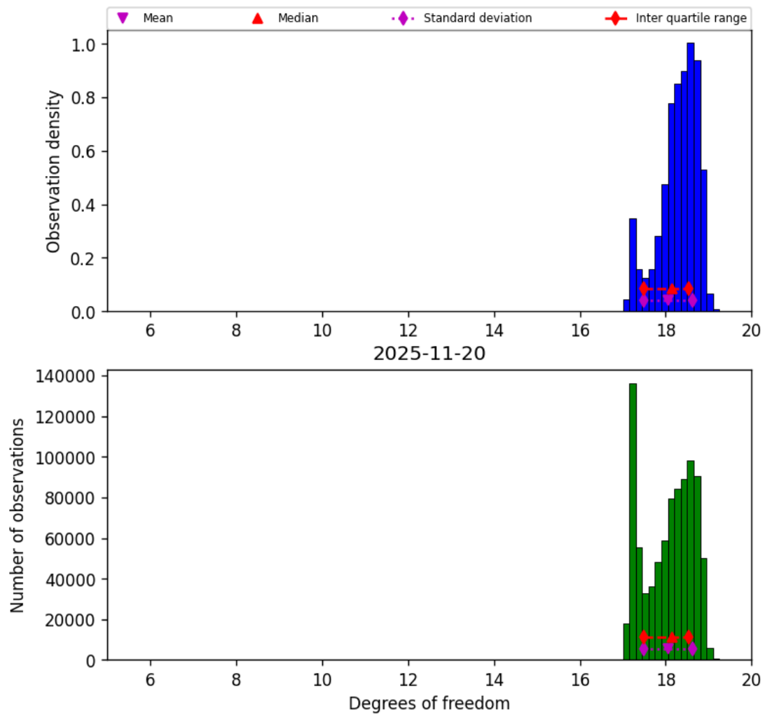
Figure 30: Histogram of “Degrees of freedom” for 2025-11-19 to 2025-11-21
