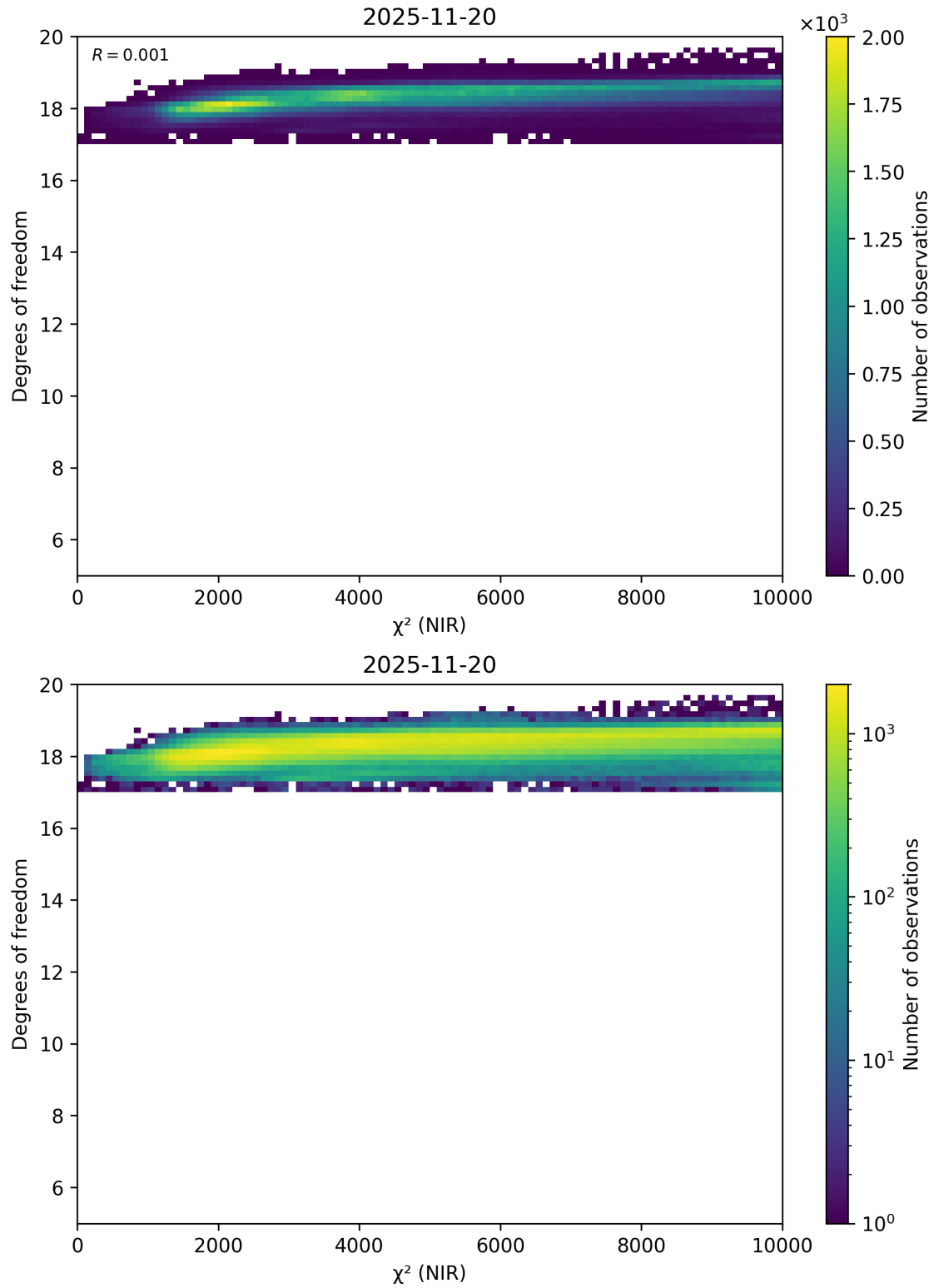
Figure 44: Scatter density plot of “ \chi^2 (NIR)” against “Degrees of freedom” for 2025-11-19 to 2025-11-21.
