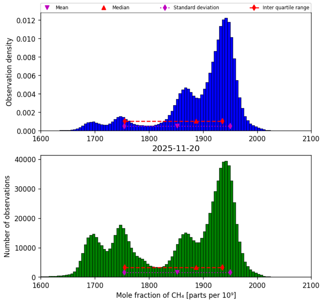
Figure 23: Histogram of “Mole fraction of CH 4 ” for 2025-11-19 to 2025-11-21
