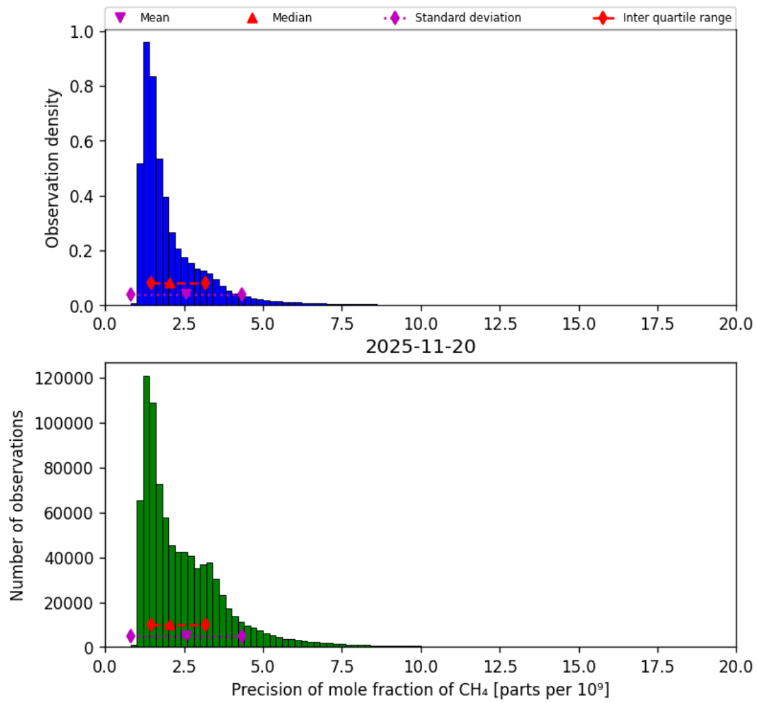
Figure 24: Histogram of “Precision of mole fraction of CH 4 ” for 2025-11-19 to 2025-11-21
