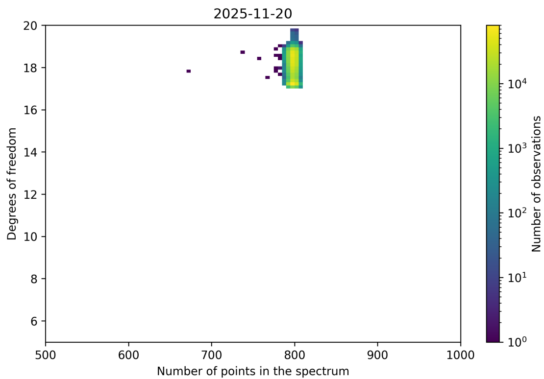
Figure 90: Scatter density plot of “Number of points in the spectrum” against “Degrees of freedom” for 2025-11-19 to 2025-11-21.
