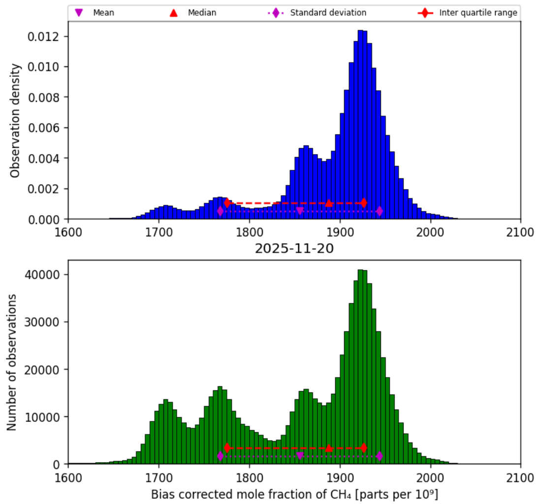
Figure 25: Histogram of “Bias corrected mole fraction of CH 4 ” for 2025-11-19 to 2025-11-21
