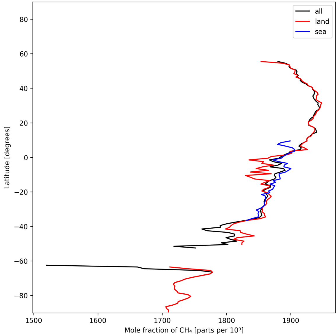
Figure 12: Zonal average of “Mole fraction of CH 4 ” for 2025-11-19 to 2025-11-21.
