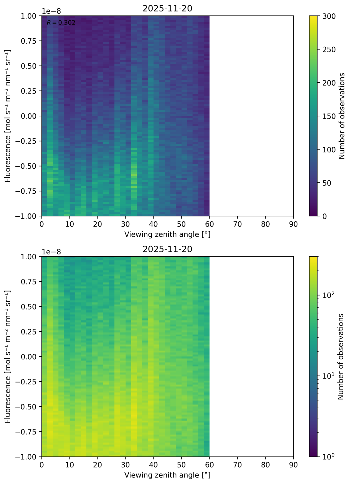
Figure 108: Scatter density plot of “Viewing zenith angle” against “Fluorescence” for 2025-11-19 to 2025-11-21.
