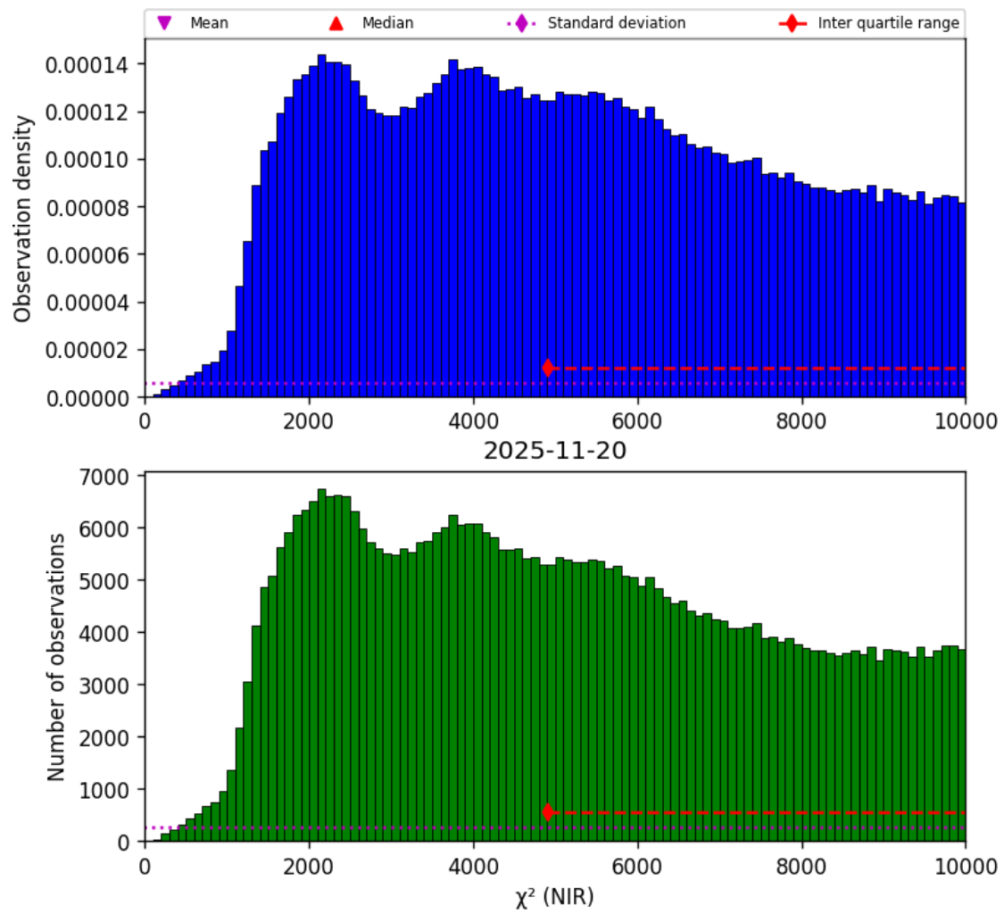
Figure 29: Histogram of “ \chi^2 (NIR)” for 2025-11-19 to 2025-11-21
