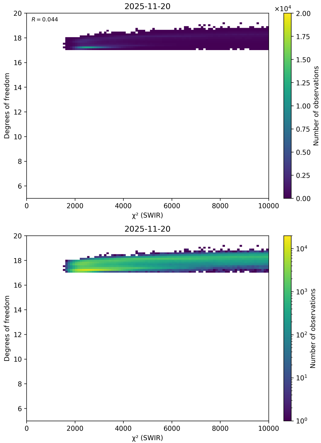
Figure 48: Scatter density plot of “ \chi^2 (SWIR)” against “Degrees of freedom” for 2025-11-19 to 2025-11-21.
