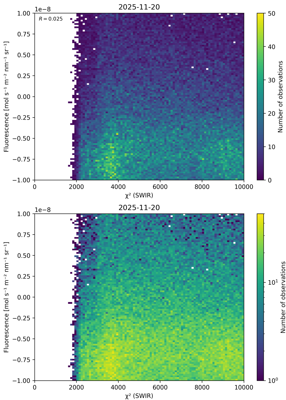
Figure 49: Scatter density plot of “ \chi^2 (SWIR)” against “Fluorescence” for 2025-11-19 to 2025-11-21.
