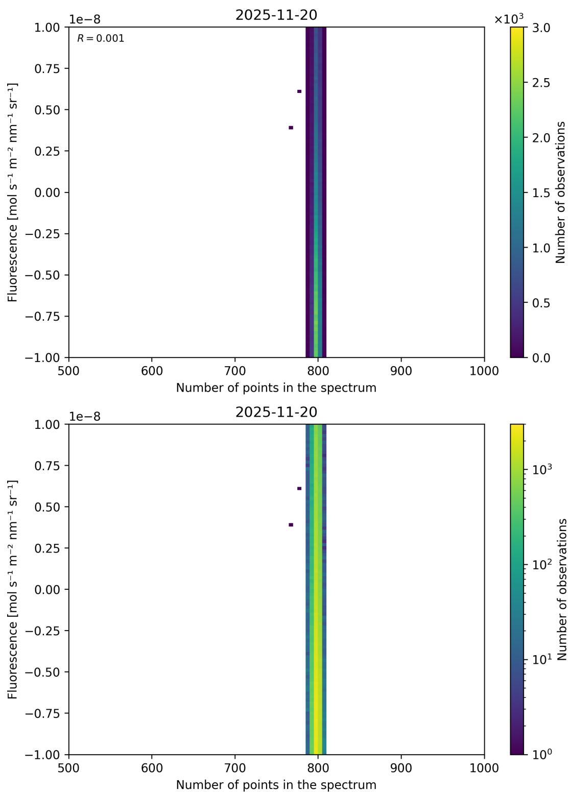
Figure 91: Scatter density plot of “Number of points in the spectrum” against “Fluorescence” for 2025-11-19 to 2025-11-21.
