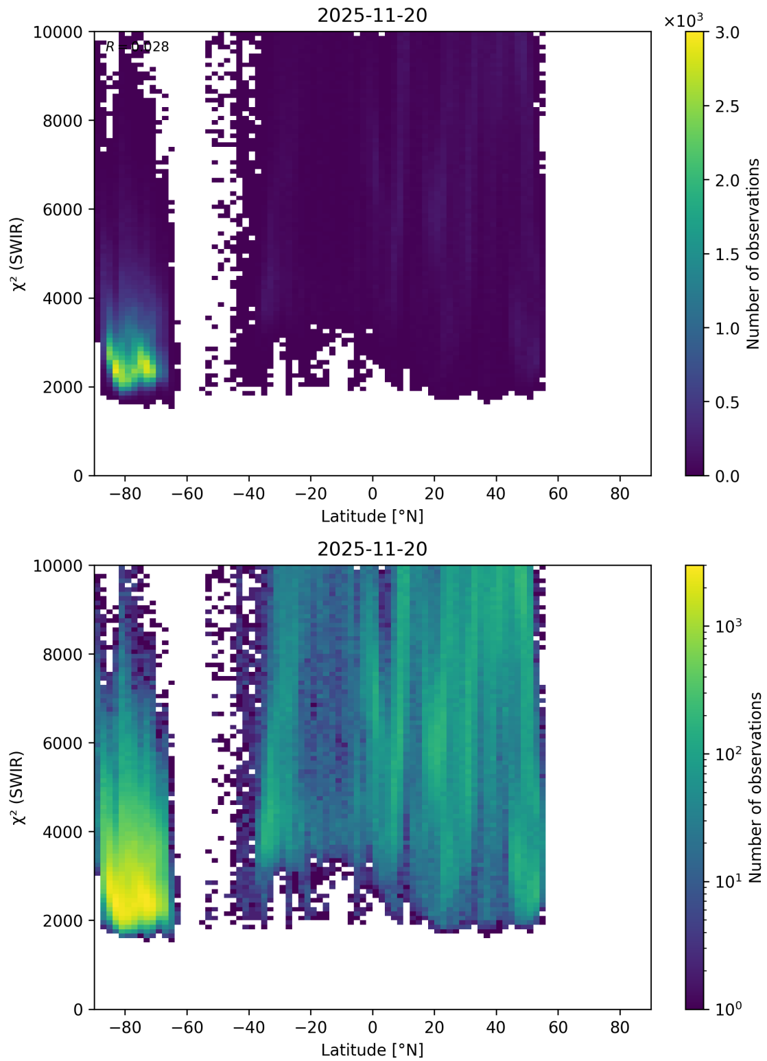
Figure 54: Scatter density plot of “Latitude” against “ \chi^2 (SWIR)” for 2025-11-19 to 2025-11-21.
