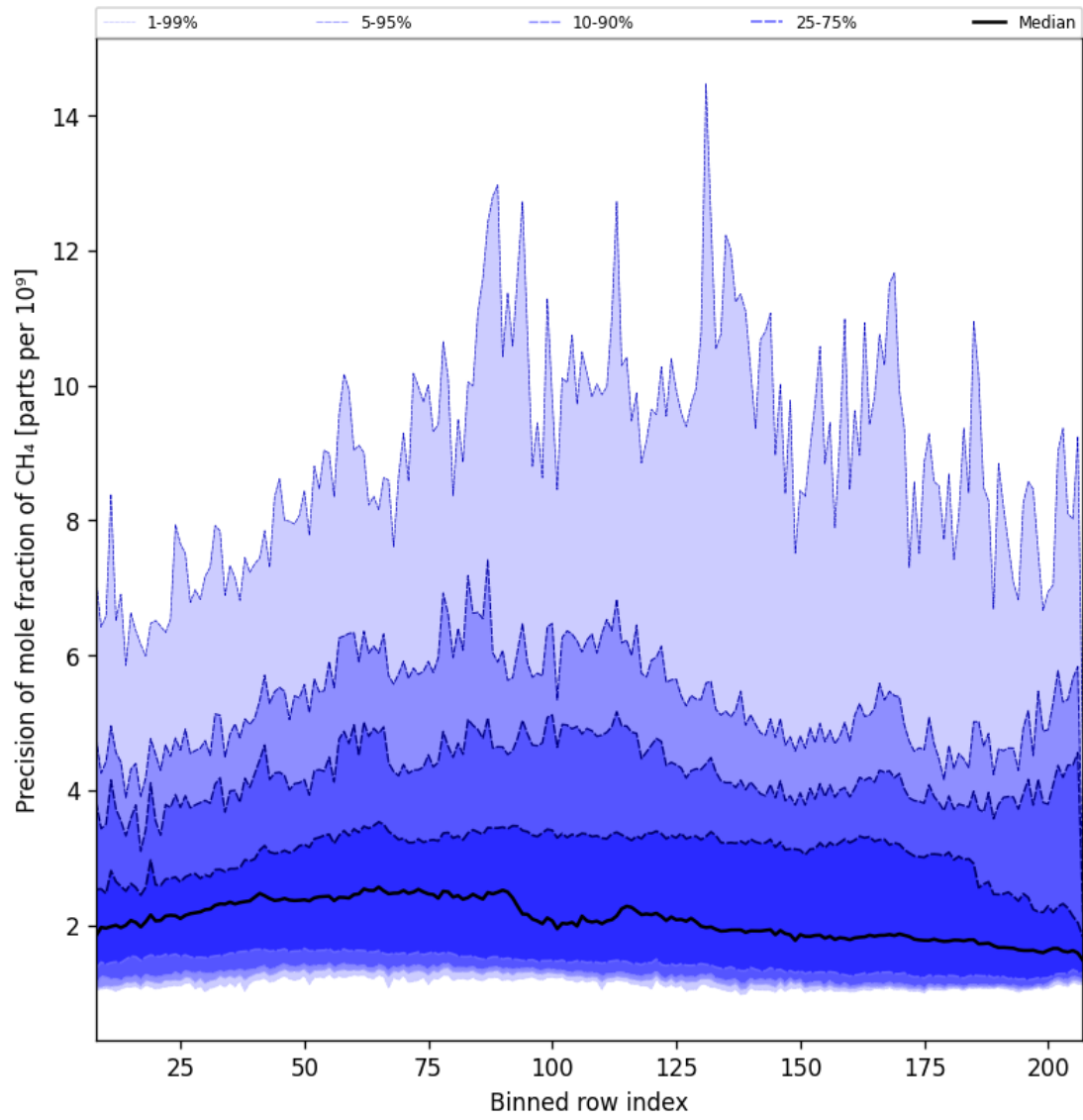
Figure 35: Along track statistics of “Precision of mole fraction of CH 4 ” for 2025-11-19 to 2025-11-21
