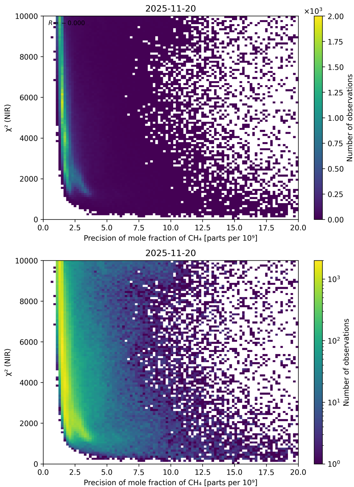
Figure 78: Scatter density plot of “Precision of mole fraction of CH 4 ” against “ \chi^2 (NIR)” for 2025-11-19 to 2025-11-21.
