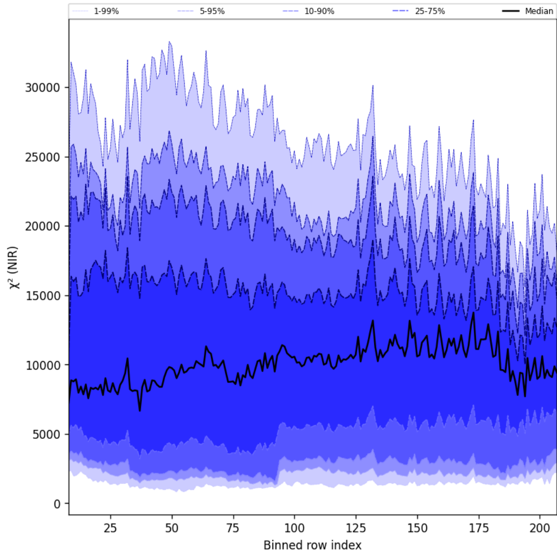
Figure 40: Along track statistics of " \chi^2 (NIR)" for 2025-11-19 to 2025-11-21
