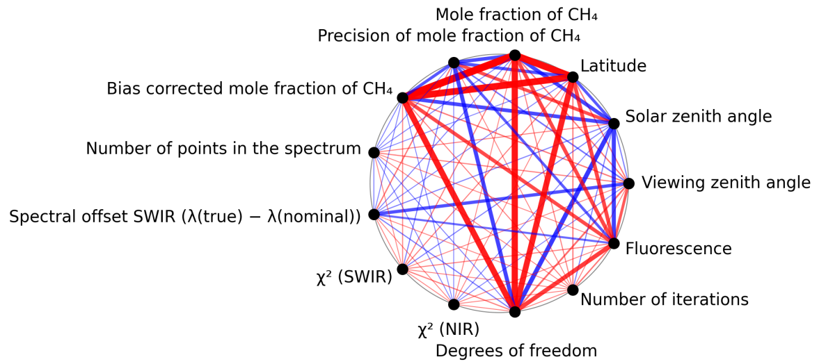
Figure 1: Map of correlation graph for 2025-11-19 to 2025-11-21.
