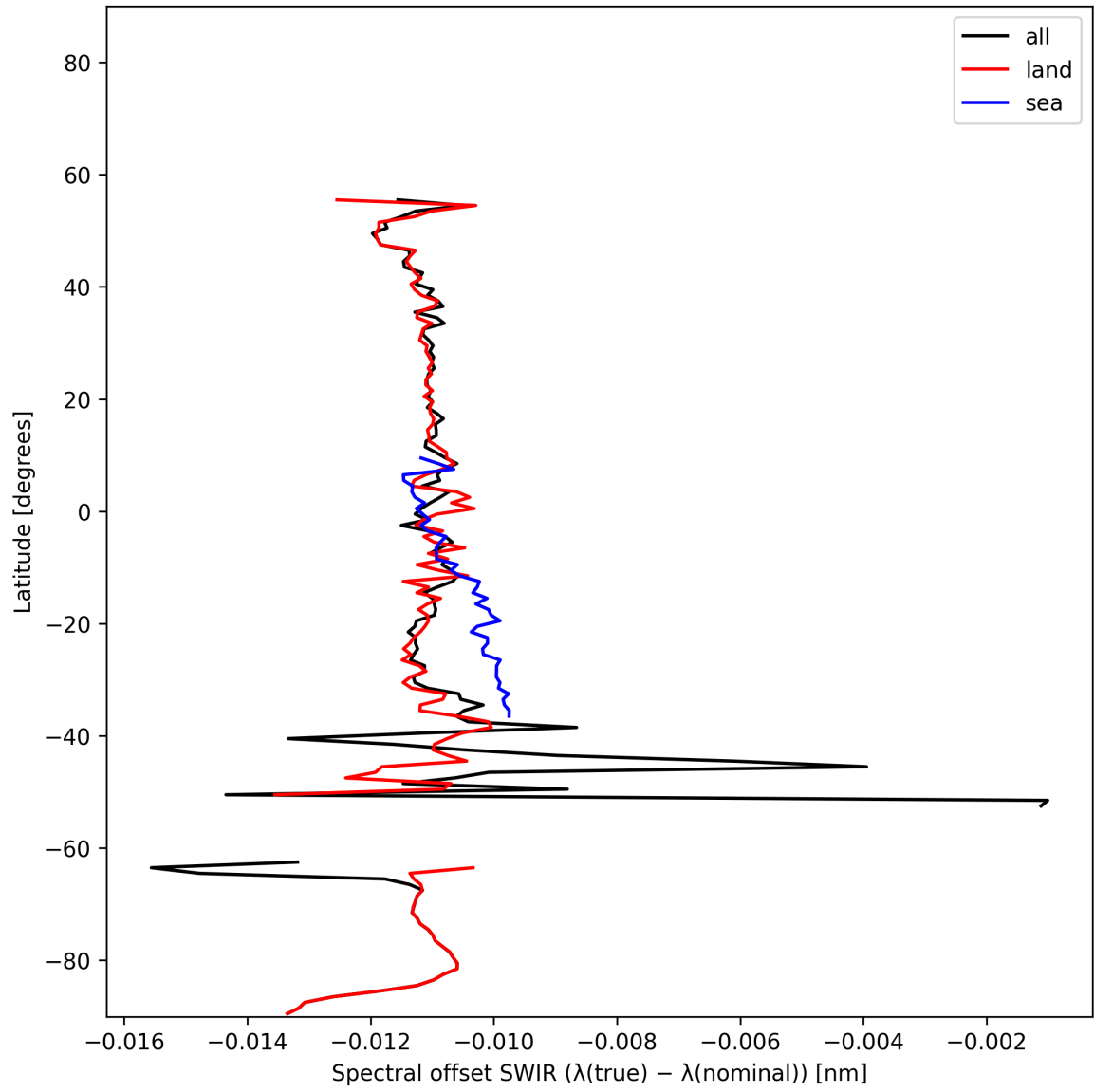
Figure 16: Zonal average of “Spectral offset SWIR ( \lambda_{\text{true}} - \lambda_{\text{nominal}} )” for 2025-11-19 to 2025-11-21.
