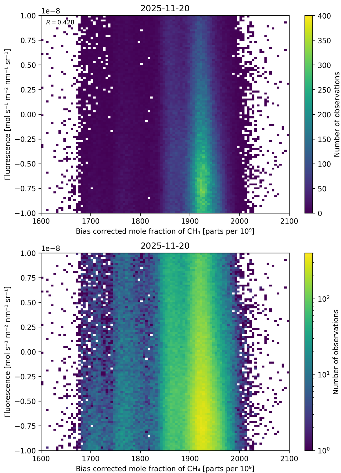
Figure 66: Scatter density plot of “Bias corrected mole fraction of \text{CH}_4 ” against “Fluorescence” for 2025-11-19 to 2025-11-21.
