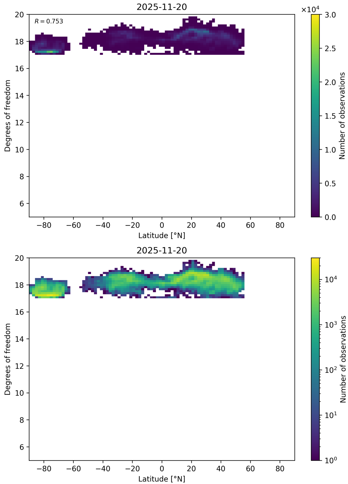
Figure 55: Scatter density plot of “Latitude” against “Degrees of freedom” for 2025-11-19 to 2025-11-21.
