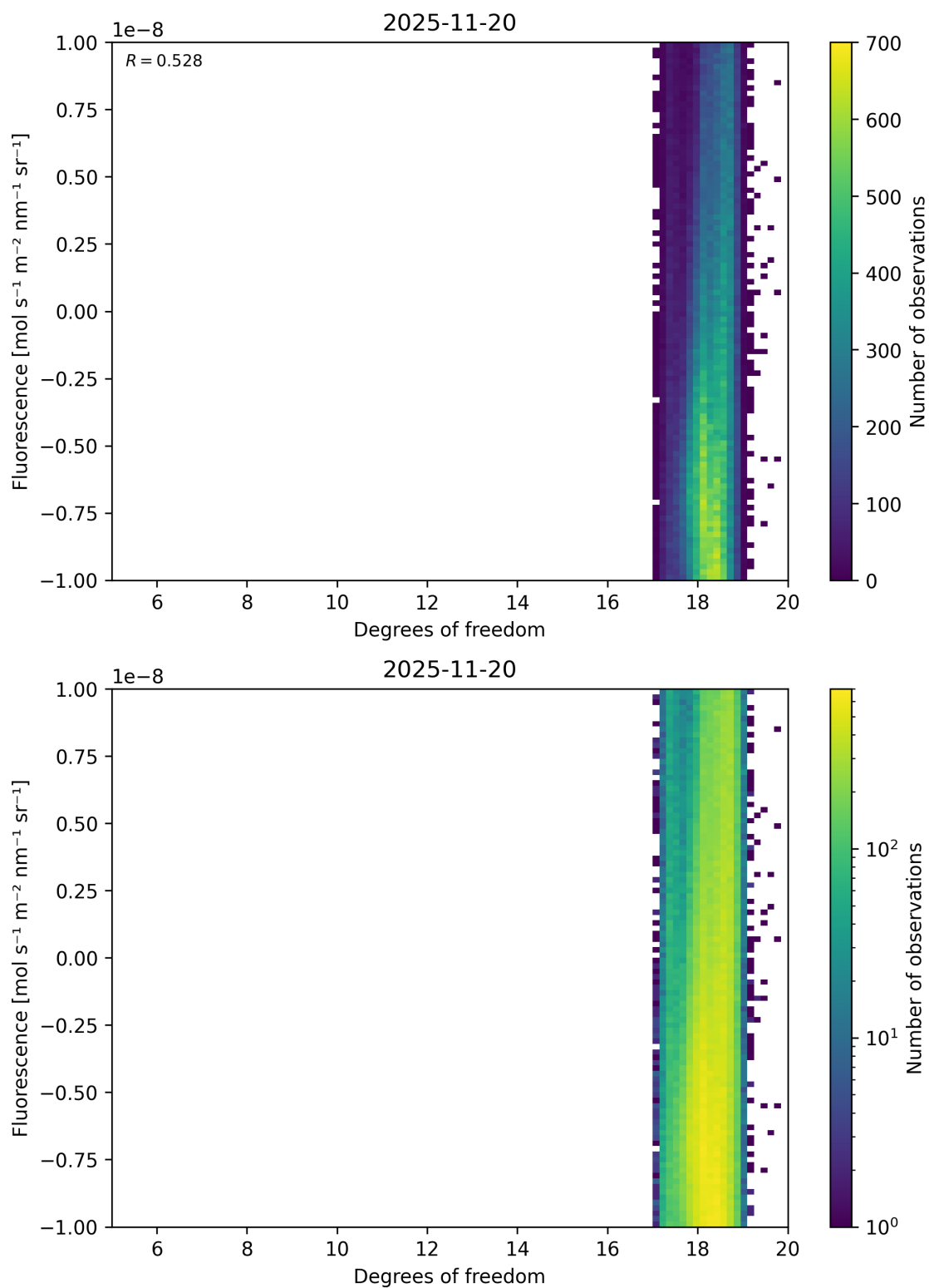
Figure 51: Scatter density plot of “Degrees of freedom” against “Fluorescence” for 2025-11-19 to 2025-11-21.
