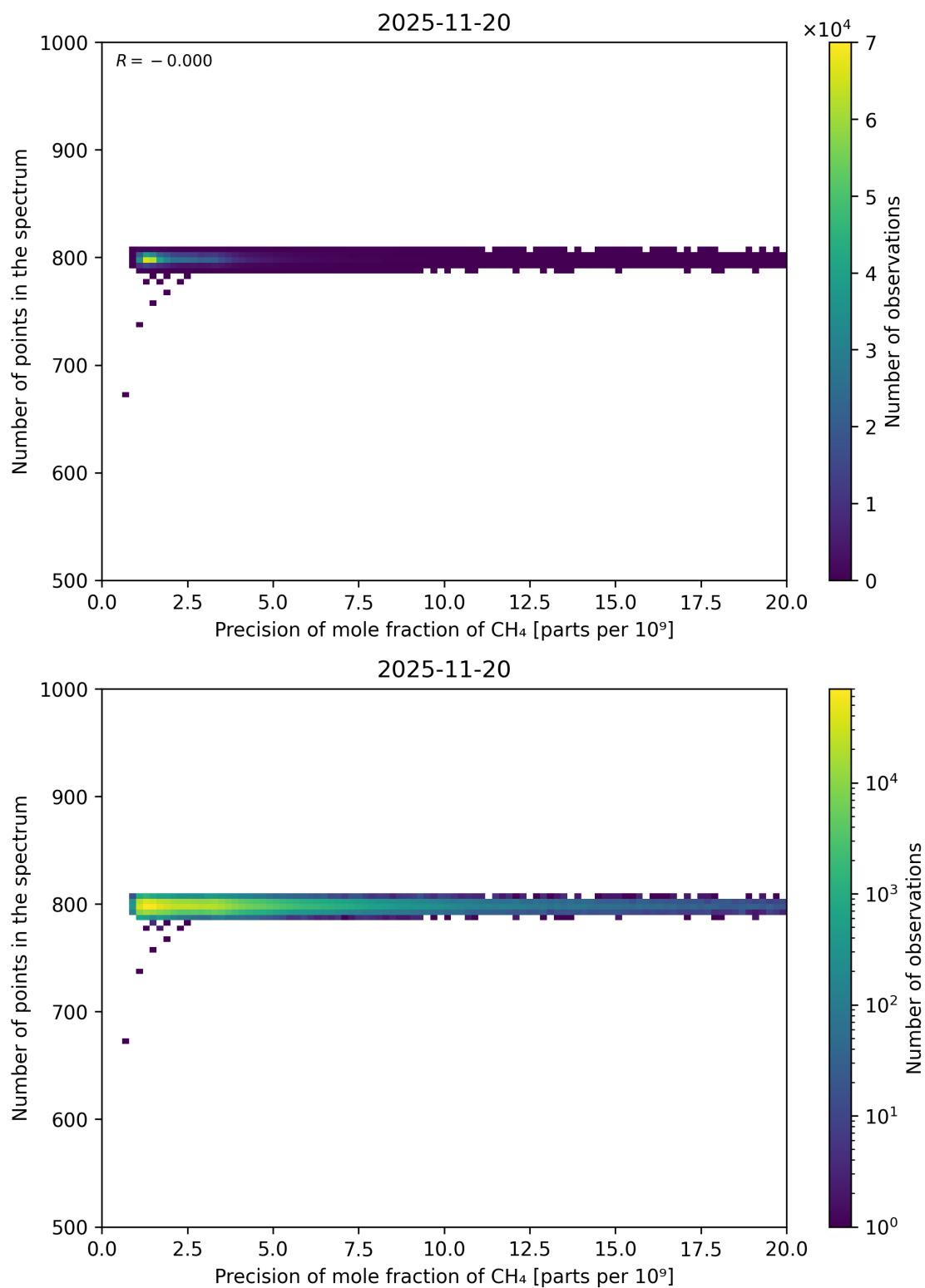
Figure 84: Scatter density plot of “Precision of mole fraction of CH 4 ” against “Number of points in the spectrum” for 2025-11-19 to 2025-11-21.
