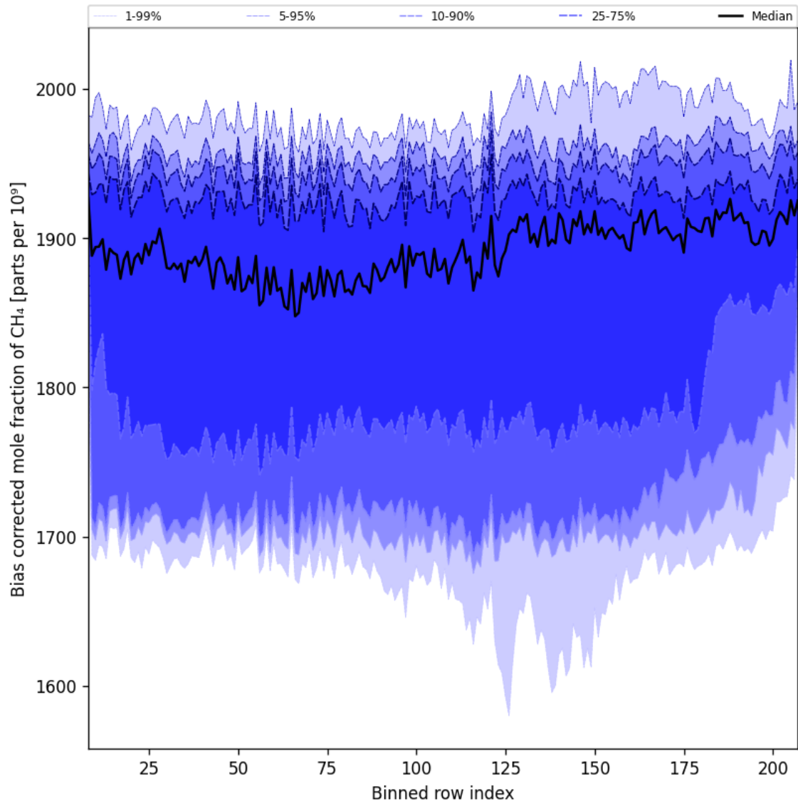
Figure 36: Along track statistics of “Bias corrected mole fraction of CH 4 ” for 2025-11-19 to 2025-11-21
