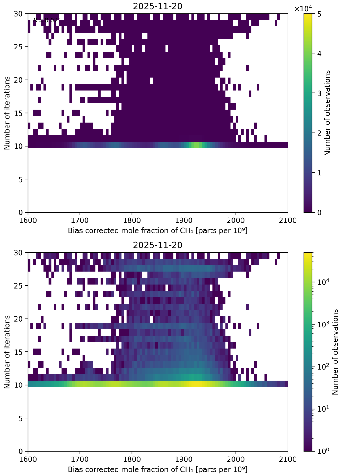
Figure 67: Scatter density plot of “Bias corrected mole fraction of CH 4 ” against “Number of iterations” for 2025-11-19 to 2025-11-21.
