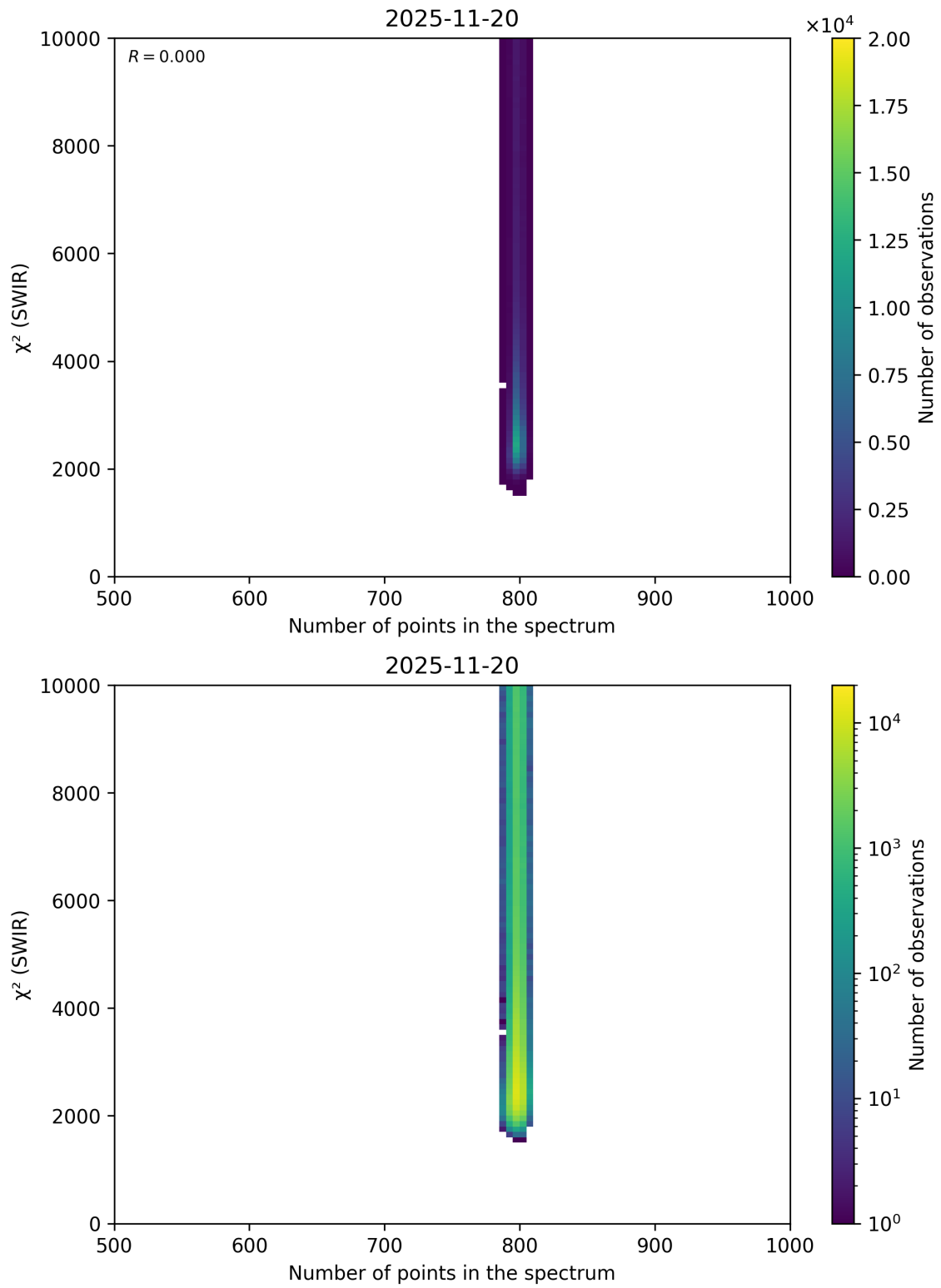
Figure 89: Scatter density plot of “Number of points in the spectrum” against “ \chi^2 (SWIR)” for 2025-11-19 to 2025-11-21.
