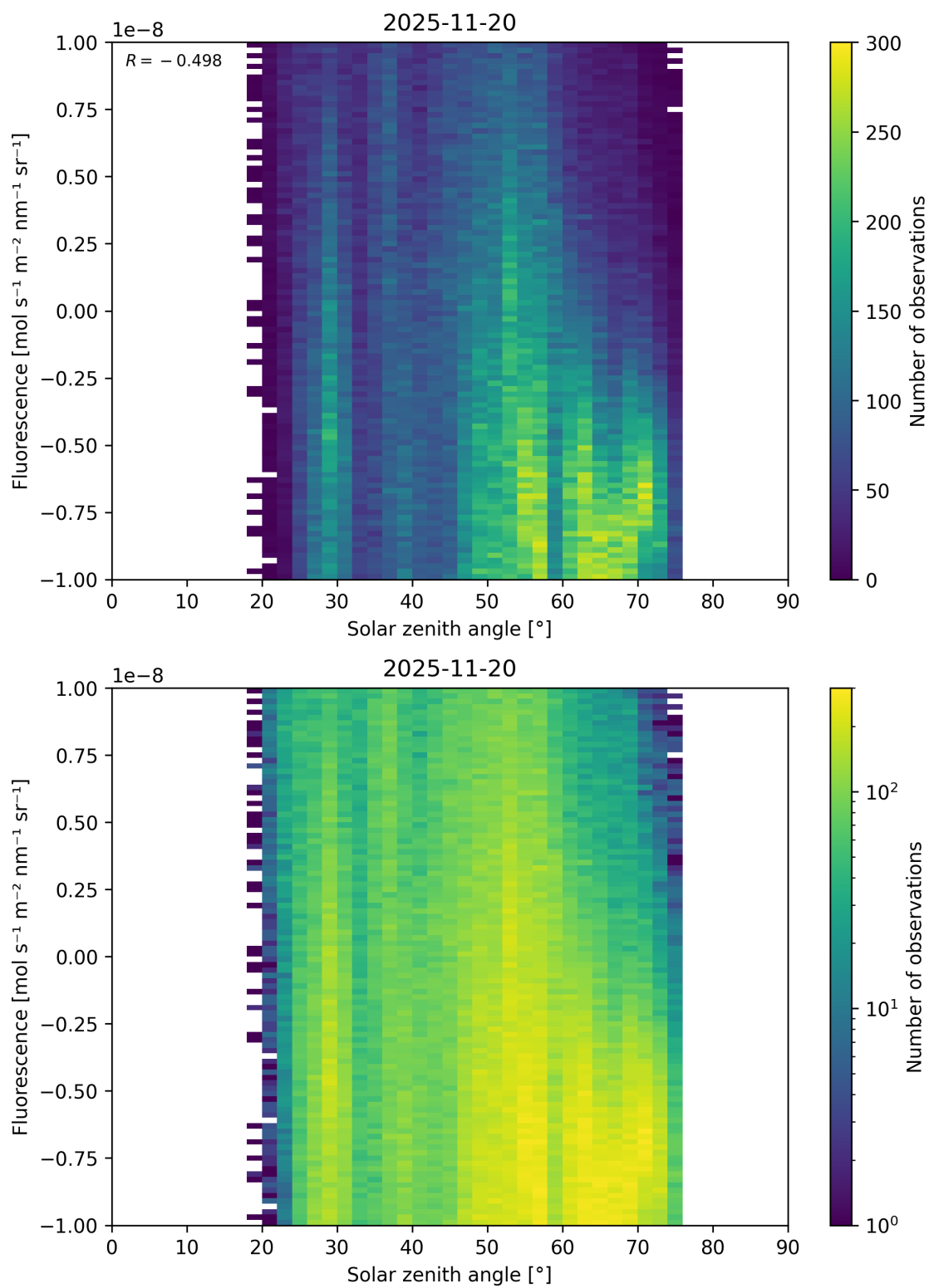
Figure 97: Scatter density plot of “Solar zenith angle” against “Fluorescence” for 2025-11-19 to 2025-11-21.
