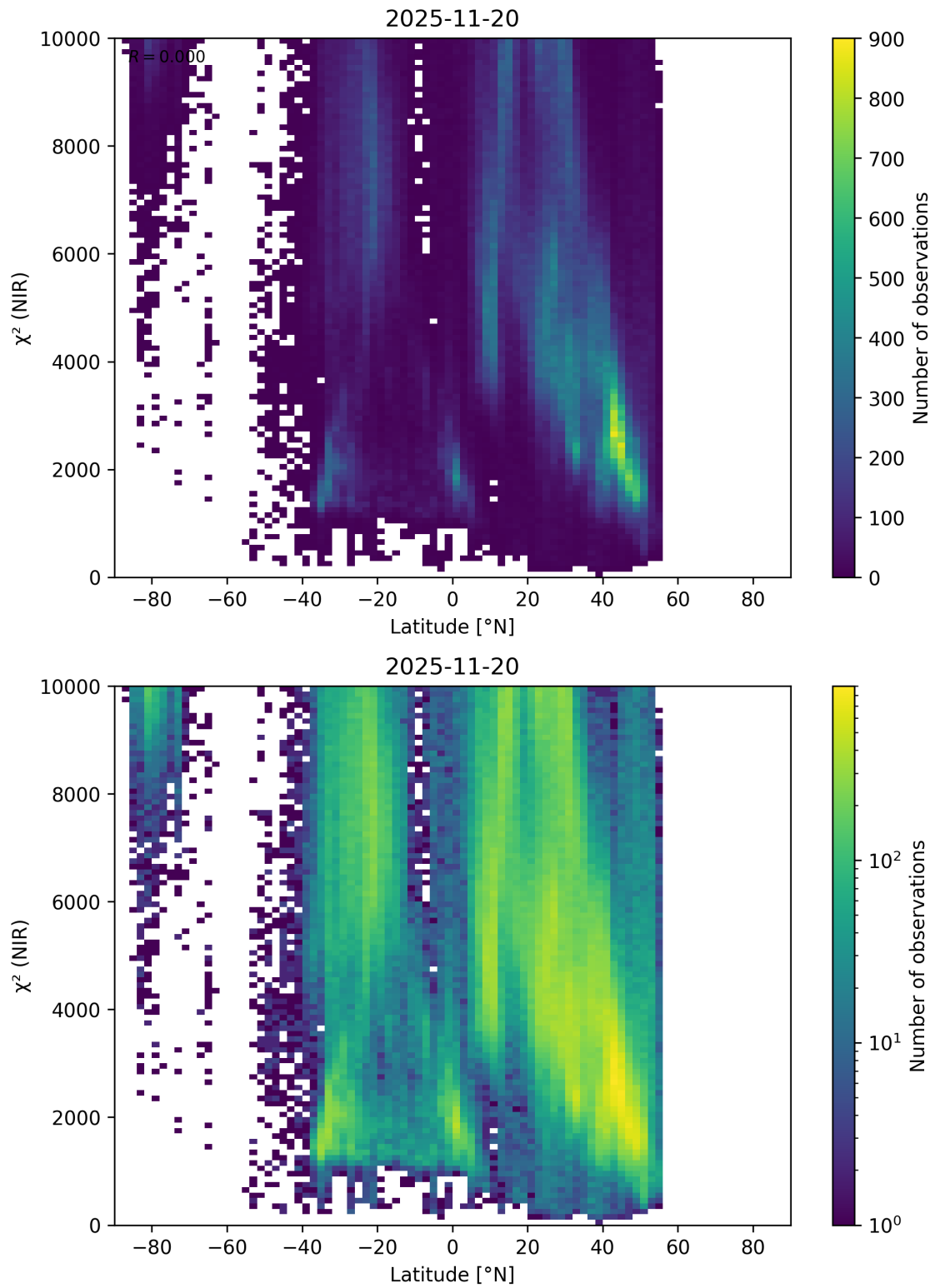
Figure 53: Scatter density plot of “Latitude” against “ \chi^2 (NIR)” for 2025-11-19 to 2025-11-21.
