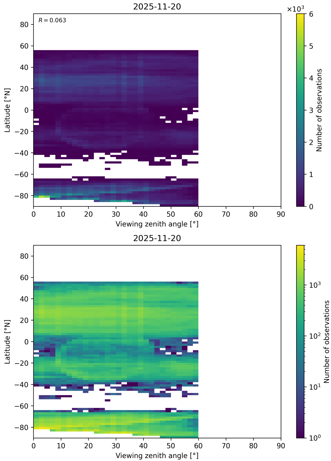
Figure 109: Scatter density plot of “Viewing zenith angle” against “Latitude” for 2025-11-19 to 2025-11-21.
