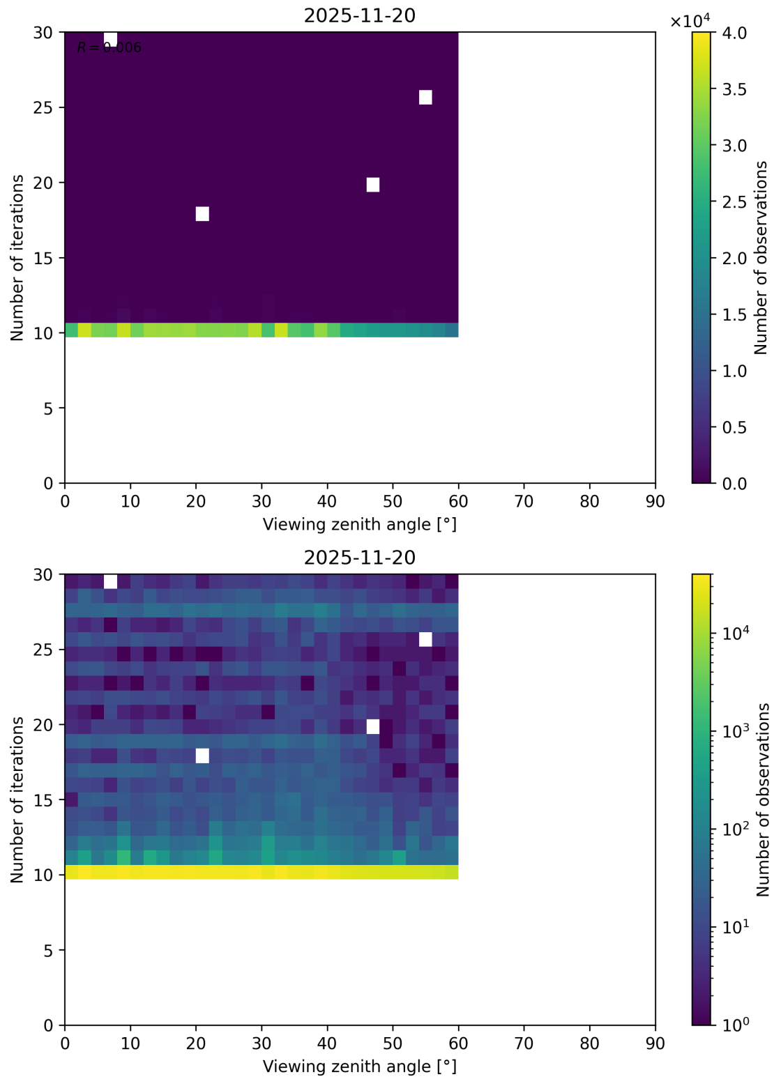
Figure 113: Scatter density plot of “Viewing zenith angle” against “Number of iterations” for 2025-11-19 to 2025-11-21.
