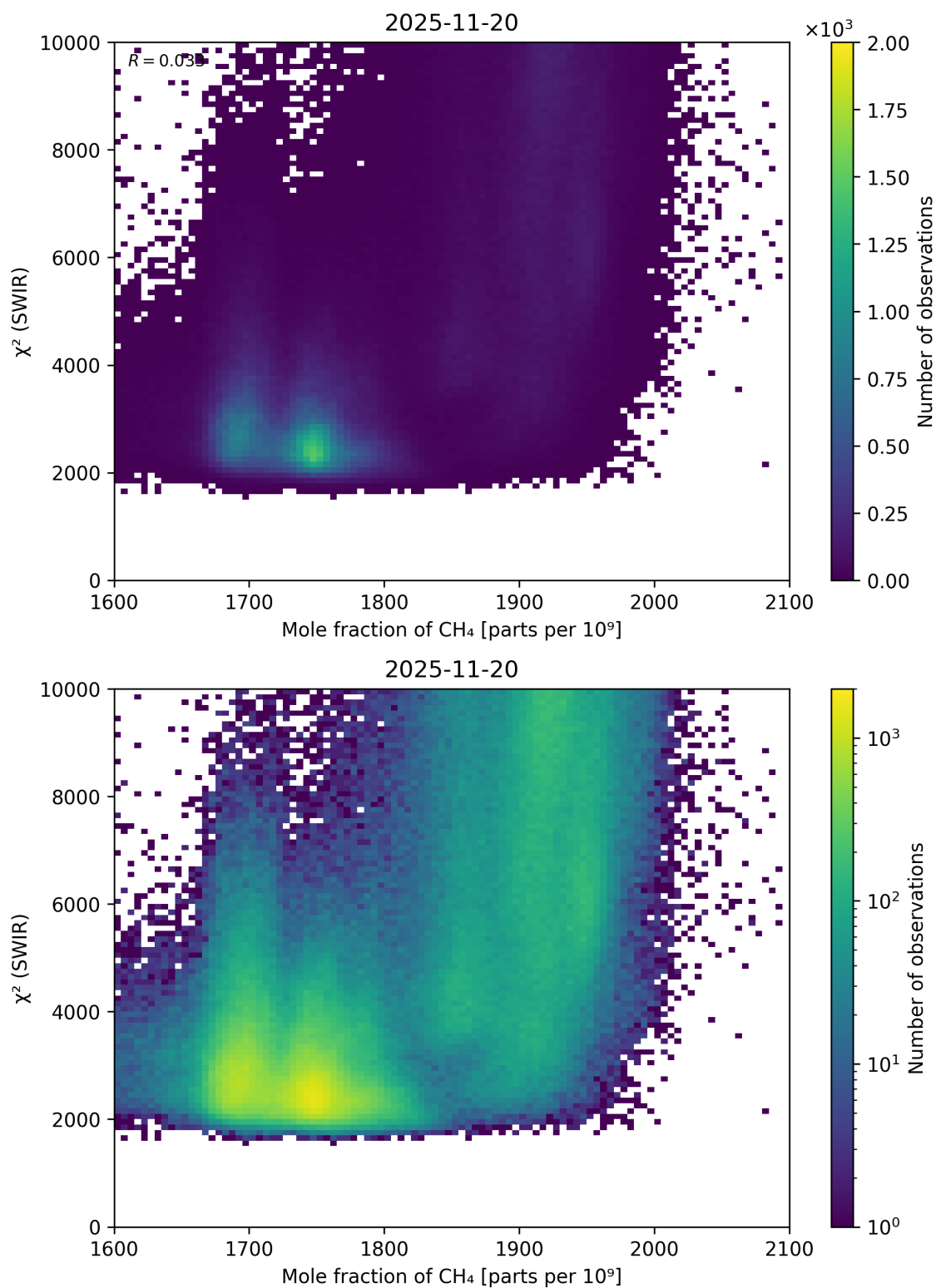
Figure 71: Scatter density plot of “Mole fraction of \text{CH}_4 ” against “ \chi^2 (SWIR)” for 2025-11-19 to 2025-11-21.
