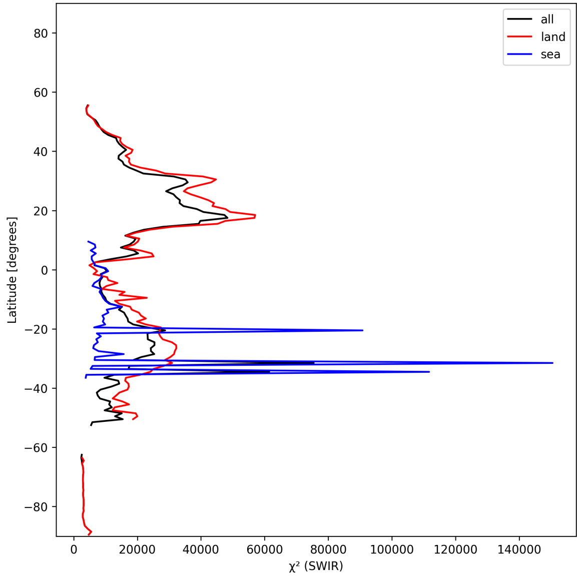
Figure 17: Zonal average of “ \chi^2 (SWIR)” for 2025-11-19 to 2025-11-21.
