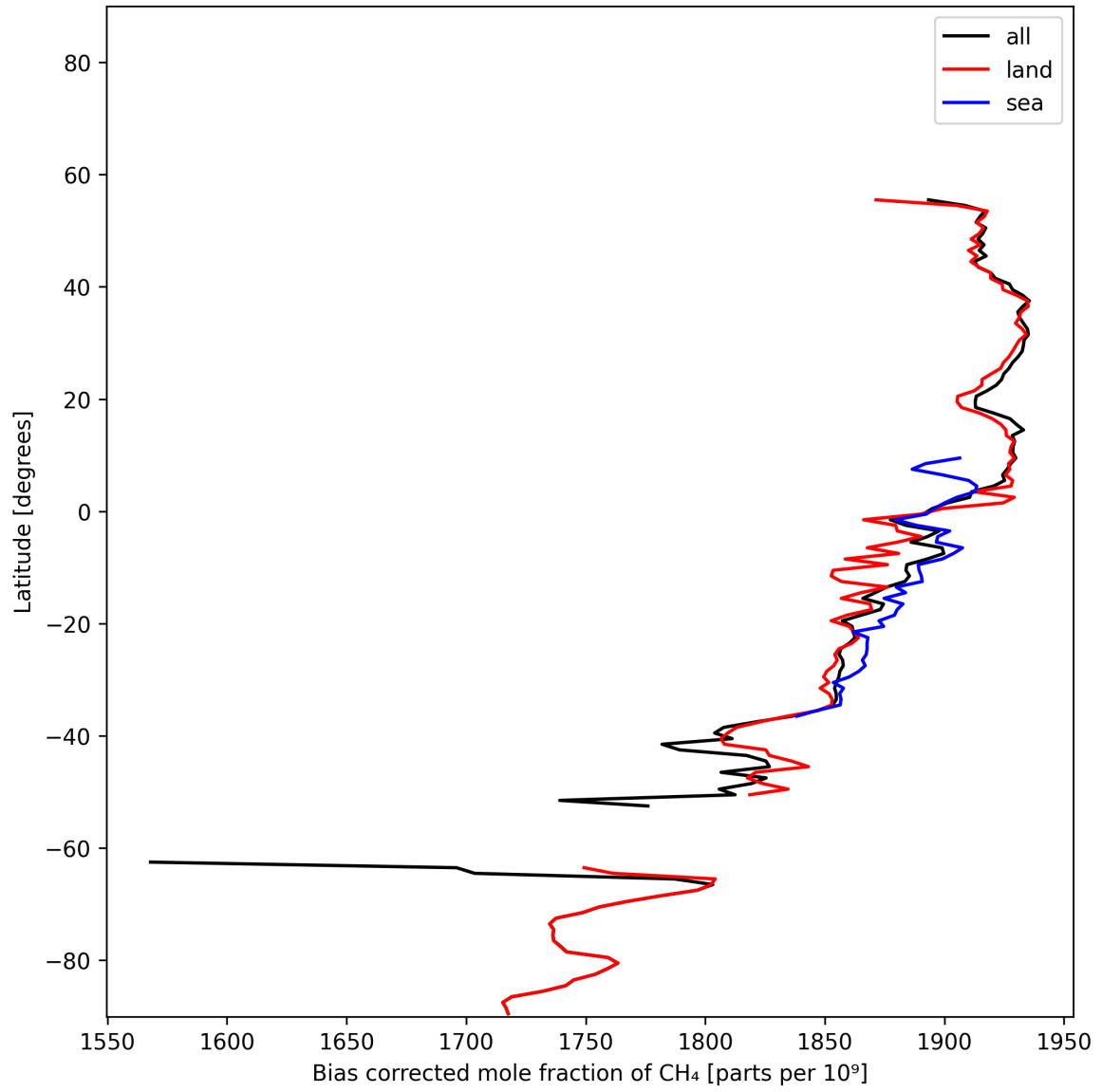
Figure 14: Zonal average of “Bias corrected mole fraction of CH 4 ” for 2025-11-19 to 2025-11-21.
