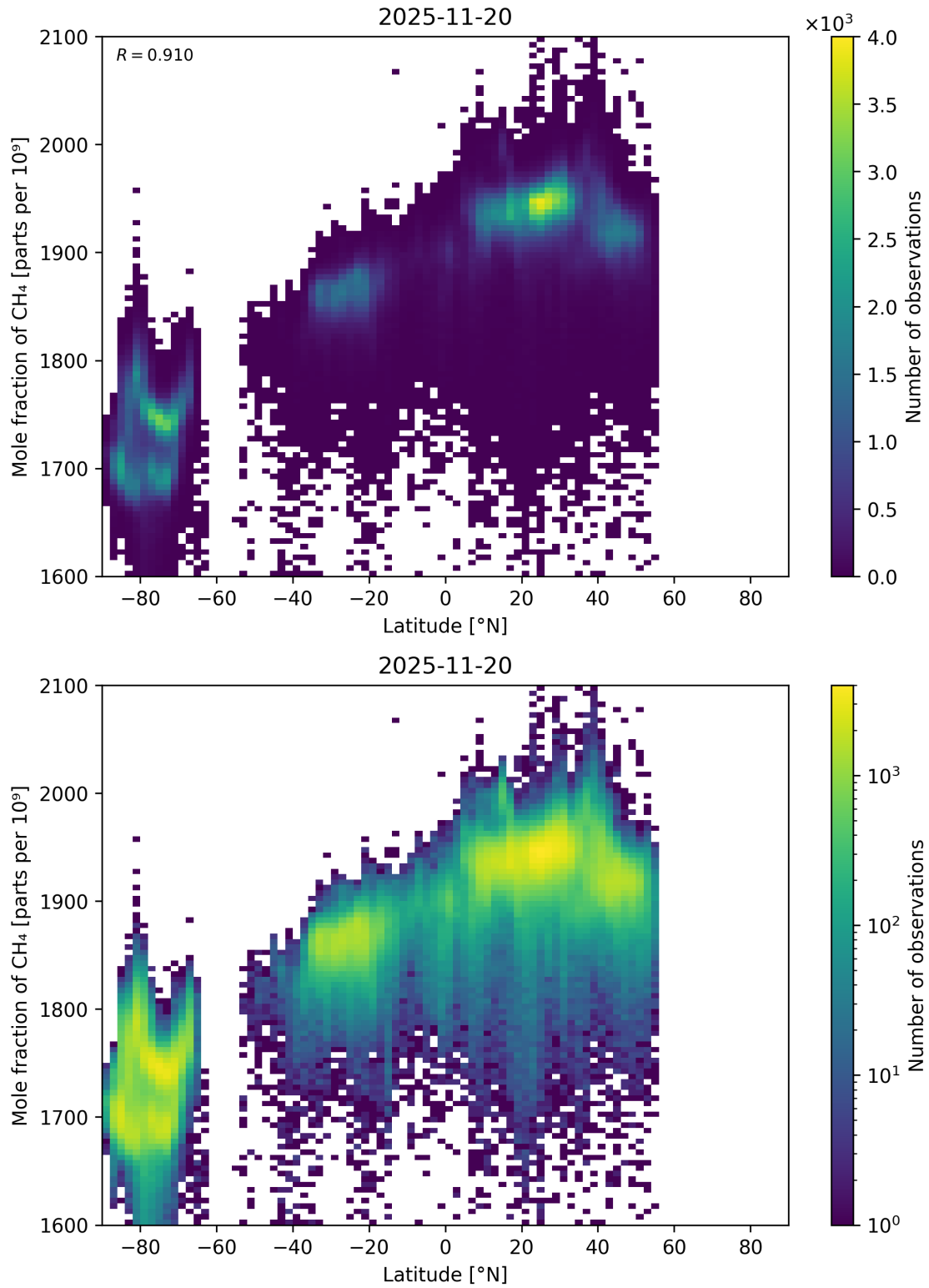
Figure 57: Scatter density plot of “Latitude” against “Mole fraction of CH 4 ” for 2025-11-19 to 2025-11-21.
