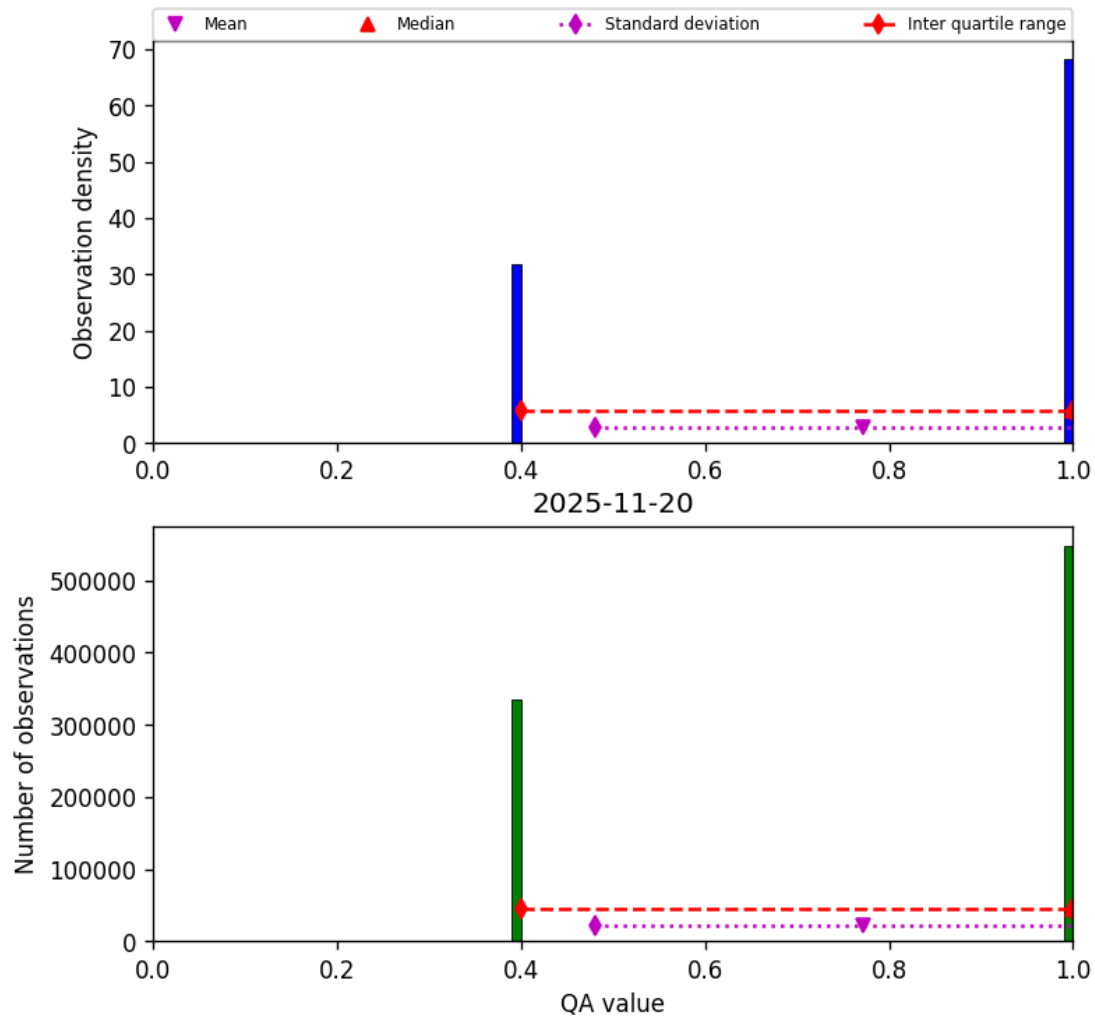
Figure 22: Histogram of “QA value” for 2025-11-19 to 2025-11-21
