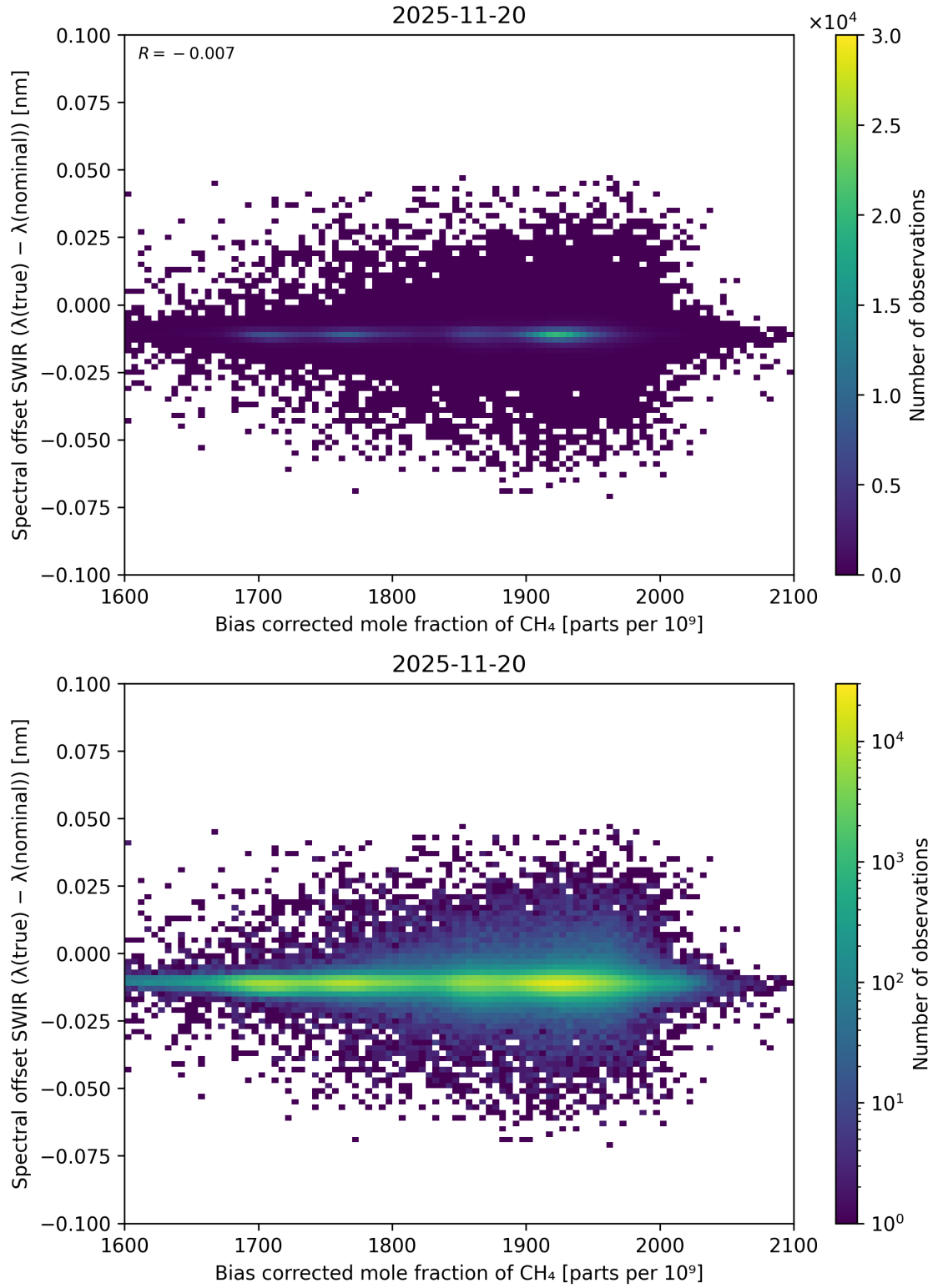
Figure 69: Scatter density plot of “Bias corrected mole fraction of \text{CH}_4 ” against “Spectral offset SWIR ( \lambda_{\text{true}} - \lambda_{\text{nominal}} )” for 2025-11-19 to 2025-11-21.
