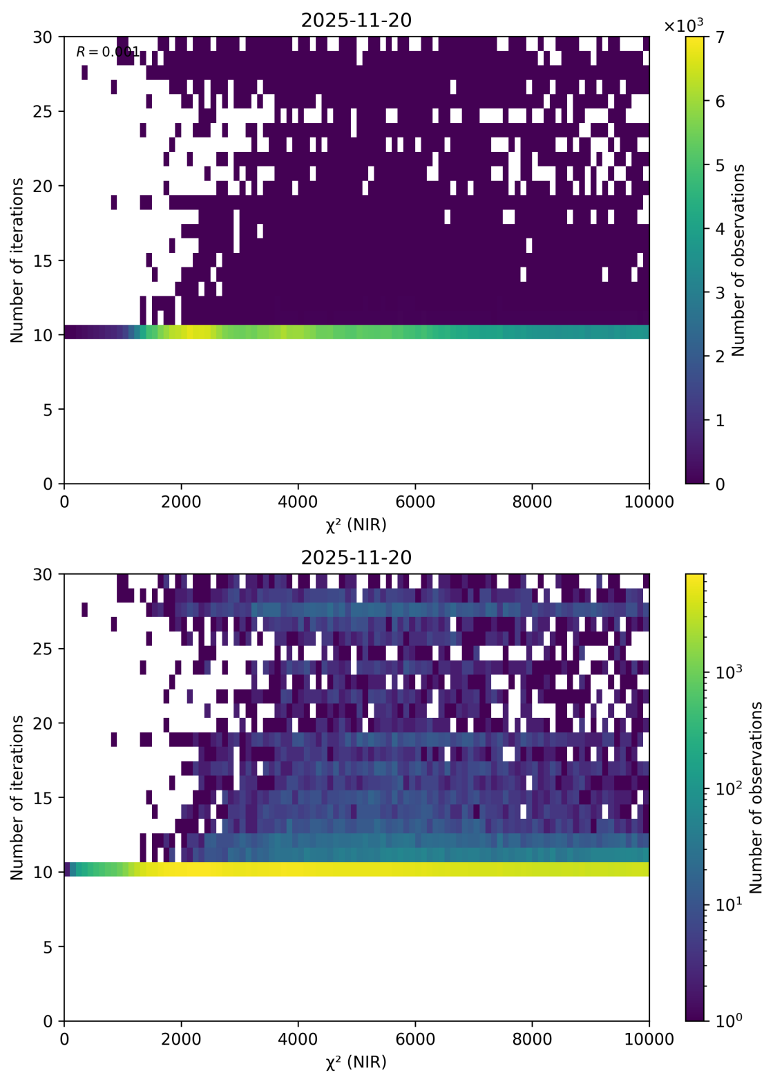
Figure 46: Scatter density plot of “ \chi^2 (NIR)” against “Number of iterations” for 2025-11-19 to 2025-11-21.
