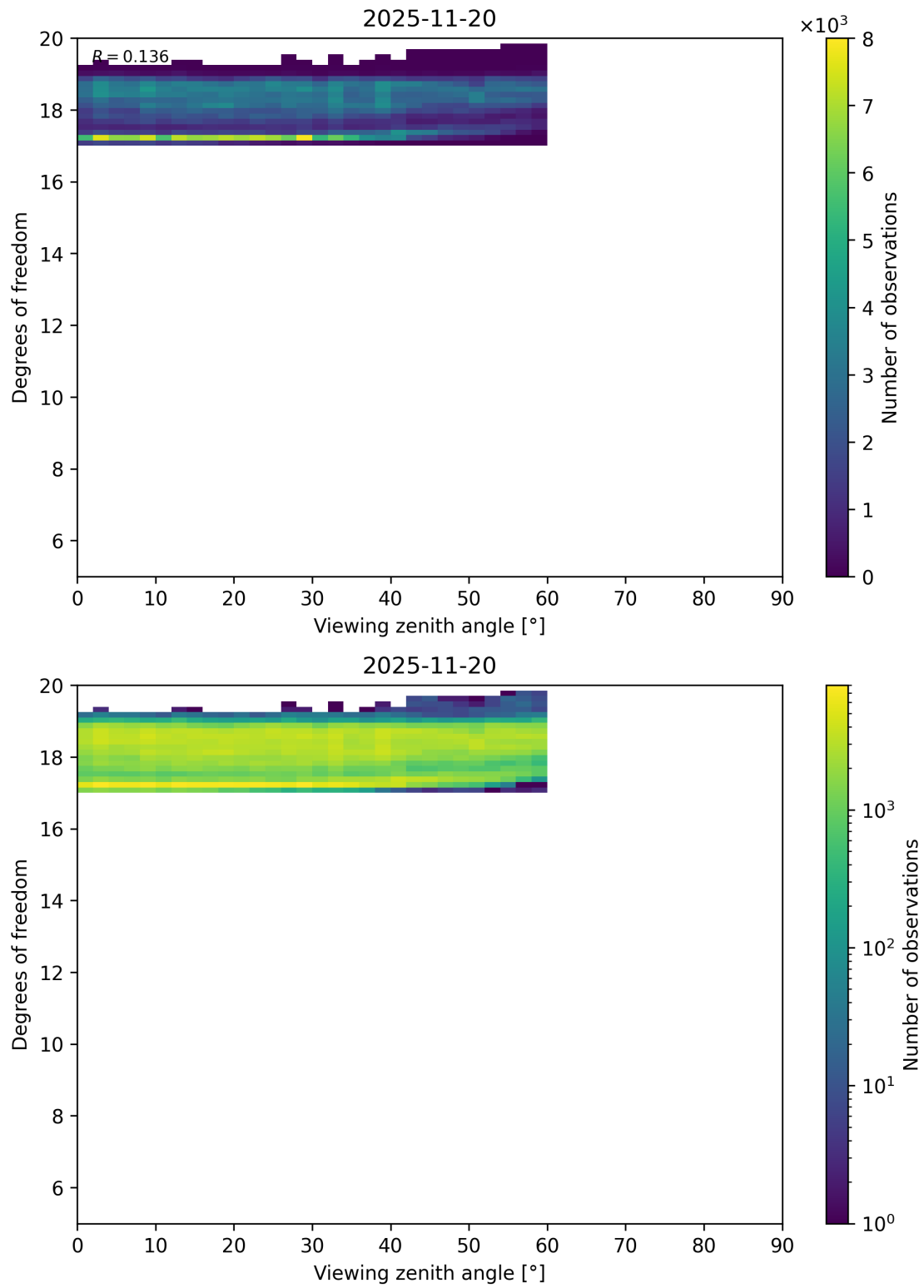
Figure 107: Scatter density plot of “Viewing zenith angle” against “Degrees of freedom” for 2025-11-19 to 2025-11-21.
