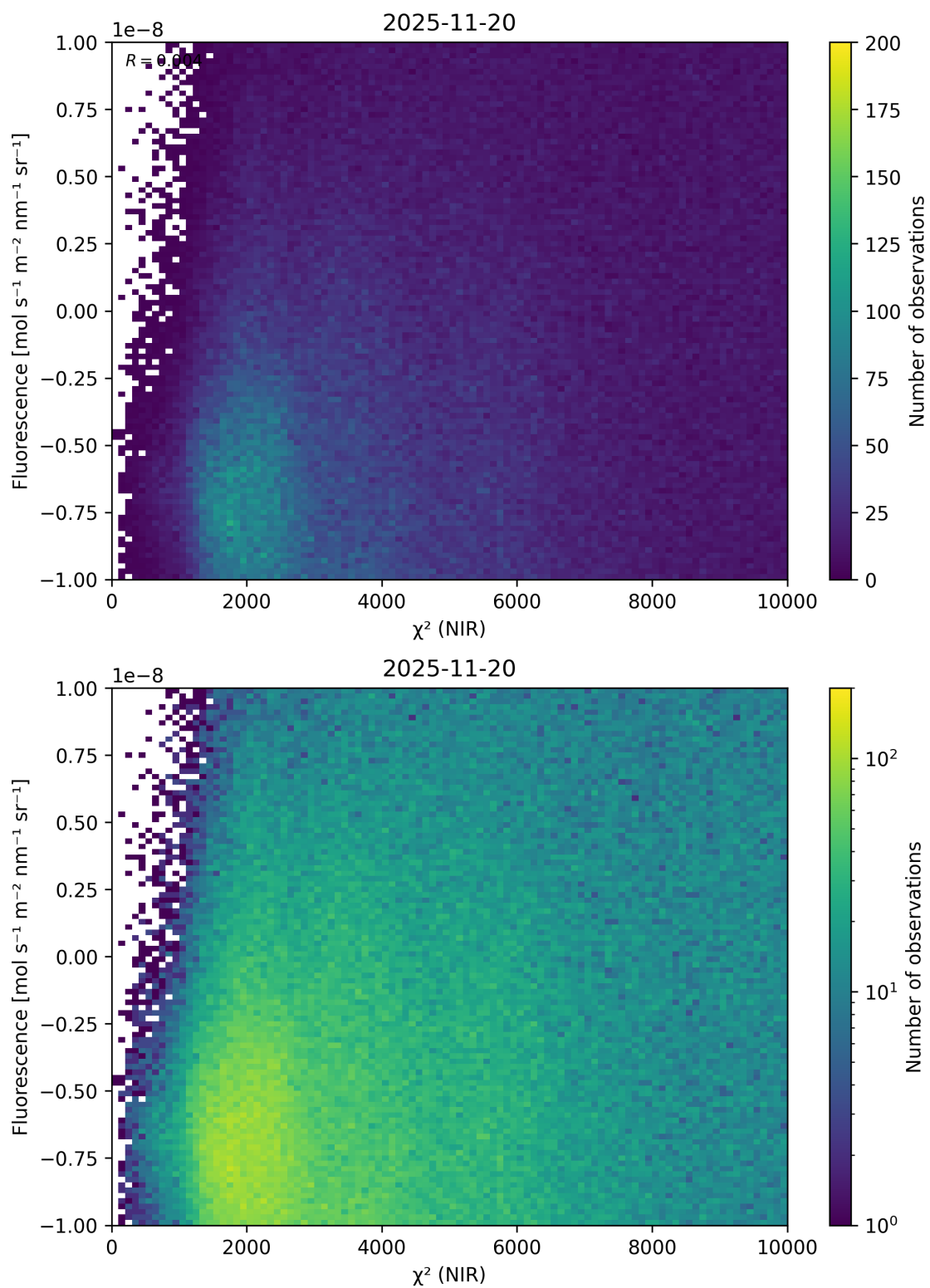
Figure 45: Scatter density plot of “ \chi^2 (NIR)” against “Fluorescence” for 2025-11-19 to 2025-11-21.
