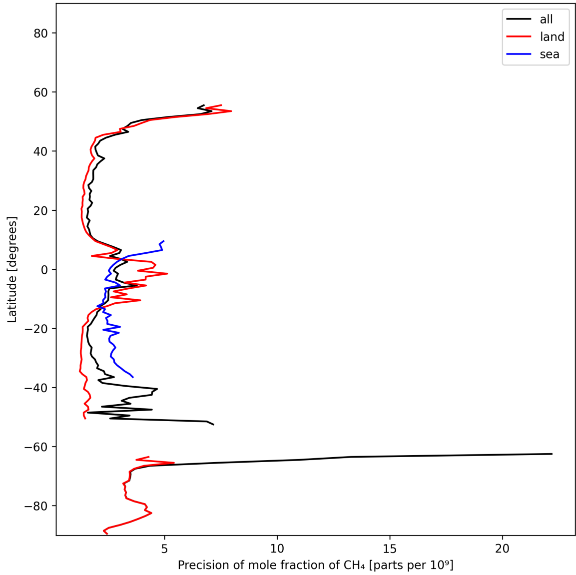
Figure 13: Zonal average of “Precision of mole fraction of CH 4 ” for 2025-11-19 to 2025-11-21.
