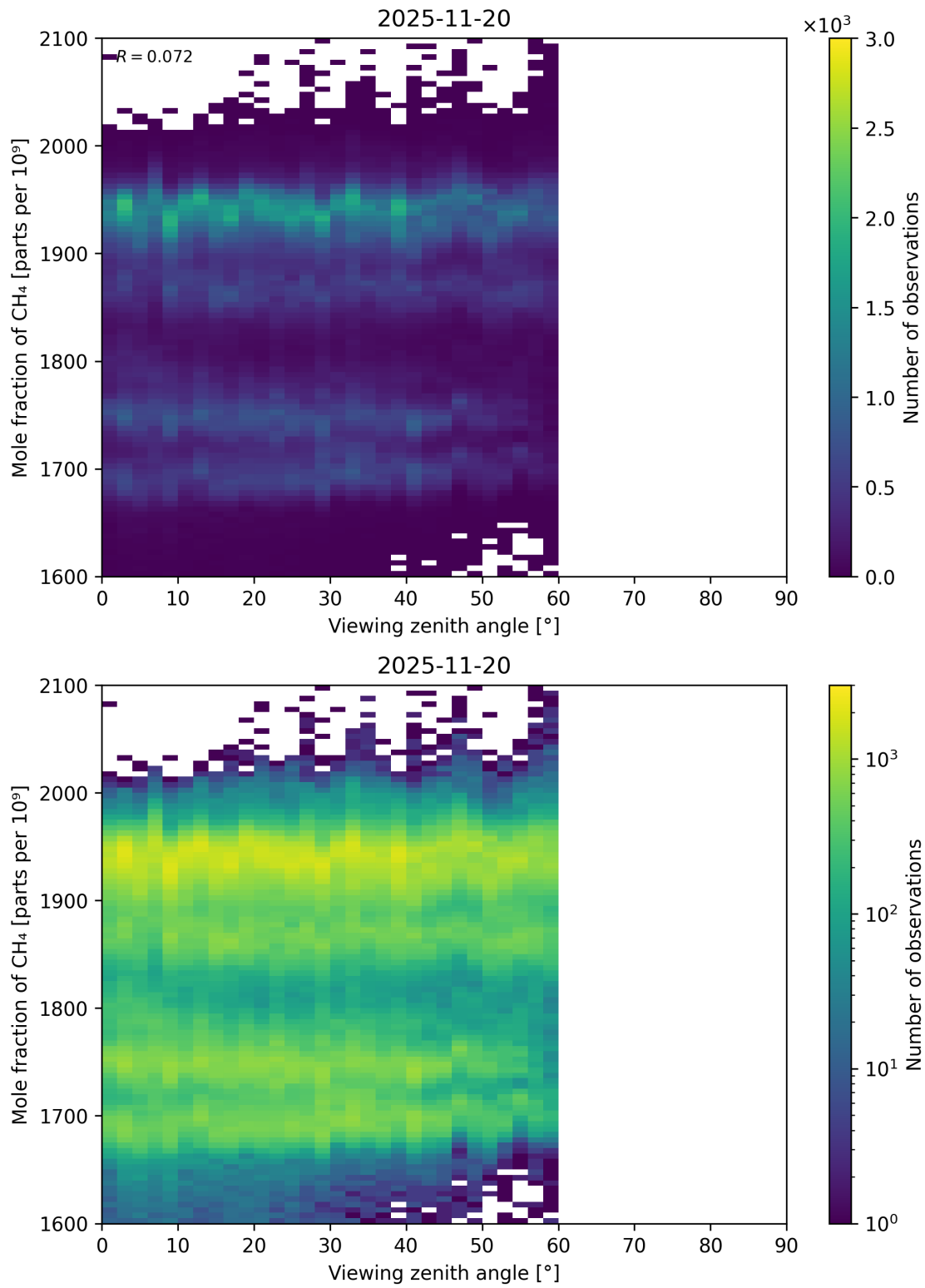
Figure 110: Scatter density plot of “Viewing zenith angle” against “Mole fraction of \text{CH}_4 ” for 2025-11-19 to 2025-11-21.
