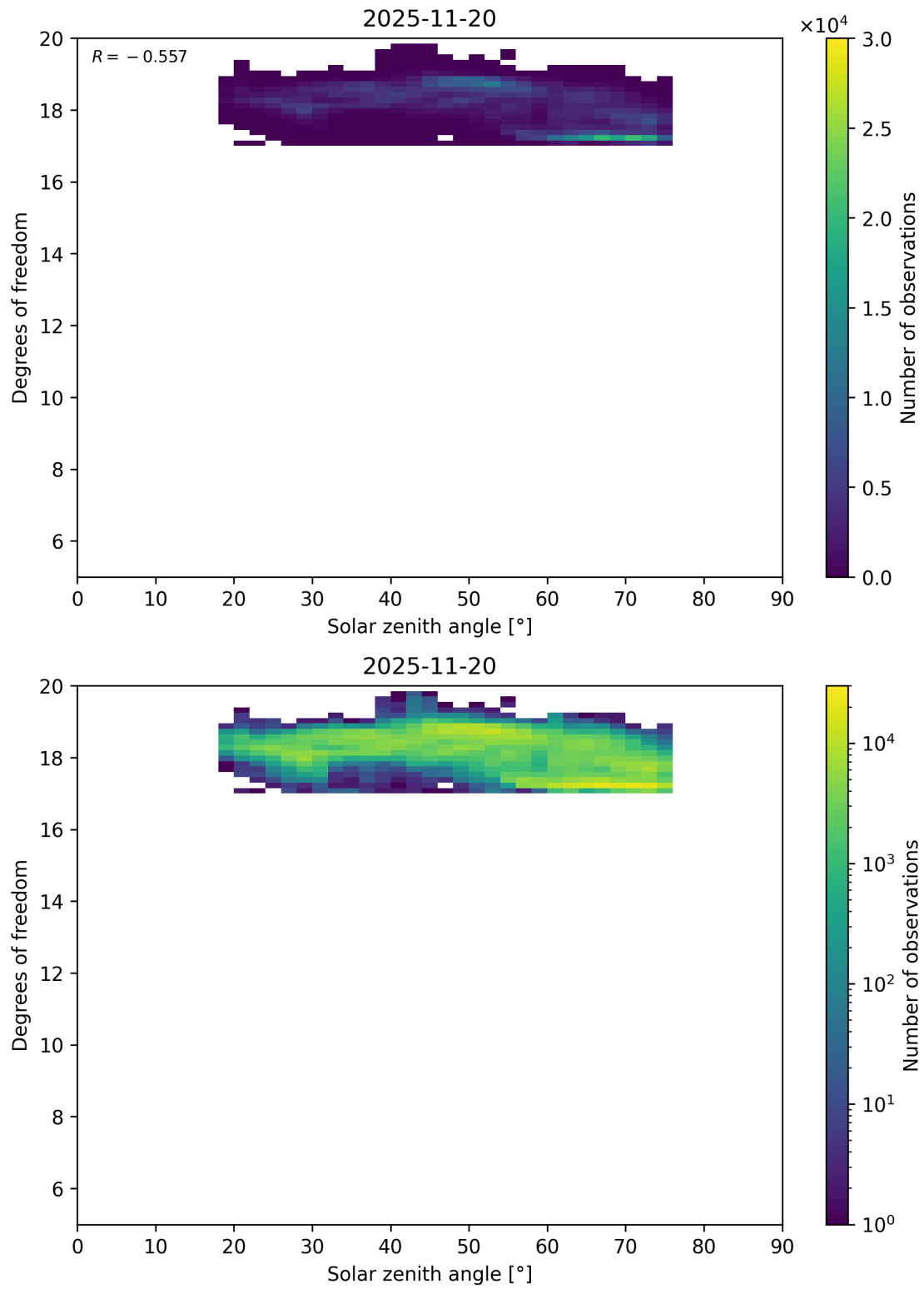
Figure 96: Scatter density plot of “Solar zenith angle” against “Degrees of freedom” for 2025-11-19 to 2025-11-21.
