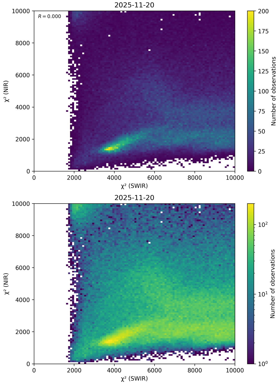
Figure 47: Scatter density plot of “ \chi^2 (SWIR)” against “ \chi^2 (NIR)” for 2025-11-19 to 2025-11-21.
