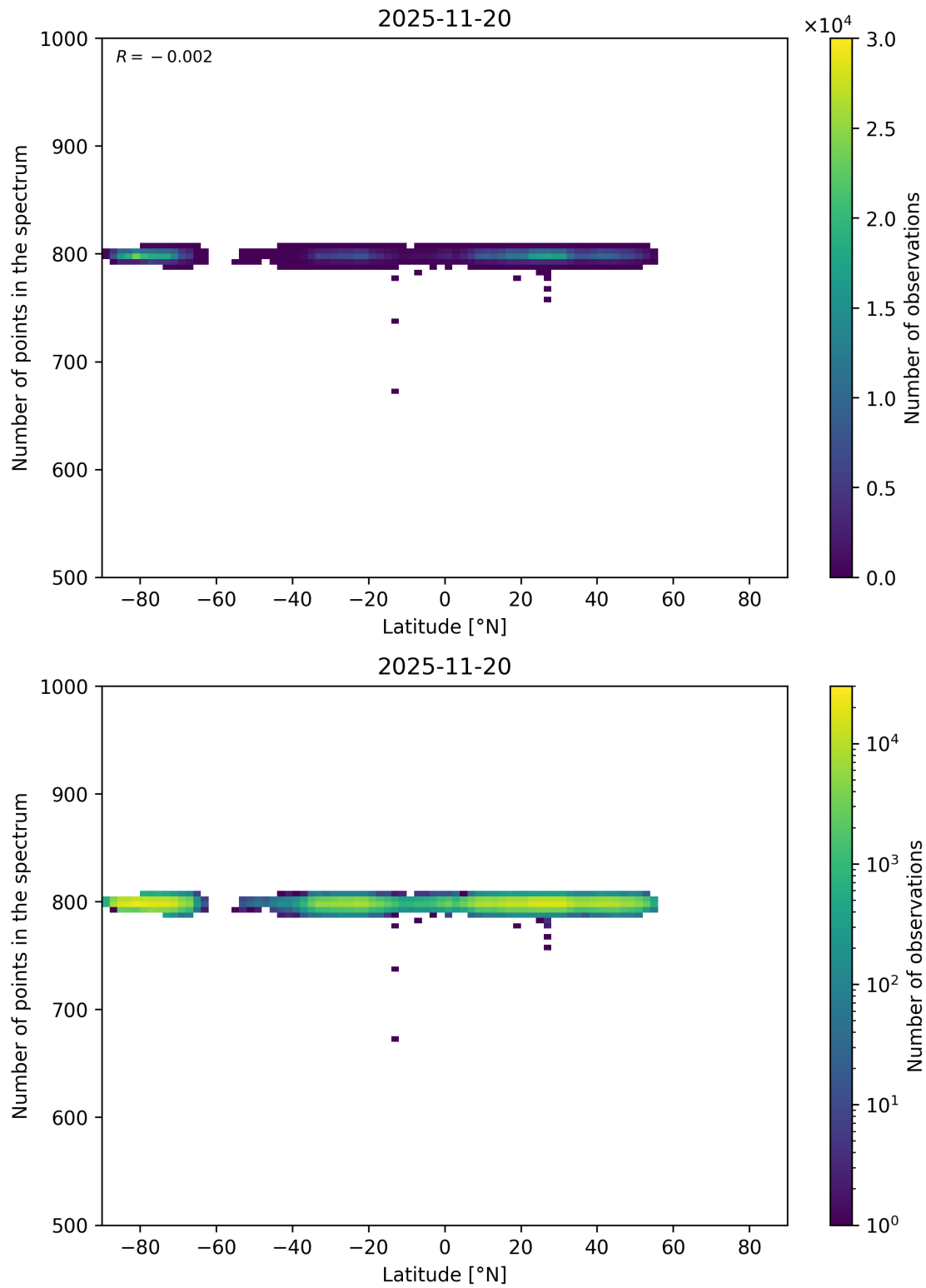
Figure 61: Scatter density plot of “Latitude” against “Number of points in the spectrum” for 2025-11-19 to 2025-11-21.
