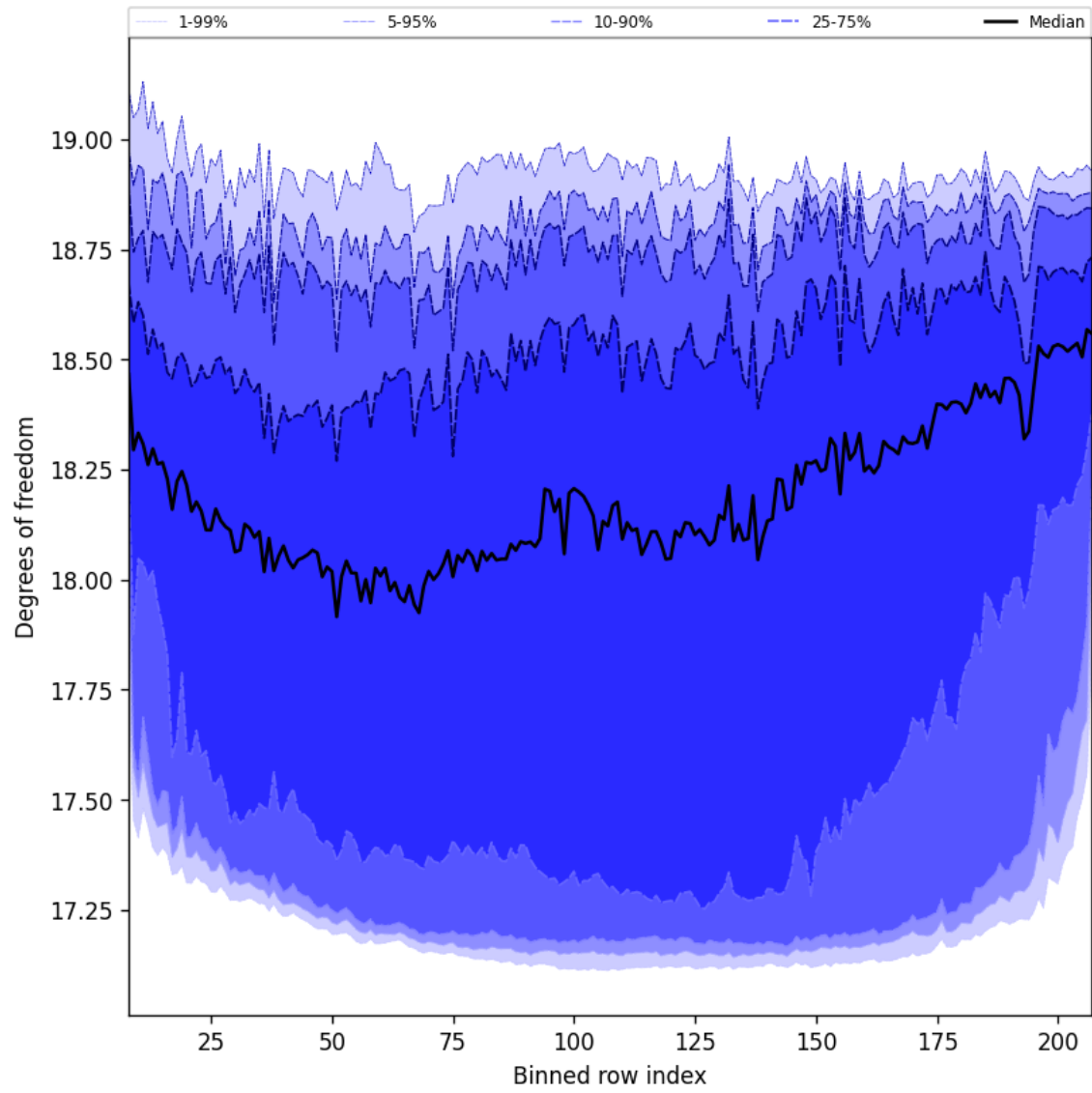
Figure 41: Along track statistics of “Degrees of freedom” for 2025-11-19 to 2025-11-21
