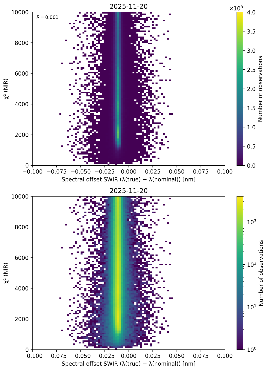
Figure 117: Scatter density plot of “Spectral offset SWIR ( \lambda_{\text{true}} - \lambda_{\text{nominal}} )” against “ \chi^2 (NIR)” for 2025-11-19 to 2025-11-21.
