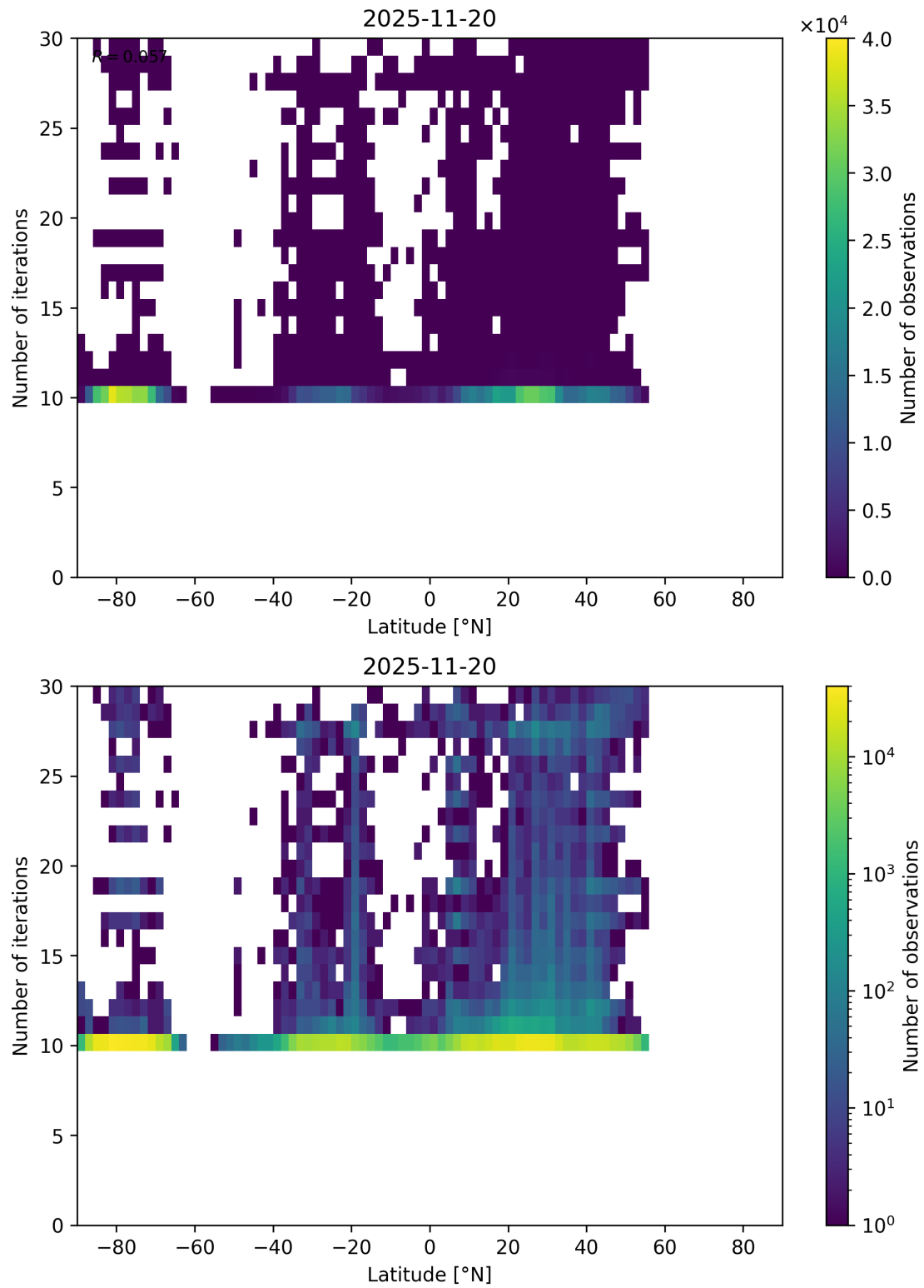
Figure 60: Scatter density plot of “Latitude” against “Number of iterations” for 2025-11-19 to 2025-11-21.
