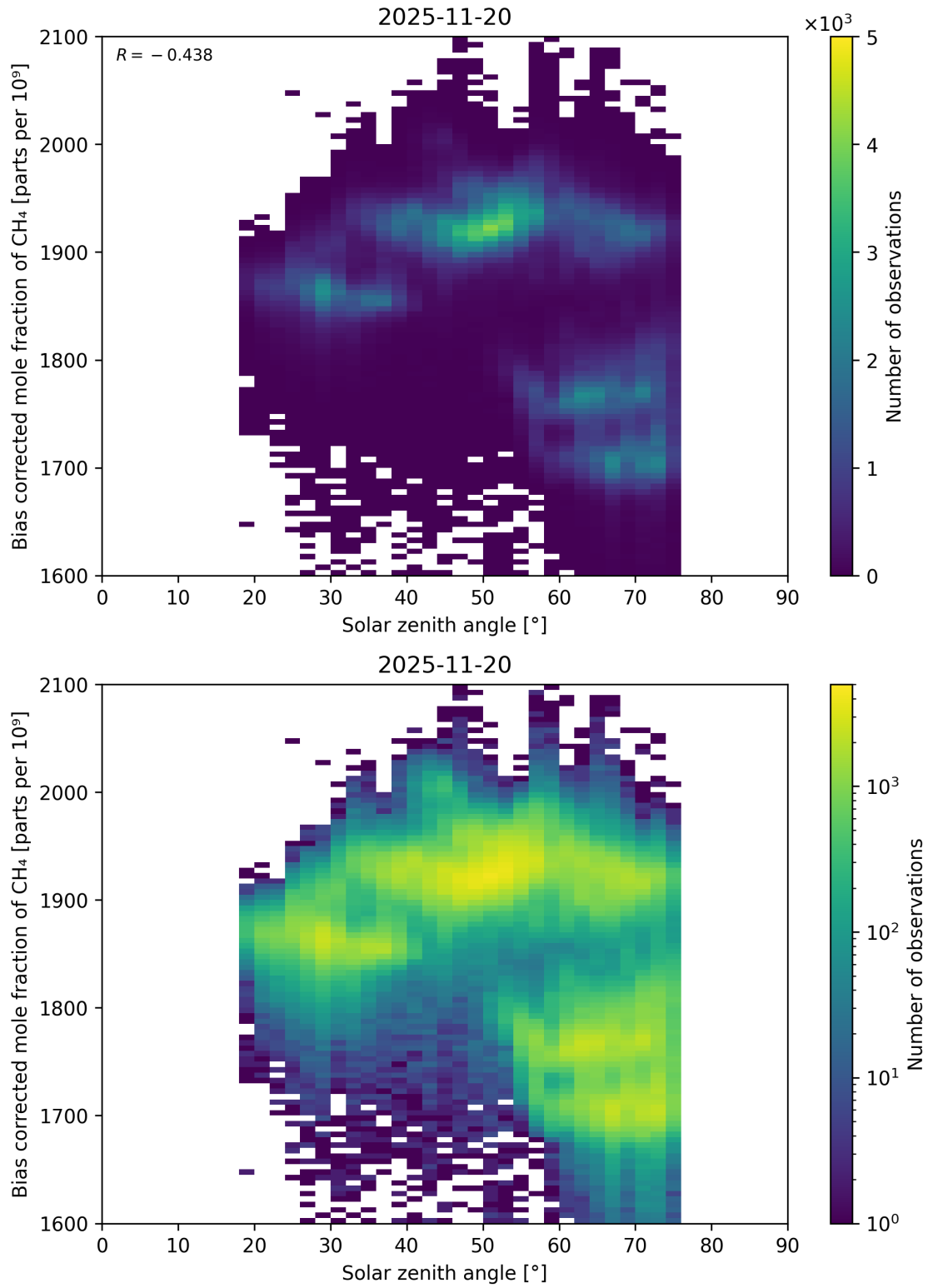
Figure 100: Scatter density plot of “Solar zenith angle” against “Bias corrected mole fraction of CH 4 ” for 2025-11-19 to 2025-11-21.
