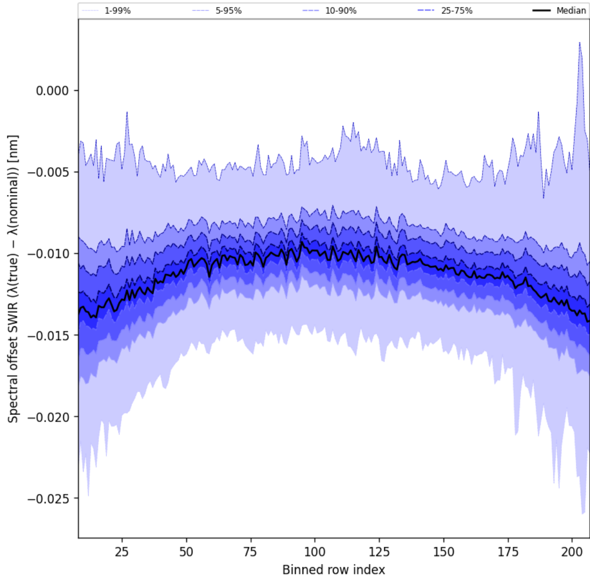
Figure 38: Along track statistics of “Spectral offset SWIR ( \lambda_{\text{true}} - \lambda_{\text{nominal}} )” for 2025-11-19 to 2025-11-21
