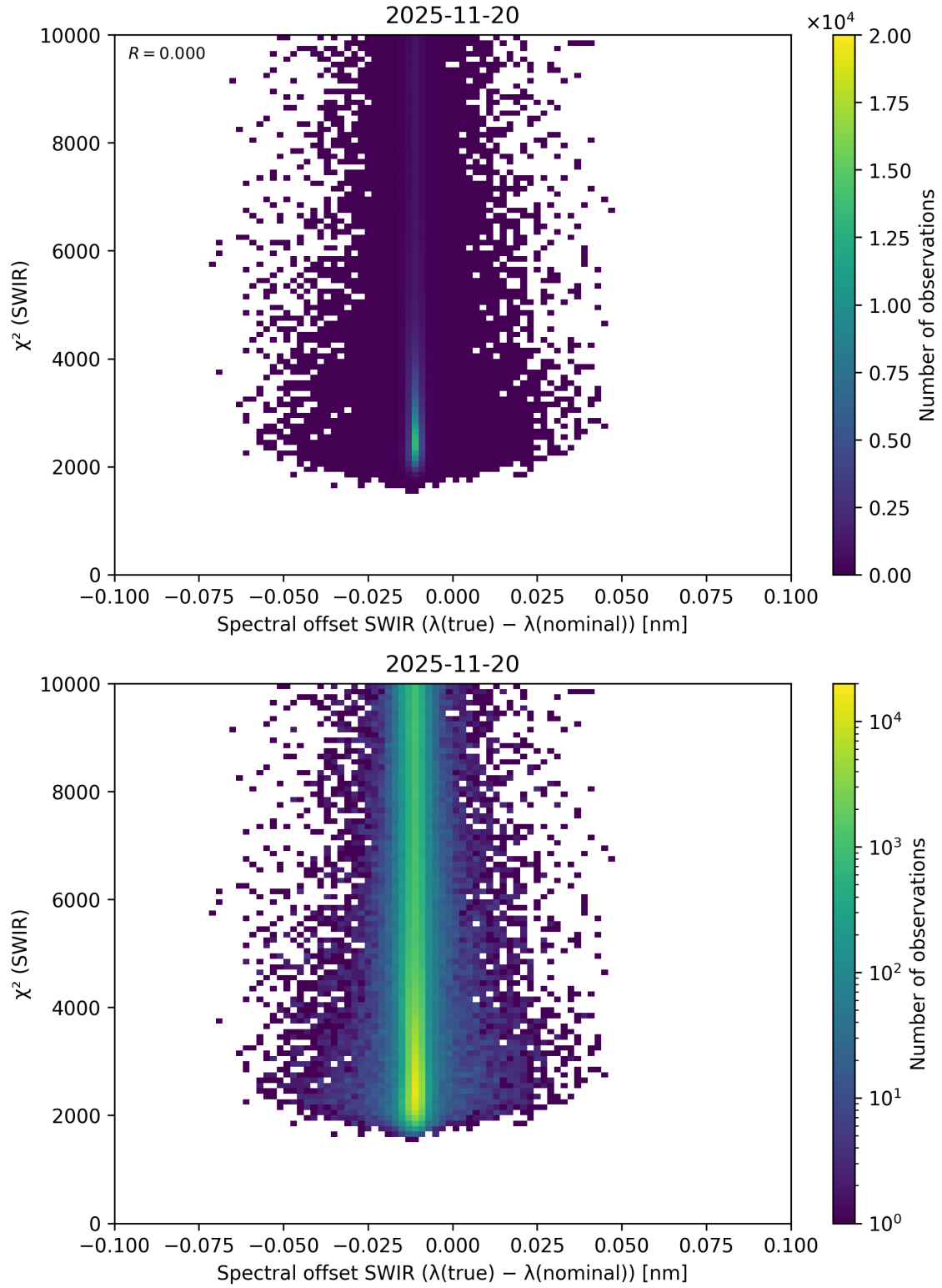
Figure 118: Scatter density plot of “Spectral offset SWIR ( \lambda_{\text{true}} - \lambda_{\text{nominal}} )” against “ \chi^2 (SWIR)” for 2025-11-19 to 2025-11-21.
