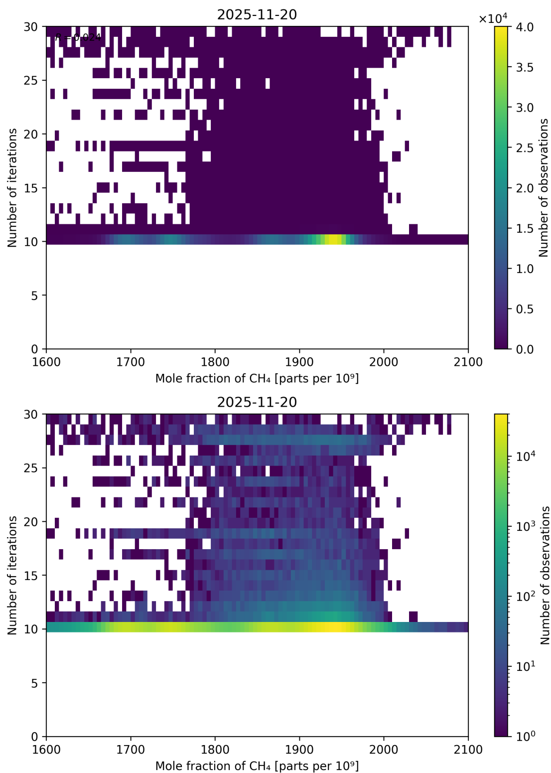
Figure 76: Scatter density plot of “Mole fraction of CH 4 ” against “Number of iterations” for 2025-11-19 to 2025-11-21.
