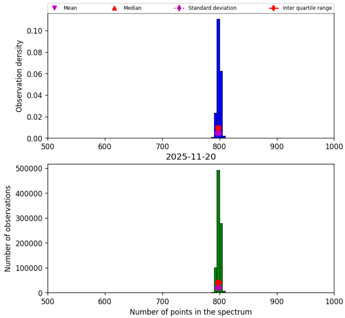
Figure 26: Histogram of “Number of points in the spectrum” for 2025-11-19 to 2025-11-21
