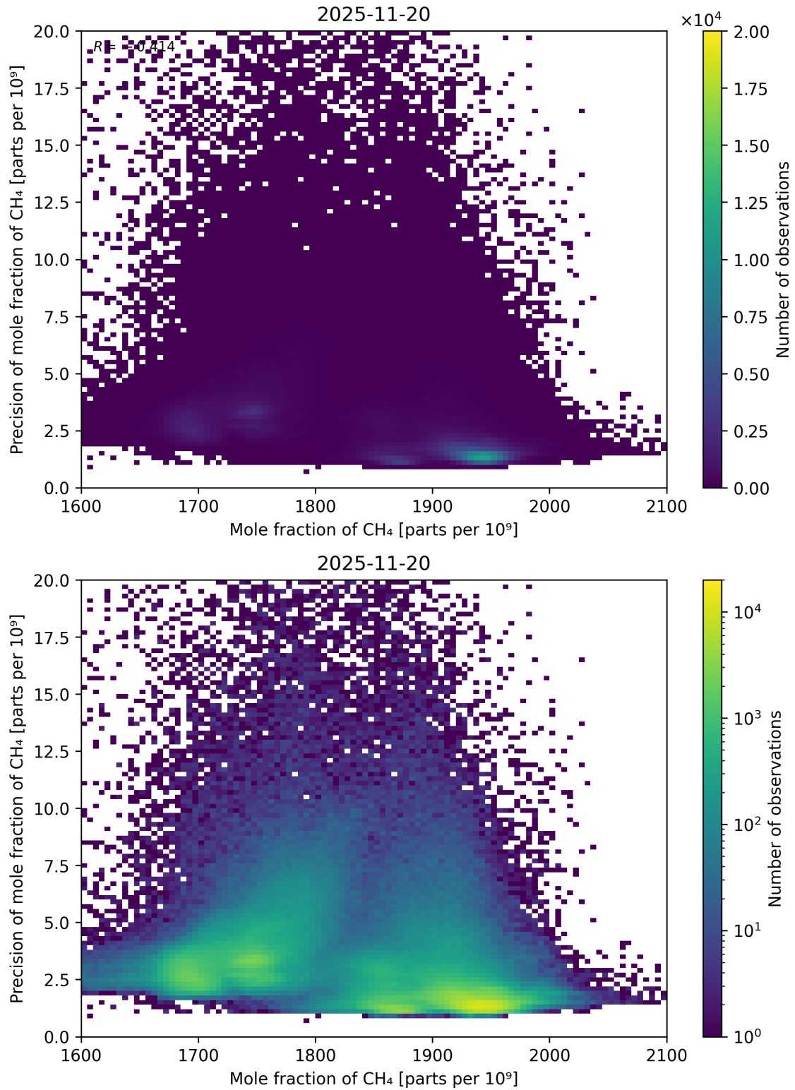
Figure 75: Scatter density plot of “Mole fraction of CH 4 ” against “Precision of mole fraction of CH 4 ” for 2025-11-19 to 2025-11-21.
