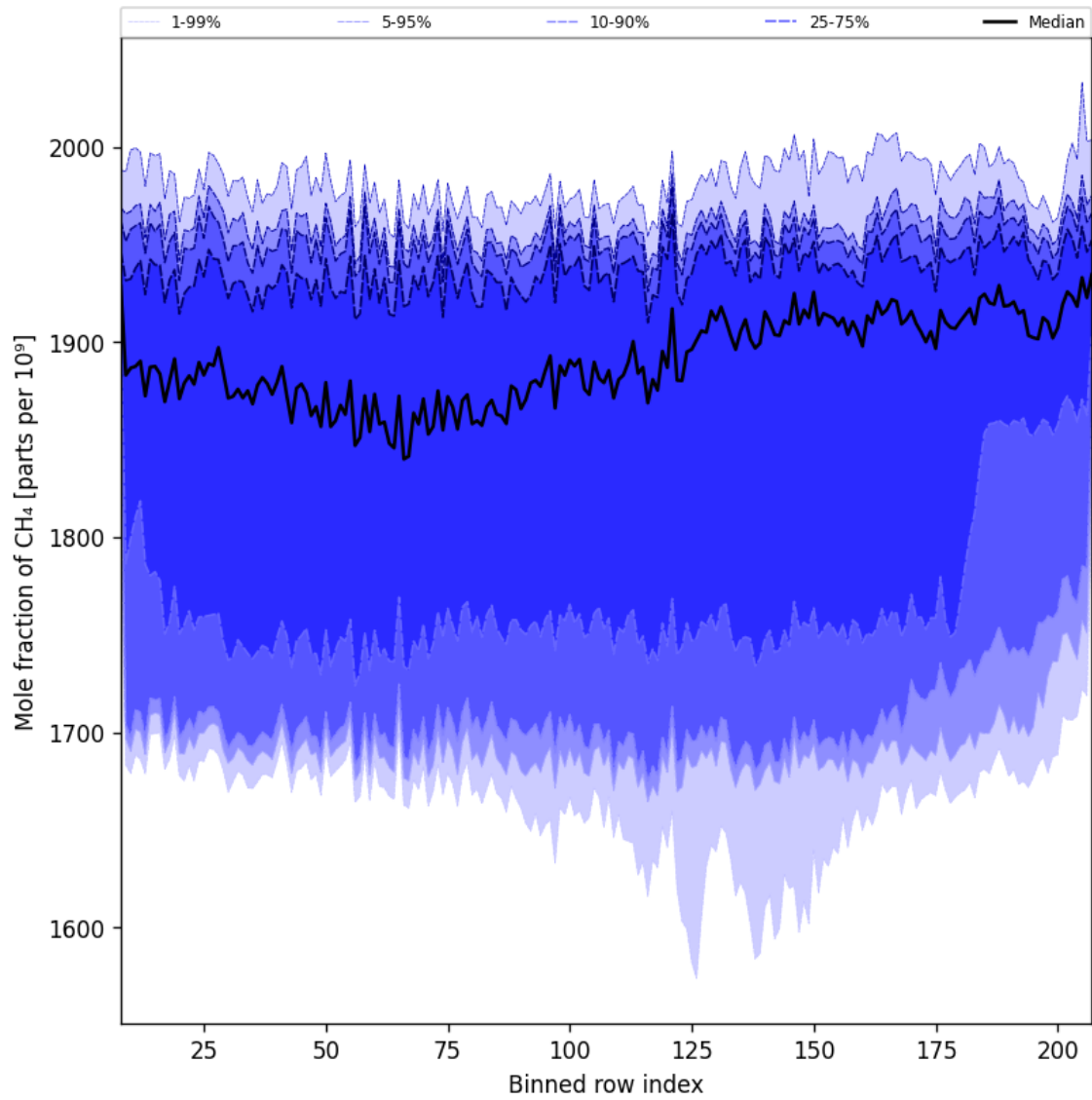
Figure 34: Along track statistics of “Mole fraction of CH 4 ” for 2025-11-19 to 2025-11-21
