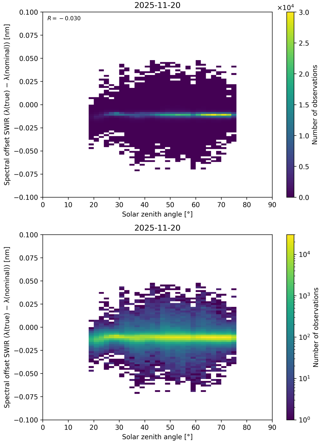
Figure 104: Scatter density plot of “Solar zenith angle” against “Spectral offset SWIR ( \lambda_{\text{true}} - \lambda_{\text{nominal}} )” for 2025-11-19 to 2025-11-21.
