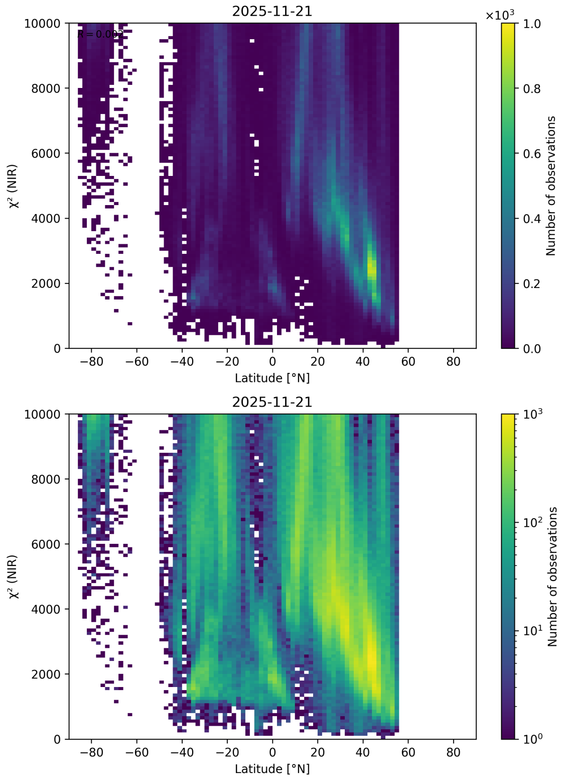
Figure 53: Scatter density plot of “Latitude” against “ \chi^2 (NIR)” for 2025-11-20 to 2025-11-22.
