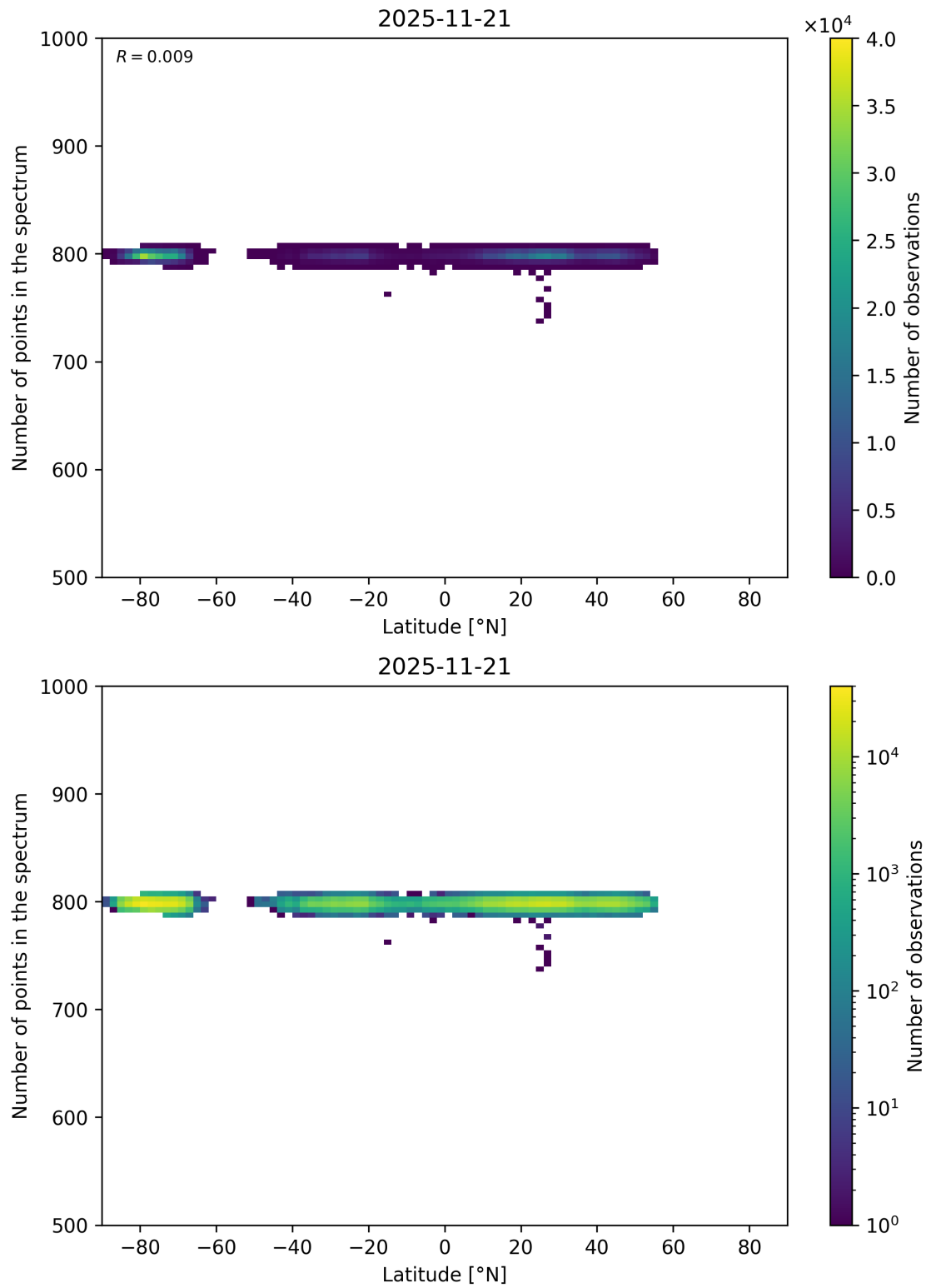
Figure 61: Scatter density plot of “Latitude” against “Number of points in the spectrum” for 2025-11-20 to 2025-11-22.
