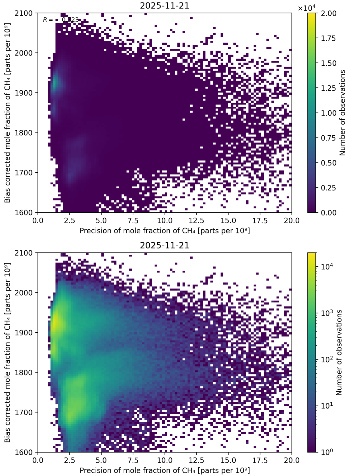
Figure 82: Scatter density plot of “Precision of mole fraction of CH 4 ” against “Bias corrected mole fraction of CH 4 ” for 2025-11-20 to 2025-11-22.
