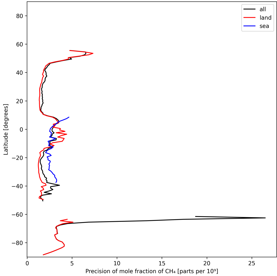
Figure 13: Zonal average of “Precision of mole fraction of CH 4 ” for 2025-11-20 to 2025-11-22.
