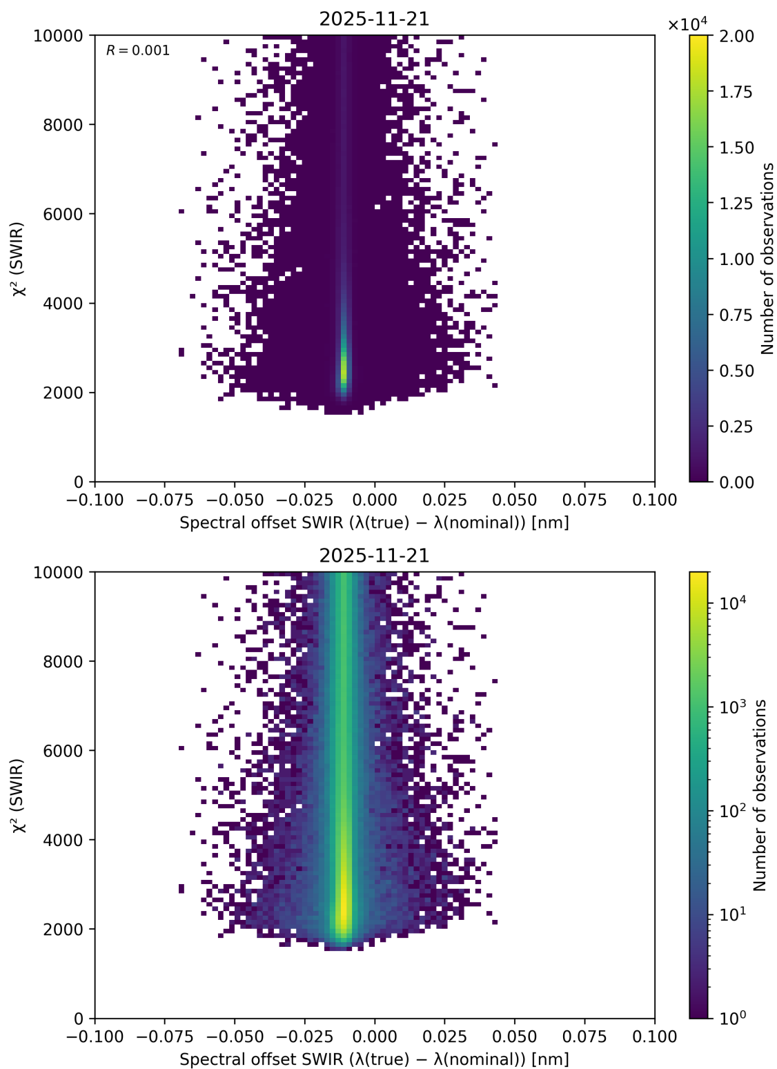
Figure 118: Scatter density plot of “Spectral offset SWIR ( \lambda_{\text{true}} - \lambda_{\text{nominal}} )” against “ \chi^2 (SWIR)” for 2025-11-20 to 2025-11-22.
