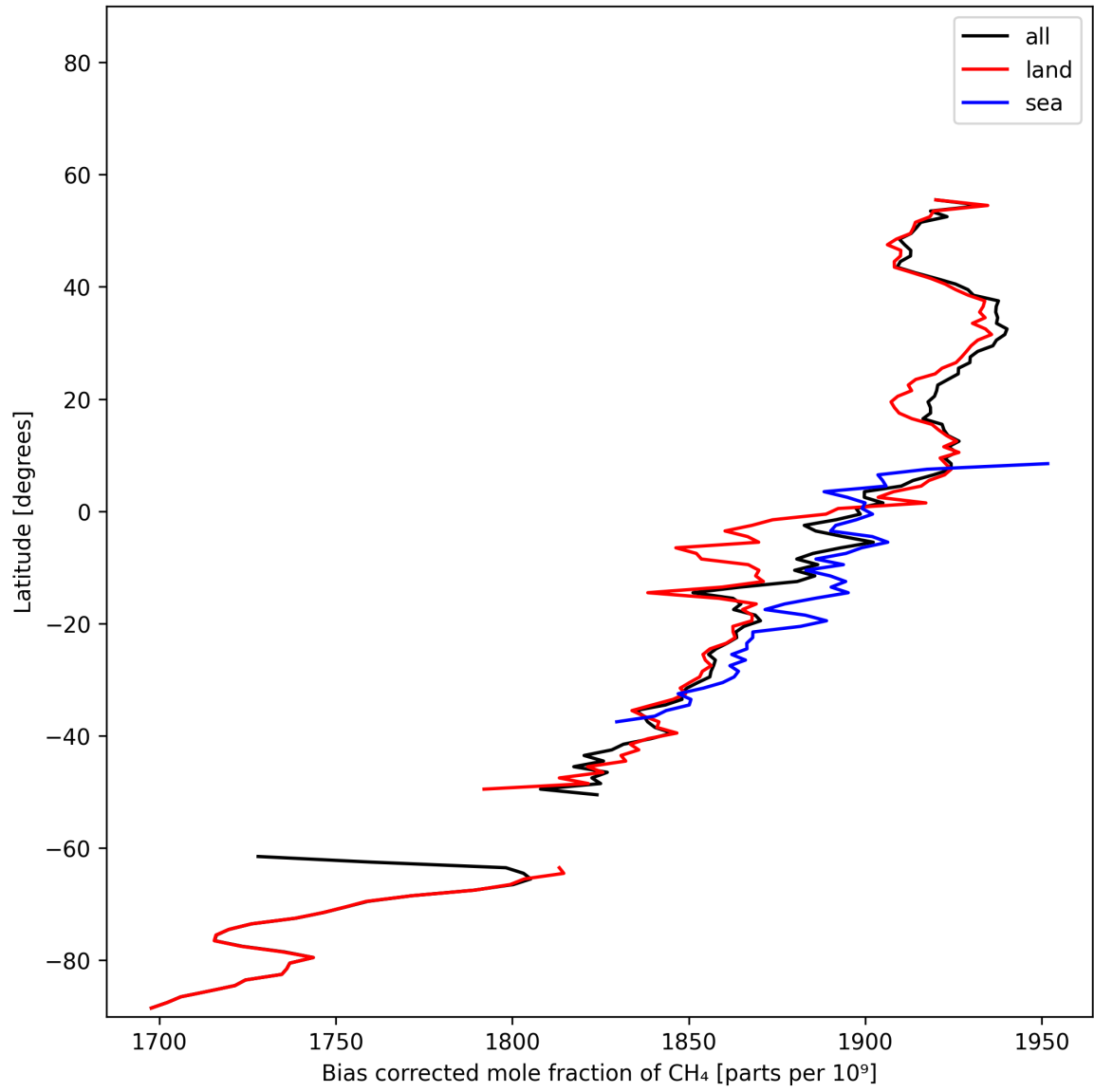
Figure 14: Zonal average of “Bias corrected mole fraction of CH 4 ” for 2025-11-20 to 2025-11-22.
