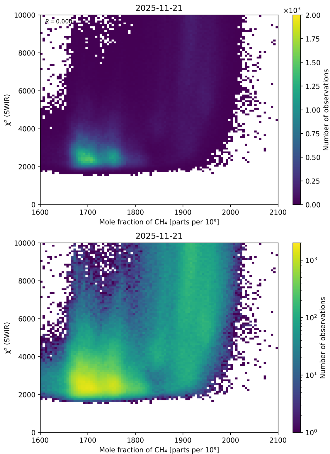
Figure 71: Scatter density plot of “Mole fraction of \text{CH}_4 ” against “ \chi^2 (SWIR)” for 2025-11-20 to 2025-11-22.
