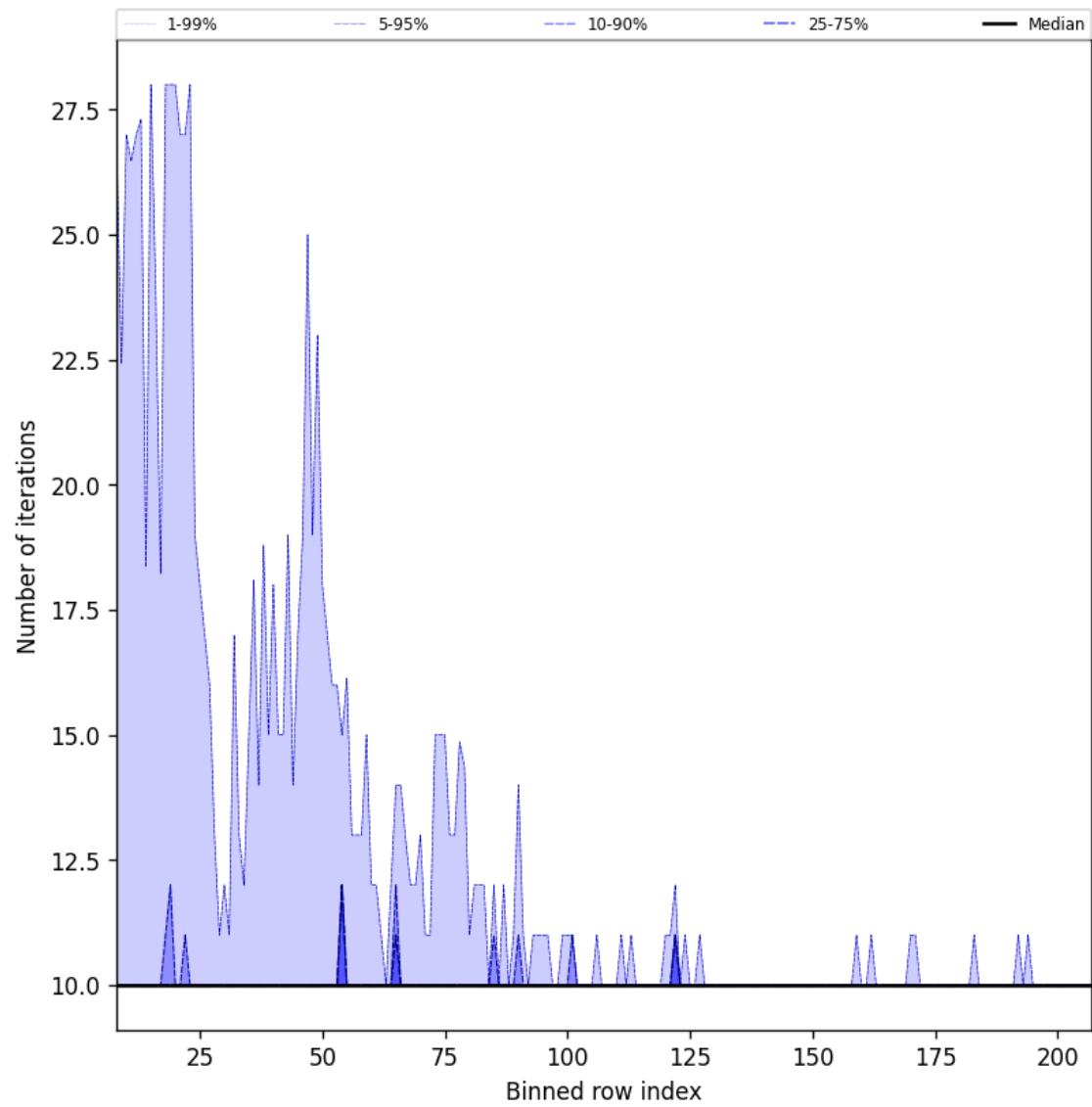
Figure 42: Along track statistics of “Number of iterations” for 2025-11-20 to 2025-11-22
