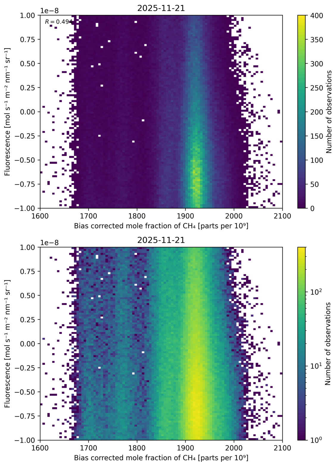
Figure 66: Scatter density plot of “Bias corrected mole fraction of \text{CH}_4 ” against “Fluorescence” for 2025-11-20 to 2025-11-22.
