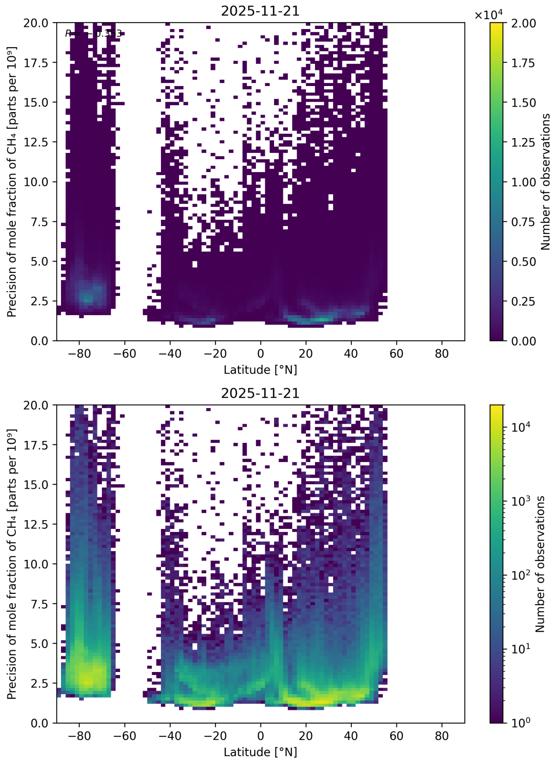
Figure 59: Scatter density plot of “Latitude” against “Precision of mole fraction of CH 4 ” for 2025-11-20 to 2025-11-22.
