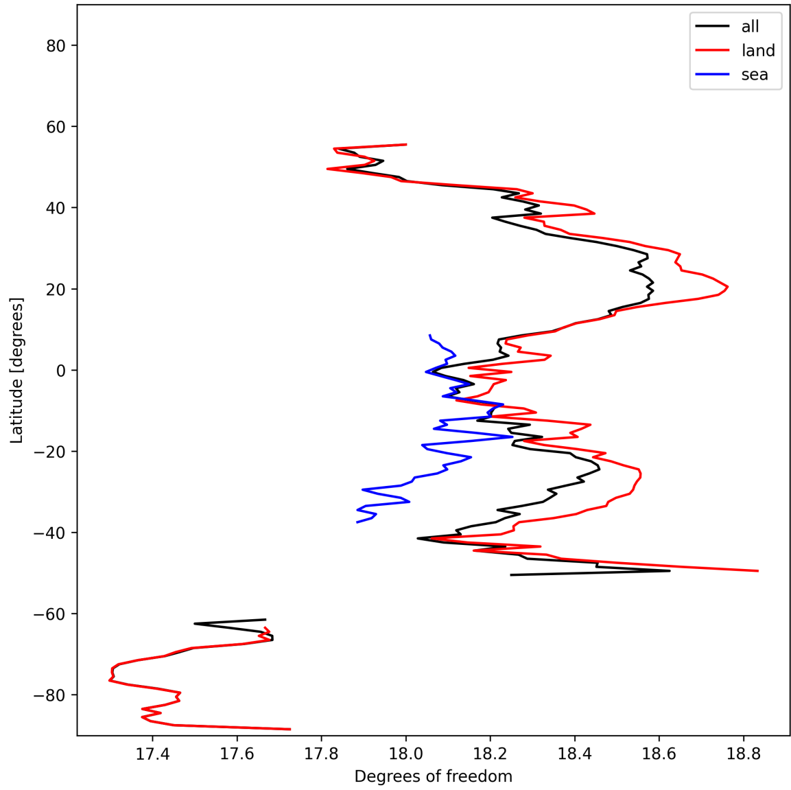
Figure 19: Zonal average of “Degrees of freedom” for 2025-11-20 to 2025-11-22.
