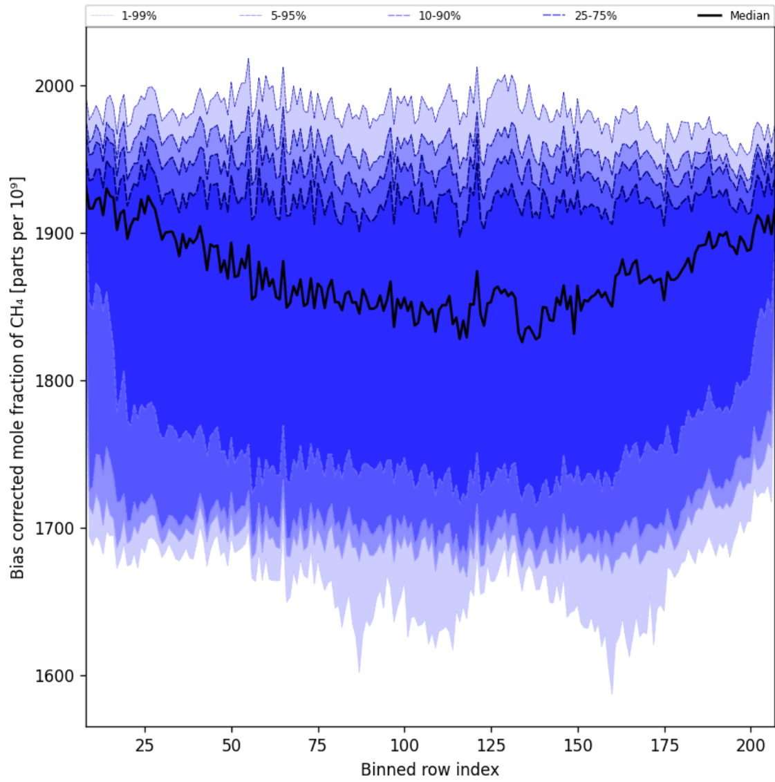
Figure 36: Along track statistics of “Bias corrected mole fraction of CH 4 ” for 2025-11-20 to 2025-11-22
