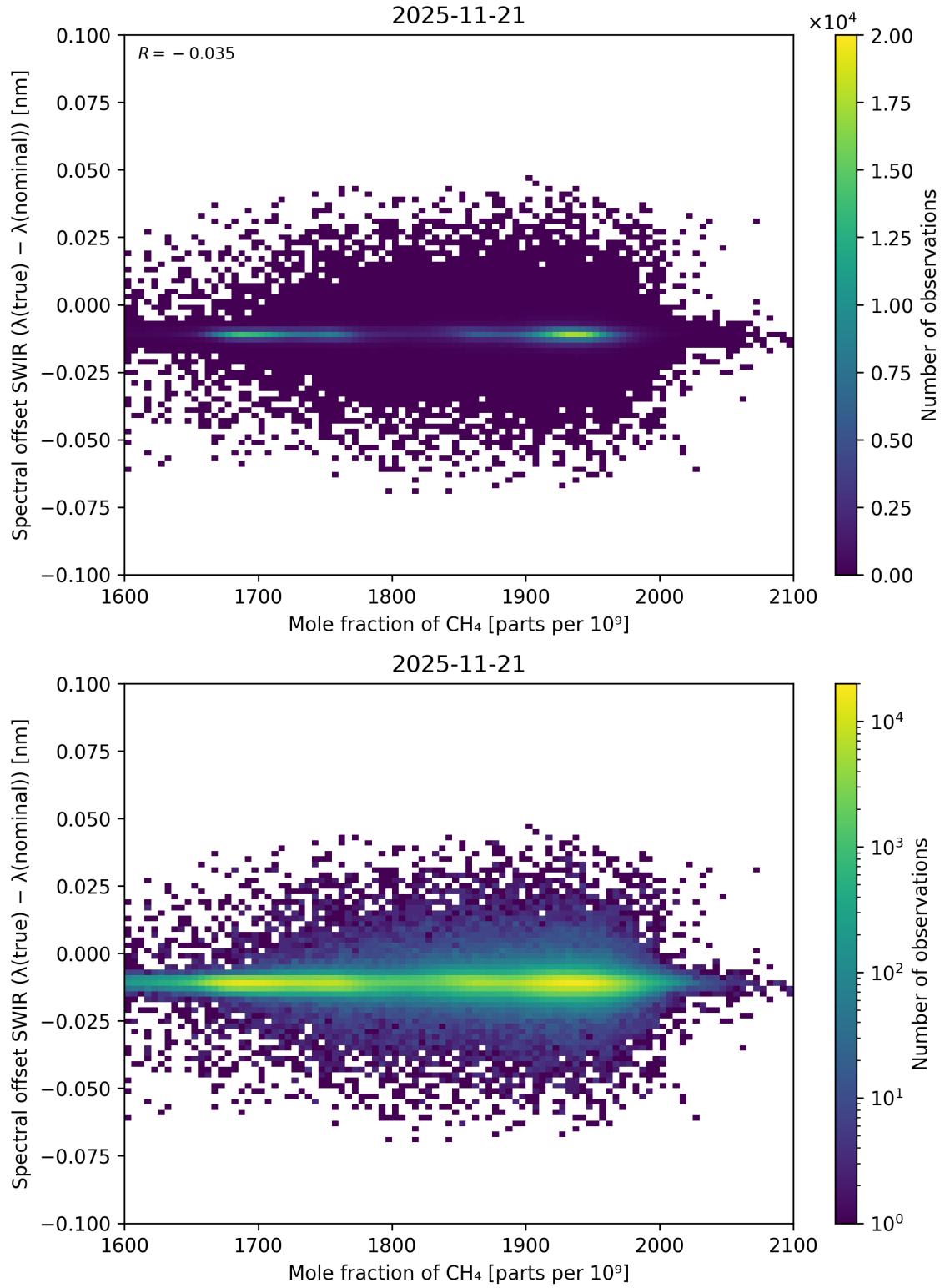
Figure 86: Scatter density plot of “Mole fraction of CH 4 ” against “Spectral offset SWIR ( \lambda_{\text{true}} - \lambda_{\text{nominal}} )” for 2025-11-20 to 2025-11-22.
