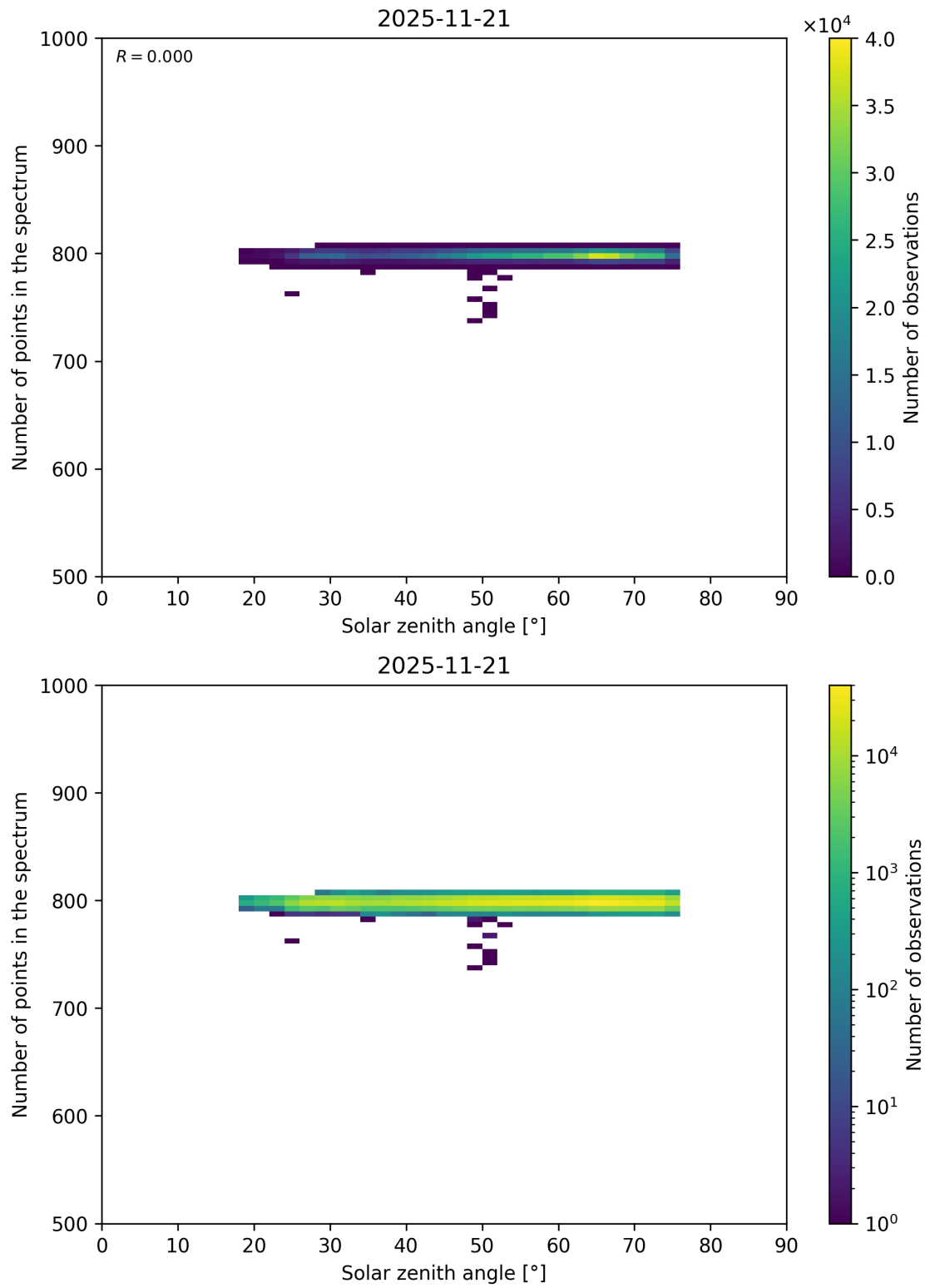
Figure 103: Scatter density plot of “Solar zenith angle” against “Number of points in the spectrum” for 2025-11-20 to 2025-11-22.
