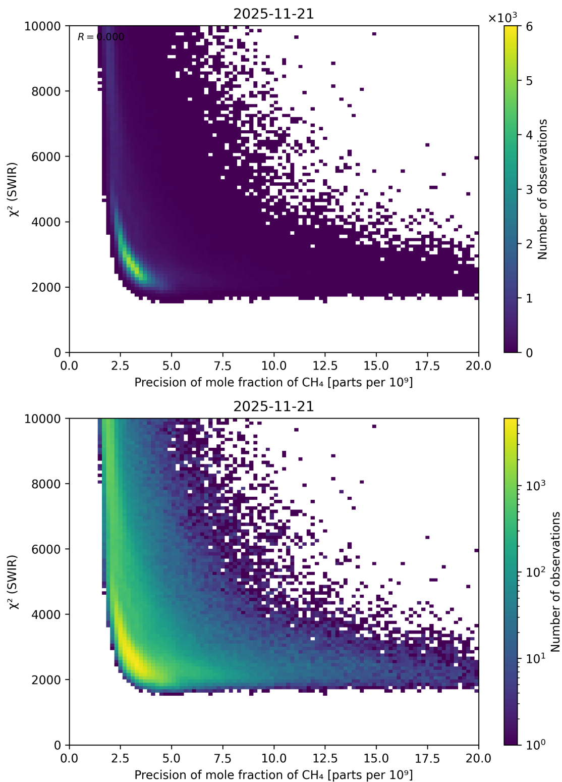
Figure 79: Scatter density plot of “Precision of mole fraction of \text{CH}_4 ” against “ \chi^2 (SWIR)” for 2025-11-20 to 2025-11-22.
