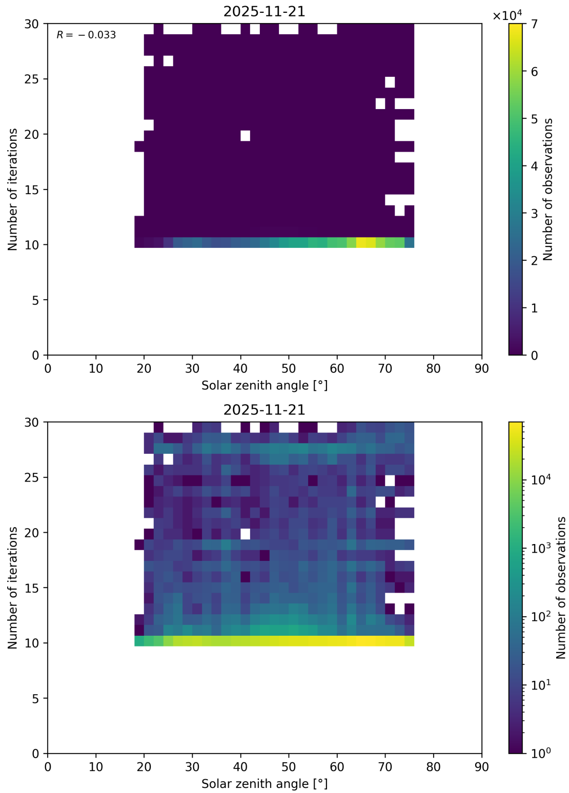
Figure 102: Scatter density plot of “Solar zenith angle” against “Number of iterations” for 2025-11-20 to 2025-11-22.
