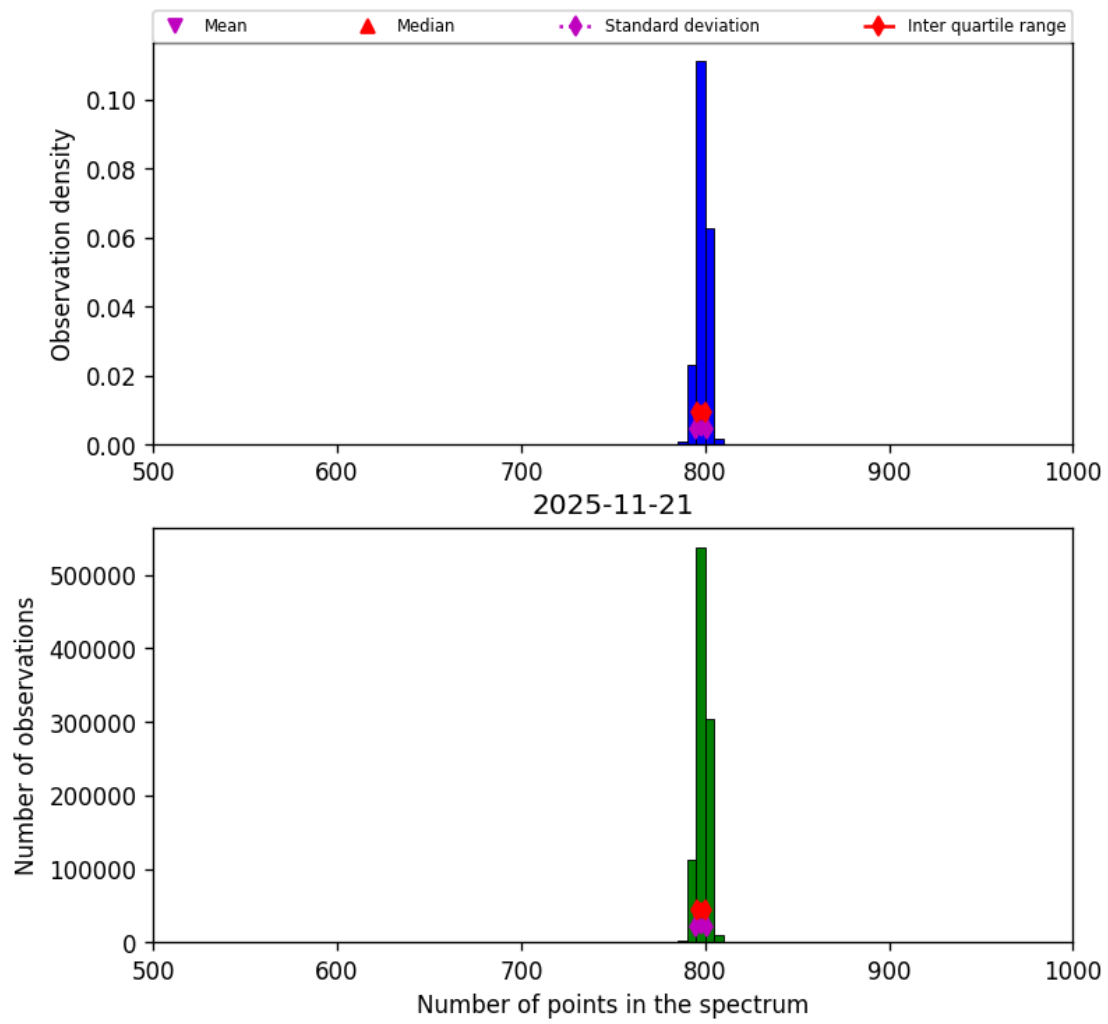
Figure 26: Histogram of “Number of points in the spectrum” for 2025-11-20 to 2025-11-22
