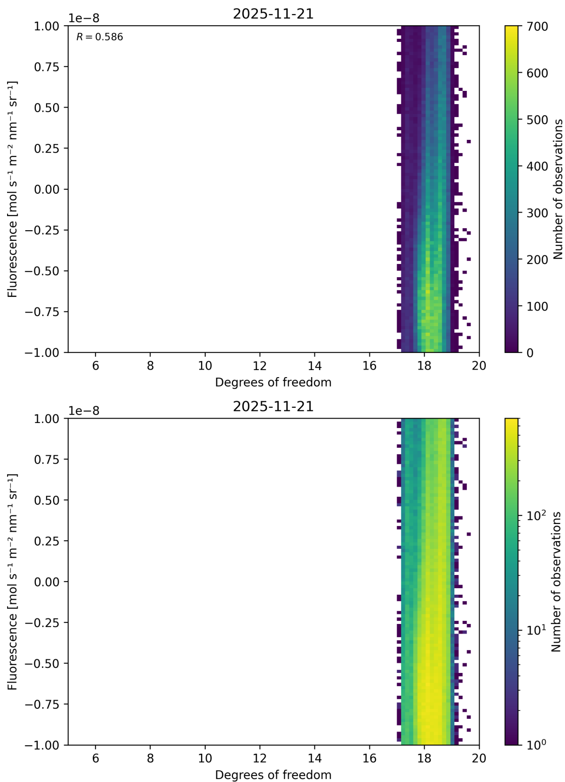
Figure 51: Scatter density plot of “Degrees of freedom” against “Fluorescence” for 2025-11-20 to 2025-11-22.
