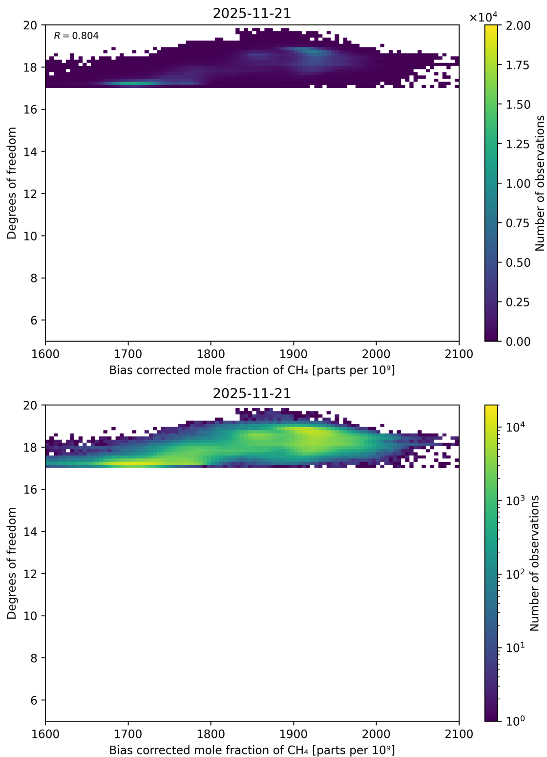
Figure 65: Scatter density plot of “Bias corrected mole fraction of \text{CH}_4 ” against “Degrees of freedom” for 2025-11-20 to 2025-11-22.
