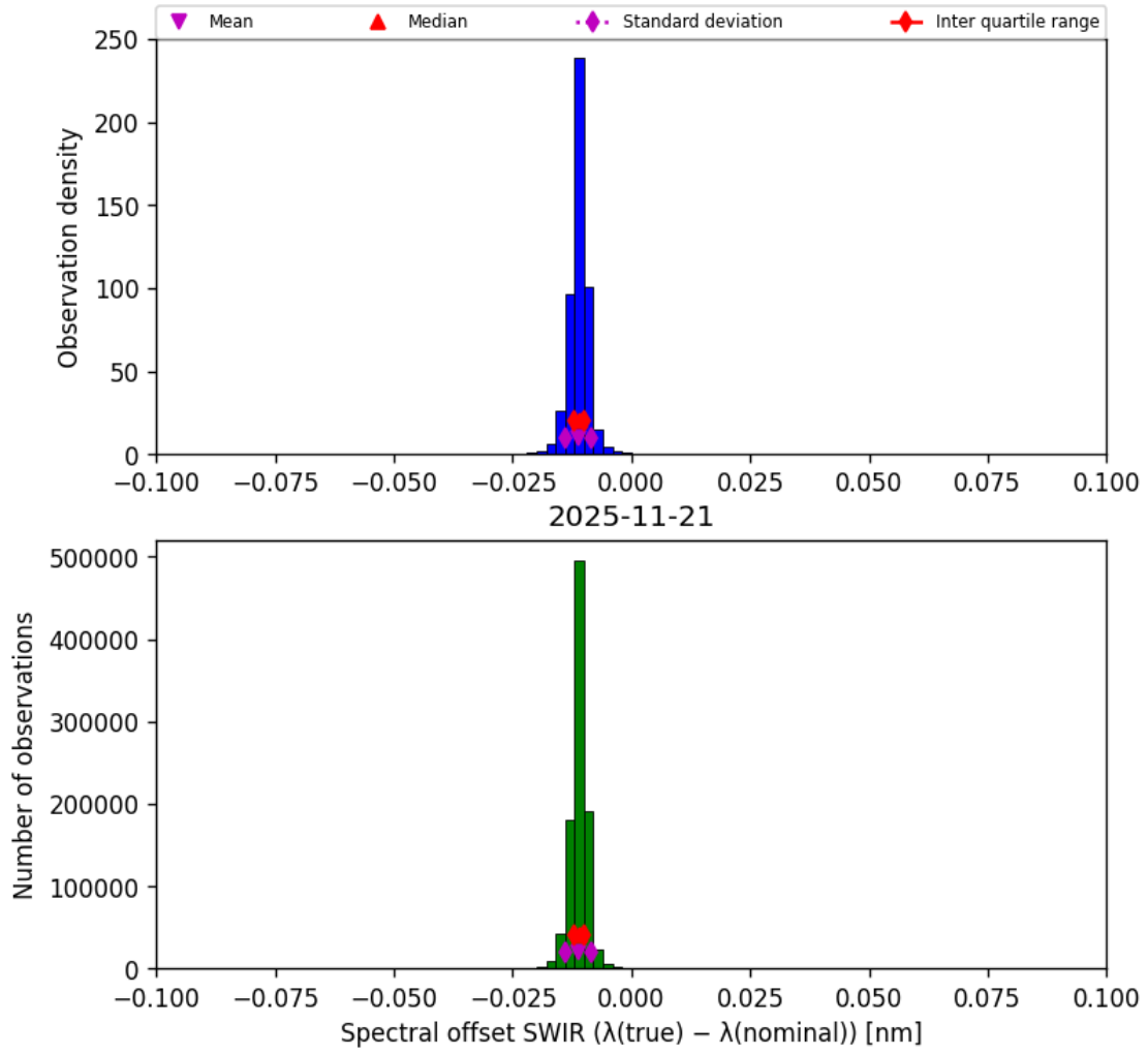
Figure 27: Histogram of “Spectral offset SWIR ( \lambda_{\text{true}} - \lambda_{\text{nominal}} )” for 2025-11-20 to 2025-11-22
