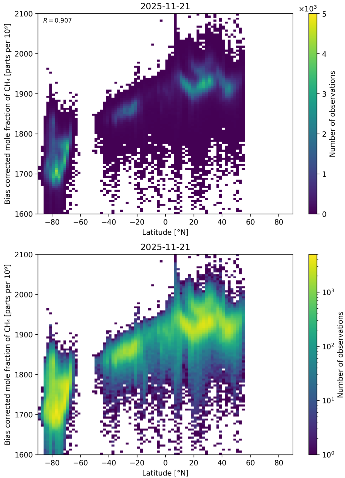
Figure 58: Scatter density plot of “Latitude” against “Bias corrected mole fraction of CH 4 ” for 2025-11-20 to 2025-11-22.
