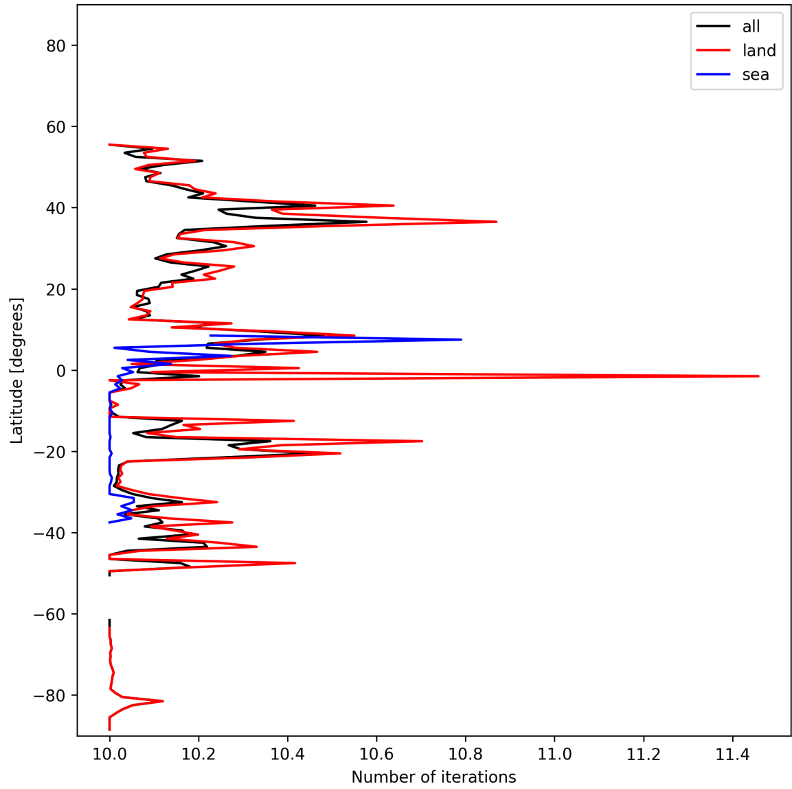
Figure 20: Zonal average of “Number of iterations” for 2025-11-20 to 2025-11-22.
