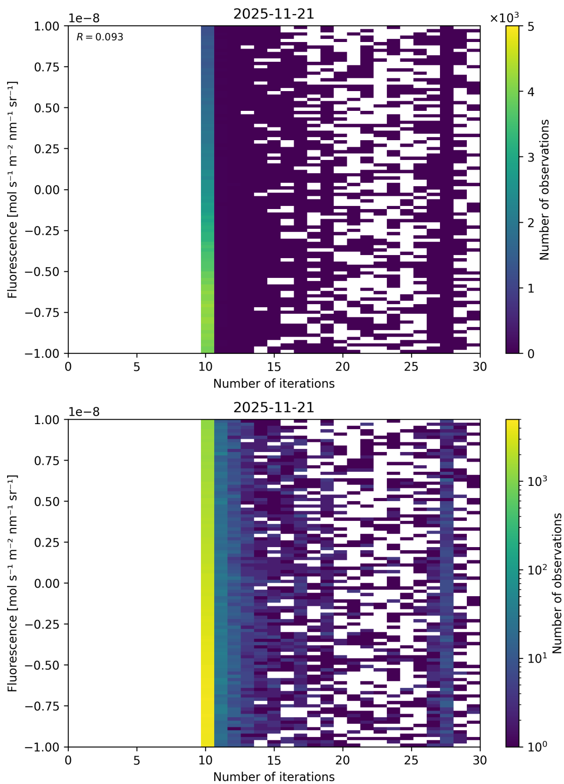
Figure 87: Scatter density plot of “Number of iterations” against “Fluorescence” for 2025-11-20 to 2025-11-22.
