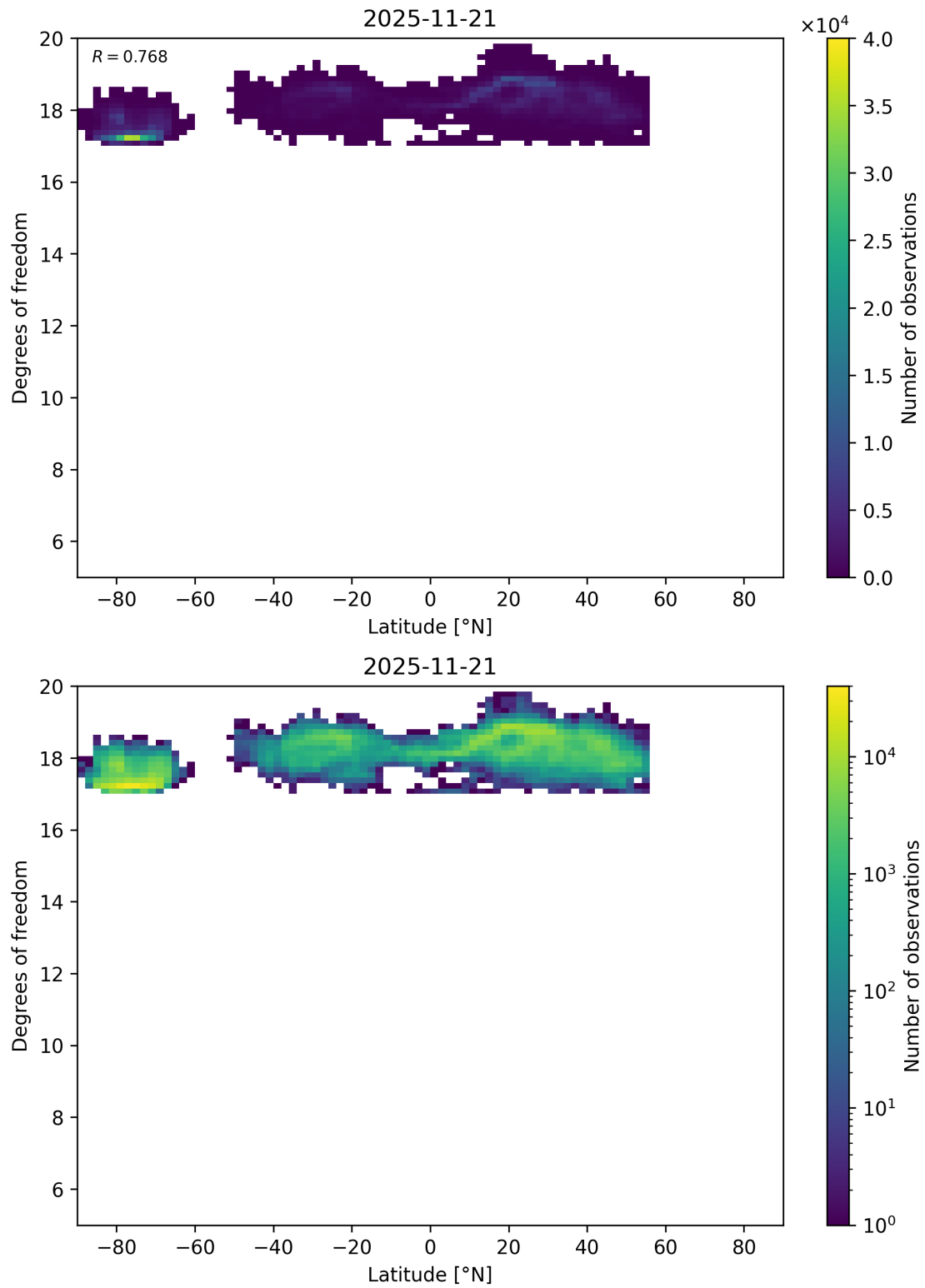
Figure 55: Scatter density plot of “Latitude” against “Degrees of freedom” for 2025-11-20 to 2025-11-22.
