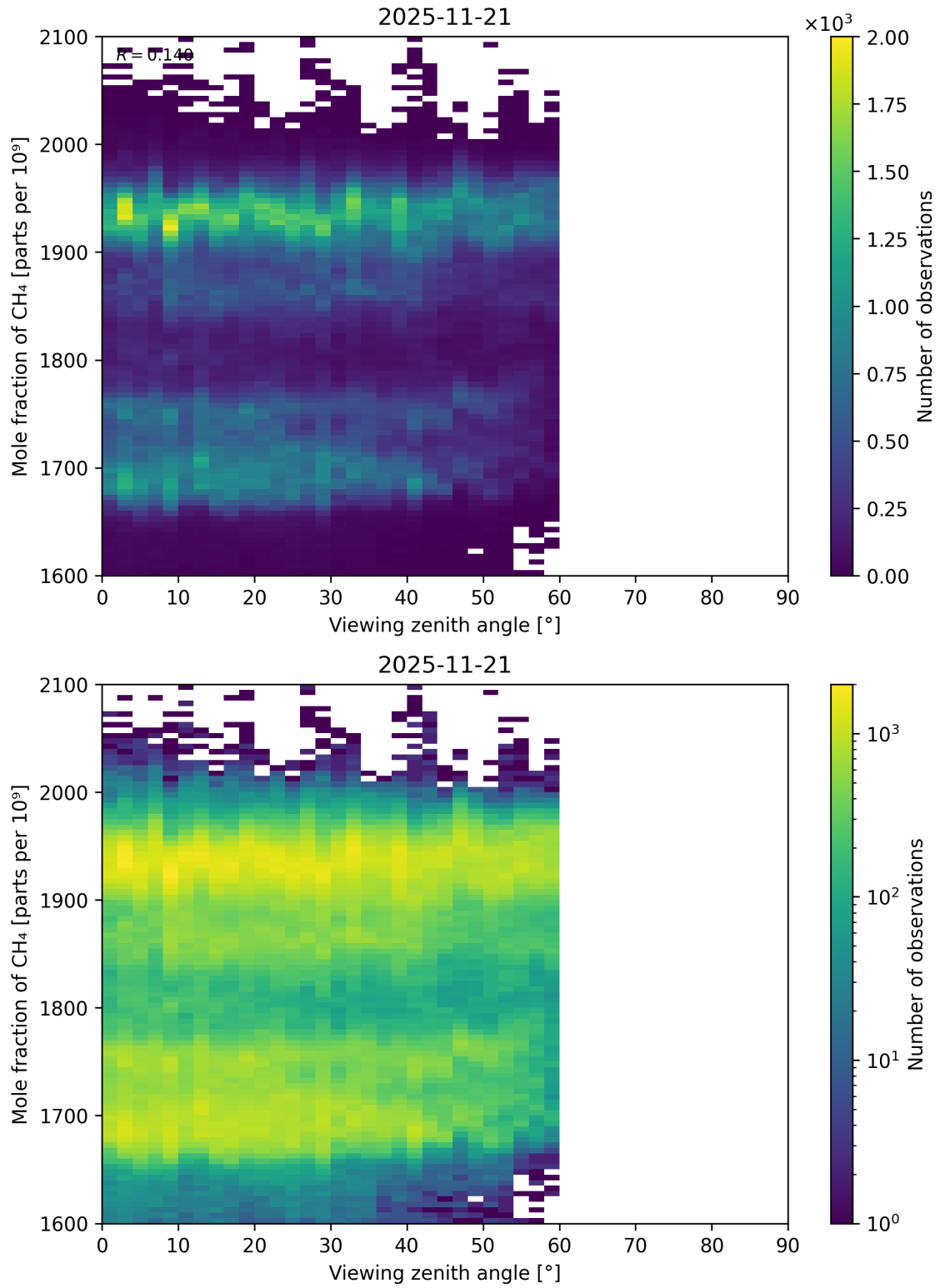
Figure 110: Scatter density plot of “Viewing zenith angle” against “Mole fraction of CH 4 ” for 2025-11-20 to 2025-11-22.
