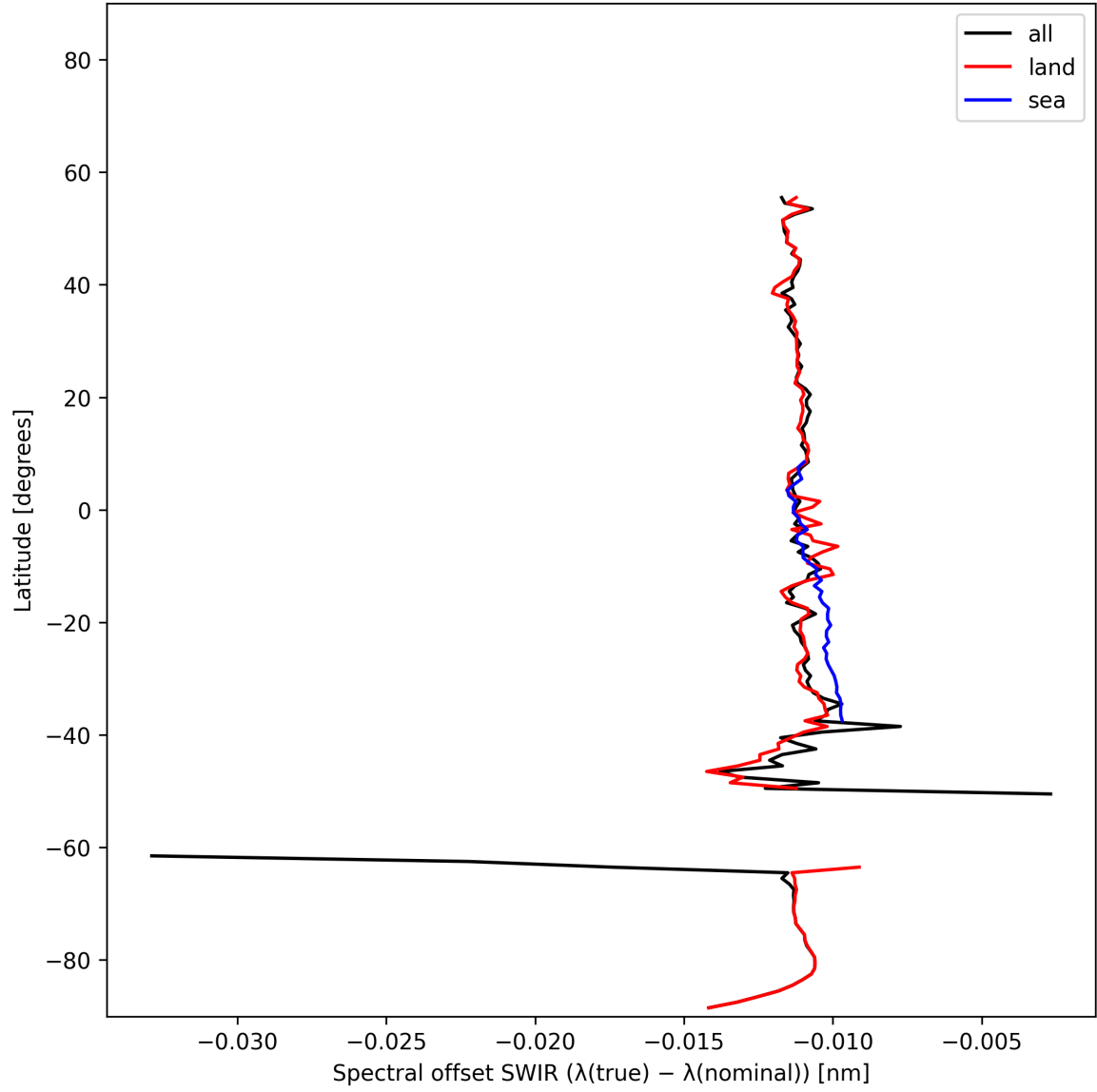
Figure 16: Zonal average of “Spectral offset SWIR ( \lambda_{\text{true}} - \lambda_{\text{nominal}} )” for 2025-11-20 to 2025-11-22.
