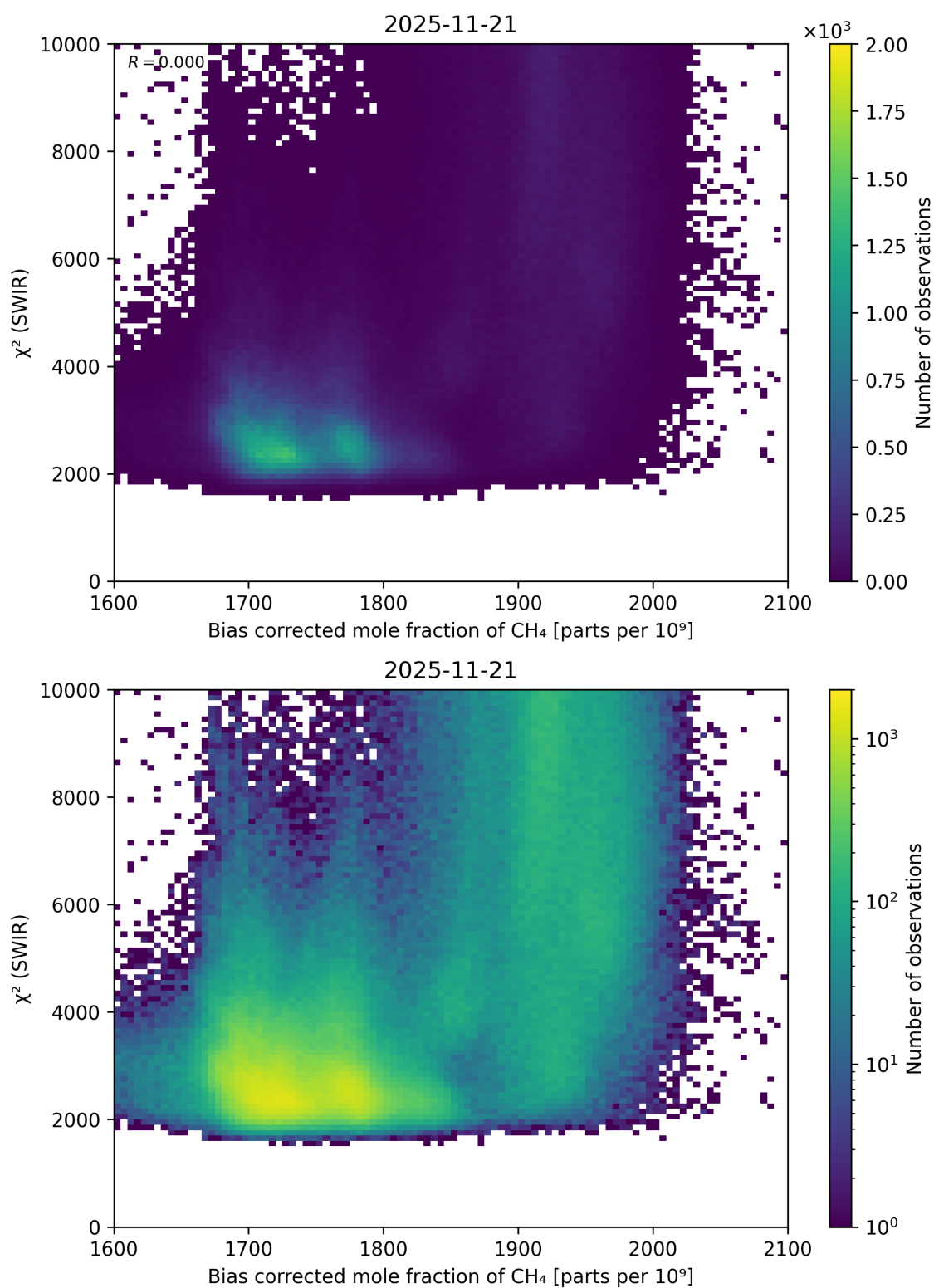
Figure 64: Scatter density plot of “Bias corrected mole fraction of CH 4 ” against “ \chi^2 (SWIR)” for 2025-11-20 to 2025-11-22.
