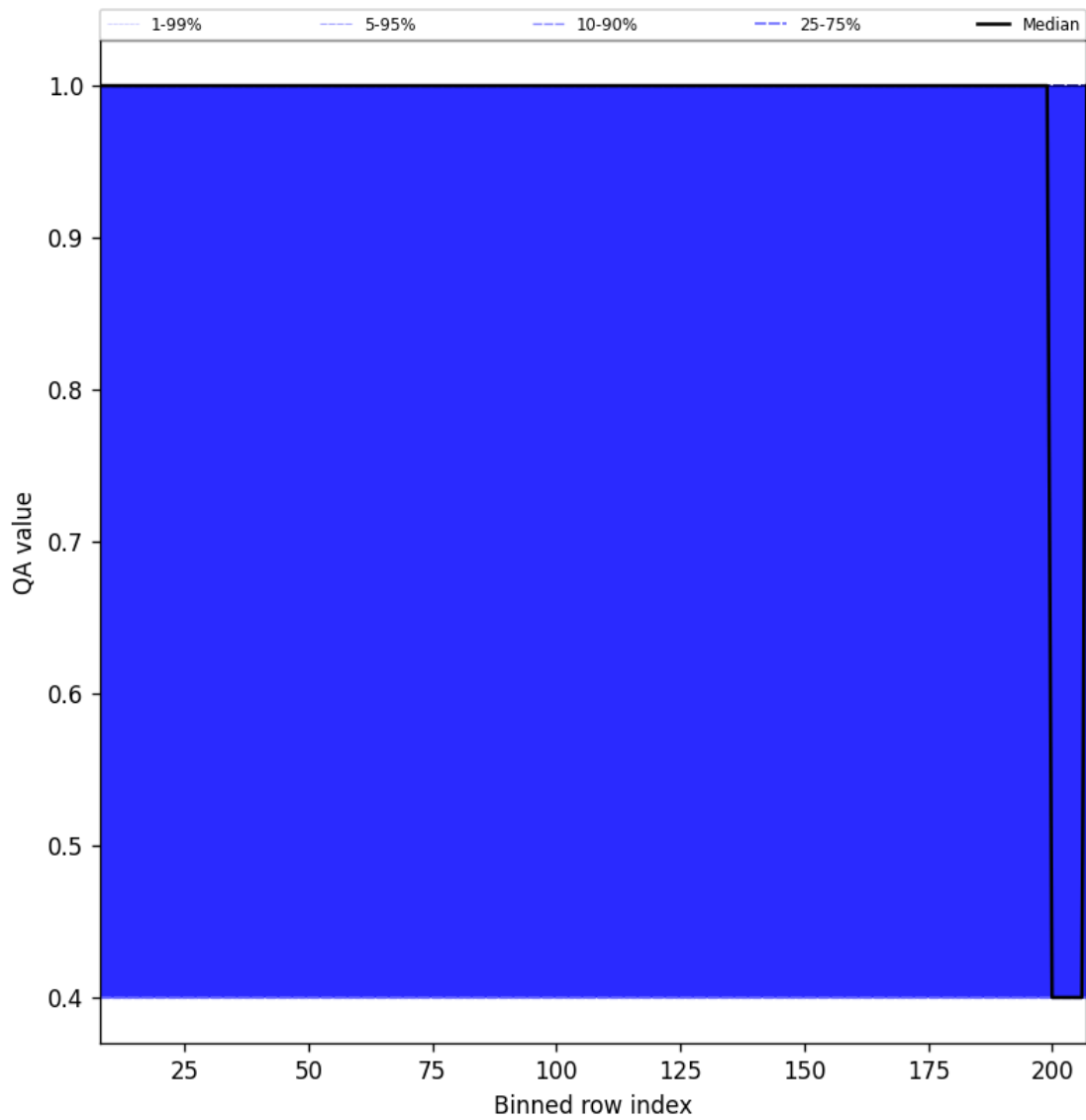
Figure 33: Along track statistics of “QA value” for 2025-11-20 to 2025-11-22
