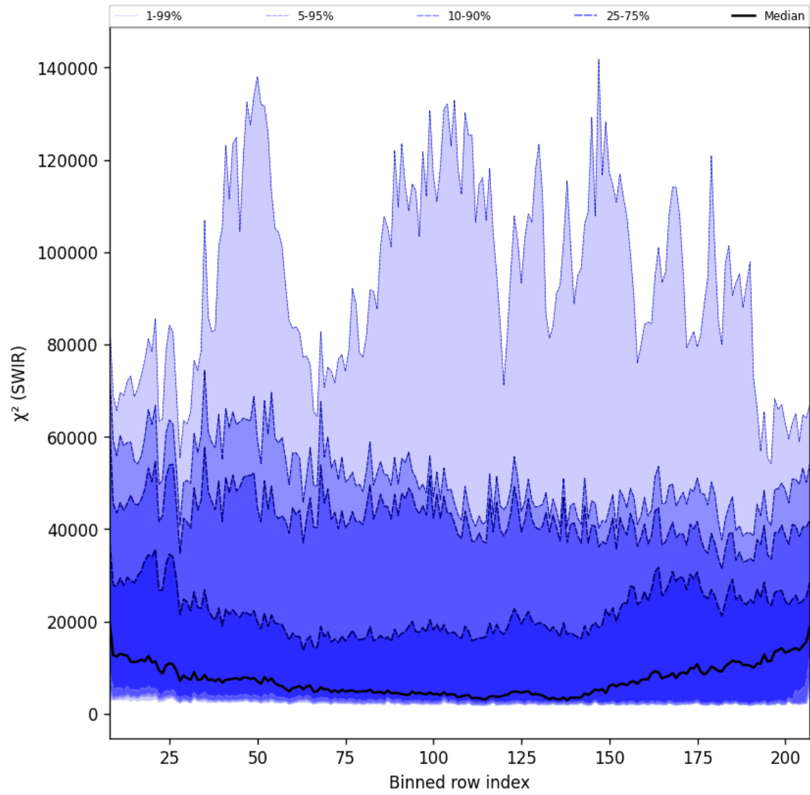
Figure 39: Along track statistics of “ \chi^2 (SWIR)” for 2025-11-20 to 2025-11-22
