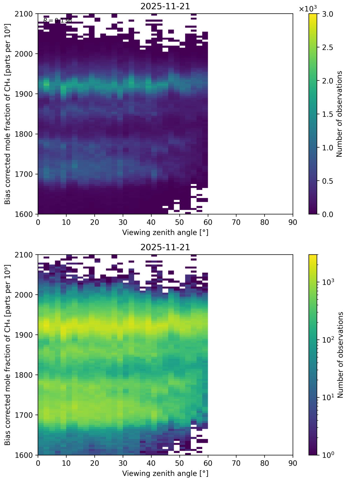
Figure 111: Scatter density plot of “Viewing zenith angle” against “Bias corrected mole fraction of CH 4 ” for 2025-11-20 to 2025-11-22.
