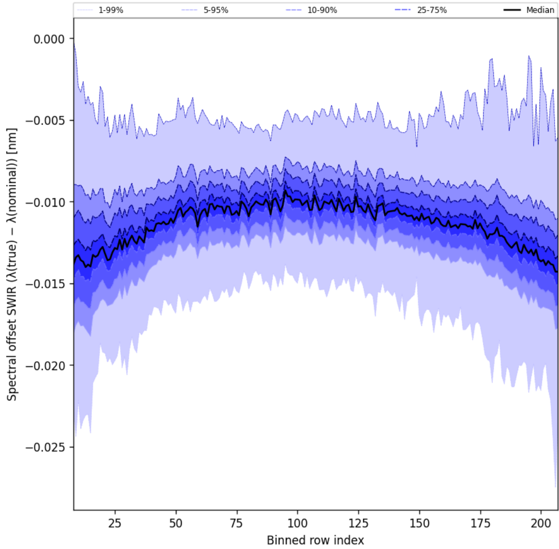
Figure 38: Along track statistics of “Spectral offset SWIR ( \lambda_{\text{true}} - \lambda_{\text{nominal}} )” for 2025-11-20 to 2025-11-22
