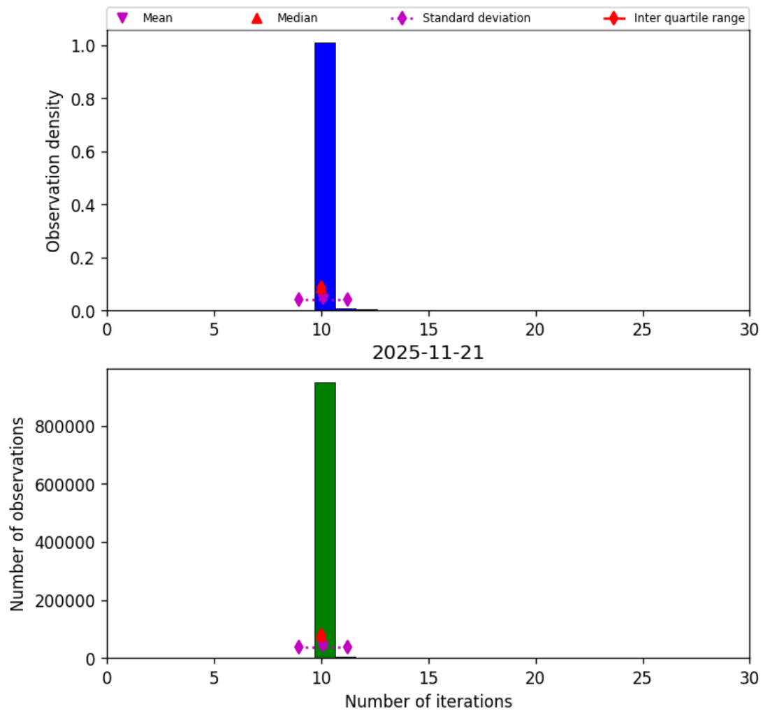
Figure 31: Histogram of “Number of iterations” for 2025-11-20 to 2025-11-22
