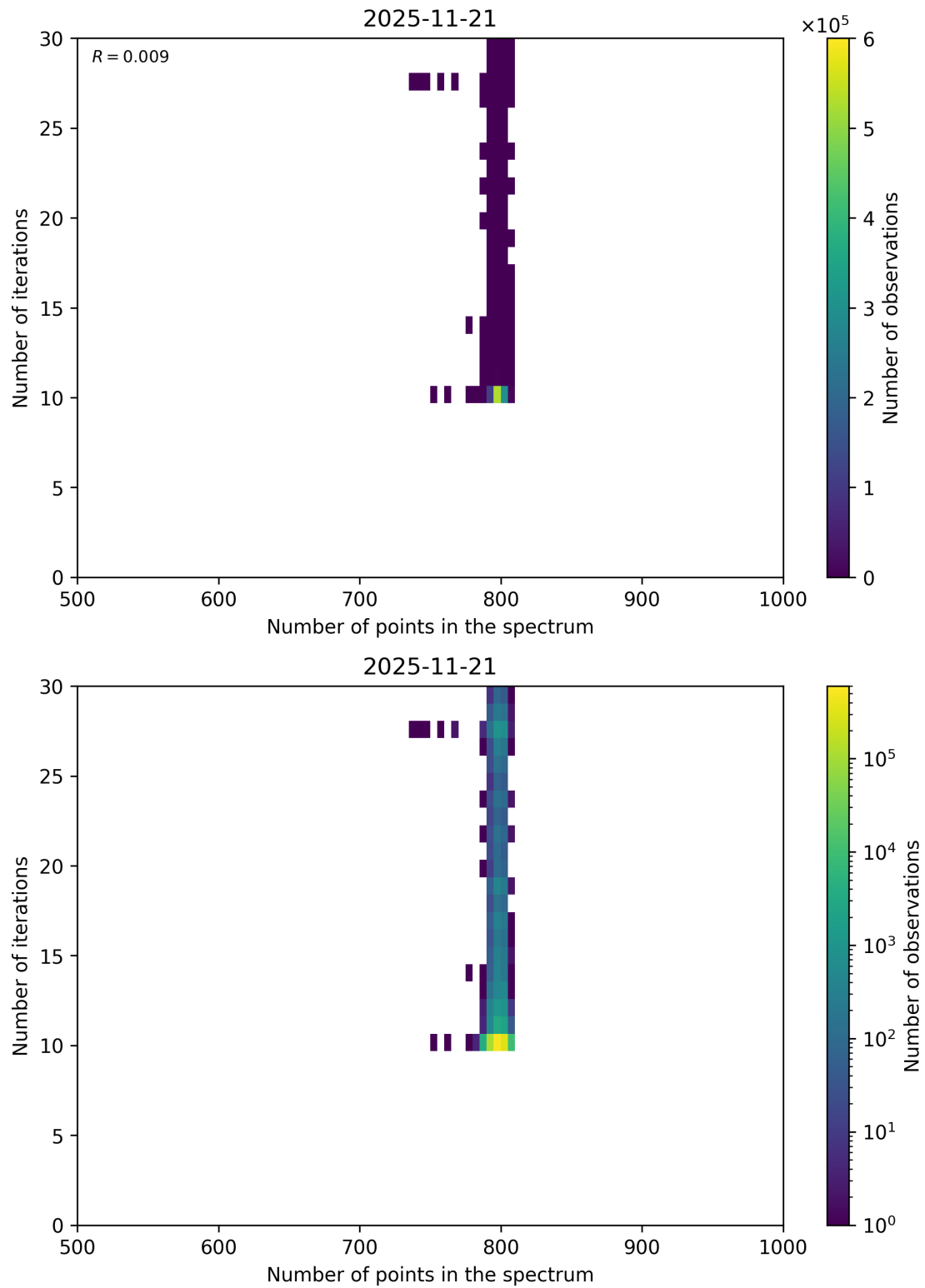
Figure 92: Scatter density plot of “Number of points in the spectrum” against “Number of iterations” for 2025-11-20 to 2025-11-22.
