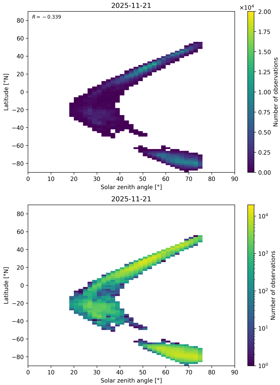
Figure 98: Scatter density plot of “Solar zenith angle” against “Latitude” for 2025-11-20 to 2025-11-22.
