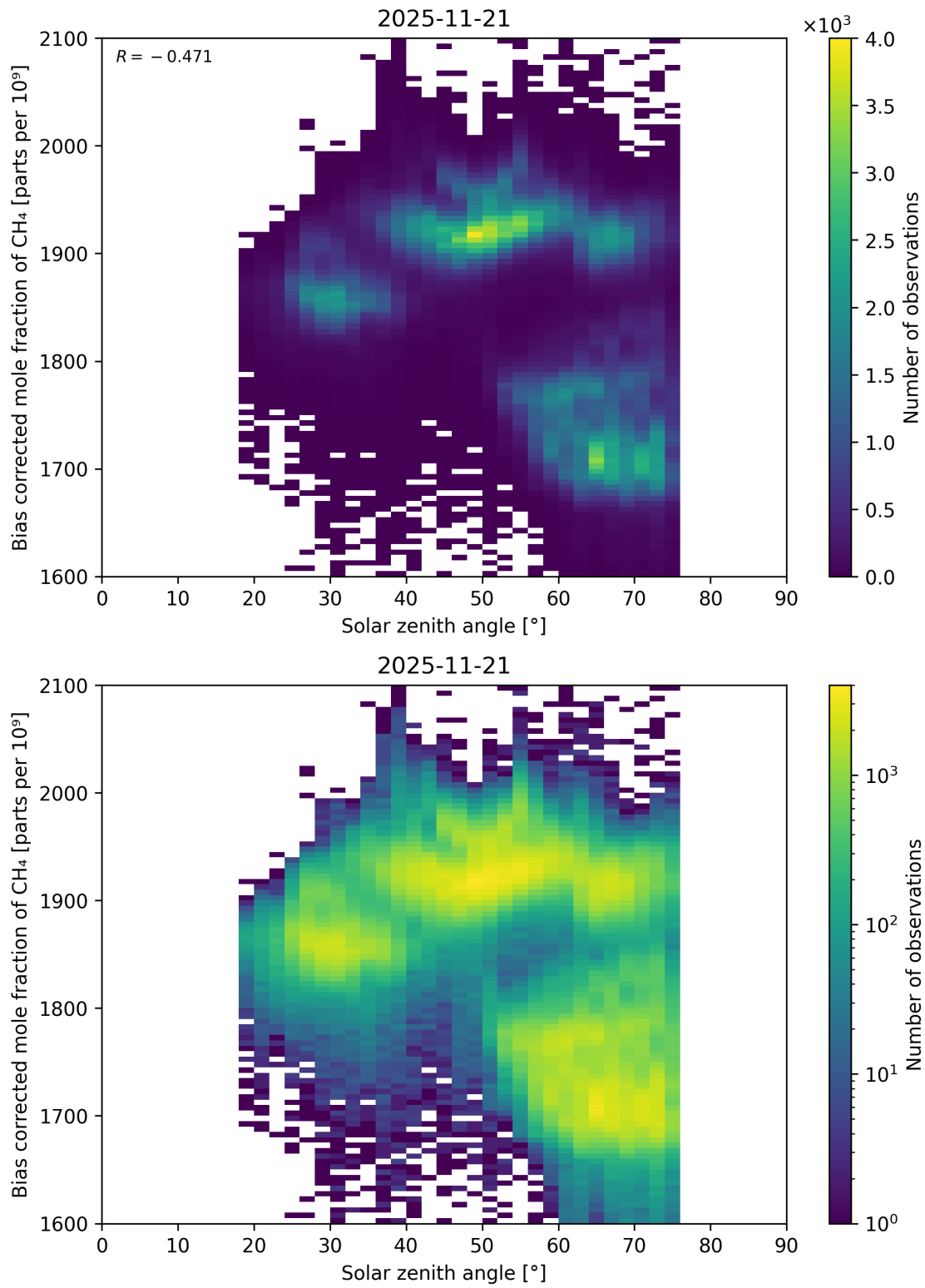
Figure 100: Scatter density plot of “Solar zenith angle” against “Bias corrected mole fraction of CH 4 ” for 2025-11-20 to 2025-11-22.
