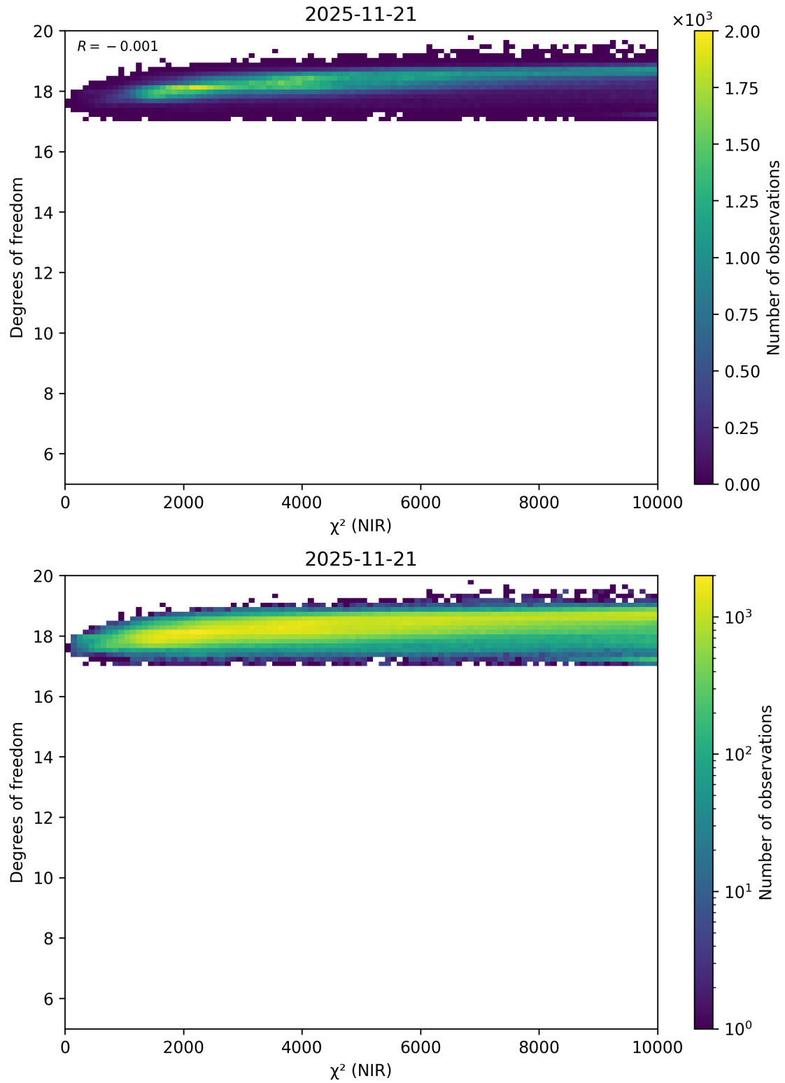
Figure 44: Scatter density plot of “ \chi^2 (NIR)” against “Degrees of freedom” for 2025-11-20 to 2025-11-22.
