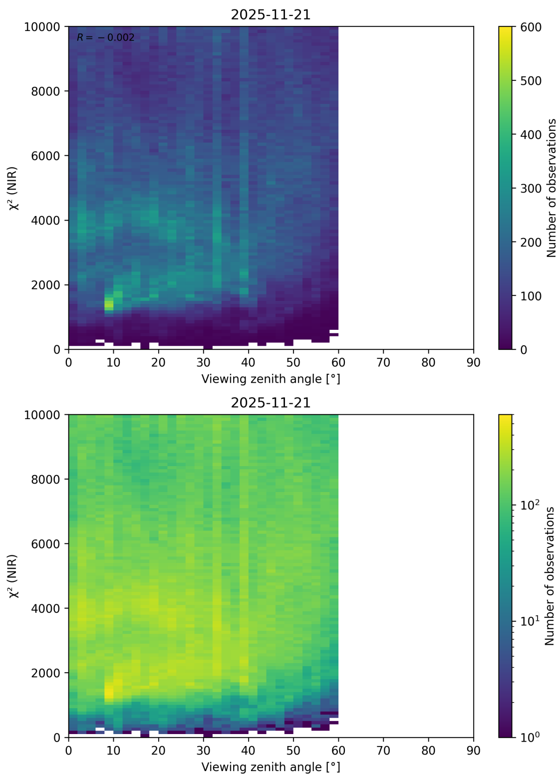
Figure 105: Scatter density plot of “Viewing zenith angle” against “ \chi^2 (NIR)” for 2025-11-20 to 2025-11-22.
