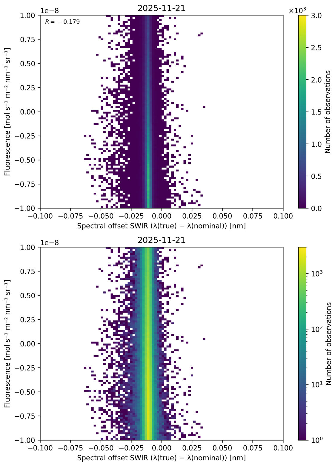
Figure 120: Scatter density plot of “Spectral offset SWIR ( \lambda_{\text{true}} - \lambda_{\text{nominal}} )” against “Fluorescence” for 2025-11-20 to 2025-11-22.
