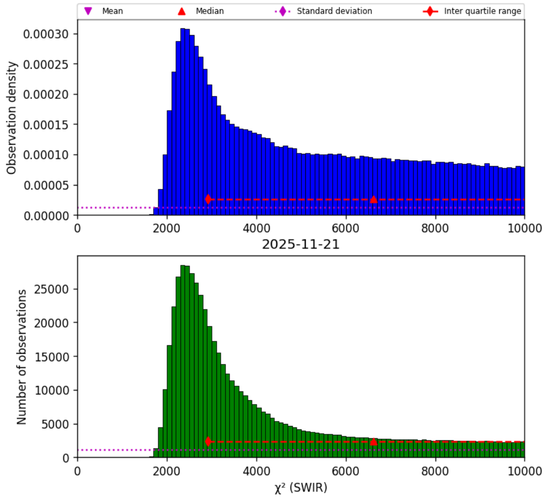
Figure 28: Histogram of “ \chi^2 (SWIR)” for 2025-11-20 to 2025-11-22
