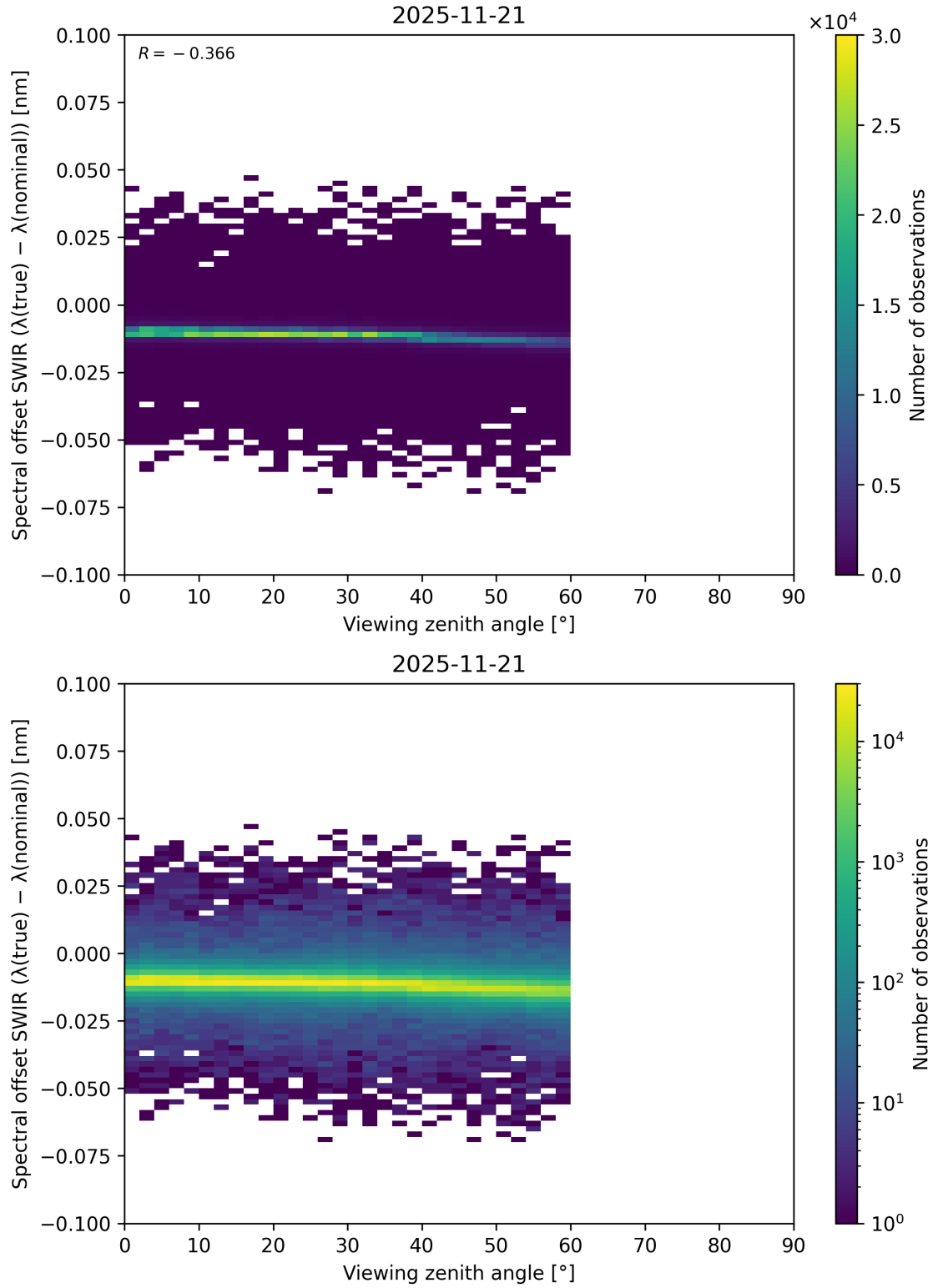
Figure 116: Scatter density plot of “Viewing zenith angle” against “Spectral offset SWIR ( \lambda_{\text{true}} - \lambda_{\text{nominal}} )” for 2025-11-20 to 2025-11-22.
