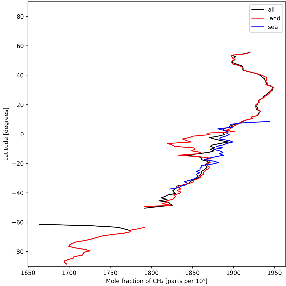
Figure 12: Zonal average of “Mole fraction of CH 4 ” for 2025-11-20 to 2025-11-22.
