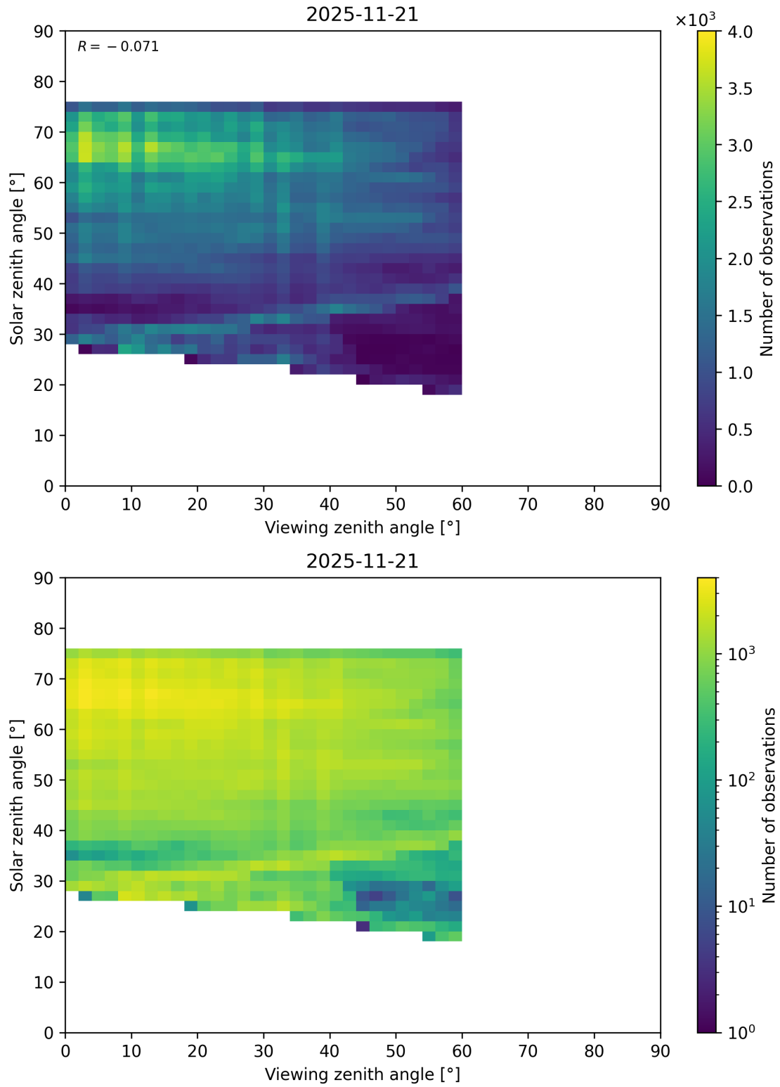
Figure 115: Scatter density plot of “Viewing zenith angle” against “Solar zenith angle” for 2025-11-20 to 2025-11-22.
