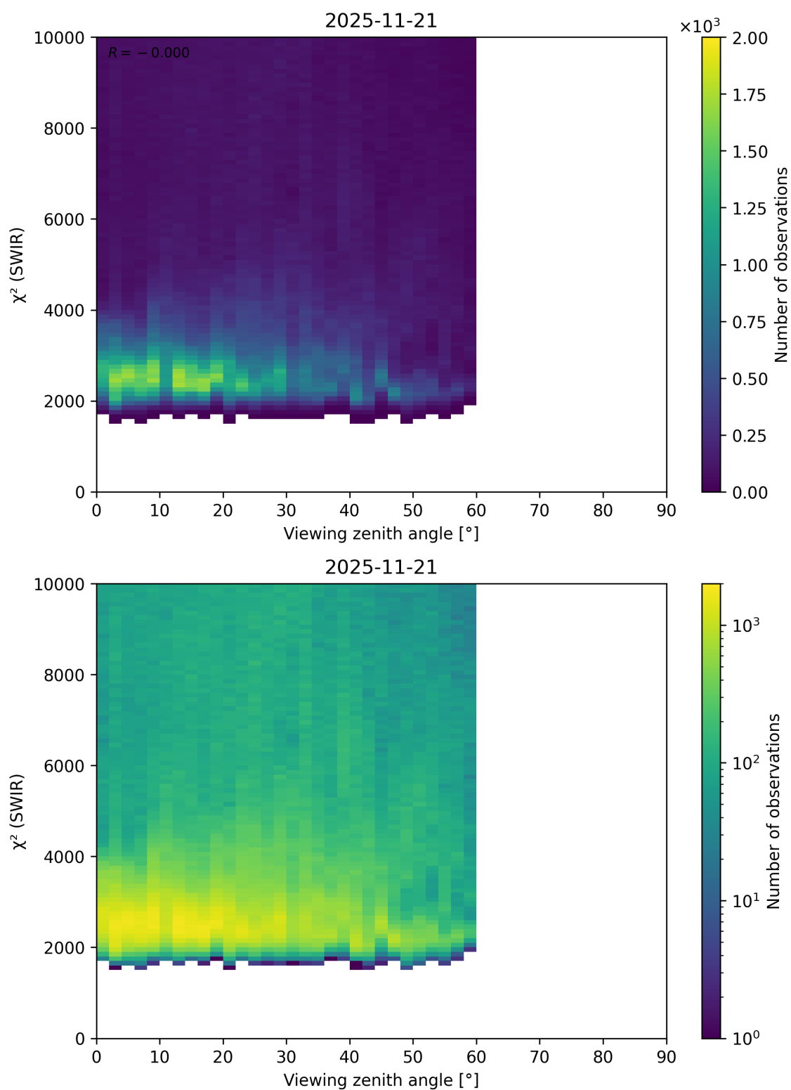
Figure 106: Scatter density plot of “Viewing zenith angle” against “ \chi^2 (SWIR)” for 2025-11-20 to 2025-11-22.
