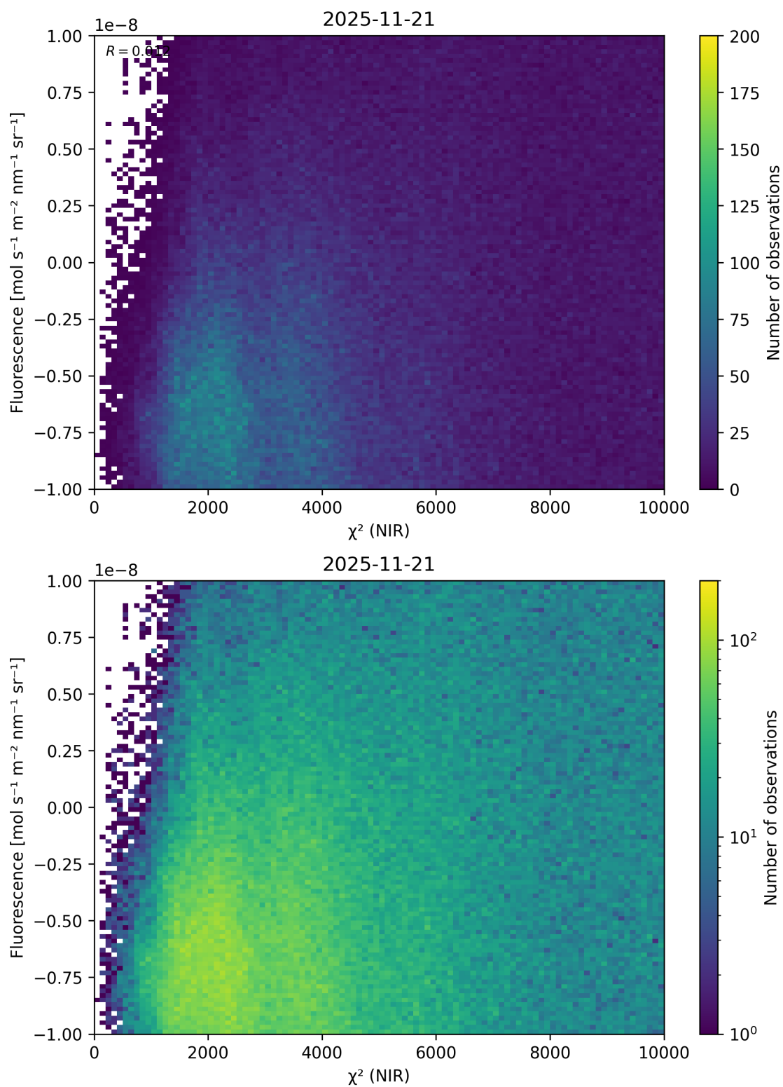
Figure 45: Scatter density plot of “ \chi^2 (NIR)” against “Fluorescence” for 2025-11-20 to 2025-11-22.
