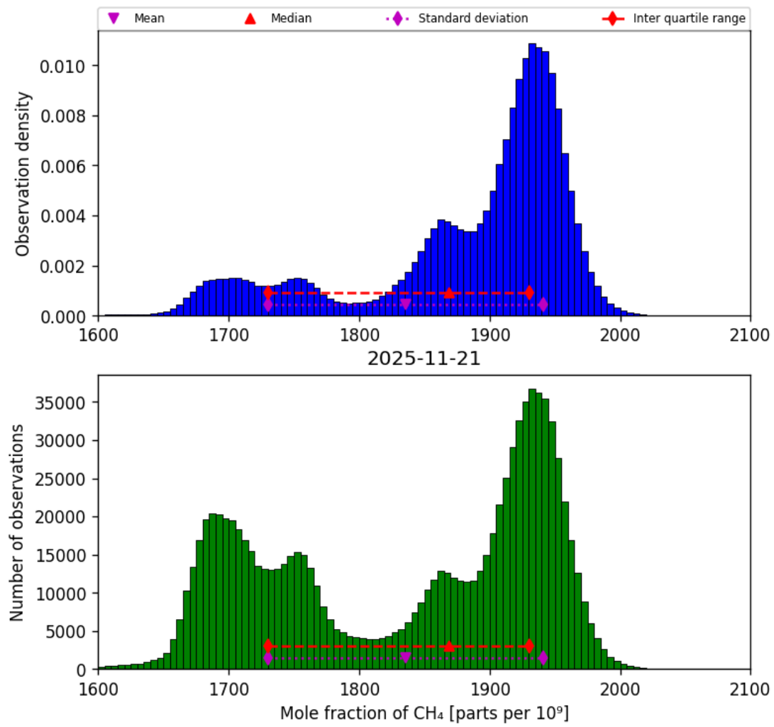
Figure 23: Histogram of “Mole fraction of CH 4 ” for 2025-11-20 to 2025-11-22
