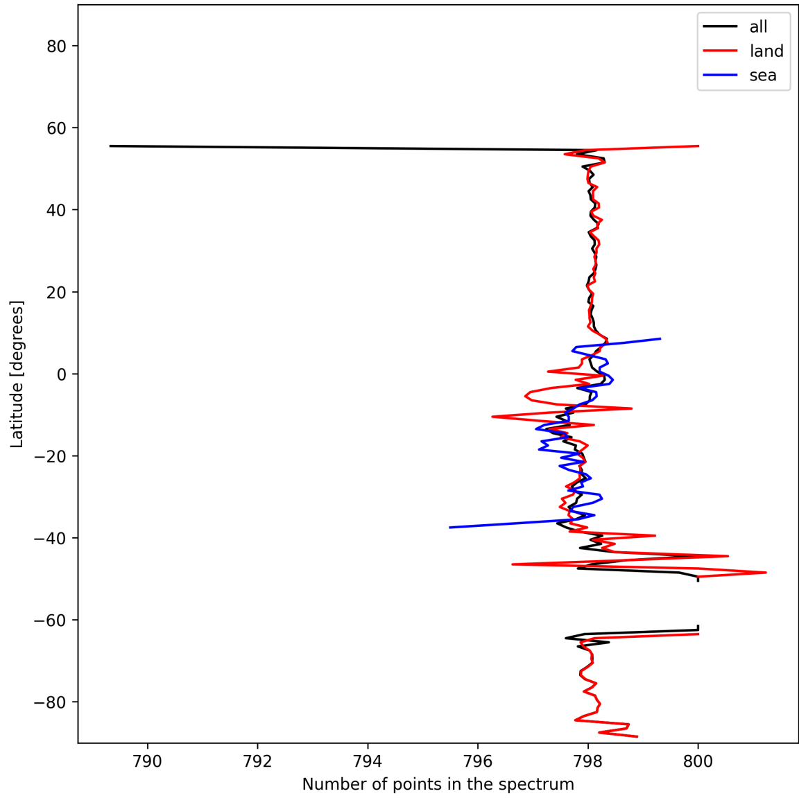
Figure 15: Zonal average of “Number of points in the spectrum” for 2025-11-20 to 2025-11-22.
