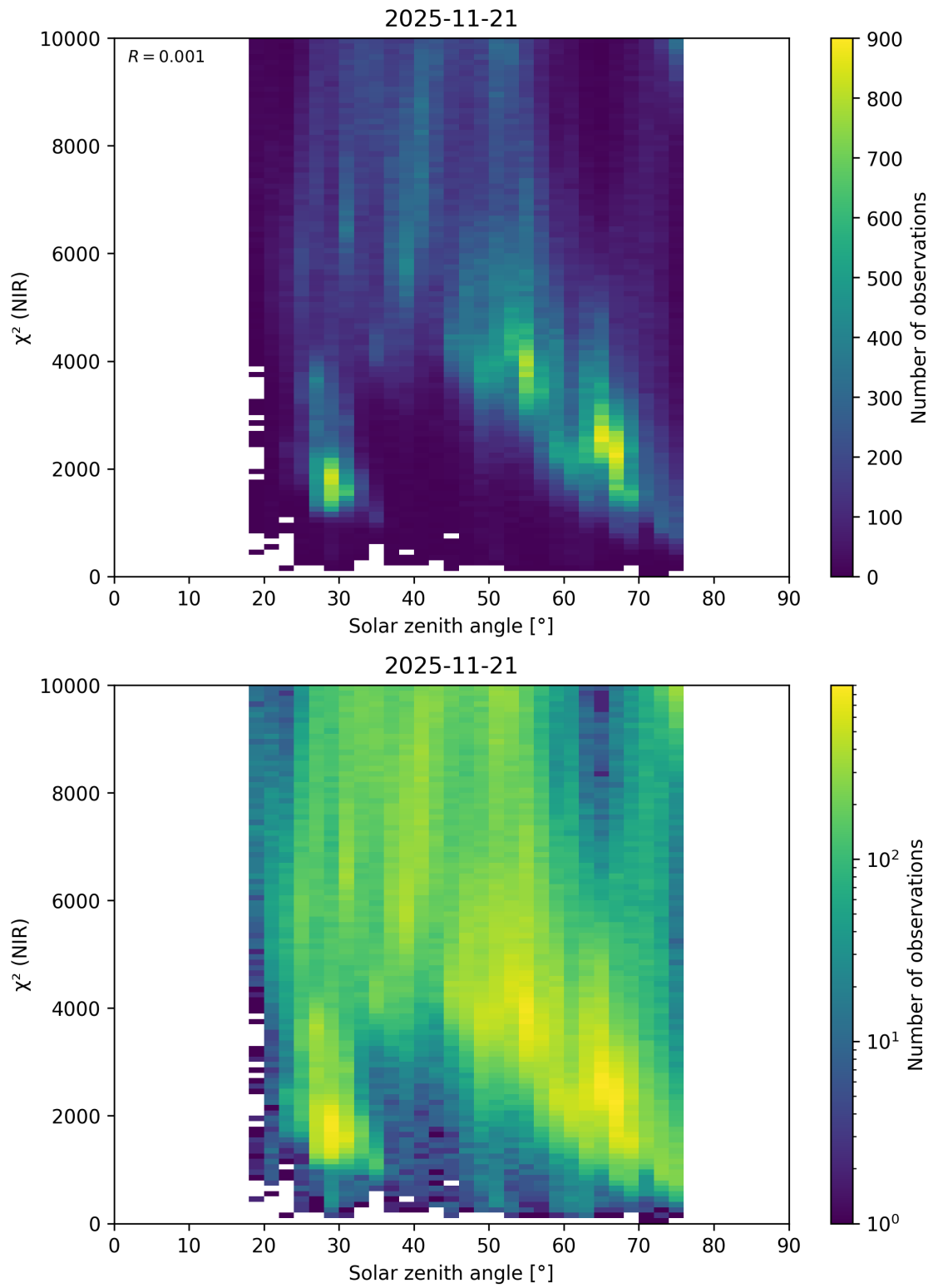
Figure 94: Scatter density plot of “Solar zenith angle” against “ \chi^2 (NIR)” for 2025-11-20 to 2025-11-22.
