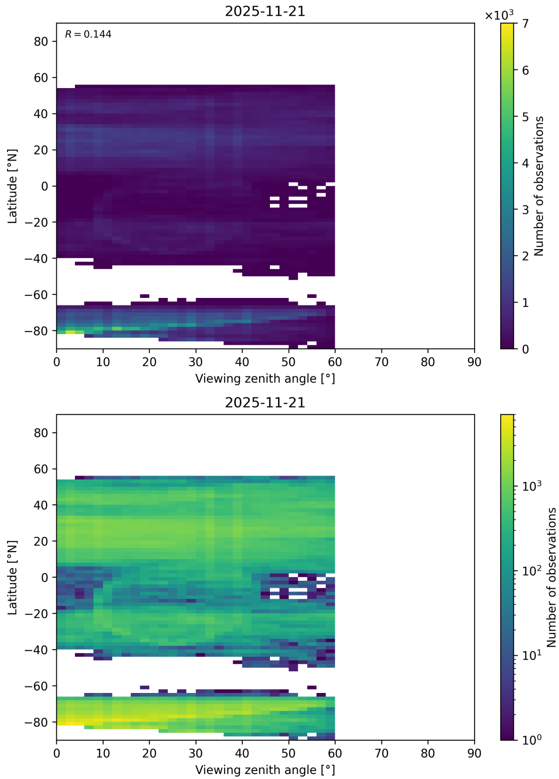
Figure 109: Scatter density plot of “Viewing zenith angle” against “Latitude” for 2025-11-20 to 2025-11-22.
