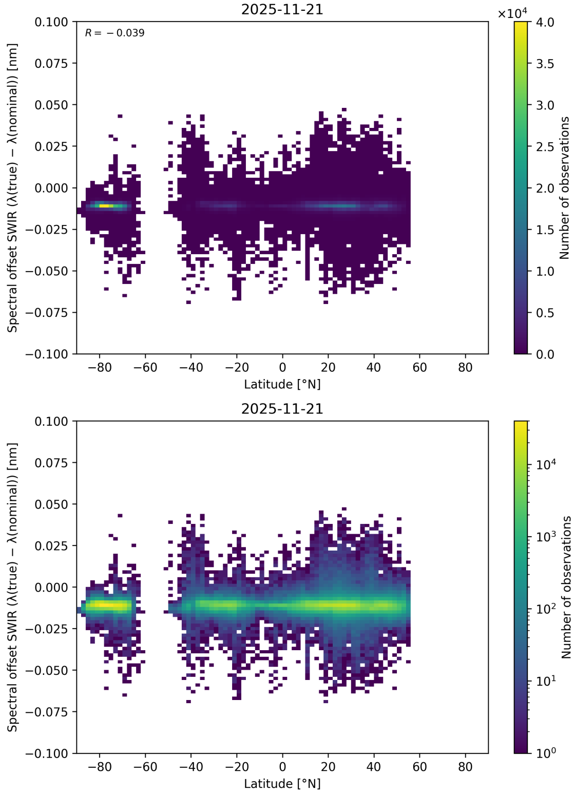
Figure 62: Scatter density plot of “Latitude” against “Spectral offset SWIR ( \lambda_{\text{true}} - \lambda_{\text{nominal}} )” for 2025-11-20 to 2025-11-22.
