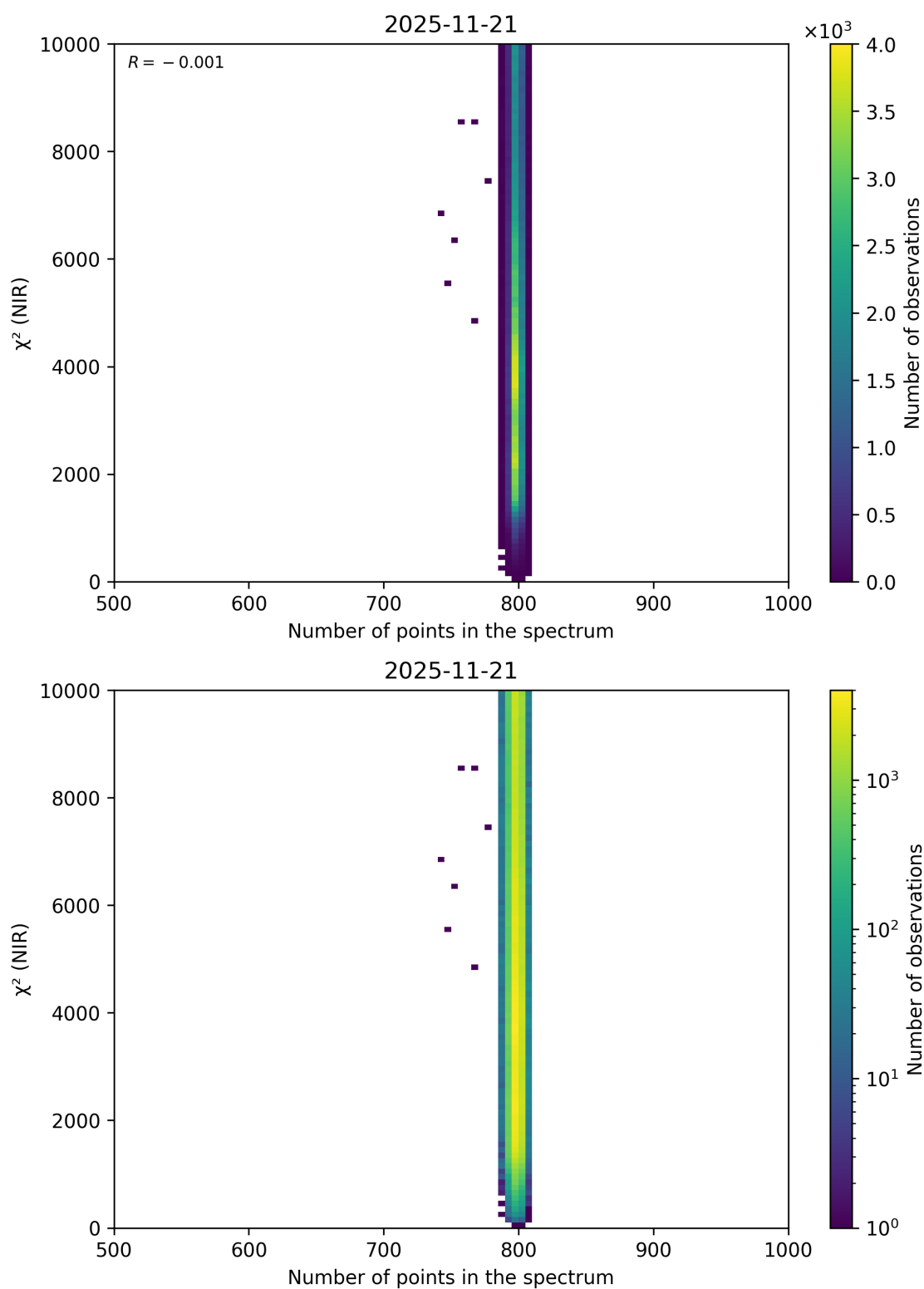
Figure 88: Scatter density plot of “Number of points in the spectrum” against “ \chi^2 (NIR)” for 2025-11-20 to 2025-11-22.
