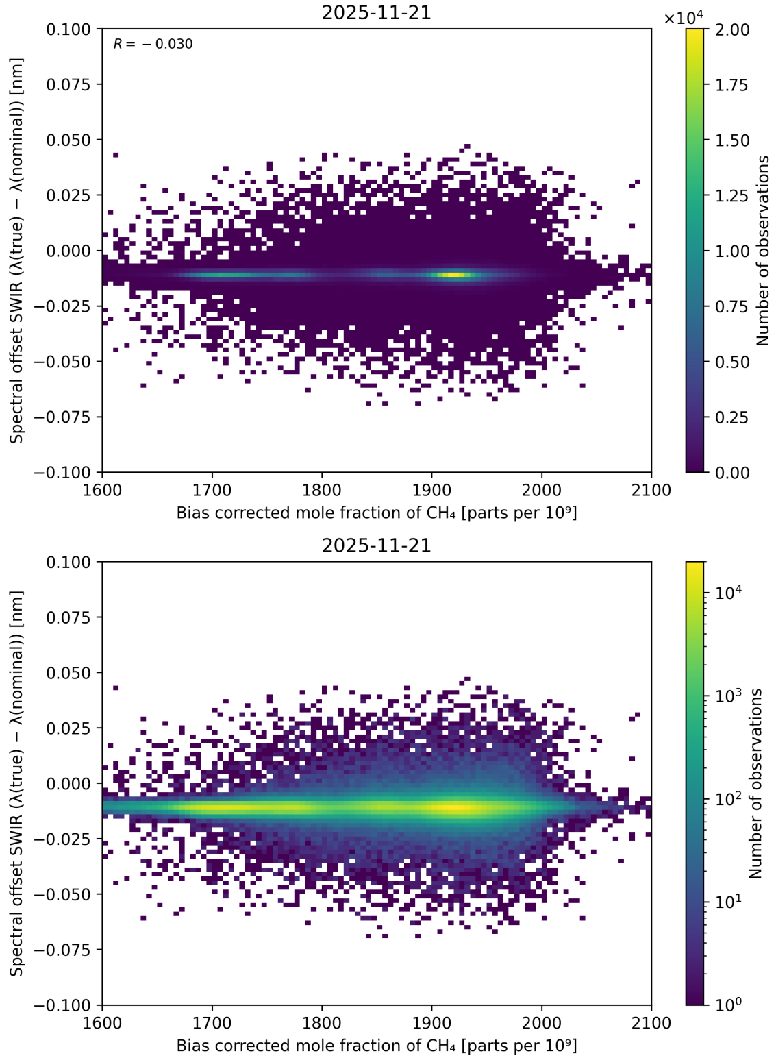
Figure 69: Scatter density plot of “Bias corrected mole fraction of \text{CH}_4 ” against “Spectral offset SWIR ( \lambda_{\text{true}} - \lambda_{\text{nominal}} )” for 2025-11-20 to 2025-11-22.
