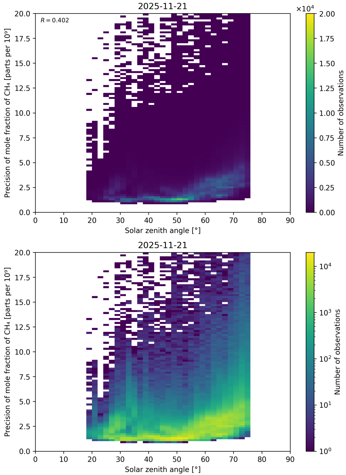
Figure 101: Scatter density plot of “Solar zenith angle” against “Precision of mole fraction of \text{CH}_4 ” for 2025-11-20 to 2025-11-22.
