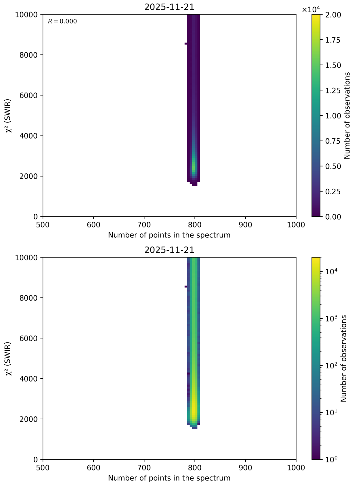
Figure 89: Scatter density plot of “Number of points in the spectrum” against “ \chi^2 (SWIR)” for 2025-11-20 to 2025-11-22.
