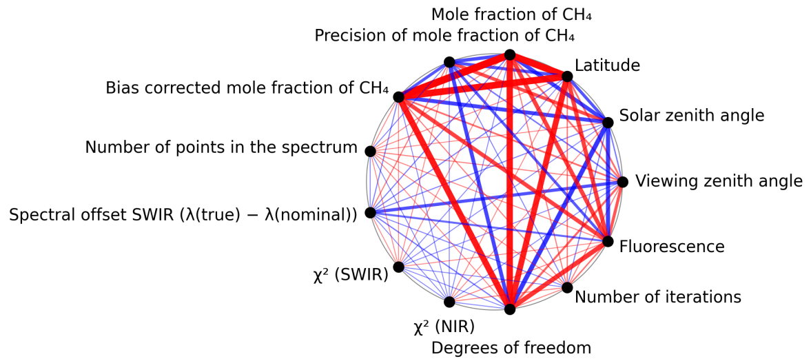
Figure 1: Map of correlation graph for 2025-11-20 to 2025-11-22.
