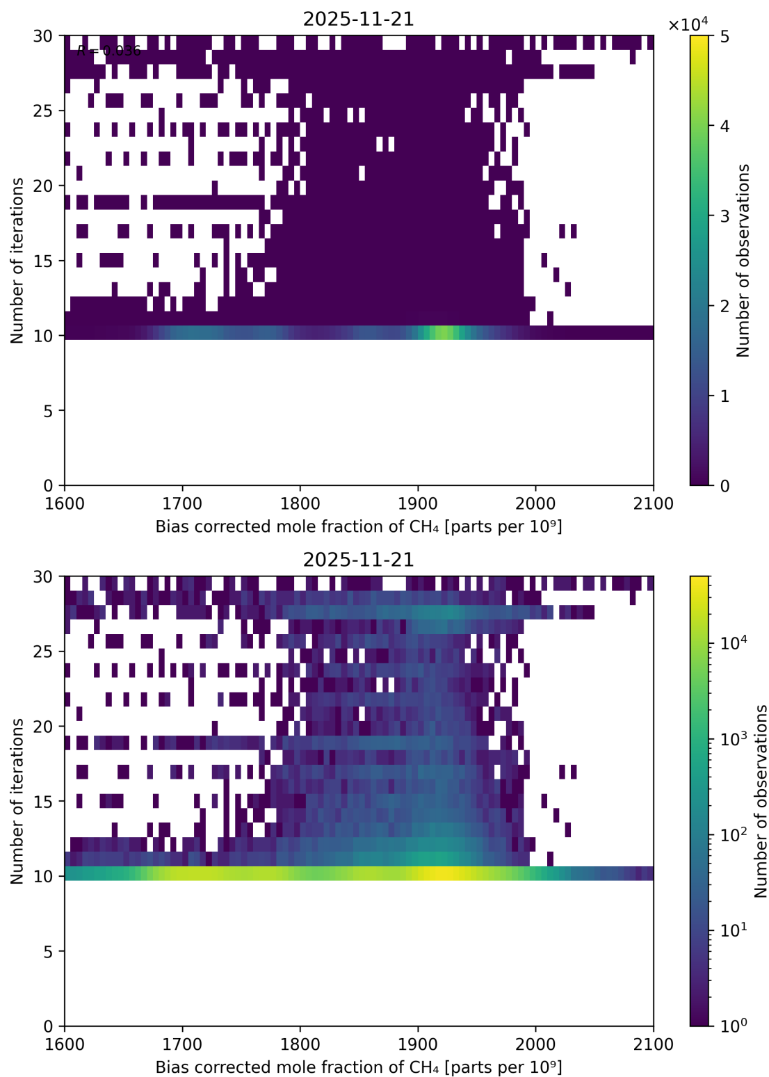
Figure 67: Scatter density plot of “Bias corrected mole fraction of CH 4 ” against “Number of iterations” for 2025-11-20 to 2025-11-22.
