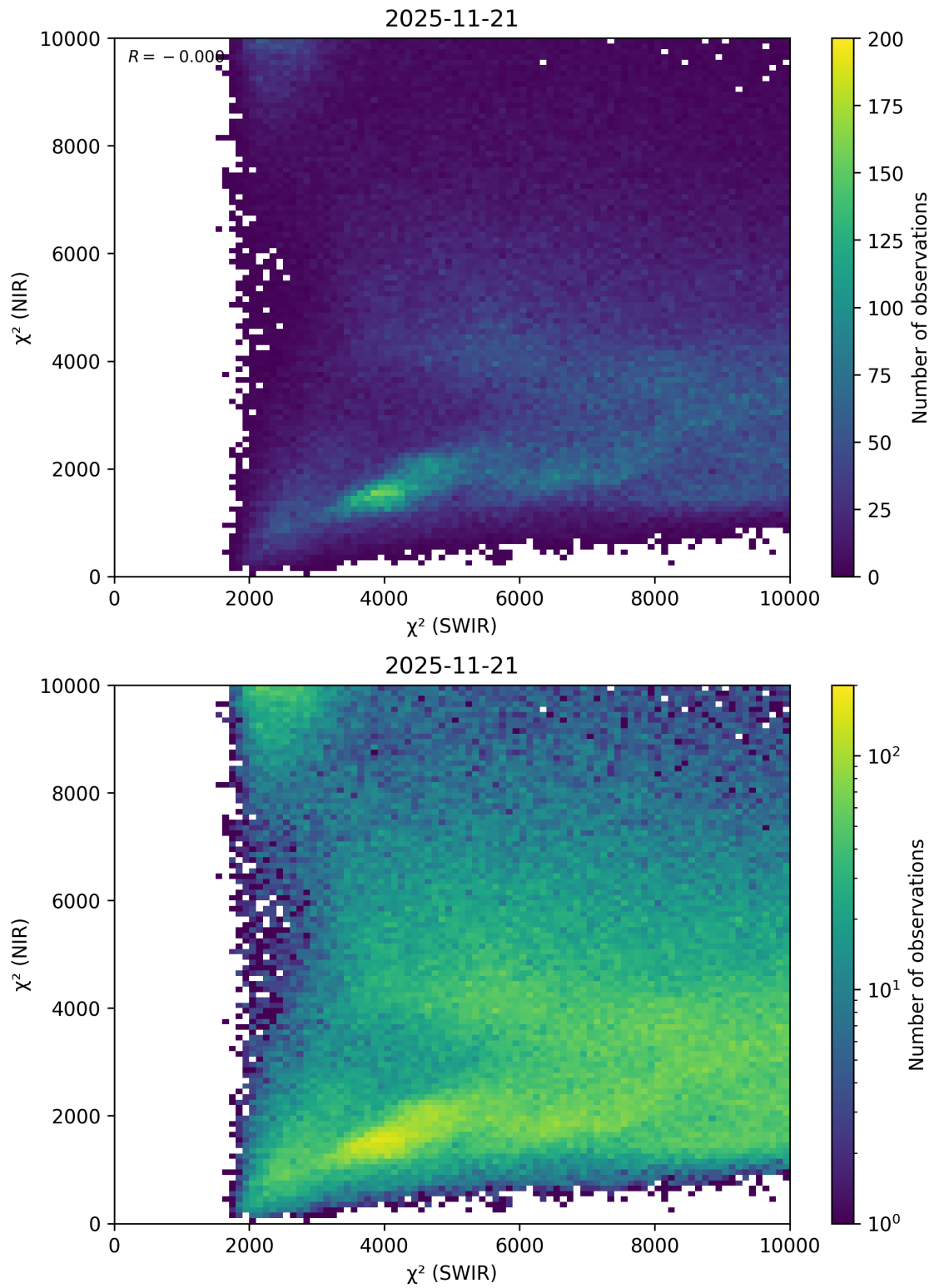
Figure 47: Scatter density plot of “ \chi^2 (SWIR)” against “ \chi^2 (NIR)” for 2025-11-20 to 2025-11-22.
