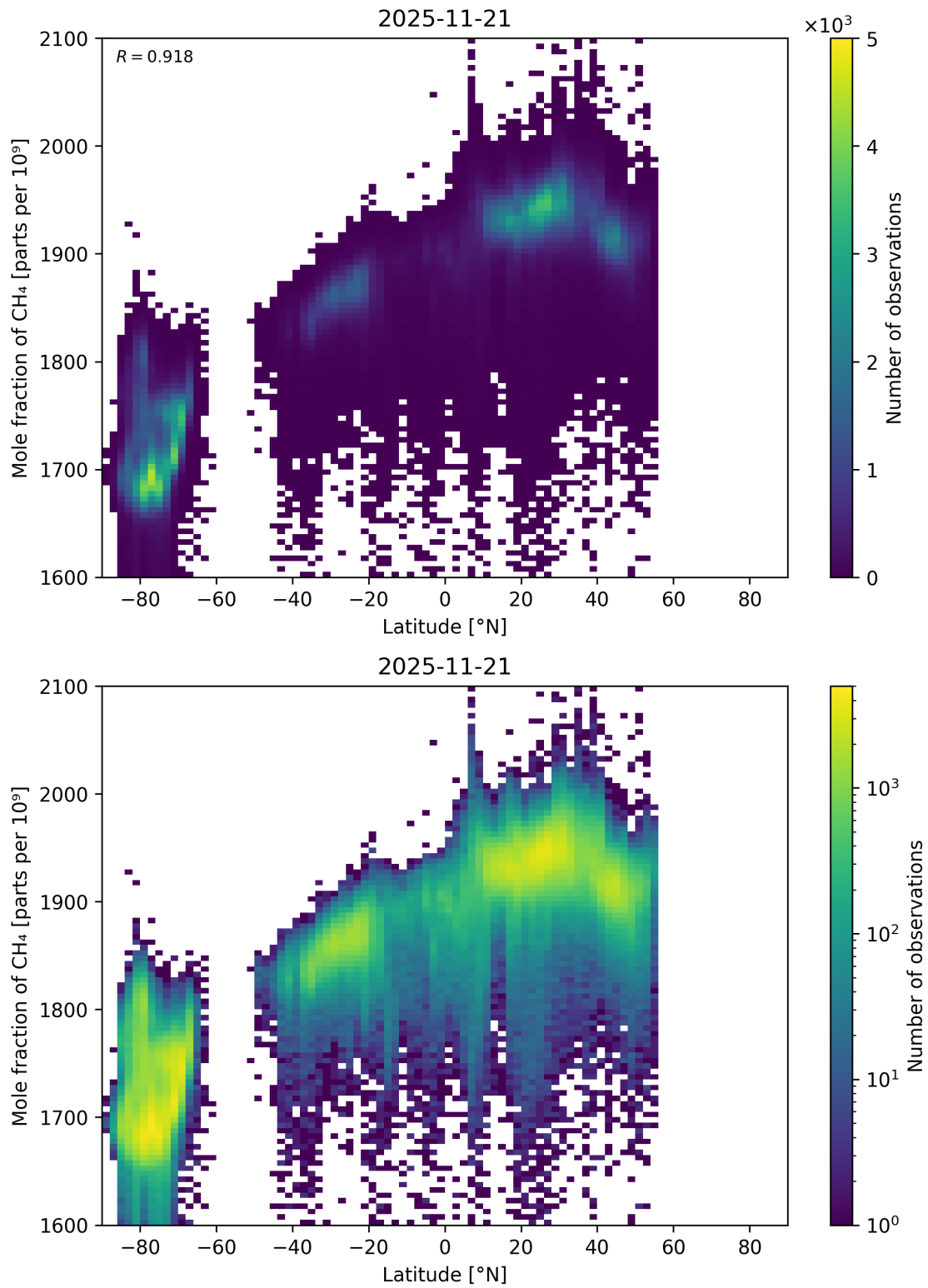
Figure 57: Scatter density plot of “Latitude” against “Mole fraction of CH 4 ” for 2025-11-20 to 2025-11-22.
