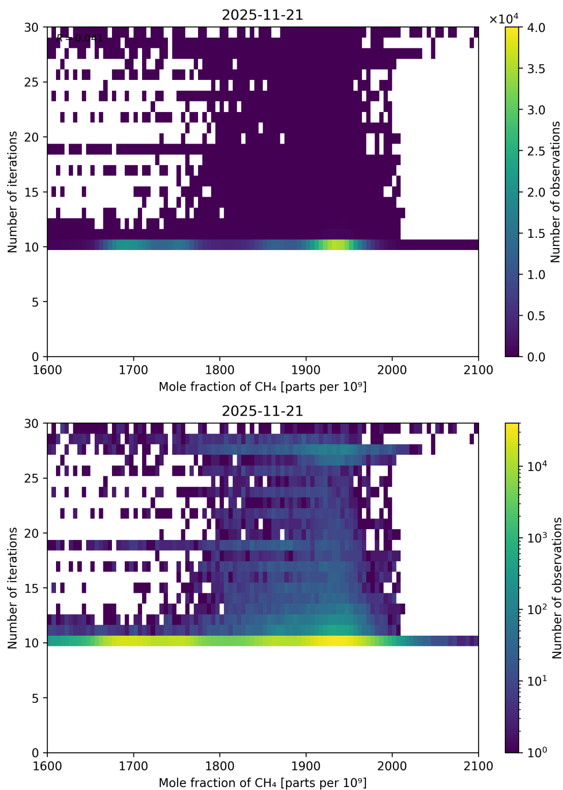
Figure 76: Scatter density plot of “Mole fraction of CH 4 ” against “Number of iterations” for 2025-11-20 to 2025-11-22.
