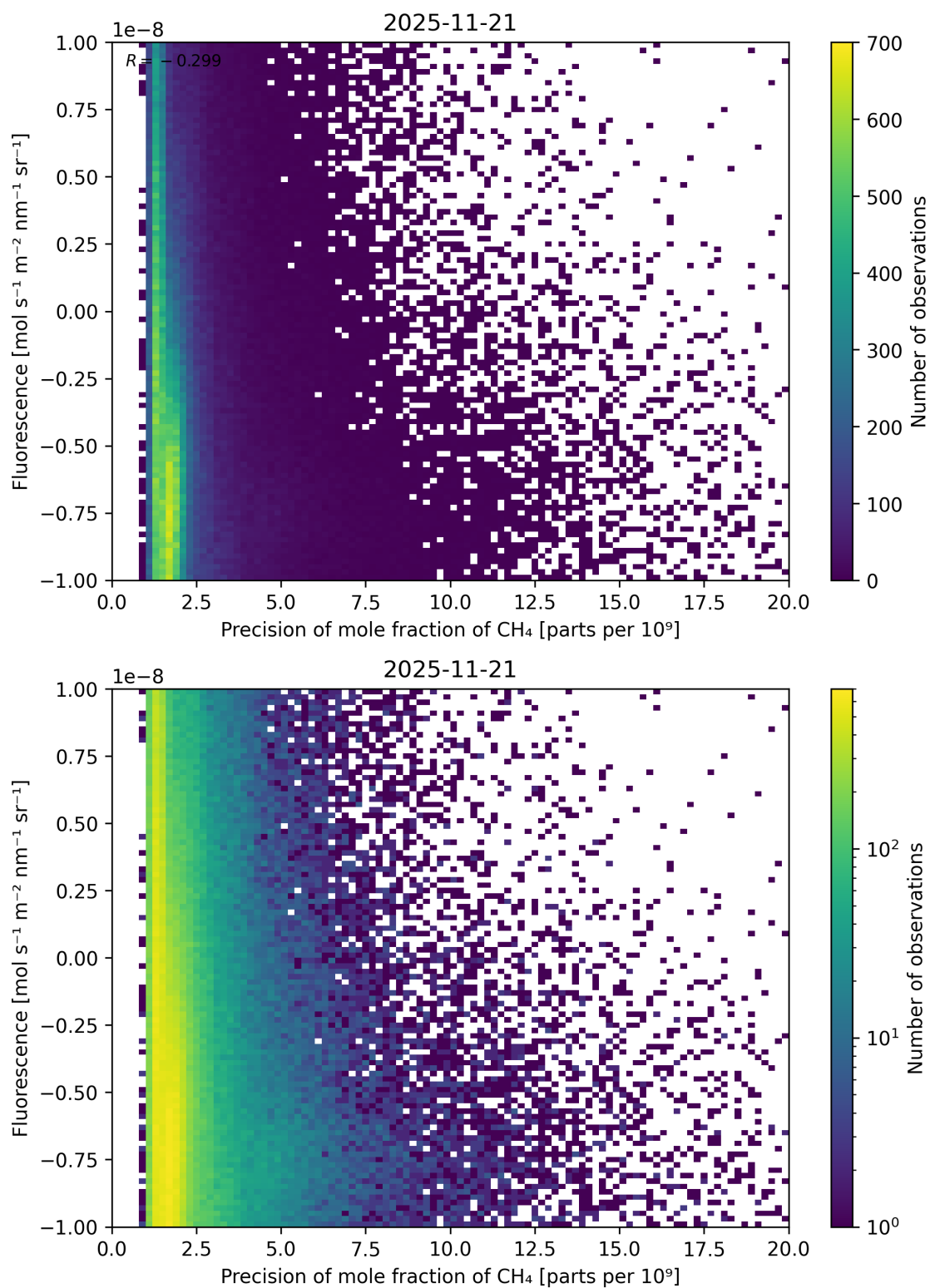
Figure 81: Scatter density plot of “Precision of mole fraction of \text{CH}_4 ” against “Fluorescence” for 2025-11-20 to 2025-11-22.
