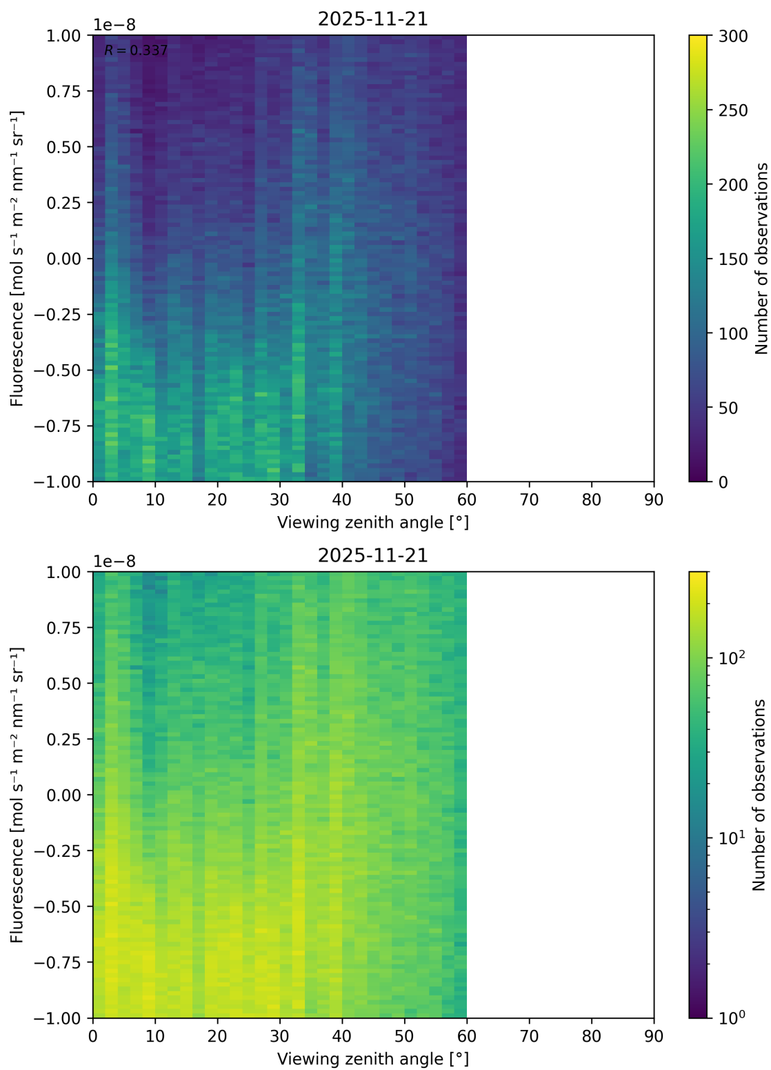
Figure 108: Scatter density plot of “Viewing zenith angle” against “Fluorescence” for 2025-11-20 to 2025-11-22.
