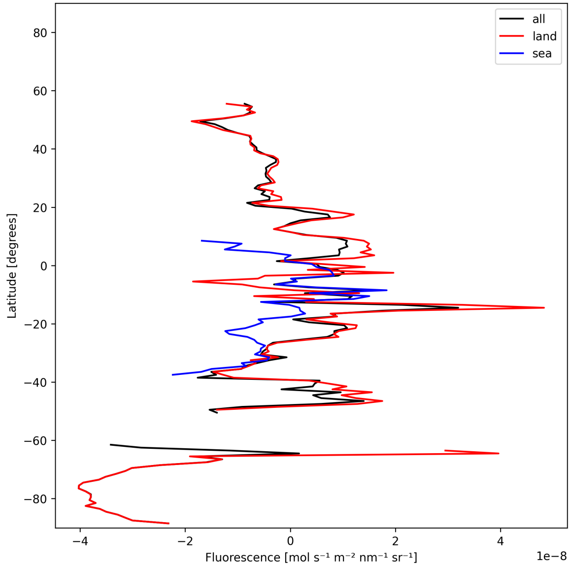
Figure 21: Zonal average of “Fluorescence” for 2025-11-20 to 2025-11-22.
