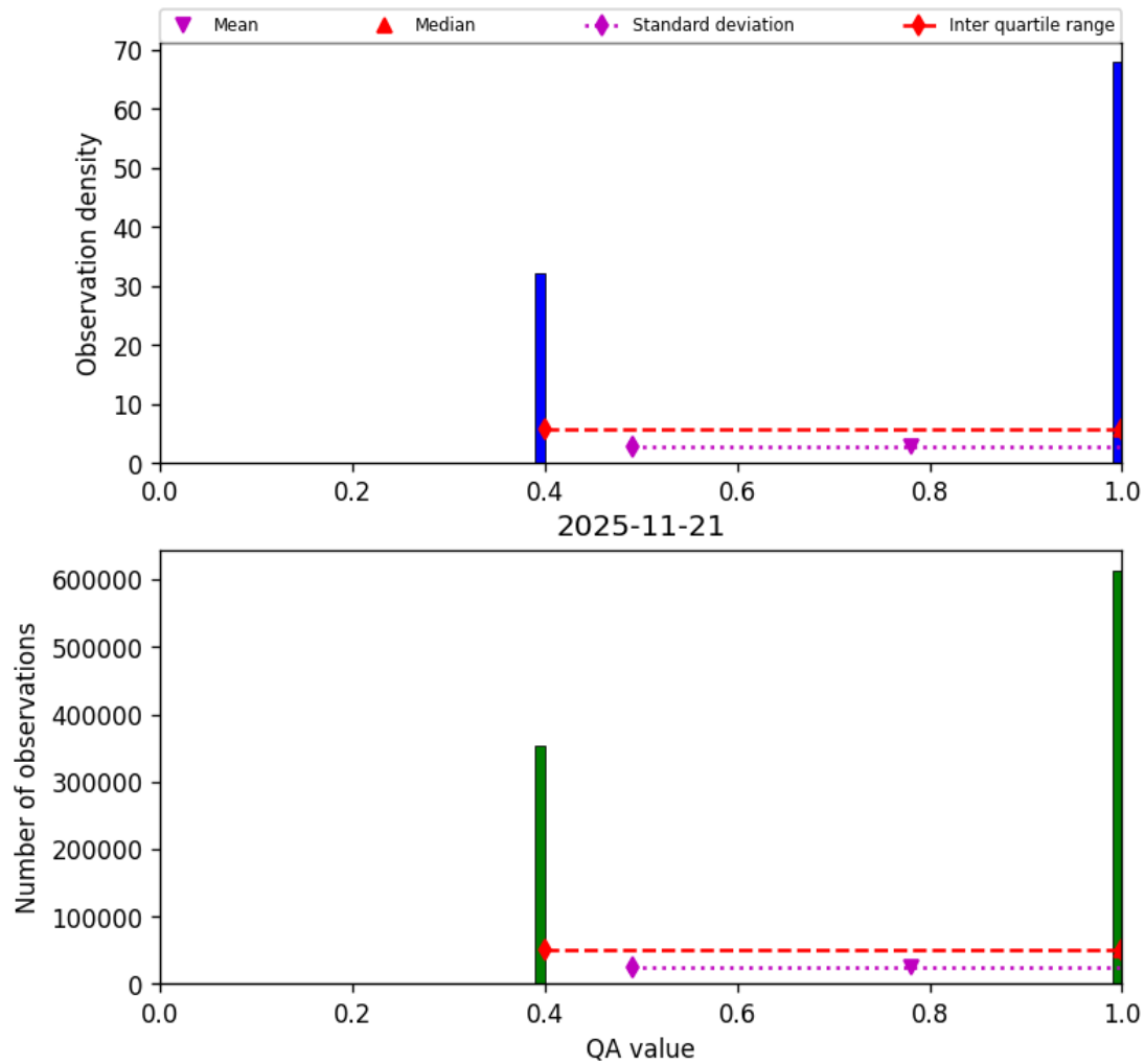
Figure 22: Histogram of “QA value” for 2025-11-20 to 2025-11-22
