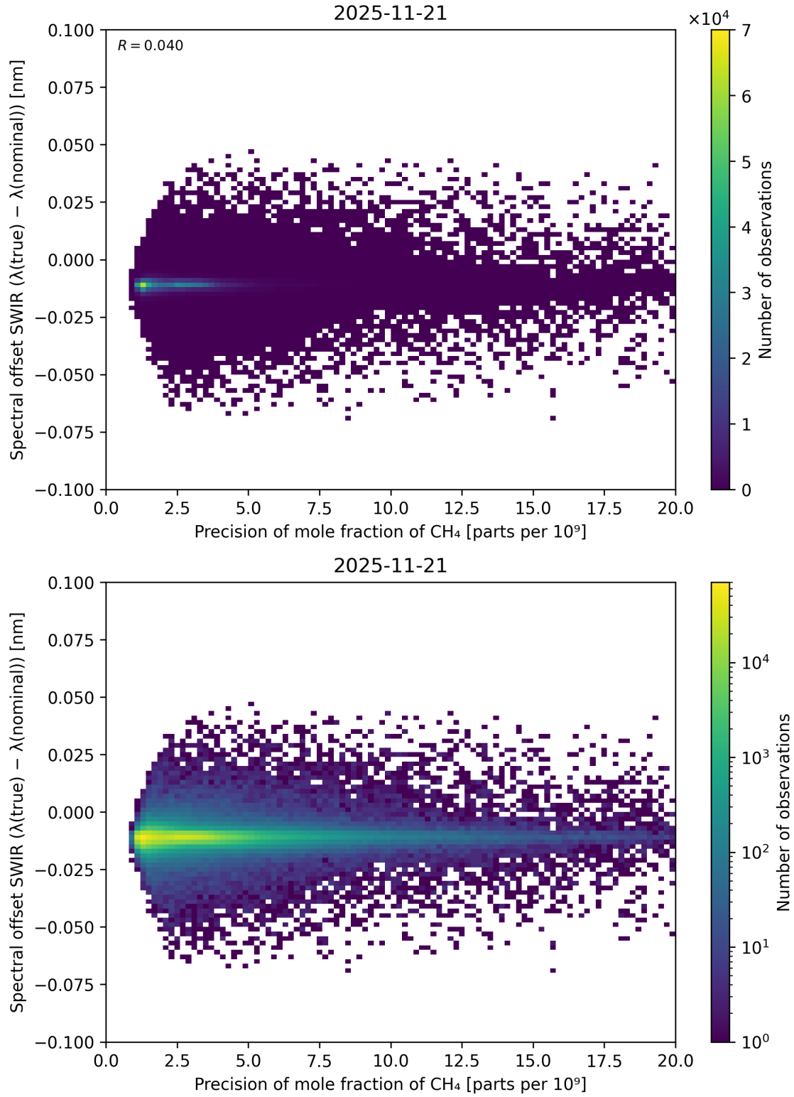
Figure 85: Scatter density plot of “Precision of mole fraction of CH 4 ” against “Spectral offset SWIR ( \lambda_{\text{true}} - \lambda_{\text{nominal}} )” for 2025-11-20 to 2025-11-22.
