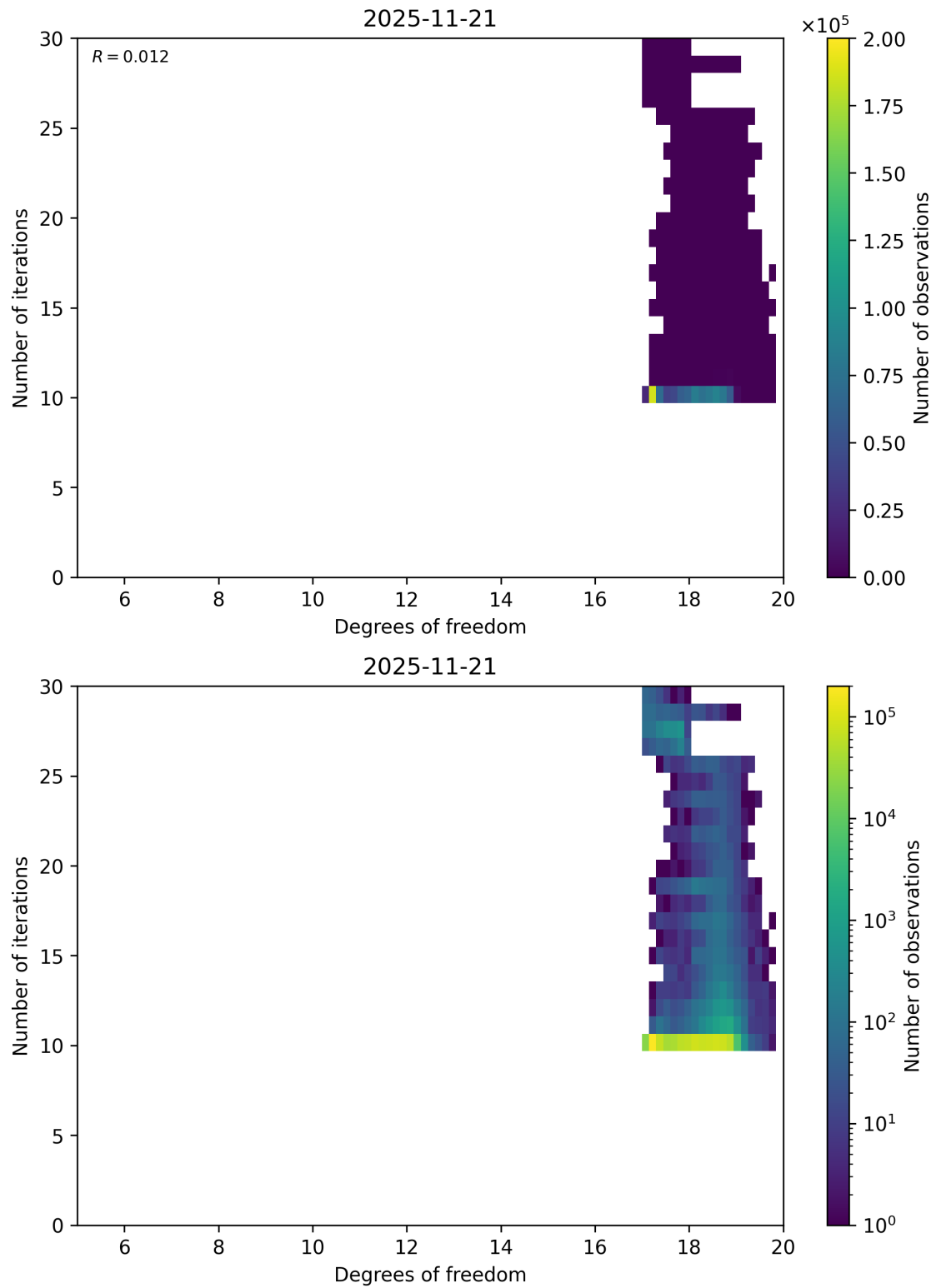
Figure 52: Scatter density plot of “Degrees of freedom” against “Number of iterations” for 2025-11-20 to 2025-11-22.
