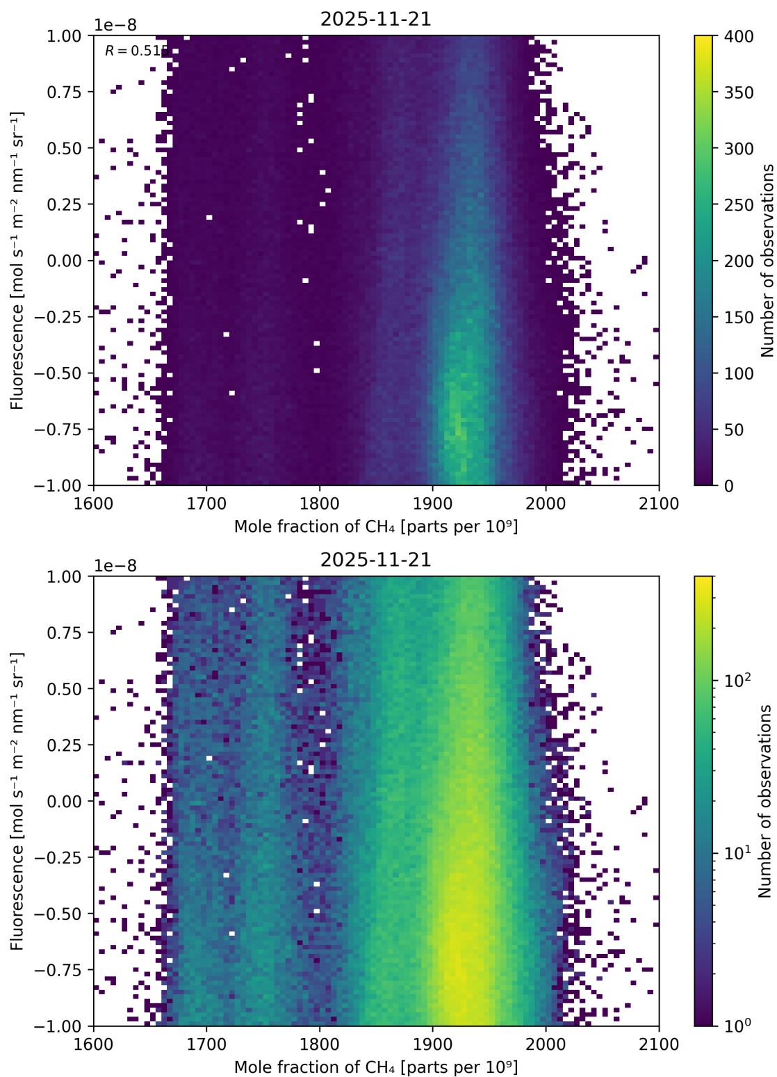
Figure 73: Scatter density plot of “Mole fraction of CH 4 ” against “Fluorescence” for 2025-11-20 to 2025-11-22.
