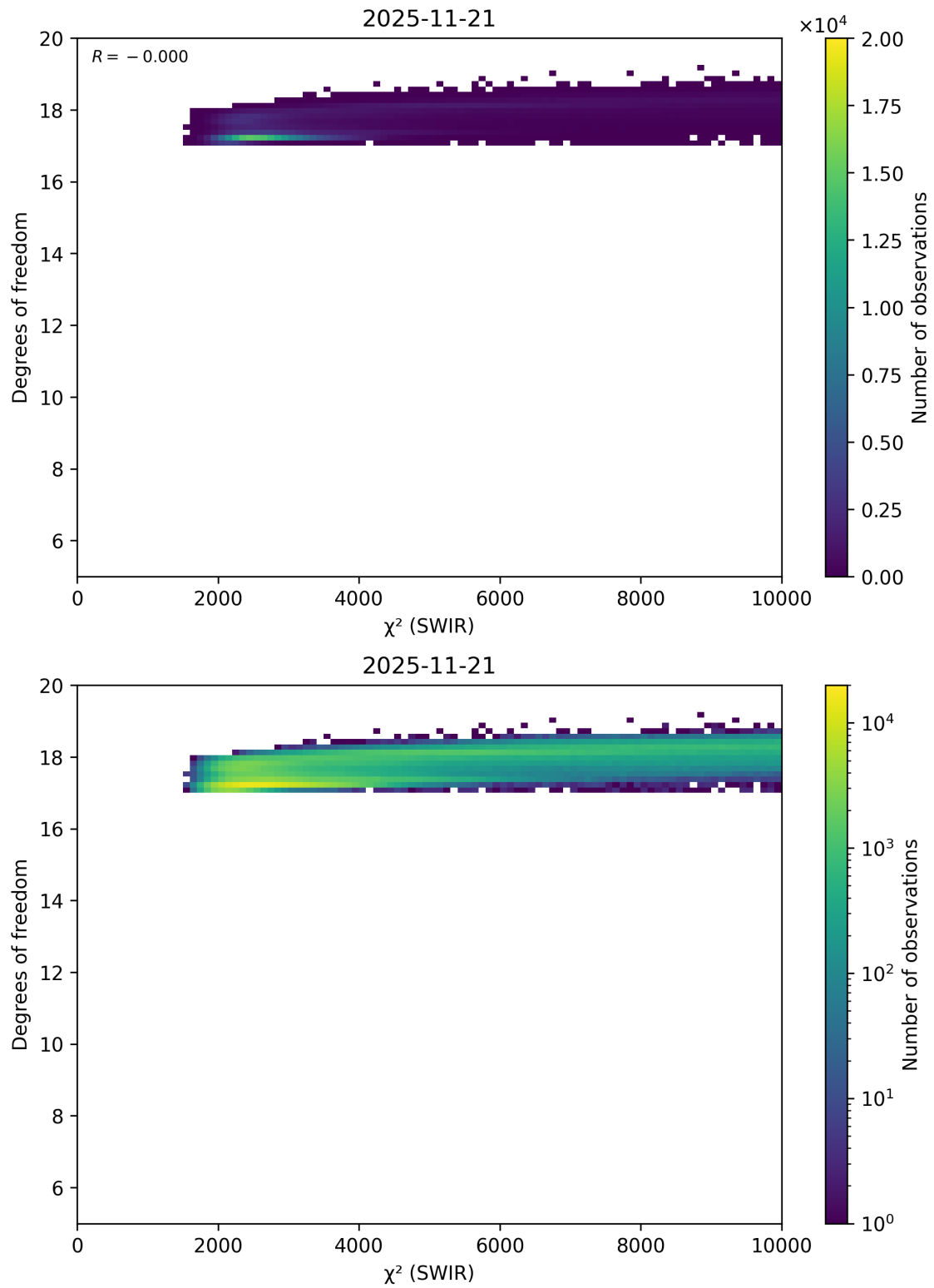
Figure 48: Scatter density plot of “ \chi^2 (SWIR)” against “Degrees of freedom” for 2025-11-20 to 2025-11-22.
