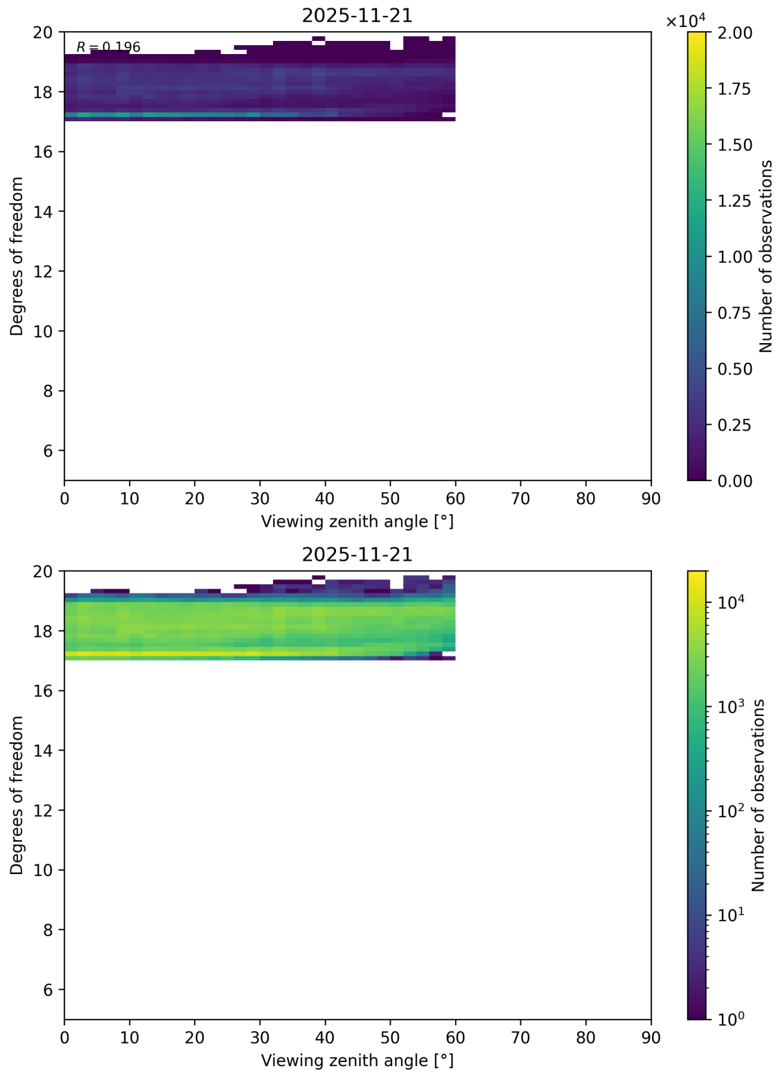
Figure 107: Scatter density plot of “Viewing zenith angle” against “Degrees of freedom” for 2025-11-20 to 2025-11-22.
