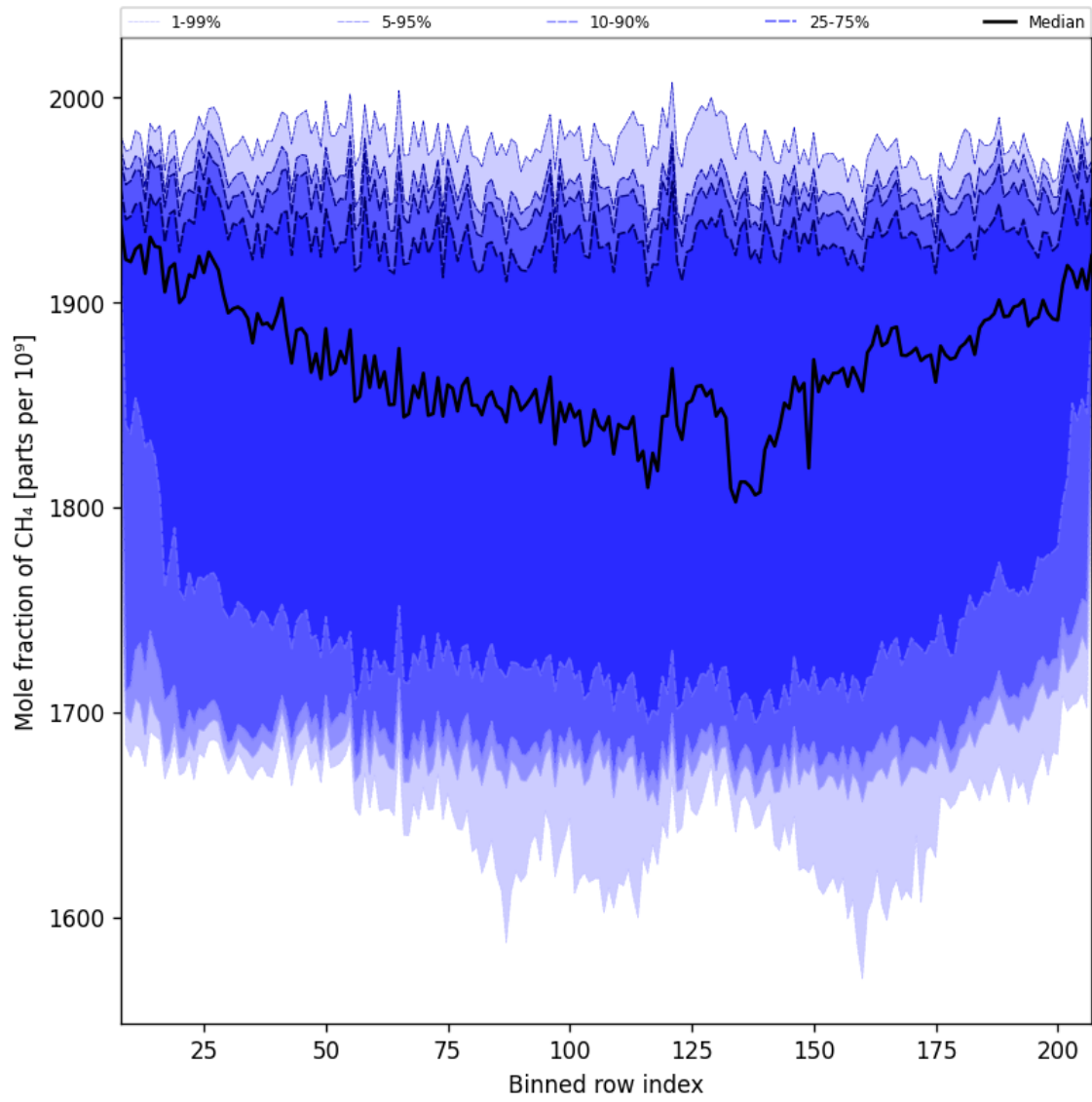
Figure 34: Along track statistics of “Mole fraction of CH 4 ” for 2025-11-20 to 2025-11-22
