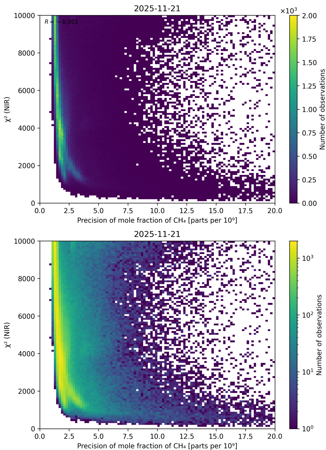
Figure 78: Scatter density plot of “Precision of mole fraction of \text{CH}_4 ” against “ \chi^2 (NIR)” for 2025-11-20 to 2025-11-22.
