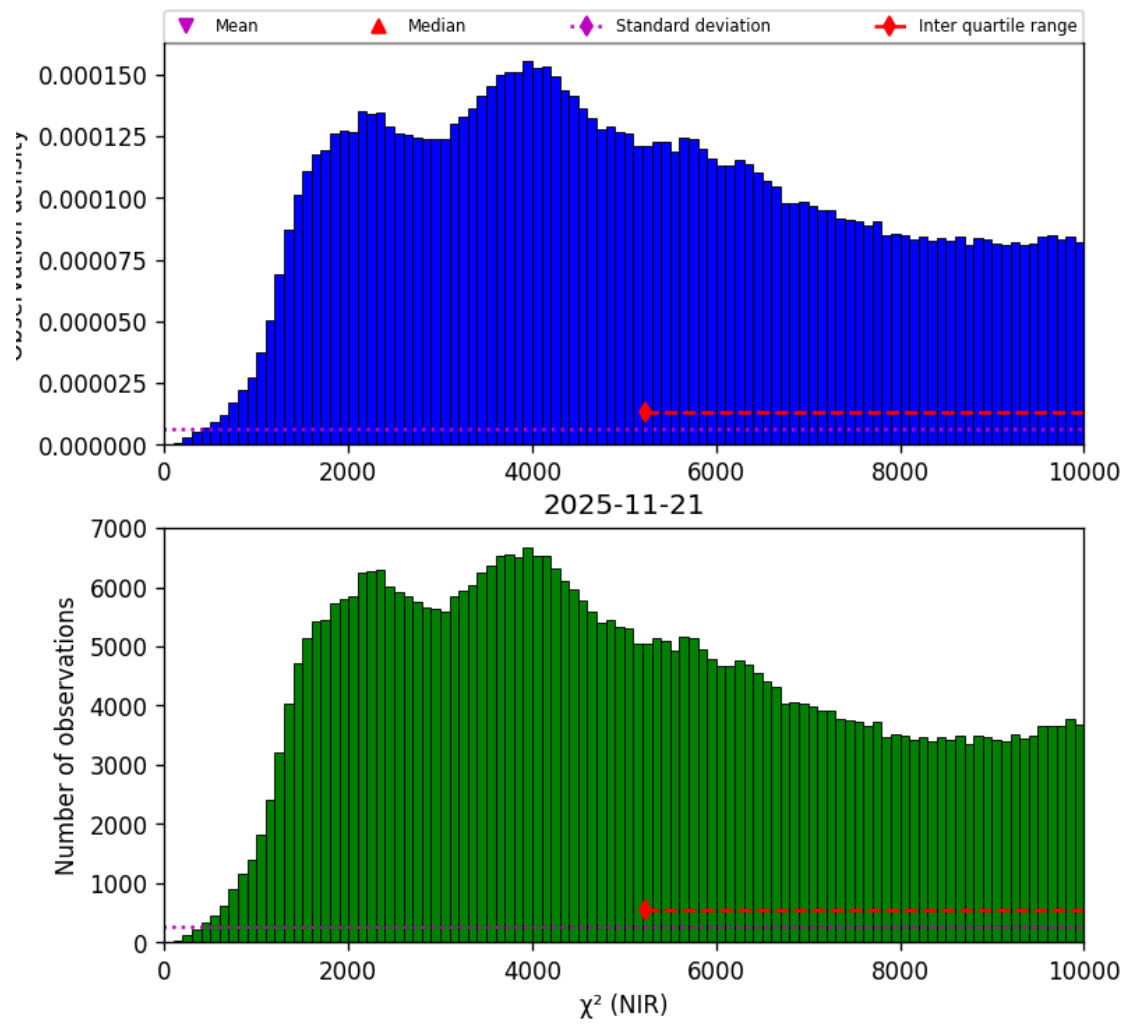
Figure 29: Histogram of “ \chi^2 (NIR)” for 2025-11-20 to 2025-11-22
