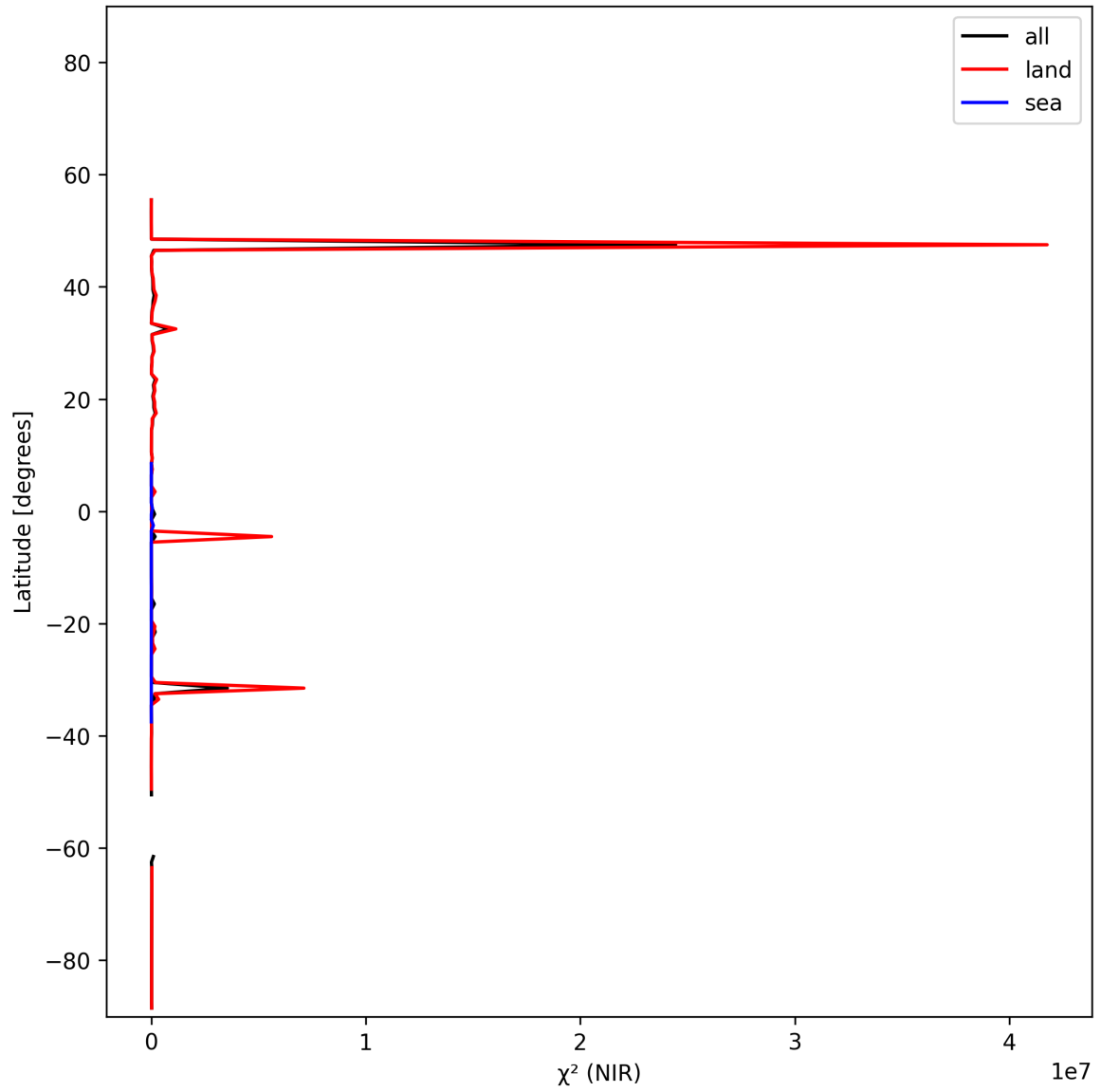
Figure 18: Zonal average of “ \chi^2 (NIR)” for 2025-11-20 to 2025-11-22.
