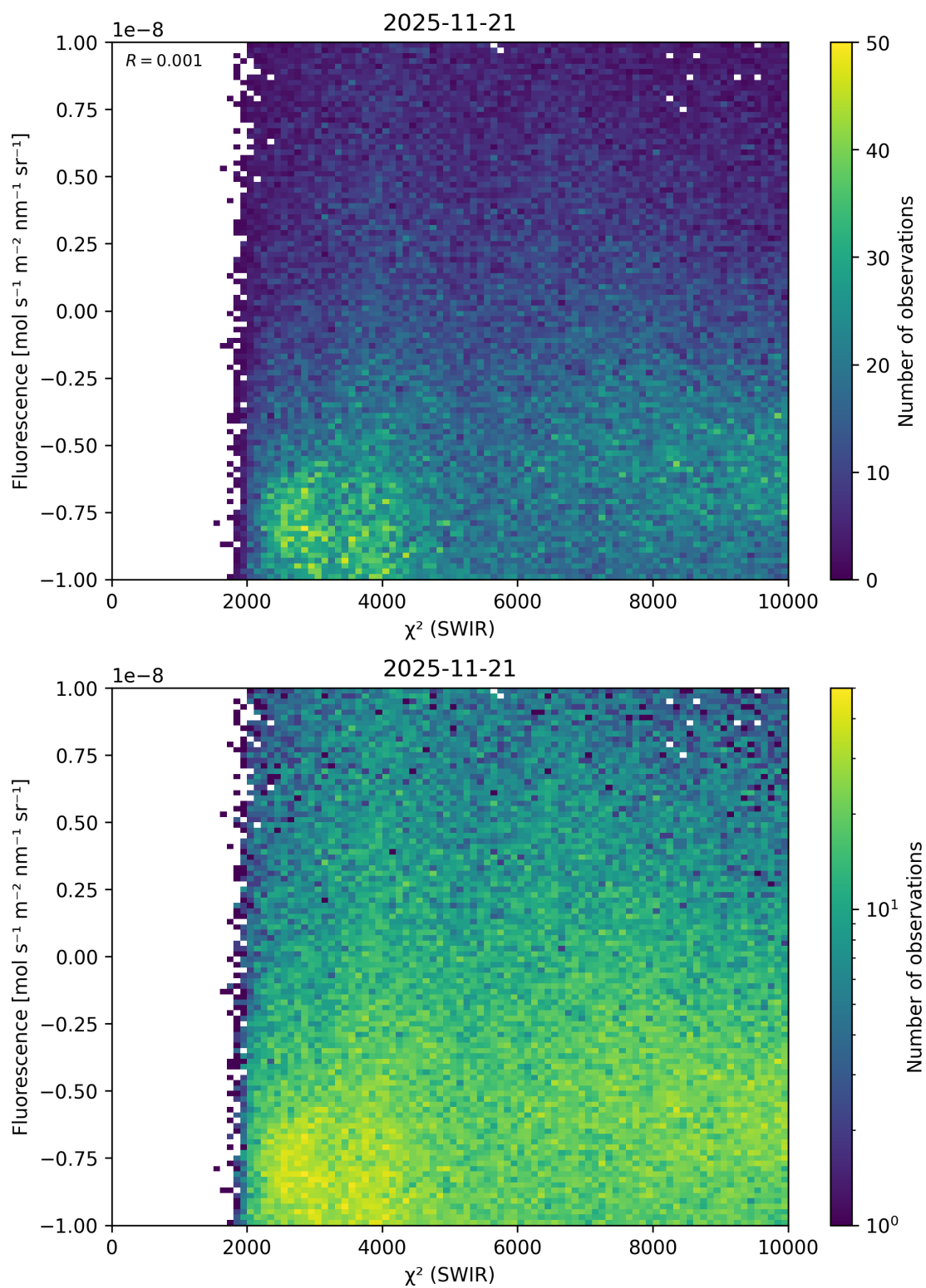
Figure 49: Scatter density plot of “ \chi^2 (SWIR)” against “Fluorescence” for 2025-11-20 to 2025-11-22.
