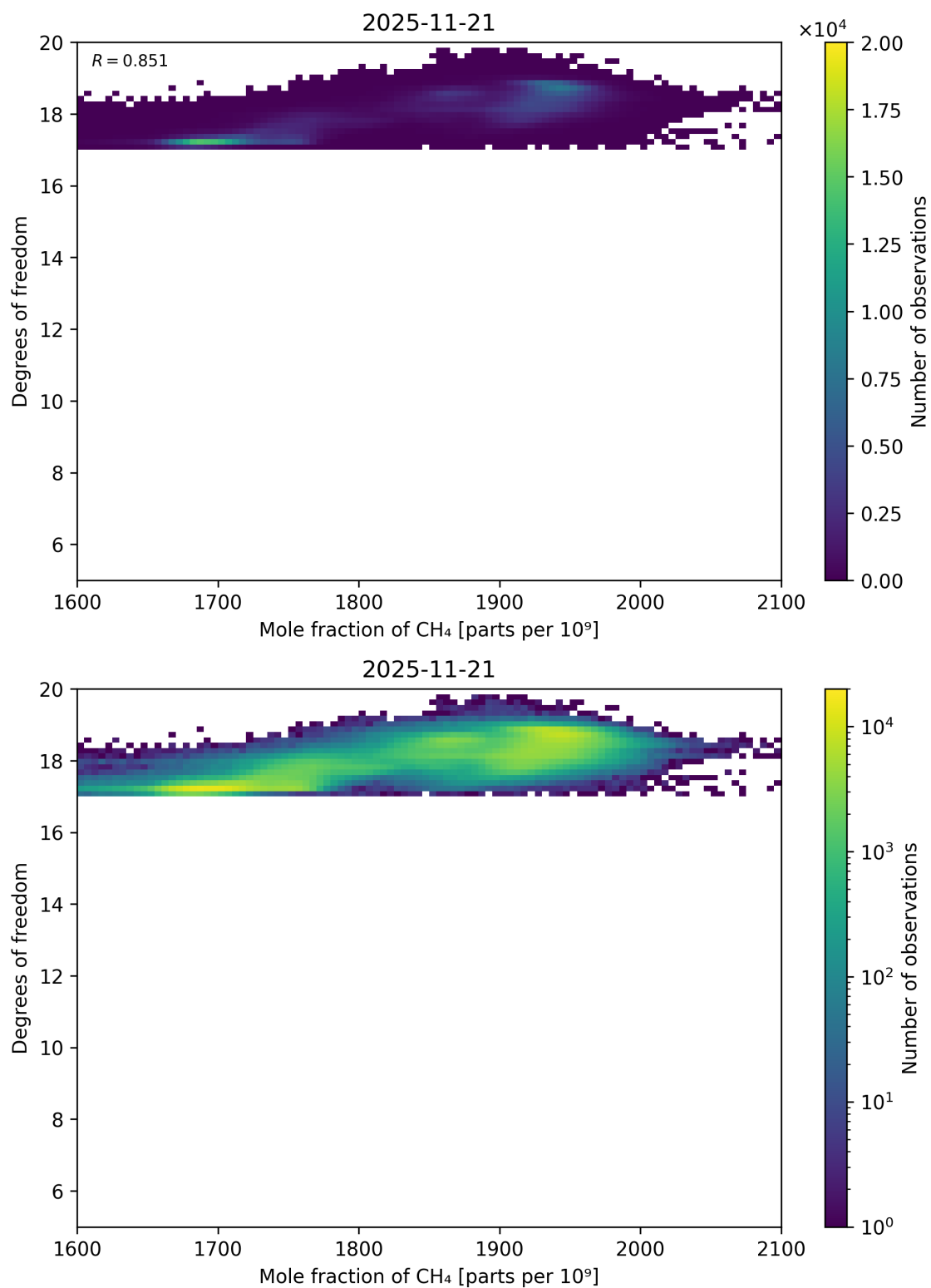
Figure 72: Scatter density plot of “Mole fraction of CH 4 ” against “Degrees of freedom” for 2025-11-20 to 2025-11-22.
