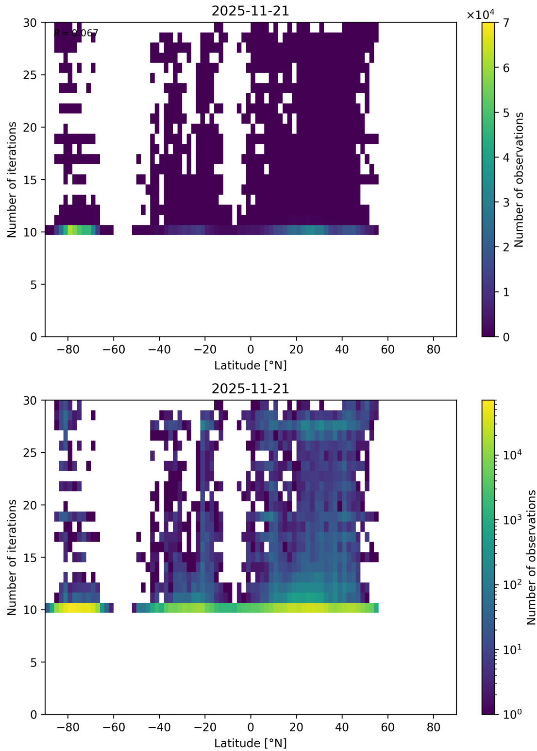
Figure 60: Scatter density plot of “Latitude” against “Number of iterations” for 2025-11-20 to 2025-11-22.
