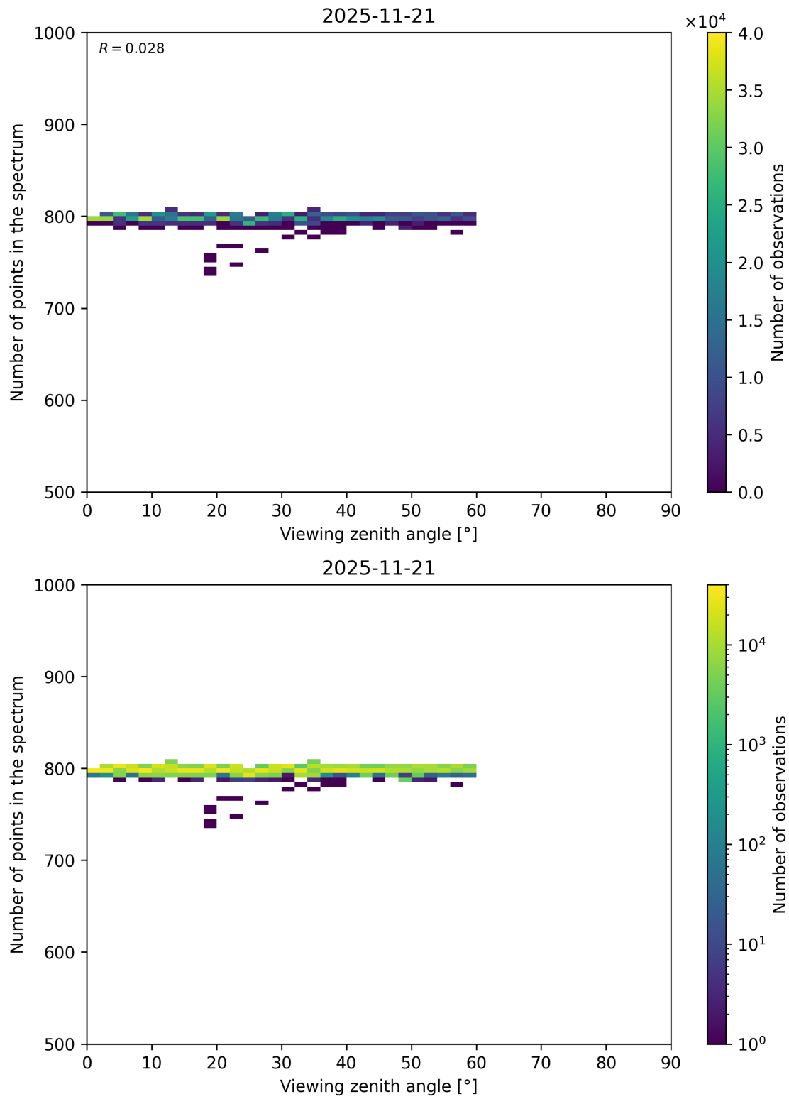
Figure 114: Scatter density plot of “Viewing zenith angle” against “Number of points in the spectrum” for 2025-11-20 to 2025-11-22.
