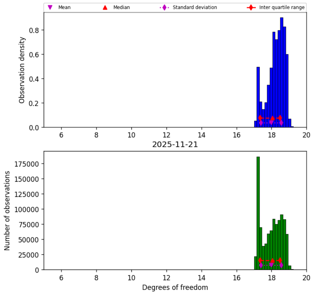
Figure 30: Histogram of “Degrees of freedom” for 2025-11-20 to 2025-11-22
