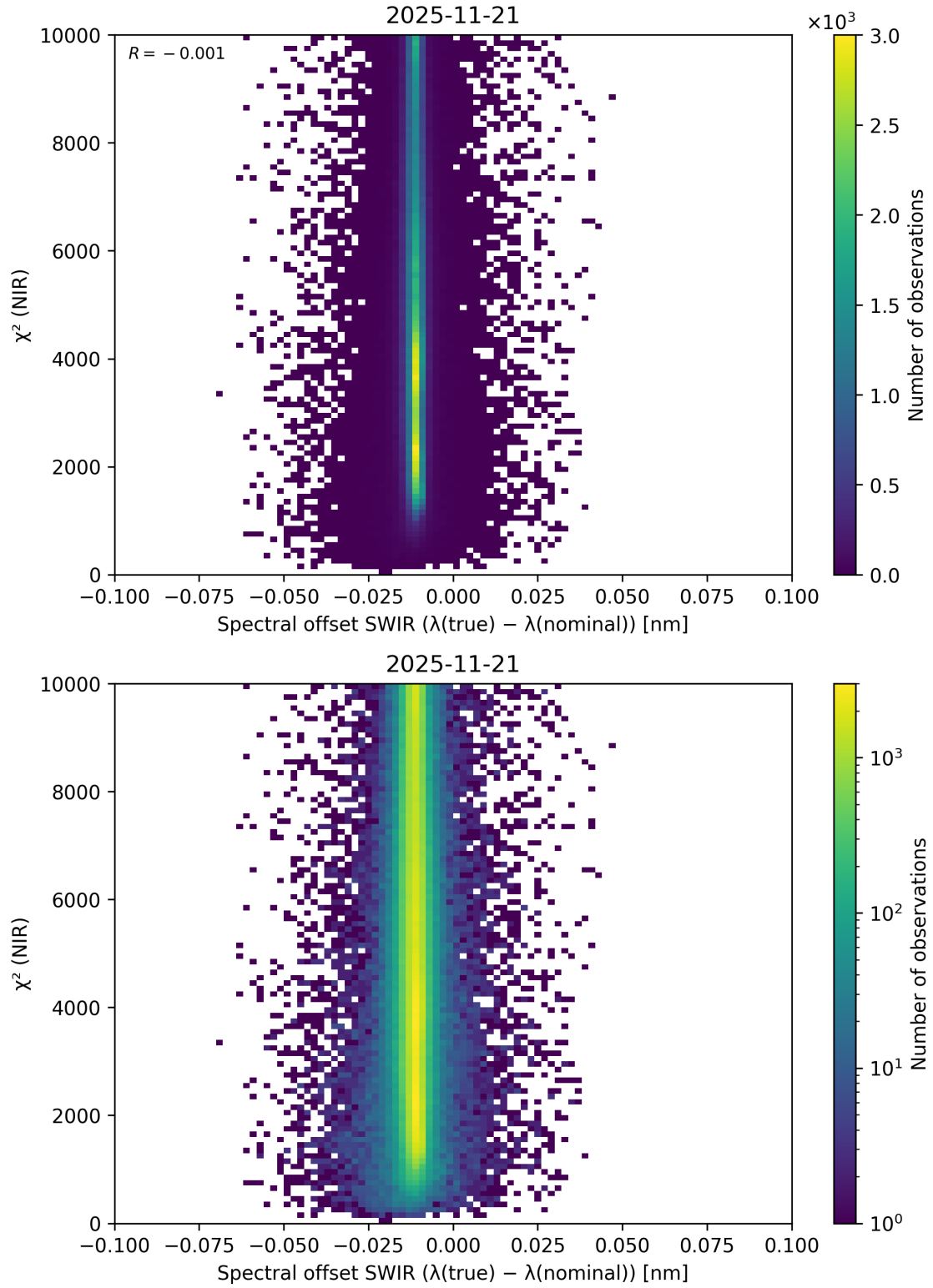
Figure 117: Scatter density plot of “Spectral offset SWIR ( \lambda_{\text{true}} - \lambda_{\text{nominal}} )” against “ \chi^2 (NIR)” for 2025-11-20 to 2025-11-22.
