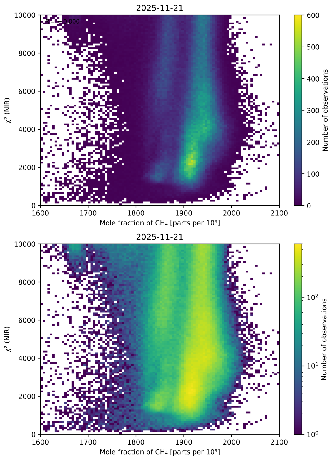
Figure 70: Scatter density plot of “Mole fraction of CH 4 ” against “ \chi^2 (NIR)” for 2025-11-20 to 2025-11-22.
