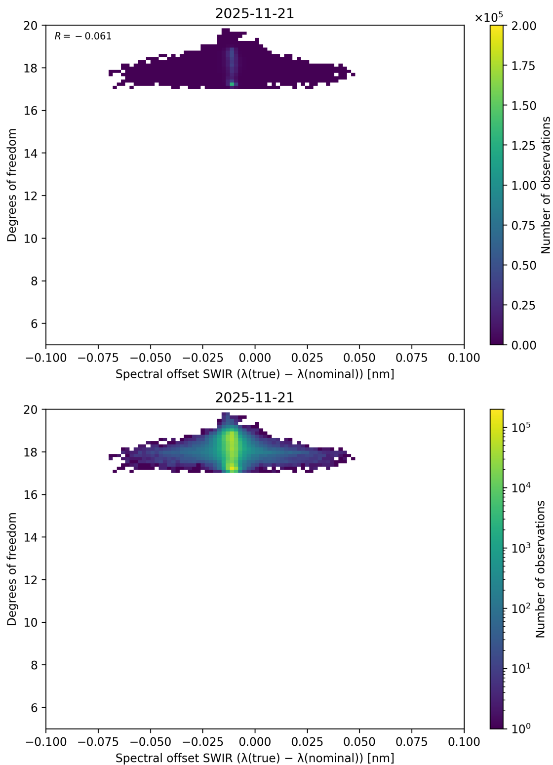
Figure 119: Scatter density plot of “Spectral offset SWIR ( \lambda_{\text{true}} - \lambda_{\text{nominal}} )” against “Degrees of freedom” for 2025-11-20 to 2025-11-22.
