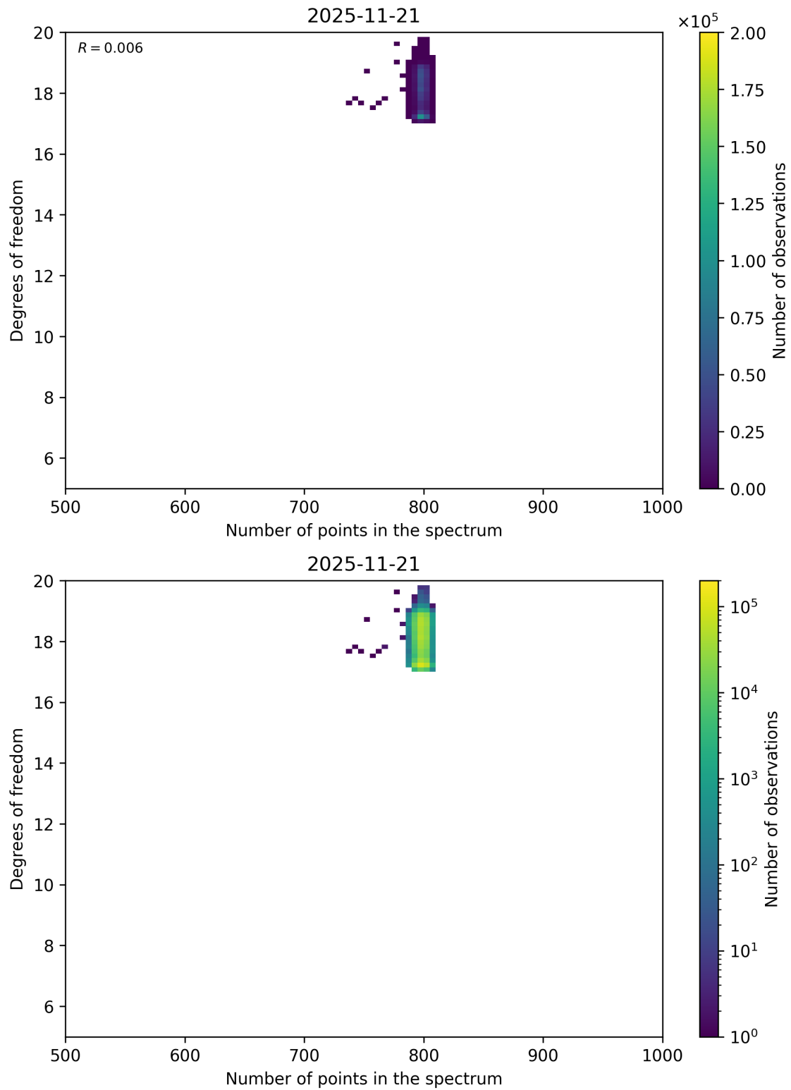
Figure 90: Scatter density plot of “Number of points in the spectrum” against “Degrees of freedom” for 2025-11-20 to 2025-11-22.
