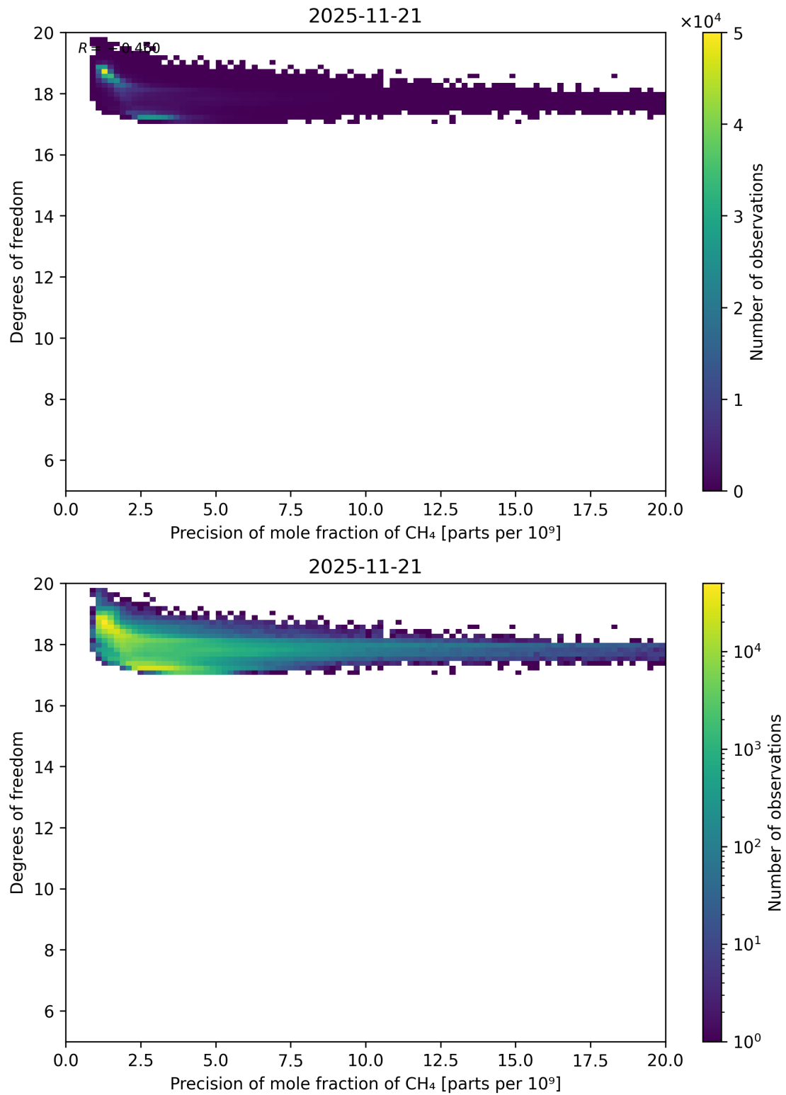
Figure 80: Scatter density plot of “Precision of mole fraction of CH 4 ” against “Degrees of freedom” for 2025-11-20 to 2025-11-22.
