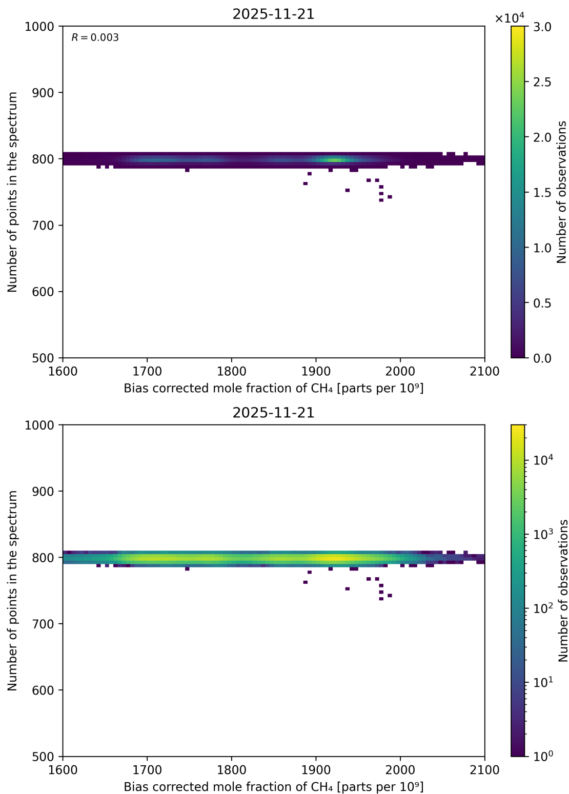
Figure 68: Scatter density plot of “Bias corrected mole fraction of CH 4 ” against “Number of points in the spectrum” for 2025-11-20 to 2025-11-22.
