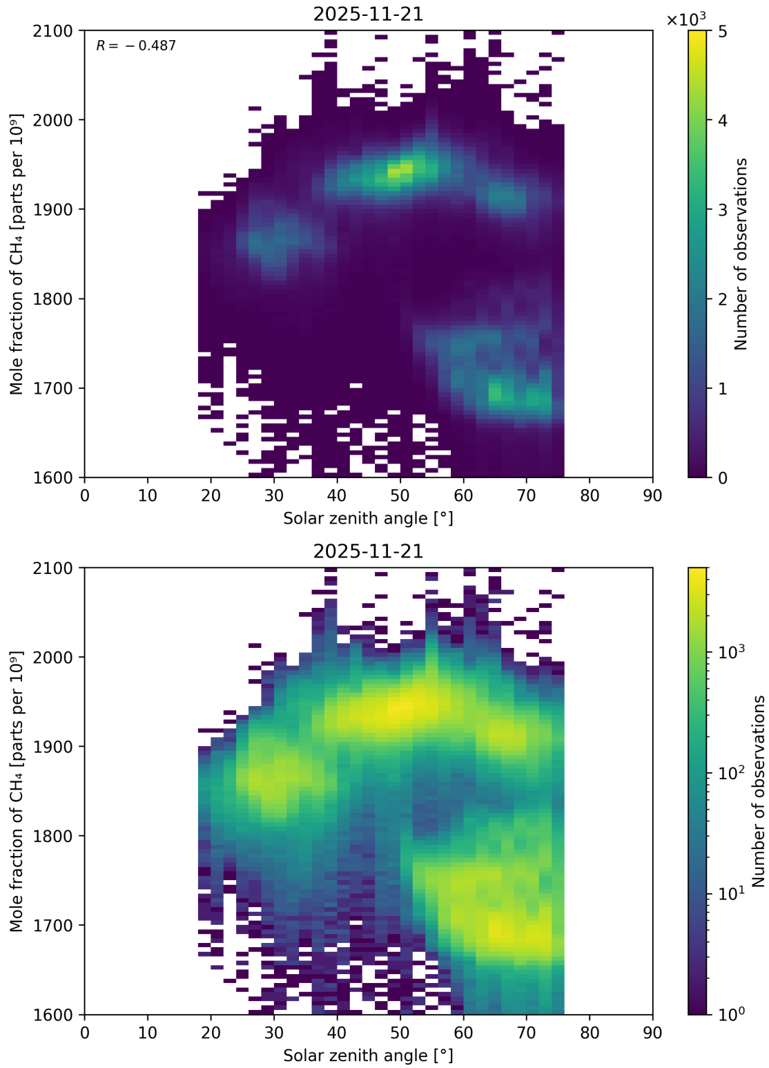
Figure 99: Scatter density plot of “Solar zenith angle” against “Mole fraction of CH 4 ” for 2025-11-20 to 2025-11-22.
