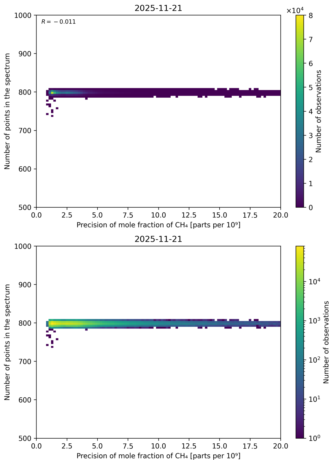
Figure 84: Scatter density plot of “Precision of mole fraction of CH 4 ” against “Number of points in the spectrum” for 2025-11-20 to 2025-11-22.
