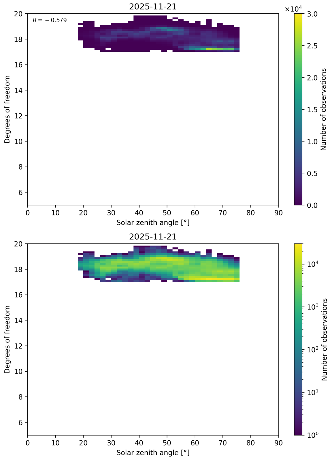
Figure 96: Scatter density plot of “Solar zenith angle” against “Degrees of freedom” for 2025-11-20 to 2025-11-22.
