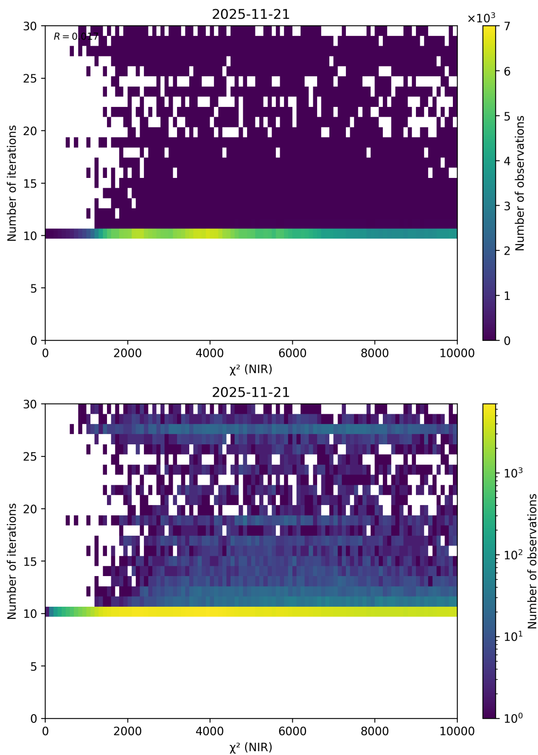
Figure 46: Scatter density plot of “ \chi^2 (NIR)” against “Number of iterations” for 2025-11-20 to 2025-11-22.
