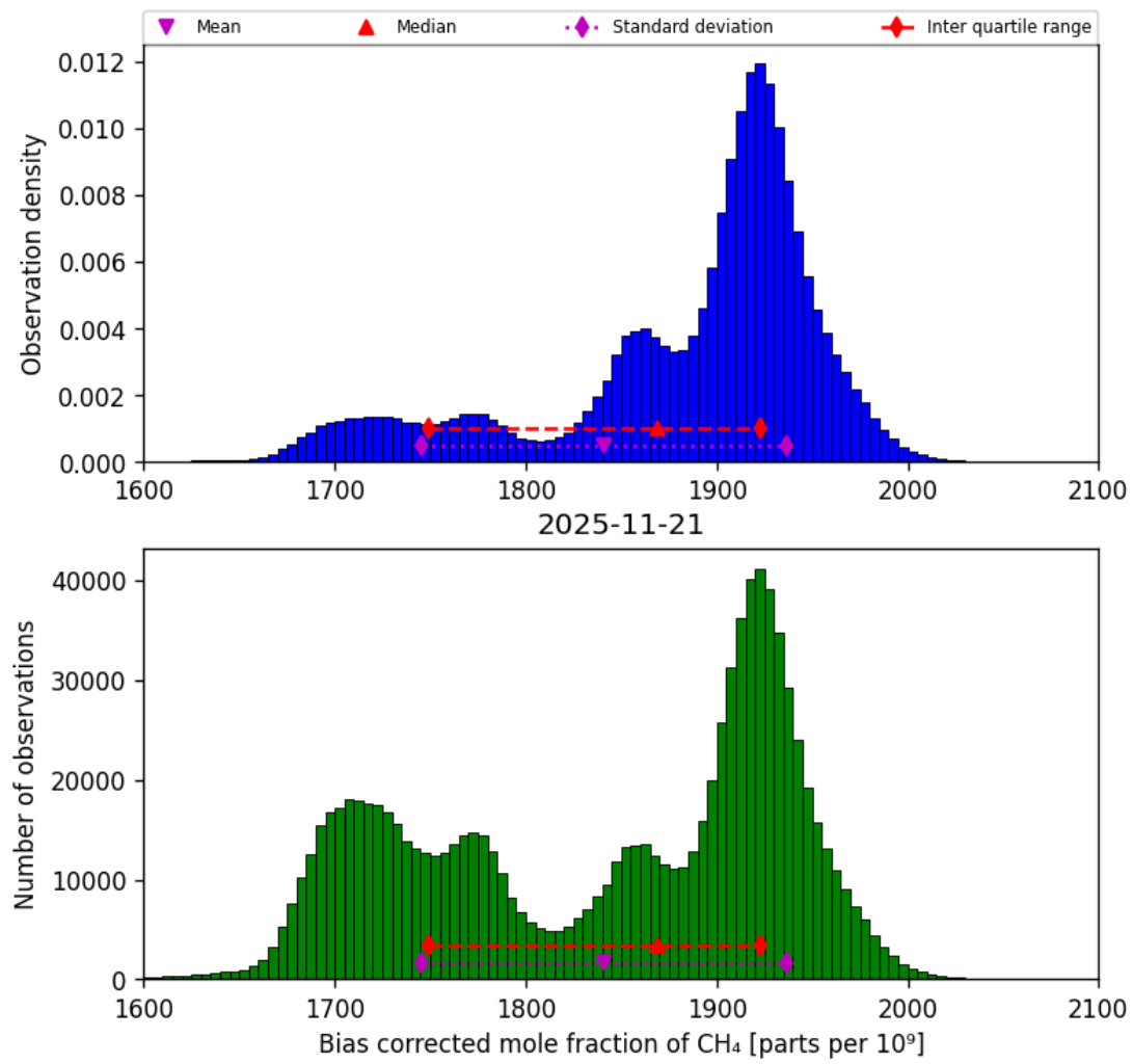
Figure 25: Histogram of “Bias corrected mole fraction of CH 4 ” for 2025-11-20 to 2025-11-22
