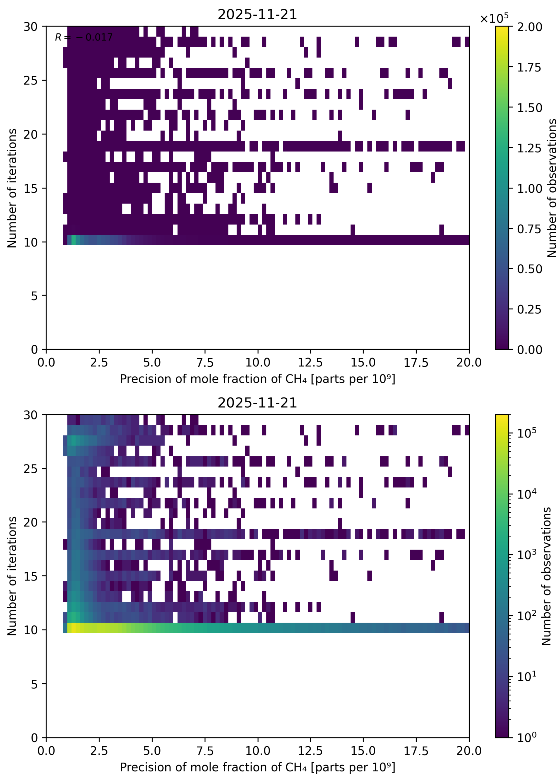
Figure 83: Scatter density plot of “Precision of mole fraction of CH 4 ” against “Number of iterations” for 2025-11-20 to 2025-11-22.
