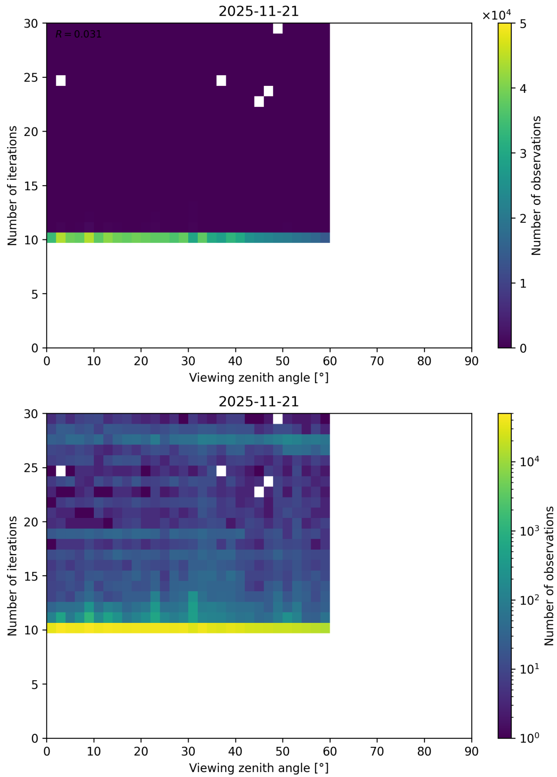
Figure 113: Scatter density plot of “Viewing zenith angle” against “Number of iterations” for 2025-11-20 to 2025-11-22.
