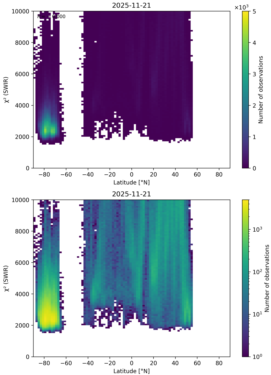
Figure 54: Scatter density plot of “Latitude” against “ \chi^2 (SWIR)” for 2025-11-20 to 2025-11-22.
