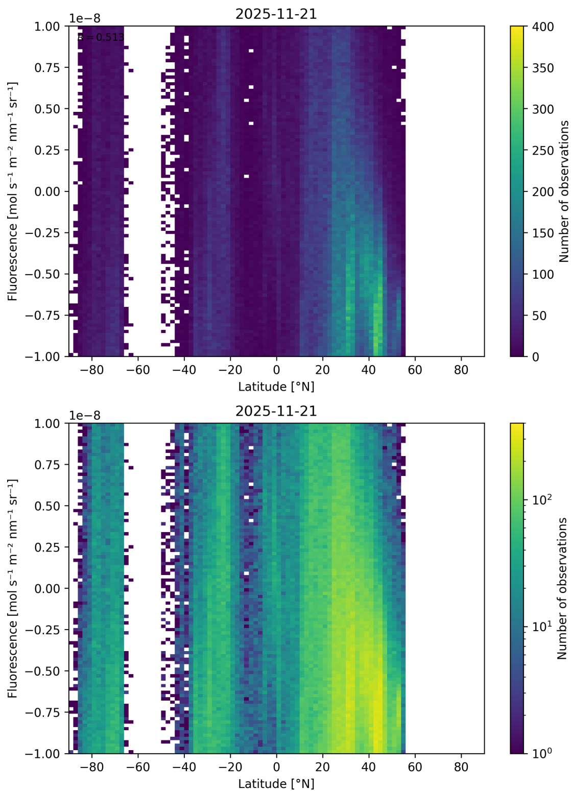
Figure 56: Scatter density plot of “Latitude” against “Fluorescence” for 2025-11-20 to 2025-11-22.
