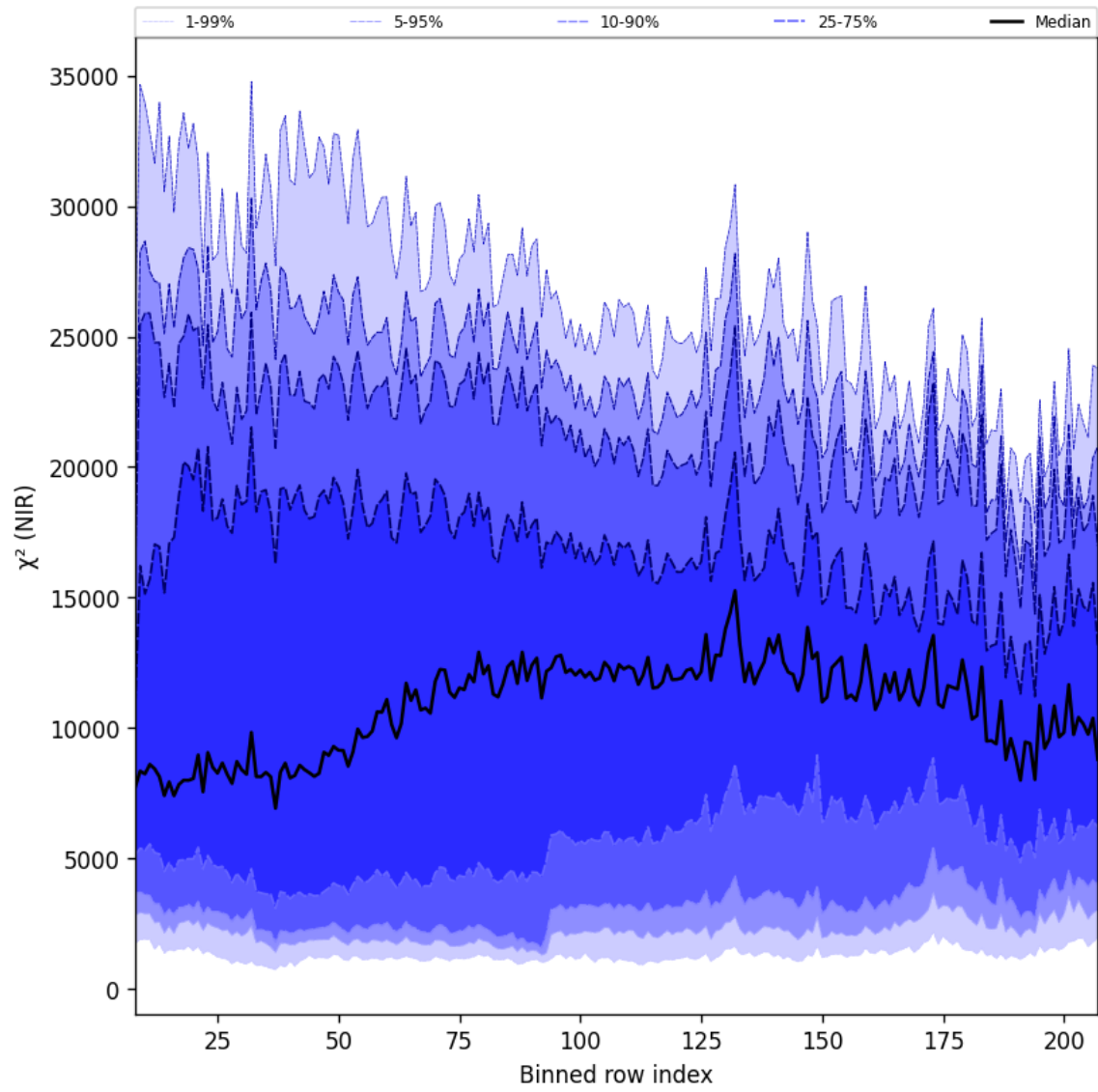
Figure 40: Along track statistics of “ \chi^2 (NIR)” for 2025-11-20 to 2025-11-22
