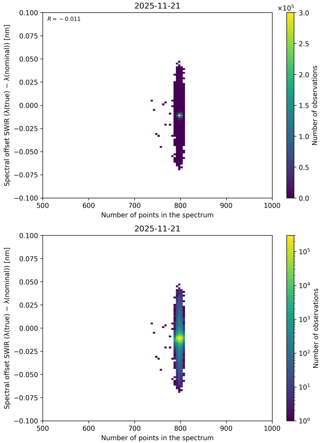
Figure 93: Scatter density plot of “Number of points in the spectrum” against “Spectral offset SWIR ( \lambda_{\text{true}} - \lambda_{\text{nominal}} )” for 2025-11-20 to 2025-11-22.
