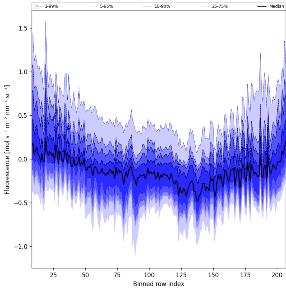
Figure 43: Along track statistics of “Fluorescence” for 2025-11-20 to 2025-11-22
