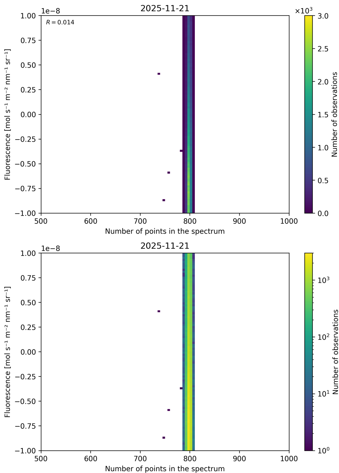
Figure 91: Scatter density plot of “Number of points in the spectrum” against “Fluorescence” for 2025-11-20 to 2025-11-22.
