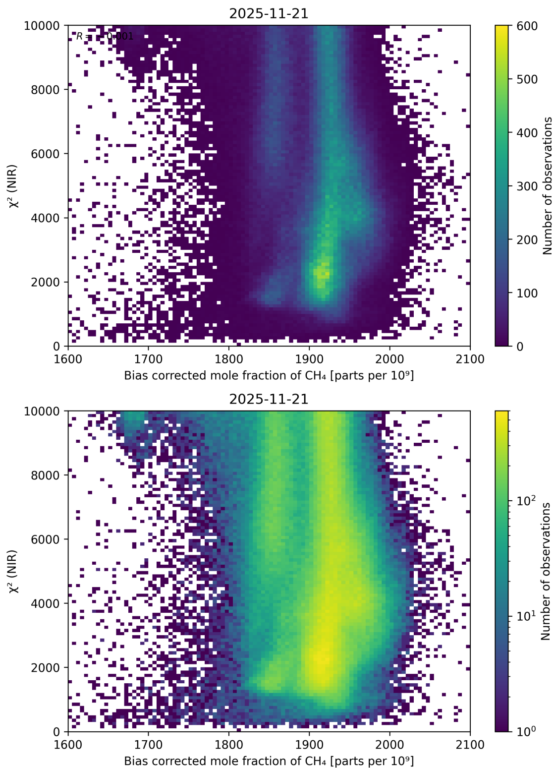
Figure 63: Scatter density plot of “Bias corrected mole fraction of \text{CH}_4 ” against “ \chi^2 (NIR)” for 2025-11-20 to 2025-11-22.
