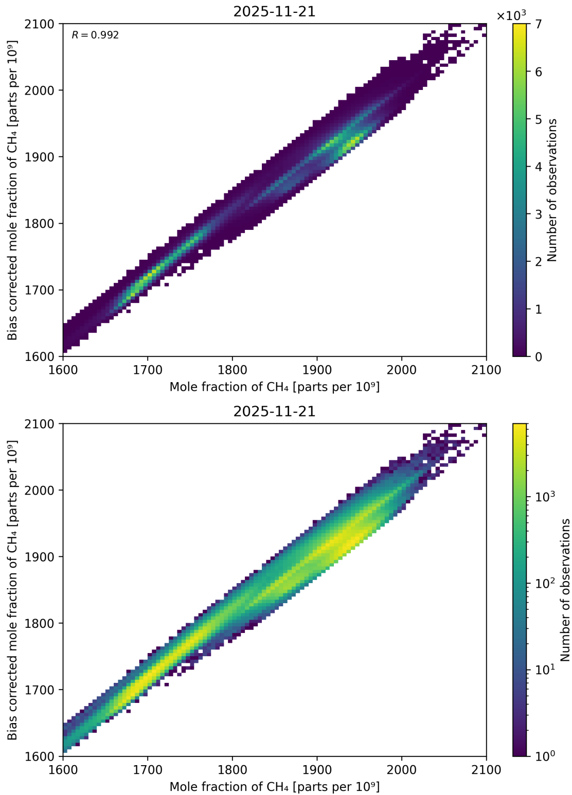
Figure 74: Scatter density plot of “Mole fraction of CH 4 ” against “Bias corrected mole fraction of CH 4 ” for 2025-11-20 to 2025-11-22.
