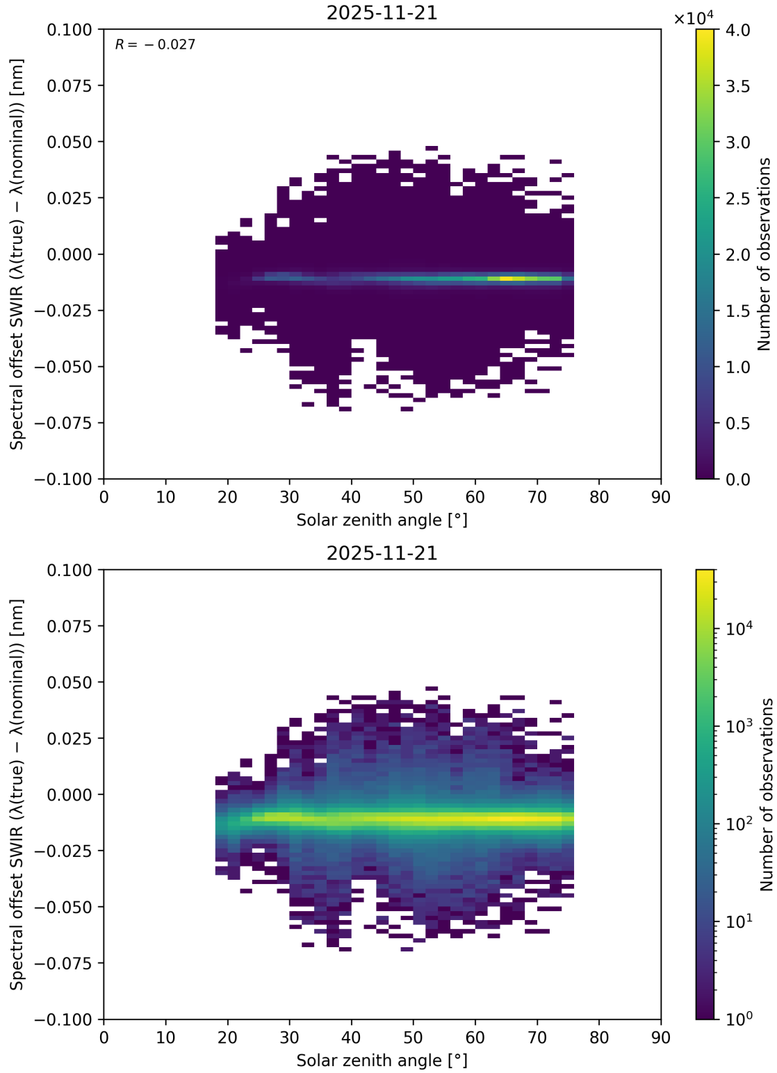
Figure 104: Scatter density plot of “Solar zenith angle” against “Spectral offset SWIR ( \lambda_{\text{true}} - \lambda_{\text{nominal}} )” for 2025-11-20 to 2025-11-22.
