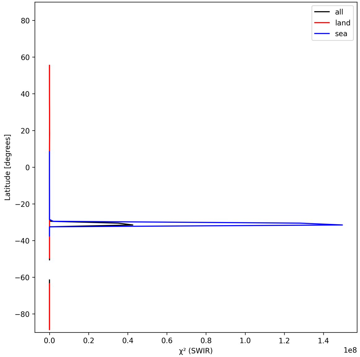
Figure 17: Zonal average of “ \chi^2 (SWIR)” for 2025-11-20 to 2025-11-22.
