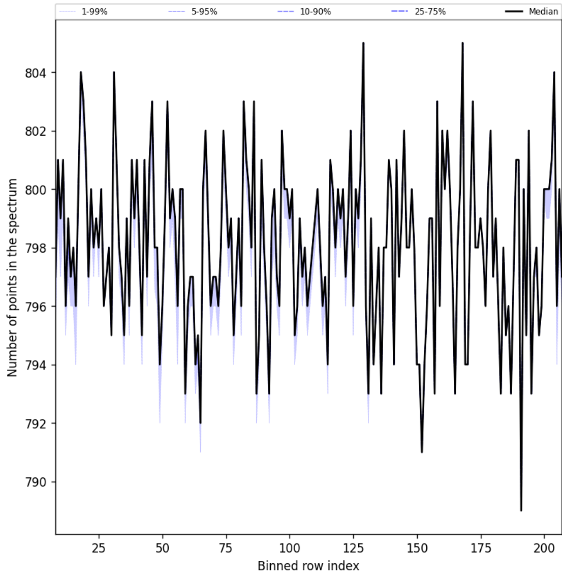
Figure 37: Along track statistics of “Number of points in the spectrum” for 2025-11-20 to 2025-11-22
