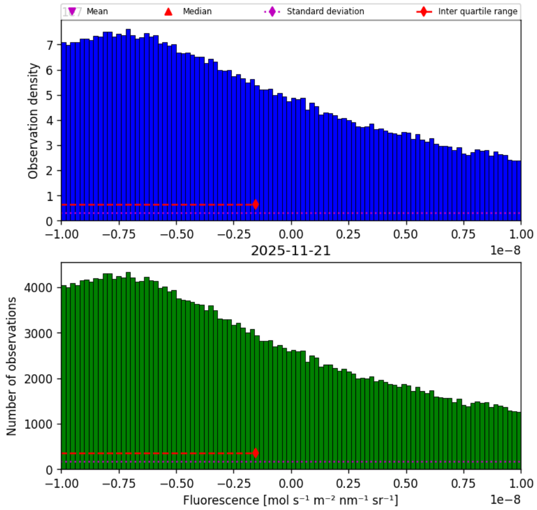
Figure 32: Histogram of “Fluorescence” for 2025-11-20 to 2025-11-22
