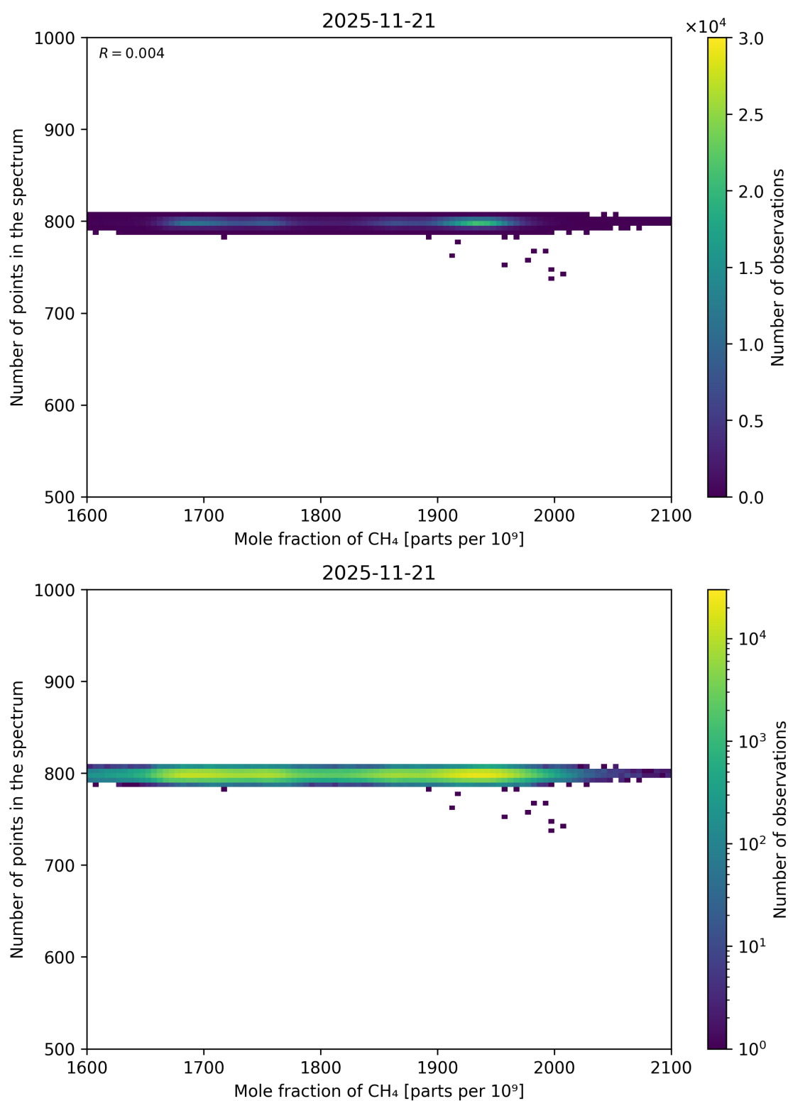
Figure 77: Scatter density plot of “Mole fraction of CH 4 ” against “Number of points in the spectrum” for 2025-11-20 to 2025-11-22.
