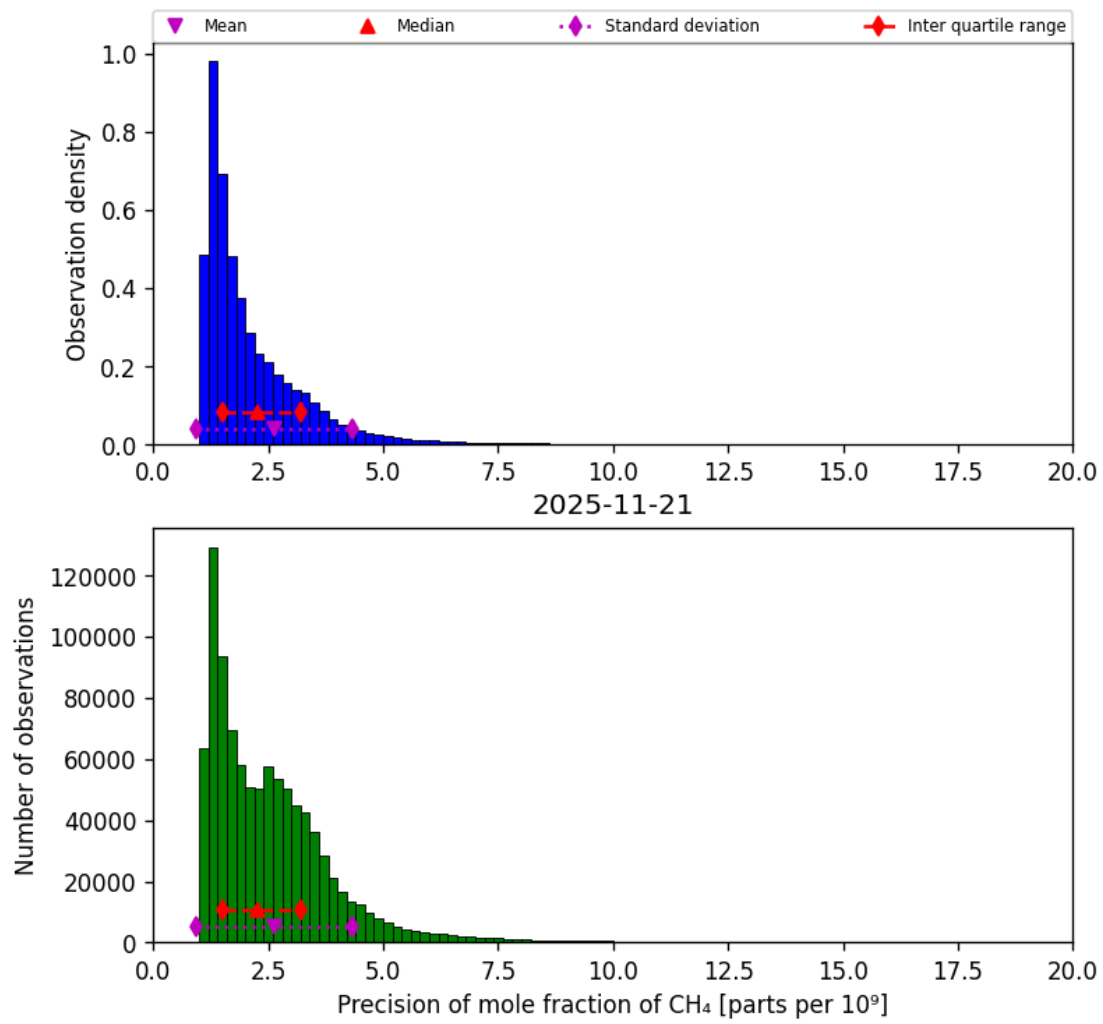
Figure 24: Histogram of “Precision of mole fraction of CH 4 ” for 2025-11-20 to 2025-11-22
