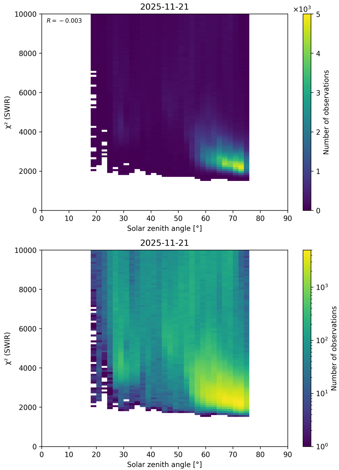
Figure 95: Scatter density plot of “Solar zenith angle” against “ \chi^2 (SWIR)” for 2025-11-20 to 2025-11-22.
