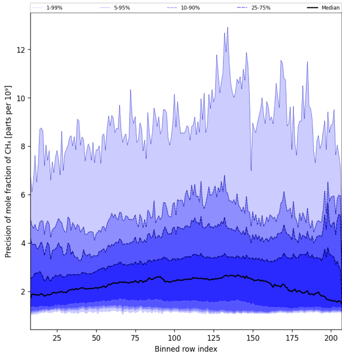
Figure 35: Along track statistics of “Precision of mole fraction of CH 4 ” for 2025-11-20 to 2025-11-22
