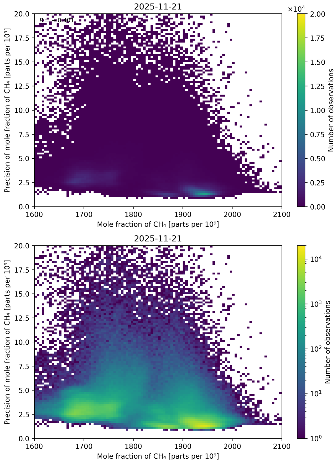
Figure 75: Scatter density plot of “Mole fraction of CH 4 ” against “Precision of mole fraction of CH 4 ” for 2025-11-20 to 2025-11-22.
