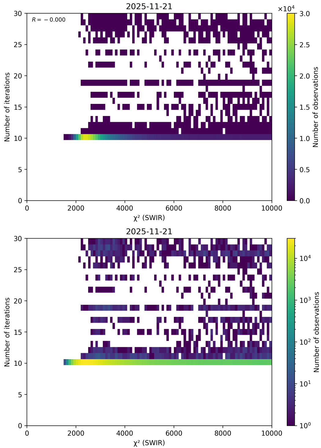
Figure 50: Scatter density plot of “ \chi^2 (SWIR)” against “Number of iterations” for 2025-11-20 to 2025-11-22.
