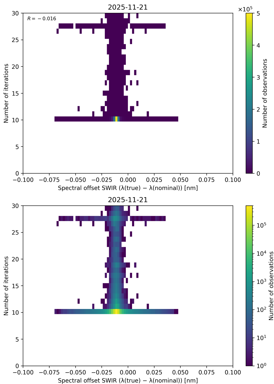
Figure 121: Scatter density plot of “Spectral offset SWIR ( \lambda_{\text{true}} - \lambda_{\text{nominal}} )” against “Number of iterations” for 2025-11-20 to 2025-11-22.
