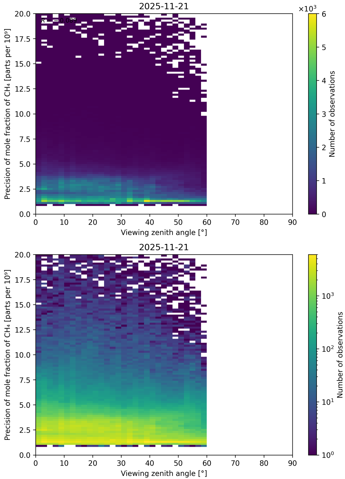
Figure 112: Scatter density plot of “Viewing zenith angle” against “Precision of mole fraction of CH 4 ” for 2025-11-20 to 2025-11-22.
