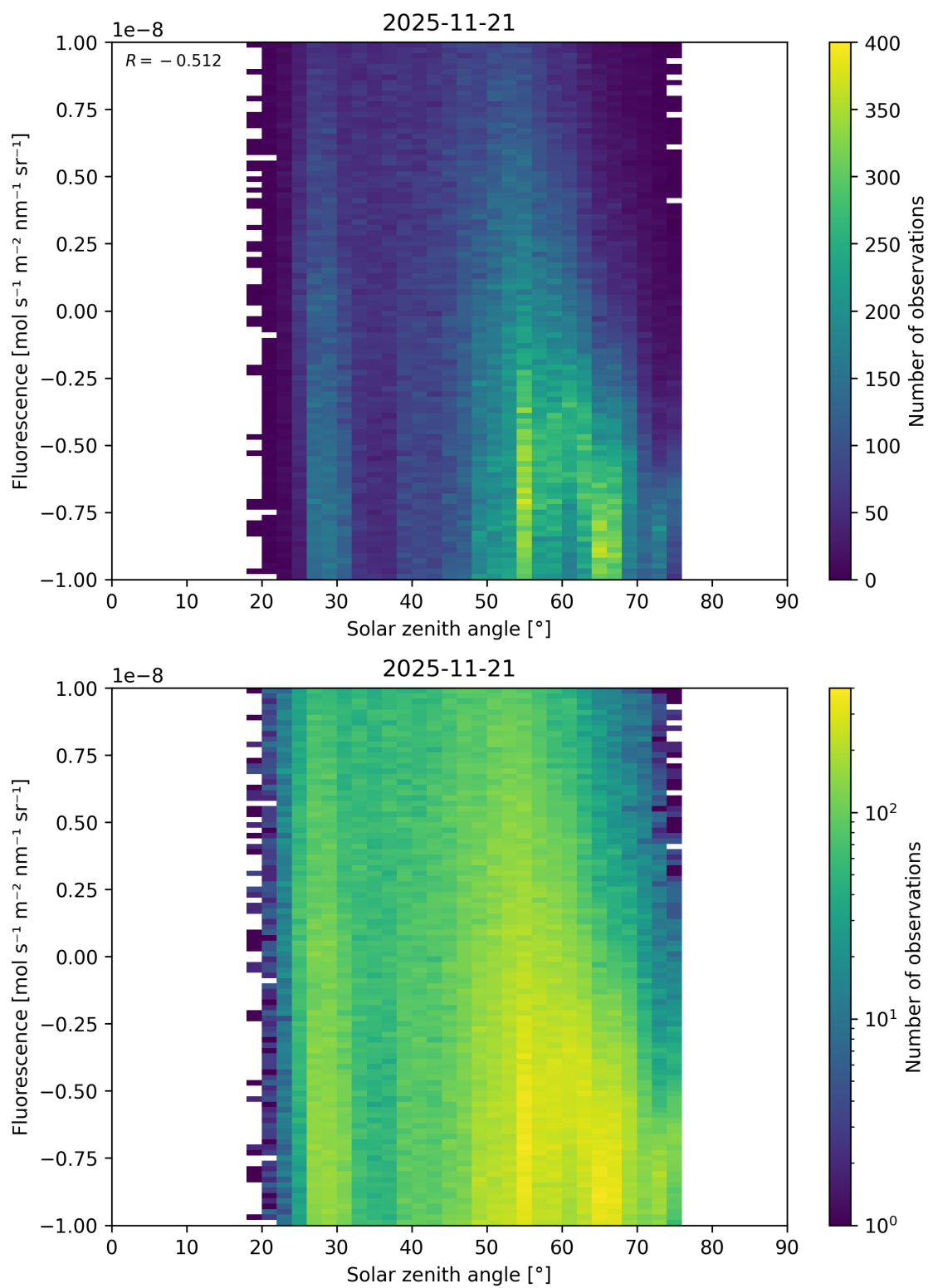
Figure 97: Scatter density plot of “Solar zenith angle” against “Fluorescence” for 2025-11-20 to 2025-11-22.
