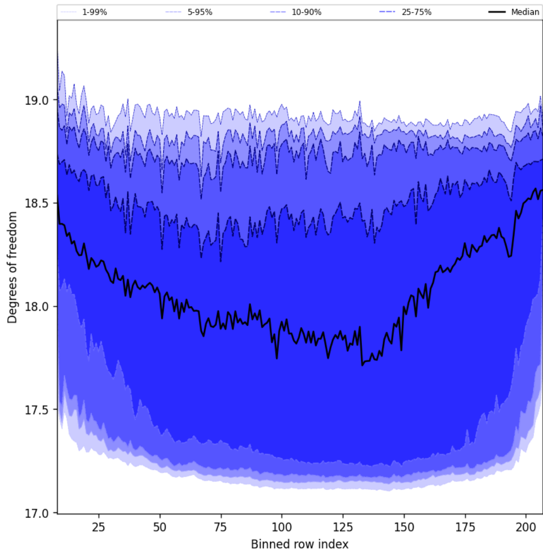
Figure 41: Along track statistics of “Degrees of freedom” for 2025-11-20 to 2025-11-22
